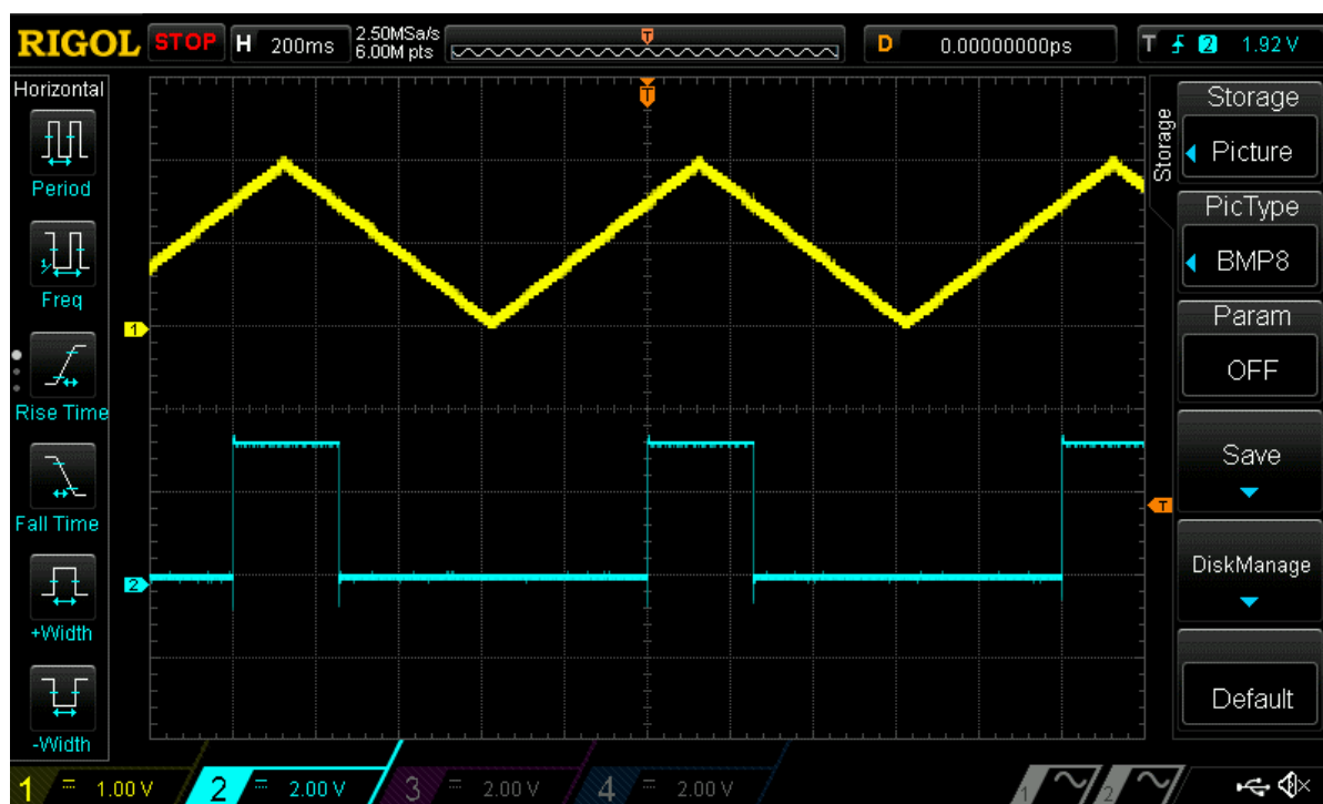
Figure 7: ACMP Output during Glitching
