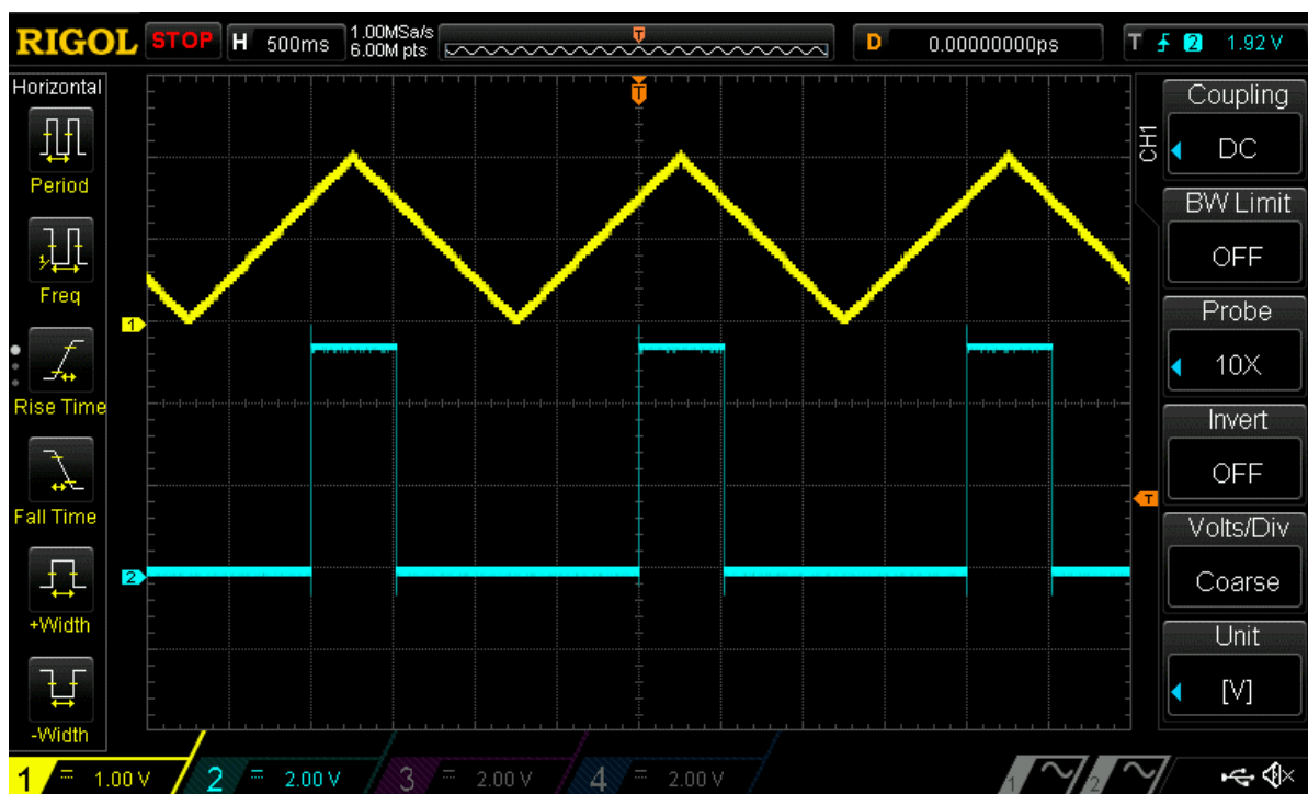
Figure 5: ACMP Output during Glitching
