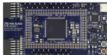
RA8E1 Fast Prototyping Board
