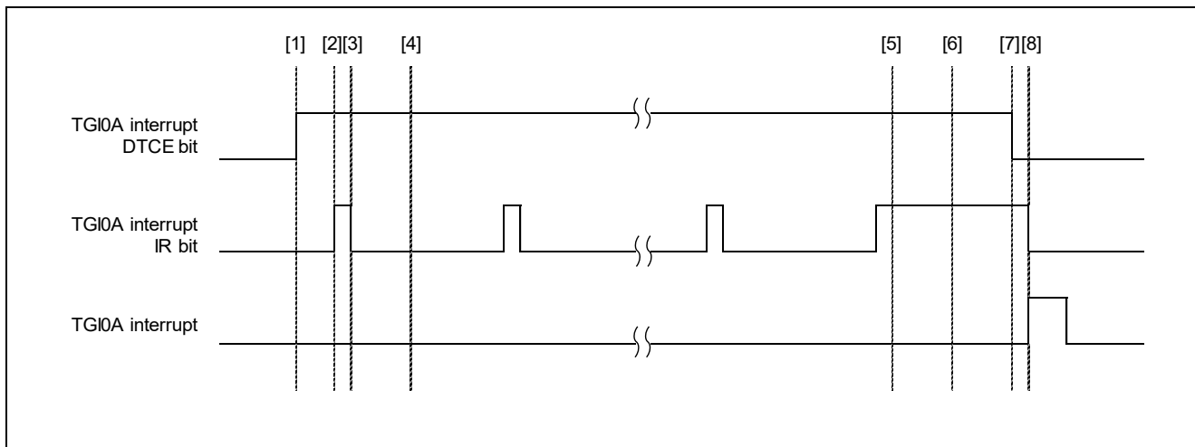
Figure 3.10 RX261 Group Chain Transfer Operation Timing
