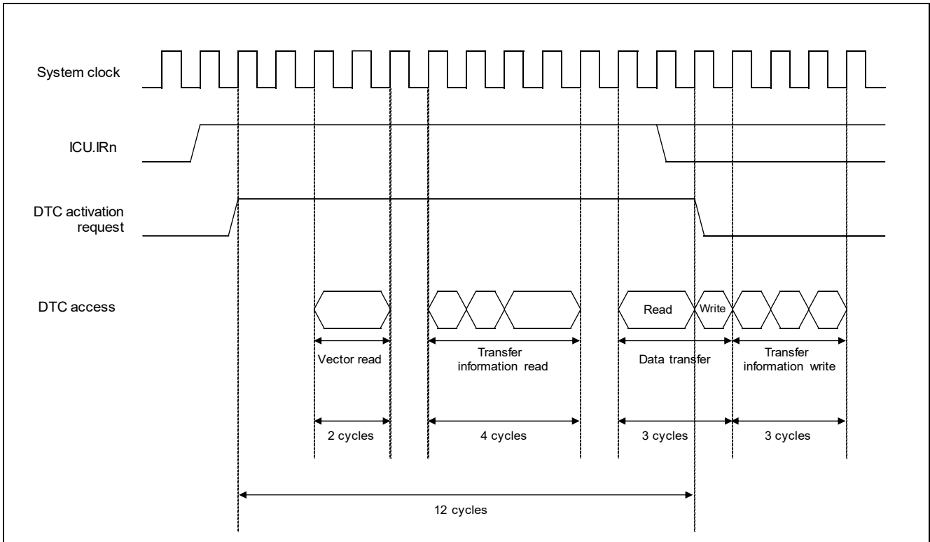
Figure 4.1 RX261 Group DTC Operation Timing Example (Short-Address Mode, Normal Transfer Mode, and Repeat Transfer Mode)
