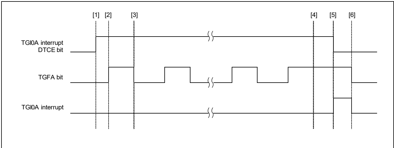
Figure 3.11 H8S/2378 Group Chain Transfer Operation Timing
