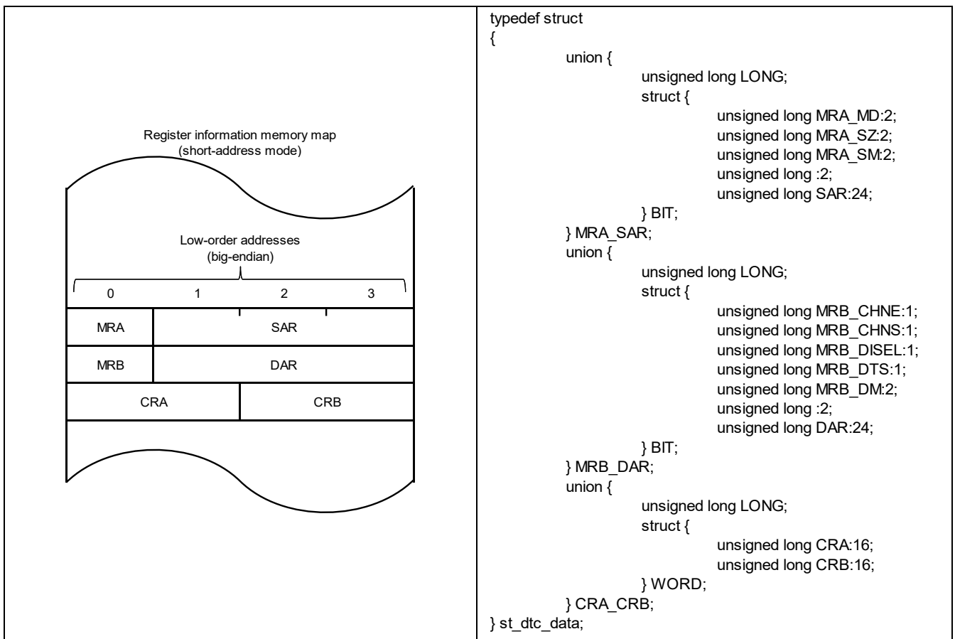
Figure 3.1 RX261 Group Register Information Memory Map and Structure
