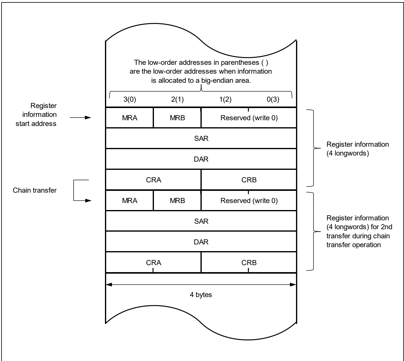
Figure 1.4 Allocation of Register Information on RX261 Group (Full-Address Mode)
