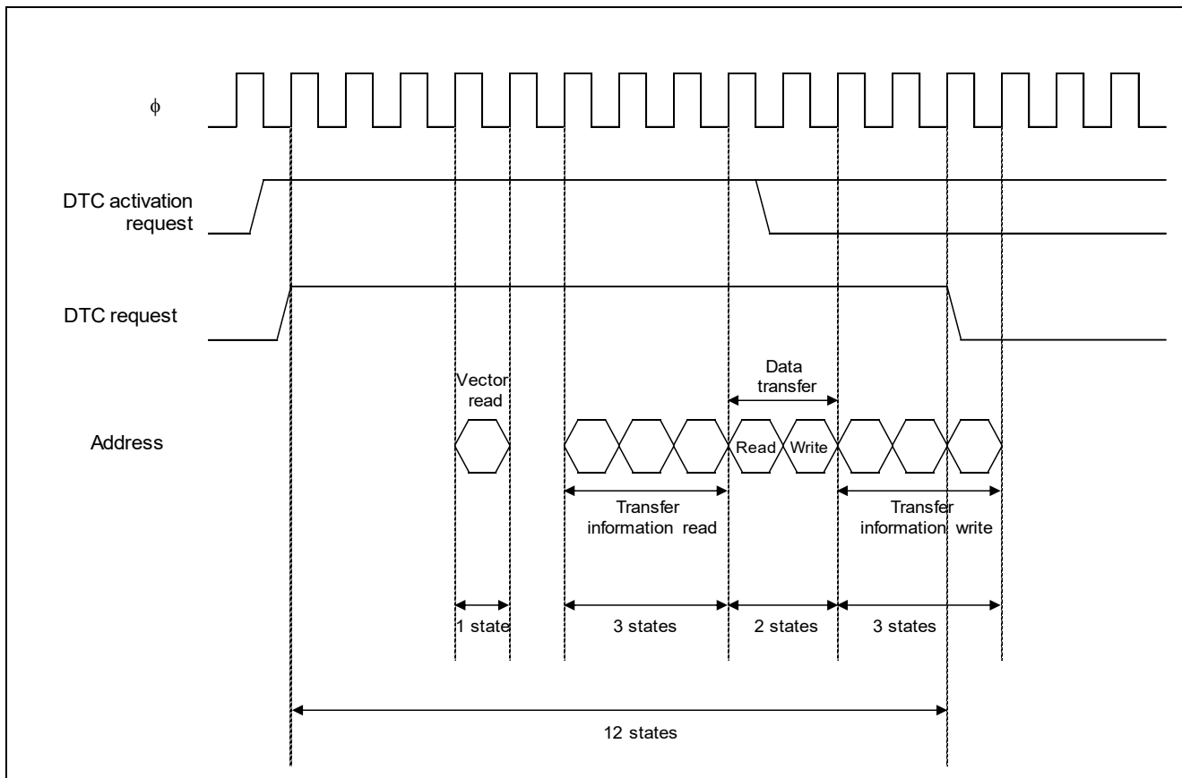
Figure 4.2 H8S/2378 Group DTC Operation Timing Example (Normal Mode and Repeat Mode)
