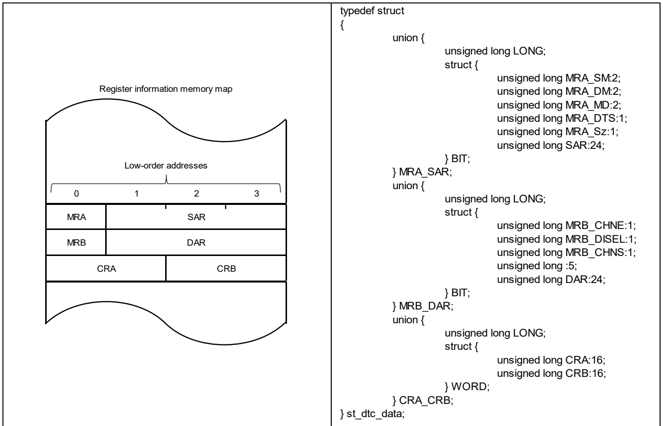
Figure 3.2 H8S/2378 Group Register Information Memory Map and Structure
