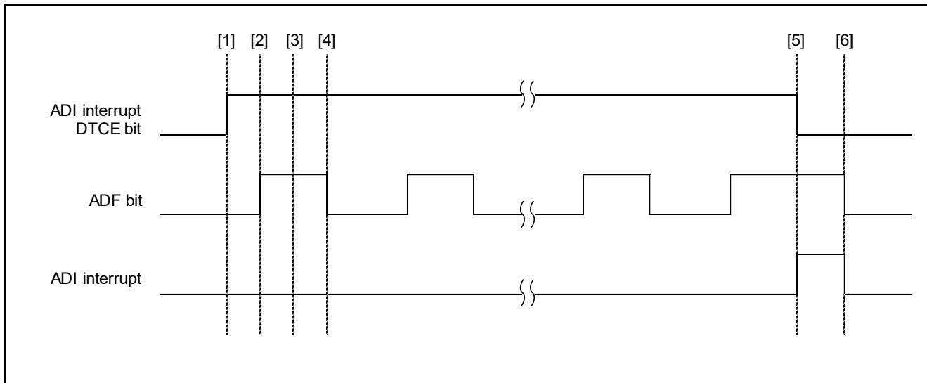
Figure 3.8 H8S/2378 Group Block Transfer Mode Operation Timing
