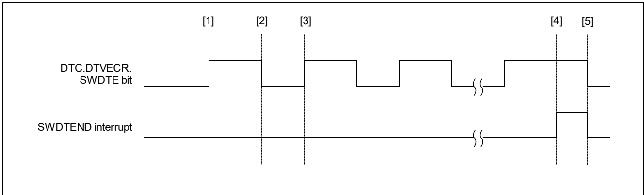
Figure 3.4 H8S/2378 Group Normal Mode Operation Timing
