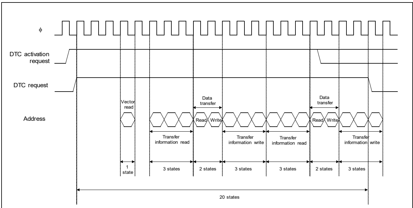
Figure 4.6 H8S/2378 Group DTC Operation Timing Example (Chain Transfer Mode)
