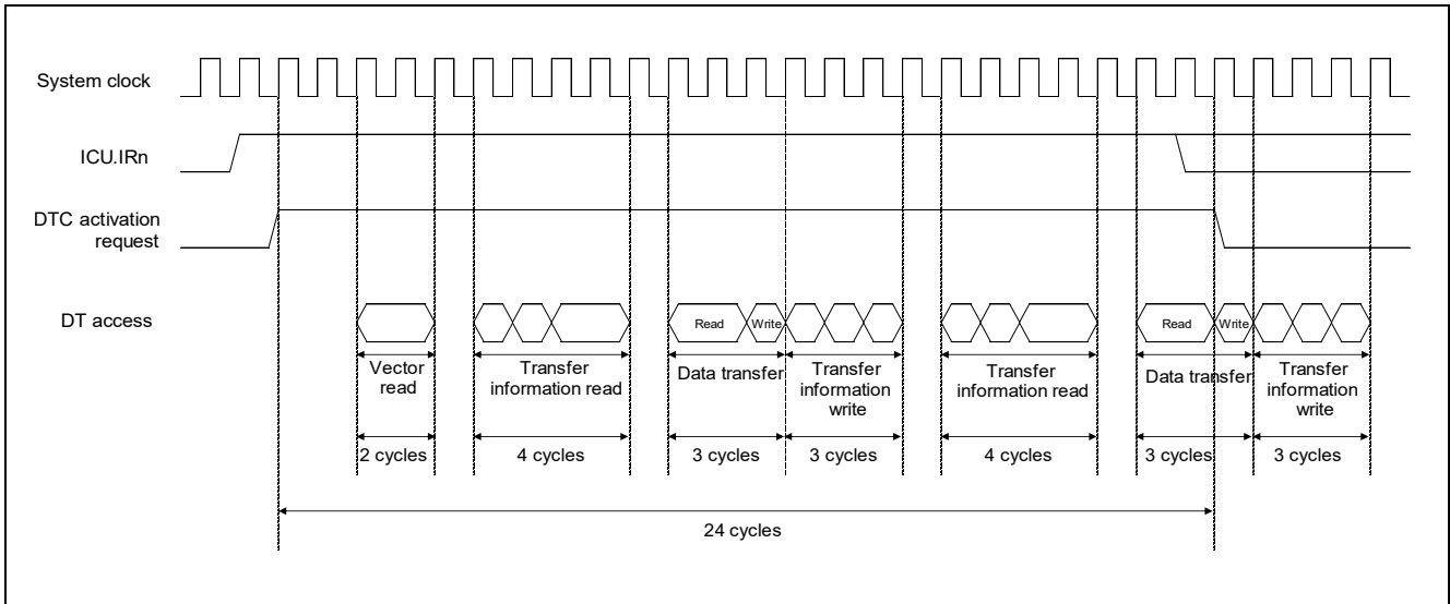
Figure 4.5 RX261 Group DTC Operation Timing Example (Chain Transfer Mode)
