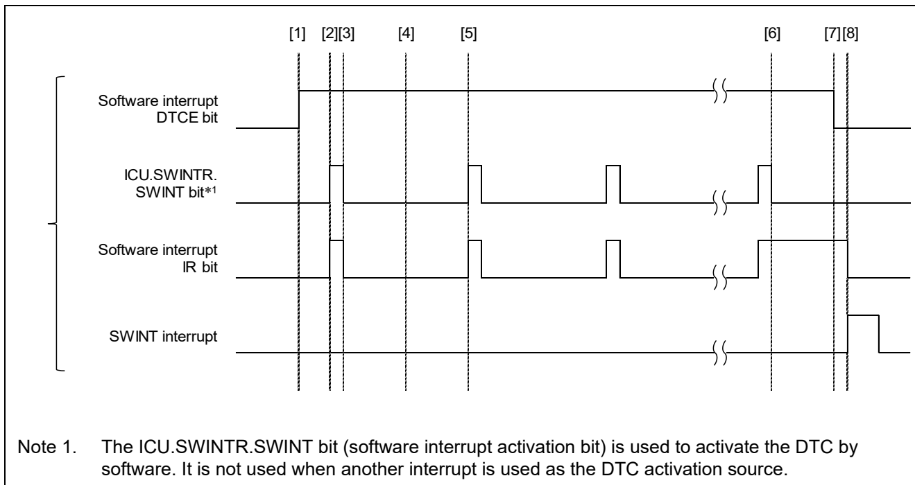
Figure 3.3 RX261 Group Normal Transfer Mode Operation Timing
