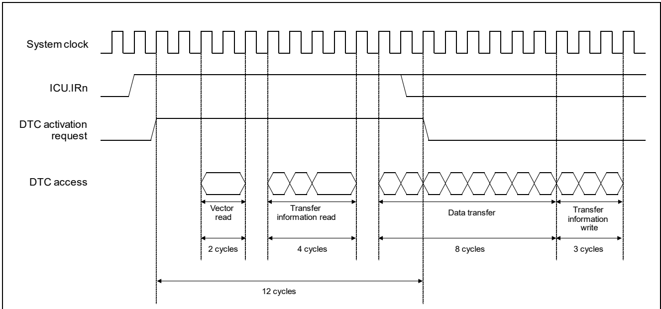
Figure 4.3 RX261 Group DTC Operation Timing Example (Short-Address Mode and Block Transfer Mode)
