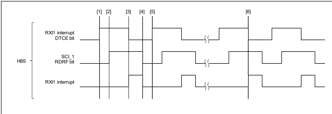
Figure 3.6 H8S/2378 Group Repeat Mode Operation Timing
