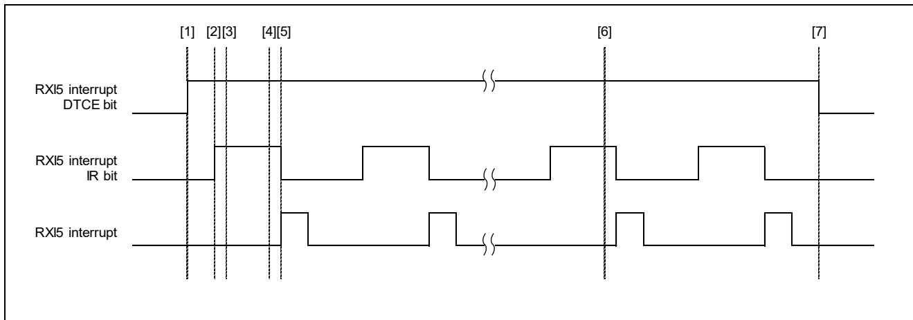
Figure 3.5 RX261 Group Repeat Transfer Mode Operation Timing
