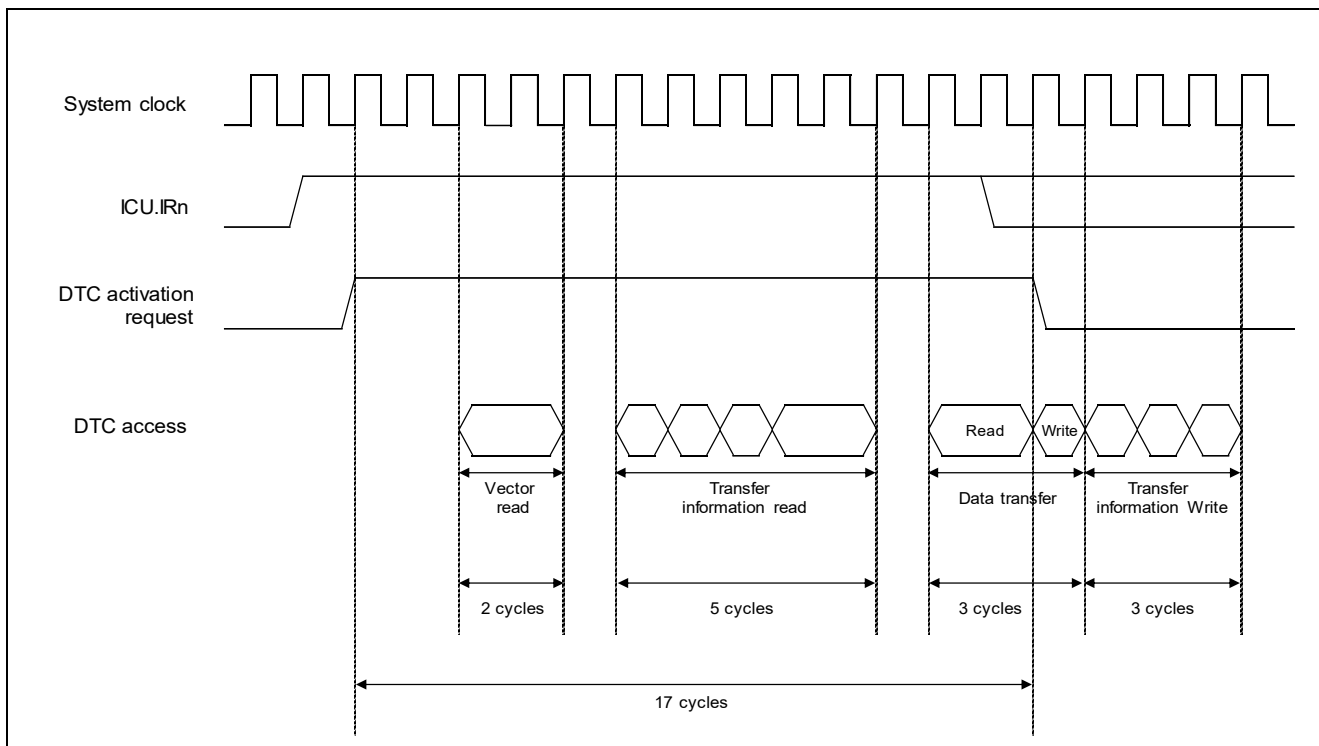
Figure 4.7 RX261 Group DTC Operation Timing Example (Full-Address Mode, Normal Transfer Mode, and Repeat Transfer Mode)
