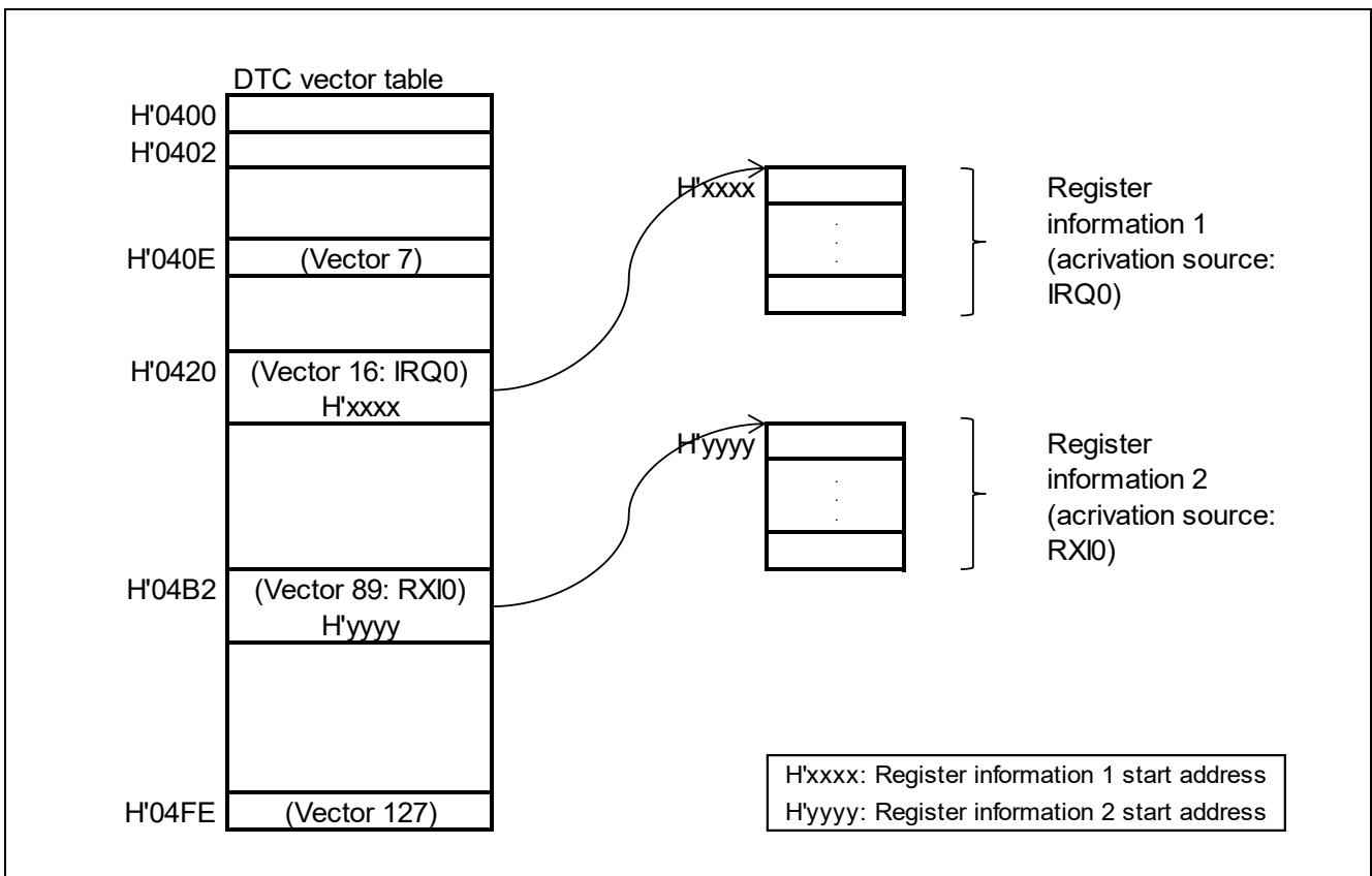
Figure 1.2 DTC Vector Configuration on H8S/2378 Group
