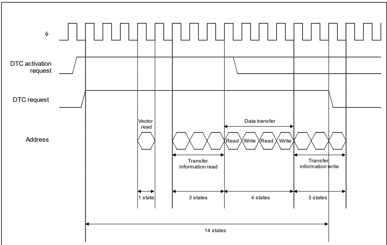
Figure 4.4 H8S/2378 Group DTC Operation Timing Example (Block Transfer Mode)
