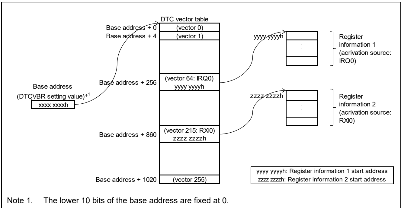
Figure 1.1 DTC Vector Configuration on RX261 Group
