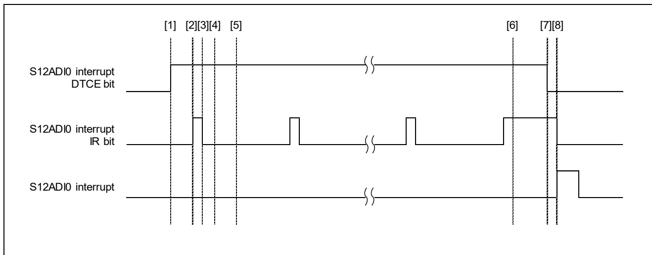
Figure 3.7 RX261 Group Block Transfer Mode Operation Timing
