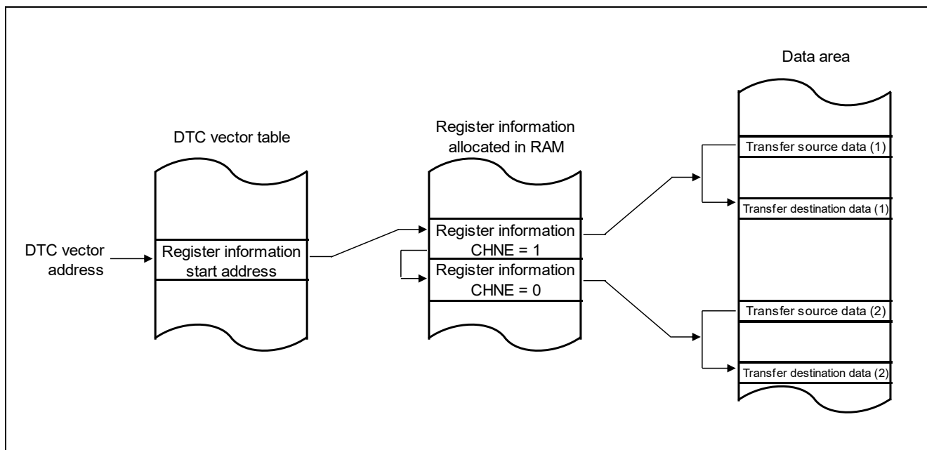
Figure 3.9 Chain Transfer Operation
