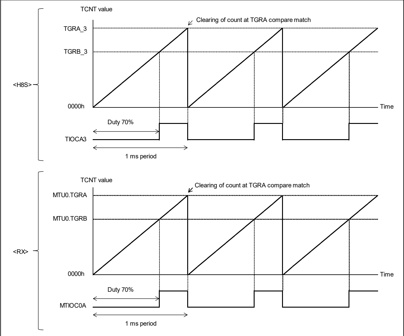
Figure 3.3 Example of PWM Mode 1 Operation on H8S/2378 Group and RX231 Group
