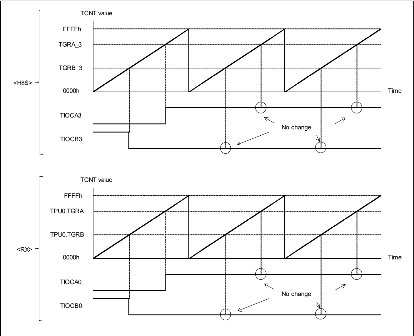
Figure 2.1 Example of Waveform Output Operation on H8S/2378 Group and RX231 Group
