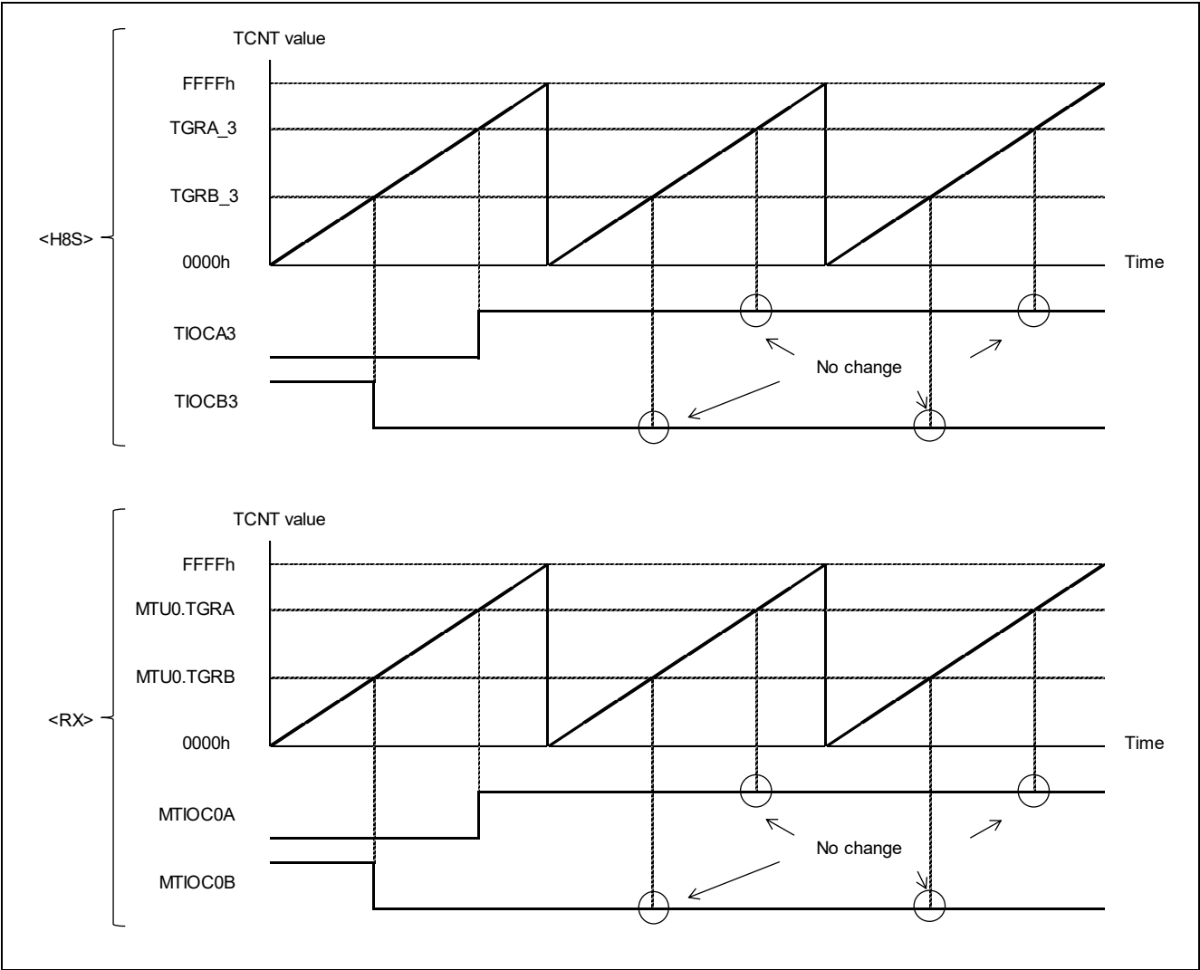
Figure 3.1 Example of Waveform Output Operation on H8S/2378 Group and RX231 Group
