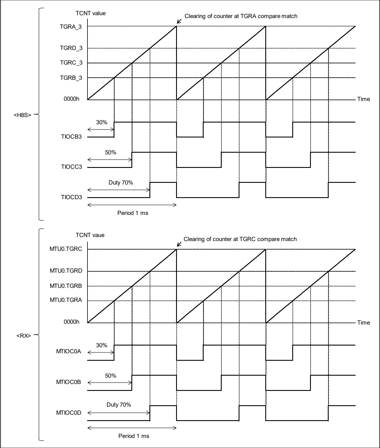
Figure 3.4 Example of PWM Mode 2 Operation on H8S/2378 Group and RX231 Group
