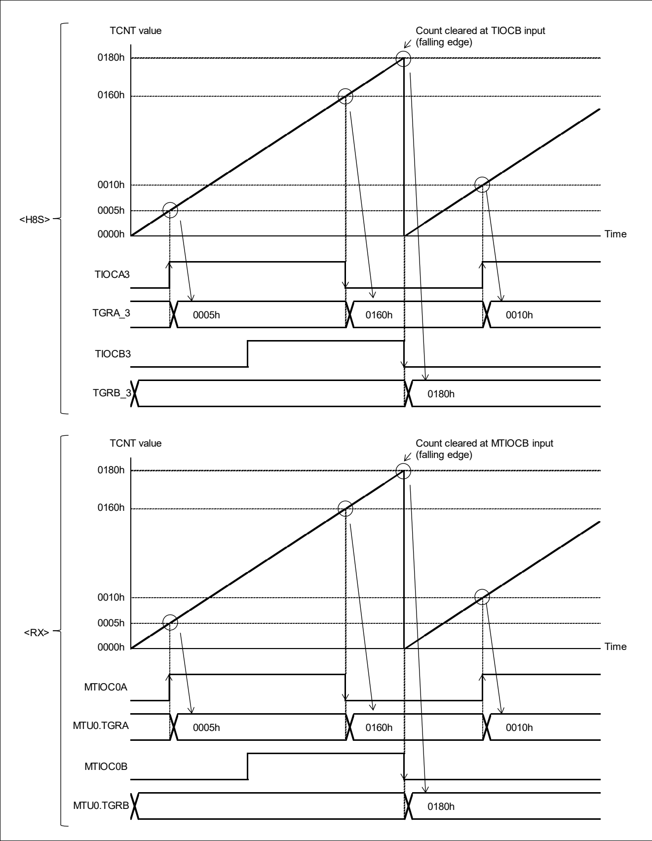
Figure 3.2 Example of Input Capture Operation on H8S/2378 Group and RX231 Group
