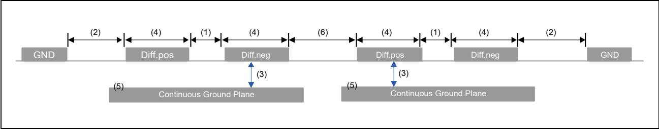
Figure 1.3 Signal Trace Example 2
