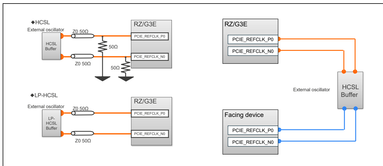
Figure 5.6 Clocking Configurations
