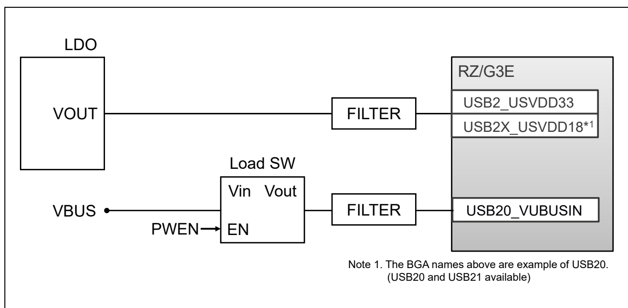
Figure 3.2 Reverse Current from the VBUS
