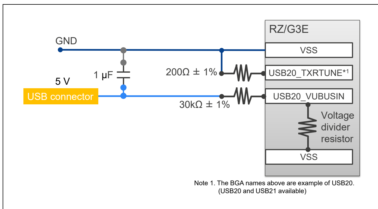
Figure 3.5 External Resistors for USB 2.0
