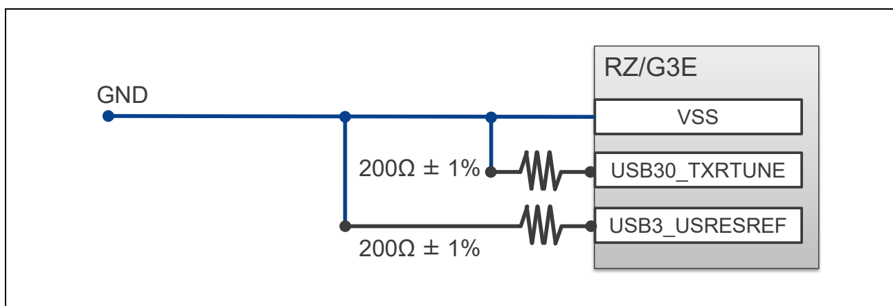
Figure 4.4 External Resistors for USB 3.2 Gen2
