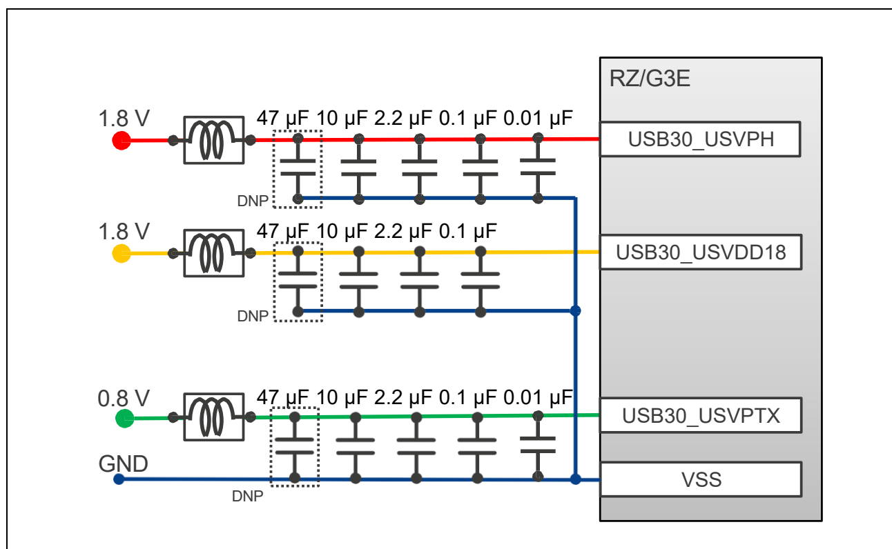
Figure 4.3 External Capacitors for USB 3.2 Gen2
