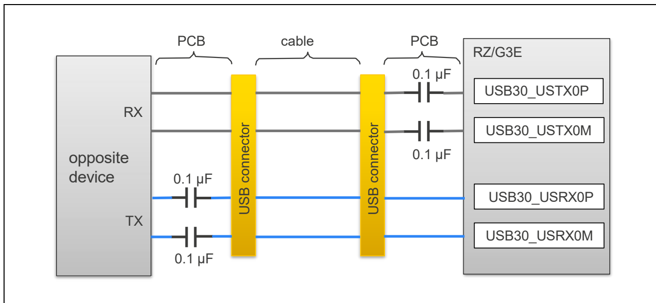
Figure 4.1 Differential Signals of USB 3.2 Gen2
