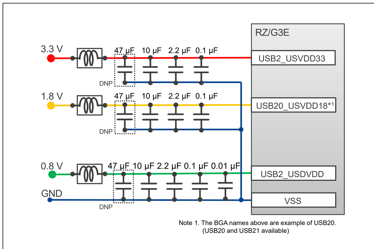
Figure 3.1 External Capacitors for USB 2.0
