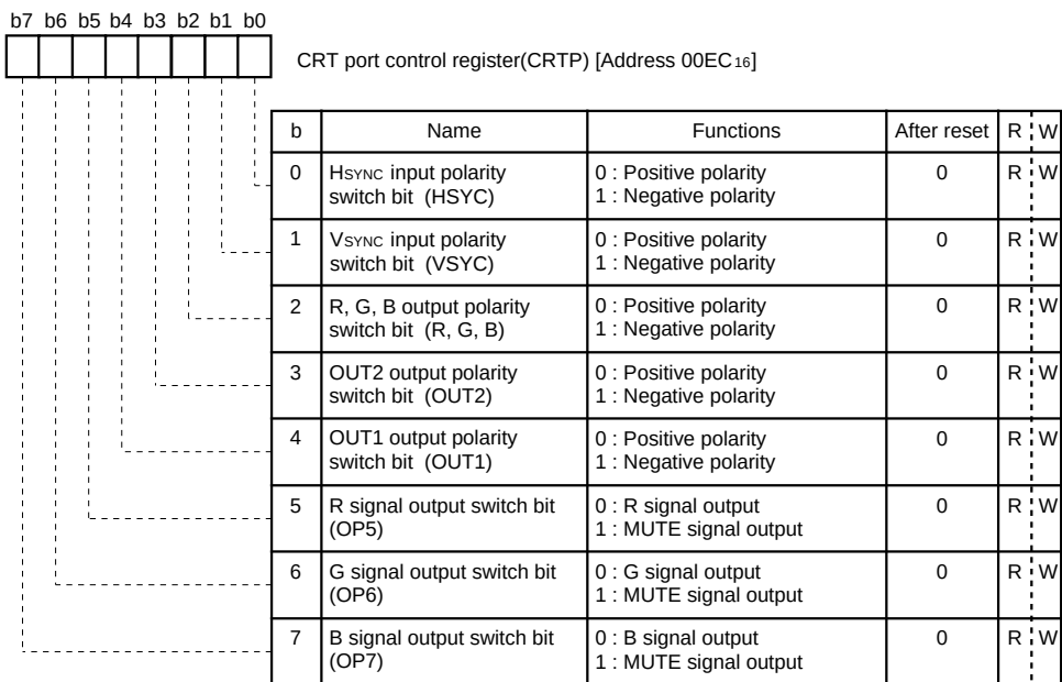
Fig. 2.5.8 CRT port control register (address 00EC 16 )
