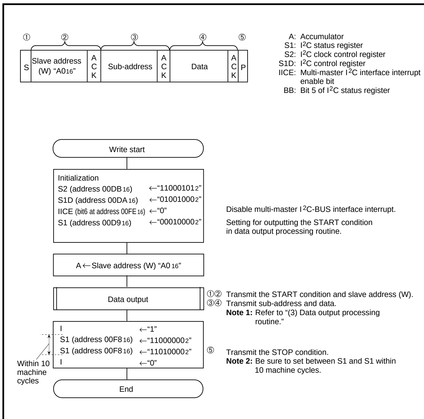
Fig. 5.4.4 Flowchart of write processing routine
