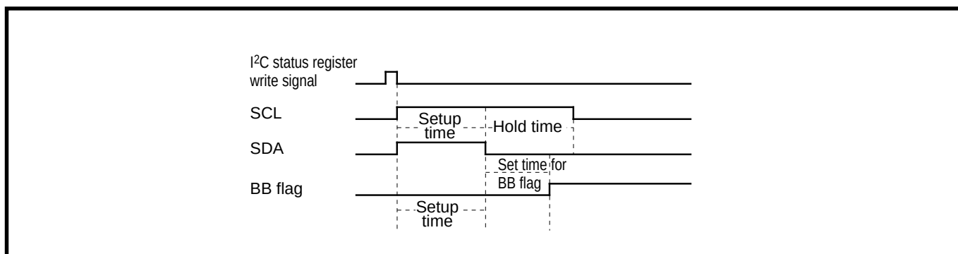
Fig. 2.8.9 START condition generation timing diagram
