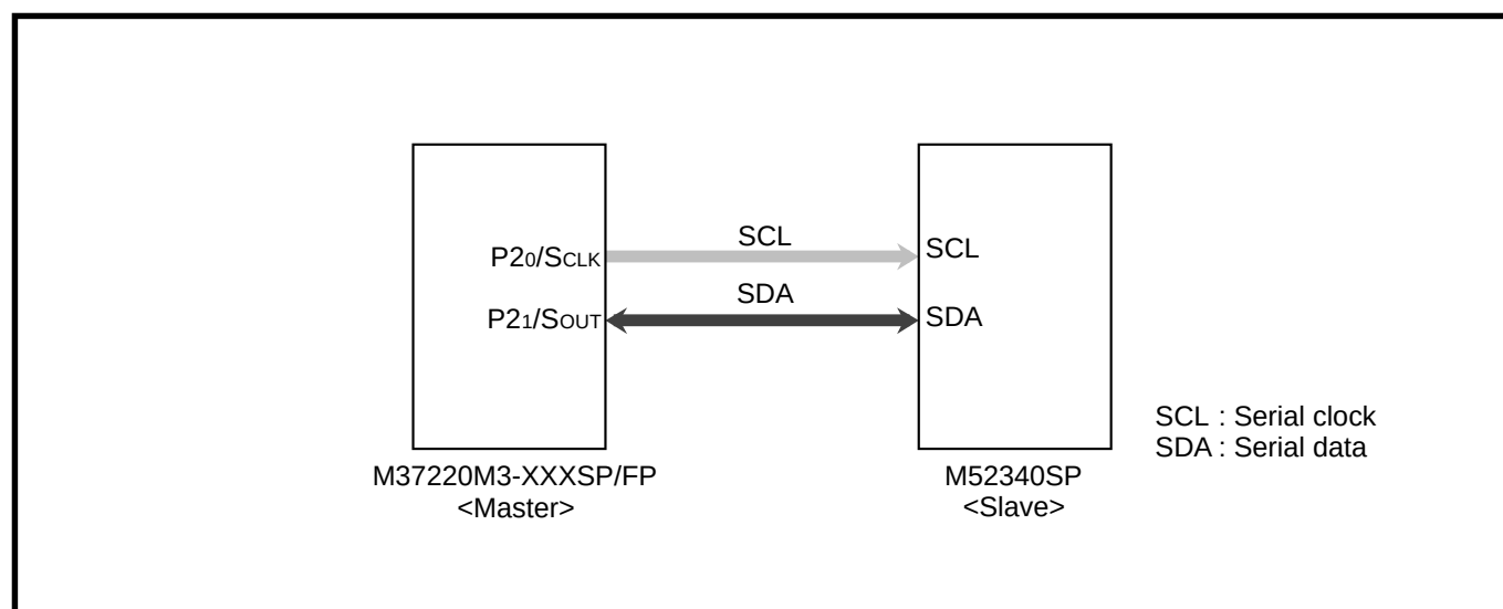
Fig. 5.5.1 Connection example
