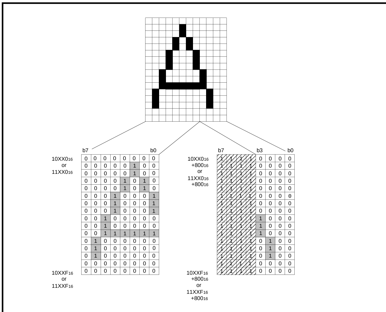
Fig. 2.11.10 Example of display character data storing form
