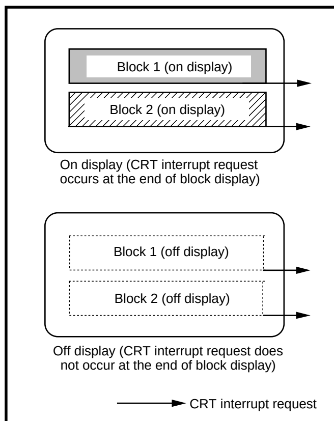
Fig. 2.11.14 Display state of blocks and occurrence of CRT interrupt request
