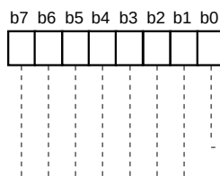
I 2 C address register (S0D) [Address 00D816]
