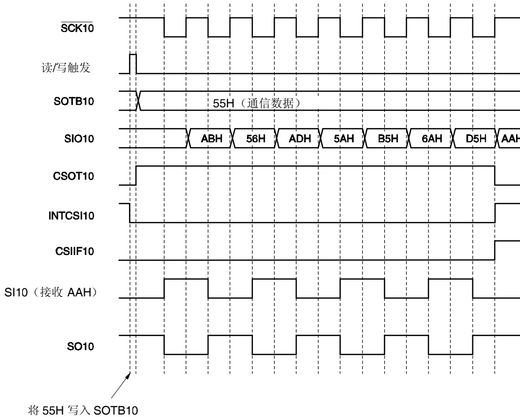
(a) 发送/接收时序 (类型 1: TRMD10 = 1, DIR10 = 0, CKP10 = 0, DAP10 = 0)
