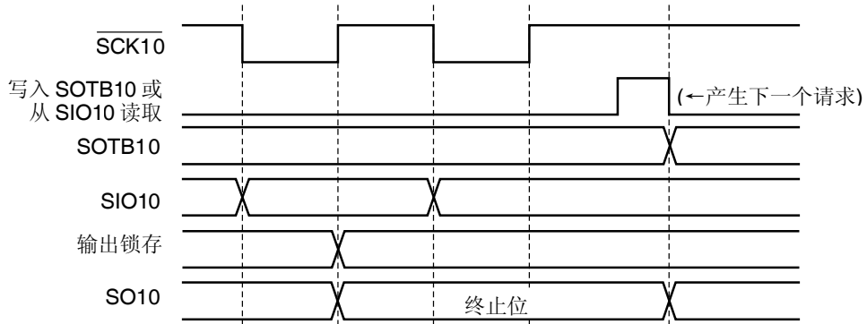
(c) 类型 2: CKP10 = 0, DAP10 = 1
