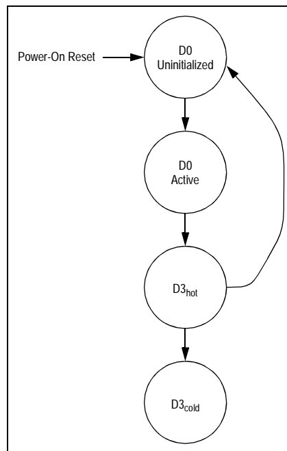
Figure 5.1 PES12N3 Power Management State Transition Diagram
