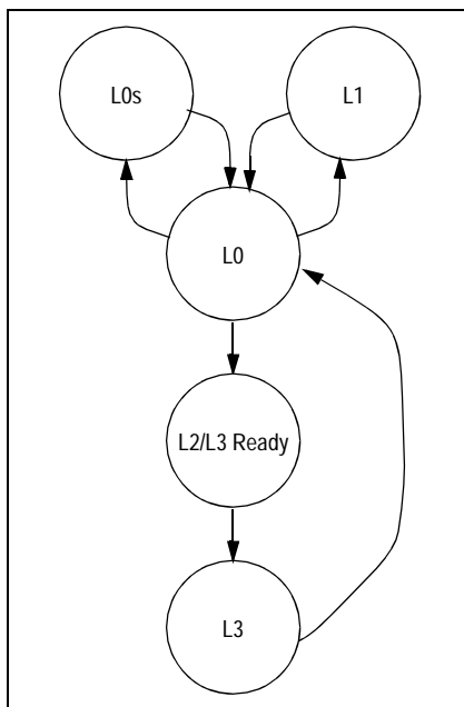
Figure 5.2 PES12N3 ASPM Link State Transitions
