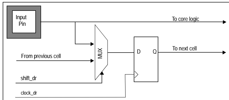
Figure 11.3 Diagram of Observe-only Input Cell
