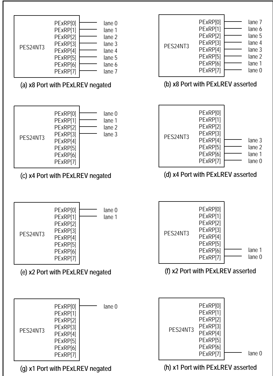
Figure 3.1 Lane Reversal for Maximum Link Width of x8
