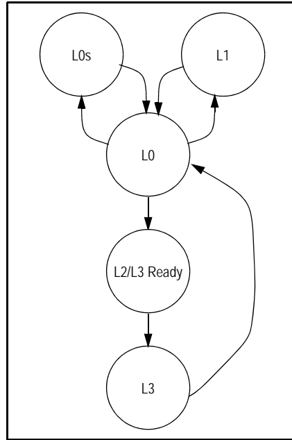
Figure 5.2 PES24NT3 ASPM Link State Transitions
