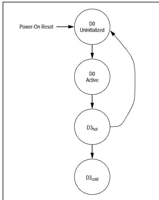
Figure 7.1 PES48H12 Power Management State Transition Diagram
