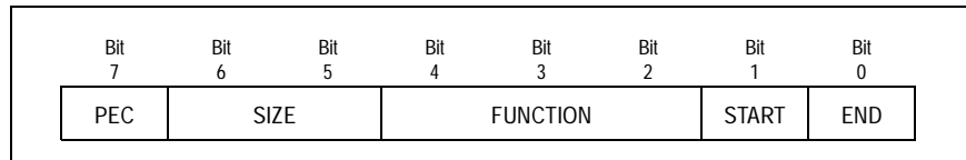
Figure 6.7 Slave SMBus Command Code Format
