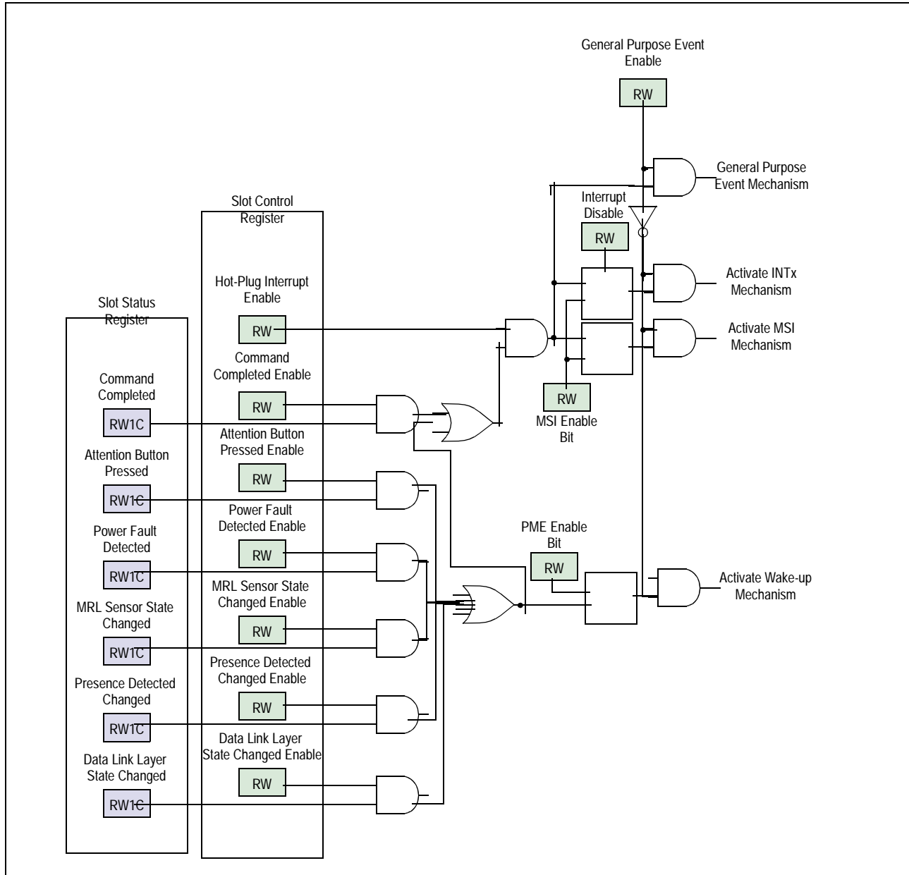
Figure 8.4 PES48H12 Hot-Plug Event Signalling
