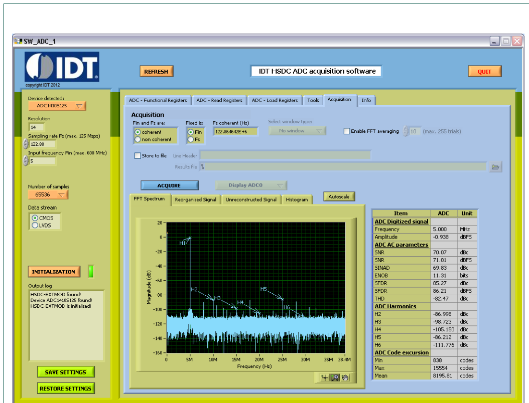
Fig 14. SW_ADC_1_r02: "Acquisition" page, FFT graph
