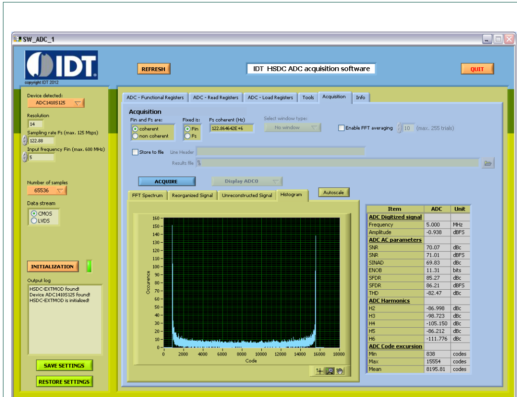
Fig 17. SW_ADC_1_r02: “Acquisition” page, code histogram graph
