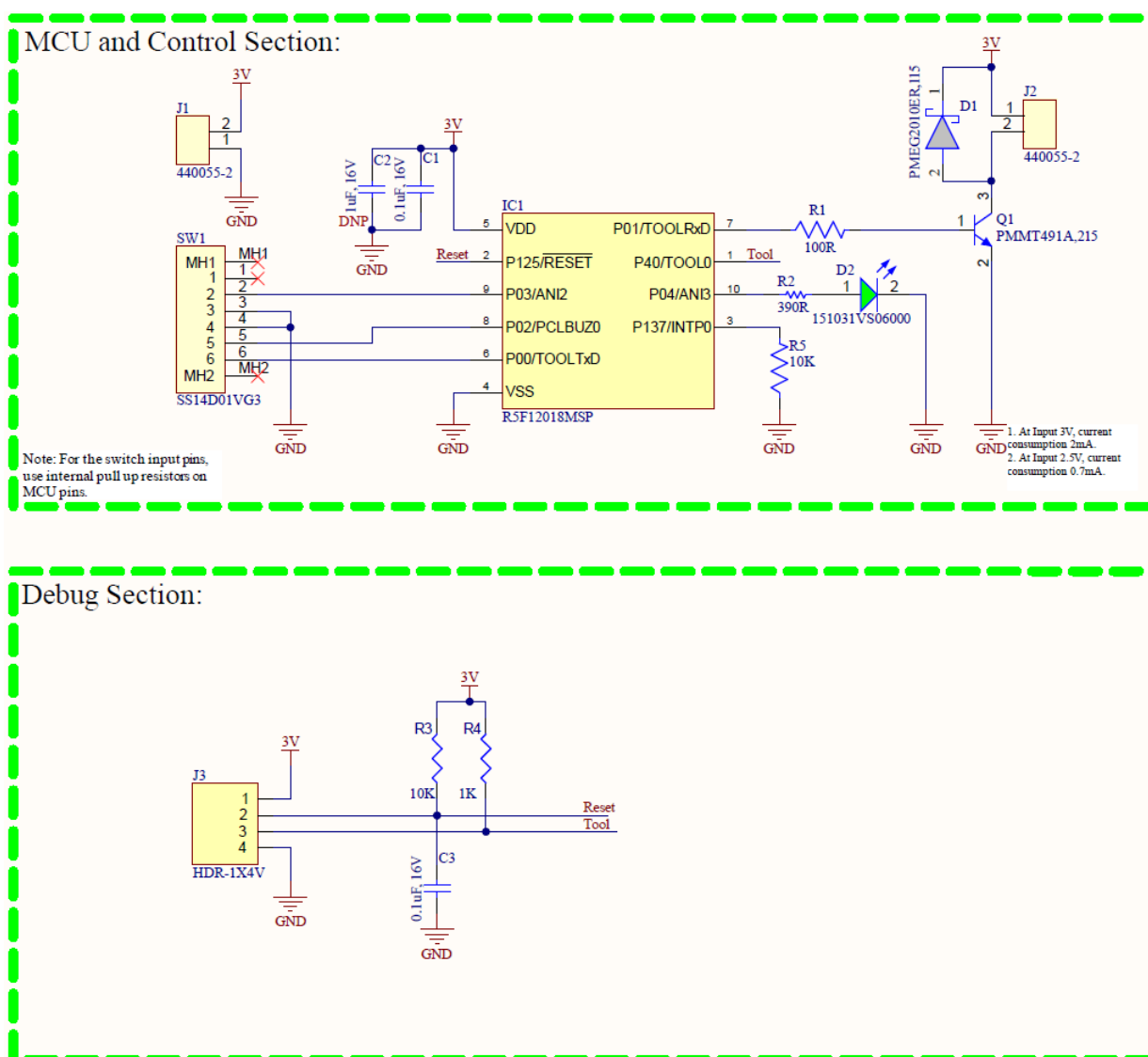
Figure 5: AS064-AIRFRSHNRREFZ Schematics
