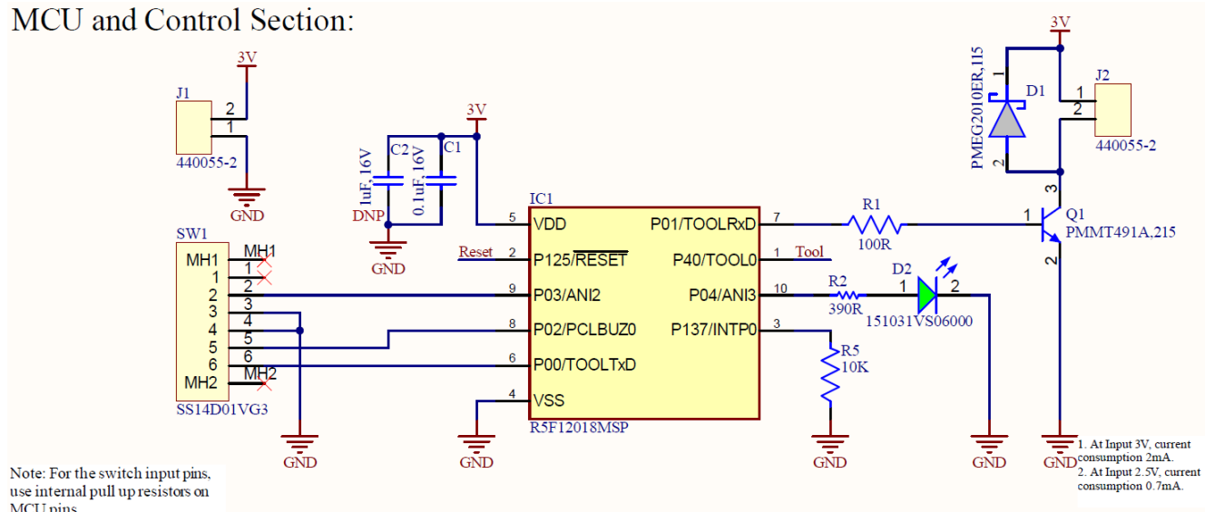
Figure 2: MCU Section
