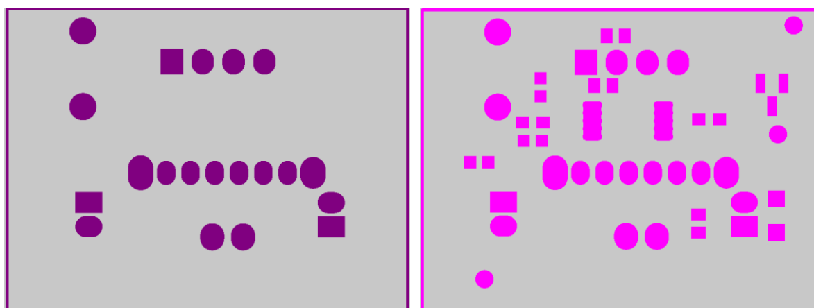
Figure 8: Top and Bottom Solder Mask
