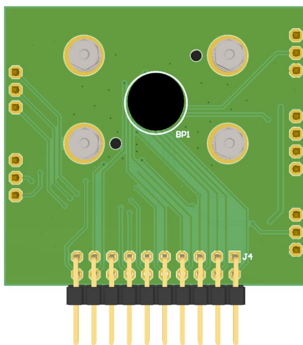
Figure 3. Bottom View
