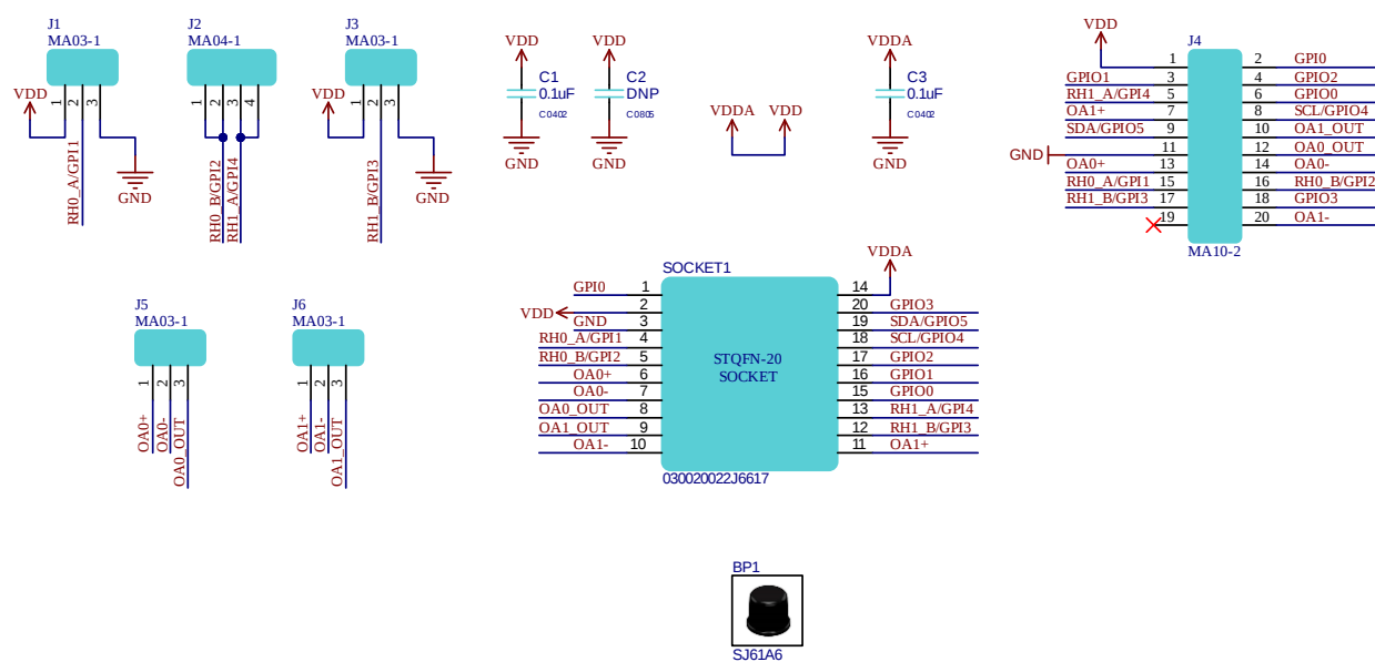
Figure 4. Board Schematic
