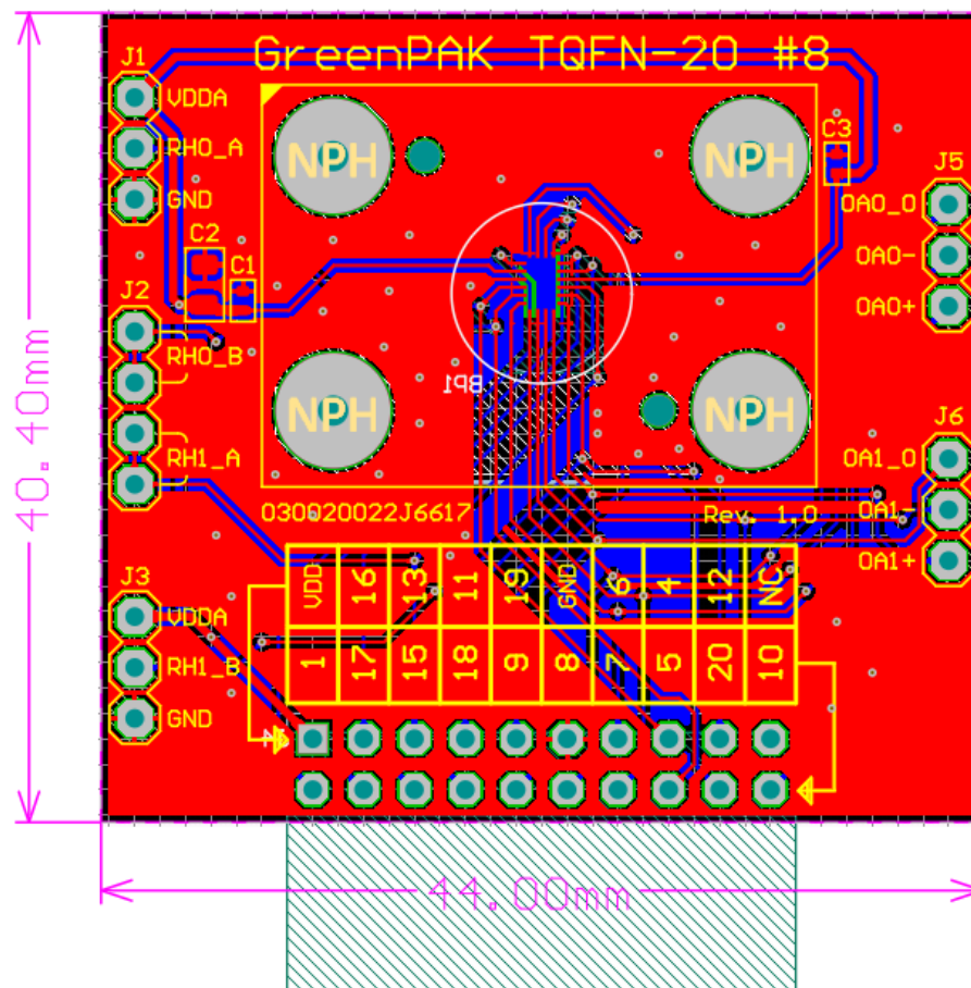
Figure 1. PCB View (All Sizes in mm)
