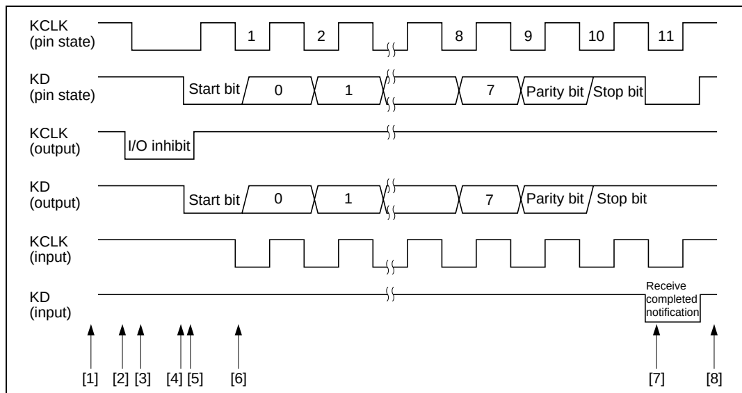
Figure 17.6 Transmit Timing
