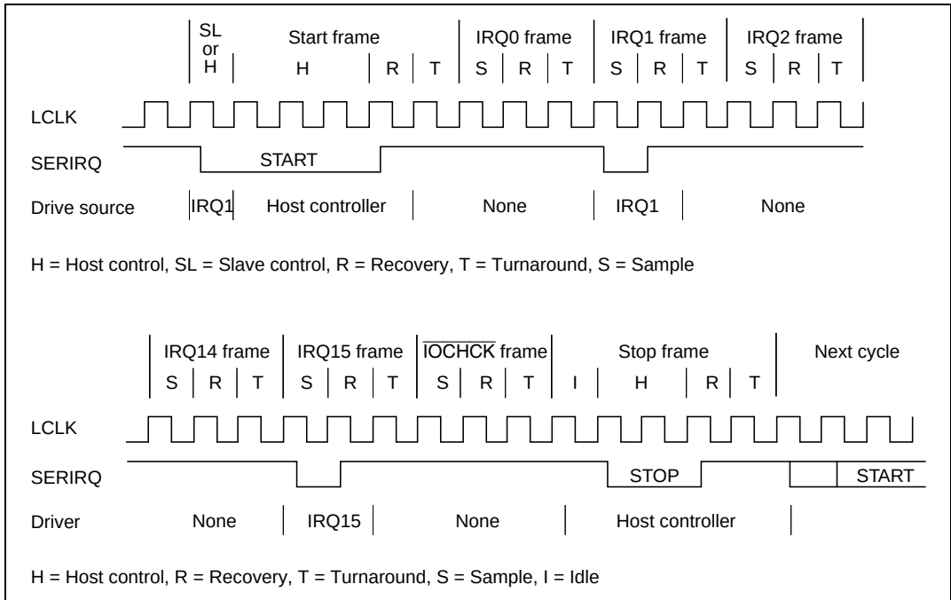
Figure 18B.6 SERIRQ Timing
