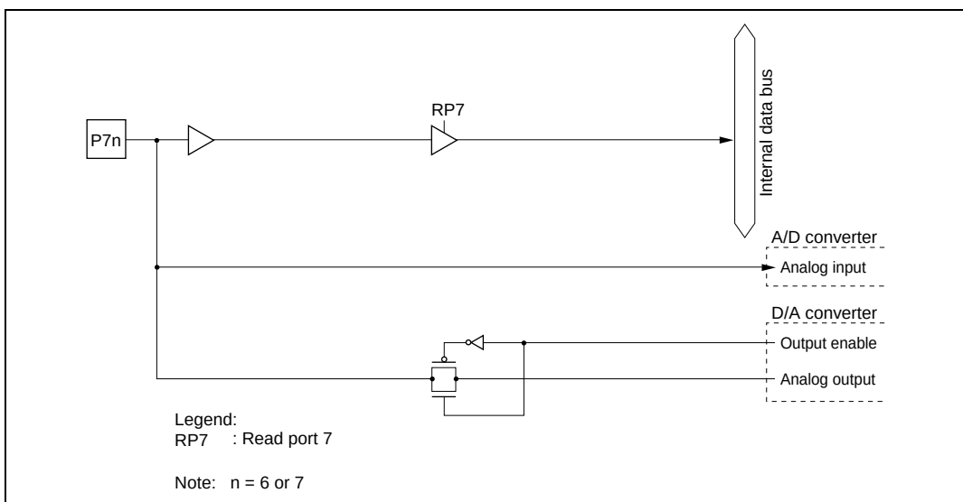
Figure C.24 Port 7 Block Diagram (Pins P76, P77)
