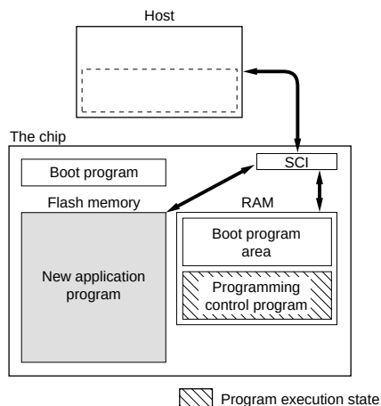
Figure 22.4 Boot Mode
