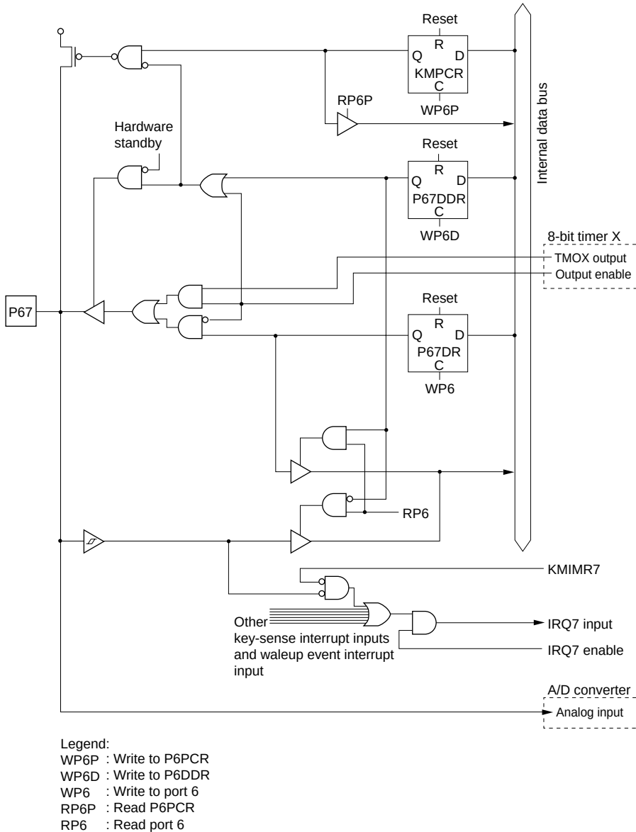
Figure C.22 Port 6 Block Diagram (Pin P67)
