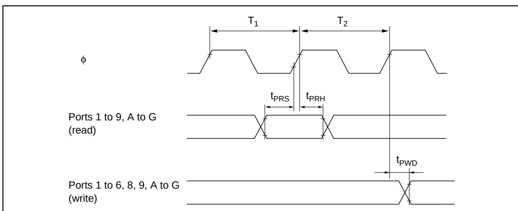
Figure 25.14 I/O Port Input/Output Timing
