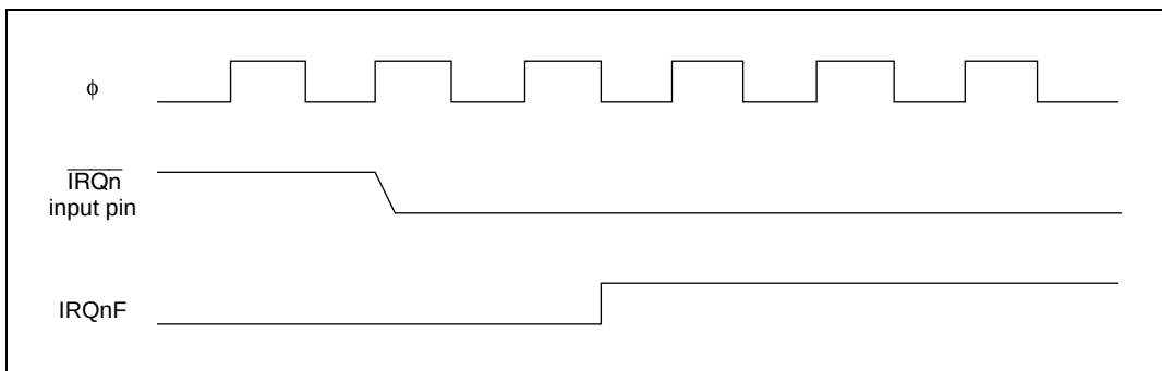
Figure 5.4 Timing of \text{IRQnF} Setting
