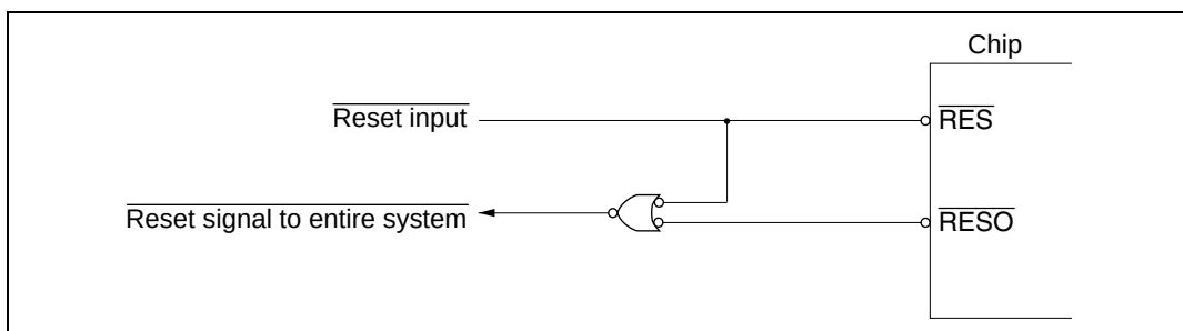
Figure 14.8 Sample Circuit for System Reset by \overline{\text{RESO}} Signal
