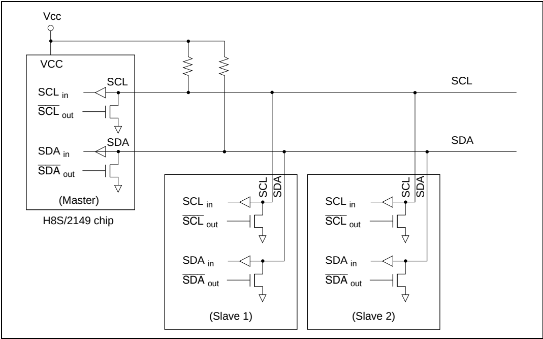
Figure 16.2 I 2 C Bus Interface Connections (Example: H8S/2169 or H8S/2149 Chip as Master)
