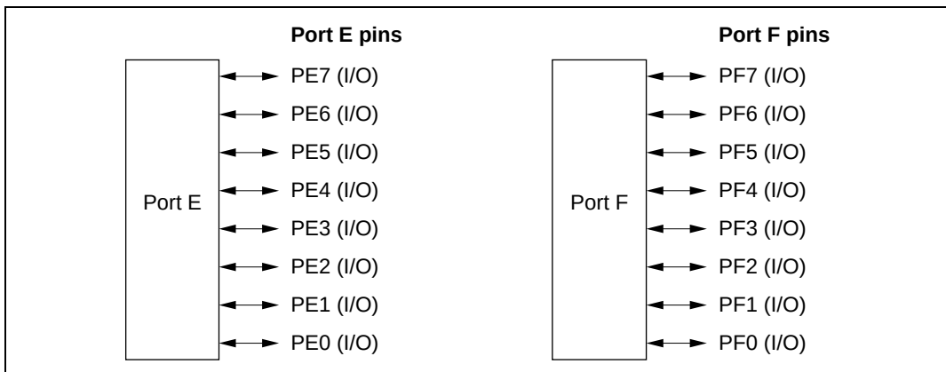
Figure 8.21 Pin Functions for Ports E and F
