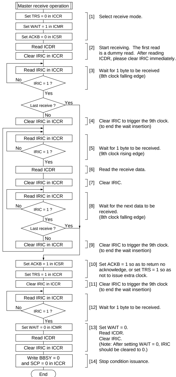
Figure 16.15 Flowchart for Master Receive Mode (Example)
