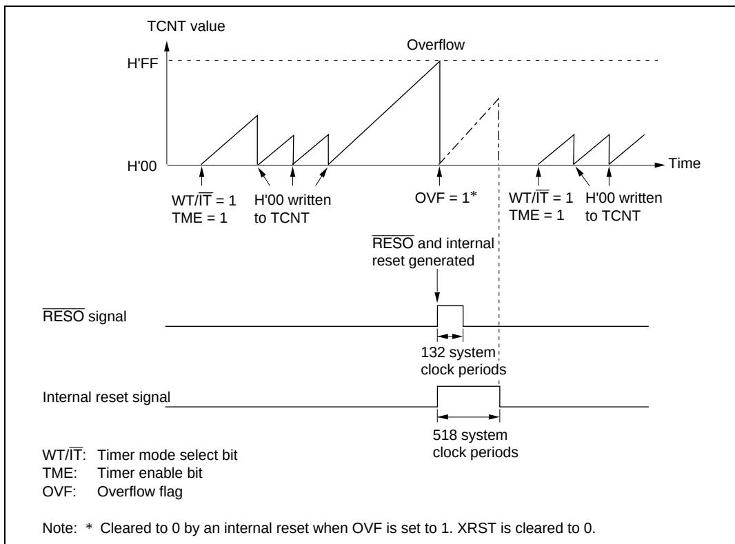
Figure 14.3 Operation in Watchdog Timer Mode ( \text{RST}/\overline{\text{NMI}} = 1 )
