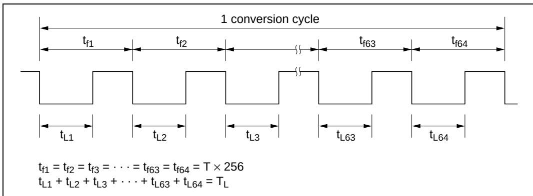
Figure 10.4 (2) Output Waveform
