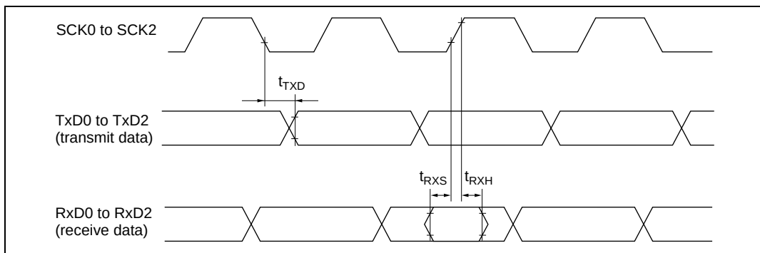
Figure 25.22 SCI Input/Output Timing (Synchronous Mode)
