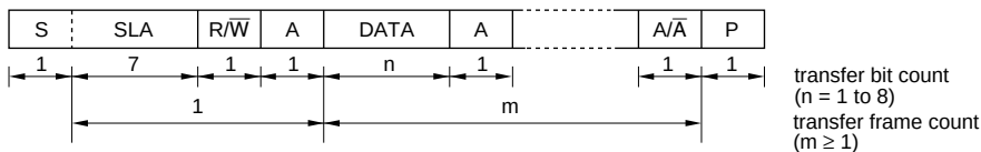
(a) I 2 C bus format (FS = 0 or FSX = 0)
