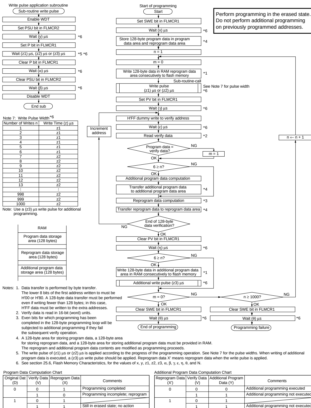
Figure 22.12 Program/Program-Verify Flowchart
