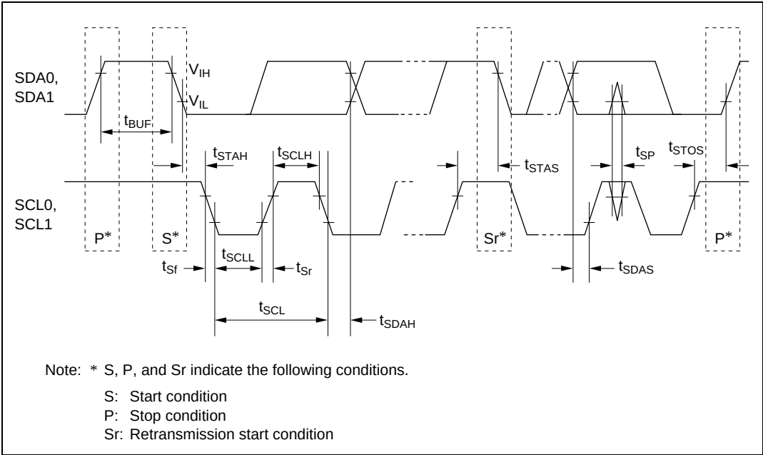
Figure 25.27 I²C Bus Interface Input/Output Timing
