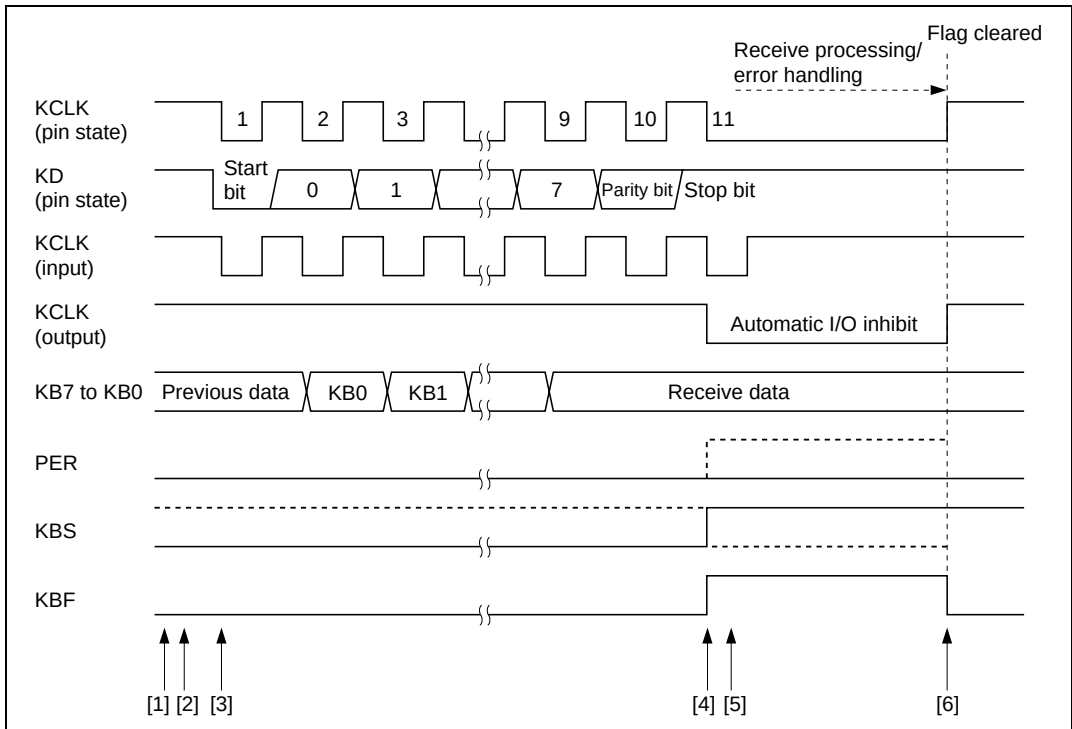
Figure 17.4 Receive Timing
