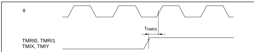
Figure 25.19 8-Bit Timer Reset Input Timing
