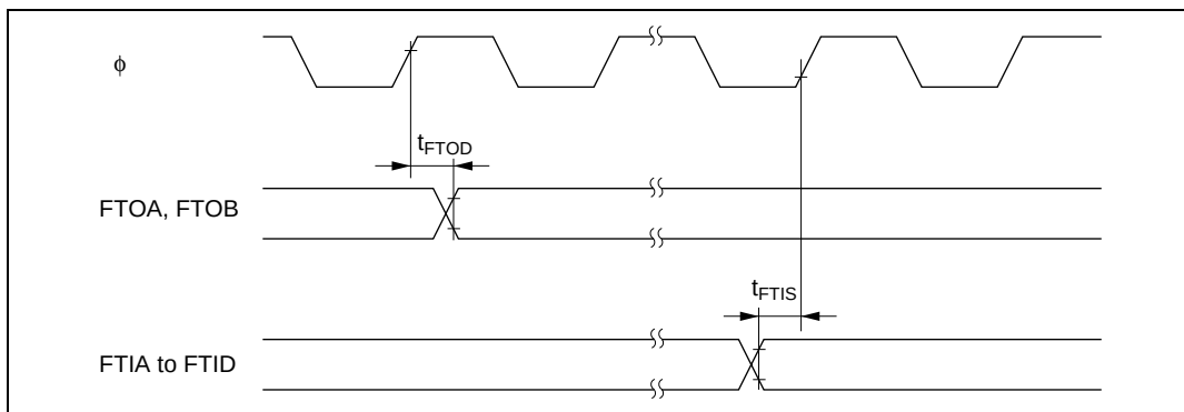
Figure 25.15 FRT Input/Output Timing
