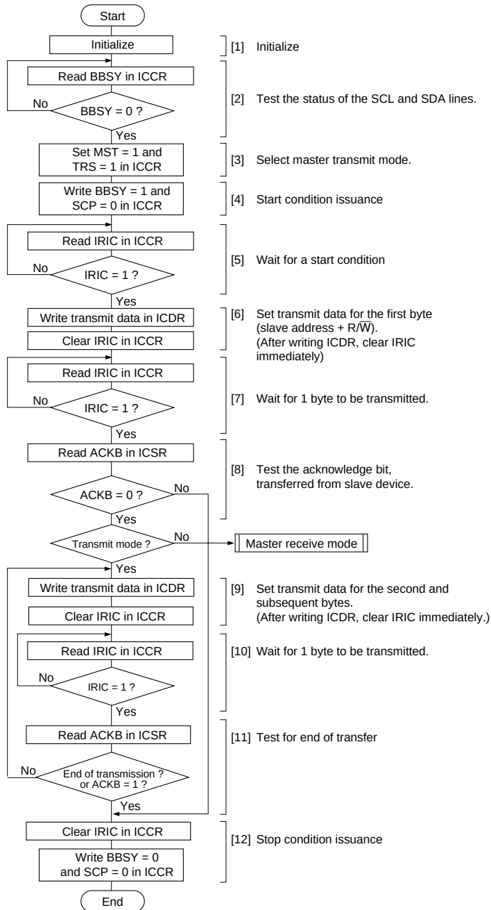
Figure 16.14 Flowchart for Master Transmit Mode (Example)
