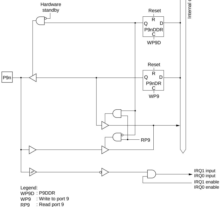
Figure C.33 Port 9 Block Diagram (Pins P91, P92)
