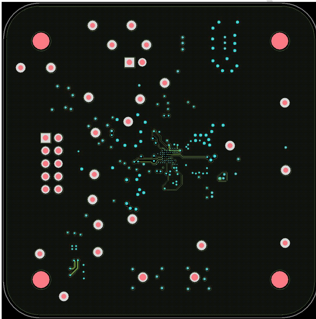
Figure 5. Mid 1 Layer
