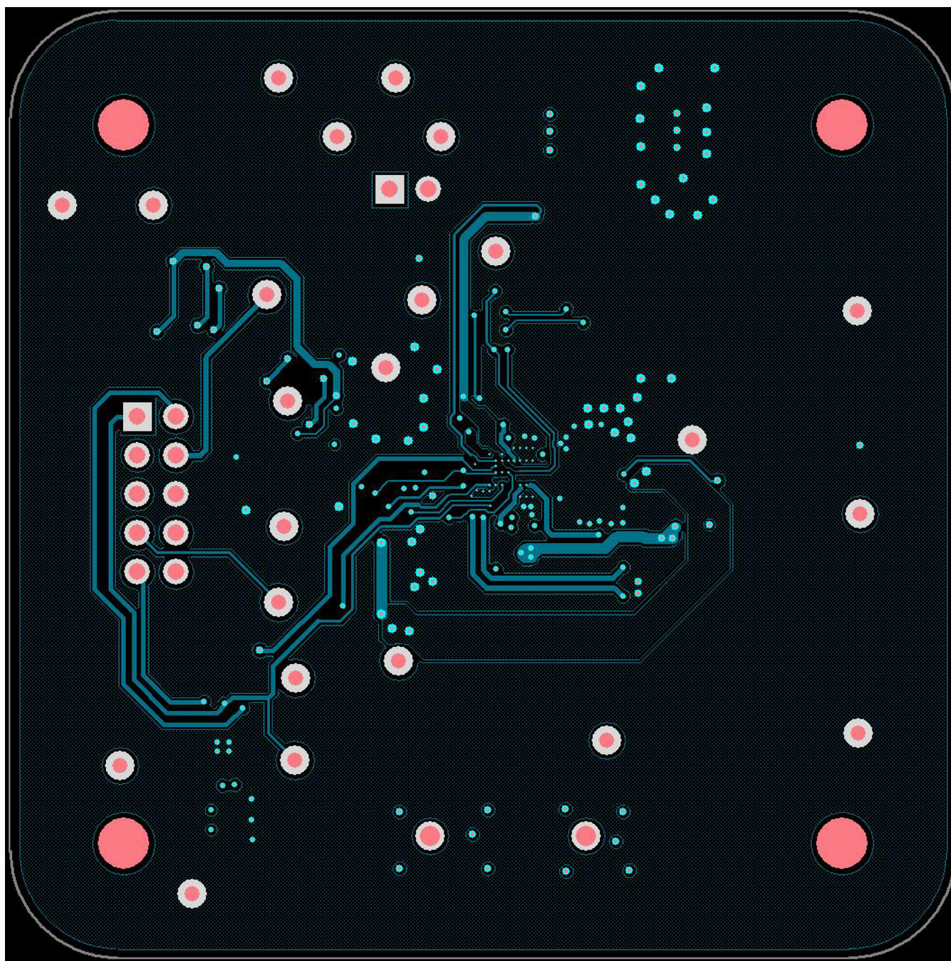
Figure 6. Mid 2 Layer
