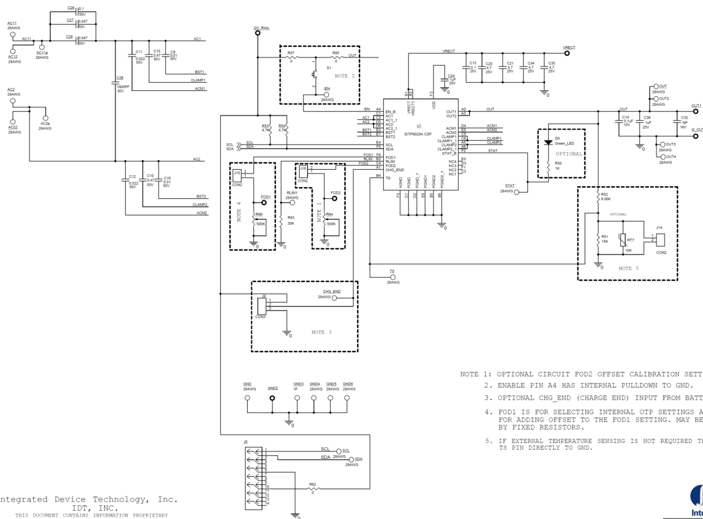
IDTP9025A CSP DEMO PCB V1.1 WPC ONLY
