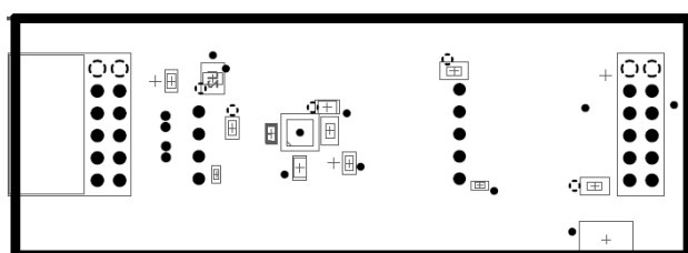
Figure 8. Int 1 (PWR)
