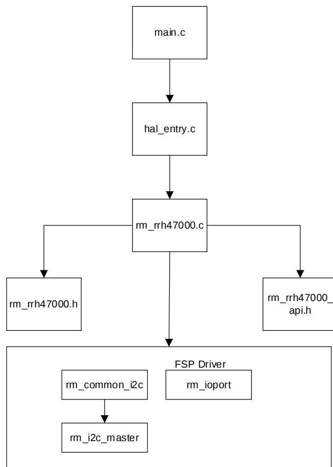
Figure 14. Code Dependency Graph
