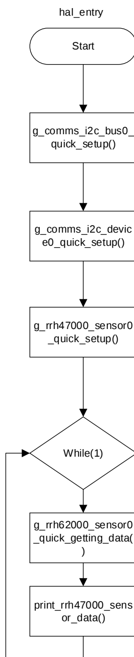
Figure 15. Algorithm Flowchart
