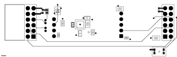
Figure 10. Bottom Layer
