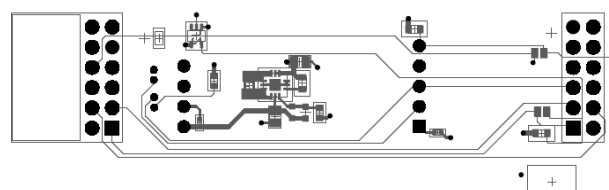
Figure 7. Bottom Layer
