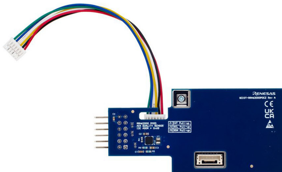
Figure 5. QCIOT-RRH62000 Pmod (Bottom)
