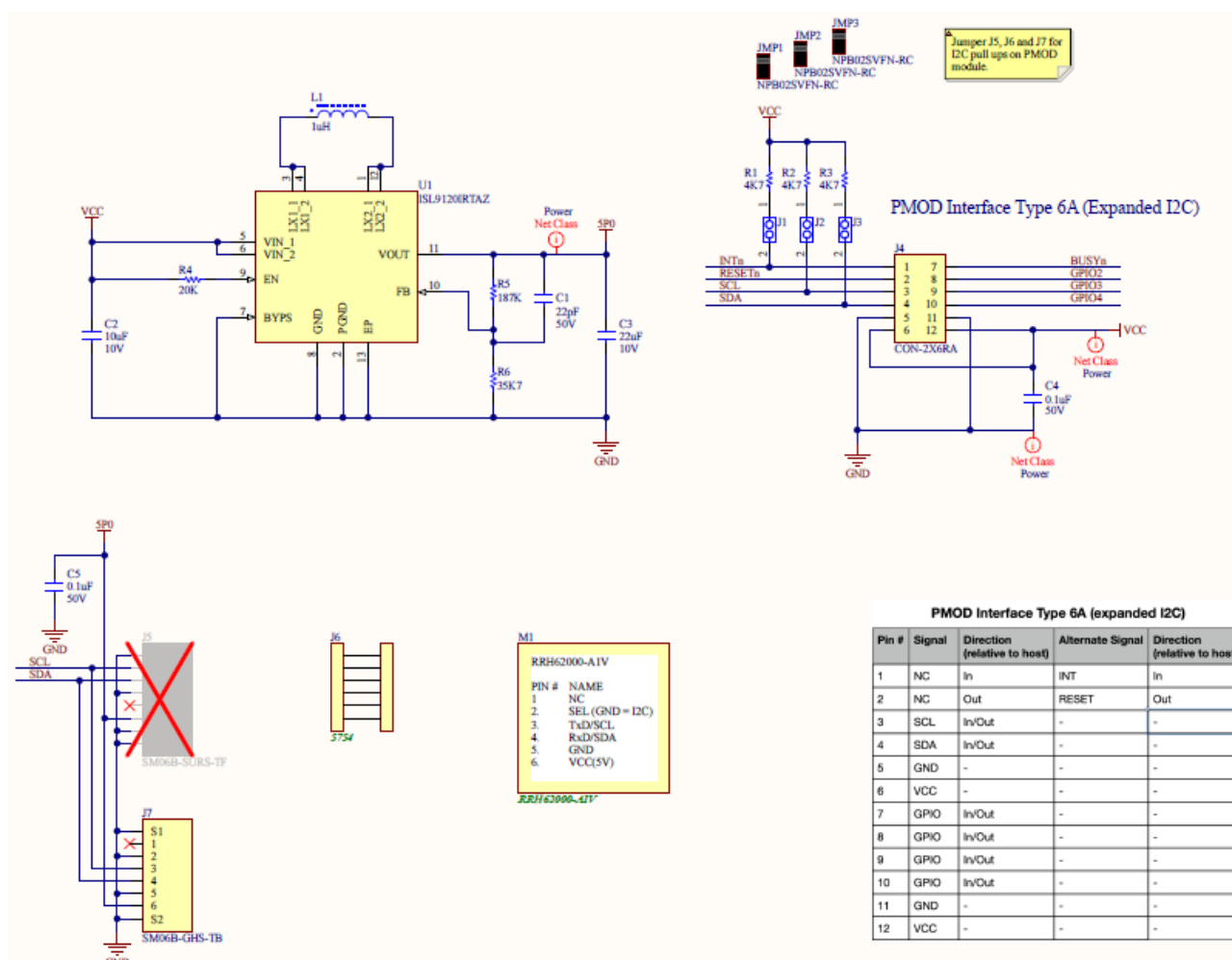
Figure 6. QCIOT-RRH62000 Pmod Schematic Diagrams
