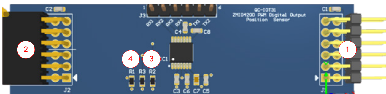
Figure 6. Evaluation Kit Connections
