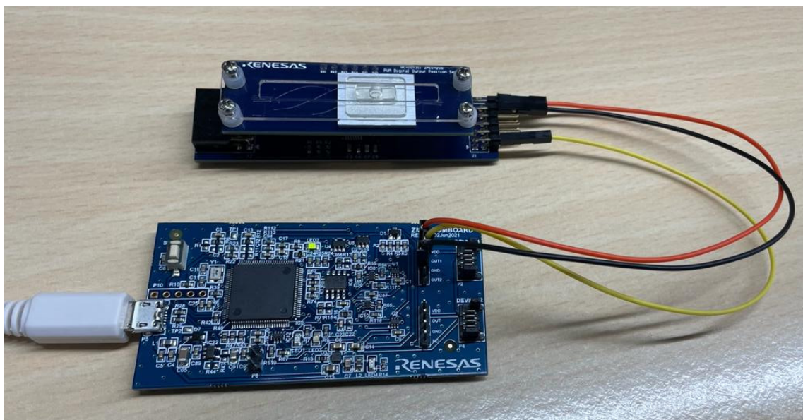
Figure 4. QCIOT31-ZMID4200POCZ and ZMID4200STKI Hardware Setup
