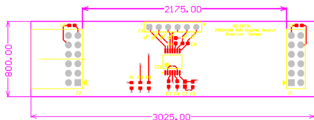
Figure 9. Top Layer
