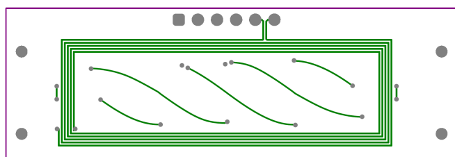
Figure 15. Internal Plane-1
