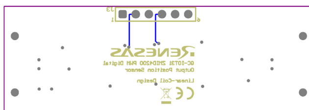
Figure 14. Bottom Layer
