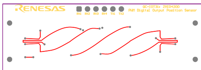
Figure 13. Top Layer
