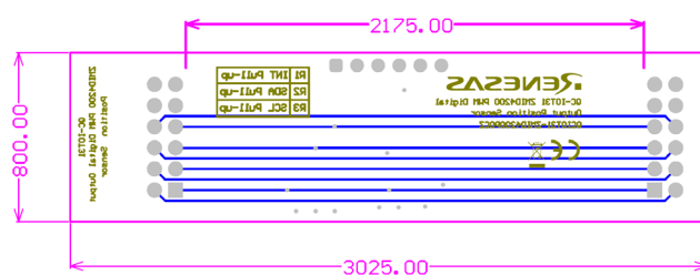
Figure 10. Bottom Layer
