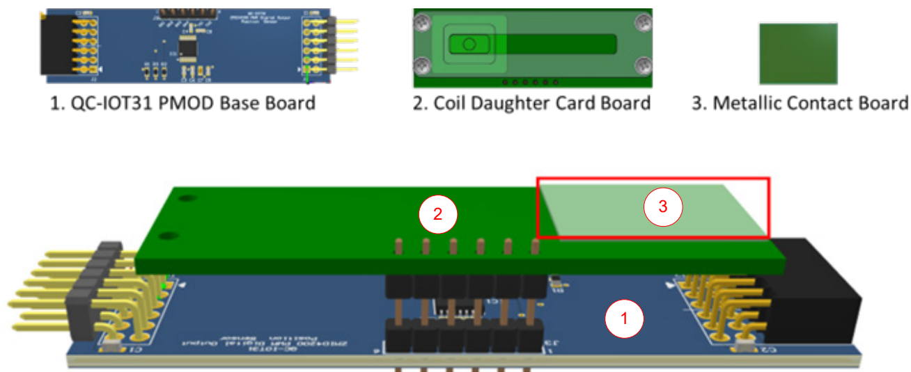
Figure 5. QCIOT31 Hardware Setup with Linear Coil
