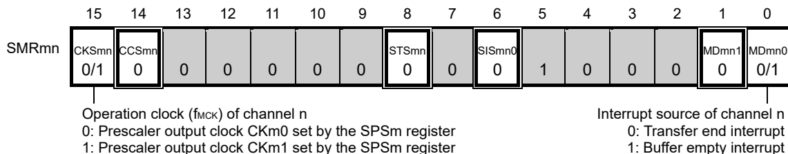
Figure 12-30. Example of Contents of Registers for Master Reception of Simplified SPI (CSI00, CSI01) (1/2)
