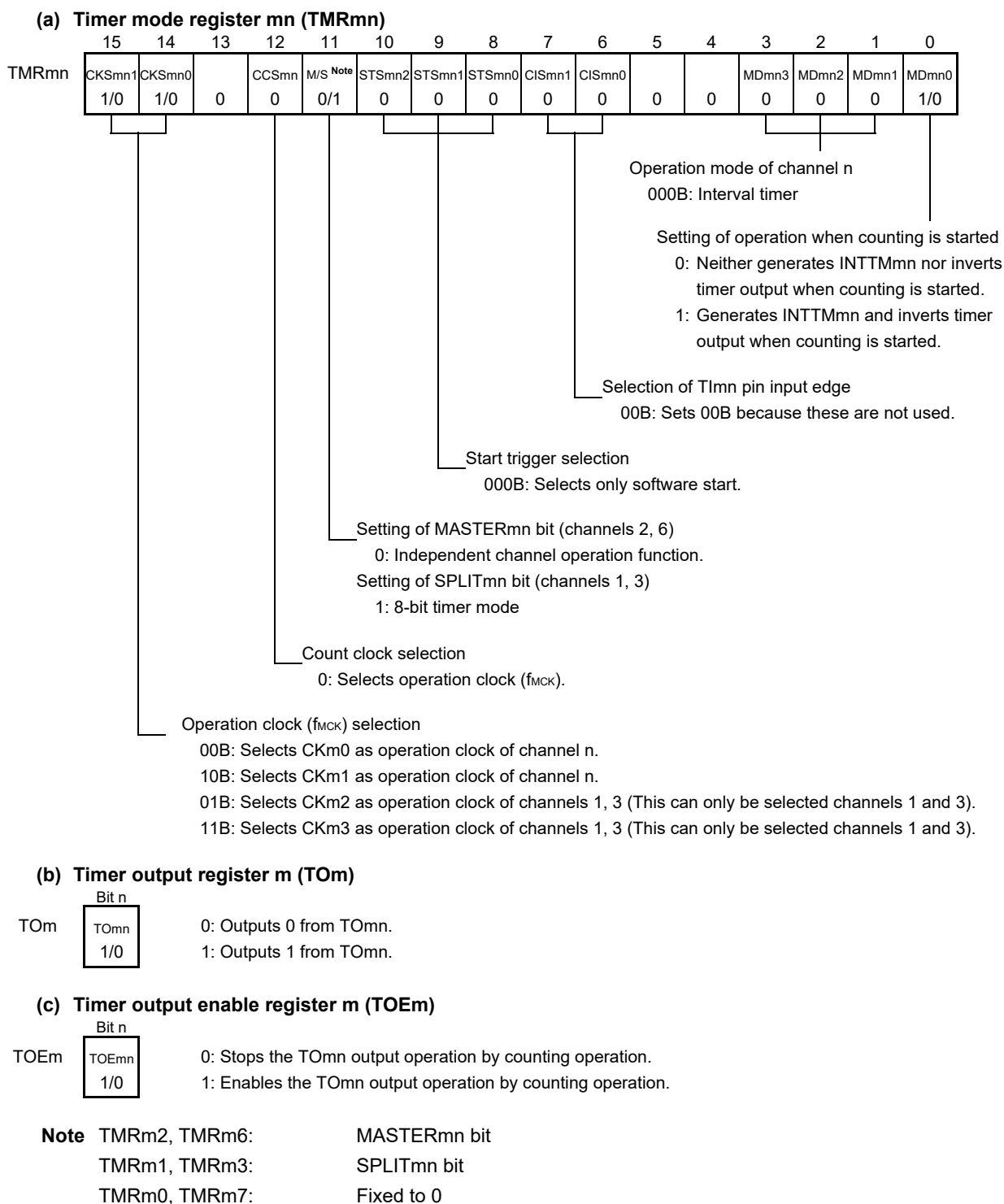
Figure 6-45. Example of Set Contents of Registers During Operation as Interval Timer/Square Wave Output (1/2)
