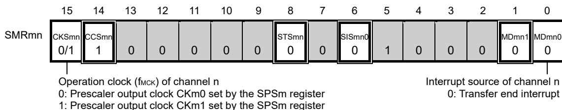
Figure 12-54. Example of Contents of Registers for Slave Reception of Simplified SPI (CSI00, CSI01) (1/2)
