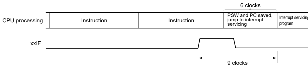
Figure 20-8. Interrupt Request Acknowledgment Timing (Minimum Time)
