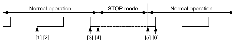
Figure 16-29. Clock Stop and Restart Procedure
