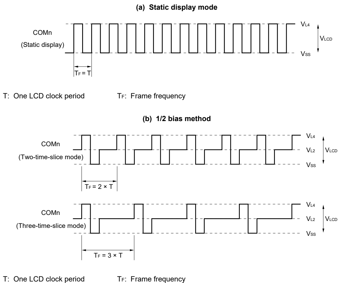
Figure 17-23. Common Signal Waveforms (1/2)
