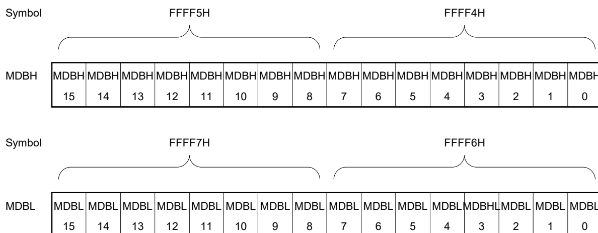
Figure 18-3. Format of Multiplication/Division Data Register B (MDBH, MDBL)
