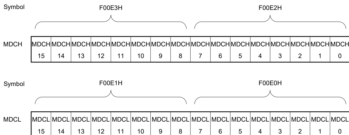
Figure 18-4. Format of Multiplication/Division Data Register C (MDCH, MDCL)
