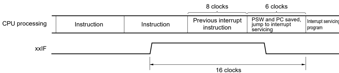
Figure 20-9. Interrupt Request Acknowledgment Timing (Maximum Time)
