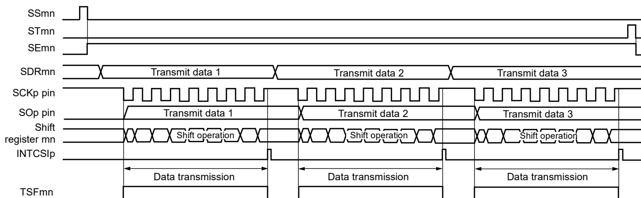
Figure 14-53. Timing Chart of Slave Transmission (in Single-Transmission Mode) (Type 1: DAPmn = 0, CKPmn = 0)
