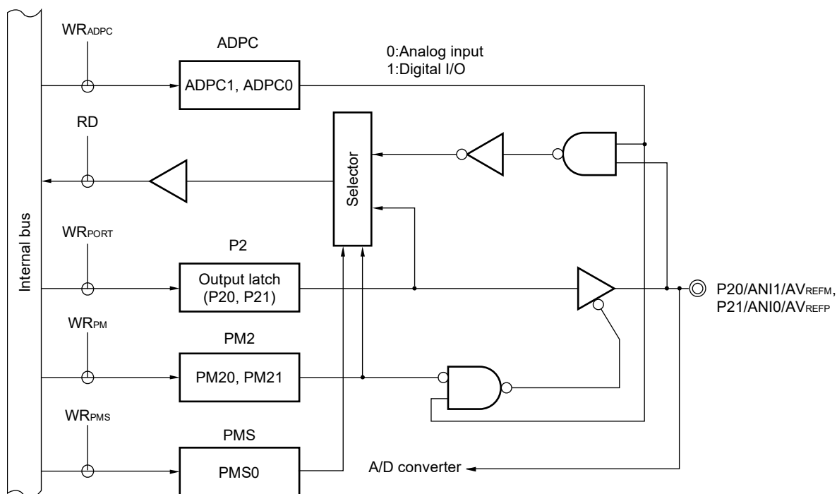
Figure 4-9. Block Diagrams of P20 and P21
