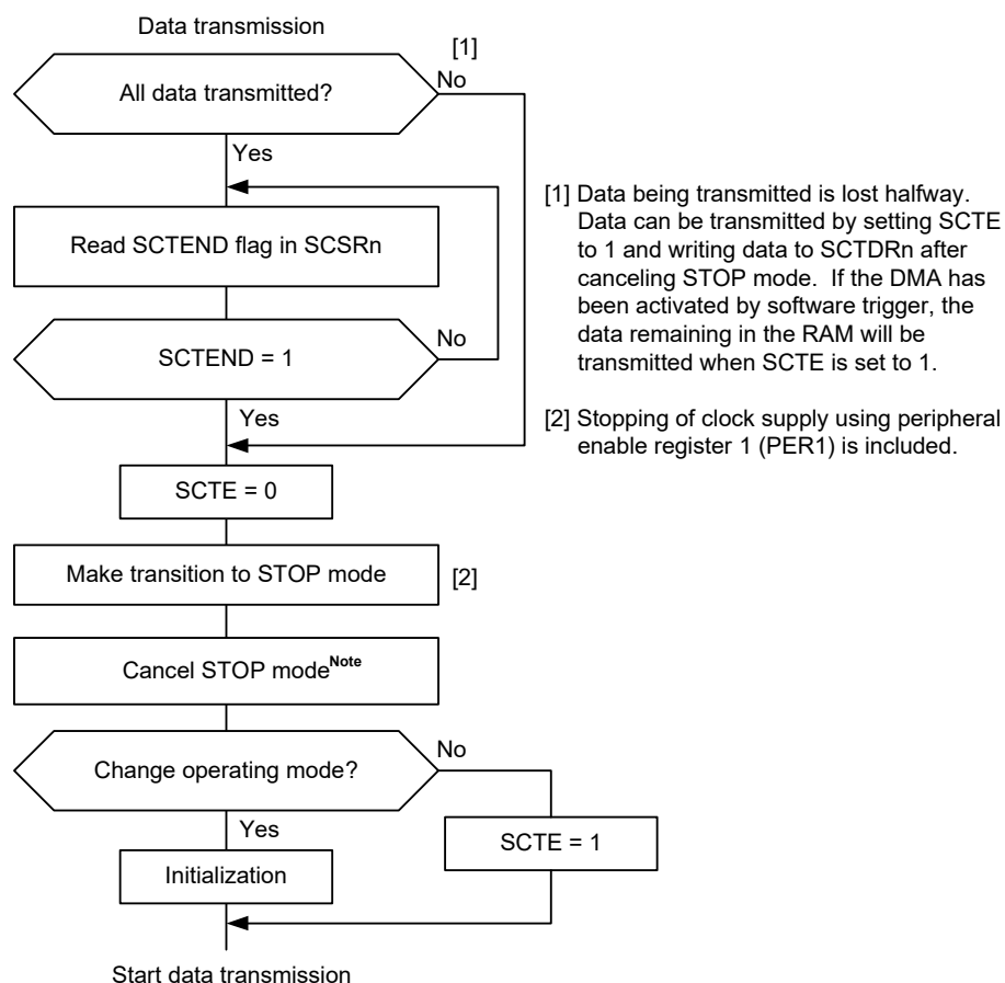
Figure 16-34. Sample Flowchart for Mode Transition During Transmission
