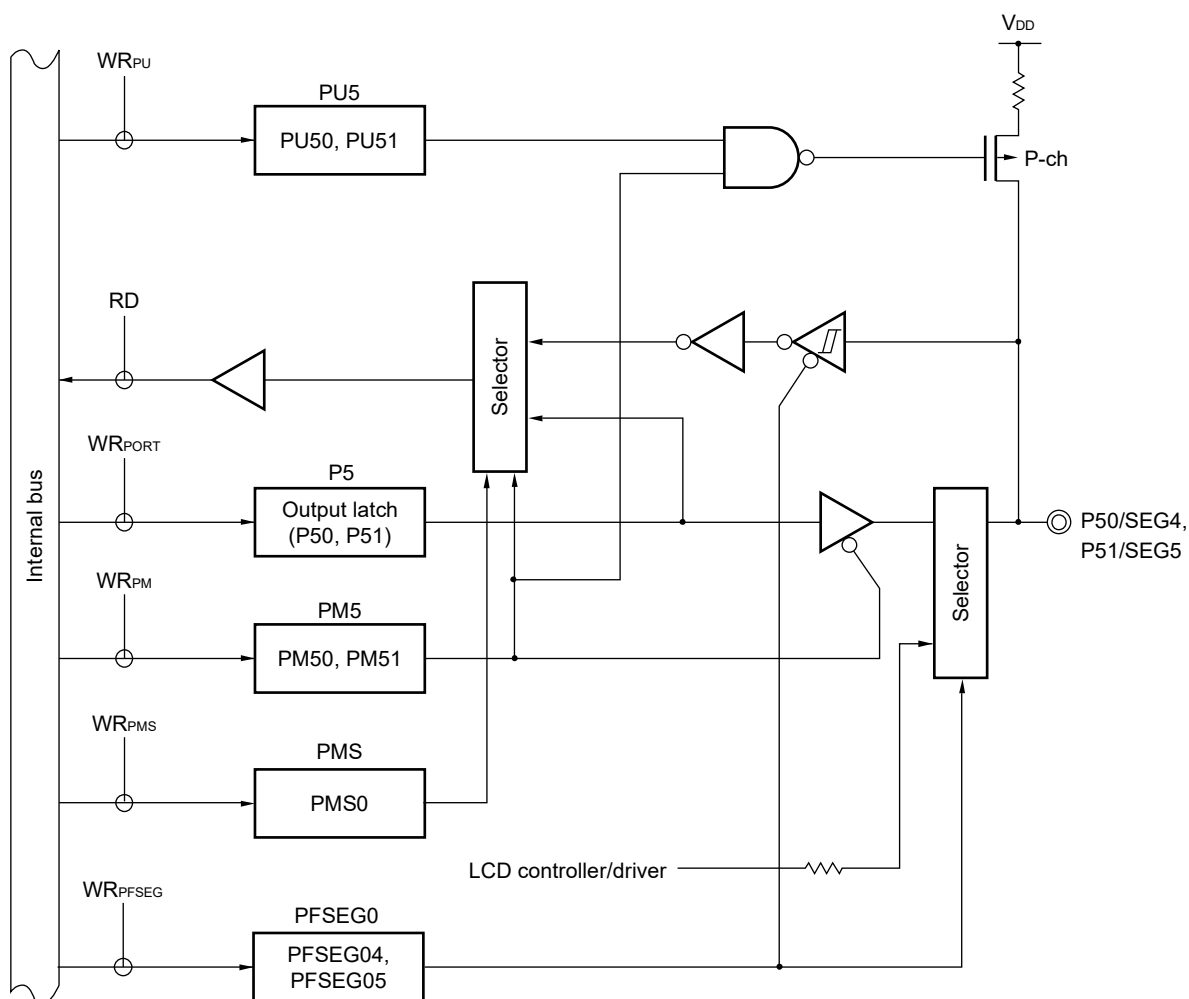
Figure 4-22. Block Diagrams of P50 and P51
