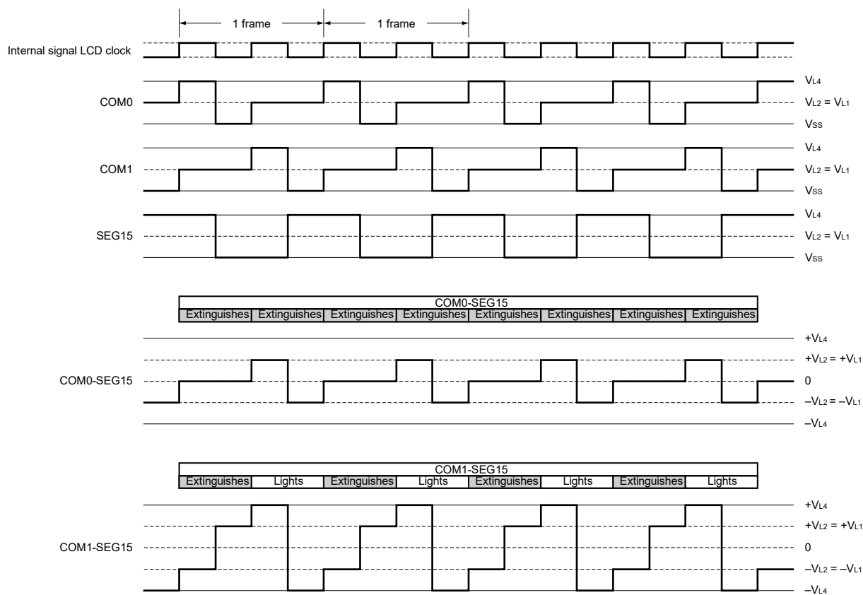
Figure 17-30. Two-Time-Slice LCD Drive Waveform Examples Between SEG15 and Each Common Signals (1/2 Bias Method)
