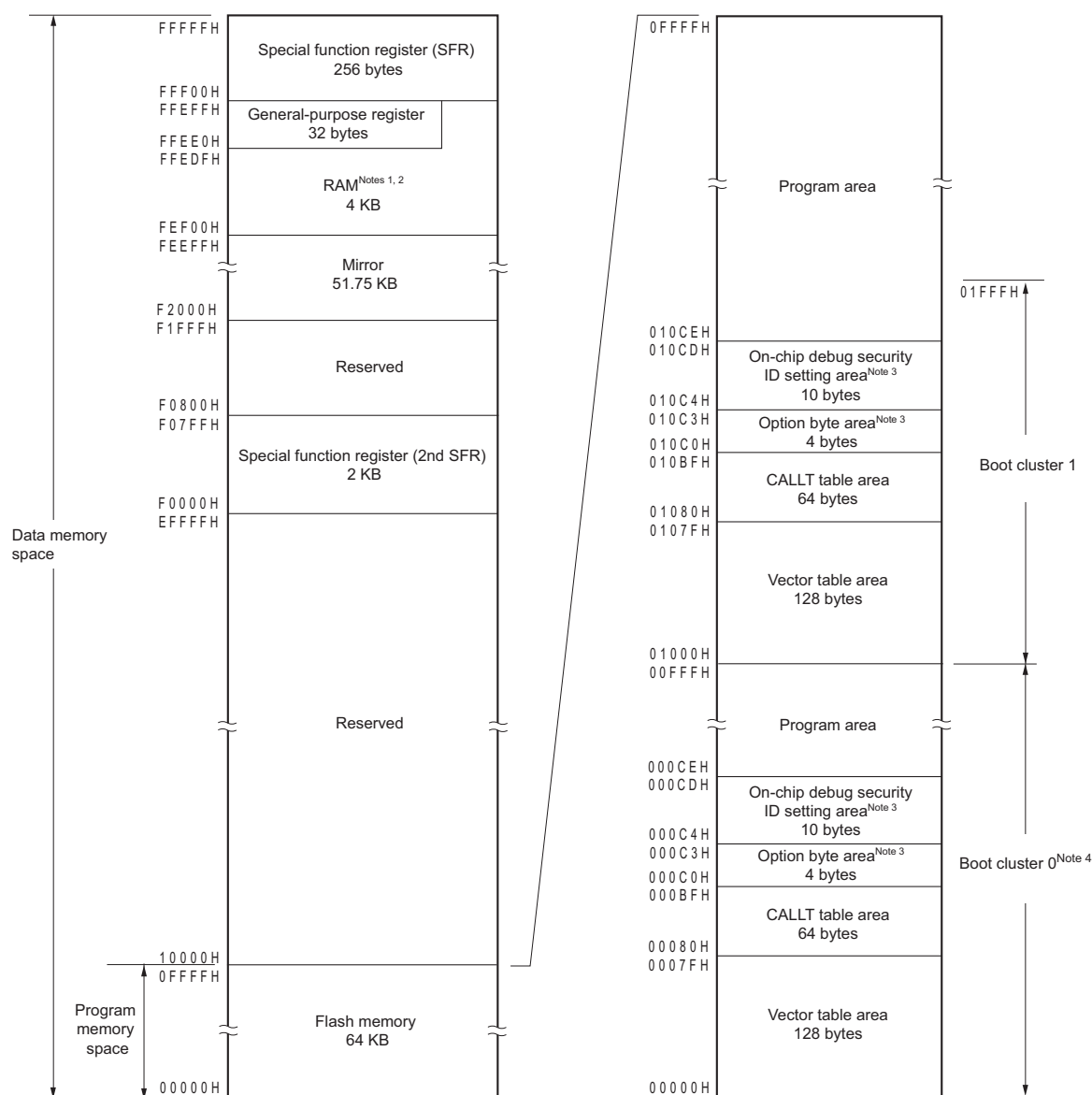
Figure 3-1. Memory Map
