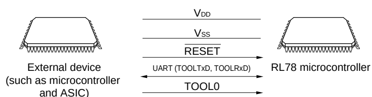
Figure 27-3. Environment for Writing Program to Flash Memory
