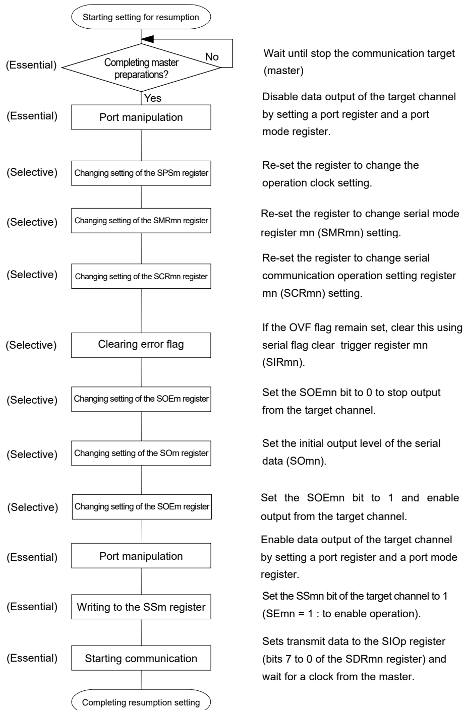
Figure 14-66. Procedure for Resuming Slave Transmission/Reception
