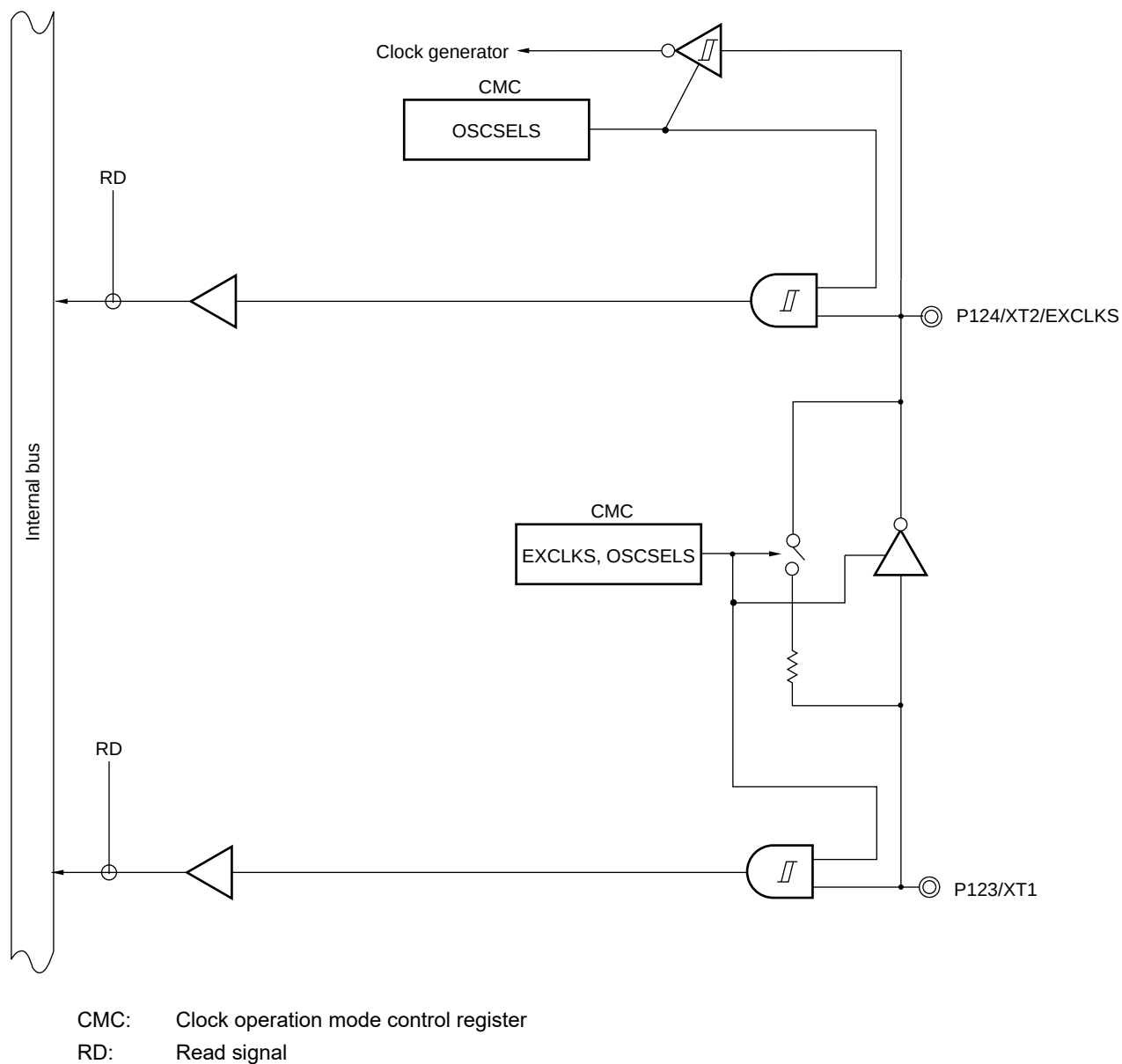
Figure 4-25. Block Diagram of P123 and P124
