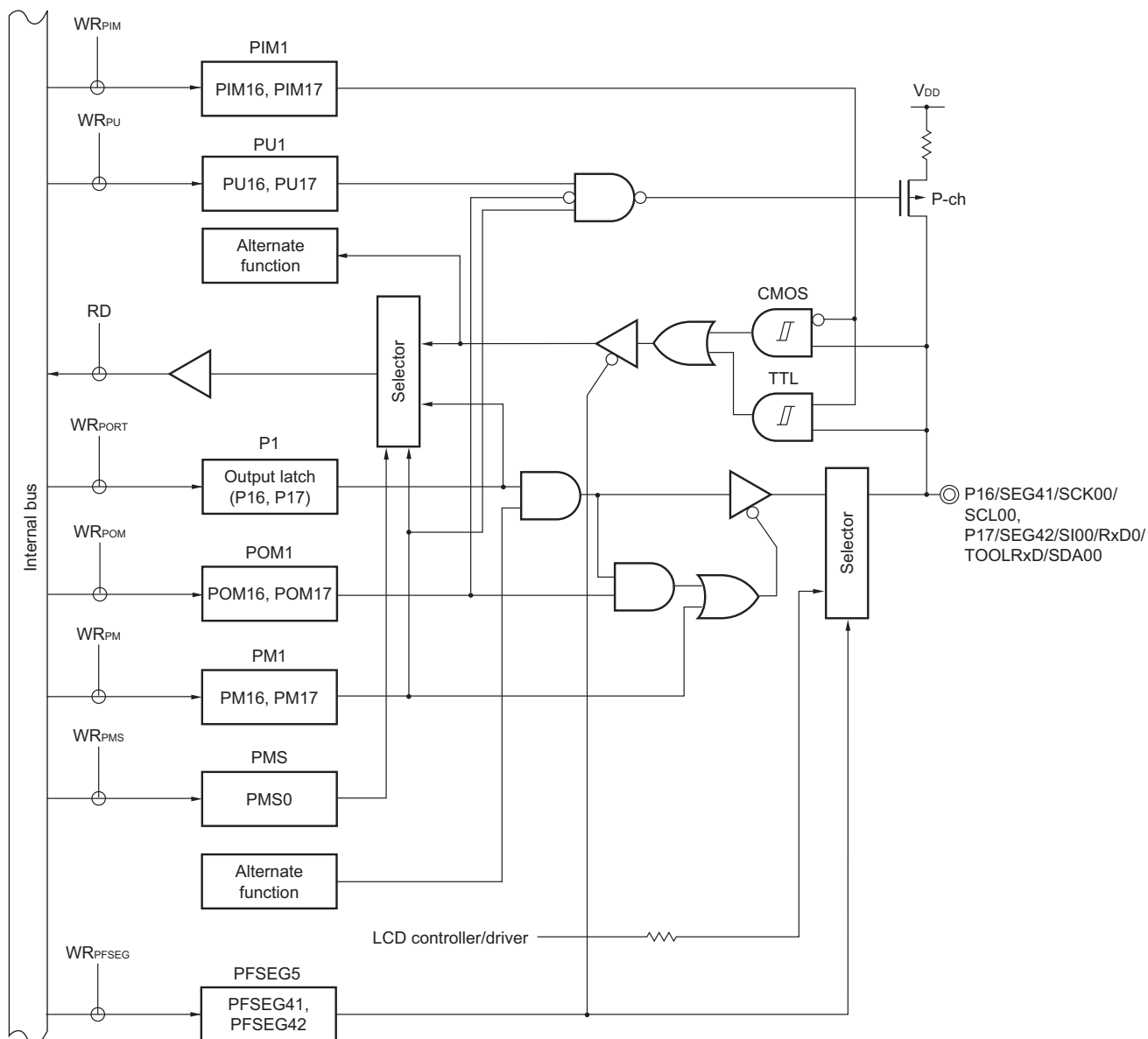
Figure 4-8. Block Diagram of P16 and P17
