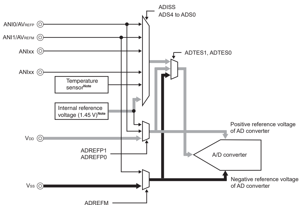
Figure 24-15. Configuration of A/D Test Function
