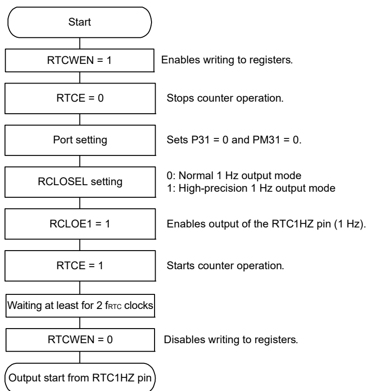
Figure 7-24. 1 Hz Output Setting Procedure
