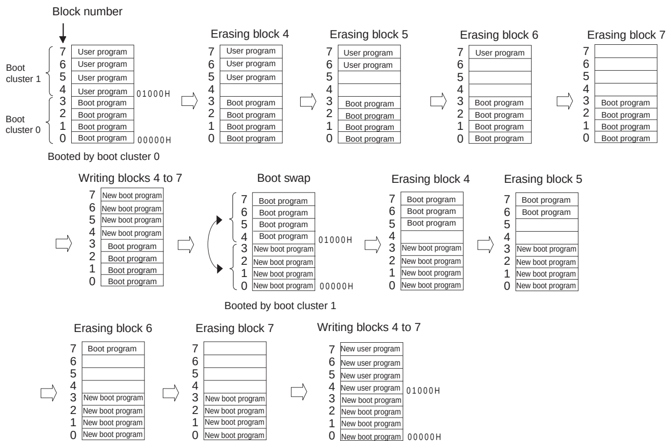
Figure 27-10. Example of Executing Boot Swapping
