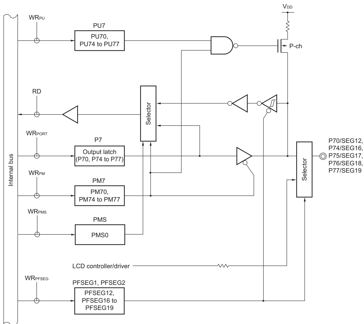
Figure 4-23. Block Diagram of P70 and P74 to P77
