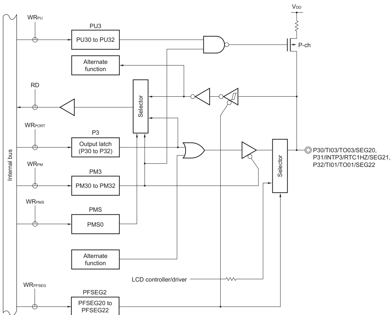
Figure 4-12. Block Diagram of P30 to P32
