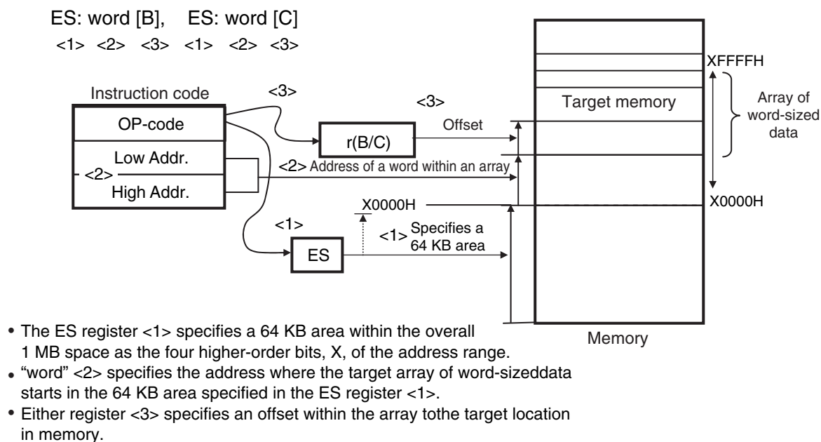
Figure 3-28. Example of ES:word[B], ES:word[C]
