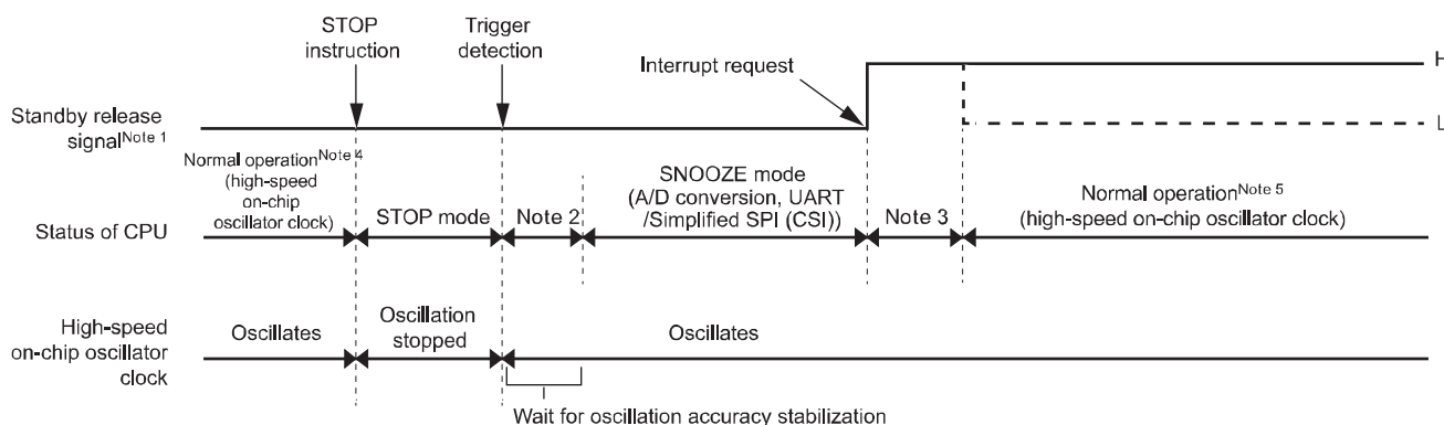
Figure 20-5. When the Interrupt Request Signal is Generated in the SNOOZE Mode
