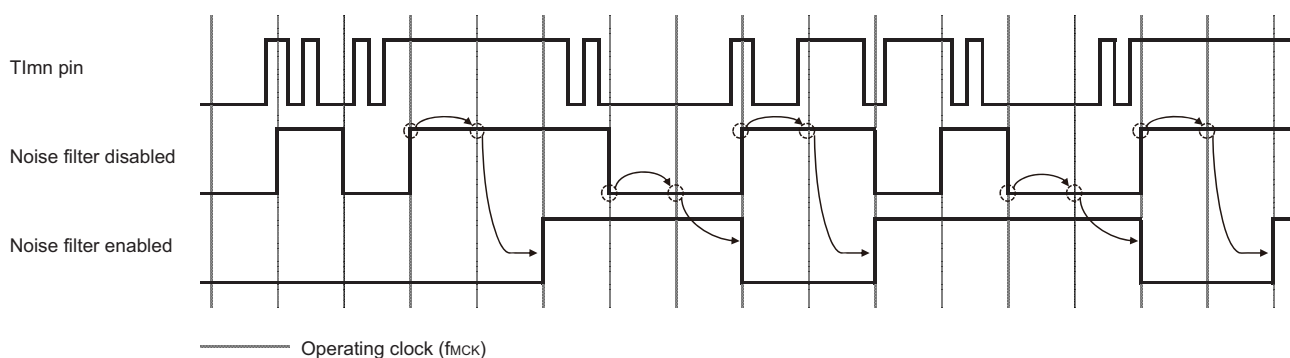
Figure 6-41. Sampling Waveforms through TImn Input Pin with Noise Filter Enabled and Disabled
