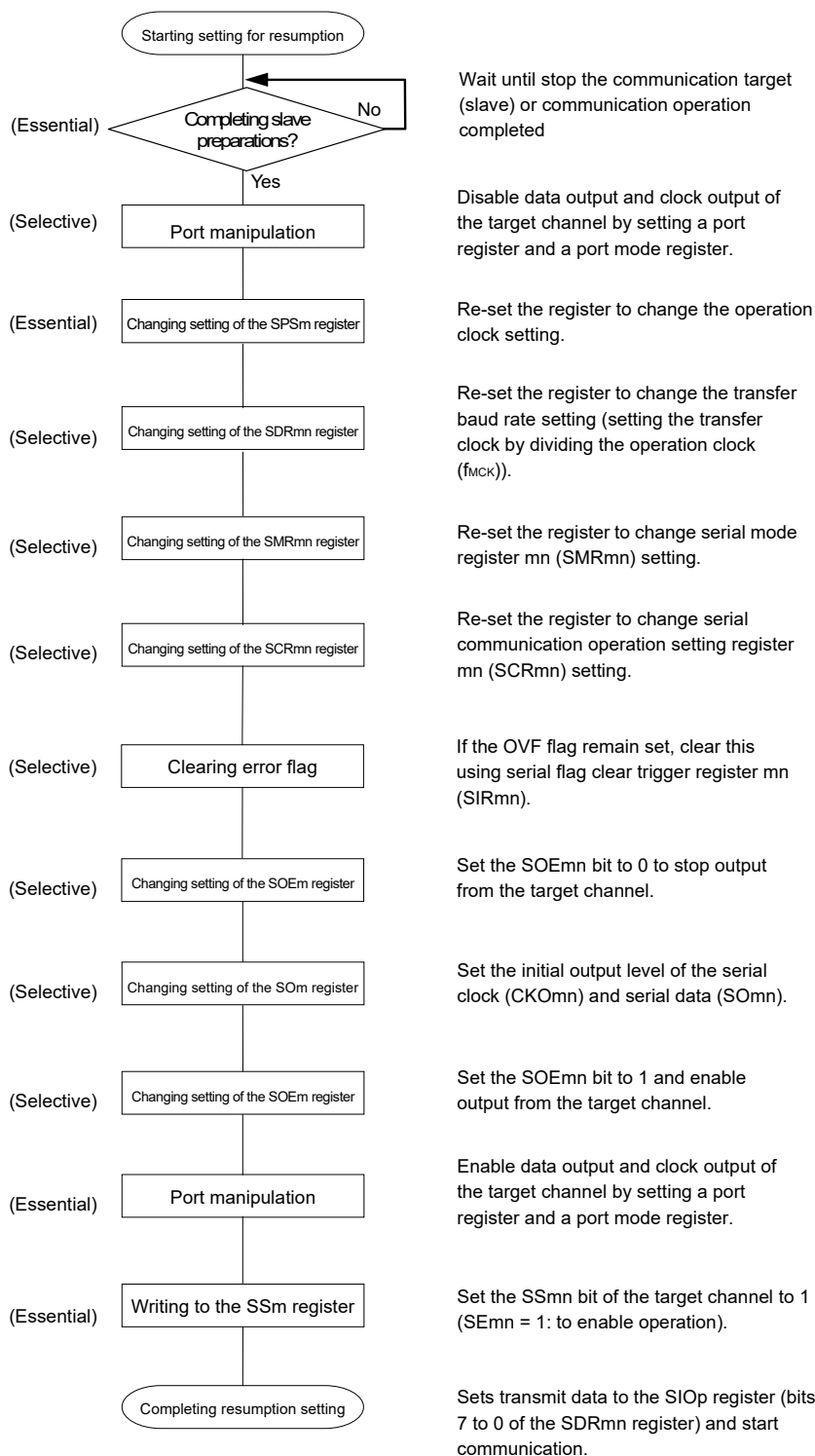
Figure 14-44. Procedure for Resuming Master Transmission/Reception
