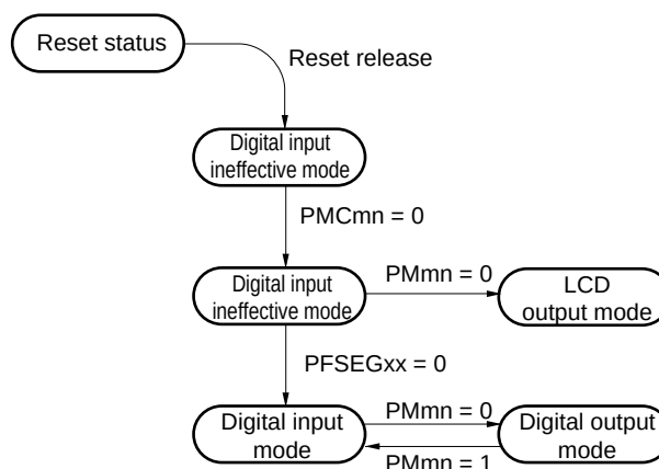
Figure 4-40. SEGxx/Port Pin Function Status Transition Diagram
