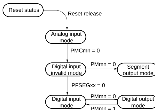
Figure 4-41. ANLxx/SEGxx/Port Pin Function Status Transition Diagram
