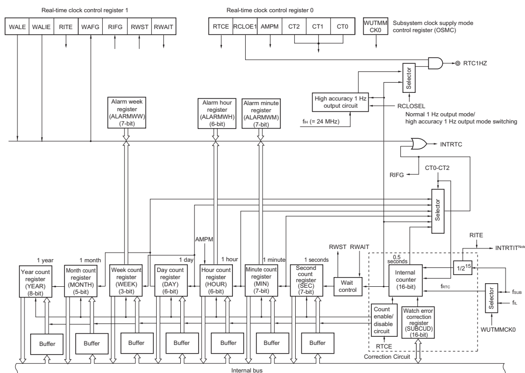
Figure 7-1. Real-time Clock 2 Diagram
