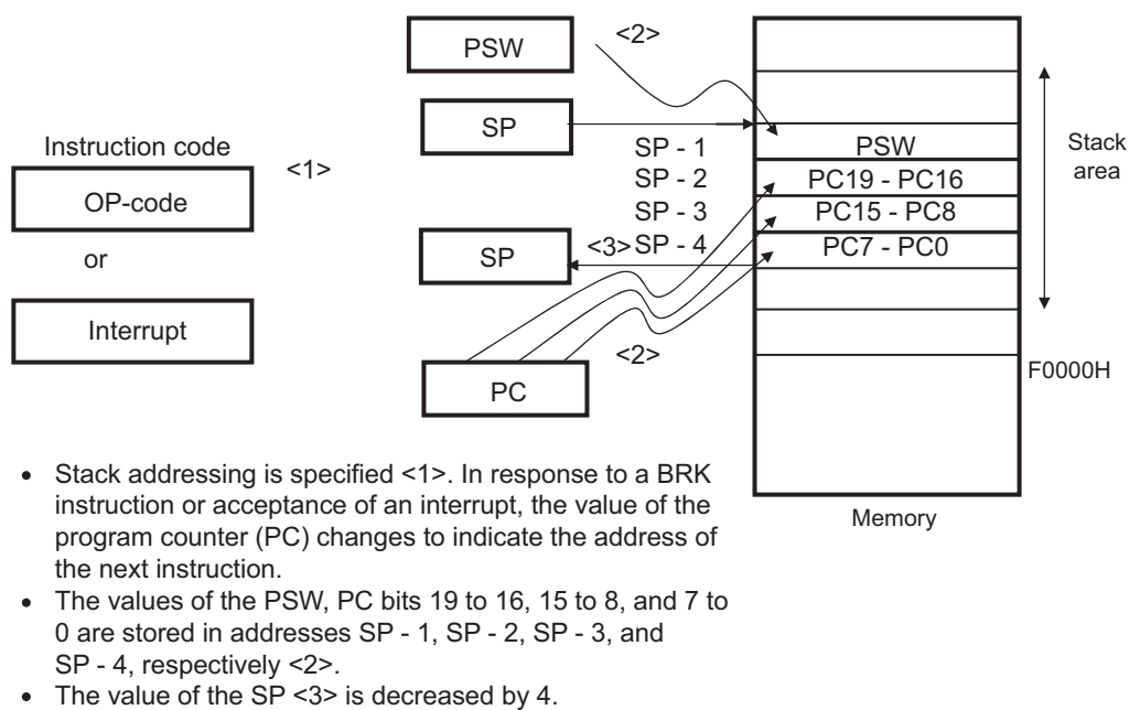
Figure 3-36. Example of Interrupt, BRK
