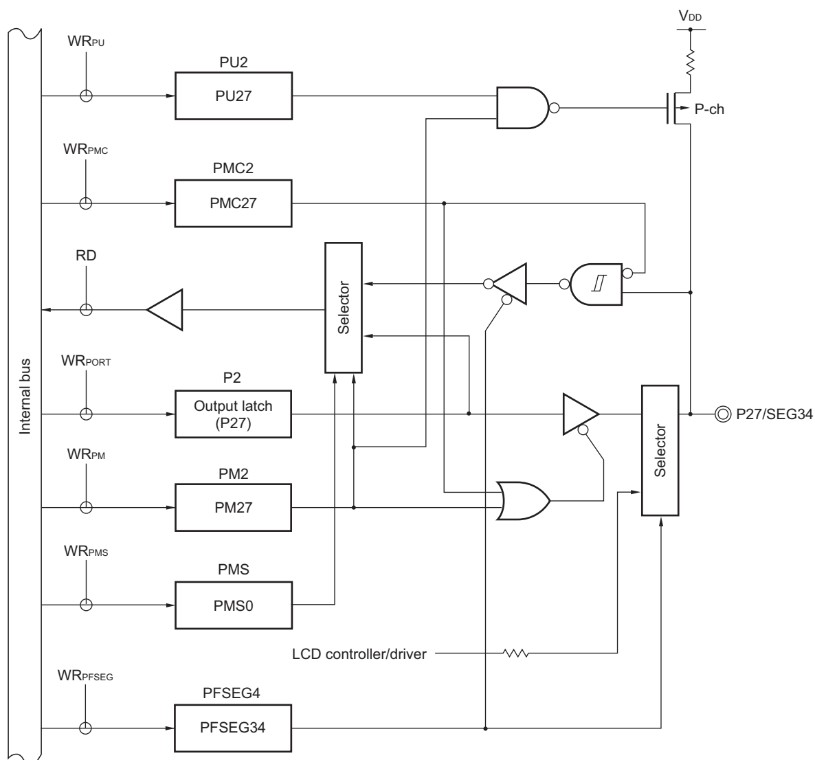
Figure 4-11. Block Diagram of P27
