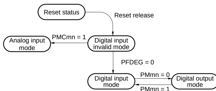
Figure 4-44. IVREF0/SEG26/Port Pin Function Status Transition Diagram
