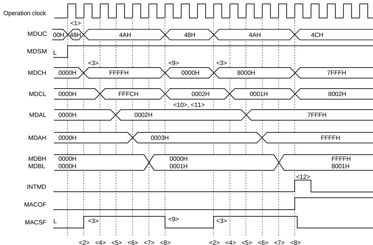
Figure 17-9. Timing Diagram of Multiply-Accumulation (Signed) Operation (2 \times 3 + (-4) = 2 \rightarrow 32767 \times (-1) + (-2147483647) = -2147516414 \text{ (overflow occurs.)})
