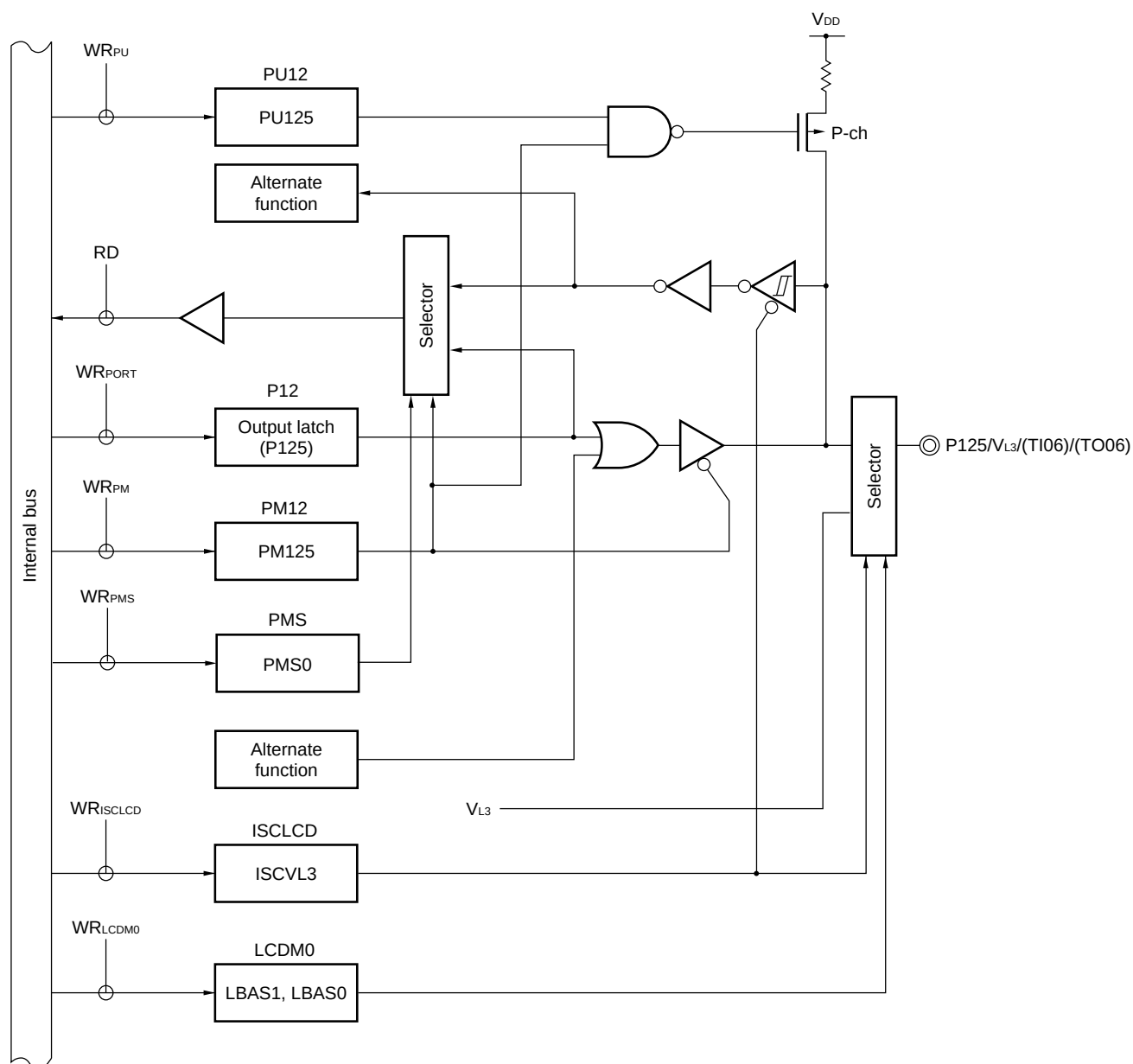
Figure 4-26. Block Diagram of P125
