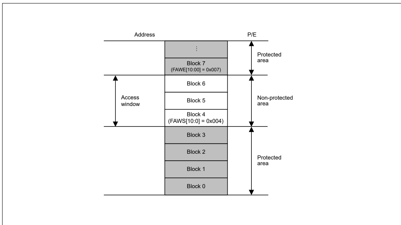
Figure 6.3 Access window overview
