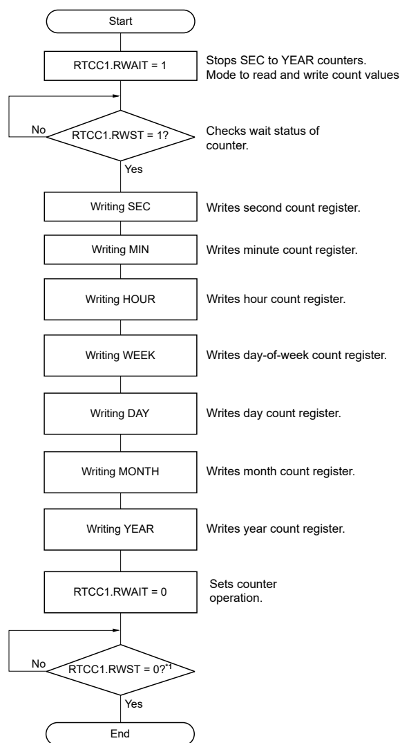
Figure 19.5 Procedure for writing realtime clock
