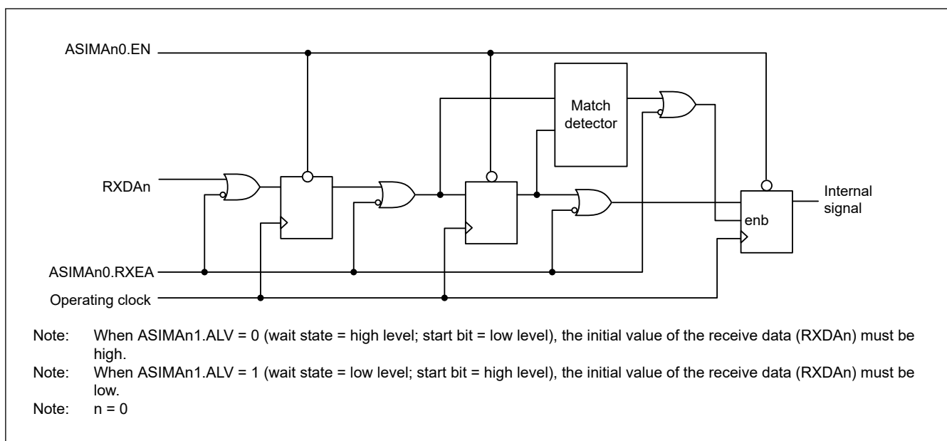
Figure 23.9 Noise filter
