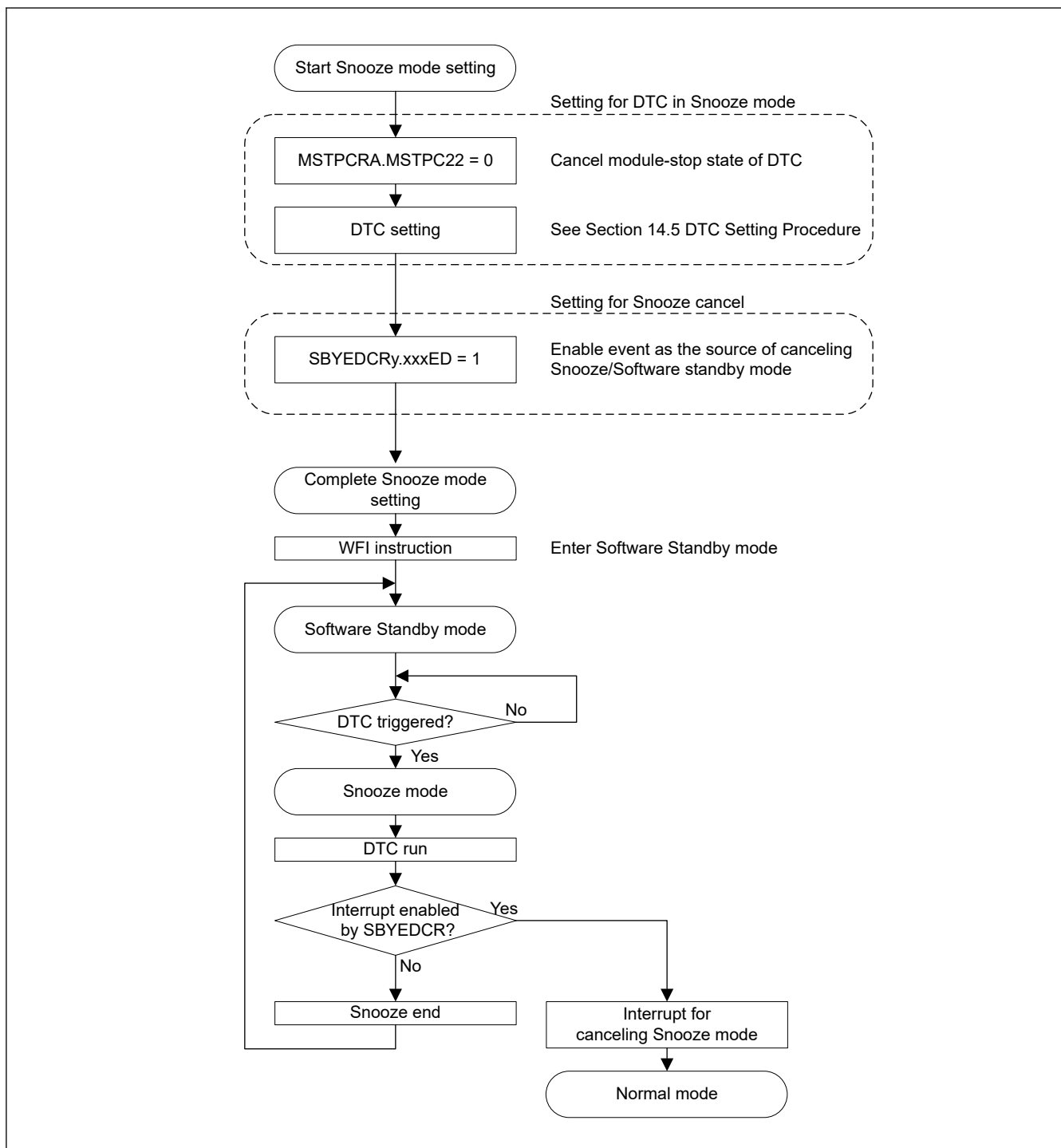
Figure 9.10 Setting example of using DTC in Snooze mode
