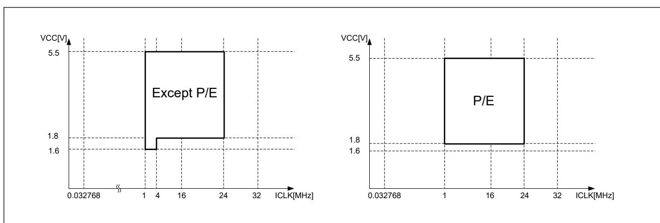
Figure 9.3 Operating voltages and frequencies in Middle-speed mode
