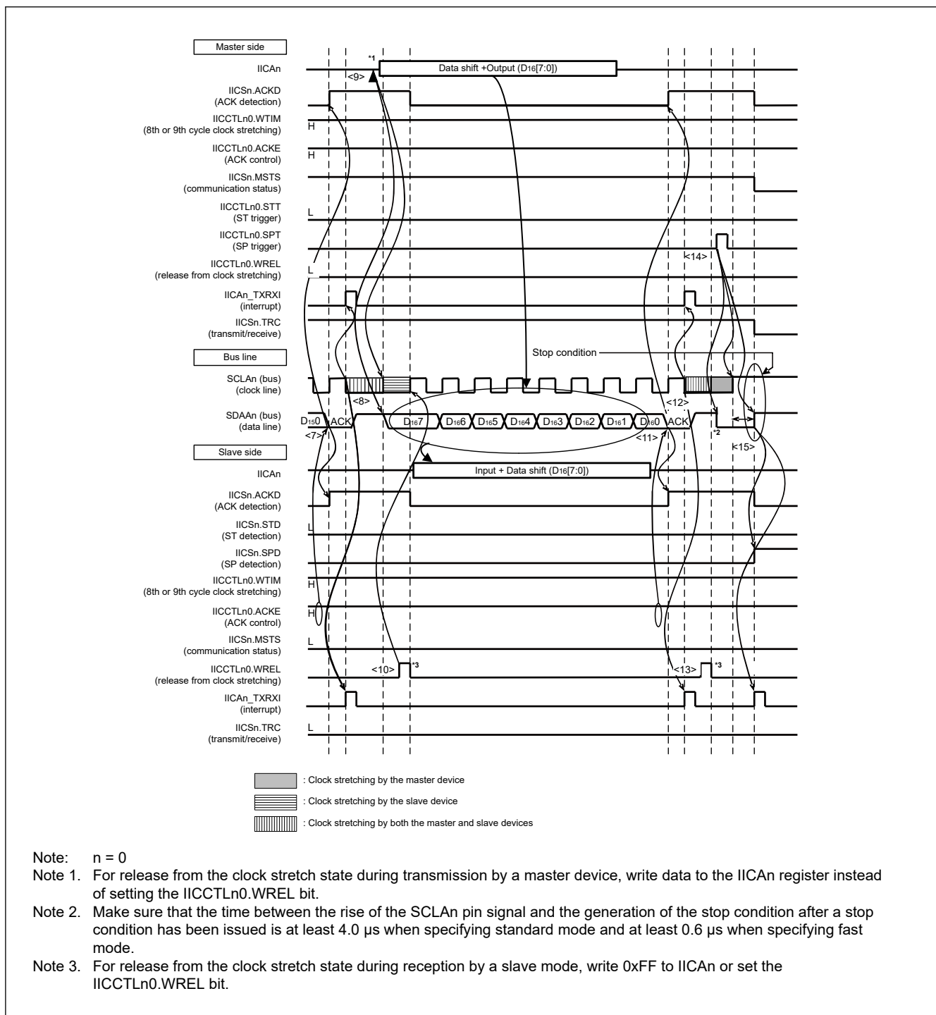
Figure 22.65 Example of master device to slave device communications (when the master device and the slave device insert clock stretching on the 9th cycle) (3/4)
