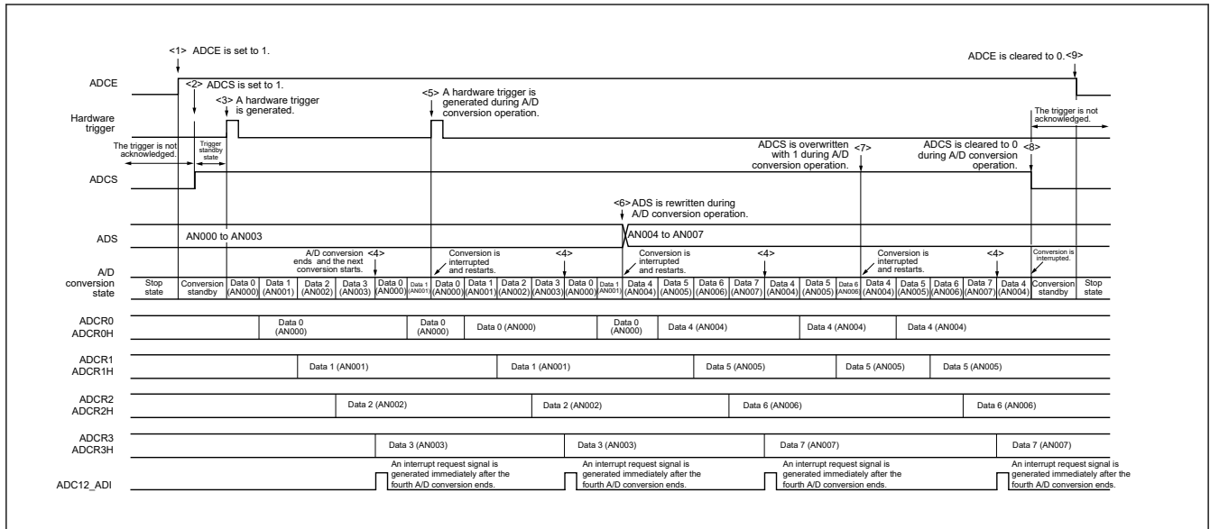
Figure 25.18 Example of hardware trigger no-wait mode (scan mode, sequential conversion mode) operation timing
