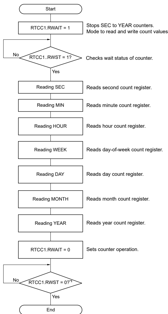
Figure 19.4 Procedure for reading realtime clock
