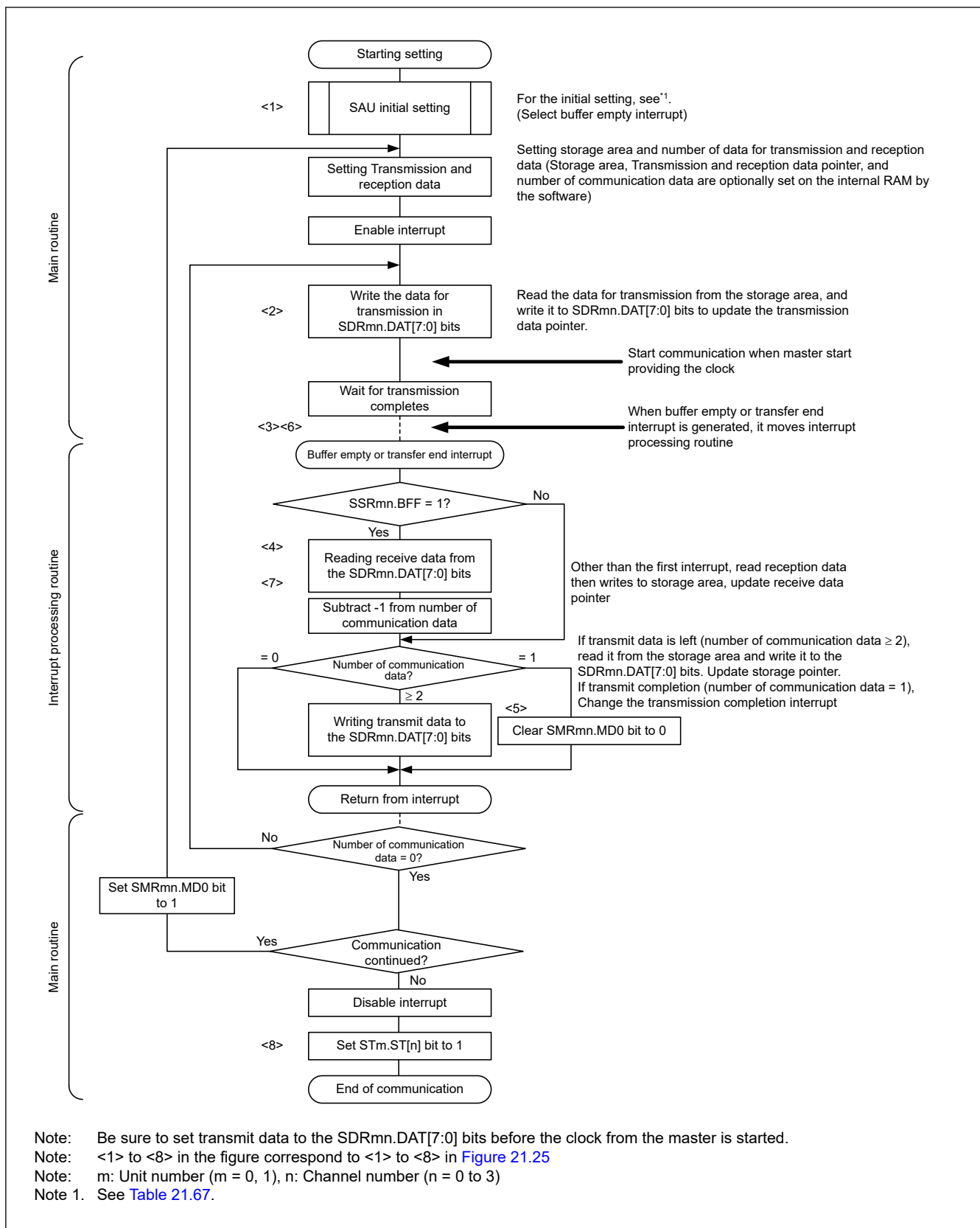
Figure 21.26 Flowchart of slave transmission and reception (in continuous transmission and reception mode)
