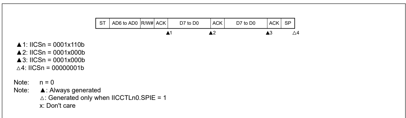
Figure 22.29 Slave device operation slave address data reception (IICCTL00.WTIM = 0)
