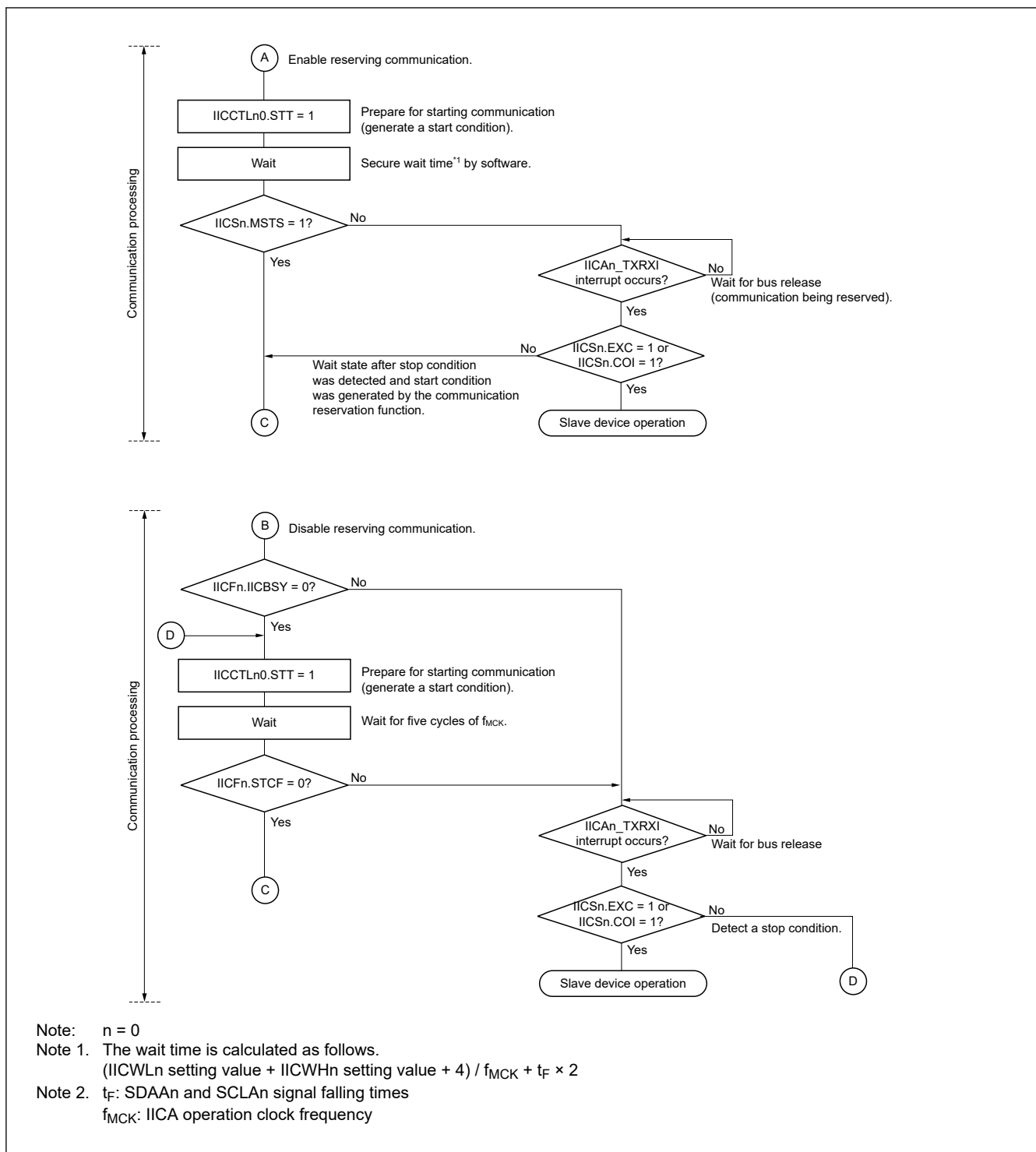
Figure 22.18 Master device operation in multi-master system (2/3)
