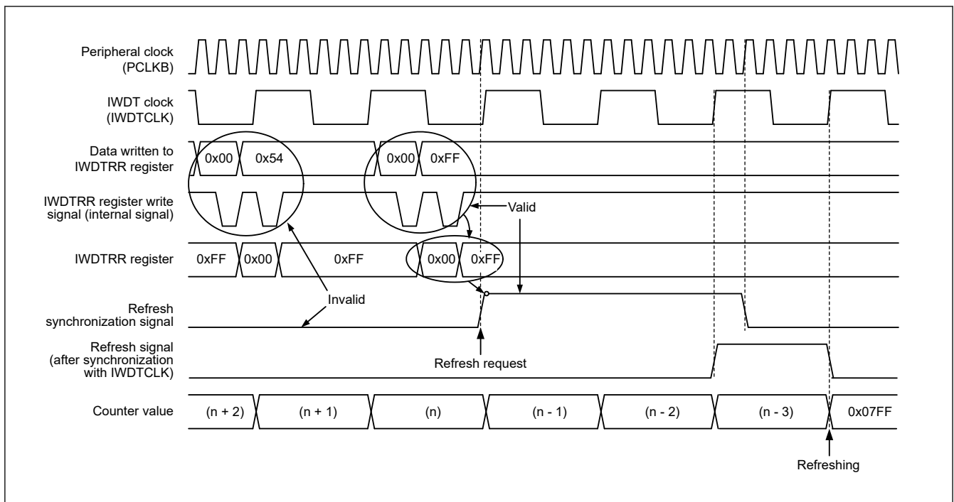
Figure 20.4 IWDT refresh operation waveforms when OFS0.IWDTCKS[3:0] = 0000b , OFS0.IWDTTOS[1:0] = 11b
