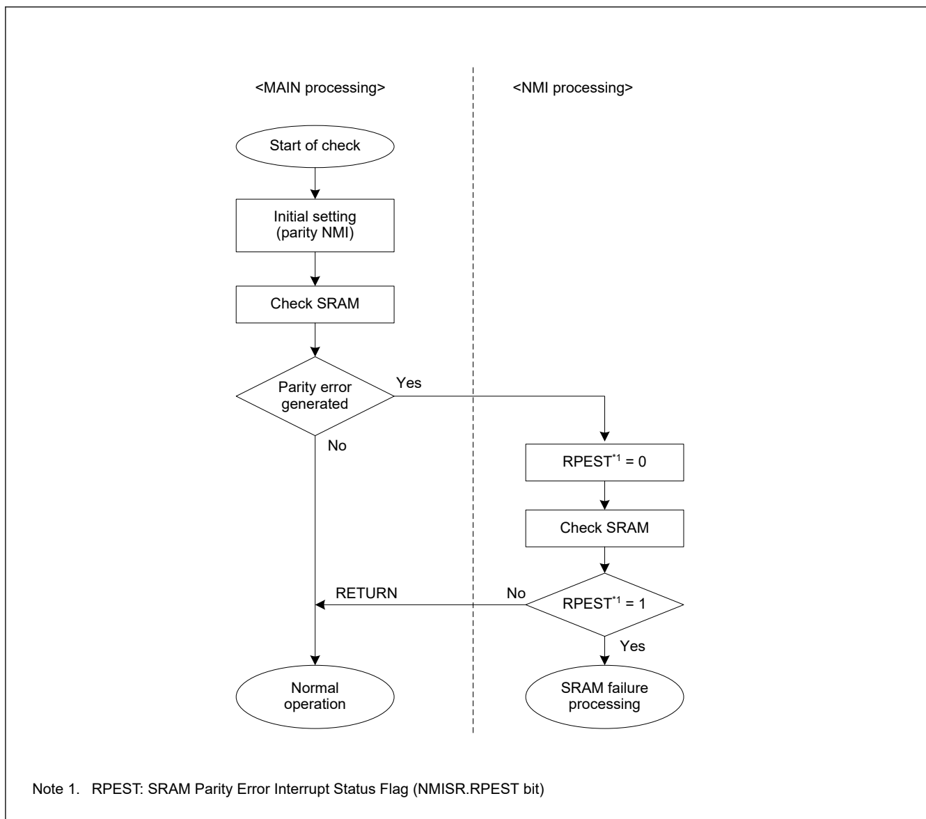
Figure 27.2 Flow of SRAM parity check when SRAM parity interrupt is enabled
