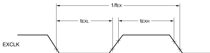
Figure 31.6 External system clock timing
