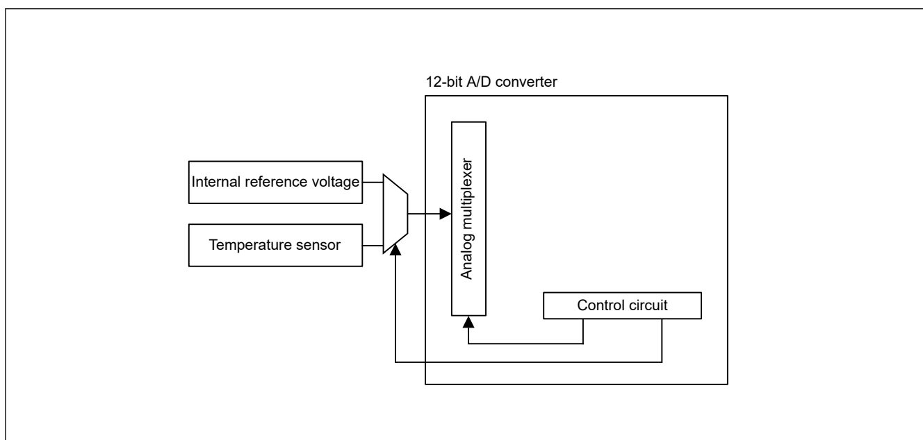
Figure 26.1 TSN block diagram
