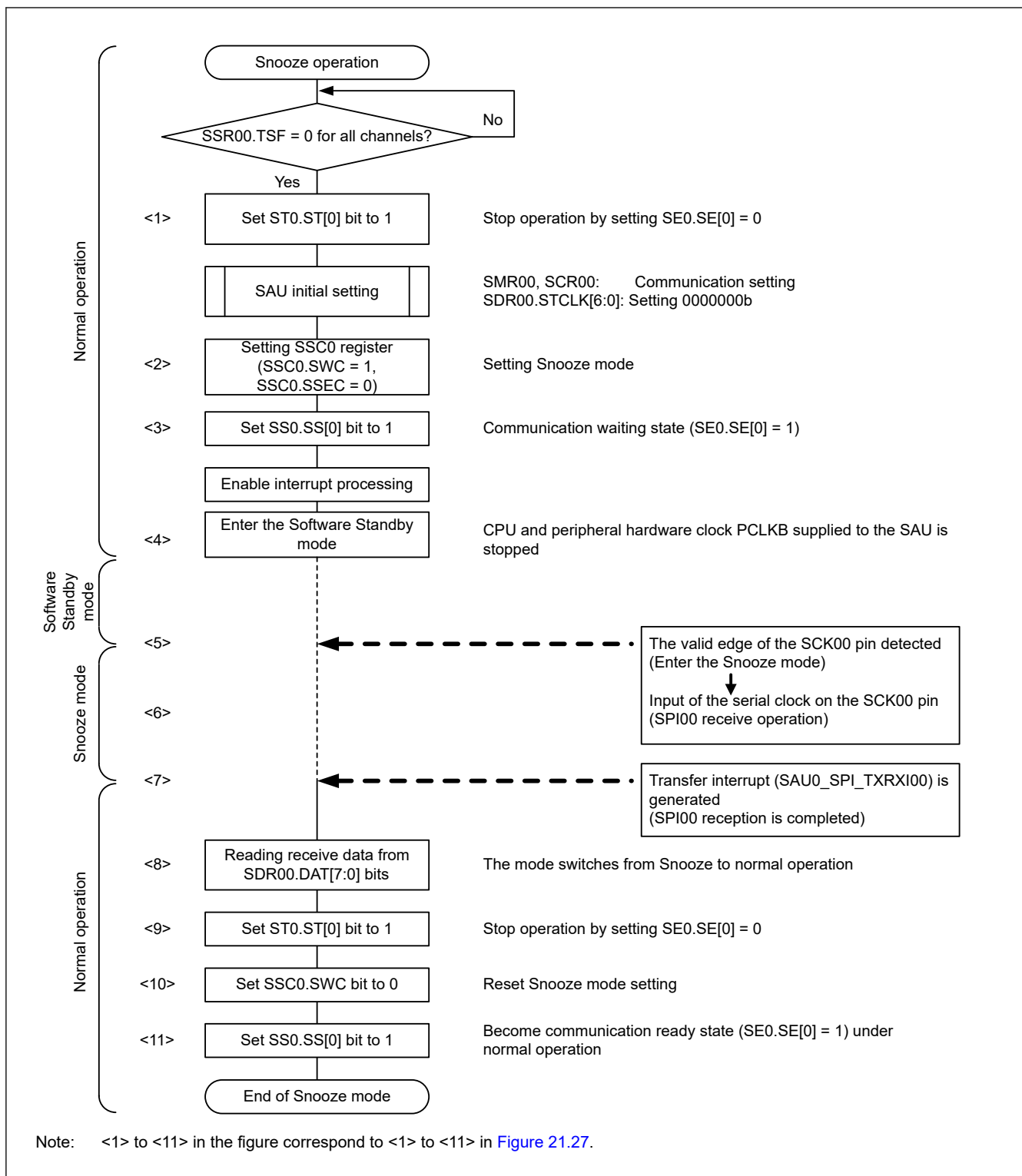
Figure 21.28 Flowchart of Snooze mode operation (on startup)
