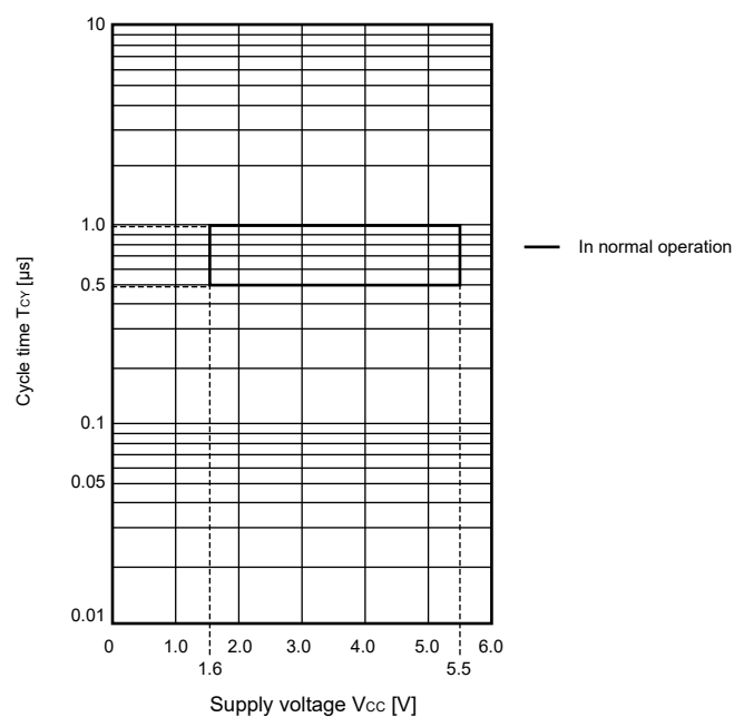
Figure 31.4 T_{cy} vs V_{cc} in low-speed mode
