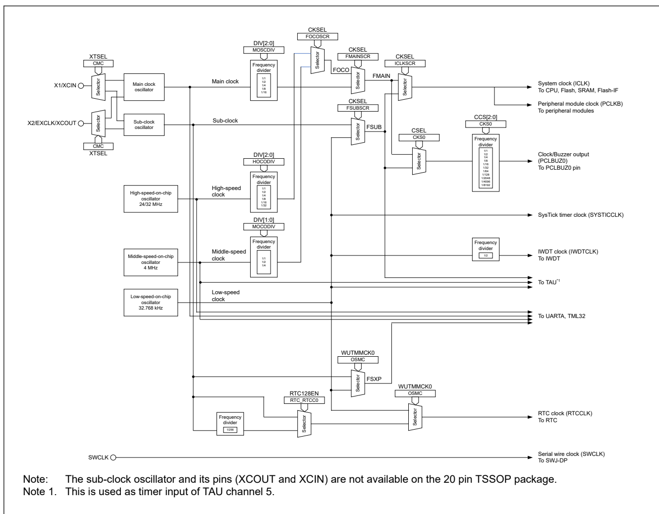
Figure 8.2 Clock generation circuit block diagram (24-, 20-, 16-pin)
