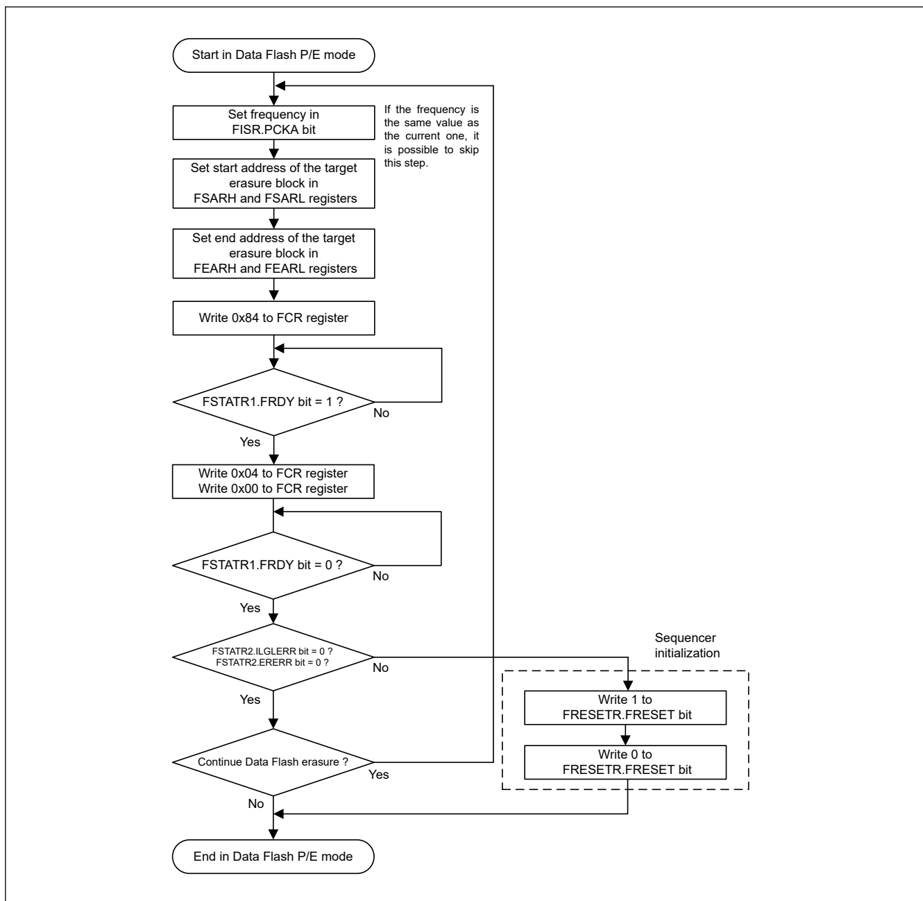
Figure 28.20 Flowchart for the data flash block erase procedure
