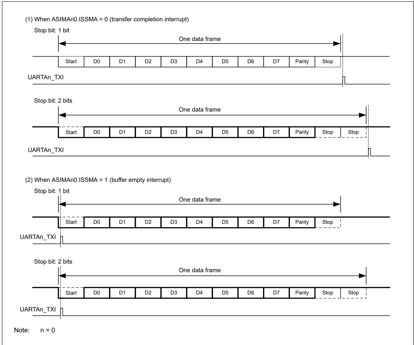
Figure 23.4 Interrupt output timing
