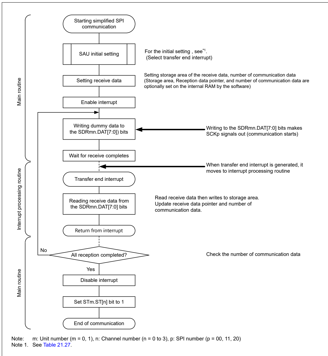
Figure 21.10 Flowchart of master reception (in single reception mode)
