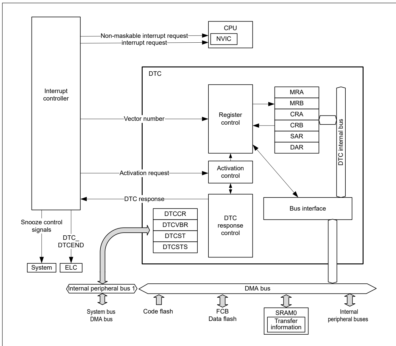
Figure 14.1 DTC block diagram
