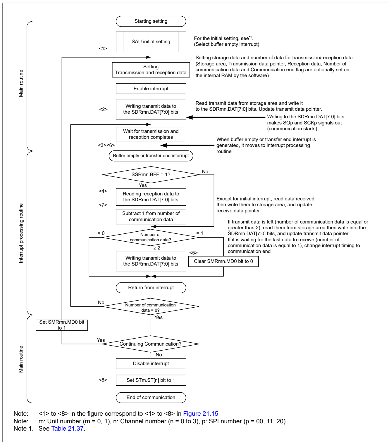
Figure 21.16 Flowchart of master transmission and reception (in continuous transmission and reception mode)
