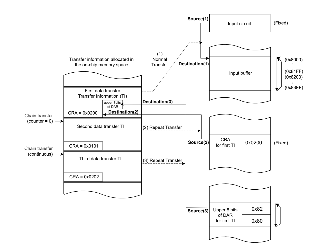
Figure 14.13 Chain transfer when counter = 0
