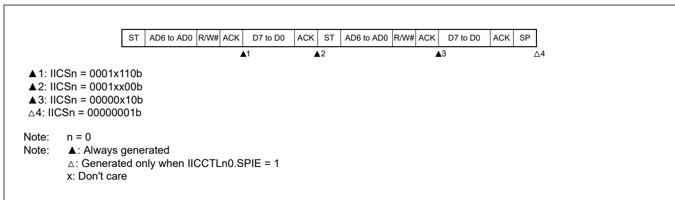
Figure 22.36 Slave device operation after normal access, does not match (IICCTL00.WTIM = 1)
