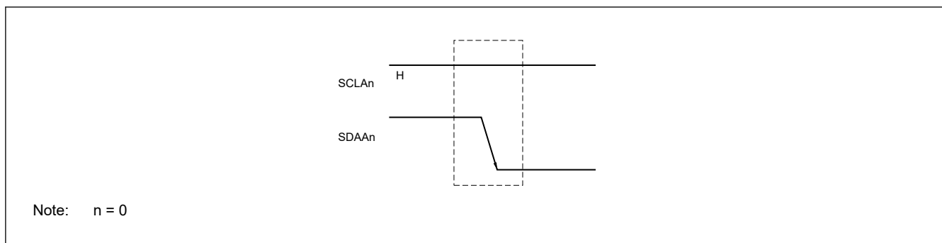
Figure 22.5 Start conditions
