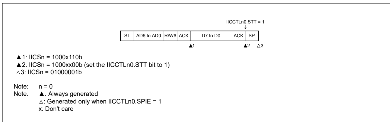
Figure 22.60 Operations when arbitration loss occurs due to a stop condition when attempting to generate a restart condition (IICCTL00.WTIM = 1)
