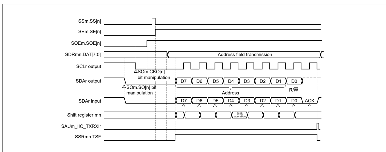
Figure 21.48 Timing of address field transmission
