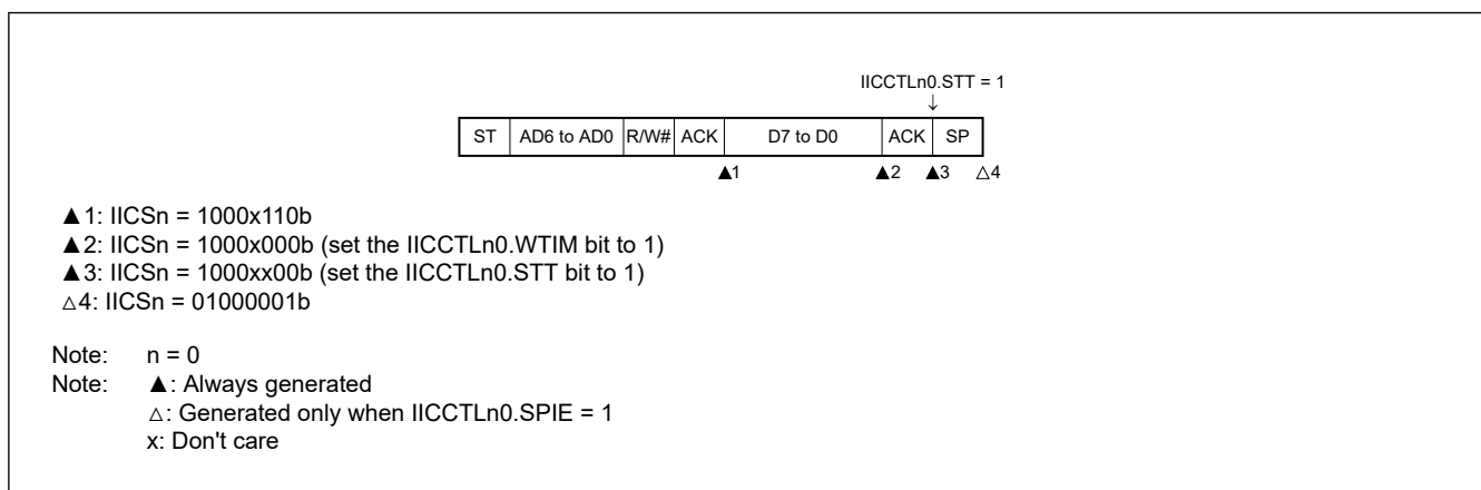
Figure 22.59 Operations when arbitration loss occurs due to a stop condition when attempting to generate a restart condition (IICCTL00.WTIM = 0)
