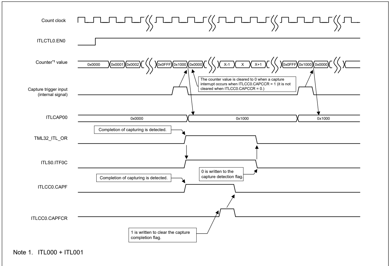
Figure 18.7 Example of capture operation
