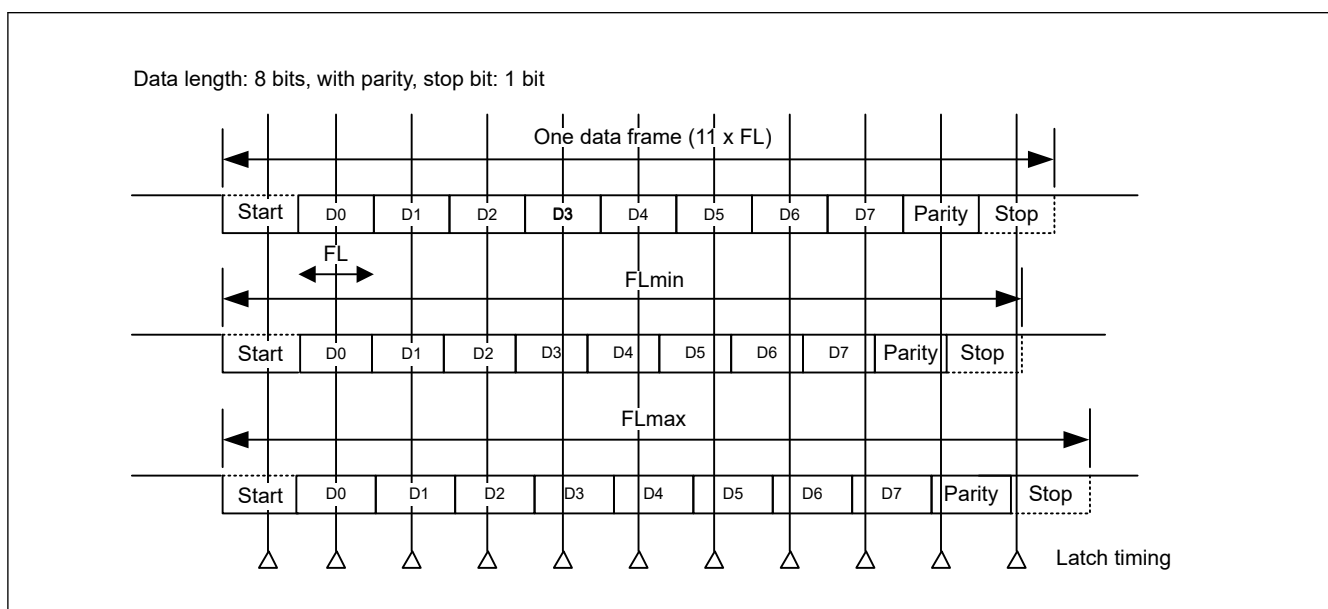
Figure 23.11 Permissible baud rate range during reception
