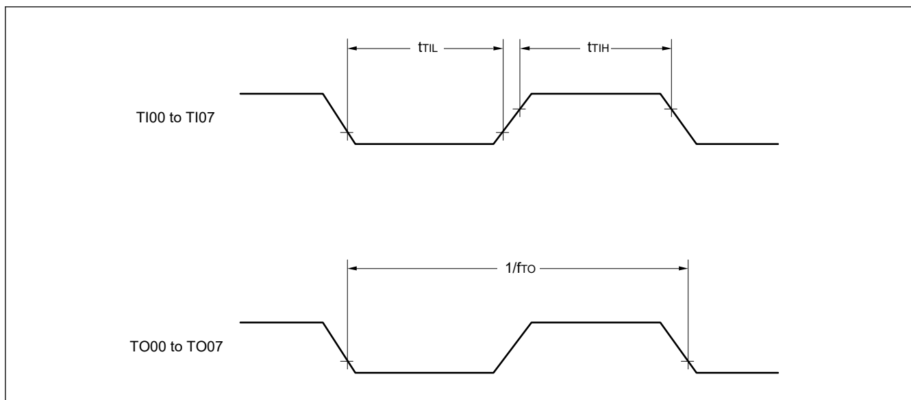
Figure 31.7 TI/TO timing
