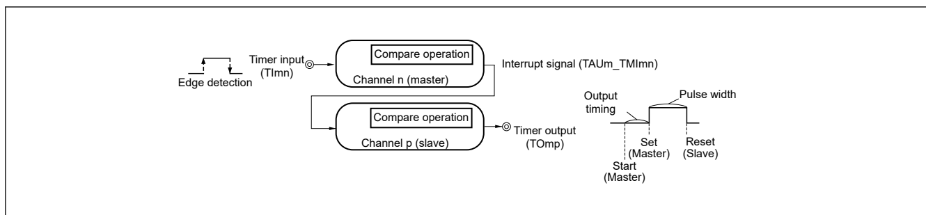
Figure 17.9 Functional image of one-shot pulse output
