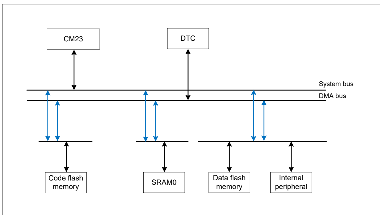
Figure 12.1 Bus configuration
