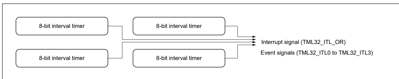
Figure 18.1 Image of four 8-bit interval timer function
