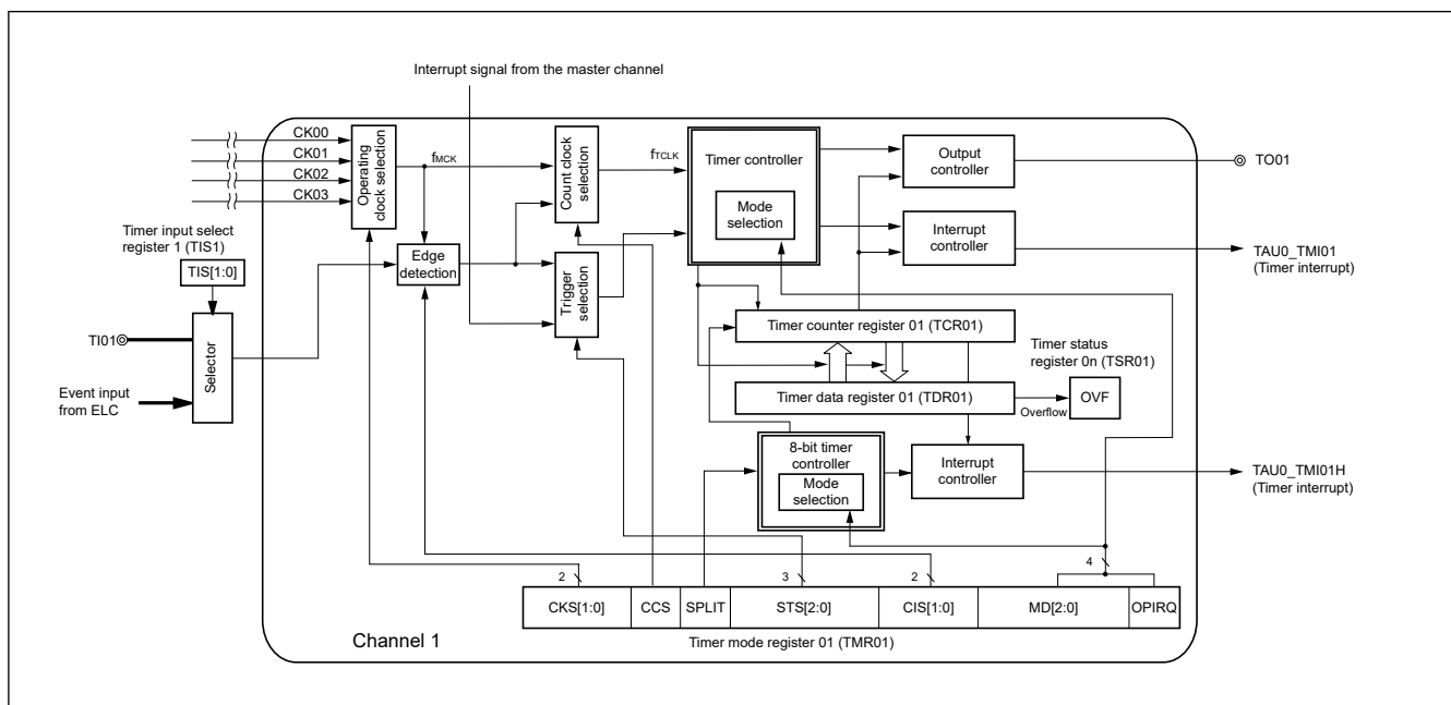
Figure 17.14 Internal block diagram of channel 1 of timer array unit 0
