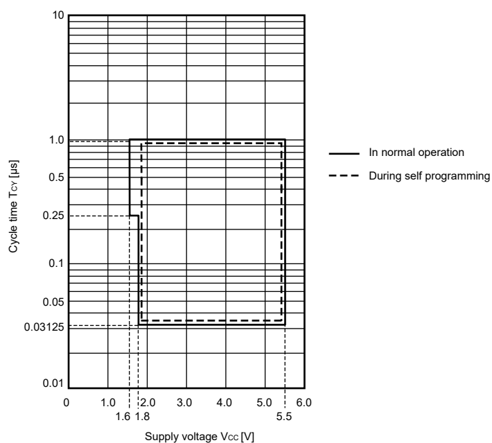
Figure 31.2 T_{cy} vs V_{cc} in high-speed mode
