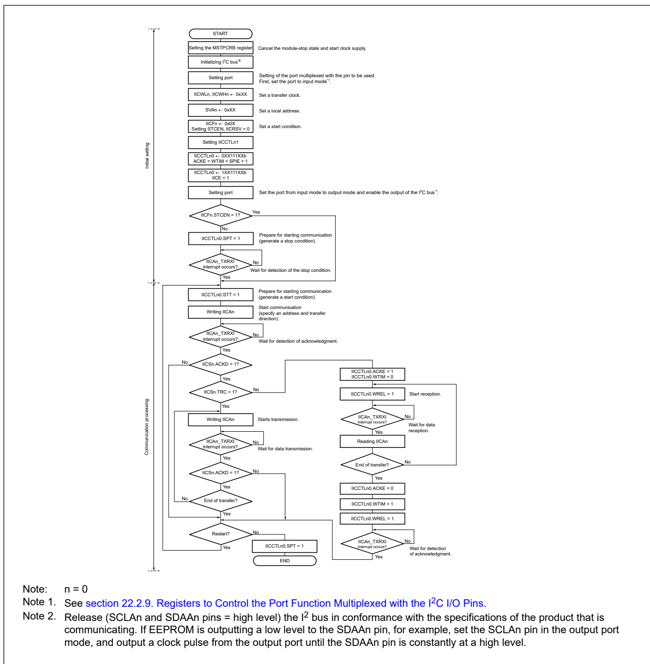
Figure 22.16 Master device operation in single-master system
