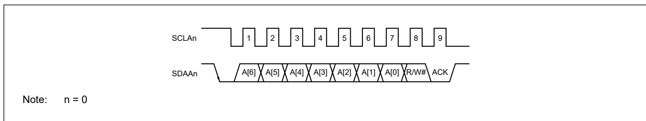
Figure 22.8 ACK
