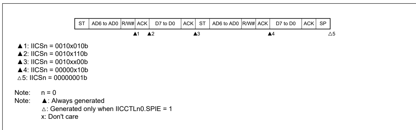
Figure 22.44 Slave device operation after code access, does not match (IICCTL00.WTIM = 1)
