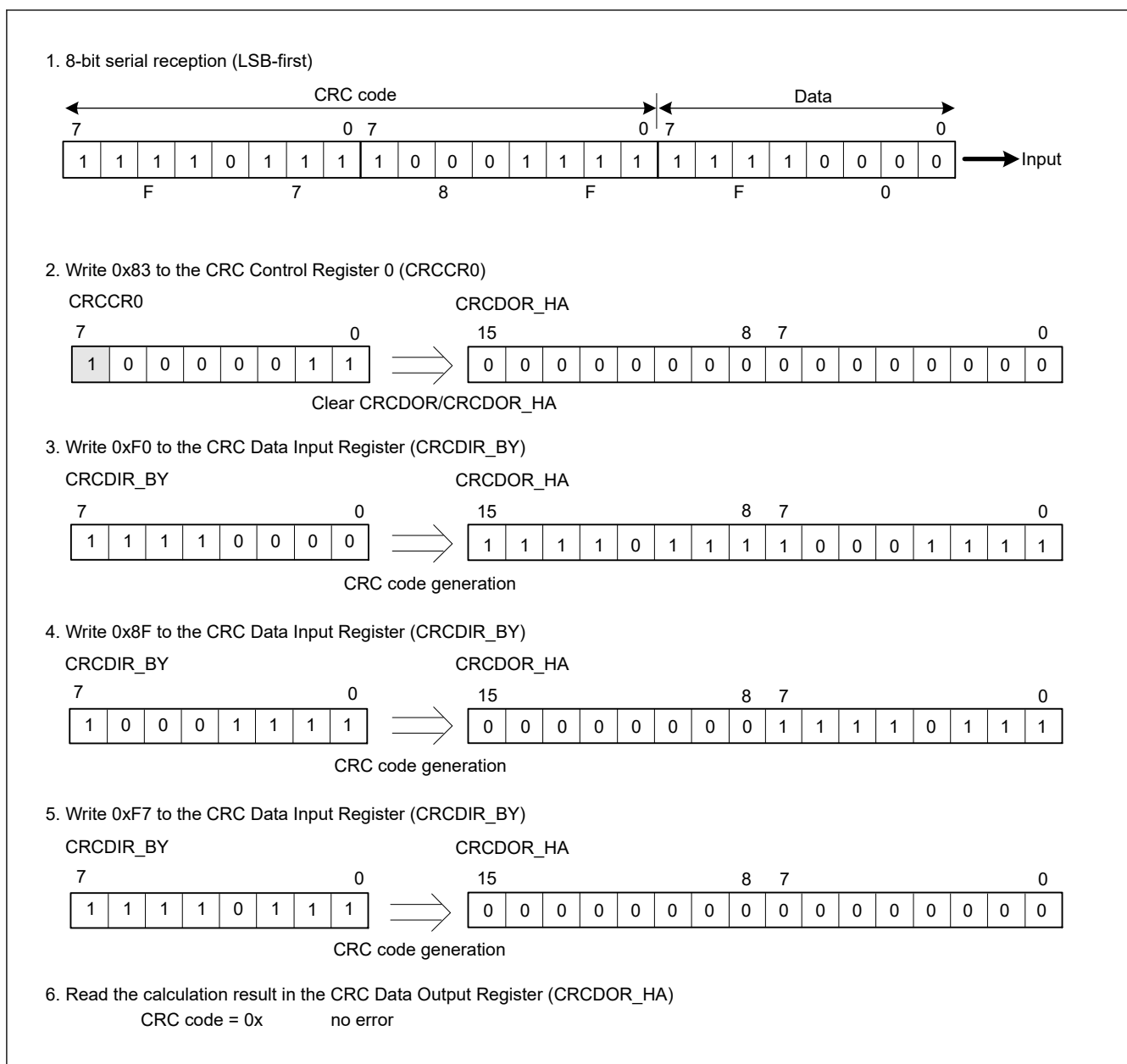
Figure 24.3 LSB-first data reception
