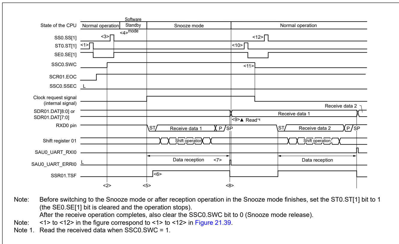
Figure 21.38 Timing of Snooze mode operation (SCR01.EOC = 1, SSC0.SSEC = 0)
