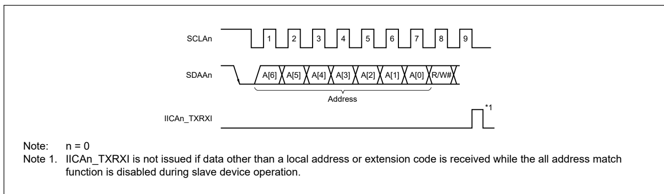
Figure 22.6 Addresses
