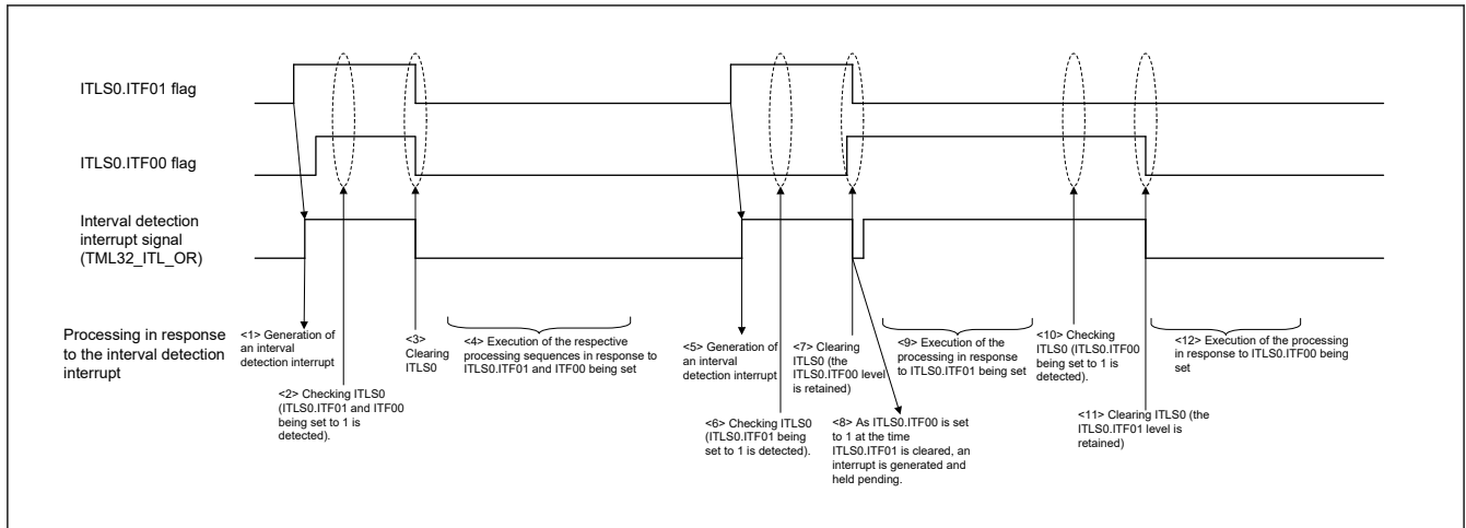
Figure 18.8 Example of clearing the detected flags
