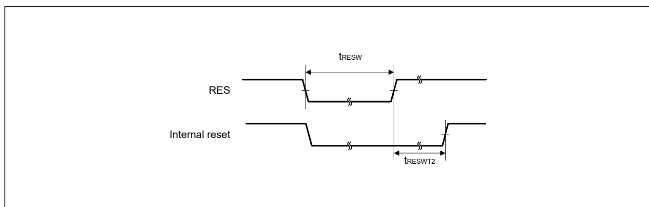
Figure 31.10 Reset input timing (1)
