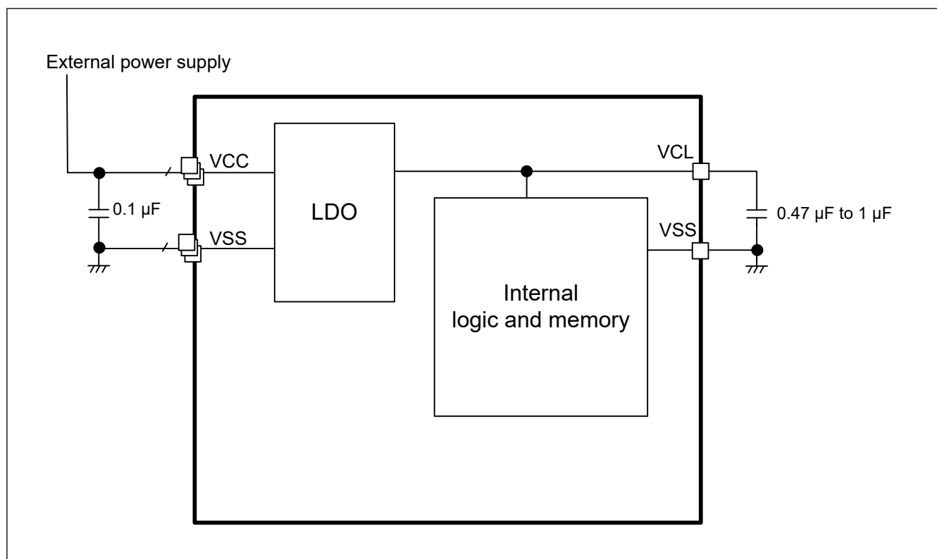
Figure 30.1 LDO settings
