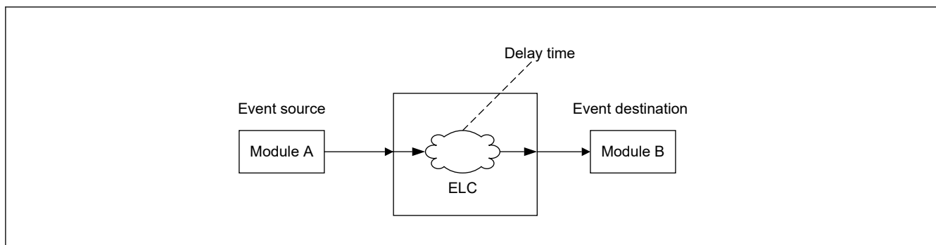
Figure 15.2 ELC delay time
