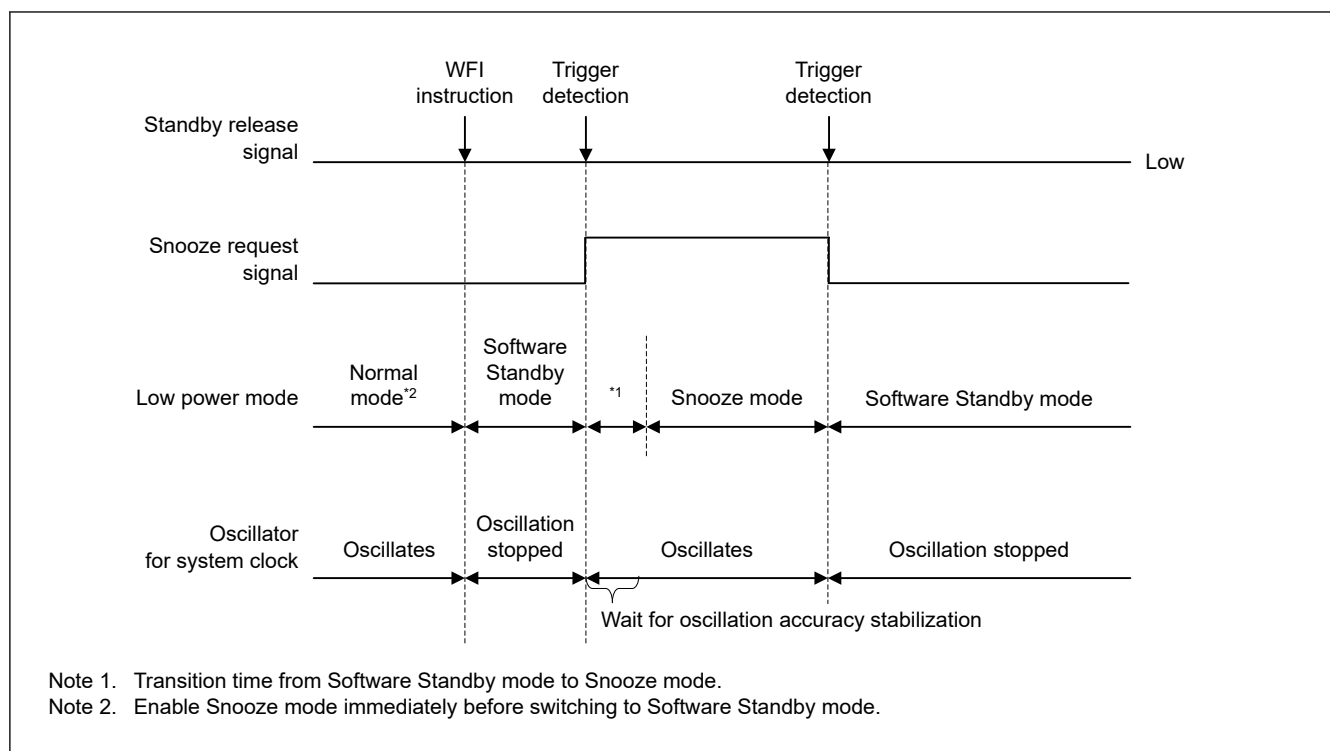
Figure 9.9 Canceling of Snooze mode when an interrupt request signal is not generated
