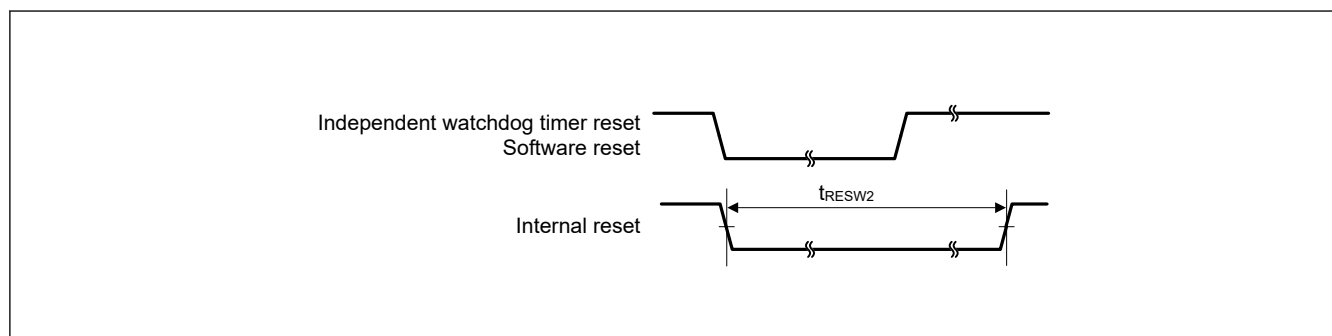
Figure 31.11 Reset input timing (2)
