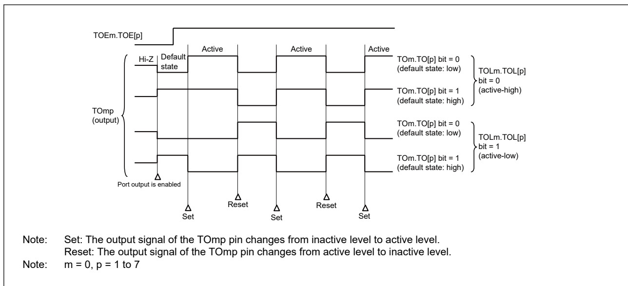
Figure 17.30 TO0p pin output states with PWM output ( \text{TOM0.TOM}[p] = 1 )
