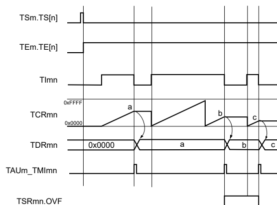
Figure 17.46 Example of basic timing during operation for input signal high- or low-level width measurement
