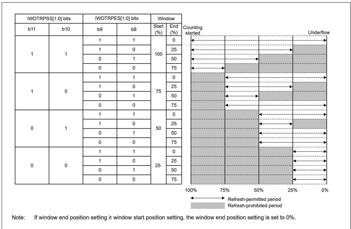
Figure 20.2 IWDTRPSS[1:0] and IWDTRPES[1:0] bit settings and refresh-permitted period
