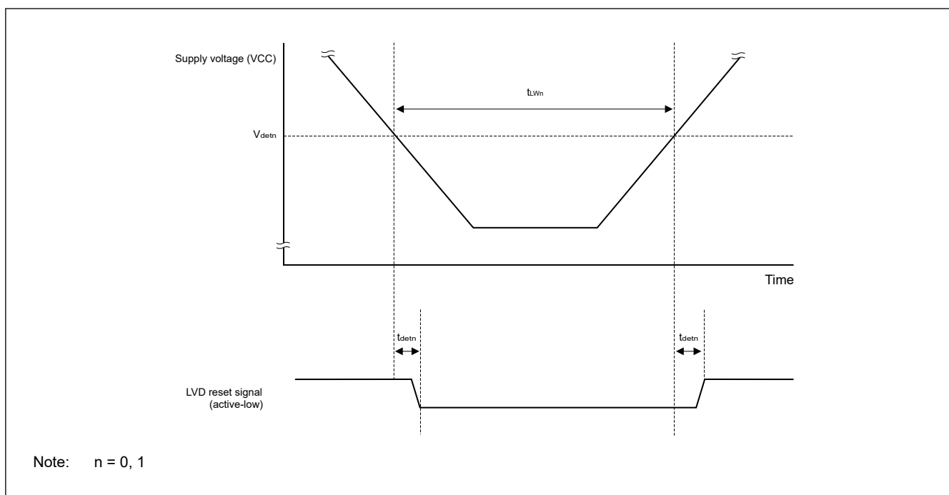
Figure 31.35 Voltage detection circuit timing
