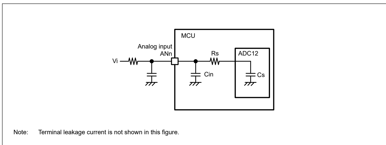
Figure 31.32 Equivalent circuit for analog input
