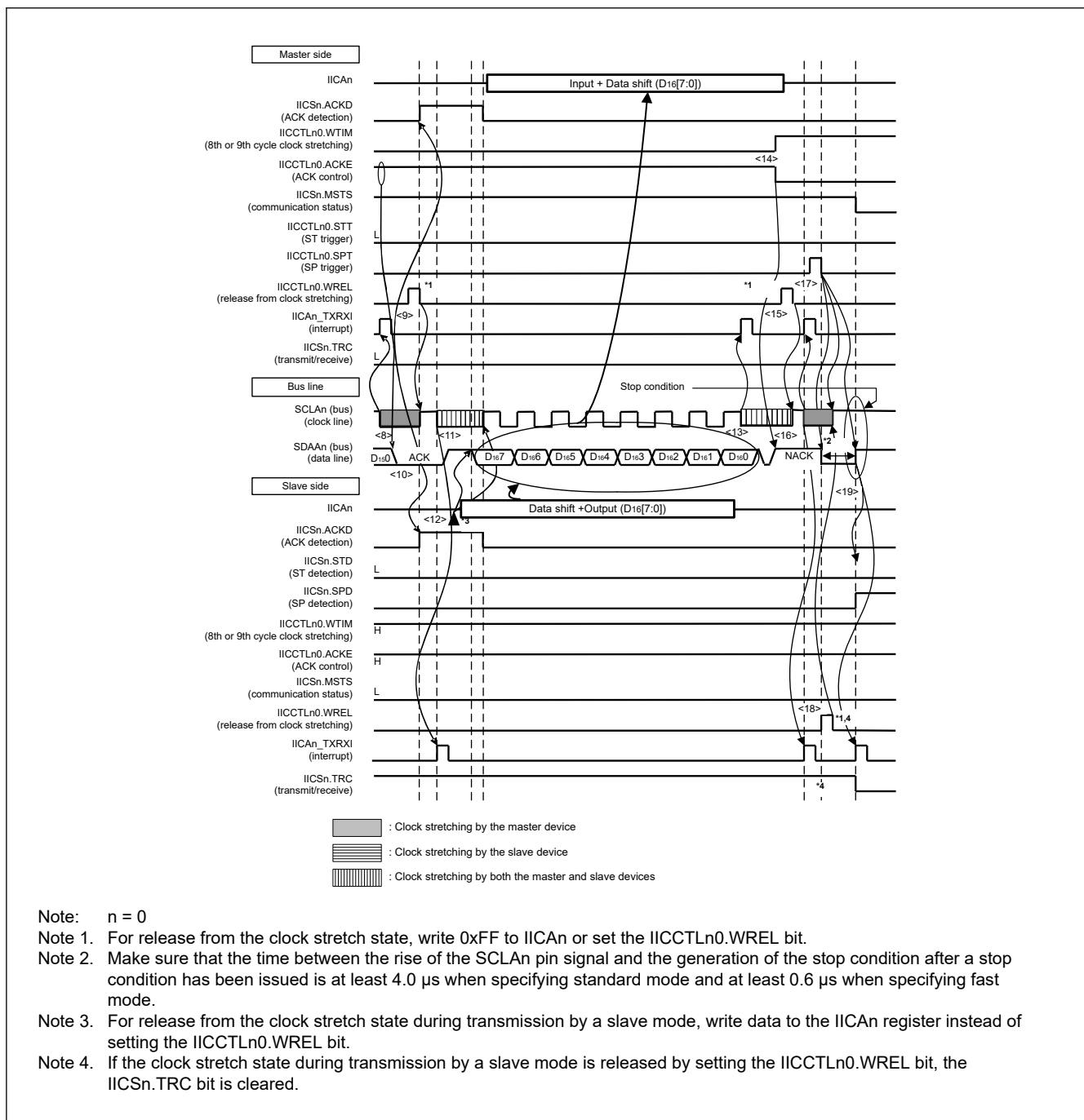
Figure 22.69 Example of slave device to master device communications (8th cycle clock stretching is selected for the master device and 9th cycle clock stretching is selected for the slave device) (3/3)
