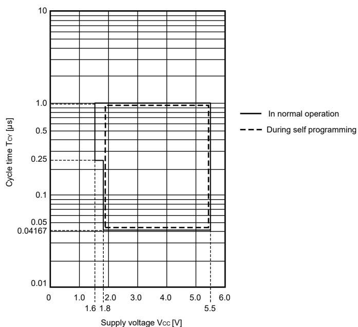
Figure 31.3 T_{cy} vs V_{cc} in middle-speed mode
