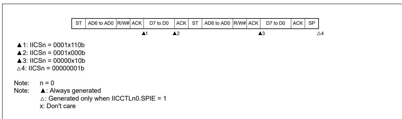
Figure 22.35 Slave device operation after normal access, does not match (IICCTL00.WTIM = 0)
