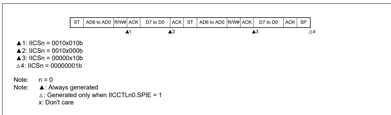
Figure 22.43 Slave device operation after code access, does not match (IICCTL00.WTIM = 0)
