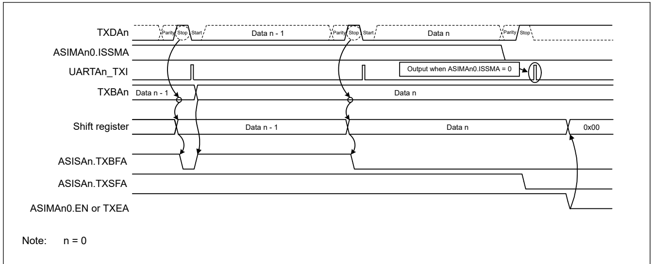
Figure 23.6 Timing when continuous transmission is completed
