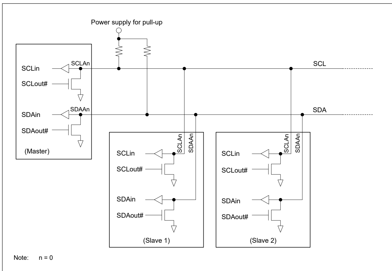
Figure 22.2 Example of the serial bus configuration using the I 2 C bus
