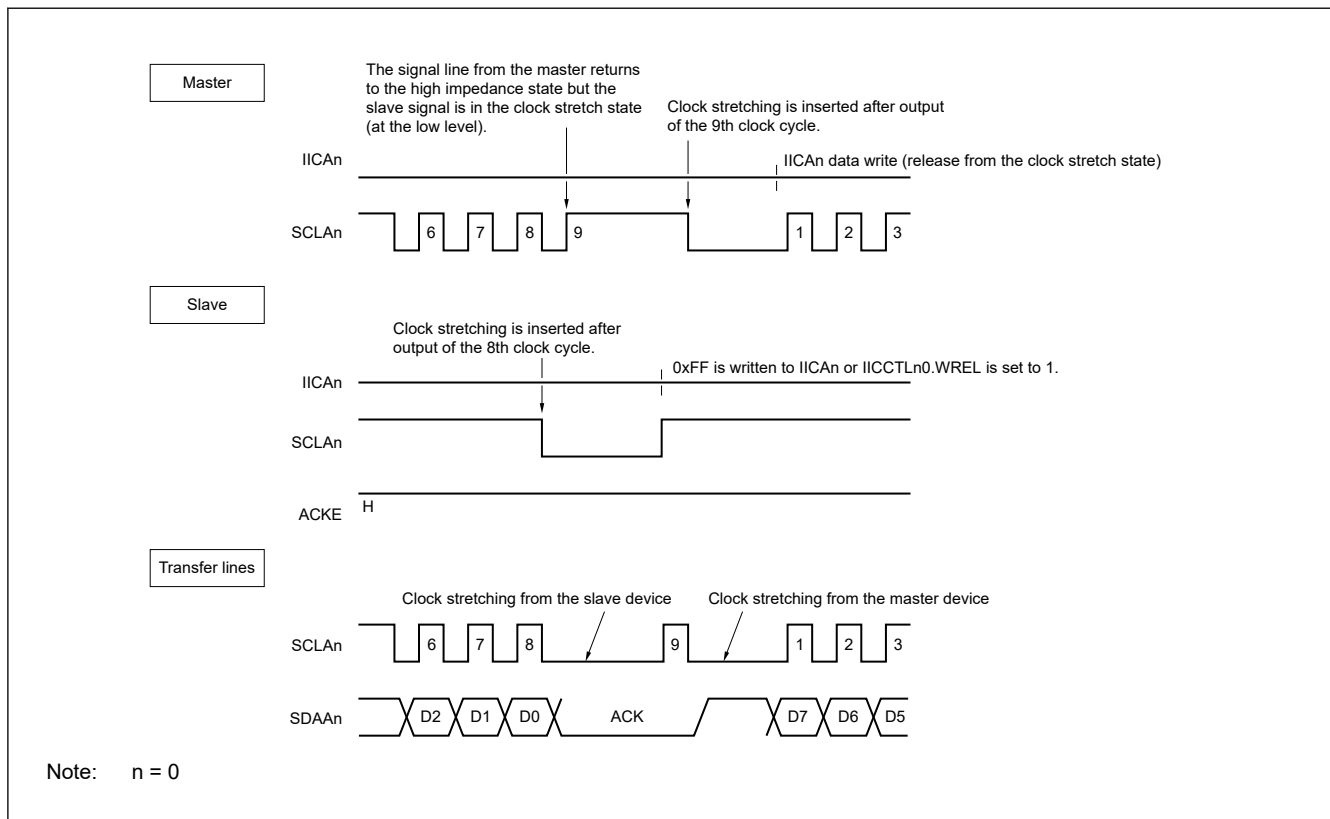
Figure 22.10 Clock stretching (1/2)
