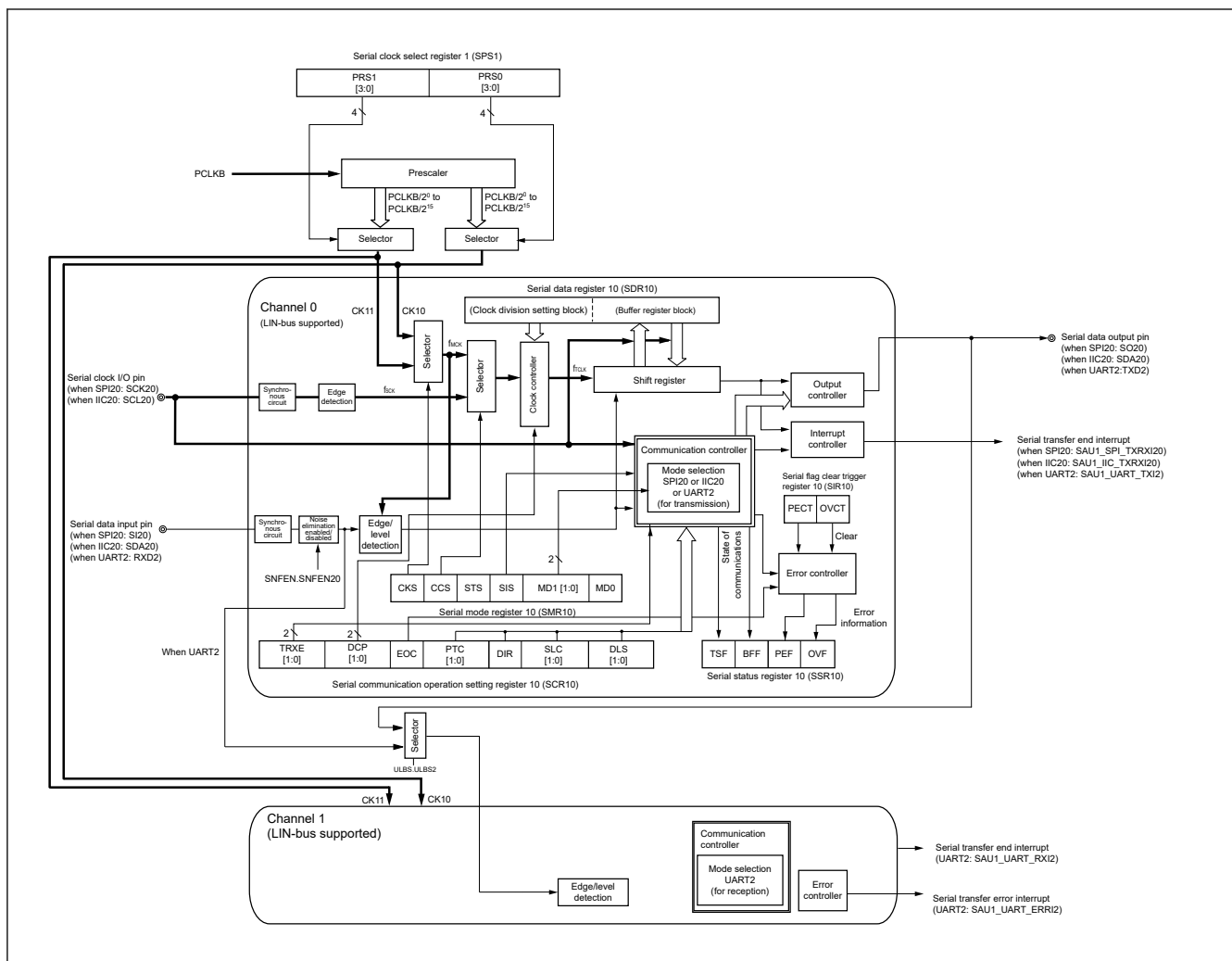
Figure 21.2 Block diagram of serial array unit 1
