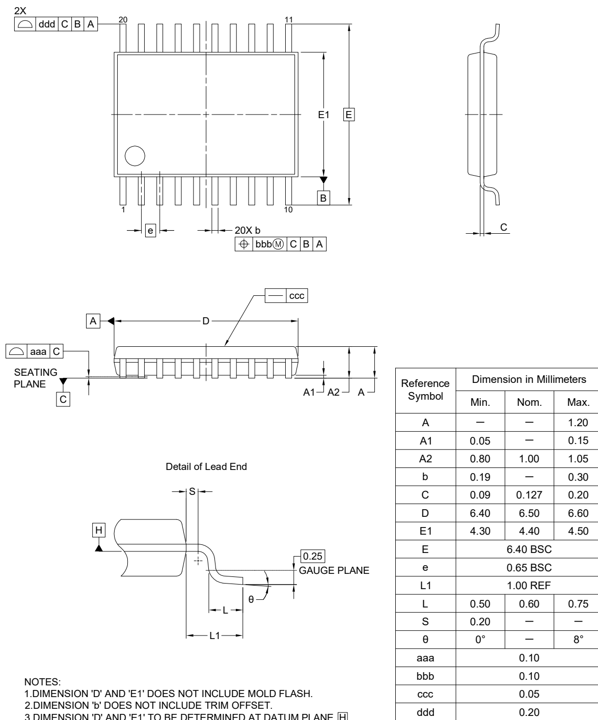
Figure A2.5 TSSOP 20-pin
