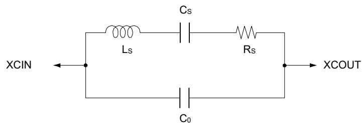
Figure 8.7 Equivalent circuit for the 32.768-kHz crystal resonator
