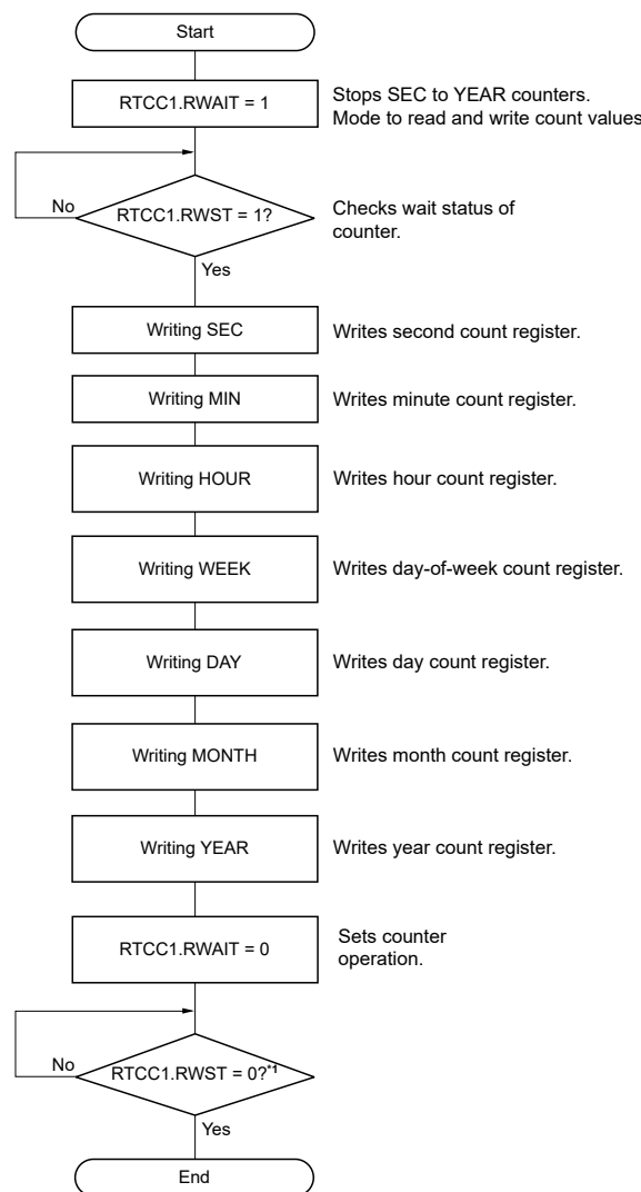
Figure 19.5 Procedure for writing realtime clock
