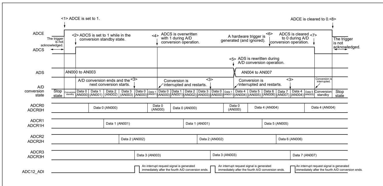
Figure 25.10 Example of software trigger no-wait mode (scan mode, sequential conversion mode)
