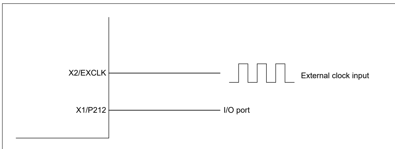
Figure 8.5 Equivalent circuit for external clock
