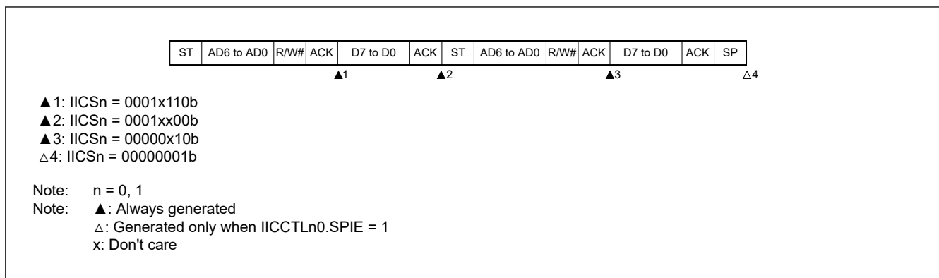
Figure 22.36 Slave device operation after normal access, does not matches (IICCTLn0.WTIM = 1)
