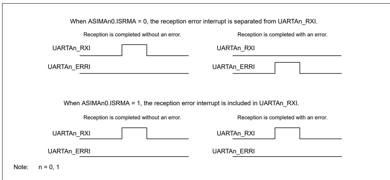
Figure 23.8 Various interrupt output waveforms depending on ASIMAn0.ISRMA setting
