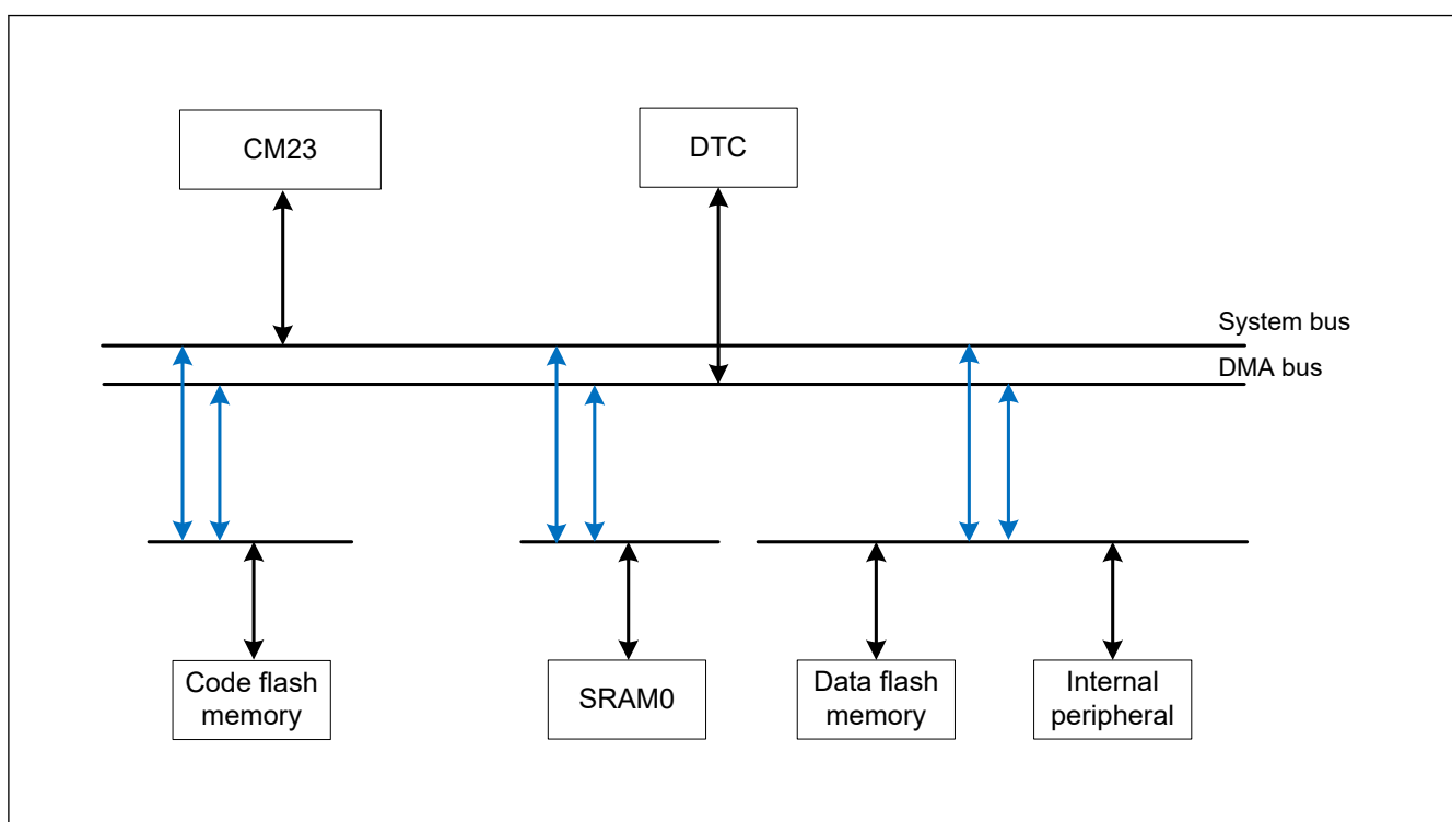
Figure 12.1 Bus configuration
