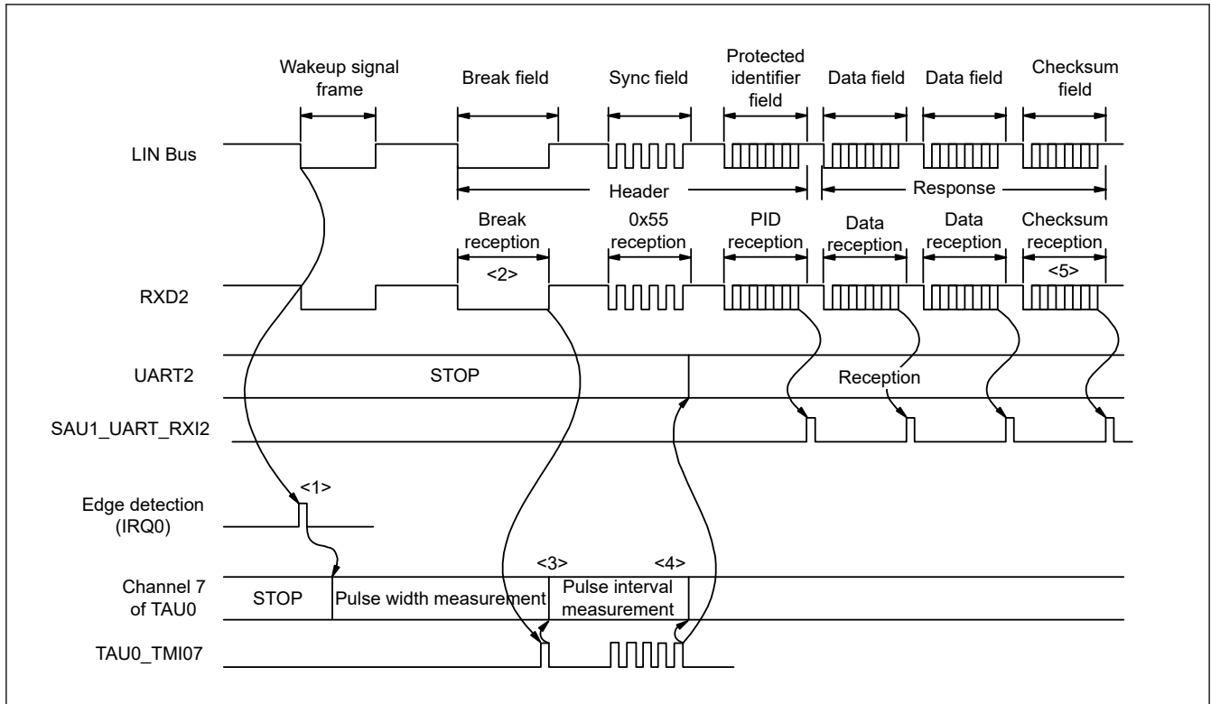
Figure 21.45 Reception operation of LIN
