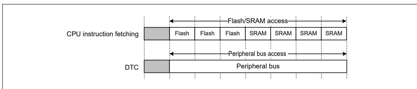
Figure 12.2 Example of parallel operations
