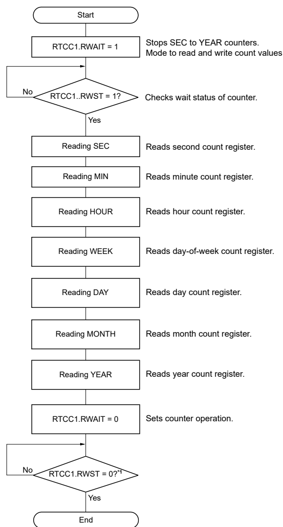
Figure 19.4 Procedure for reading realtime clock
