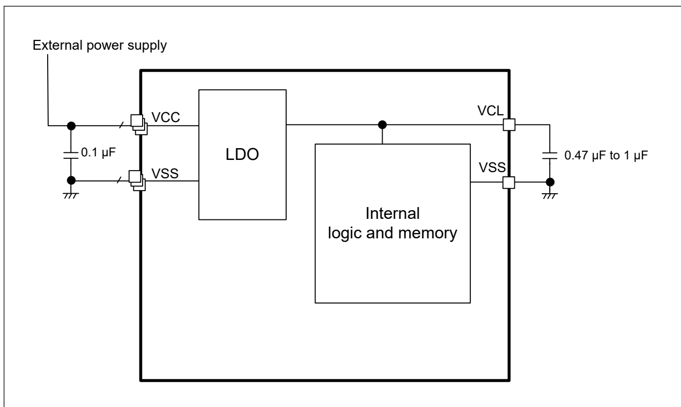
Figure 30.1 LDO settings
