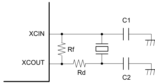
Figure 8.6 Connection example of 32.768-kHz crystal resonator
