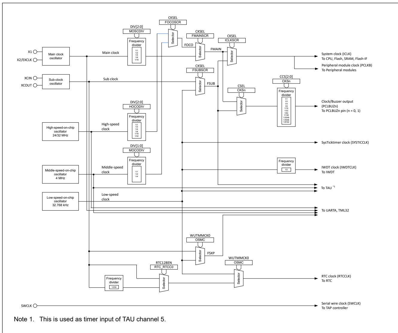
Figure 8.1 Clock generation circuit block diagram (64-, 48-, 32-pin)
