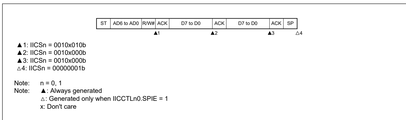
Figure 22.37 Slave device operation receiving extension code (IICCTLn0.WTIM = 0)
