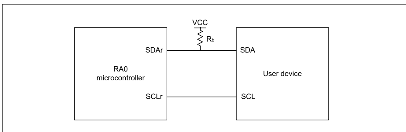
Figure 31.19 Connection in the simplified IIC communications with devices operating at the same voltage levels
