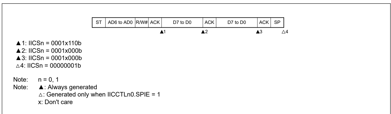
Figure 22.29 Slave device operation slave address data reception (IICCTLn0.WTIM = 0)
