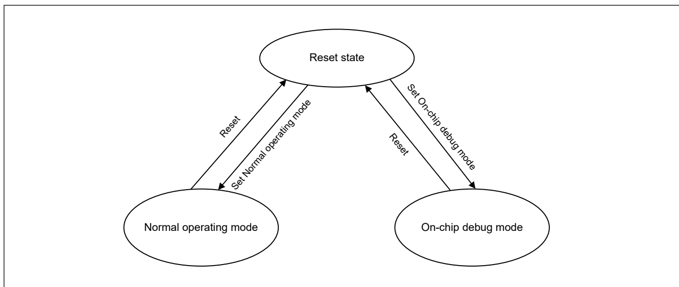
Figure 28.4 Mode transitions associated with flash memory
