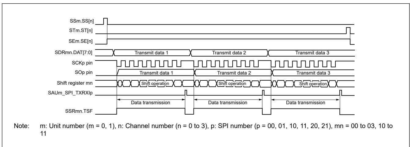
Figure 21.5 Timing of master transmission (in single transmission mode) (type 1: SCRmn.DCP[1:0] = 00b)
