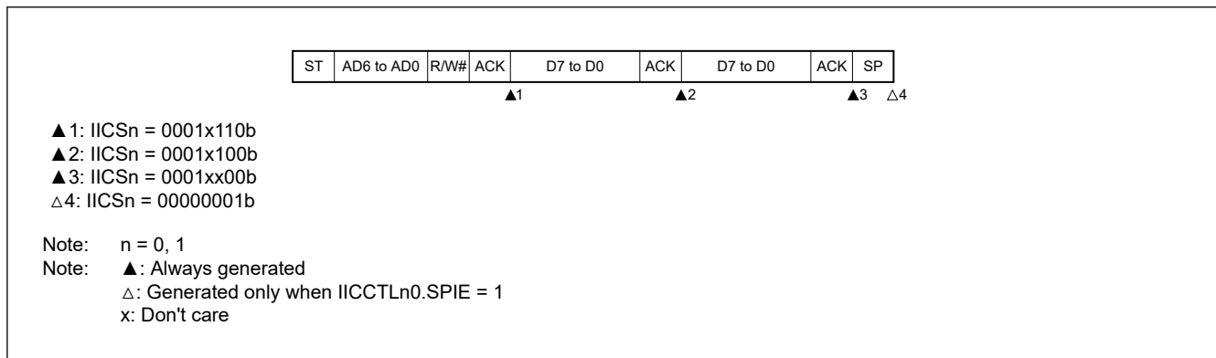
Figure 22.30 Slave device operation slave address data reception (IICCTLn0.WTIM = 1)
