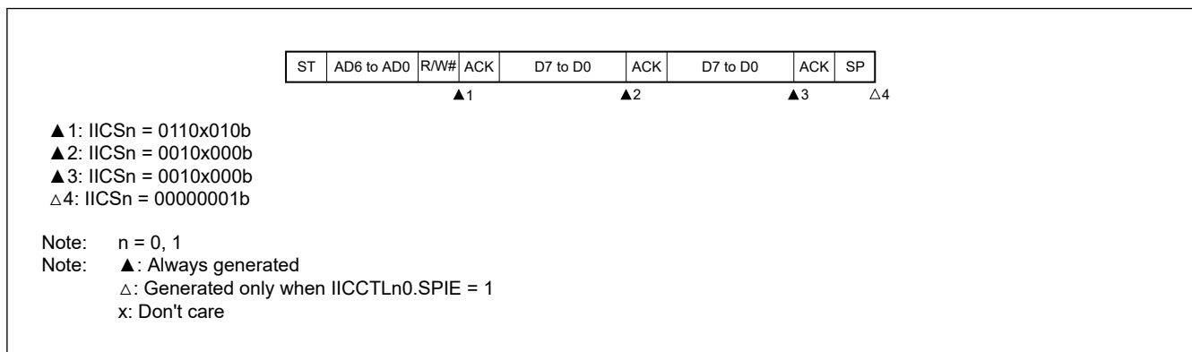
Figure 22.48 Arbitration loss when sending extension code (IICCTLn0.WTIM = 0)
