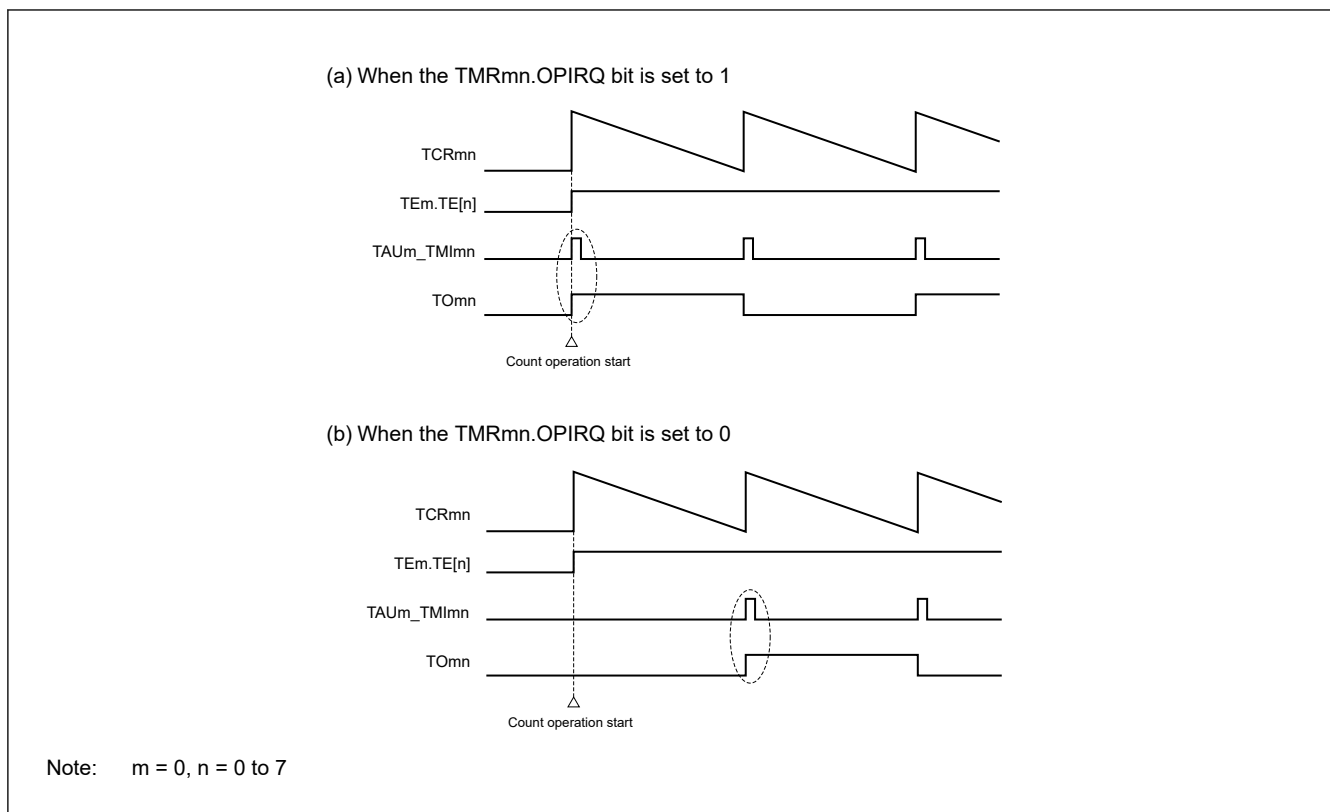
Figure 17.34 Examples of the operation of timer interrupts and T0mn outputs when counting is started
