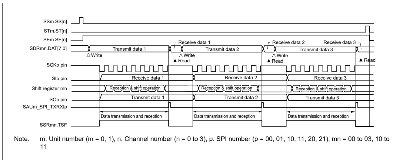
Figure 21.23 Timing of slave transmission and reception (in single transmission and reception mode)
