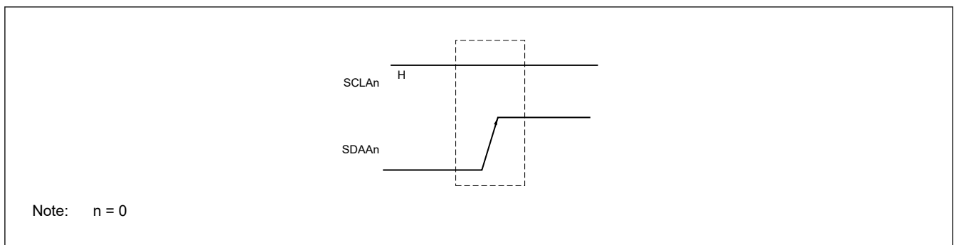
Figure 20.9 Stop condition
