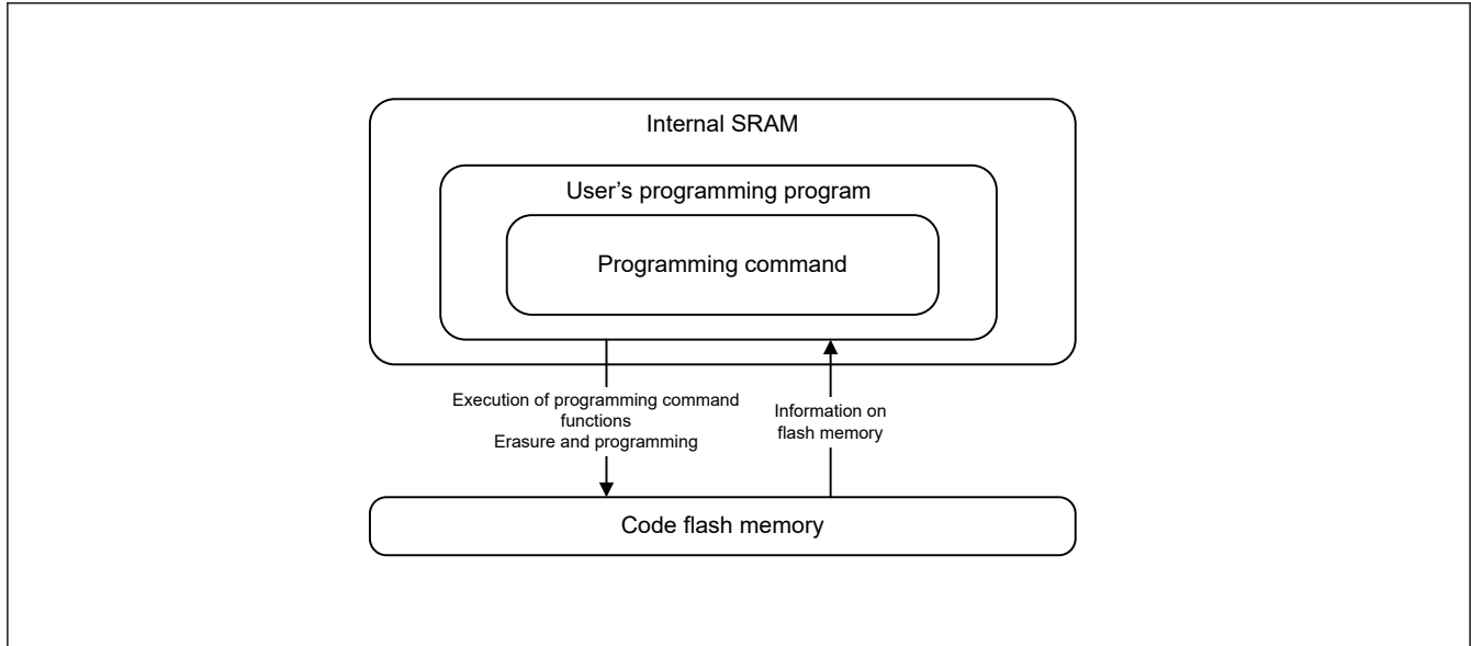
Figure 25.9 Schematic view of self-programming
