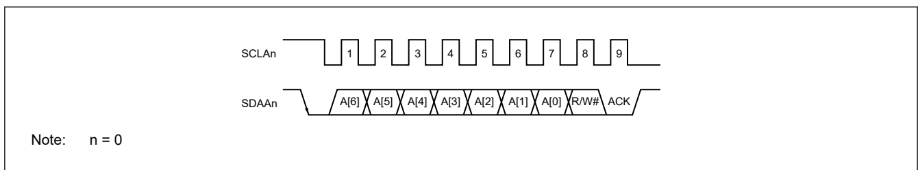
Figure 20.8 ACK
