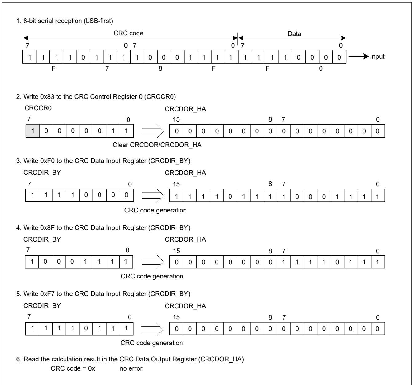
Figure 21.3 LSB-first data reception
