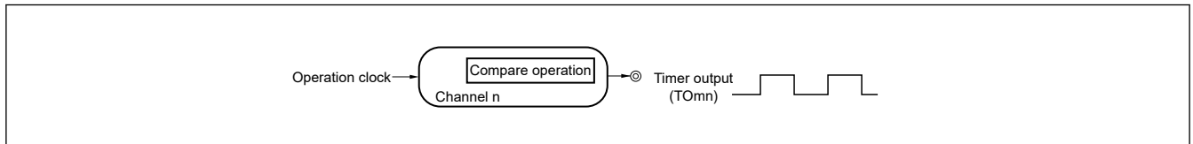
Figure 16.3 Functional image of square wave output
