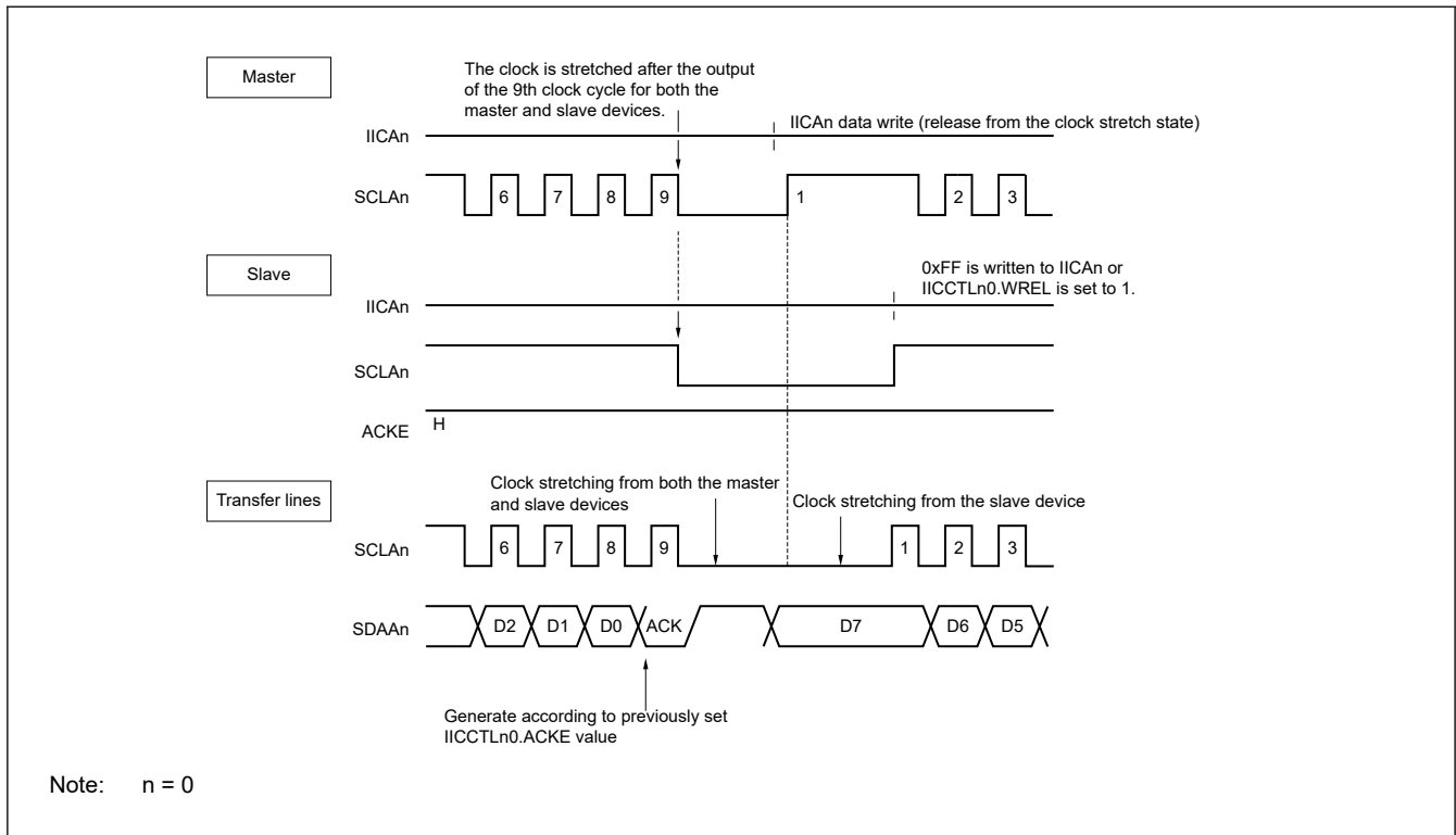
Figure 20.11 Clock stretching (2/2)
