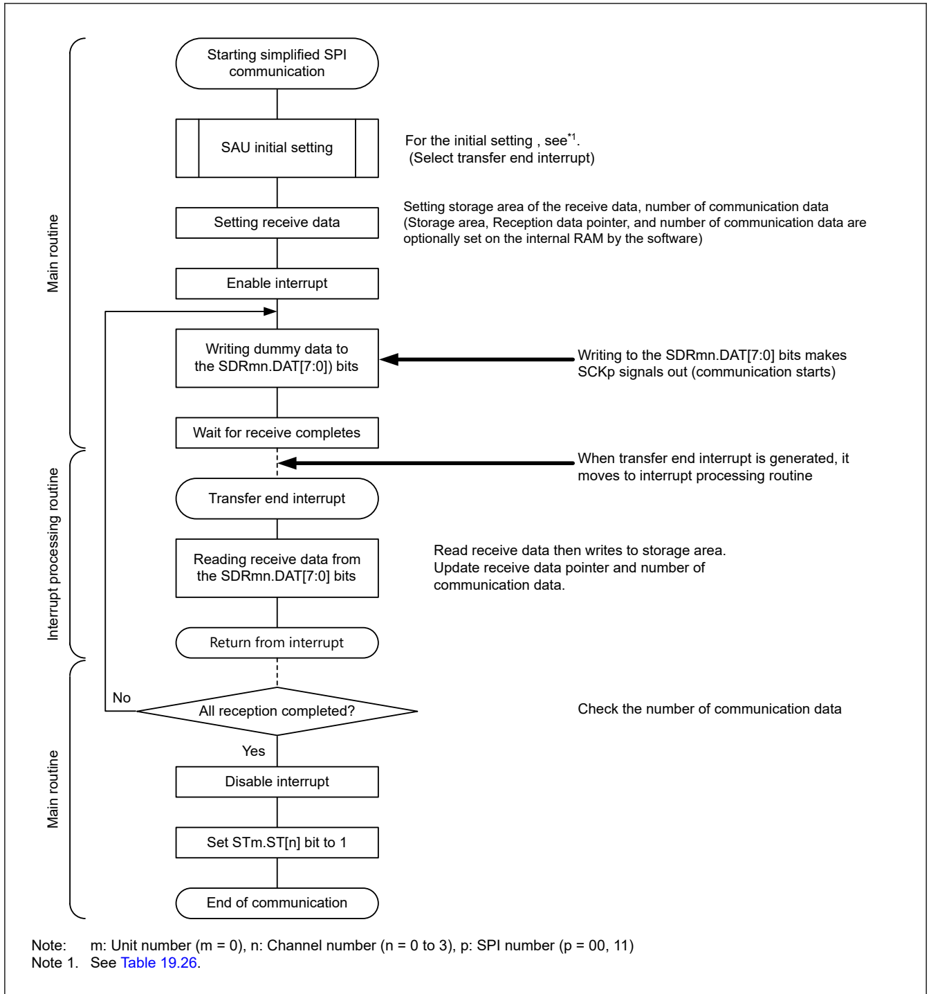
Figure 19.9 Flowchart of master reception (in single reception mode)
