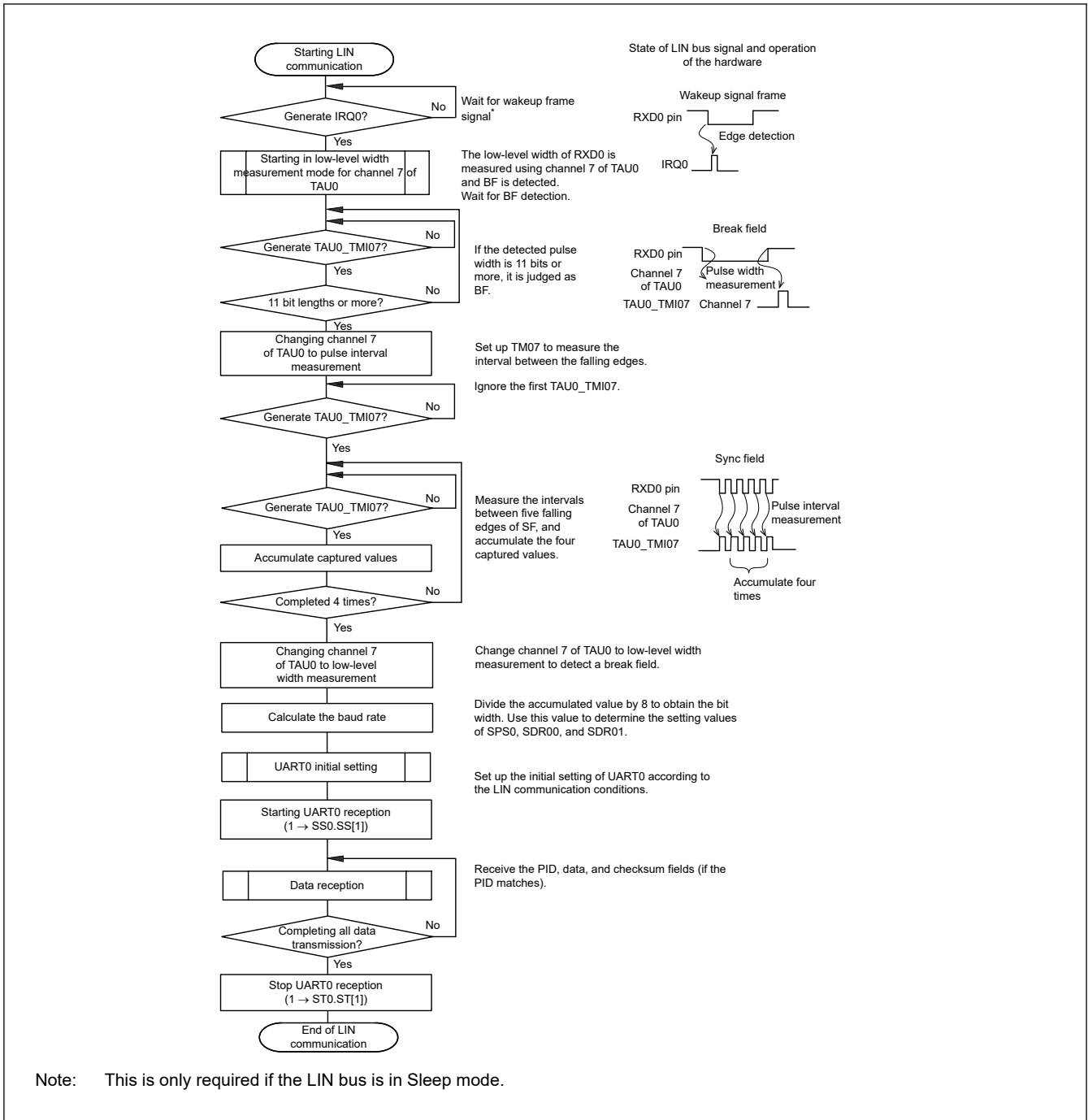
Figure 19.45 Flowchart of LIN reception
