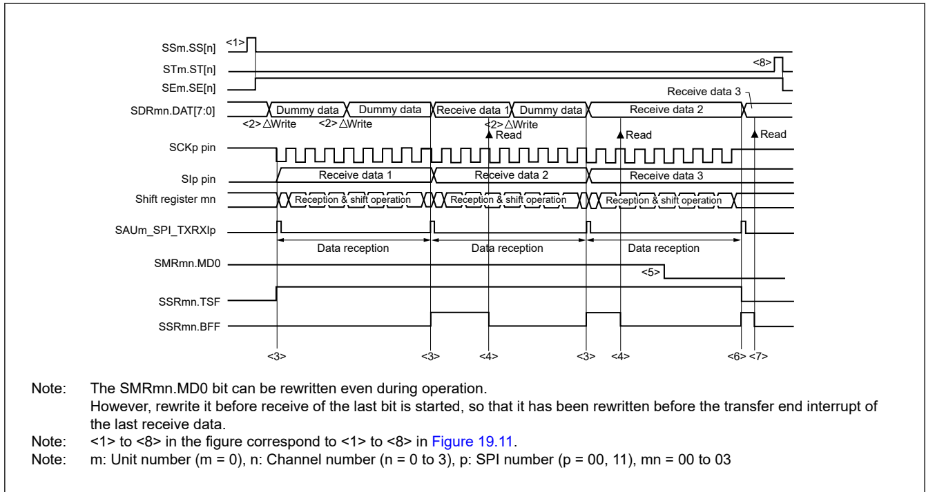
Figure 19.10 Timing of master reception (in continuous reception mode) (type 1: DCPmn[1:0] = 00b)
