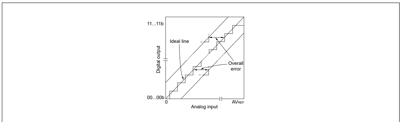
Figure 22.17 Overall error
