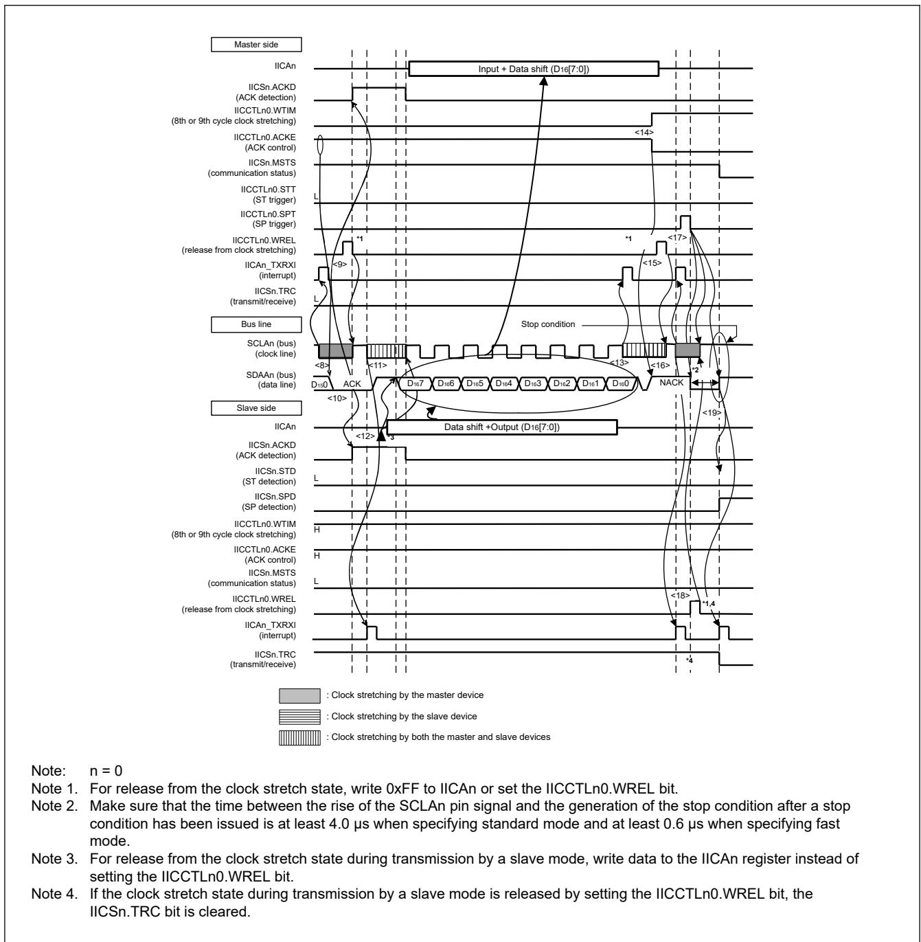
Figure 20.69 Example of slave device to master device communications (8th cycle clock stretching is selected for the master device and 9th cycle clock stretching is selected for the slave device) (3/3)
