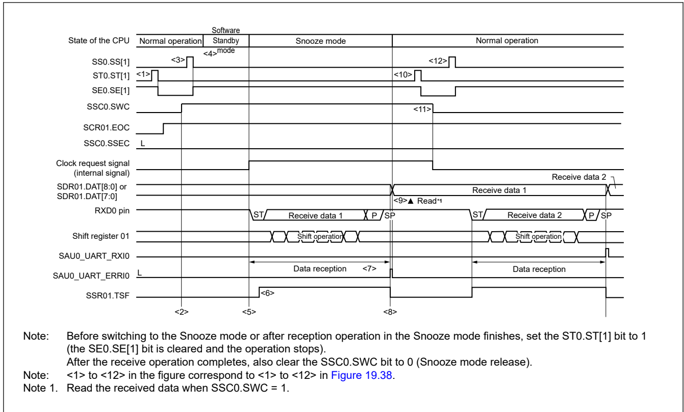
Figure 19.37 Timing of Snooze mode operation (SCR01.EOC = 1, SSC0.SSEC = 0)
