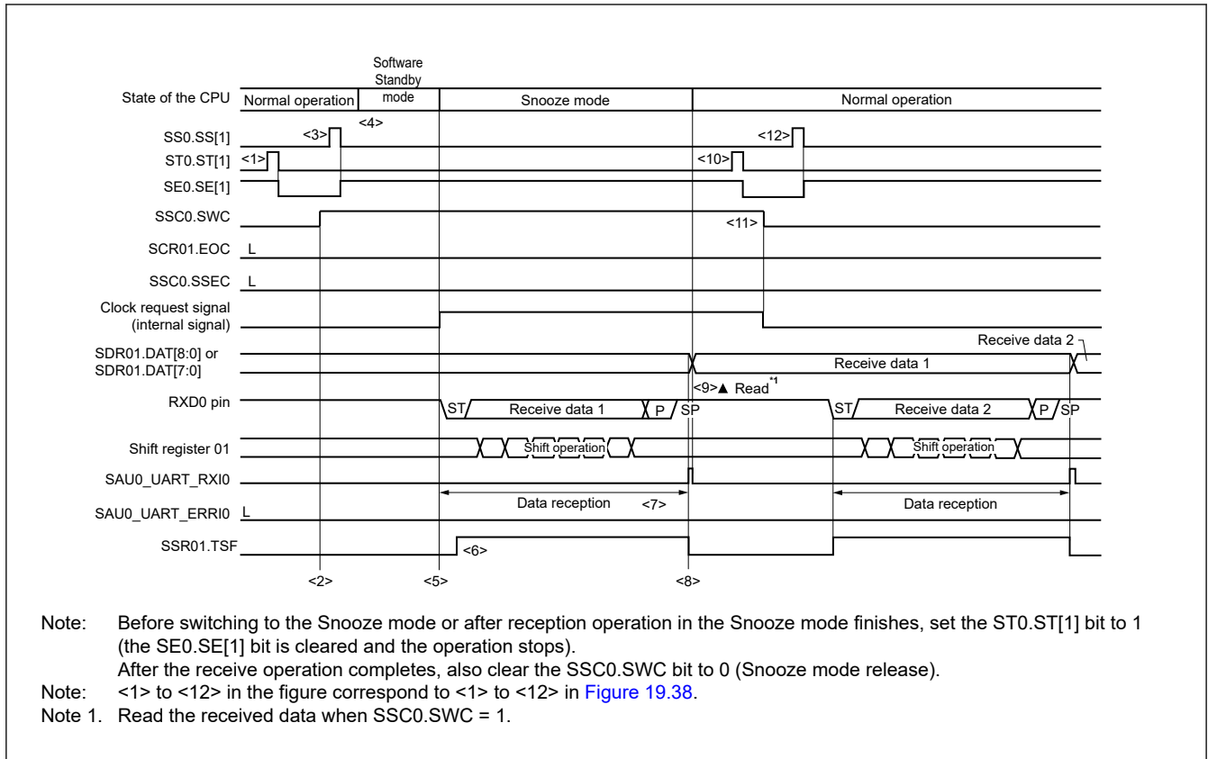
Figure 19.36 Timing of Snooze mode operation (SCR01.EOC = 0, SSC0.SSEC = 0/1)
