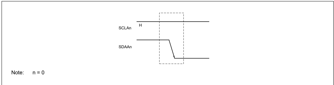
Figure 20.5 Start conditions
