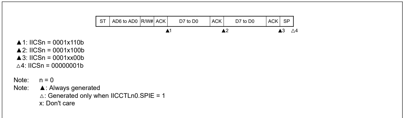
Figure 20.30 Slave device operation slave address data reception (IICCTL00.WTIM = 1)
