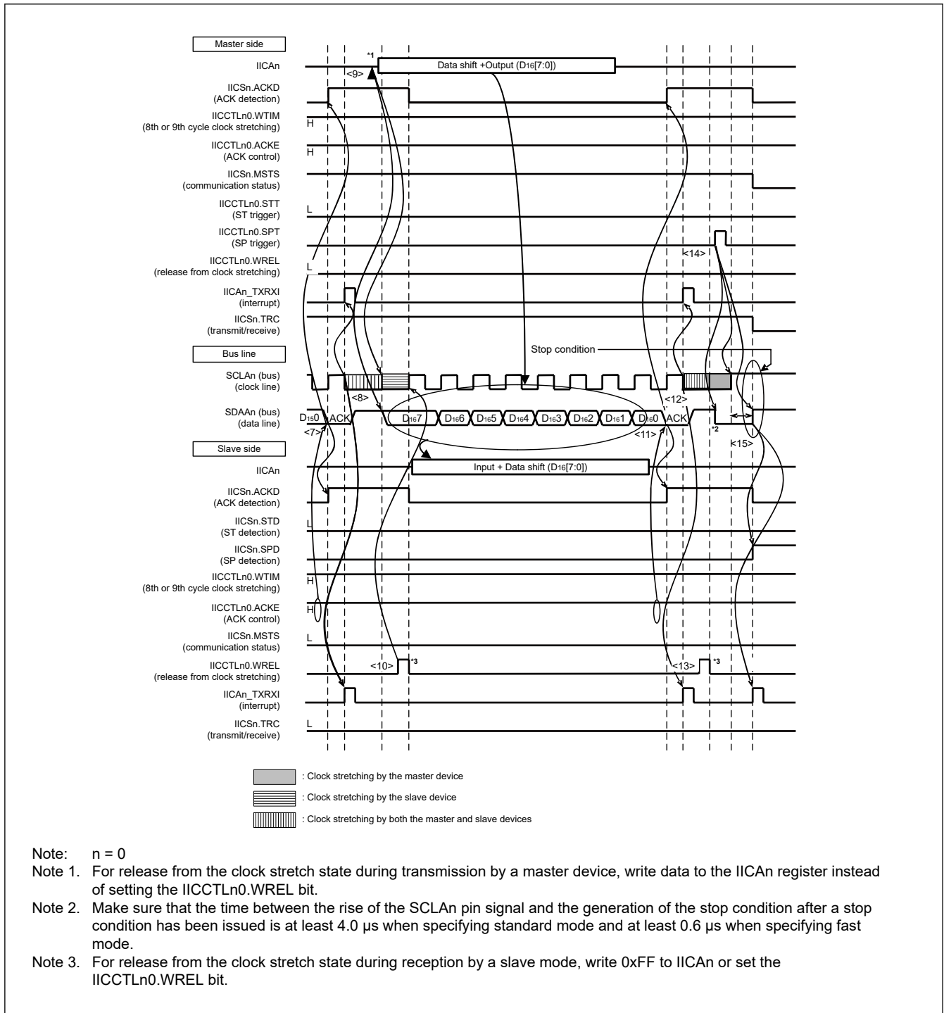
Figure 20.65 Example of master device to slave device communications (when the master device and the slave device insert clock stretching on the 9th cycle) (3/4)
