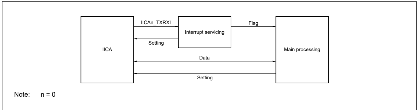
Figure 20.20 Interface configuration with the main processor in slave device operation
