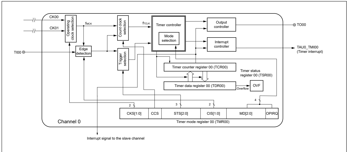
Figure 16.13 Internal block diagram of channel 0 of timer array unit 0
