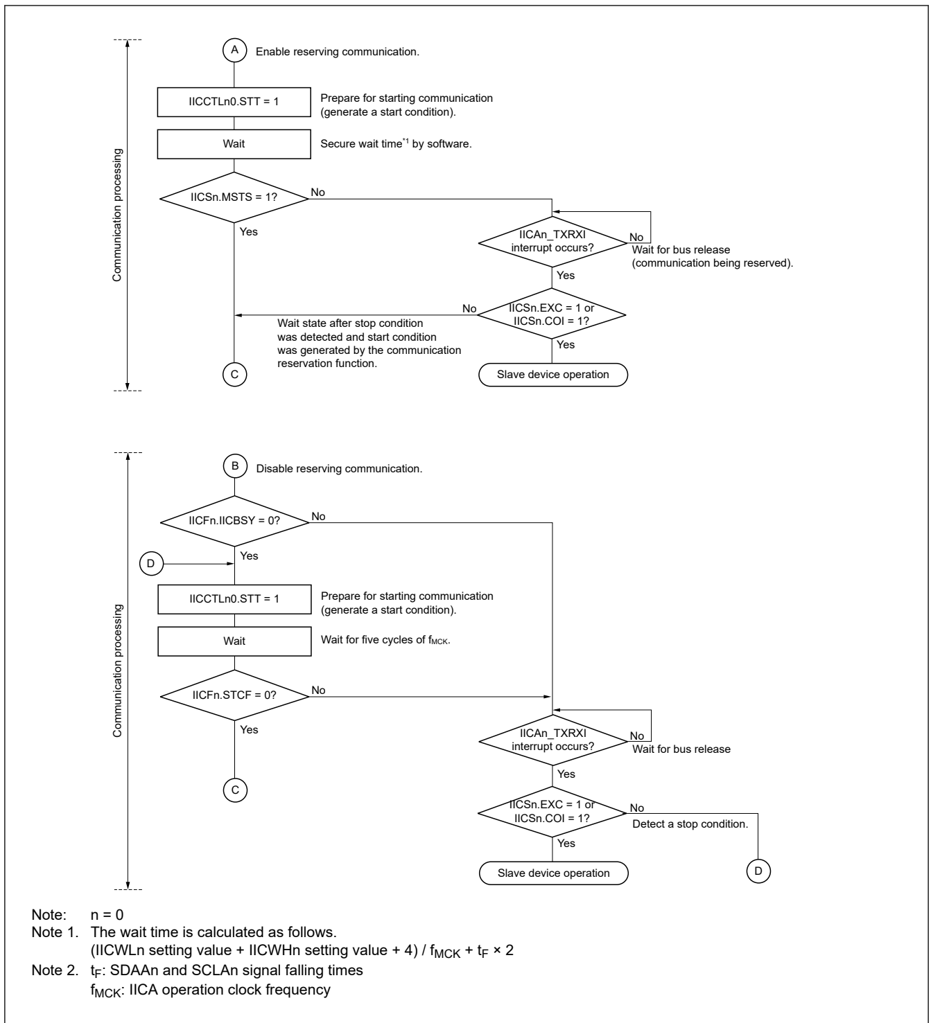
Figure 20.18 Master device operation in multi-master system (2/3)
