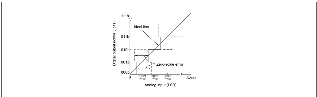
Figure 22.19 Zero-scale error
