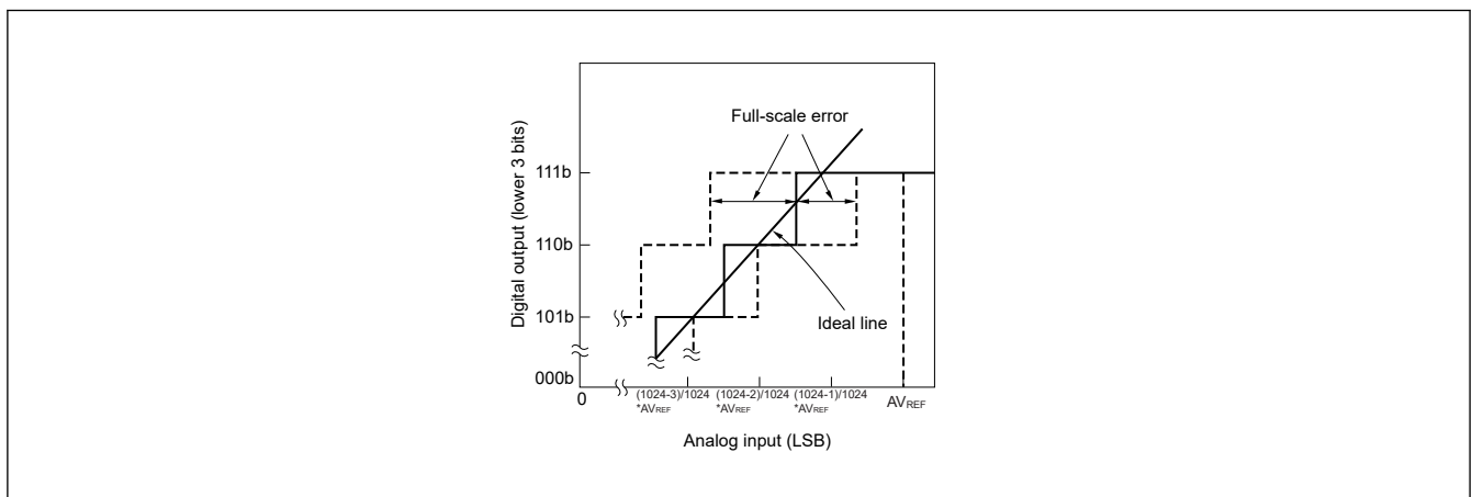
Figure 22.20 Full-scale error
