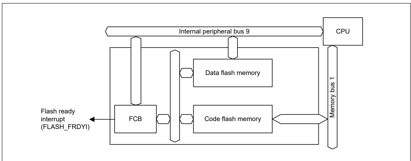
Figure 29.1 Flash memory-related modules block diagram
