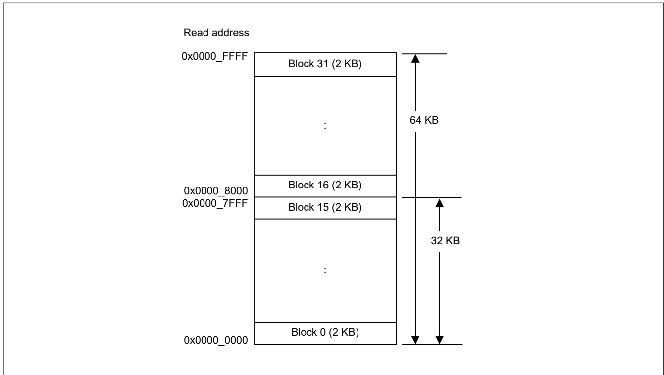
Figure 29.2 Mapping of the code flash memory
