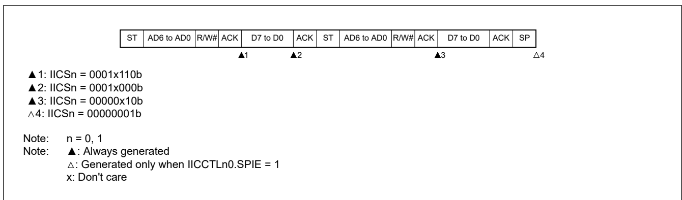
Figure 22.35 Slave device operation after normal access, does not match (IICCTLn0.WTIM = 0)
