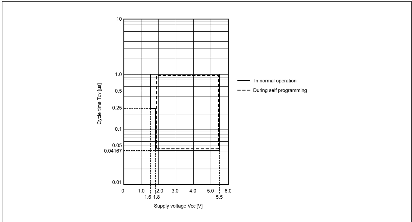
Figure 32.3 T_{CY} vs V_{CC} in Middle-speed mode
