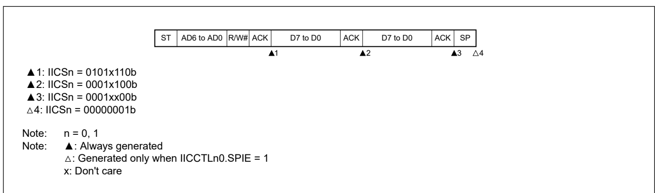
Figure 22.47 Arbitration loss when sending slave address data (IICCTLn0.WTIM = 1)
