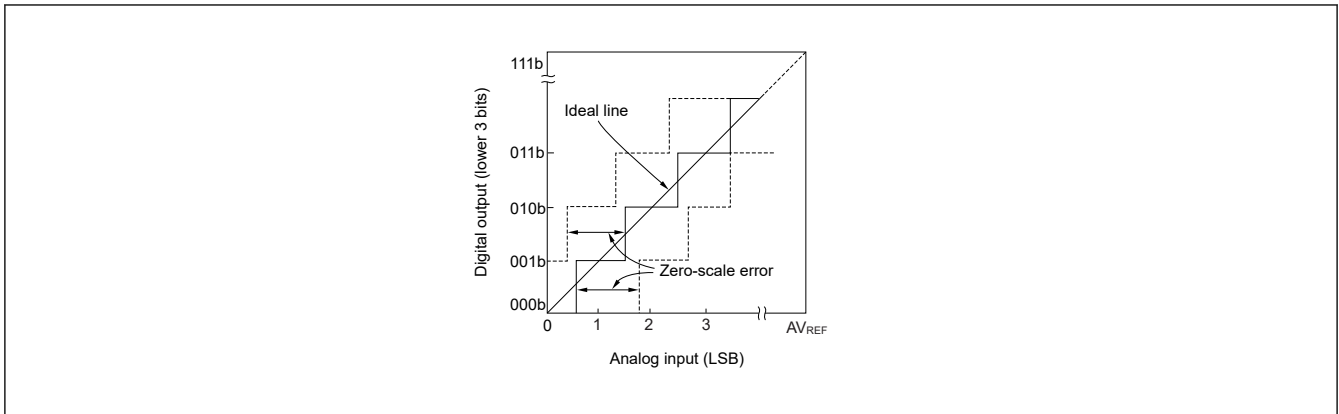
Figure 25.30 Zero-scale error
