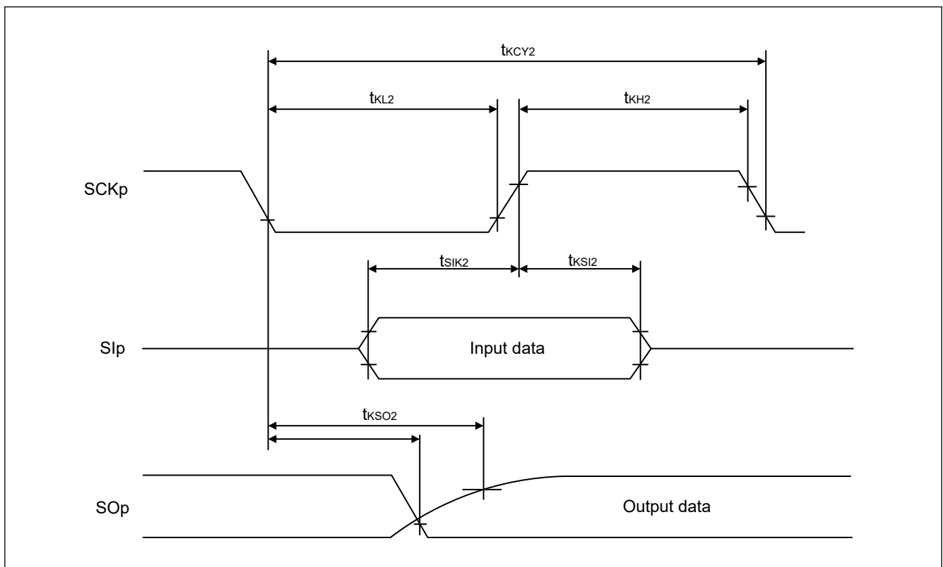
Figure 32.27 Timing of serial transfer in the simplified SPI communications in the slave mode with devices operating at different voltage levels when SCR mn .DCP[1:0] = 00b or 11b
