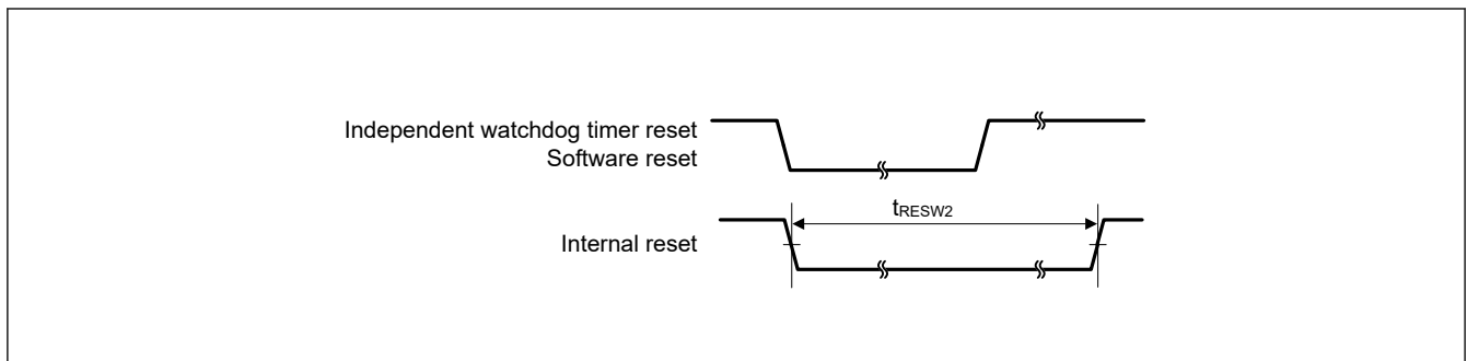
Figure 32.11 Reset input timing (2)
