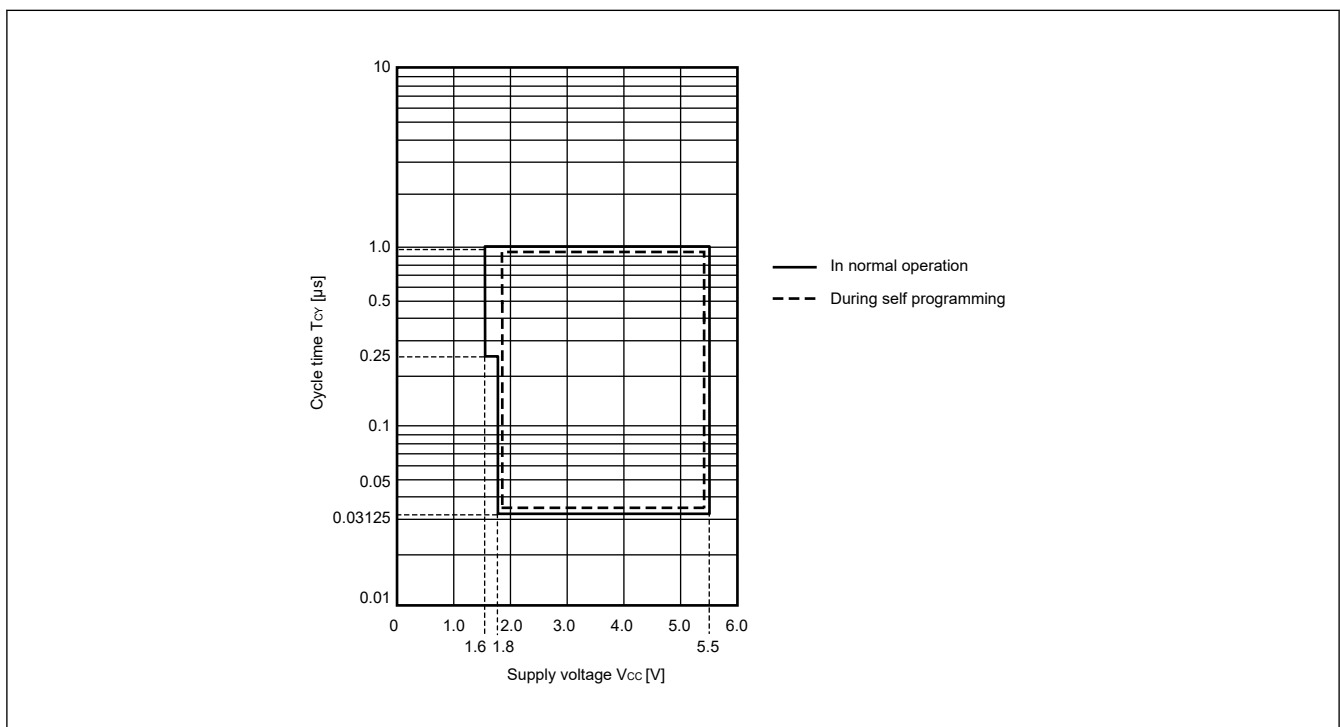
Figure 32.2 T CY vs V CC in High-speed mode
