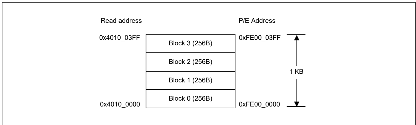
Figure 29.3 Mapping of the data flash memory
