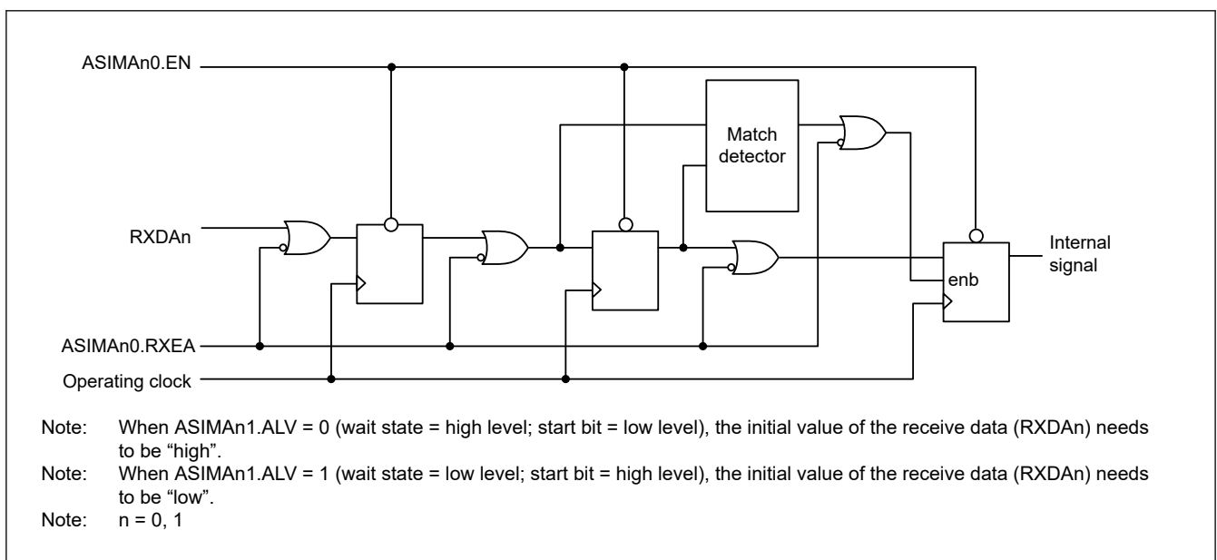
Figure 23.9 Noise filter
