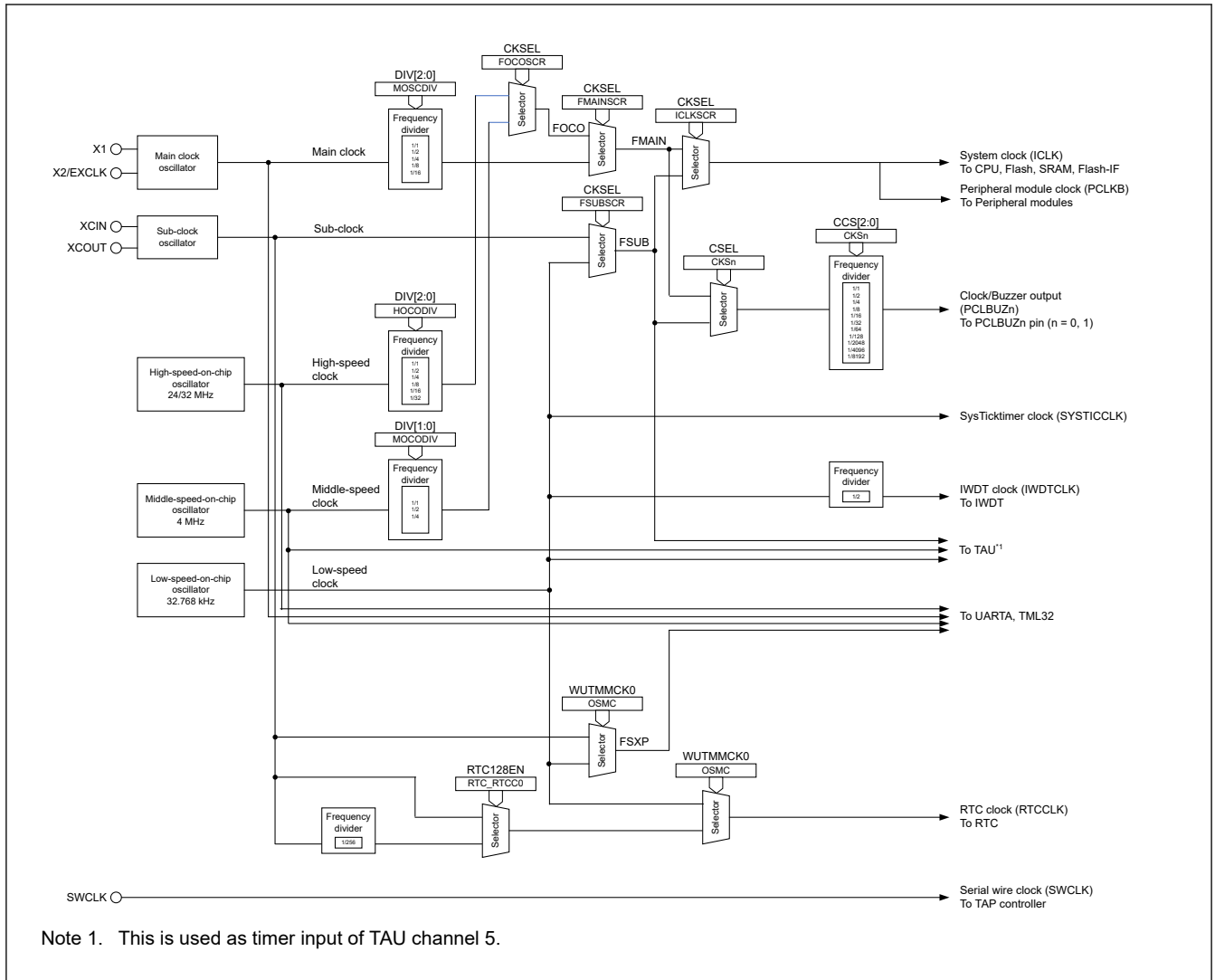
Figure 8.1 Clock generation circuit block diagram (48- and 32-pin)
