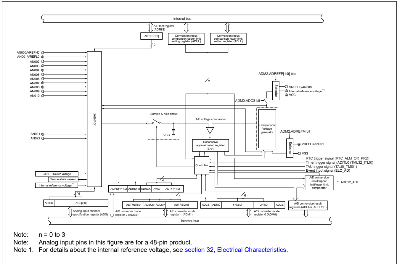
Figure 25.1 Block diagram of A/D converter
