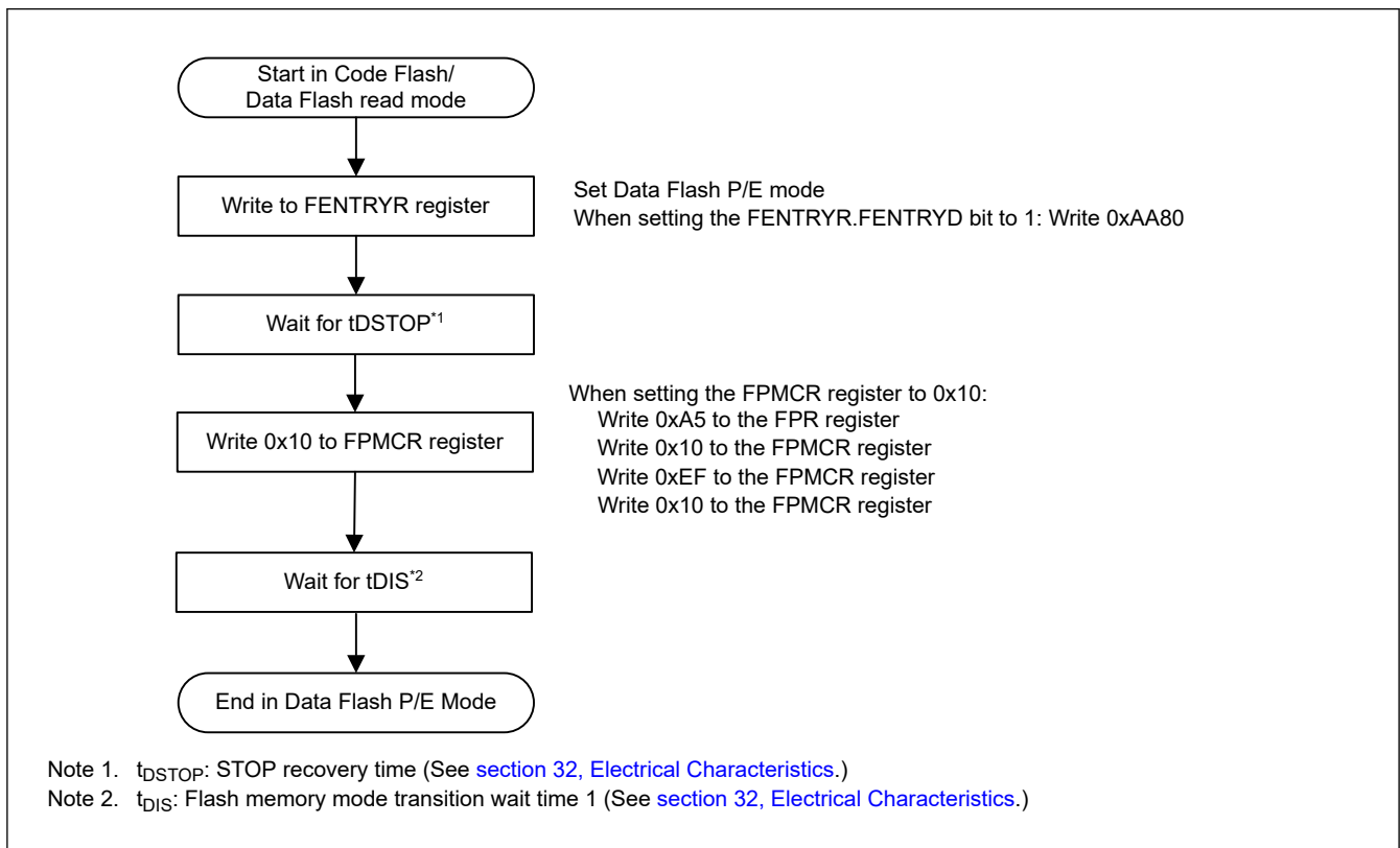
Figure 29.14 Procedure for changing from read mode to data flash P/E mode
