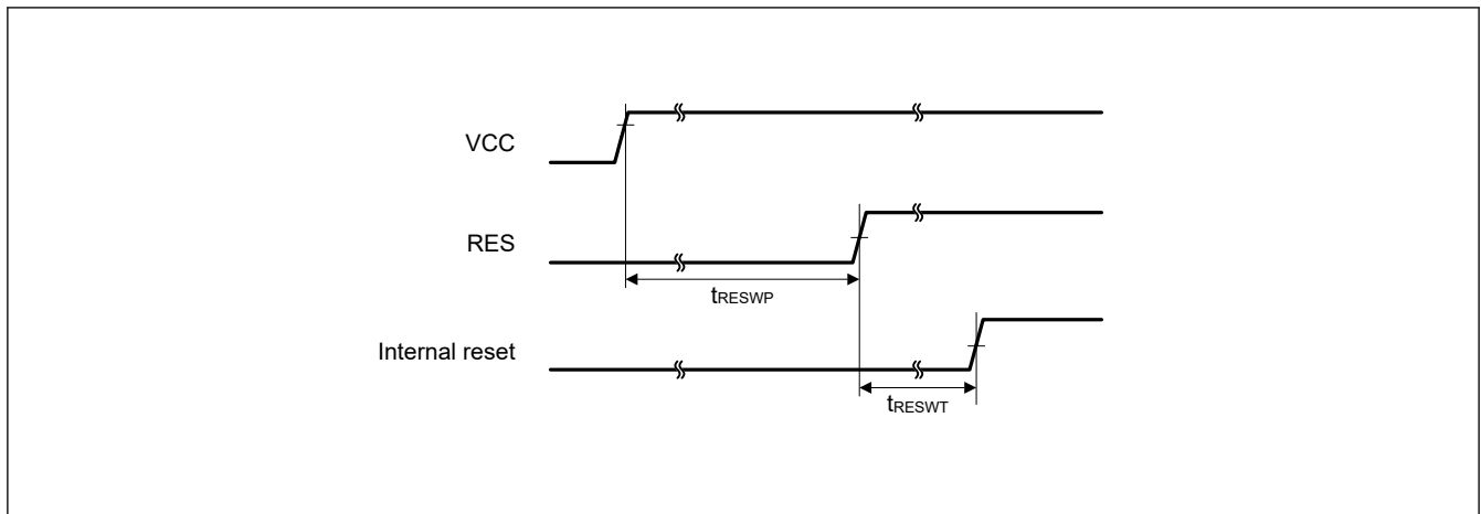
Figure 32.9 Reset input timing at power-on
