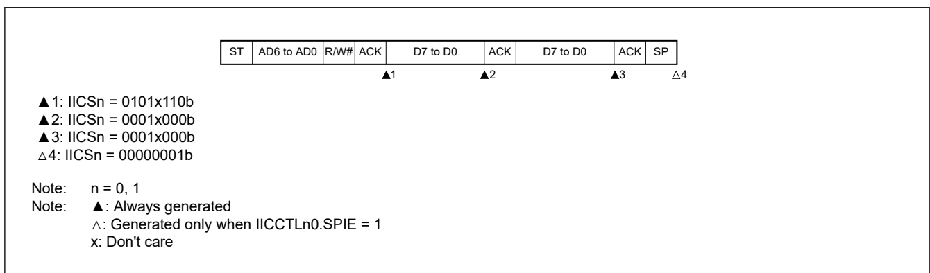
Figure 22.46 Arbitration loss when sending slave address data (IICCTLn0.WTIM = 0)
