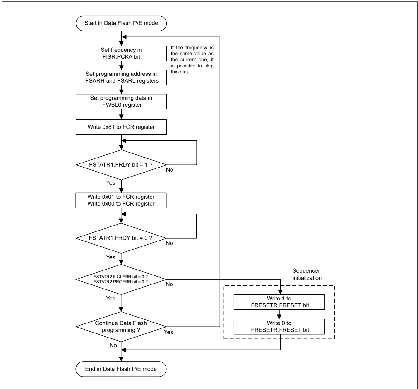
Figure 29.18 Flowchart for programming of the data flash
