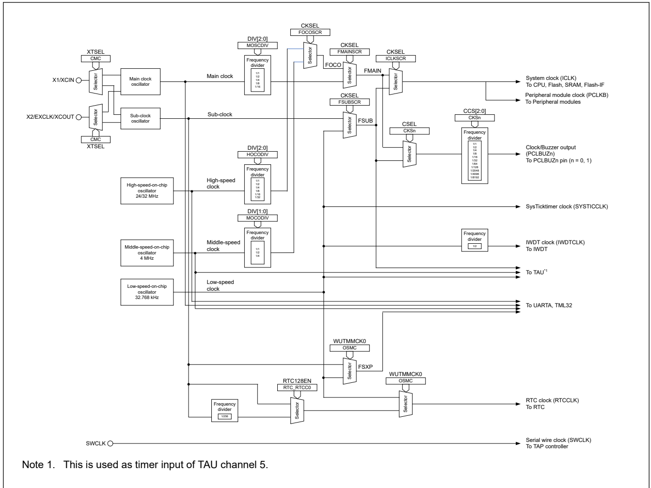
Figure 8.2 Clock generation circuit block diagram (24- and 20-pin)
