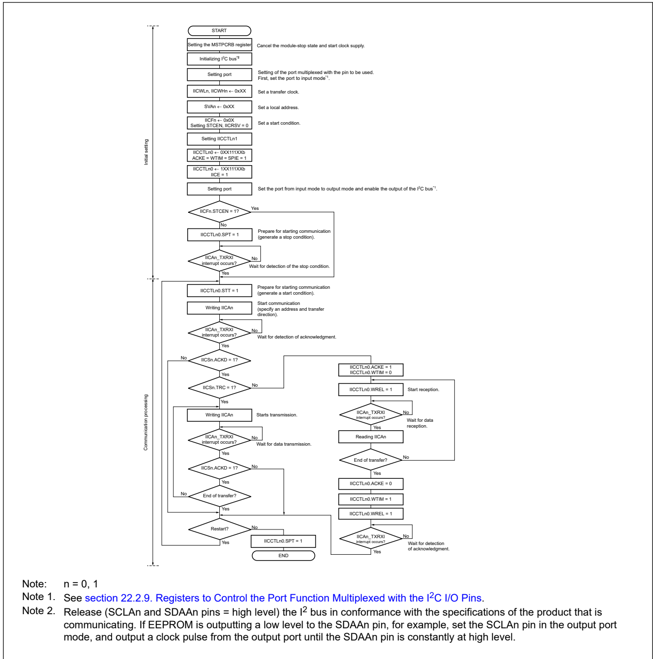
Figure 22.16 Master device operation in single-master system
