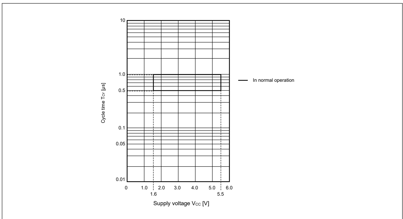
Figure 32.4 T_{CY} vs V_{CC} in Low-speed mode
