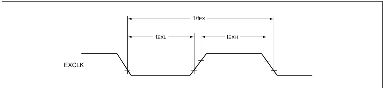
Figure 32.6 External system clock timing
