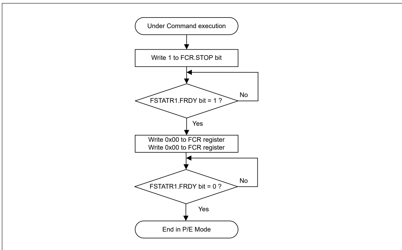
Figure 29.24 Simple flowchart for the forced stop procedure
