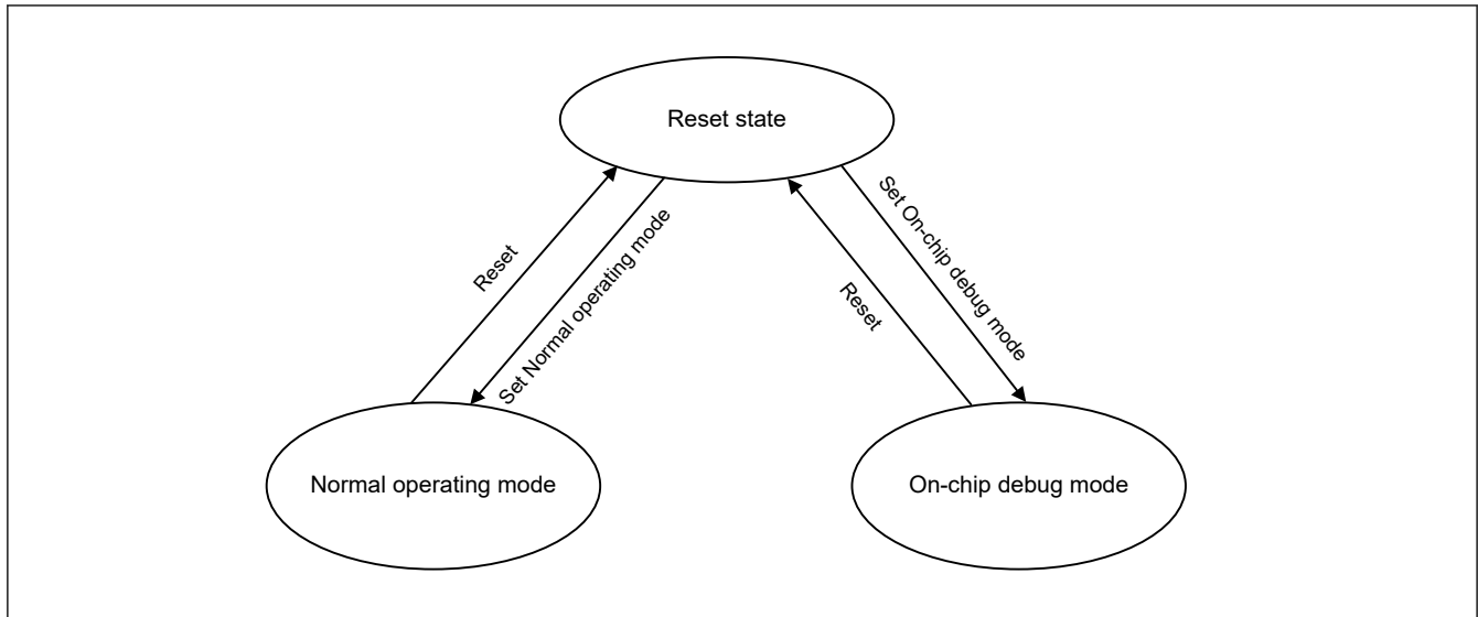
Figure 29.4 Mode transitions associated with flash memory
