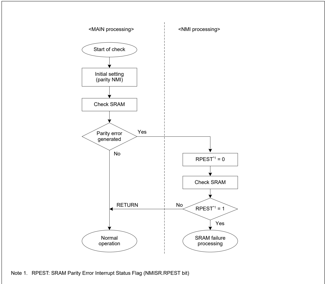
Figure 28.2 Flow of SRAM parity check when SRAM parity interrupt is enabled
