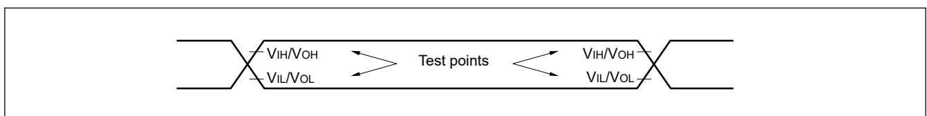
Figure 32.5 AC timing test points
