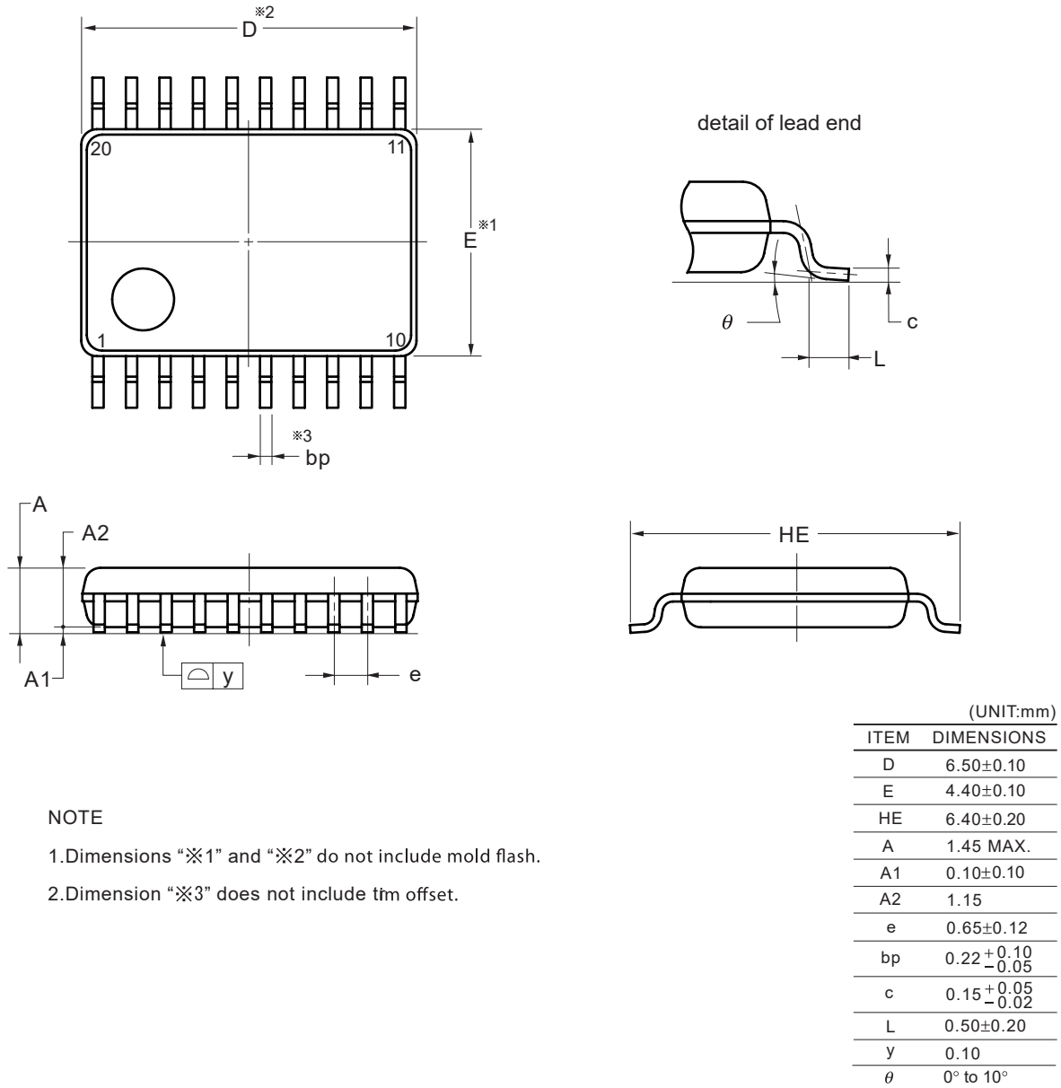
Figure A2.6 LSSOP 20-pin
