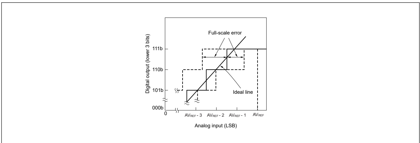
Figure 25.31 Full-scale error
