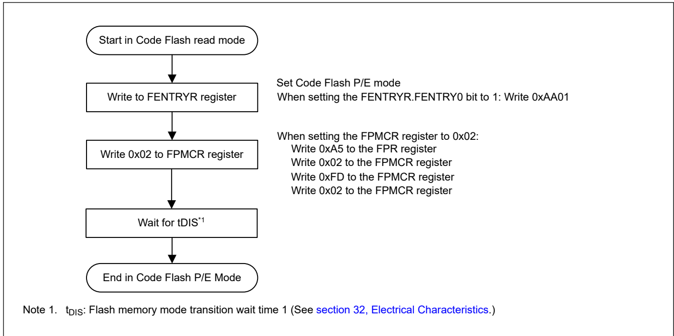
Figure 29.13 Procedure for changing from read mode to code flash P/E mode
