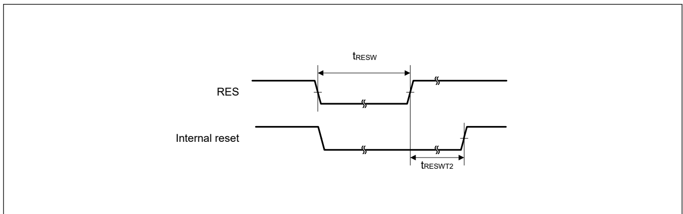
Figure 32.10 Reset input timing (1)
