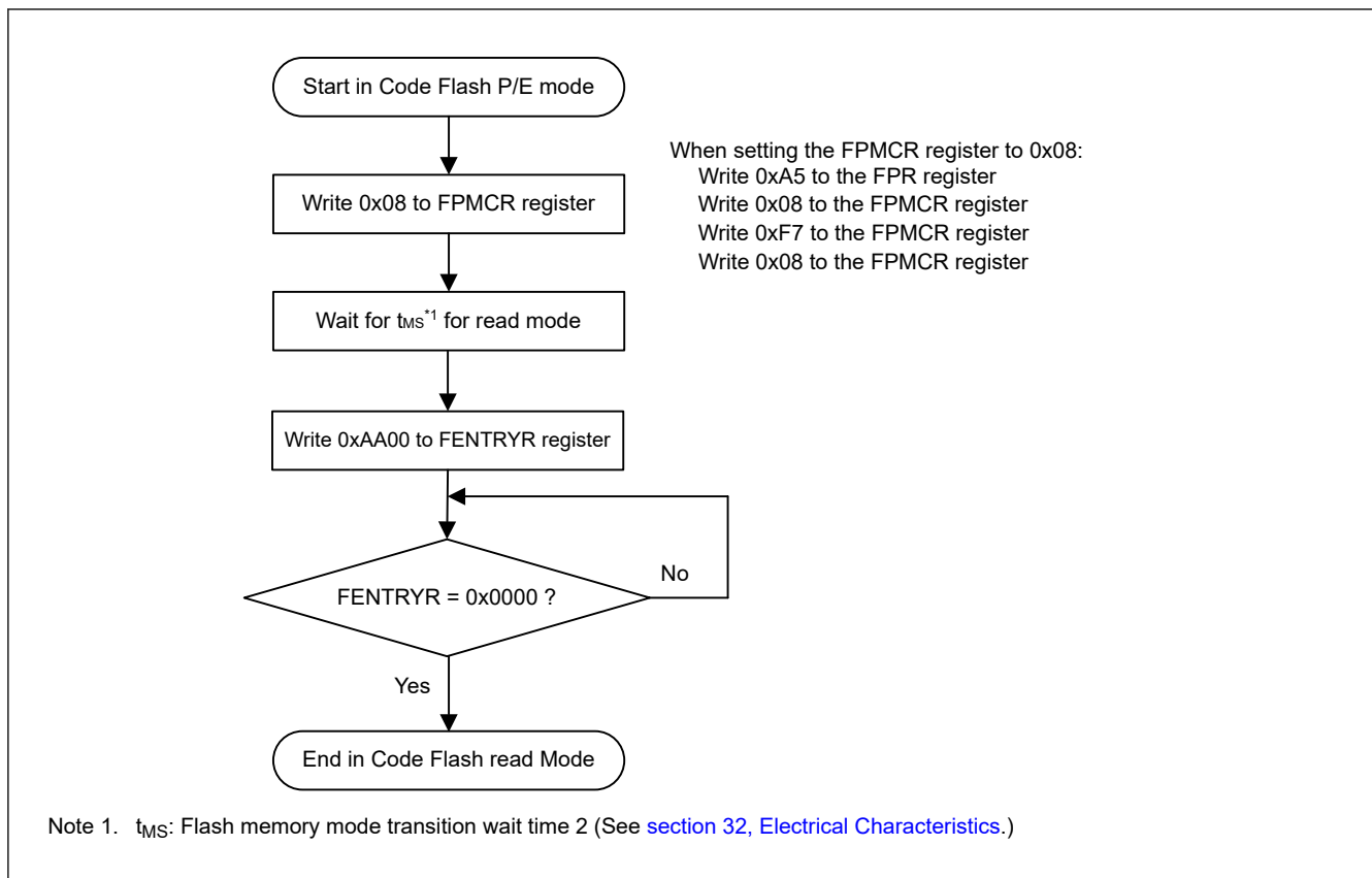
Figure 29.15 Procedure for changing from code flash P/E mode to read mode
