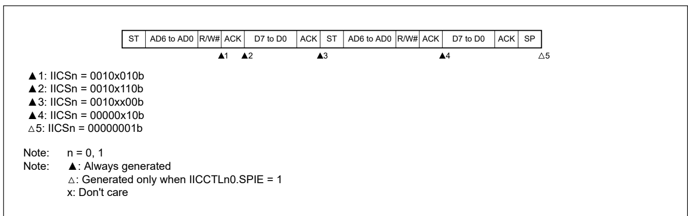
Figure 22.44 Slave device operation after code access, does not match (IICCTLn0.WTIM = 1)
