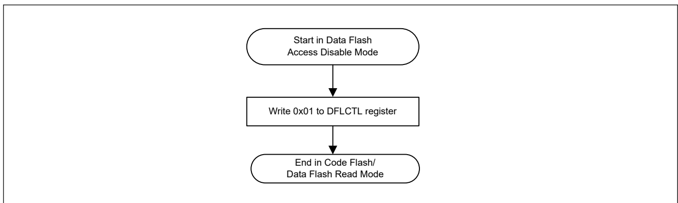
Figure 29.12 Mode transitions to read mode from data flash access disable mode
