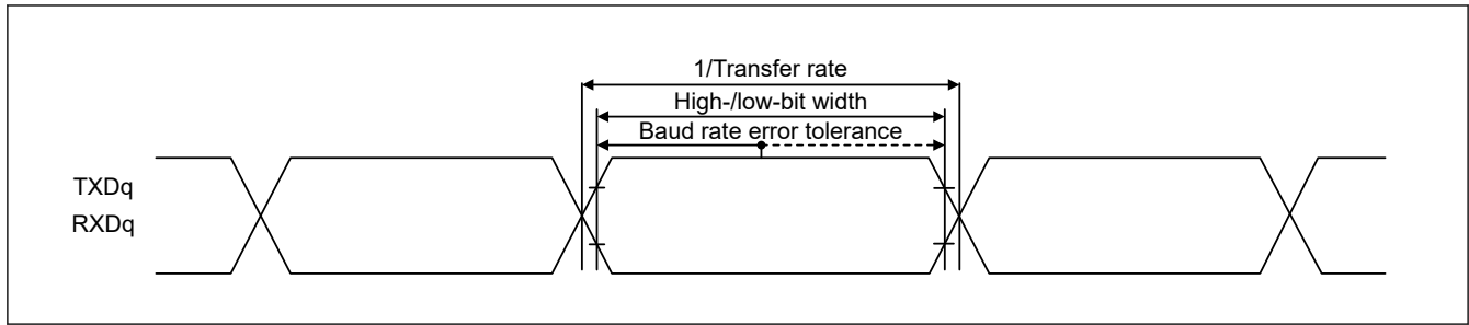
Figure 32.15 Bit width in the UART communications when interfacing devices operate at the same voltage level (reference)
