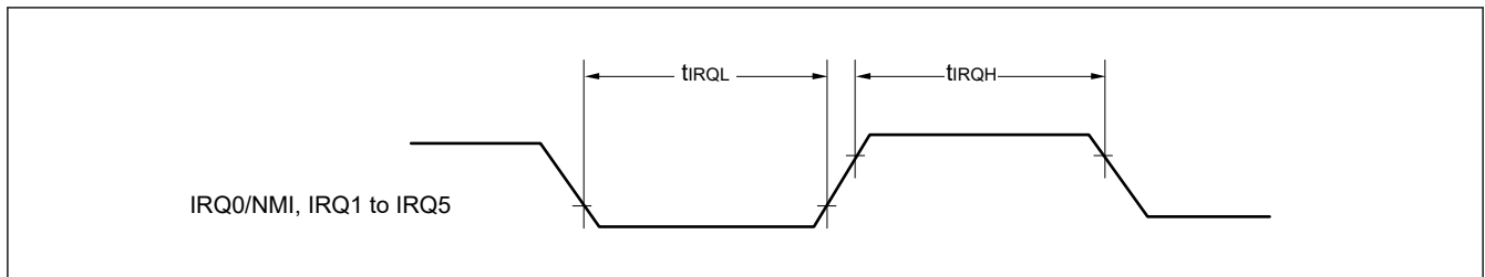
Figure 32.8 IRQ interrupt input timing
