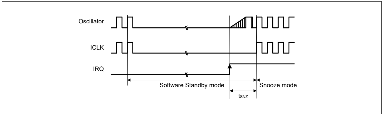
Figure 32.13 Recovery timing from Software Standby mode to Snooze mode
