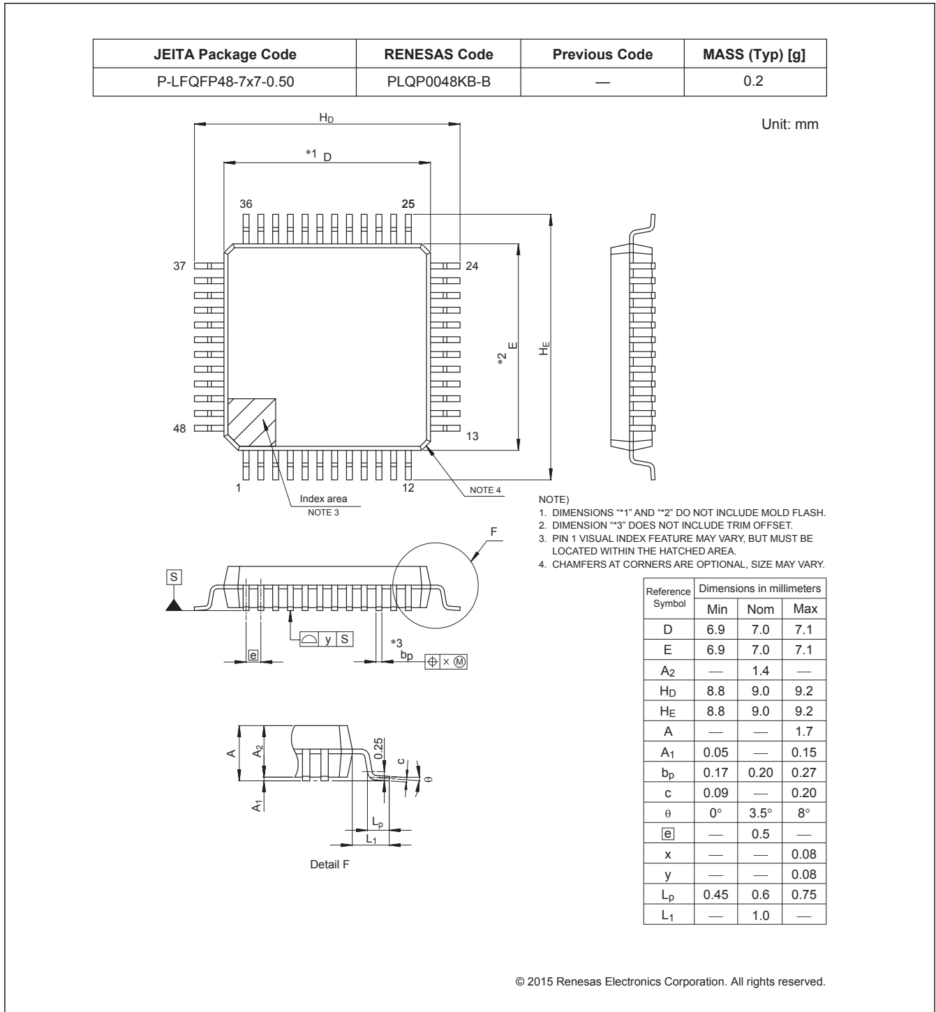
Figure A2.1 LFQFP 48-pin
