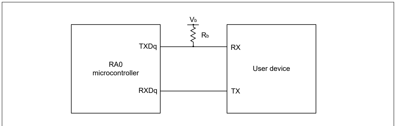
Figure 32.21 In UART communications with devices operating at different voltage levels
