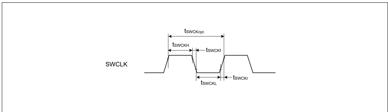
Figure 32.37 SWD SWCLK timing
