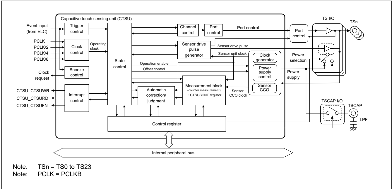
Figure 27.3 CTSU block diagram
