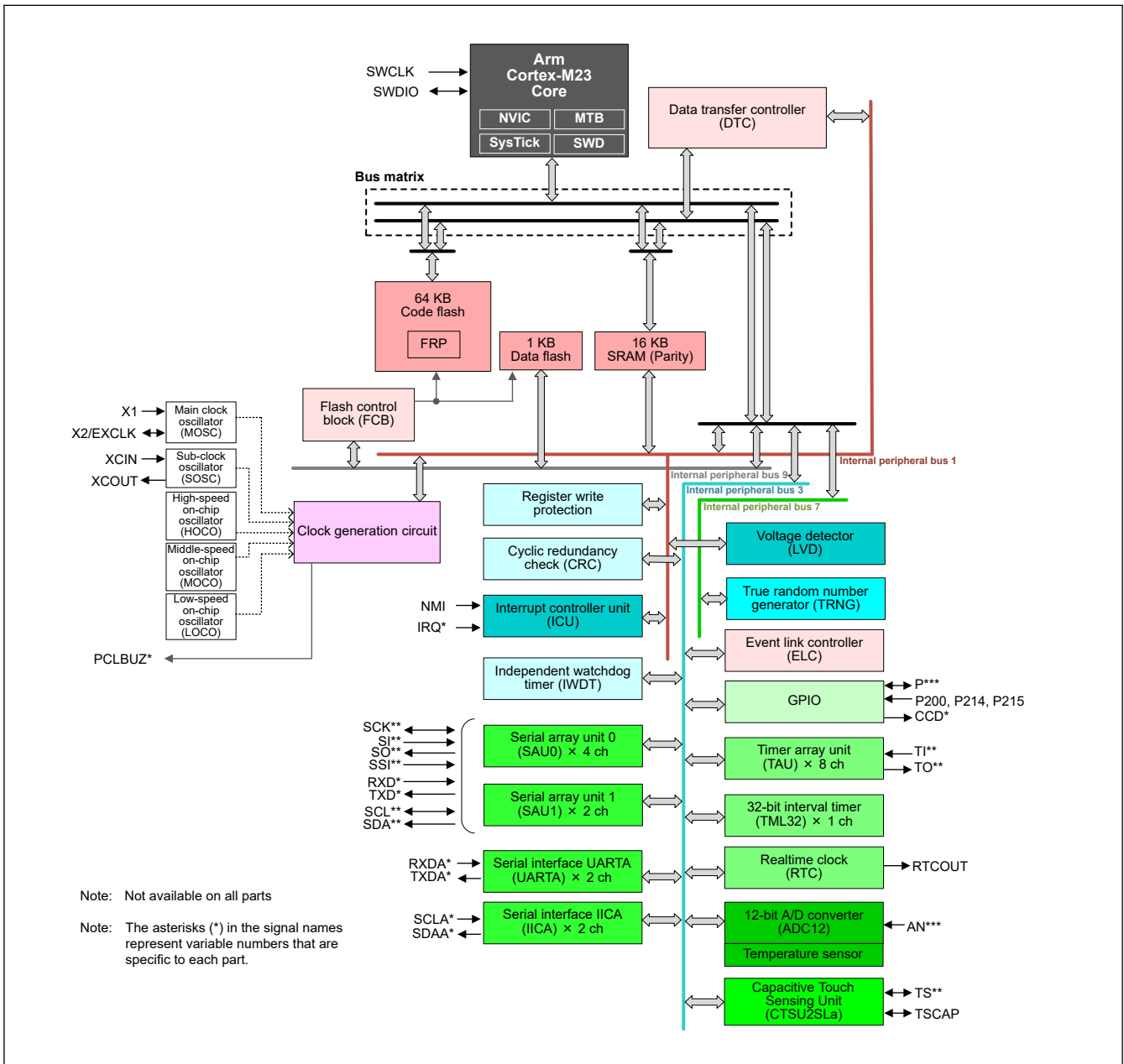
Figure 1.1 Block diagram
