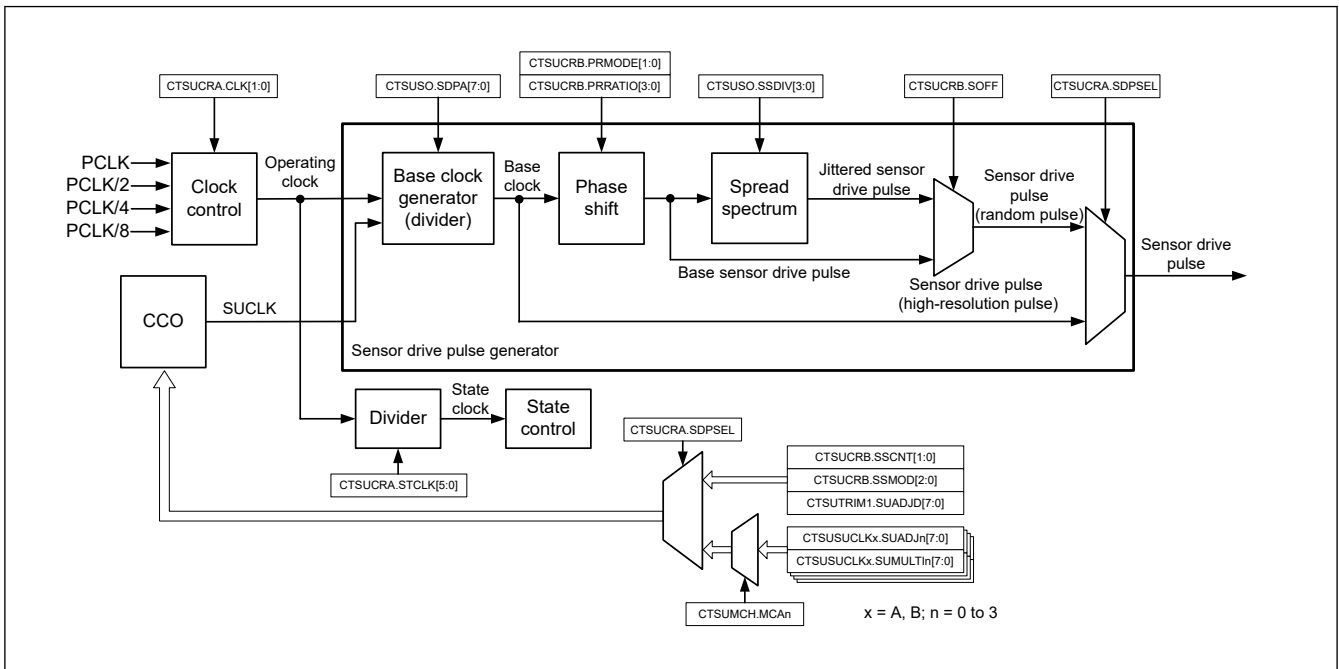
Figure 27.4 Generation of sensor drive pulse
