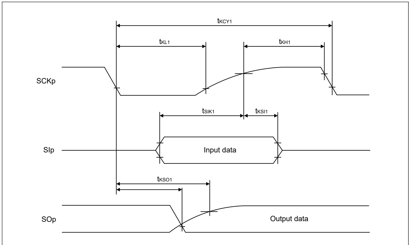
Figure 32.24 Timing of serial transfer in the simplified SPI communications in the master mode with devices operating at different voltage levels when SCRmn.DCP[1:0] = 00b or 11b
