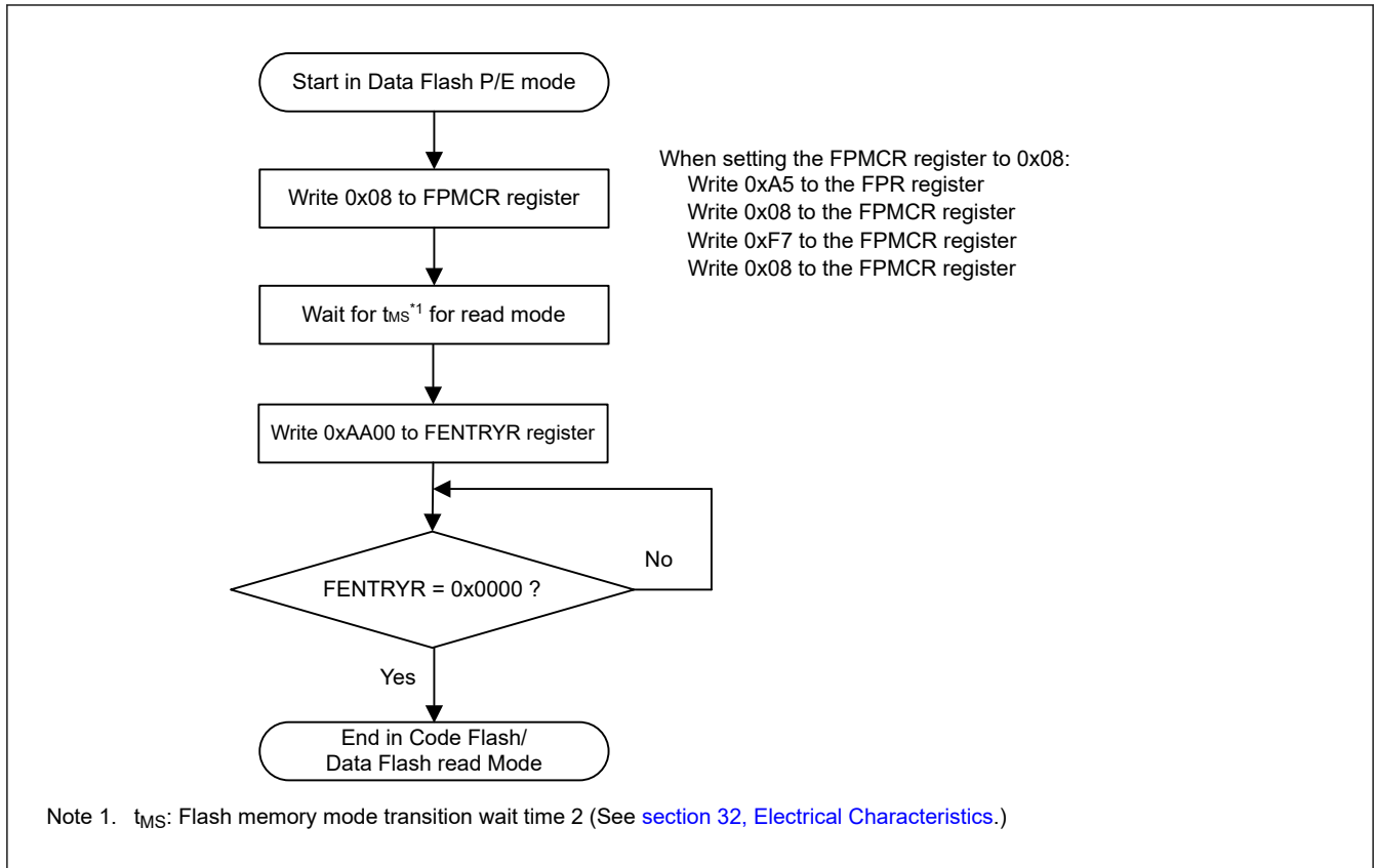
Figure 29.16 Procedure for changing from data flash P/E mode to read mode
