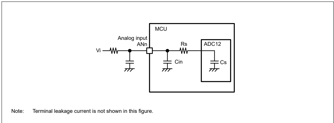
Figure 32.32 Equivalent circuit for analog input
