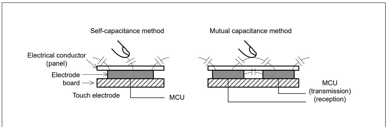
Figure 27.2 Self-capacitance and mutual capacitance methods
