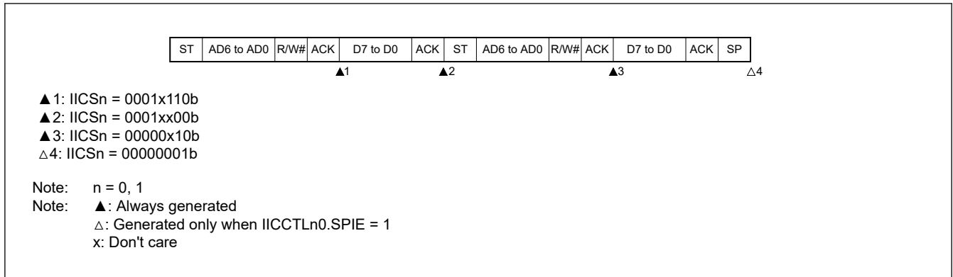
Figure 22.36 Slave device operation after normal access, does not match (IICCTLn0.WTIM = 1)
