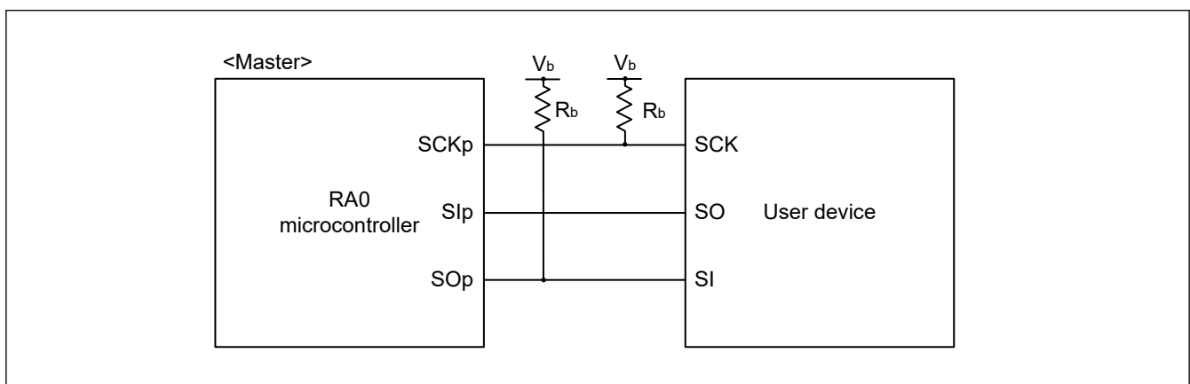
Figure 32.23 Connection in the simplified SPI communications with devices operating at different voltage levels
