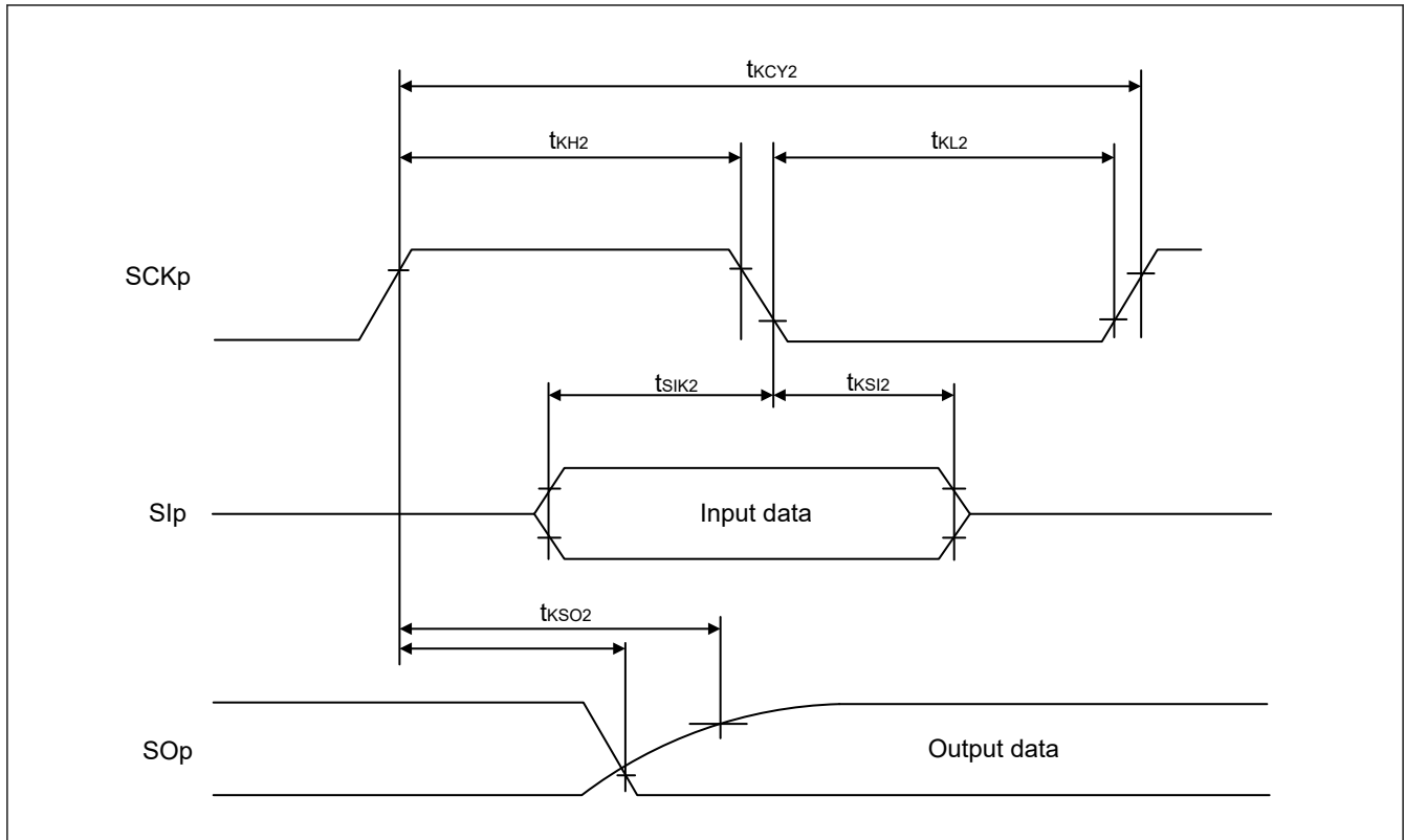
Figure 32.28 Timing of serial transfer in the simplified SPI communications in the slave mode with devices operating at different voltage levels when SCRmn.DCP[1:0] = 01b or 10b
