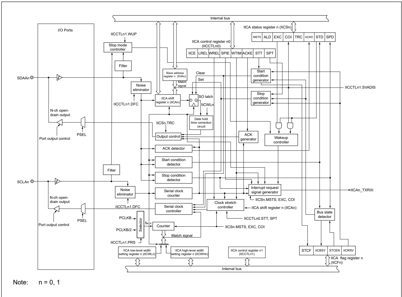
Figure 22.1 Block diagram of I 2 C bus interface
