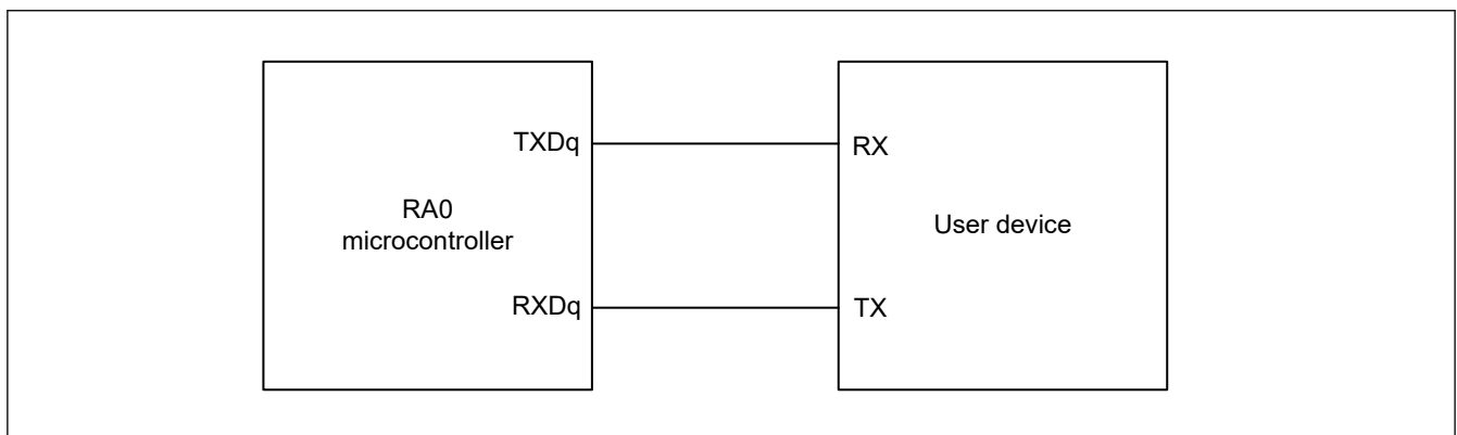
Figure 32.14 Connection in the UART communications with devices operating at same voltage levels
