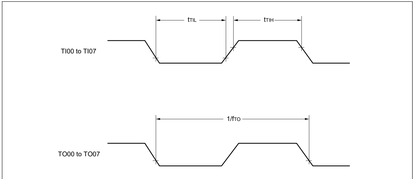
Figure 32.7 TI/TO timing
