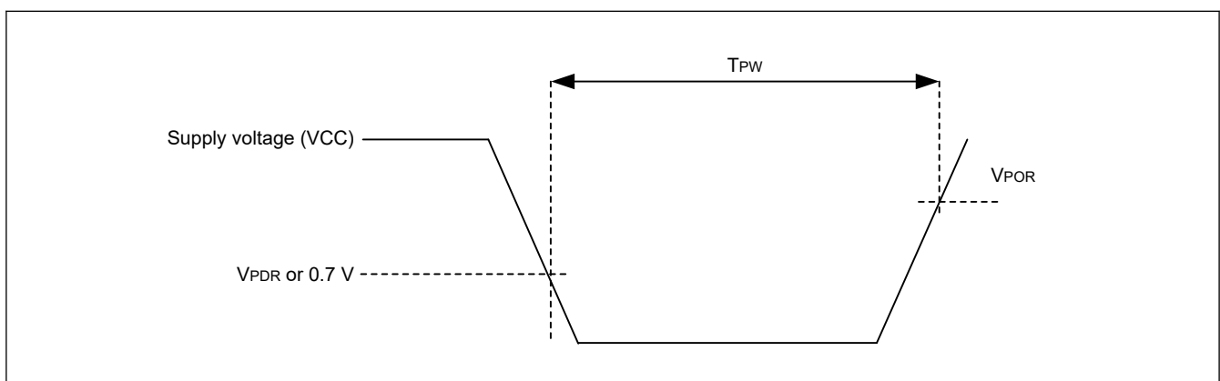
Figure 32.34 Minimum VCC pulse width
