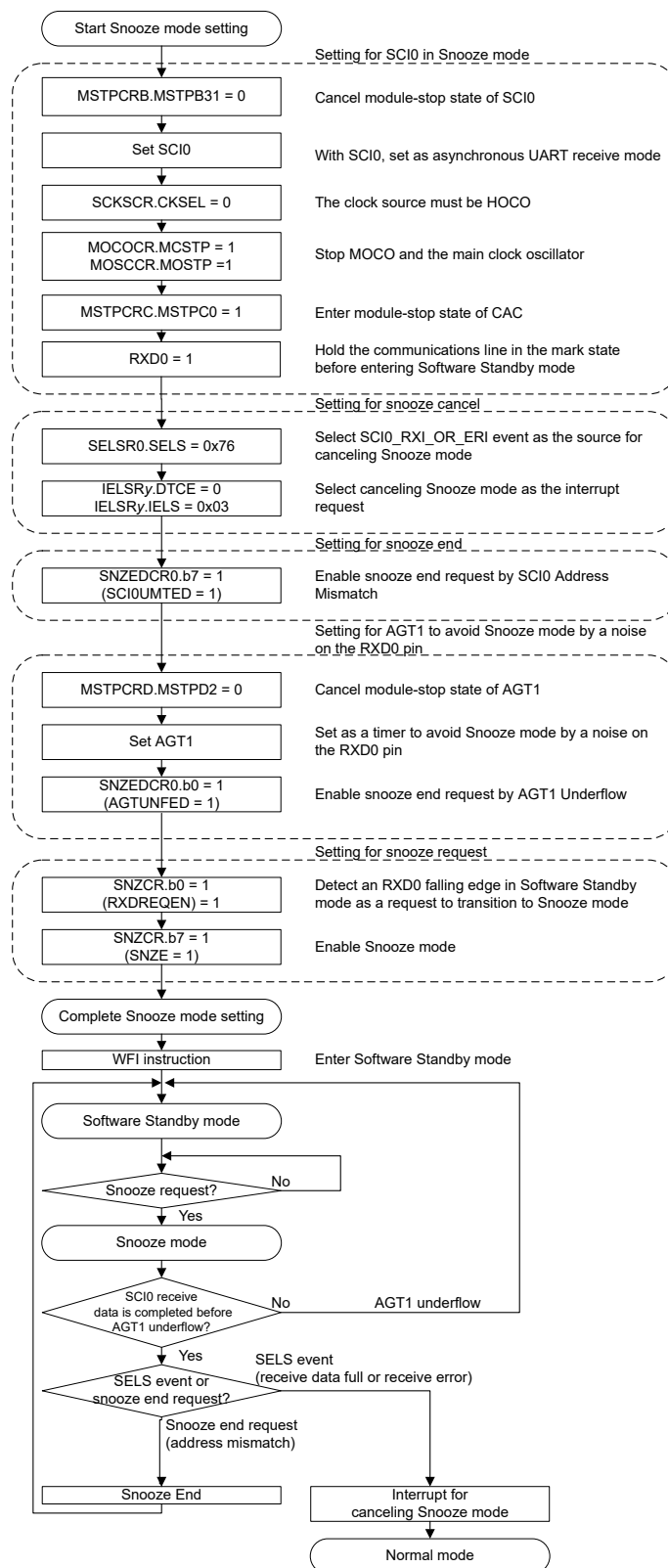
Figure 10.13 Setting example of using SCI0 in Snooze mode entry
