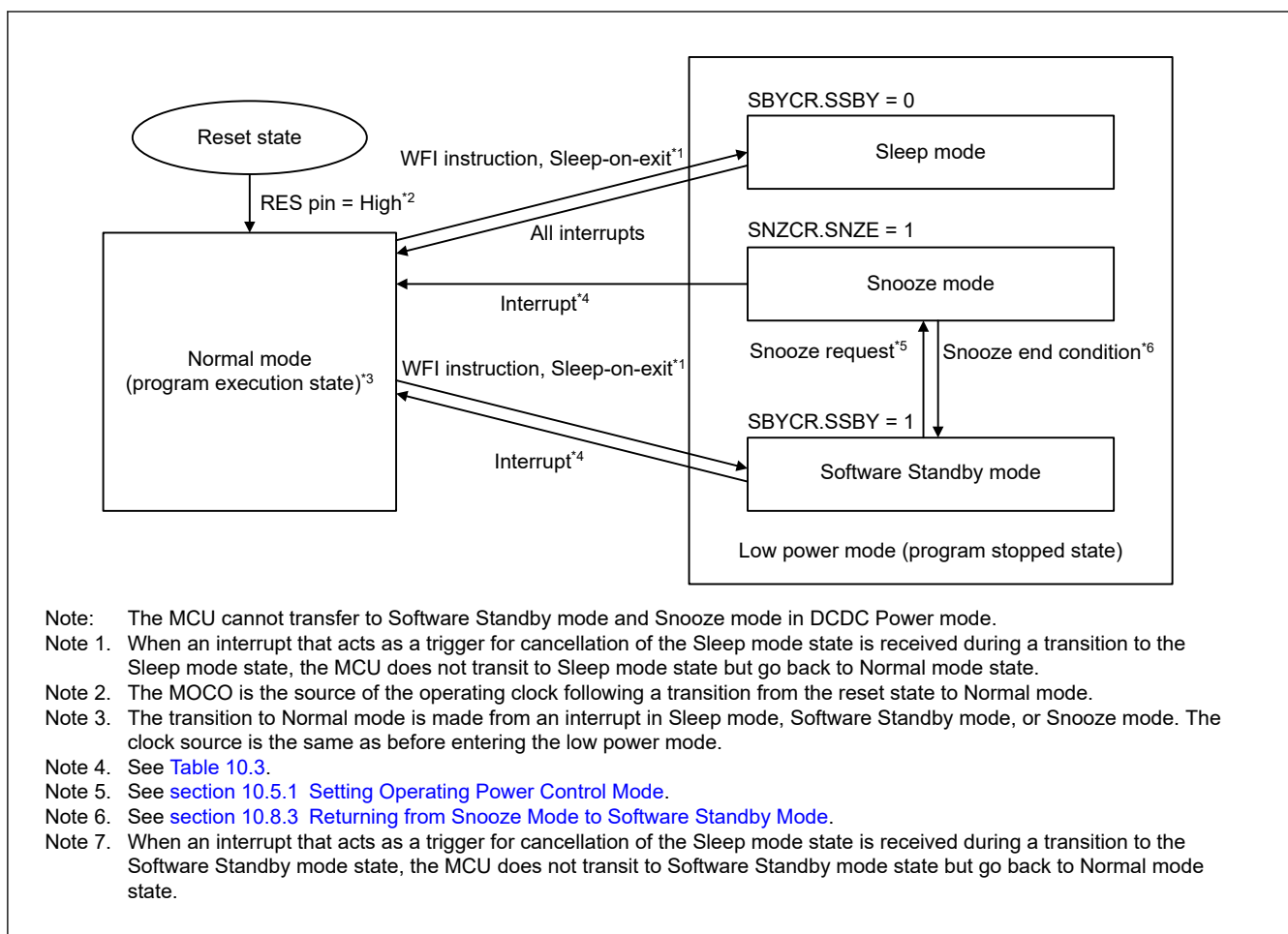
Figure 10.1 Low power mode transitions
