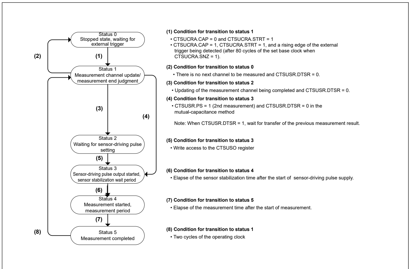
Figure 34.10 Status operation transitions
