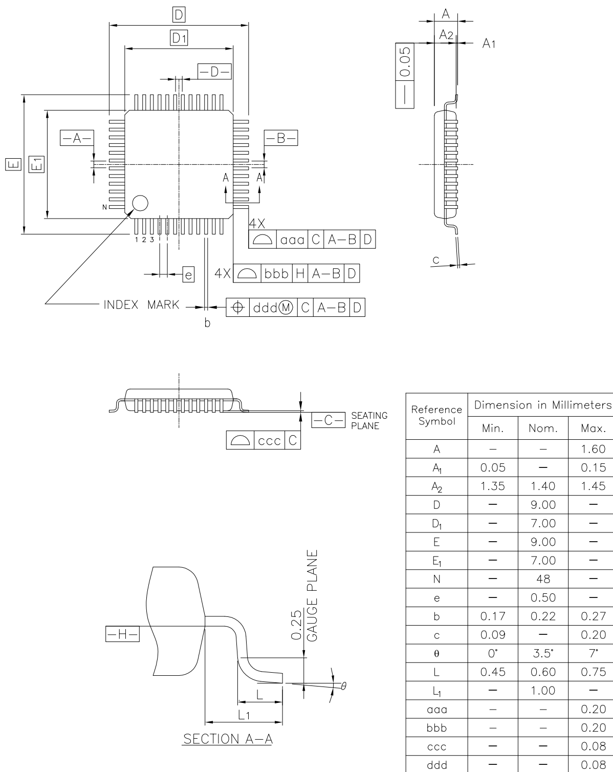
Figure A2.6 LQFP 48-pin (2)
