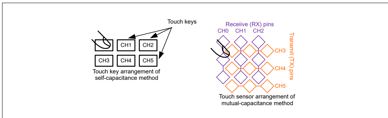
Figure 34.11 Overview of self-capacitance and mutual-capacitance methods
