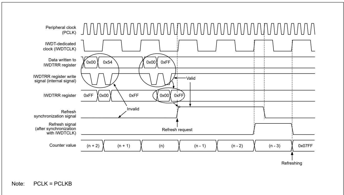
Figure 24.4 IWDTR refresh operation waveforms when OFS0.IWDTCKS[3:0] = 0000b, OFS0.IWDTTOPS[1:0] = 11b
