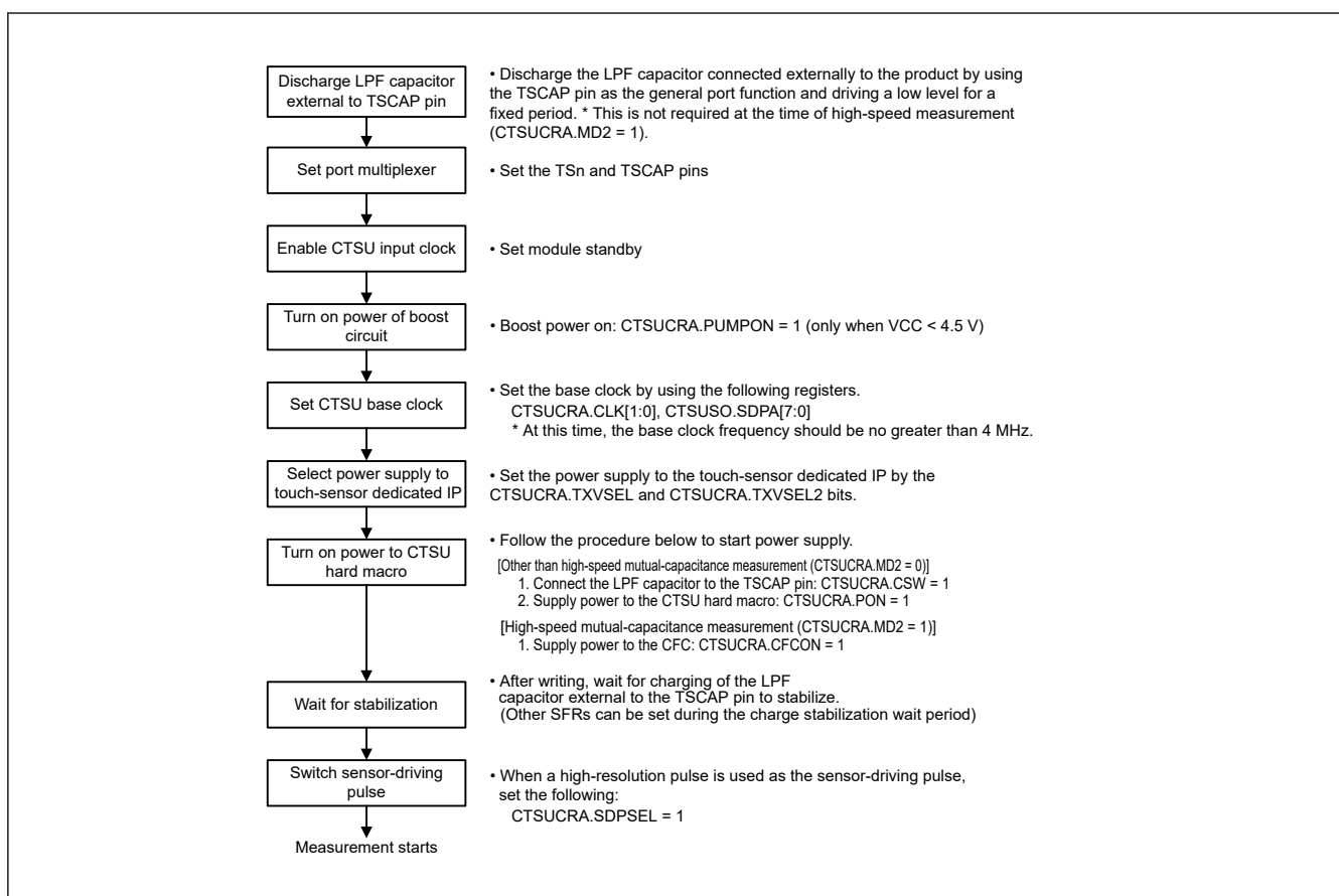
Figure 34.8 Initial setting flow of CTSU
