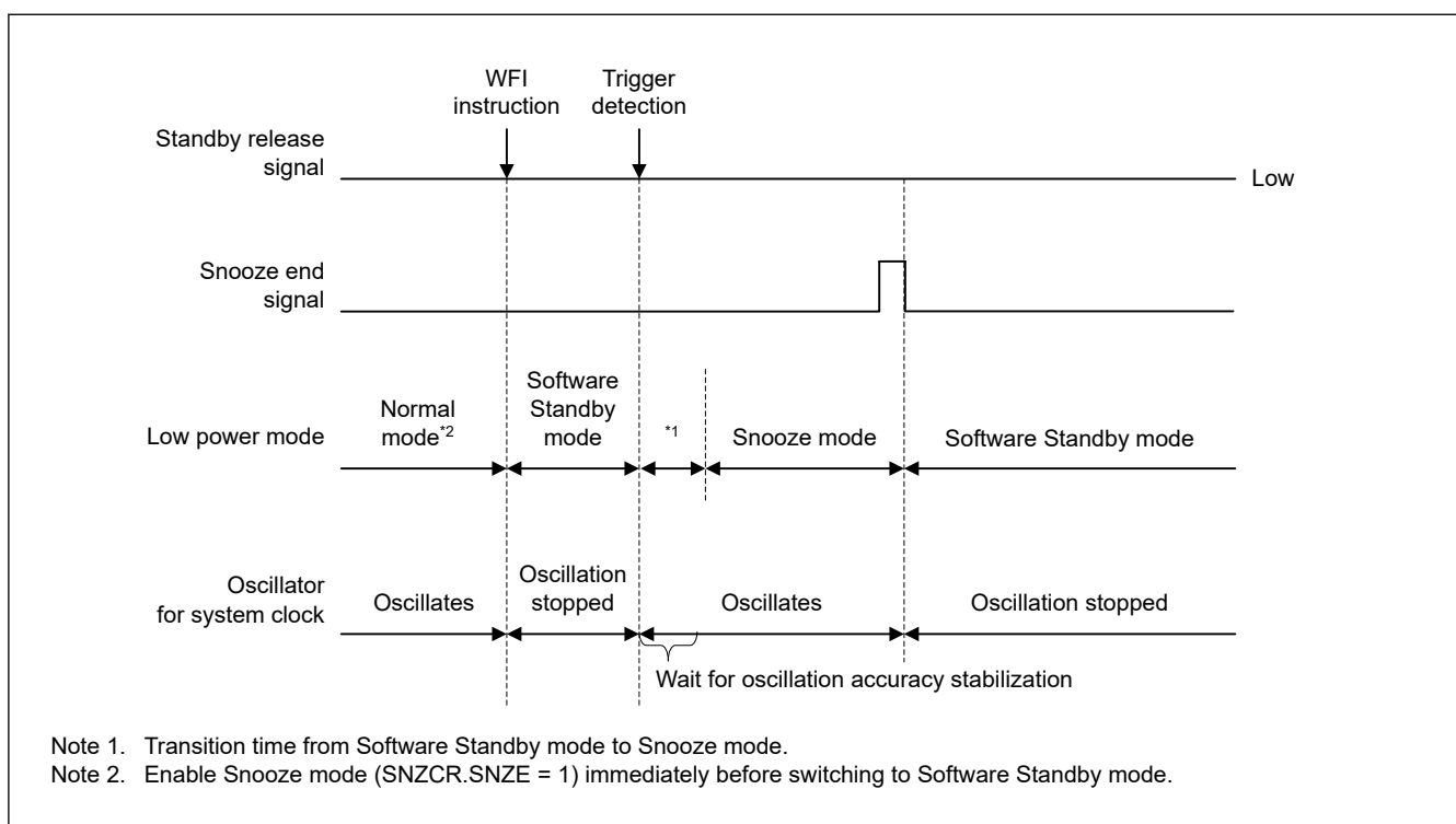
Figure 10.11 Canceling of Snooze mode when an interrupt request signal is not generated
