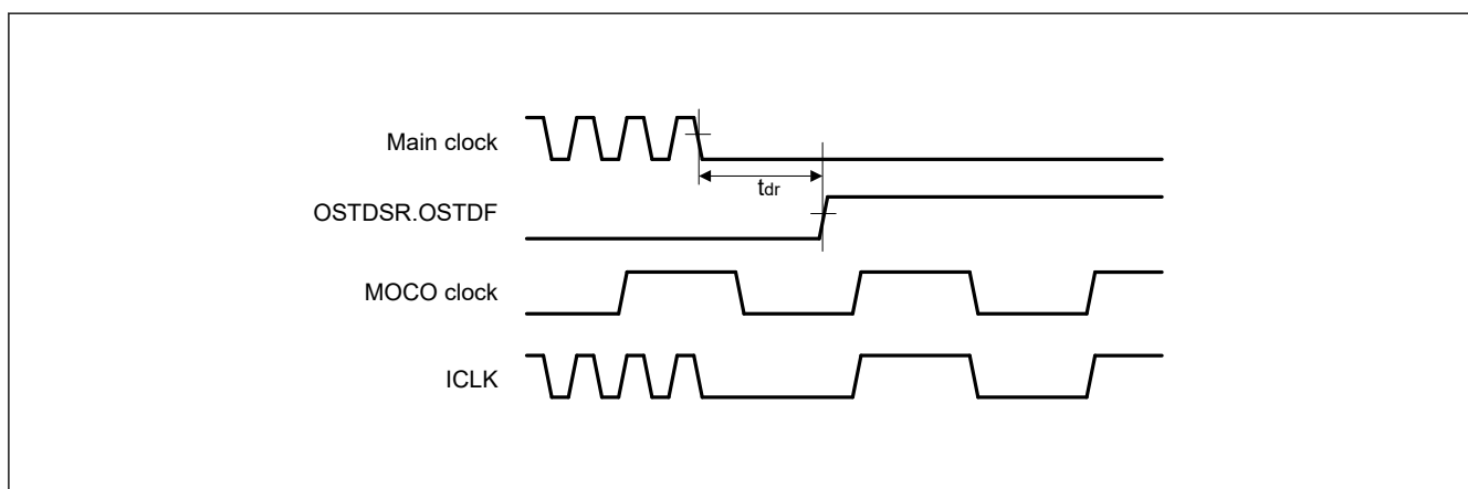
Figure 41.41 Oscillation stop detection timing
