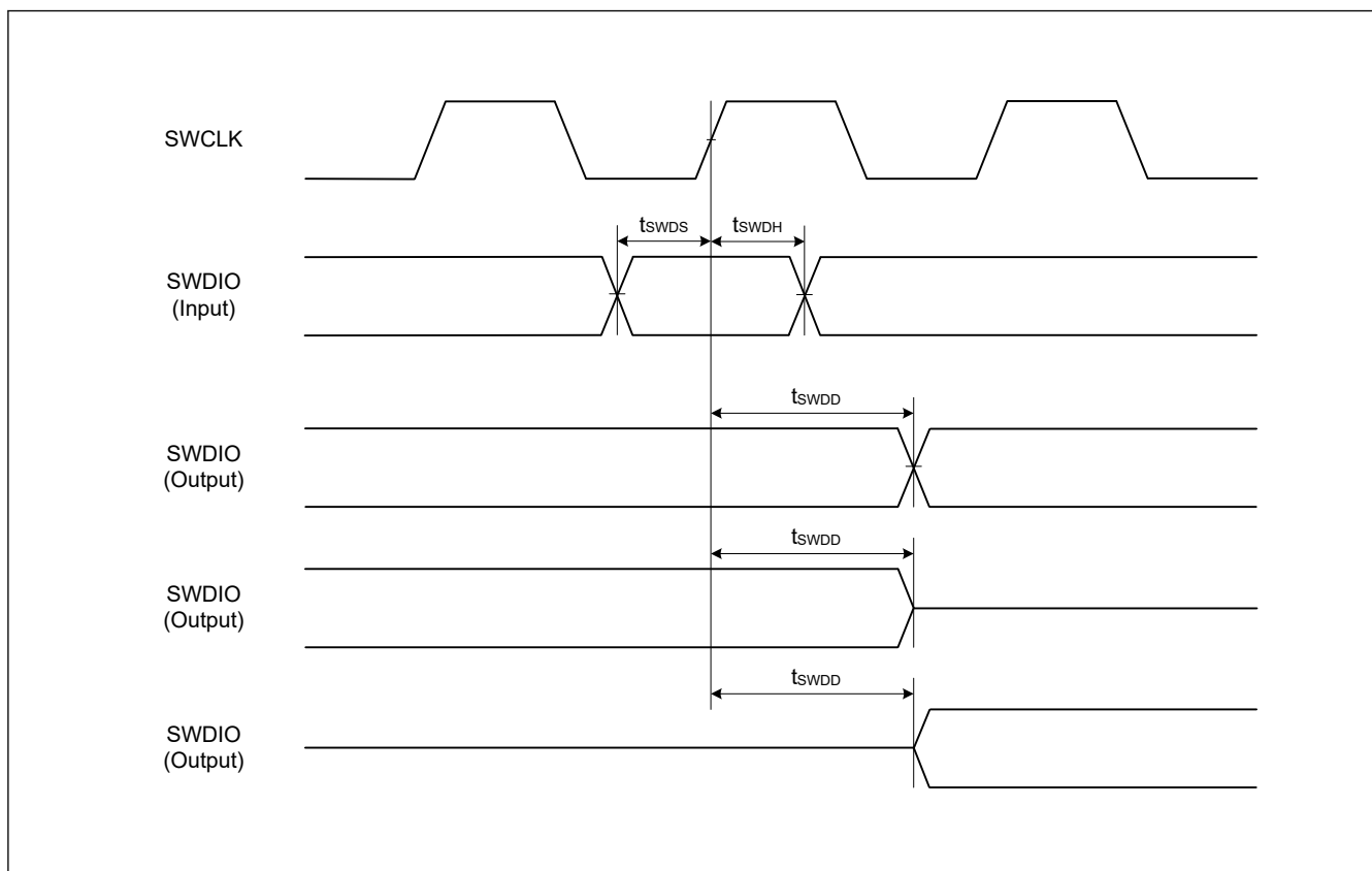
Figure 41.50 SWD input/output timing
