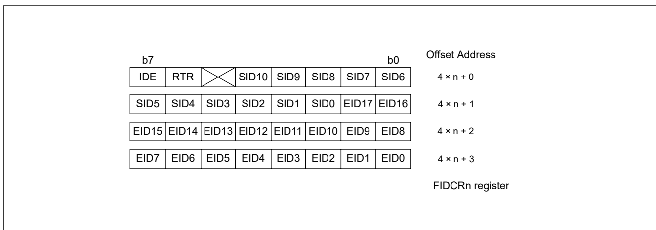
Figure 27.15 Structure of the FIDCRn registers (n = 0)
