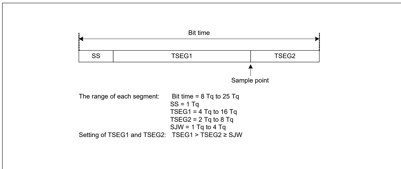
Figure 27.12 Bit timing
