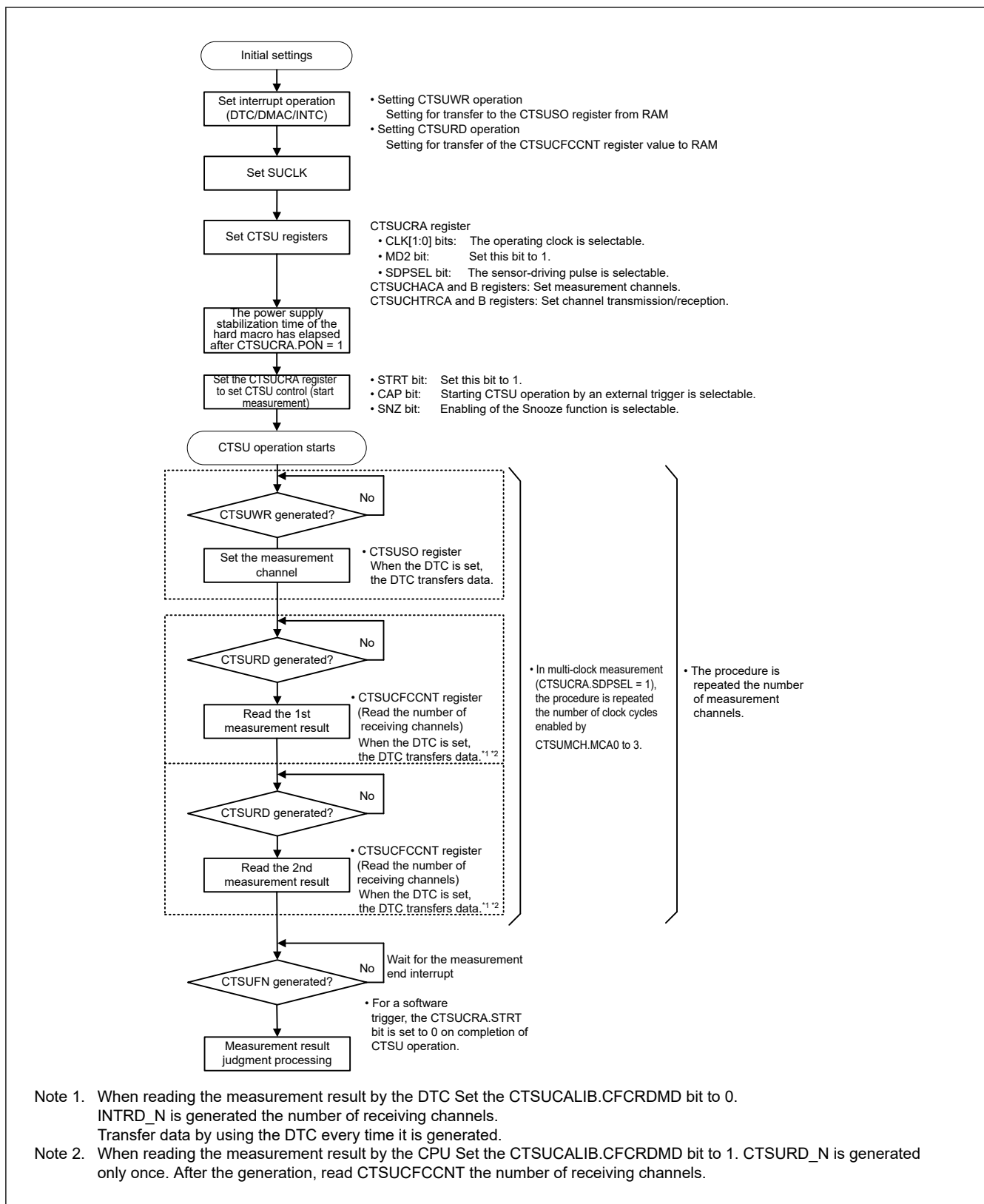
Figure 34.15 Software flow and operation example of high-speed measurement method
