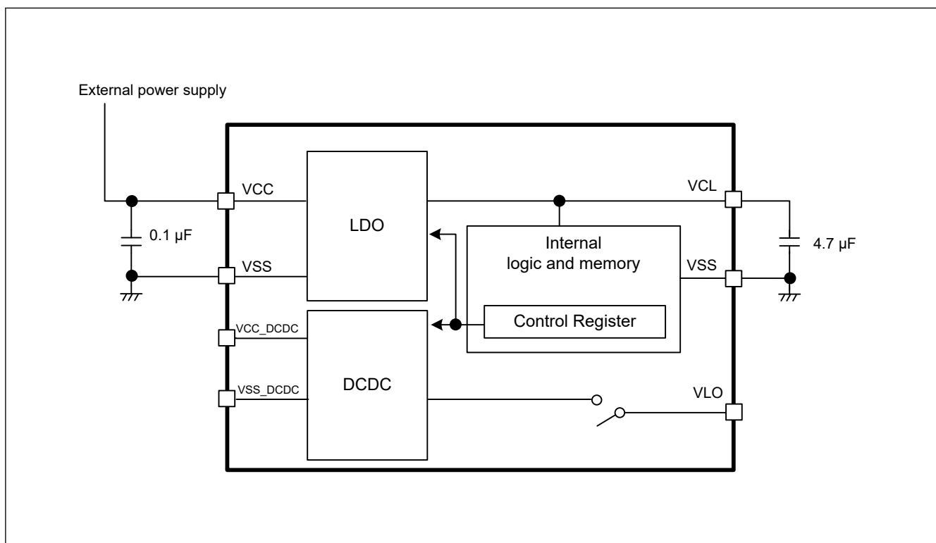
Figure 40.1 LDO settings
