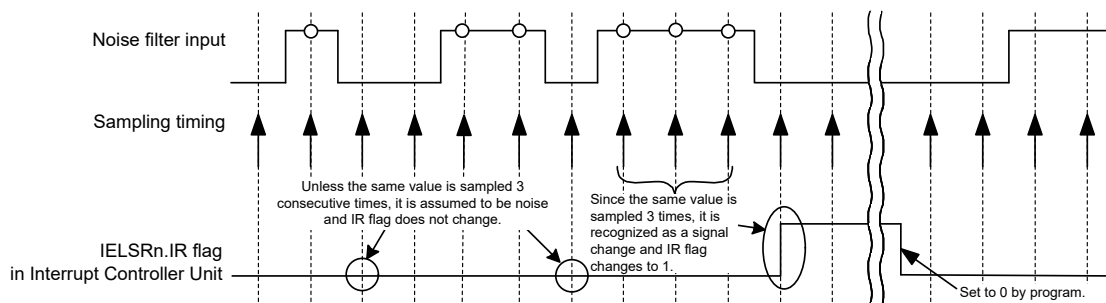
Figure 33.6 Noise filter and interrupt operation example
