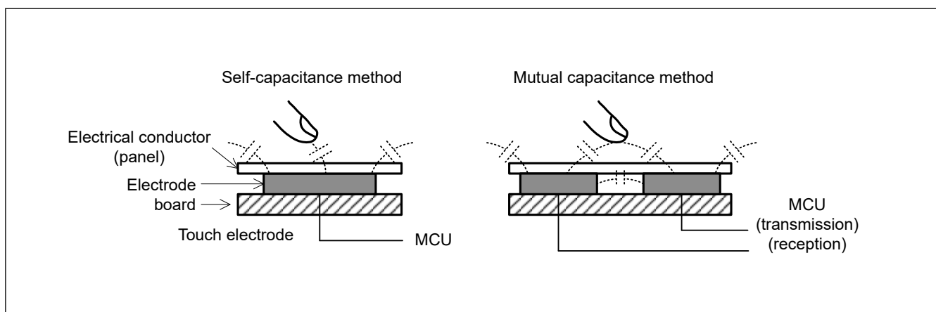
Figure 34.2 Self-capacitance and mutual capacitance methods
