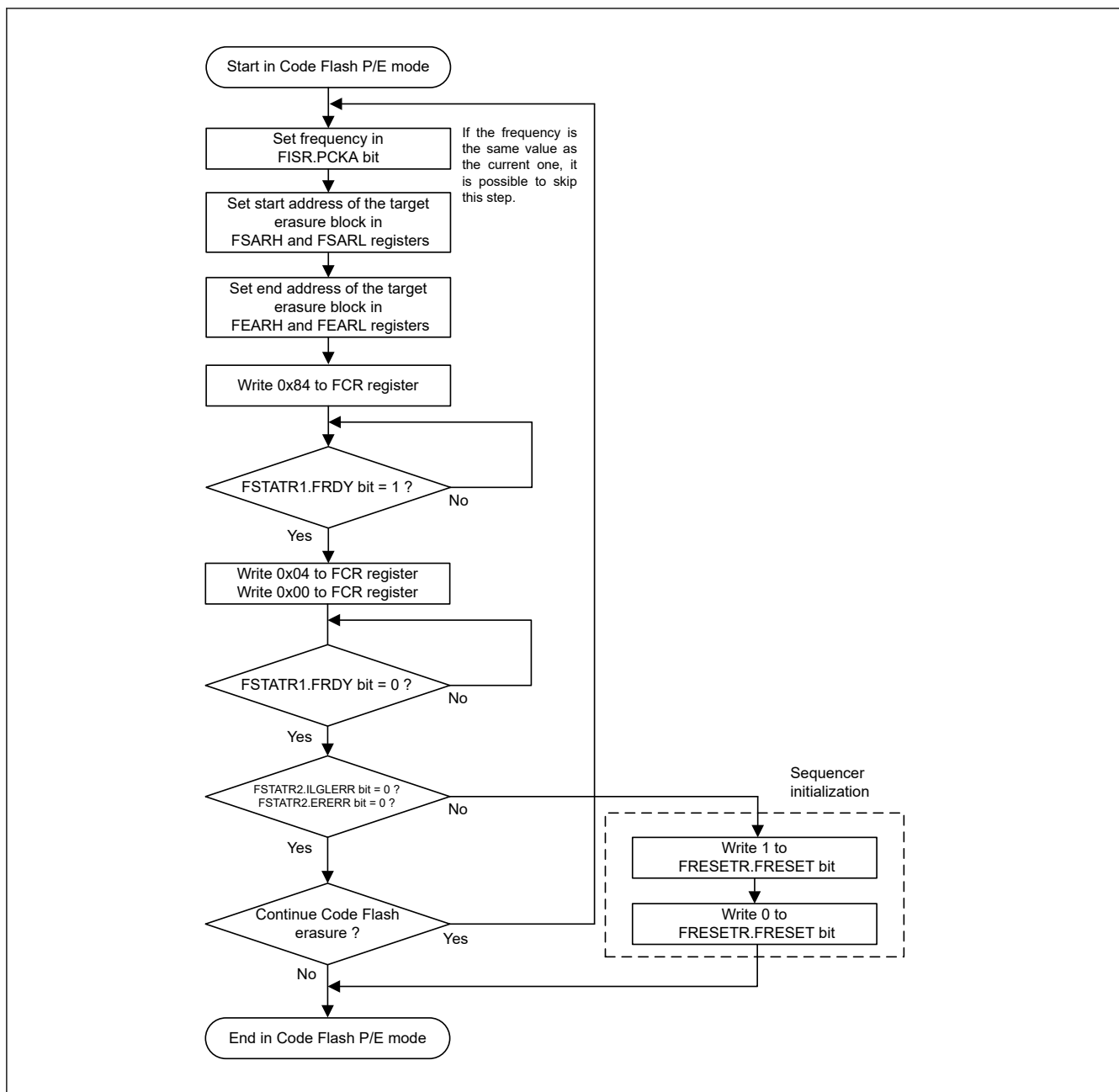
Figure 37.23 Flowchart for the code flash block erase procedure
