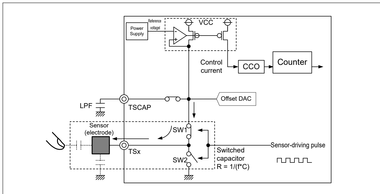
Figure 34.5 Self-capacitance charging operation
