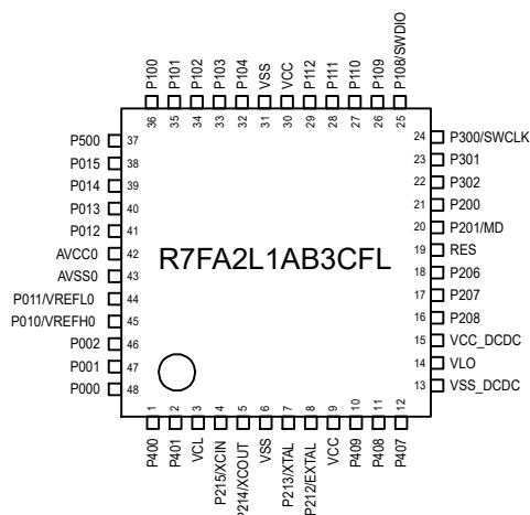
Figure 1.6 Pin assignment for LQFP 48-pin (top view)
