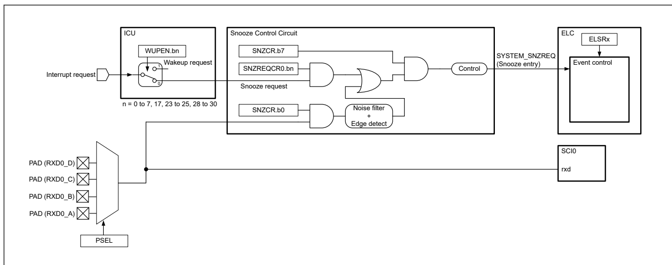
Figure 10.9 Snooze mode entry configuration
