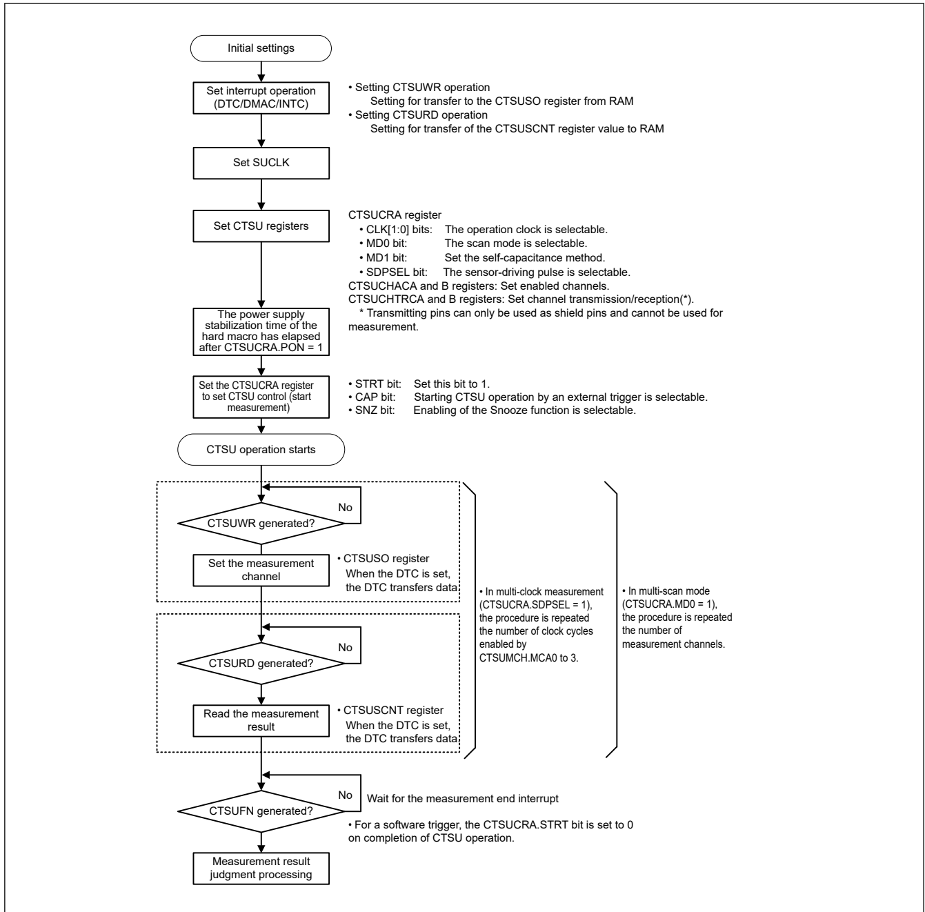
Figure 34.12 Software flow and operation example of self-capacitance method
