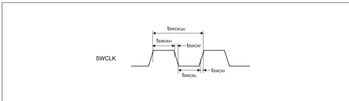
Figure 41.49 SWD SWCLK timing
