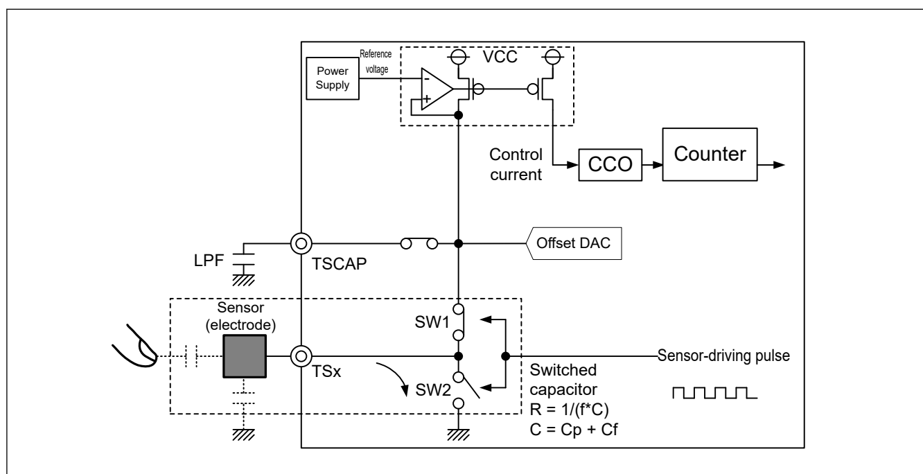
Figure 34.6 Self-capacitance discharging operation
