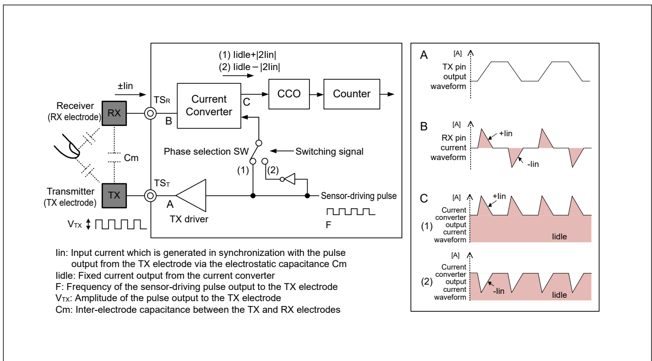
Figure 34.14 Measurement block circuit for high-speed measurement
