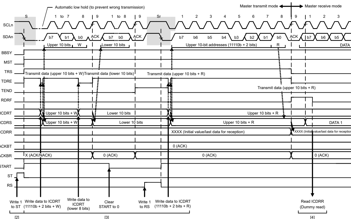
Figure 26.13 Master receive operation timing (2) with 10-bit address format when RDRFS = 0
