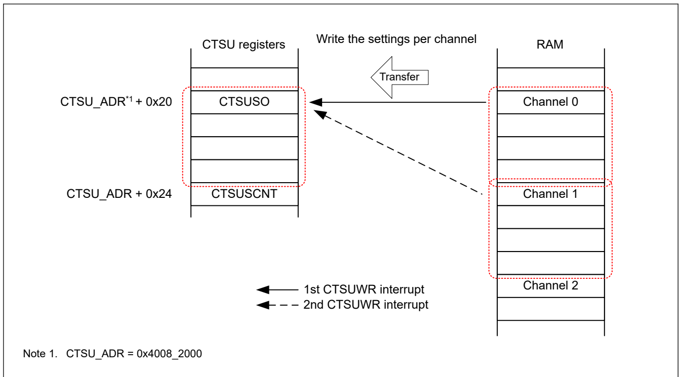
Figure 34.16 Example of DTC transfer operation using CTSUWR interrupt
