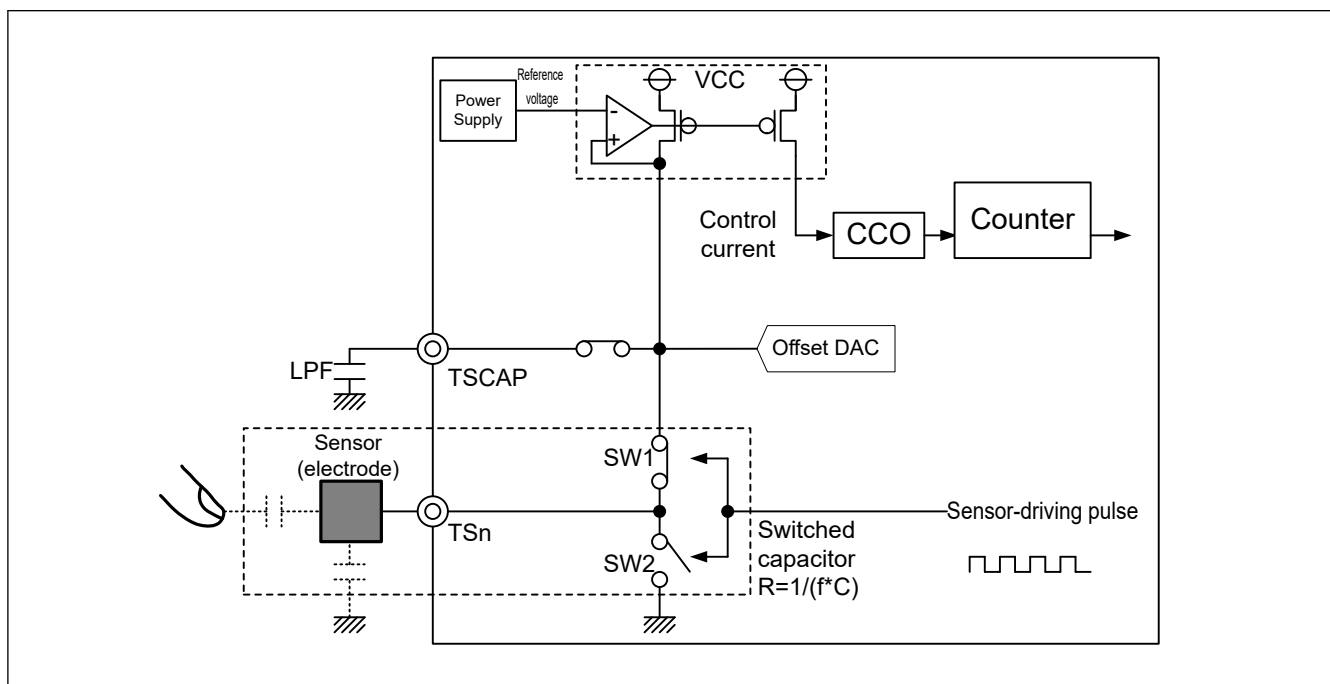
Figure 34.4 Self-capacitance measurement block circuit
