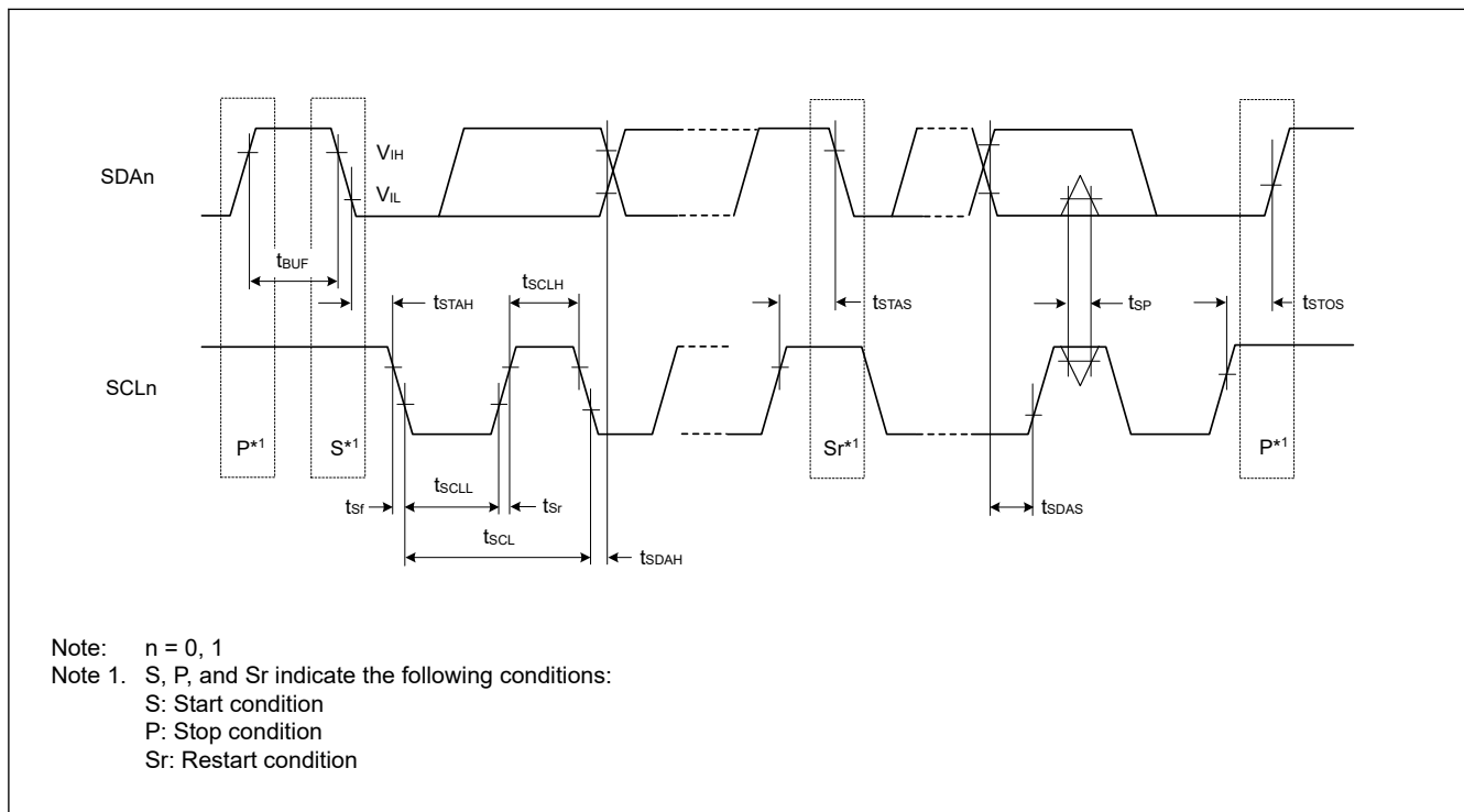
Figure 41.35 I²C bus interface input/output timing
