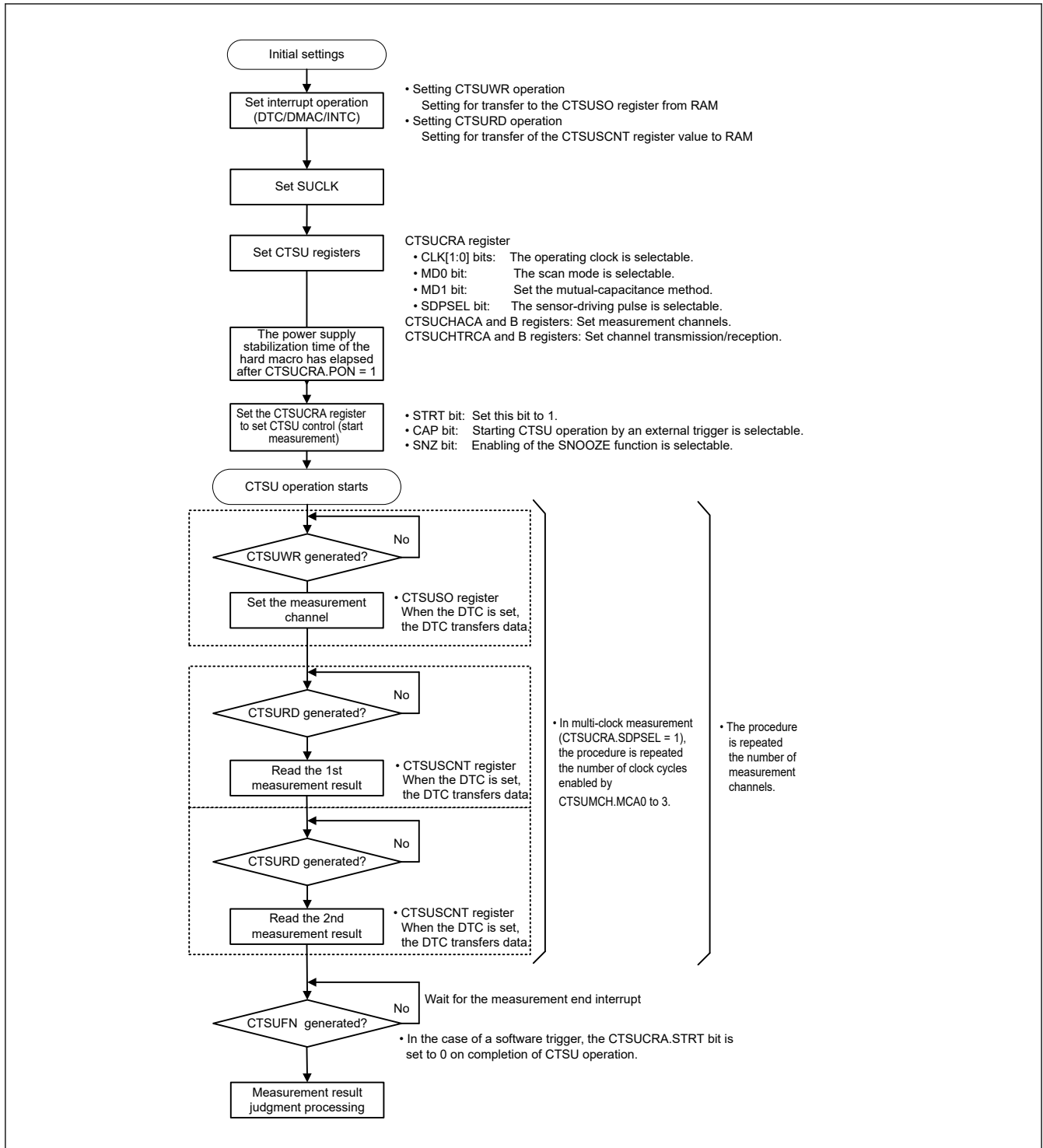
Figure 34.13 Software flow and operation example of mutual capacitance method
