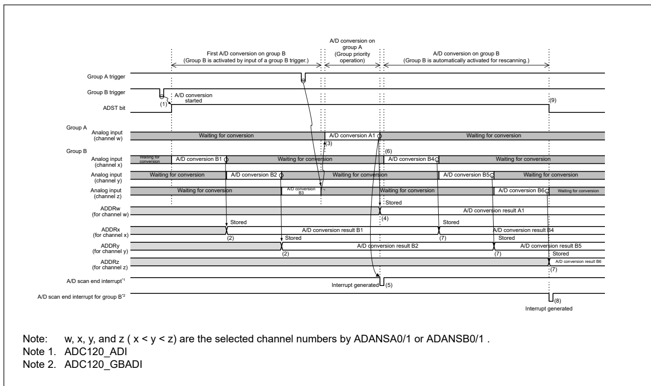
Figure 30.17 Example of group priority operation 1-1: Group A trigger input during group B scanning when rescanning is enabled (when ADGSPCR.GBRSCN = 1, ADGSPCR.GBRP = 0)
