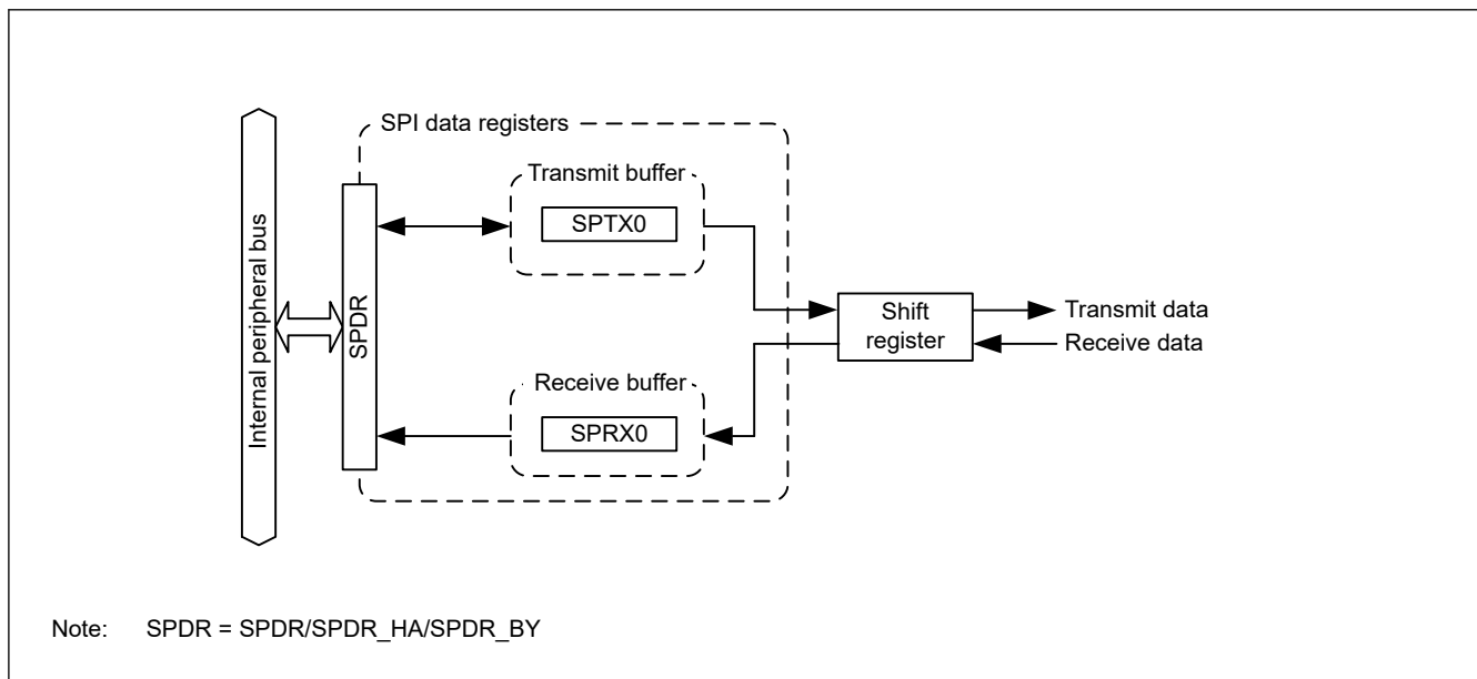
Figure 28.2 Configuration of SPDR/SPDR_HA/SPDR_BY
