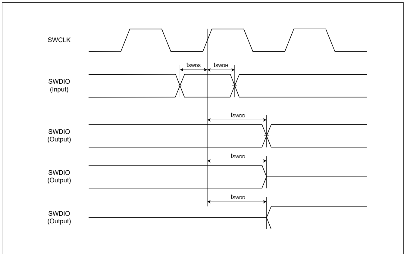
Figure 41.50 SWD input/output timing
