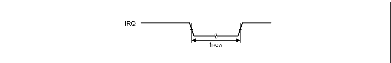
Figure 41.13 IRQ interrupt input timing
