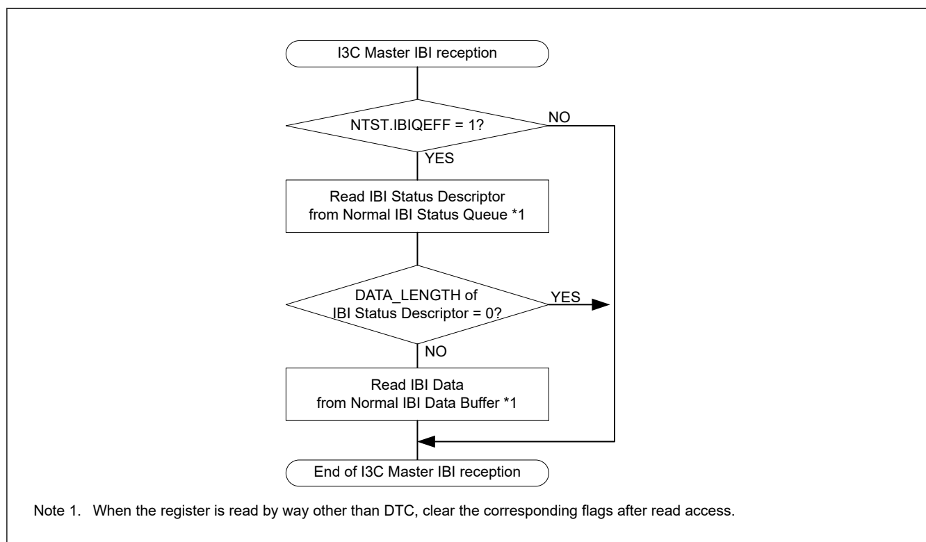
Figure 28.108 Example flowchart of I3C master IBI reception
