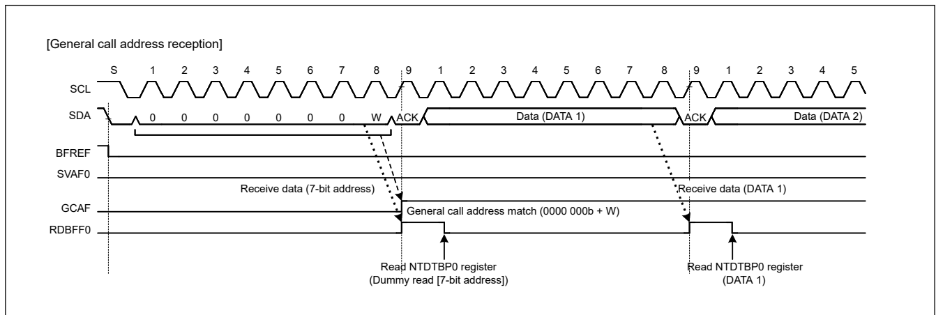
Figure 28.60 Timing of GCAF flag setting during reception of general call address
