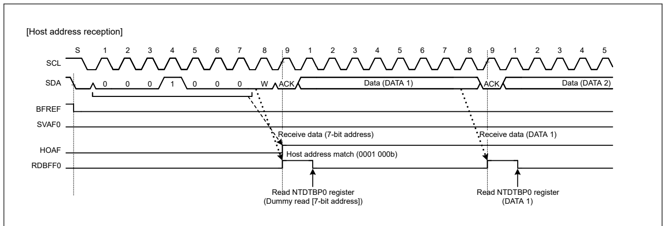
Figure 28.62 HOAF flag set timing during reception of host address
