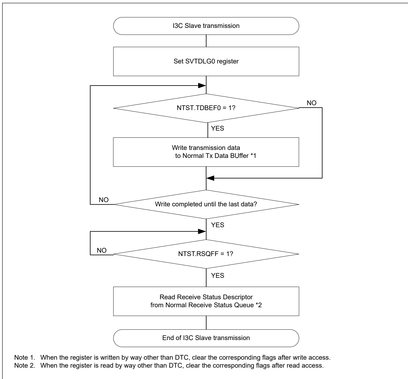
Figure 28.111 Example flowchart of I3C slave transmission (normal FIFO buffer transfer)
