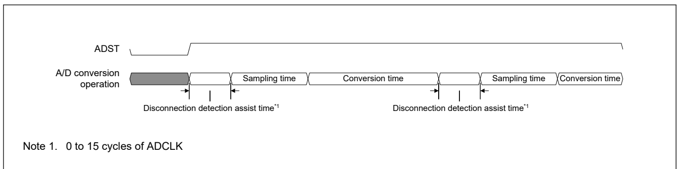
Figure 34.27 Operation of A/D conversion when disconnection detection assist function is used
