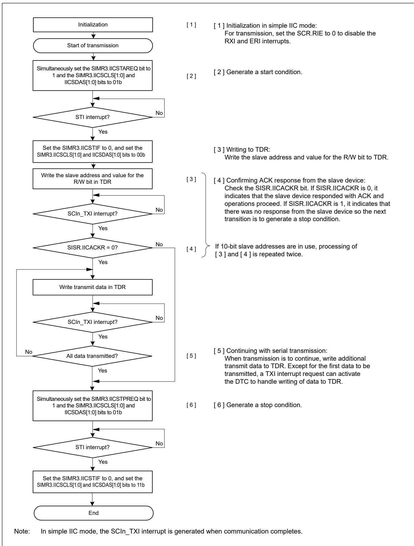
Figure 27.65 Example flow of master transmission in simple IIC mode with transmission interrupts and reception interrupts
