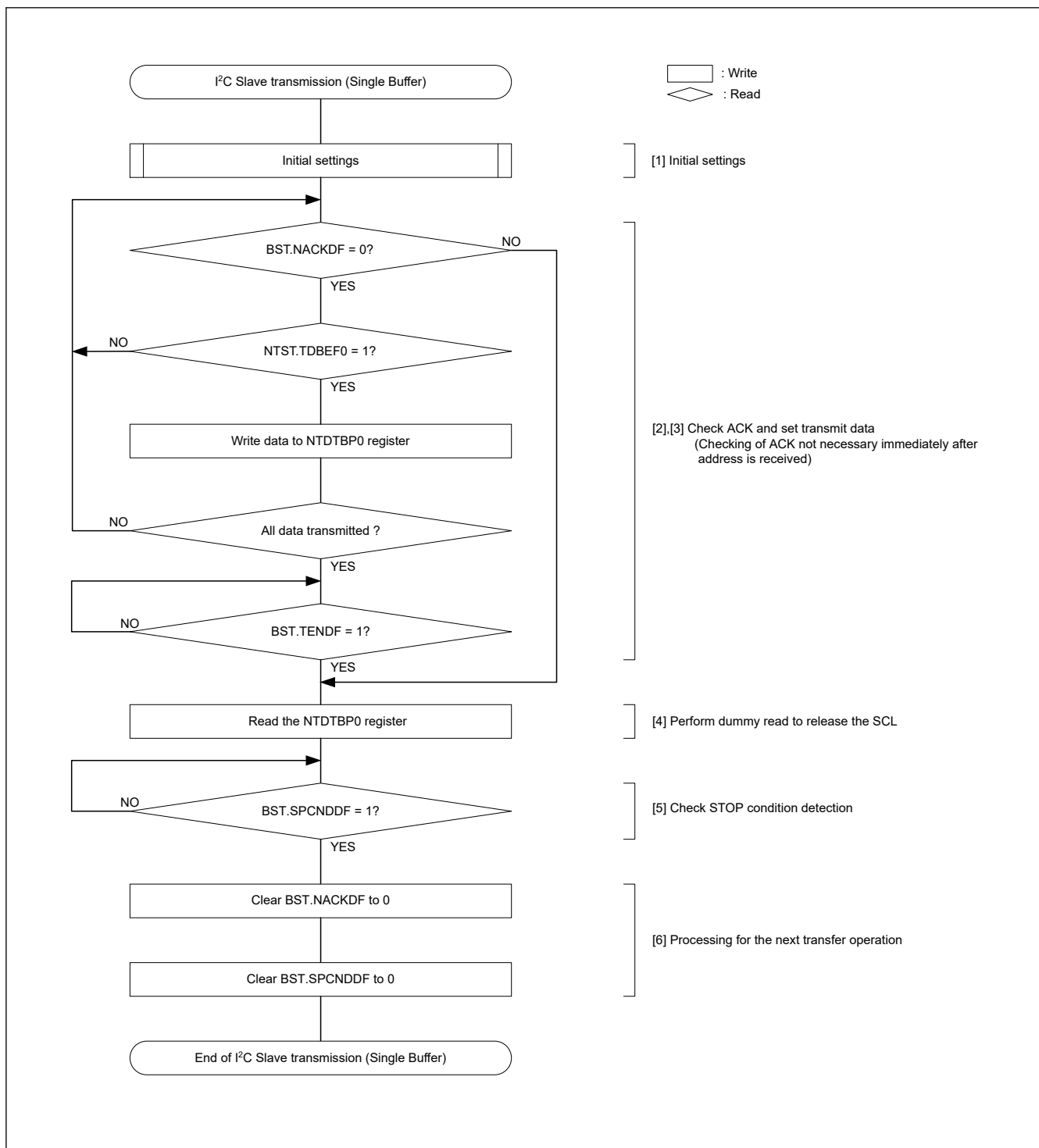
Figure 28.109 Example flowchart of I 2 C slave transmission (single buffer transfer)
