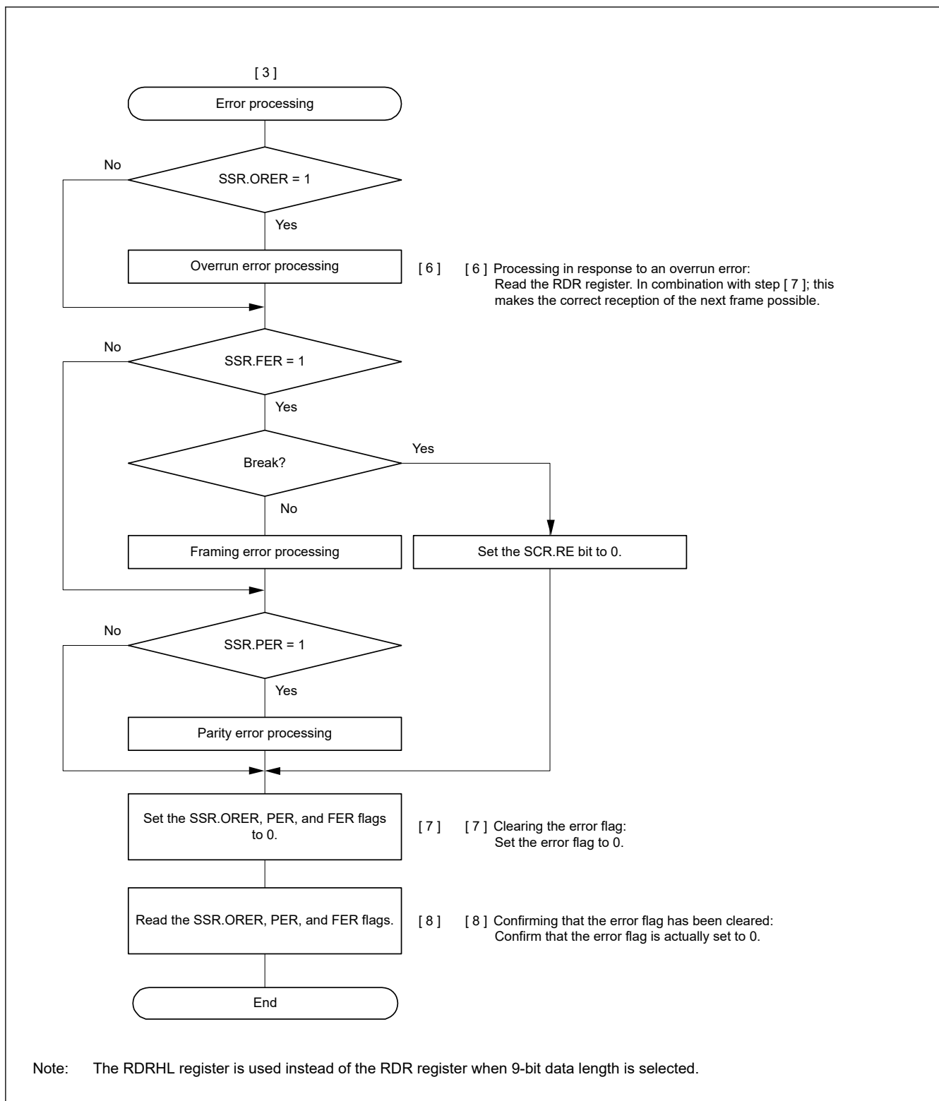
Figure 27.19 Example flow of serial reception in asynchronous mode (FIFO not selected and address matching enabled) (3)
