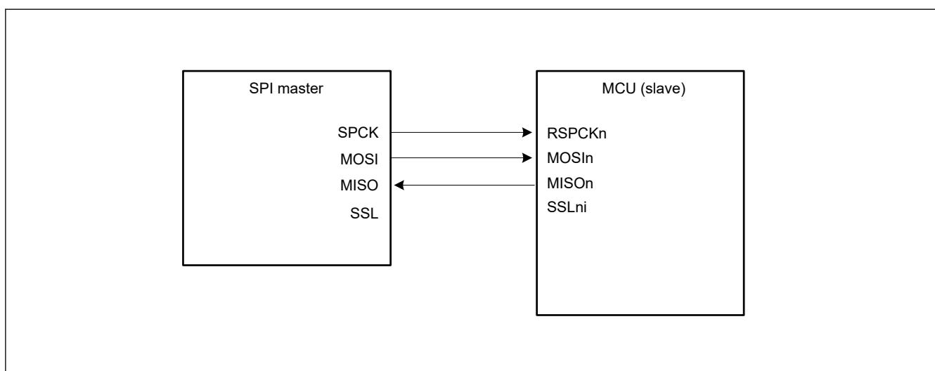
Figure 30.12 Clock synchronous master/slave configuration example with the MCU as a slave and CPHA = 1
