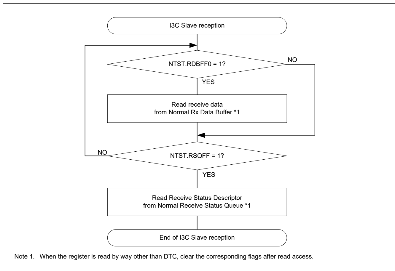
Figure 28.113 Example flowchart of I3C slave reception (normal FIFO buffer transfer)
