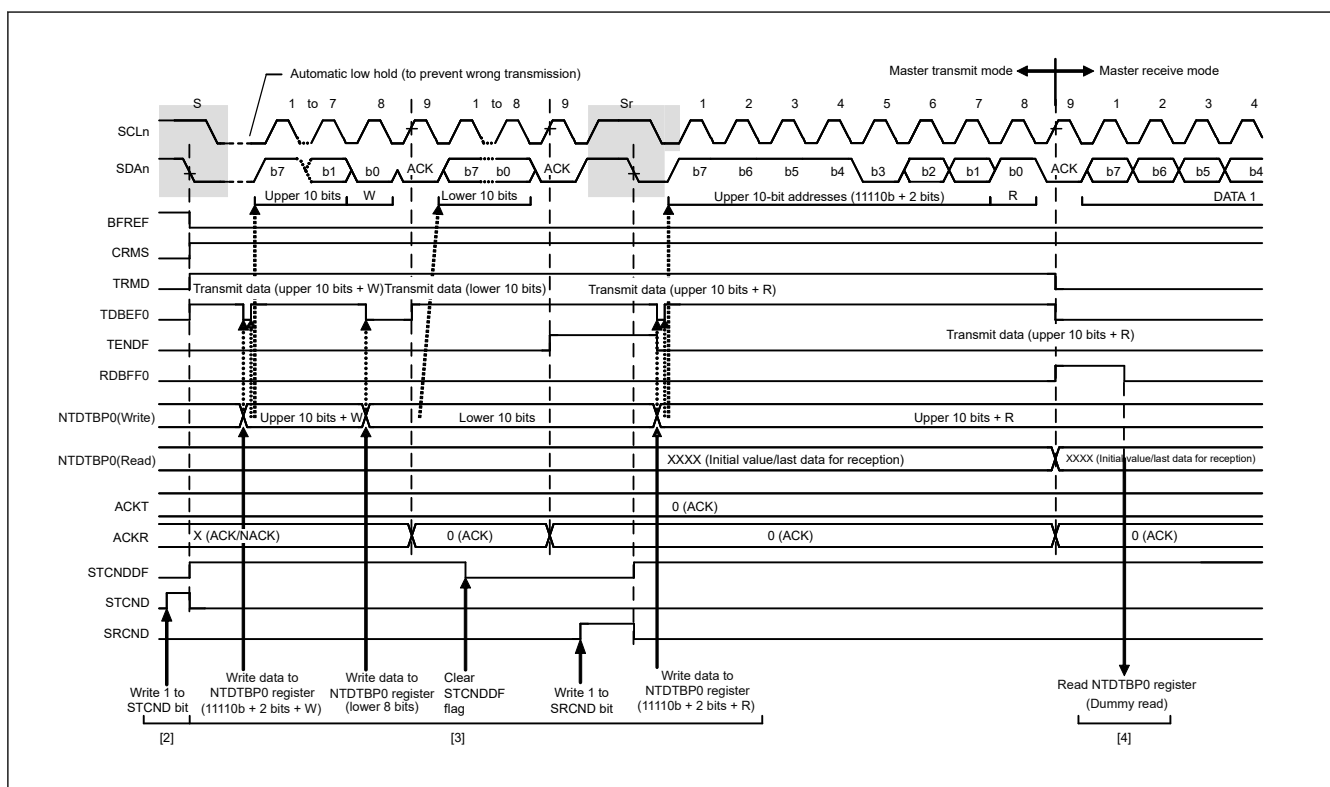
Figure 28.10 Master receive operation timing (2) (10-bit address format, when ACKTWE = 0)
