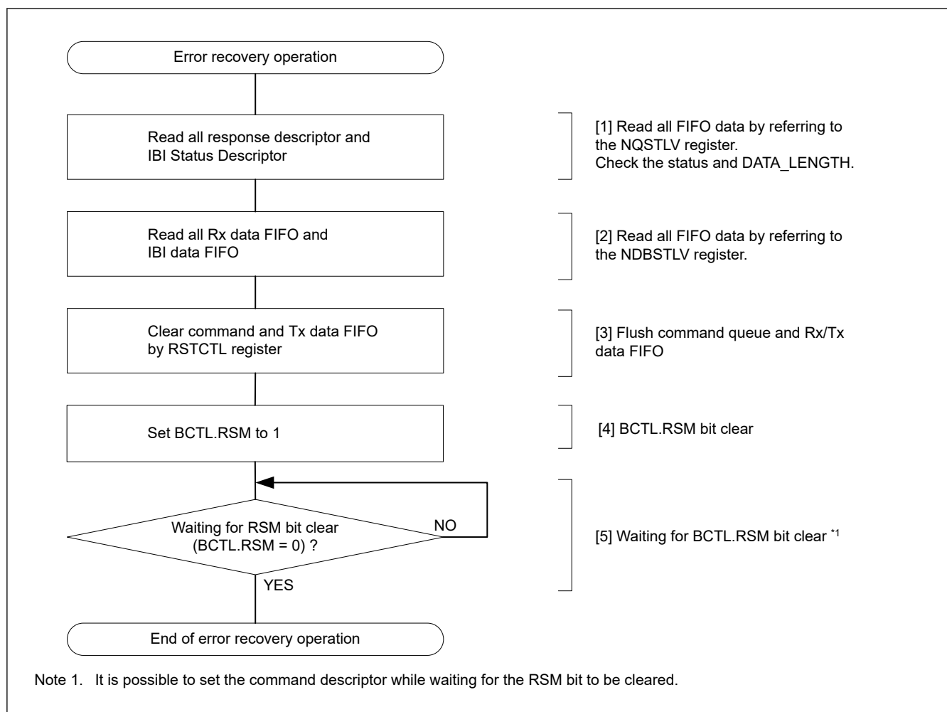
Figure 28.95 Example flowchart of an error recovery operation for I3C master
