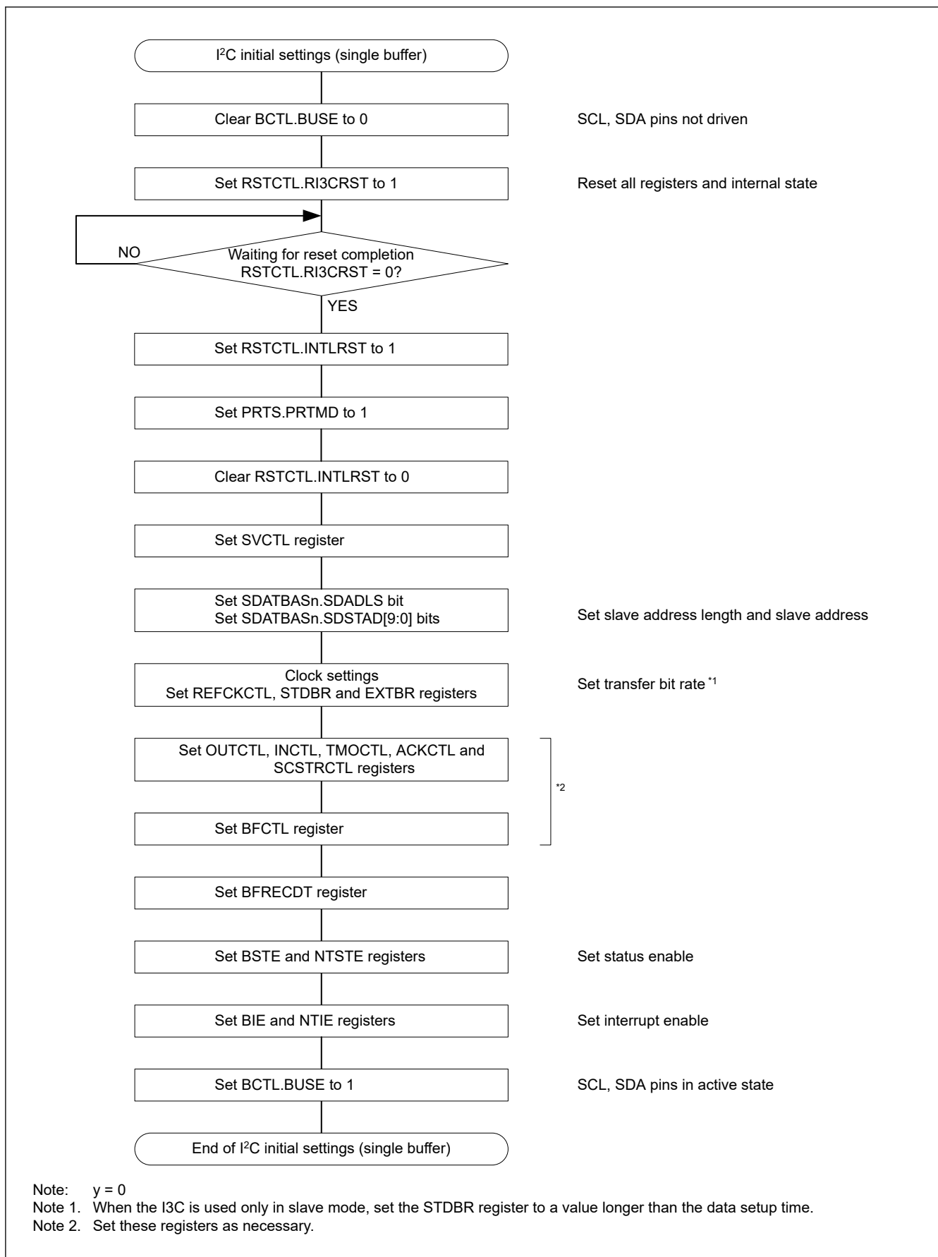
Figure 28.100 Example flowchart of I2C initialization (single buffer transfer)
