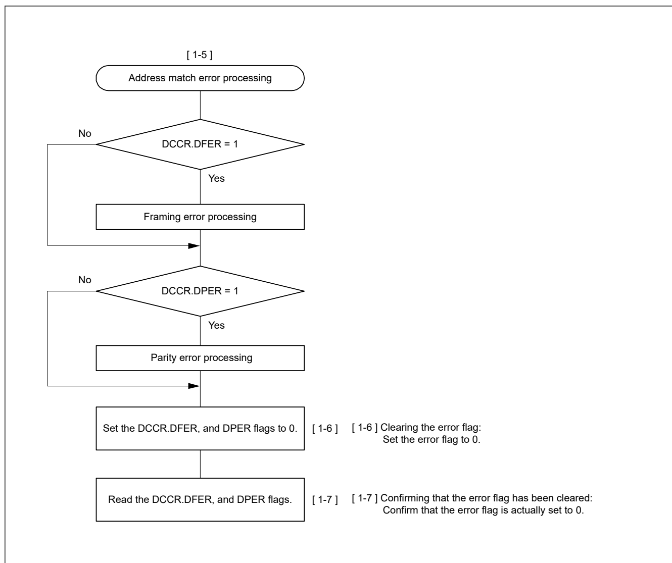
Figure 27.24 Example flow of serial reception in asynchronous mode (FIFO selected and address matching enabled) (2)
