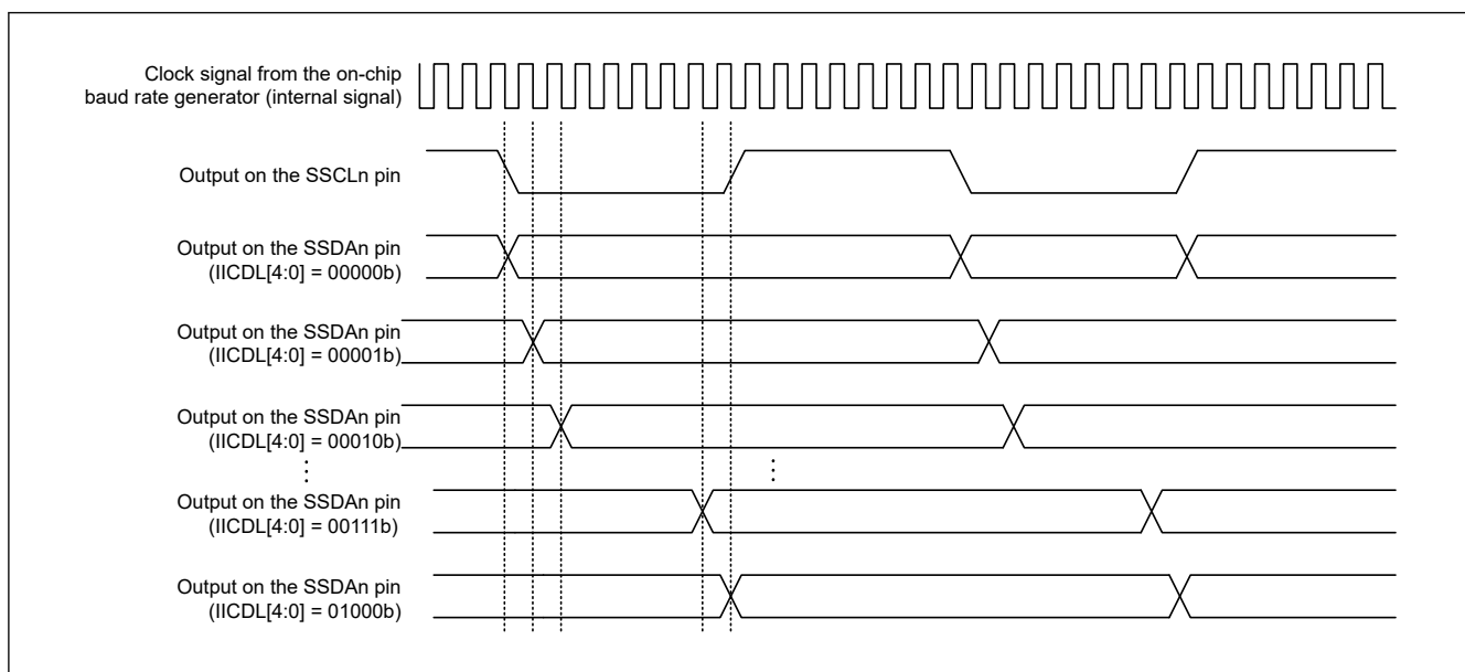
Figure 27.62 Timing of delays in SDAn output
