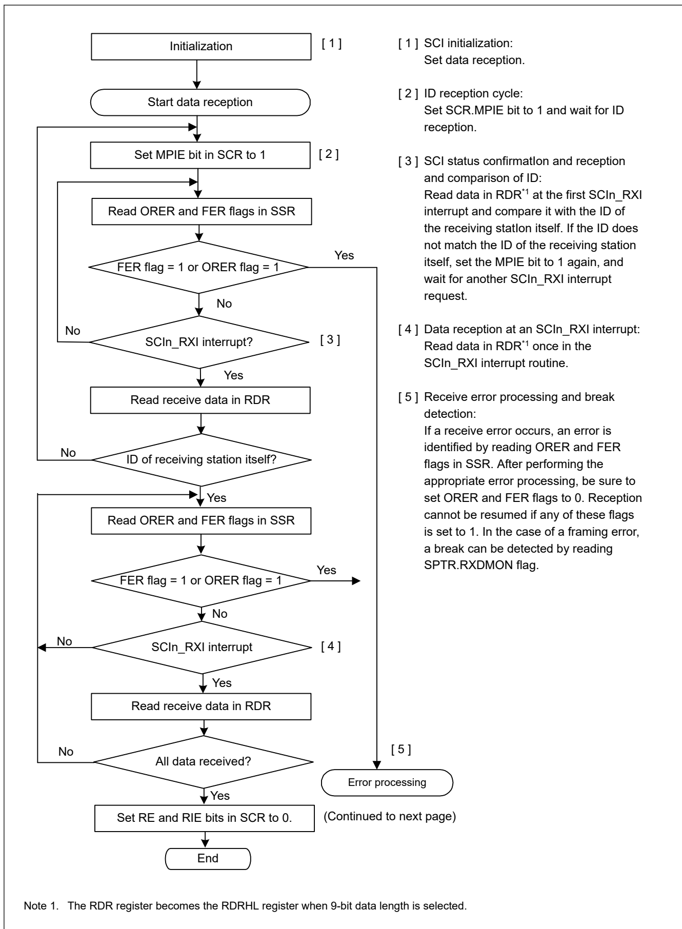
Figure 27.31 Example flow of multi-processor serial reception with non-FIFO selected (1)
