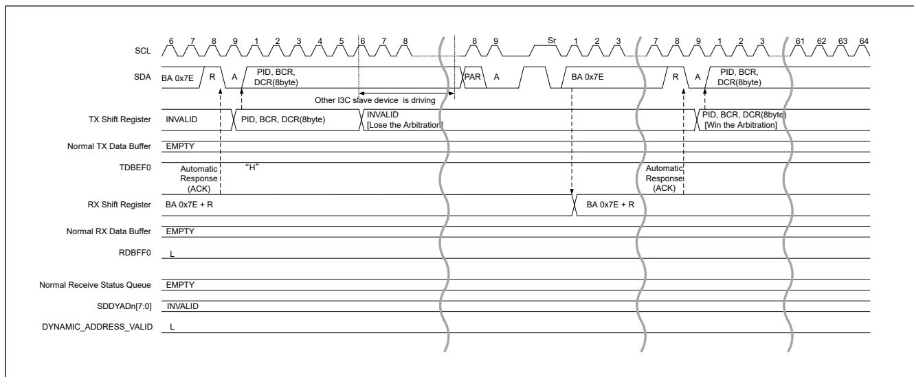
Figure 28.32 Dynamic address assign procedure (ENTDAA CCC) timing (2/3)
