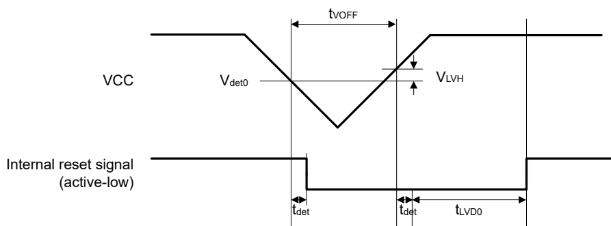
Figure 41.59 Voltage detection circuit timing ( V_{det0} )
