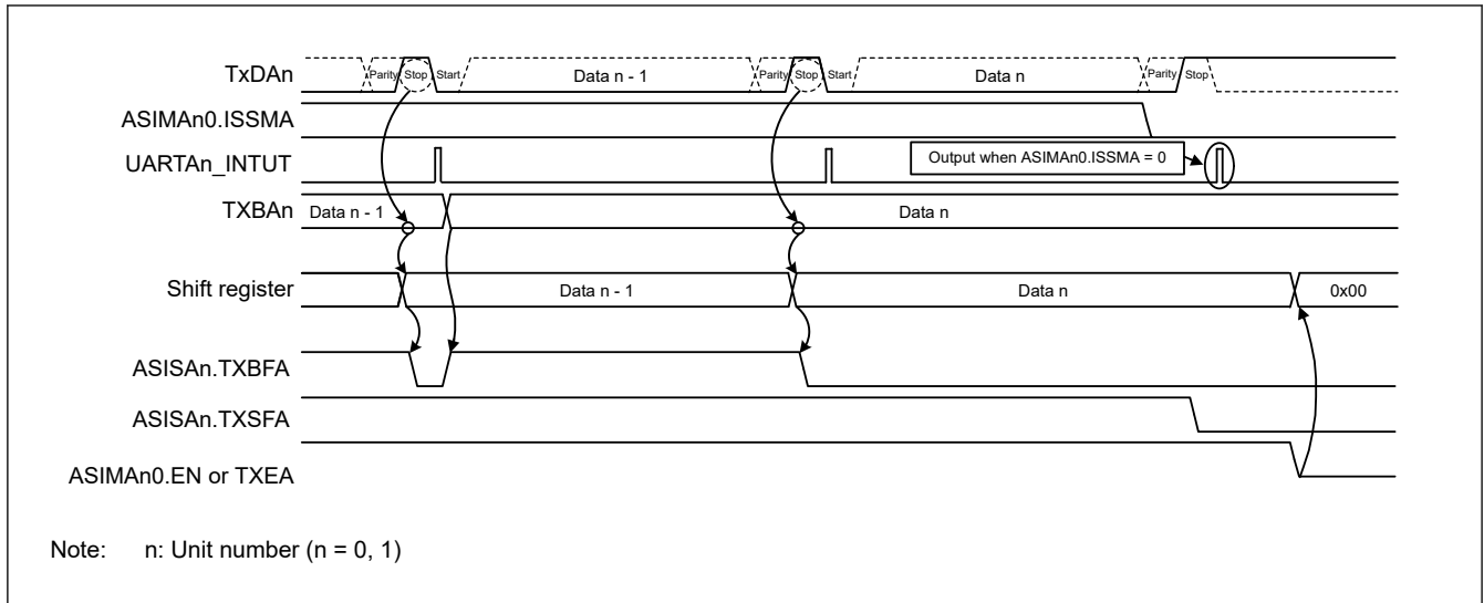
Figure 31.6 Timing when continuous transmission is completed
