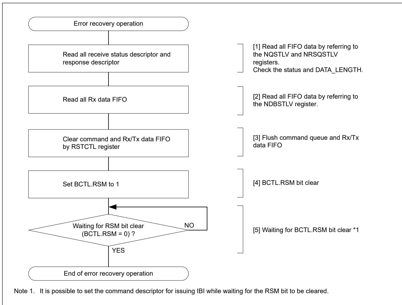
Figure 28.96 Example flowchart of an error recovery operation for I3C slave
