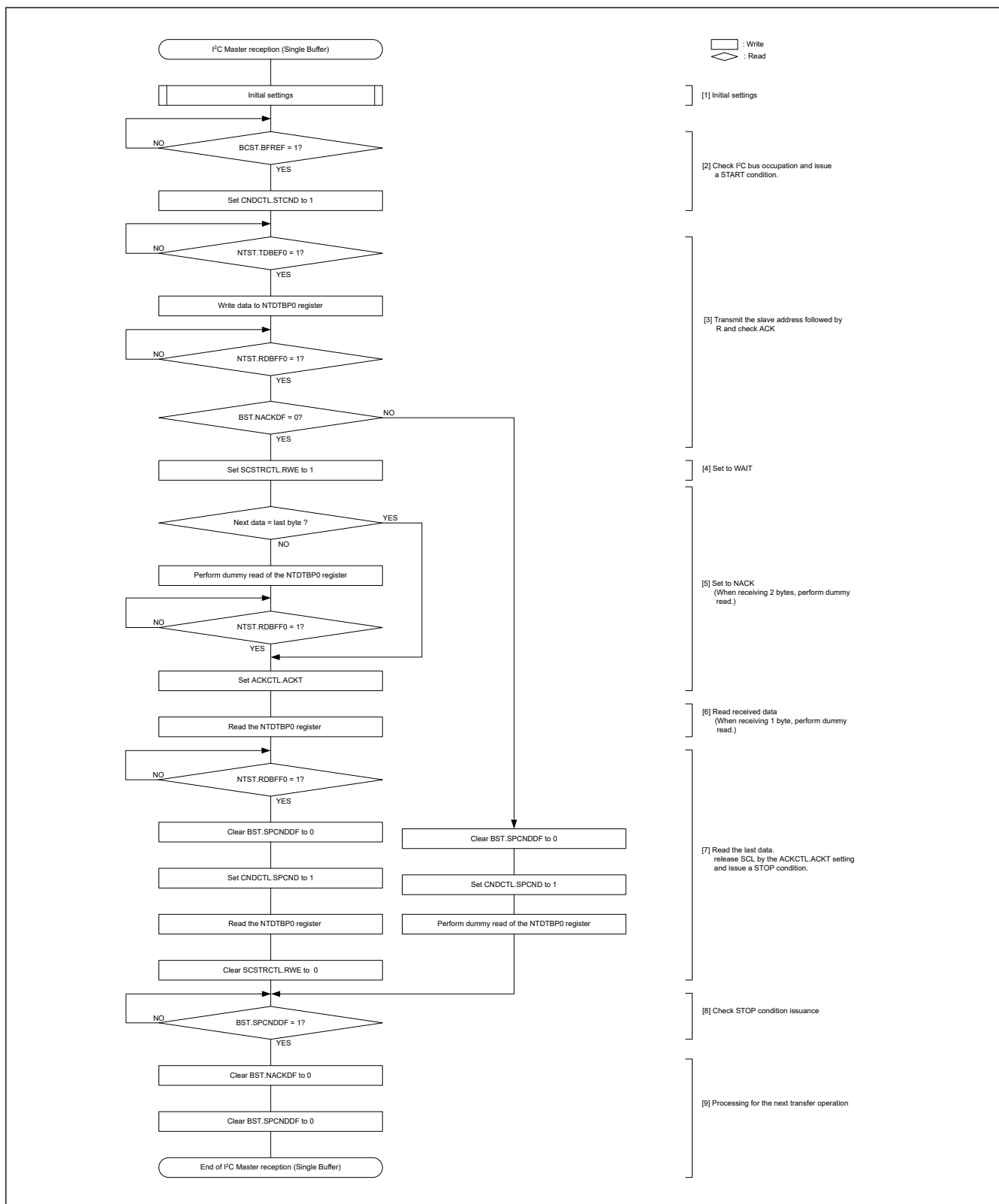
Figure 28.104 Example flowchart of I 2 C master reception (7-bit address format, 1 or 2 bytes)
