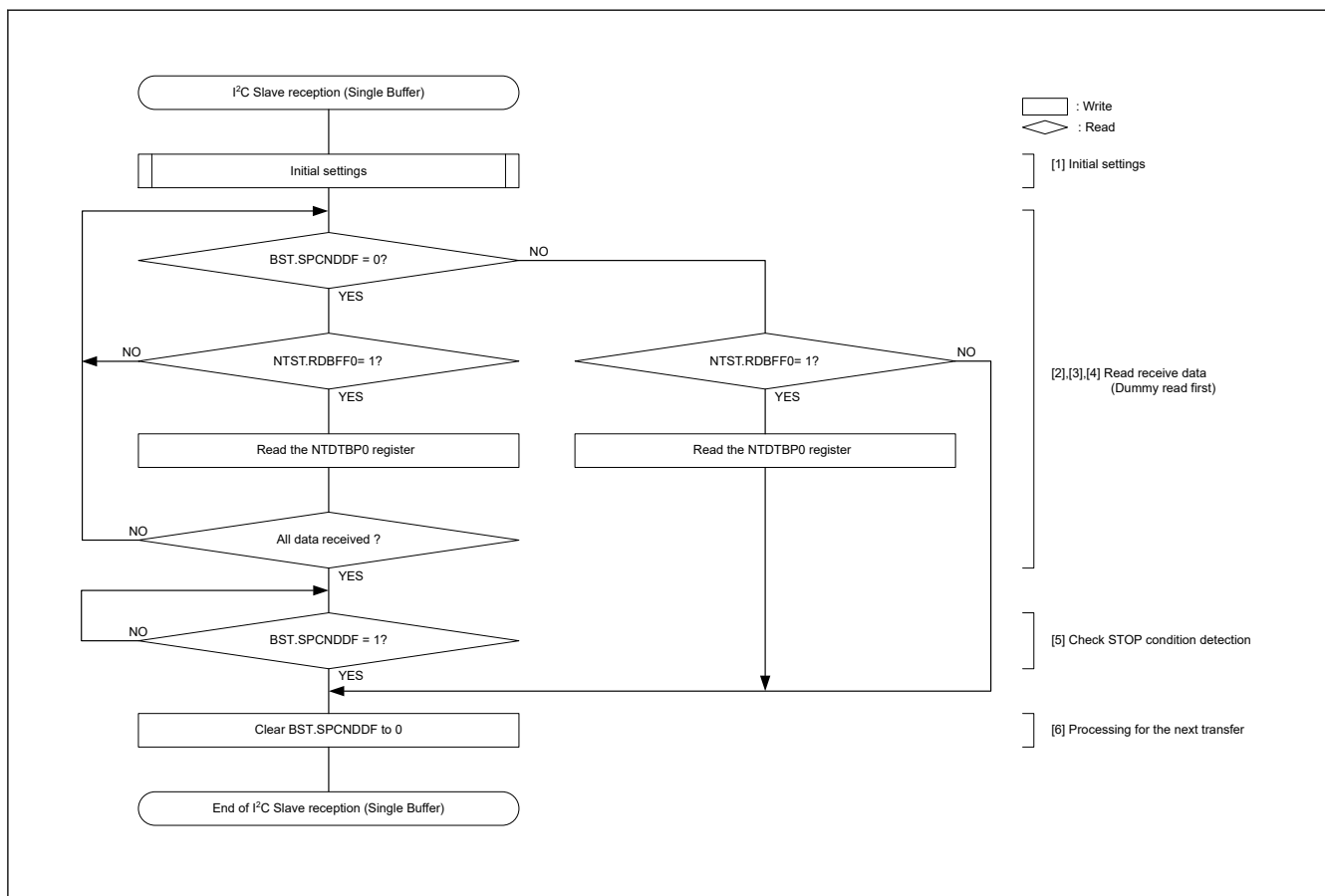
Figure 28.110 Example flowchart of I 2 C slave reception (single buffer transfer)
