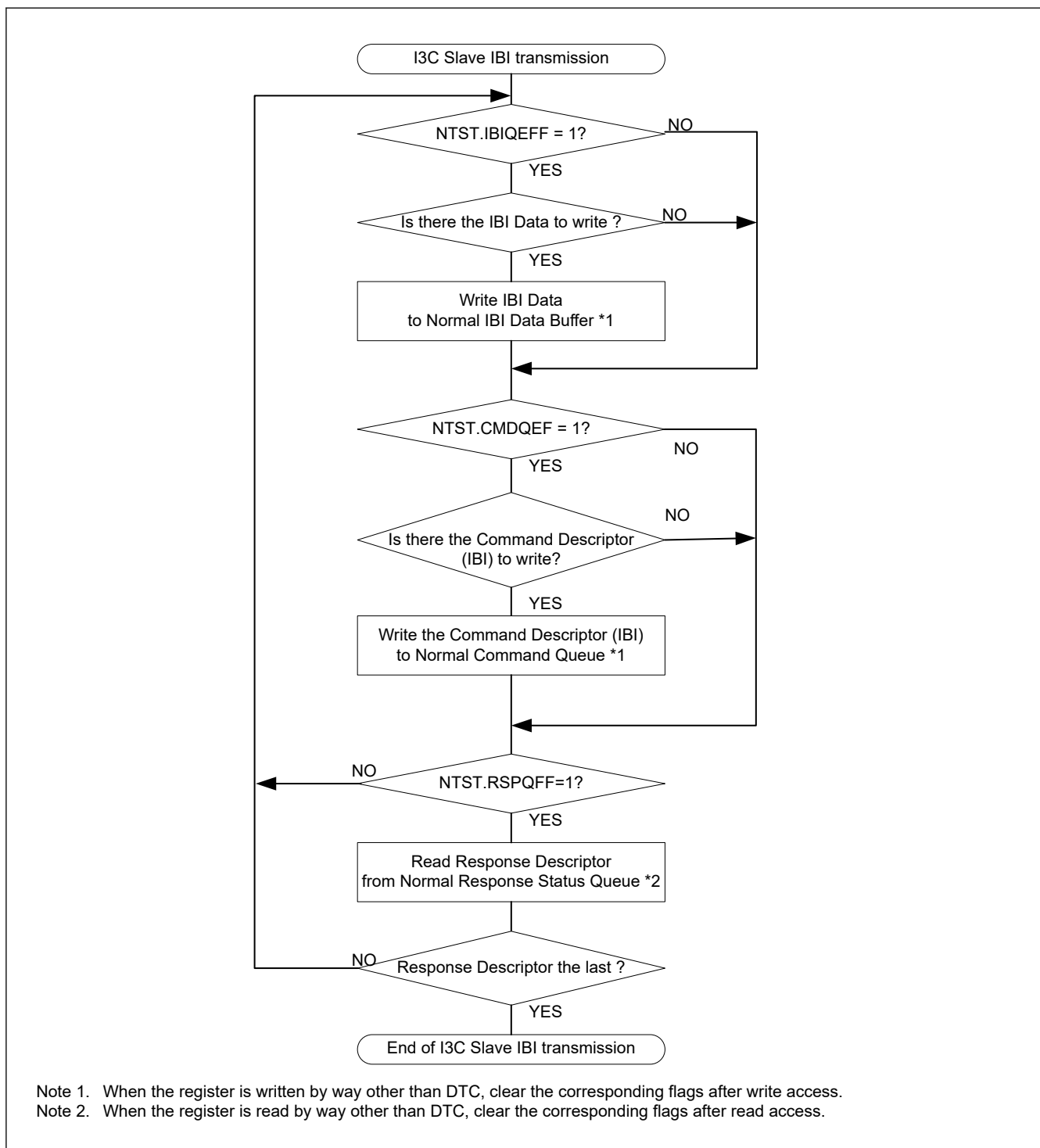
Figure 28.114 Example flowchart of I3C slave IBI transmission
