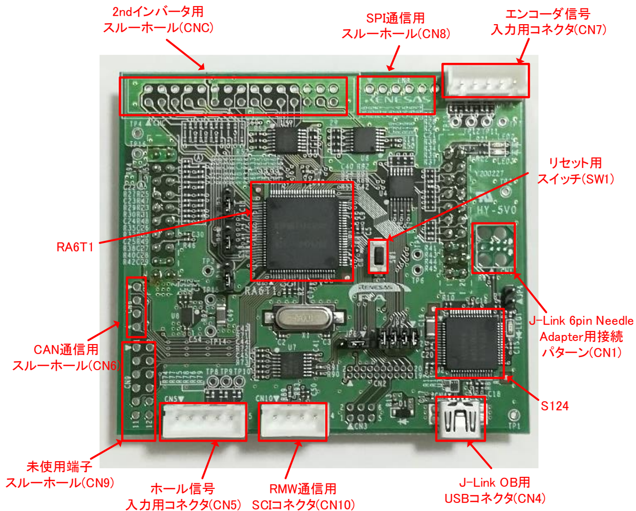
図 1-1 RA6T1 CPU Card (上面)
