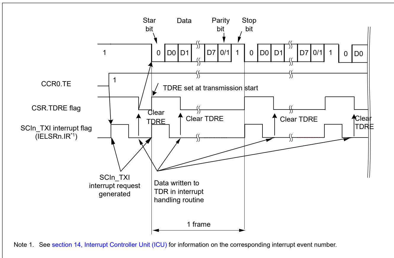
Figure 38.15 Example of Operation for Serial Transmission in Asynchronous Mode (4)(with 8-Bit Data, Parity, 1 Stop Bit, CTS Function Not Used, from the Middle of Transmission until Transmission Completion)
