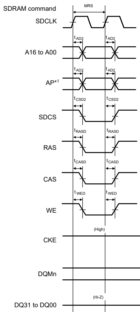
Figure 69.50 SDRAM mode register set timing
