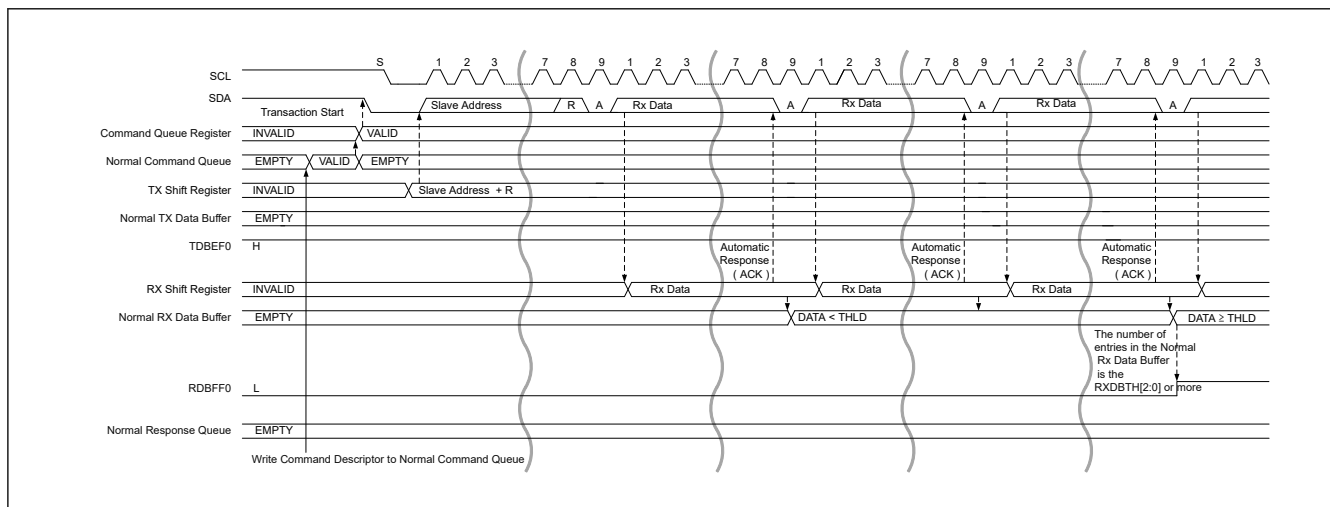
Figure 40.20 SDR data read transfer timing (1/2)
