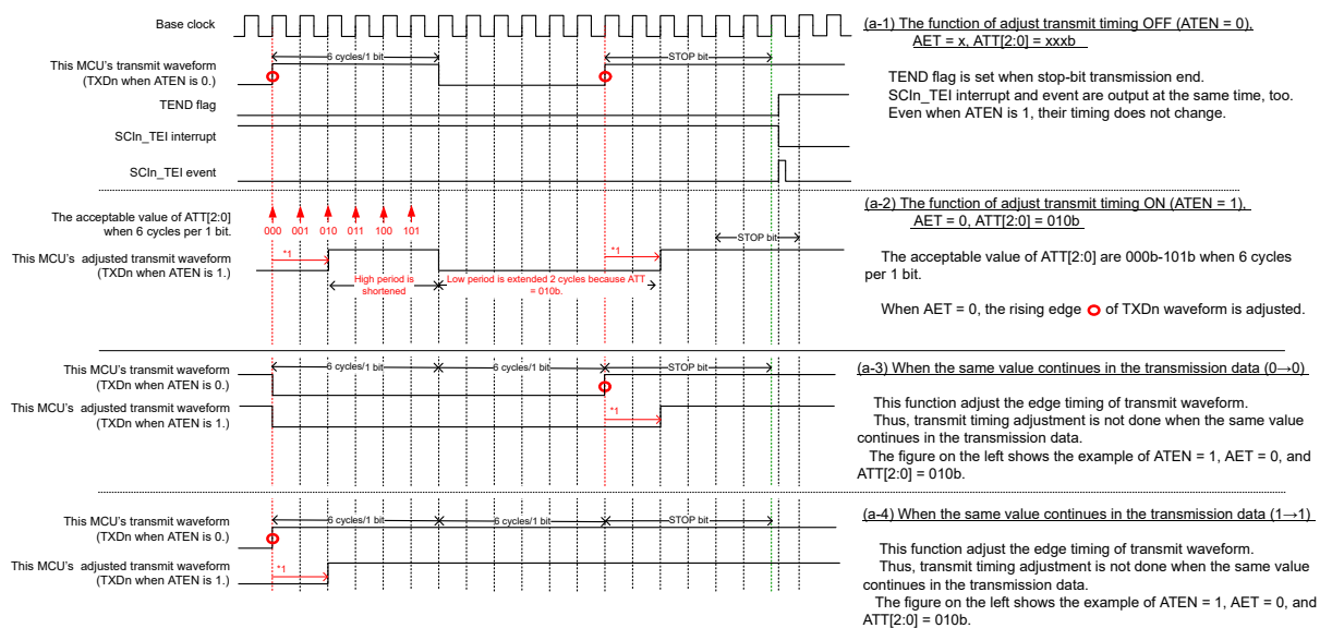
Figure 38.33 The adjustment operation explanation for the transmit timing when AET is 0
