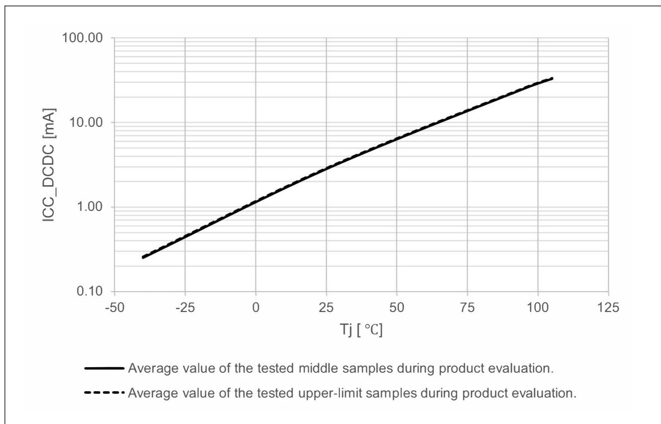
Figure 69.4 Temperature dependency in Software Standby mode ( ICC\_DCDC , SS2LP\_0 , SVSCR\_5 ) (reference data)
