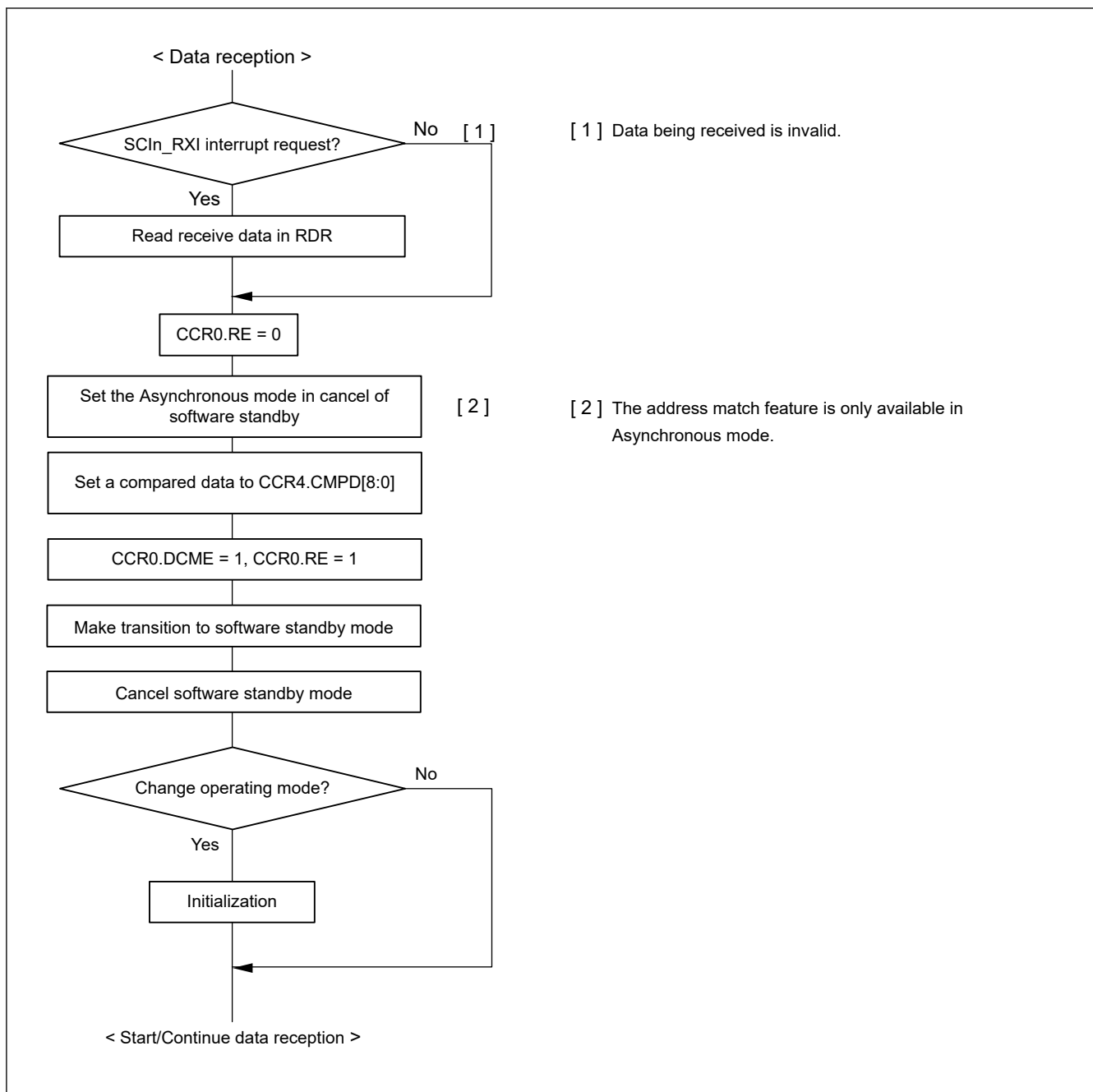
Figure 38.121 Example of Flowchart for Reception to Software Standby Mode during Reception with Address match
