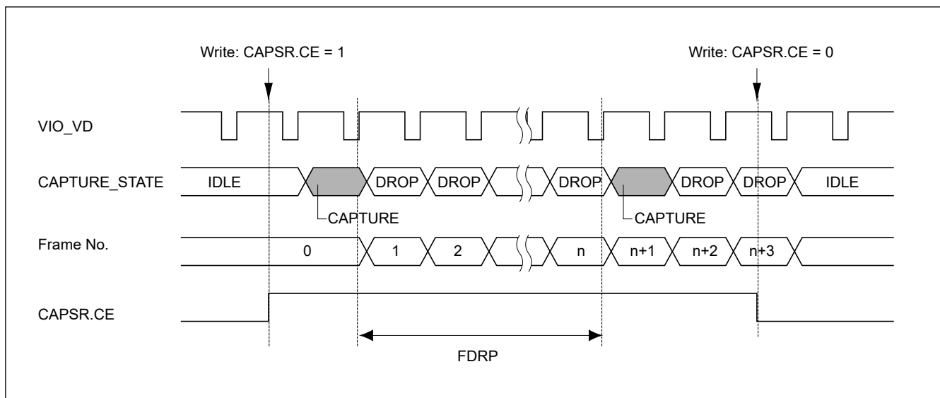
Figure 60.9 Setting of FDRP bits and frame drop timing
