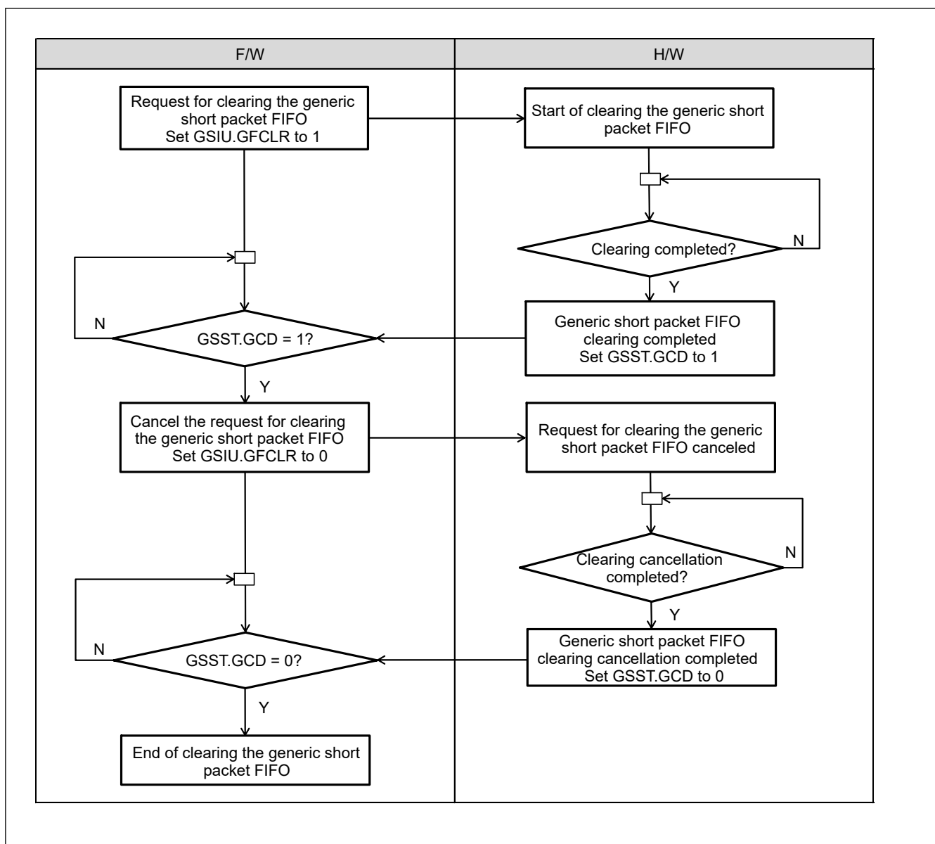
Figure 66.5 Clearing the generic short packet FIFO
