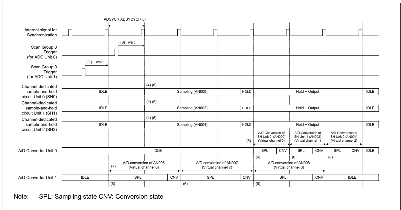
Figure 53.32 Example of synchronous operation using with channel-dedicated sample-and-hold circuit
