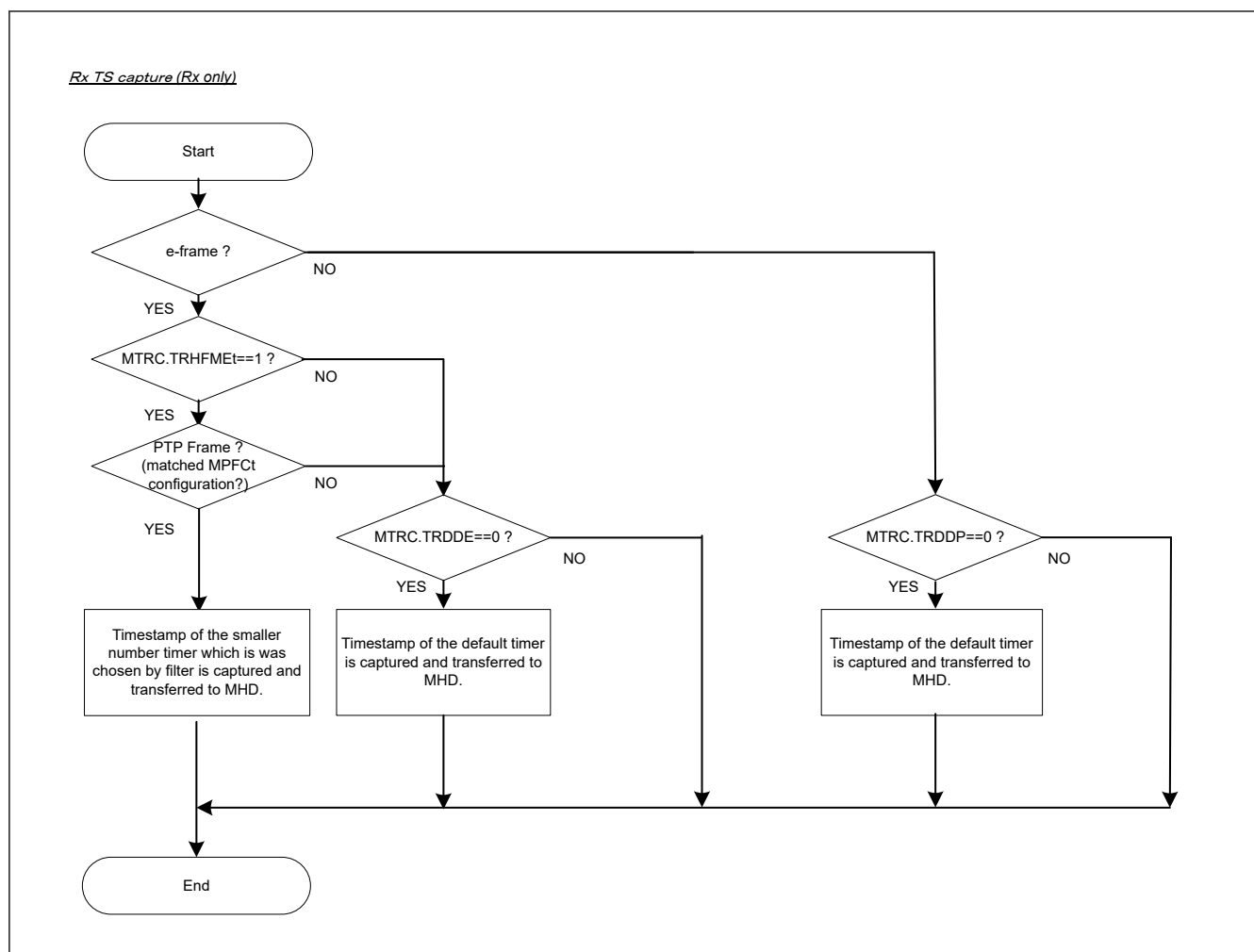
Figure 33.24 Rx TS capture (Rx only)
