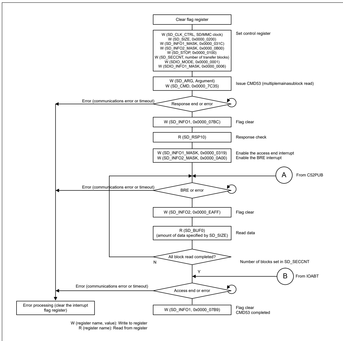
Figure 47.17 Example of IO_RW_EXTENDED command (CMD53) for multiple block read operation
