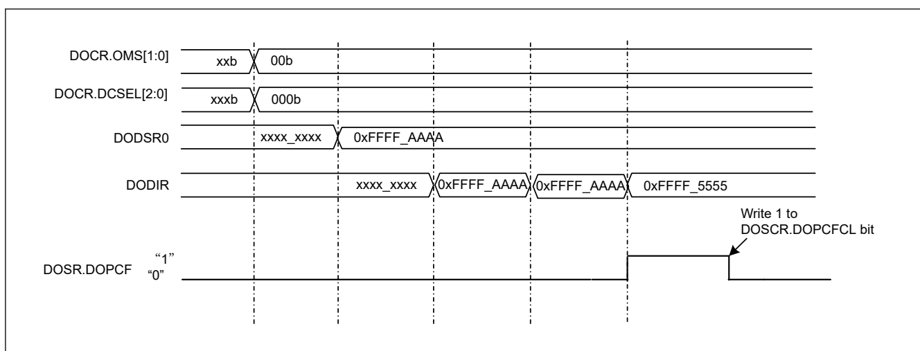
Figure 57.2 Example of Operation in Data Comparison Mode (Detection condition: Mismatch)
