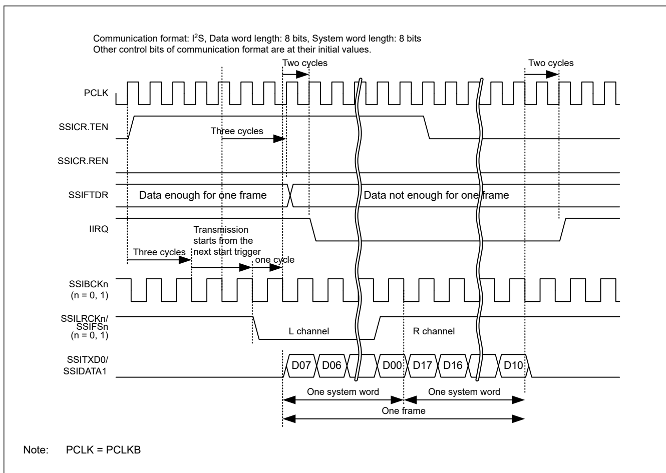
Figure 46.14 IIRQ setting timing (transmission)
