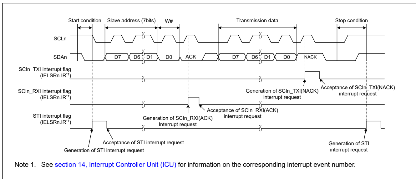
Figure 38.92 Example 2 of operations for master transmission in simple IIC mode with 7-bit slave addresses, ACK interrupts, and NACK interrupts (ICR.IICINTM = 0)
