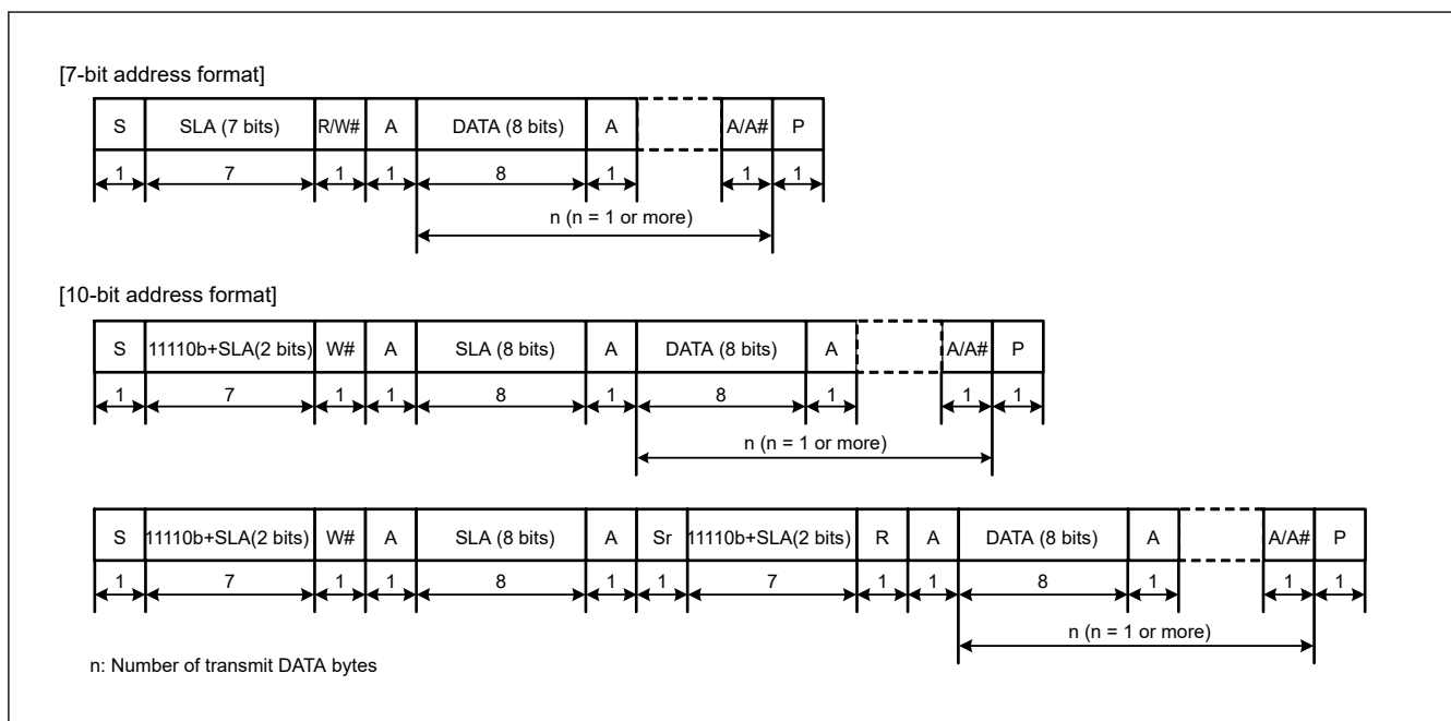
Figure 40.69 I 2 C bus format
