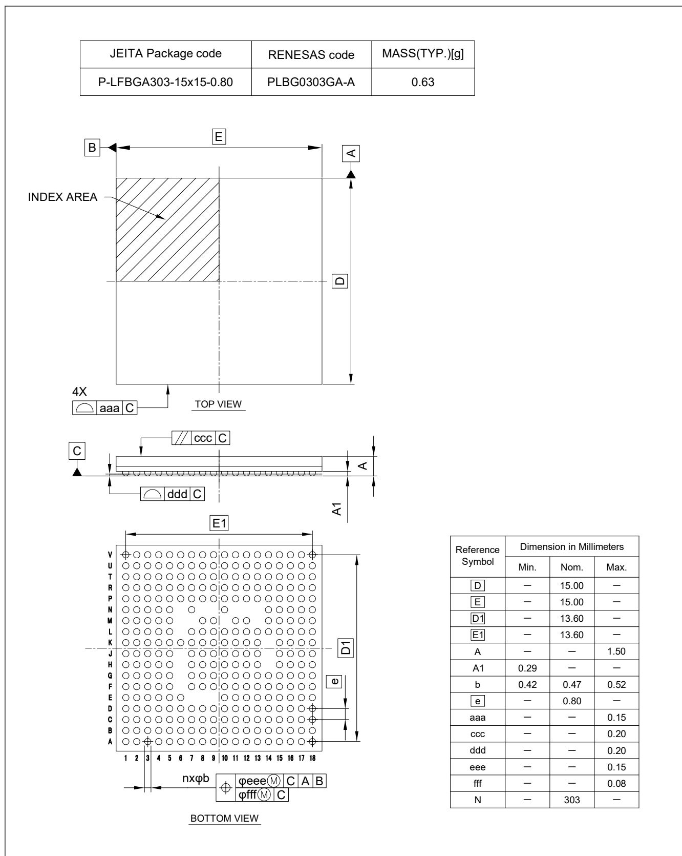
Figure A2.3 BGA 303-pin
