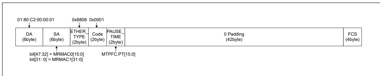
Figure 33.15 PAUSE frame format
