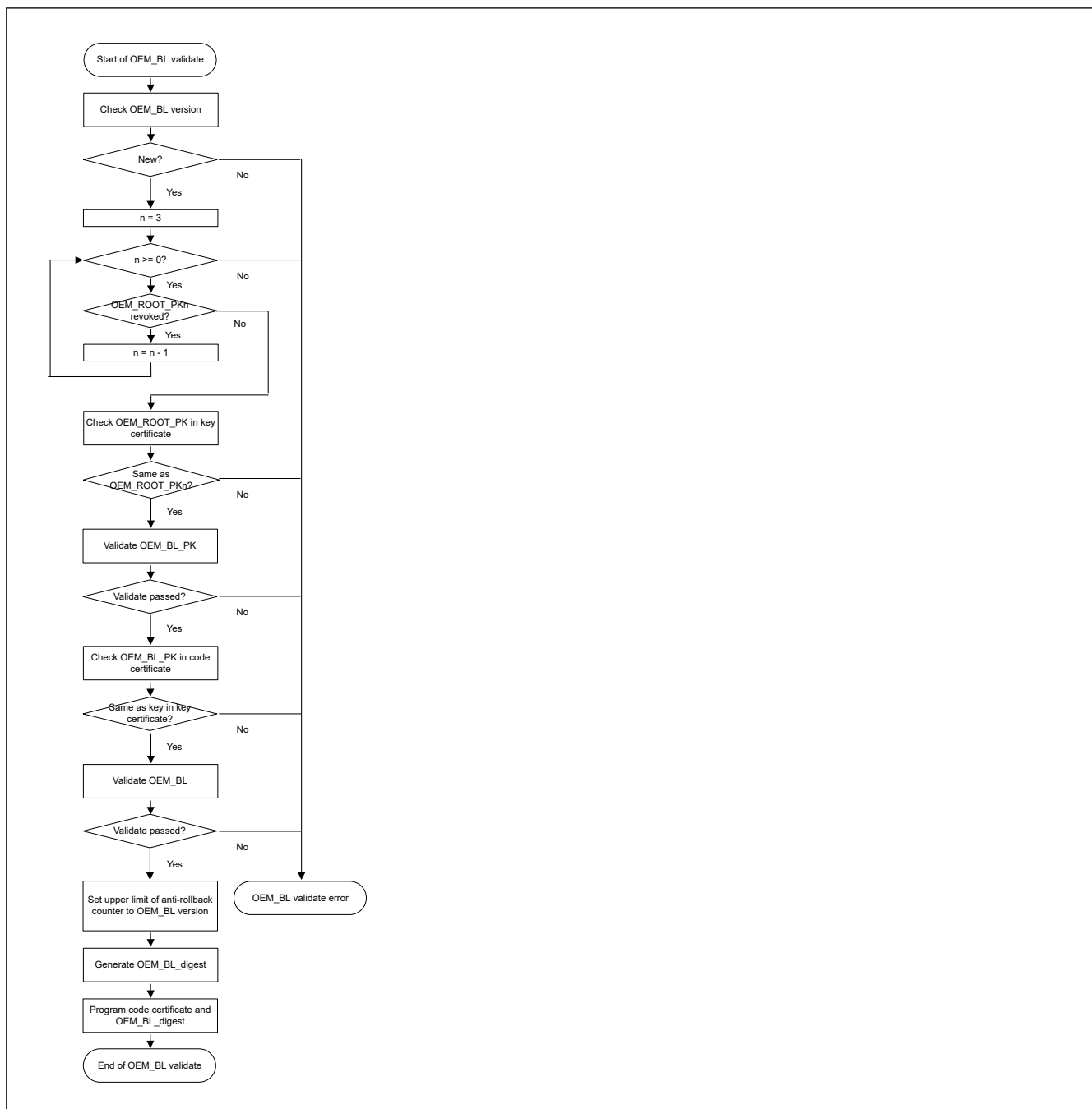
Figure 51.11 OEM_BL validation flow in serial programming mode
