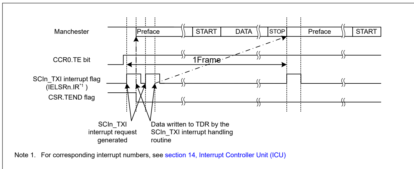
Figure 38.52 Example of Start-of-Transmission Operation for Serial Transmission in Manchester mode (with Preface but Without the CTS Function)
