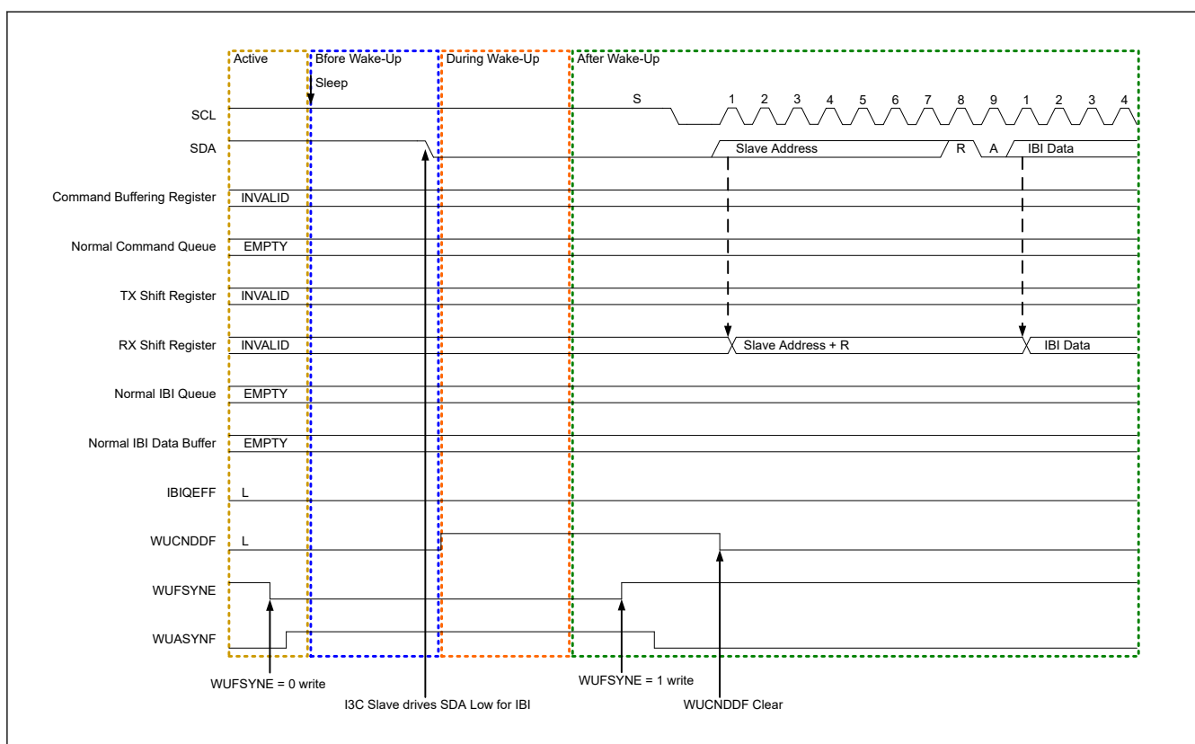
Figure 40.134 I3C master wake-up operation
