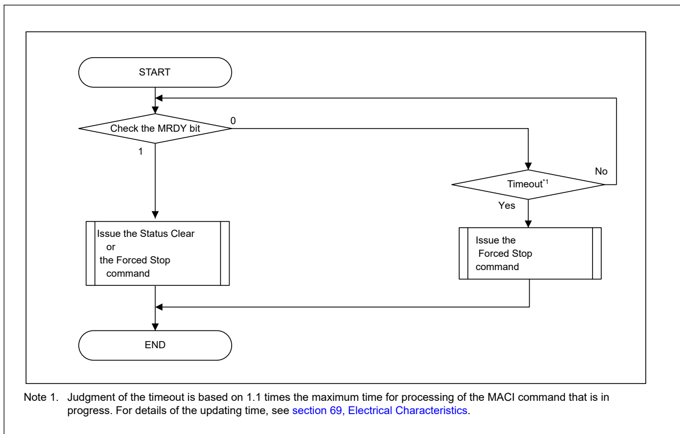
Figure 59.12 Recovery from the command-locked state
