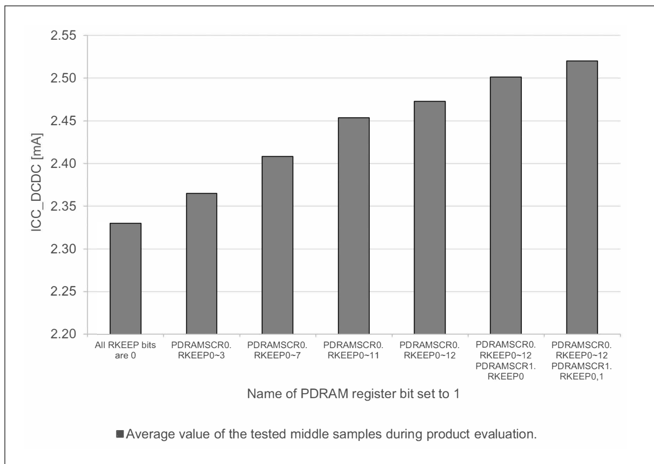
Figure 69.11 Software Standby current per SRAM state (ICC_DCDC, SS2LP_0, SVSCR_2) (reference data)
