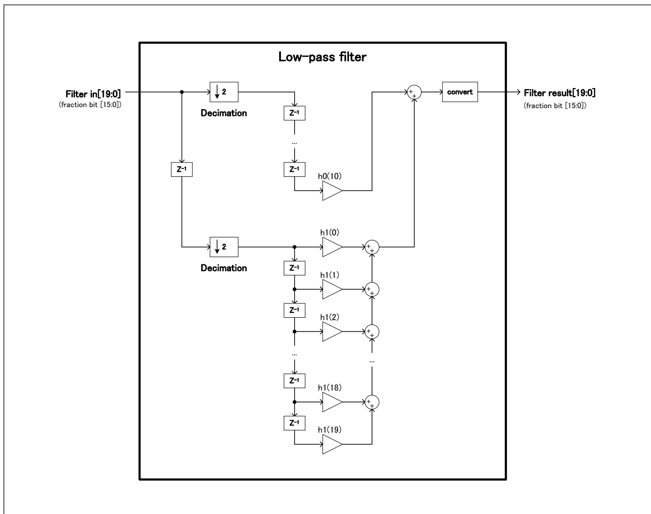
Figure 49.6 Low-pass filter block diagram
