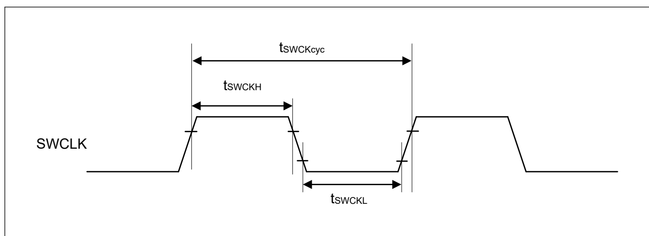
Figure 69.158 SWD SWCLK timing
