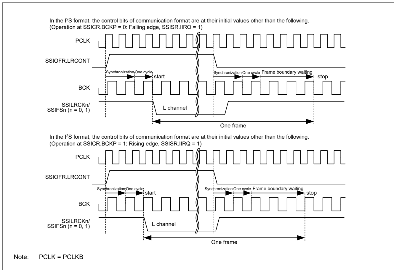
Figure 46.44 Example of disabling LR clock/frame synchronization continuation by SSIOFR.LRCONT
