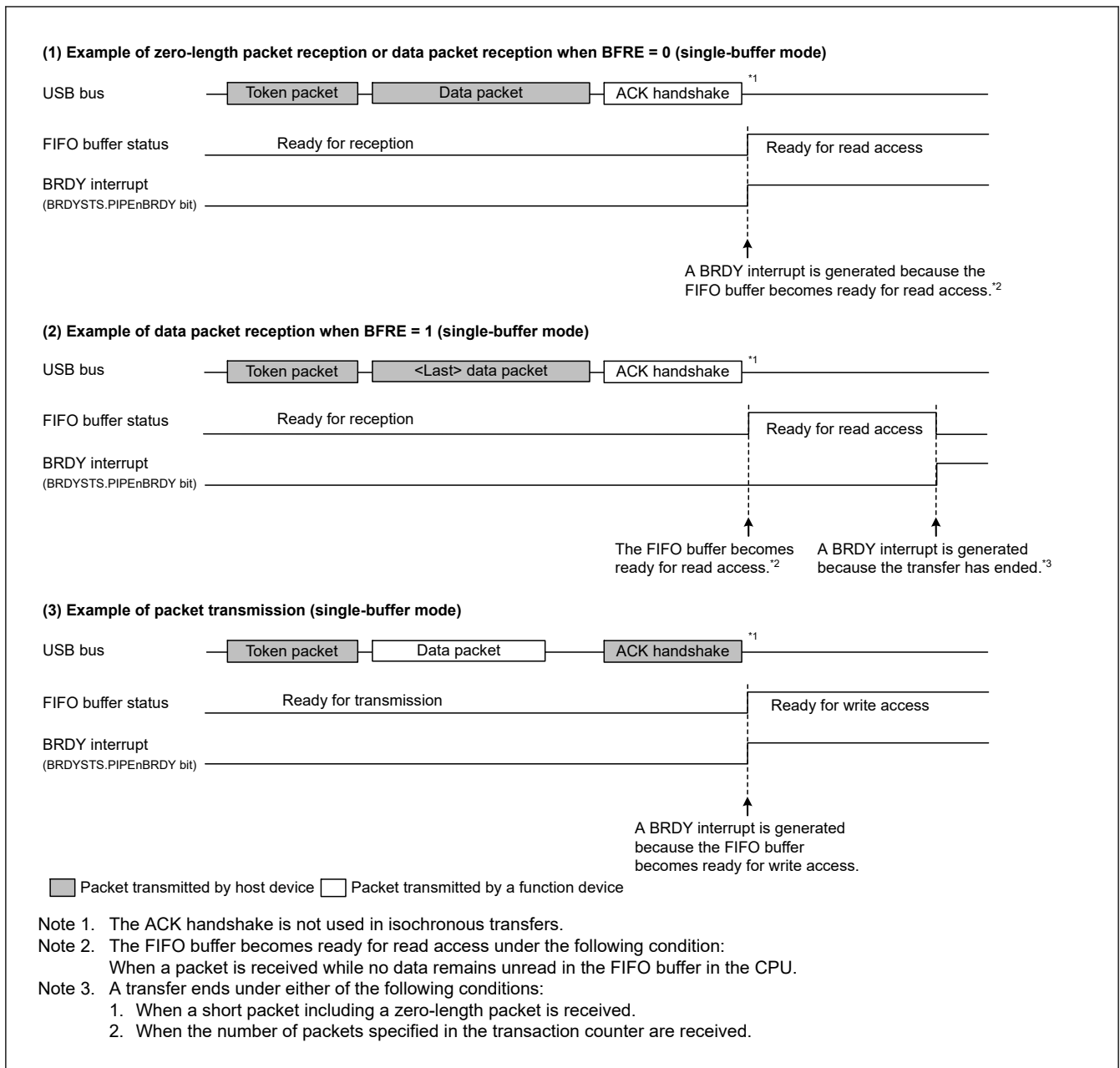
Figure 36.11 Timing of BRDY interrupt generation
