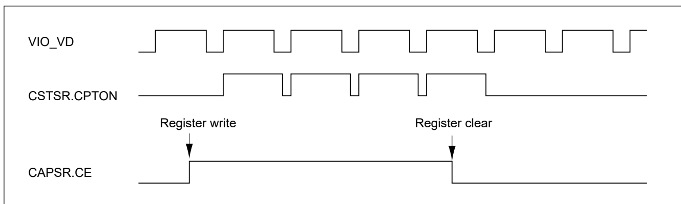
Figure 60.8 Continuous-frame capture
