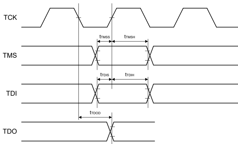
Figure 69.153 Boundary scan input/output timing (1)
