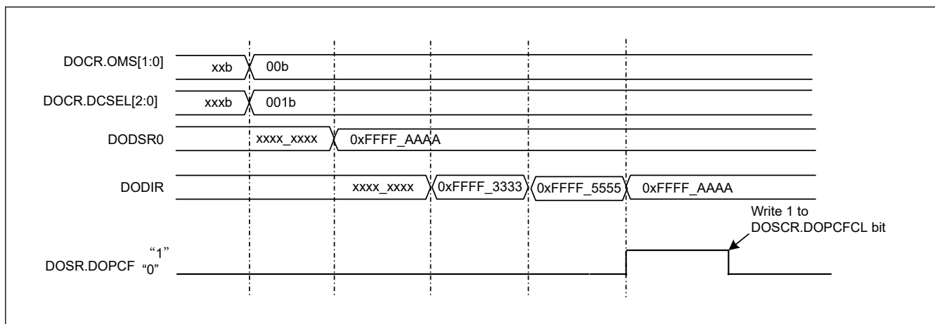
Figure 57.3 Example of Operation in Data Comparison Mode (Detection condition: Match)
