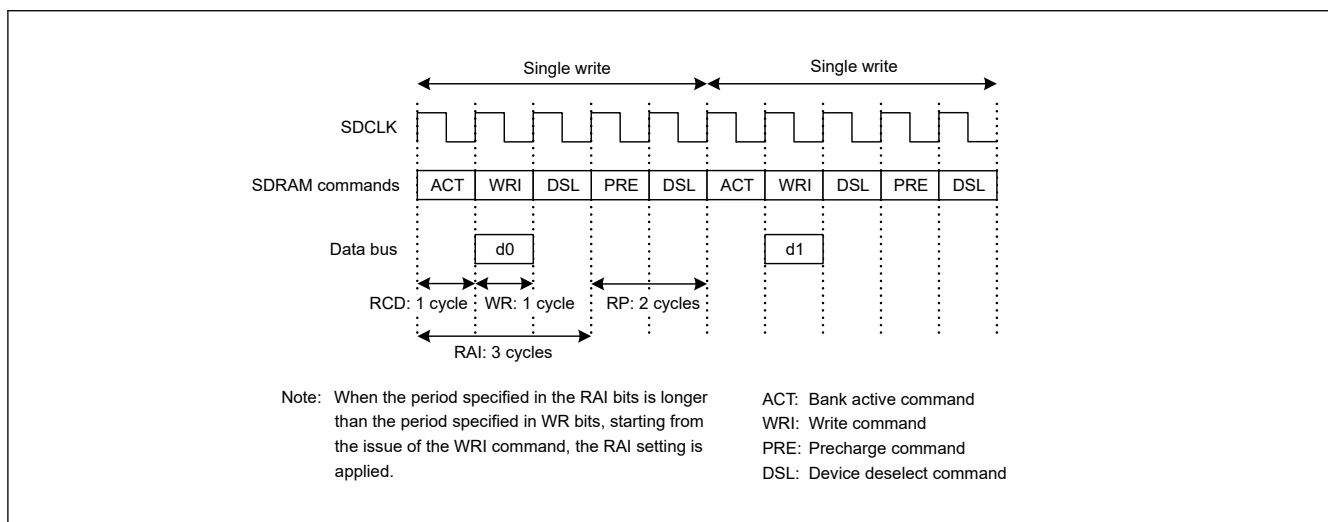
Figure 15.56 Example timing for single write (1)
