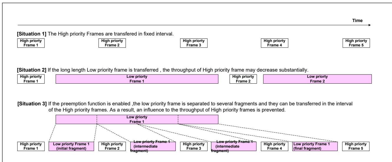
Figure 33.13 Effective of Preemption
