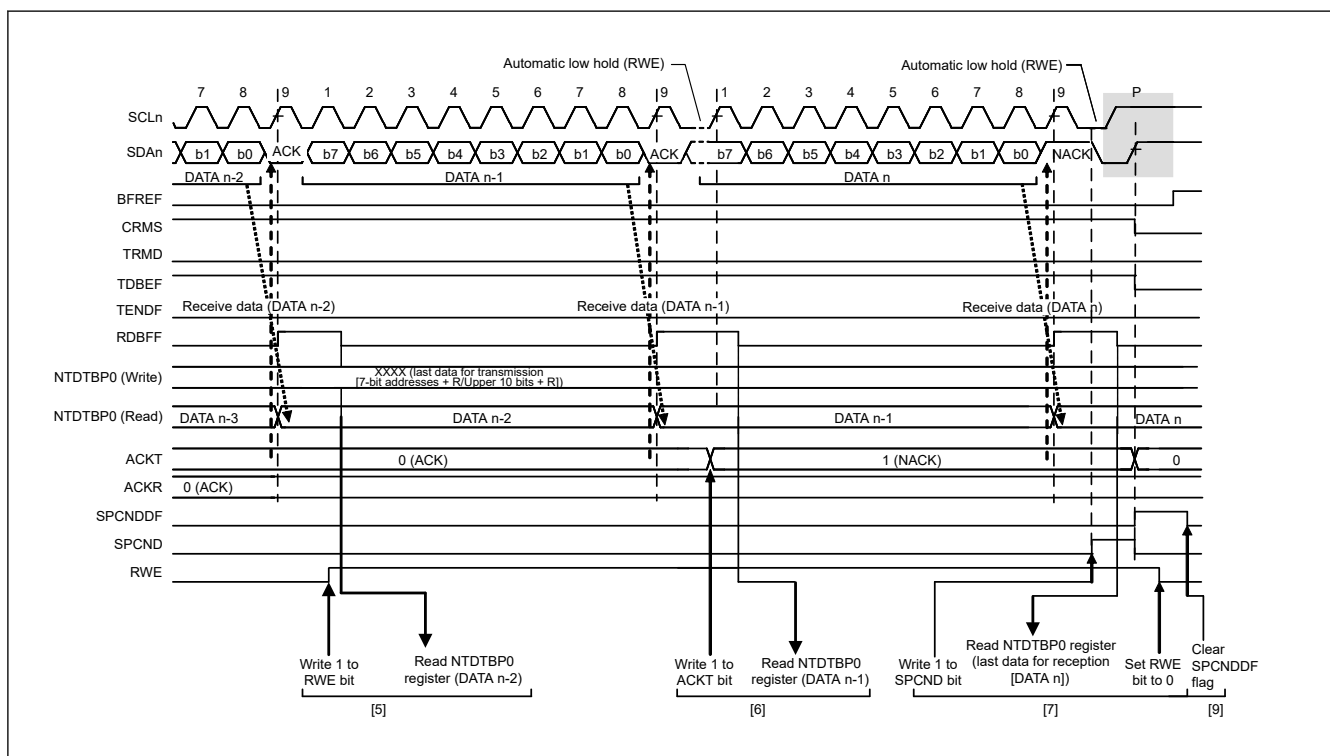
Figure 40.11 Master receive operation timing (3) (when ACKTWE = 0)
