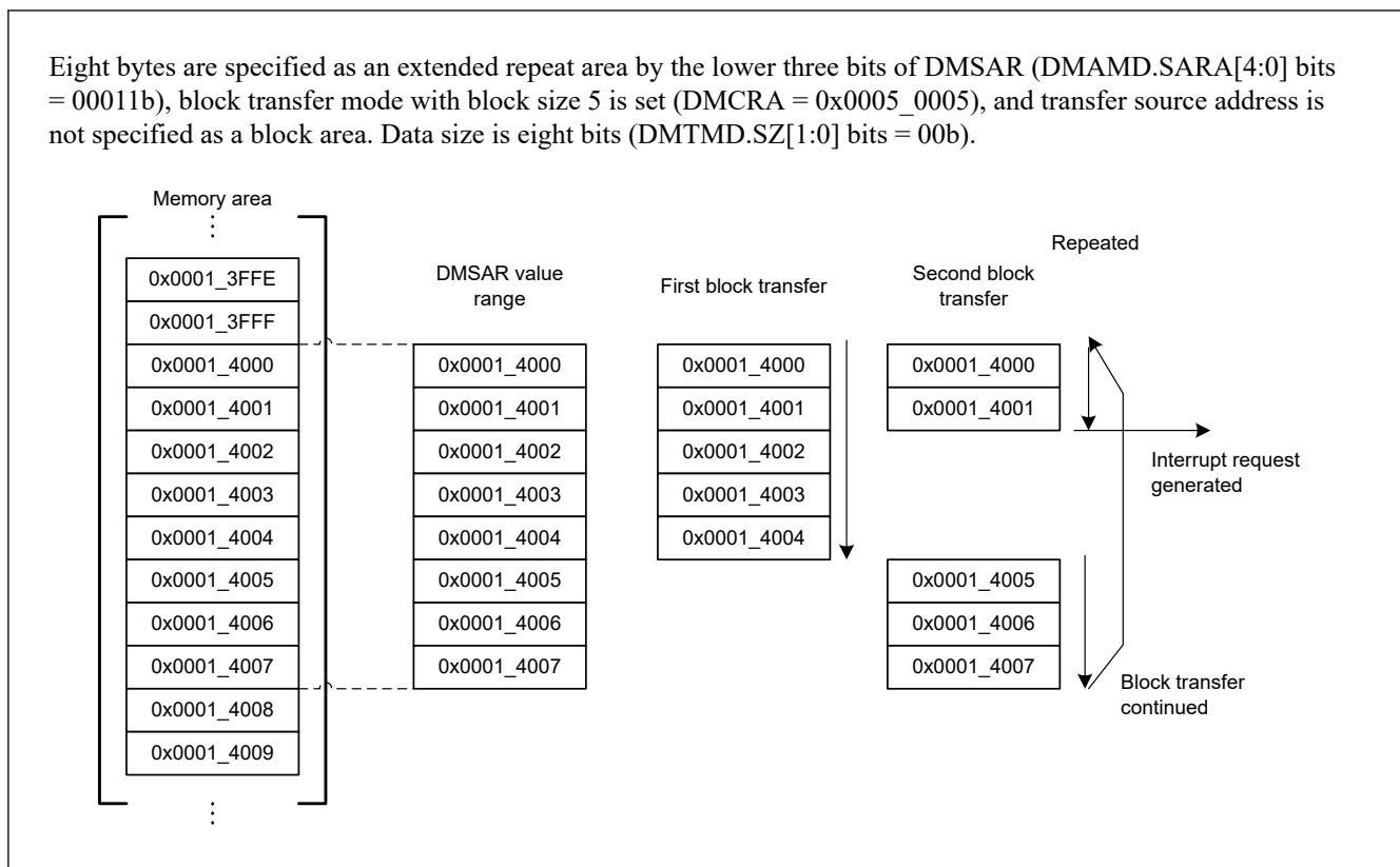
Figure 17.8 Example of extended repeat area function in block transfer mode
