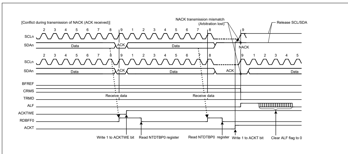
Figure 40.91 Example of arbitration-lost detection during transmission of NACK (NALE = 1)
