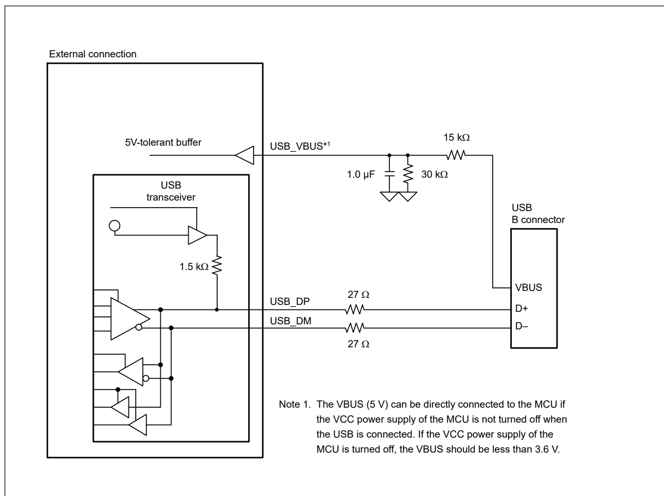
Figure 36.3 Example device connection in a self-powered system
