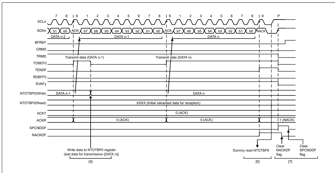
Figure 40.40 Slave transmit operation timing (2)
