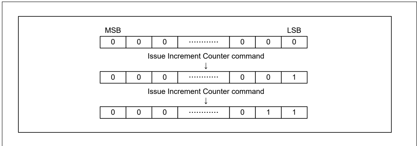
Figure 59.22 Increment image of anti-rollback counter
