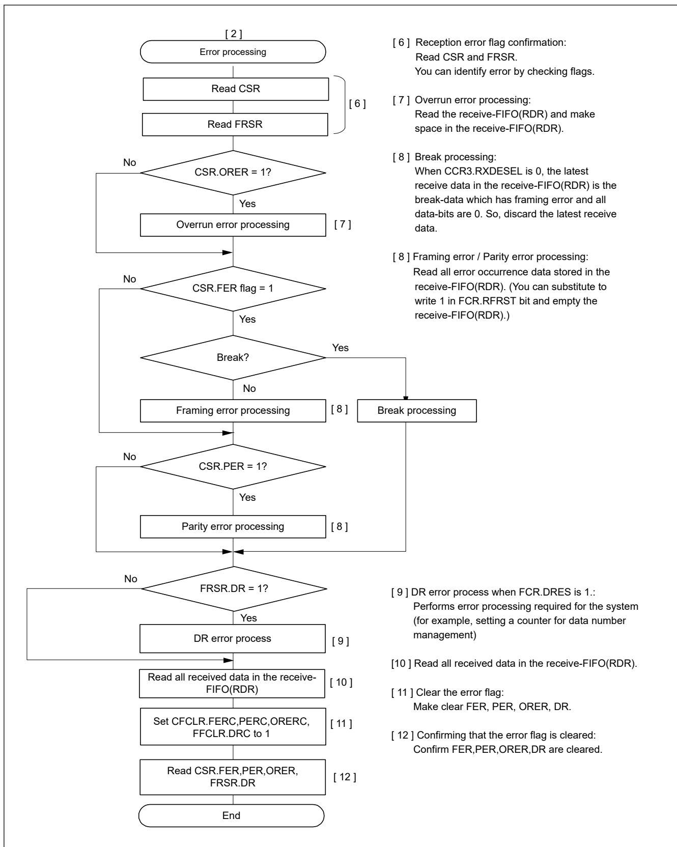
Figure 38.25 Example flow of serial reception in Asynchronous mode with FIFO selected Address Matching Disabled (2)
