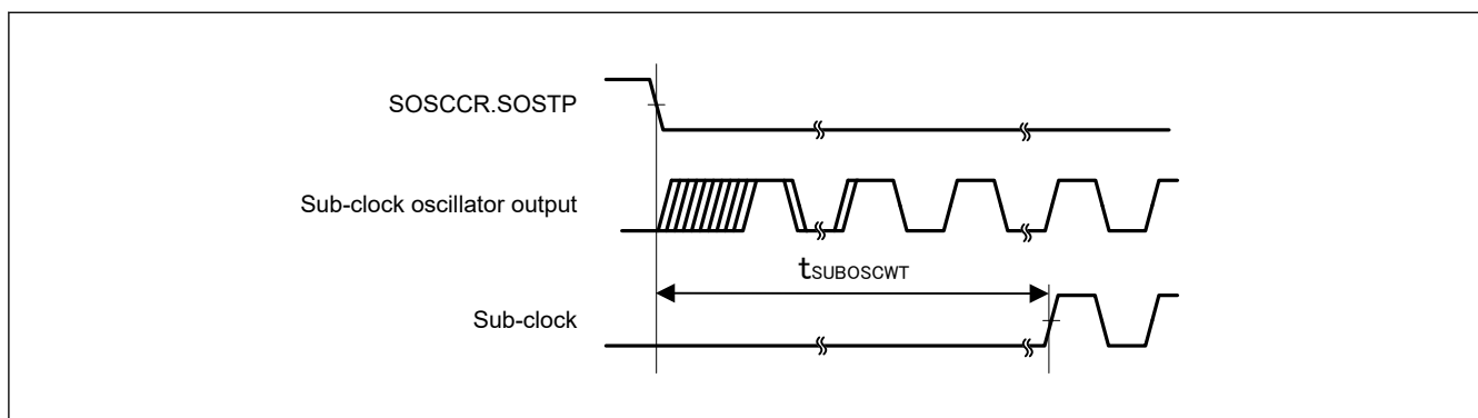
Figure 69.30 Sub-clock oscillation start timing
