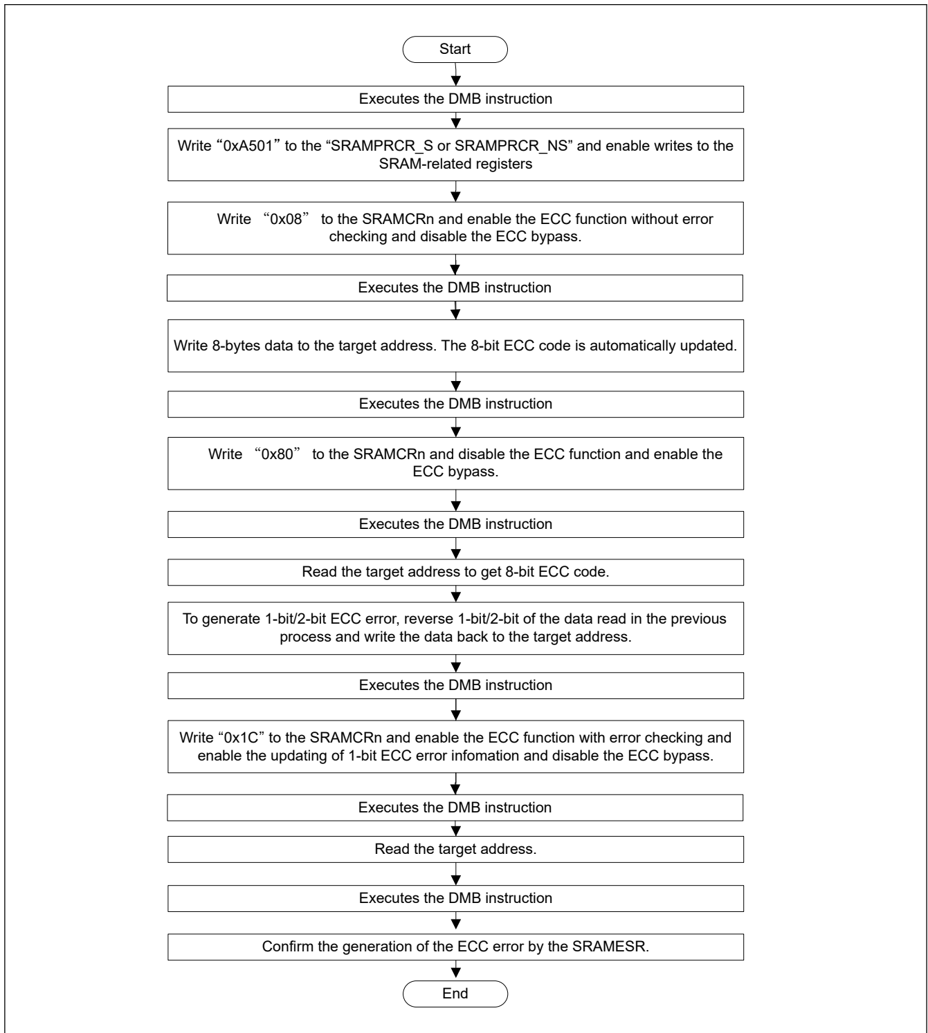
Figure 58.2 ECC decoder testing
