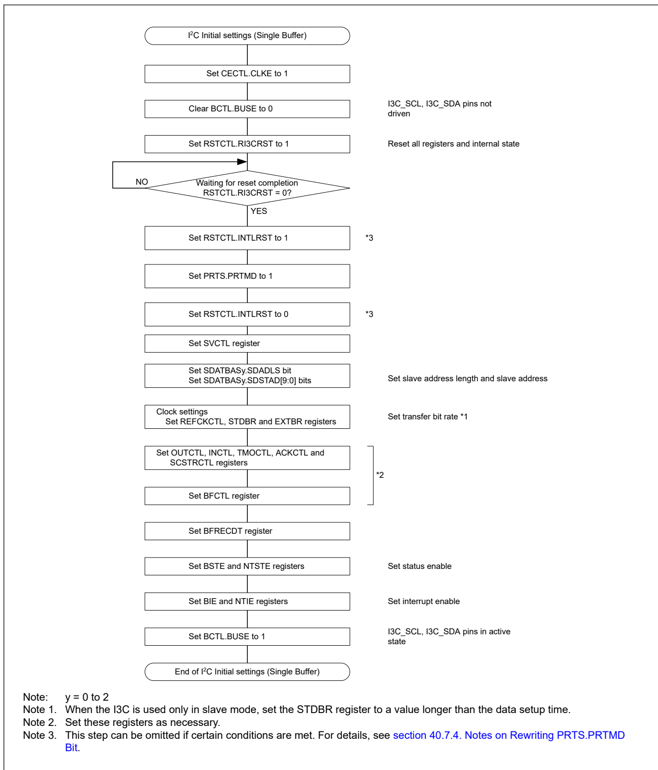
Figure 40.140 Example of I 2 C initialization flowchart (single buffer transfer)
