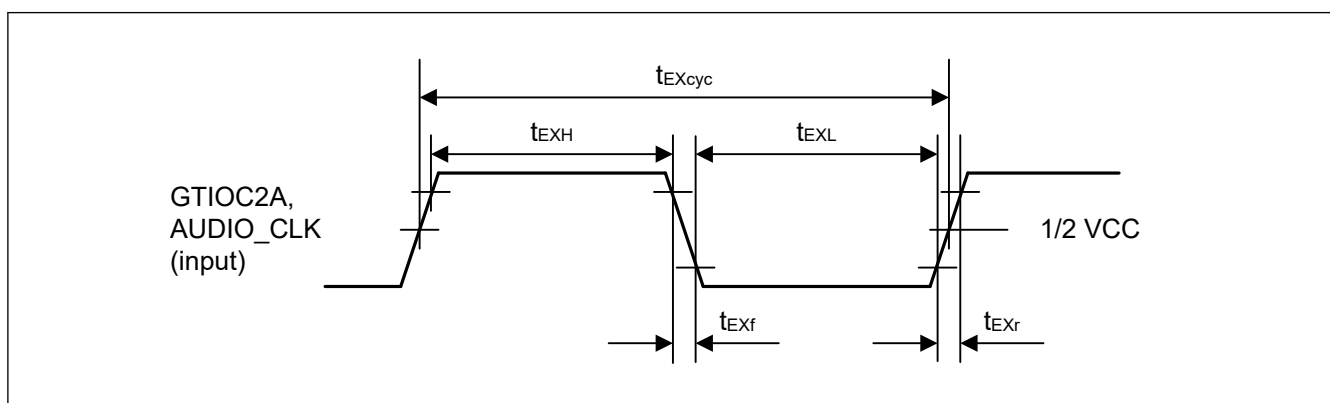
Figure 69.103 Clock input timing
