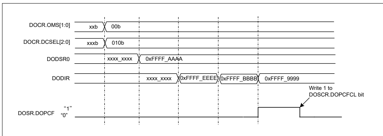
Figure 57.4 Example of Operation in Data Comparison Mode (Detection condition: Lower)
