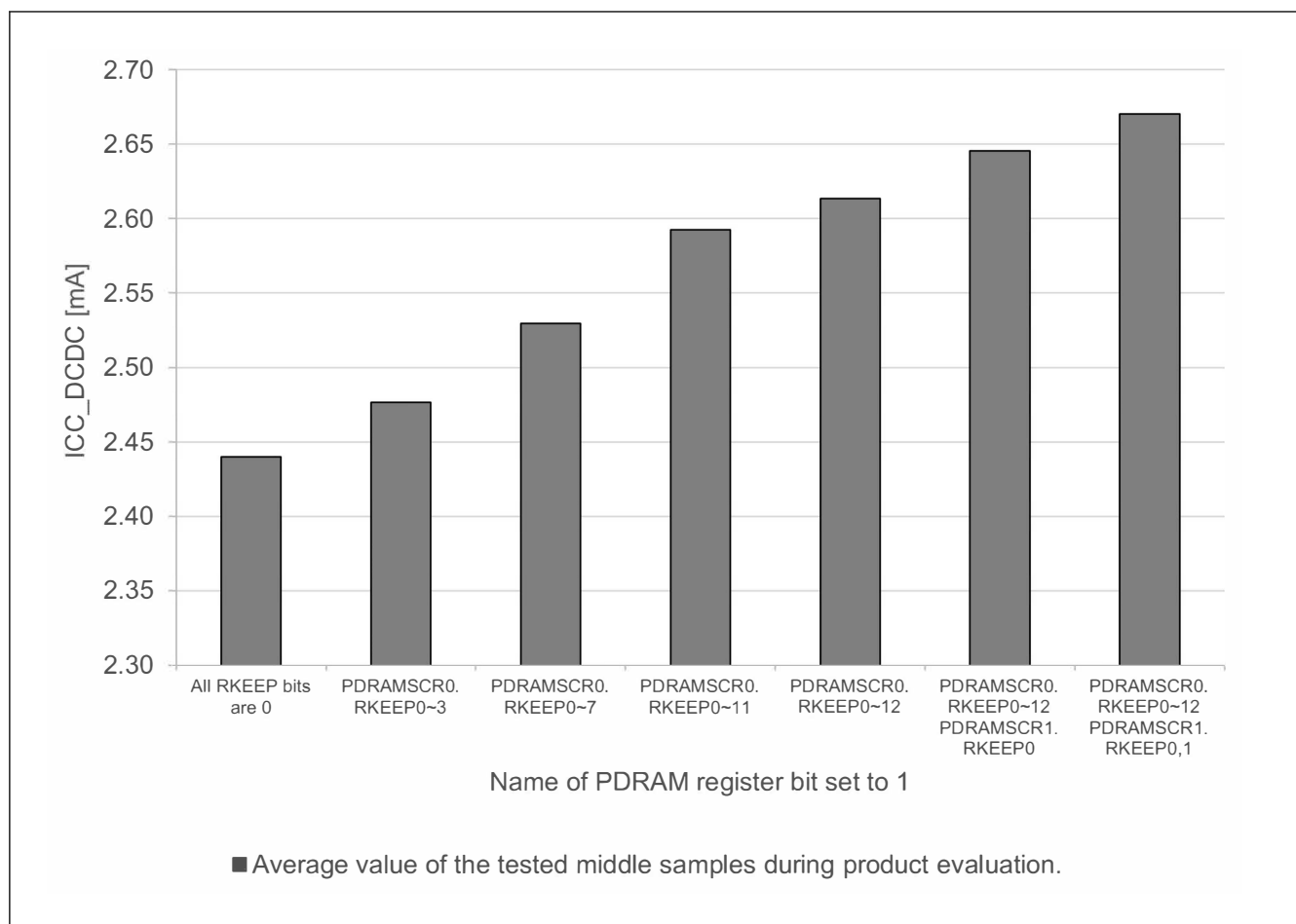
Figure 69.10 Software Standby current per SRAM state (ICC_DCDC, SS2LP_0, SVSCR_1) (reference data)
