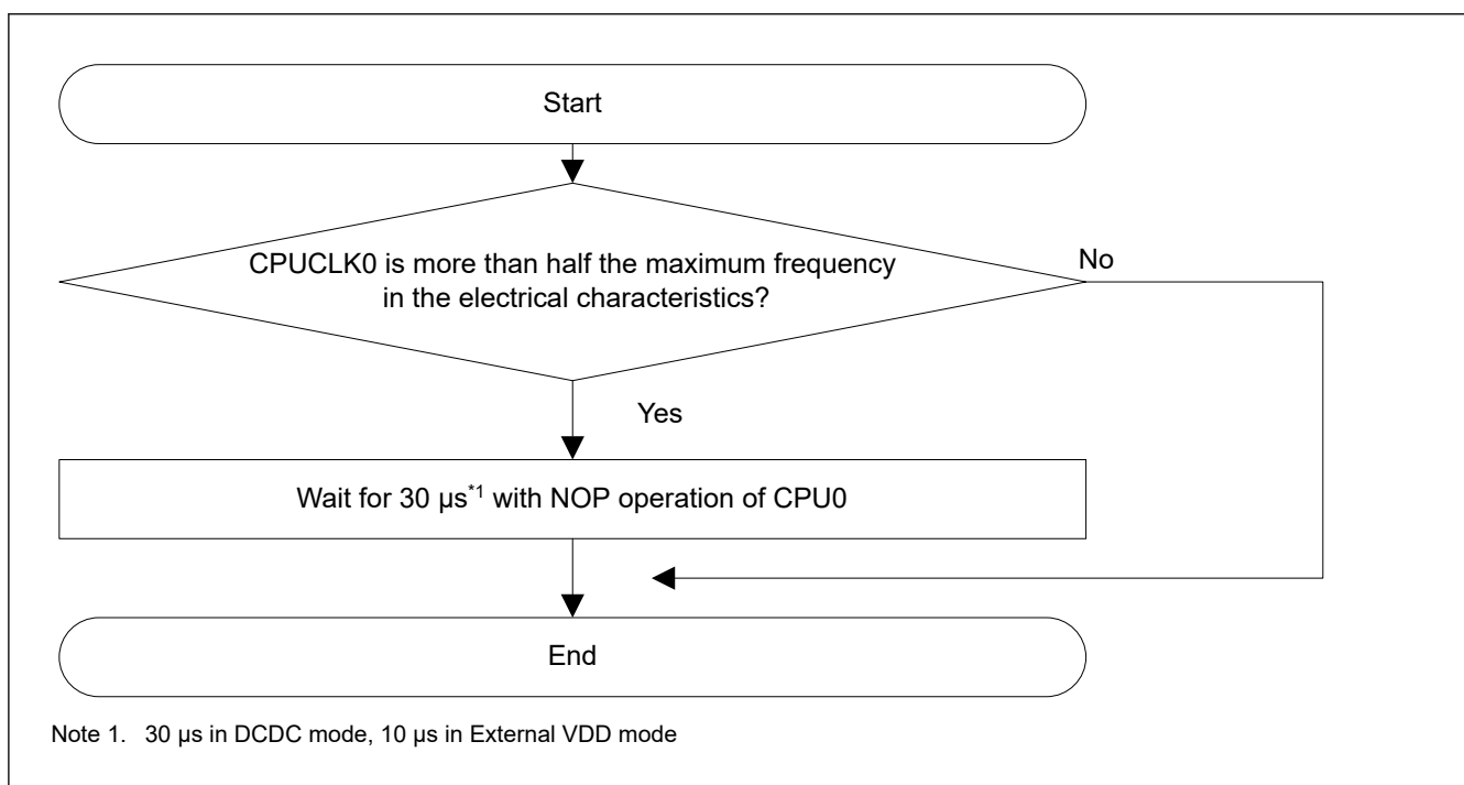
Figure 11.8 Additional flow for the return from CPU0 Sleep mode, CPU0 Deep Sleep mode with CPUDSCR.PGD0 bit is 1 according to CPUCLK0 frequency
