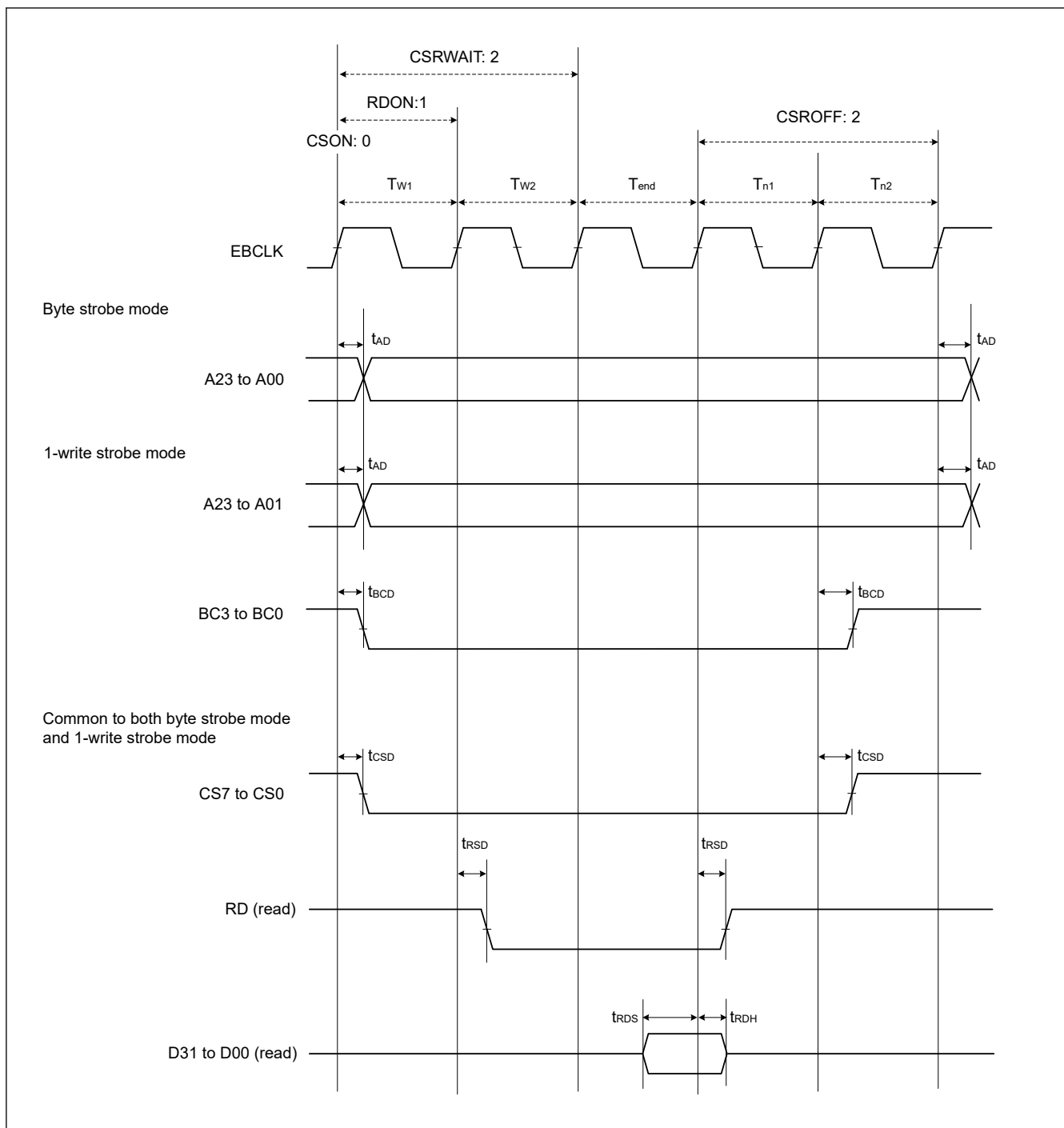
Figure 69.40 External bus timing for normal read cycle with bus clock synchronized
