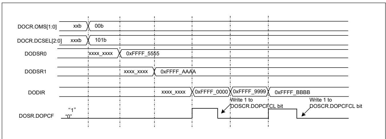
Figure 57.7 Example of Operation in Data Comparison Mode (Detection condition: Outside window)
