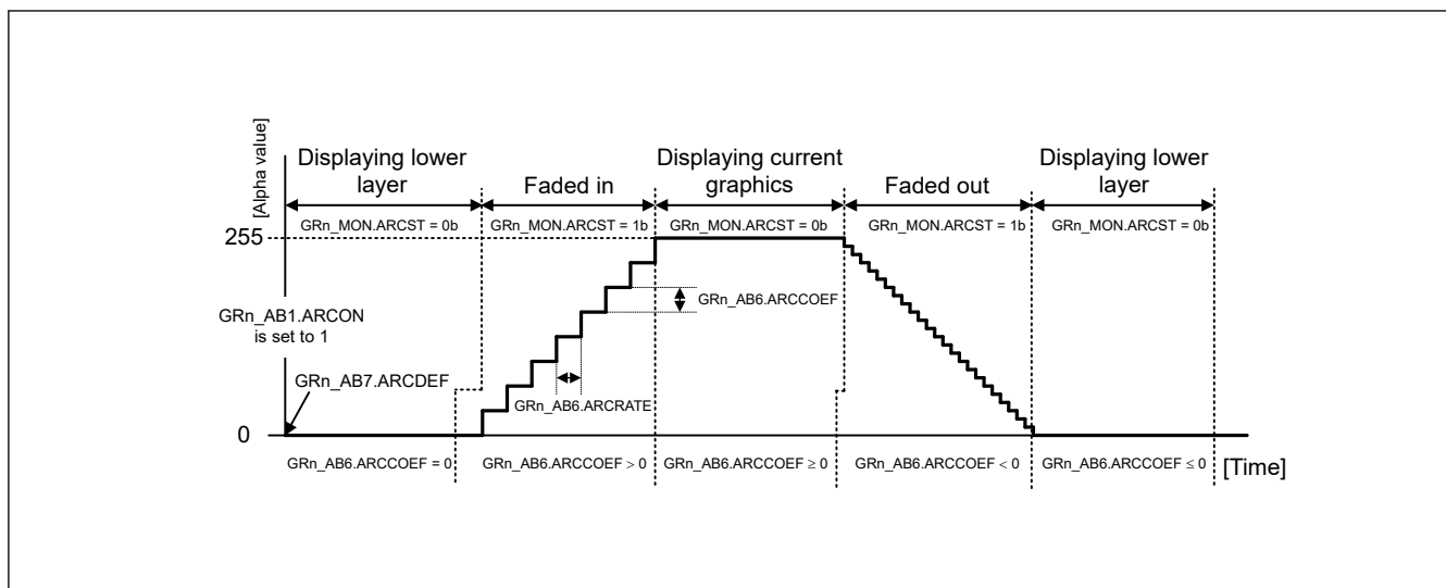
Figure 63.9 Updating of alpha blending value
