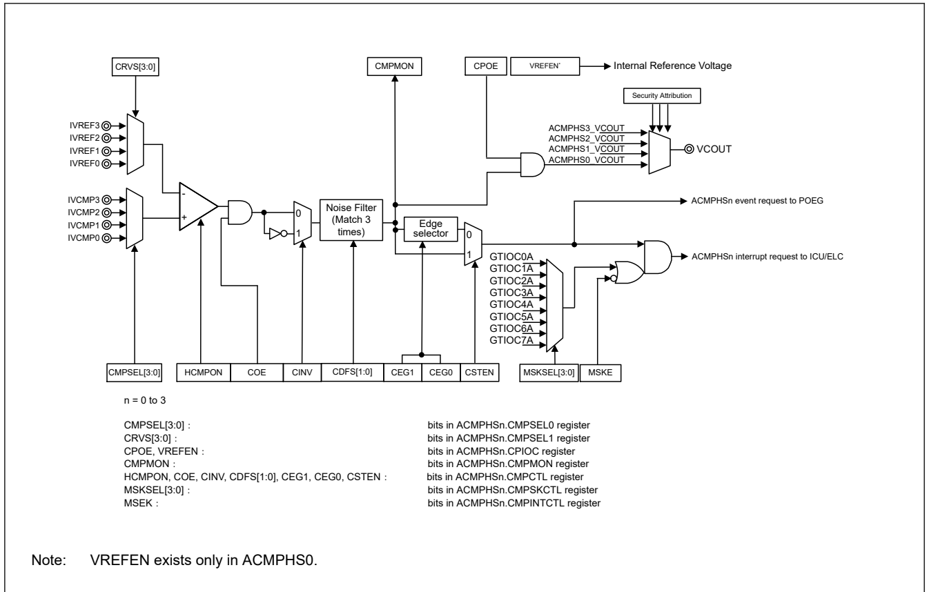
Figure 56.1 ACMPHS block diagram
