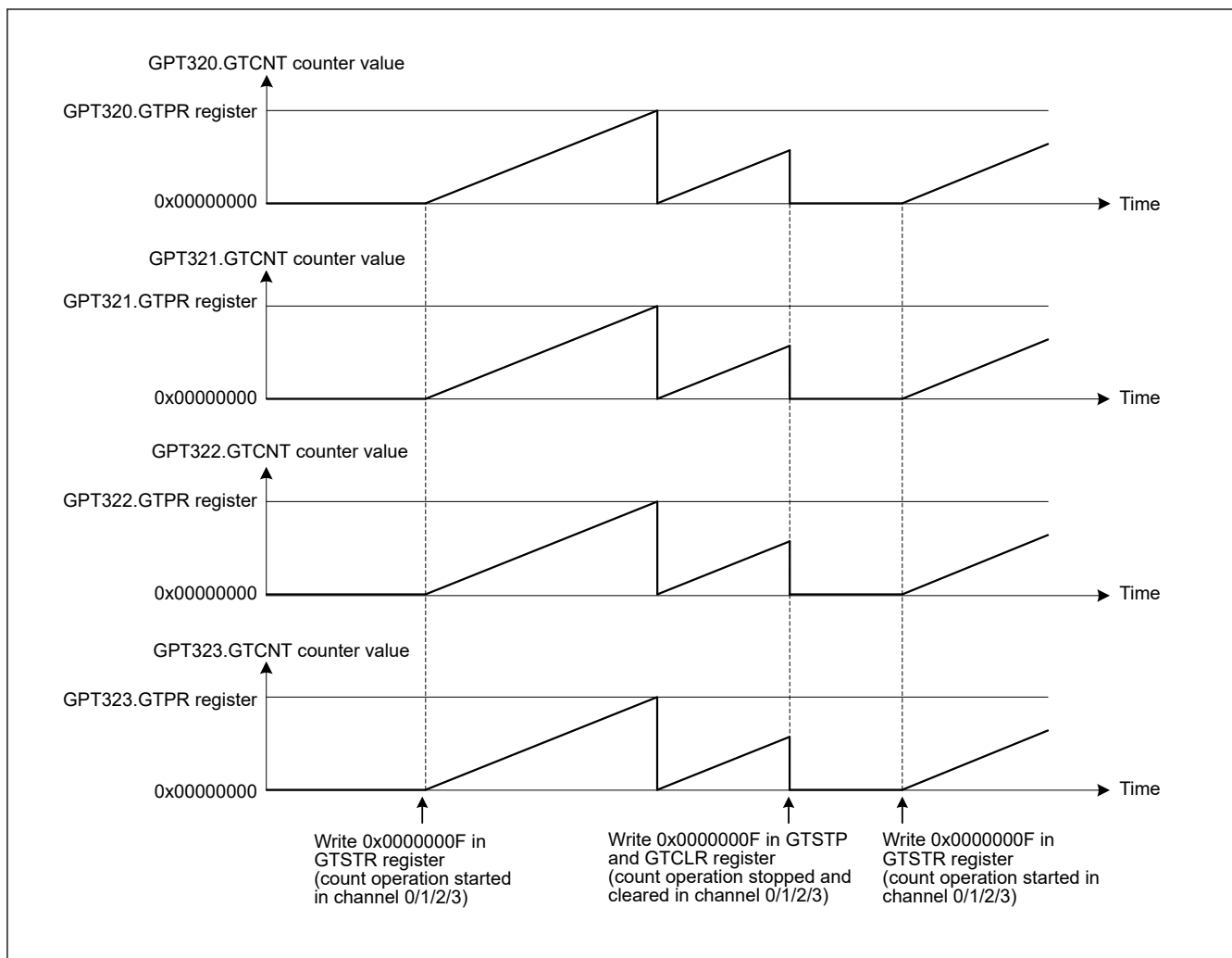
Figure 22.93 Example of a simultaneous start, stop, and clear by software with the same count cycle (GTPR register value)
