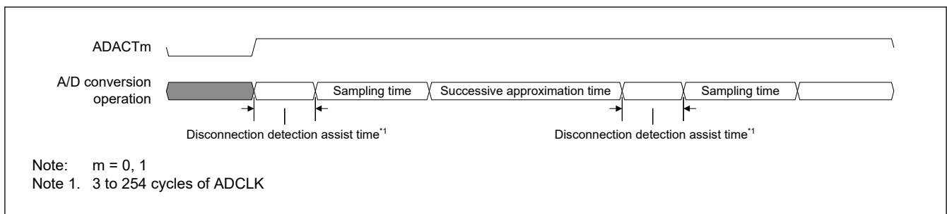
Figure 53.24 Operation of A/D conversion when disconnection detection assist function is used
