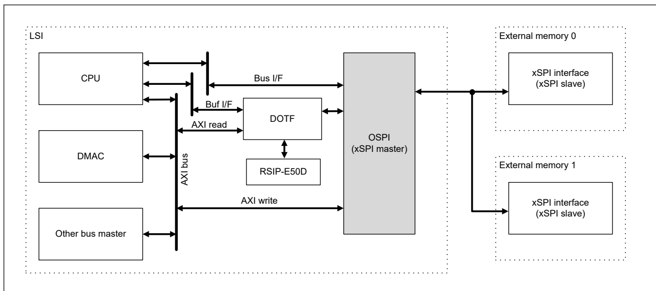
Figure 44.1 Block diagram
