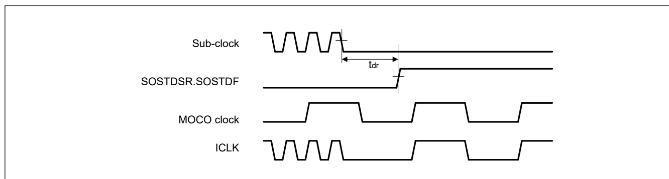
Figure 69.141 Sub-clock oscillation stop detection timing
