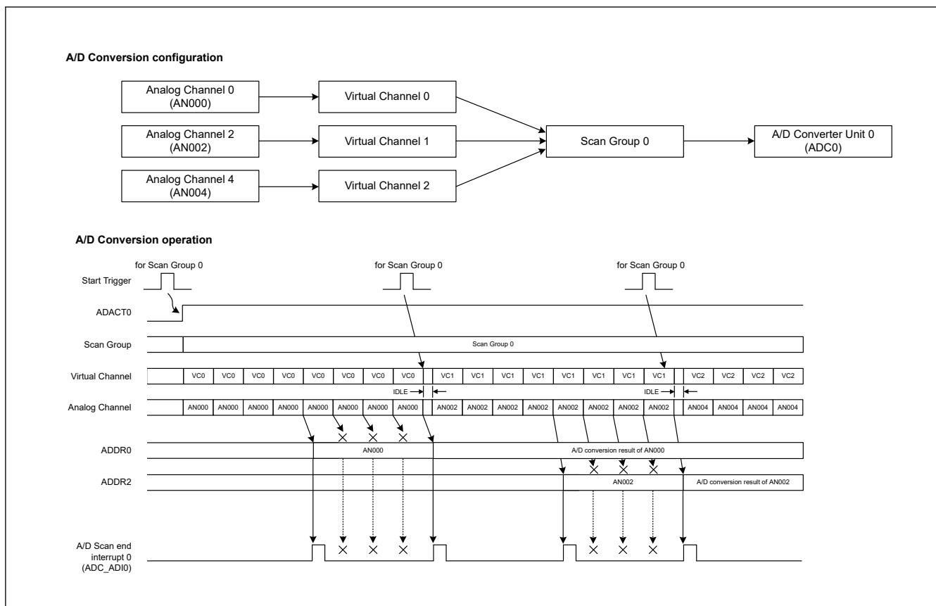
Figure 53.54 Example of data output decimation function (output every 4 times)
