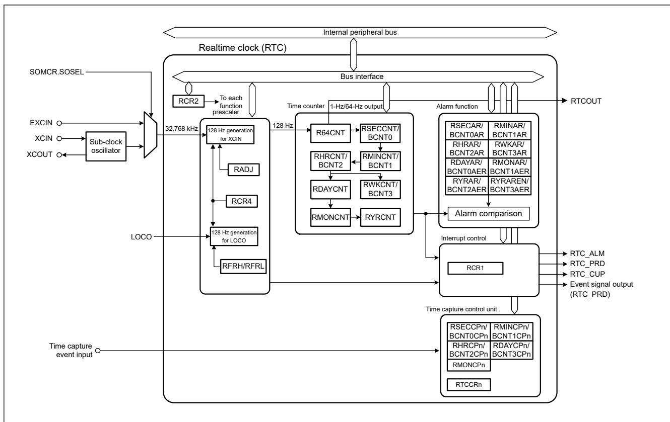
Figure 26.1 RTC block diagram
