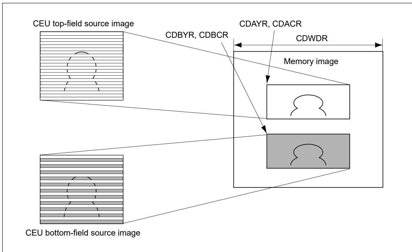
Figure 60.25 Image of storing captured both-field images in memory
