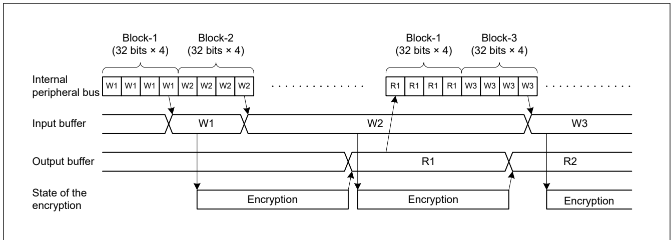
Figure 52.5 Encryption and decryption timing (AES)
