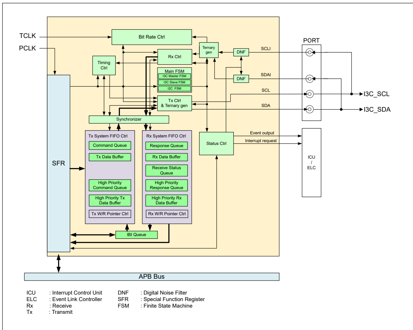
Figure 40.1 I3C block diagram
