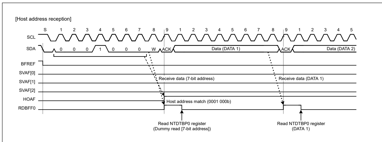
Figure 40.87 HOAF flag set timing during reception of host address
