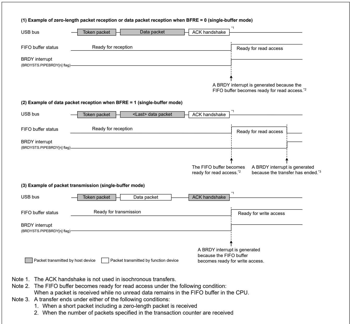
Figure 37.5 Timing of BRDY interrupt generation
