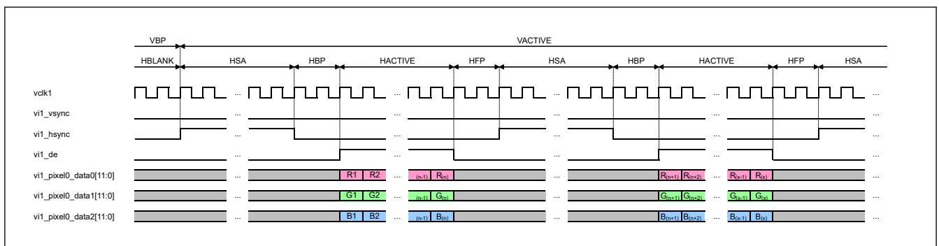
Figure 65.12 VBP end and VACTIVE start (RGB)
