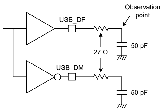
Figure 69.129 Test circuit in full-speed mode
