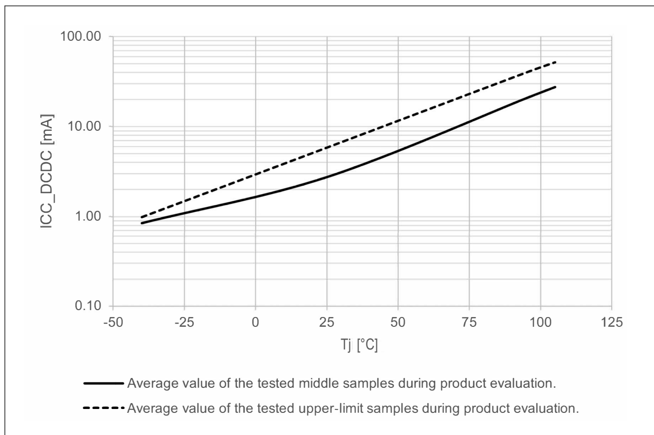
Figure 69.3 Temperature dependency in Software Standby mode ( ICC\_DCDC , SS2LP\_0 , SVSCR\_1 ) (reference data)
