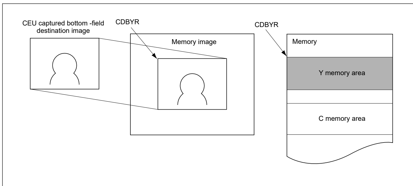
Figure 60.37 Relationship between captured bottom-field image and luminance component memory area
