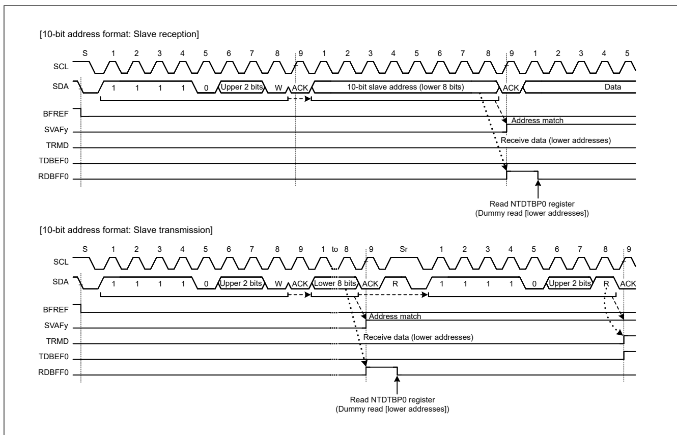
Figure 40.83 SVAfy flag set timing with 10-bit address format selected
