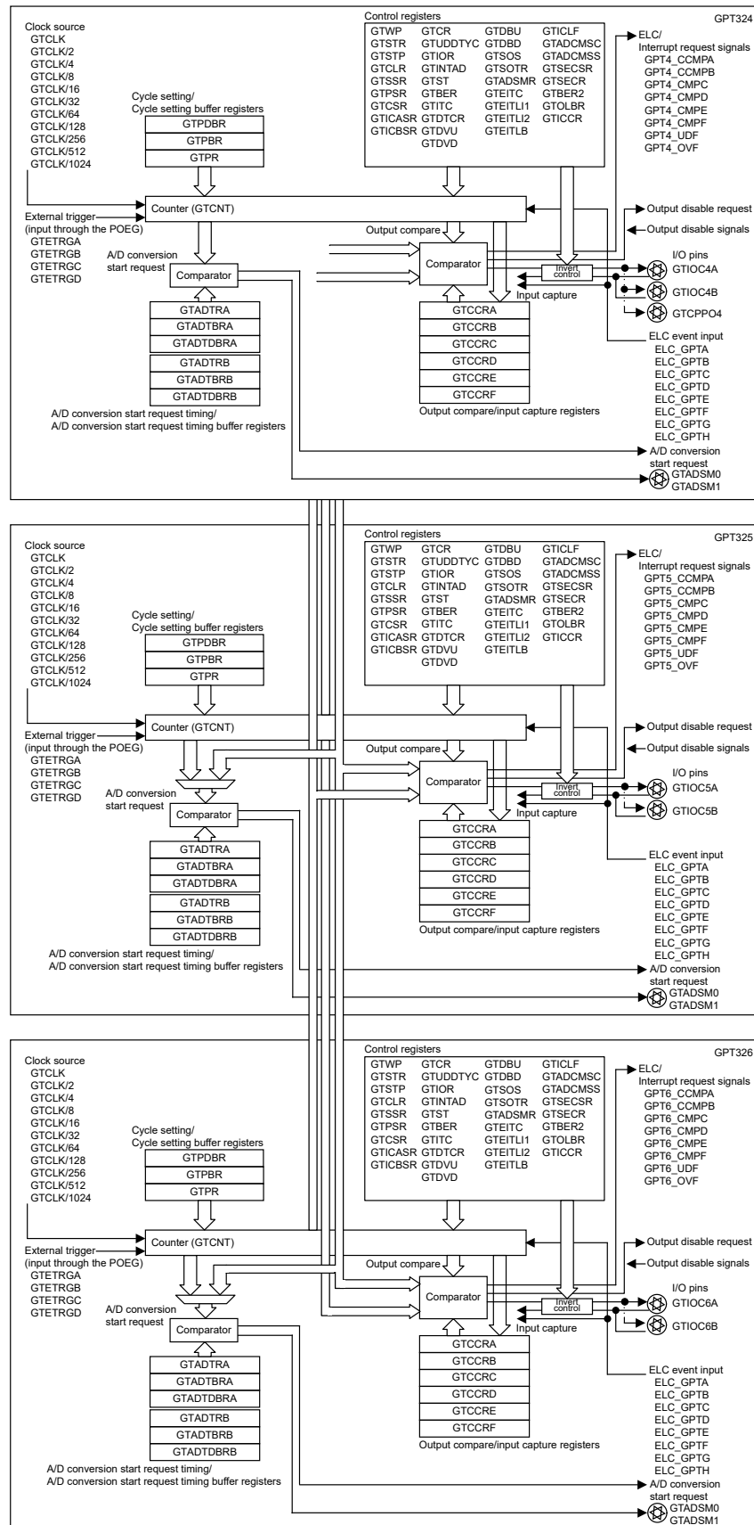
Figure 22.2 GPT block diagram (Saw-wave PWM mode 1, 2, Saw-wave one-shot pulse mode, Triangle-wave PWM mode1,2,3, Complementary PWM mode 1, 2, 3, 4)
