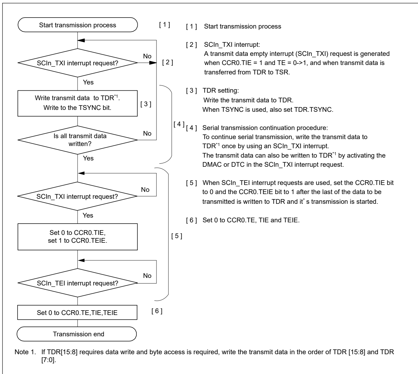
Figure 38.51 Example of Serial Transmission Flowchart in Manchester Mode
