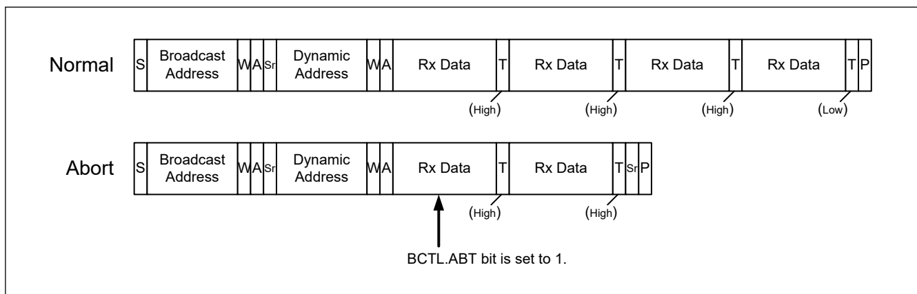
Figure 40.117 Abort operation of SDR read transfer
