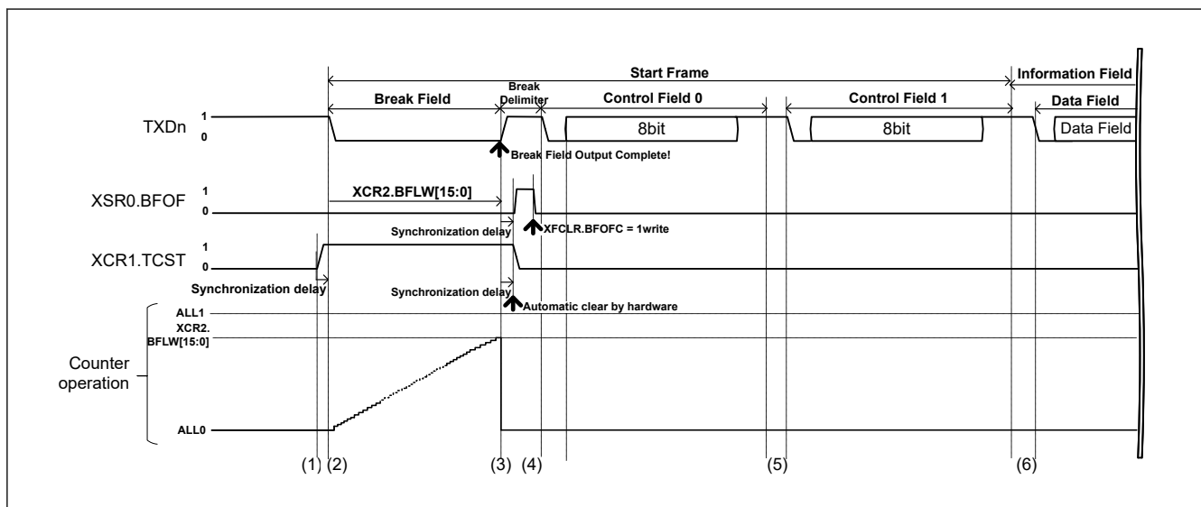
Figure 38.102 Start Frame Transmission Example
