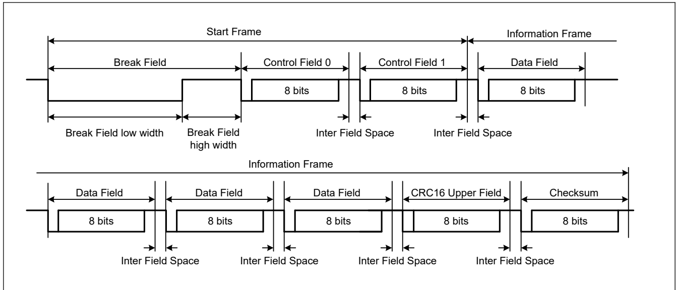
Figure 38.101 Simple LIN Protocol Example
