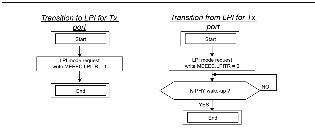
Figure 33.10 LPI transition for Tx port
