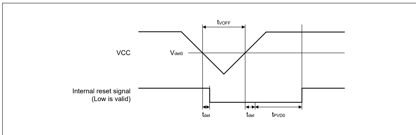
Figure 69.143 Voltage detection circuit timing ( V_{det0} )
