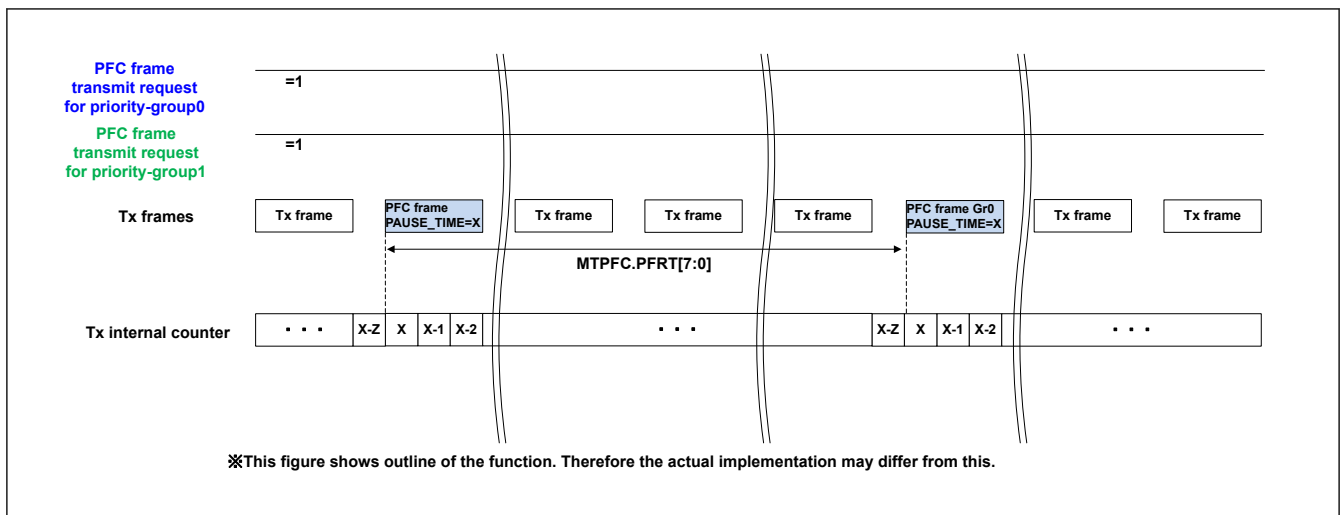
Figure 33.20 Transmitting PFC frame (part 2)
