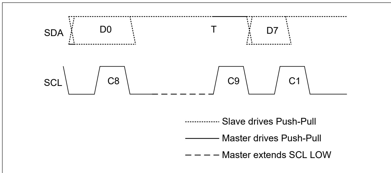
Figure 40.98 Master clock stalling in T-bit before next read data
