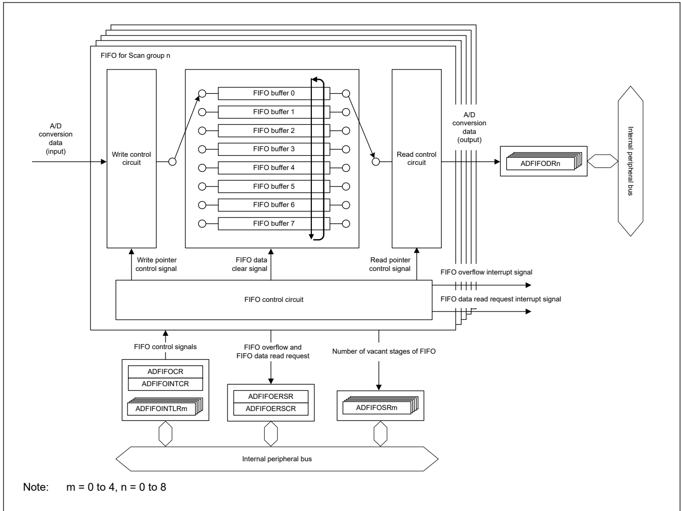
Figure 53.53 The block diagram of FIFO
