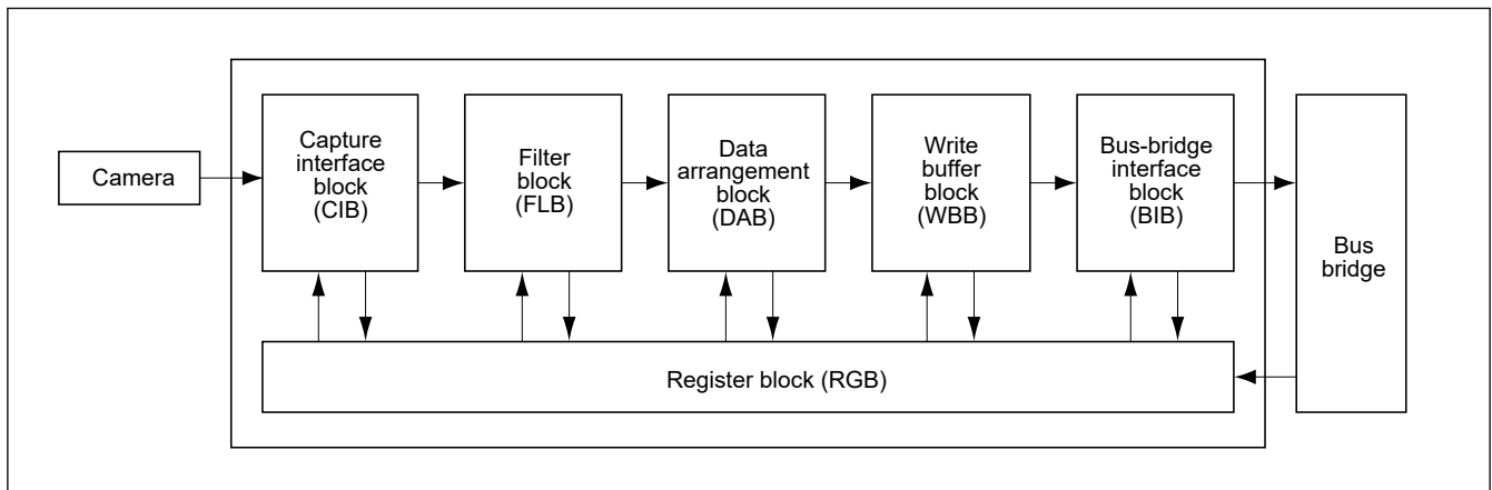
Figure 60.1 Block diagram of CEU
