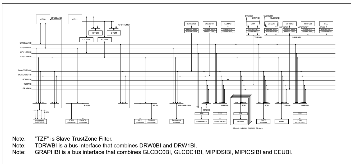
Figure 15.1 System bus connection
