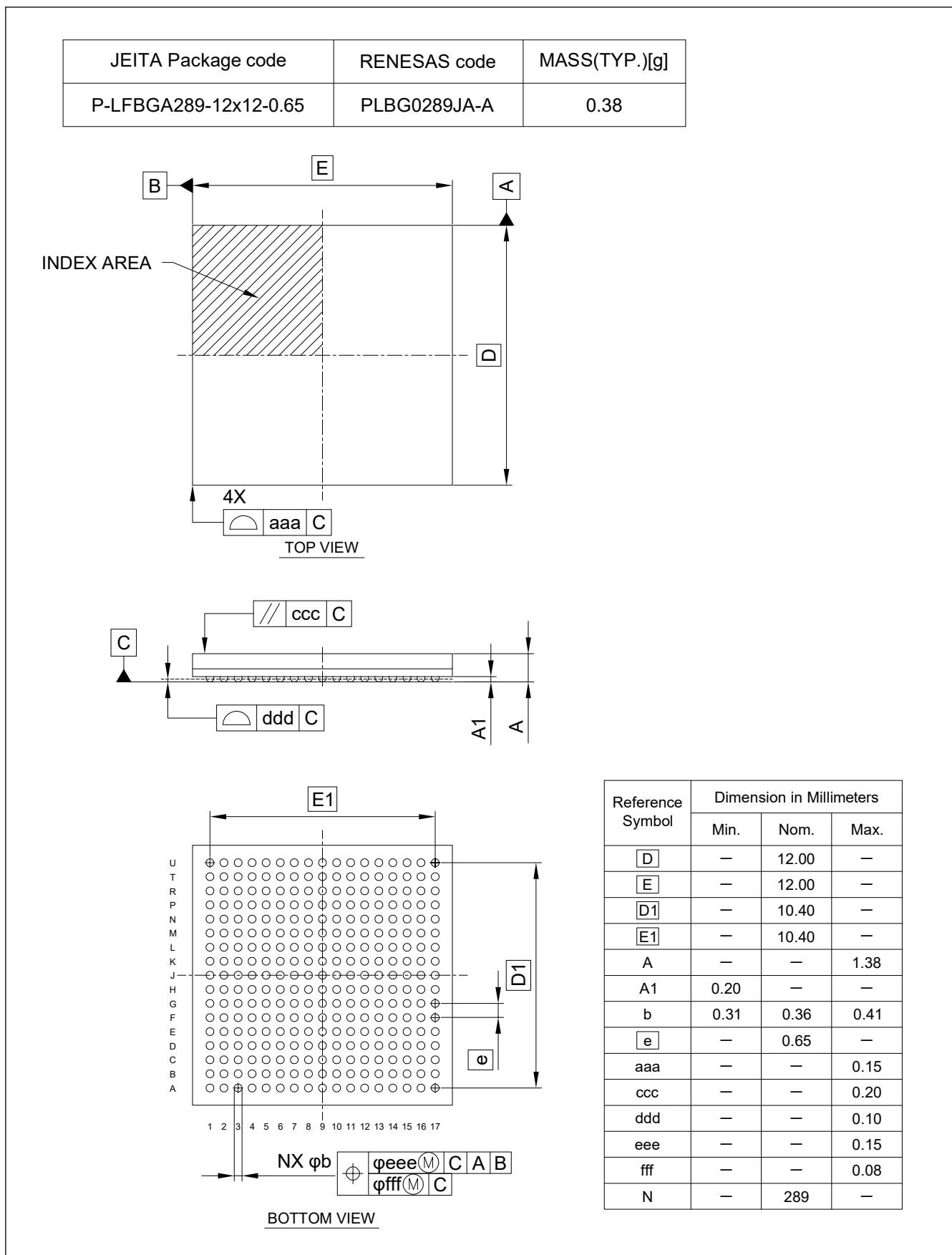
Figure A2.1 BGA 289-pin
