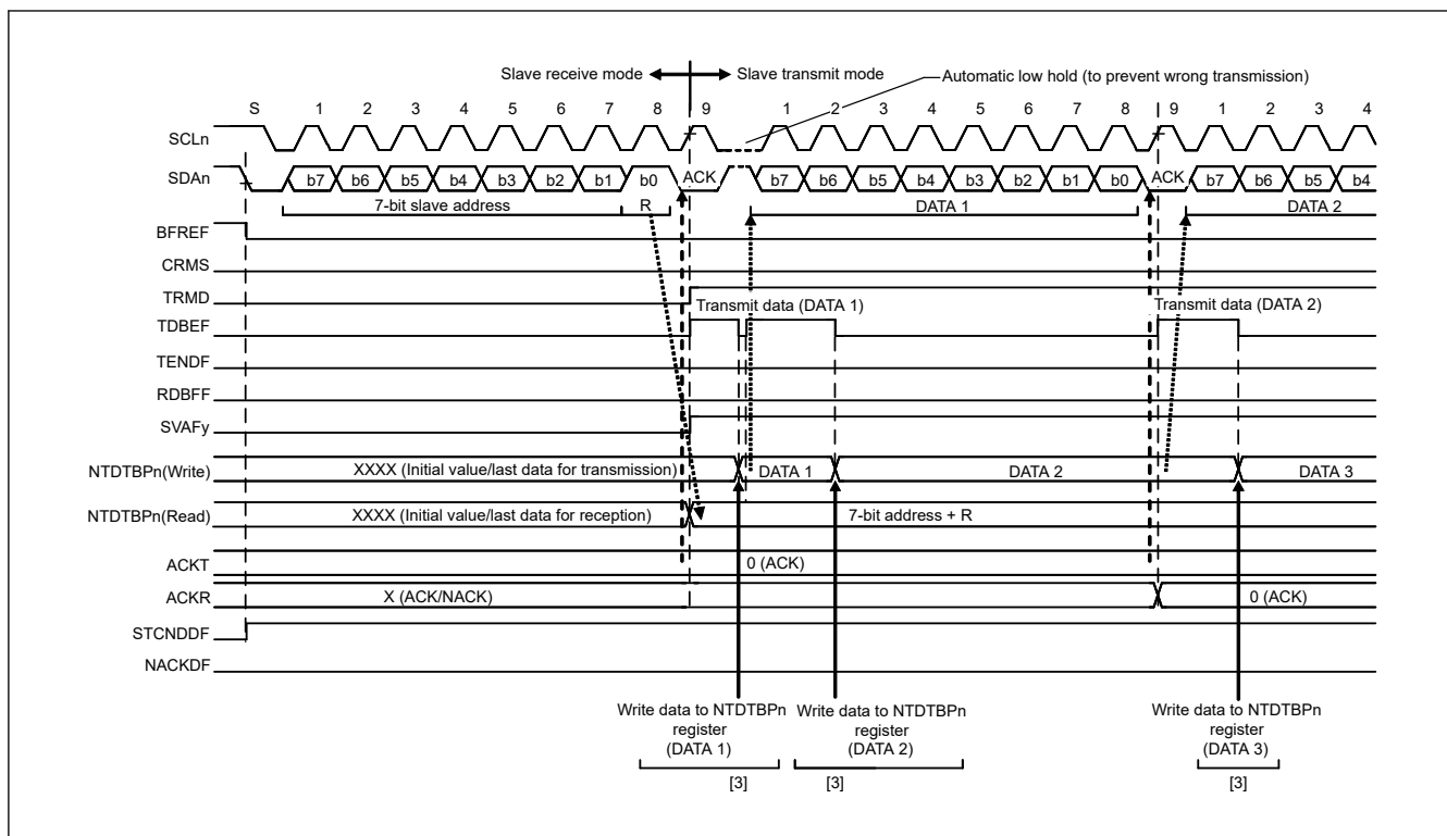
Figure 40.39 Slave transmit operation timing (1) (7-bit address format)
