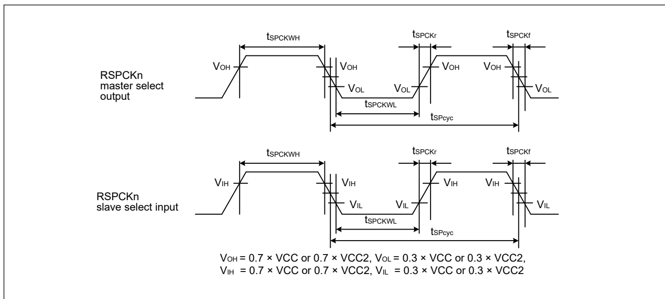
Figure 69.75 SPI clock timing
