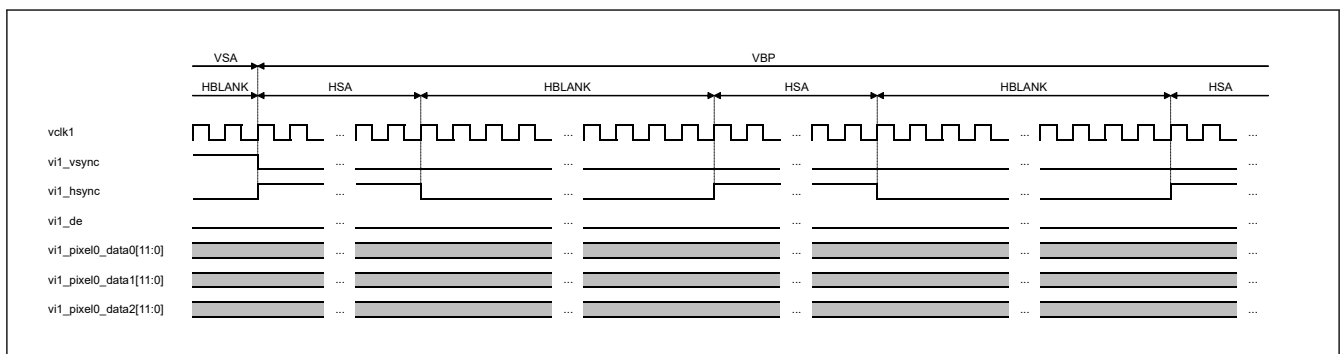
Figure 65.11 VSA end and VBP start
