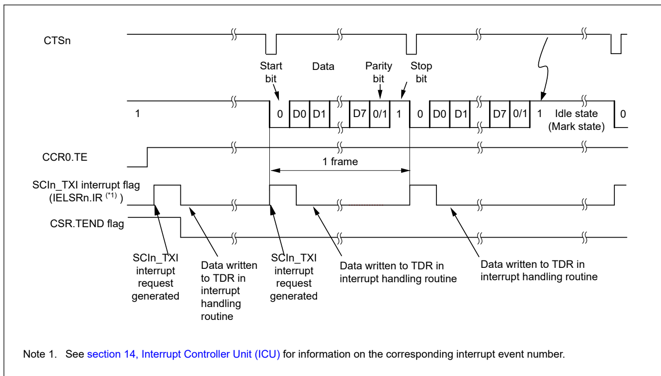
Figure 38.13 Example operation for serial transmission in Asynchronous mode (2) with 8-bit data, parity bit, one stop bit, CTS function used, and at the beginning of transmission
