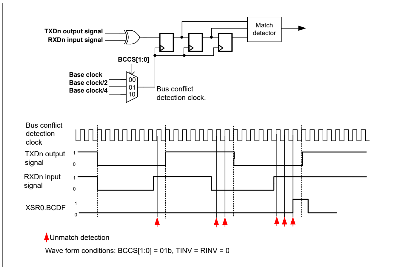
Figure 38.110 Operation Example of the Bus Conflict Detection Function
