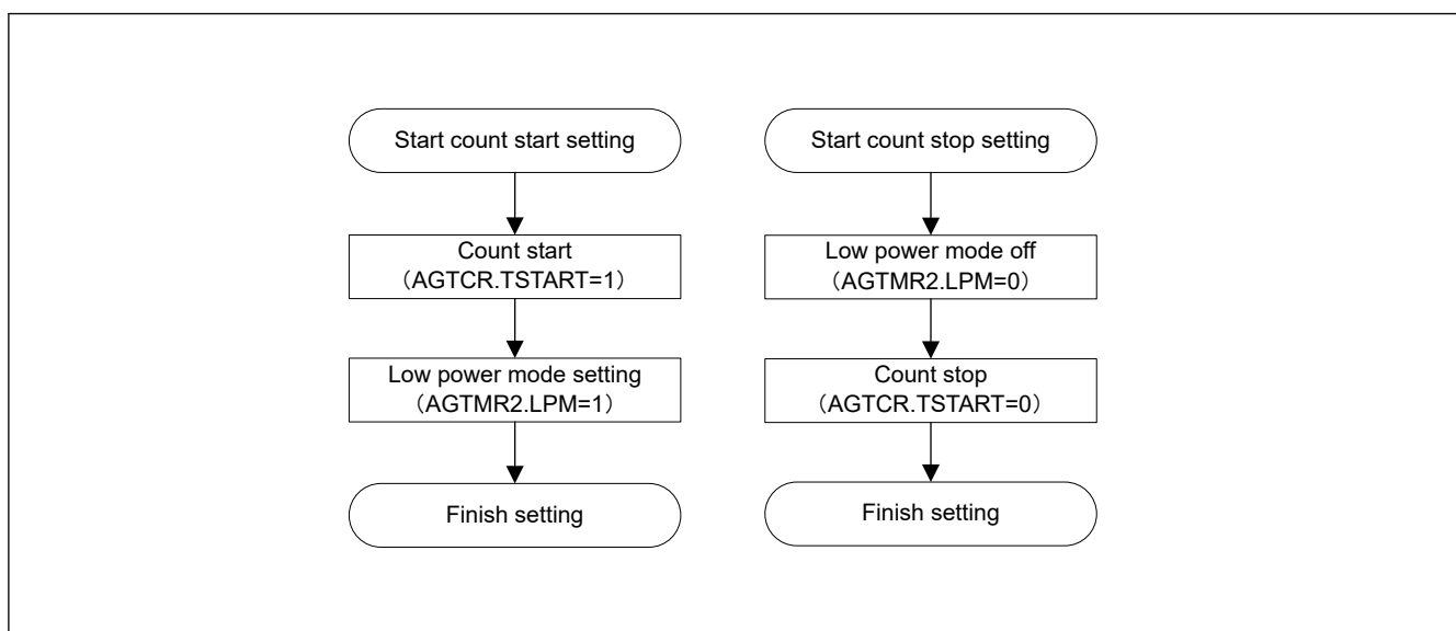
Figure 24.2 LPM how to write flow chart
