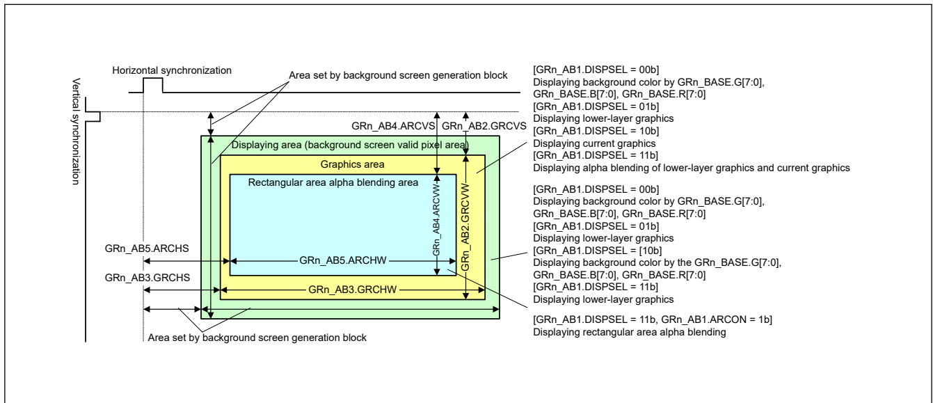
Figure 63.10 Selection of graphics display plane
