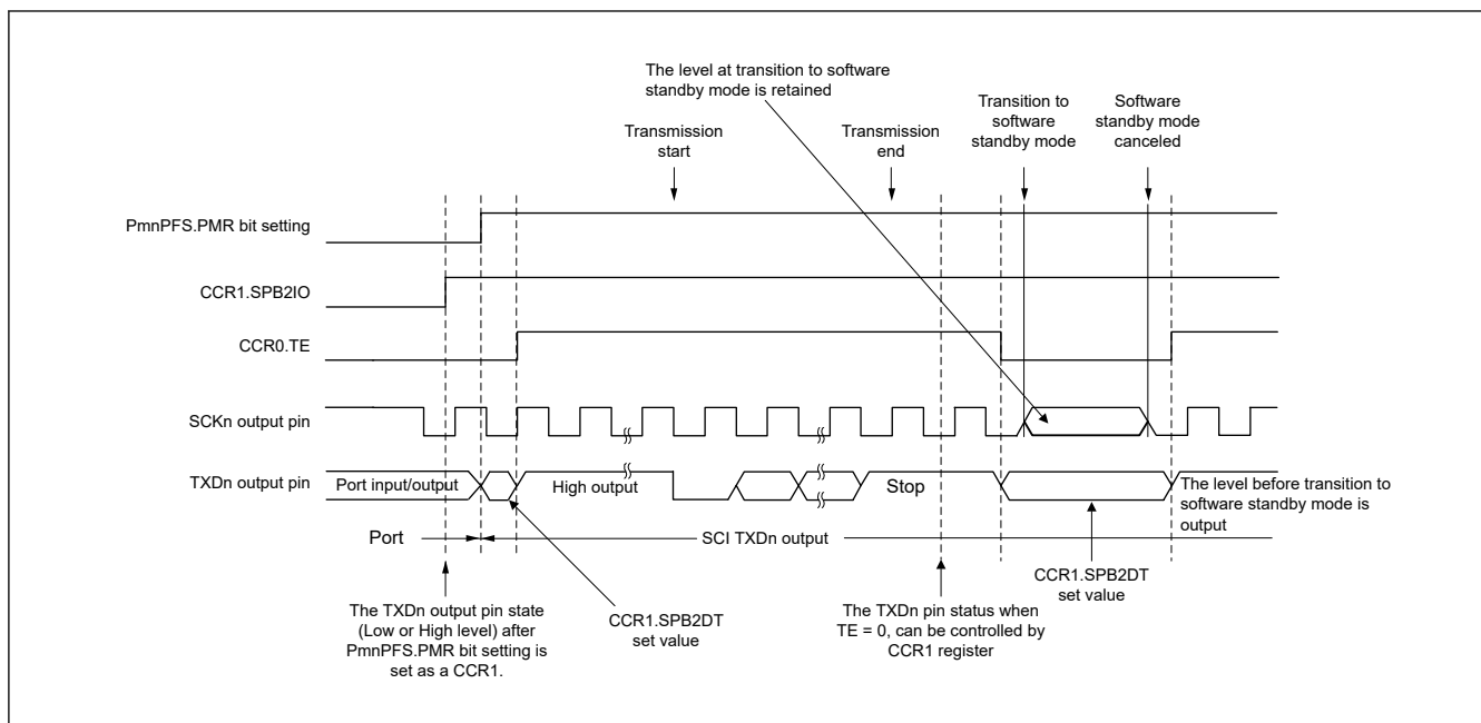
Figure 38.118 Port Pin States during Transition to Software Standby Mode (Internal Clock, Asynchronous Transmission)
