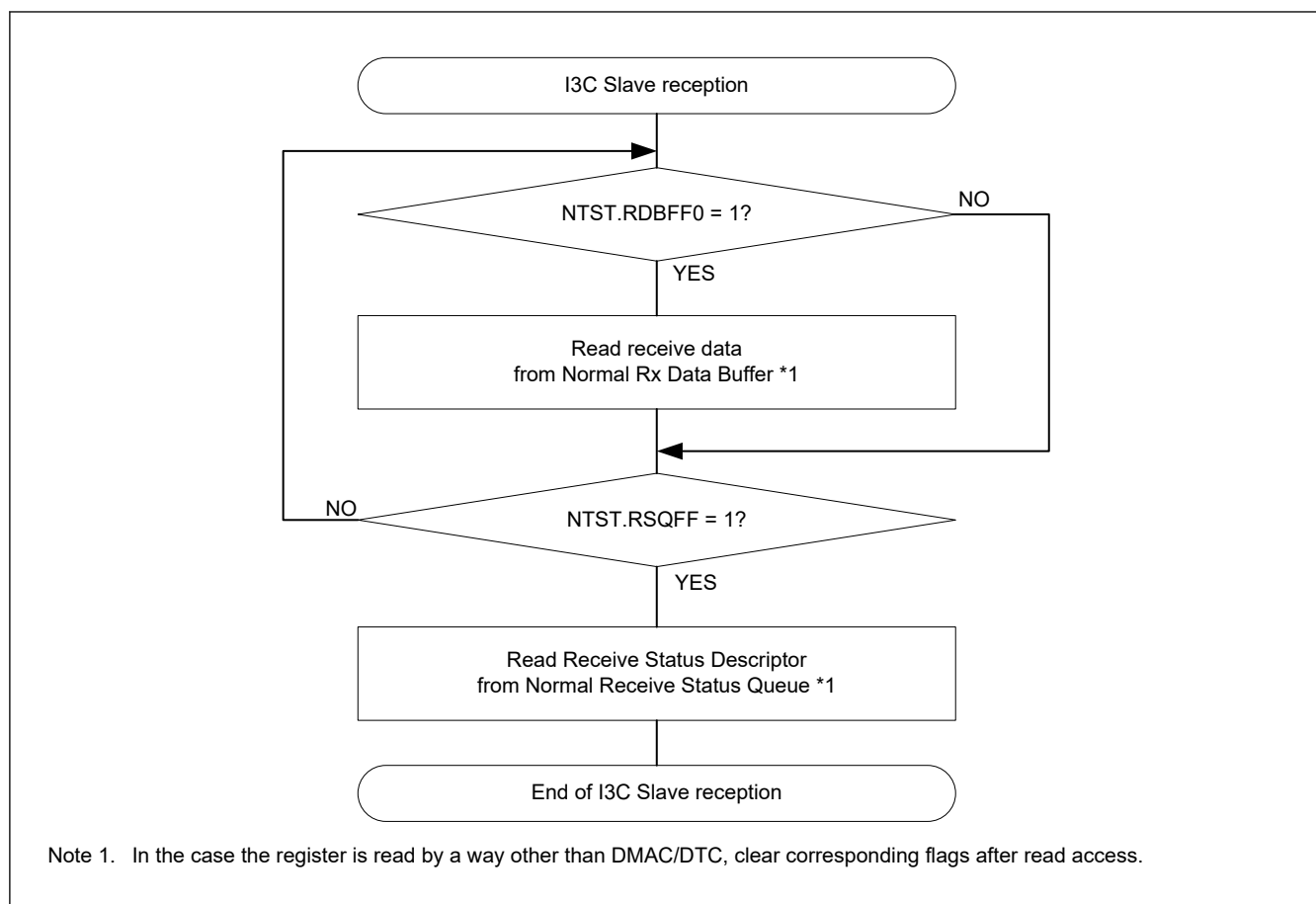
Figure 40.155 Example of I3C slave reception flowchart (normal FIFO buffer transfer)
