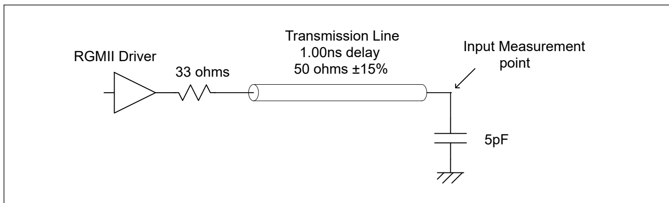
Figure 69.122 RGMII output timing measurement conditions
