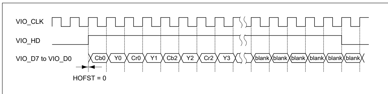
Figure 60.20 Timing when HD is data enable signal (8-bit interface)
