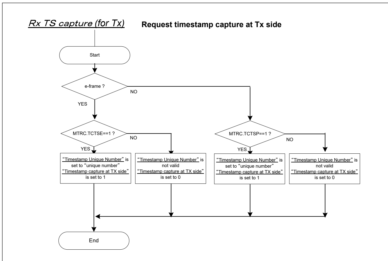
Figure 33.25 Rx timestamp capture flow
