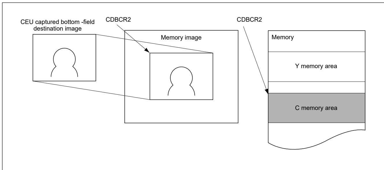
Figure 60.54 Relationship between captured bottom-field image and chrominance component memory area
