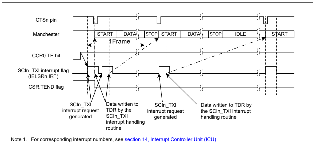
Figure 38.53 Example of Start-of-Transmission Operation for Serial Transmission in Manchester Mode (Without Preface but with the CTS Function)
