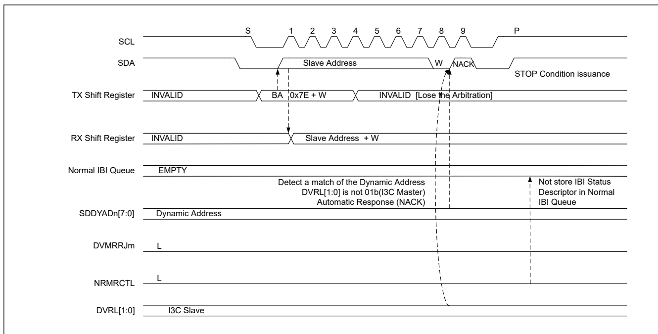
Figure 40.107 Mastership request : NACK (Device Role[1:0] is not 01 (I3C master)) and NRMRCTL = 0
