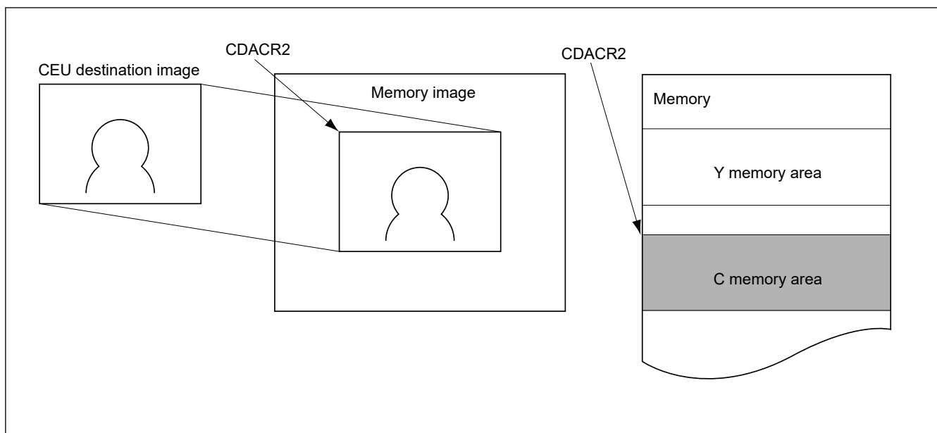
Figure 60.51 Relationship between captured image and chrominance component memory area
