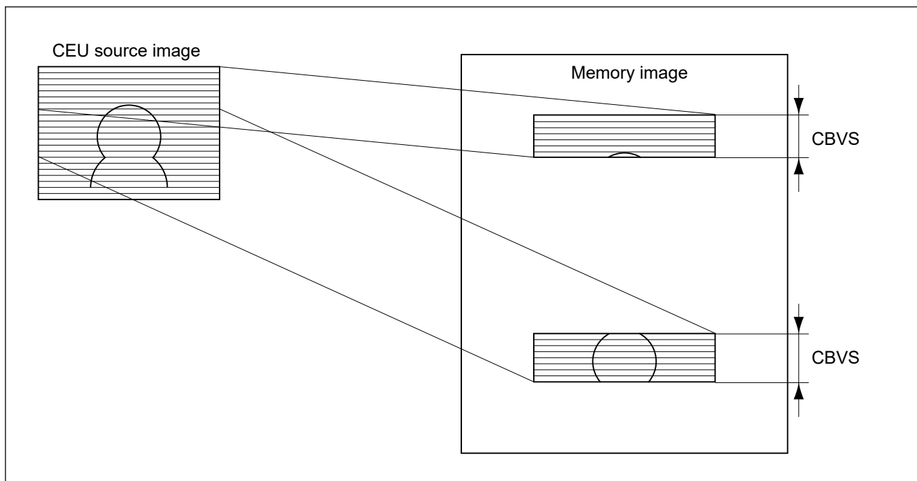
Figure 60.40 Image of storing captured image in memory by bundle write
