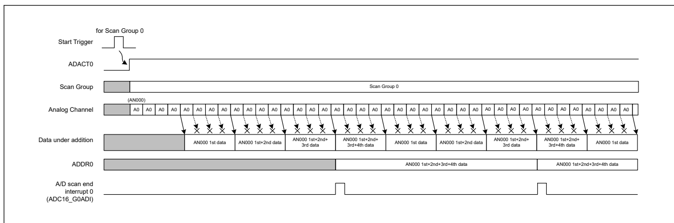
Figure 53.55 Example of data output decimation function (output every 4 times) when addition function is enabled (addition count is 4 times)
