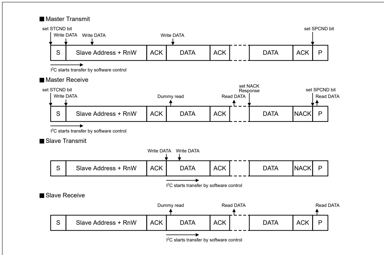
Figure 40.66 Data handler with single buffer transfer
