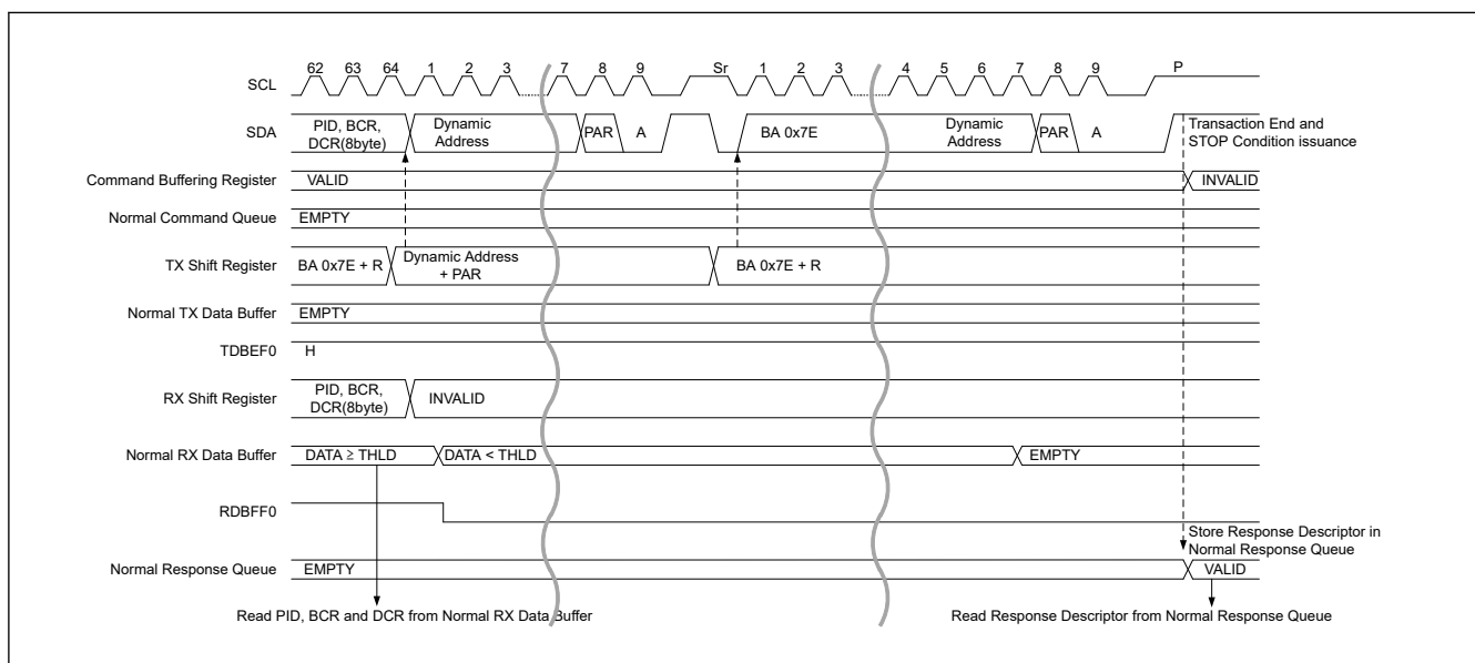
Figure 40.14 Dynamic address assign procedure (ENTDAA CCC) timing (3/3)
