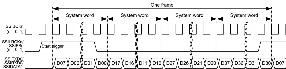
Figure 46.41 TDM format (without padding: system word length = data word length)
