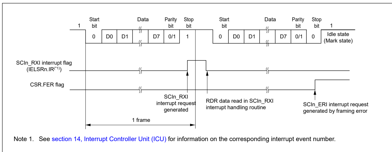
Figure 38.19 Example of SCI operation for serial reception in Asynchronous mode (1) when the RTS function is not used, and with 8-bit data, parity bit, and 1 stop bit
