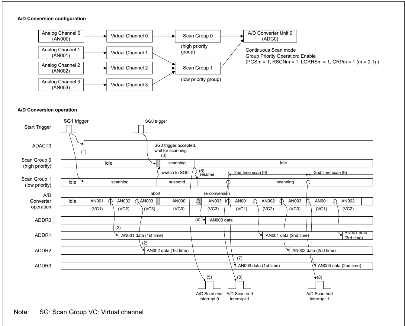
Figure 53.29 Example of group priority operation in SAR mode – Continuous scan mode (2 groups)
