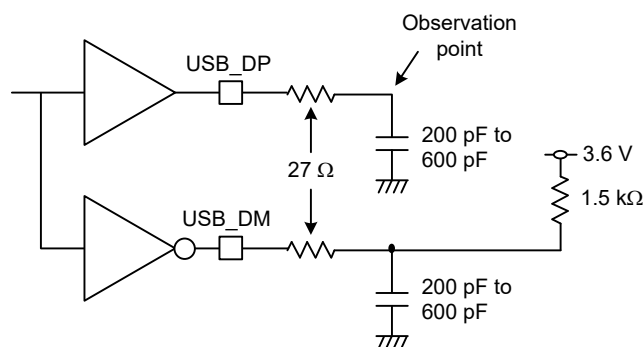
Figure 69.127 Test circuit in low-speed mode
