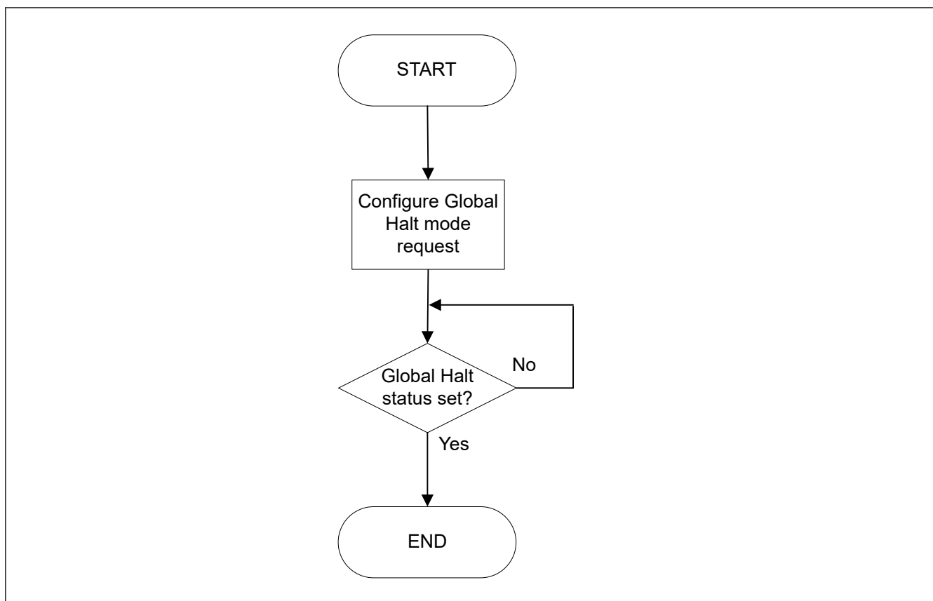
Figure 41.7 Procedure for entering Global Halt mode
