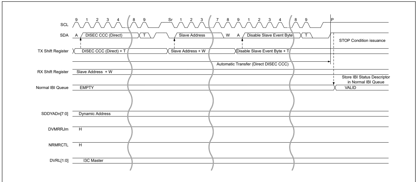
Figure 40.109 Mastership request : NACK (DVMRRJ = 1) and NRMRACTL = 1 (2/2)
