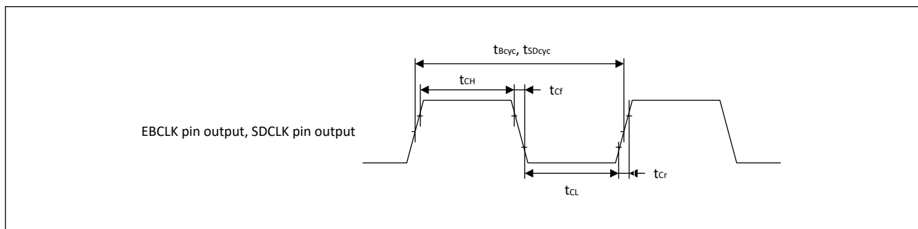
Figure 69.25 EBCLK and SDCLK output timing
