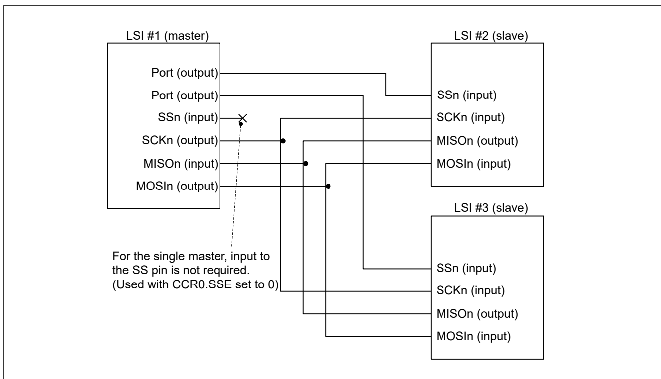
Figure 38.98 Example connections using simple SPI mode in single master mode with CCR0.SSE bit = 0
