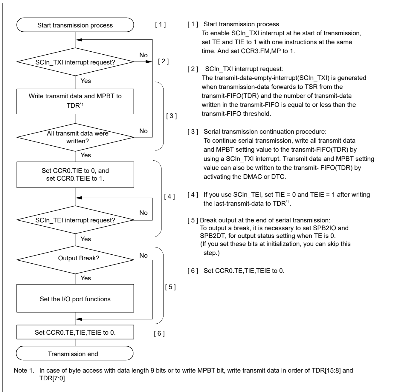
Figure 38.38 Example flow of serial transmission in multi-processor mode with FIFO selected
