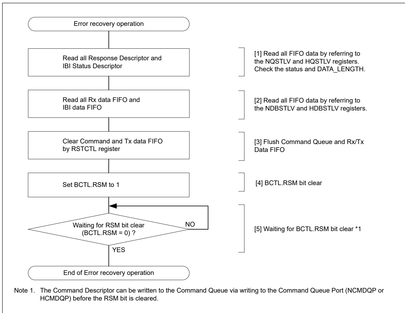
Figure 40.122 Example of error recovery operation flowchart for I3C master
