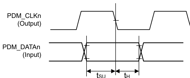
Figure 69.125 Receive Timing (Synchronized with the fall of PDM_CLKn)
