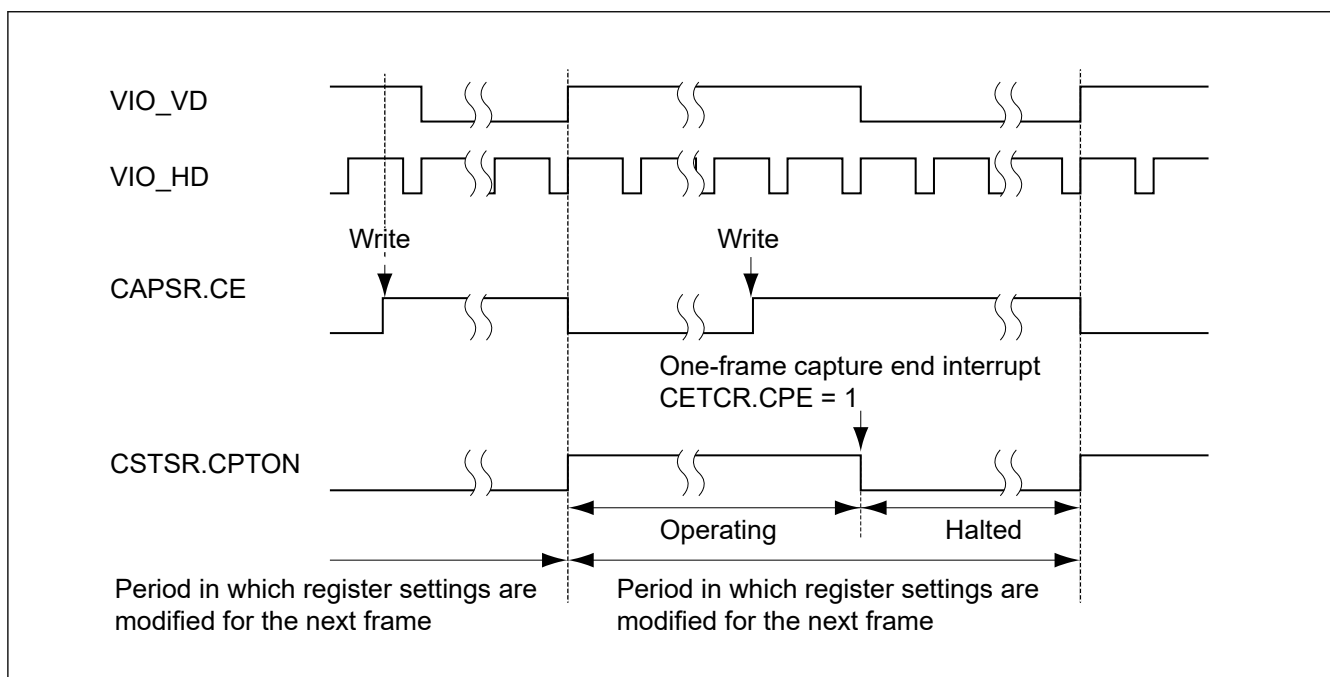
Figure 60.7 Timing of modifying CE bit and register setting in one frame capture
