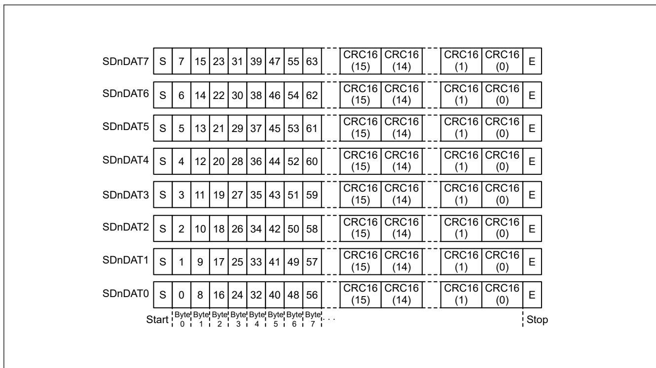
Figure 47.4 SDnDAT in 8-bit width mode
