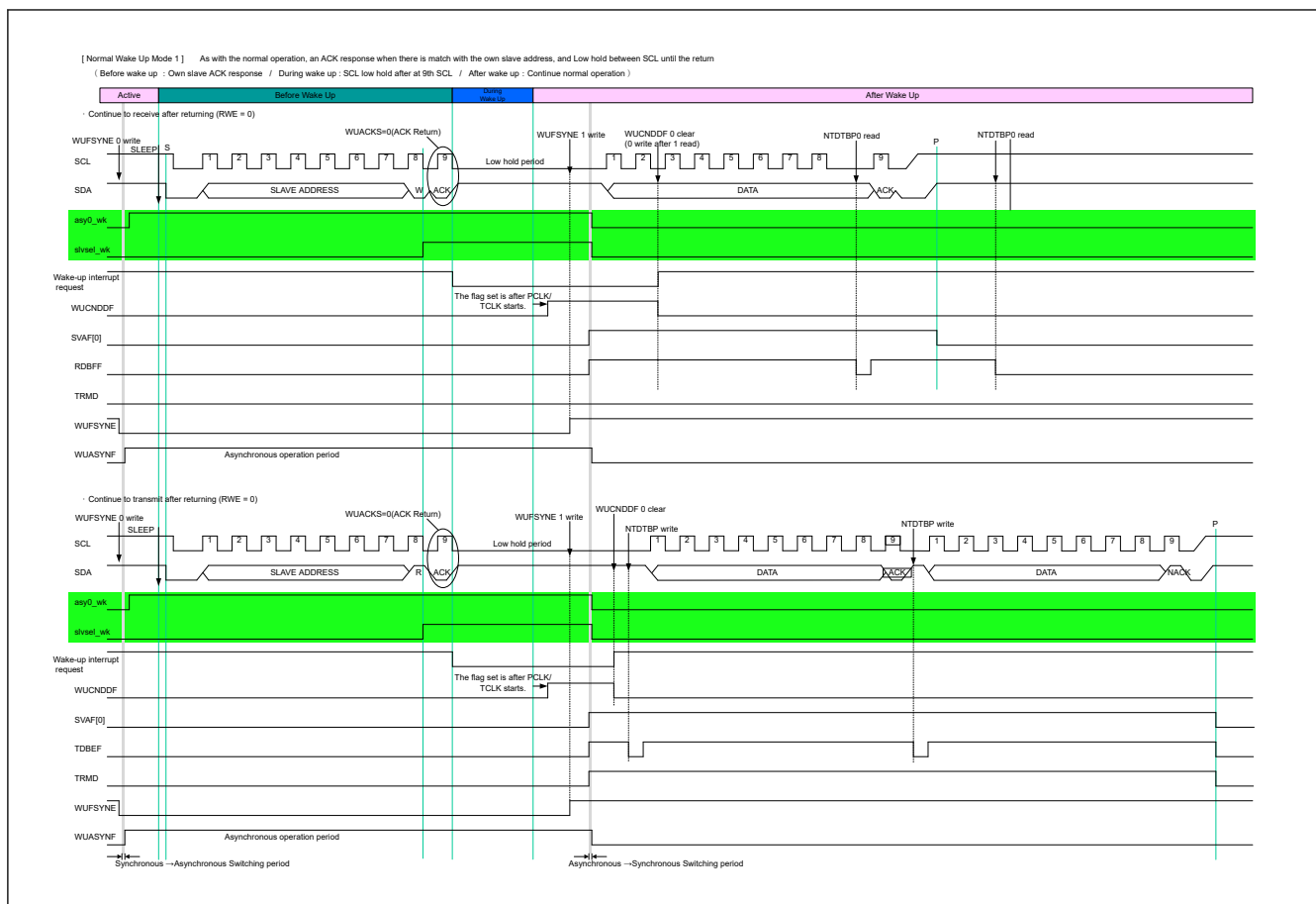
Figure 40.128 Timing of normal wake up mode 1
