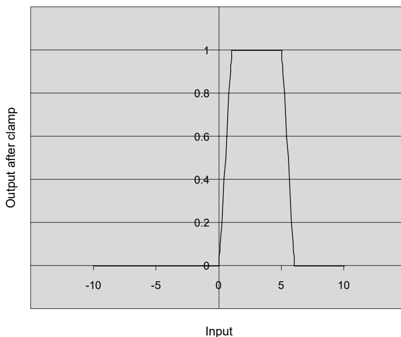
Figure 62.11 Band filter output after clamp with w = 7
