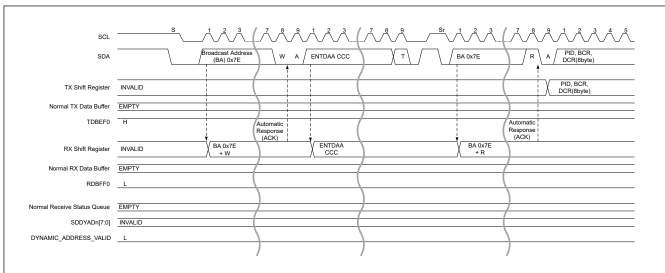
Figure 40.41 Dynamic address assign procedure (ENTDAA CCC) timing (1/3)
