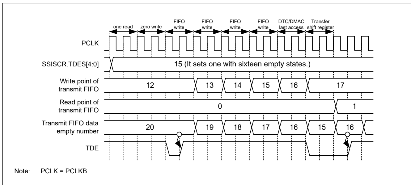
Figure 46.29 Timing diagram for setting and clearing TDE
