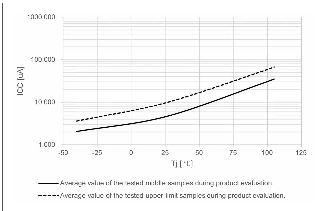
Figure 69.8 Temperature dependency in Deep Software Standby mode 2 (reference data)
