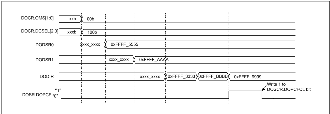
Figure 57.6 Example of Operation in Data Comparison Mode (Detection condition: Inside window)
