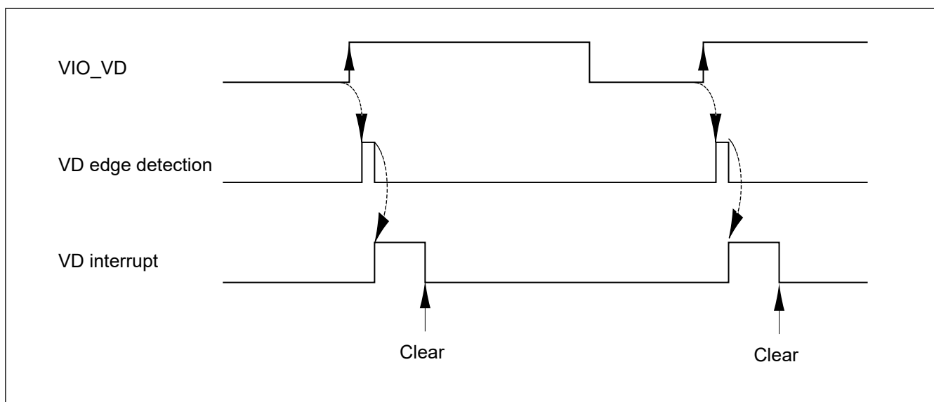
Figure 60.14 Relationship between VIO_VD and VD interrupt when VD is high-active (in data enable fetch mode)
