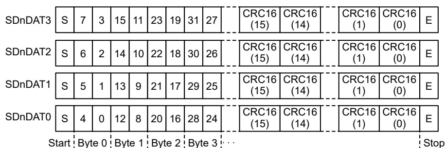
Figure 47.3 SDnDAT in 4-bit width mode
