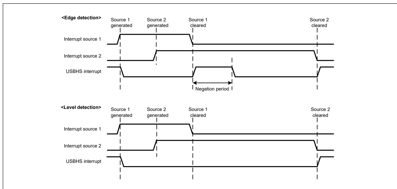
Figure 37.3 USBHS interrupt operation
