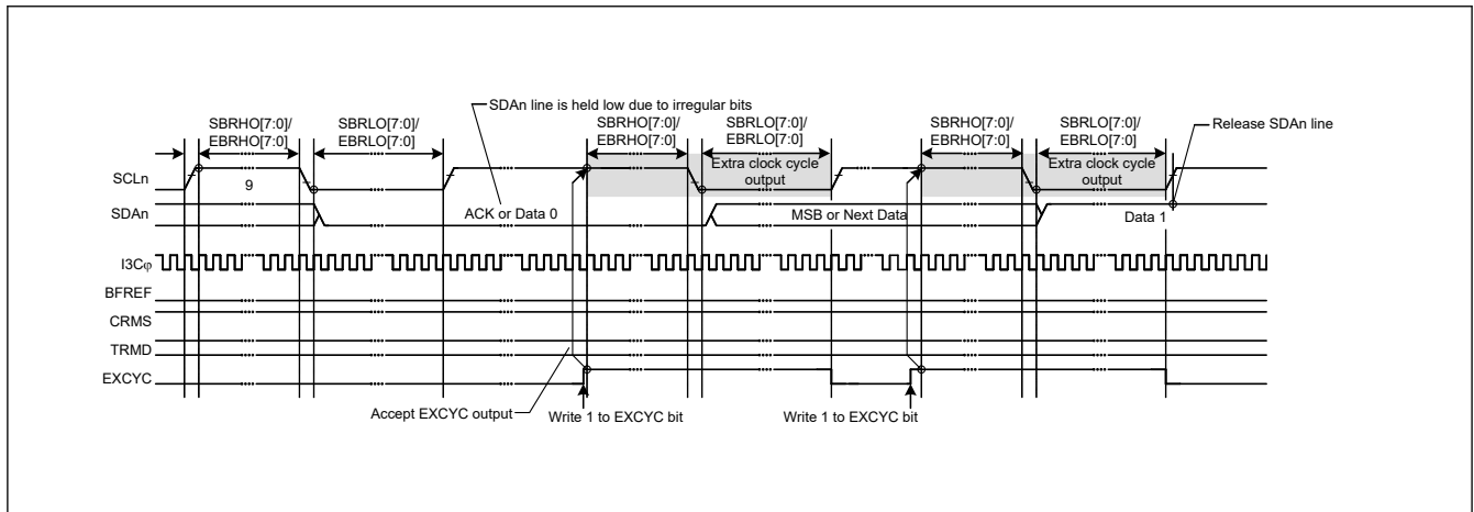
Figure 40.113 Extra SCL clock cycle output function (EXCYC bit)
