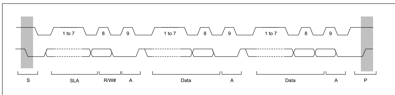
Figure 40.70 I 2 C bus timing (SLA = 7 bits)
