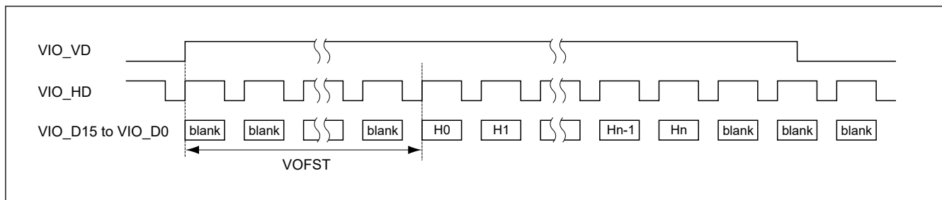
Figure 60.17 Vertical offset
