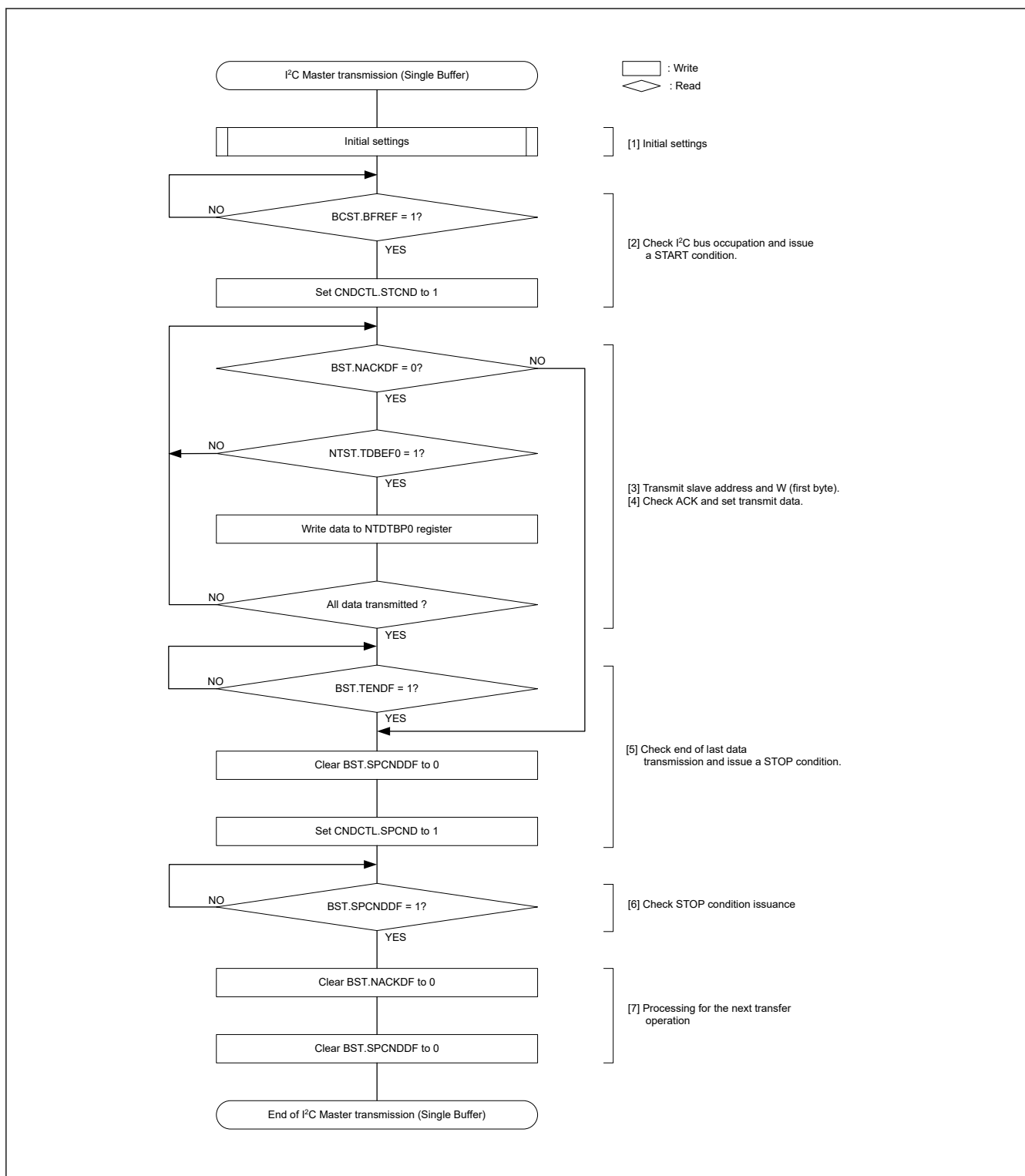
Figure 40.143 Example of I 2 C master transmission flowchart (single buffer transfer)
