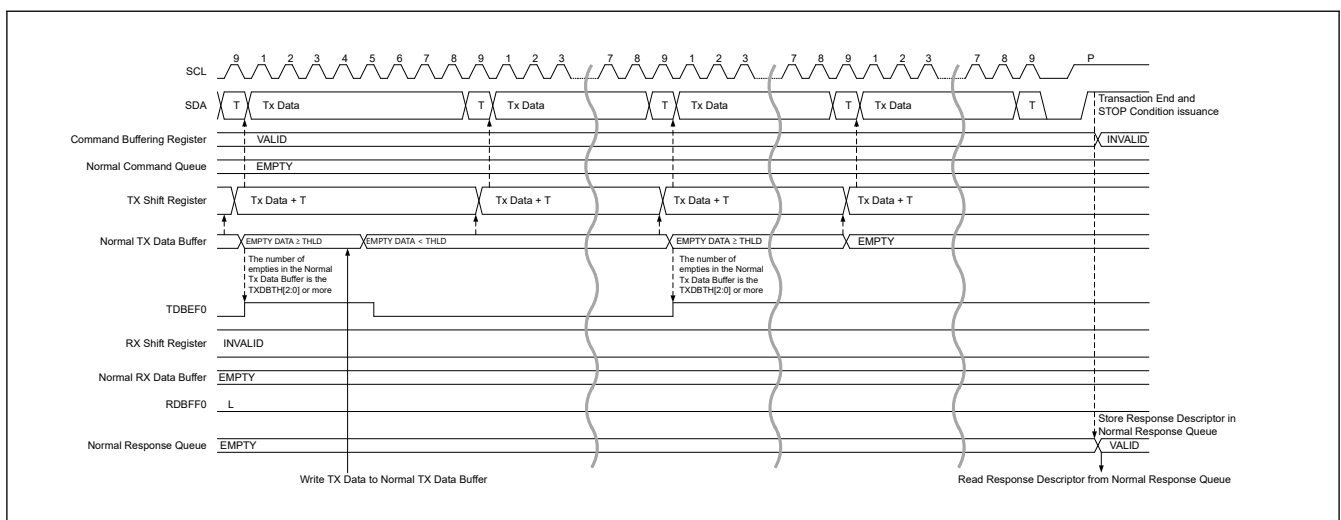
Figure 40.17 SDR data write transfer timing (2/2)
