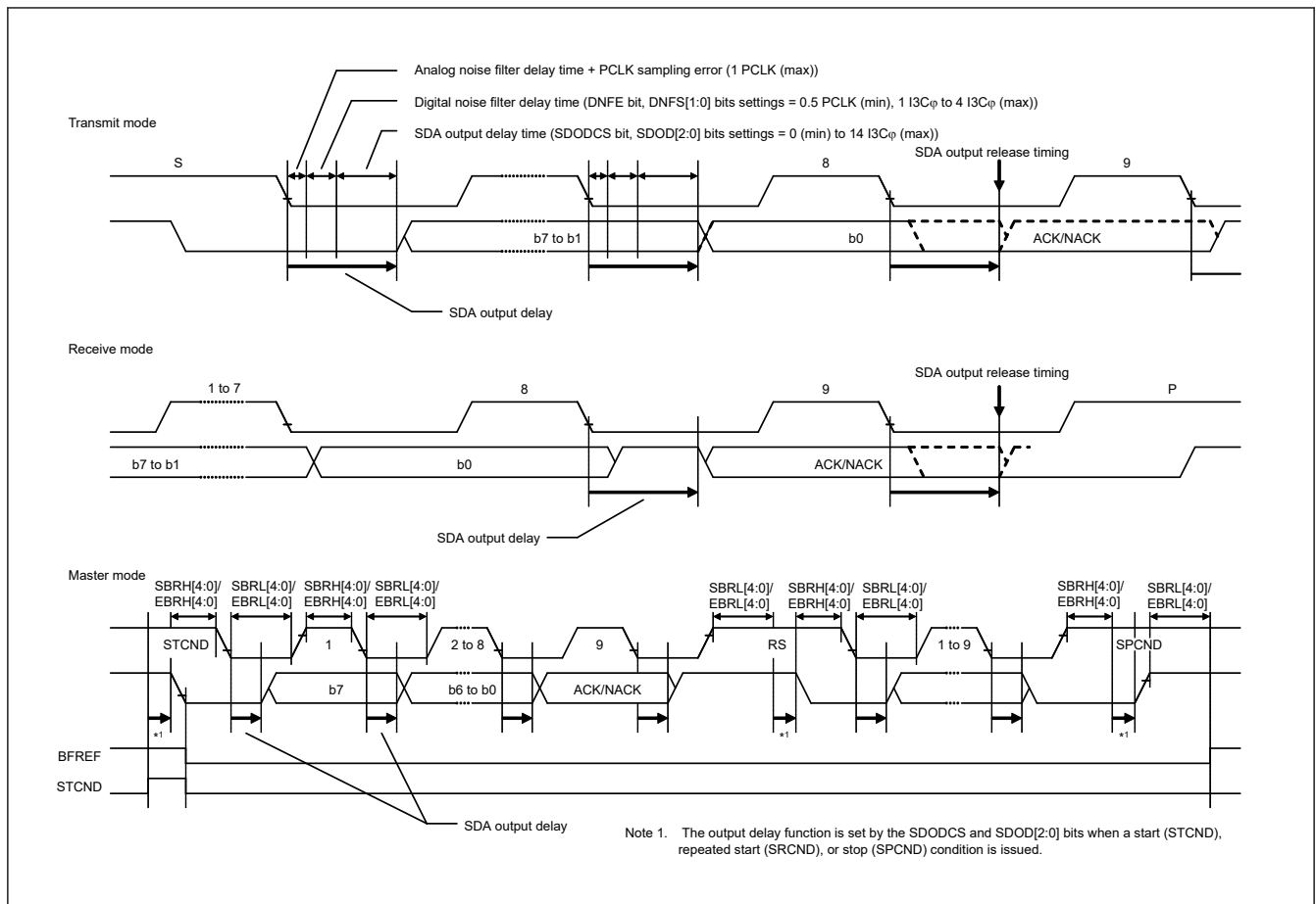
Figure 40.138 SDA output delay facility
