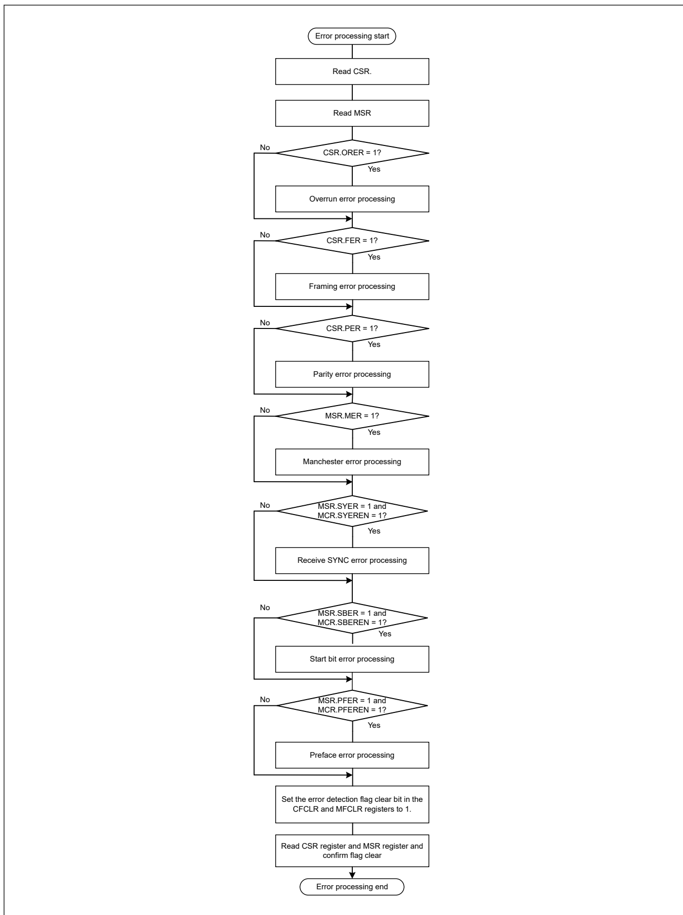
Figure 38.58 Example of Serial Reception Flowchart in Manchester Mode (Error Processing)
