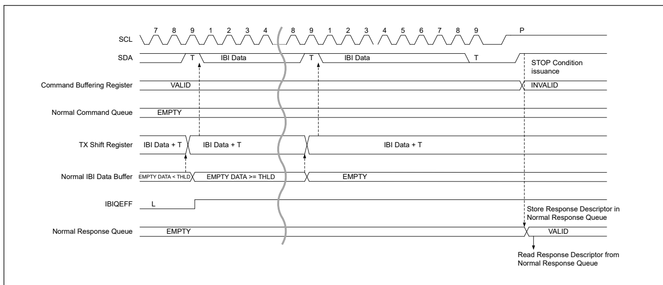
Figure 40.64 I3C slave IBI transfer timing (2/2)
