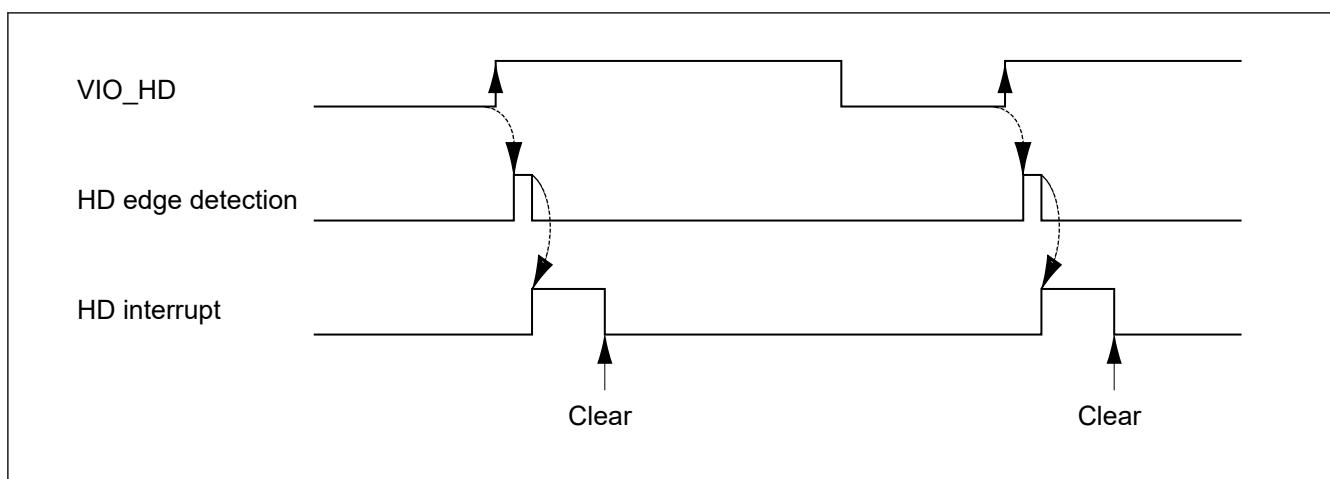
Figure 60.16 Relationship between VIO_HD and HD interrupt when HD is high-active
