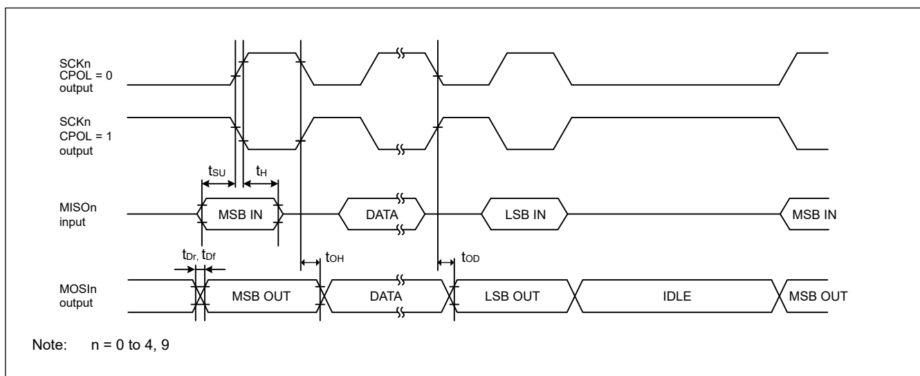
Figure 69.70 SCI simple SPI mode timing for master when CPHA = 0
