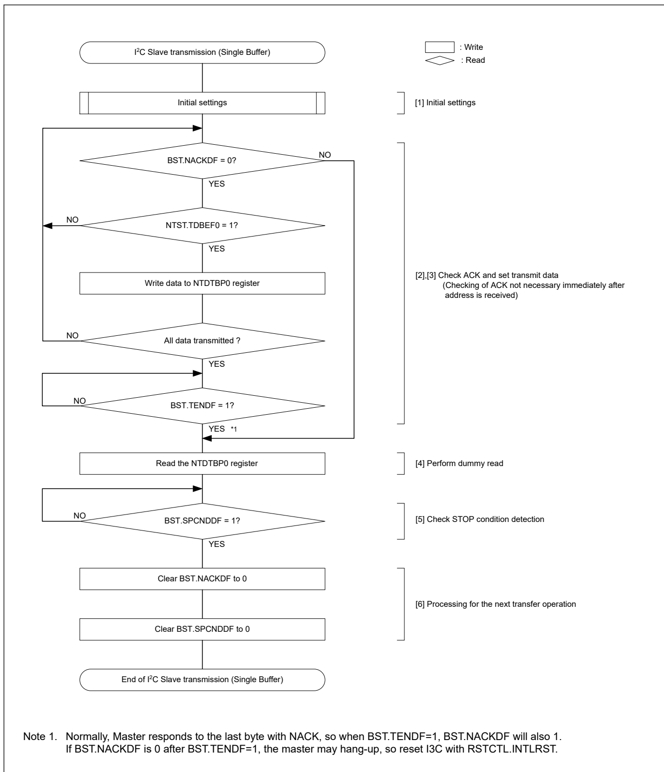
Figure 40.152 Example of I 2 C slave transmission flowchart (single buffer transfer)
