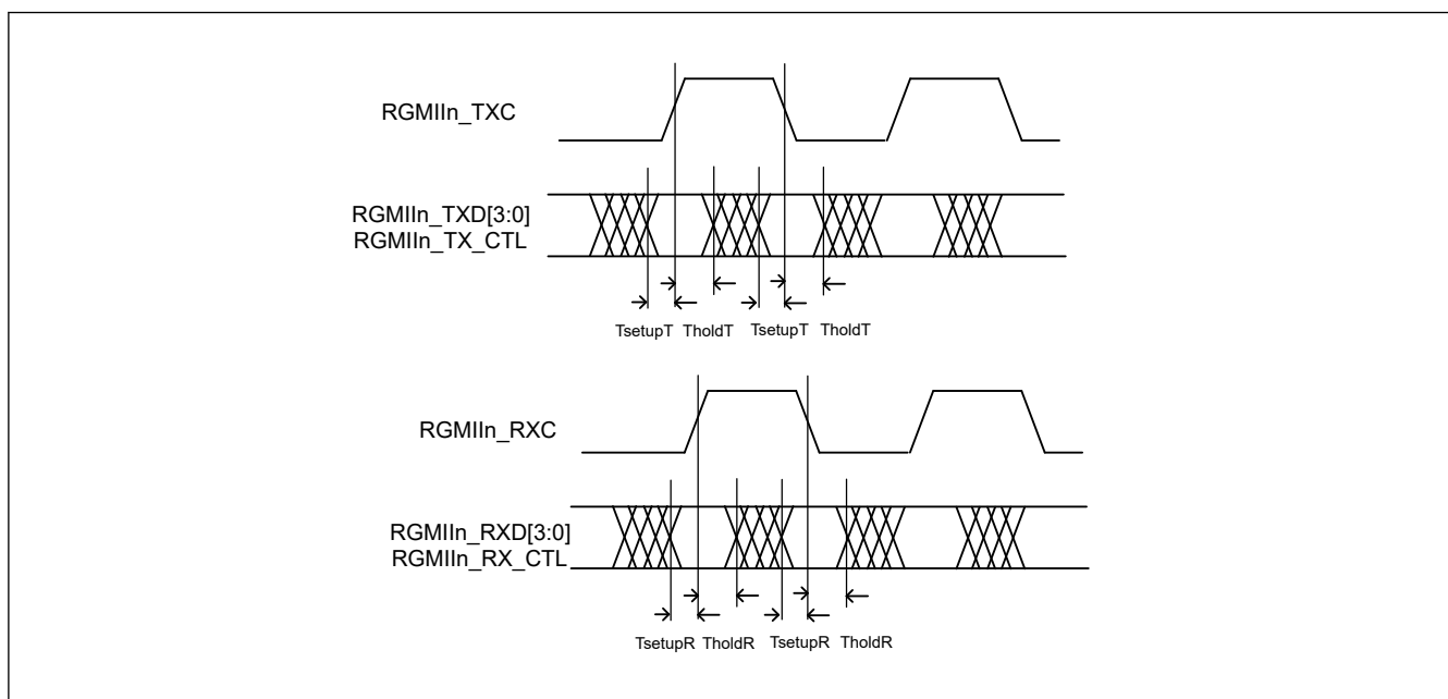
Figure 69.121 RGMII timing (RGMII-ID)
