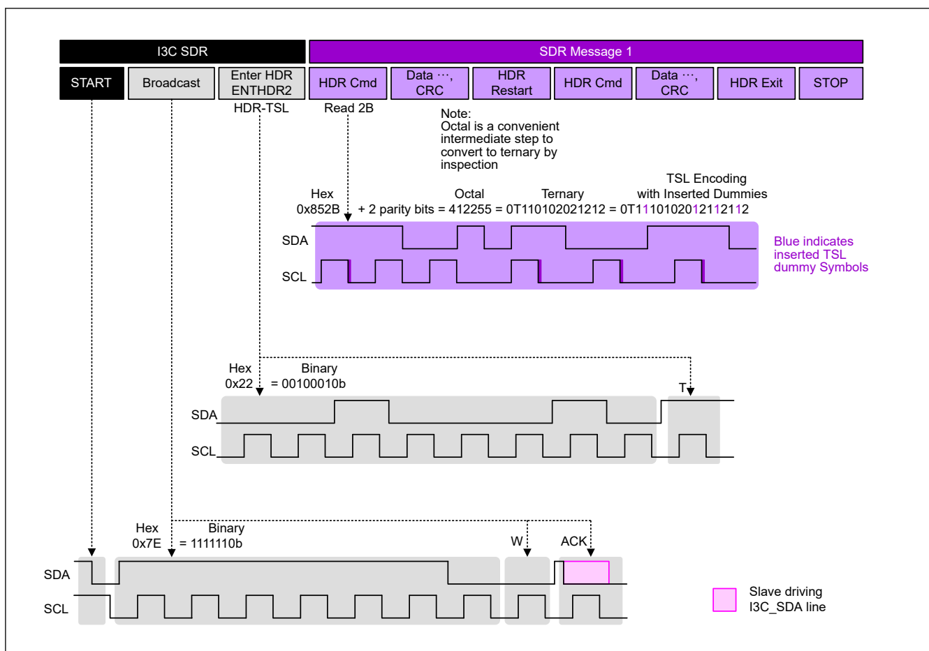
Figure 40.76 Example communication using HDR-TSL protocol
