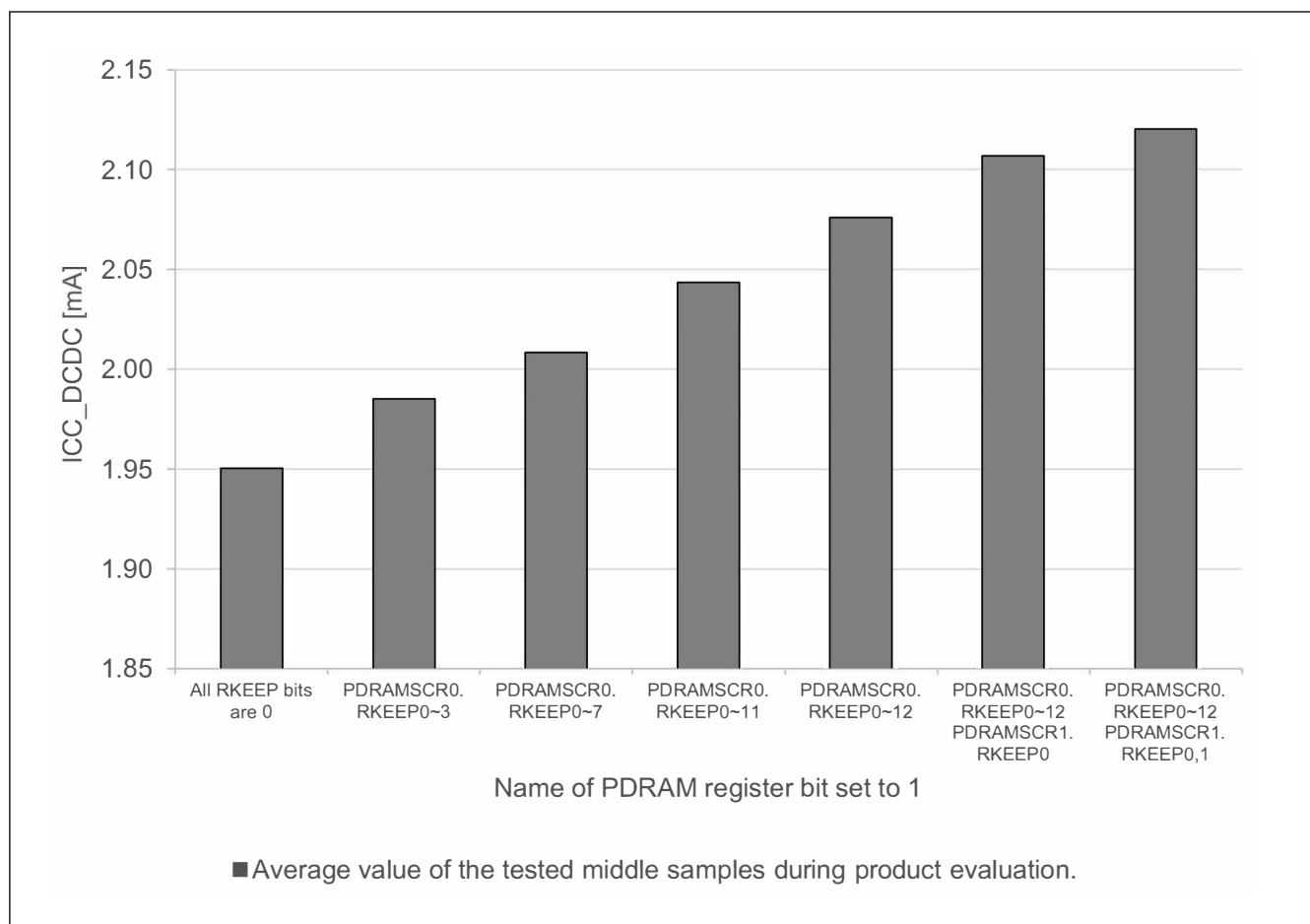
Figure 69.15 Software Standby current per SRAM state ( ICC\_DCDC , SS2LP\_1 , SVSCR\_2 ) (reference data)
