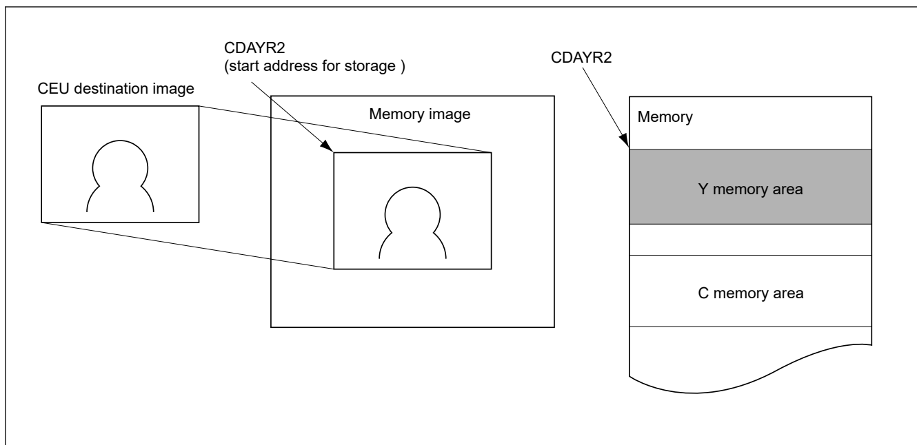
Figure 60.50 Relationship between captured image and luminance component memory area
