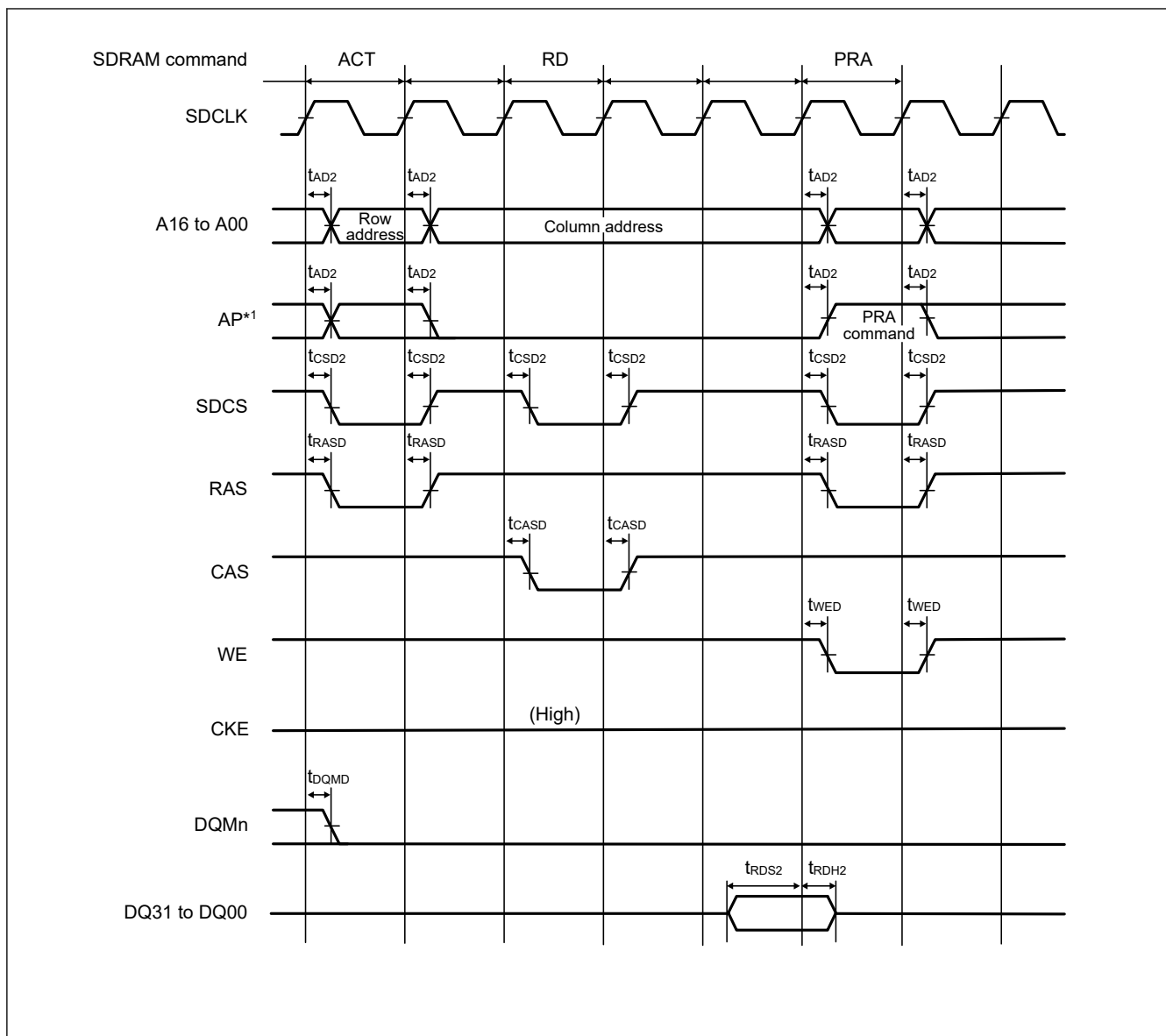
Figure 69.45 SDRAM single read timing
