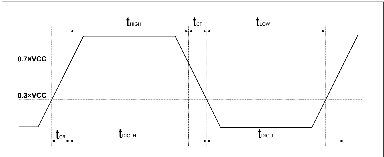
Figure 69.91 t_{DIG\_H} and t_{DIG\_L}
