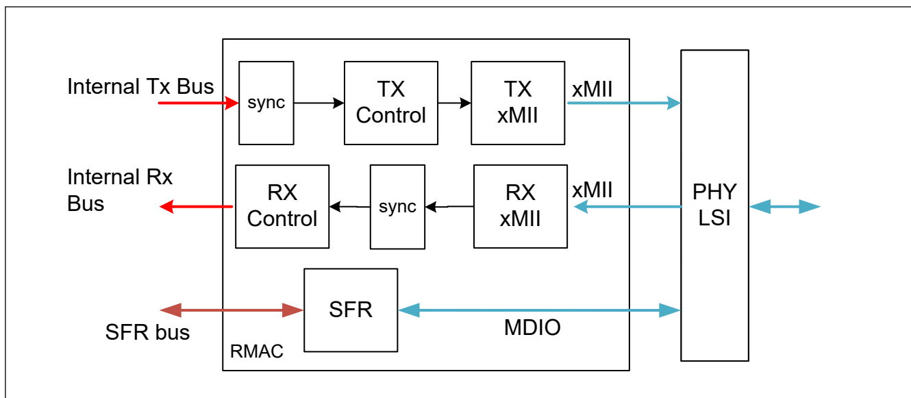
Figure 33.1 RMAC block diagram
