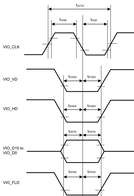
Figure 69.109 Capture Engine Unit Module Signal Timing of data capturing on the falling edge of VIO_CLK
