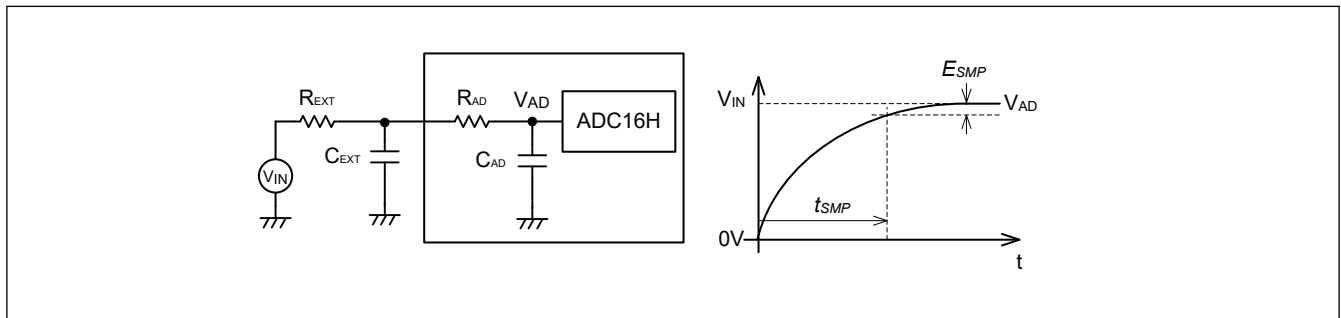
Figure 53.67 Simplified model of sample-and-hold circuit for A/D converter
