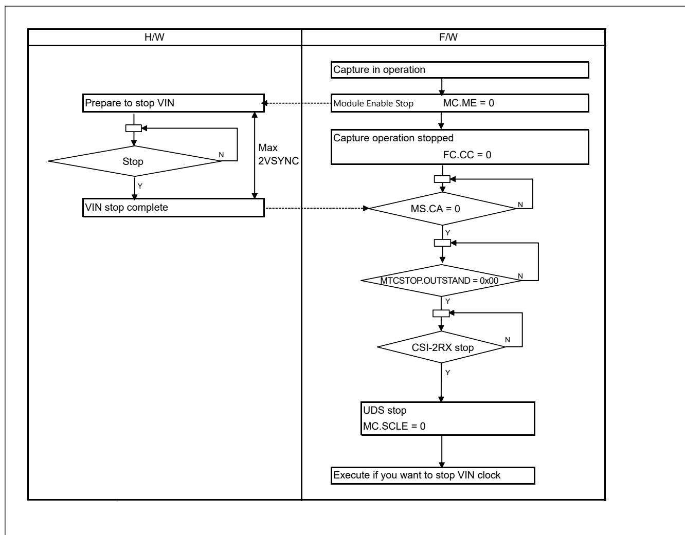
Figure 67.18 Stopping capture operation
