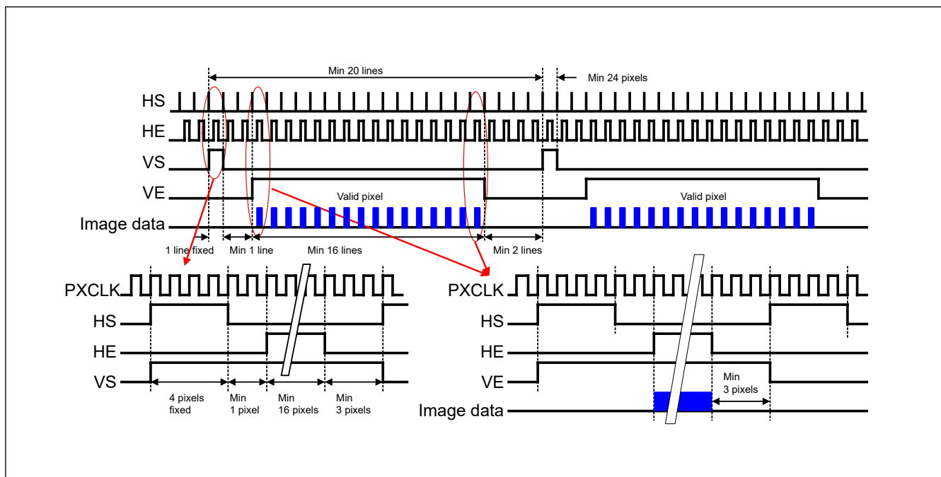
Figure 63.23 Image data carrier signals in the GLCDC
