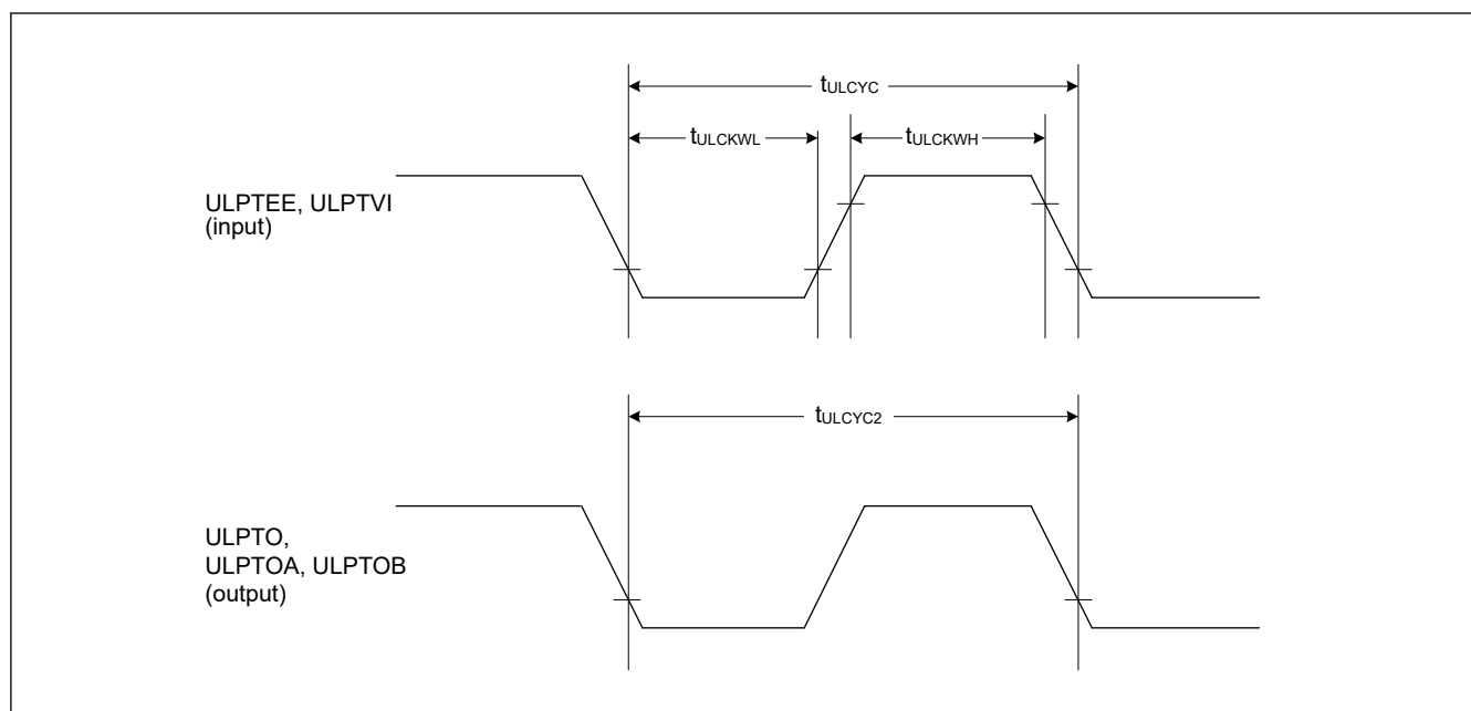
Figure 69.66 ULPT input/output timing
