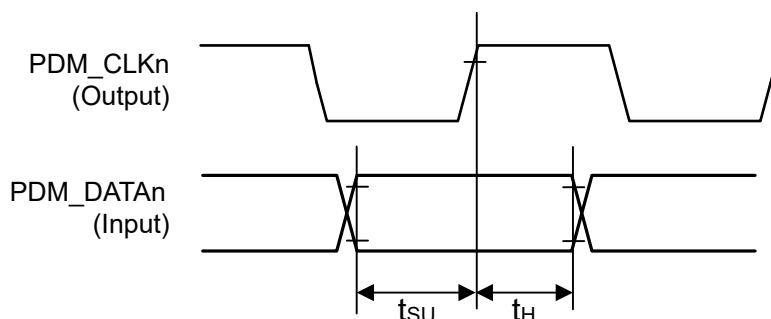
Figure 69.124 Receive Timing (Synchronized with the rise of PDM_CLKn)
