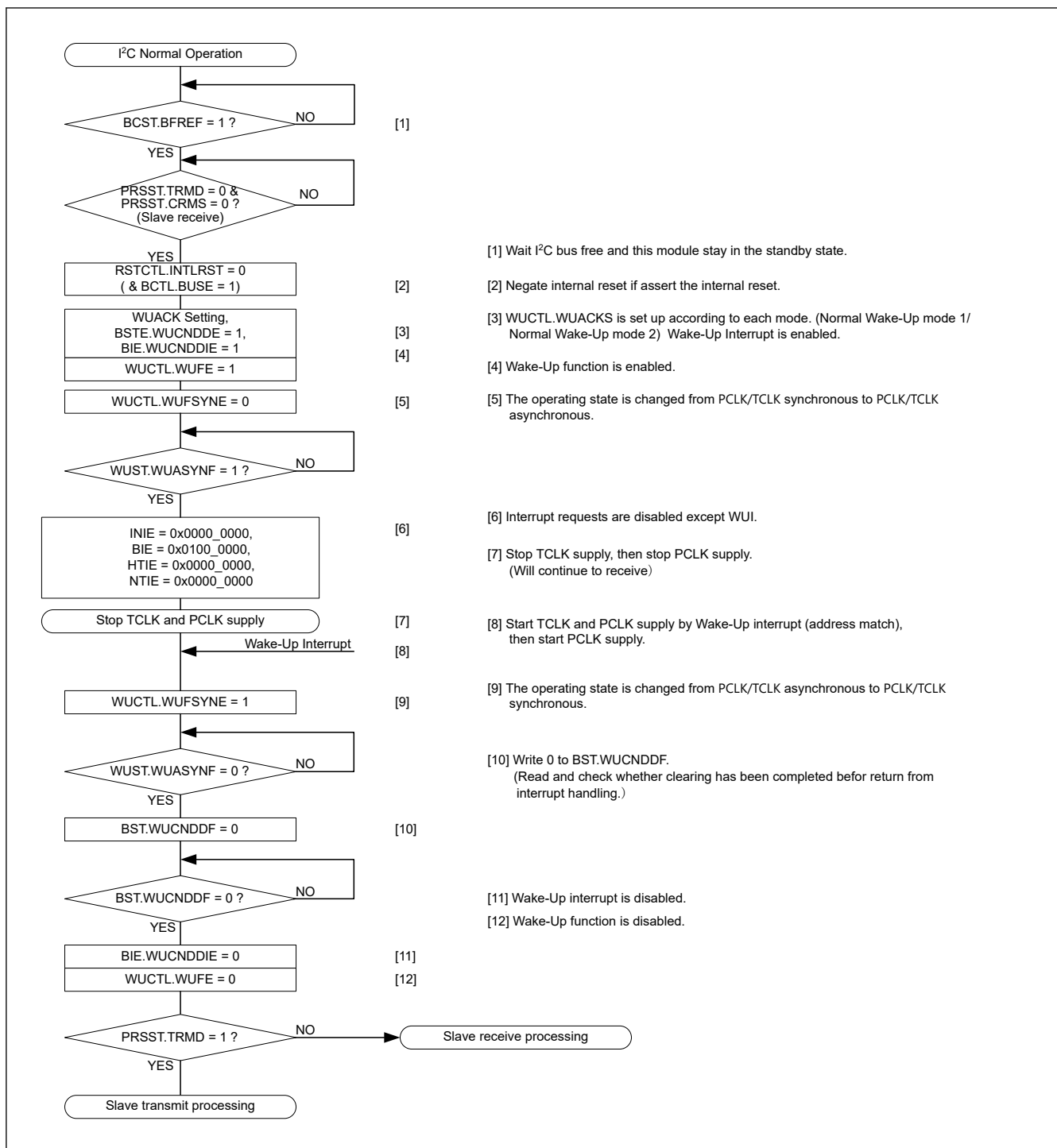
Figure 40.129 Use case of normal WU mode 2 (wake-up recovery by a wake-up interrupt triggered by the match of the slave address)
