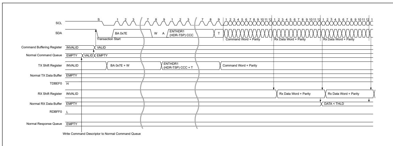
Figure 40.32 HDR data read transfer (HDR-TSP, TSL) timing (1/2)
