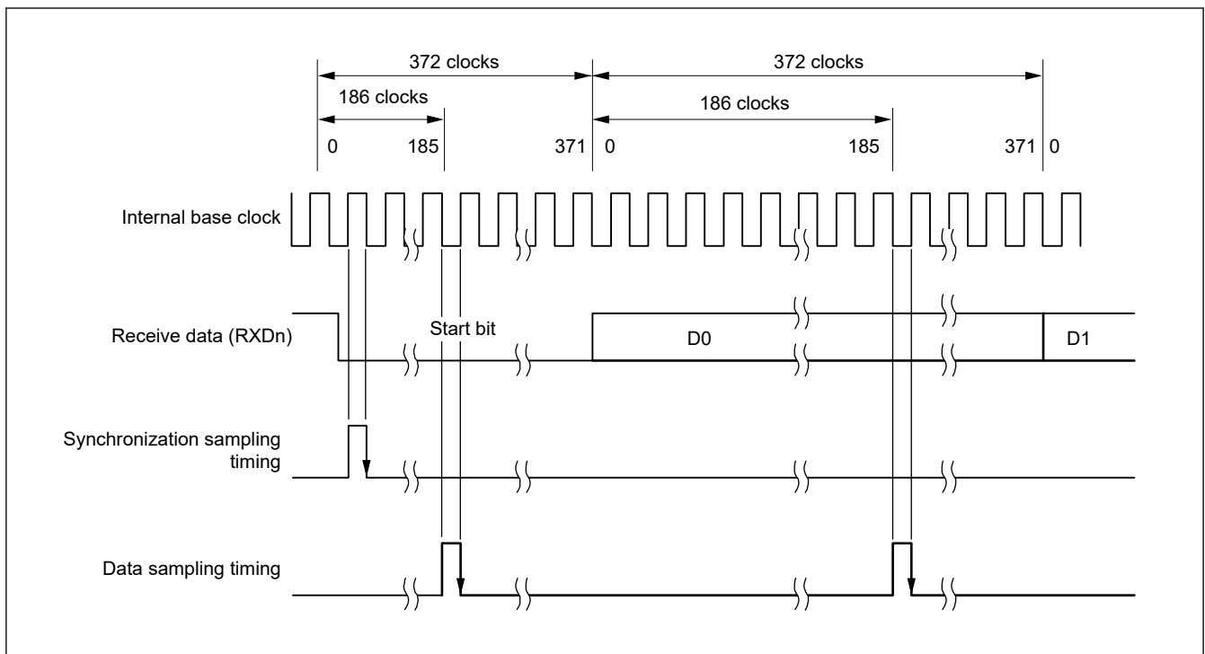
Figure 38.78 Receive data sampling timing in smart card interface mode when the clock frequency is 372 times the bit rate
