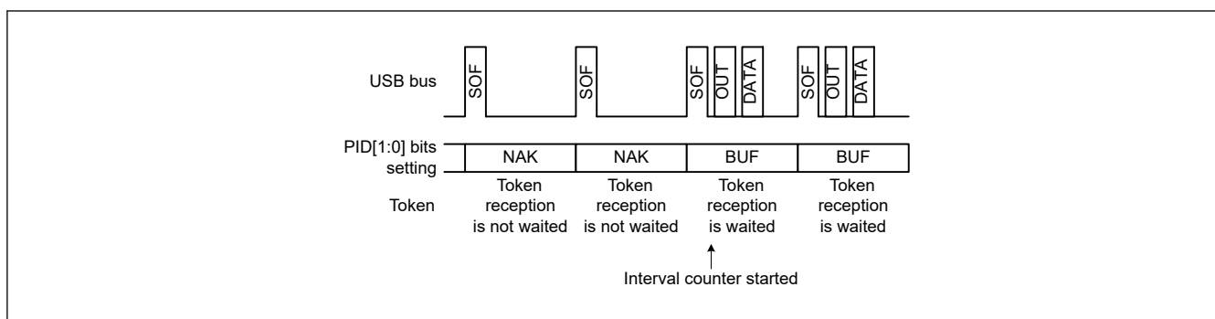
Figure 37.14 Relationship between frames and expected token reception when IITV[2:0] = 0
