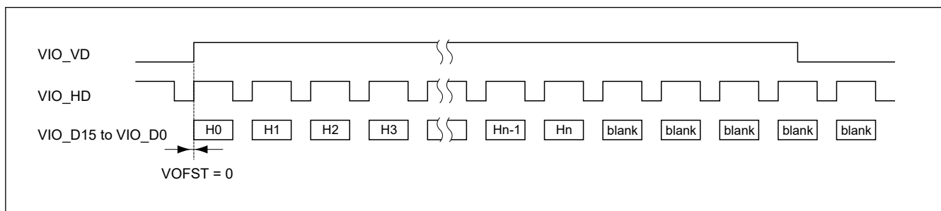
Figure 60.18 Timing when VD is data enable signal
