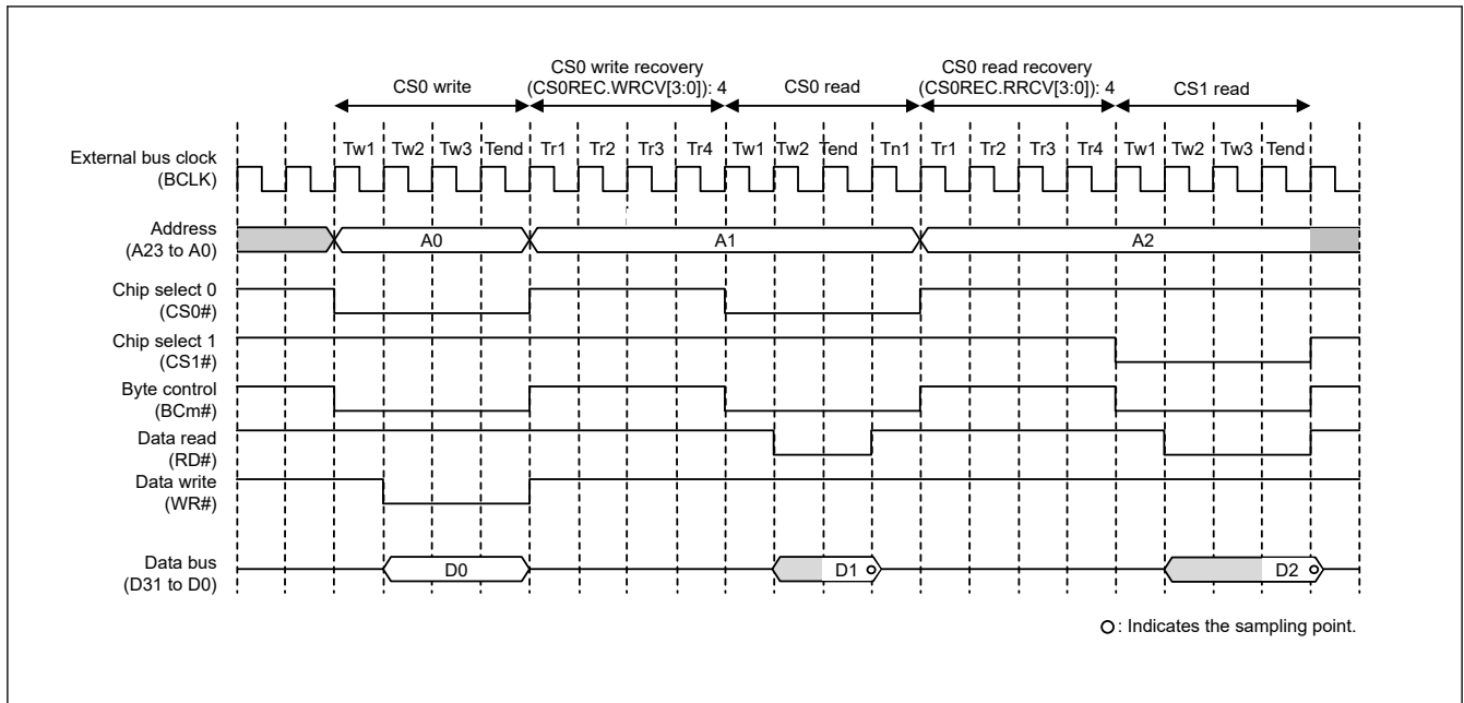
Figure 15.30 Example recovery cycle insertion with separate bus interface ( m = 0 to 3)
