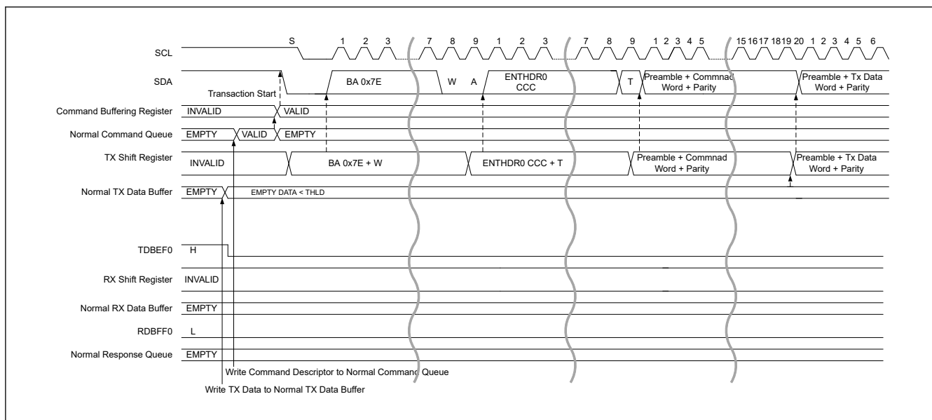
Figure 40.24 HDR data write transfer (HDR-DDR) timing (1/4)
