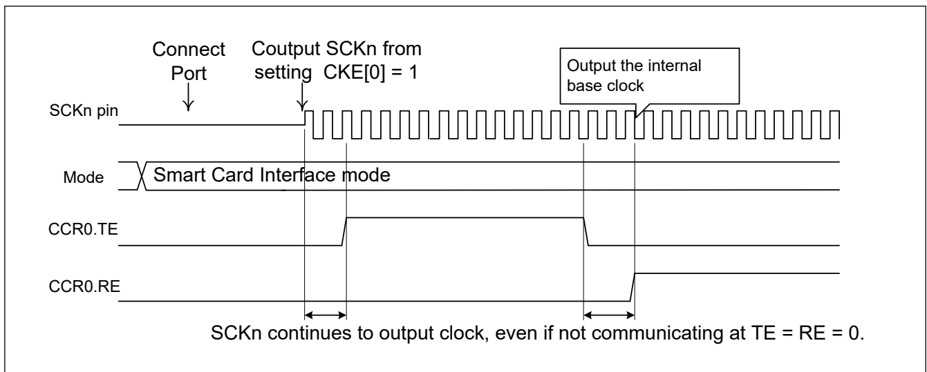
Figure 38.79 Example of Timing chart of data transmission in Smart Card Interface Mode
