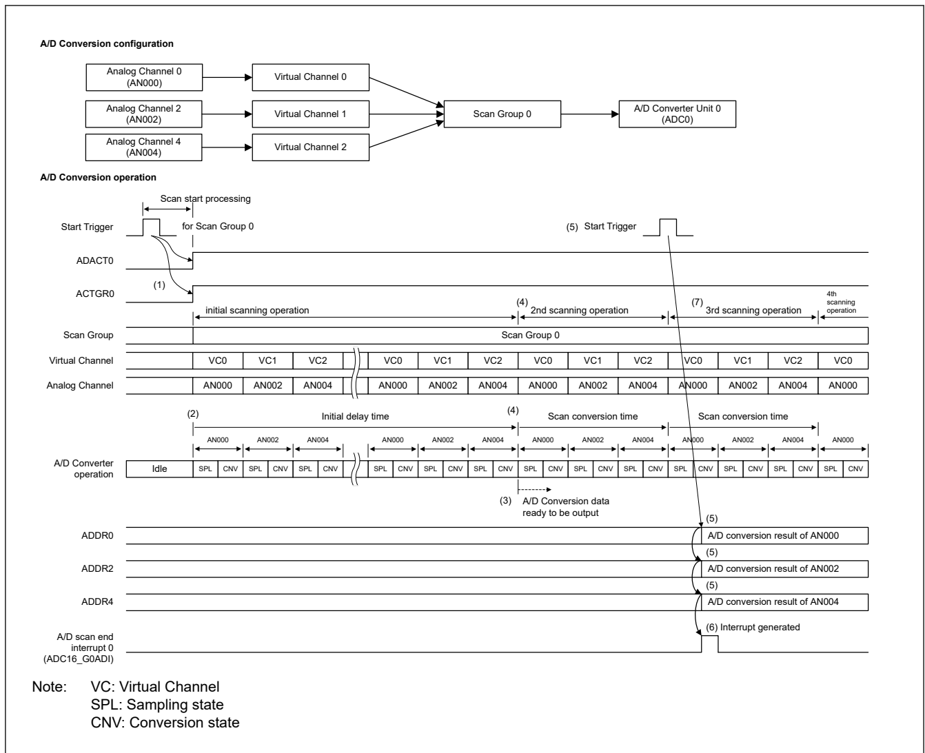
Figure 53.14 Example of scanning operation in Hybrid mode – Background continuous scan mode
