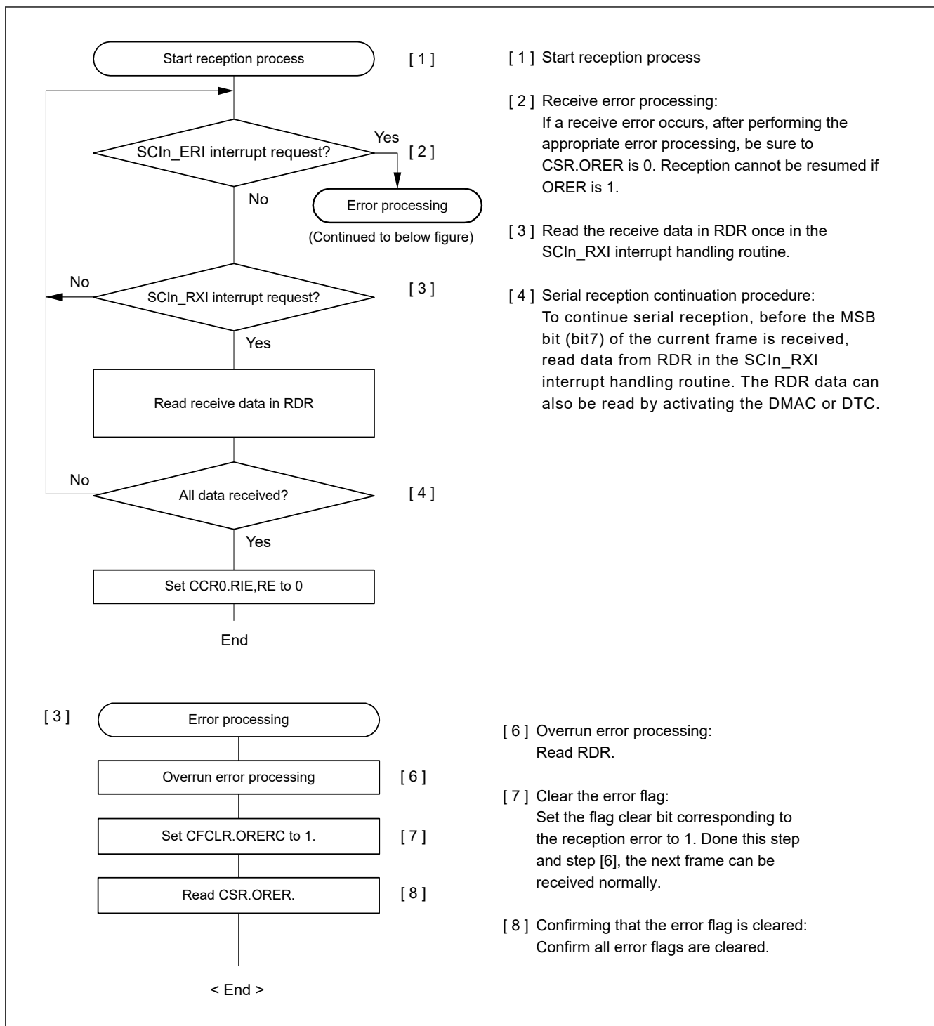
Figure 38.69 Example flow of serial reception in clock synchronous mode with non-FIFO selected
