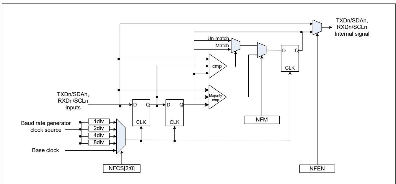
Figure 38.113 Digital noise filter circuit block diagram
