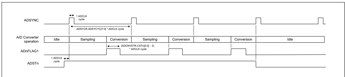
Figure 53.33 A/D conversion monitor signals
