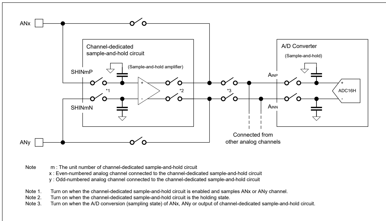
Figure 53.17 Internal configuration of channel-dedicated sample-and-hold circuit in Differential input mode
