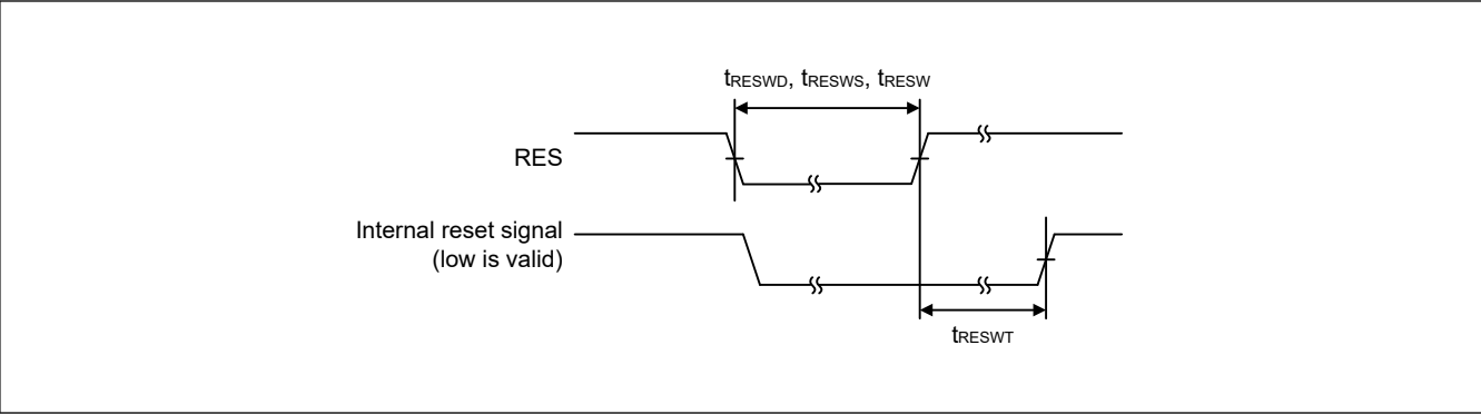
Figure 69.33 Reset input timing
