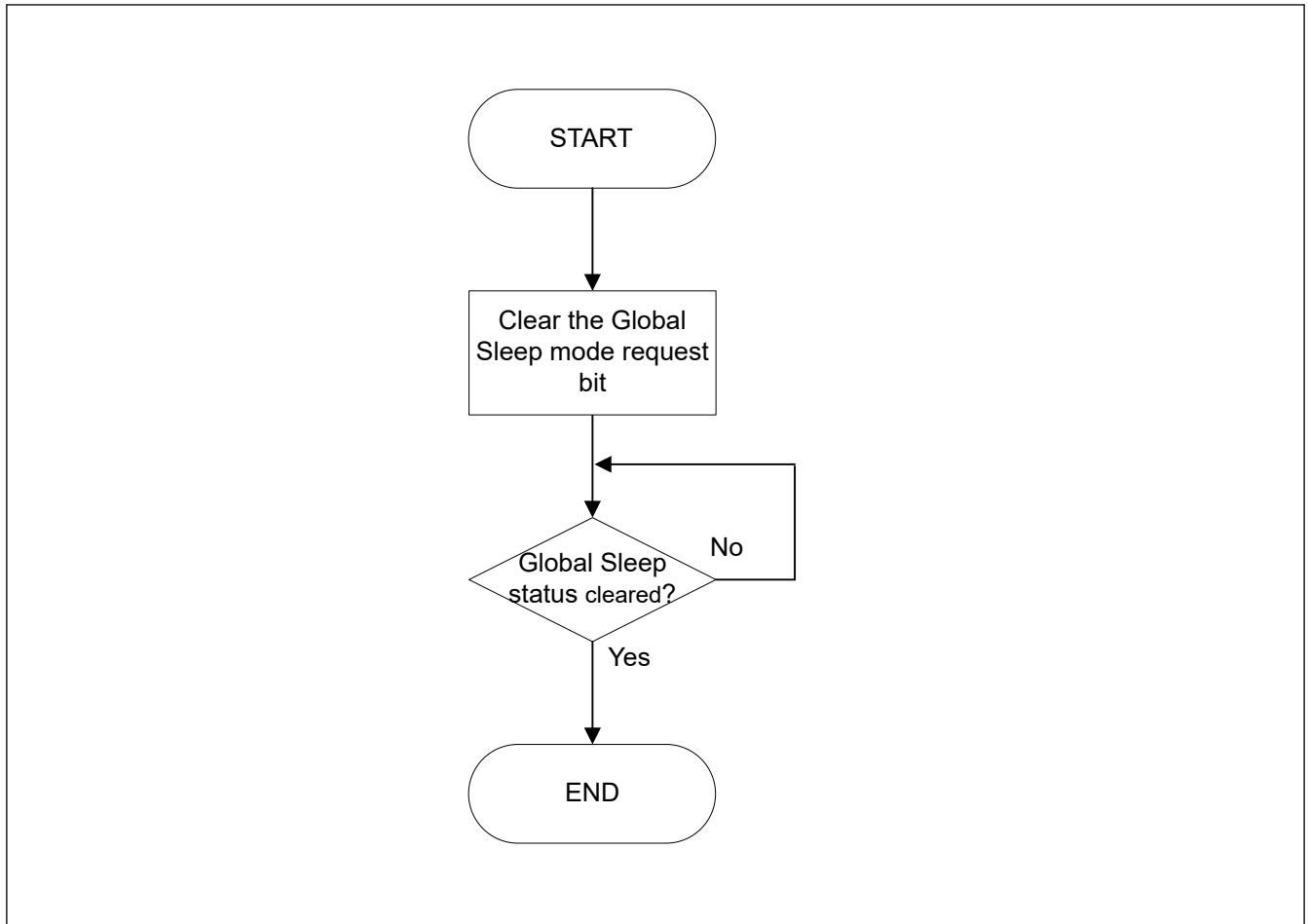
Figure 41.4 Procedure for exiting Global Sleep mode
