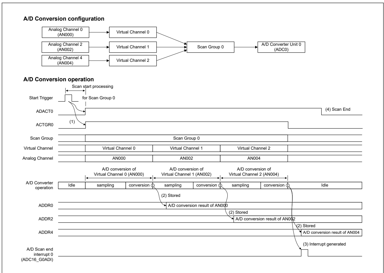
Figure 53.7 Example of the scanning operation in SAR mode – Single scan mode
