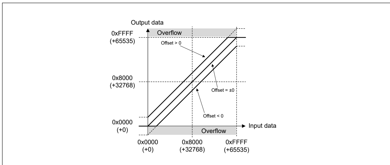
Figure 53.38 User's Offset Adjustment (16-bit data length format and Unsigned data format)
