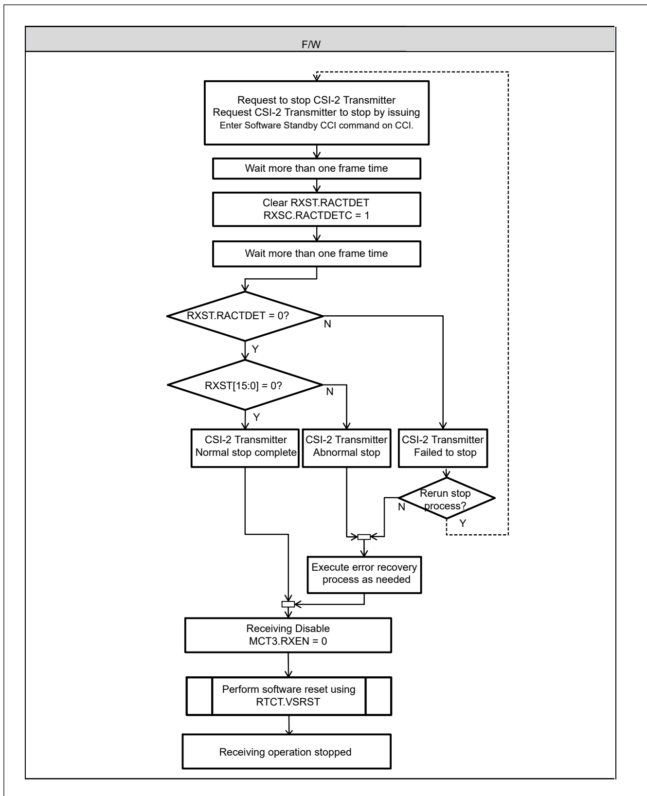
Figure 66.2 Receiving operation stopped
