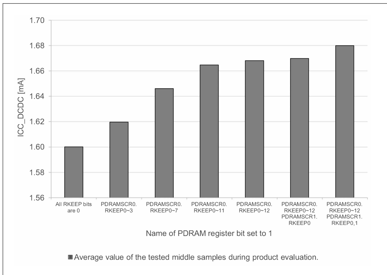
Figure 69.12 Software Standby current per SRAM state (ICC_DCDC, SS2LP_0, SVSCR_3) (reference data)
