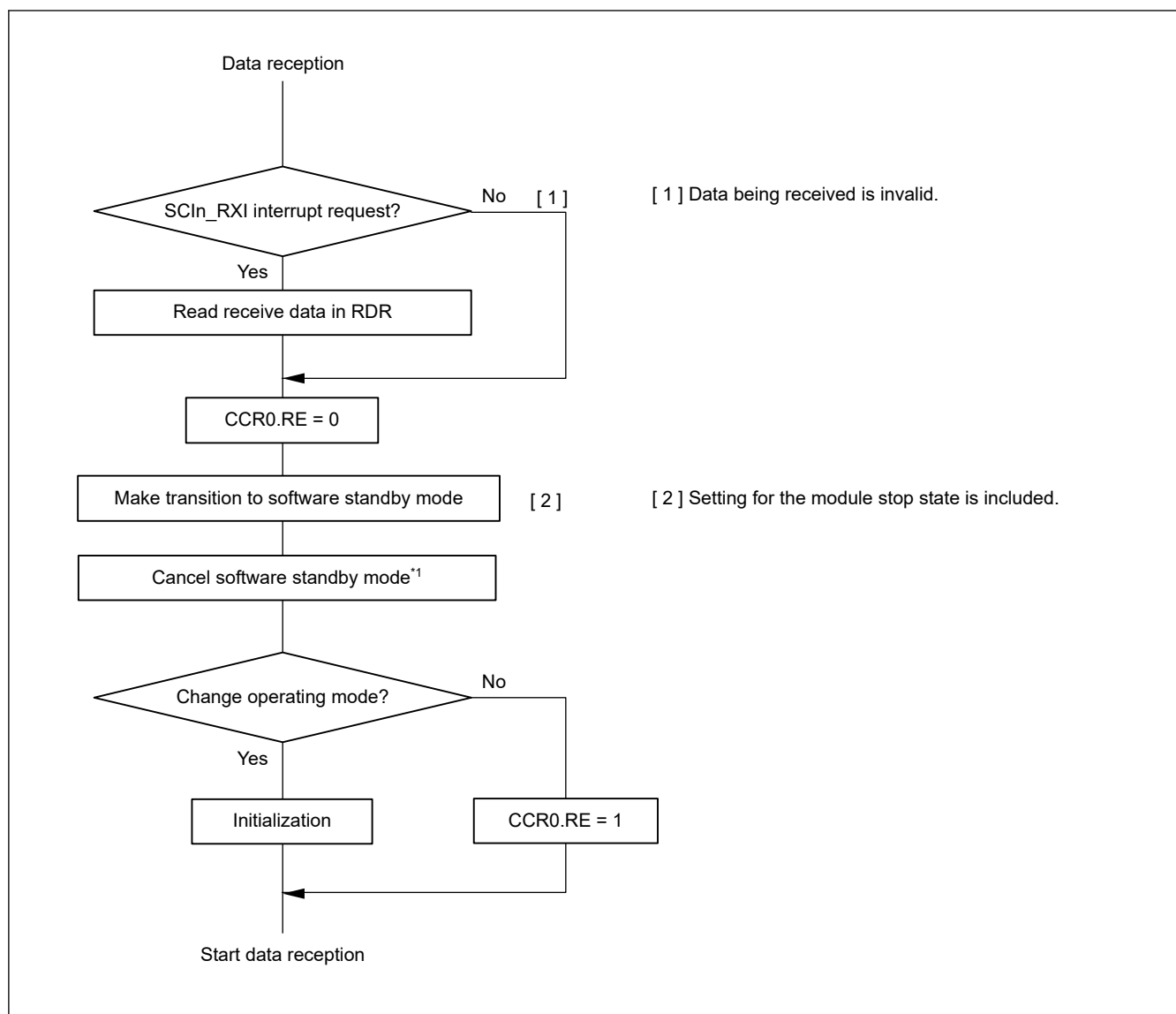
Figure 38.120 Example of Flowchart for Reception to Software Standby Mode during Reception
