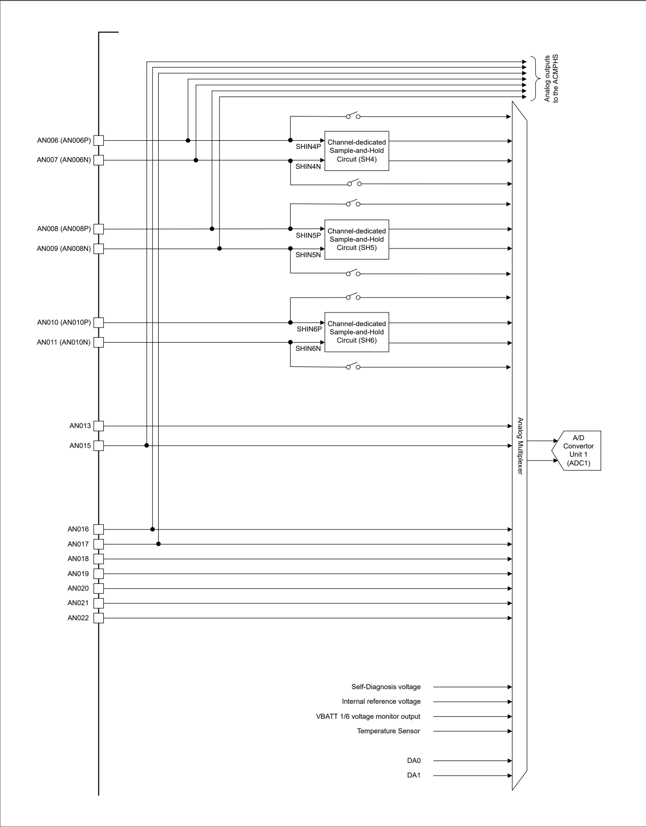
Figure 53.3 Analog channel structure for A/D converter unit 1
