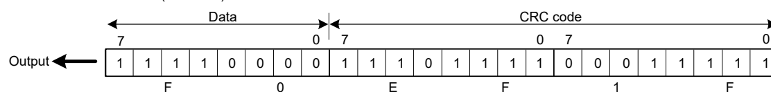
Figure 48.3 MSB-first data transmission
