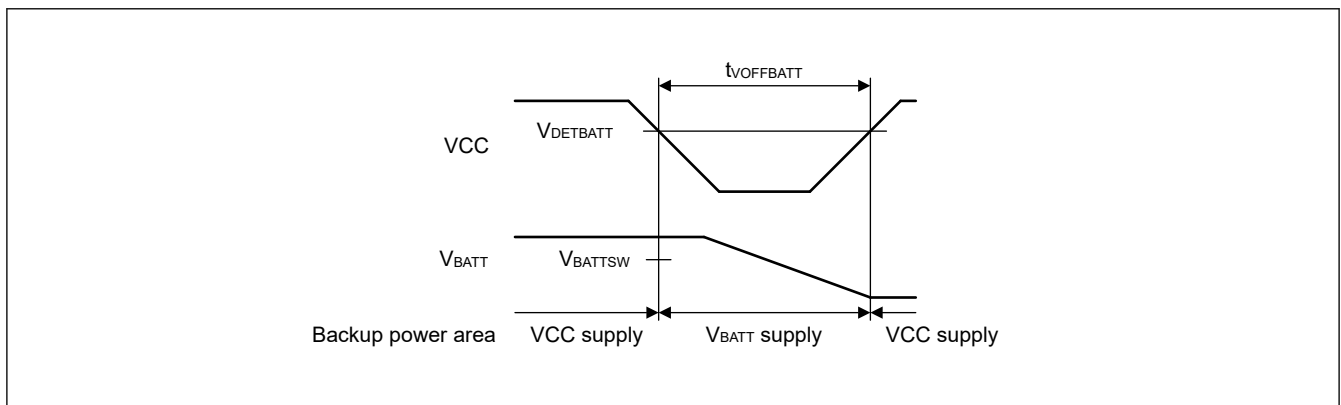
Figure 69.150 Battery backup function characteristics
