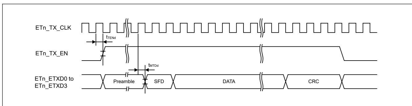
Figure 69.116 MII transmission timing in normal operation
