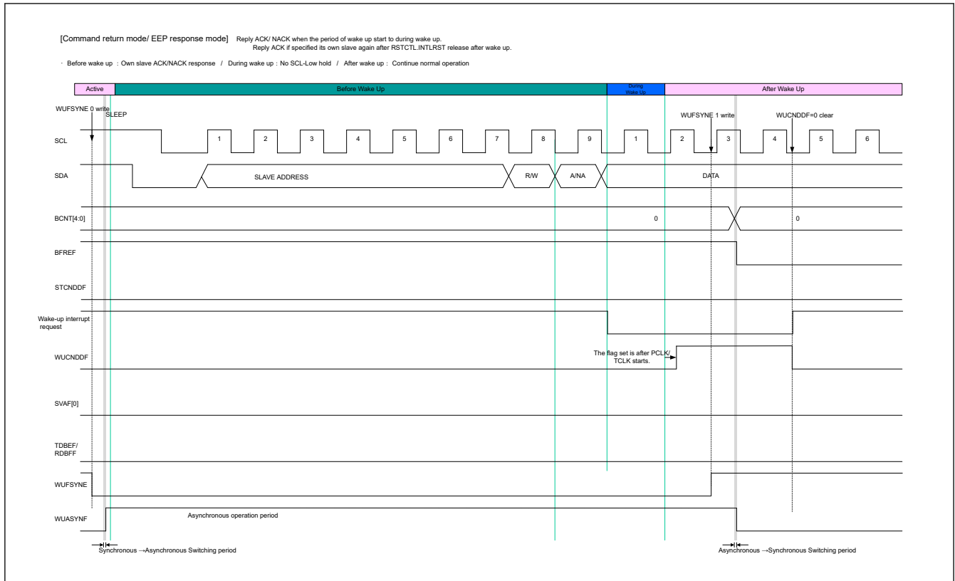
Figure 40.133 Timing of command recovery mode/EEP response mode
