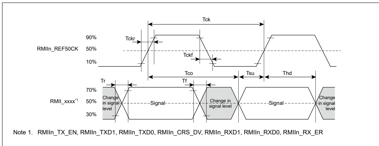
Figure 69.115 RMIIIn_REF50CK and RMII signal timing
