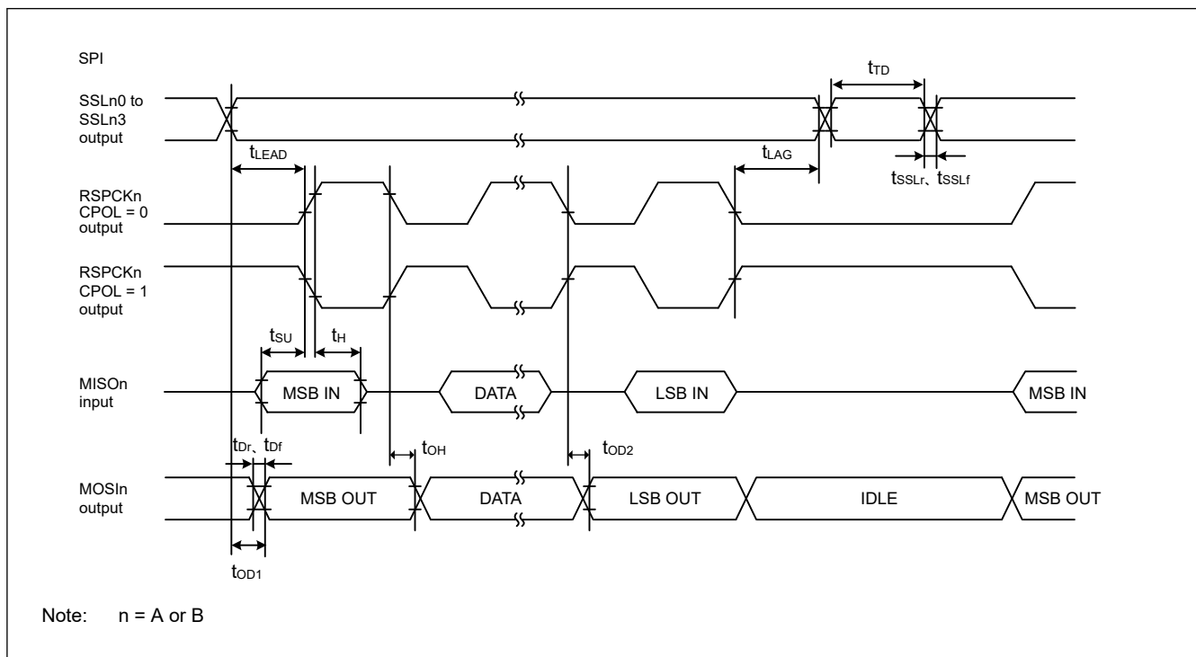
Figure 69.76 SPI timing for Motorola SPI master when CPHA = 0
