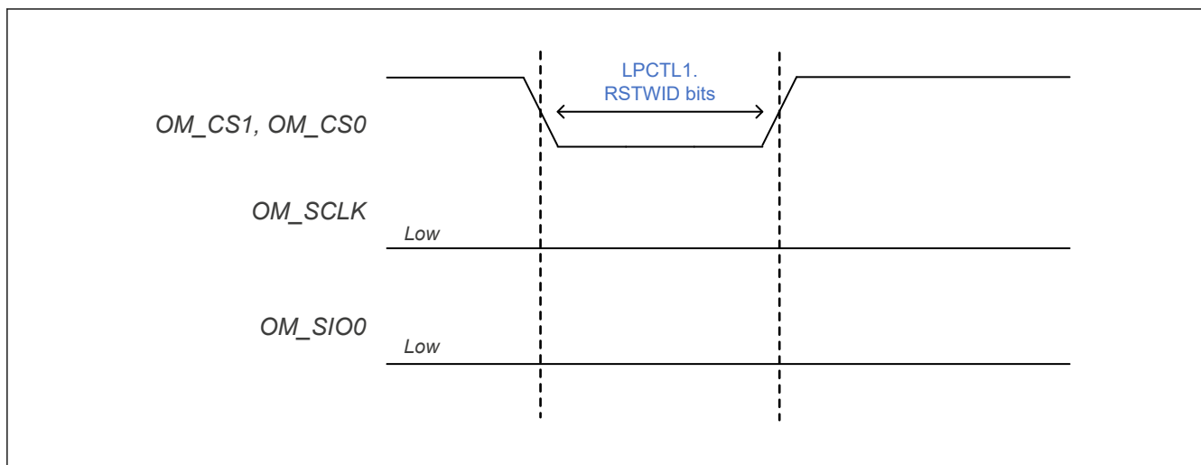
Figure 44.21 CS-only pattern
