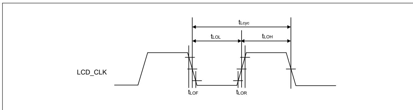
Figure 69.111 LCD_CLK clock output timing
