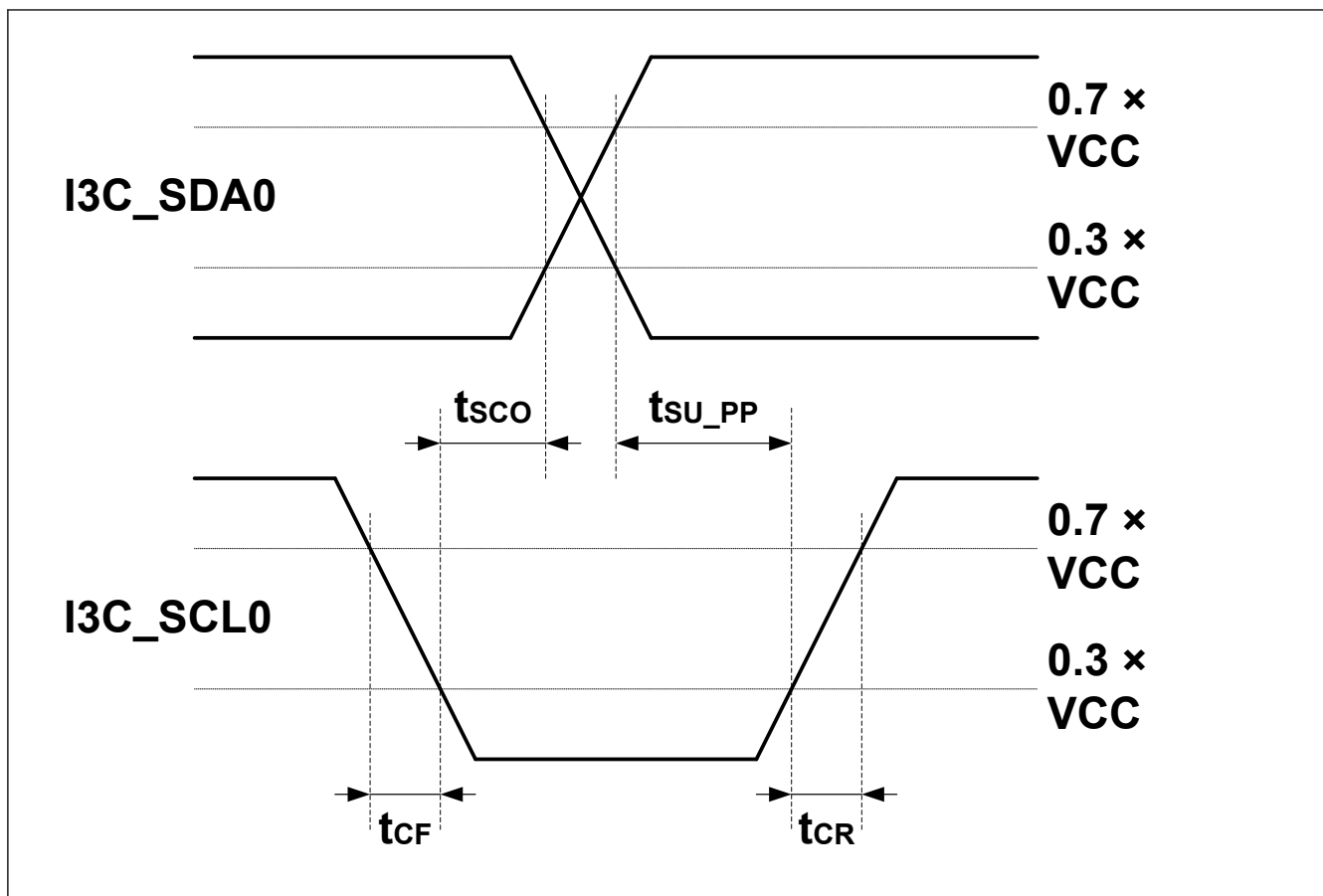
Figure 69.96 I3C Slave Out Timing
