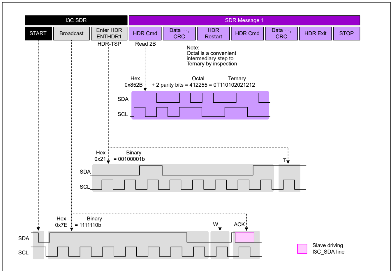
Figure 40.77 Example communication using HDR-TSP protocol
