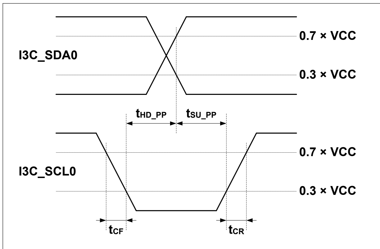
Figure 69.95 I3C Master Out Timing
