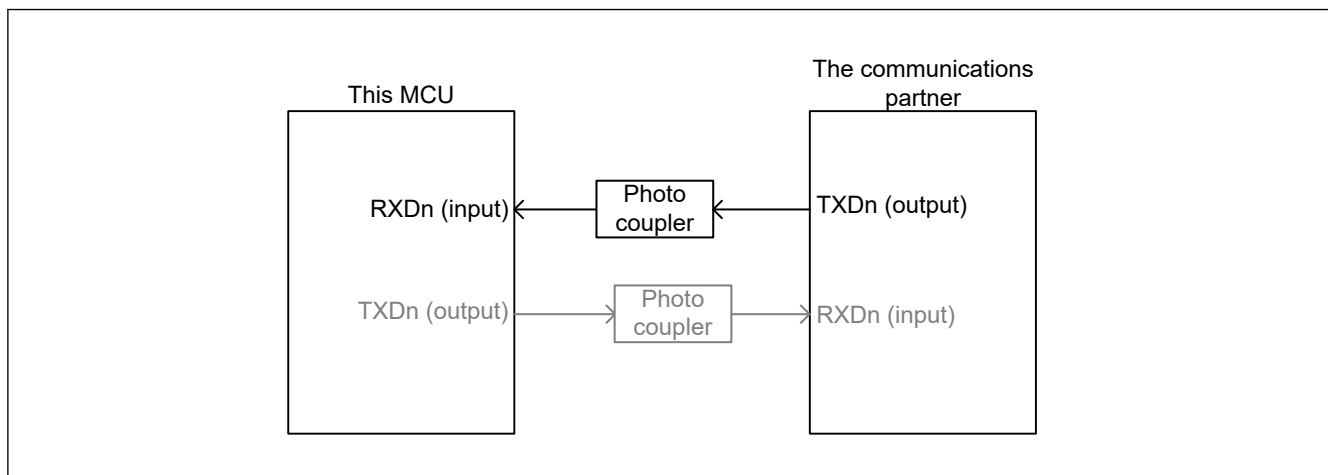
Figure 38.26 block diagram image of the reception through a photo coupler
