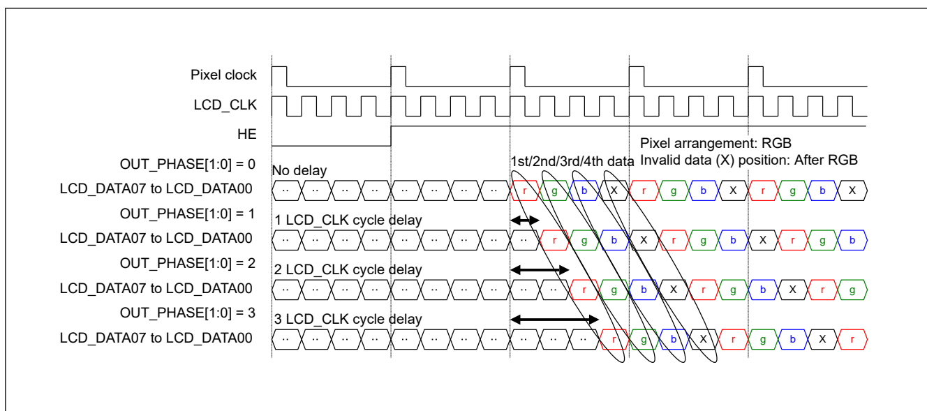
Figure 63.5 Serial RGB888 (4x speed) output timing
