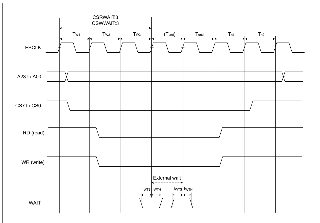
Figure 69.44 External bus timing for external wait control
