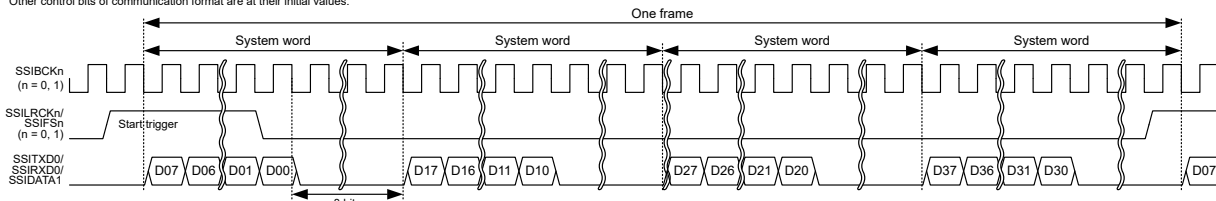
Figure 46.42 TDM format (with padding: system word length > data word length)
