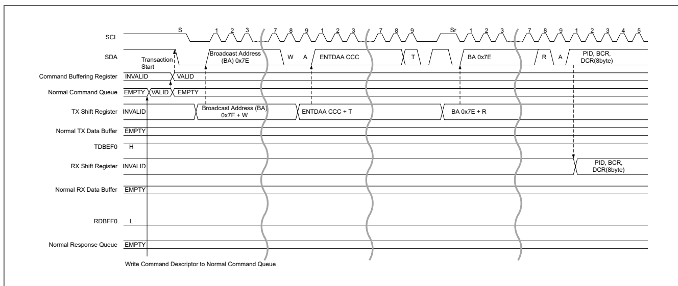
Figure 40.12 Dynamic address assign procedure (ENTDAAs CCC) timing (1/3)
