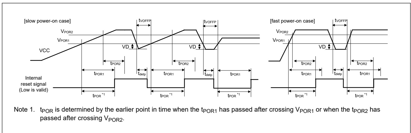
Figure 69.142 Power-on reset timing
