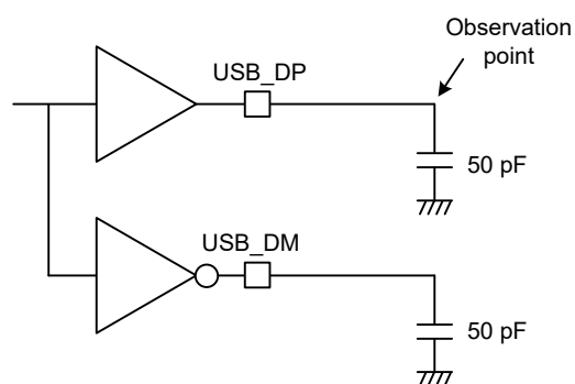
Figure 69.133 Test circuit in full-speed mode
