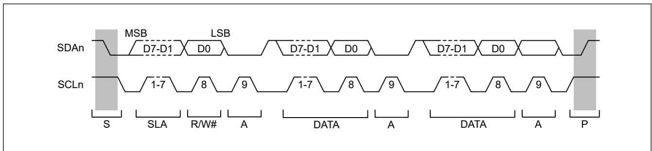
Figure 38.87 I 2 C bus timing when SLA is 7 bits
