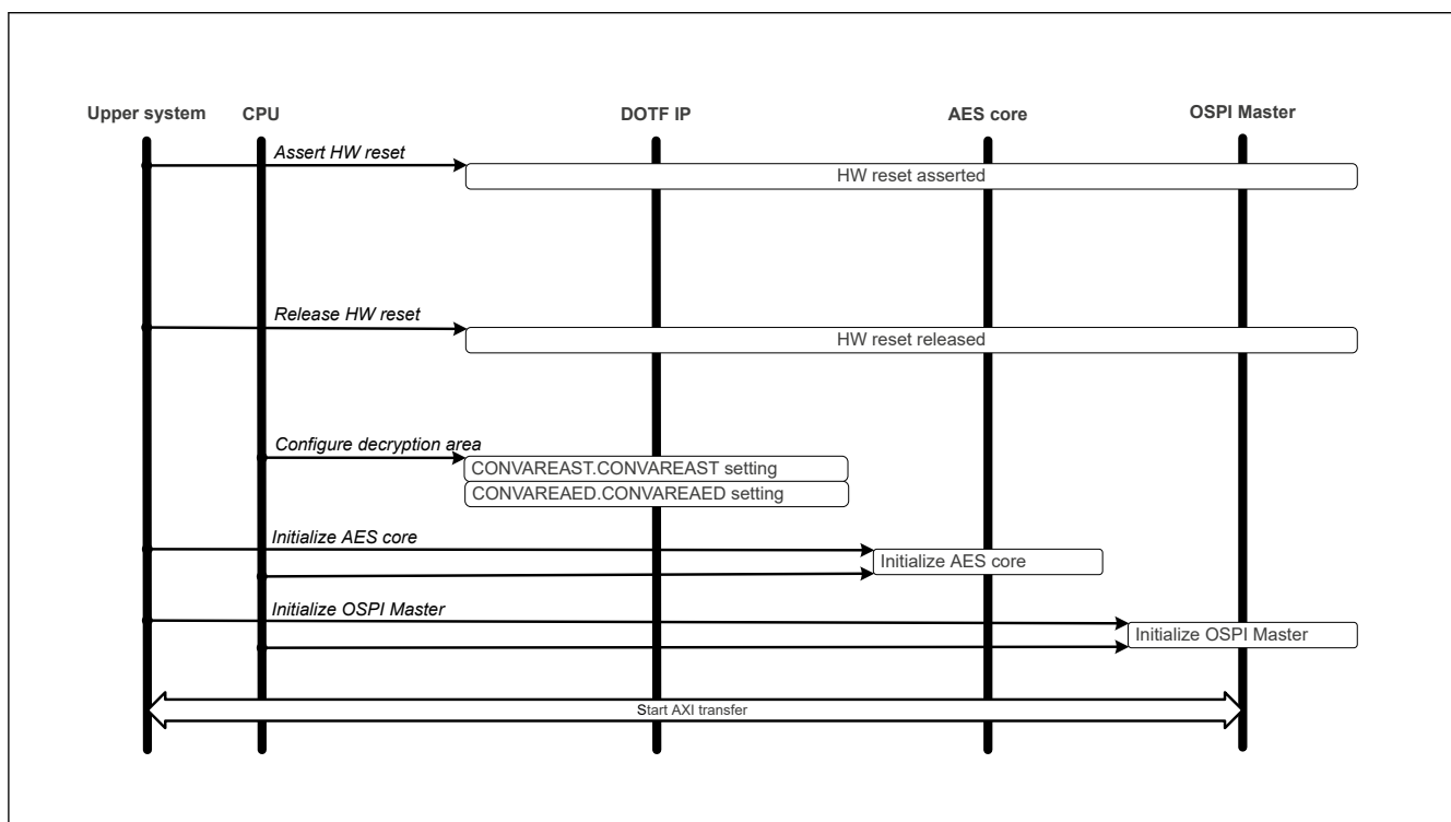
Figure 45.3 Initialization flow
