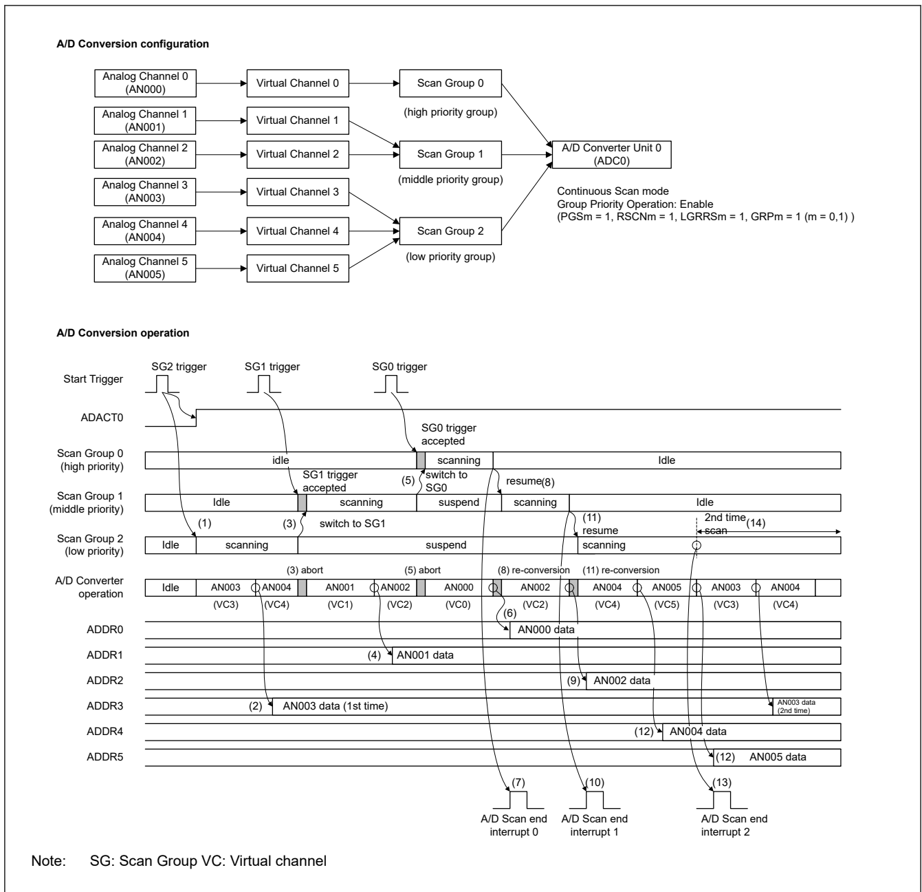
Figure 53.30 Example of group priority operation in SAR mode – Continuous scan mode (3 groups)
