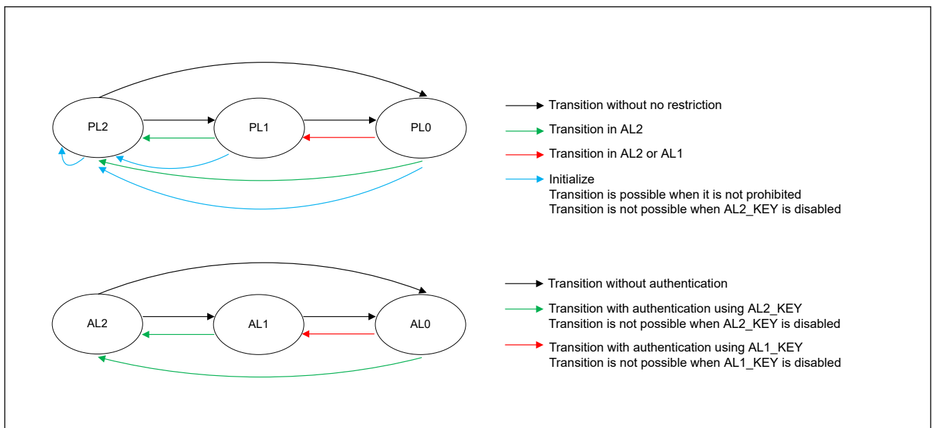
Figure 51.8 PL and AL states and transitions
