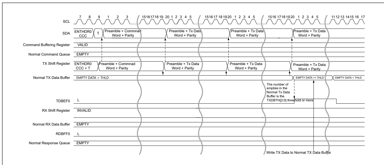
Figure 40.25 HDR data write transfer (HDR-DDR) timing (2/4)
