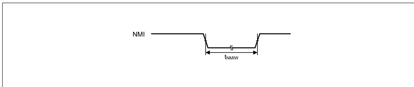
Figure 69.36 NMI interrupt input timing
