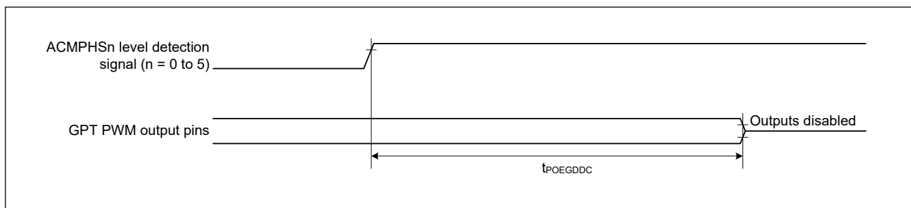
Figure 69.60 Output Disable Time for POEG in Response to Level Detection Signal from a Comparator
