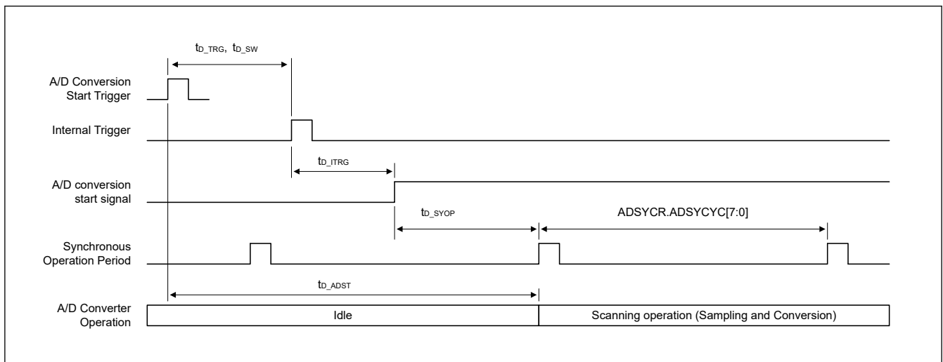
Figure 53.56 Scan start processing time
