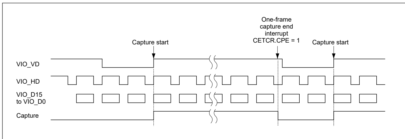
Figure 60.46 CPE generation timing
