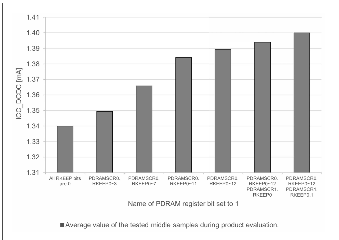
Figure 69.16 Software Standby current per SRAM state (ICC_DCDC, SS2LP_1, SVSCR_3) (reference data)
