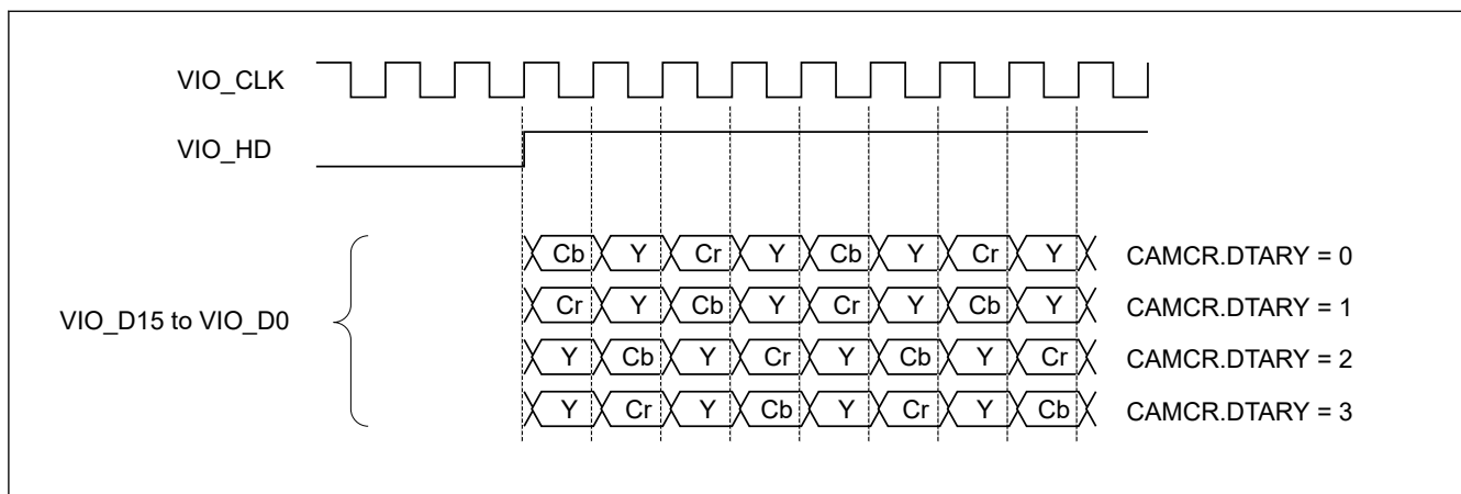
Figure 60.11 Input order of image data
