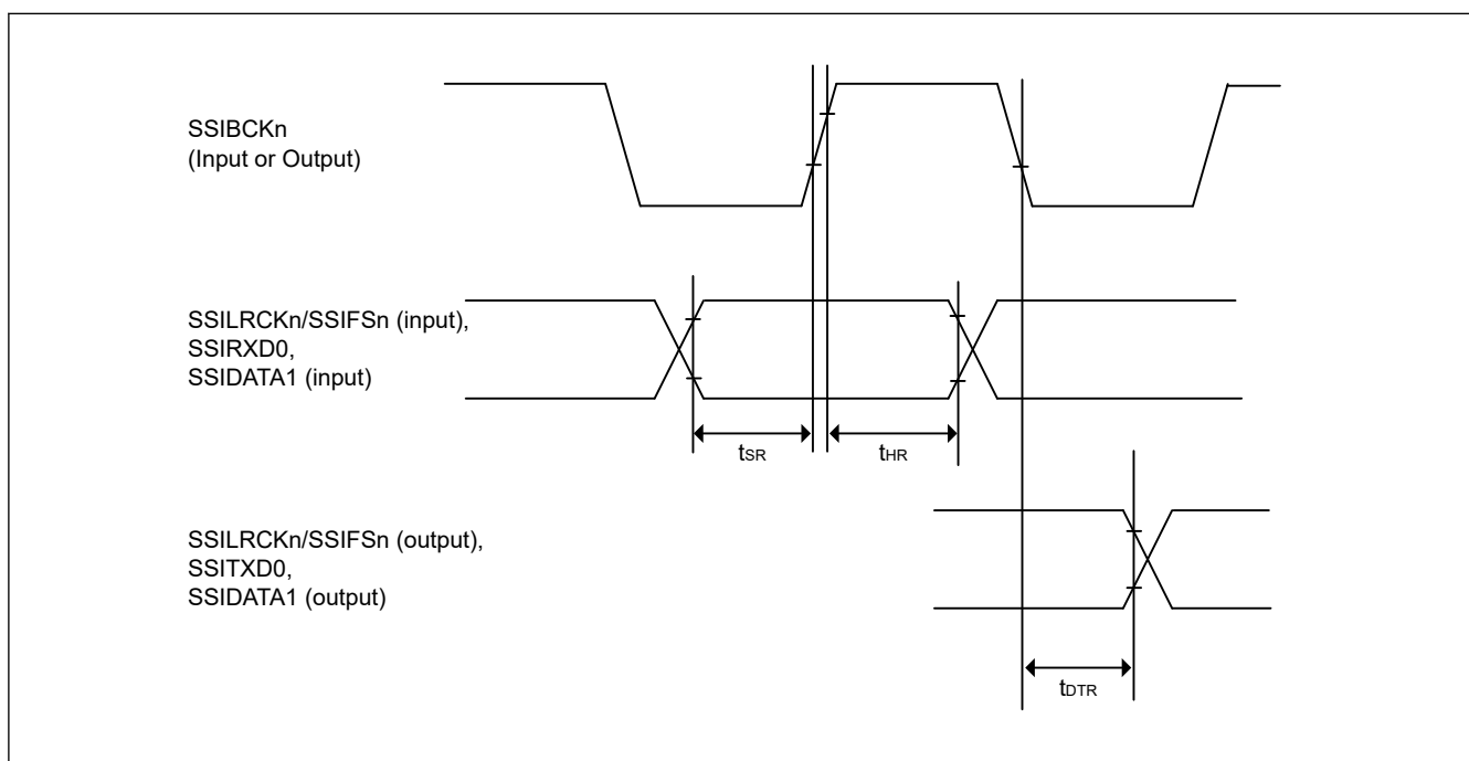
Figure 69.104 SSIE data transmit and receive timing when SSICR.BCKP = 0
