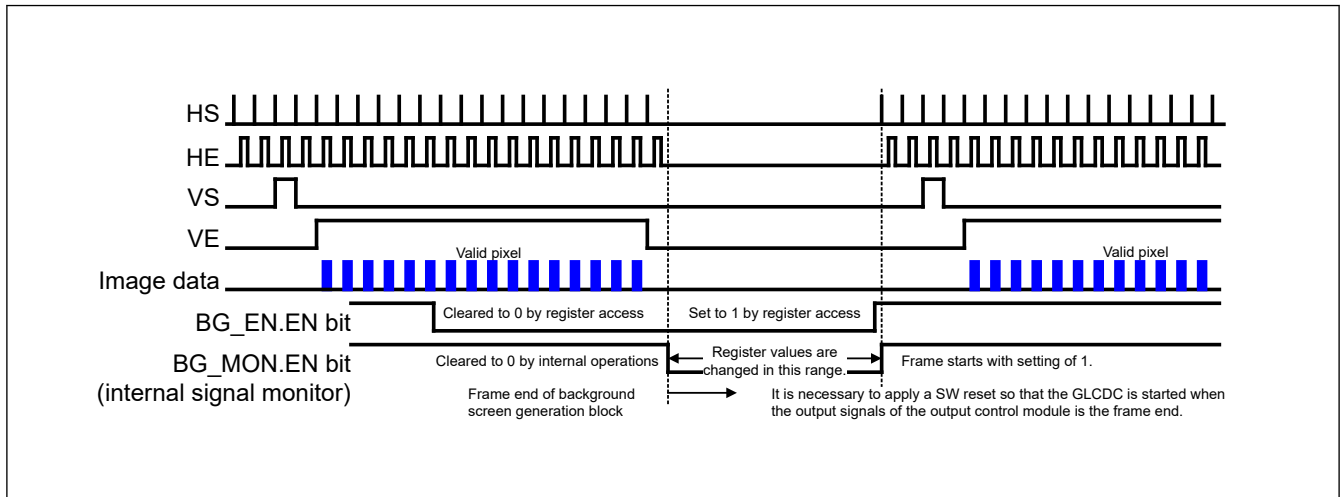
Figure 63.25 Stop and restart in normal operation
