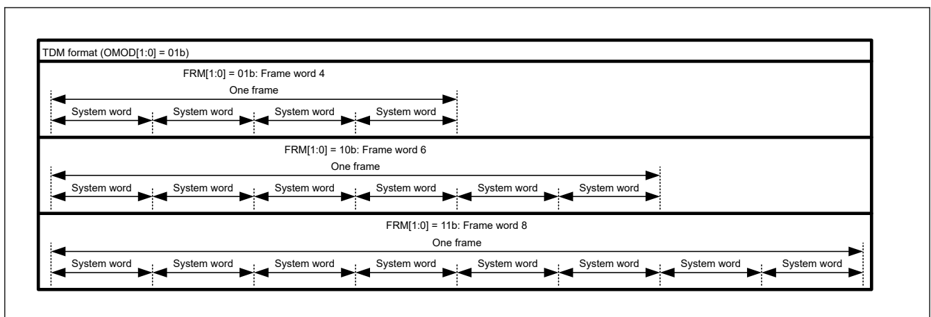
Figure 46.13 Frame word number
