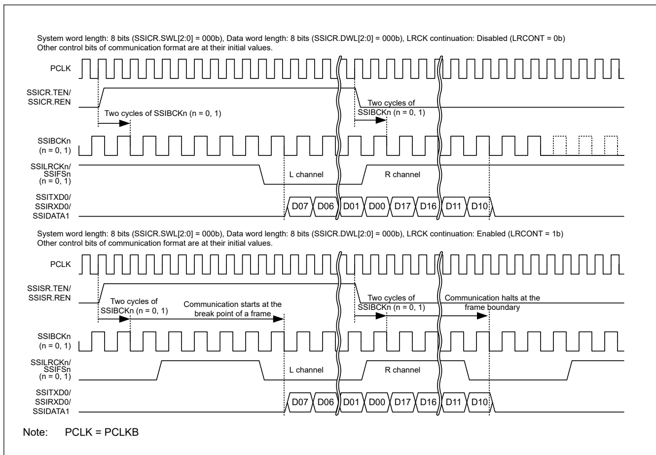
Figure 46.33 Example of LR clock/frame synchronization continuation operation
