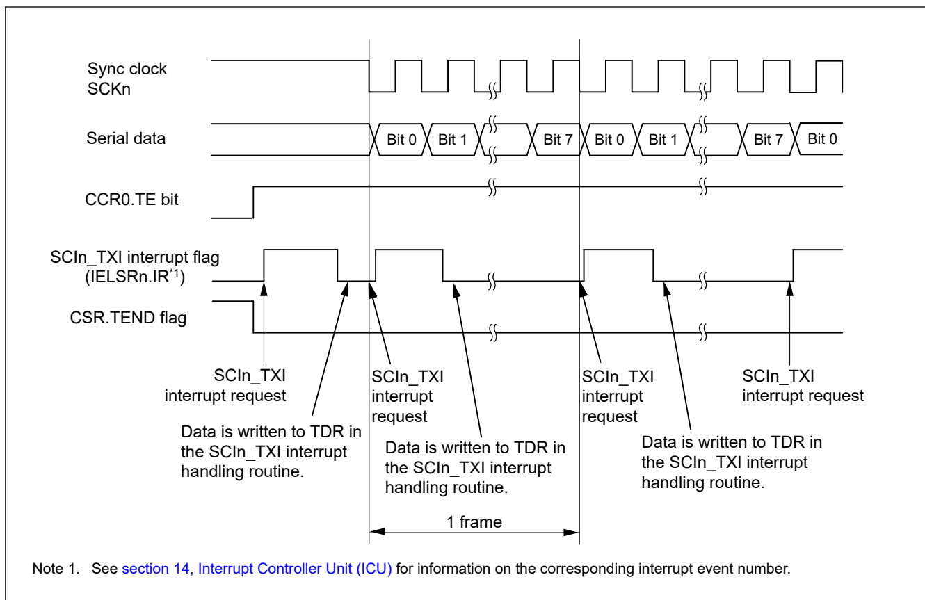
Figure 38.62 Example of serial data transmission in clock synchronous mode when the CTS function is not used at the beginning of transmission
