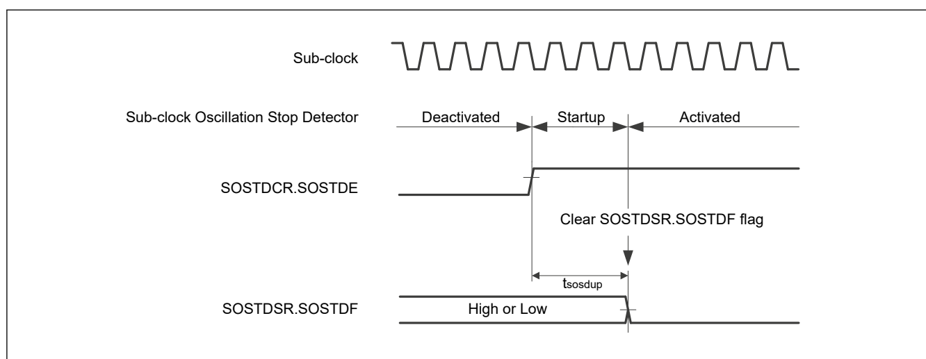
Figure 69.140 Sub-clock Oscillation Stop Detector start-up time
