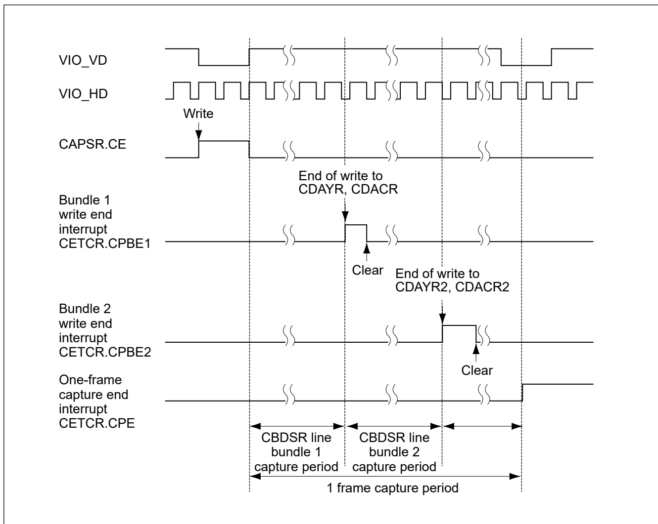
Figure 60.42 Timing of write end interrupts (Image capture, data synchronous fetch)
