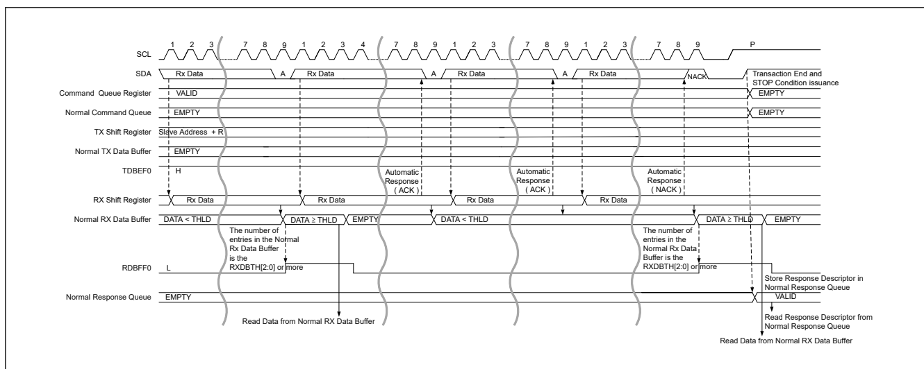
Figure 40.21 SDR data read transfer timing (2/2)
