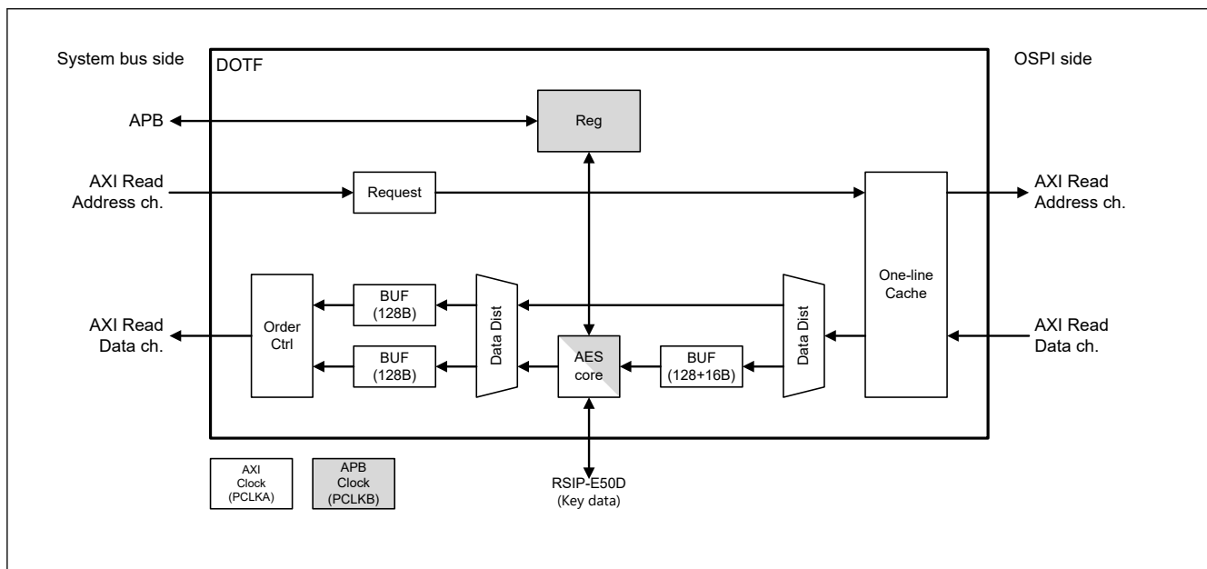
Figure 45.1 Block diagram
