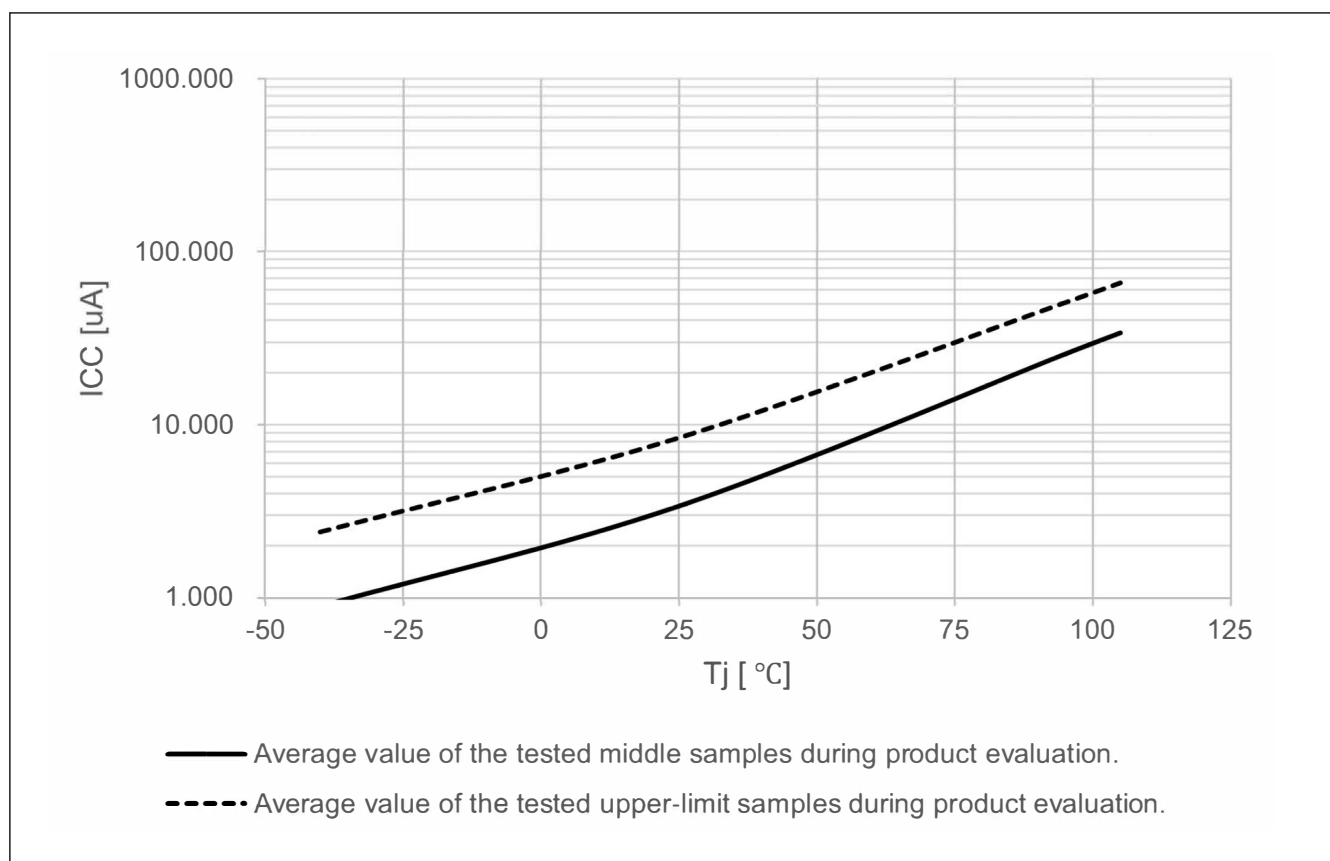
Figure 69.9 Temperature dependency in Deep Software Standby mode 3 (reference data)
