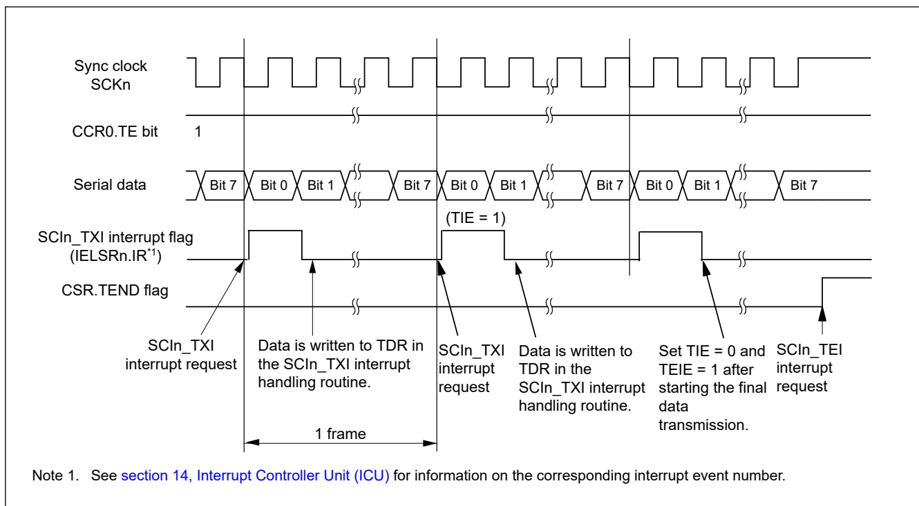
Figure 38.64 Example of serial data transmission in clock synchronous mode from the middle of transmission until transmission completion
