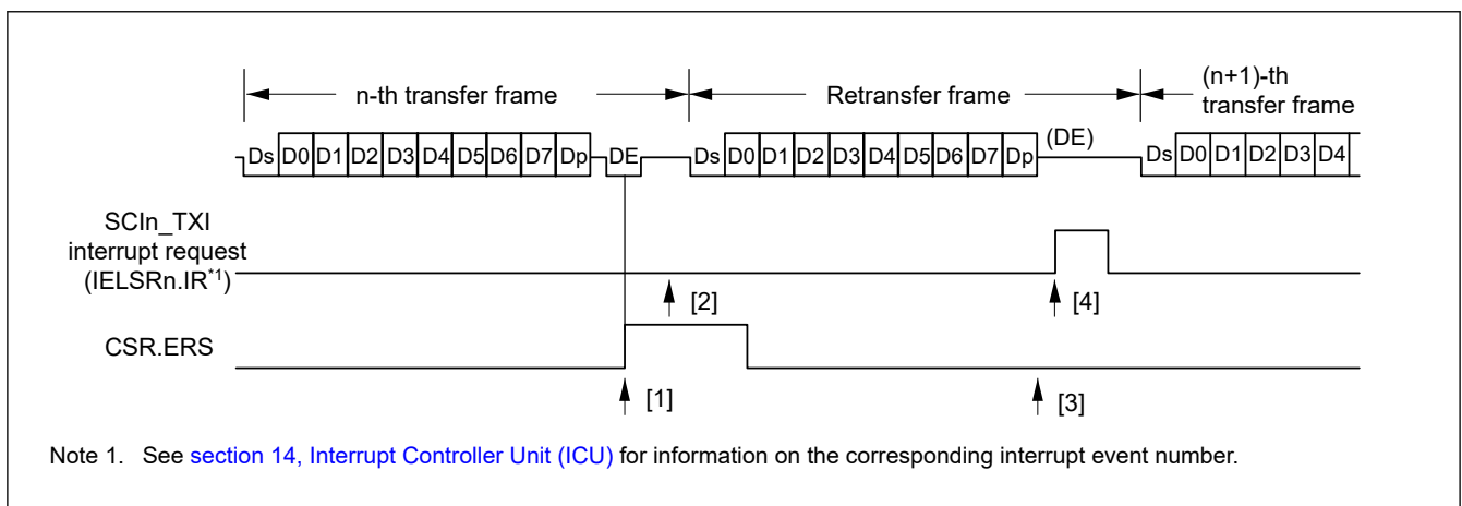
Figure 38.80 Data re-transfer operation in smart card interface transmission mode
