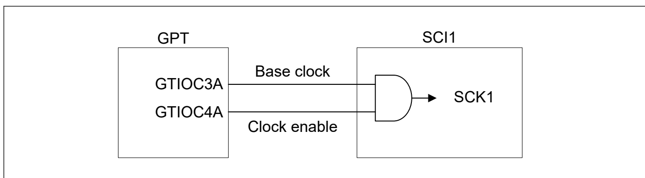
Figure 38.4 Example of GPT and SCI connection
