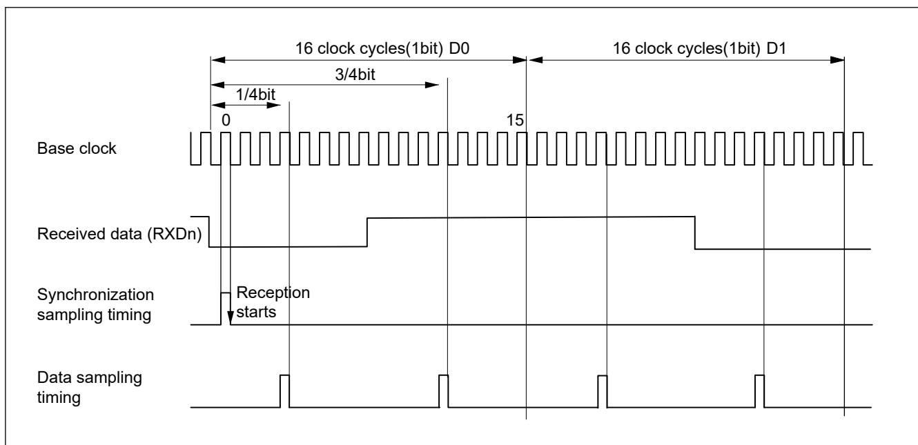
Figure 38.55 Data Reception Sampling Timing in Manchester Mode
