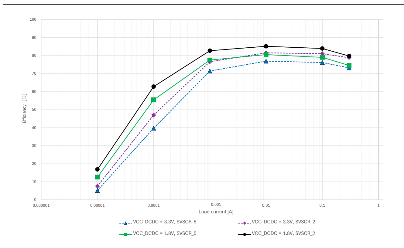
Figure 69.22 Typical DCDC efficiency (%) vs load current (A) in Software Standby mode (SSCR1.SS2LP = SS2LP_1), Tj = 105 °C
