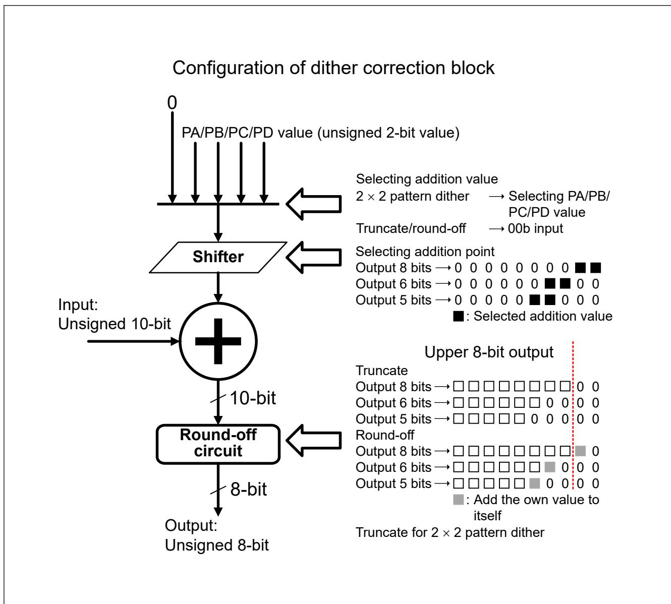
Figure 63.13 Configuration of dither correction block
