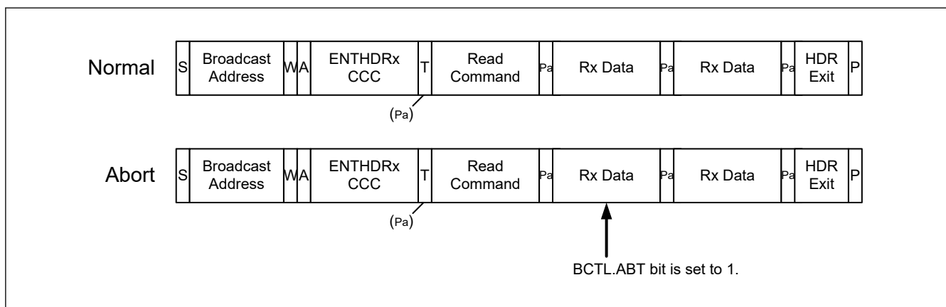
Figure 40.121 Abort operation of HDR-TSP/TSL read transfer
