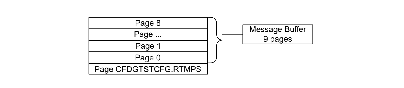
Figure 41.52 RAM page structure
