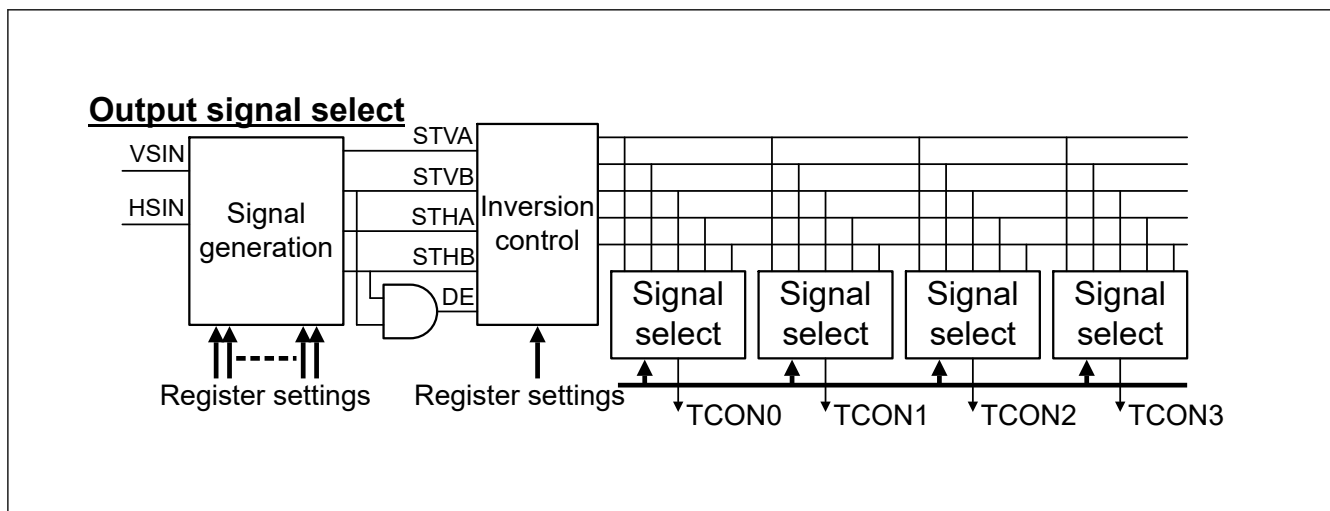
Figure 63.19 Configuration of inversion control and output signal selects
