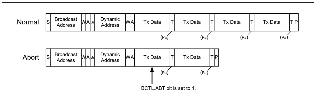
Figure 40.116 Abort operation of SDR write transfer
