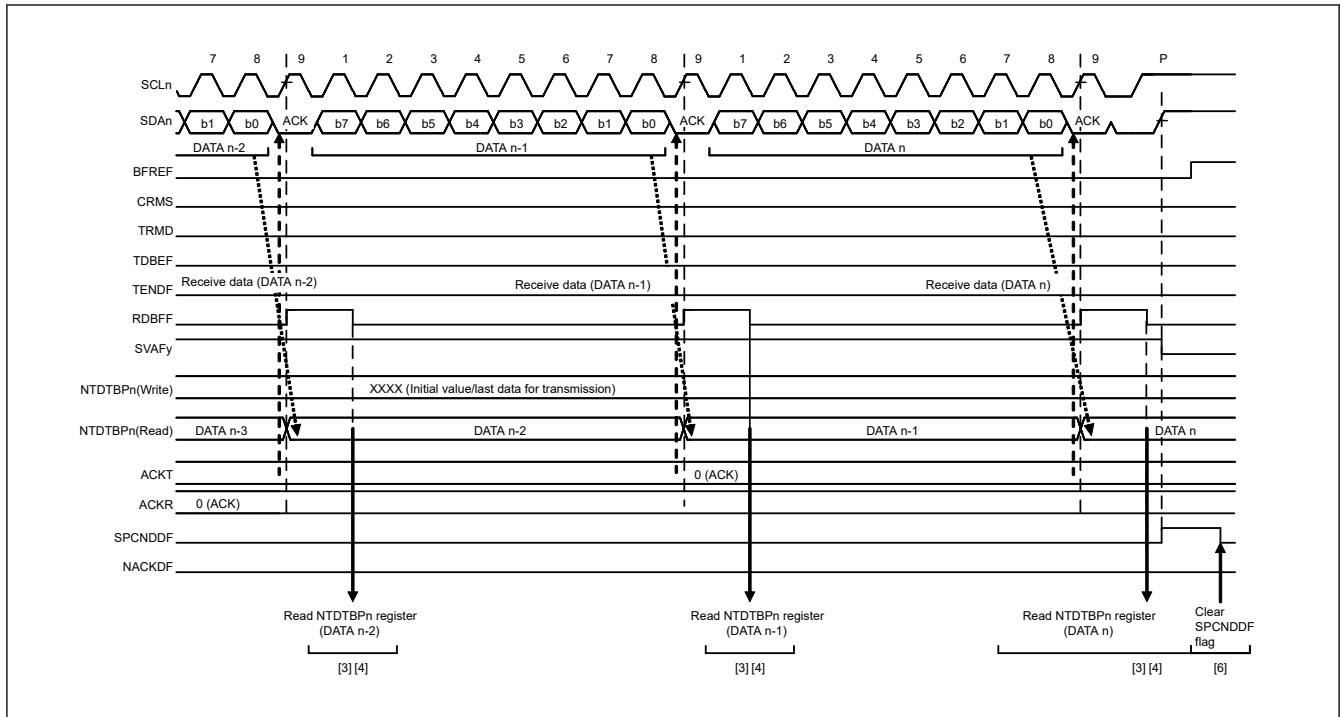
Figure 40.38 Slave receive operation timing (2) (when ACKTWE = 0)
