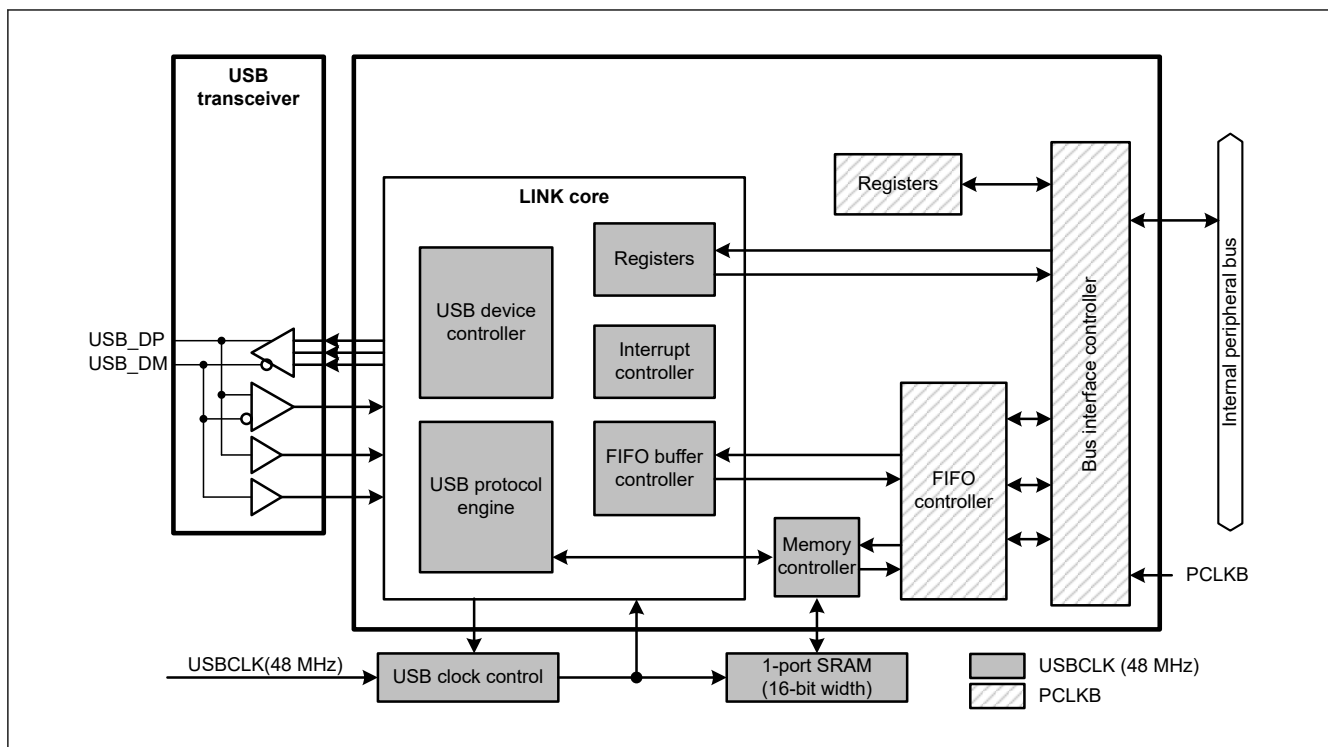
Figure 36.1 USBFS block diagram
