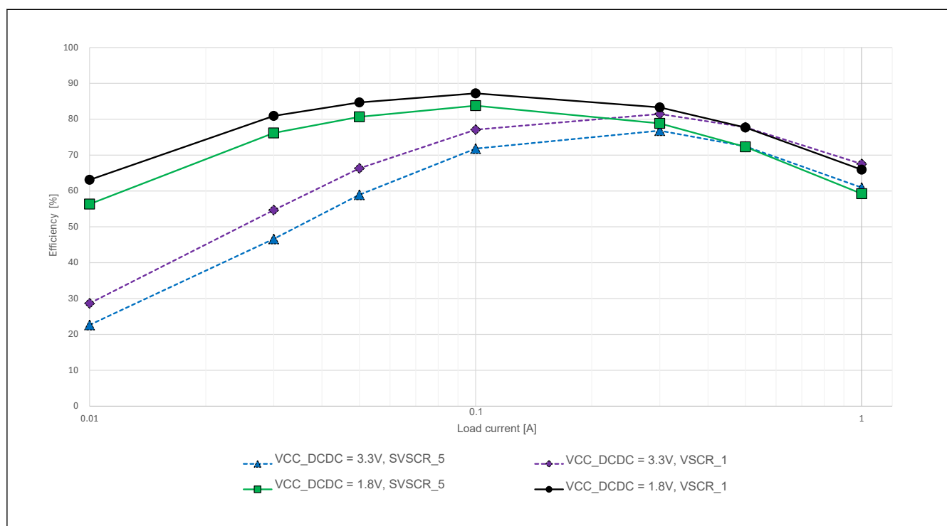
Figure 69.20 Typical DCDC efficiency (%) vs load current (A) in High-speed mode and Software Standby mode (SSCR1.SS2LP = SS2LP_0), Tj = 105 °C
