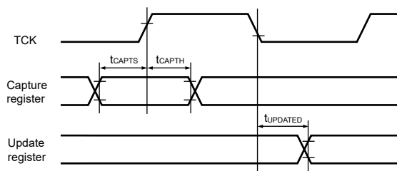
Figure 69.154 Boundary scan input/output timing (2)
