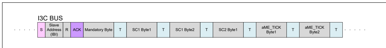
Figure 40.112 Example of asynchronous mode 1 timestamp data transfer
