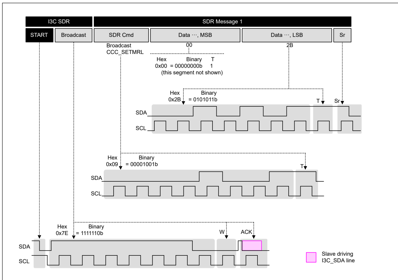
Figure 40.74 Example communication using I3C coding SDR with CCC broadcast
