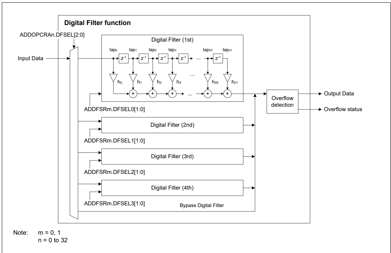
Figure 53.35 Block diagram of digital filter
