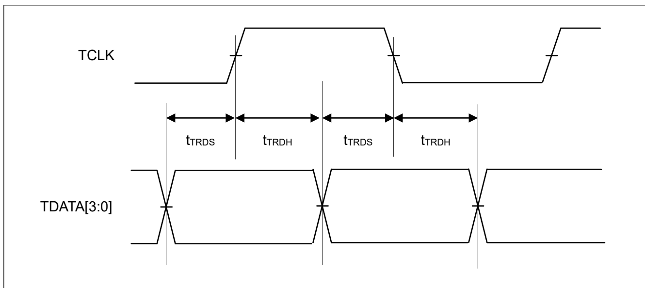
Figure 69.161 ETM output timing
