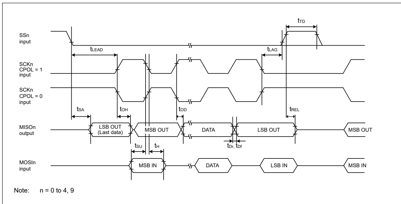
Figure 69.73 SCI simple SPI mode timing for slave when CPHA = 1
