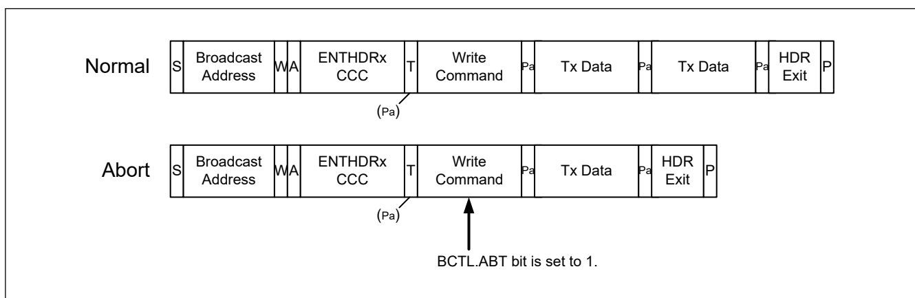
Figure 40.120 Abort operation of HDR-TSP/TSL write transfer
