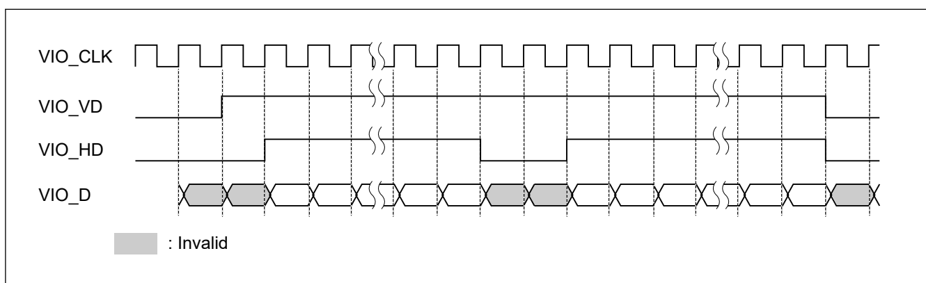
Figure 60.12 Data enable fetch timing (HD asserted (high) while VD is high)
