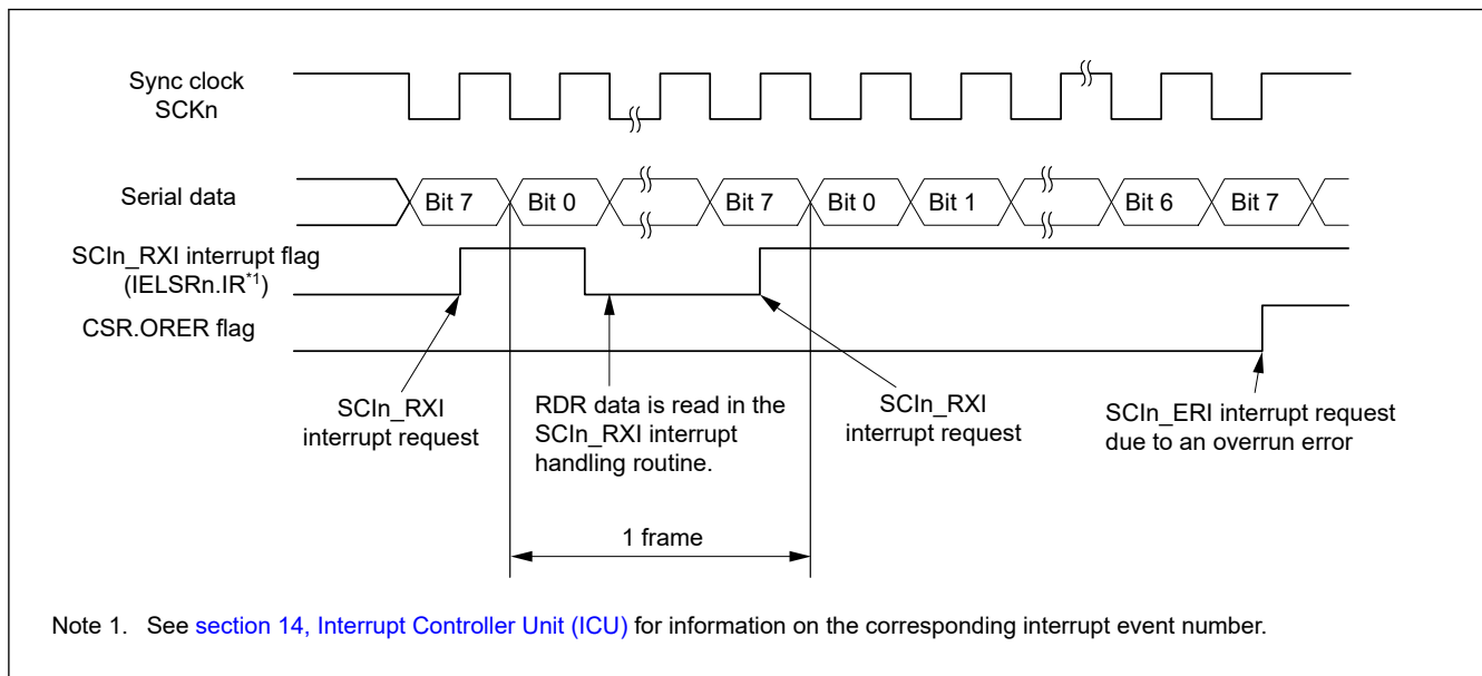
Figure 38.67 Example operation for serial reception in clock synchronous mode (1) when the RTS function is not used
