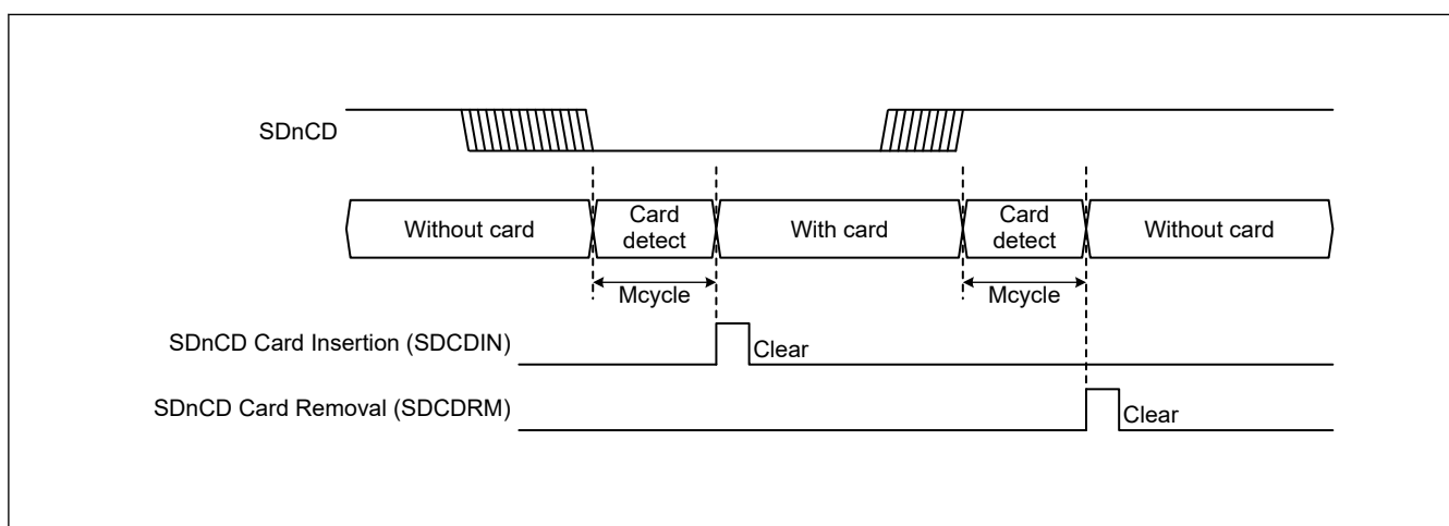
Figure 47.7 Example of card detect with SDnCD
