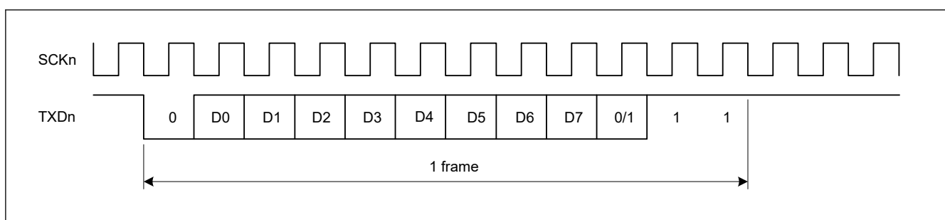
Figure 38.8 Phase relationship between output clock and transmit data in Asynchronous mode when CCR1.PE = 1, CCR3.CHR[1:0] = 10b, MP = 0, and STP = 1
