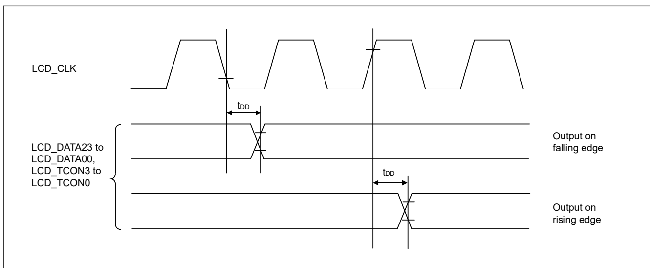
Figure 69.112 Display output timing
