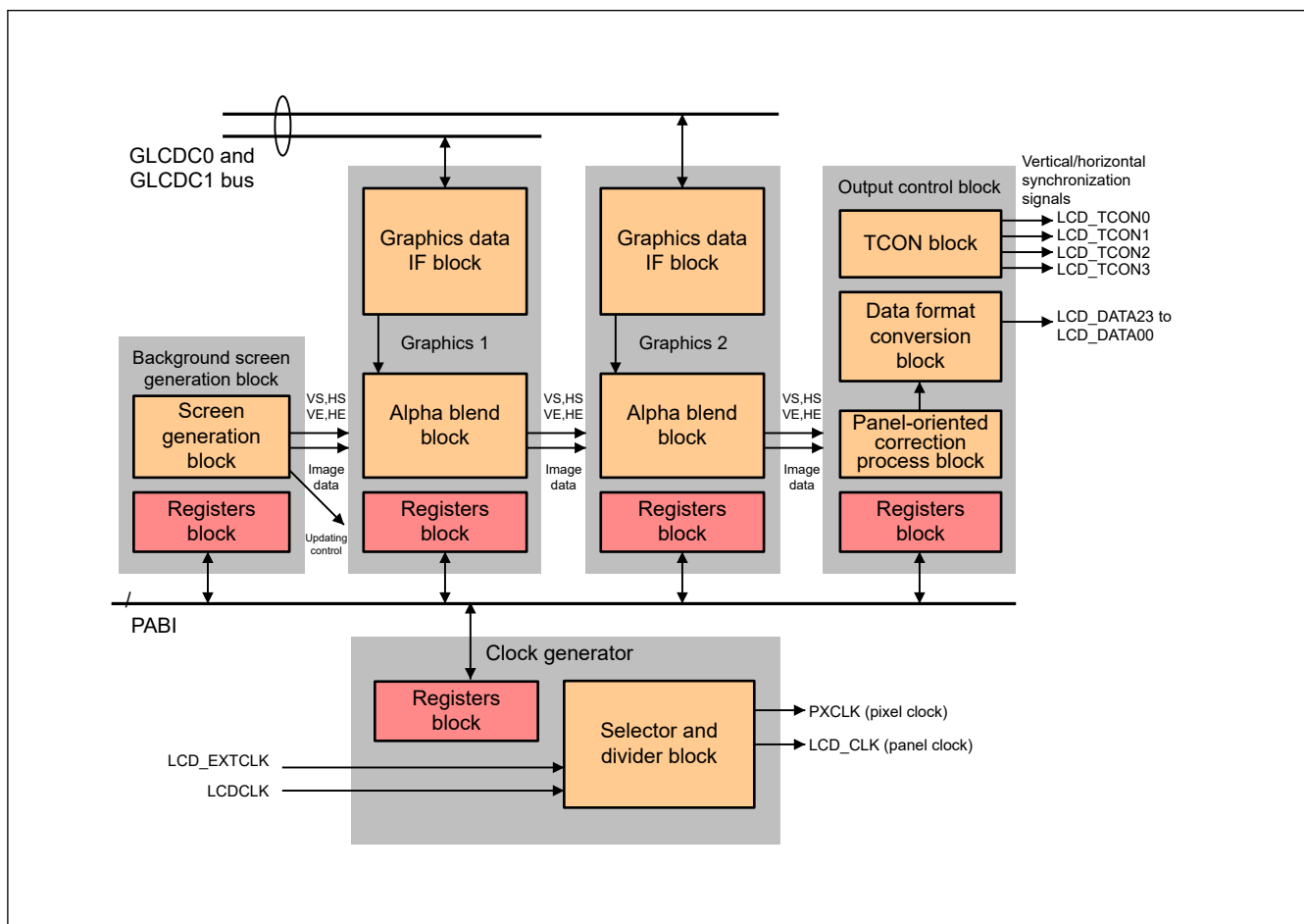
Figure 63.1 GLCDC block diagram
