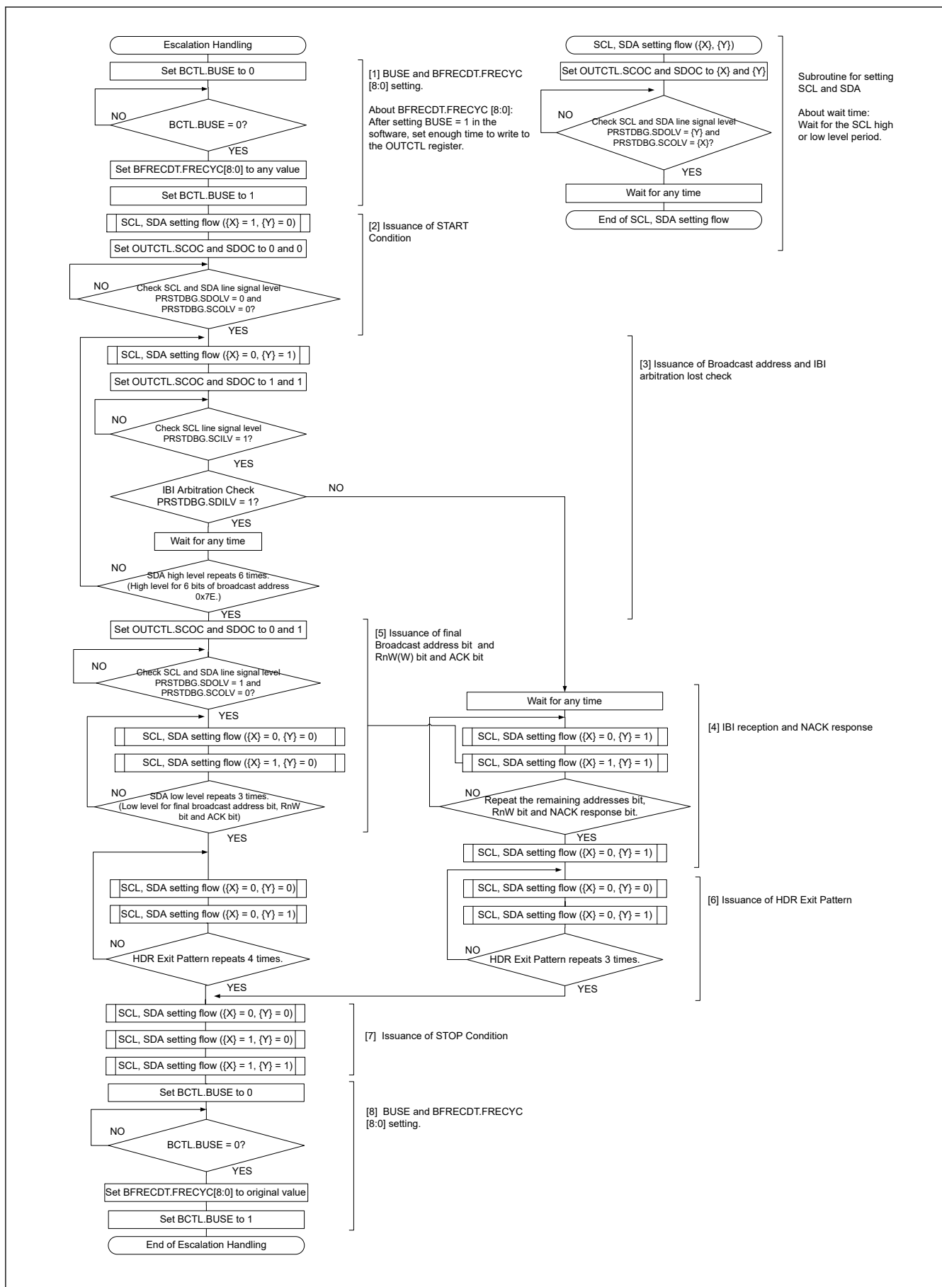
Figure 40.124 Escalation handling flowchart for I3C master
