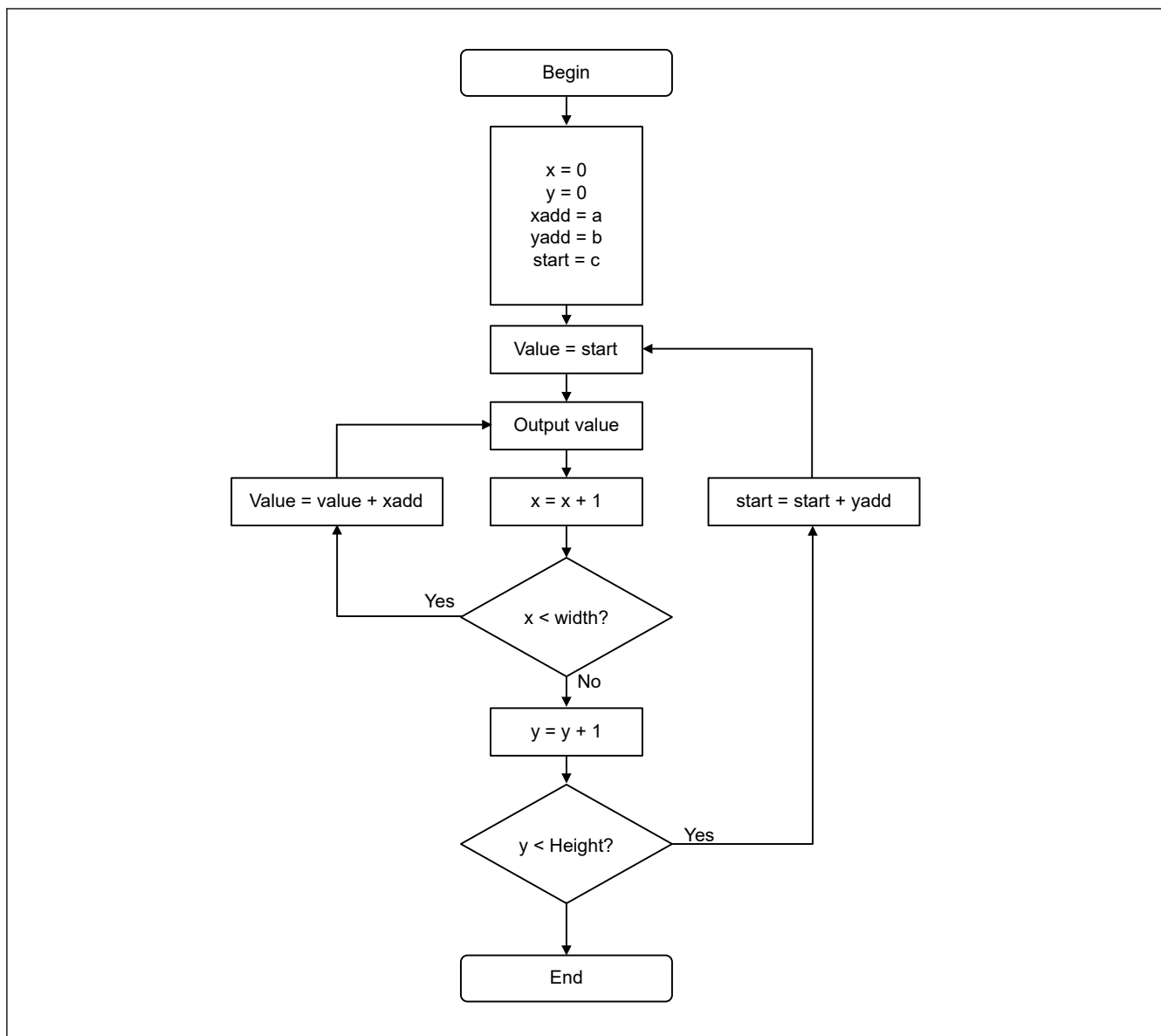
Figure 62.8 Operation flow of the linear limiter
