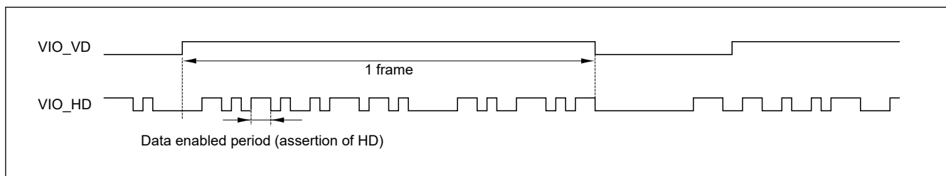
Figure 60.5 Frame timing (data enable fetch)
