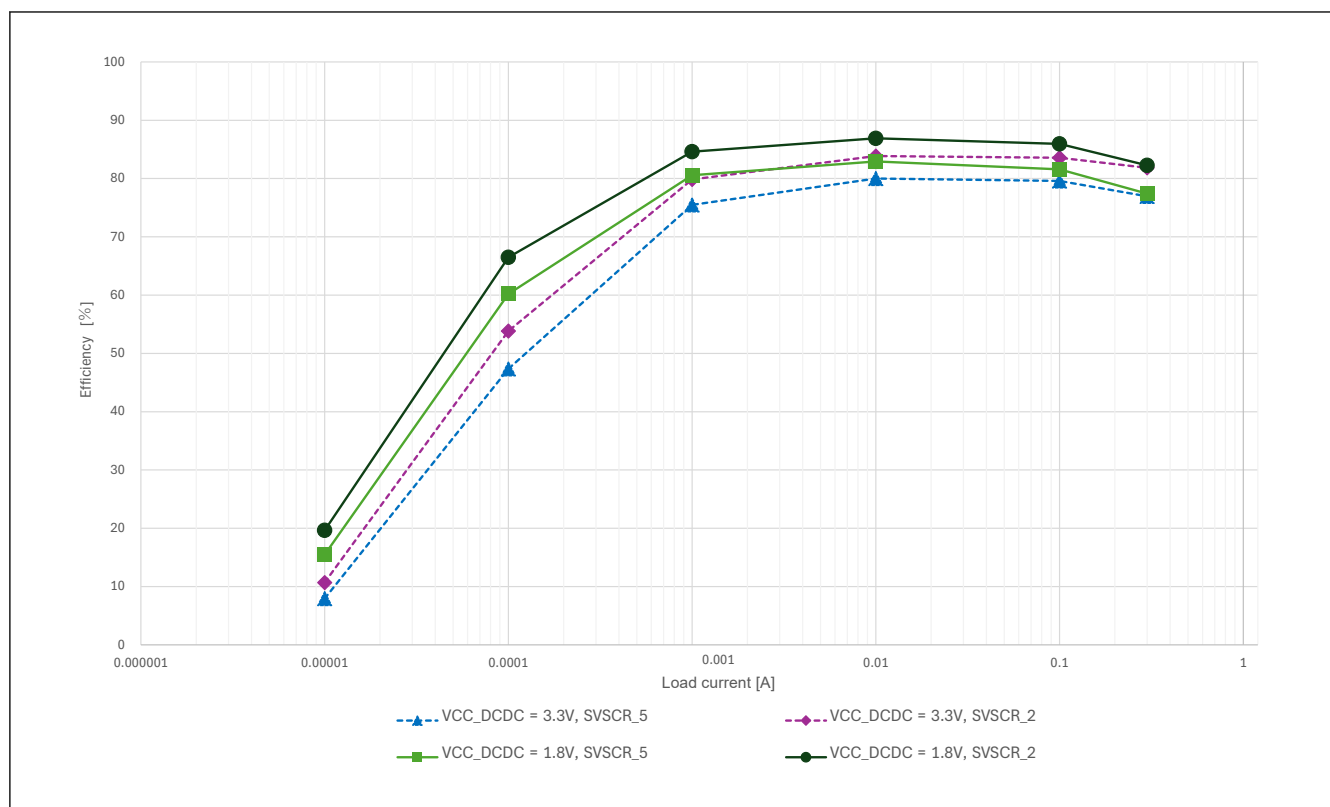
Figure 69.21 Typical DCDC efficiency (%) vs load current (A) in Software Standby mode (SSCR1.SS2LP = SS2LP_1), Tj = 25 °C
