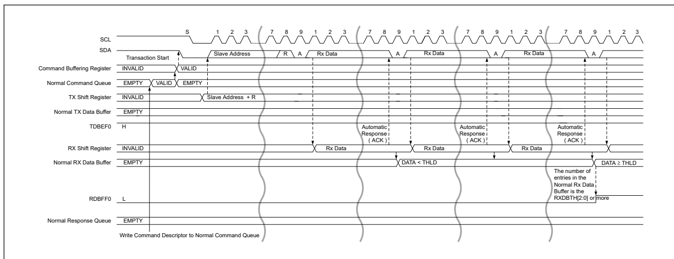
Figure 40.22 Legacy I2C message data read transfer timing (1/2)
