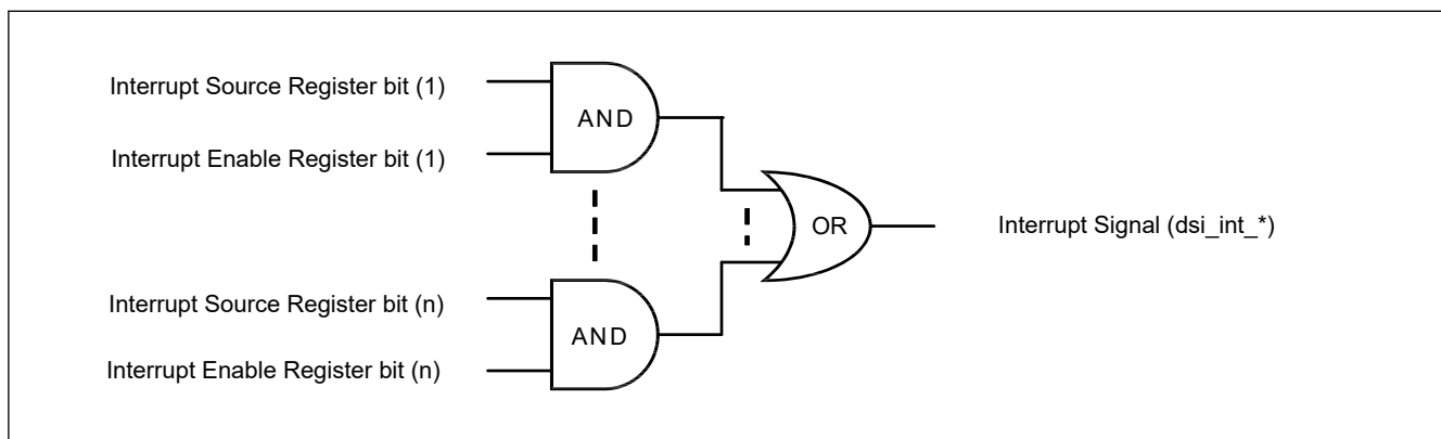
Figure 65.3 Interrupt signal output
