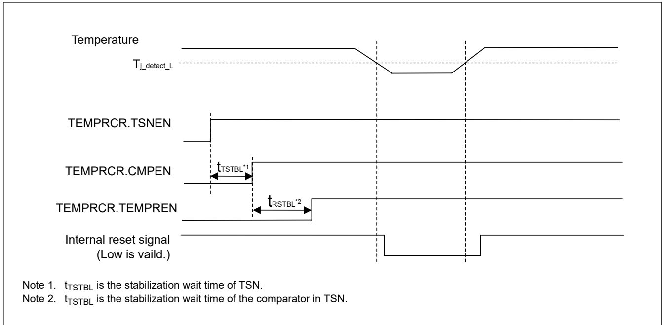
Figure 69.149 Timing of temperature monitor reset (Low-temperature detection)
