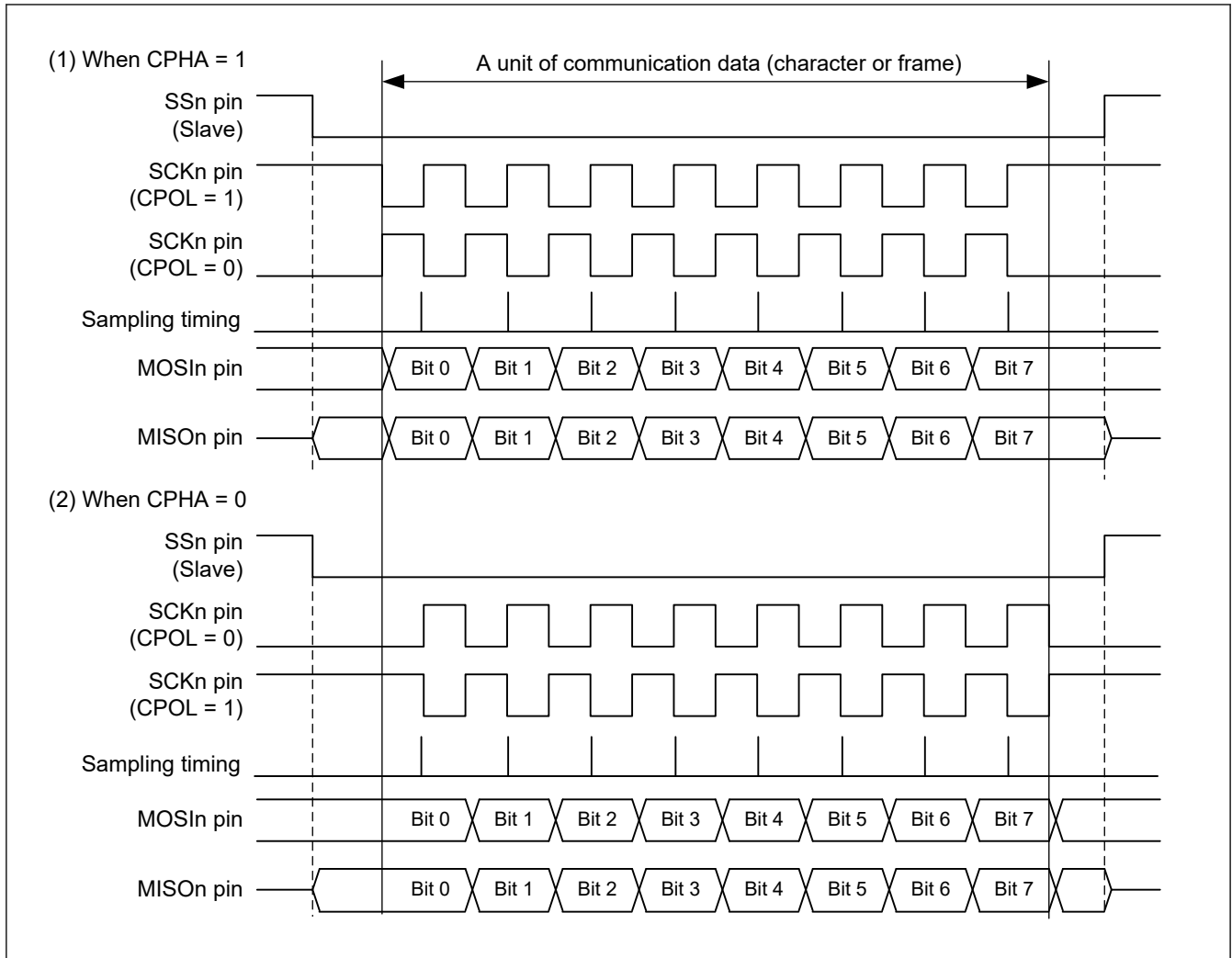
Figure 38.99 Relation between clock signal and transmit or receive data in simple SPI mode
