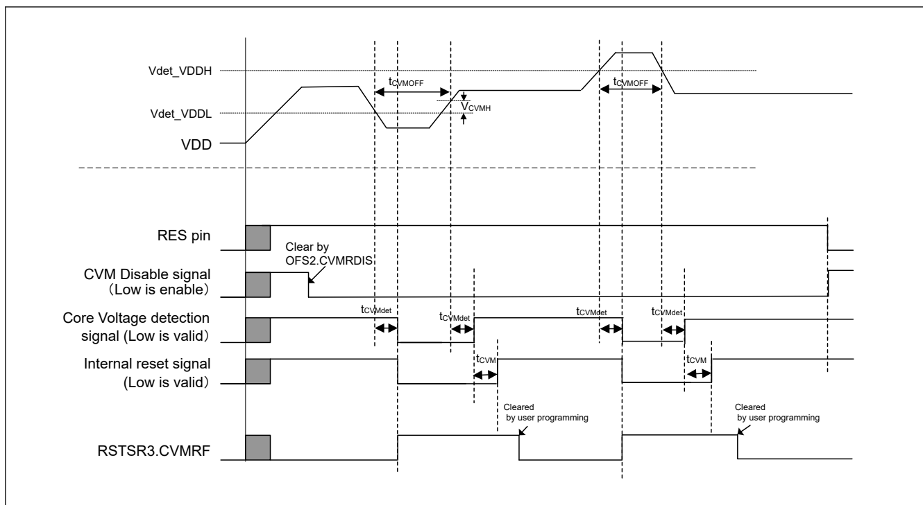
Figure 69.147 Timing of core voltage monitor reset
