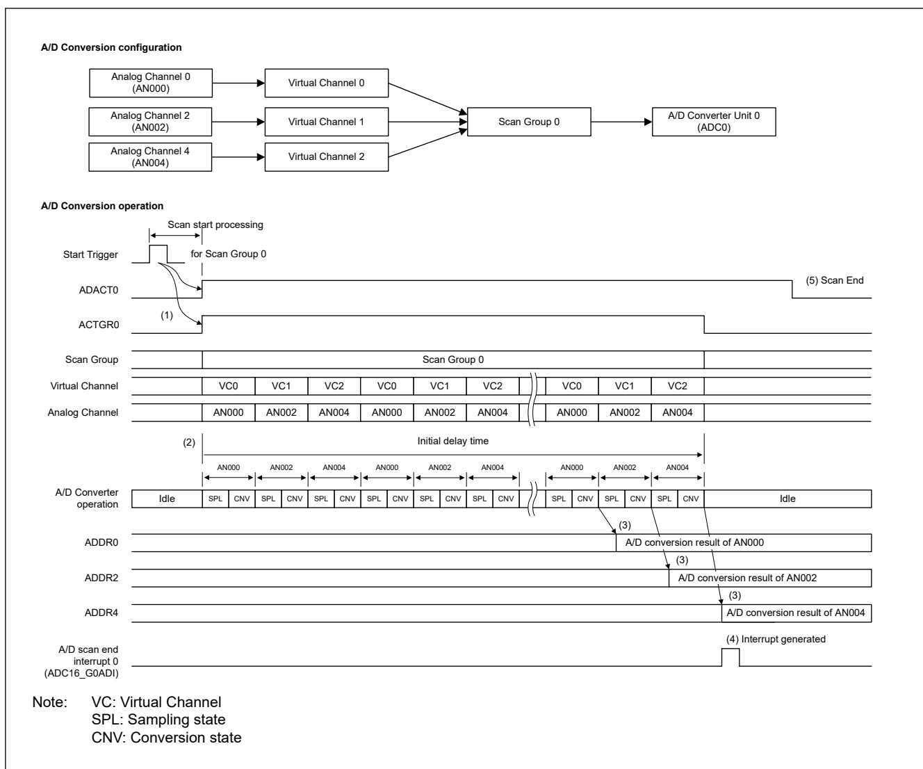
Figure 53.12 Example of scanning operation in Hybrid mode – Single scan mode
