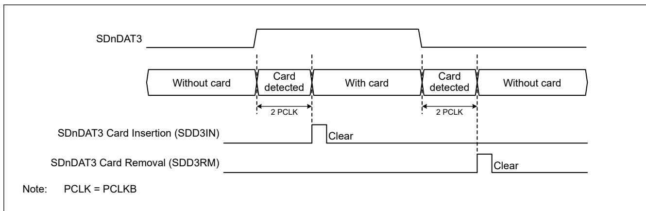
Figure 47.8 SD card detect with SDnDAT3
