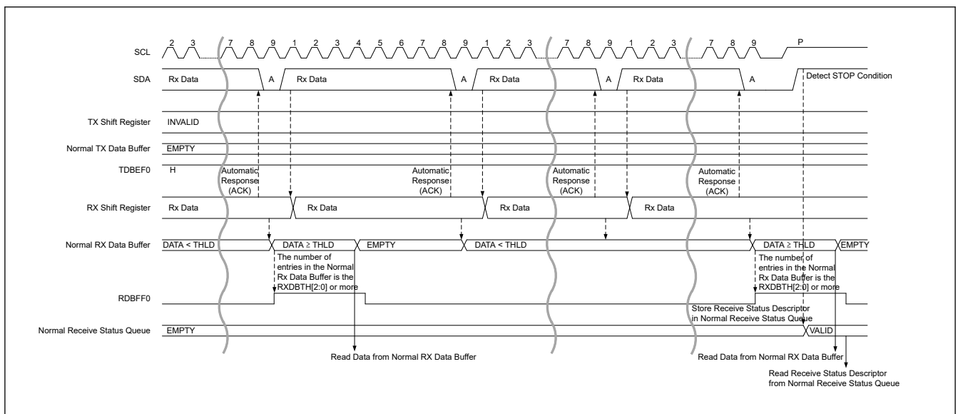
Figure 40.48 Legacy I 2 C message data write transfer timing (2/2)
