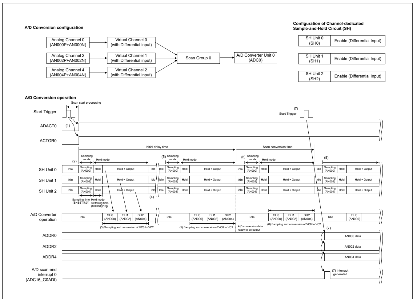
Figure 53.22 Basic operation of channel-dedicated sample-and-hold circuit in Hybrid mode – Background continuous scan mode
