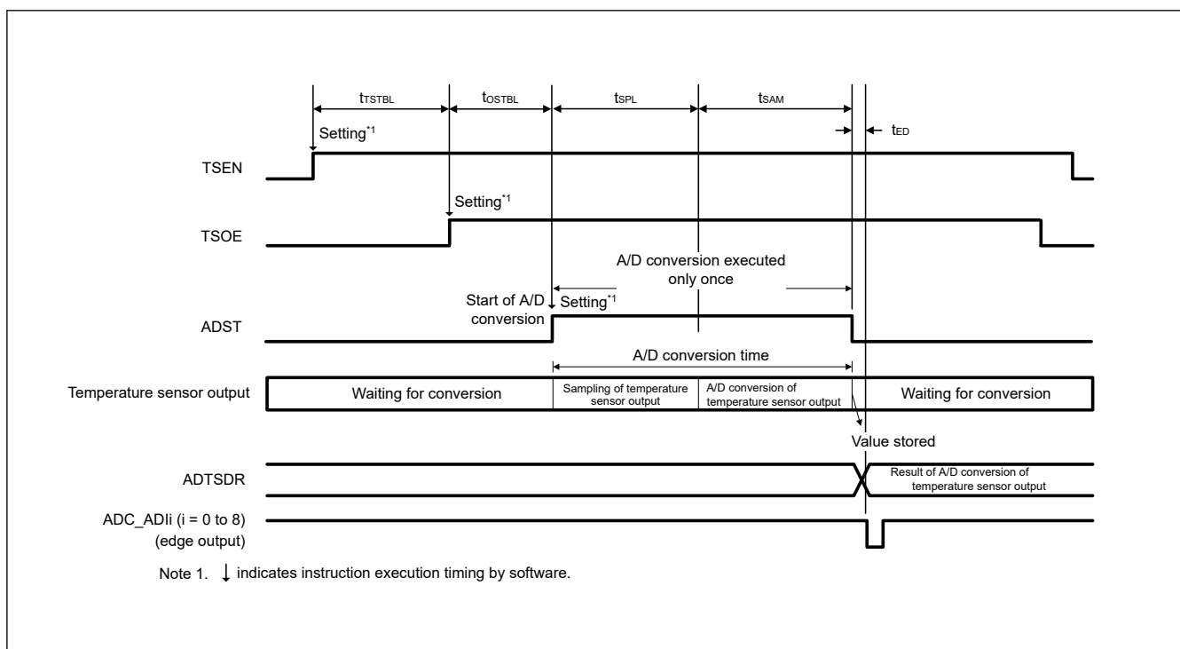
Figure 55.3 Timing from start of temperature sensor operation until completion of A/D conversion
