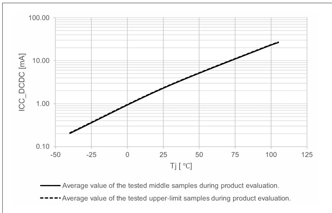
Figure 69.6 Temperature dependency in Software Standby mode ( ICC\_DCDC , SS2LP\_1 , SVSCR\_5 ) (reference data)
