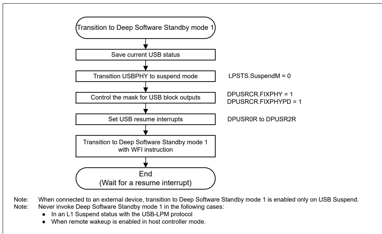
Figure 37.22 USBHS setup flow for transition to Deep Software Standby mode 1 as a host or device controller
