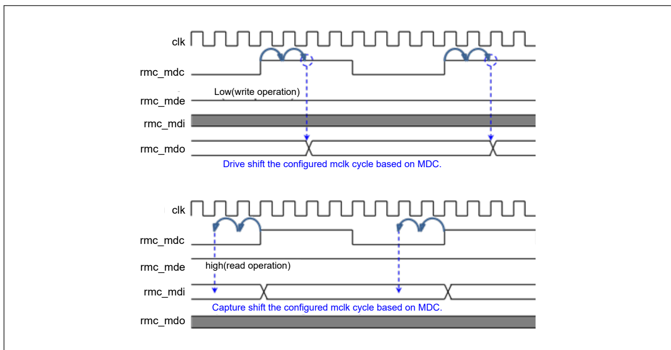
Figure 33.27 Management data timing adjustment
