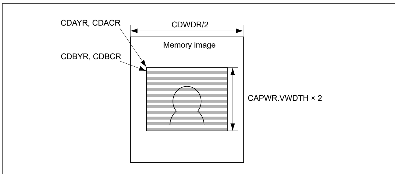
Figure 60.29 Image of storing Interlace input as frame image in memory
