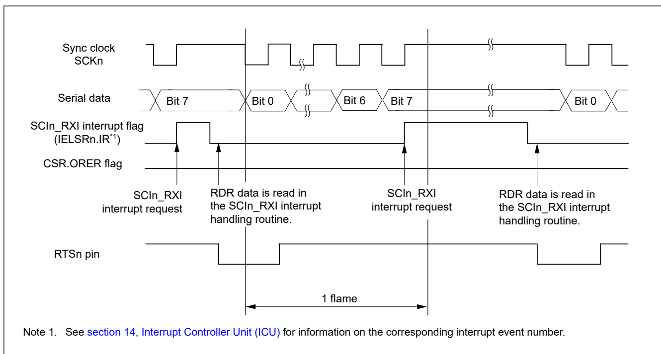
Figure 38.68 Example operation for serial reception in clock synchronous mode (2) when RTS function is used
