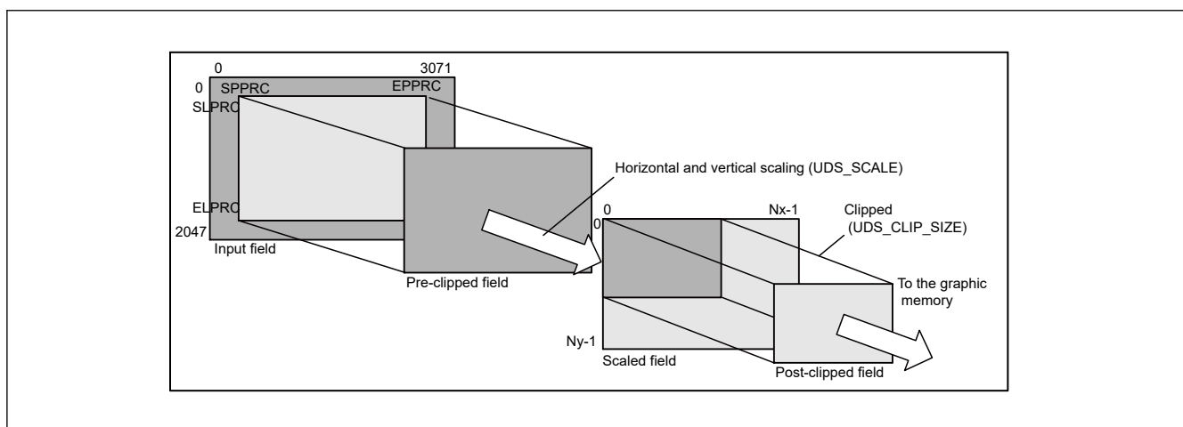
Figure 67.7 Example of clipping
