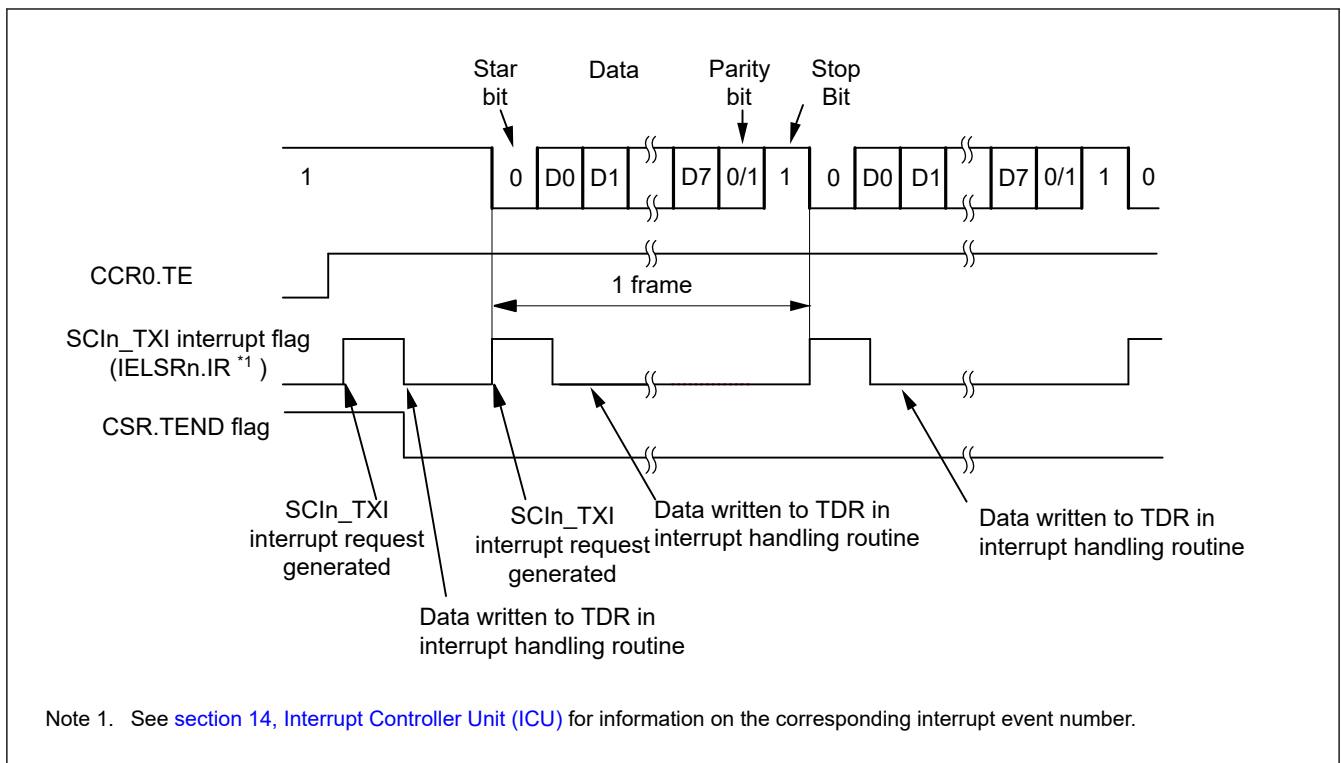
Figure 38.12 Example operation for serial transmission in Asynchronous mode (1) with 8-bit data, parity bit, 1 stop bit, CTS function not used, and at the beginning of transmission
