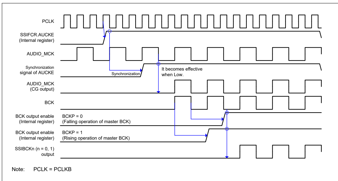
Figure 46.26 Timing diagram for the operation from system reset to start of master-mode communication
