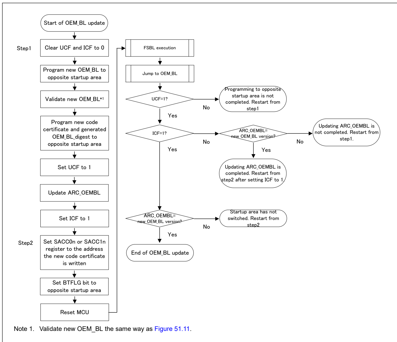
Figure 51.15 OEM_BL update flow
