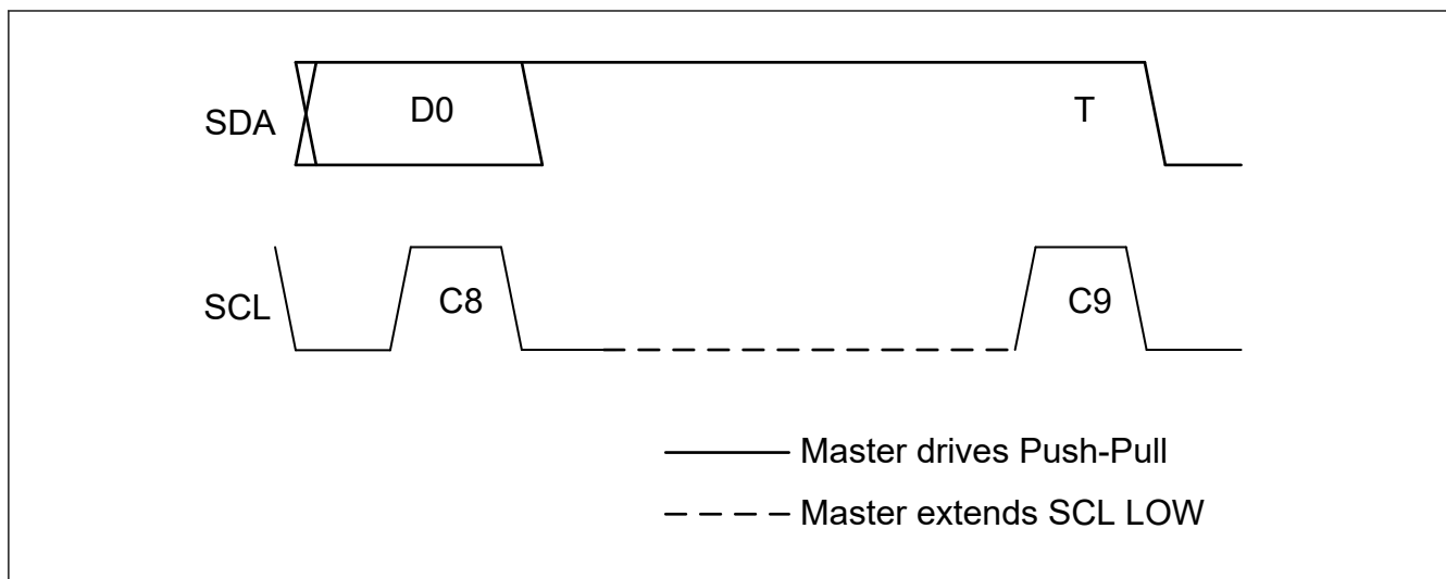
Figure 40.97 Master clock stalling in write parity bit
