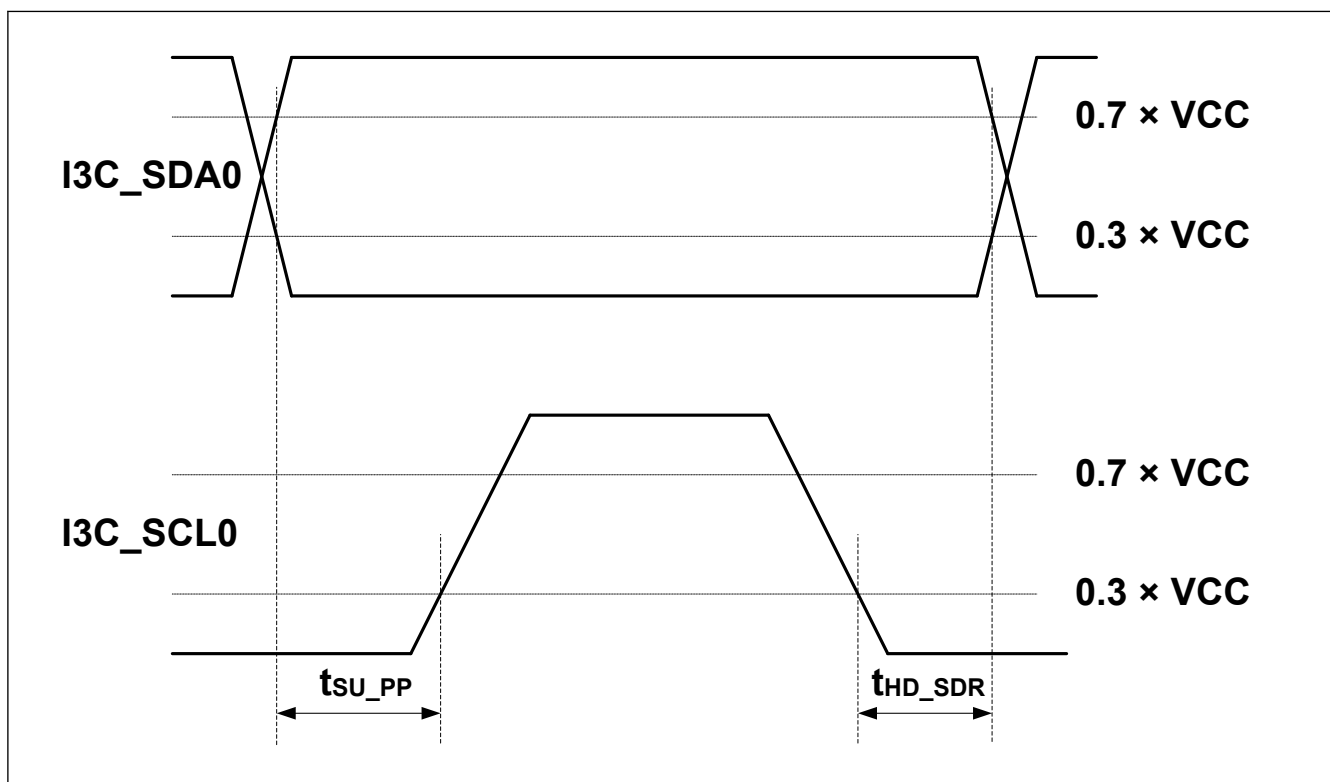
Figure 69.97 Master SDR Timing
