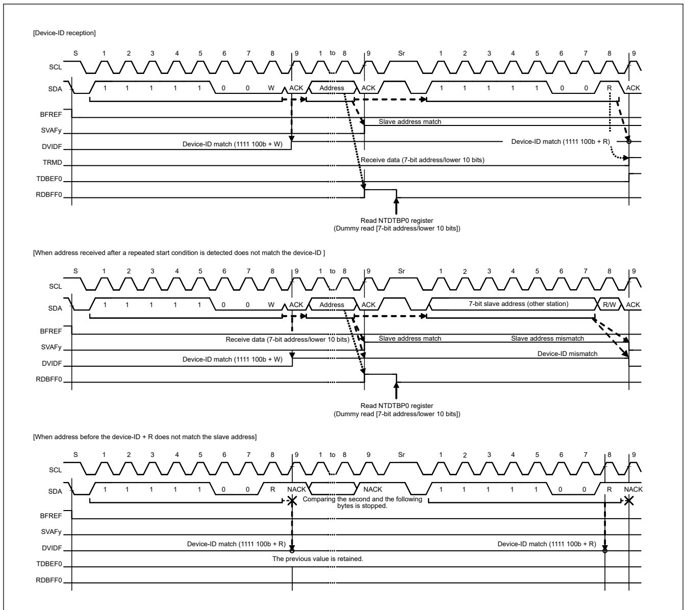
Figure 40.86 SVAfY/DVIDF flag set/clear timing during reception of device-ID
