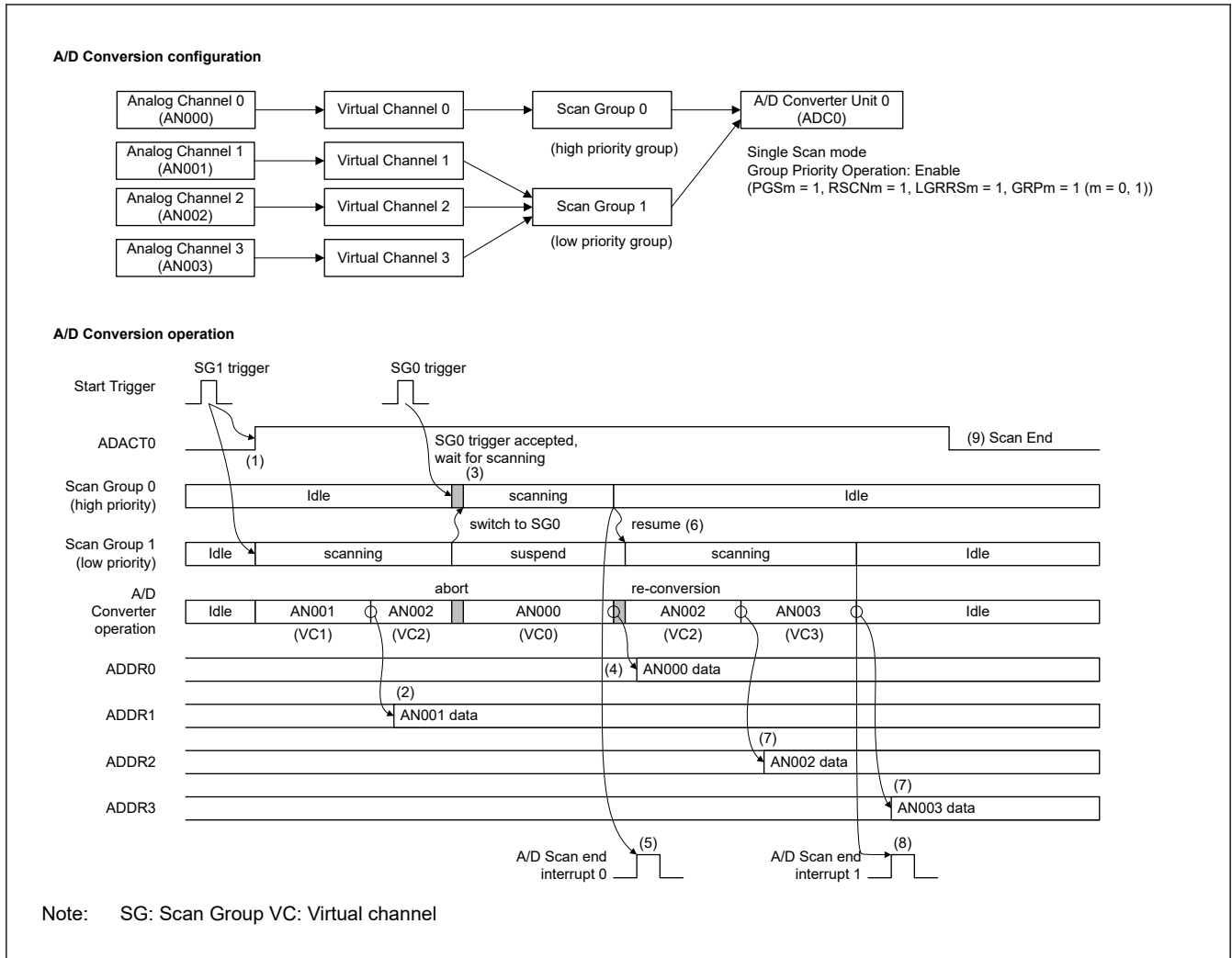
Figure 53.28 Example of group priority operation in SAR mode – Single scan mode (2 groups)
