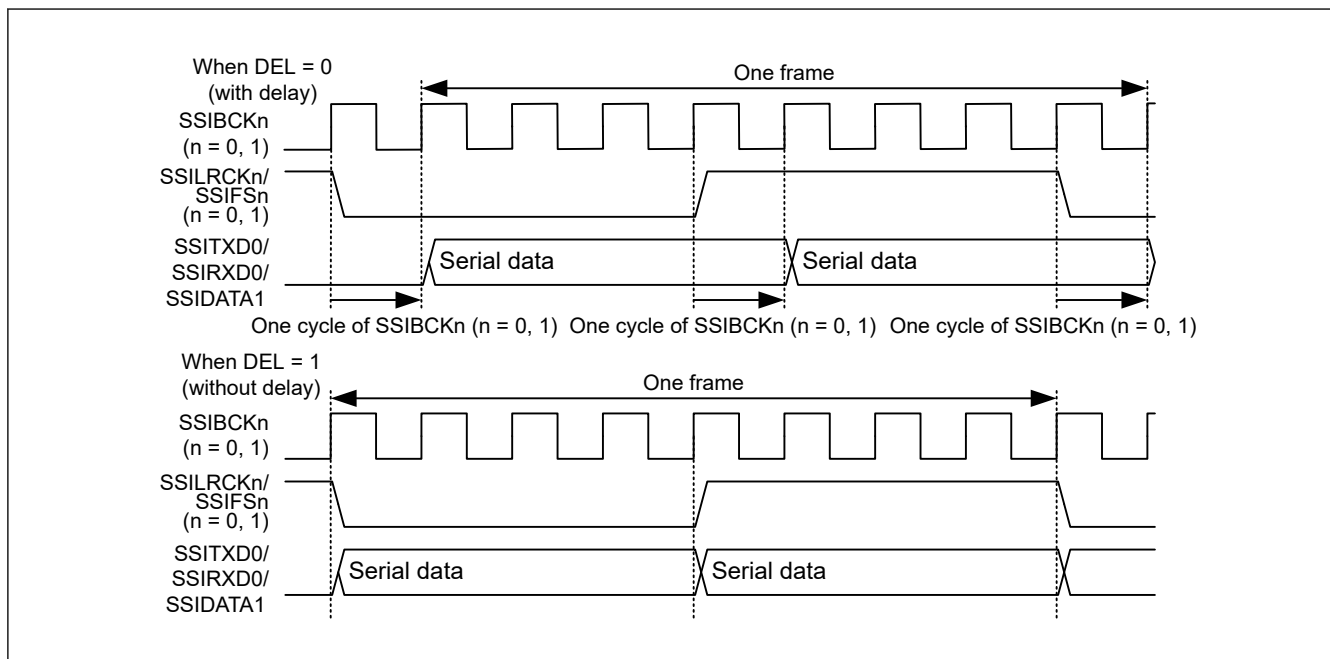
Figure 46.7 Setting of delay in serial data
