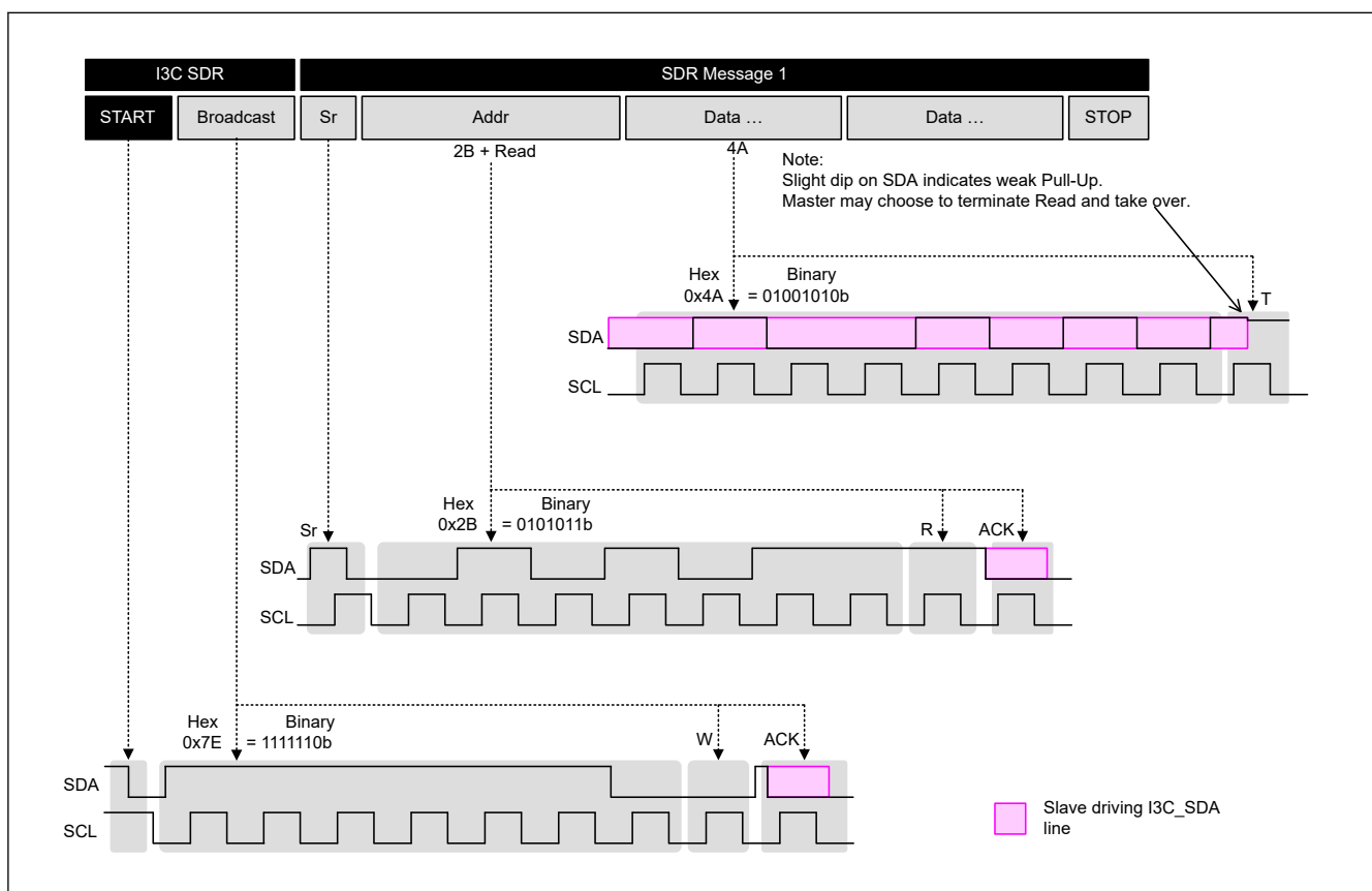
Figure 40.71 Example communication using I3C coding SDR with broadcast (0x7E)
