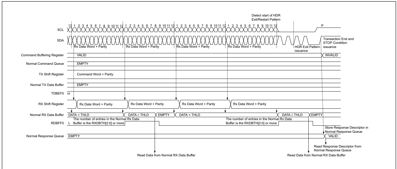
Figure 40.33 HDR data read transfer (HDR-TSP, TSL) timing (2/2)
