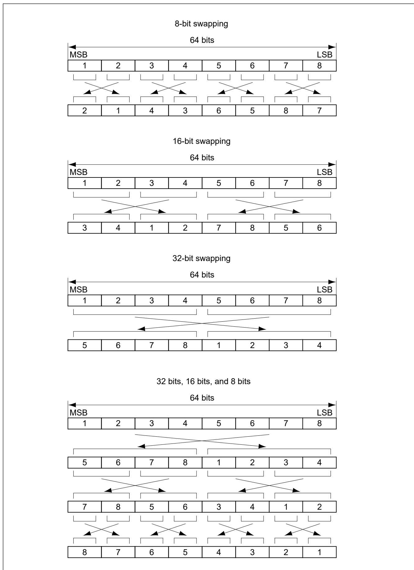
Figure 60.44 Data swapping by data aligner
