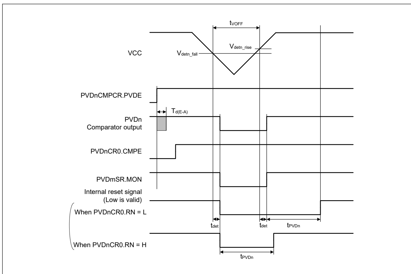
Figure 69.144 Voltage detection circuit timing ( V_{\text{detn}} ) ( n = 1, 2, 4, 5 )
