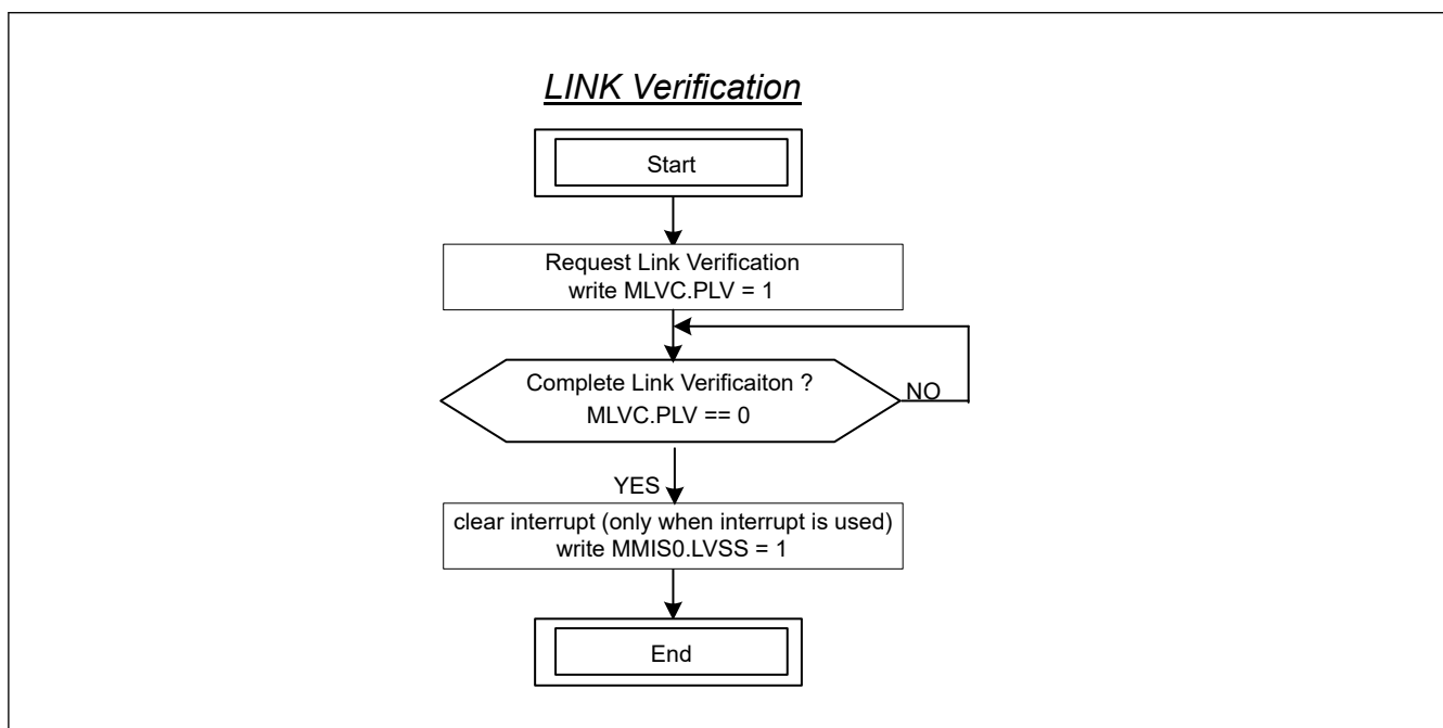
Figure 33.11 Link Verification flow
