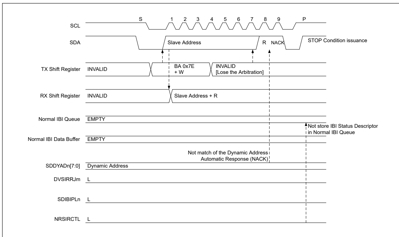
Figure 40.102 Slave interrupt request : NACK (not match the SDDYAD[7:0] of DAT) and NRSIRCTL = 0
