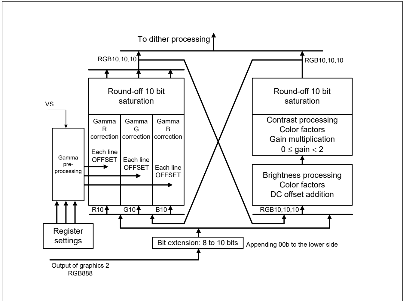
Figure 63.6 Configuration of panel-oriented correction circuit
