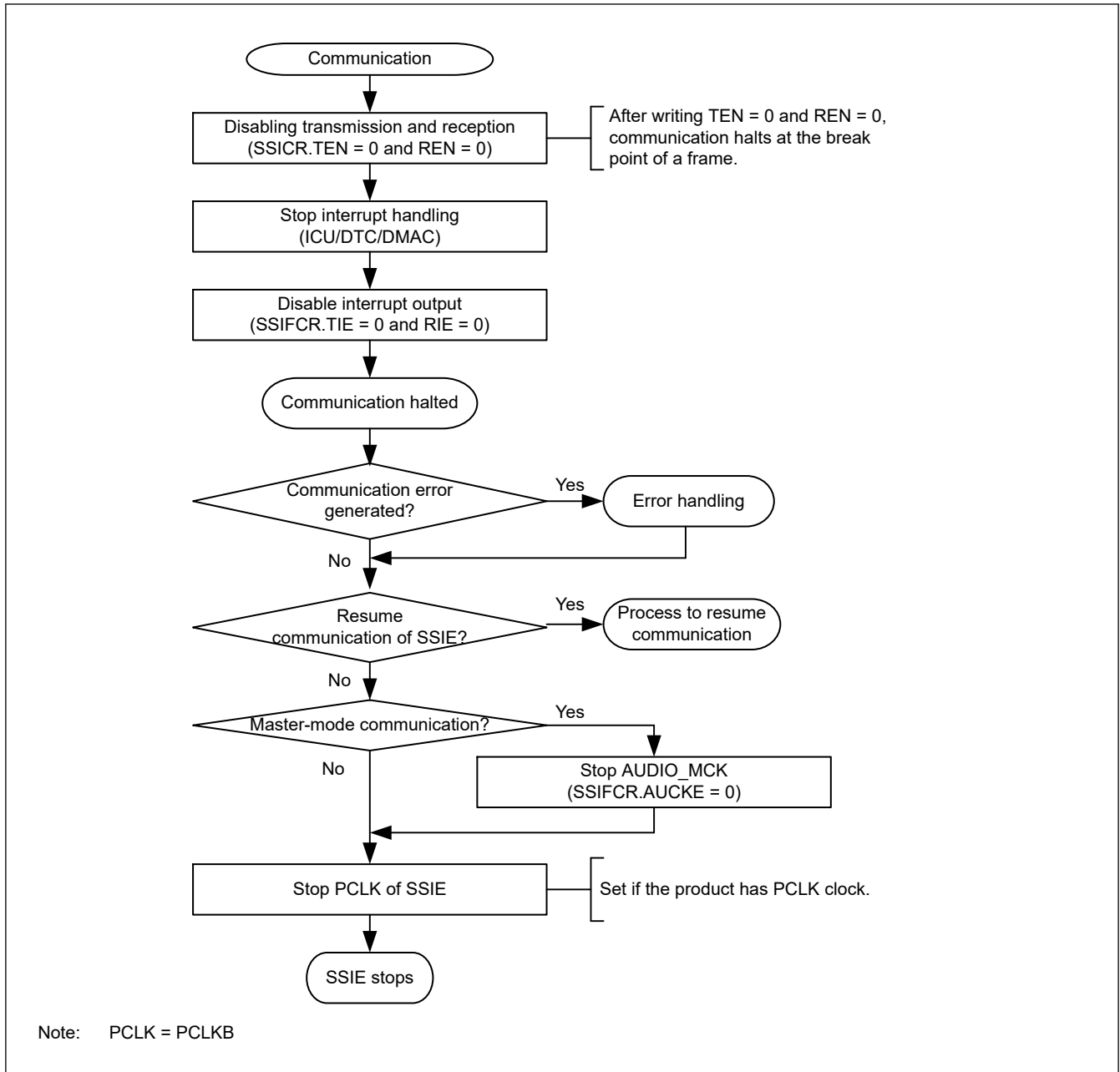
Figure 46.56 Procedure to halt communication (CPU operation procedure)
