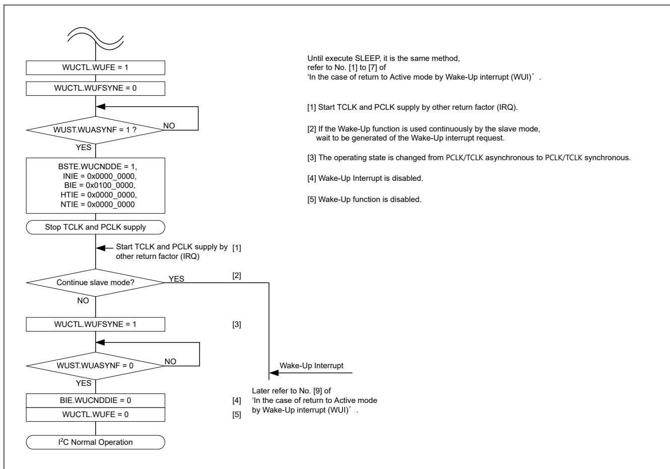
Figure 40.127 Use case of normal WU modes 1 and 2 (wake-up recovery by other recovery causes (IRQ))
