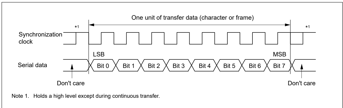
Figure 38.61 Data format in clock synchronous serial communications with LSB-first order
