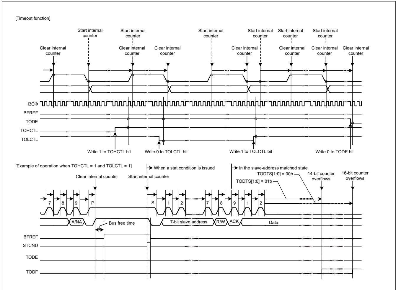
Figure 40.115 Timeout error detection (TODE, TODTS[1:0], TOHCTL, and TOLCTL bits)
