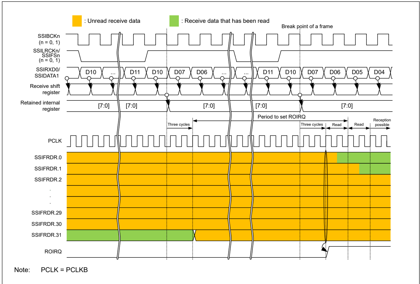
Figure 46.16 ROIRQ setting timing
