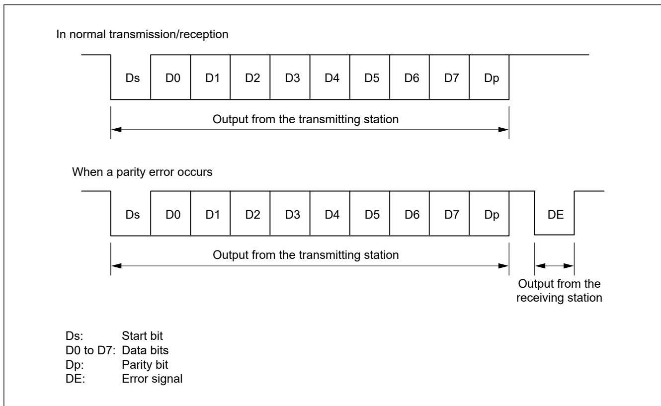
Figure 38.75 Data formats in smart card interface mode
