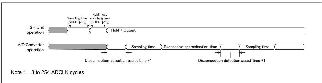
Figure 53.25 Operation of A/D conversion when the disconnection detection assist function and channel-dedicated sample-and-hold circuit are used
