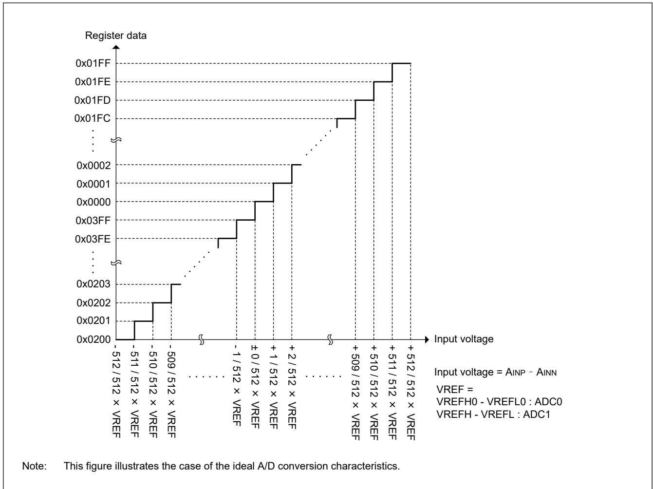
Figure 53.49 Data range of A/D conversion result (10-bit data length, Signed data, Differential input)
