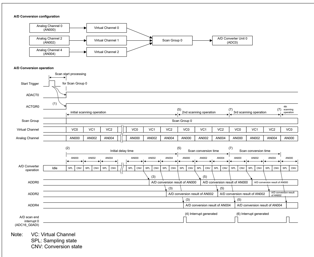
Figure 53.13 Example of scanning operation in Hybrid mode – Continuous scan mode
