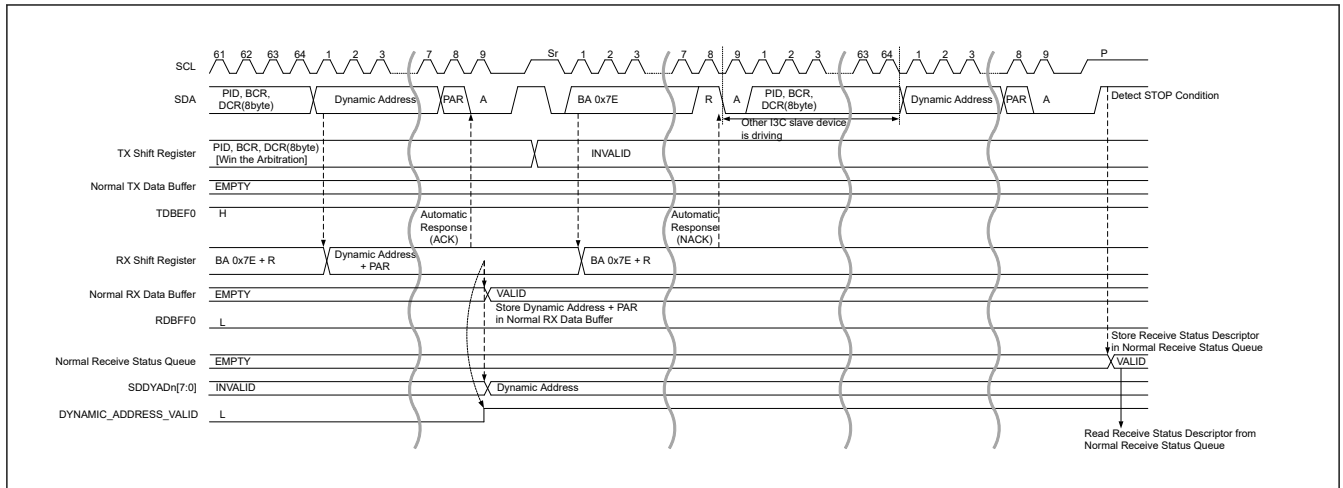
Figure 40.43 Dynamic address assign procedure (ENTDAA CCC) timing (3/3)
