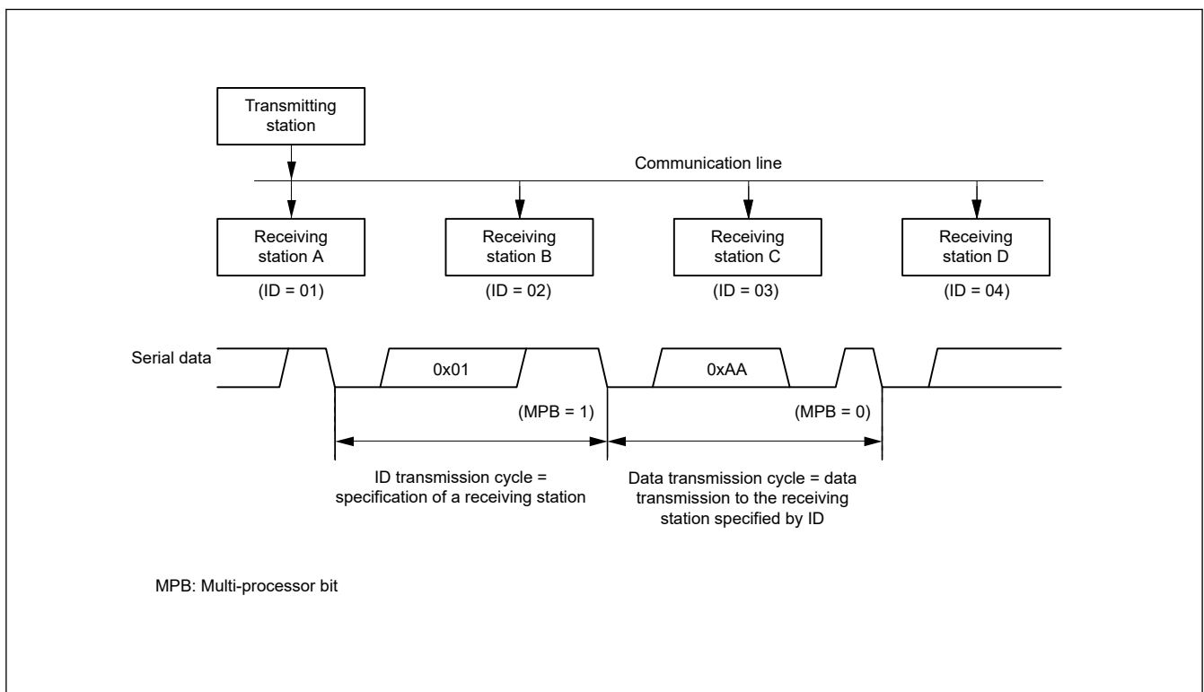
Figure 38.35 Example of communication using multi-processor format with transmission of data 0xAA to receiving station A
