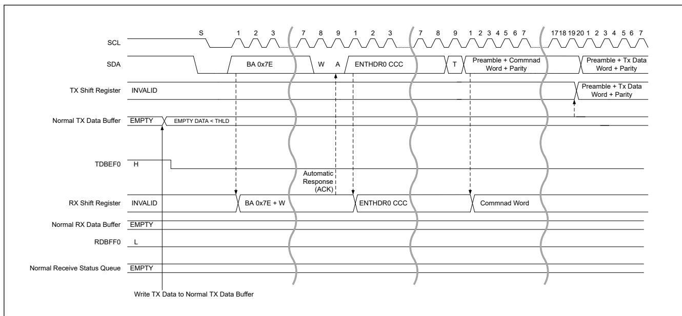
Figure 40.58 HDR data read transfer (HDR-DDR) timing (1/3)
