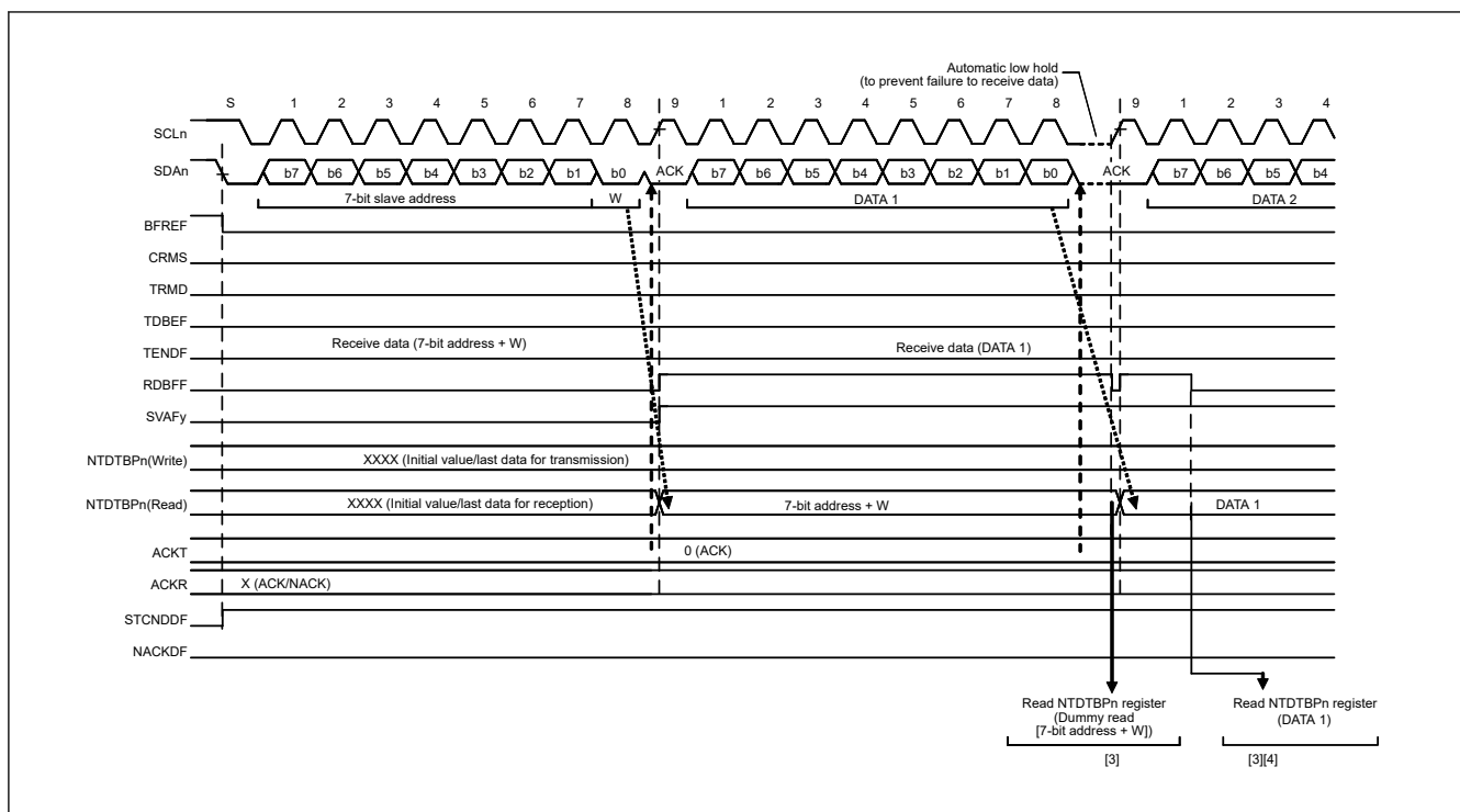
Figure 40.37 Slave receive operation timing (1) (7-bit address format, when ACKTWE = 0)
