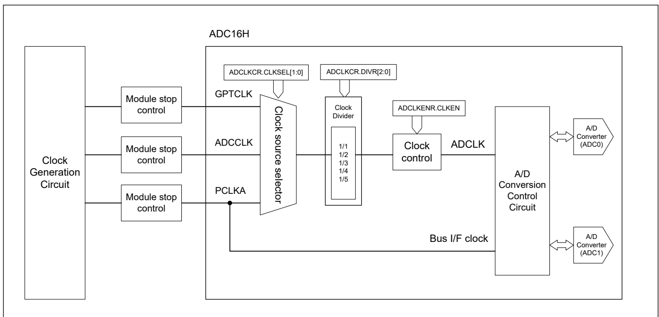
Figure 53.4 Clock structure
