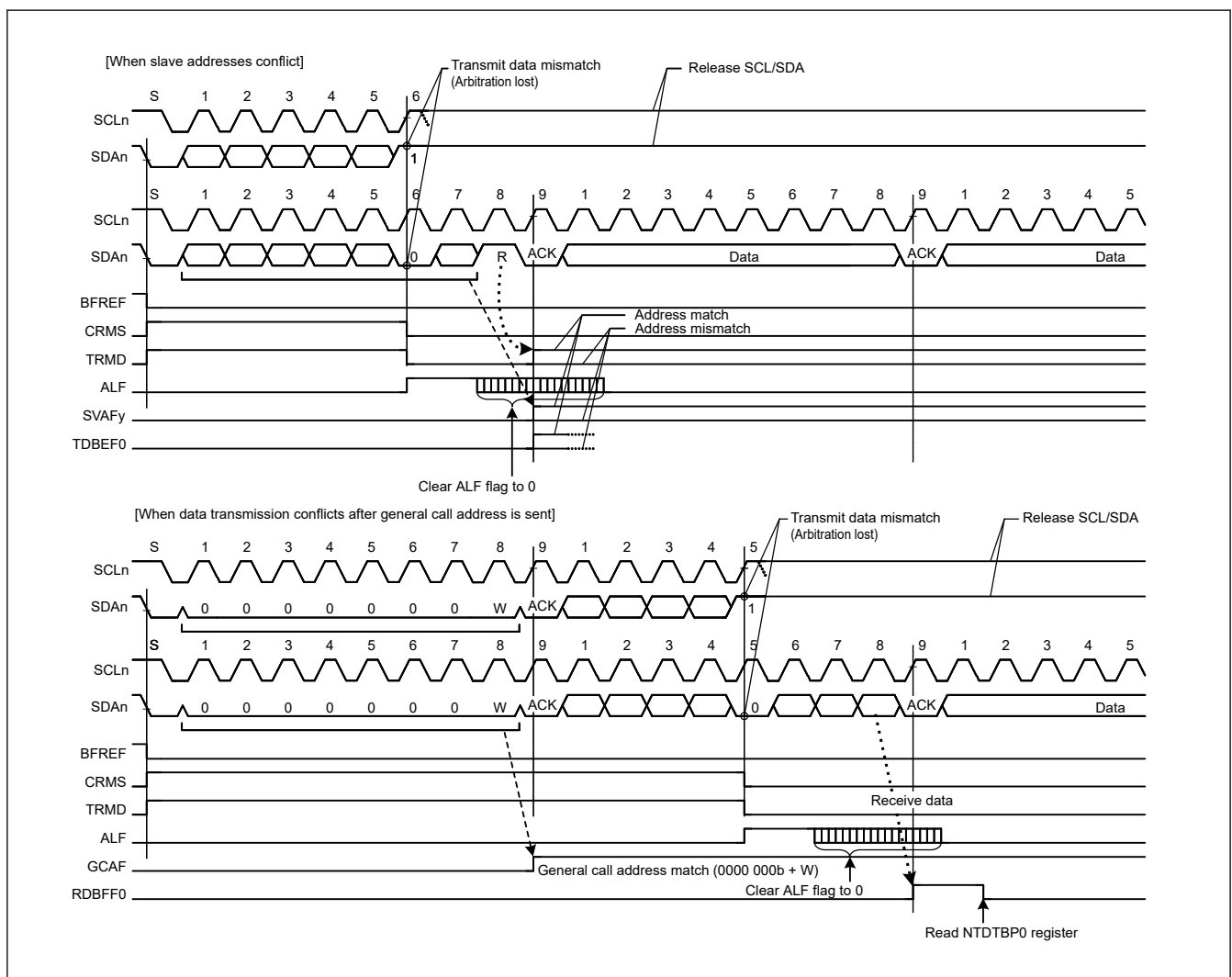
Figure 40.89 Examples of master arbitration-lost detection (MALE = 1)
