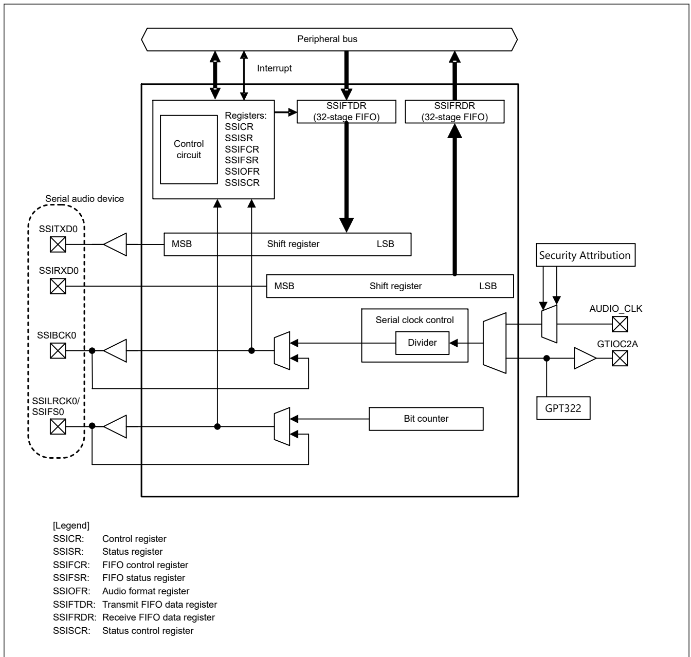
Figure 46.2 SSIE block diagram (SSIE0)
