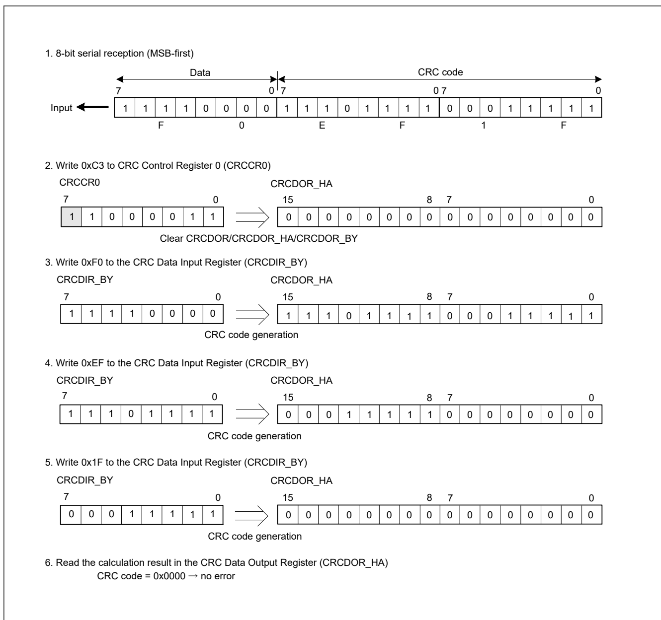
Figure 48.5 MSB-first data reception
