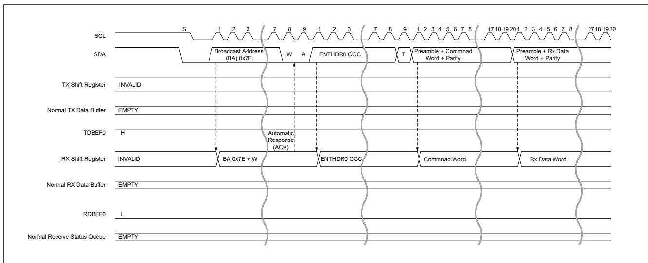
Figure 40.53 HDR data write transfer (HDR-DDR) timing (1/3)
