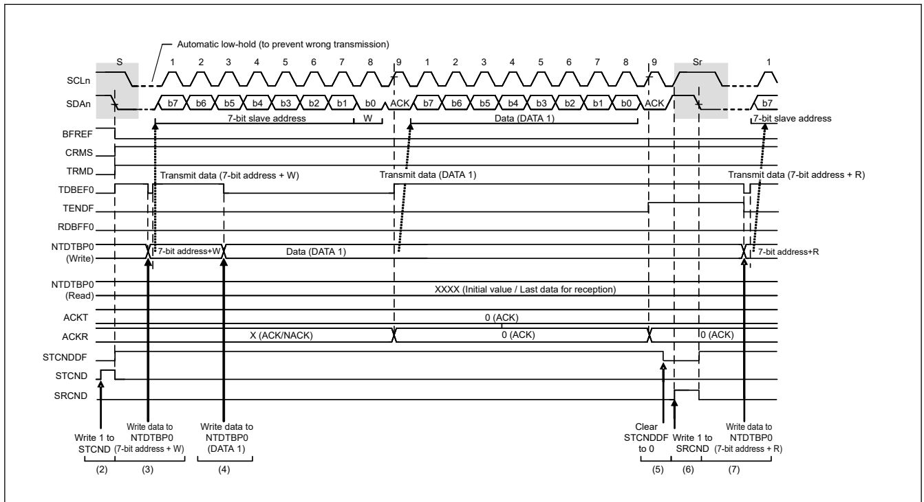
Figure 40.80 Repeated START condition issuance after the master transmission timing
