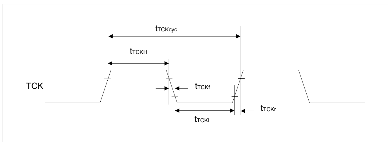
Figure 69.156 JTAG TCK timing
