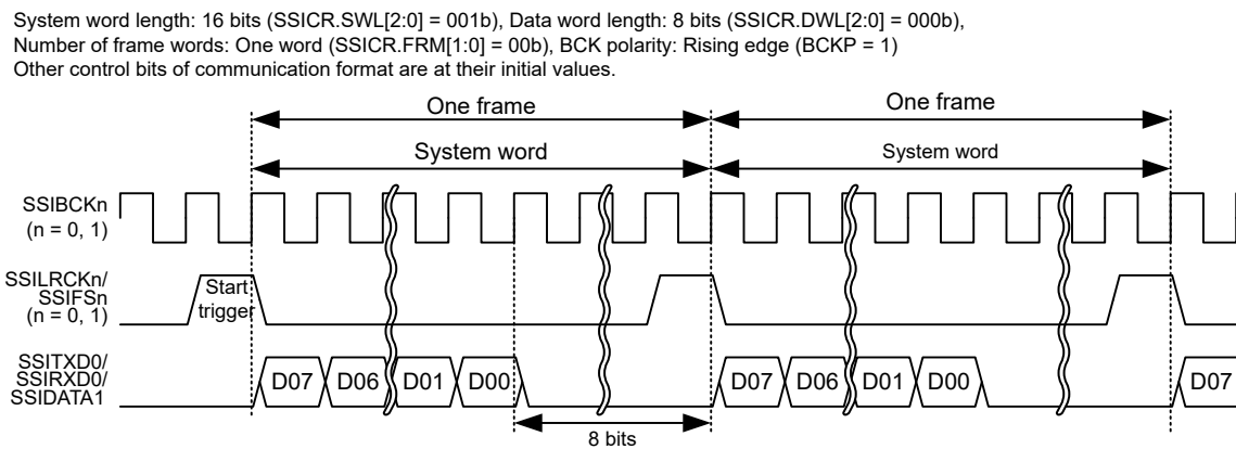
Figure 46.39 Short frame in monaural format (with padding: system word length > data word length)
