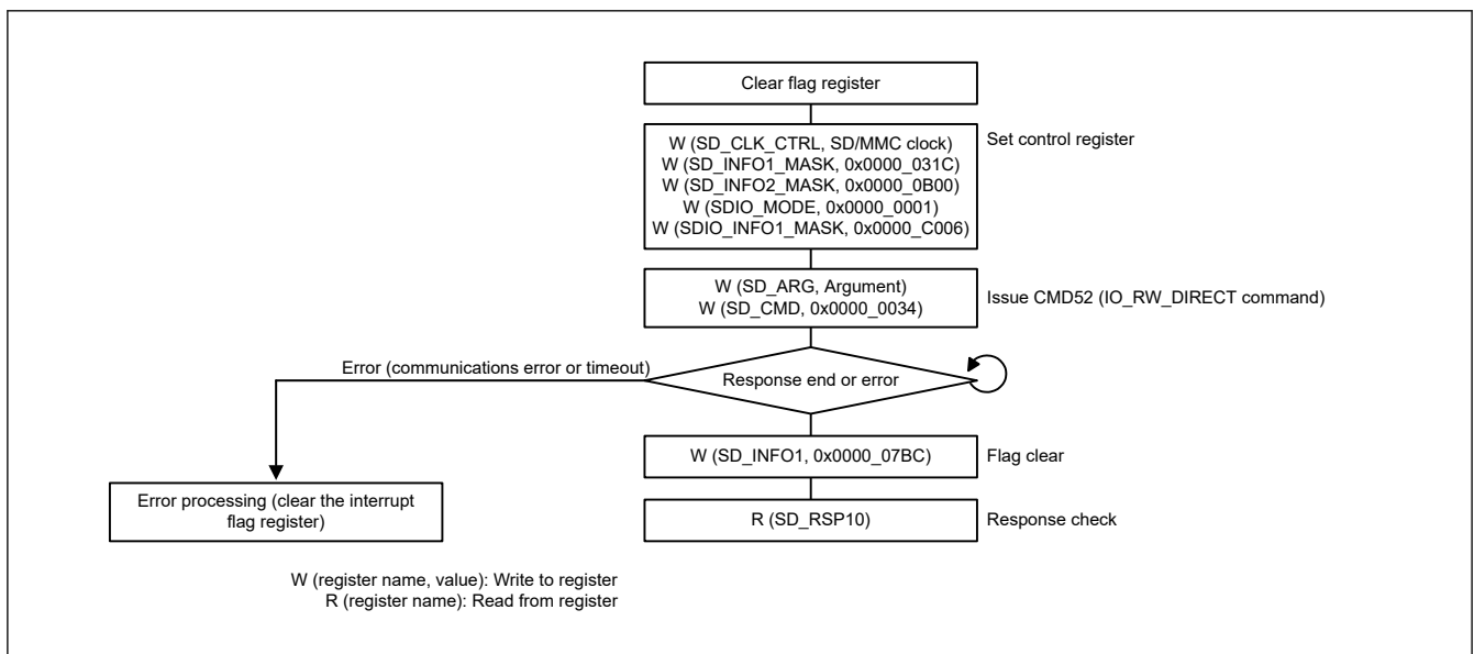
Figure 47.16 Example of IO_RW_DIRECT command (CMD52) operation
