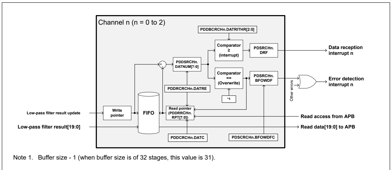
Figure 49.11 Data buffer function
