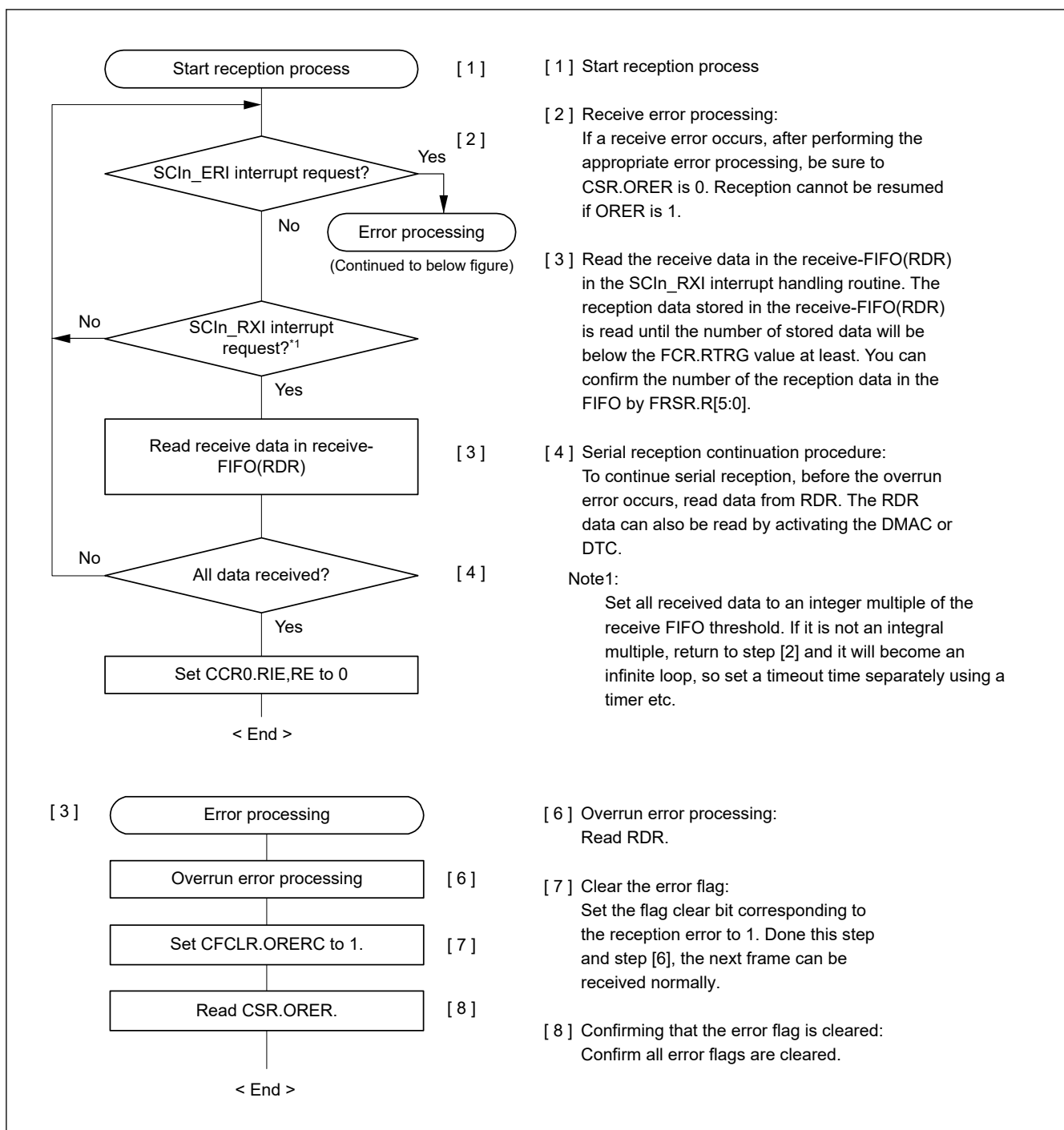
Figure 38.70 Example flow of serial reception in clock synchronous mode with FIFO selected
