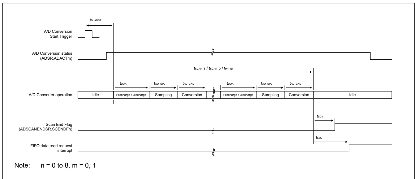
Figure 53.62 Scan end processing time (SAR/Oversampling/Hybrid mode – Single scan mode)
