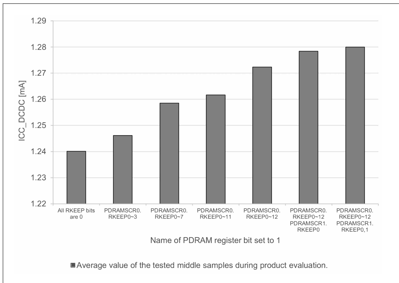
Figure 69.14 Software Standby current per SRAM state (ICC_DCDC, SS2LP_0, SVSCR_5) (reference data)
