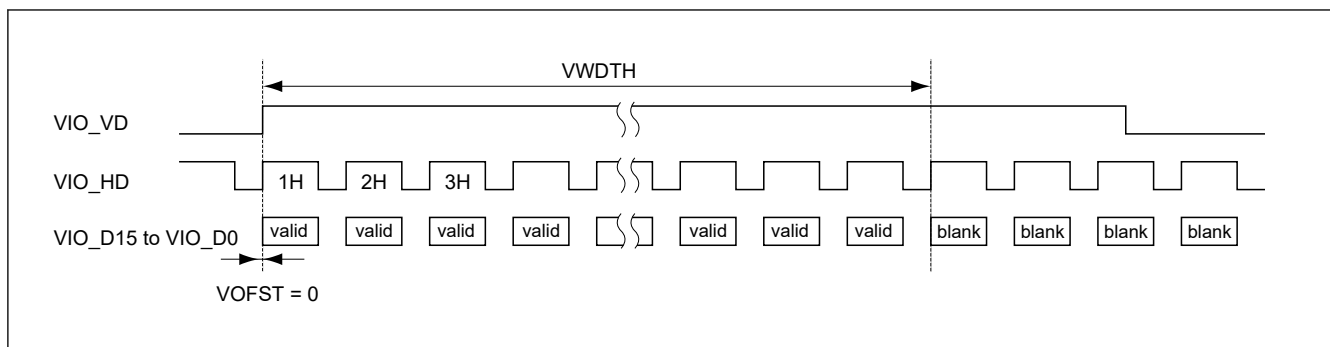
Figure 60.21 Vertical capture timing
