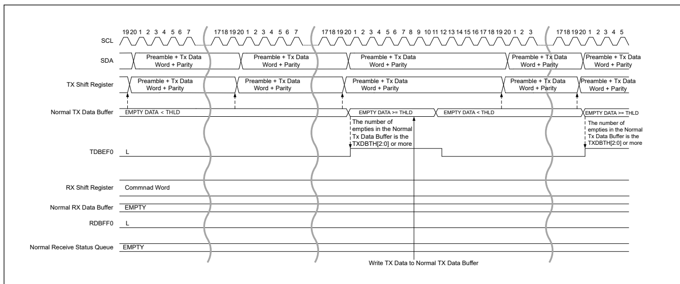
Figure 40.59 HDR data read transfer (HDR-DDR) timing (2/3)
