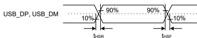
Figure 69.136 USB_DP and USB_DM output timing (high-speed)
