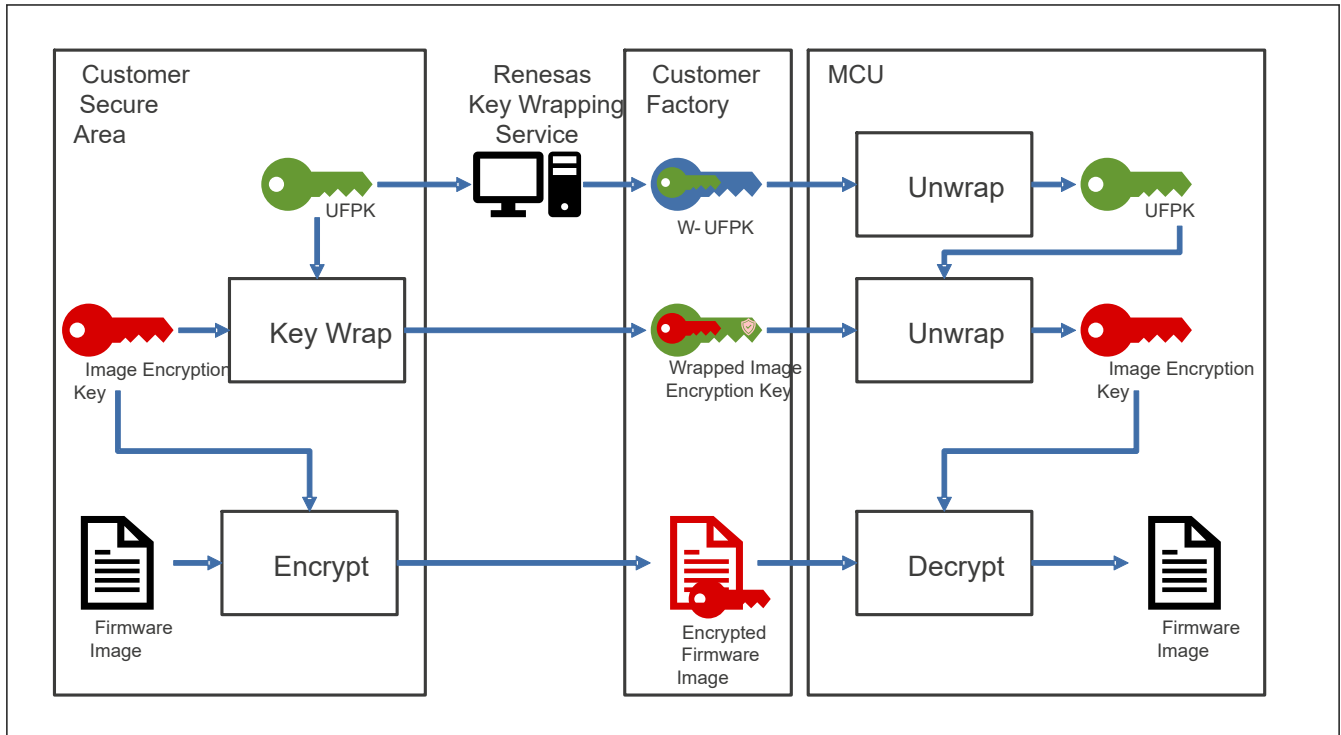
Figure 51.10 Secure factory encrypted image programming
