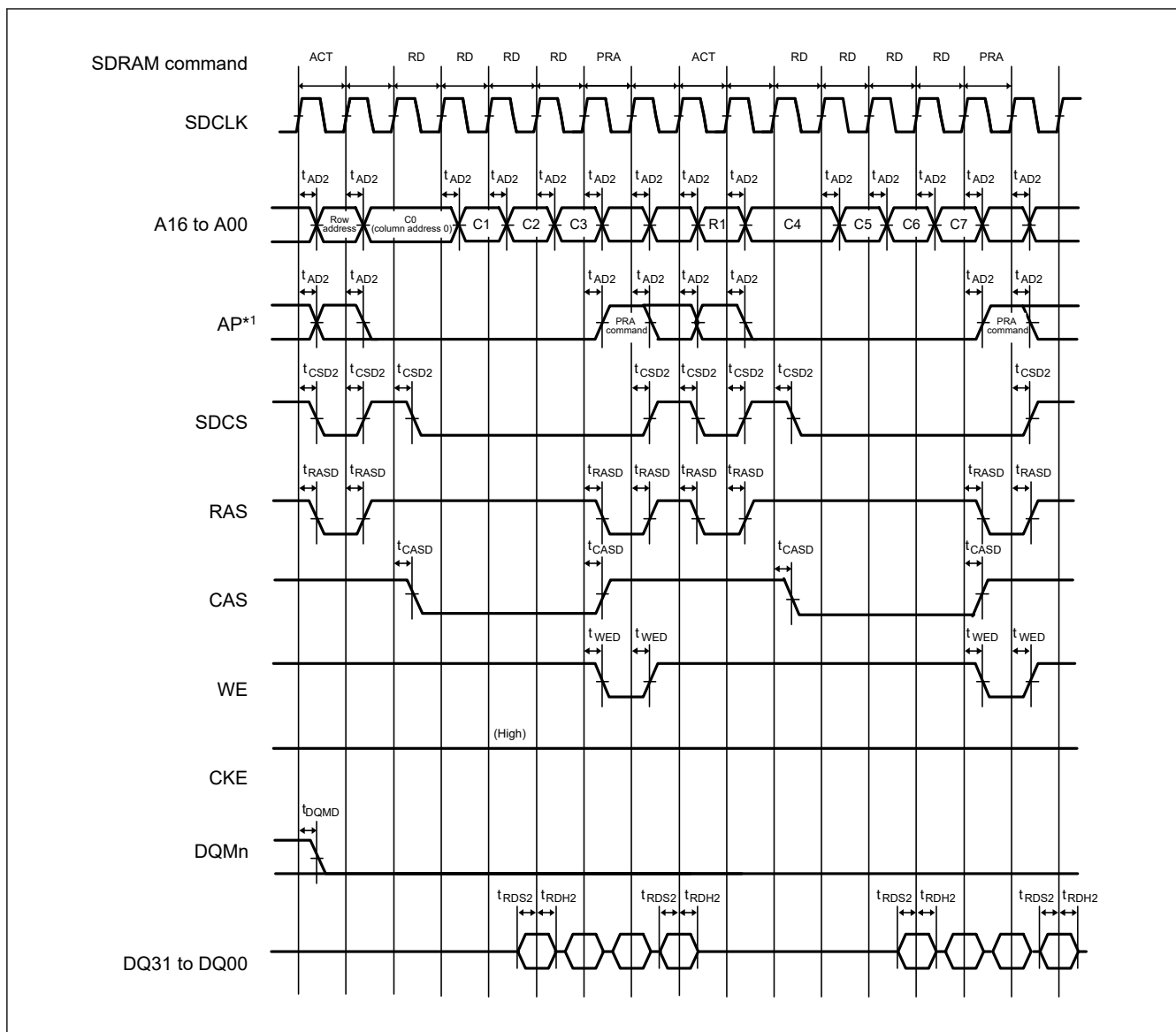
Figure 69.49 SDRAM multiple read line stride timing
