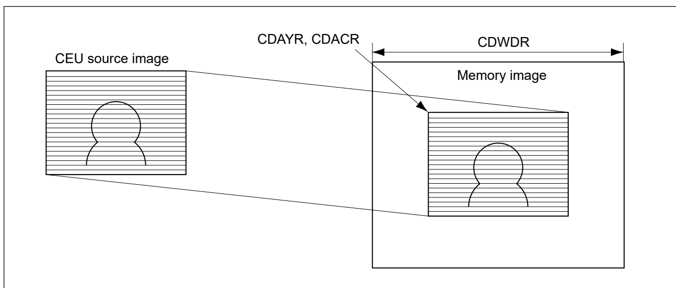
Figure 60.24 Image of storing captured frame image or captured one-field image in memory
