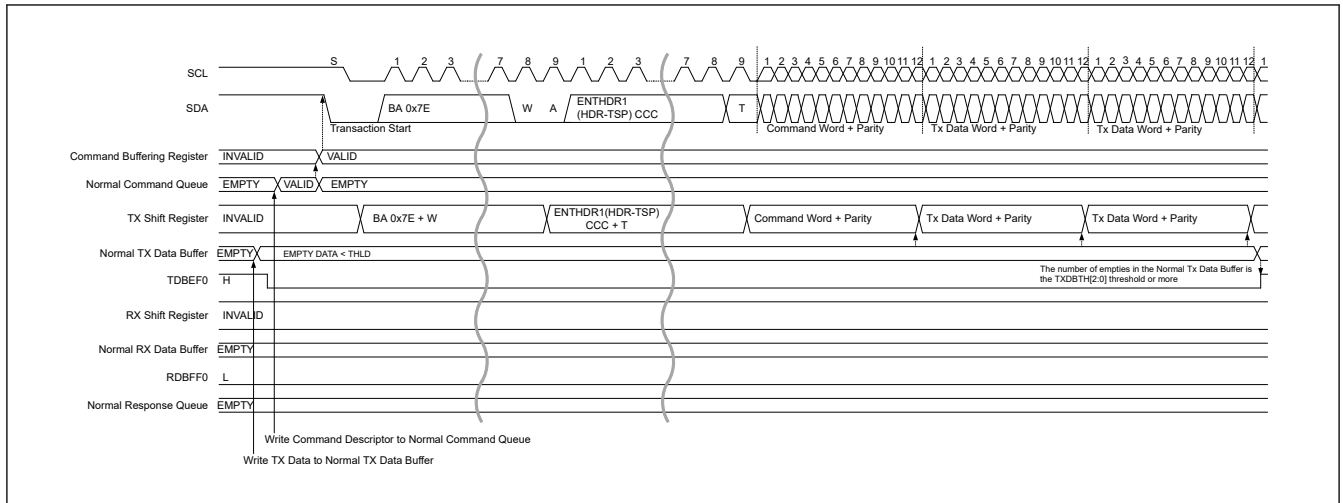
Figure 40.28 HDR data write transfer (HDR-TSP, TSL) timing (1/2)
