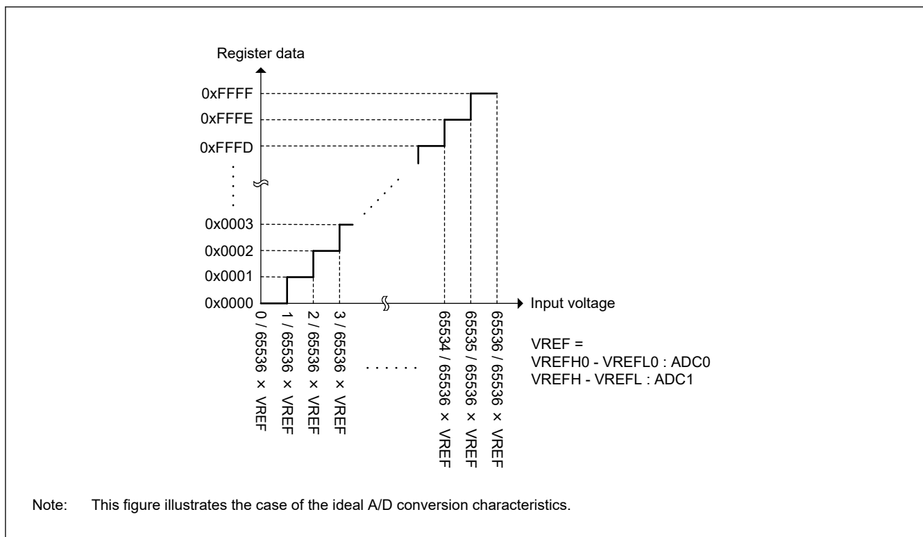
Figure 53.44 Data range of A/D conversion result (16-bit data length, Unsigned data, Single-ended input)
