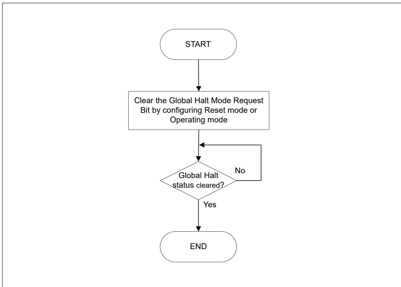
Figure 41.8 Procedure for exiting Global Halt mode
