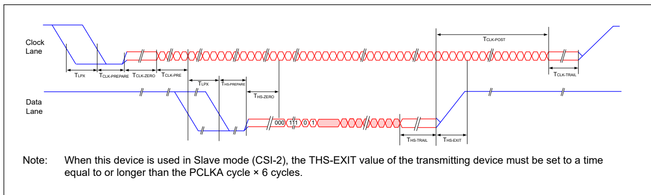
Figure 64.1 High-speed data transmission in normal mode
