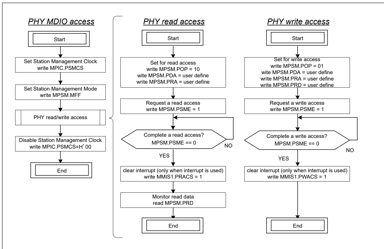
Figure 33.8 PHY MDIO access flow
