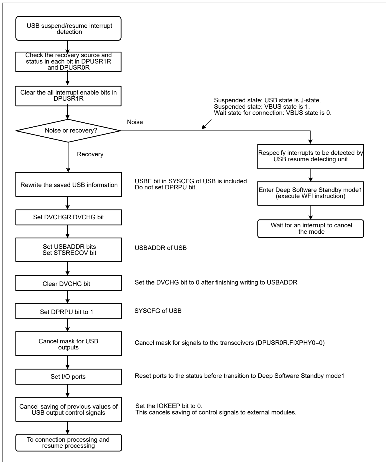
Figure 36.9 USBFS setup flow for canceling Deep Software Standby mode 1 as device controller
