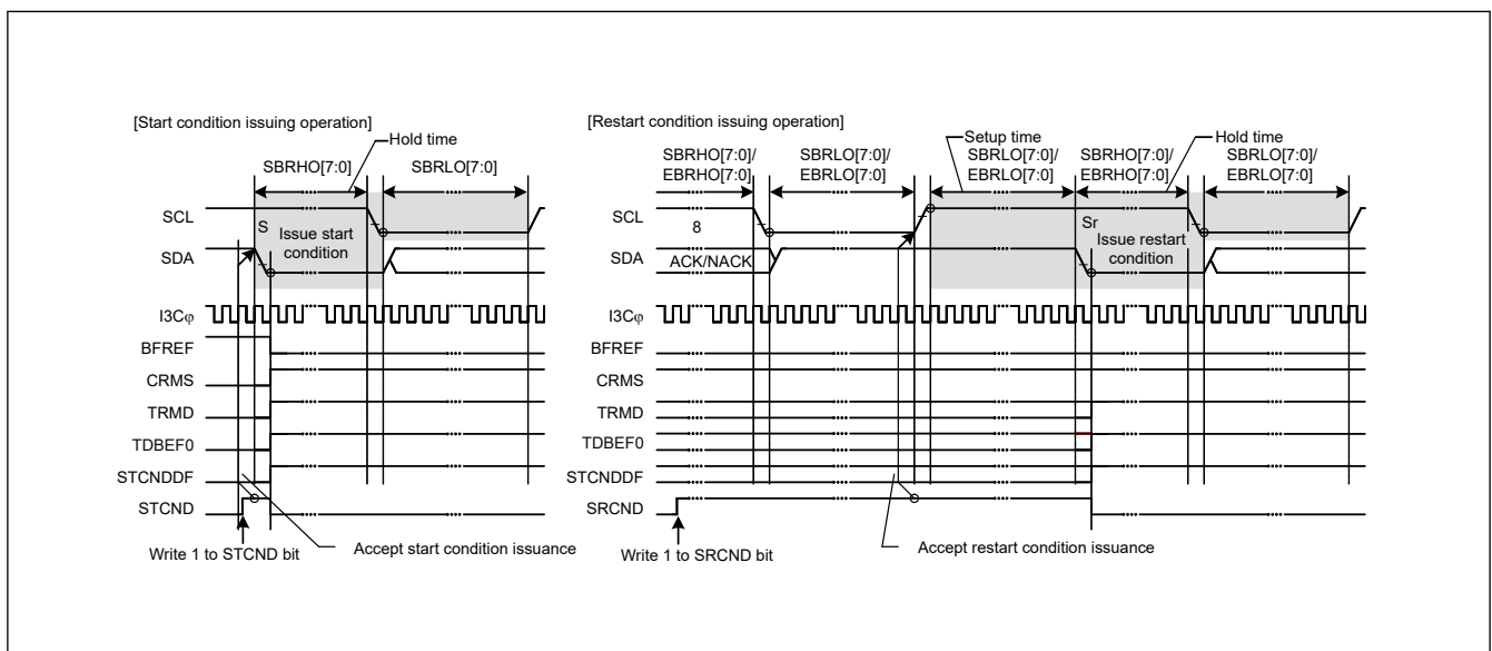
Figure 40.79 START condition / repeated START condition issue timing (STCND and SRCND bits)
