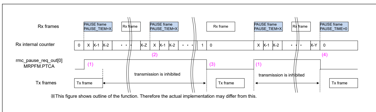
Figure 33.17 Reception of PAUSE frame
