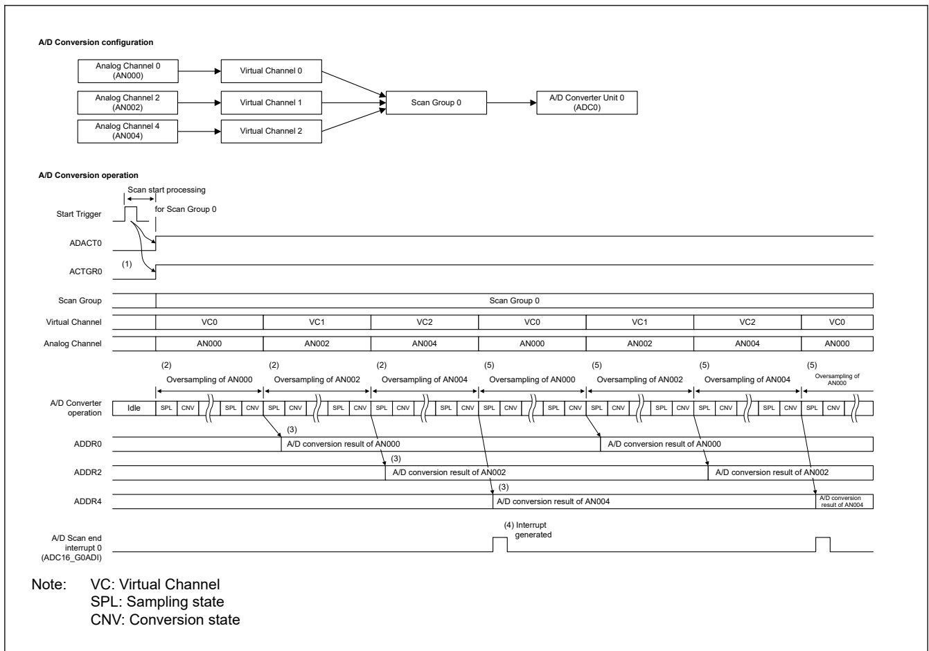
Figure 53.10 Example of scanning operation in Oversampling mode – Continuous scan mode
