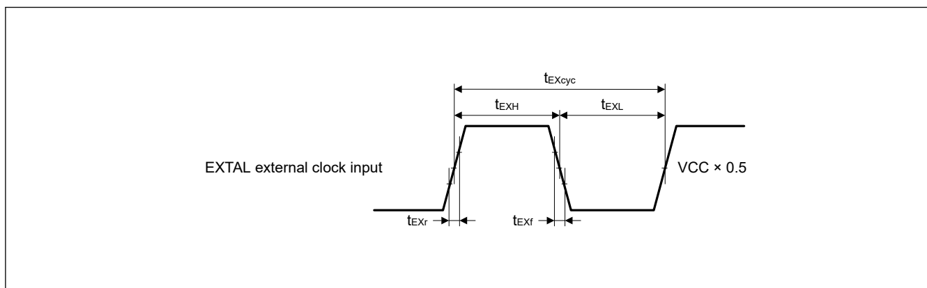
Figure 69.26 EXTAL external clock input timing
