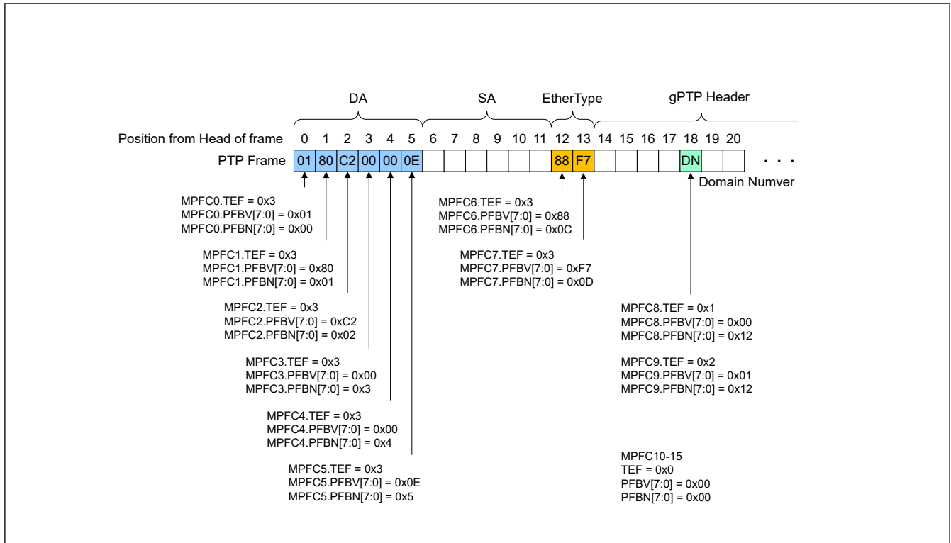
Figure 33.26 Example configuration of PTP message filter
