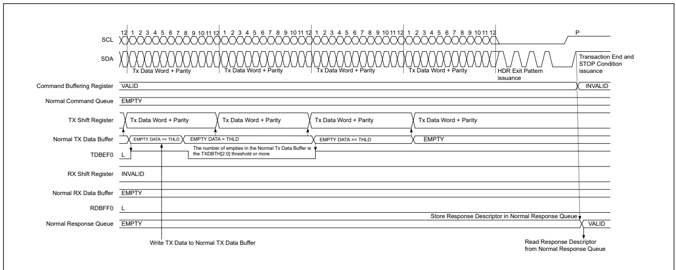
Figure 40.29 HDR data write transfer (HDR-TSP, TSL) timing (2/2)
