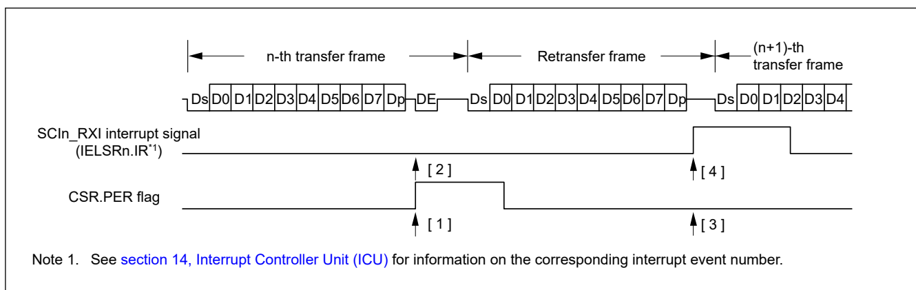
Figure 38.83 Data re-transfer operation in smart card interface reception mode
