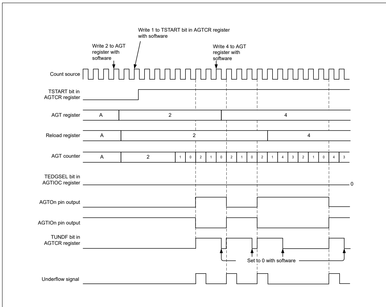
Figure 24.7 Operation example in pulse output mode
