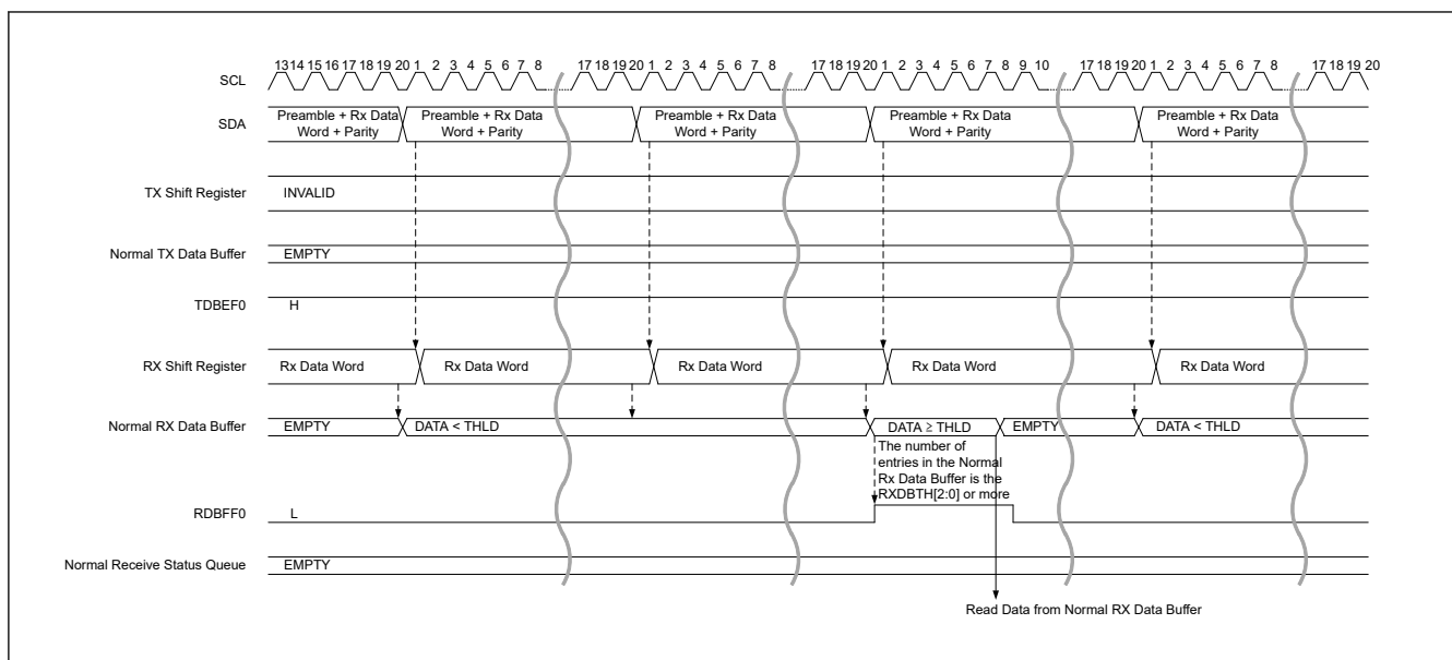
Figure 40.54 HDR data write transfer (HDR-DDR) timing (2/3)
