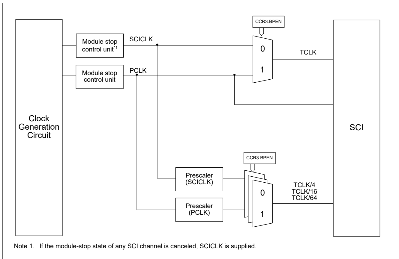
Figure 38.2 Clock source selector block diagram
