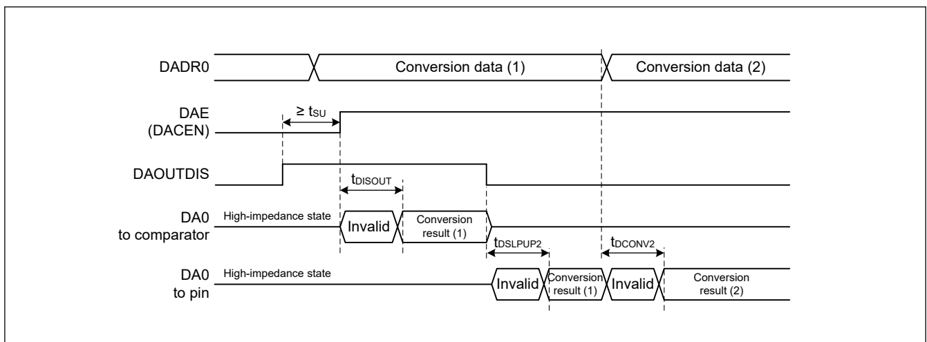
Figure 54.2 Example of DAC12 operation (DAC output mode)
