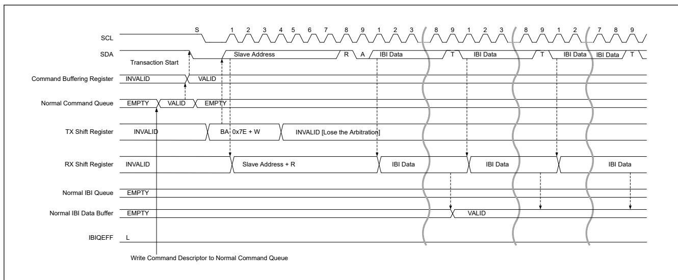
Figure 40.34 I3C master IBI transfer timing (1/2)
