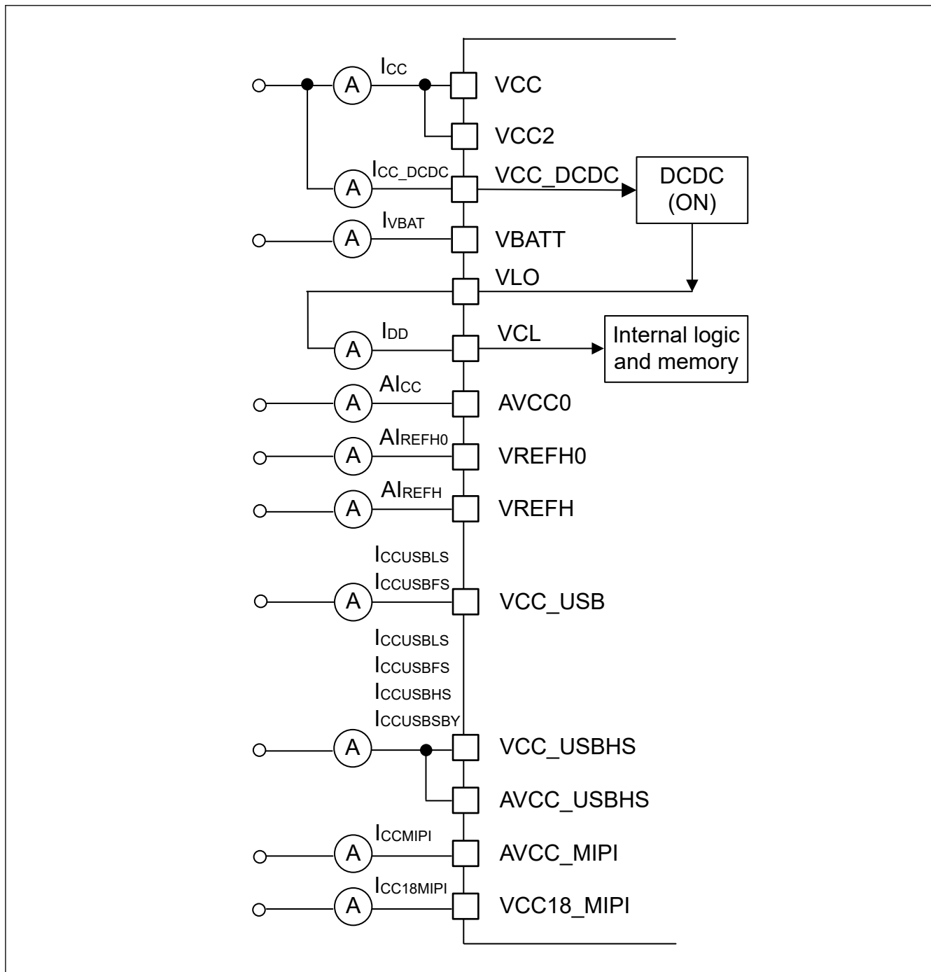
Figure 69.2 Consumption current measurement diagram (DCDC mode)
