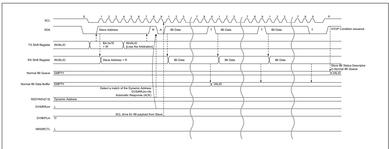
Figure 40.100 Slave interrupt request : ACK and DVIBIPL = 1
