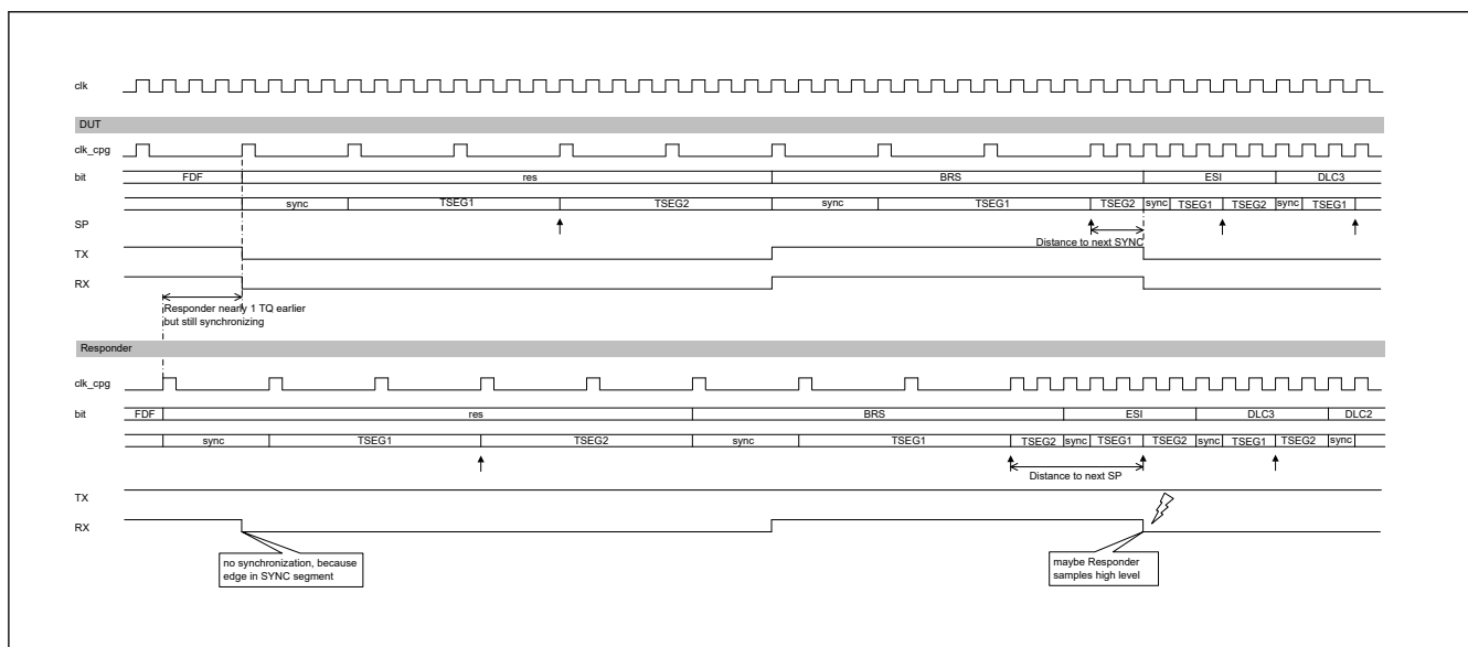
Figure 41.21 Loss of synchronization between two CAN nodes
