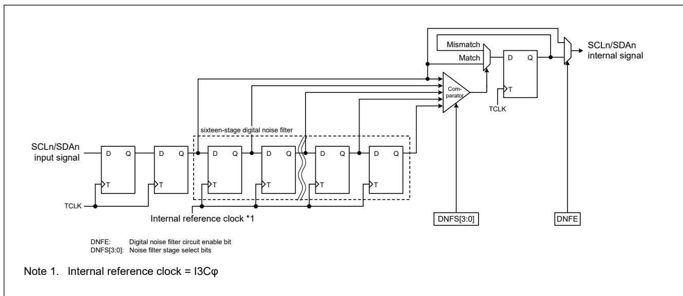
Figure 40.139 Block diagram of digital noise filter circuit
