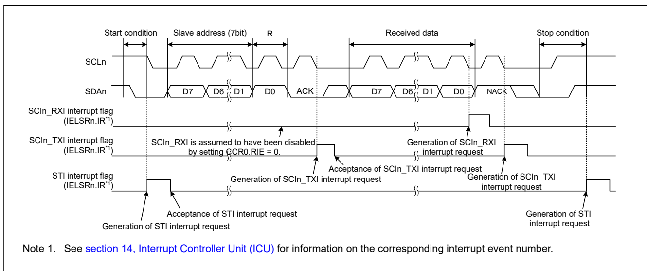
Figure 38.94 Example operations for master reception in simple IIC mode with 7-bit slave addresses, transmission interrupts, and reception interrupts (ICR.IICINTM = 1)
