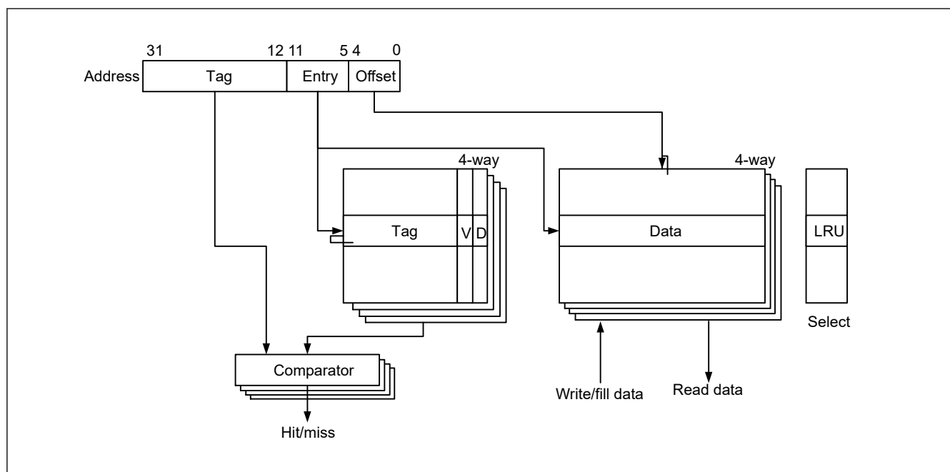
Figure 2.7 Detailed cache structure
