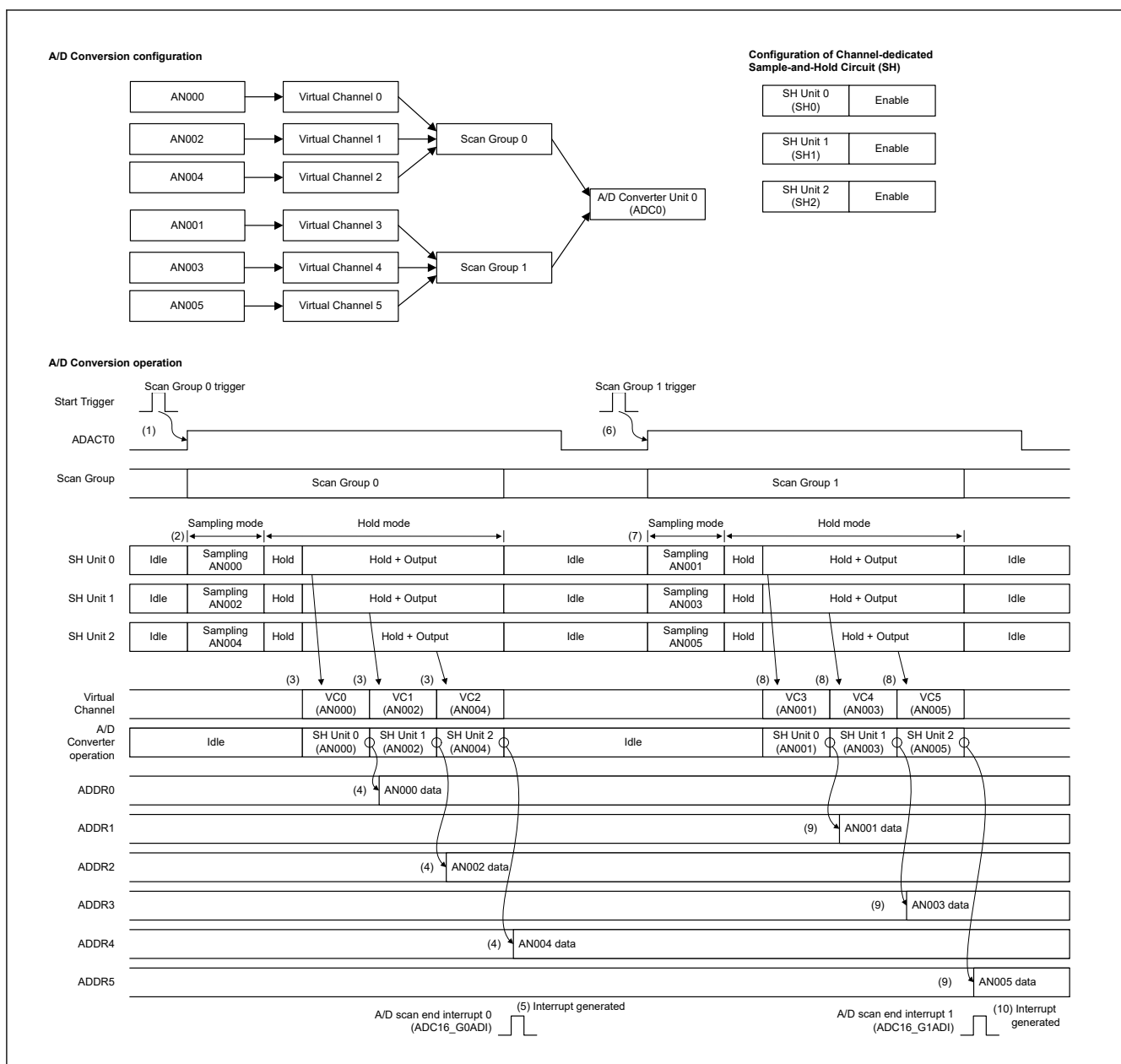
Figure 53.19 Example operation when channel-dedicated sample-and-hold circuit is shared with two analog channels in SAR mode
