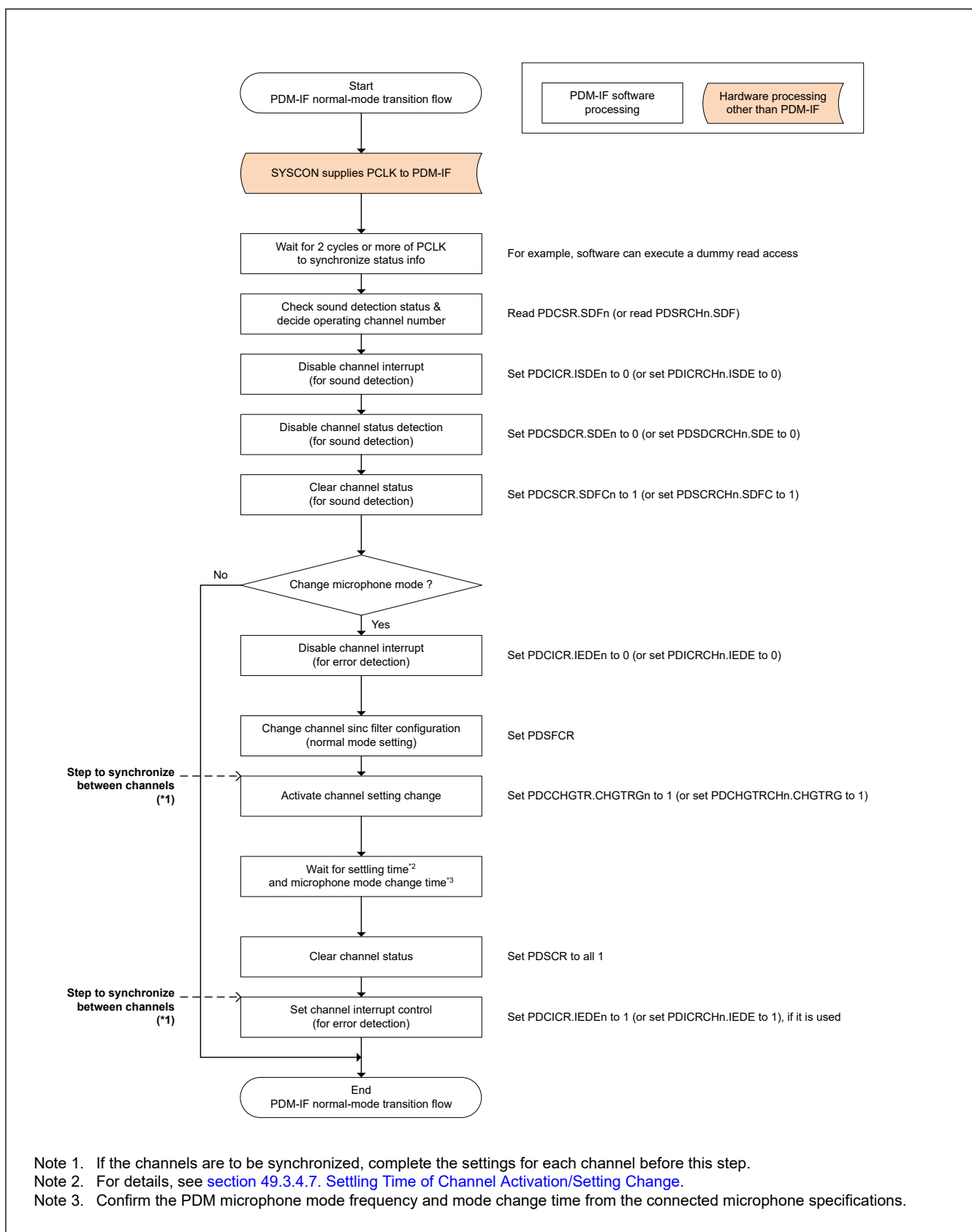
Figure 49.21 PDM-IF normal-mode transition flow
