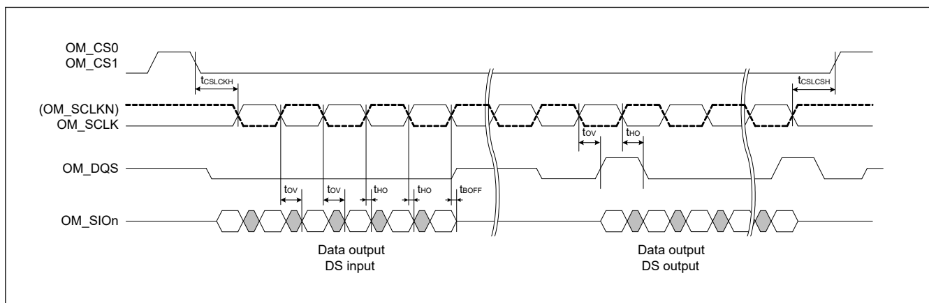
Figure 69.86 DDR transmit/receive timing (HyperRAM write)
