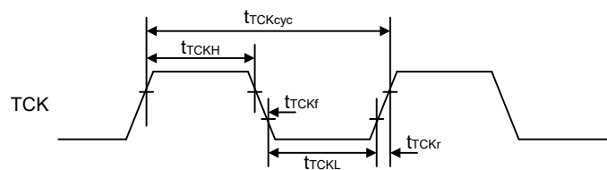
Figure 69.152 Boundary scan TCK timing
