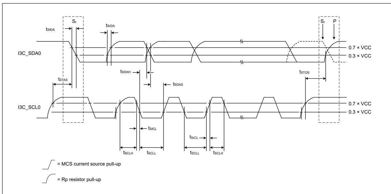
Figure 69.90 I 2 C bus interface input/output timing (Hs-mode)
