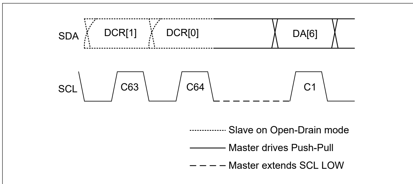
Figure 40.99 Master clock stalling in dynamic address first bit
