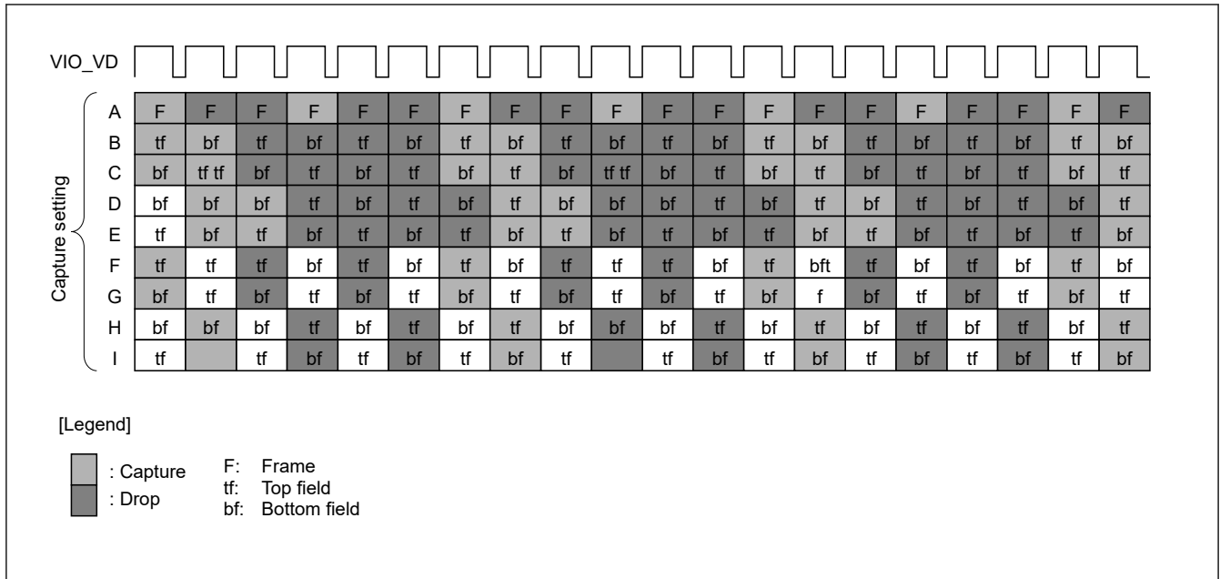
Figure 60.10 Image of frame drop timing for capture settings (FDRP[7:0] = 0x2)
