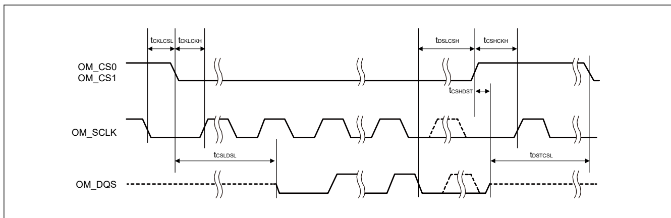
Figure 69.87 DS to CS signal timing
