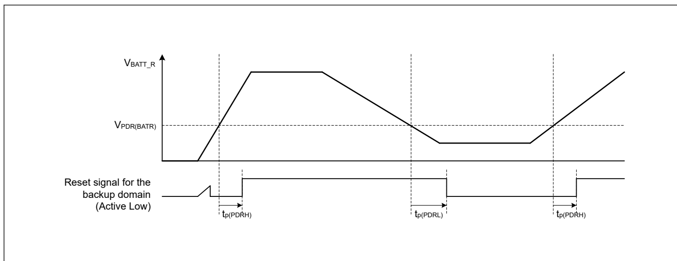
Figure 69.151 Backup domain reset characteristics
