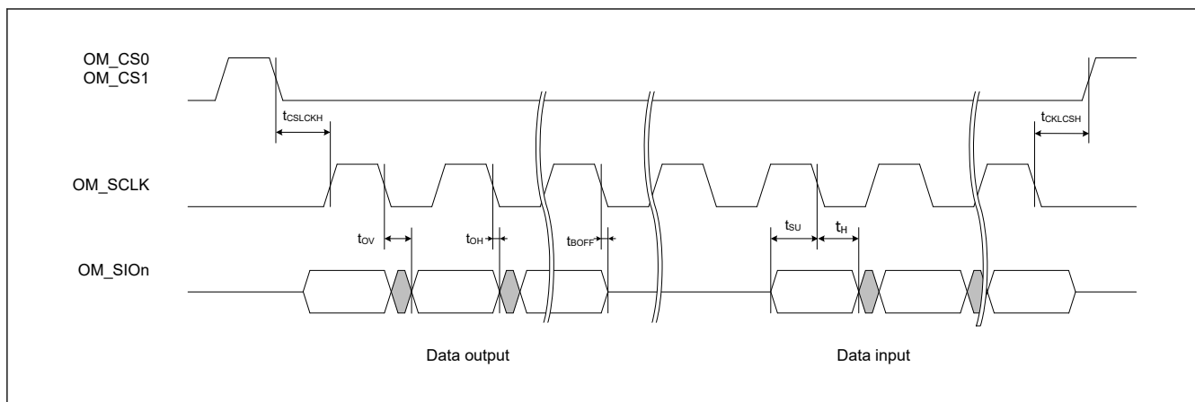
Figure 69.84 SDR transmit/receive timing (1S-1S-1S, 1S-2S-2S, 2S-2S-2S, 1S-4S-4S, 4S-4S-4S)
