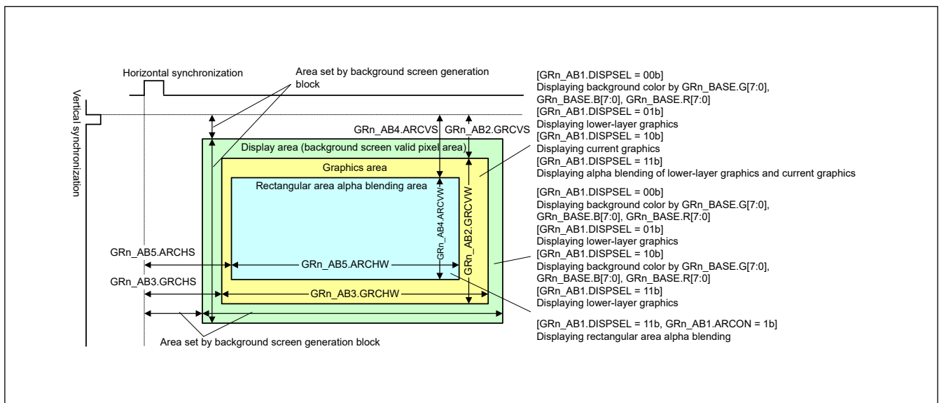
Figure 63.8 Graphics display selection
