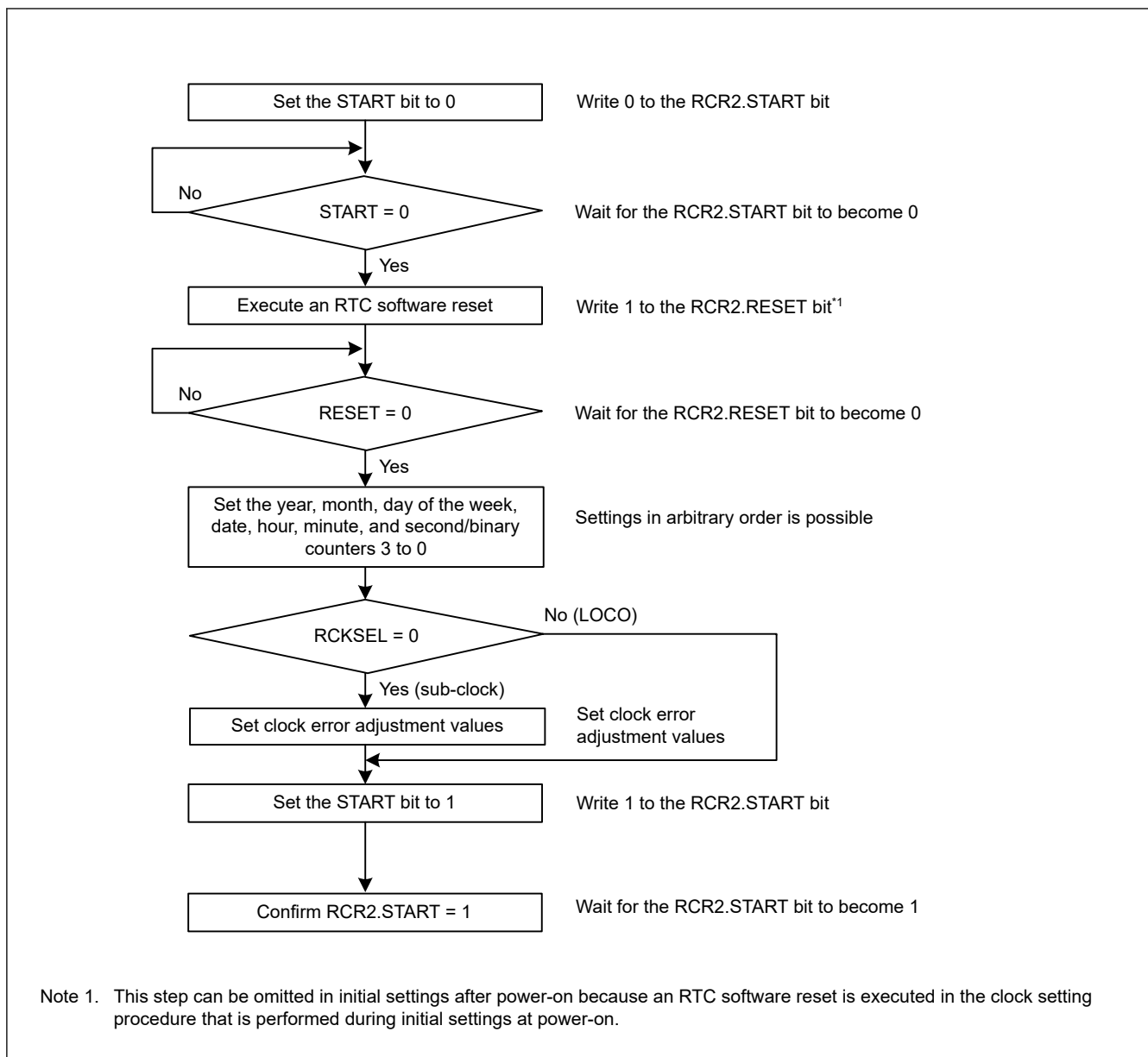
Figure 26.4 Setting the time
