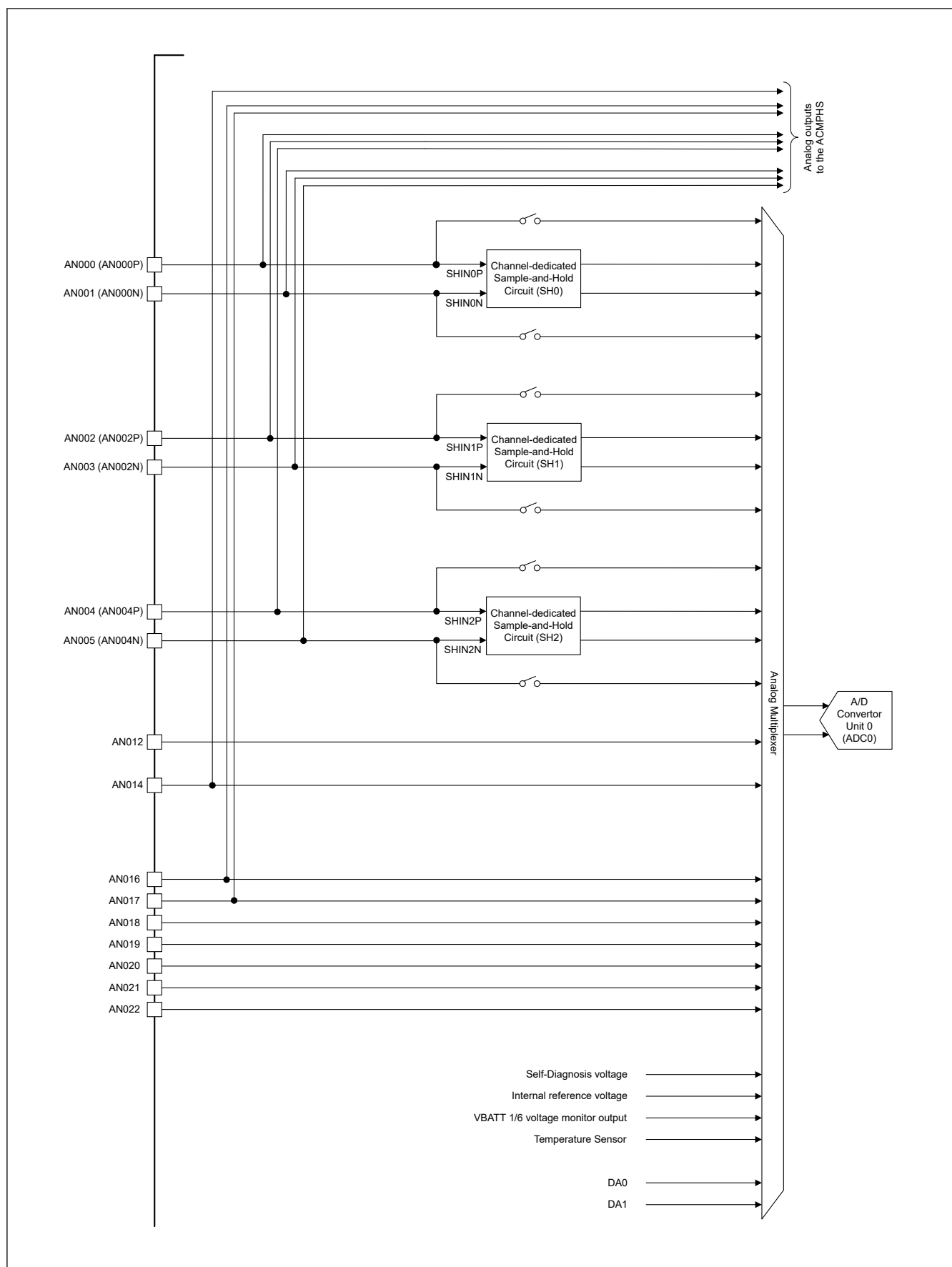
Figure 53.2 Analog channel structure for A/D converter unit 0
