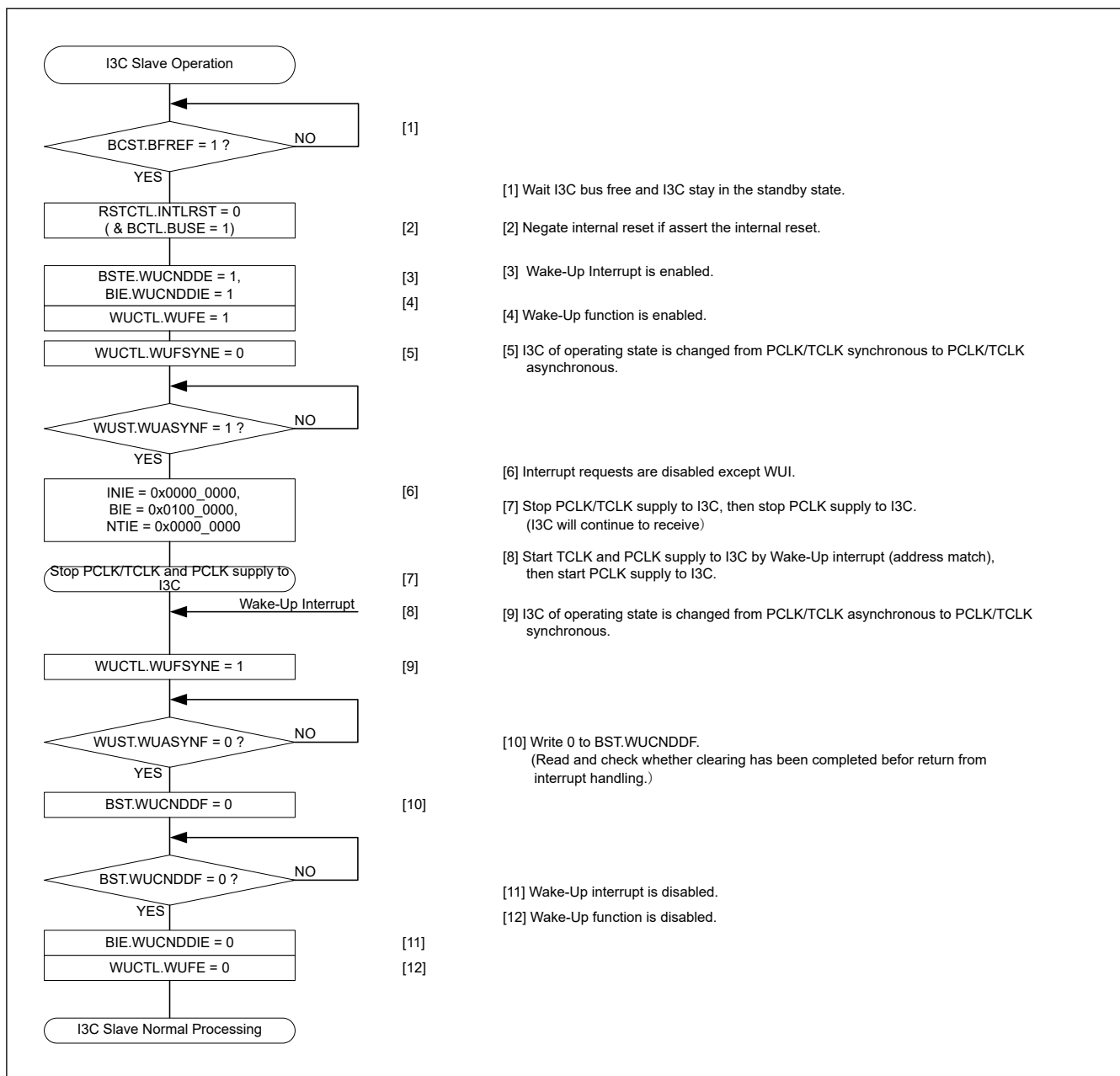
Figure 40.157 Use case of I3C slave wake-up (wake-up recovery by a wake-up interrupt triggered by the match of the slave address)
