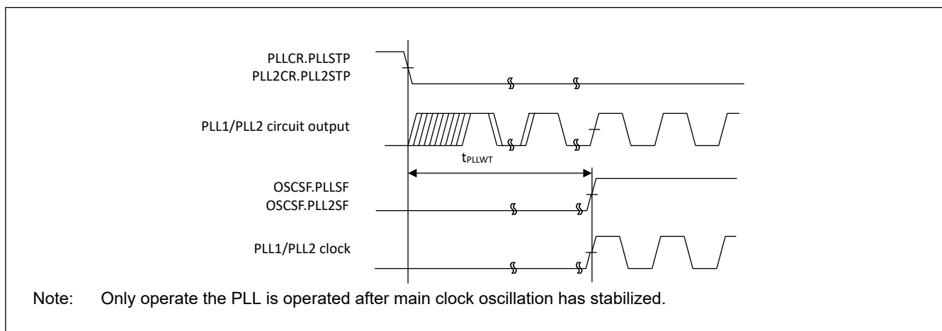
Figure 69.29 PLL1/PLL2 clock oscillation start timing
