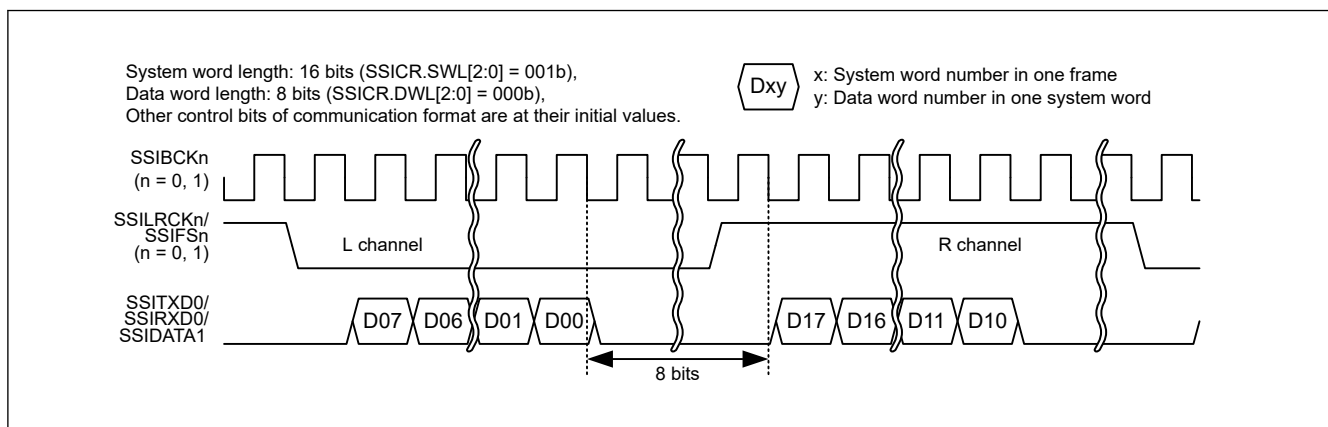
Figure 46.36 Example of padding bit transfer (I 2 S format: system word length > data word length)
