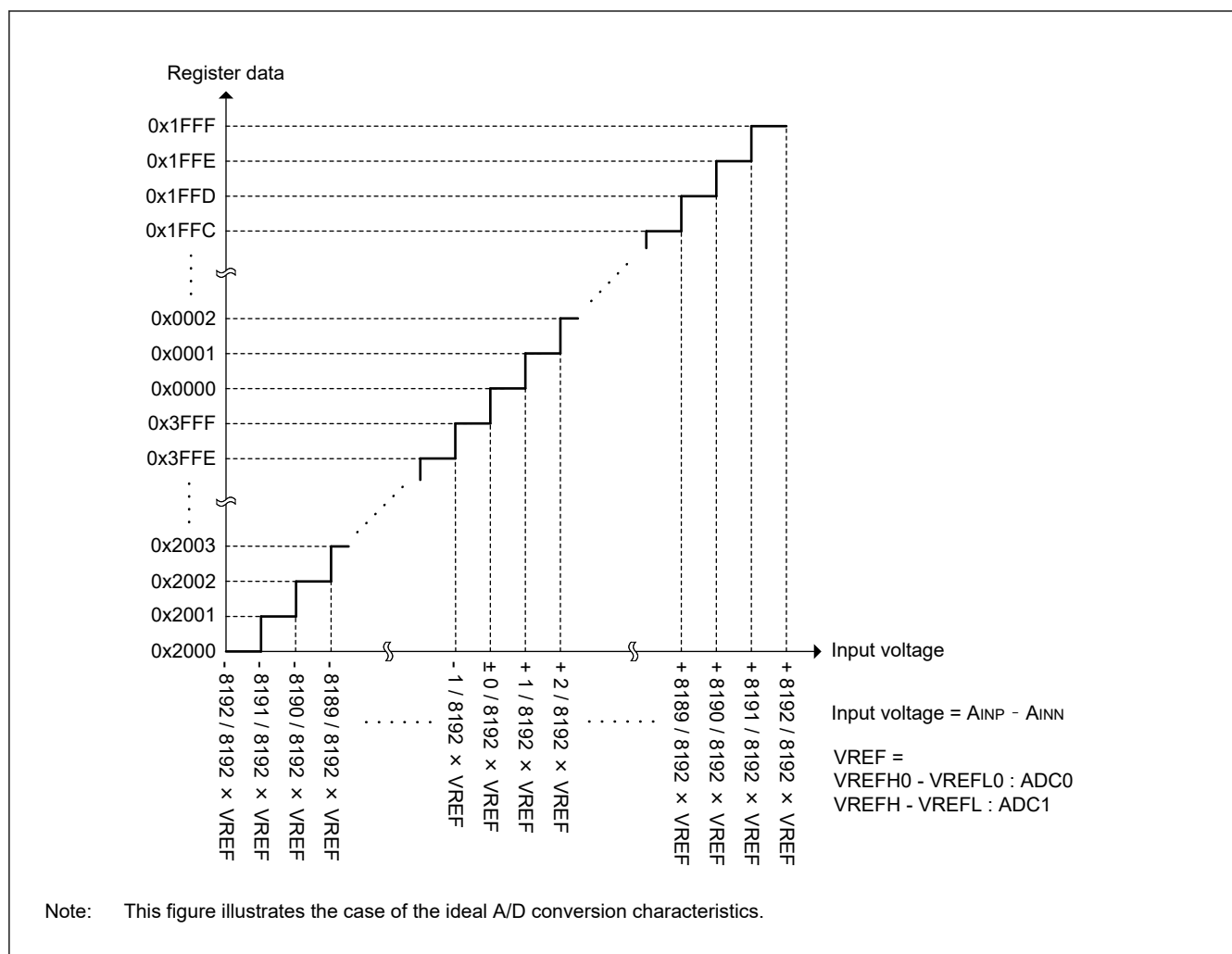
Figure 53.45 Data range of A/D conversion result (14-bit data length, Signed data, Differential input)
