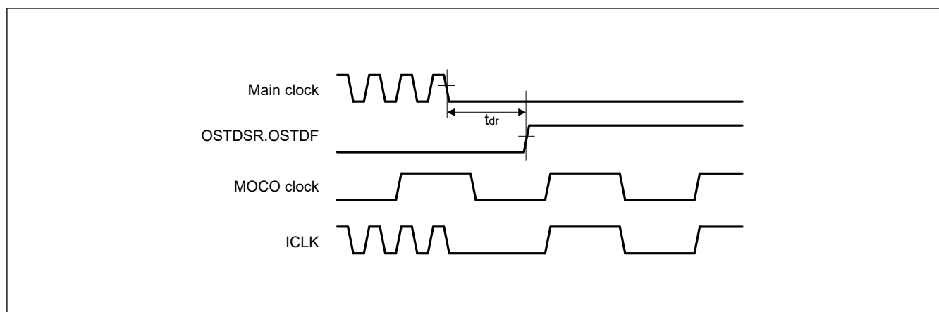
Figure 69.139 Oscillation stop detection timing
