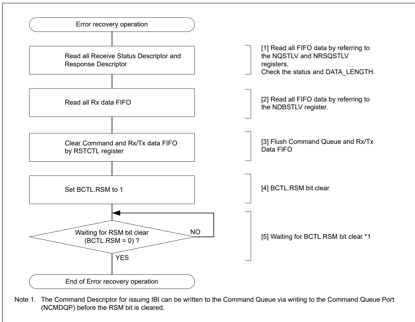
Figure 40.123 Example of error recovery operation flowchart for I3C slave
