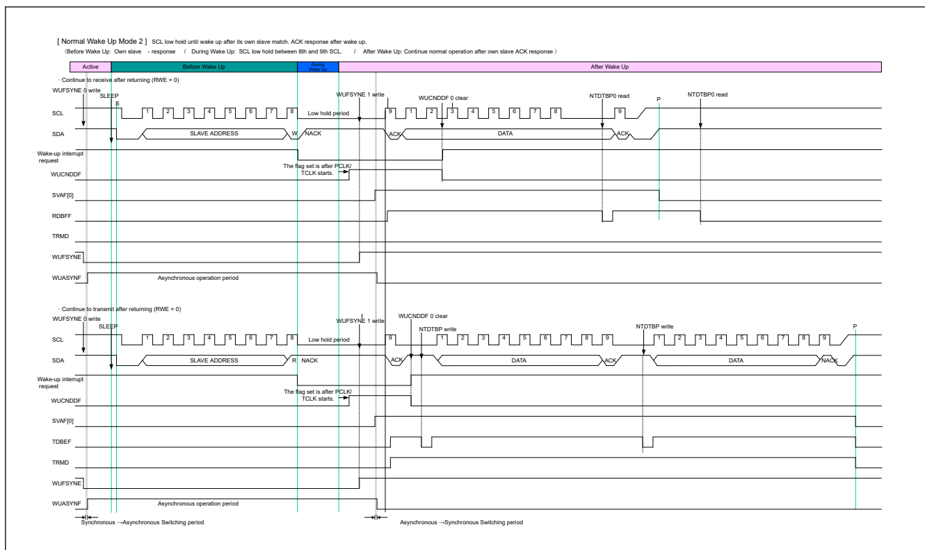
Figure 40.130 Timing of normal wake up mode 2
