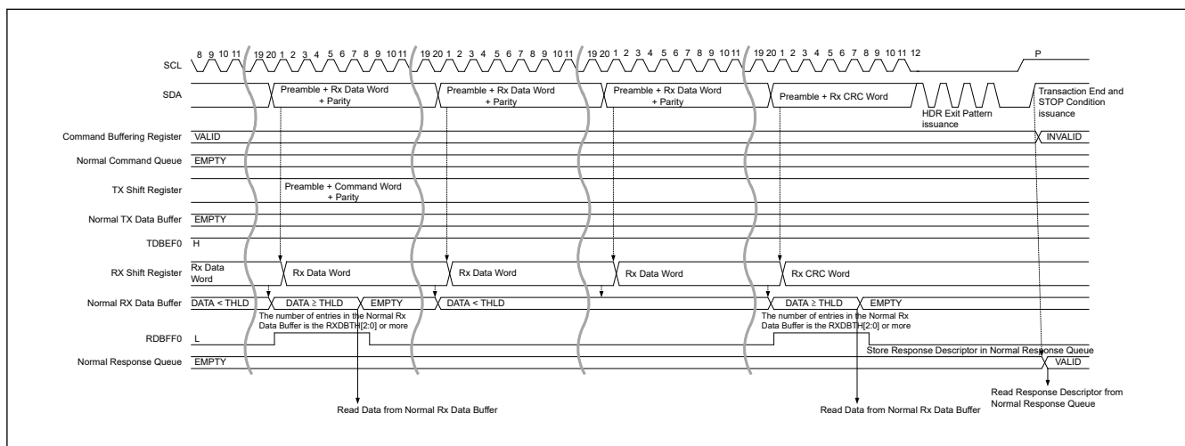
Figure 40.31 HDR data read transfer (HDR-DDR) timing (2/2)
