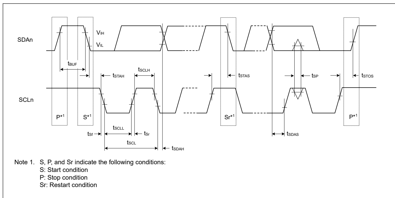
Figure 69.88 I 2 C bus interface input/output timing
