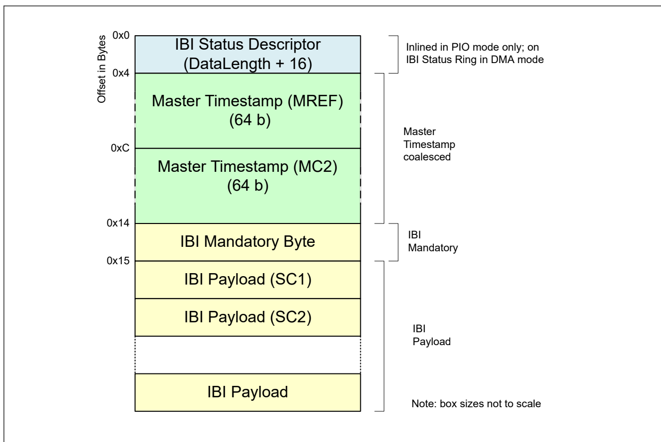
Figure 40.110 Master timestamp counters for IBI event
