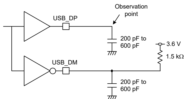
Figure 69.131 Test circuit in low-speed mode
