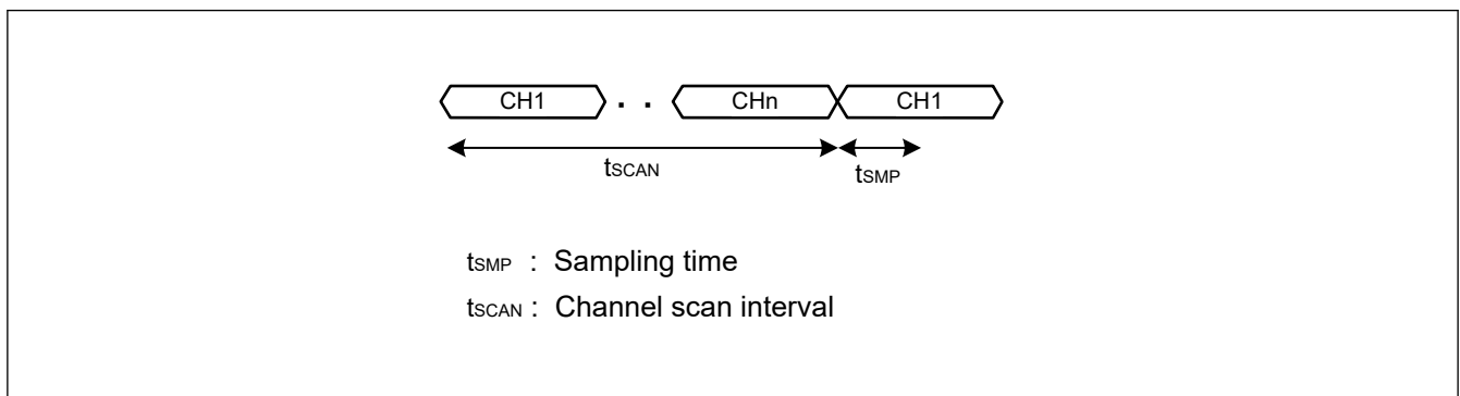
Figure 53.68 Definition of channel scan interval
