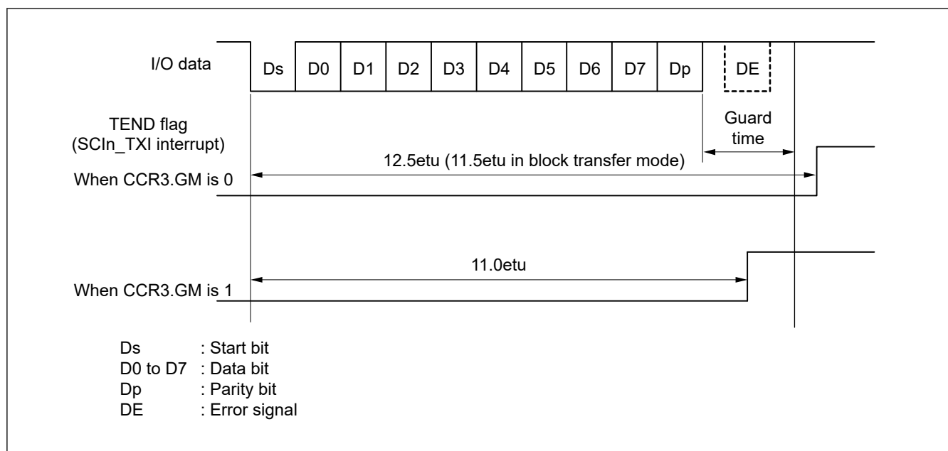
Figure 38.81 CSR.TEND flag generation timing during transmission
