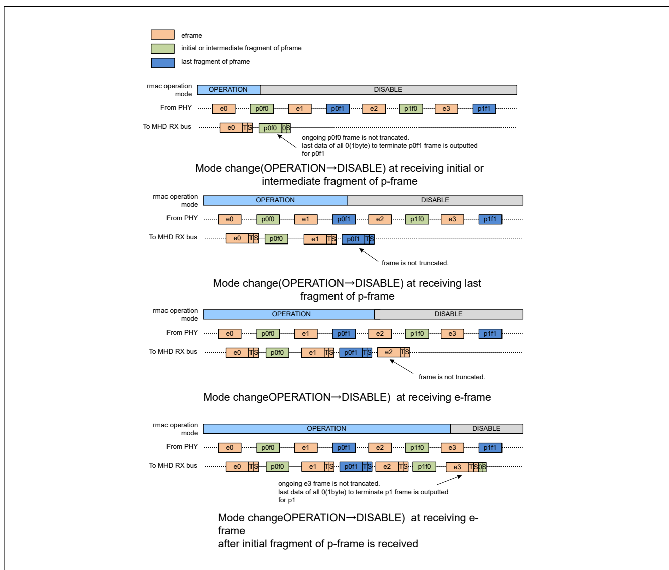
Figure 33.4 Mode change (OPERATION→DISABLE) on Rx
