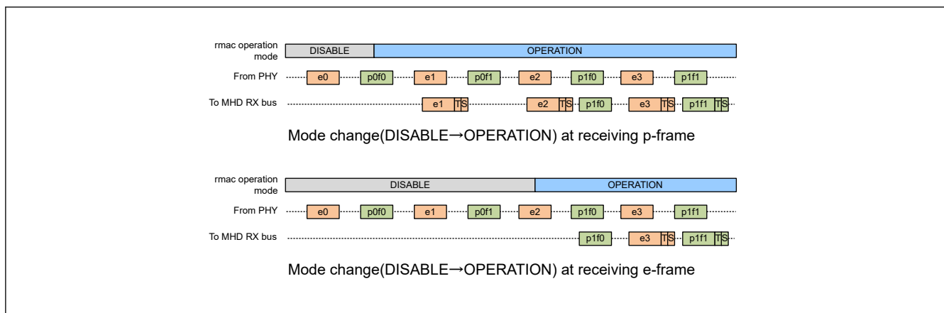
Figure 33.3 Mode change (DISABLE→OPERATION) on Rx
