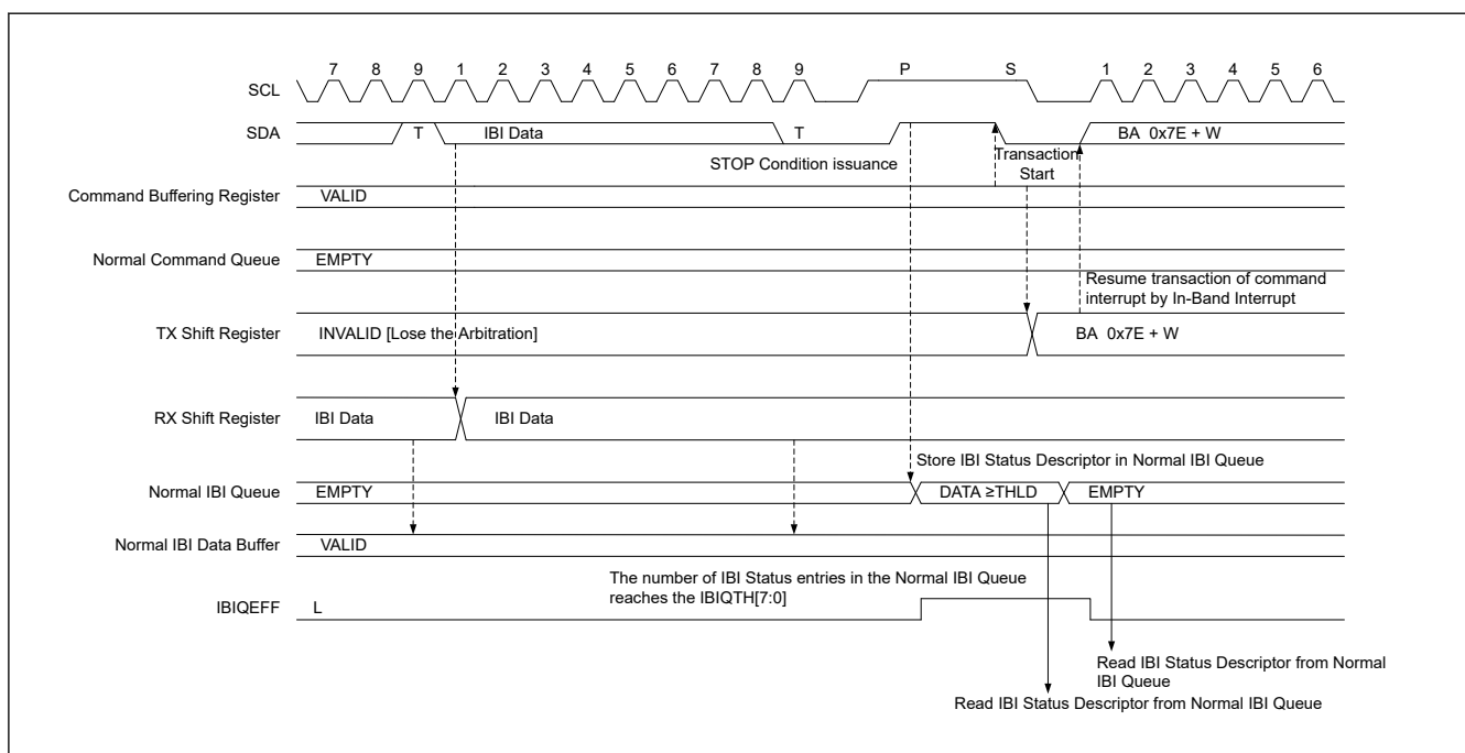
Figure 40.35 I3C master IBI transfer timing (2/2)
