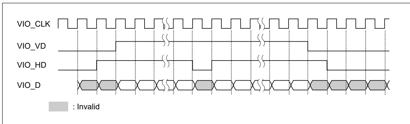
Figure 60.13 Data enable fetch timing (HD asserted (high) when VD is not high)
