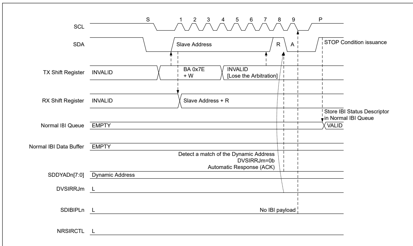
Figure 40.101 Slave interrupt request : ACK and DVIBIPL = 0
