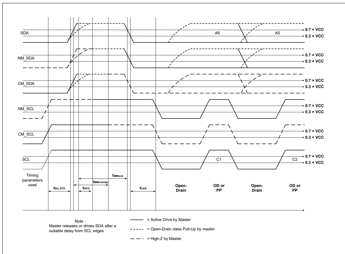
Figure 69.100 Master to Master Bus Handoff
