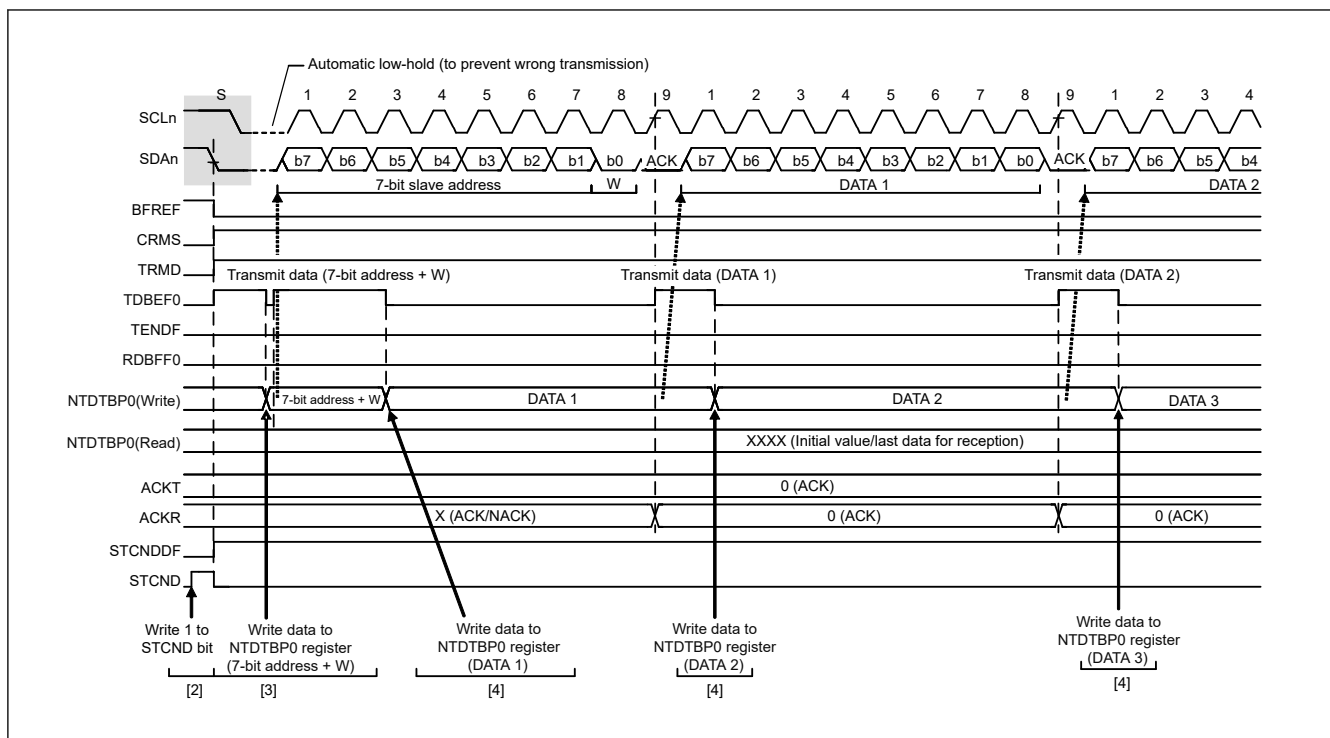
Figure 40.6 Master transmit operation timing (1) (7-bit address format)
