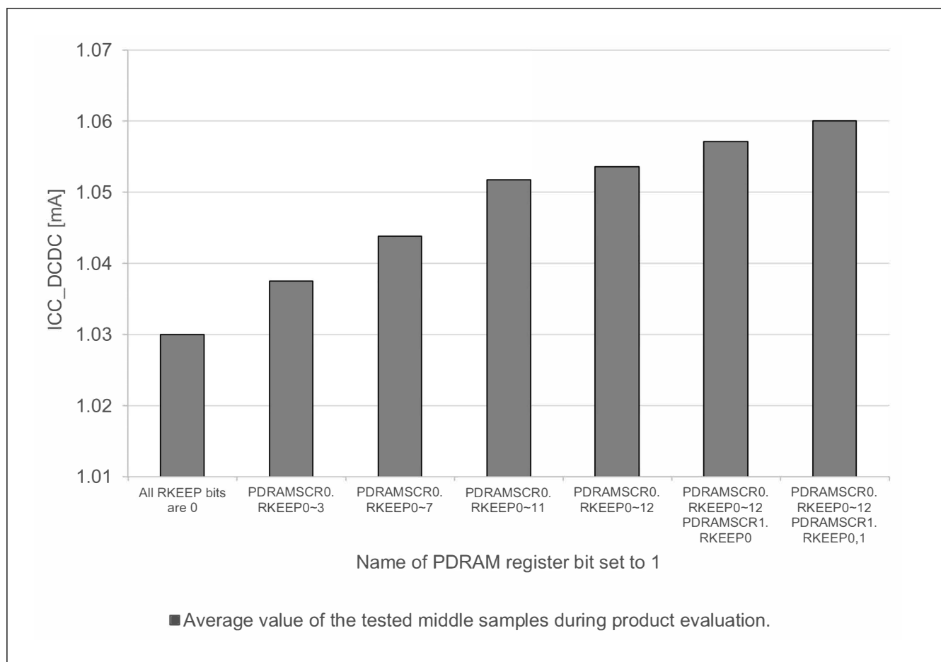
Figure 69.18 Software Standby current per SRAM state (ICC_DCDC, SS2LP_1, SVSCR_5) (reference data)
