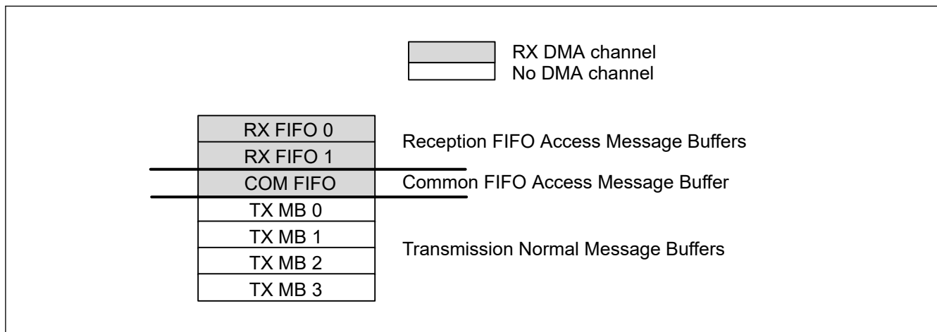
Figure 41.32 Message buffer connectable to a DMA channel
