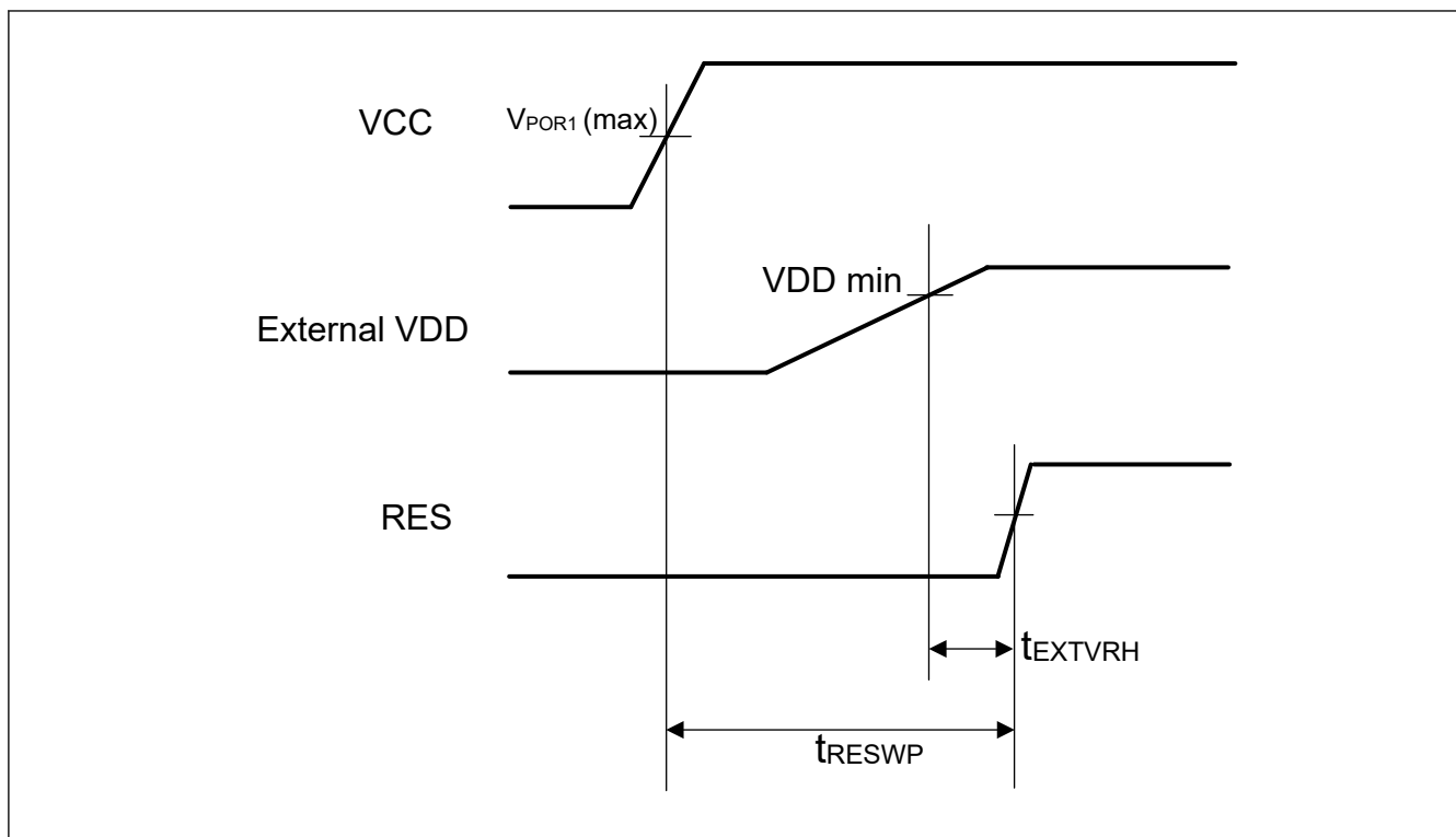
Figure 69.145 Power-up sequence of external VDD mode with using RES pin
