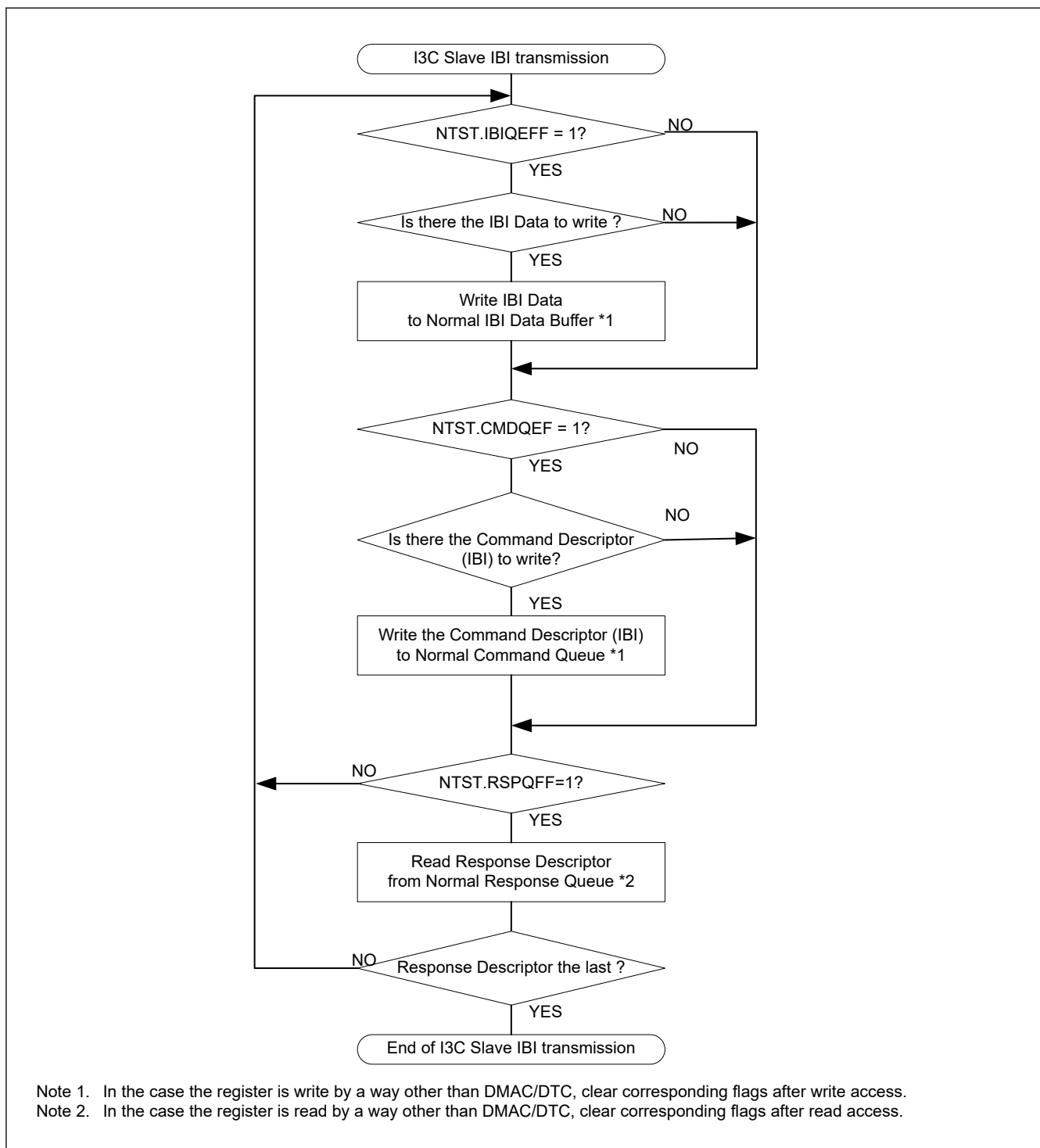
Figure 40.156 Example of I3C slave IBI transmission flowchart
