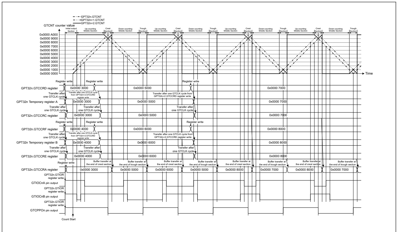
Figure 22.51 Example of Complementary PWM Mode 3 Operation (Double buffer operation, GTIOcNA pin = High / GTIOcNB pin = High as initial output, GTIOcNA pin = Low / GTIOcNB pin = High at GTCCRA register compare match during up-counting, GTIOcNA pin = High / GTIOcNB pin = Low at GTCCRA register compare match during down-counting, the dead time value is 0x0000 1000 and updating GTCRD register in middle section) (n = 4, 7)
