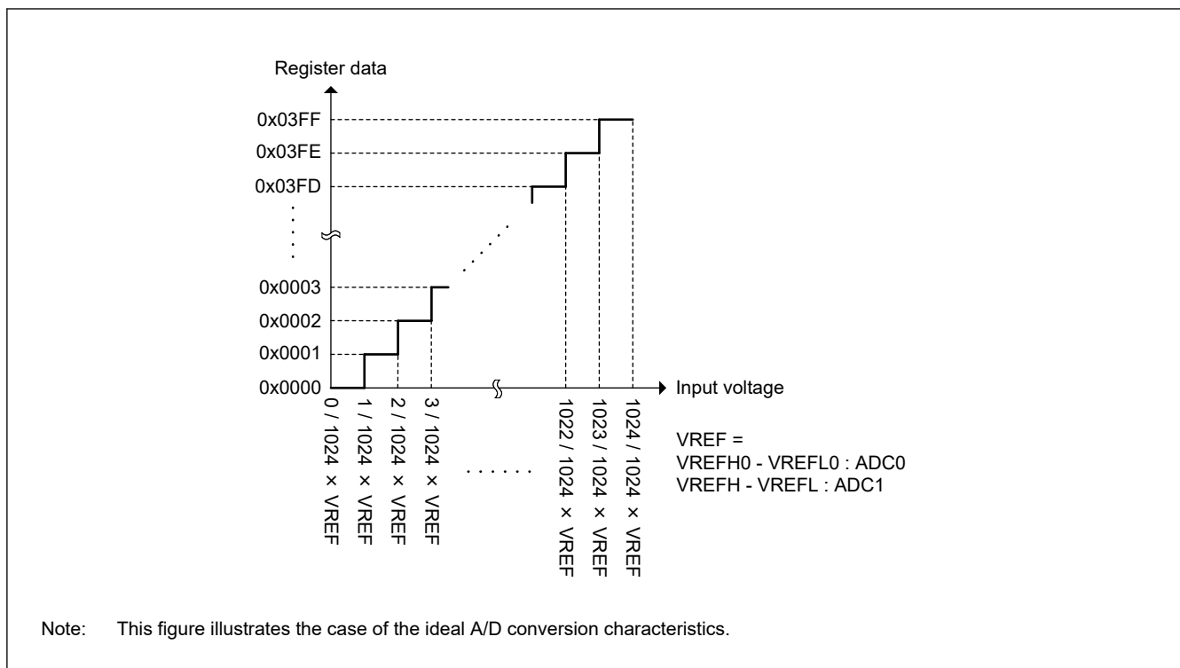
Figure 53.50 Data range of A/D conversion result (10-bit data length, Unsigned data, Single-ended input)
