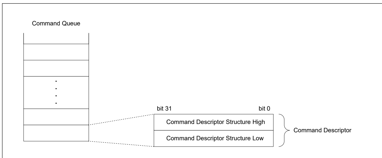
Figure 40.2 Command descriptor data structure
