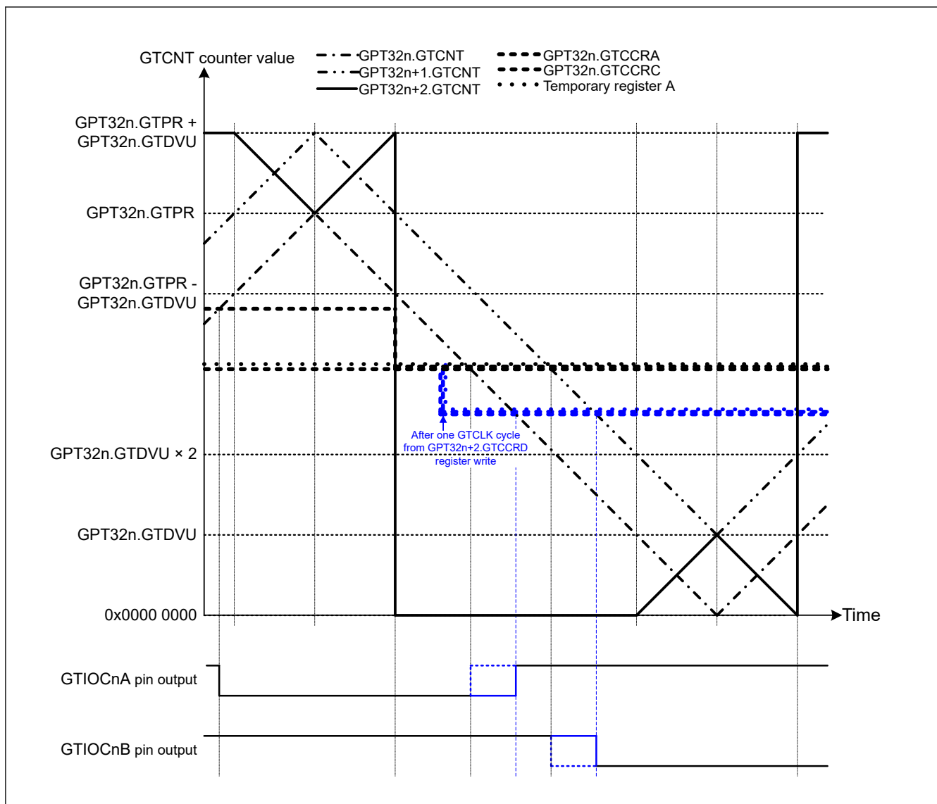
Figure 22.71 Example of Complementary PWM Mode 4 Single Buffer Operation (Down-Counting Middle Section) (Complementary PWM mode 4 single buffer operation, GTIOcNA pin = Low / GTIOcNB pin = High at GTCCRA register compare match during up-counting, GTIOcNA pin = High / GTIOcNB pin = Low at GTCCRA register compare match during down-counting, when a value smaller than the GPT32n.GTCNT value is written to GTCCRD register before down-counting compare match) (n = 4, 7)
