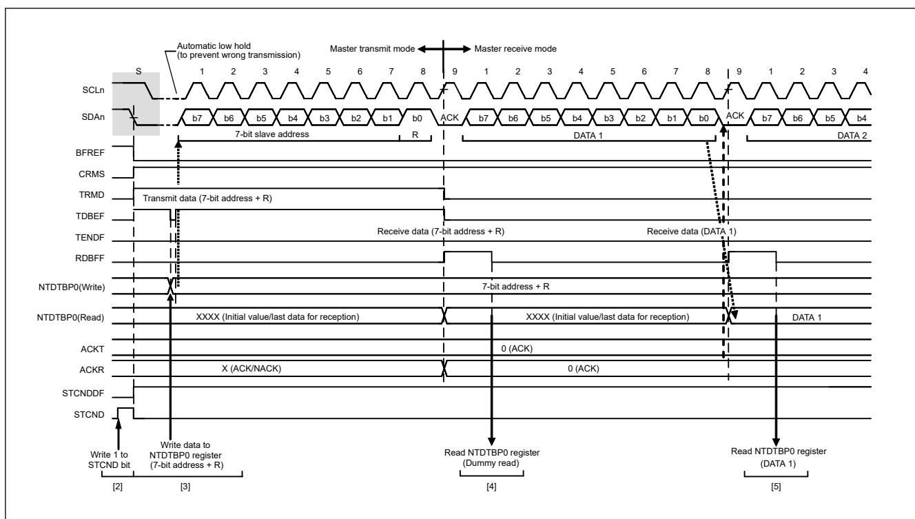
Figure 40.9 Master receive operation timing (1) (7-bit address format, when ACKTWE = 0)
