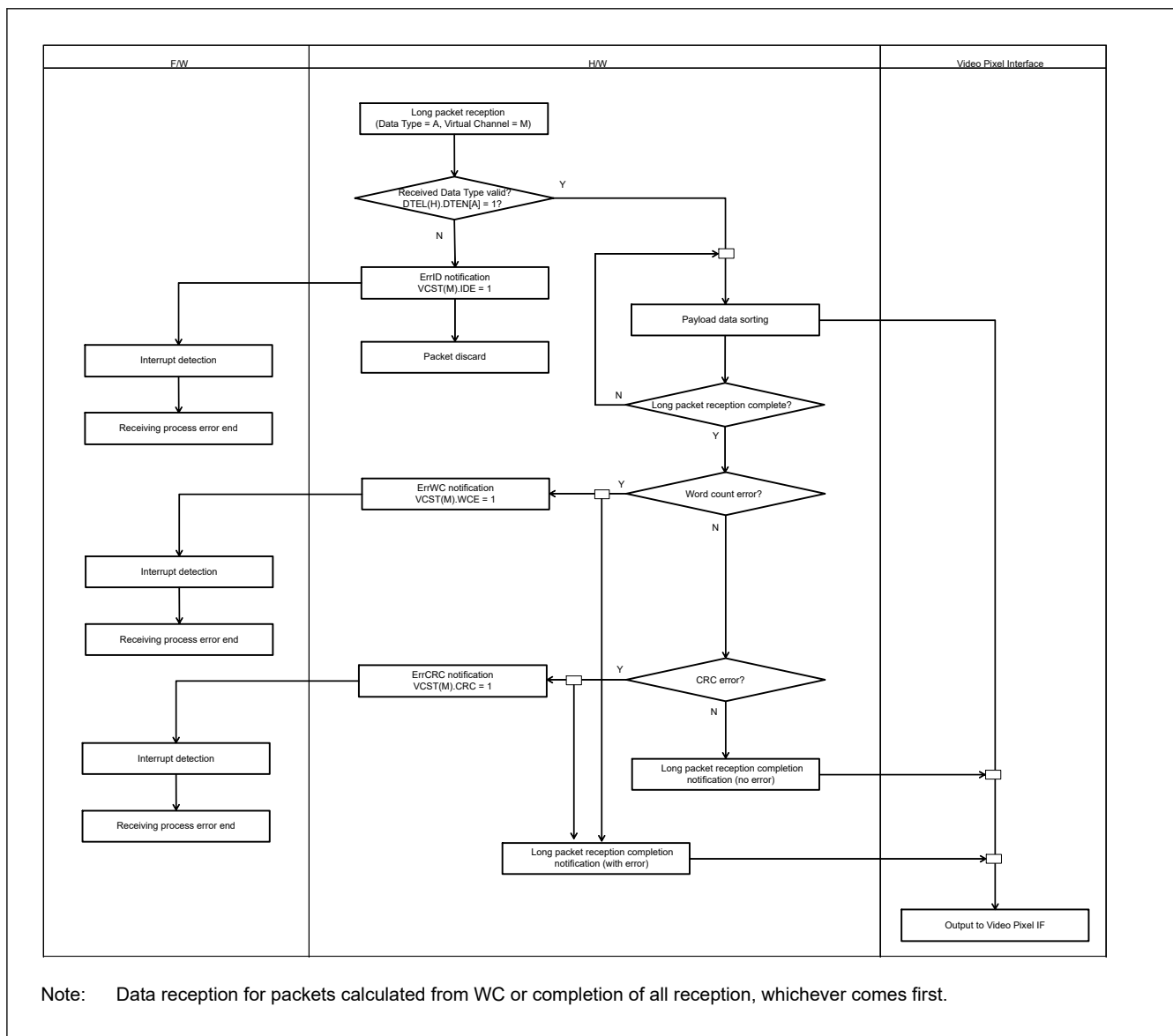
Figure 66.6 Long packet reception processing
