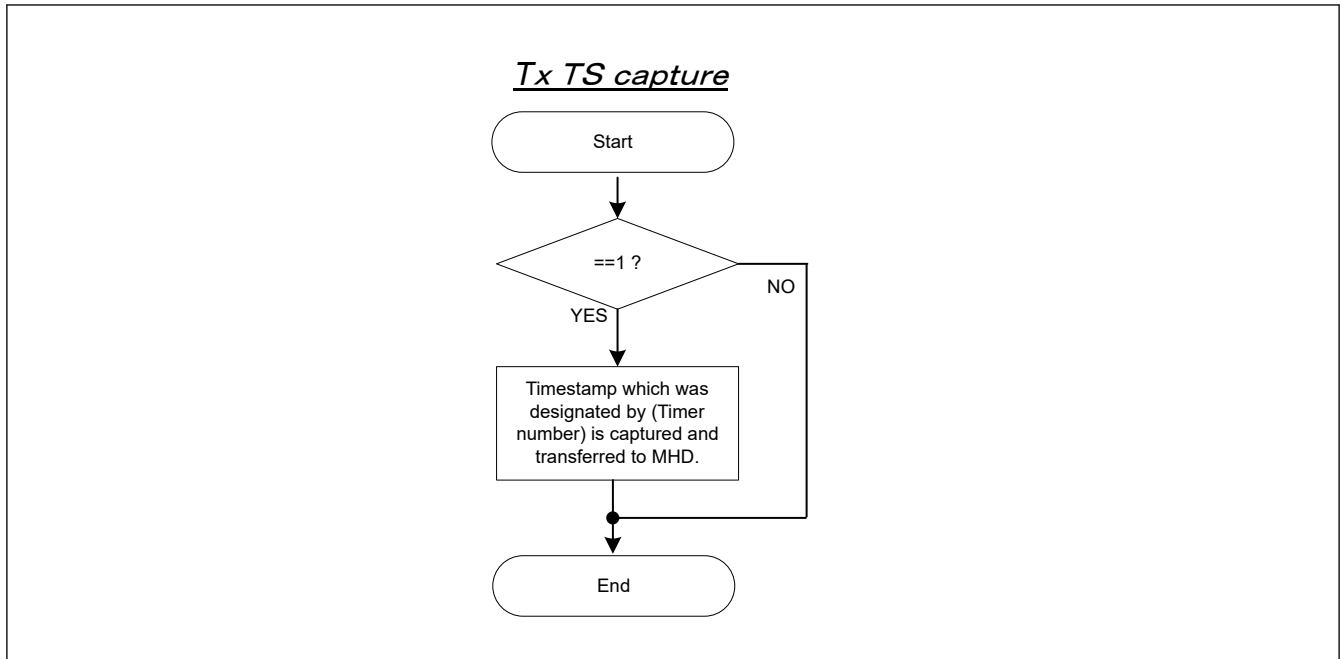
Figure 33.23 Tx Timestamp capture flow
