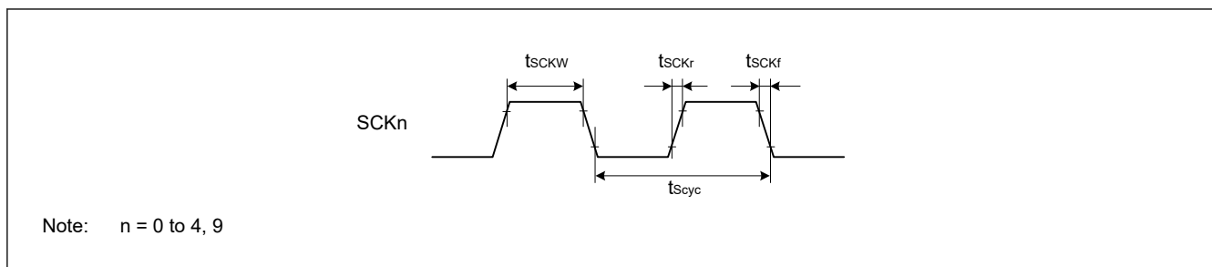
Figure 69.68 SCK clock input/output timing
