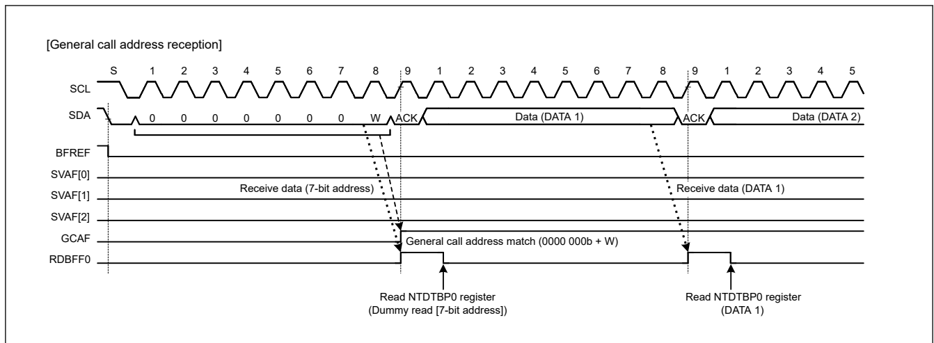
Figure 40.85 Timing of GCAF flag setting during reception of general call address
