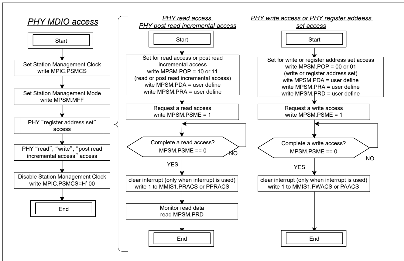
Figure 33.9 PHY eMDIO access flow
