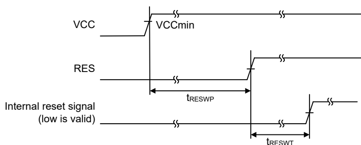
Figure 69.32 RES pin input timing under the condition that VCC exceeds V_{POR} voltage threshold
