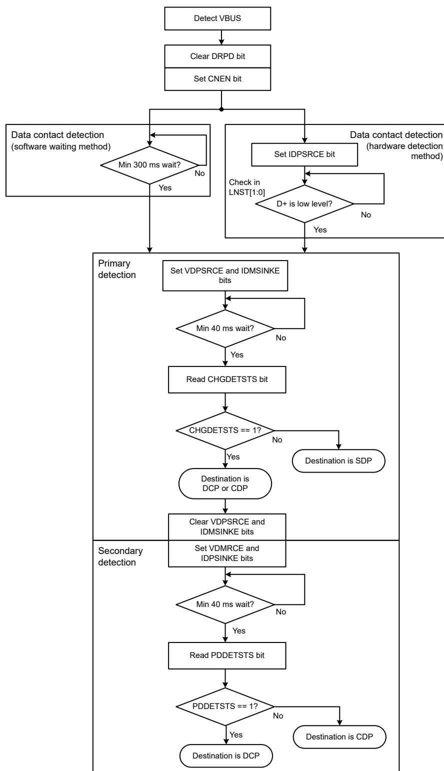
Figure 37.19 Processing flow as portable device
