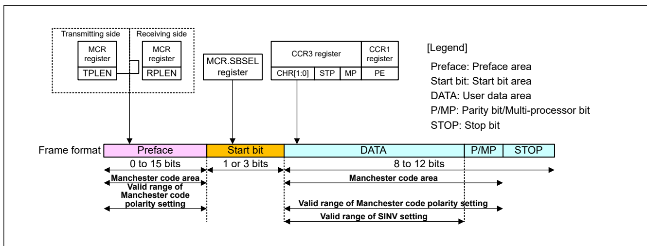
Figure 38.46 Frame Format in Manchester Mode
