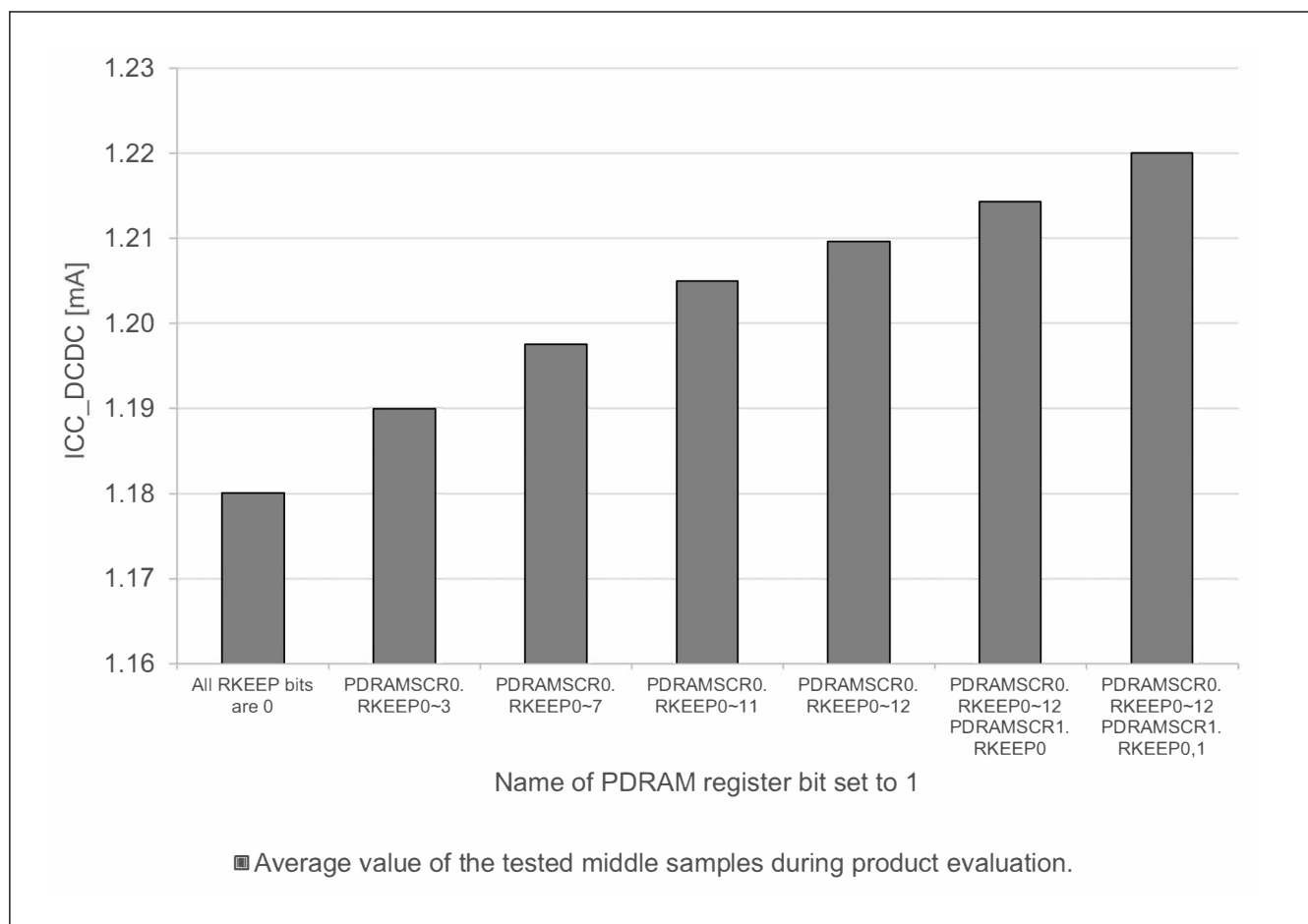
Figure 69.17 Software Standby current per SRAM state (ICC_DCDC, SS2LP_1, SVSCR_4) (reference data)
