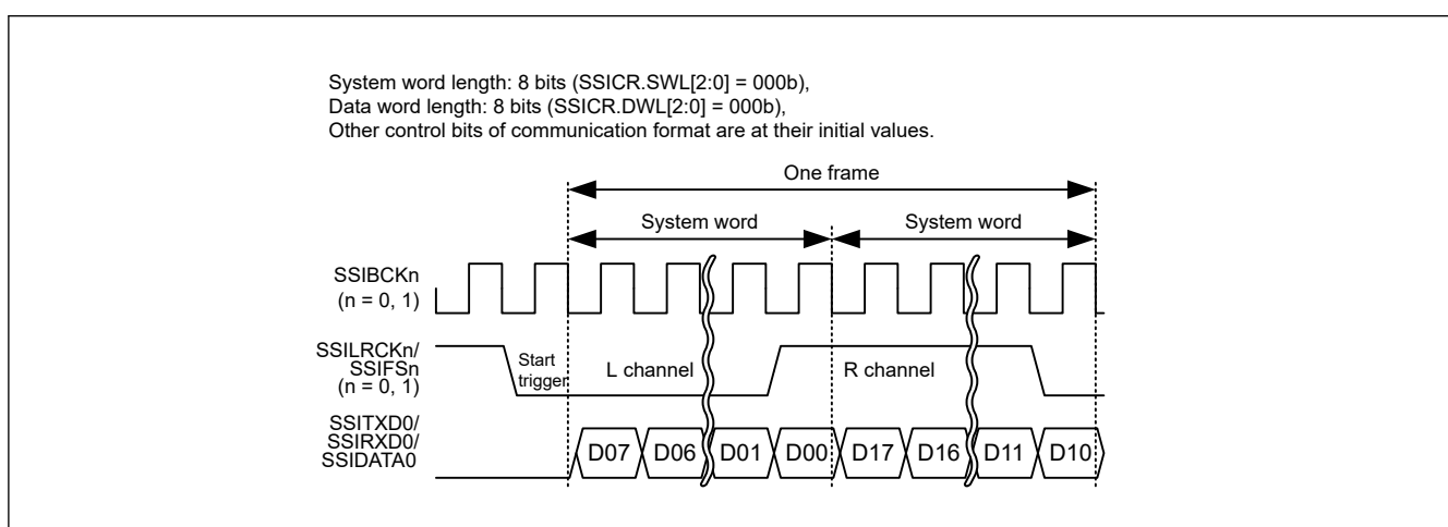
Figure 46.37 I 2 S format (without padding: system word length = data word length)
