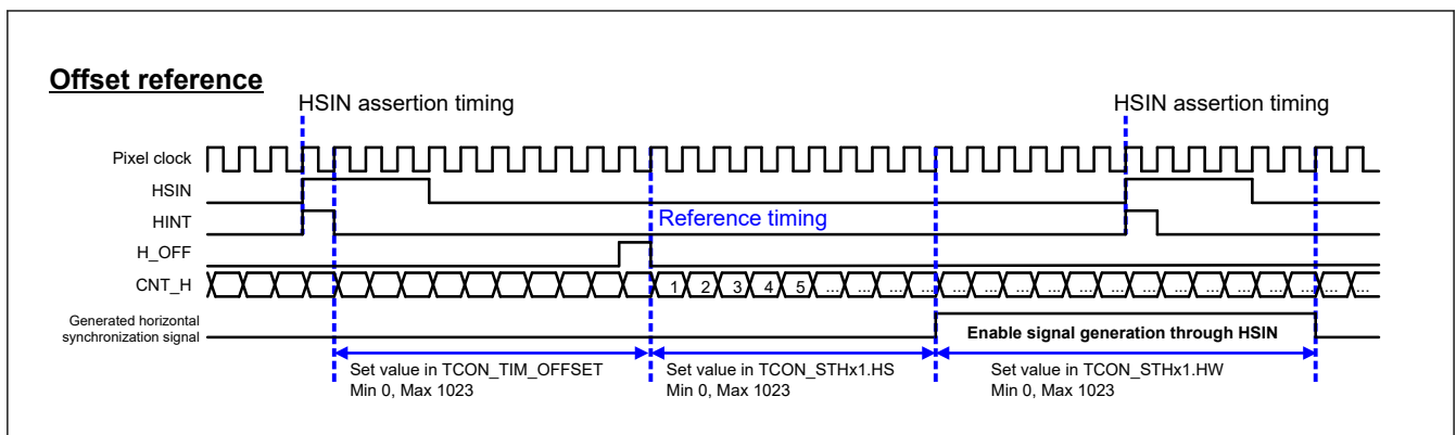
Figure 63.21 Horizontal synchronization signal generation based on offset
