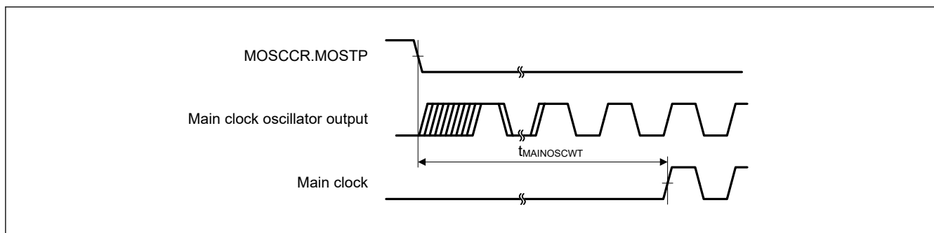
Figure 69.27 Main clock oscillation start timing
