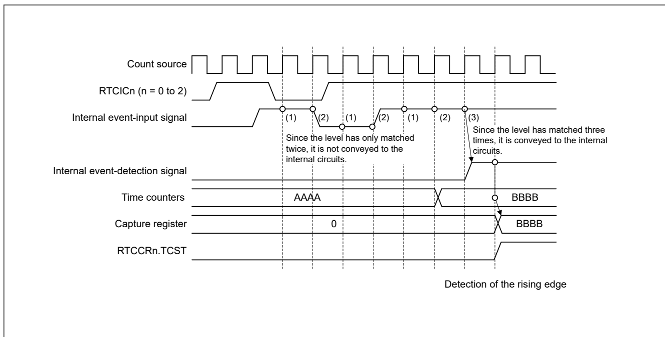
Figure 26.10 Timing of a time capture operation with the noise filter on
