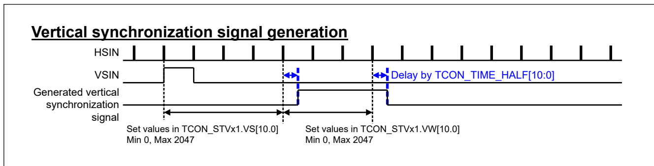
Figure 63.18 Generation of vertical synchronization signal
