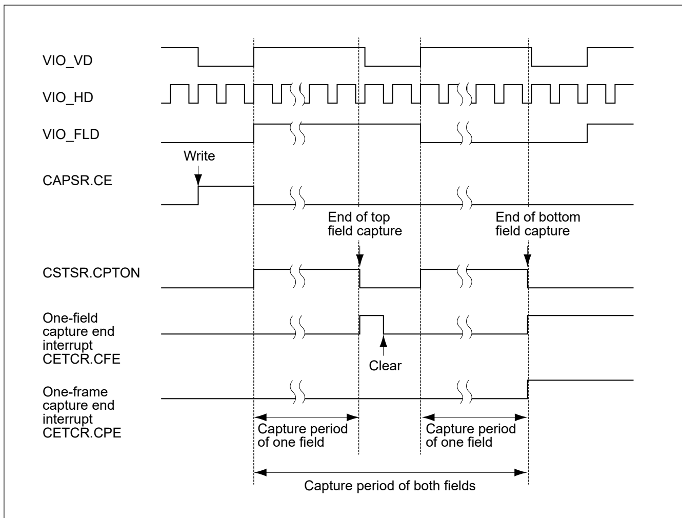
Figure 60.23 One-frame capture end interrupt and one-field capture end interrupt in both-field image capture
