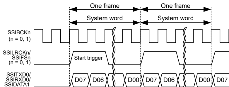
Figure 46.40 Long frame in monaural format (without padding)
