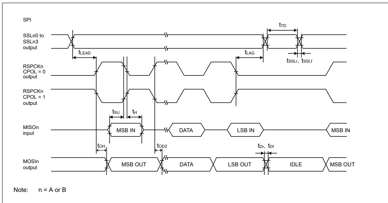
Figure 69.77 SPI timing for Motorola SPI master when CPHA = 1
