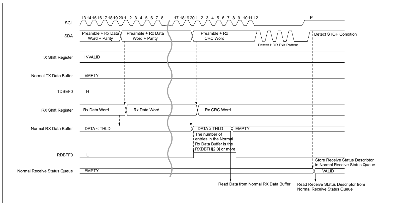
Figure 40.55 HDR data write transfer (HDR-DDR) timing (3/3)
