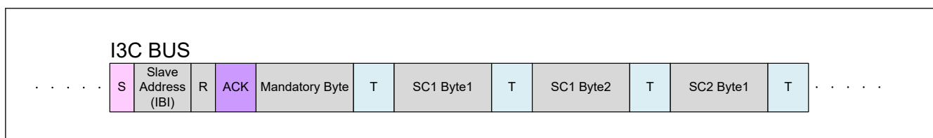
Figure 40.111 Example of asynchronous mode 0 timestamp data transfer
