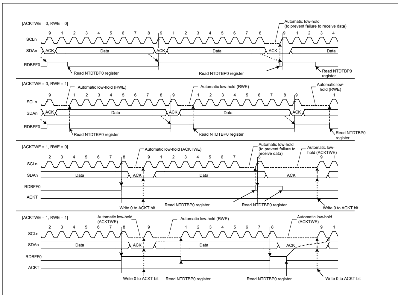
Figure 40.95 Automatic low-hold operation in receive mode (using ACKTWE and RWE bits)
