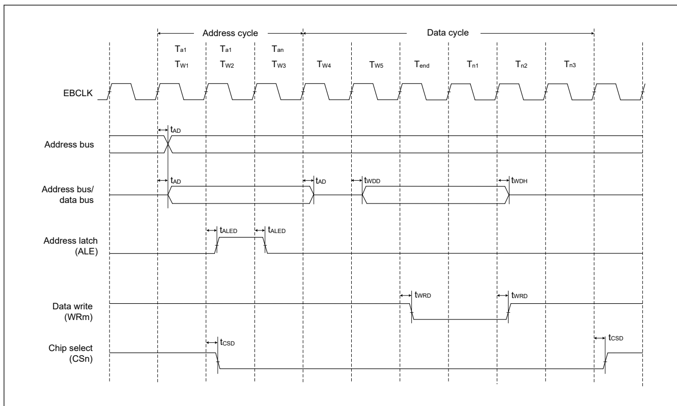
Figure 69.39 Address/data multiplexed bus write access timing
