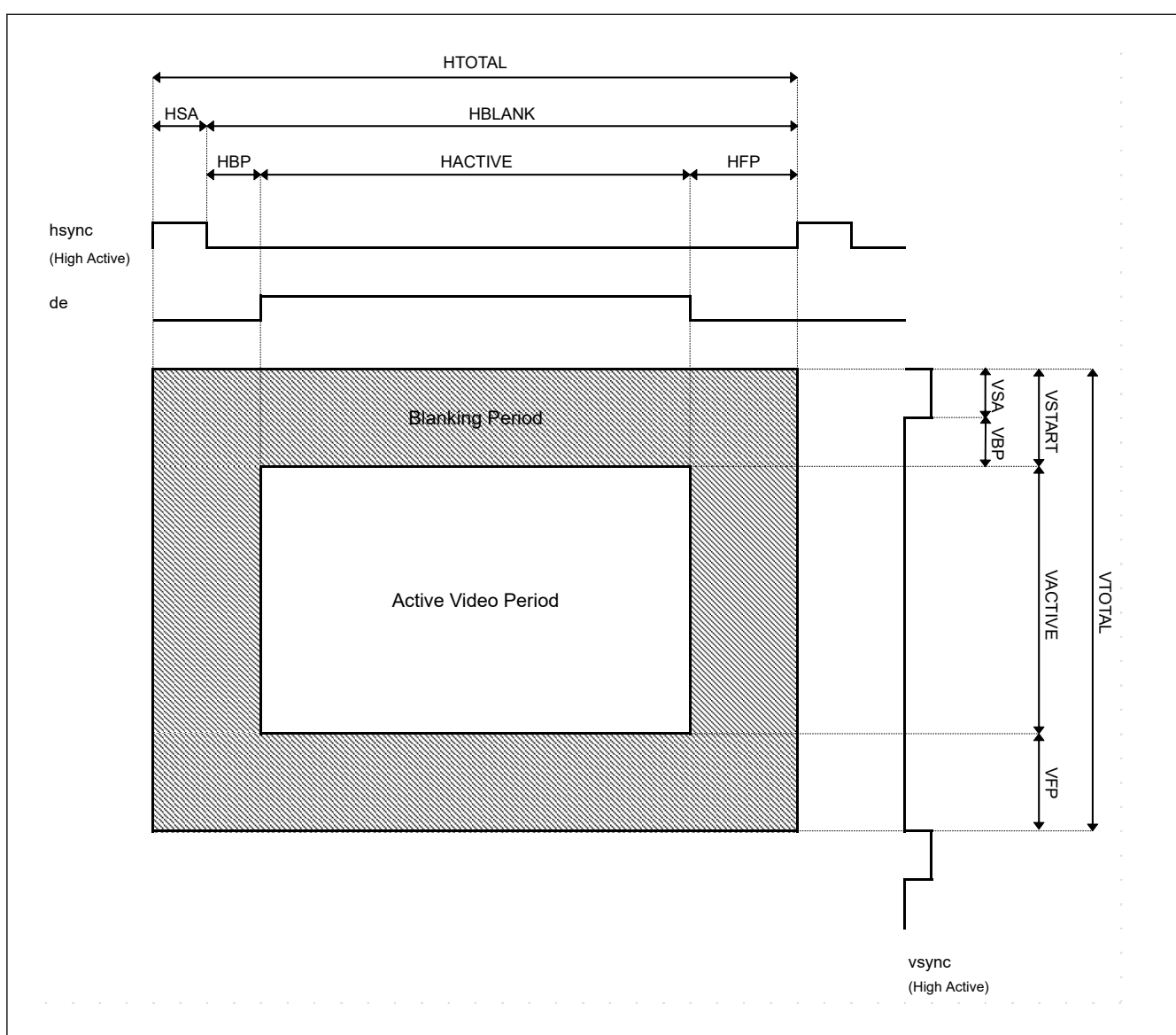
Figure 65.9 Video mode timing
