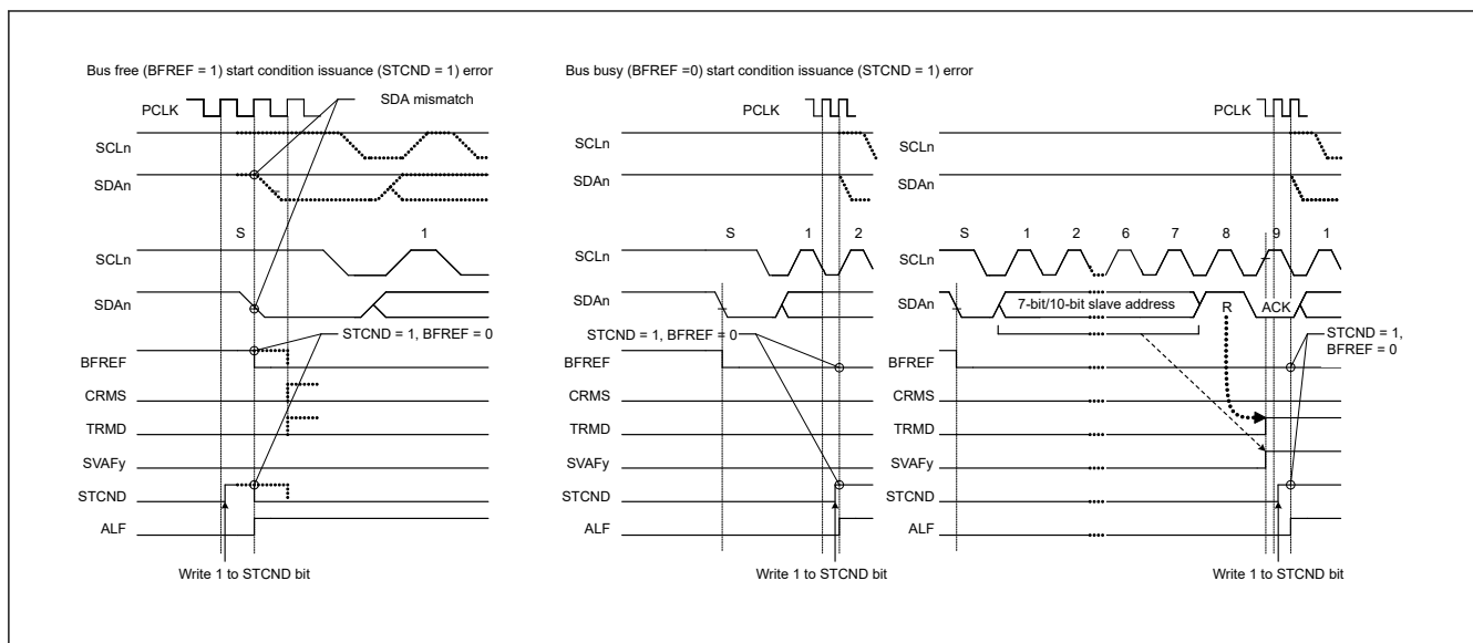
Figure 40.90 Arbitration-lost detection when a START condition is issued (MALE = 1)
