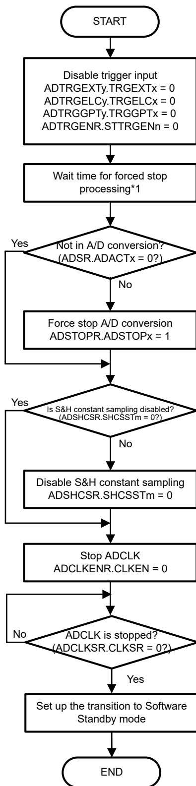
Figure 53.64 Example procedure for entering Software Standby mode
