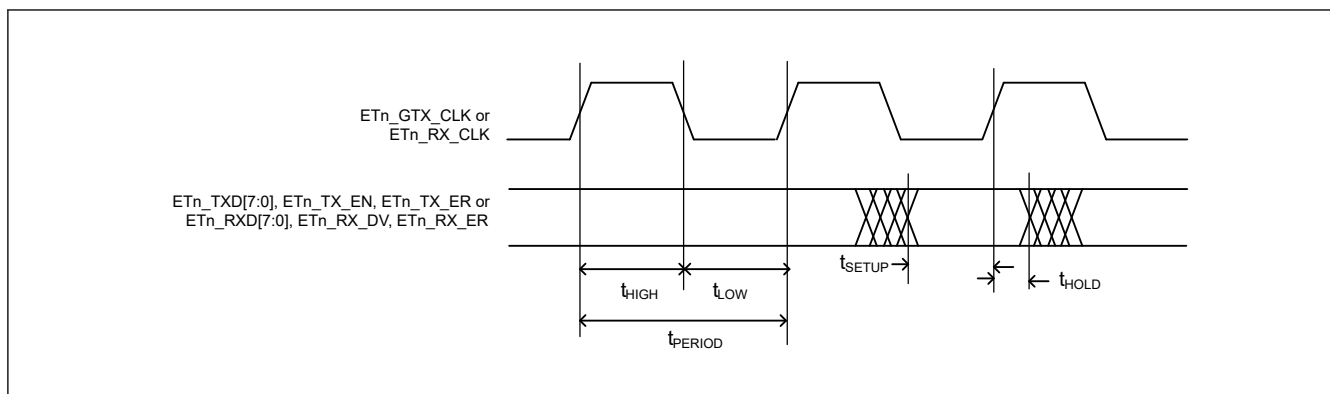
Figure 69.118 GMII timing
