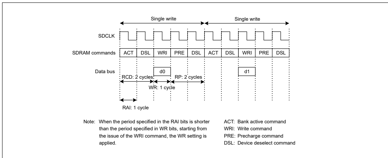
Figure 15.57 Example timing for single write (2)
