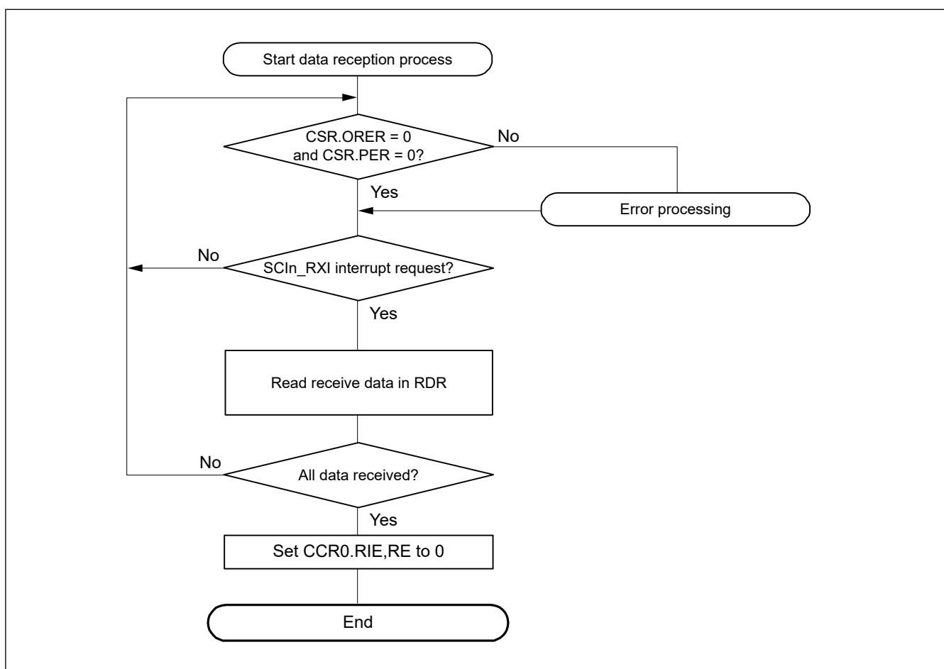
Figure 38.84 Example flow of smart card interface reception
