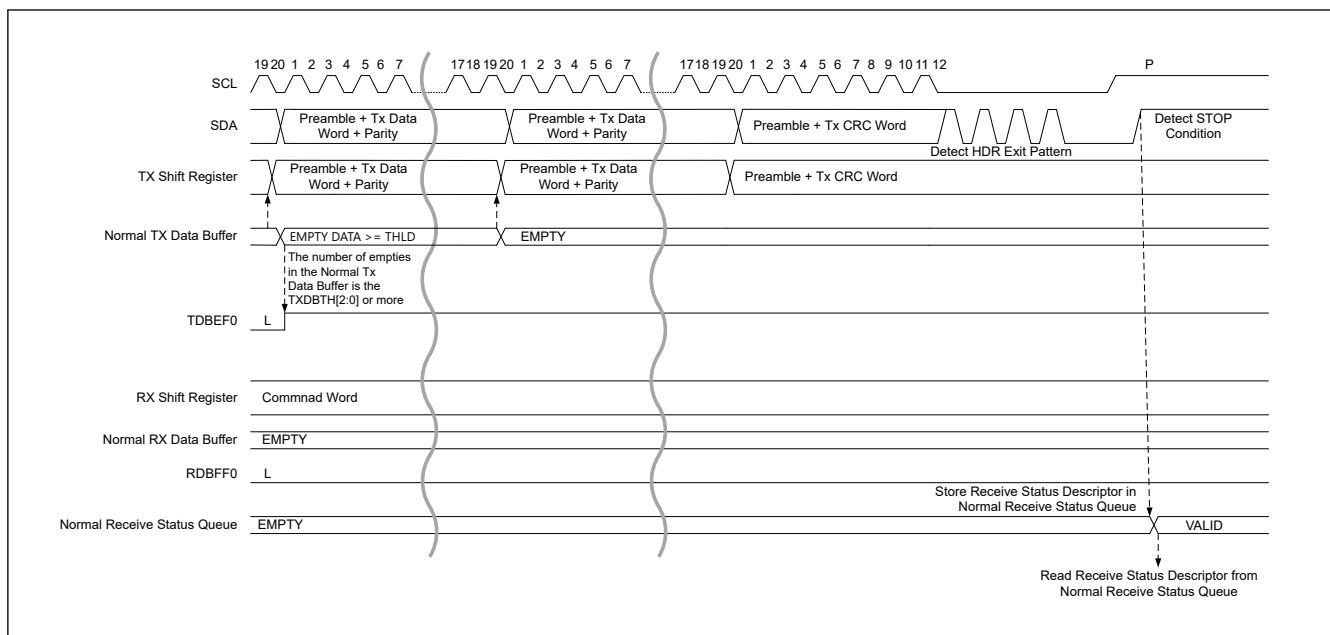
Figure 40.60 HDR data read transfer (HDR-DDR) timing (3/3)
