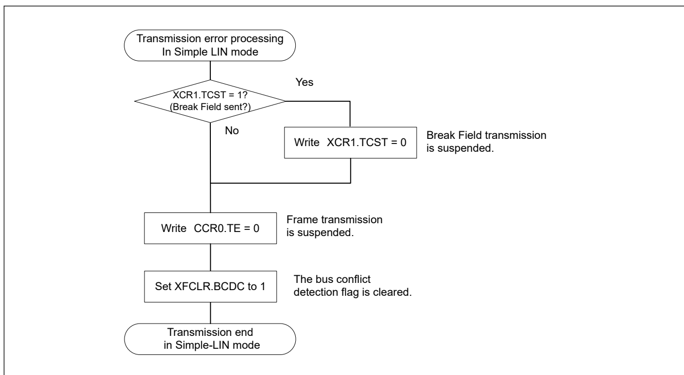
Figure 38.111 SCIn_ERI Interrupt handling flow at transmission in Simple LIN mode
