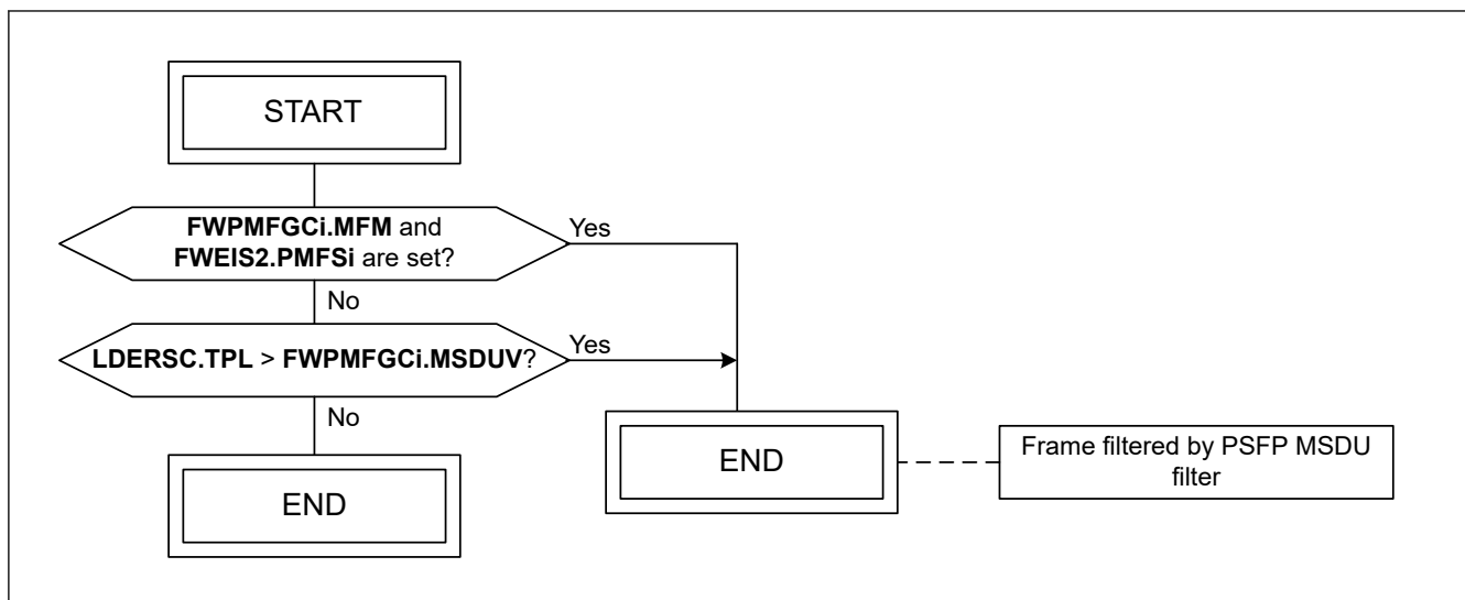
Figure 30.103 MSDU filtering flow for MSDU filter i
