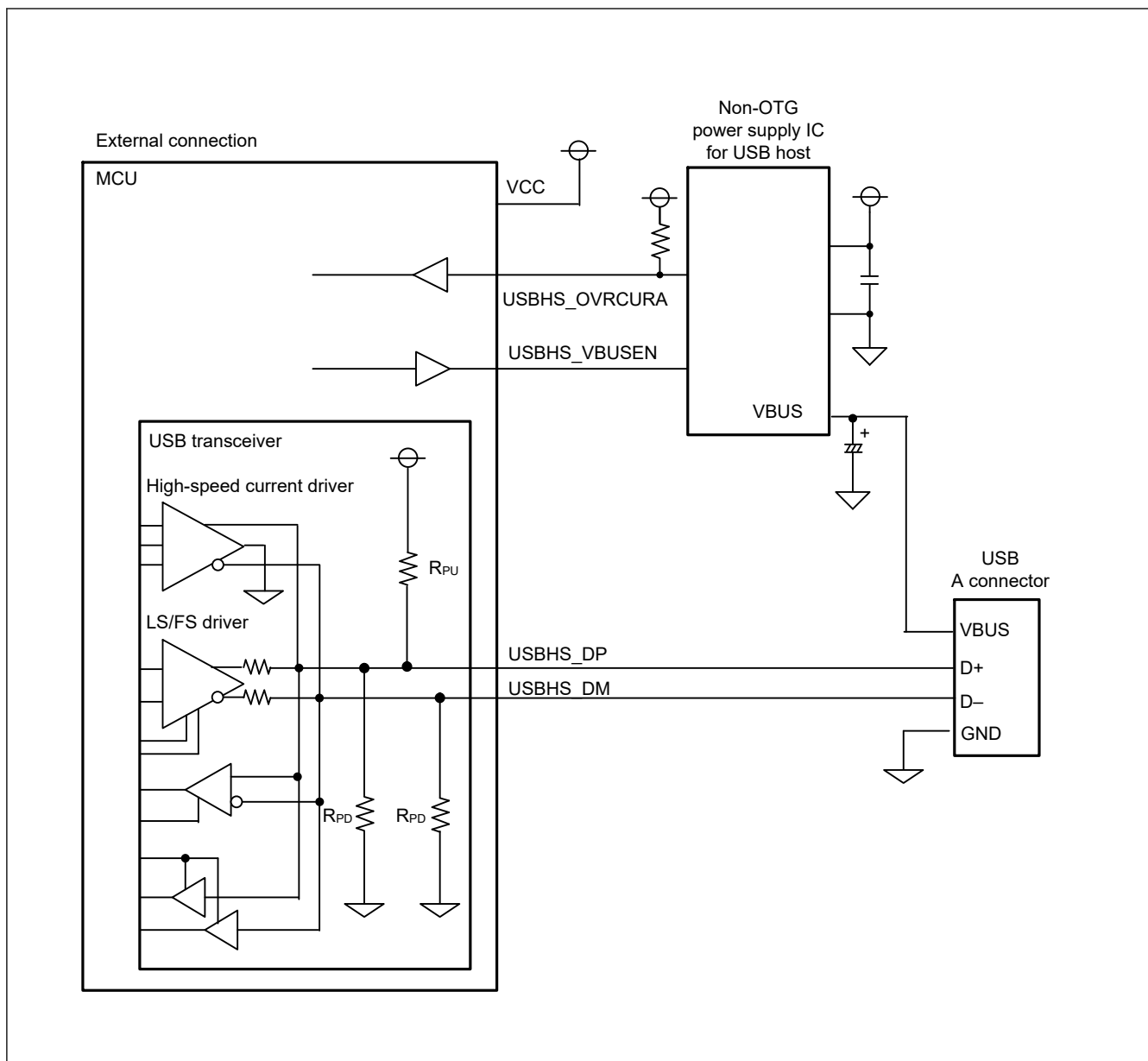
Figure 37.30 Example USB host connection
