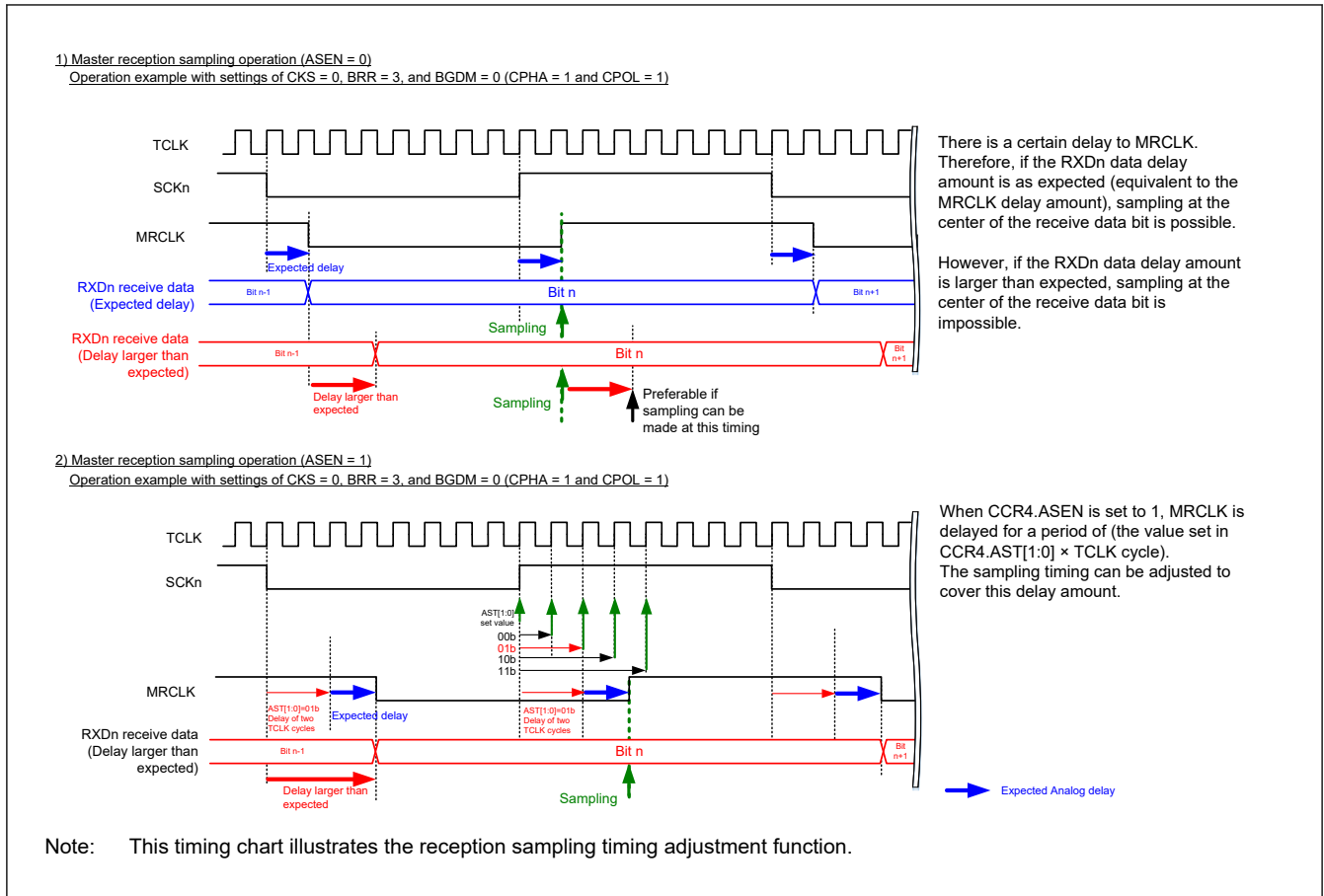
Figure 38.73 Reception Sampling Timing Adjustment Operation in Clock Synchronous Mode (Master)
