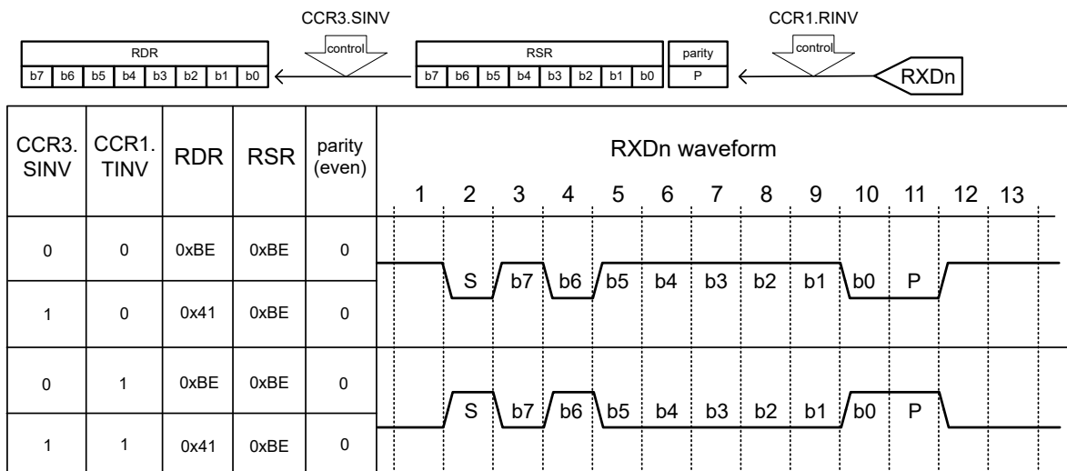
Figure 38.3 Example of receive or transmit data control
