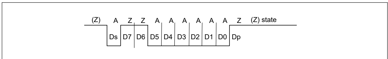
Figure 38.77 Inverse convention with LSBF in CCR3 = 0, SINV in CCR3 = 1, and PM in CCR1 = 1
