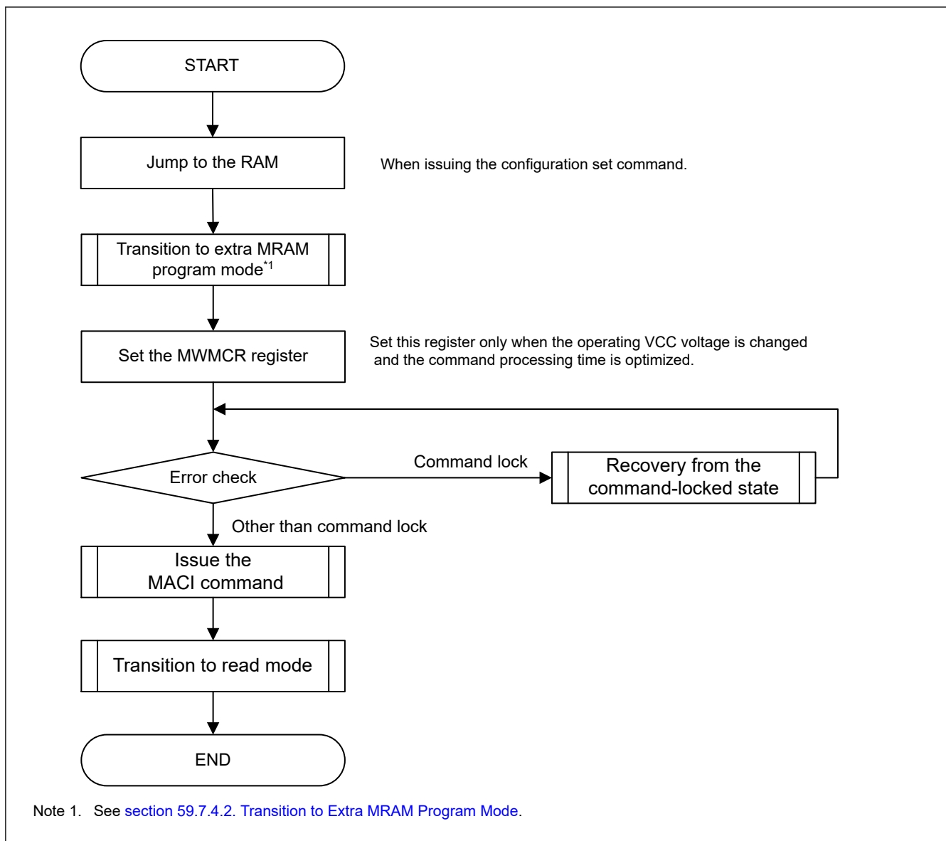
Figure 59.9 Overview of command usage in extra MRAM program mode
