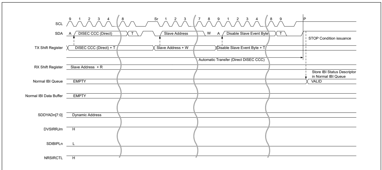
Figure 40.104 Slave interrupt request : NACK (DVSIRRJ = 1) and NRSIRCTL = 1 (2/2)
