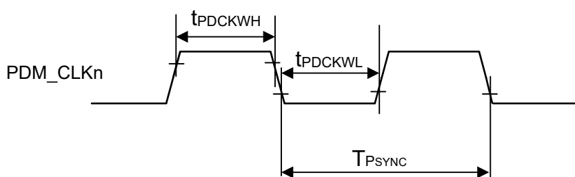
Figure 69.123 Timing of clock output (PDM_CLKn)
