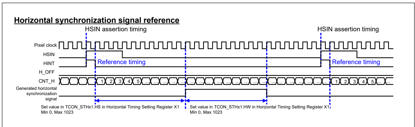
Figure 63.20 Signal generation based on input horizontal synchronization signal (HSIN)
