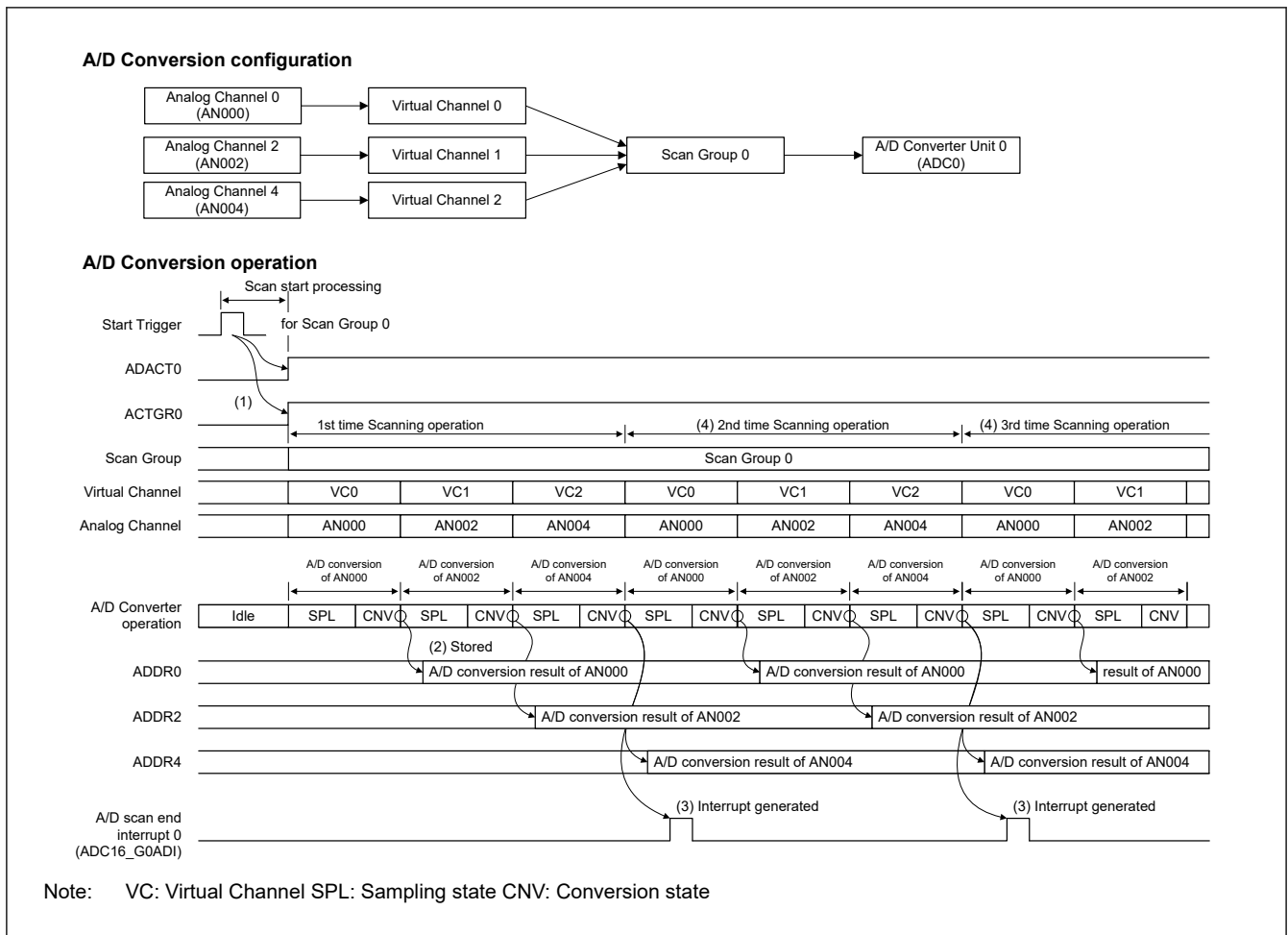
Figure 53.8 Example of scanning operation in SAR mode – Continuous scan mode
