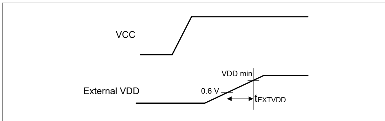
Figure 69.146 Power-up sequence of external VDD mode without using RES pin
