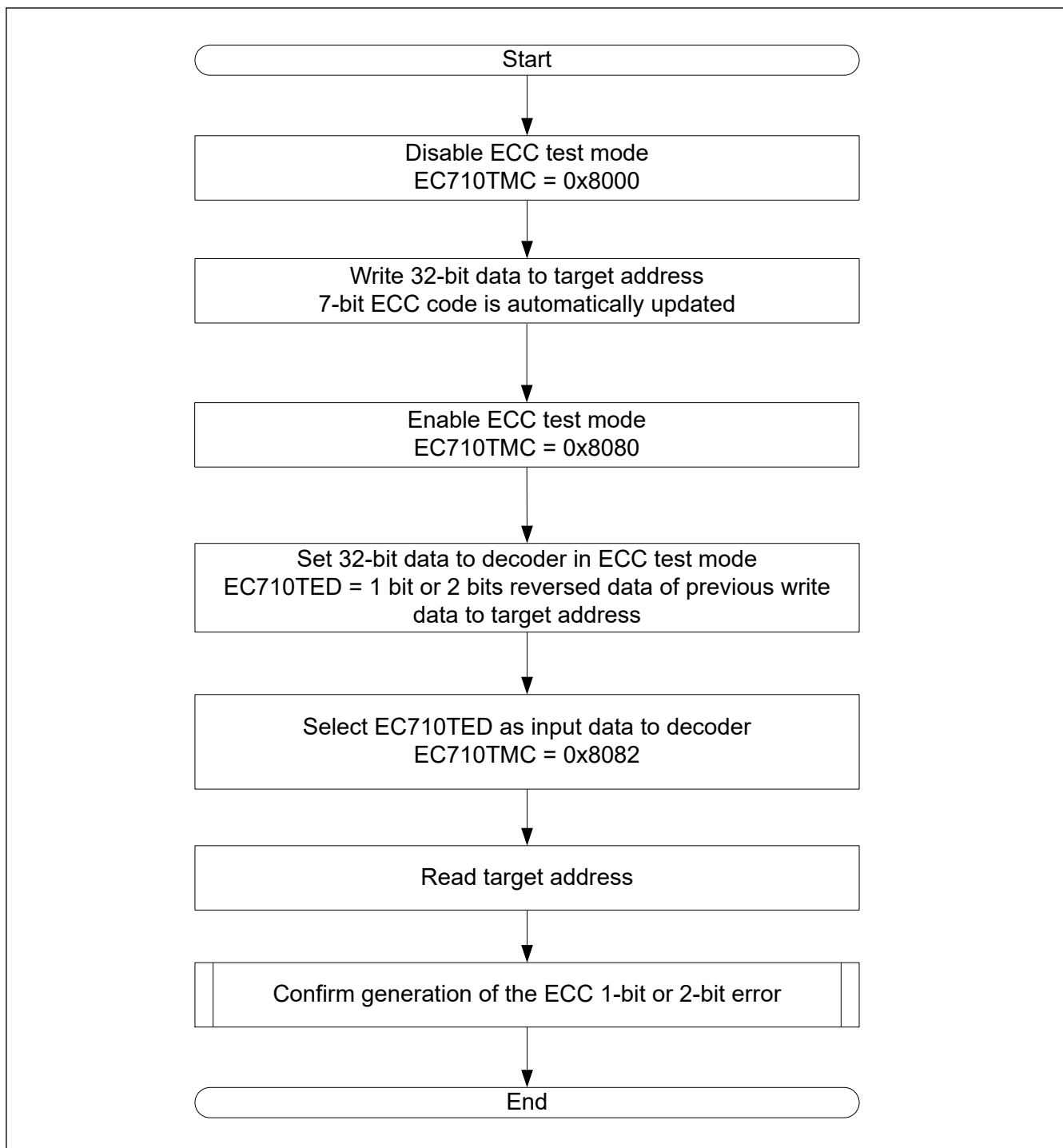
Figure 42.2 Testing procedure for ECC decoder
