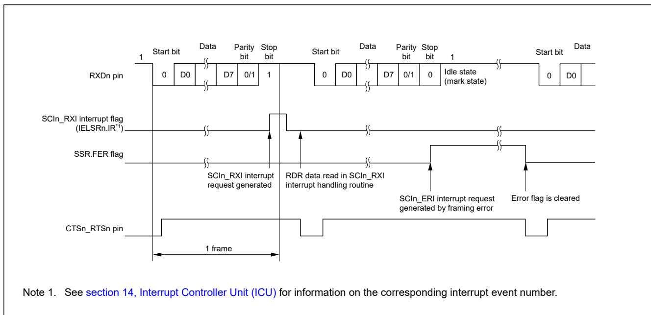
Figure 38.20 Example of SCI operation for serial reception in Asynchronous mode (2) when RTS function is used, and with 8-bit data, parity bit, and 1 stop bit
