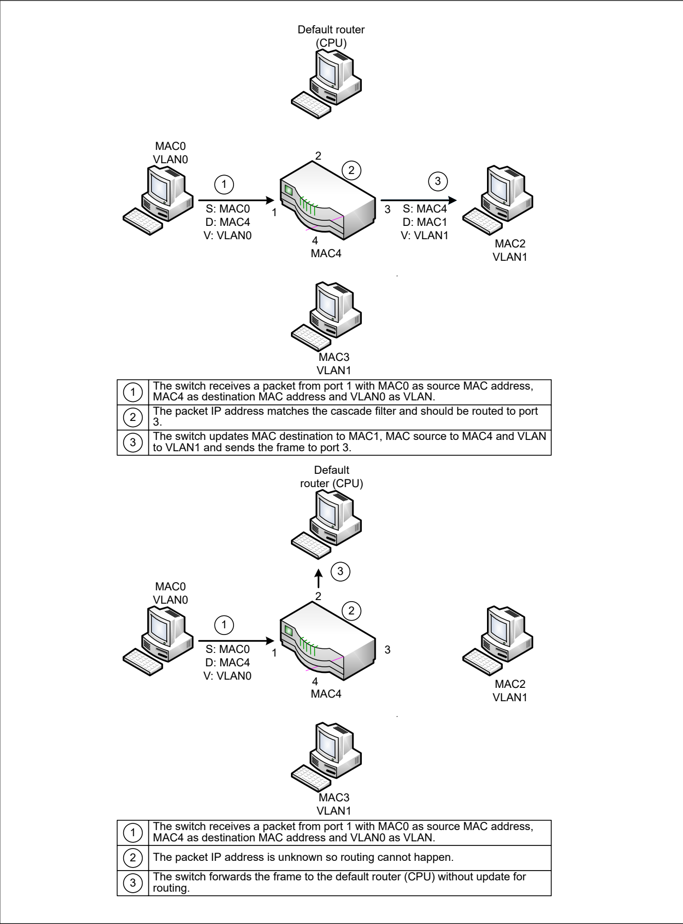
Figure 29.10 Layer 3 switch operation
