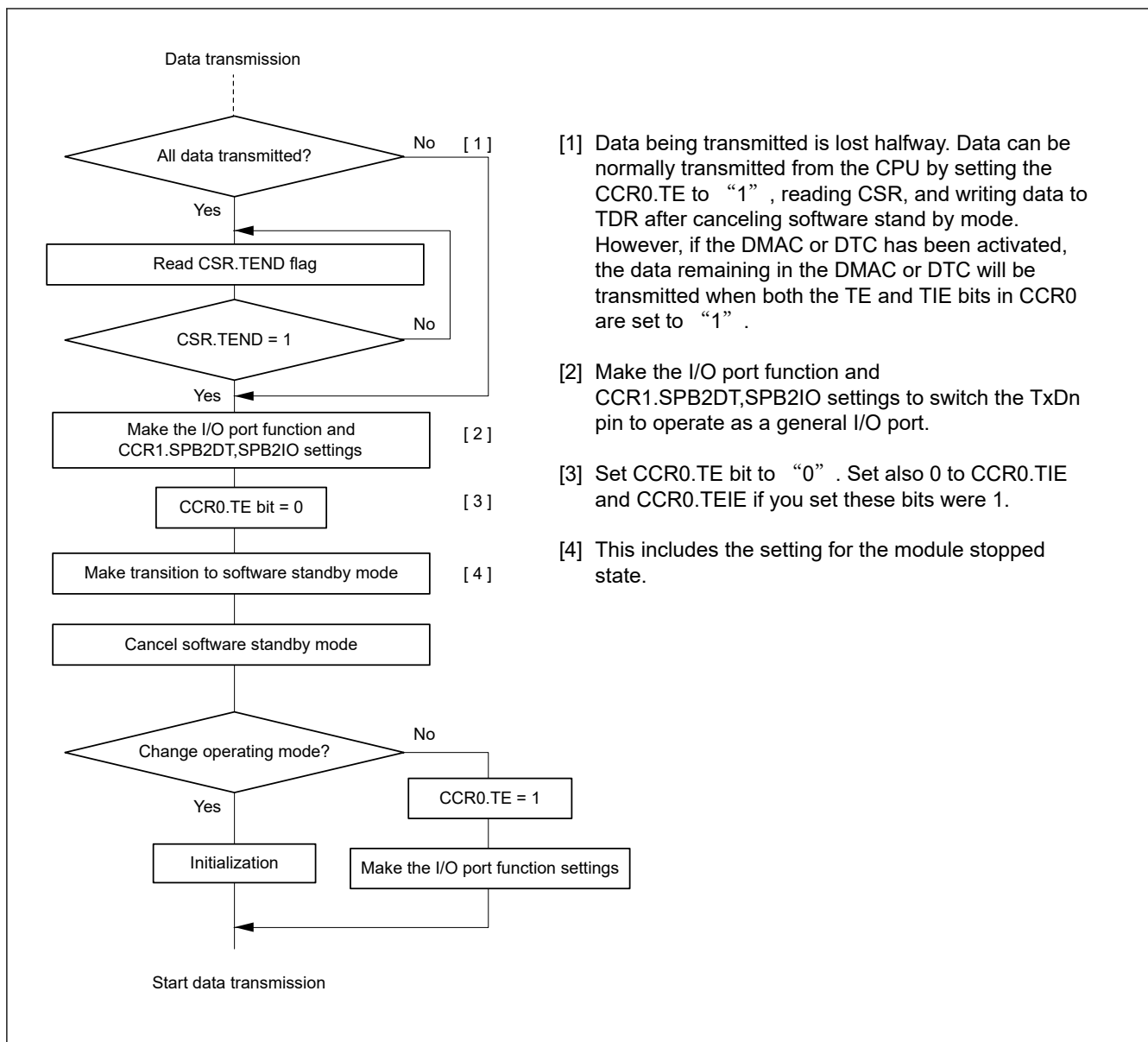
Figure 38.117 Example of Flowchart for Transition to Software Standby Mode during Transmission
