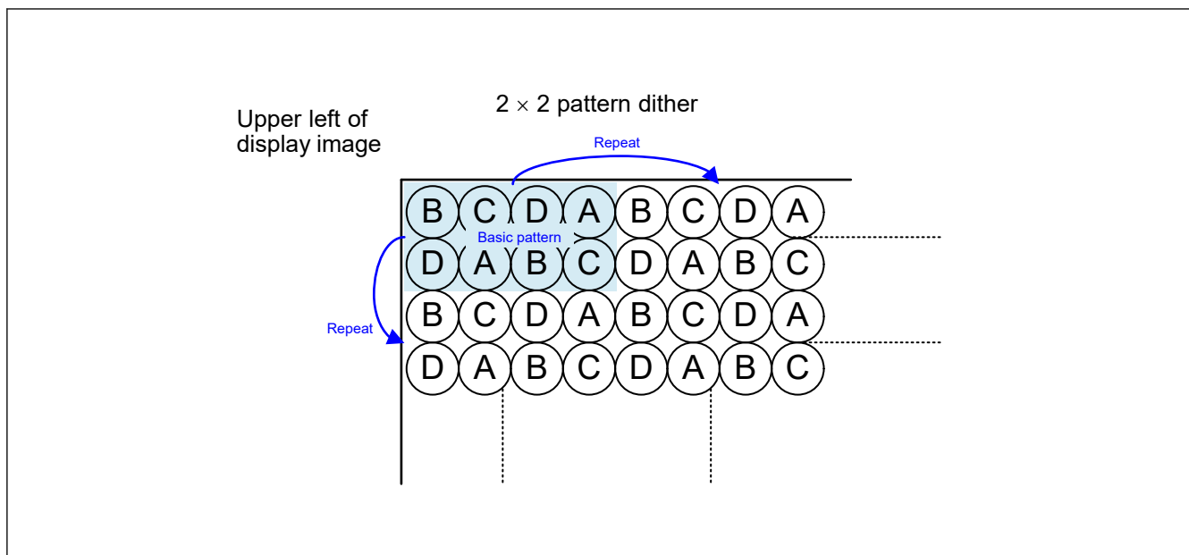
Figure 63.14 Addition value selection method for 2 × 2 pattern dither
