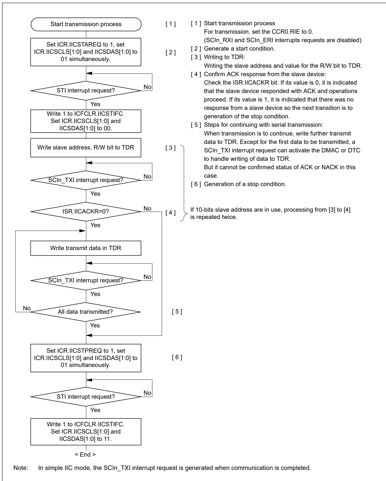
Figure 38.93 Example flow of master transmission in simple IIC mode with transmission interrupts and reception interrupts
