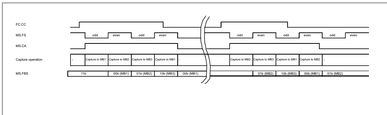
Figure 67.6 Data output frame memory in continuous frame capture mode (Example of operation)
