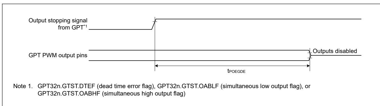
Figure 69.56 Output Disable Time for POEG in Response to Detection of the Output Stopping Signal from GPT
