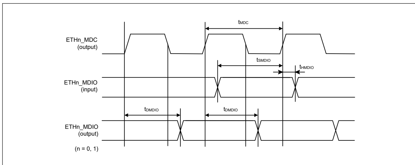
Figure 69.123 ETn_MDIO, ETn_MDC timing
