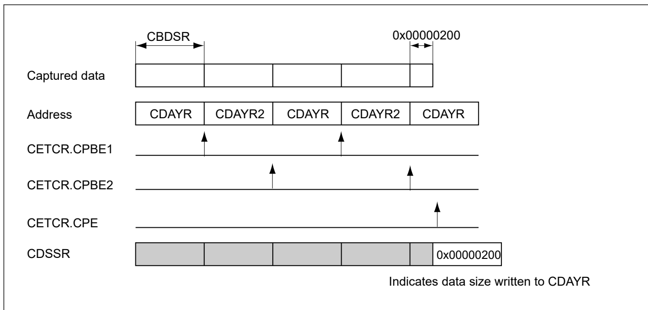
Figure 60.49 Overall timing of CDSSR operation in bundle write (when bundle write end and capture end do not coincide)
