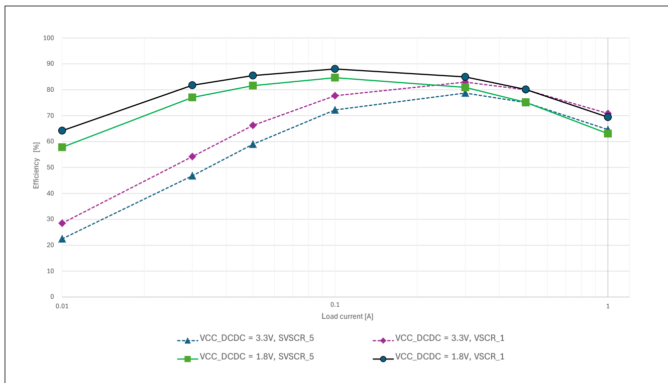
Figure 69.19 Typical DCDC efficiency (%) vs load current (A) in High-speed mode and Software Standby mode (SSCR1.SS2LP = SS2LP_1), Tj = 25 °C
