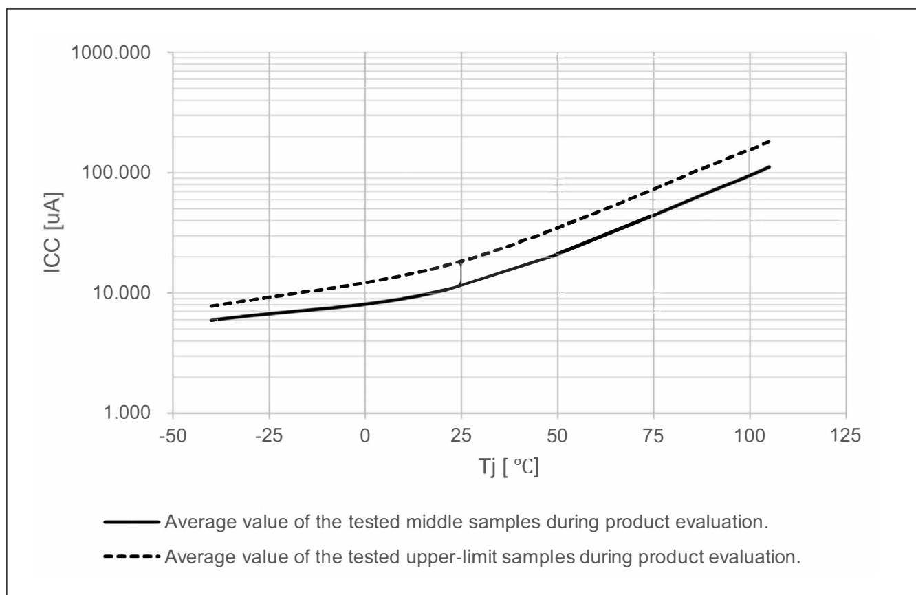
Figure 69.7 Temperature dependency in Deep Software Standby mode 1 (reference data)
