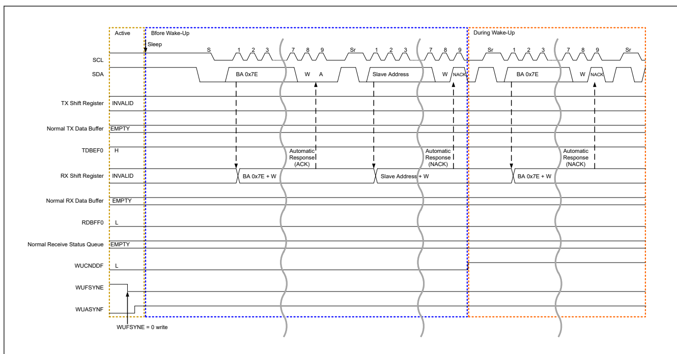
Figure 40.135 I3C slave wake-up operation (1/2)
