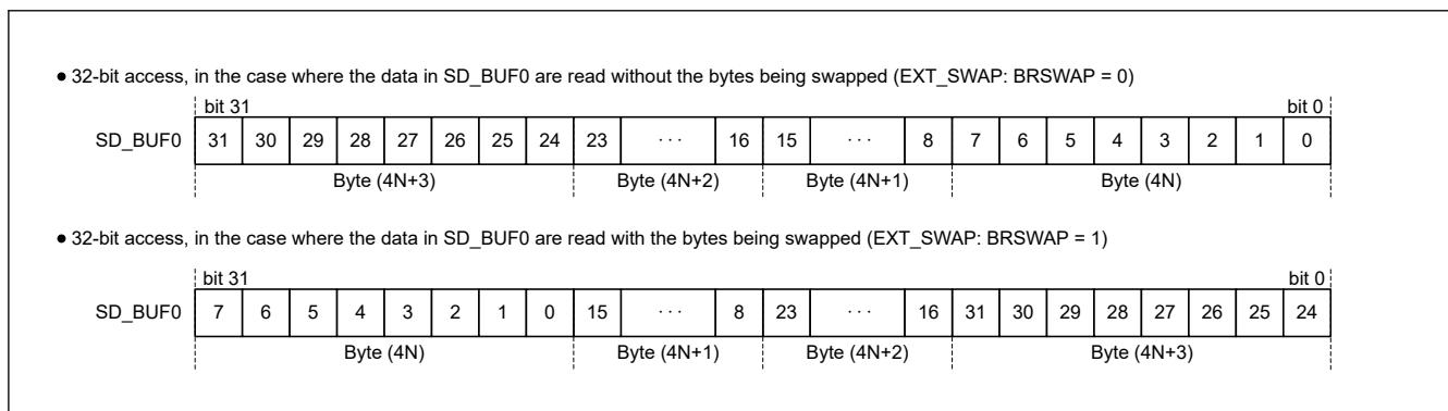
Figure 47.6 Read from SD_BUF0
