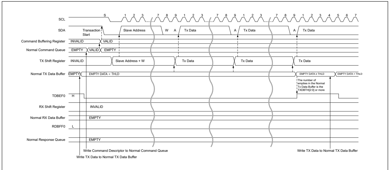
Figure 40.18 Legacy I2C message data write timing (1/2)
