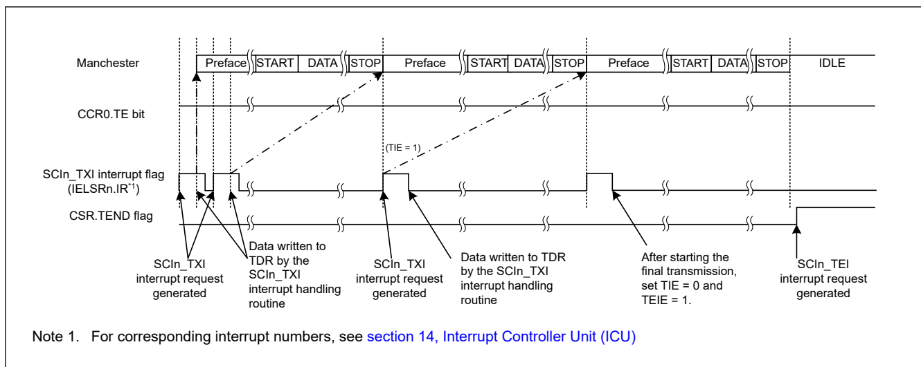
Figure 38.54 Example of End-of-Transmission Operation for Serial Transmission in Manchester Mode (with Preface but Without the CTS Function)
