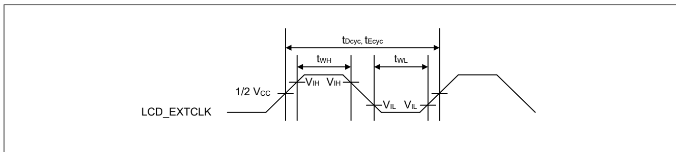
Figure 69.110 LCD_EXTCLK clock timing
