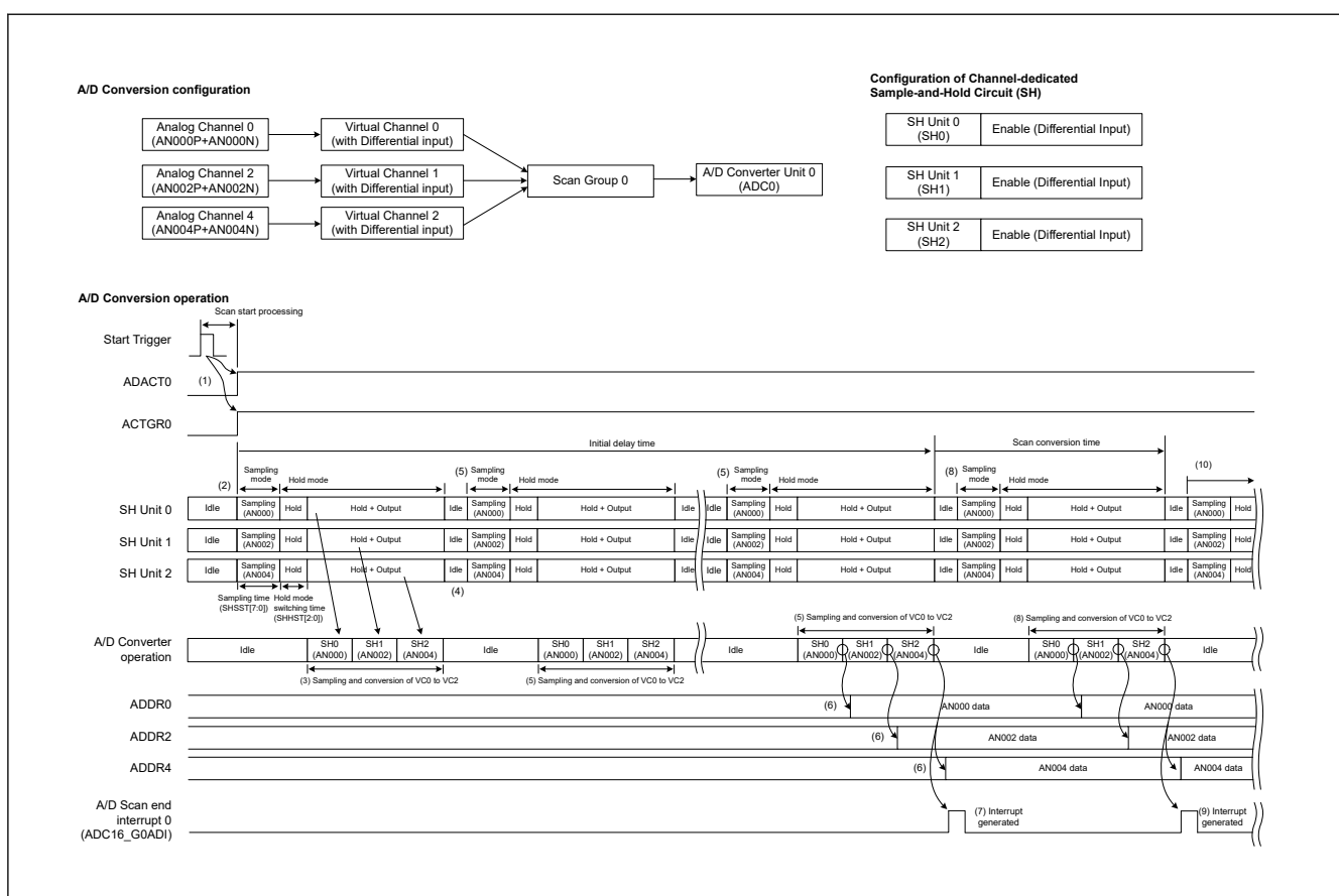
Figure 53.21 Basic operation of channel-dedicated sample-and-hold circuit in Hybrid mode – Continuous scan mode
