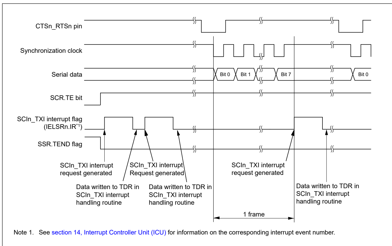
Figure 38.63 Example of serial data transmission in clock synchronous mode when the CTS function is used at the beginning of transmission
