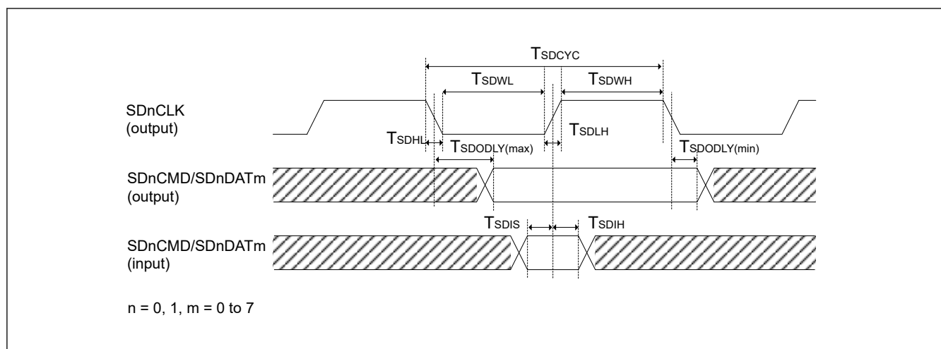
Figure 69.107 SD/MMC Host Interface signal timing
