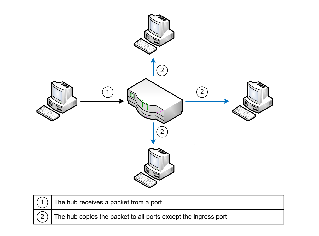
Figure 29.7 Hub operation
