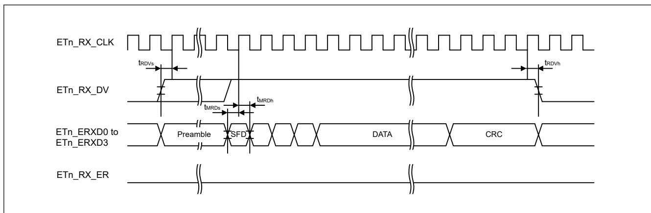
Figure 69.117 MII reception timing in normal operation
