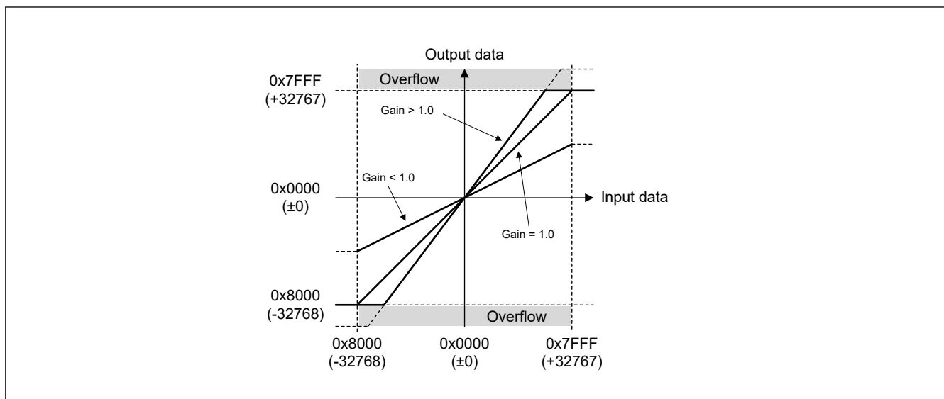
Figure 53.37 User's Gain Adjustment (16-bit data length format and Signed data format)
