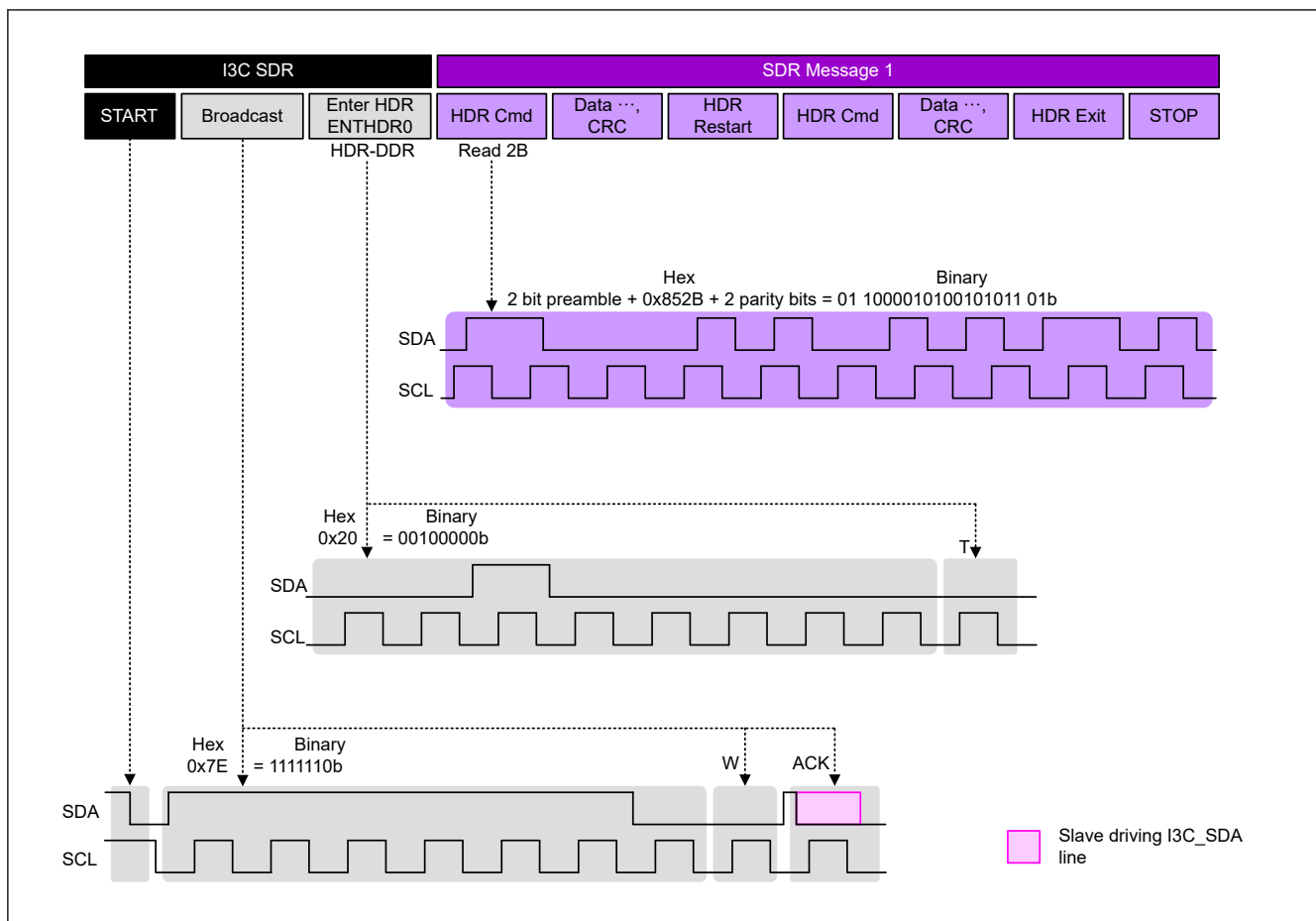
Figure 40.75 Example communication using HDR-DDR protocol
