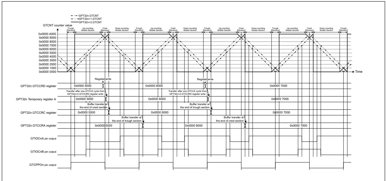
Figure 22.50 Example of Complementary PWM Mode 3 Operation (Single buffer operation, GTIOcNA pin = Low / GTIOcNB pin = High at GTCCRA register compare match during up-counting, GTIOcNA pin = High / GTIOcNB pin = Low at GTCCRA register compare match during down-counting, the dead time value is 0x0000 1000 and updating GTCRD register in crest and trough sections) (n = 4, 7)
