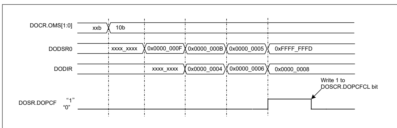
Figure 57.9 Example of Operation in Data Subtraction Mode
