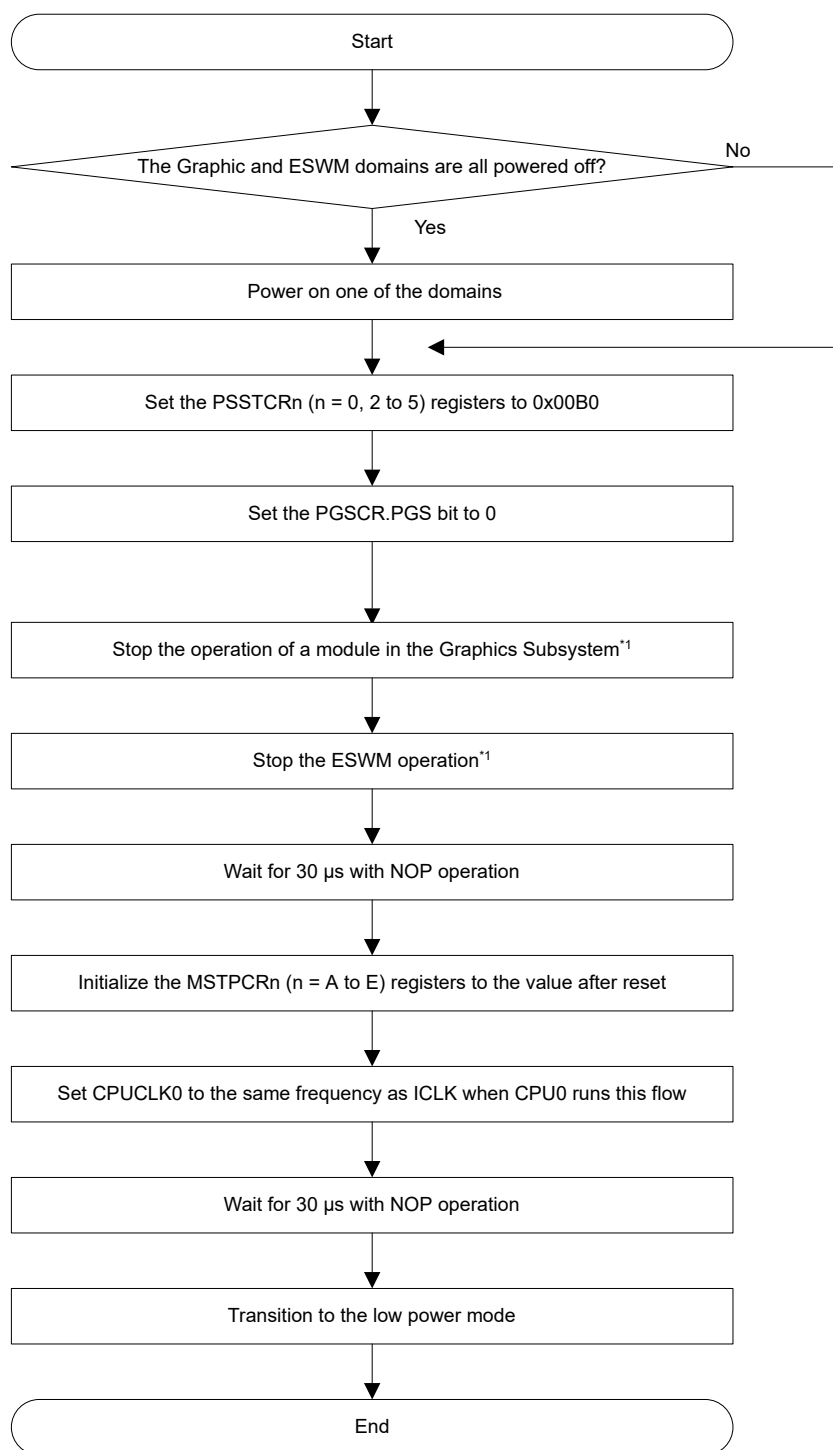
Figure 11.11 Additional flow for the transition to Software Standby mode and Deep Software Standby mode 1/2/3
