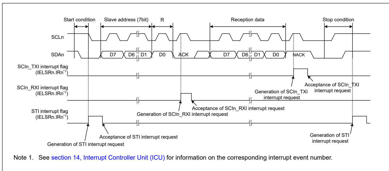
Figure 38.95 Example of Operations for Master Reception in Simple IIC Mode (7bit Slave address, ACK and NACK interrupt in use (ICR.IICINTM = 0))
