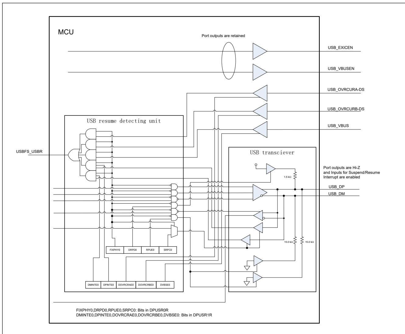
Figure 36.6 Connection between the USB resume detecting unit and the USB I/O pins
