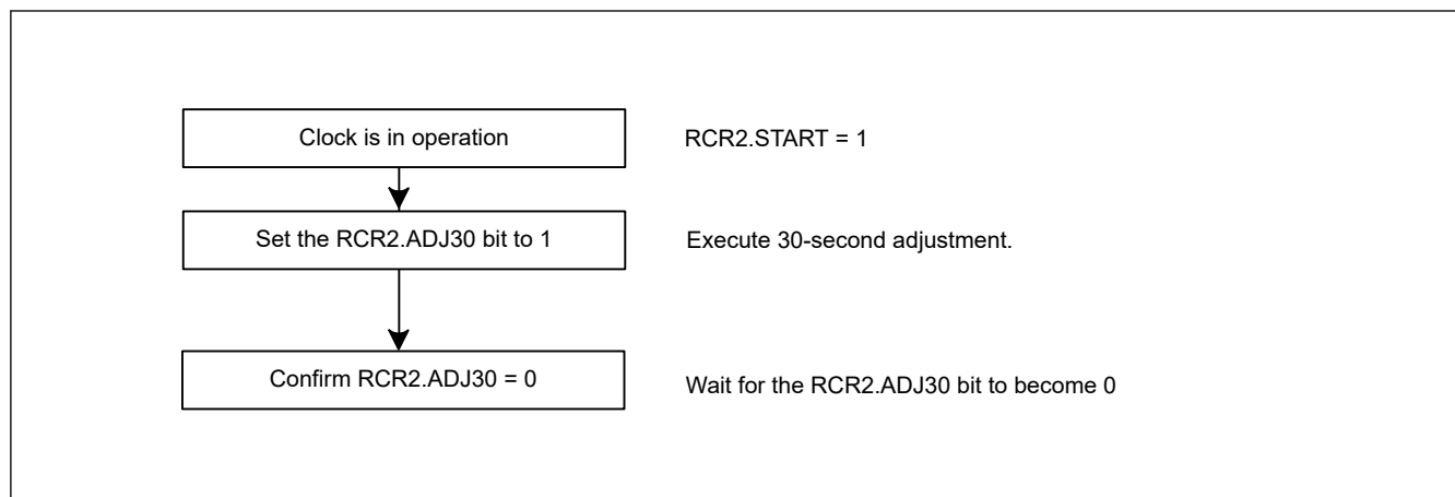
Figure 26.5 30-second adjustment
