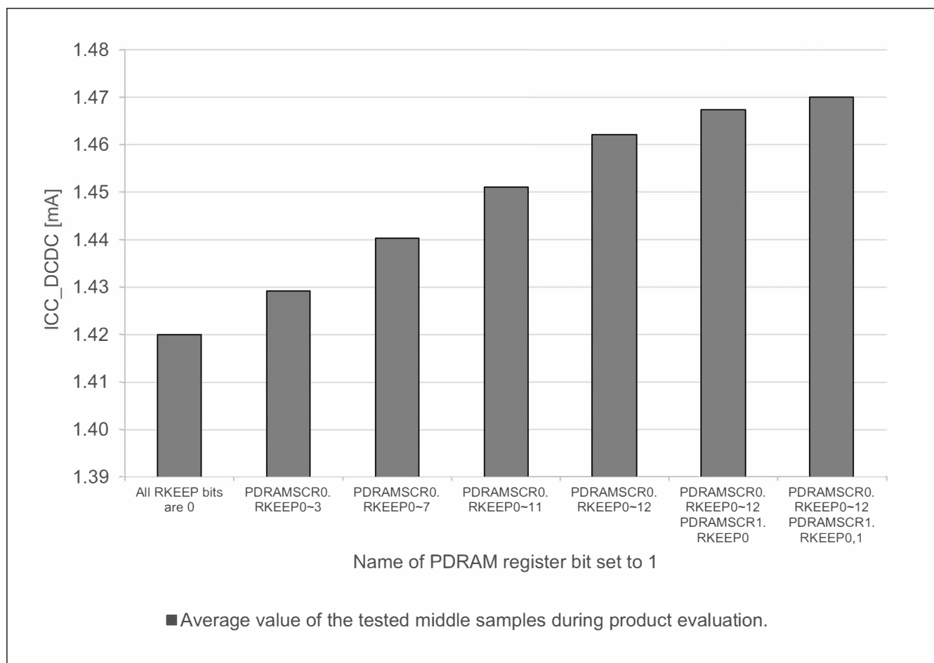
Figure 69.13 Software Standby current per SRAM state (ICC_DCDC, SS2LP_0, SVSCR_4) (reference data)
