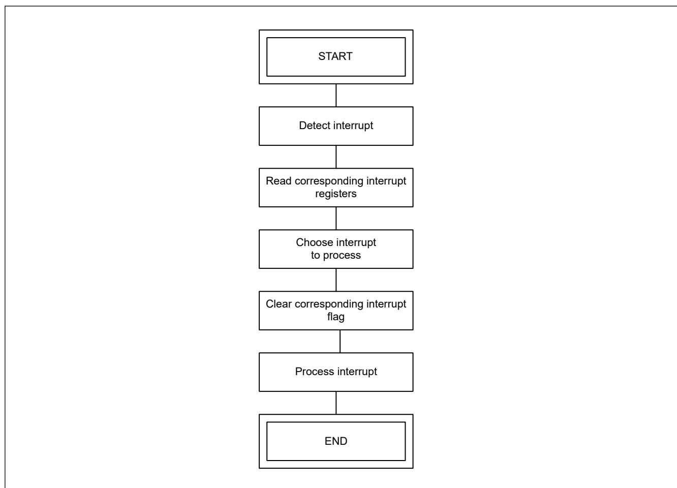
Figure 33.7 Interrupt handling flow
