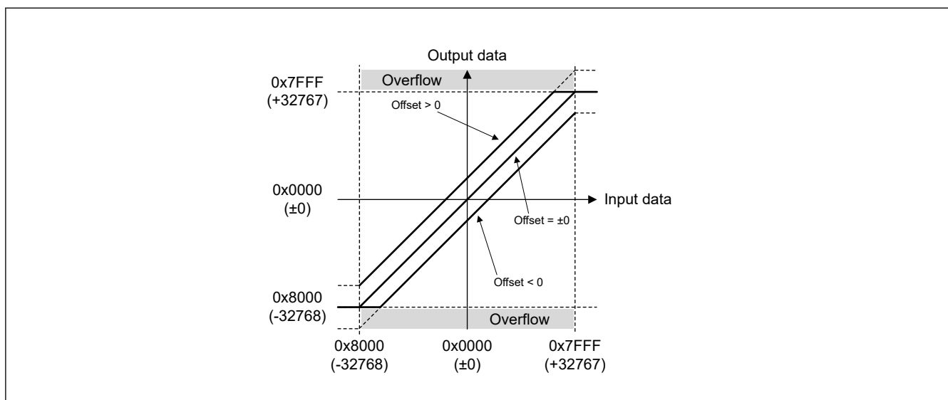
Figure 53.39 User's Offset Adjustment (16-bit data length format and Signed data format)
