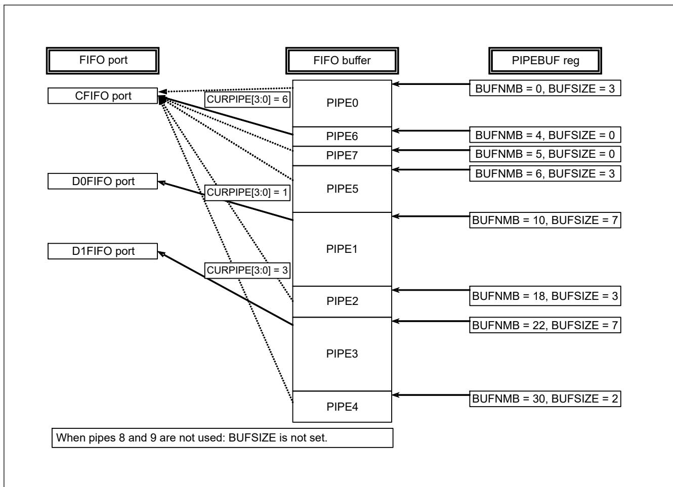
Figure 37.11 Example memory map of the FIFO buffer
