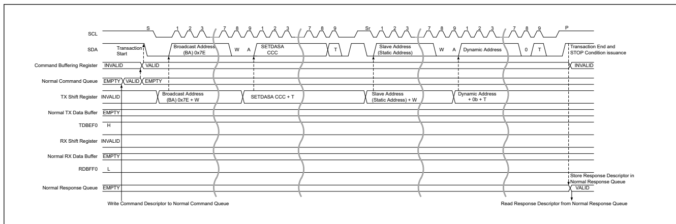
Figure 40.15 Dynamic address assign procedure (SETDASA CCC) timing
