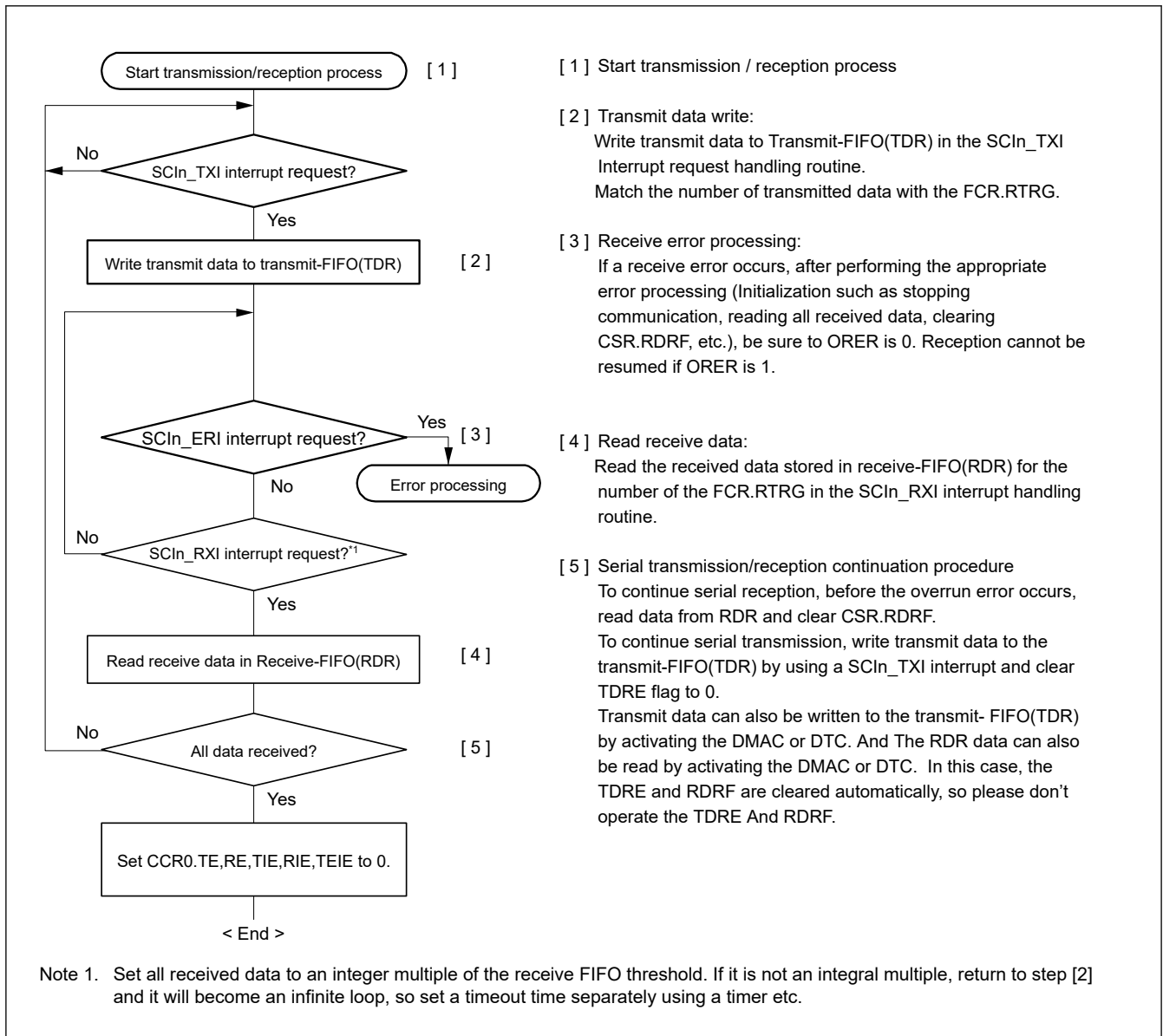
Figure 38.72 Example flow of simultaneous serial transmission and reception in clock synchronous mode with FIFO selected
