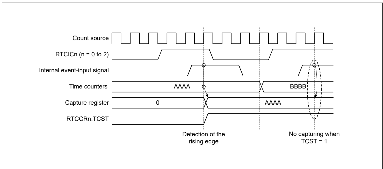
Figure 26.9 Timing of a time capture operation with the noise filter off
