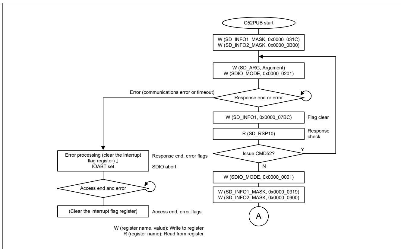
Figure 47.22 Flow when CMD52 (SDIO no abort) is issued during a CMD53 multiple block write
