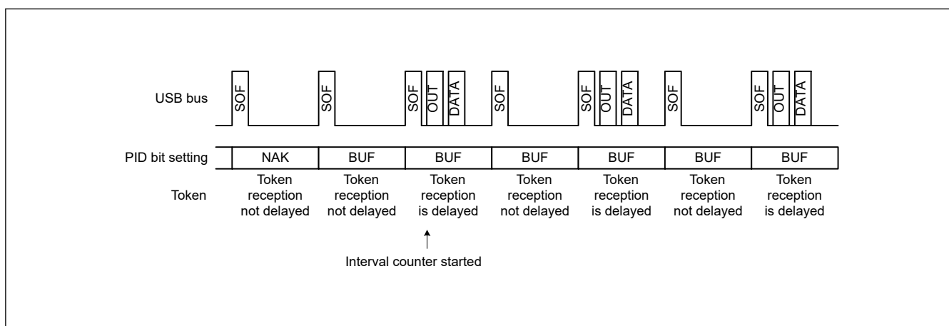
Figure 36.19 Relationship between frames and expected token reception when IITV[2:0] ≠ 0
