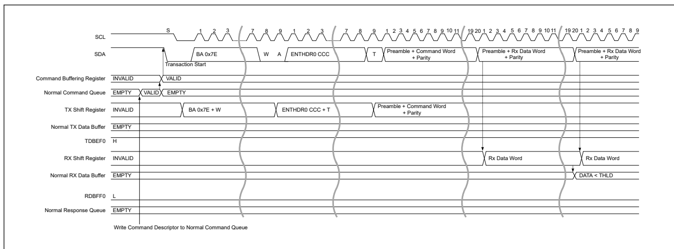
Figure 40.30 HDR data read transfer (HDR-DDR) timing (1/2)
