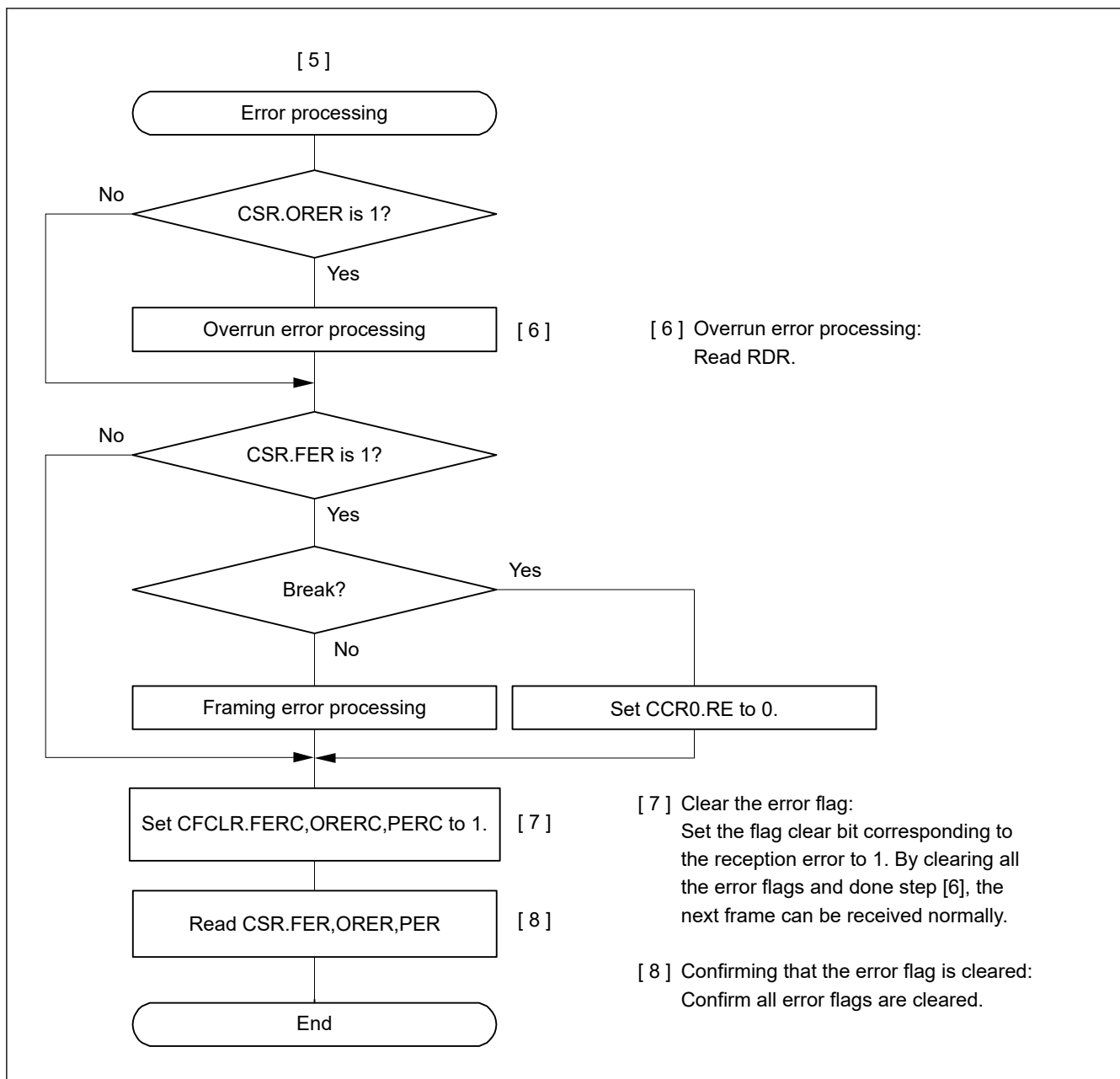
Figure 38.41 Example flow of multi-processor serial reception with non-FIFO selected (2)
