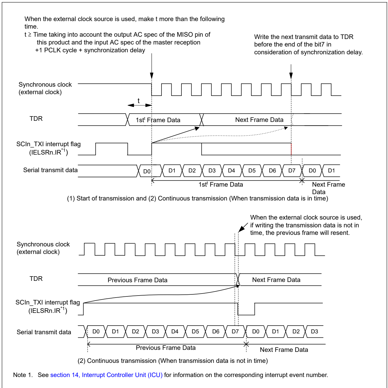
Figure 38.122 Restrictions on Use of External Clock in Clock Synchronous Transmission
