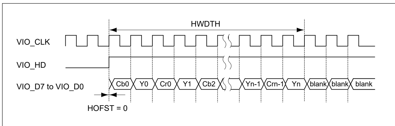
Figure 60.22 Horizontal capture timing (image capture with 8-bit interface)
