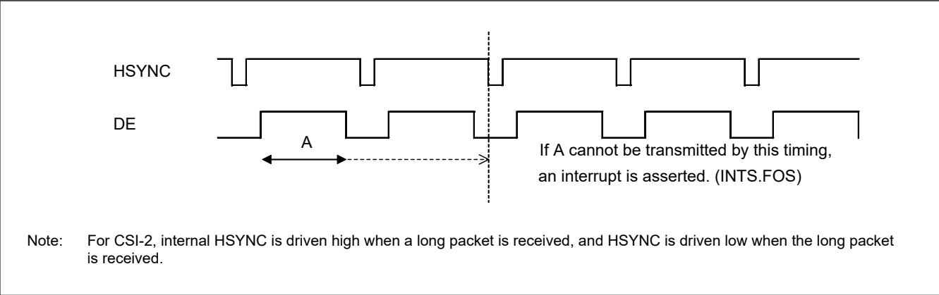
Figure 67.16 Overflow
