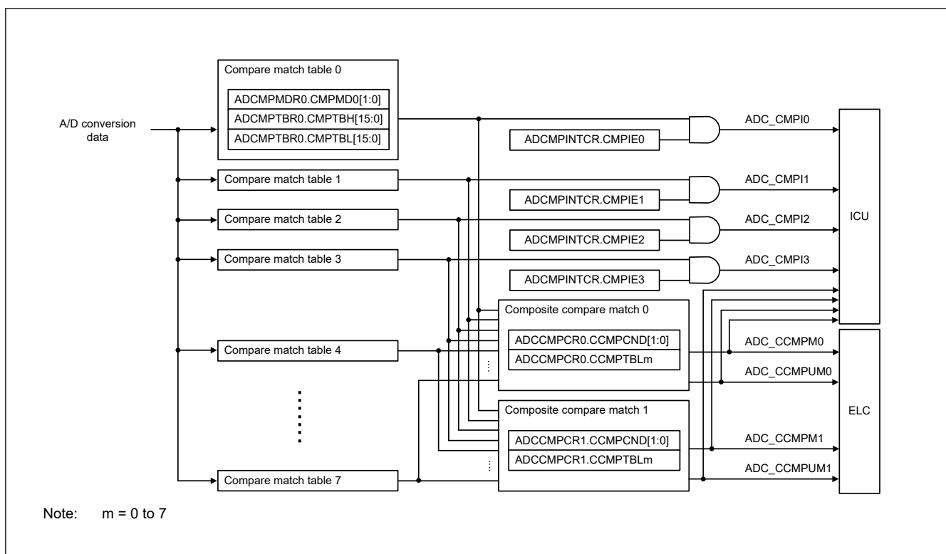
Figure 53.52 Relationship between composite compare match function and compare match function
