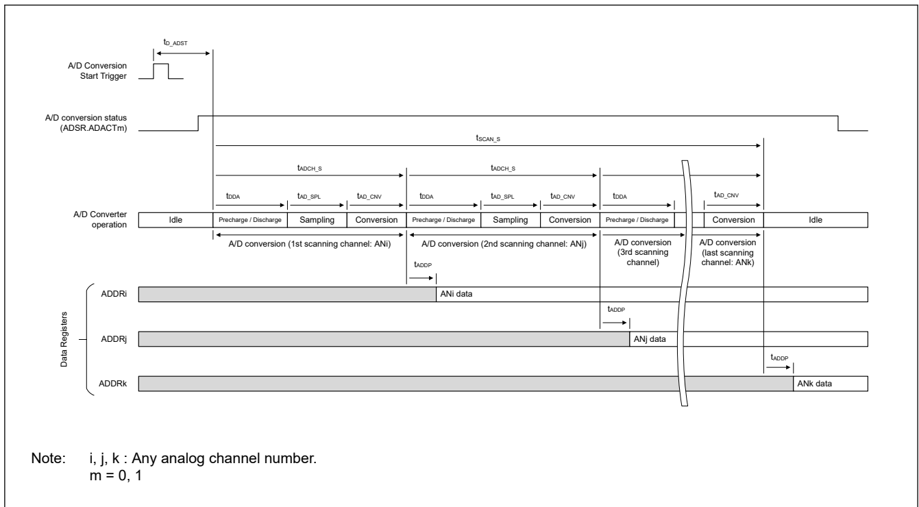
Figure 53.57 A/D conversion processing time (SAR mode)
