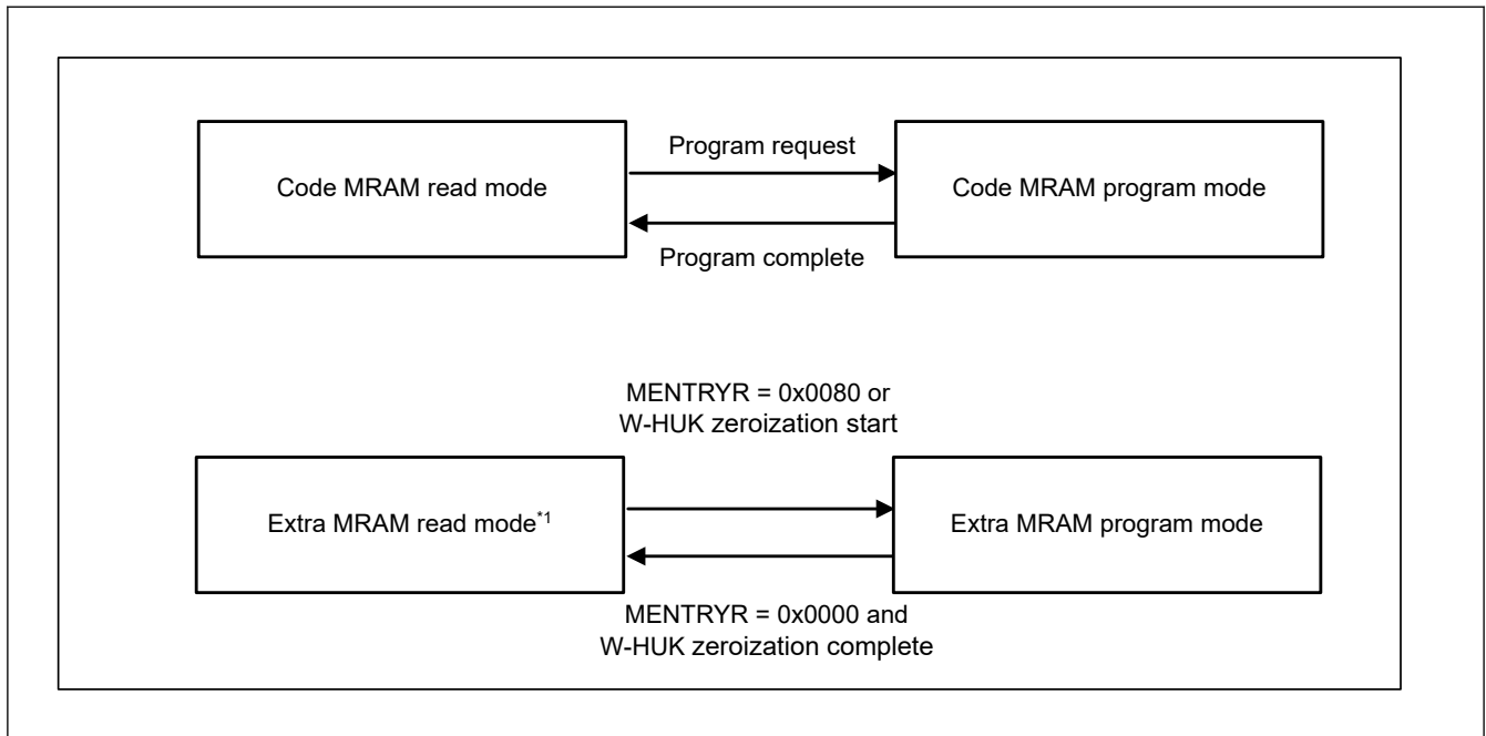
Figure 59.7 MRAM read/program mode transition
