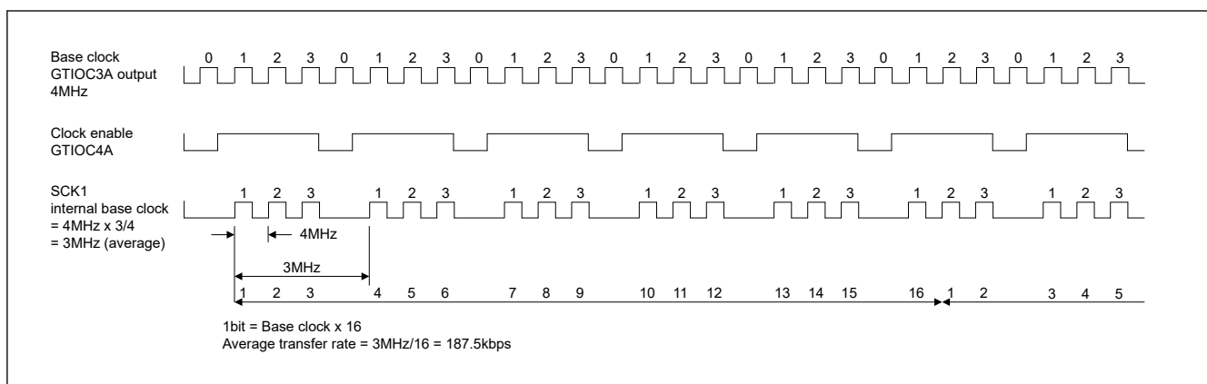
Figure 38.5 Example of average transfer rate setting when GPT clock is input
