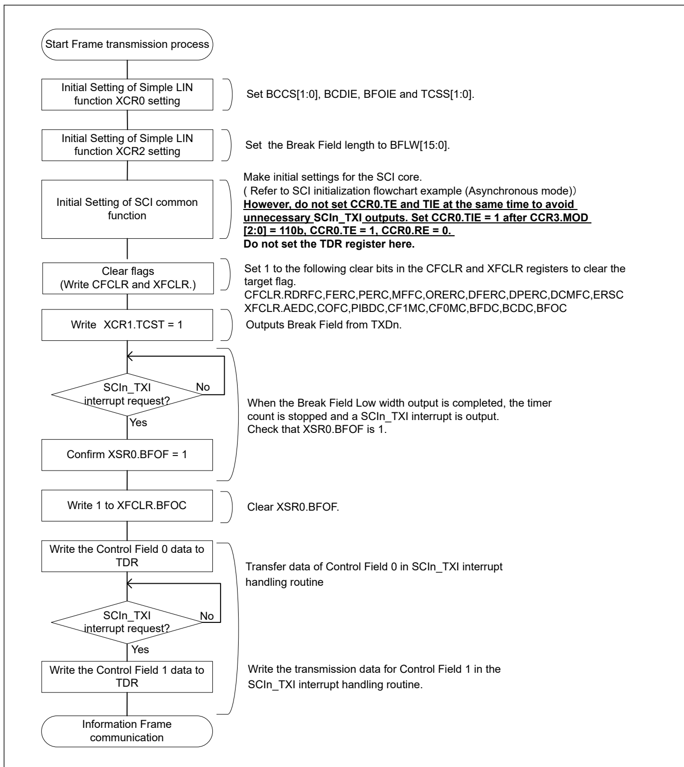
Figure 38.103 Start Frame Transmission Flowchart Example
