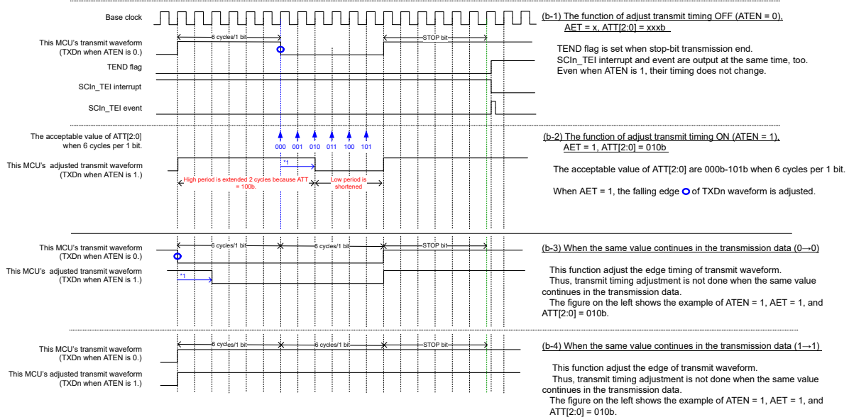
Figure 38.34 The adjustment operation explanation for the transmit timing when AET is 1
