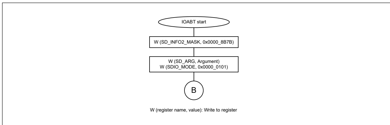
Figure 47.21 Flow when CMD52 (SDIO Abort) is issued during a CMD53 multiple block write
