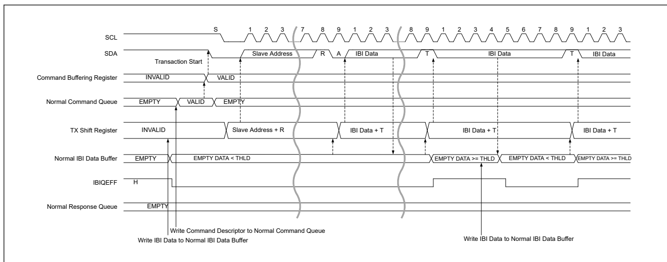
Figure 40.63 I3C slave IBI transfer timing (1/2)
