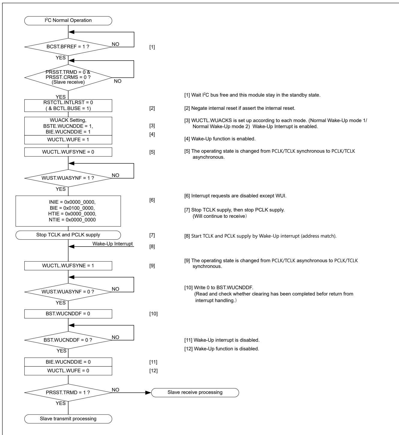
Figure 40.126 Use case of normal WU mode 1 (wake-up recovery by a wake-up interrupt triggered by the match of the slave address)
