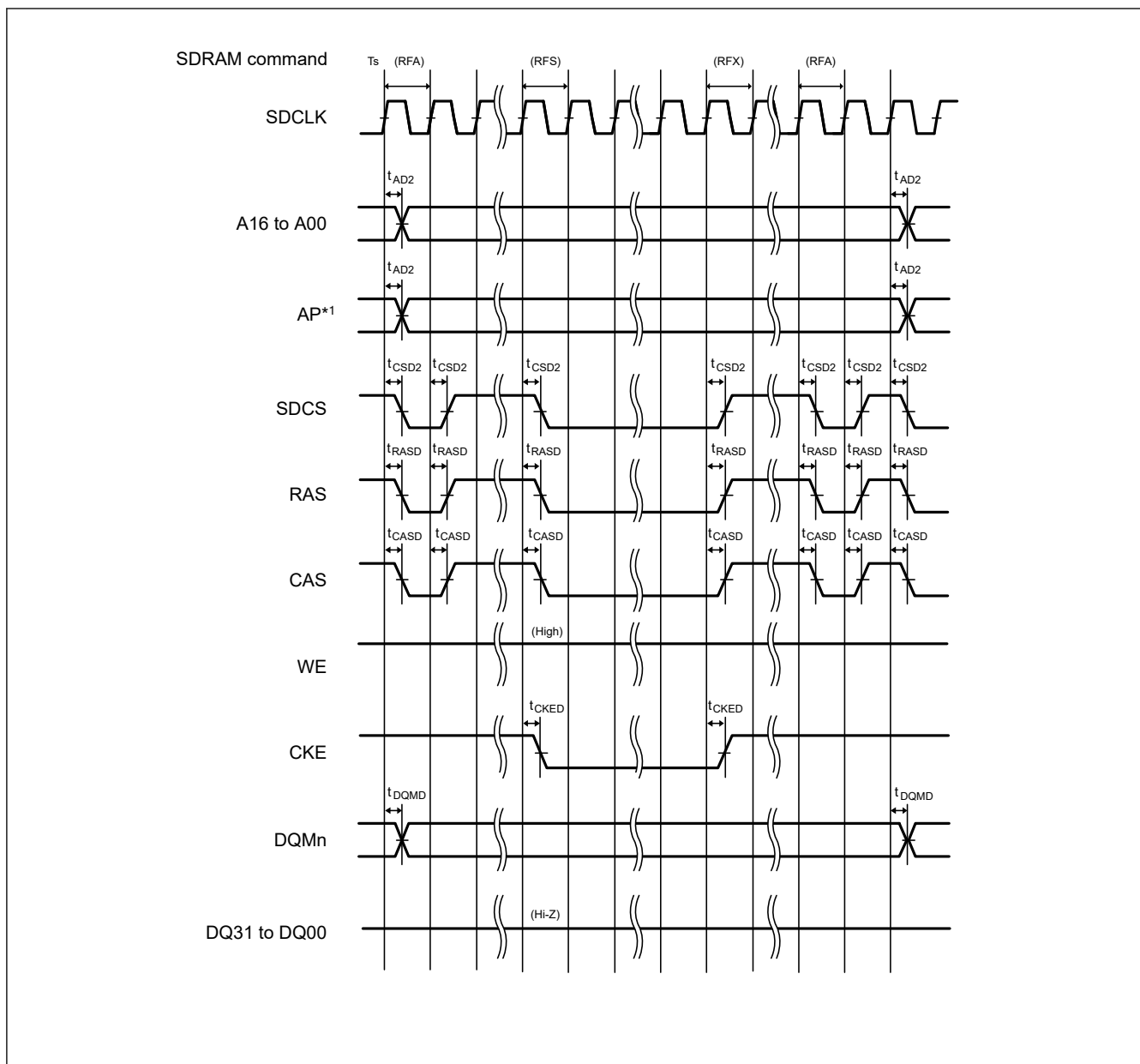
Figure 69.51 SDRAM self-refresh timing
