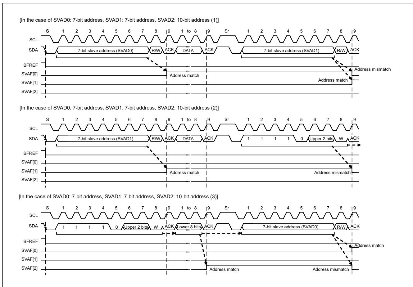
Figure 40.84 SVAFy flag set/clear timing with 7-bit/10-bit address formats mixed
