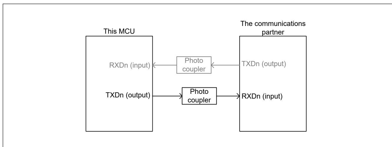
Figure 38.30 block diagram image of the transmission through a photo coupler
