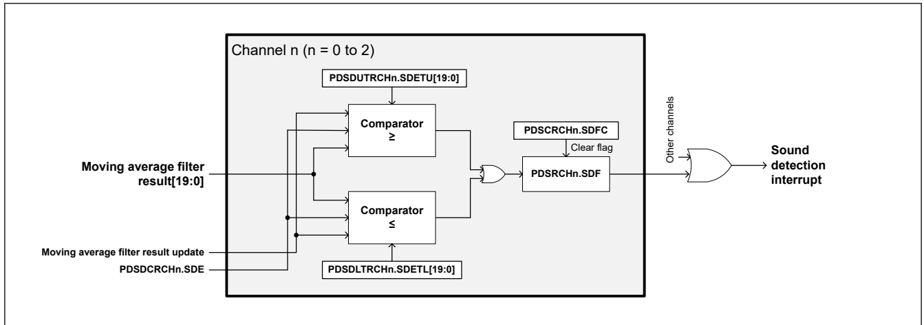
Figure 49.10 Sound detection function
