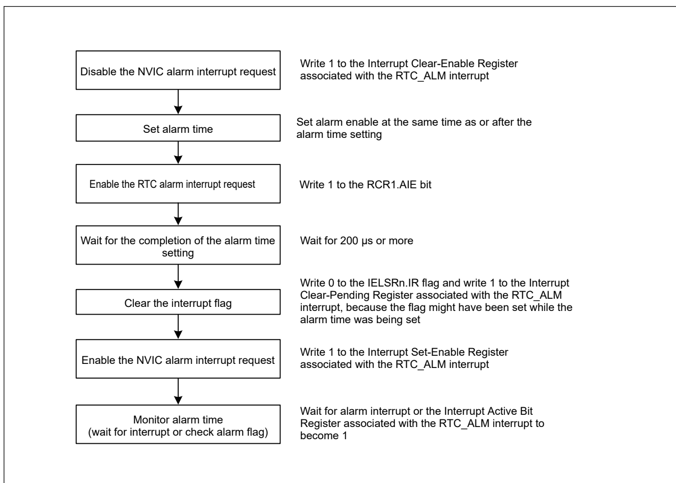
Figure 26.7 Using the alarm function
