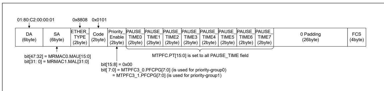
Figure 33.18 PFC frame Format
