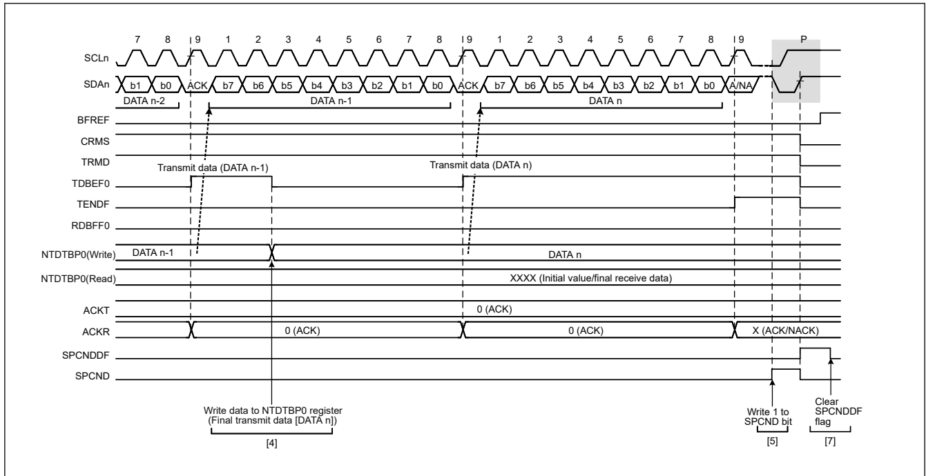
Figure 40.8 Master transmit operation timing (3)
