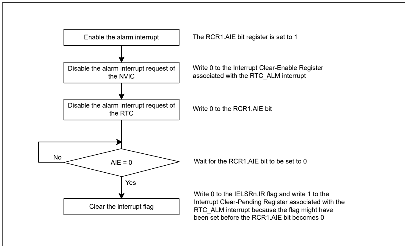
Figure 26.8 Procedure for disabling alarm interrupt request
