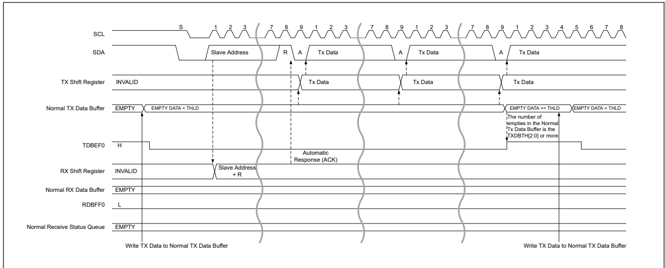
Figure 40.51 Legacy I 2 C message data read transfer timing (1/2)
