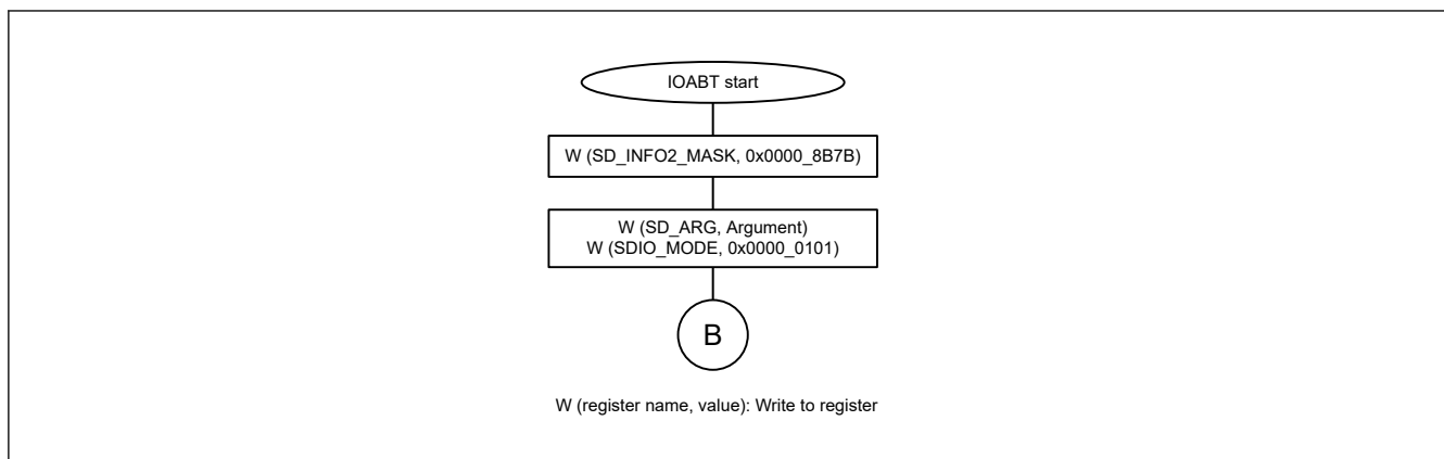
Figure 47.18 Flow when CMD52 (SDIO abort) is issued during a CMD53 multiple block read
