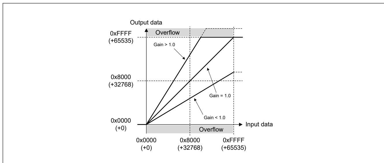
Figure 53.36 User's Gain Adjustment (16-bit data length format and Unsigned data format)
