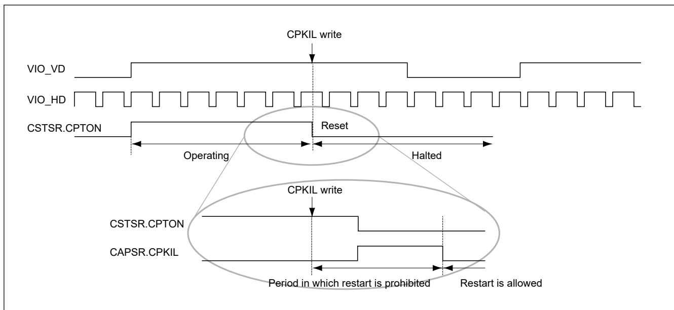
Figure 60.6 Timing of software reset and restart of capturing
