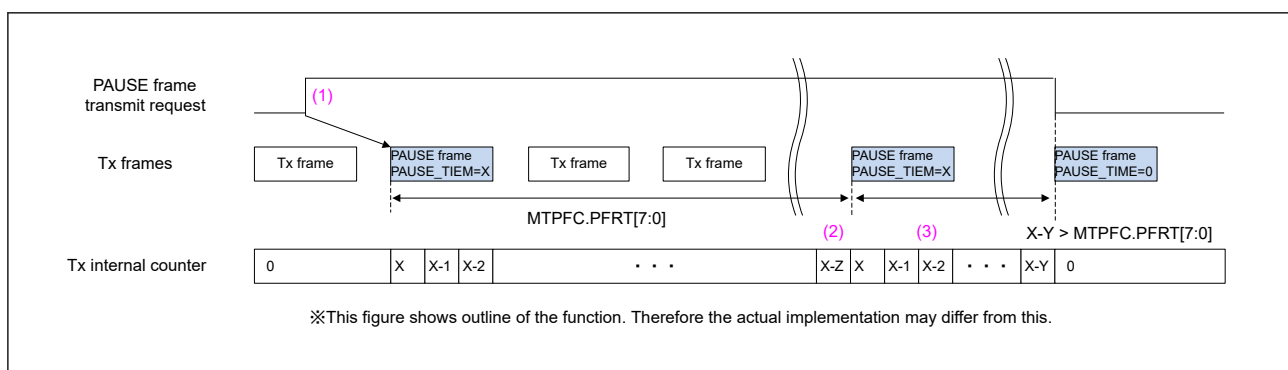
Figure 33.16 Transmission of PAUSE frame
