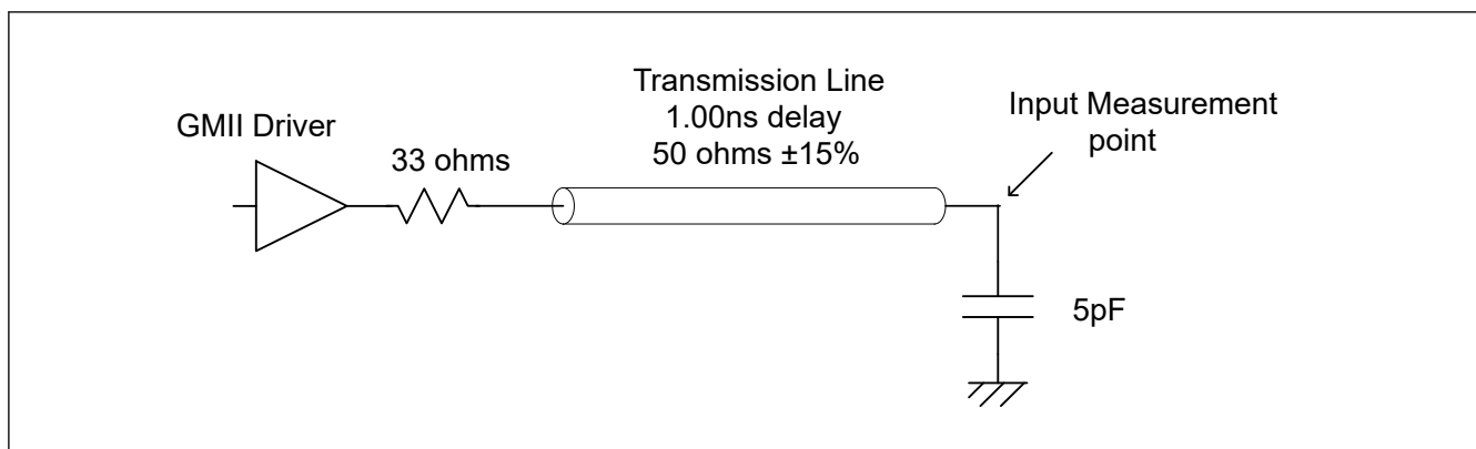
Figure 69.119 GMII output timing measurement conditions
