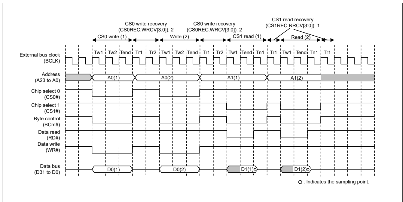
Figure 15.31 Example recovery cycle insertion when bus access is split, with separate bus interface and normal access ( m = 0 to 3)
