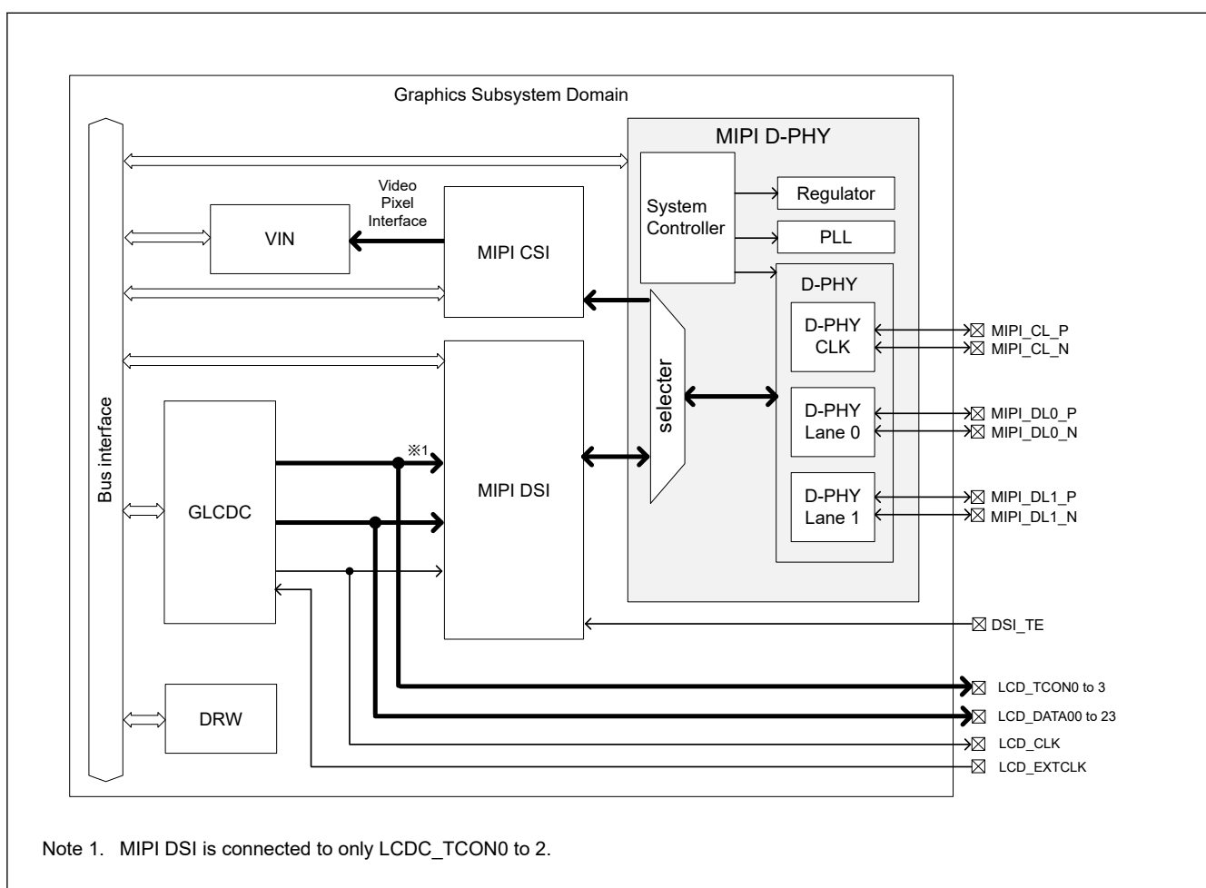
Figure 61.1 Graphics domain block diagram
