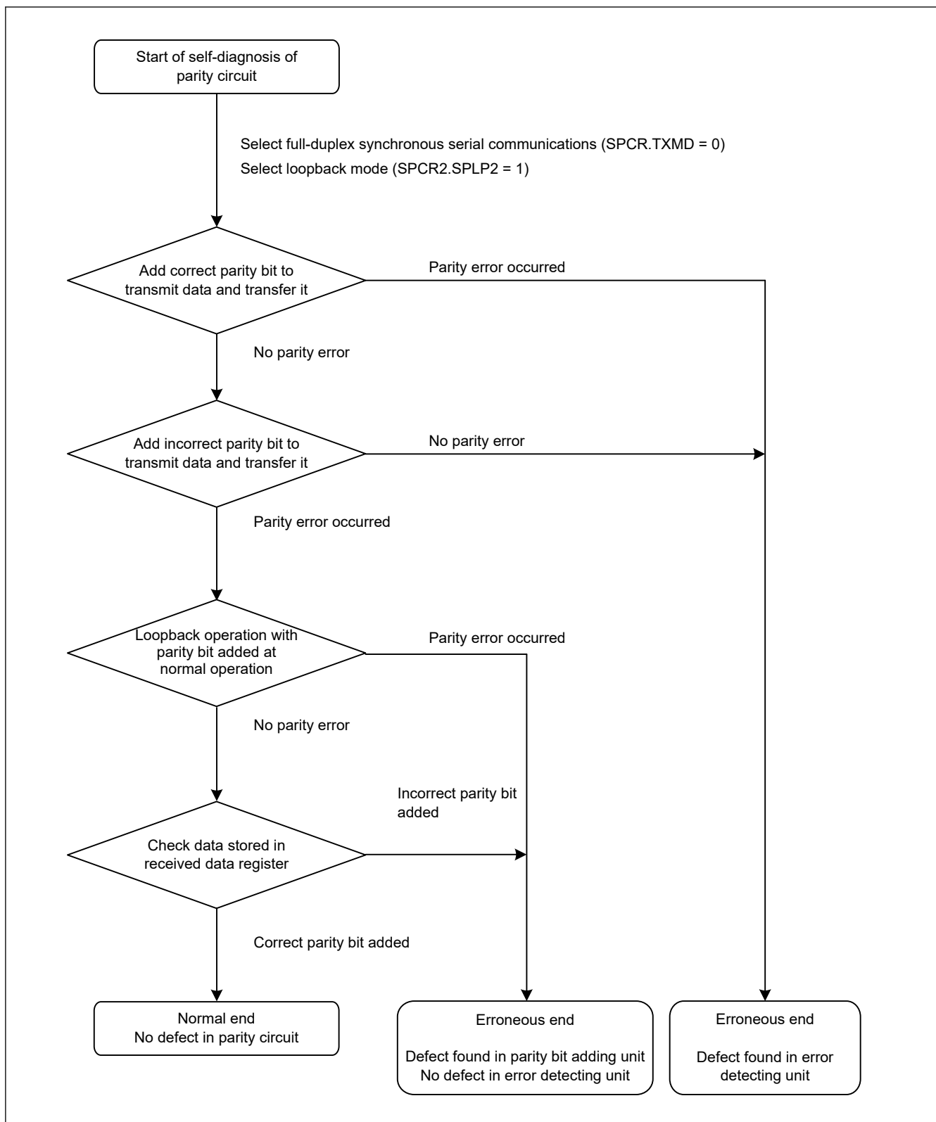
Figure 43.79 Self-diagnosis flow for parity circuit
