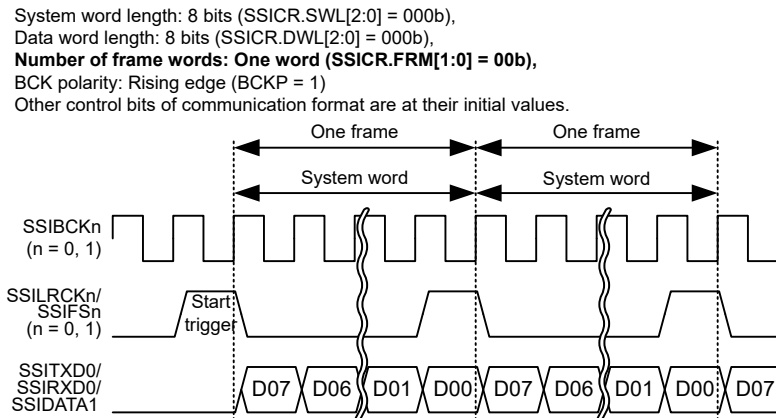
Figure 46.38 Short frame in monaural format (without padding: system word length = data word length)
