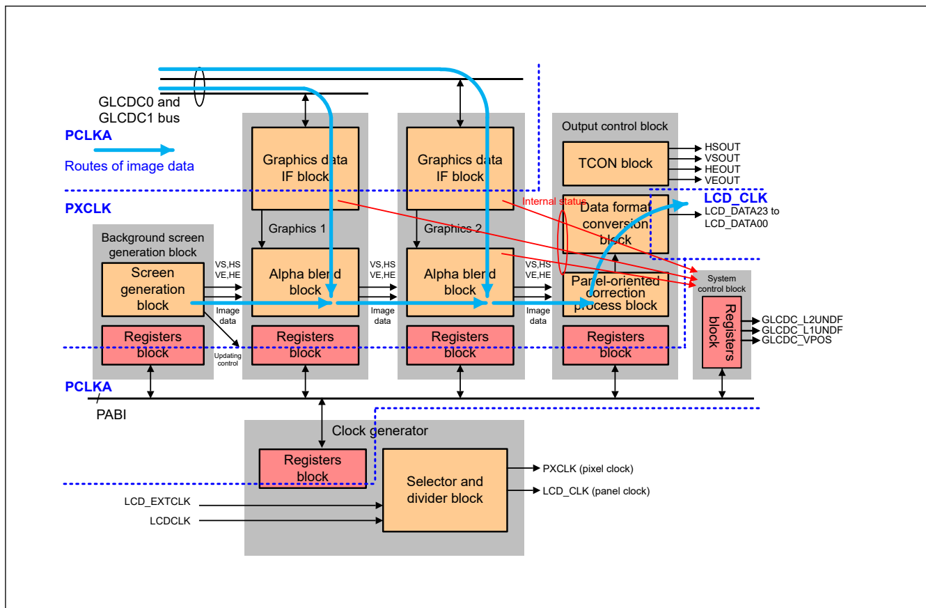
Figure 63.22 GLCDC configuration
