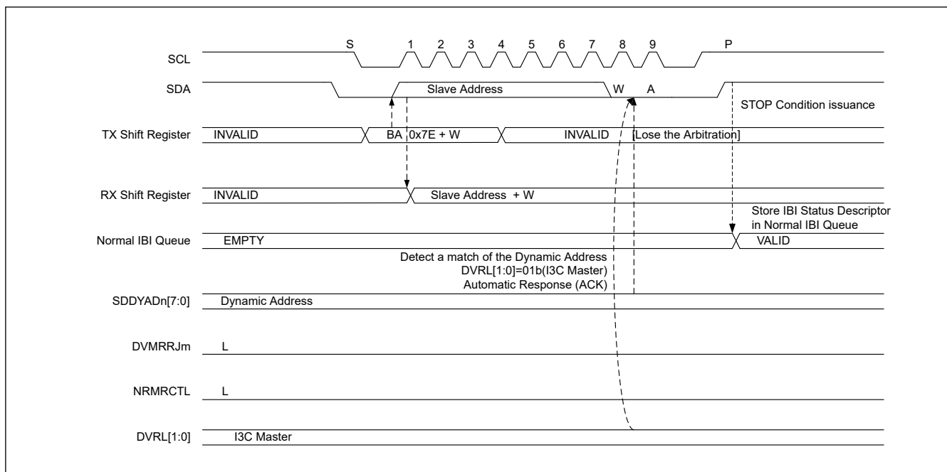
Figure 40.105 Mastership request : ACK
