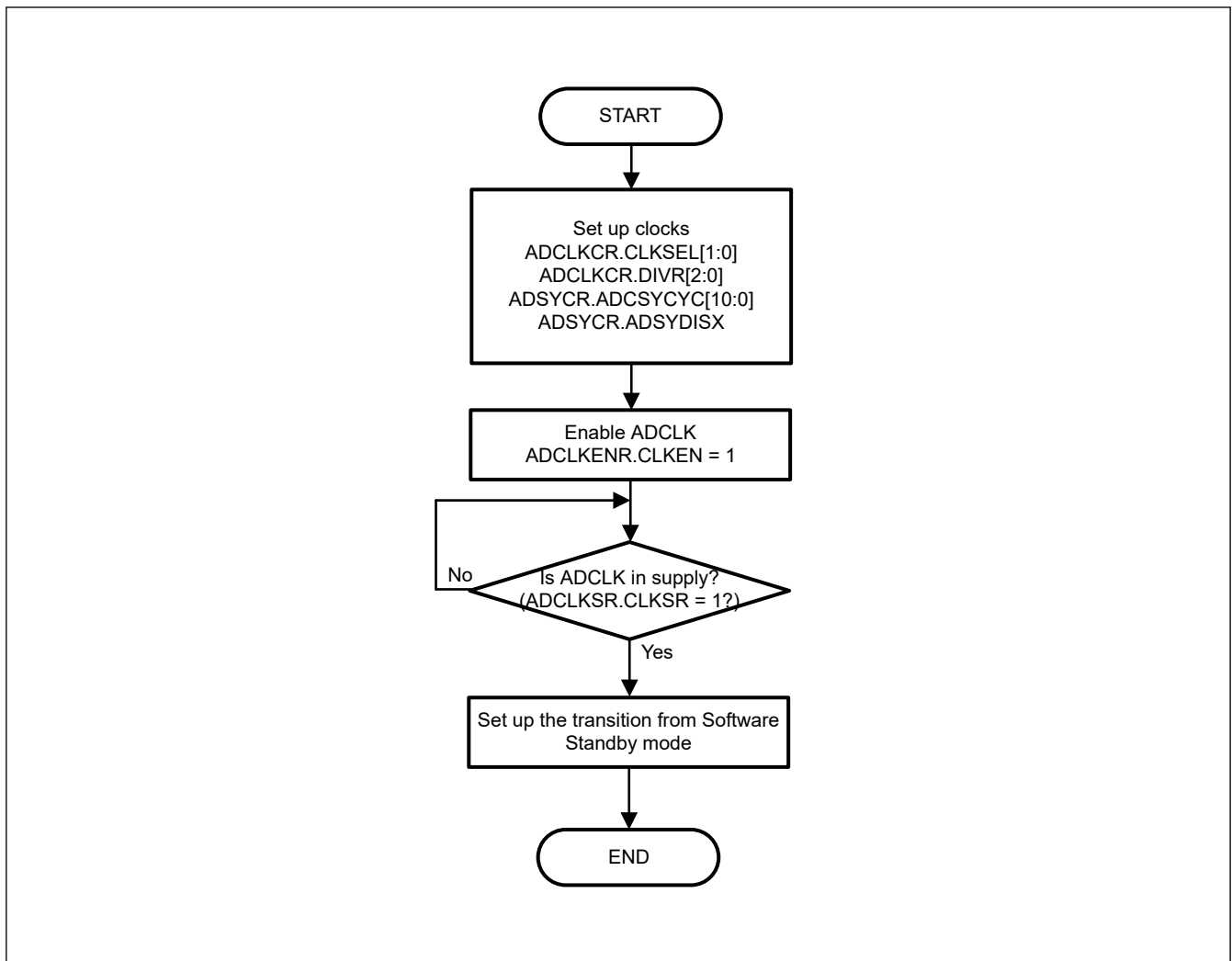
Figure 53.65 Example procedure for resuming Software Standby mode
