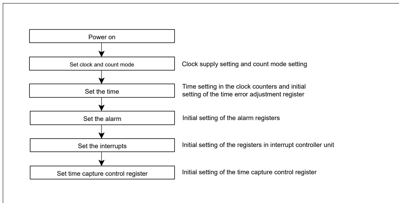
Figure 26.2 Outline of initial settings after a power on
