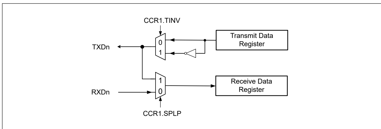
Figure 38.115 Shift register input output configuration image in loopback mode
