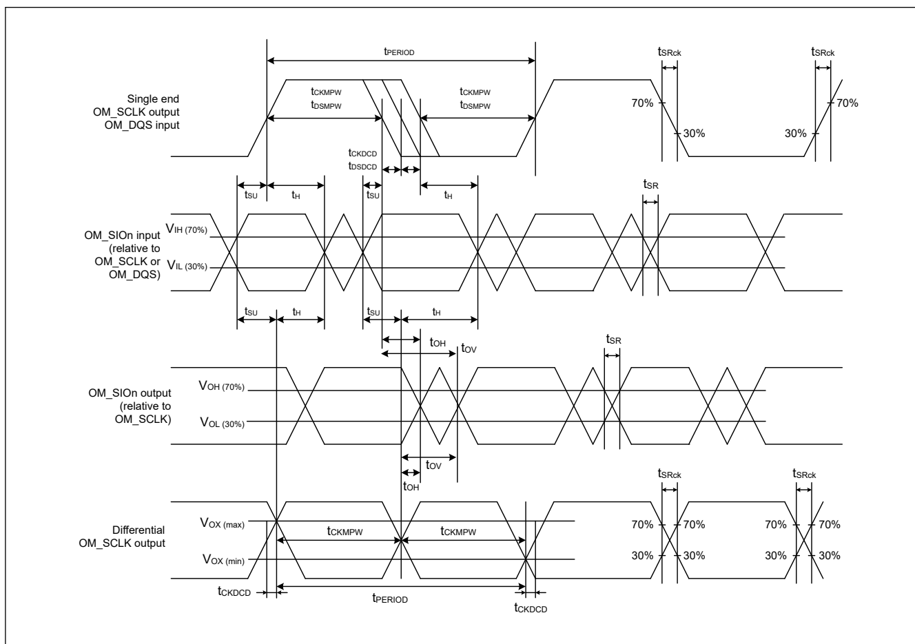
Figure 69.83 OSPI clock / DS timing
