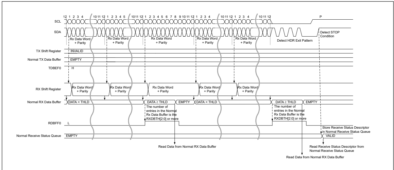
Figure 40.57 HDR data write transfer (HDR-TSP, TSL) timing (2/2)
