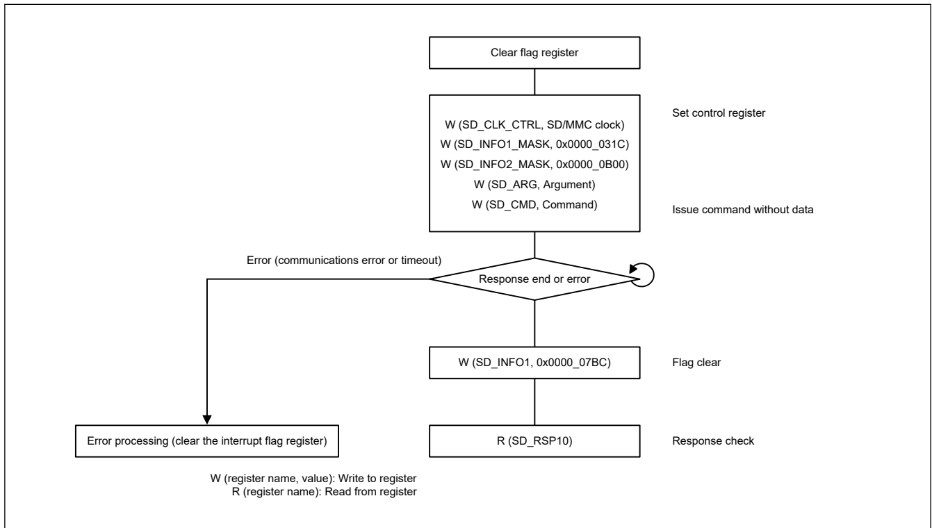
Figure 47.10 Example flow of command without data
