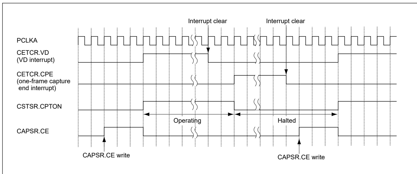
Figure 60.47 Operating status during capturing
