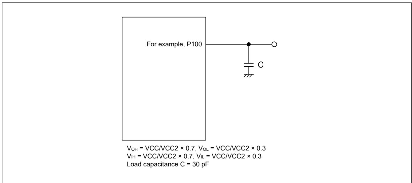
Figure 69.1 Input or output timing measurement conditions
