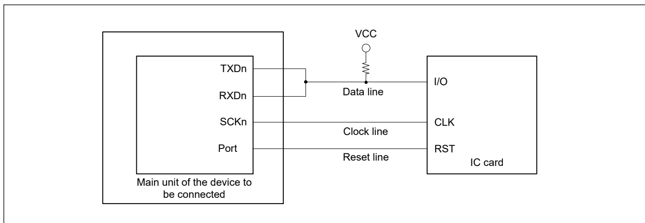
Figure 38.74 Example connection with a smart card (IC card)
