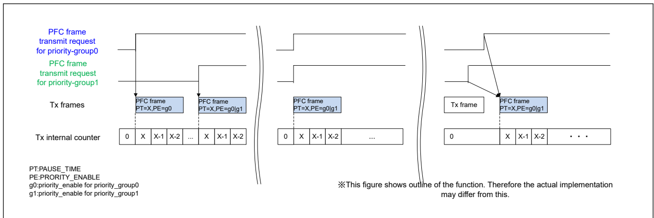
Figure 33.19 Transmitting PFC frame (part 1)
