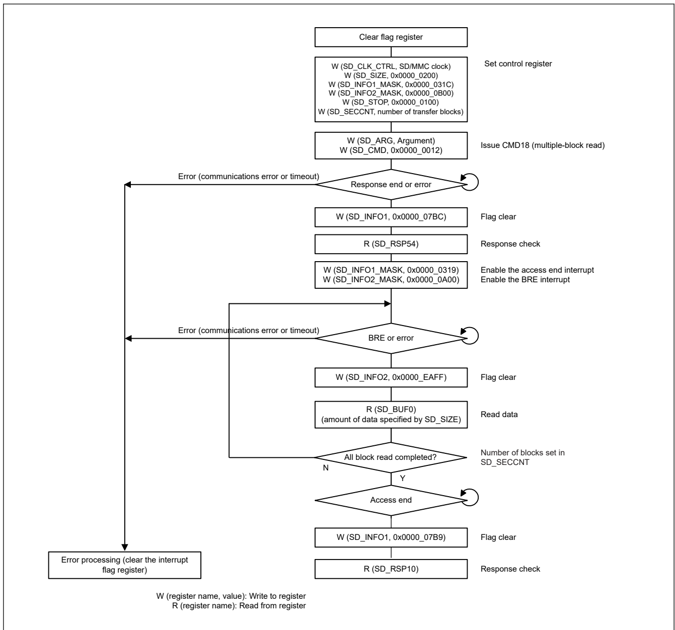
Figure 47.13 Example of multiple block read operation
