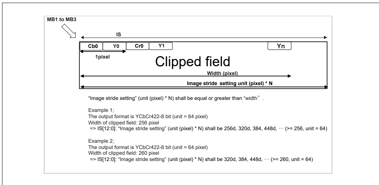
Figure 67.2 Image stride setting example memory base 1 register (MB1)
