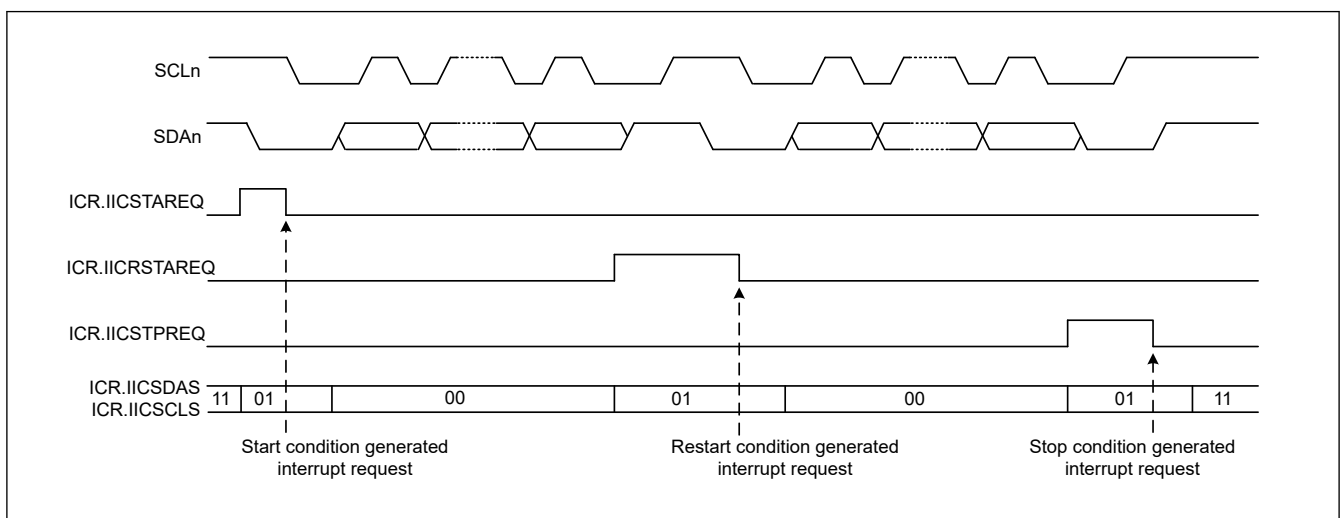
Figure 38.88 Timing of operations in generation of start, restart, and stop conditions
