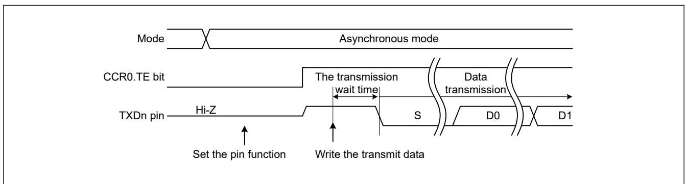
Figure 38.11 Data transmission timing example in Asynchronous mode
