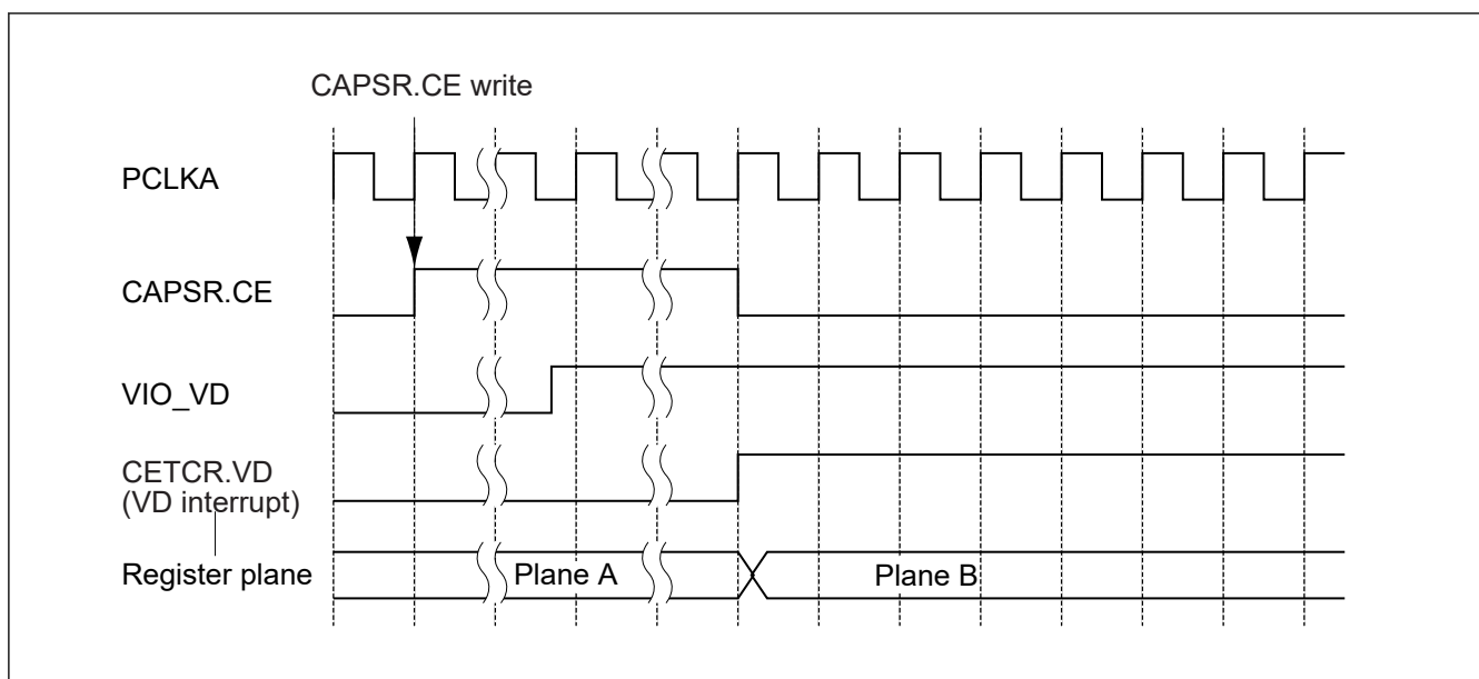
Figure 60.2 Register plane switching timing (VD polarity is high-active in data enable fetch mode)
