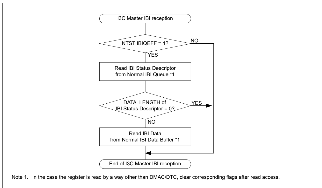
Figure 40.150 Example of I3C master IBI reception flowchart
