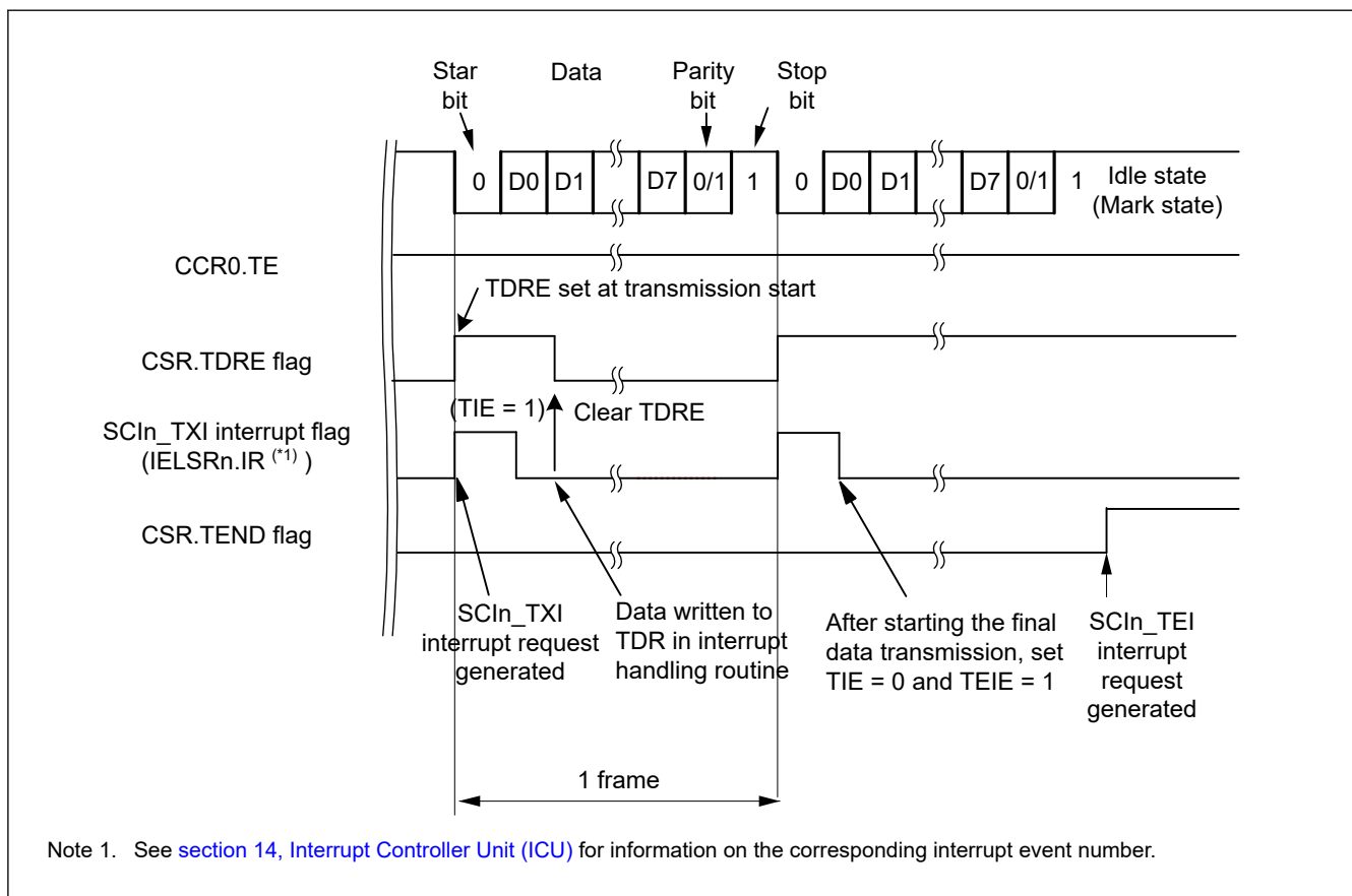
Figure 38.14 Example operation for serial transmission in Asynchronous mode (3) with 8-bit data, parity bit, one stop bit, CTS function not used, and from the middle of transmission until transmission completion
