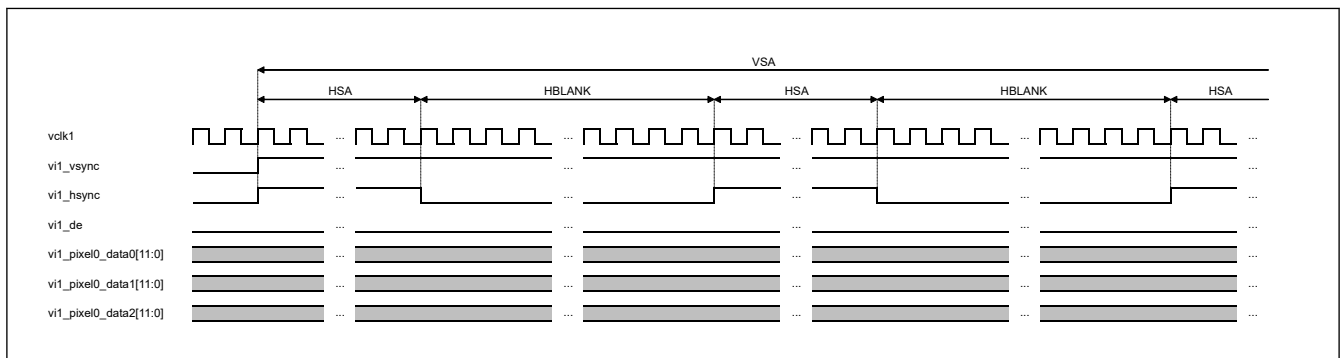
Figure 65.10 VSA start (and VFP end)
