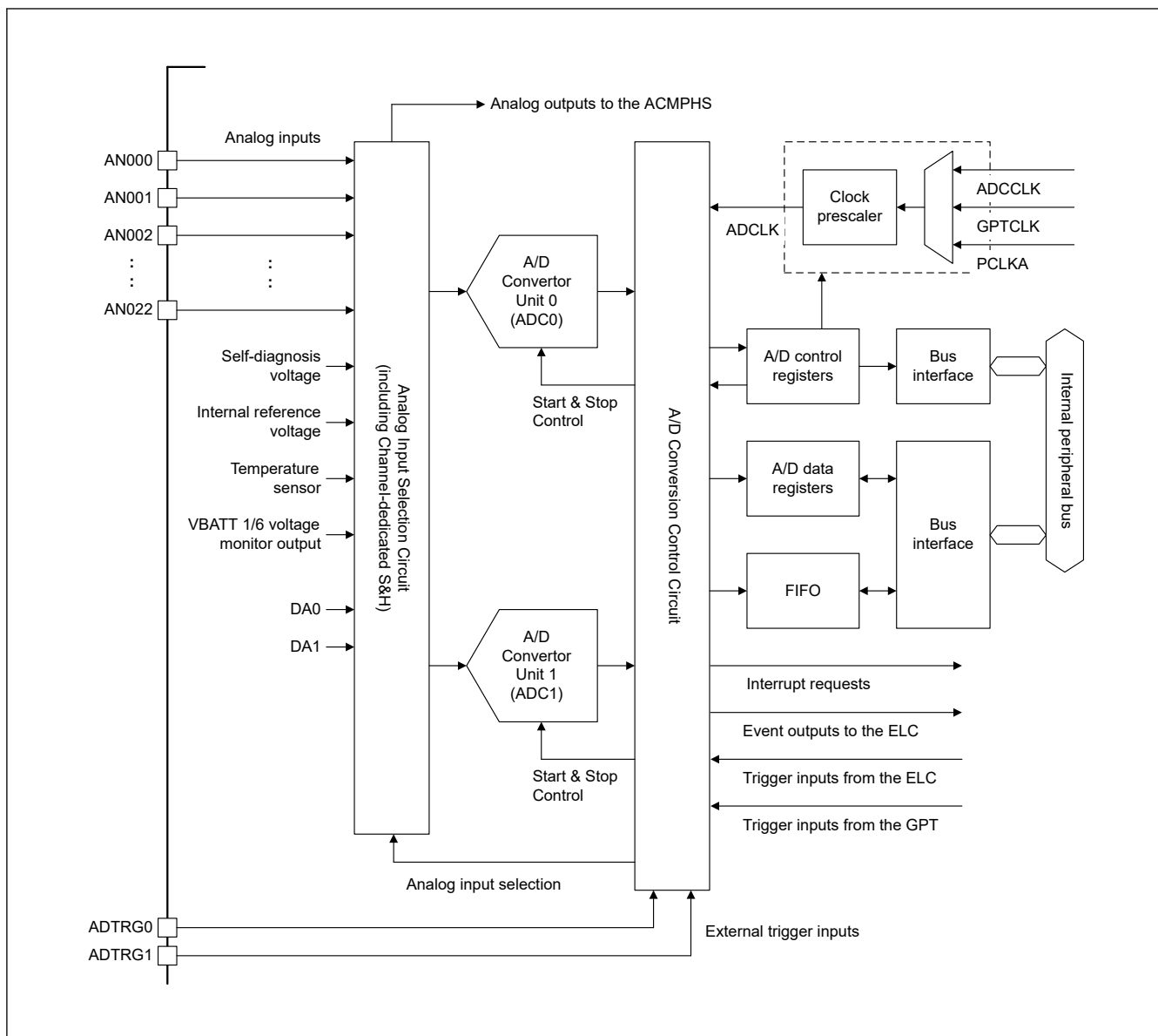
Figure 53.1 Block diagram of ADC16H
