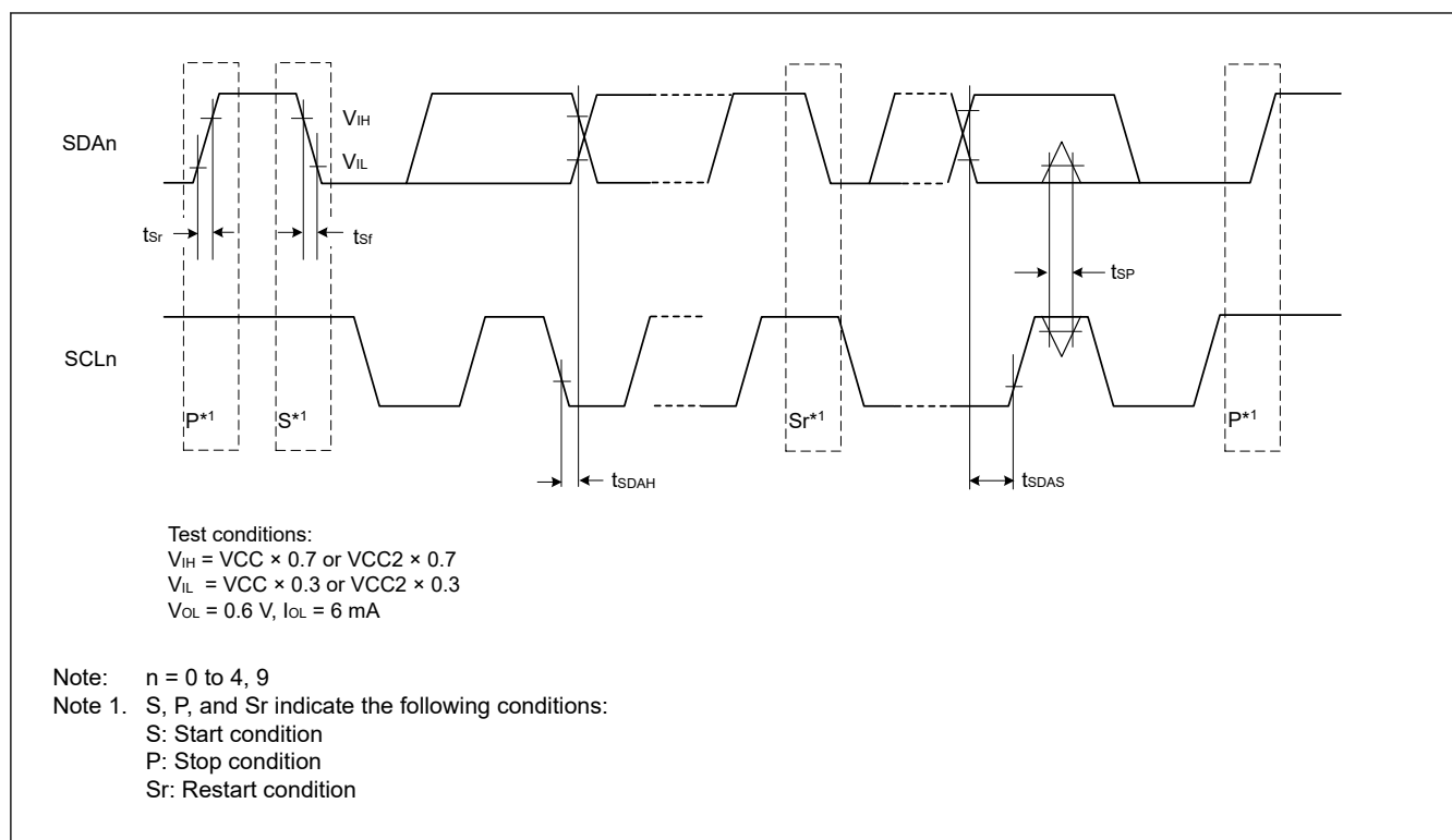
Figure 69.74 SCI simple IIC mode timing
