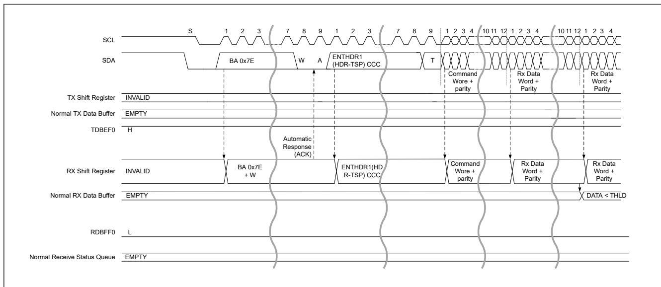
Figure 40.56 HDR data write transfer (HDR-TSP, TSL) timing (1/2)
