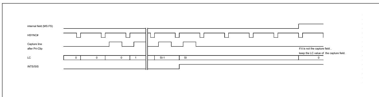
Figure 67.3 Scanline interrupt status generation timing
