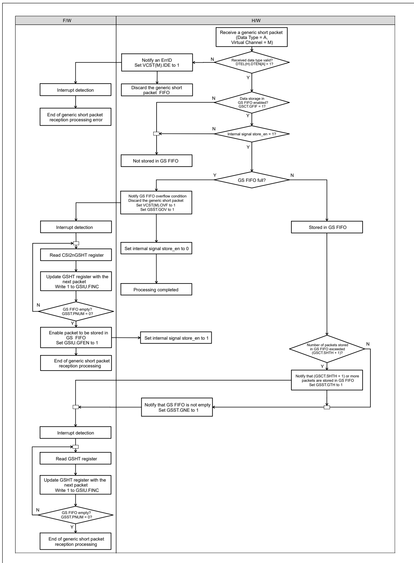
Figure 66.4 Generic short packet receive processing
