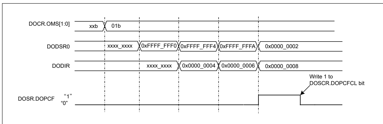
Figure 57.8 Example of Operation in Data Addition Mode
