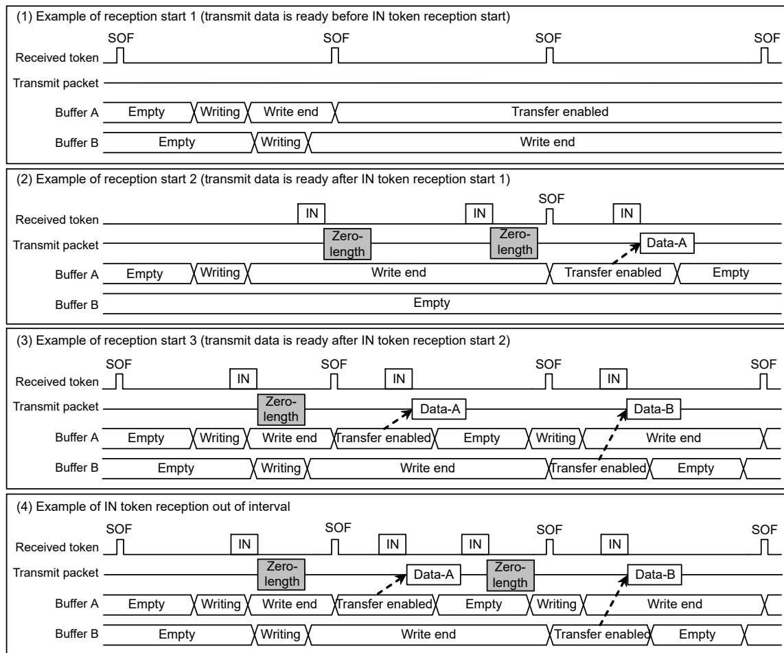
Figure 37.16 Example data setup operation
