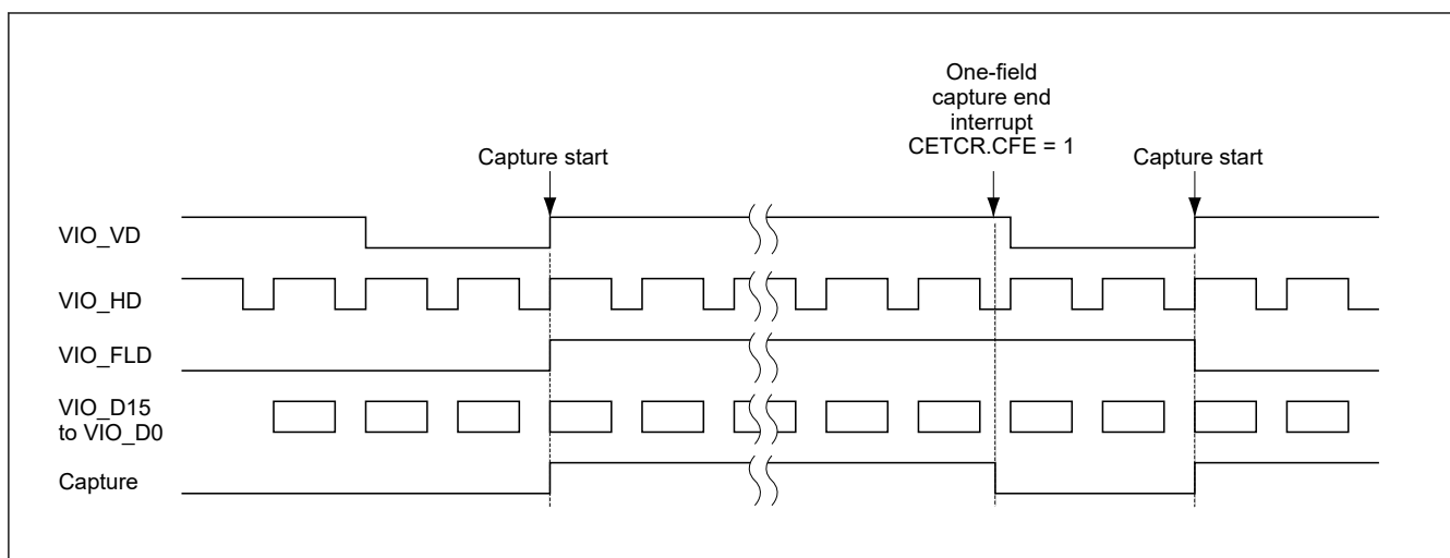
Figure 60.45 CFE generation timing
