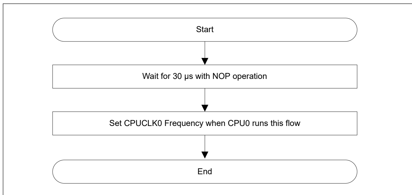
Figure 11.12 Additional flow for the return from Software Standby mode (assuming that CPUCLK0 and ICLK are the same frequency when returning)
