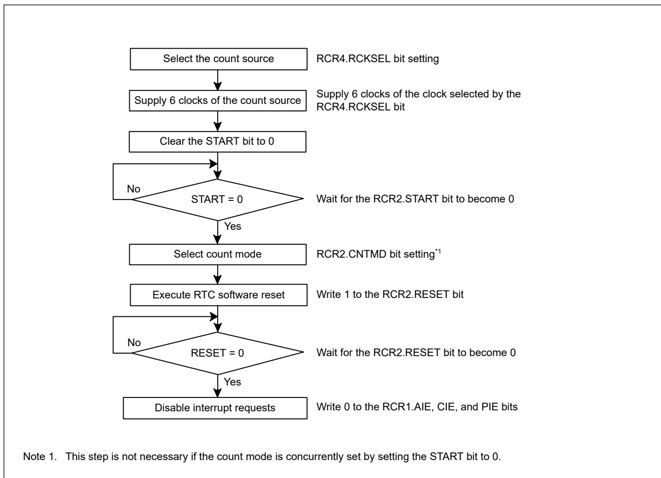
Figure 26.14 Initialization procedure
