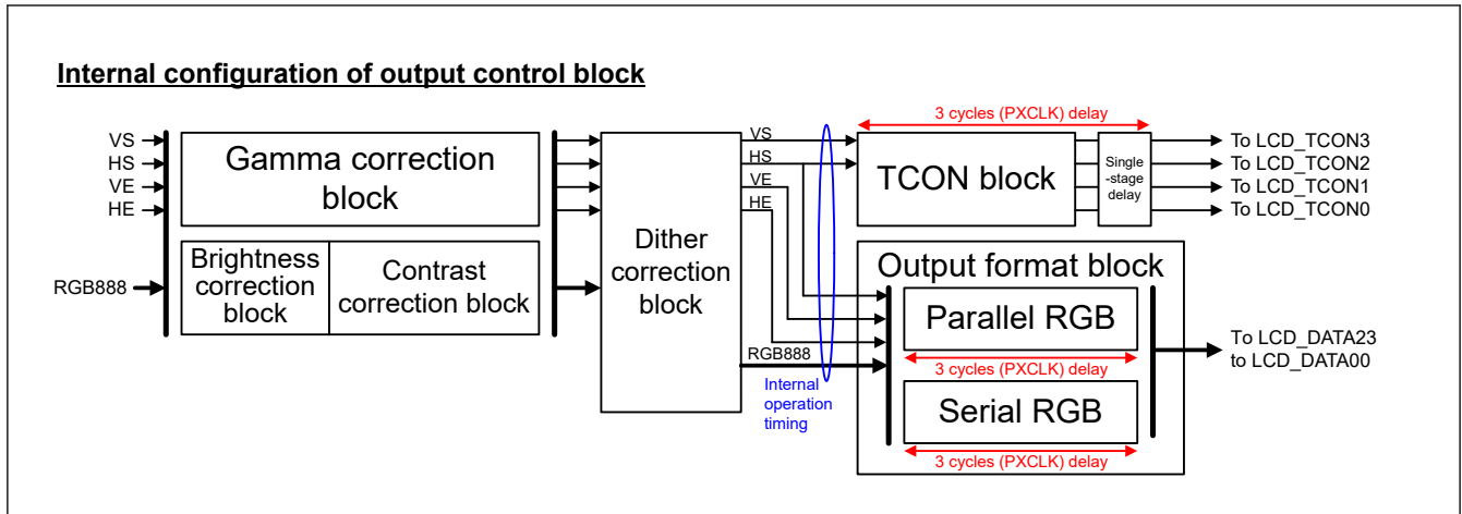
Figure 63.17 Internal configuration of output control block
