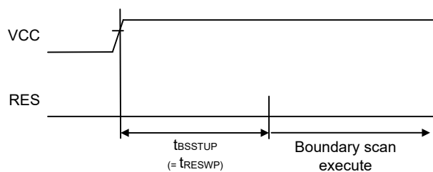
Figure 69.155 Boundary scan circuit startup timing
