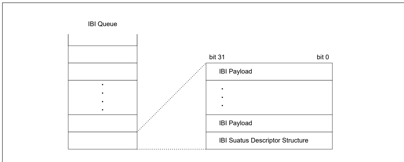
Figure 40.4 IBI status descriptor data structure
