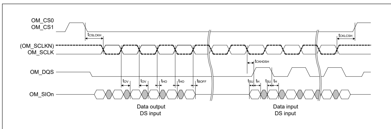
Figure 69.85 DDR transmit/receive timing (4S-4D-4D, 8D-8D-8D)
