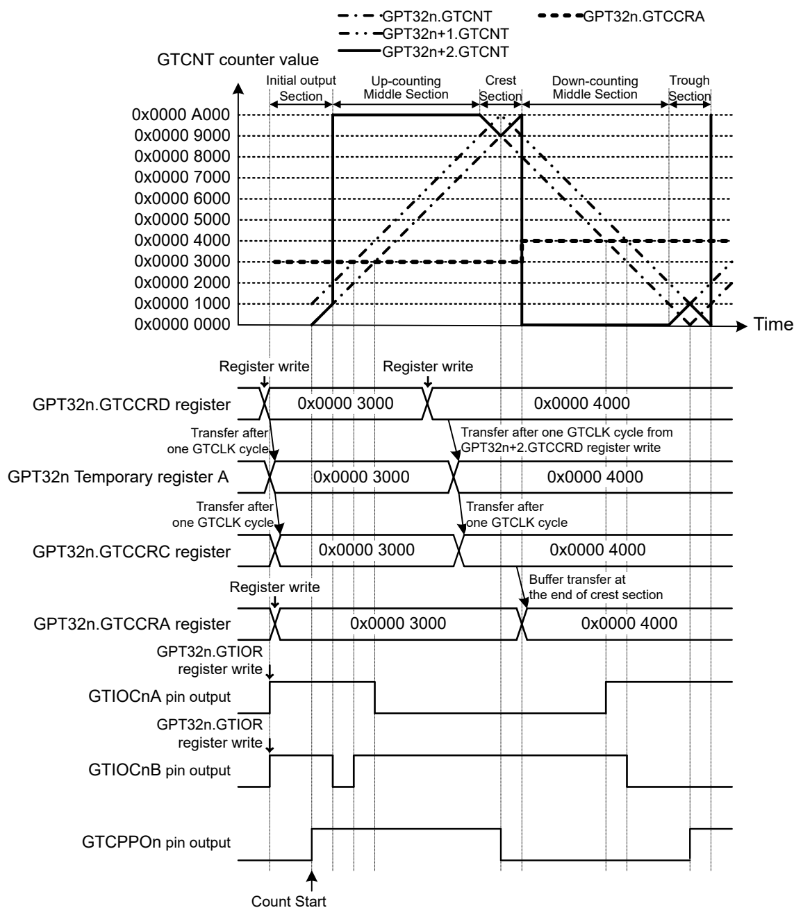
Figure 22.65 Example of Complementary PWM Mode Initial Output Operation (Complementary PWM mode 1 operation, GTIOCnA pin = Low / GTIOCnB pin = High at GTCCRA register compare match during up-counting, GTIOCnA pin = High / GTIOCnB pin = Low at GTCCRA register compare match during down-counting, the dead time value is 0x0000 1000, in the case that the initial GTCCRA register value is larger than the dead time value) (n = 4, 7)
