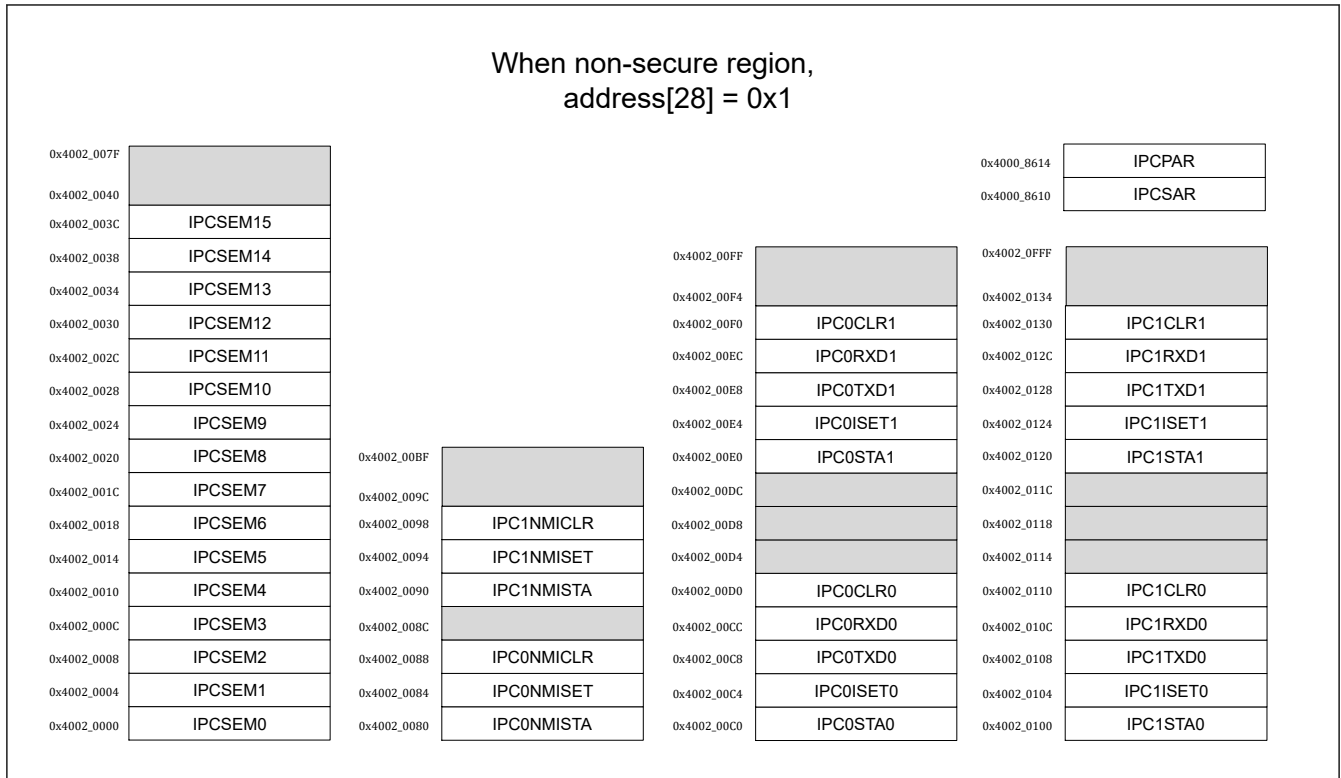
Figure 3.1 IPC register address map
