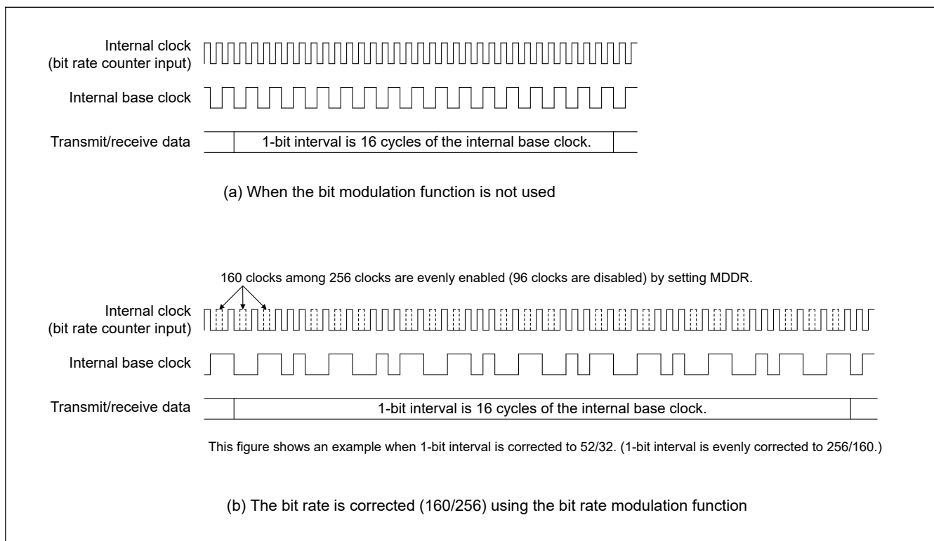
Figure 38.100 Example internal base clock when bit rate modulation function is used
