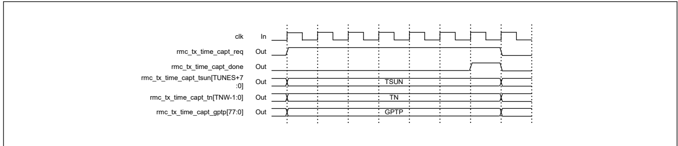
Figure 33.2 TX capture interface time chart
