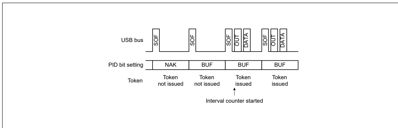
Figure 36.16 Token issuance when IITV = 0
