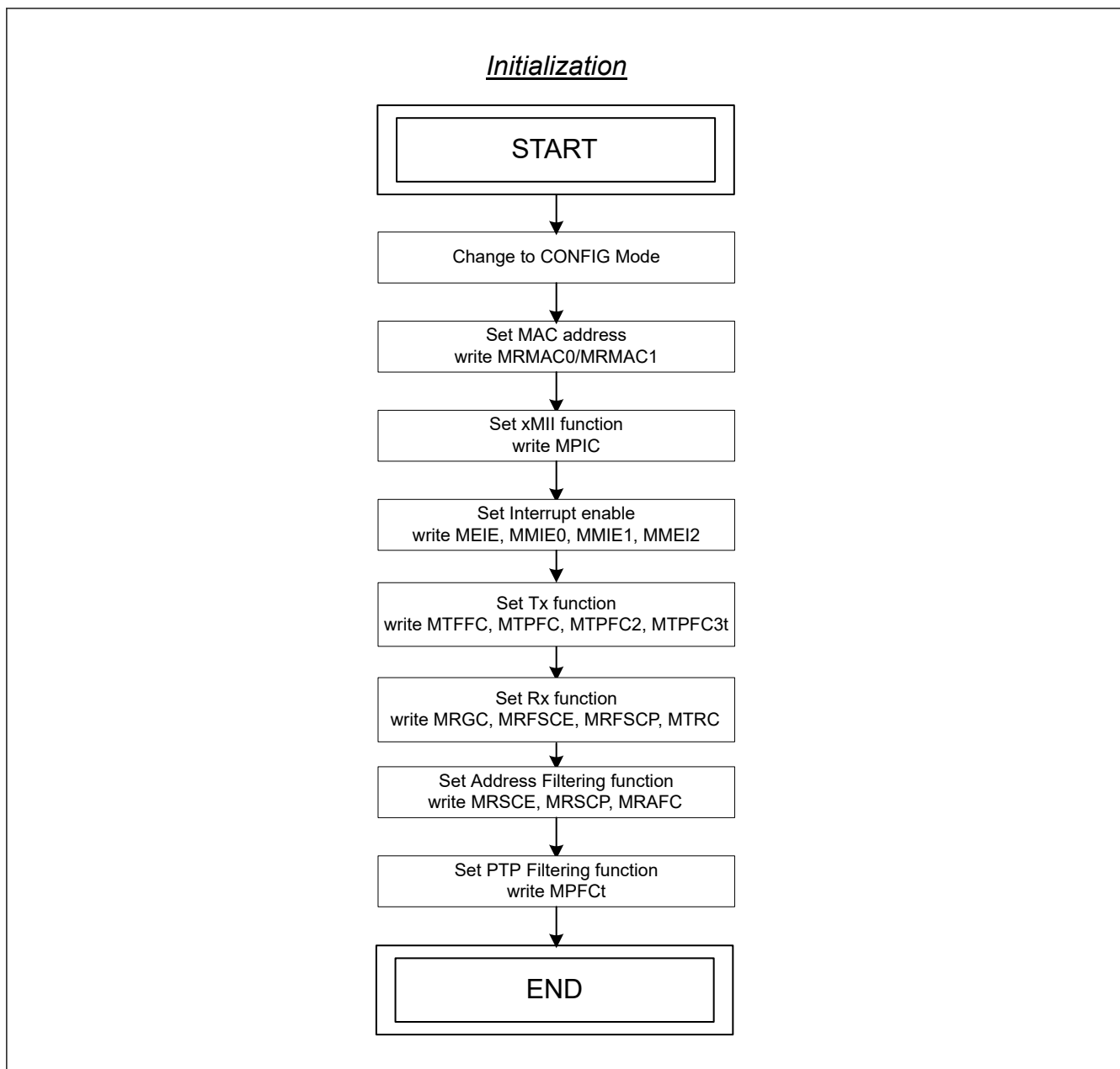
Figure 33.6 Initialization flow
