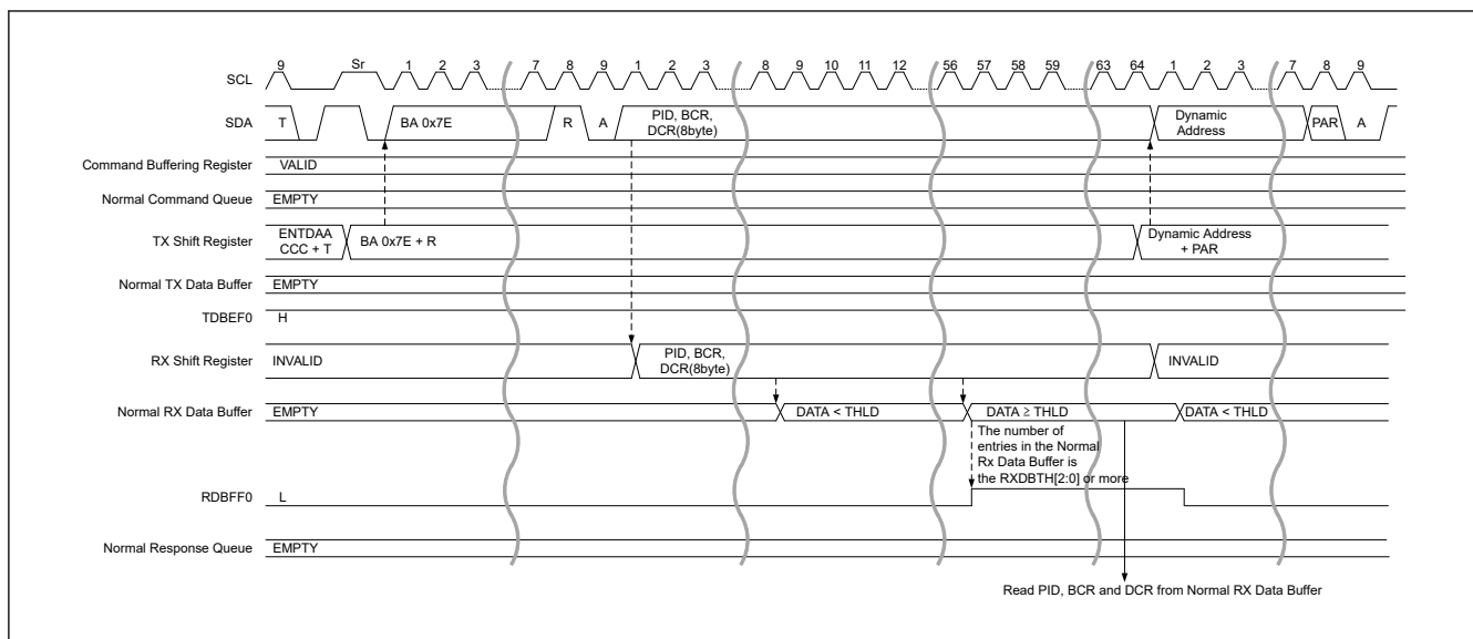
Figure 40.13 Dynamic address assign procedure (ENTDAA CCC) timing (2/3)
