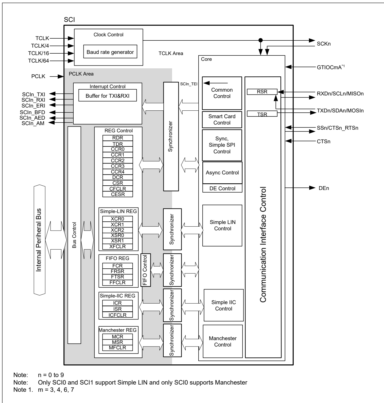
Figure 38.1 SCI block diagram
