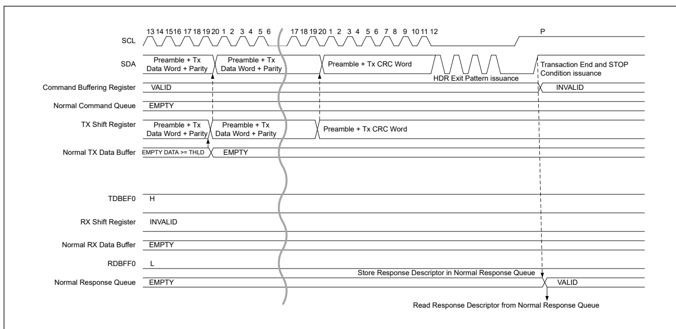
Figure 40.27 HDR data write transfer (HDR-DDR) timing (4/4)
