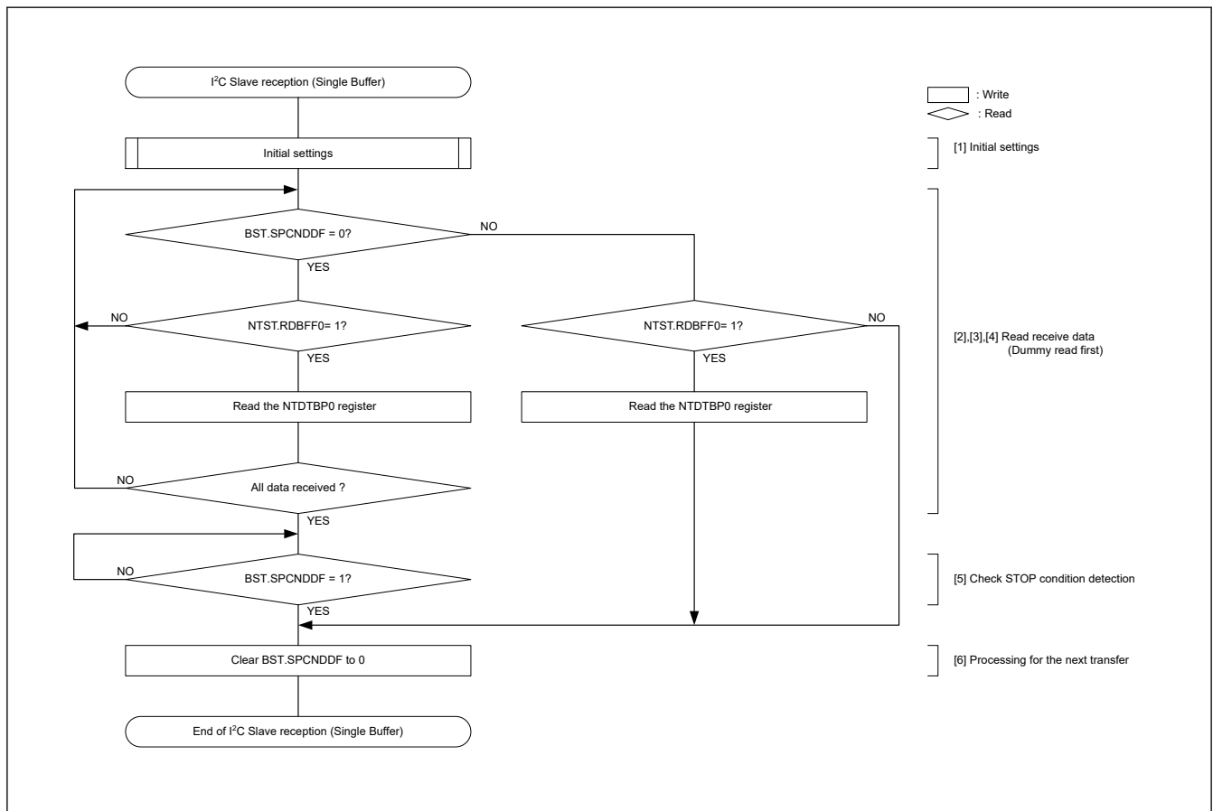
Figure 40.153 Example of I 2 C slave reception flowchart (single buffer transfer)
