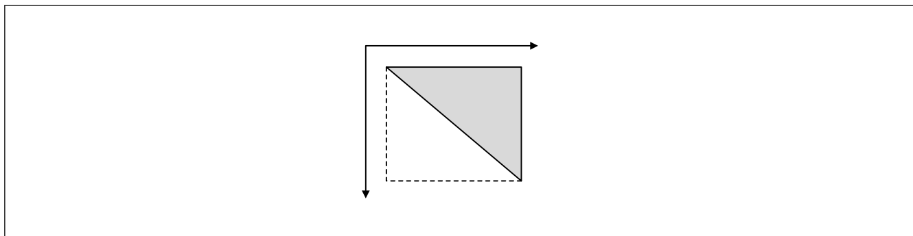
Figure 62.15 Triangle where the first edge is monotone growing
