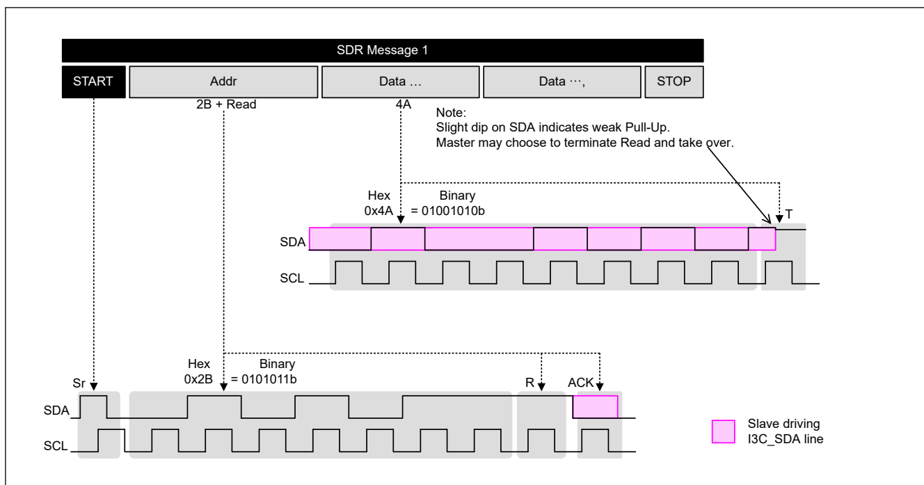
Figure 40.72 Example communication using I3C coding SDR without broadcast (0x7E)
