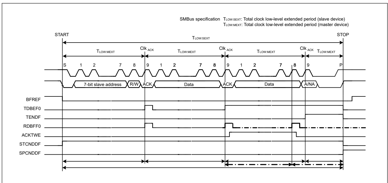
Figure 40.114 SMBus timeout measurement
