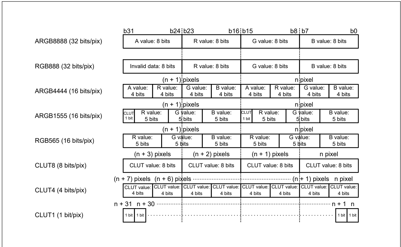
Figure 63.4 Frame data format
