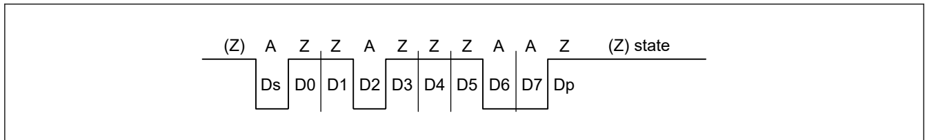
Figure 38.76 Direct convention with LSBF in CCR3 = 1, SINV in CCR3 = 0, and PM in CCR1 = 0
