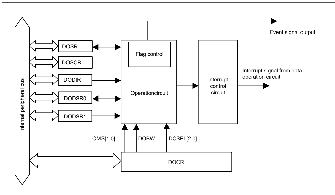
Figure 57.1 DOC block diagram
