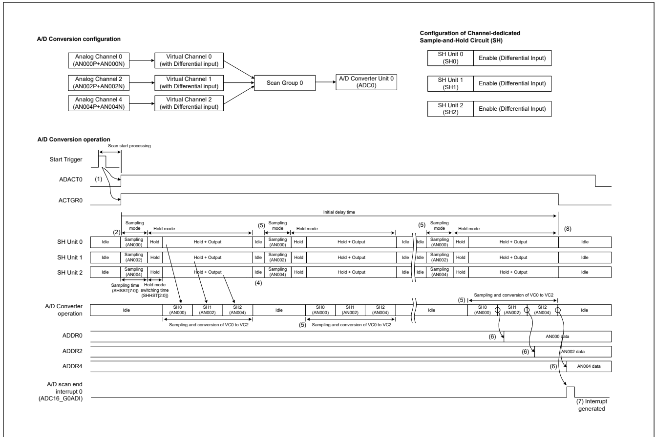
Figure 53.20 Basic operation of channel-dedicated sample-and-hold circuit in Hybrid mode – Single scan mode
