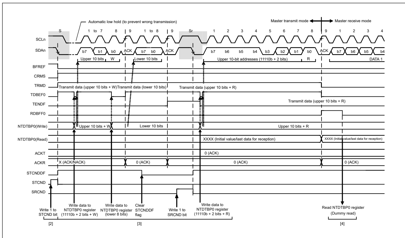
Figure 40.10 Master receive operation timing (2) (10-bit address format, when ACKTWE = 0)
