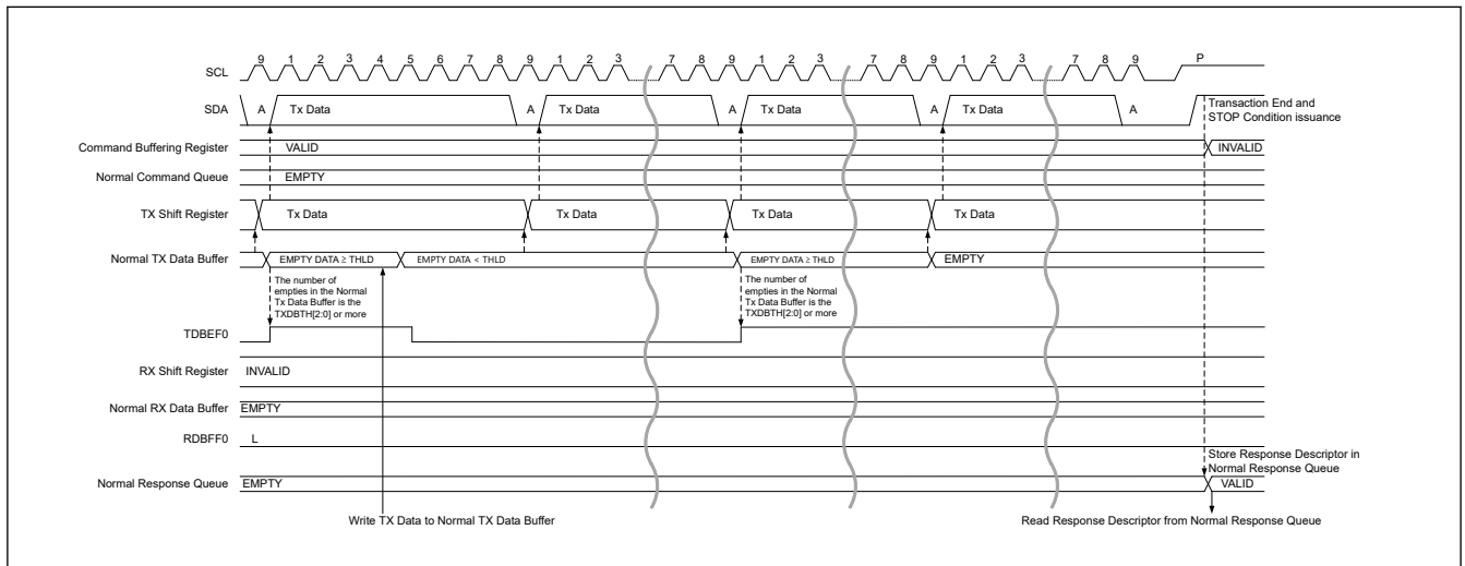
Figure 40.19 Legacy I2C message data write timing (2/2)
