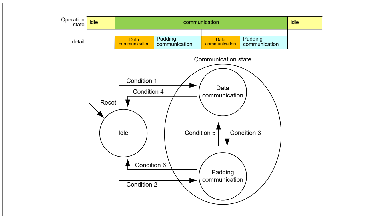
Figure 46.46 Communication state transition
