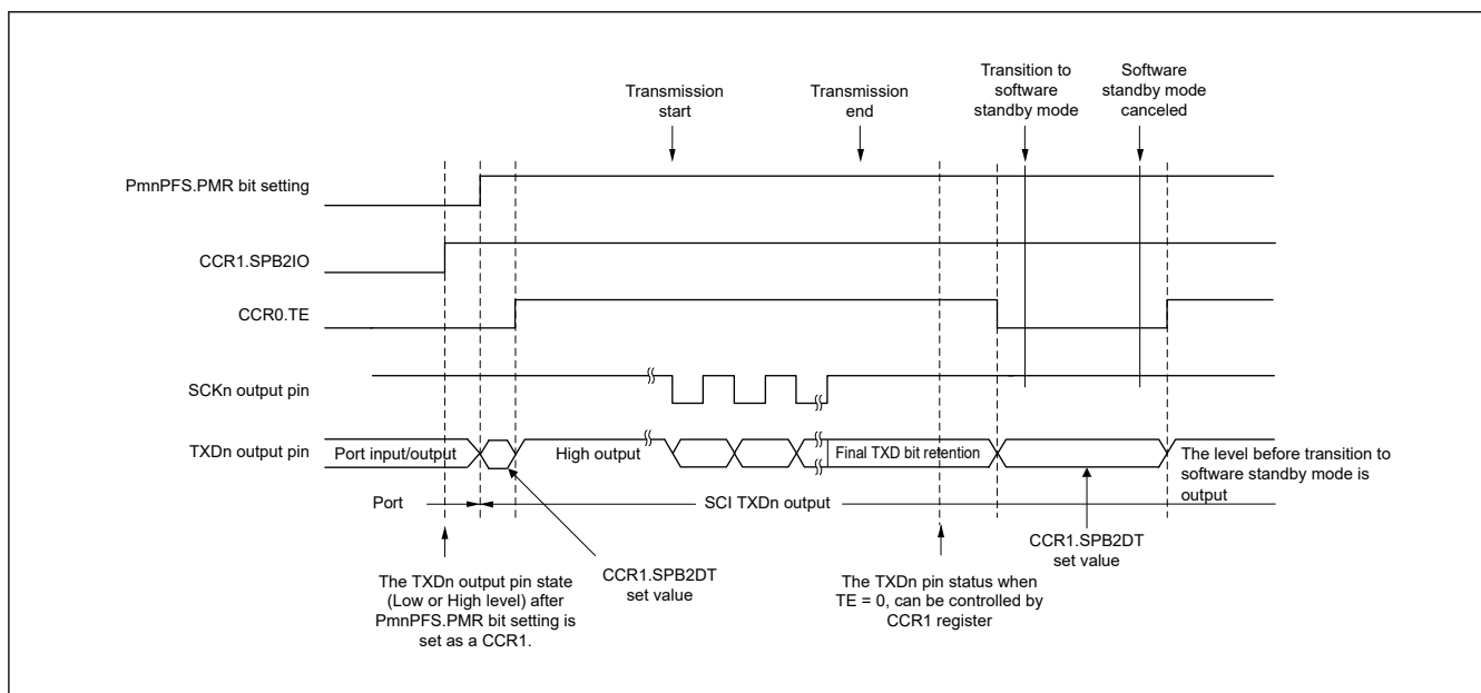
Figure 38.119 Port Pin States during Transition to Software Standby Mode (Internal Clock, Clock Synchronous Transmission)
