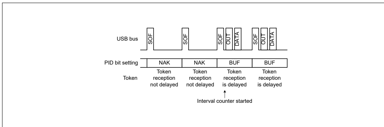
Figure 36.18 Relationship between frames and expected token reception when IITV[2:0] = 0
