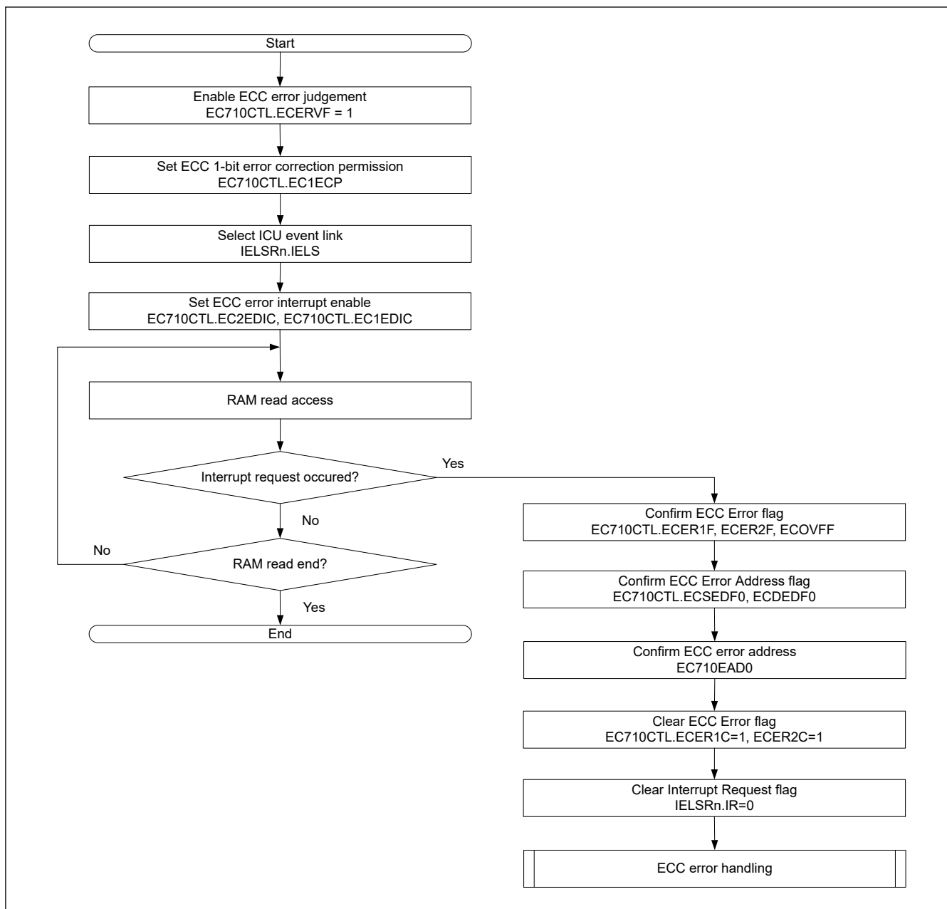
Figure 42.1 Setting procedure for ECC function
