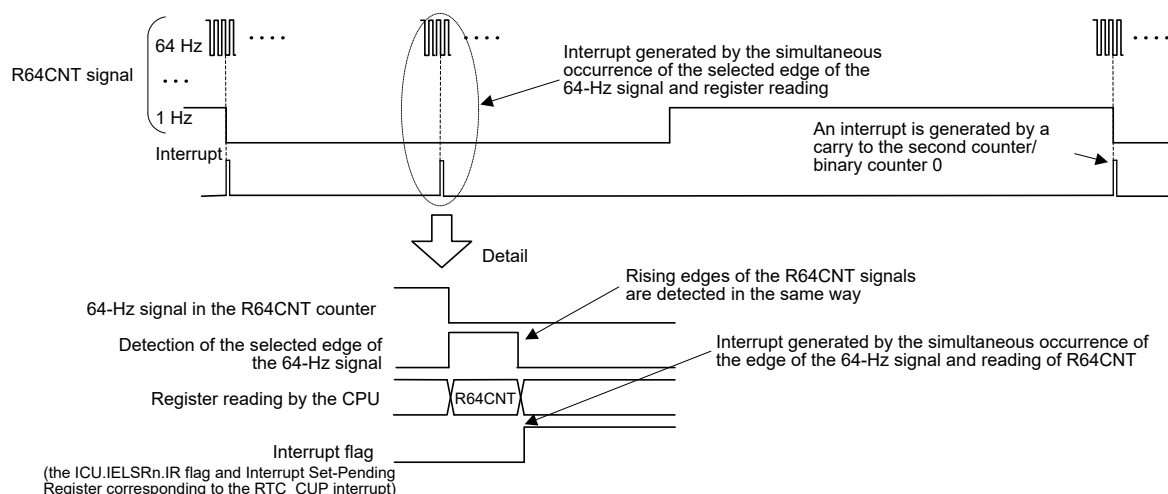
Figure 26.12 Timing for the carry interrupt (RTC_CUP)
