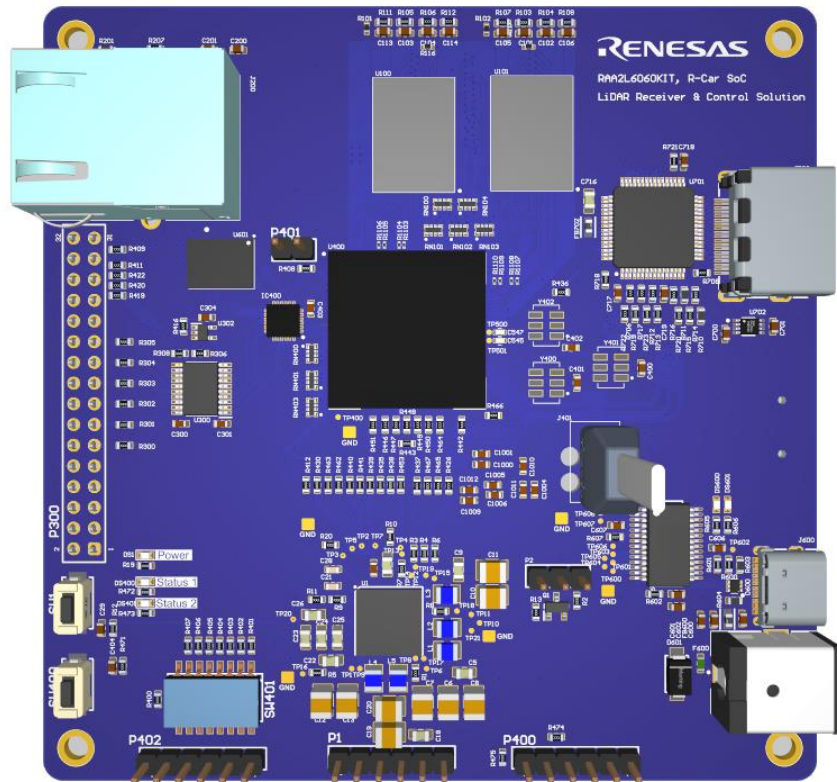
Figure 2: R-Car V3M SoC Board
