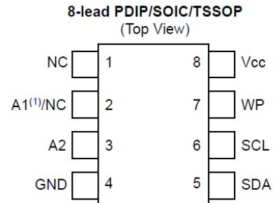
Figure 18. EEPROM Pin Description
