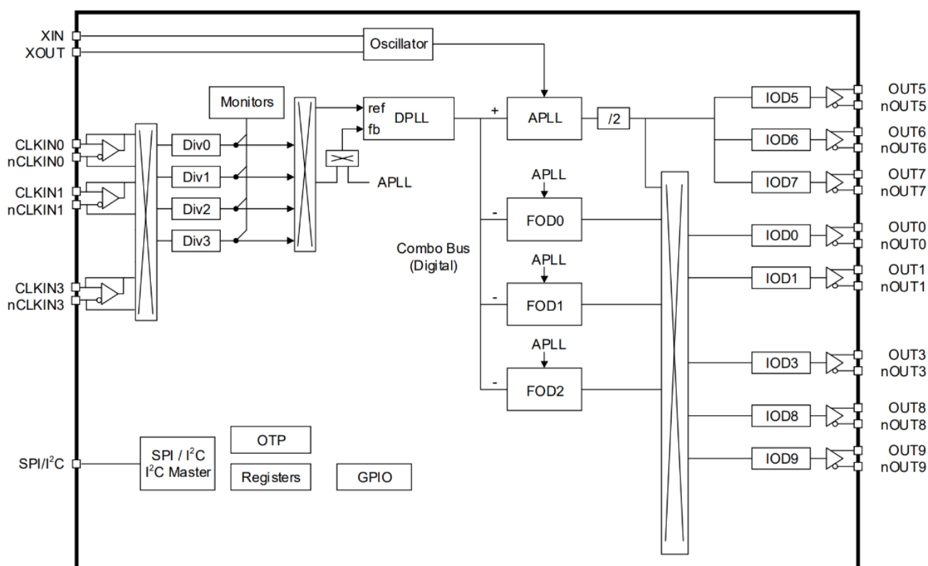
Figure 1. RC32308A Block Diagram
