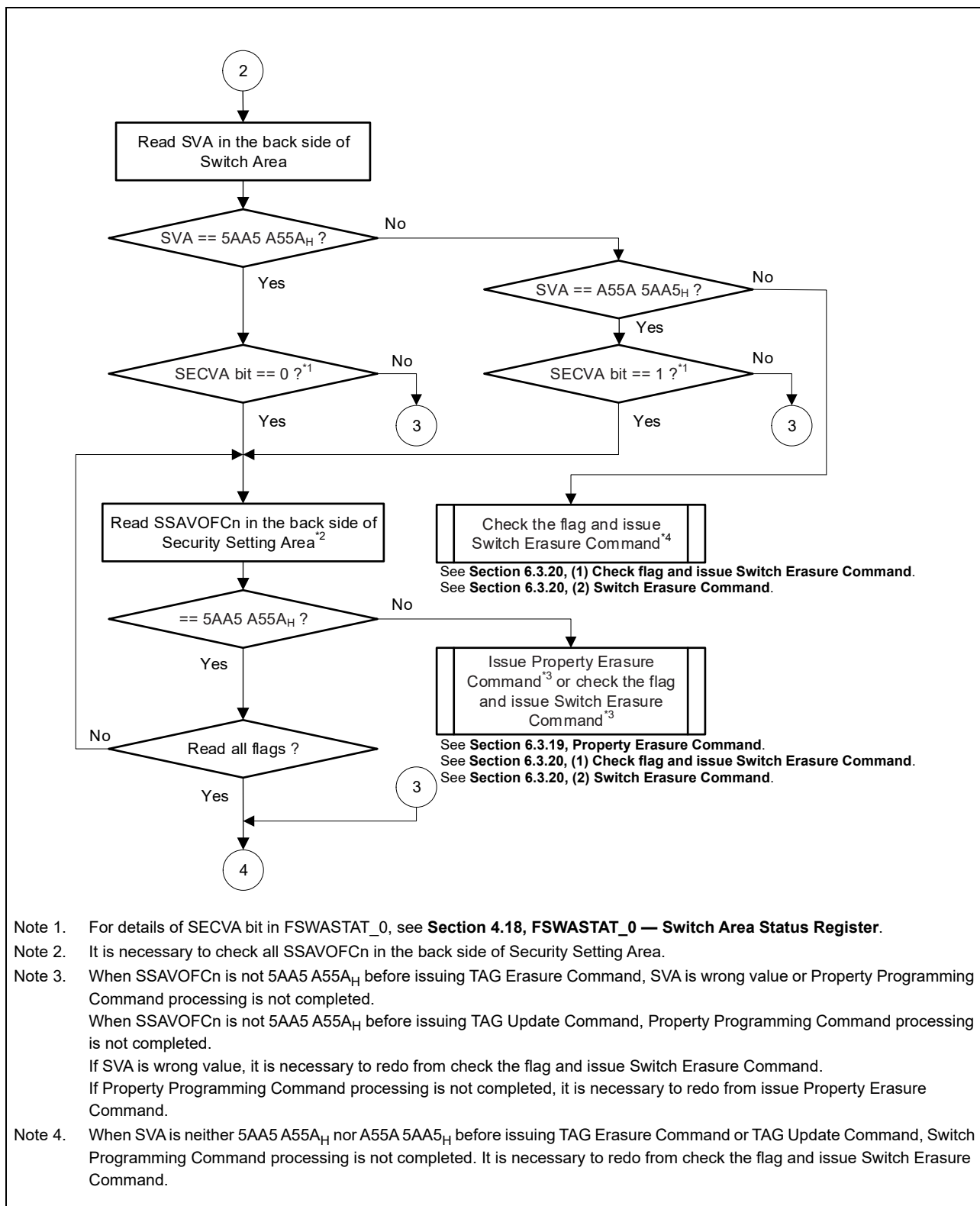
Figure 6.27 Check the flag before issuing TAG Erasure/Update Command (2)
