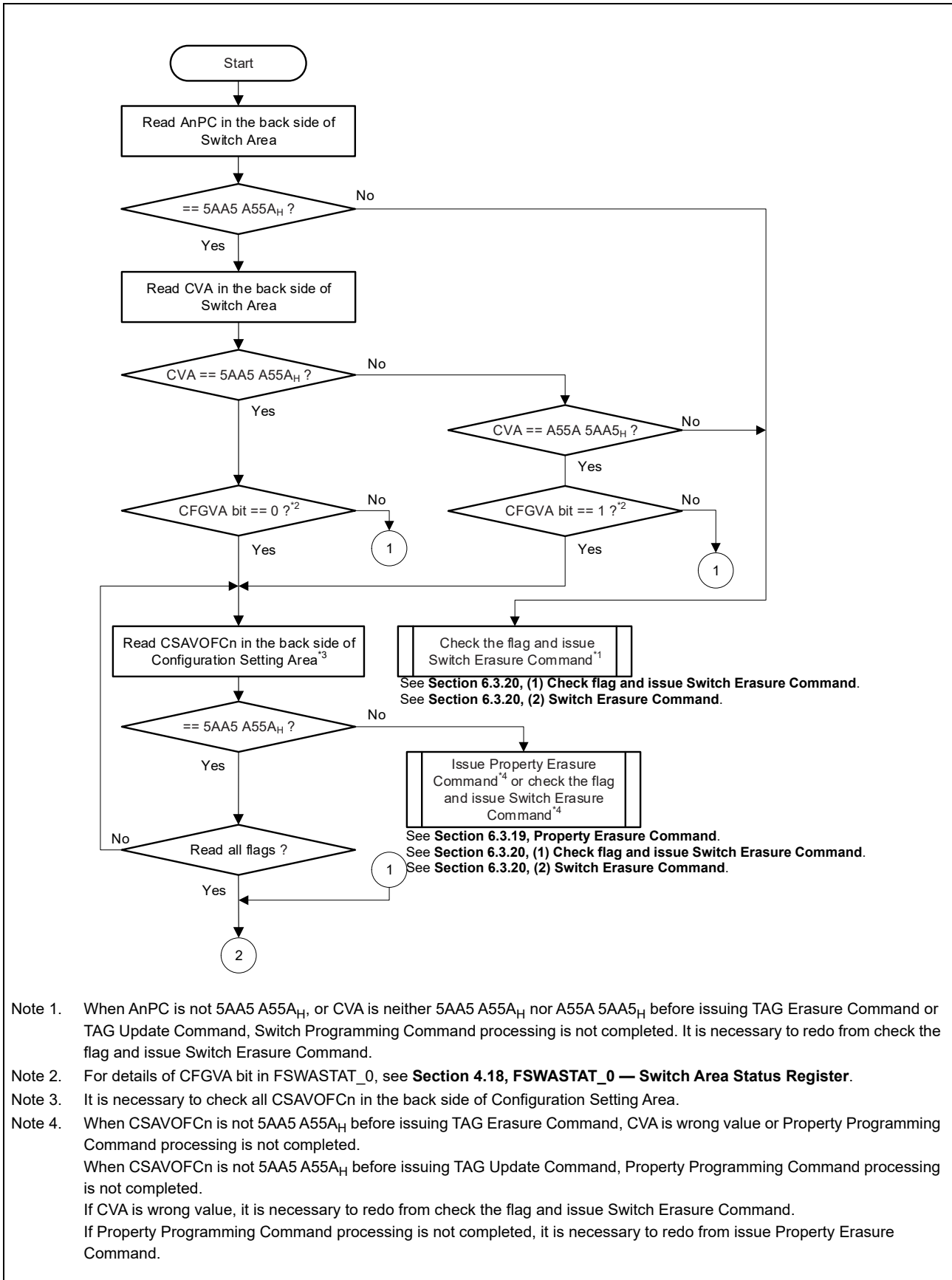
Figure 6.26 Check the flag before issuing TAG Erasure/Update Command (1)
