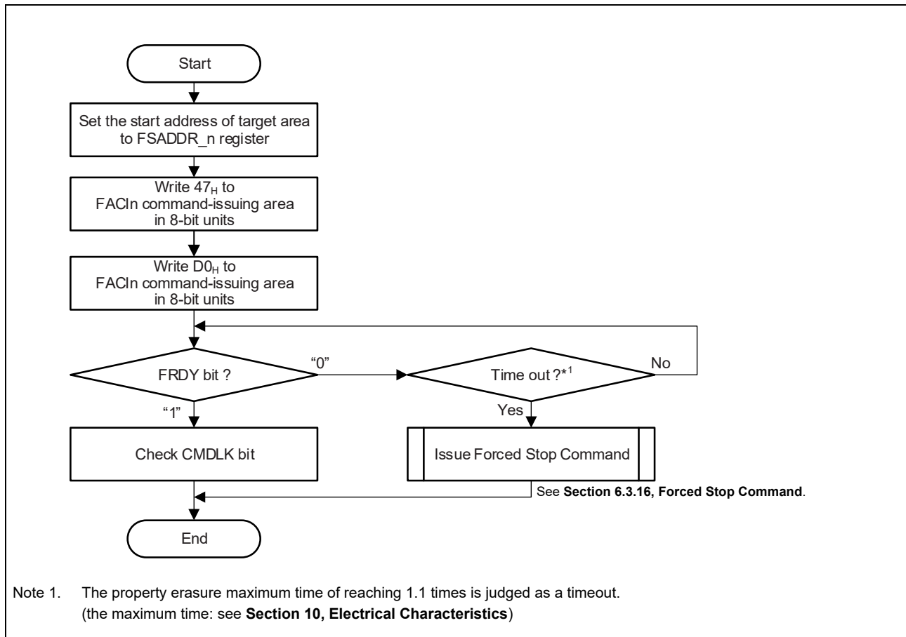
Figure 6.21 Property Erasure Command Usage
