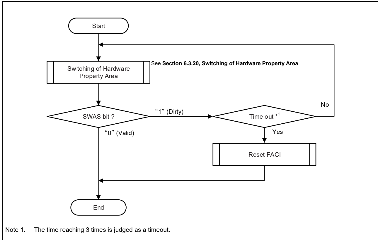
Figure 6.32 Flow of Recovering Switch Area Status.
