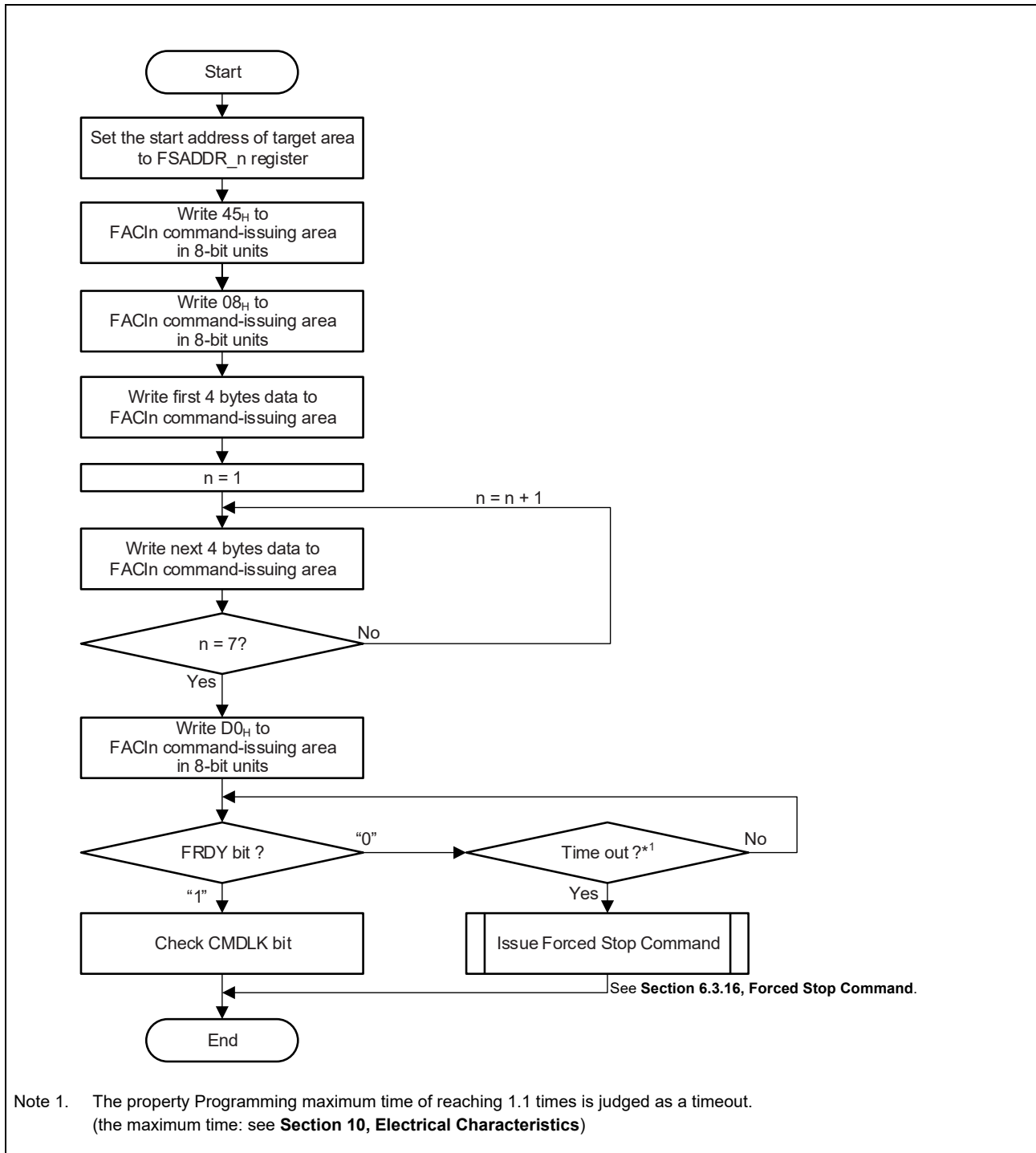
Figure 6.20 Property Programming Command Usage
