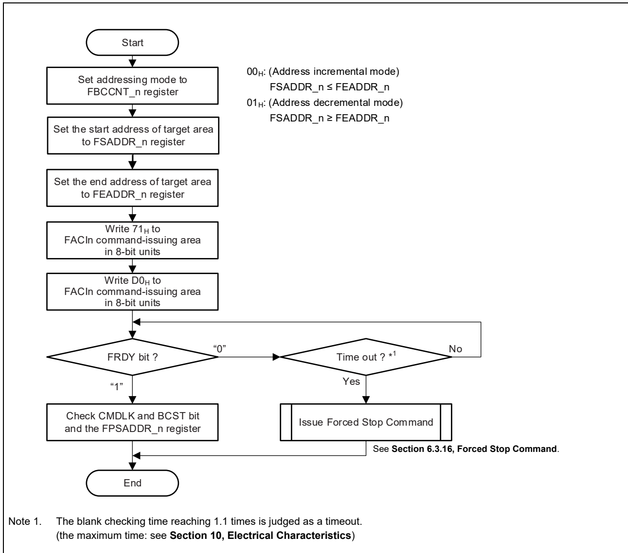
Figure 6.19 Blank Checking Command Usage
