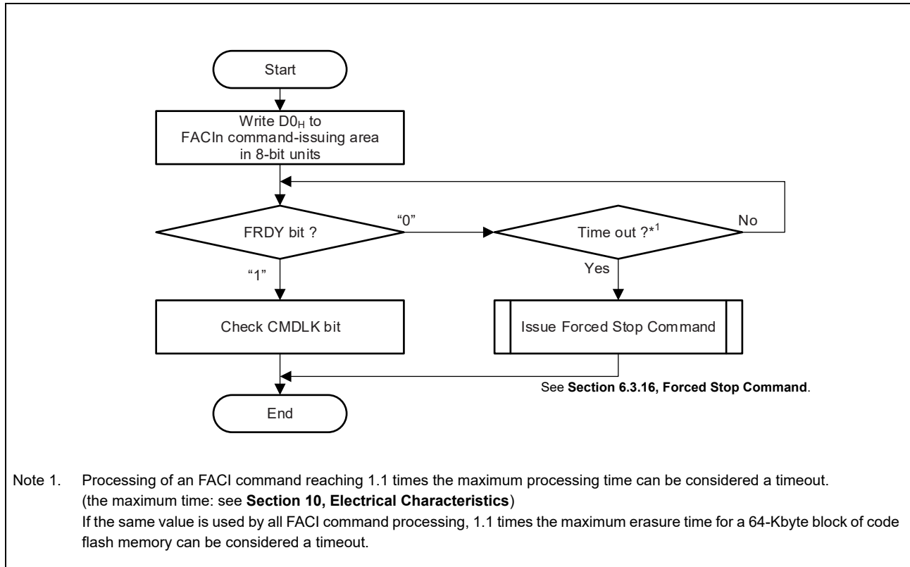
Figure 6.16 Programming/Erase Resumption Command Usage
