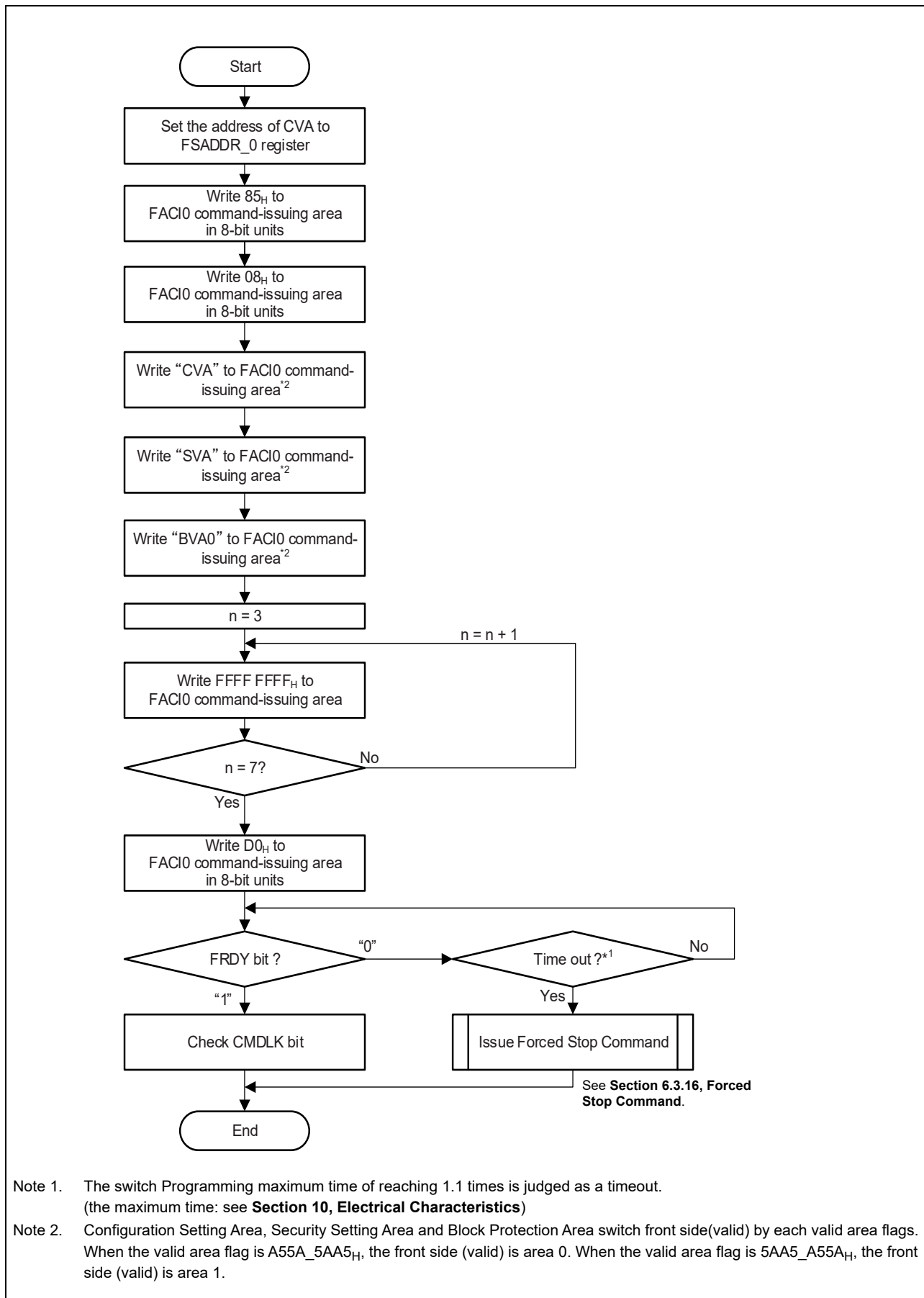
Figure 6.25 Switch Programming Command Usage
