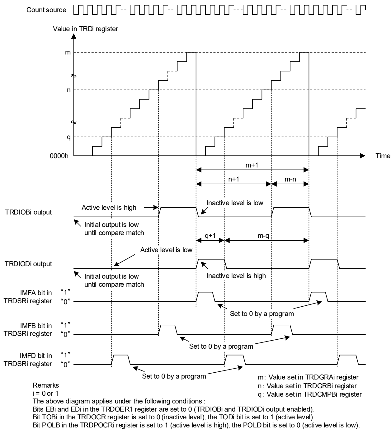
Figure 8-62. Operation Example in Extended PWM Mode
