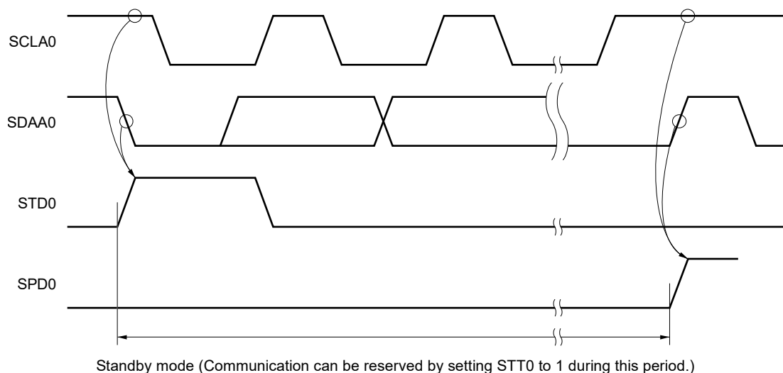
Figure 16-27. Timing for Accepting Communication Reservations
