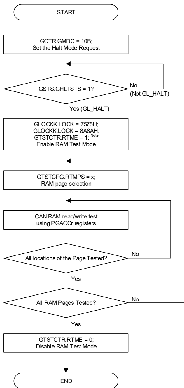
Figure 18-43. RAM Test Mode SW Flow
