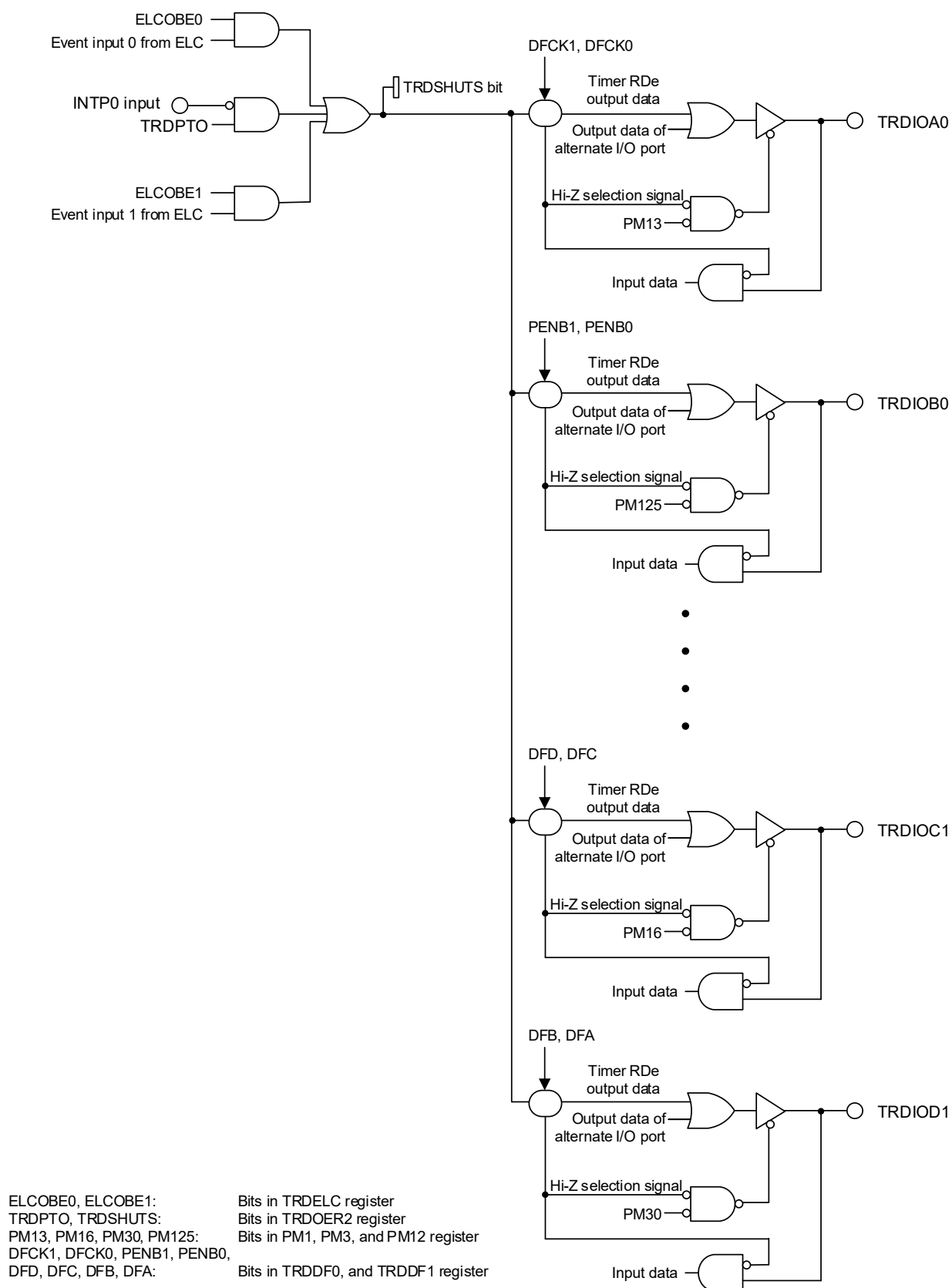
Figure 8-41. Pulse Output Forced Cutoff
