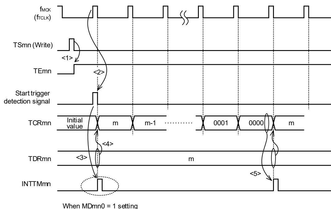
Figure 6-29. Operation Timing (In Interval Timer Mode)
