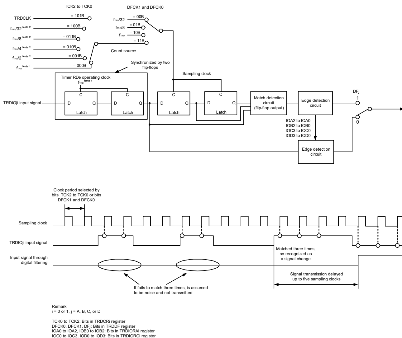
Figure 8-46. Block Diagram of Digital Filter
