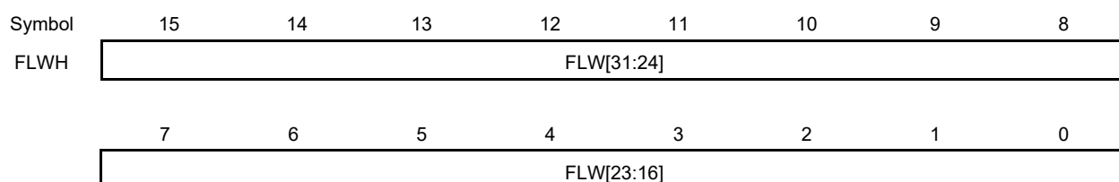
Figure 28-30. Format of Flash Write Buffer Register (FLWH / FLWL)
