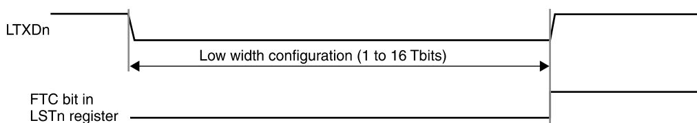
Figure 17-18. Wake-up Transmission Timing
