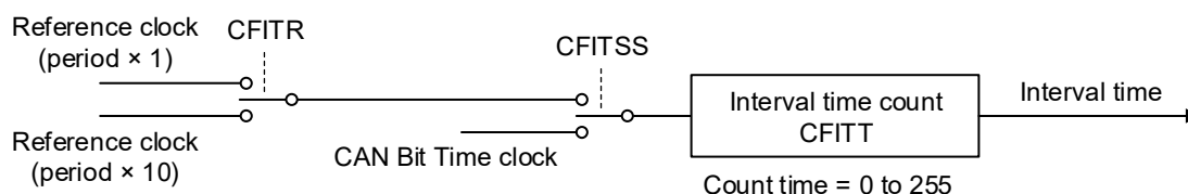
Figure 18-35. Block Diagram of FIFO Interval Timer
