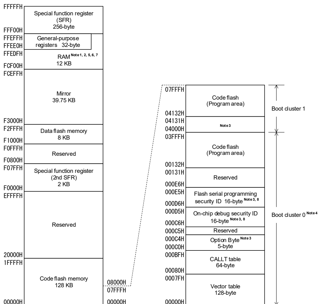
Figure 3-2. Memory Map (RL78/F23)
