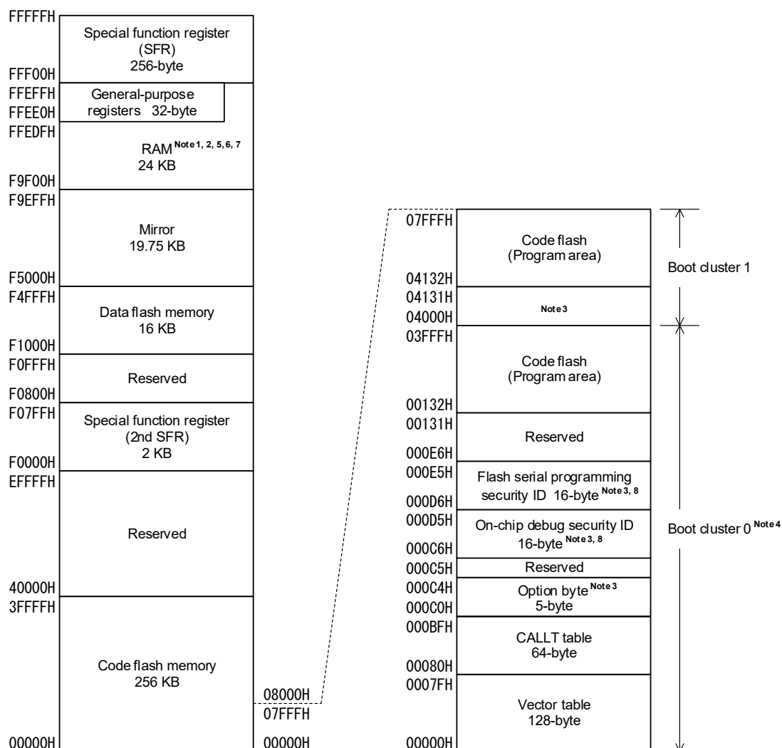
Figure 3-1. Memory Map (RL78/F24)
