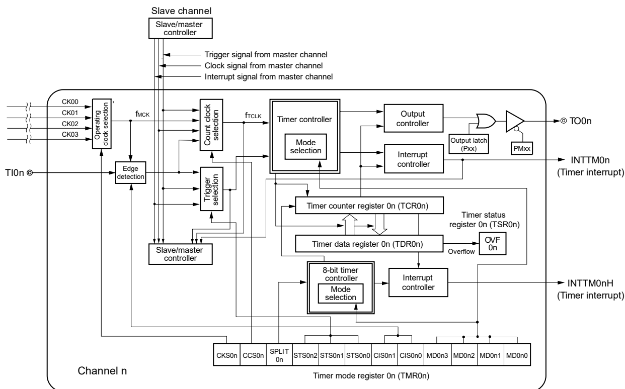
Figure 6-5. Internal Block Diagram of Channels 1, 3 of Timer Array Unit 0
