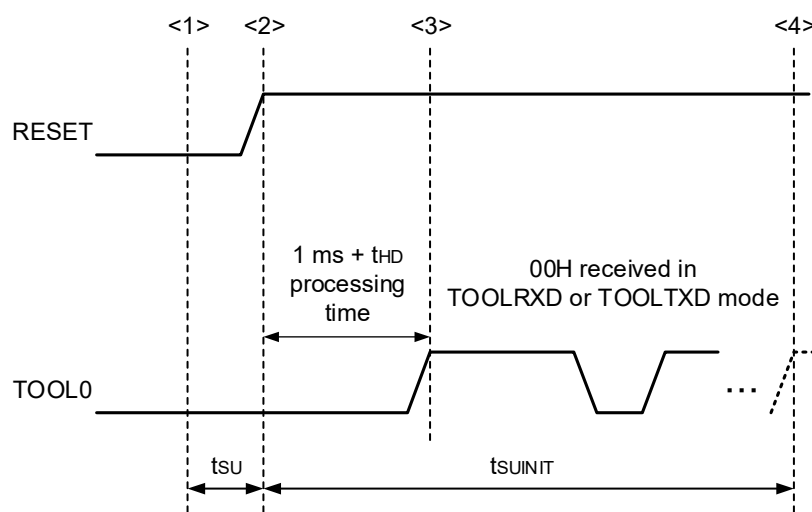
Figure 32-7. Setting of Flash Memory Programming Mode
