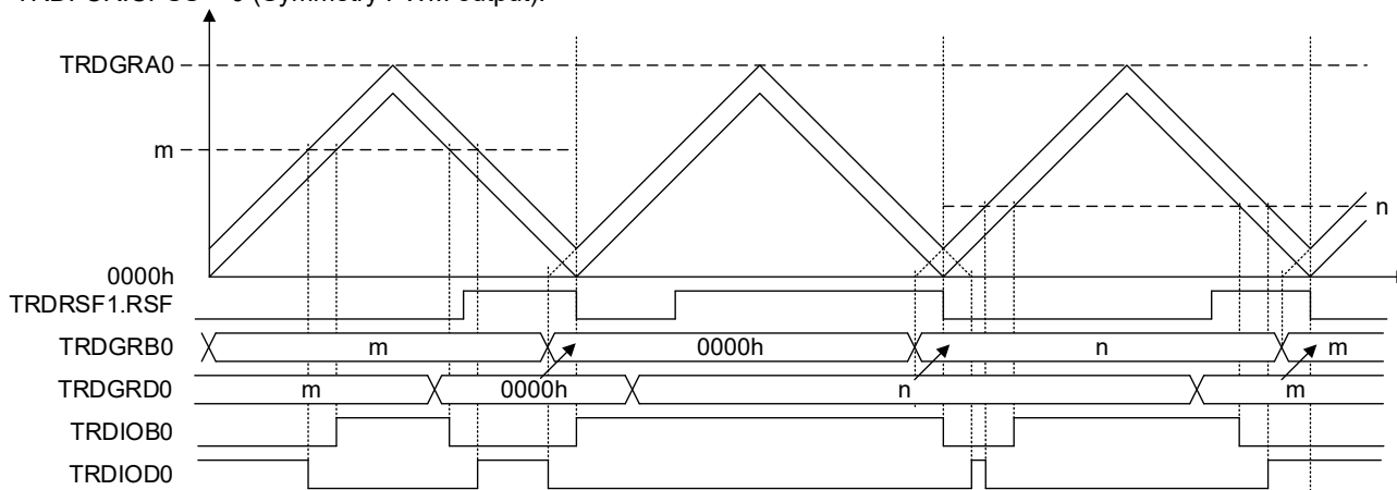
Figure 8-83. Operation Example (Duty Cycle 100%)
