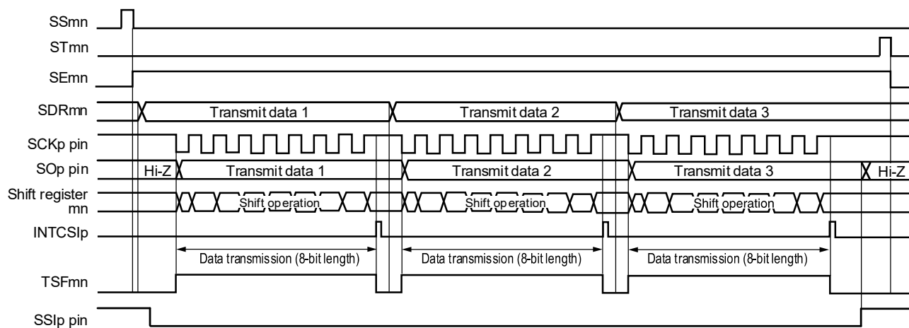
Figure 15-104. Timing Chart of Slave Transmission (in Single-Transmission Mode) (Type 1: DAPmn = 0, CKPmn = 0)
