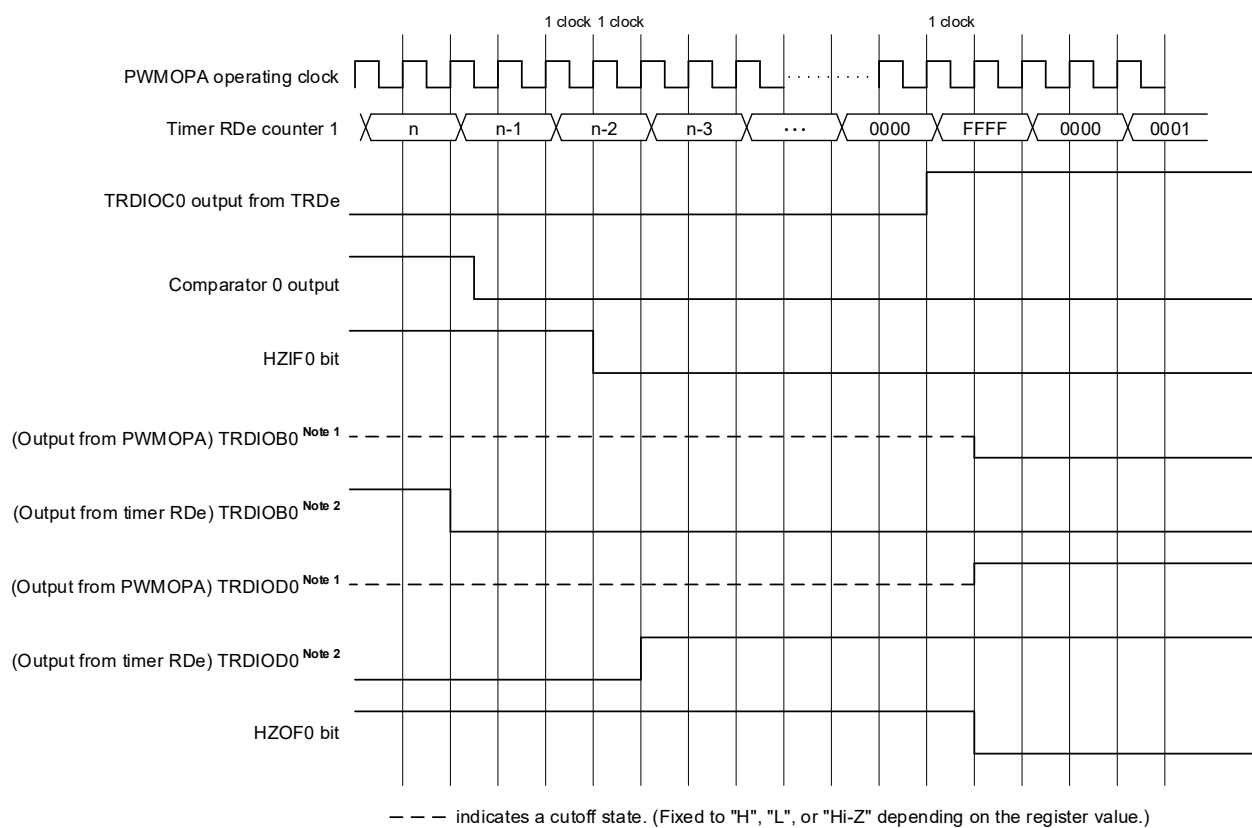
Figure 8-101. Cutoff Release Detailed Timing Diagram (Timer RDe Count Source = f_{CLK}/2 , TRD1 Decrementd) (An Example of TRDIOB0 and TRDIOD0)
