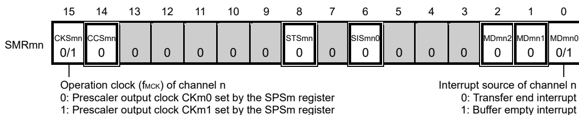
Figure 15-76. Example of Contents of Registers for Master Transmission of SPI Function (CSI00, CSI01, CSI10, CSI11) (1/2)
