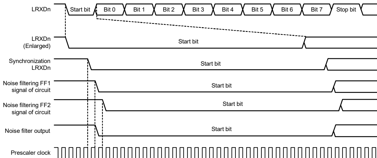
Figure 17-46. Determination of Received Data when Noise Filter is Used
