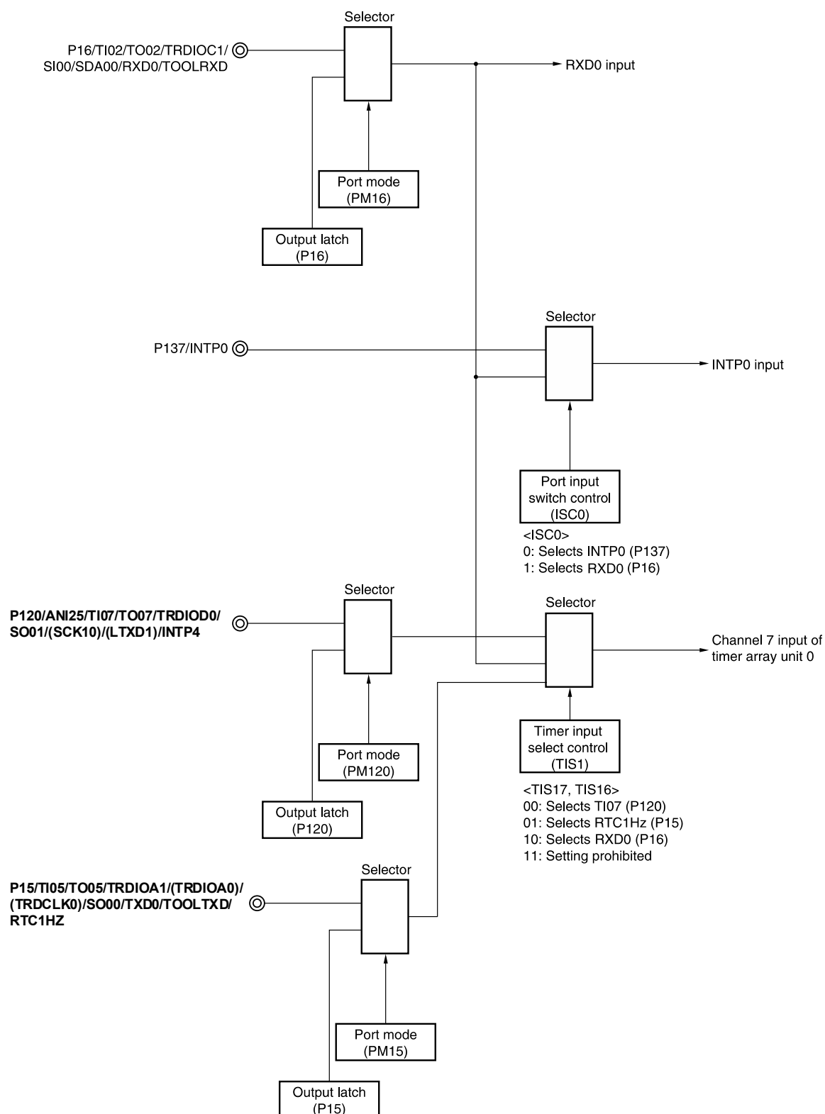
Figure 15-144. Port Configuration for Manipulating Reception of LIN
