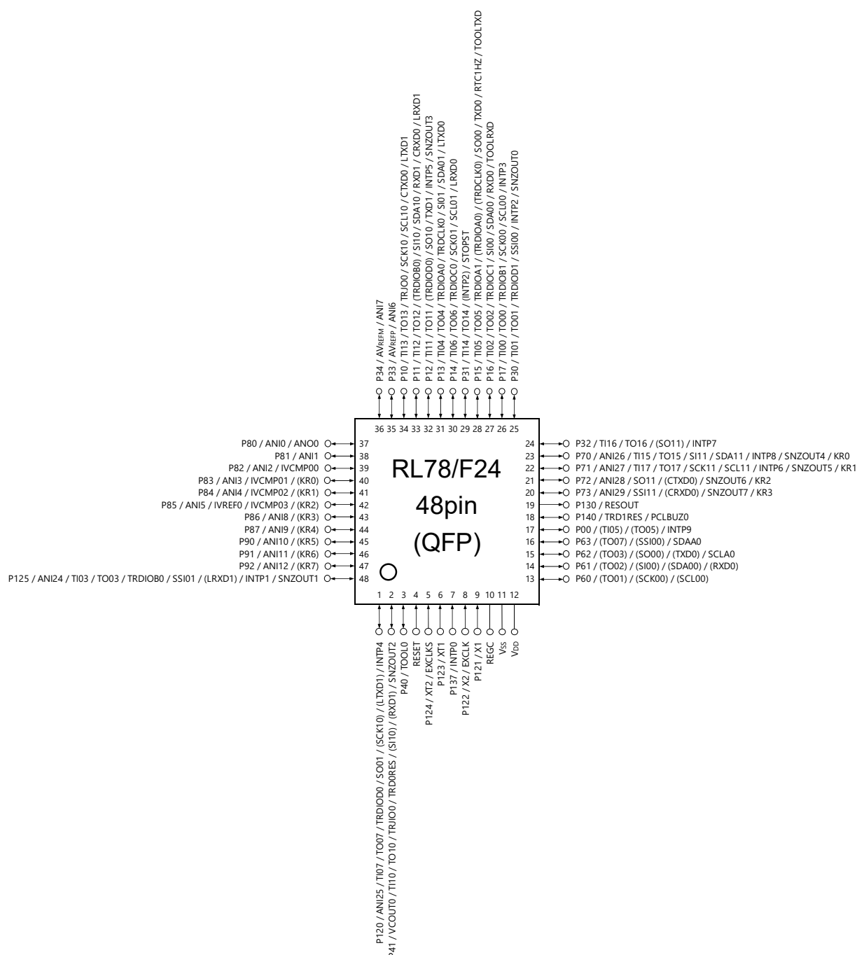
Figure 1-15. RL78/F24 Pin Configuration for 48-pin Products
