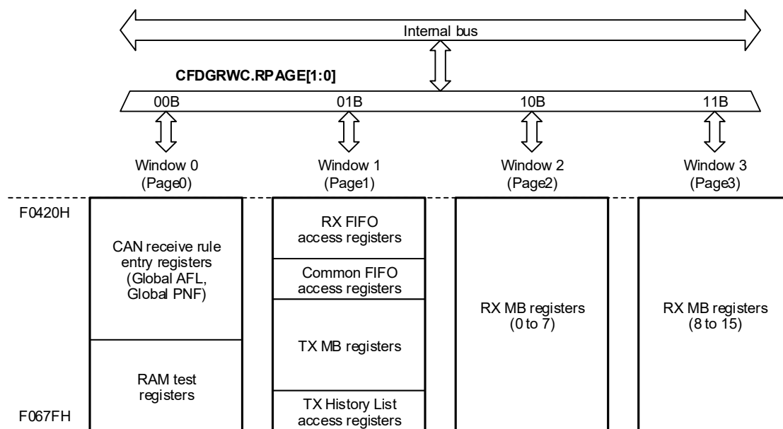
Figure 18-49. RAM Window
