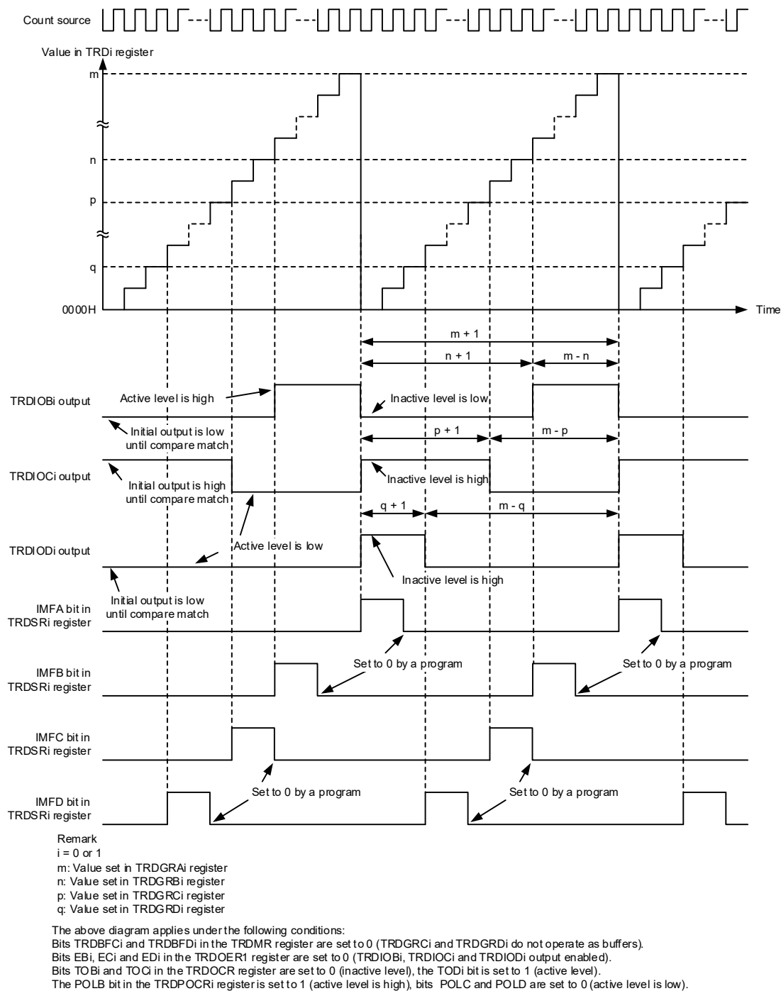
Figure 8-52. Operation Example in PWM Function
