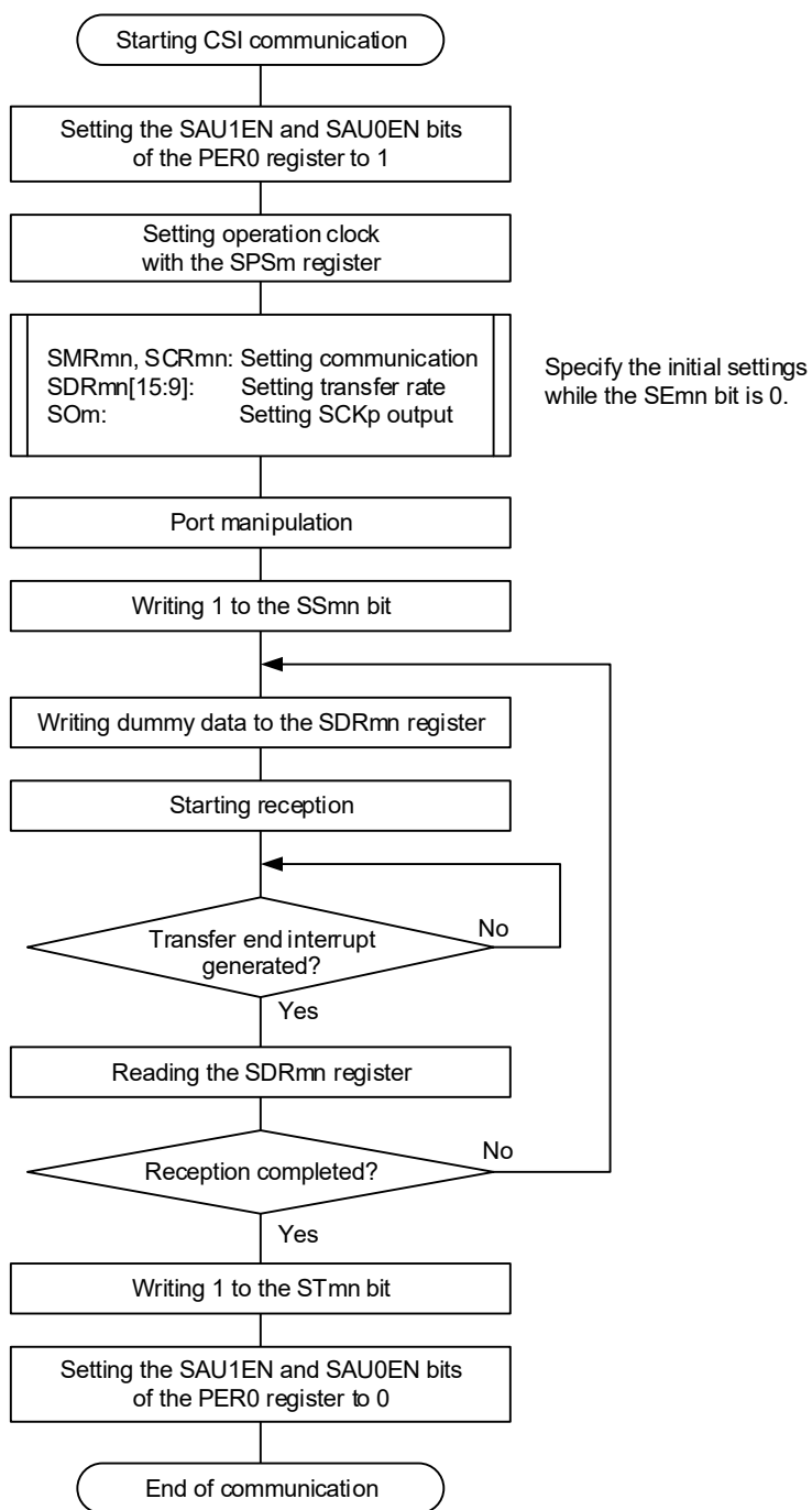
Figure 15-89. Flowchart of Master Reception (in Single-Reception Mode)
