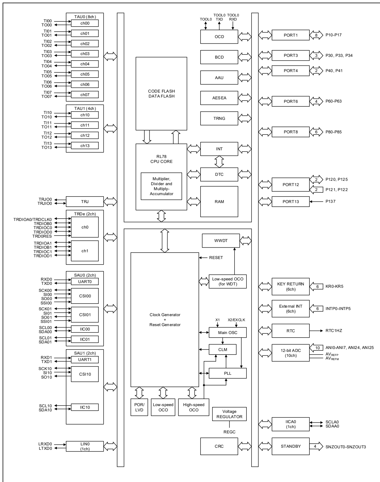
Figure 1-9. Block Diagram
