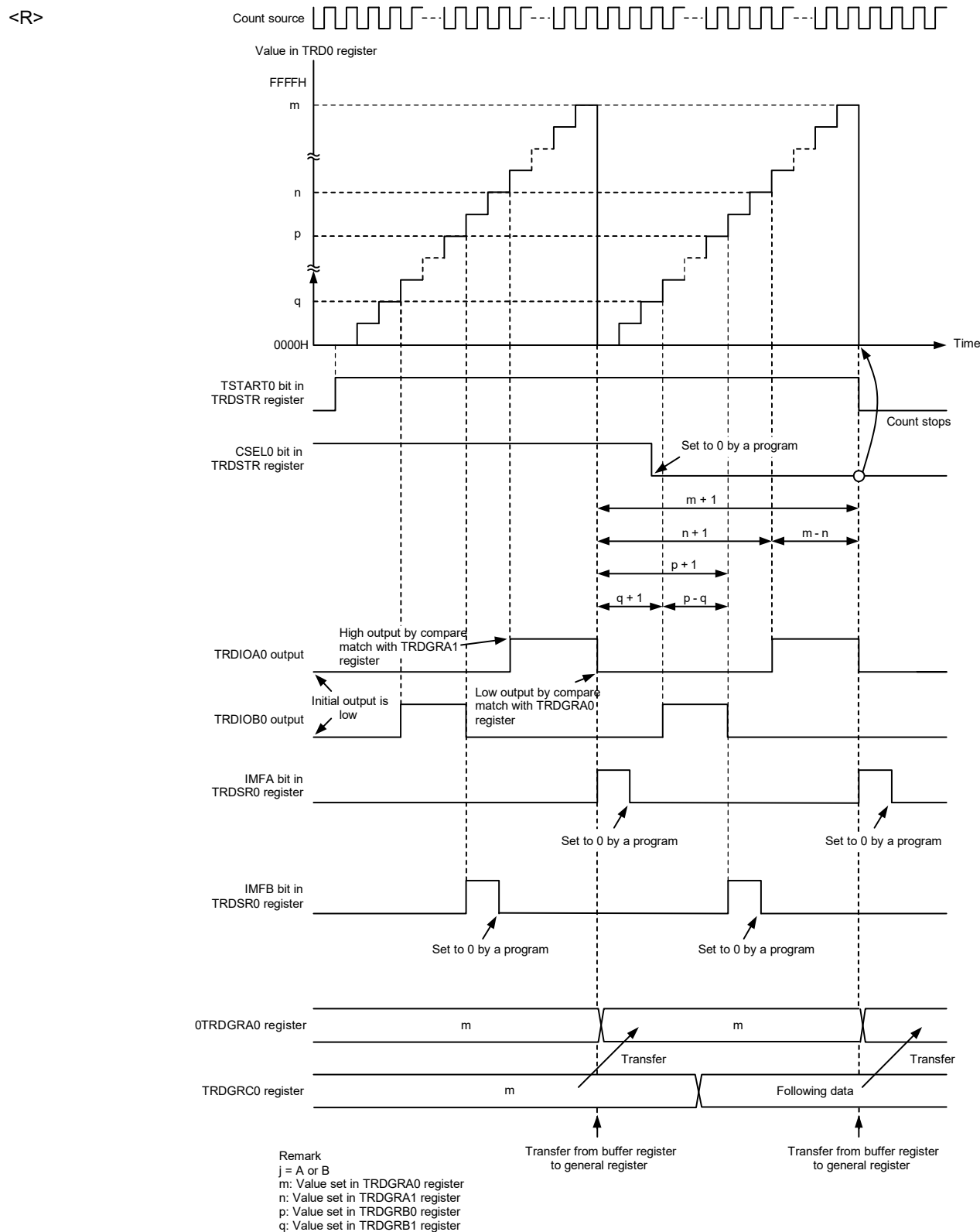
Figure 8-60. Operation Example in PWM3 Mode
