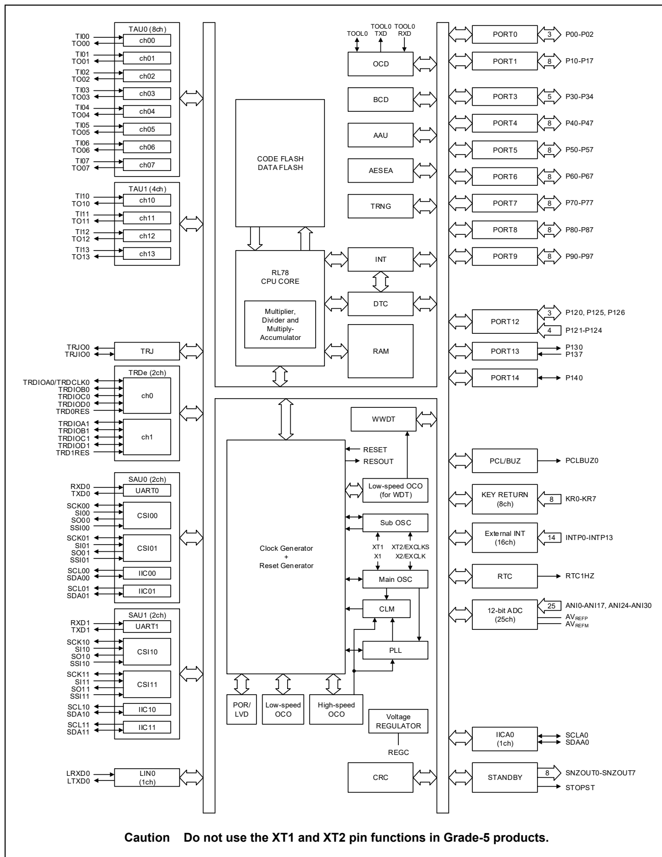
Figure 1-6. Block Diagram
