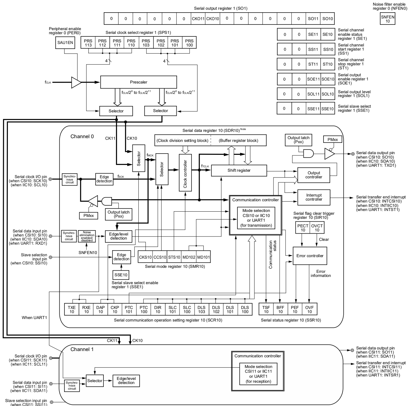
Figure 15-2. Block Diagram of Serial Array Unit 1
