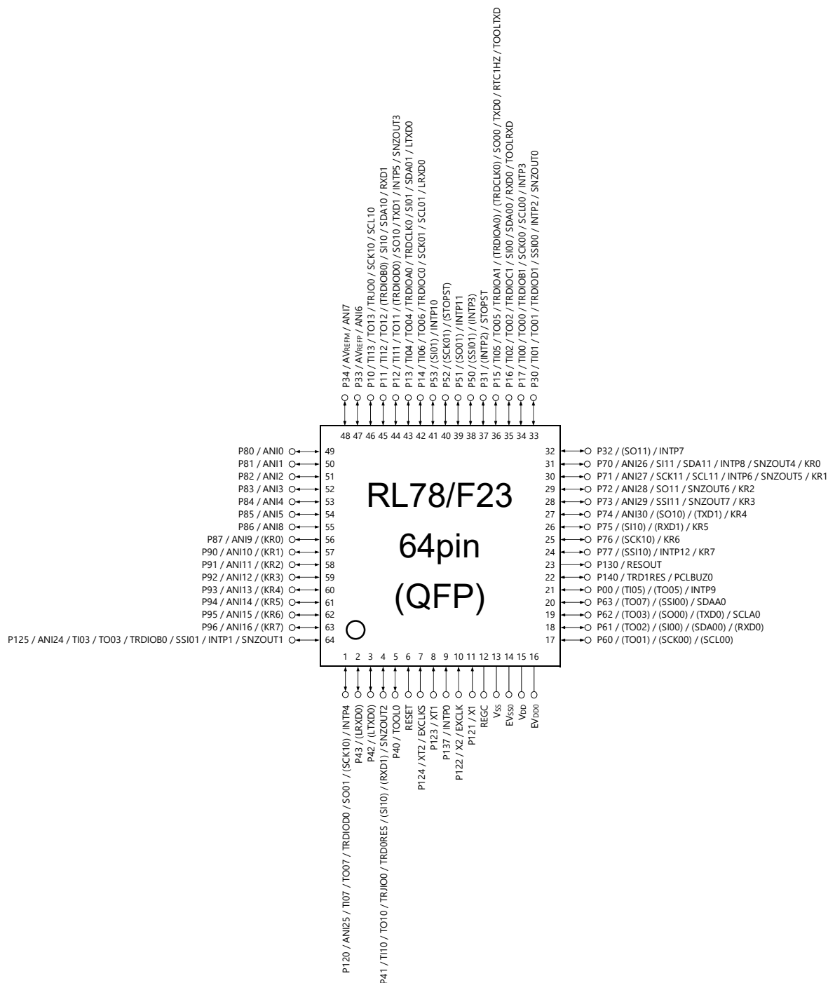
Figure 1-14. RL78/F23 Pin Configuration for 64-pin Products
