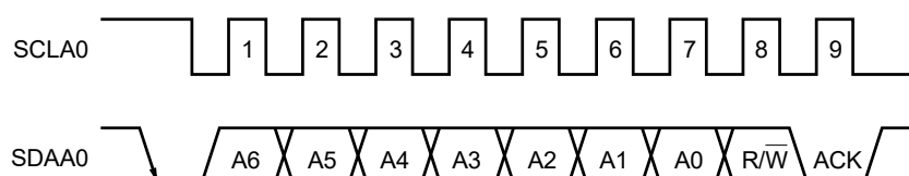
Figure 16-19. ACK
