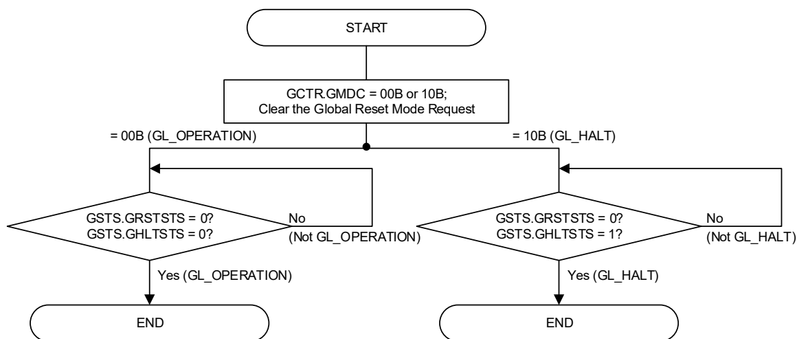
Figure 18-9. Procedure for Exiting Global Reset Mode
