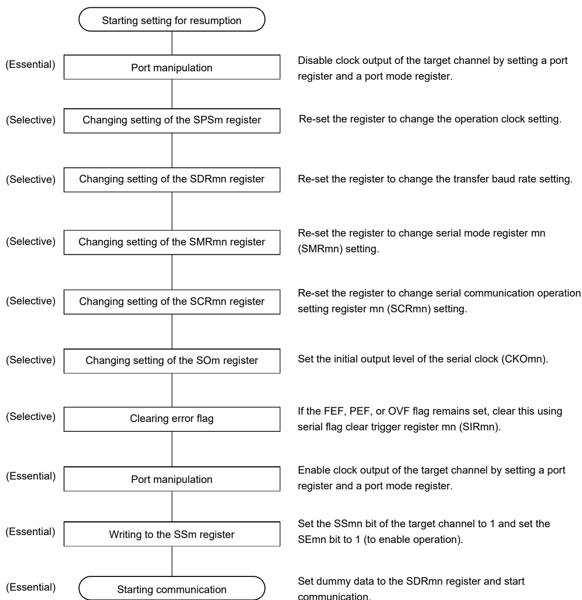
Figure 15-87. Procedure for Resuming Master Reception
