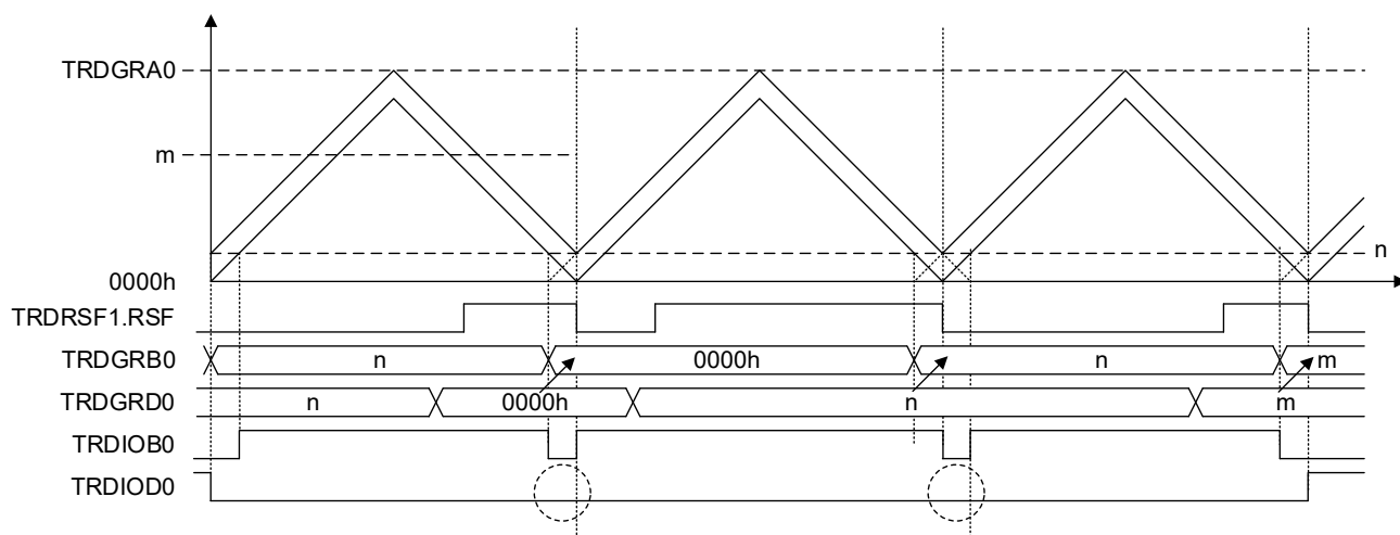
Figure 8-84. Notes on Duty Cycle 100% Setting
