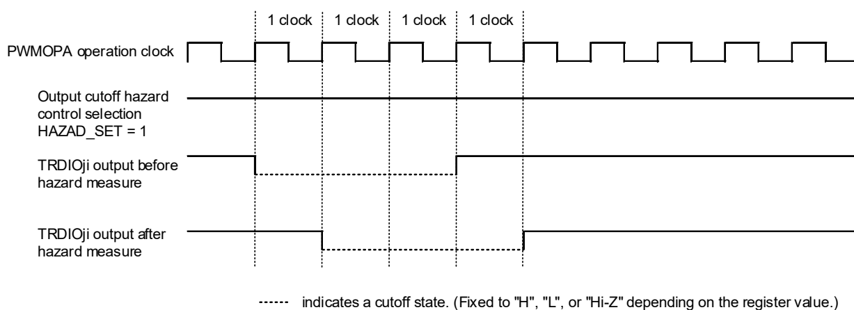
Figure 8-109. Hazard Control Timing Diagram
