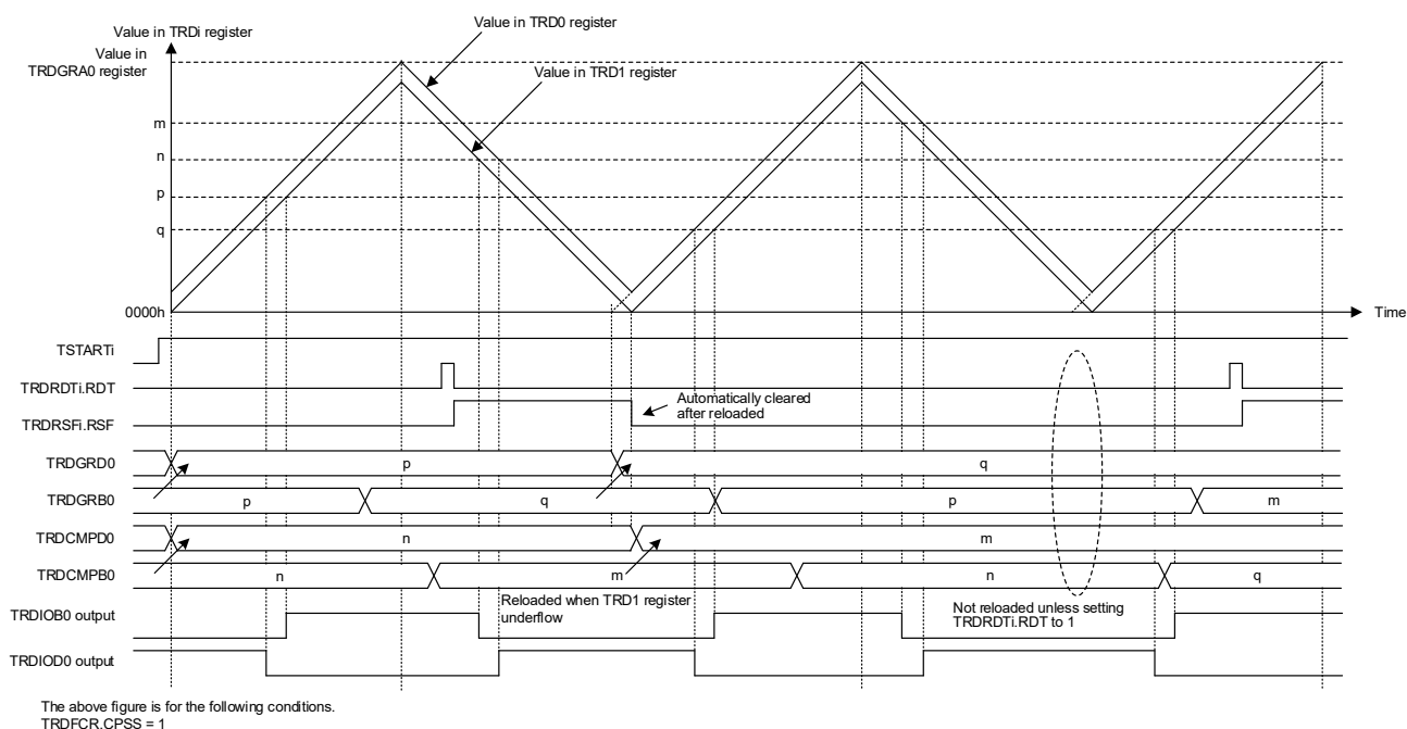
Figure 8-43. Reload Function in Extended Complementary PWM Mode
