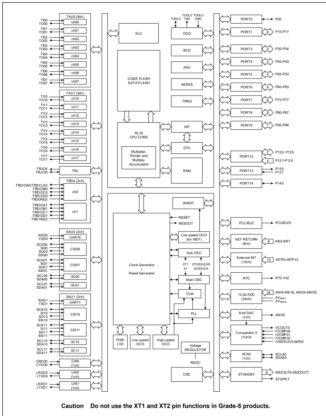
Figure 1-3. Block Diagram
