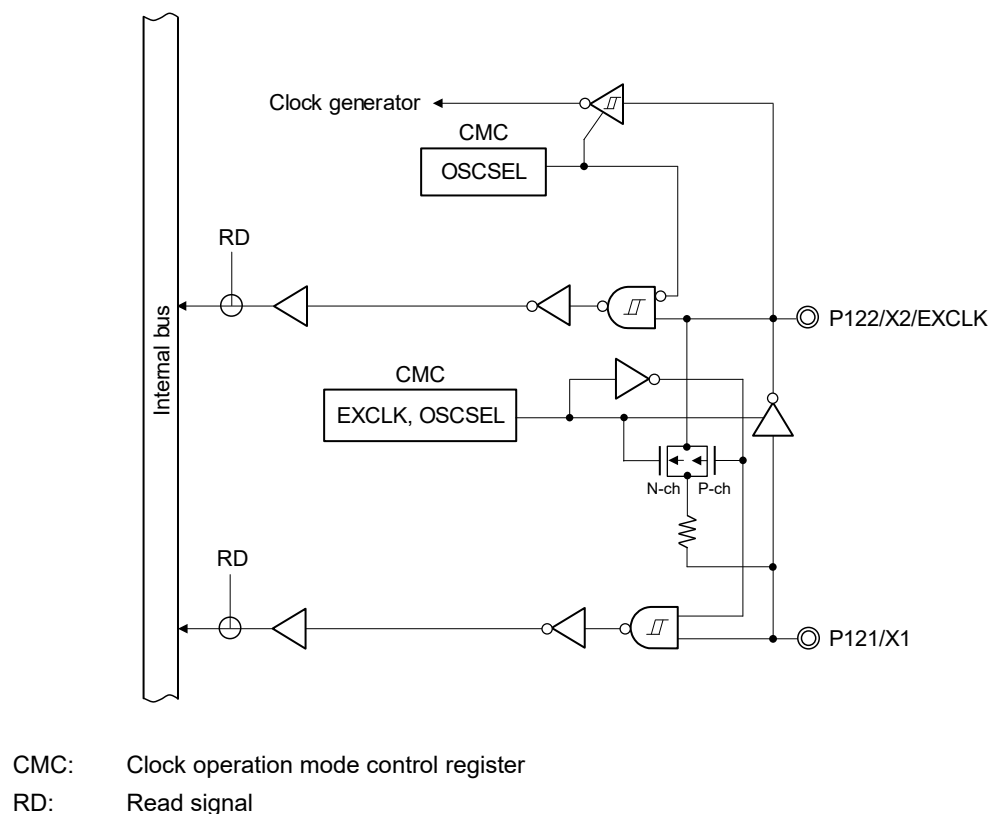
Figure 4-62. Block Diagram of P121 and P122
