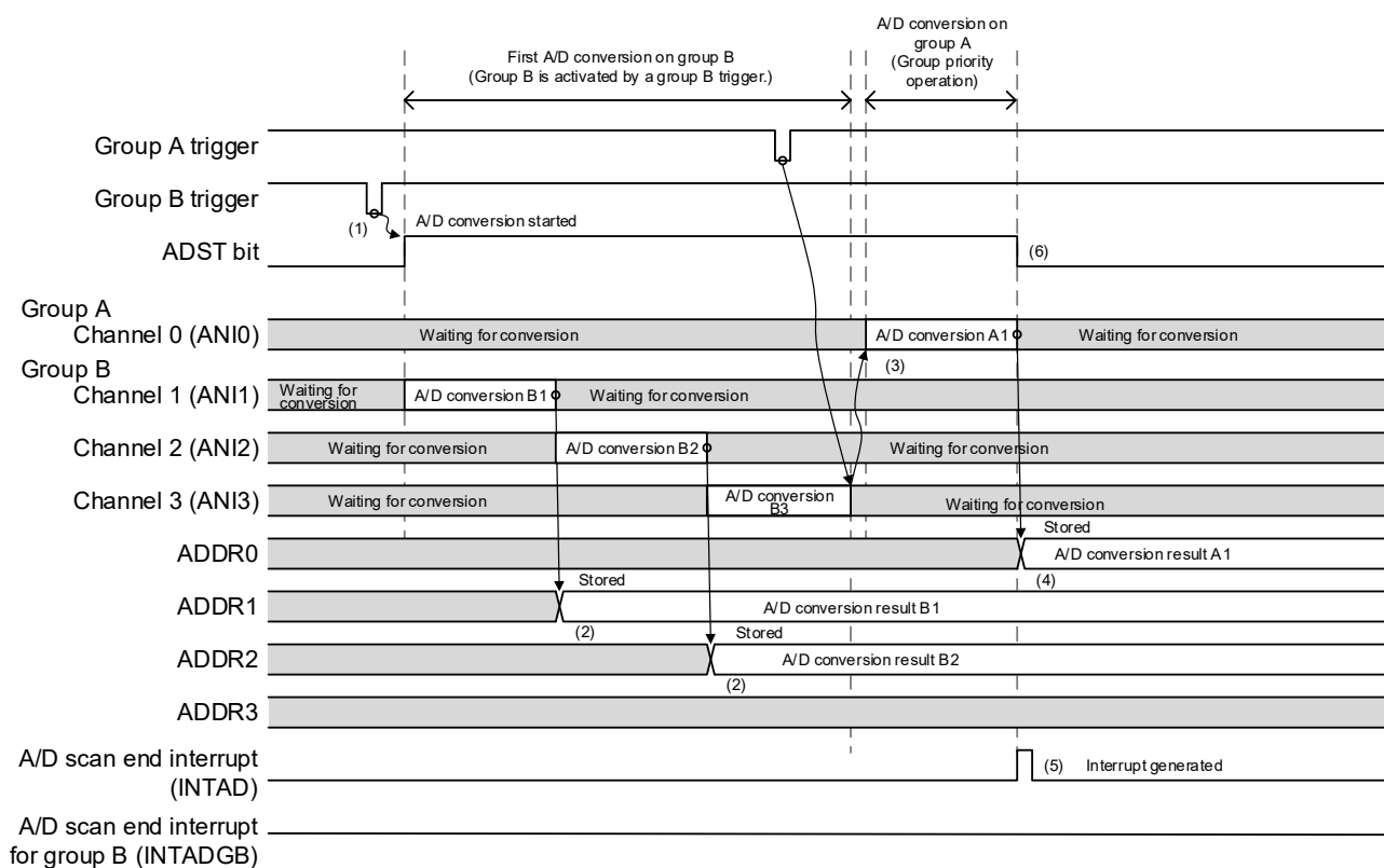
Figure 12-33. Group Priority Operation Example 4: Group A Trigger is Input During Group B Scan when Rescanning is Disabled (when \text{ADGSPCR.GBRSCN} = 0 , \text{ADGSPCR.GBRP} = 0 , and \text{ADGSPCR.LGRRS} = 0 )
