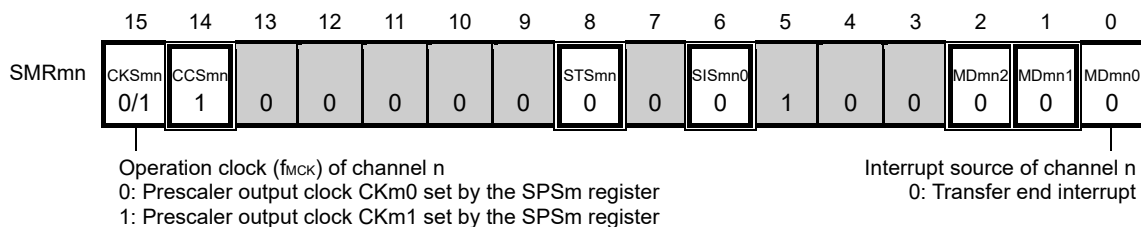
Figure 15-59. Example of Contents of Registers for Slave Reception of 3-Wire Serial I/O (CSI00, CSI01, CSI10, CSI11) (1/2)
