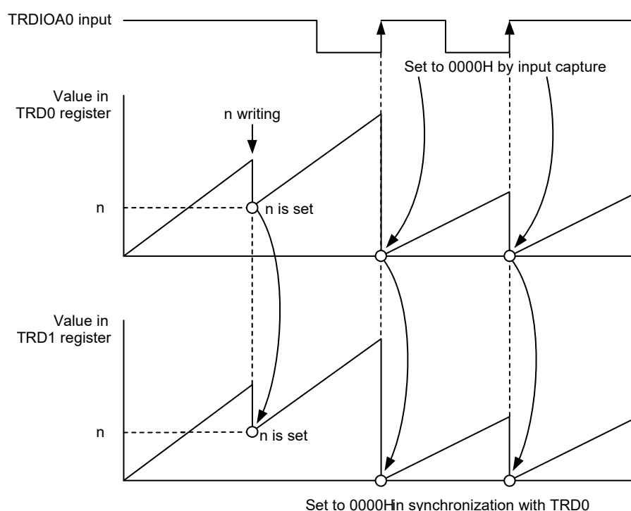
Figure 8-40. Synchronous Operation
