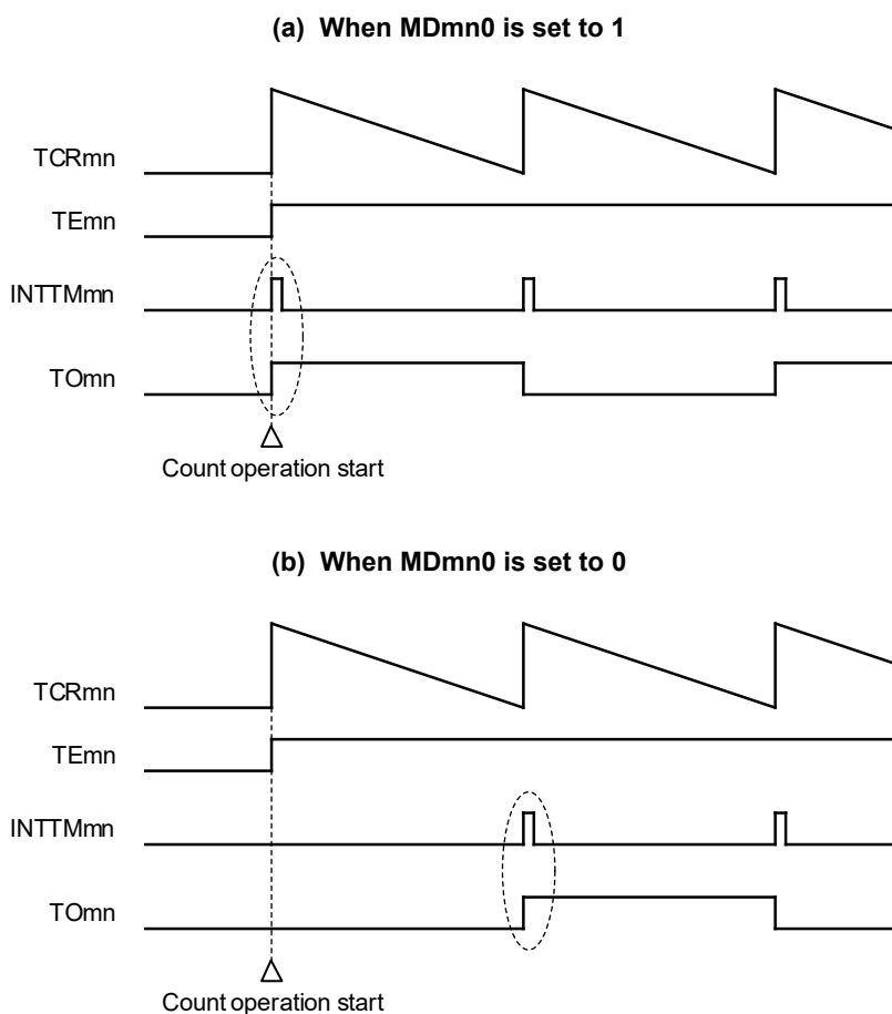
Figure 6-42. Operation Examples of Timer Interrupt at Count Operation Start and TOMn Output
