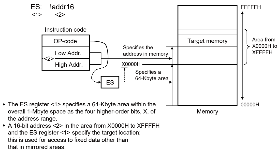
Figure 3-20. Example of ES:!addr16
