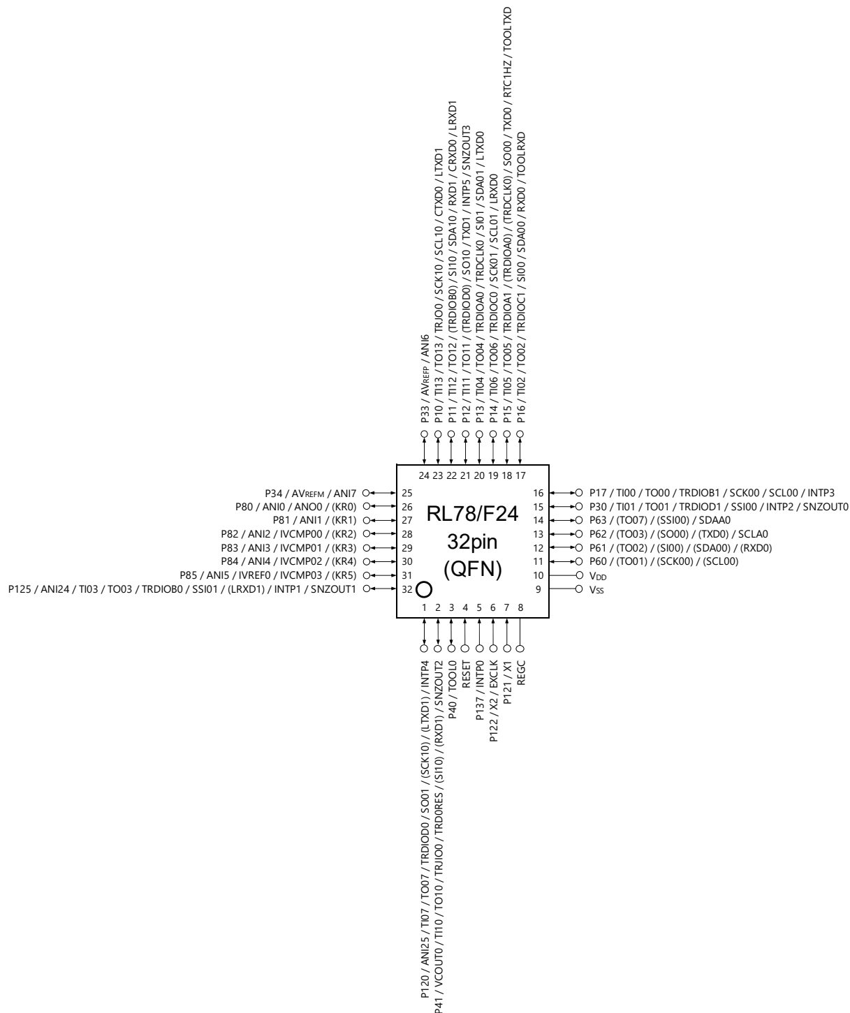
Figure 1-17. RL78/F24 Pin Configuration for 32-pin Products
