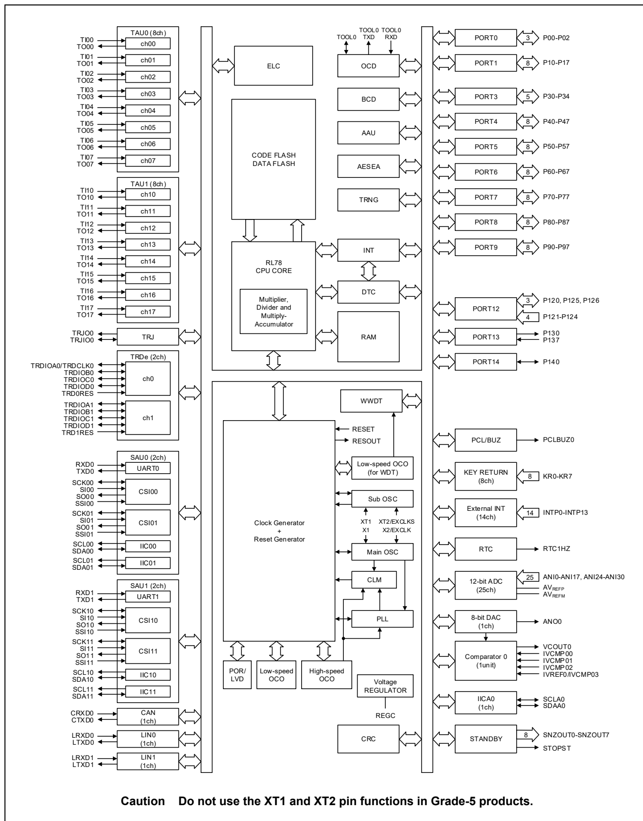
Figure 1-2. Block Diagram
