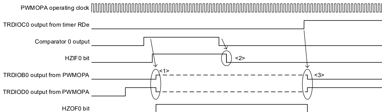
Figure 8-98. Operation Example of Hardware Cutoff Release Function (An Example of TRDIOB0 and TRDIOD0)
