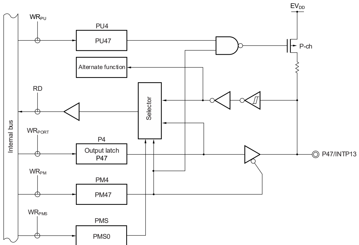
Figure 4-24. Block Diagram of P47
