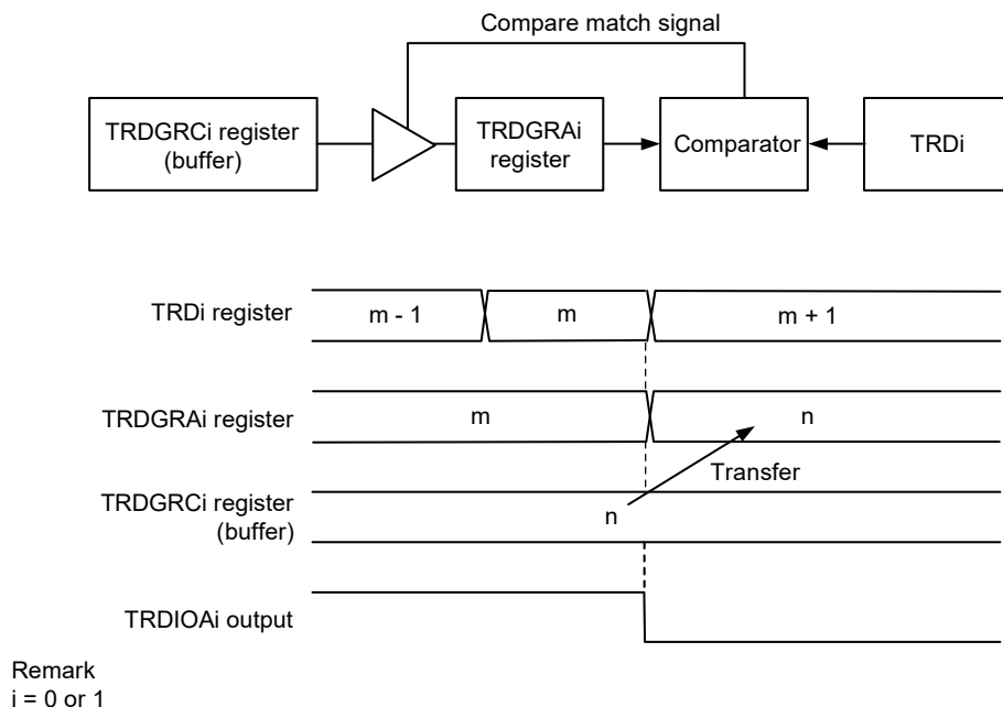
Figure 8-39. Buffer Operation in Output Compare Function
