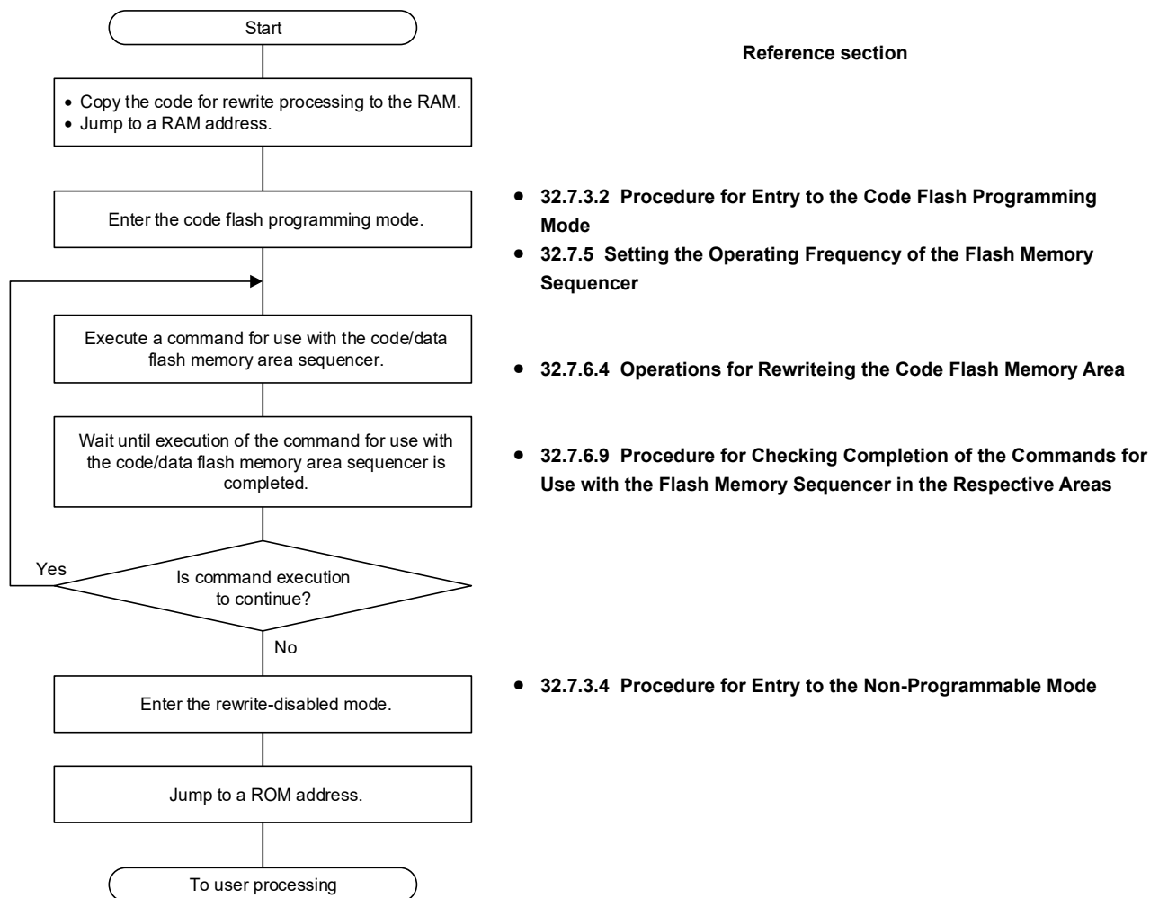
Figure 32-29. Flow of Executing the Commands to Rewrite the Code Flash Memory Area
