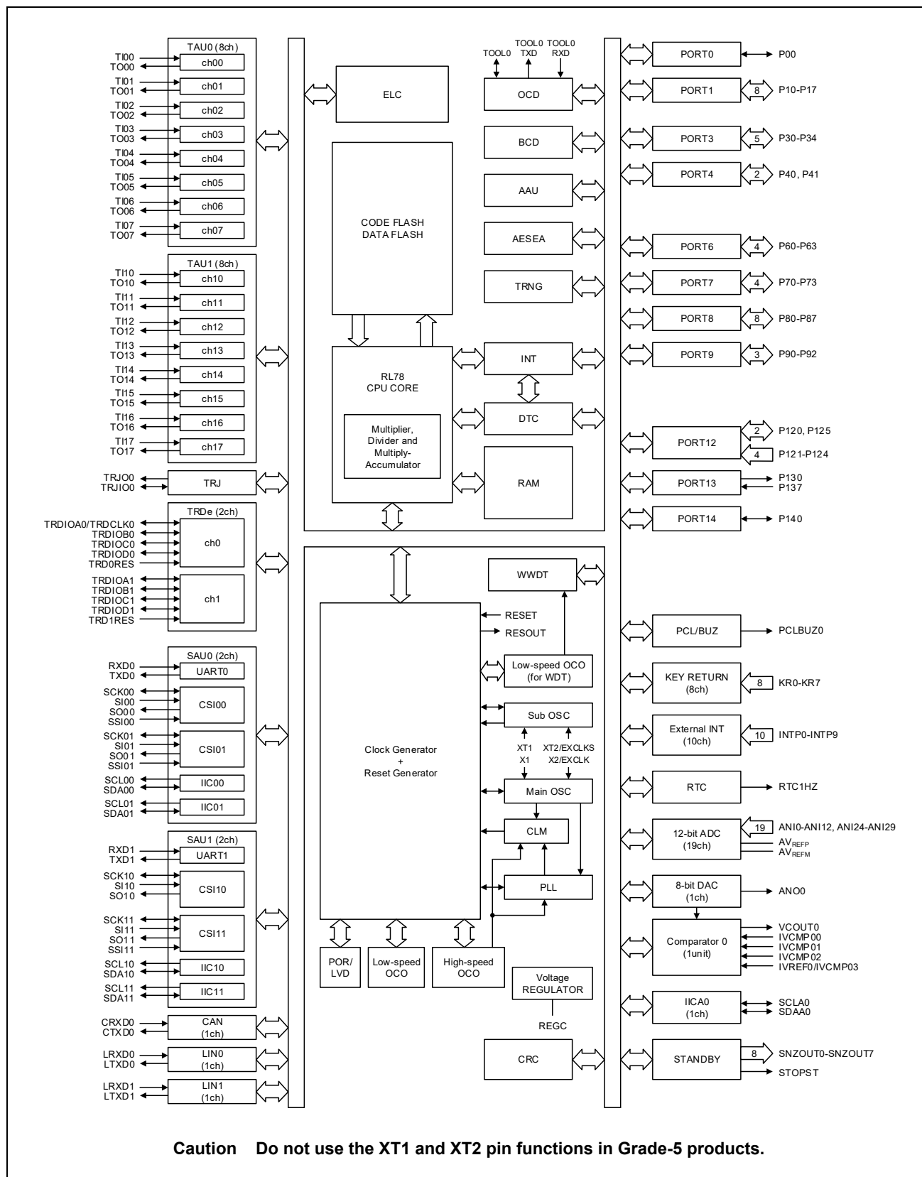
Figure 1-4. Block Diagram
