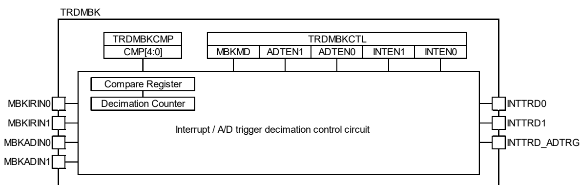
Figure 8-116. TRDMBK Block Diagram
