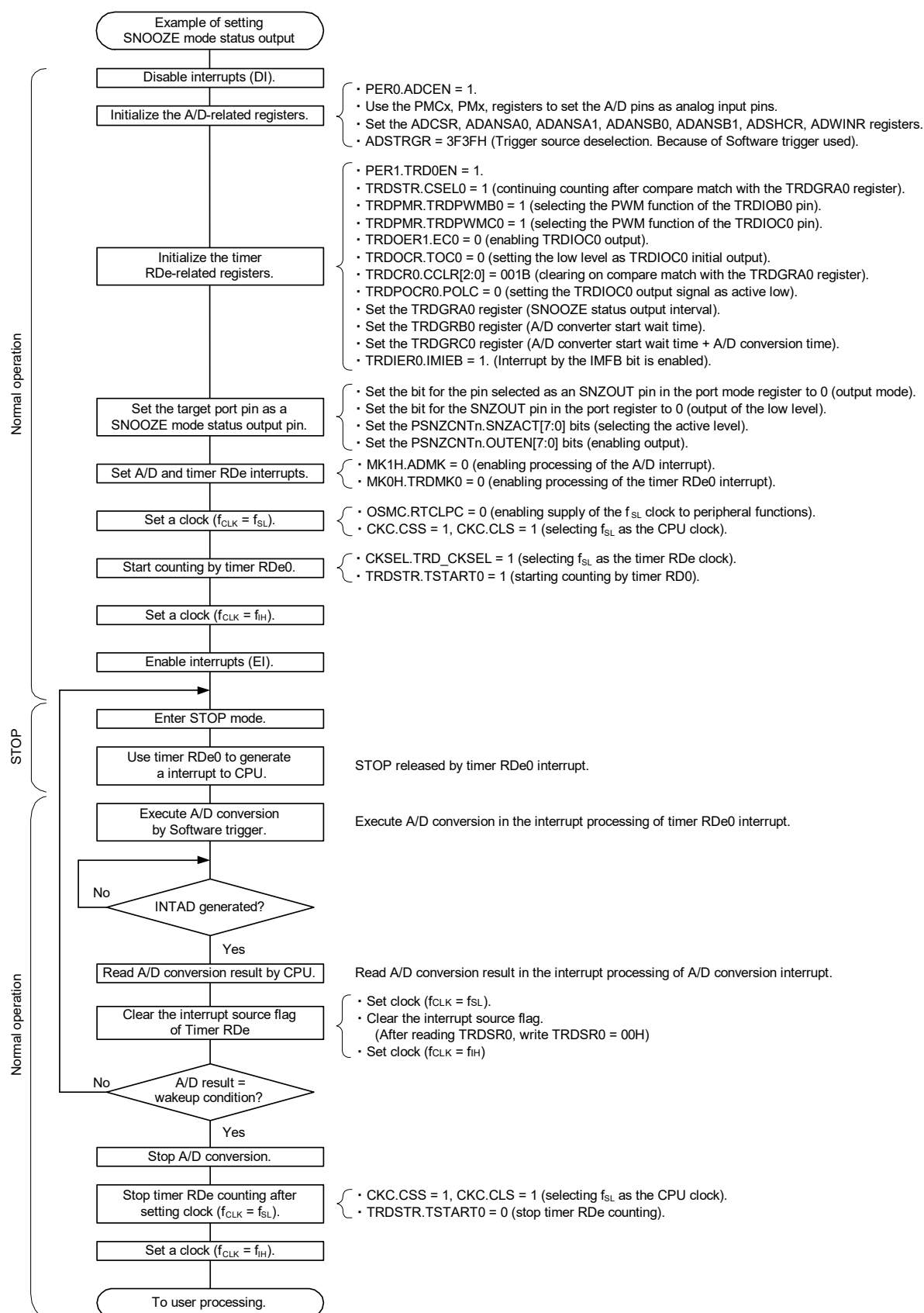
Figure 23-10. Example of Settings for SNOOZE Mode Status Output
