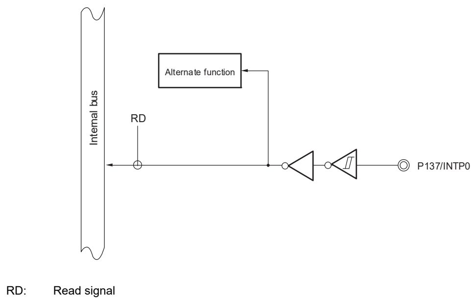
Figure 4-67. Block Diagram of P137
