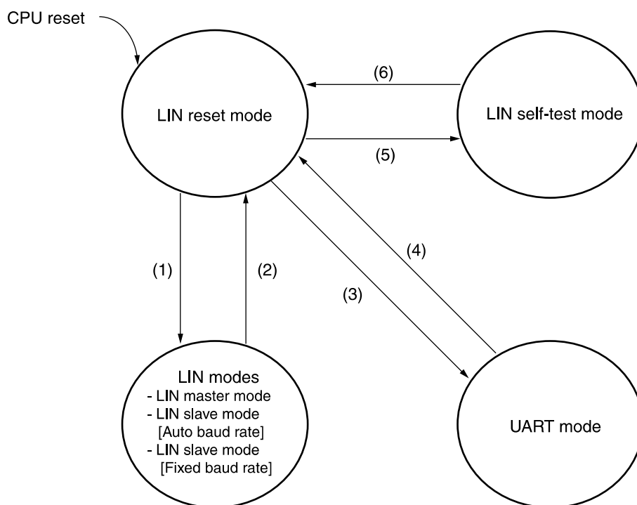
Figure 17-3. Mode Transitions
