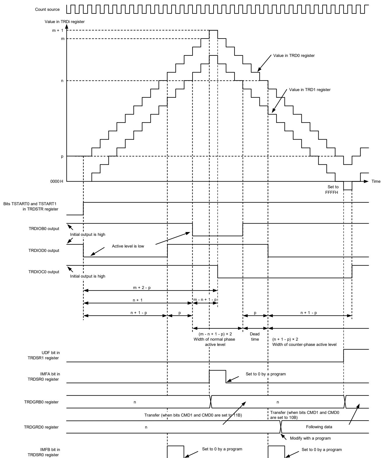
Figure 8-58. Operation Example in Complementary PWM Mode
