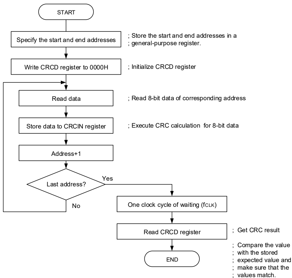
Figure 28-7. CRC Operation Function (General-Purpose CRC)
