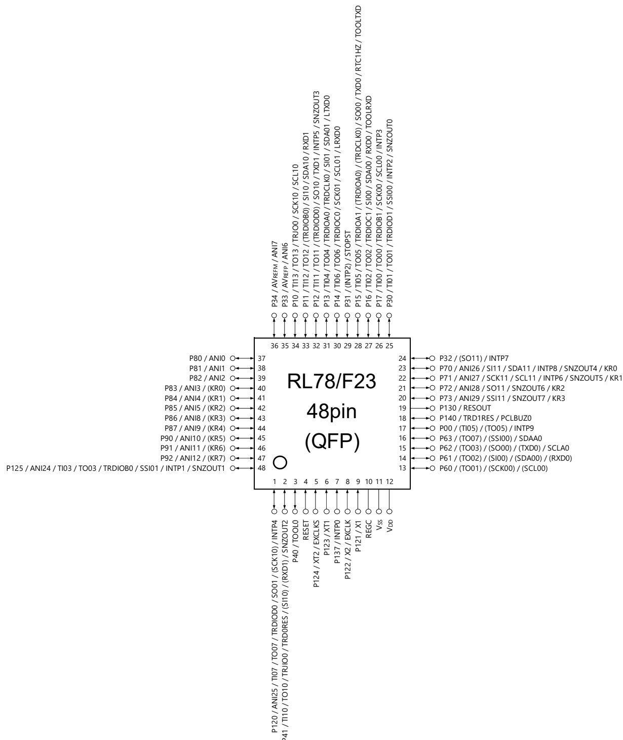
Figure 1-16. RL78/F23 Pin Configuration for 48-pin Products
