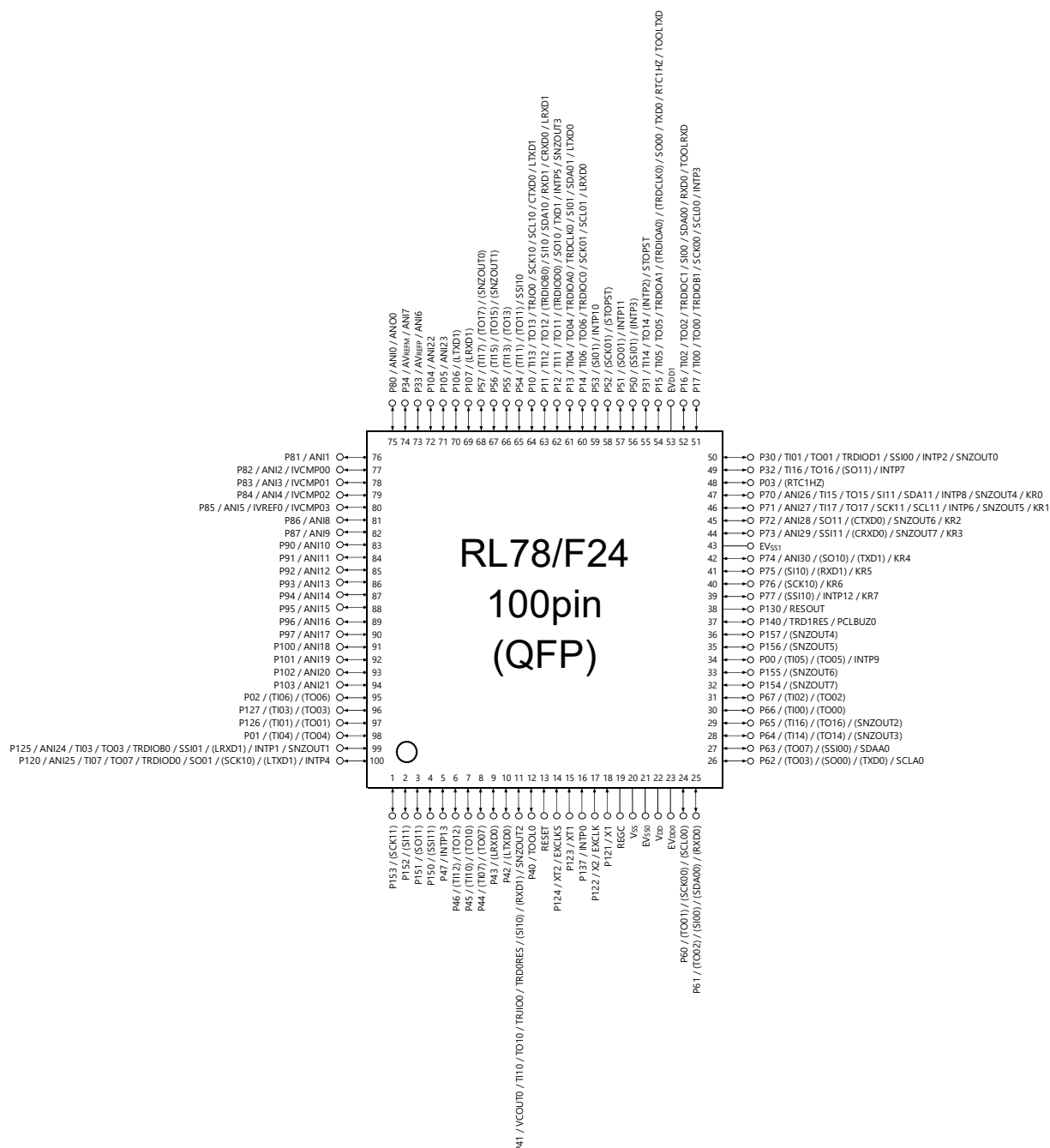
Figure 1-10. RL78/F24 Pin Configuration for 100-pin Products
