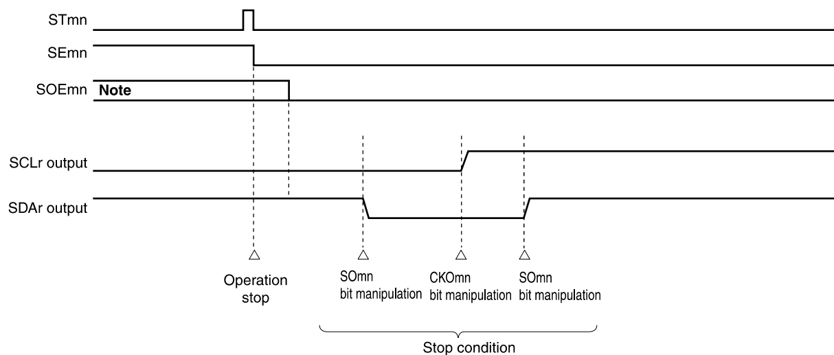
Figure 15-155. Timing Chart of Stop Condition Generation
