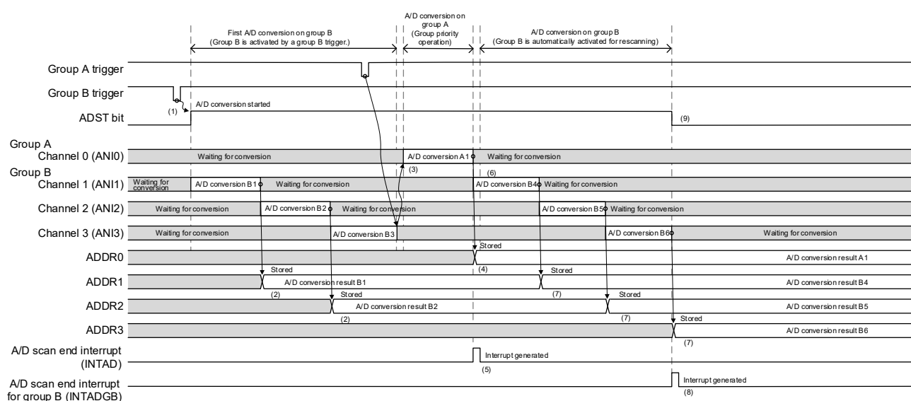
Figure 12-30. Example of Group Priority Operation 1: Group A Trigger Input During Group B Scanning when Rescanning is Enabled (when ADGSPCR.GBRSCN = 1, ADGSPCR.GBRP = 0, and ADGSPCR.LGRRS = 0)
