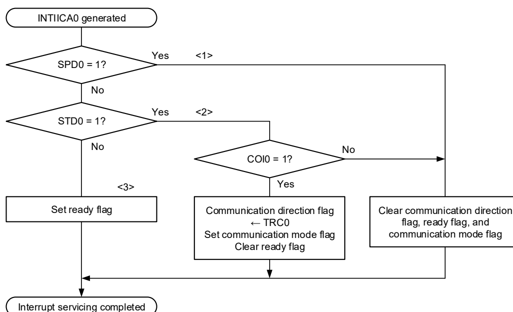
Figure 16-31. Slave Operation Flowchart (2)
