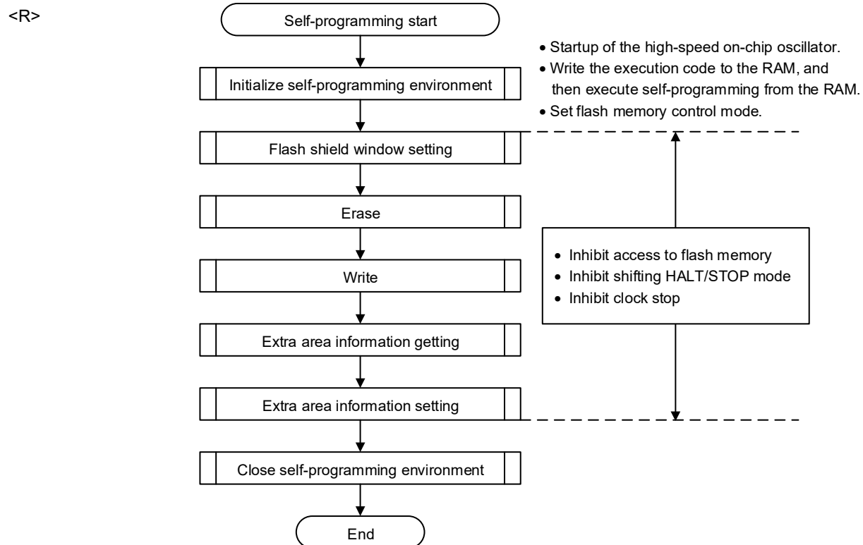
Figure 32-8. Flow of Self-Programming (Rewriting Flash Memory)
