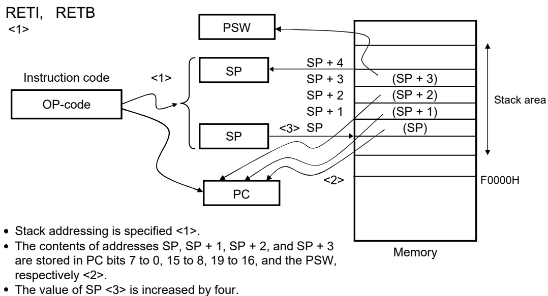
Figure 3-39. Example of RETI, RETB
