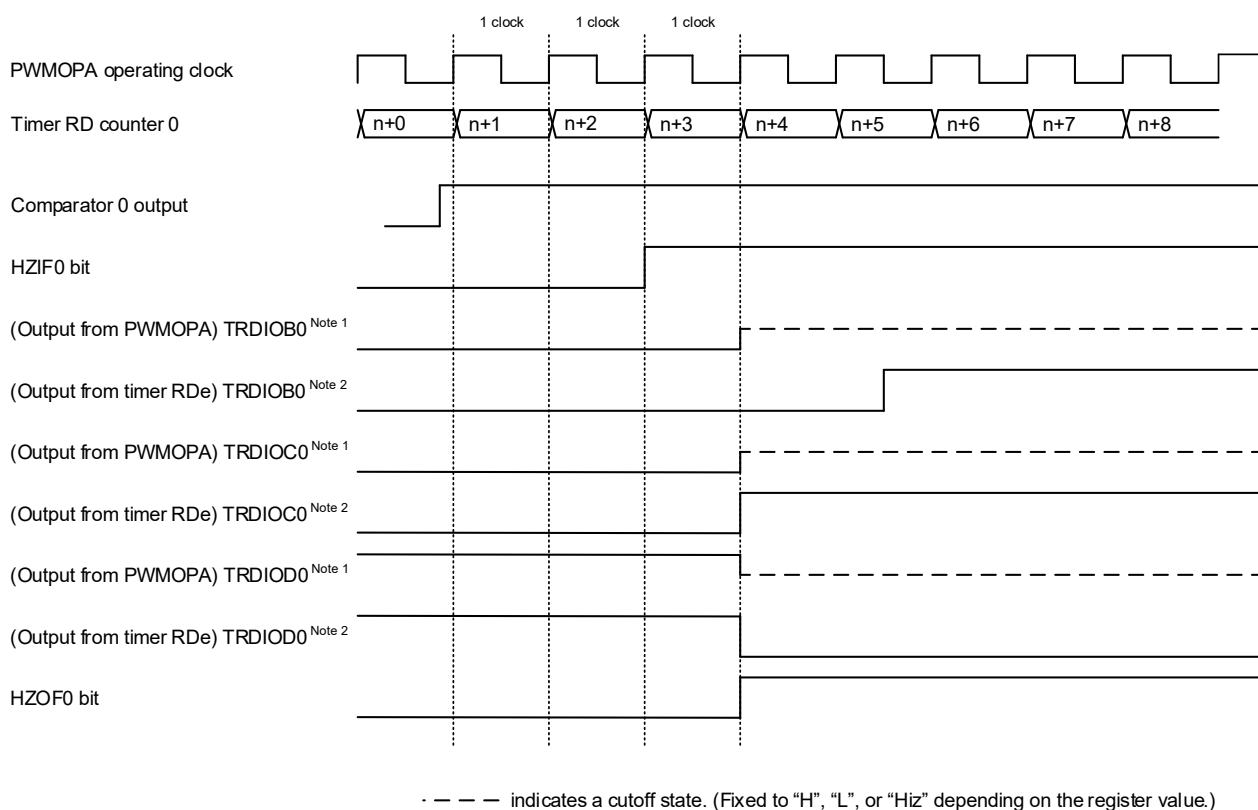
Figure 8-95. Cutoff Detailed Timing Diagram
