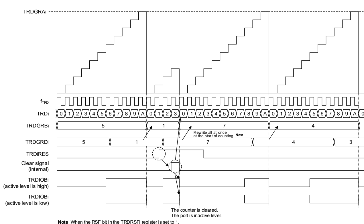
Figure 8-64. Operation Example of Counter Restart Function
