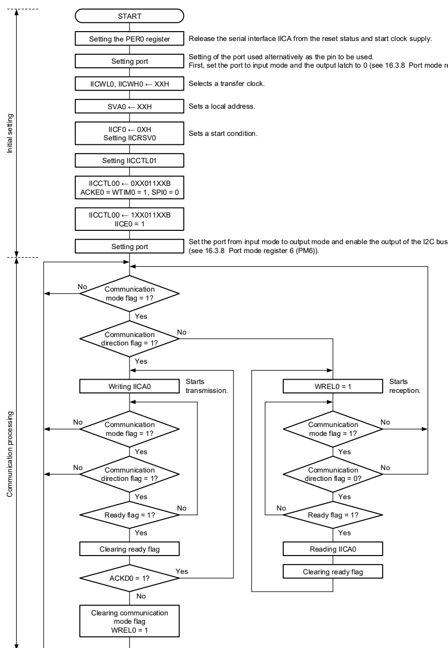
Figure 16-31. Slave Operation Flowchart (1)
