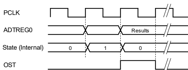
Figure 27-38. Timing Diagram of Single Arithmetic Operation
