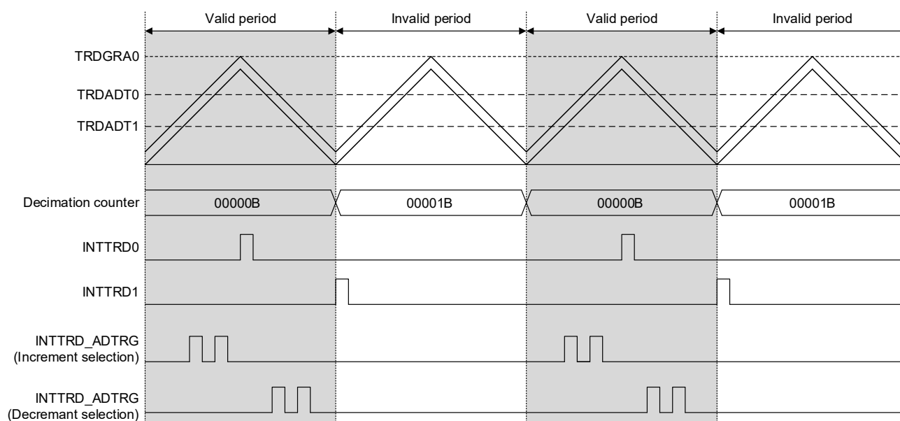
Figure 8-120. Operation Example in Extended Complementary PWM Mode (Decimated once)
