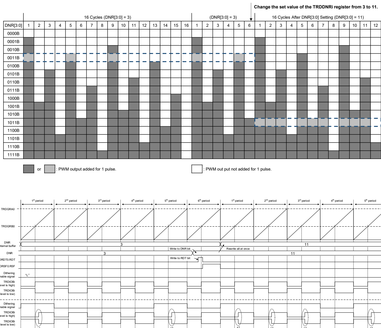
Figure 8-68. Operation Example of Dithering Function (Change the Setting Value from 3 to 11)
