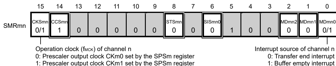
Figure 15-100. Example of Contents of Registers for Slave Transmission of SPI Function (CSI00, CSI01, CSI10, CSI11) (1/2)
