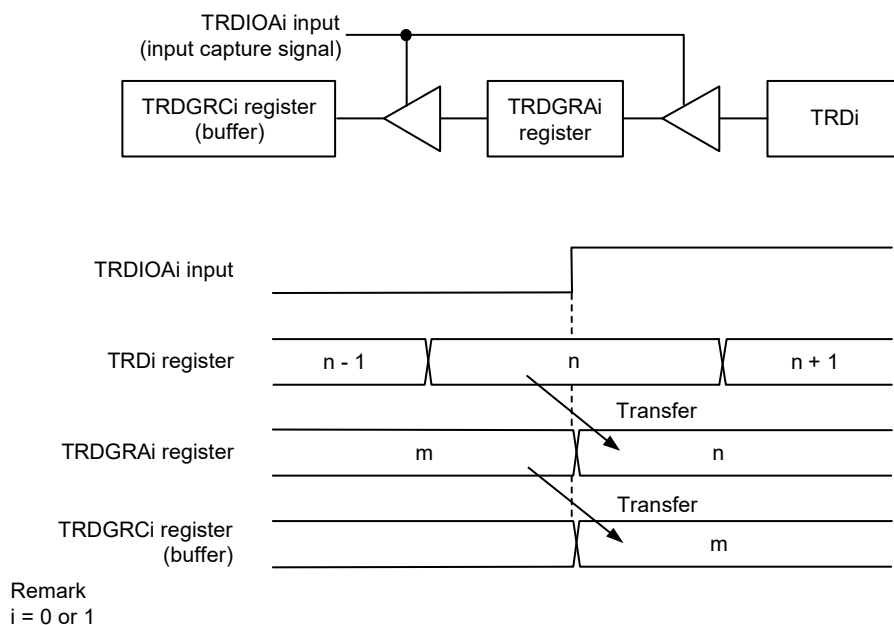
Figure 8-38. Buffer Operation in Input Capture Function
