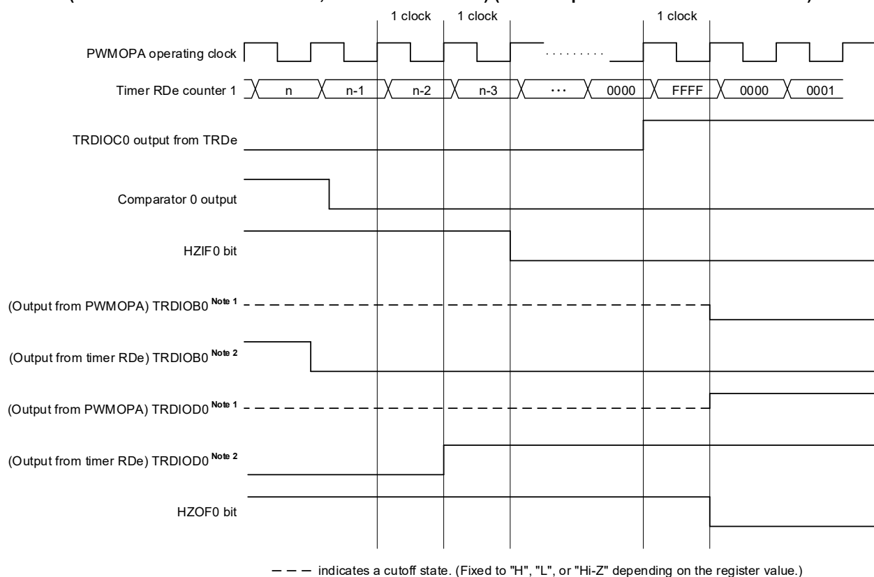
Figure 8-99. Cutoff Release Detailed Timing Diagram (Timer RDe Count Source = f_{CLK} , TRD1 Decrementing) (An Example of TRDIOB0 and TRDIOD0)
