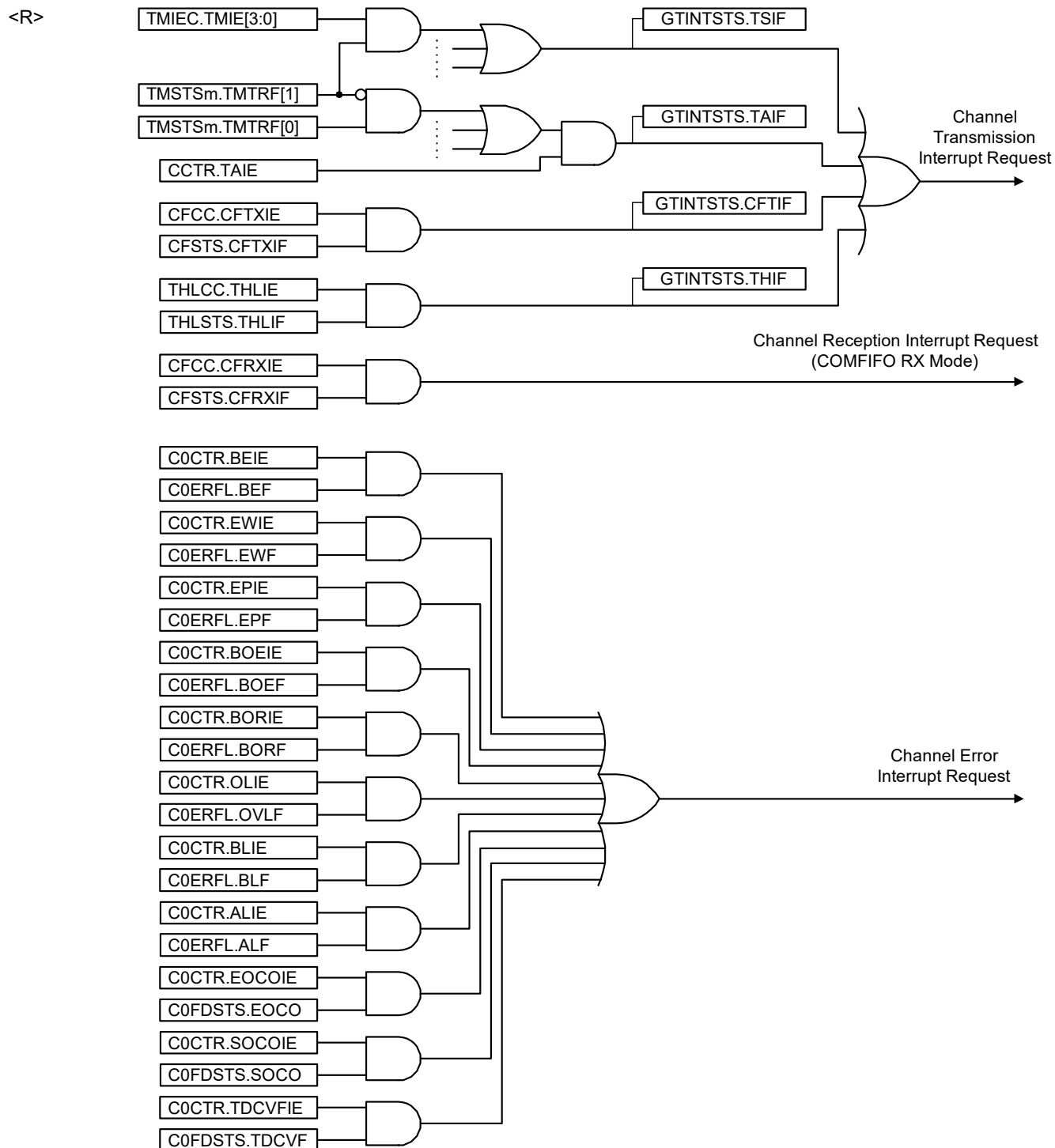
Figure 18-45. Channel Interrupt Block Diagram
