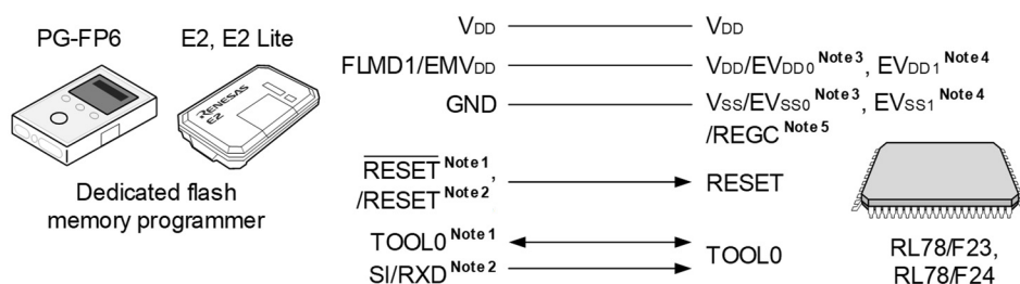
Figure 32-2. Communication with Dedicated Flash Memory Programmer
