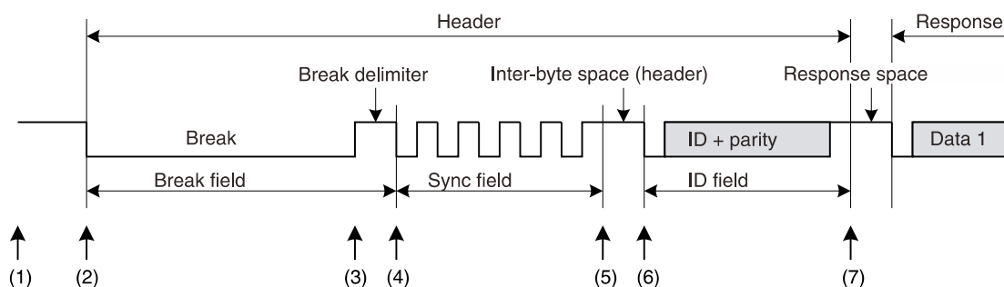
Figure 17-5. Operation in Header Transmission
