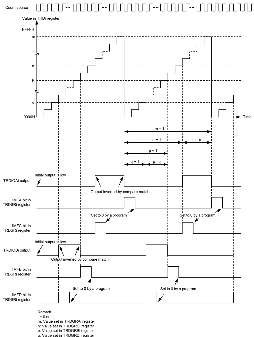
Figure 8-50. Operation Example When TRDGRCi Register is Used for Output Control of TRDIOAi Pin and TRDGRDi Register is Used for Output Control of TRDIOBi Pin
