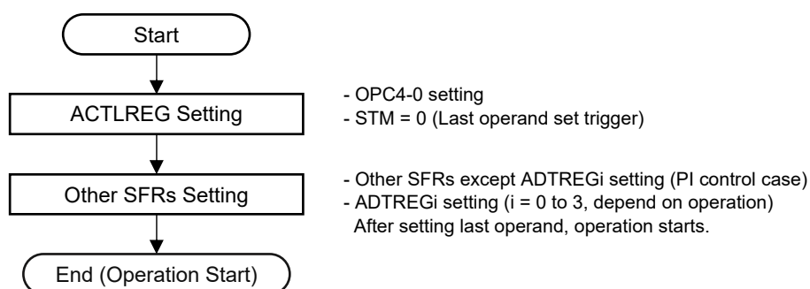
Figure 27-36. Processing Flow of Operation Start
