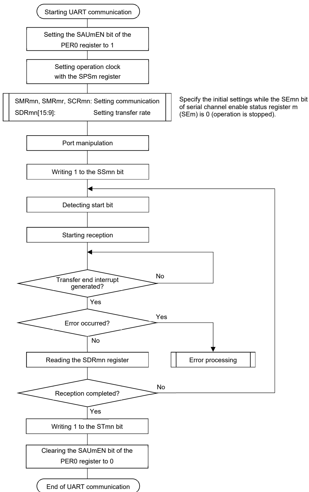
Figure 15-136. Flowchart of UART Reception
