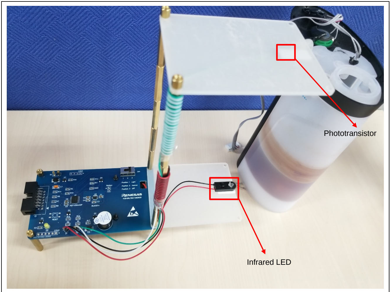
Figure 4.1 Board Picture
