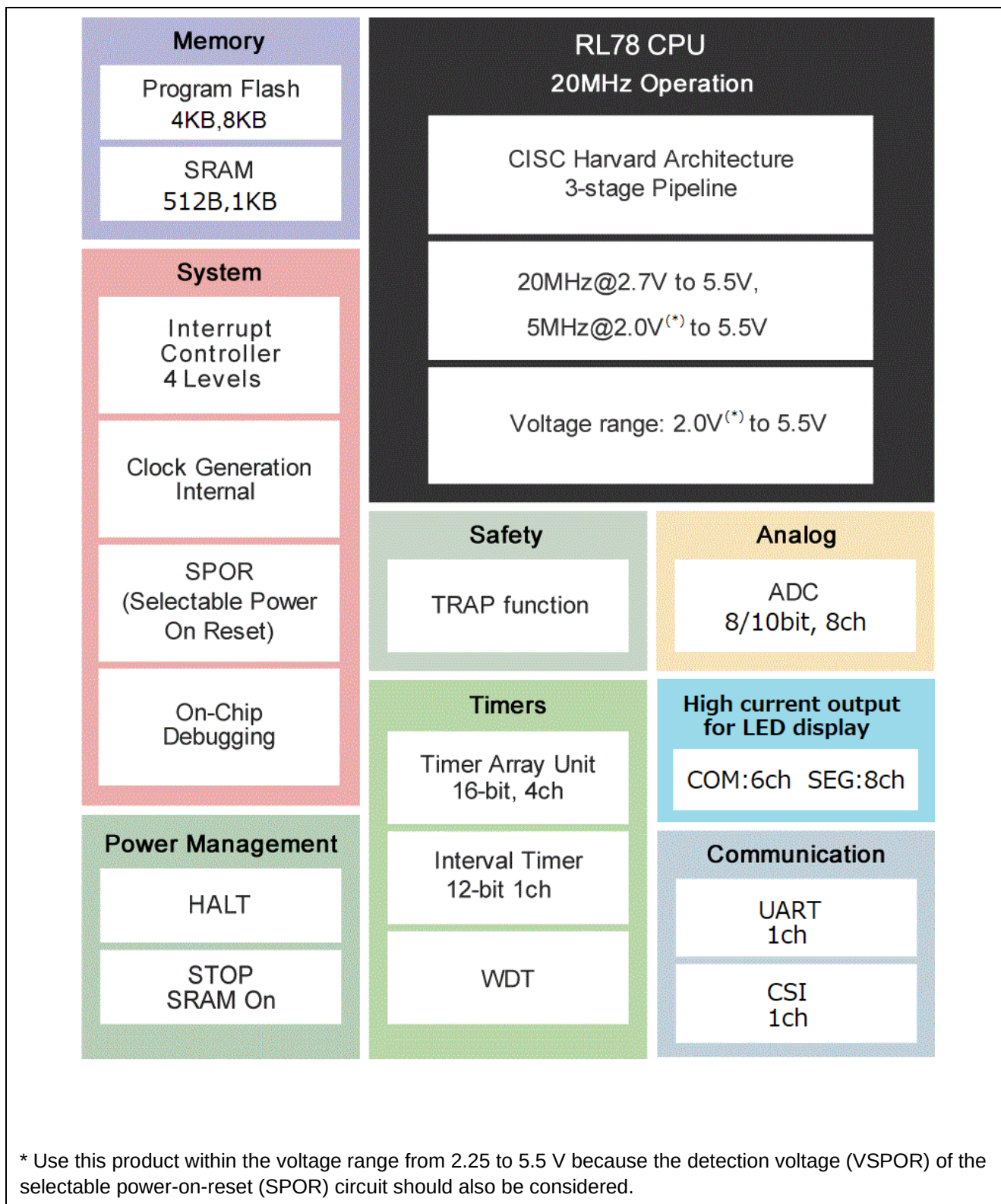
Figure 2.1 RL78/G1N (20-pin products) Block Diagram
