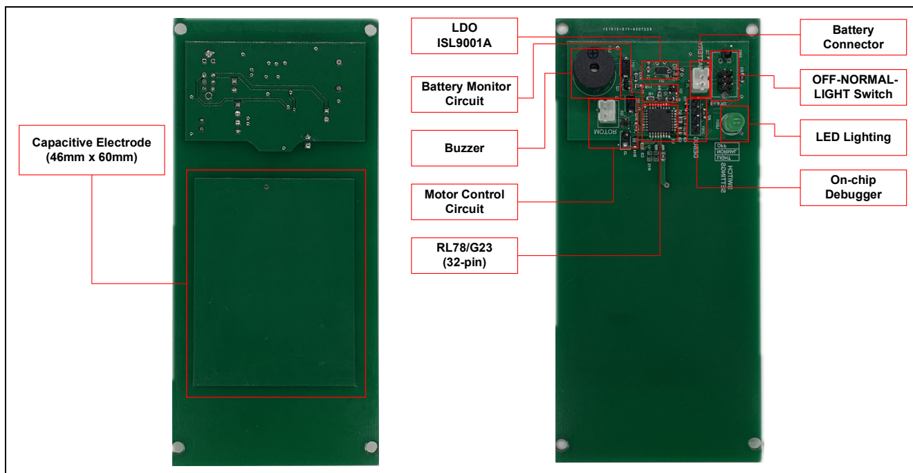
Figure 4.2 Demo Board (Top layer and Bottom layer)
