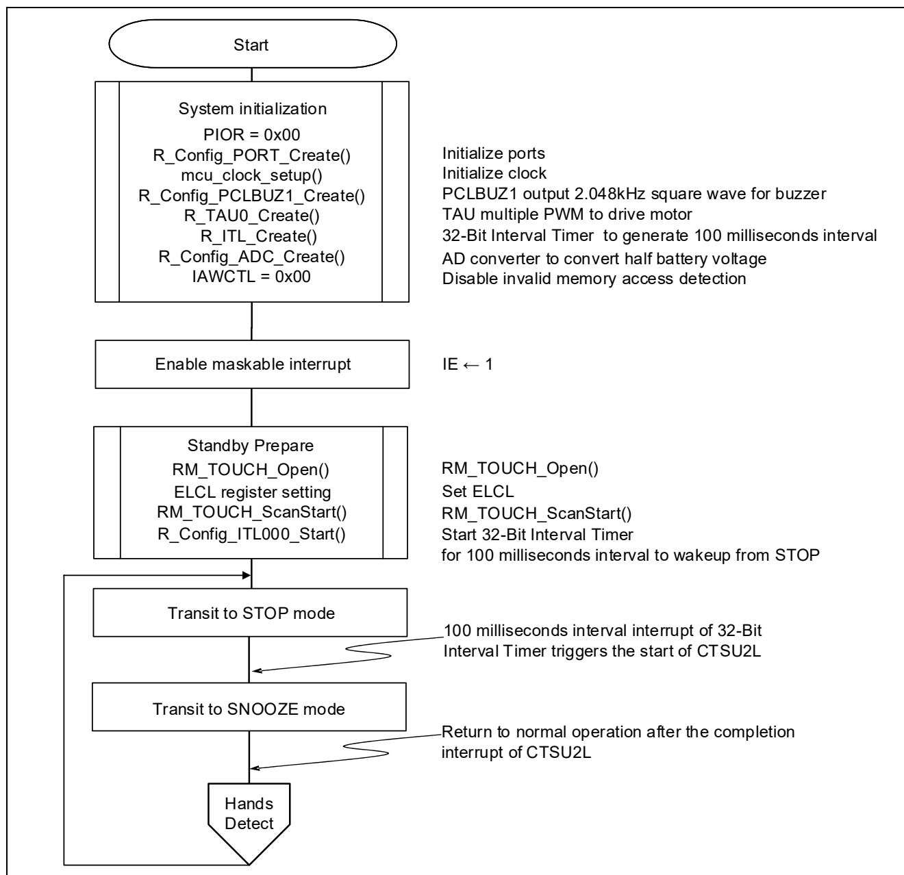
Figure 5.2 Main Processing (1/2)
