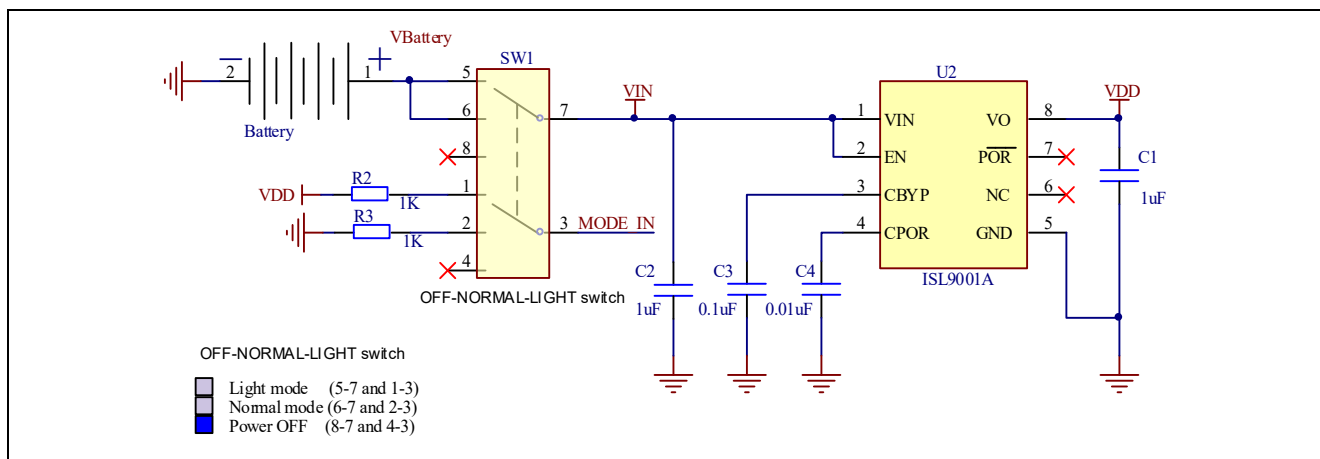
Figure 4.3 Power Supply
