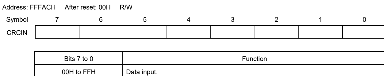
Figure 23-4. Format of CRC Input Register (CRCIN)
