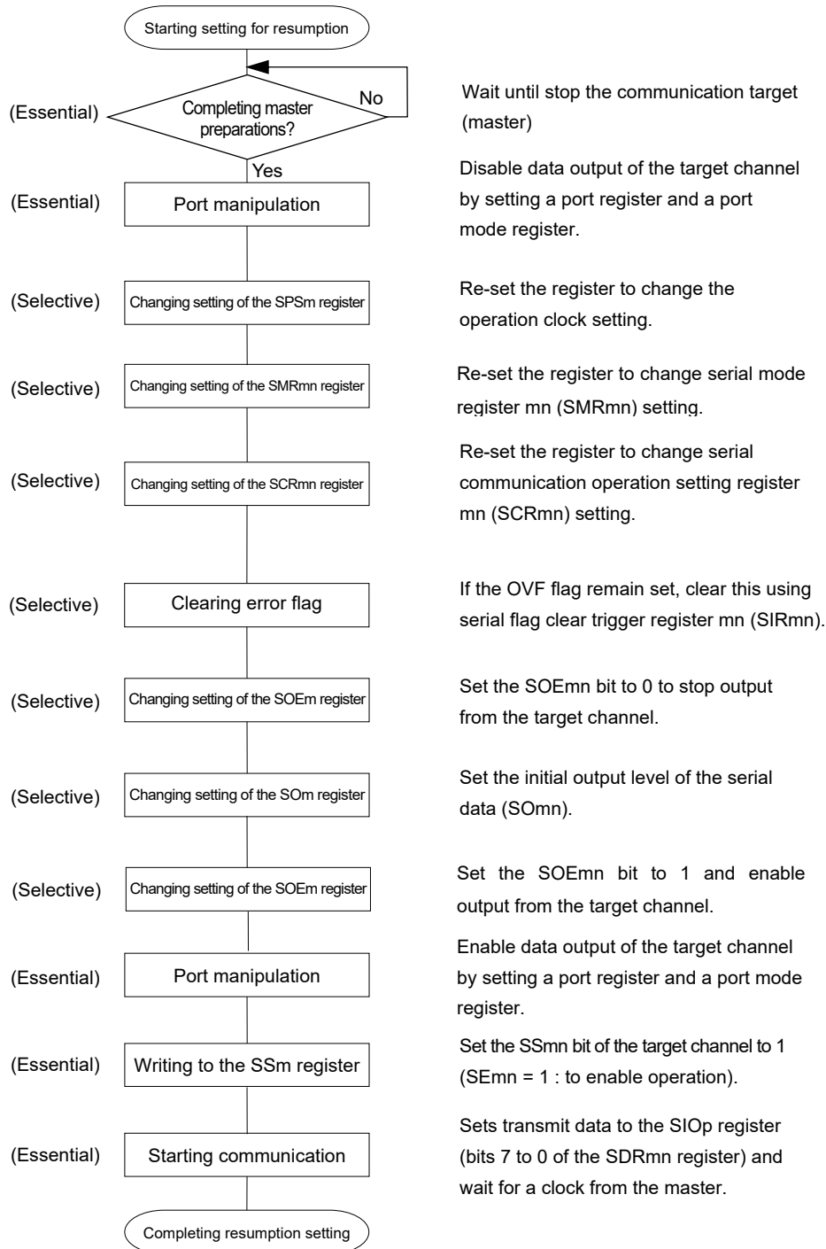
Figure 12-64. Procedure for Resuming Slave Transmission/Reception
