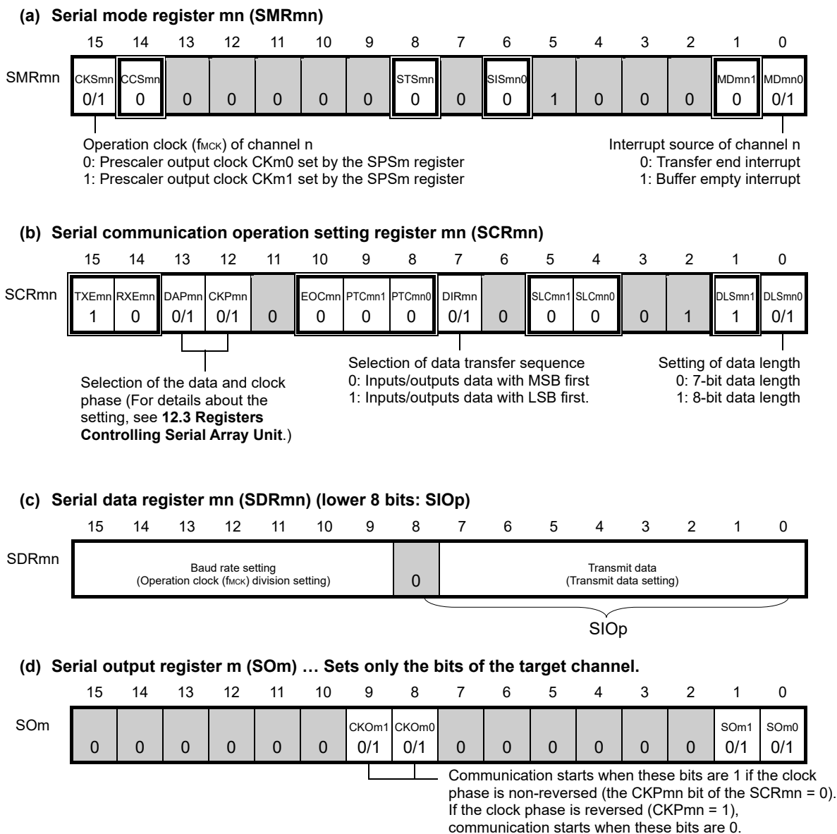
Figure 12-23. Example of Contents of Registers for Master Transmission of simplified SPI (CSI00, CSI01) (1/2)
