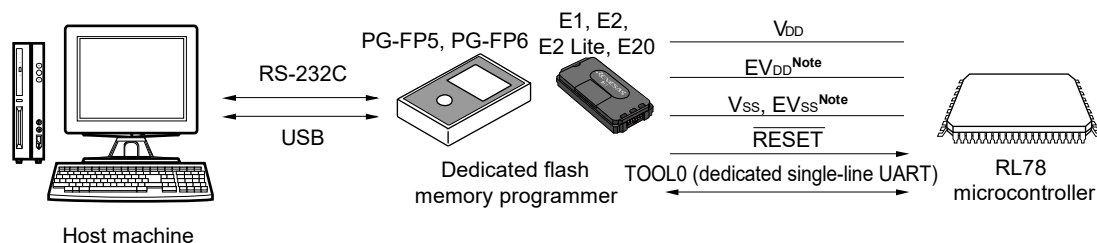
Figure 26-1. Environment for Writing Program to Flash Memory
