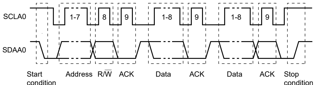
Figure 13-14. I 2 C Bus Serial Data Transfer Timing
