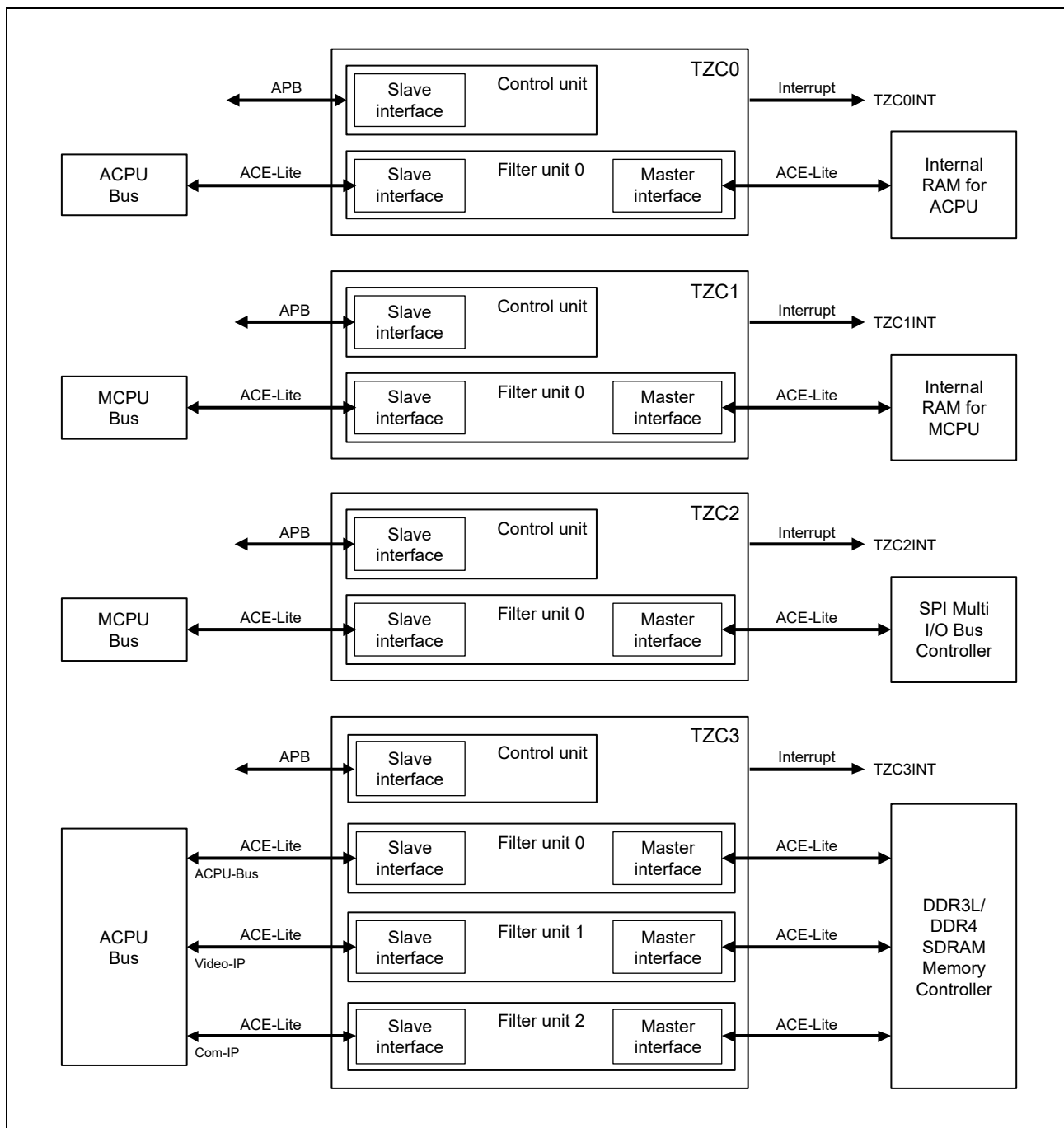
Figure 13.1 Block Diagram
