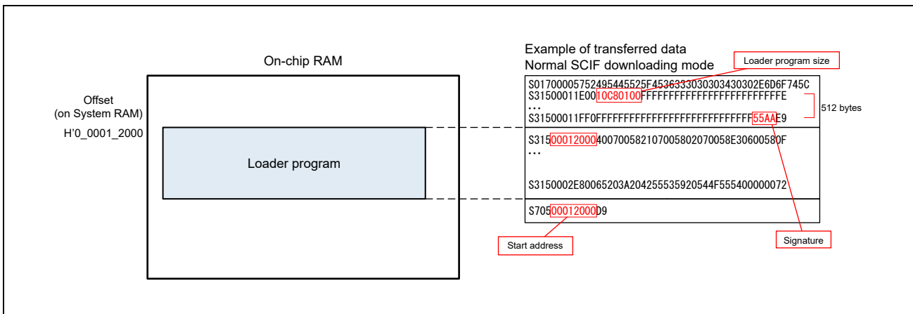
Figure 4.20 Allocation of the Loader Program for SCIF Downloading Copied to the On-chip RAM
