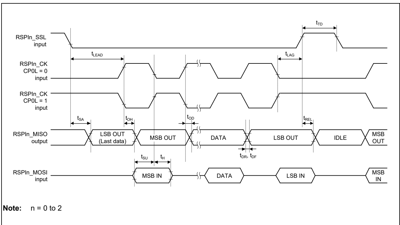
Figure 48.48 Transmission and Reception Timing (Slave, CPHA = 1)
