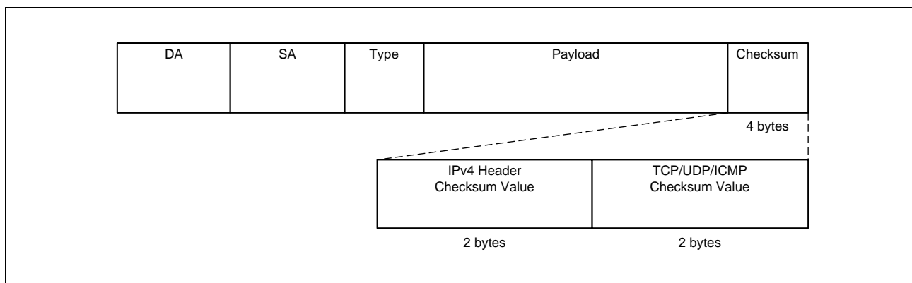
Figure 30.25 The field of checksum attaching field (Ex. Ethernet Frame of DIX)
