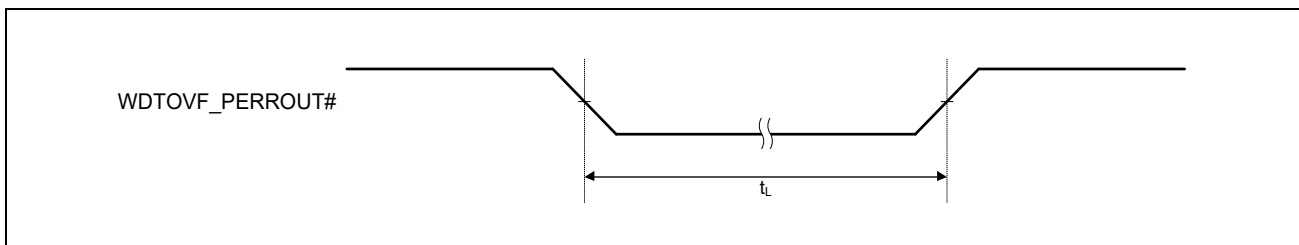
Figure 48.50 Watchdog Timer Output Timing
