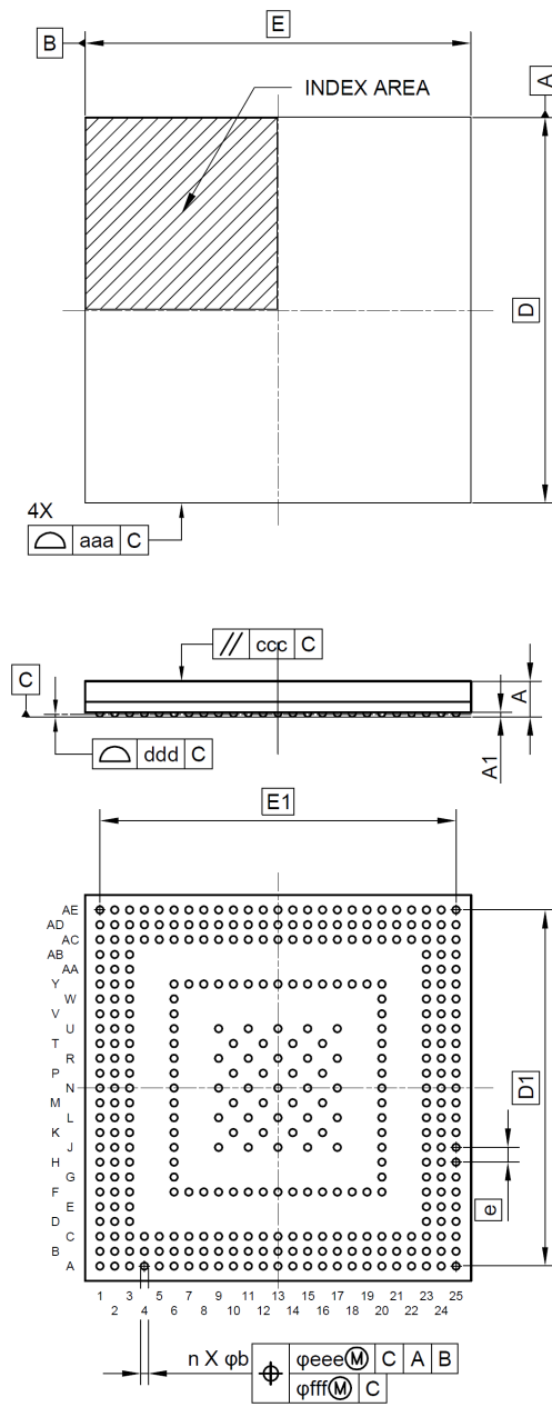
Appendix A.1 Package Dimensions (361-pin BGA, 13-mm Square, 0.5-mm Pitch)
