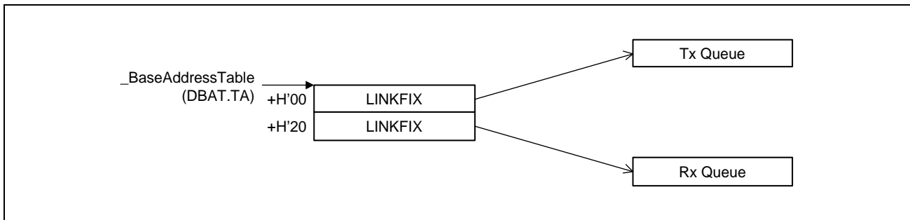
Figure 30.5 Example of a Base Address Table for Reception and Transmission Queues
