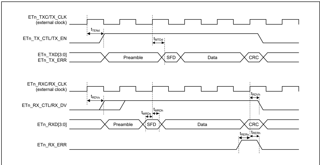
Figure 48.18 MII Transmission Timing
