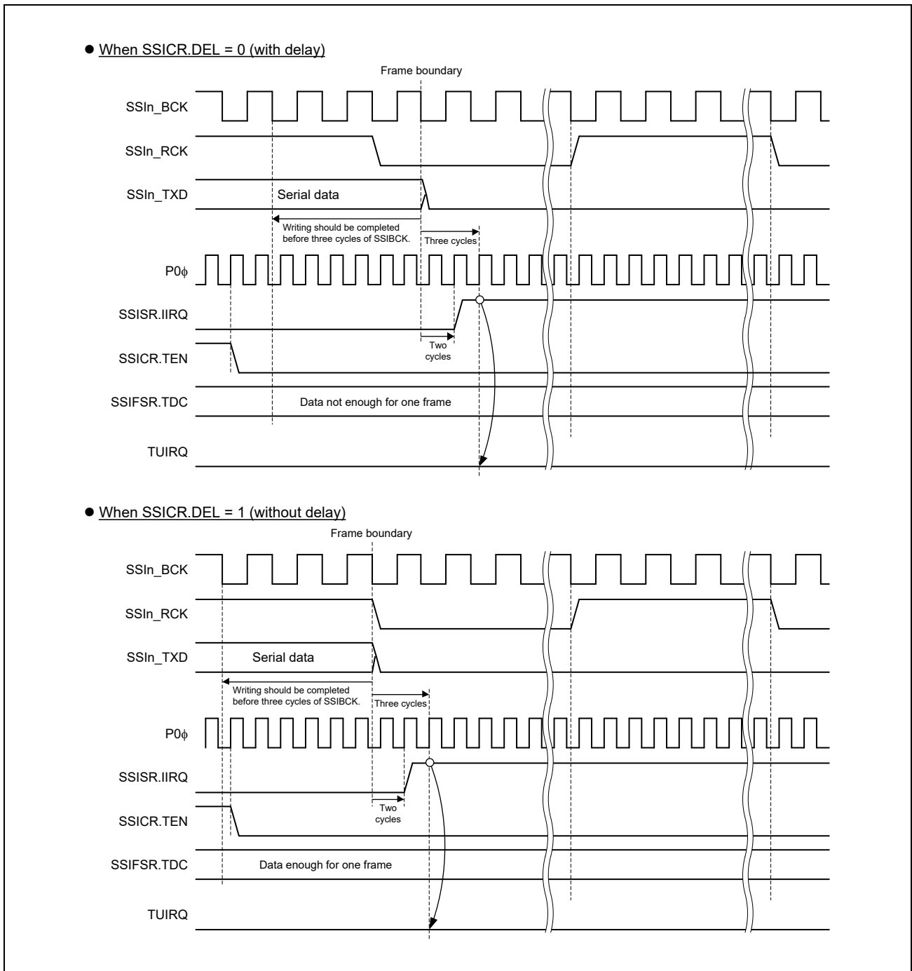
Figure 27.15 TUIRQ Setting Timing (When you stop communicating)
