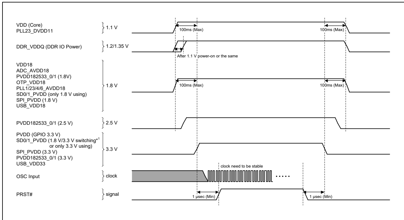
Figure 48.1 Power-On/Power-Off Sequence
