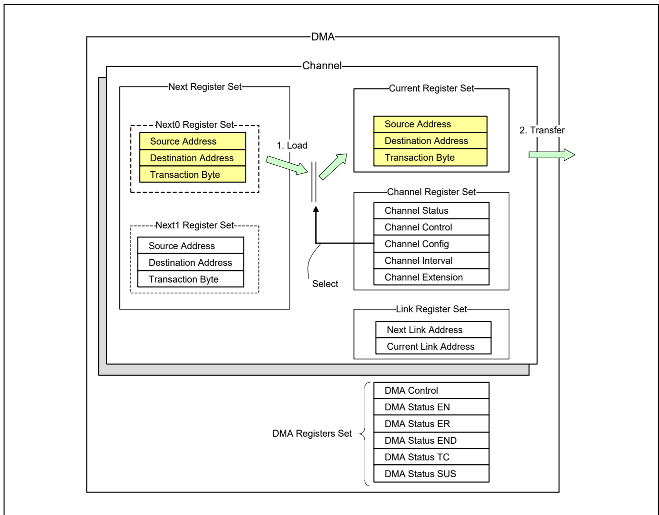
Figure 14.1 Register Configuration
