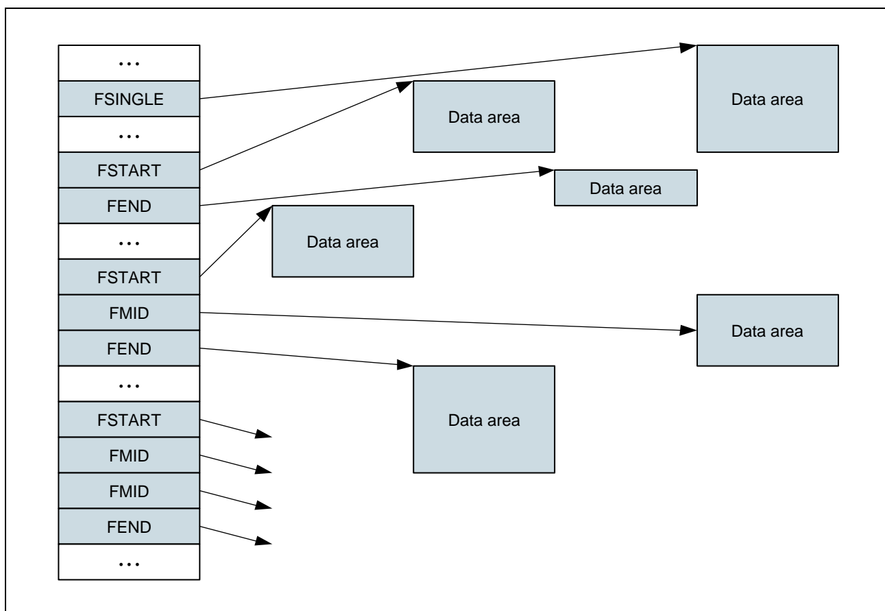
Figure 30.11 Mapping of Frame Data
