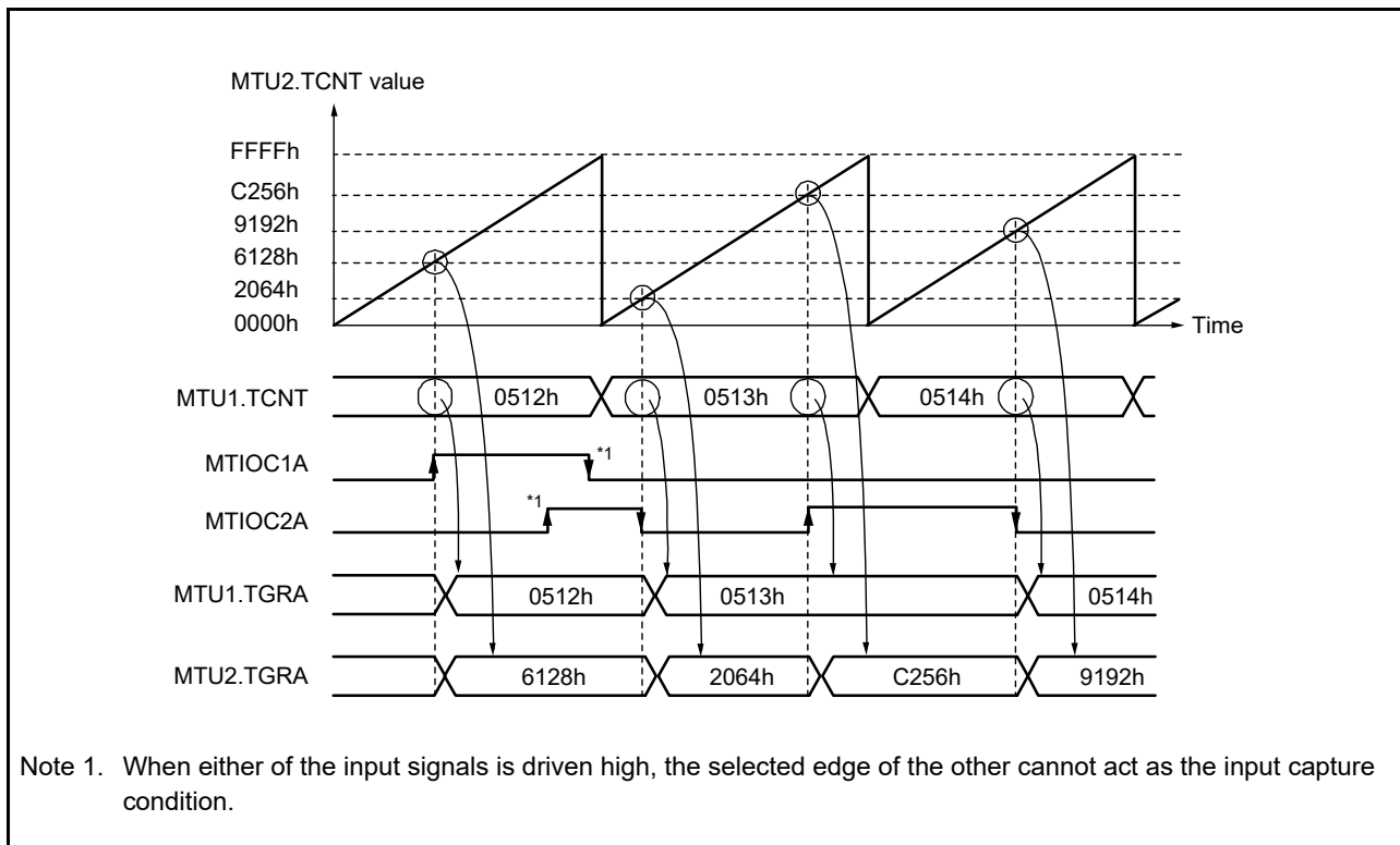
Figure 19.24 Cascaded Operation Example (c)
