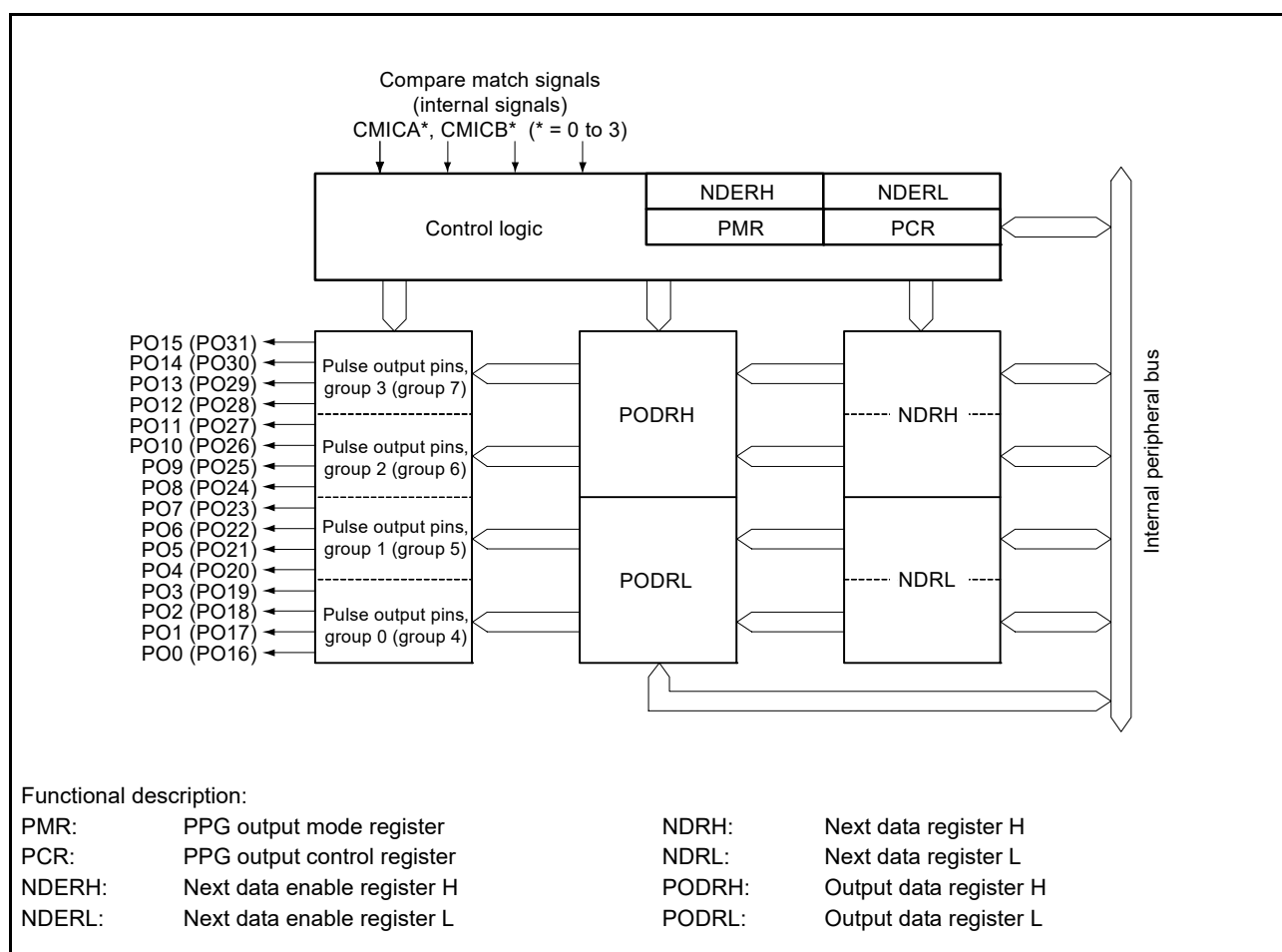
Figure 23.1 Block Diagram of PPG
