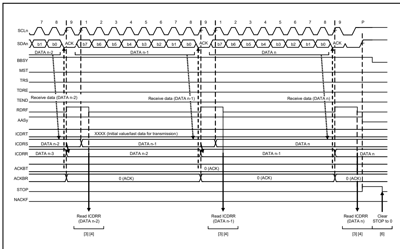
Figure 34.20 Slave Receive Operation Timing (2) (when RDRFS = 0)
