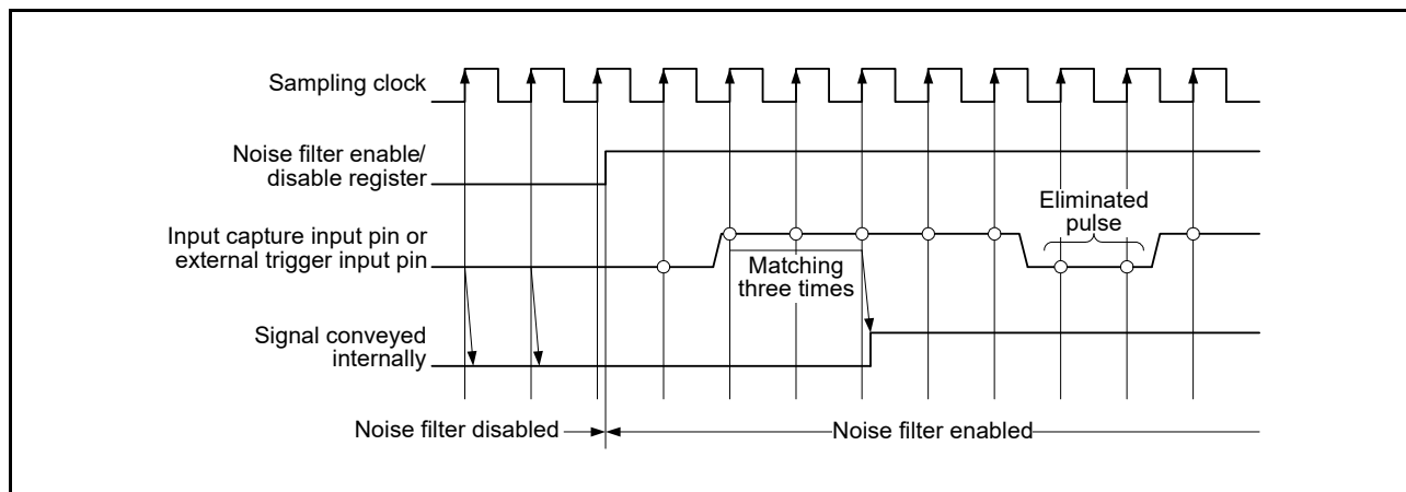
Figure 21.68 Timing of Noise Filtering
