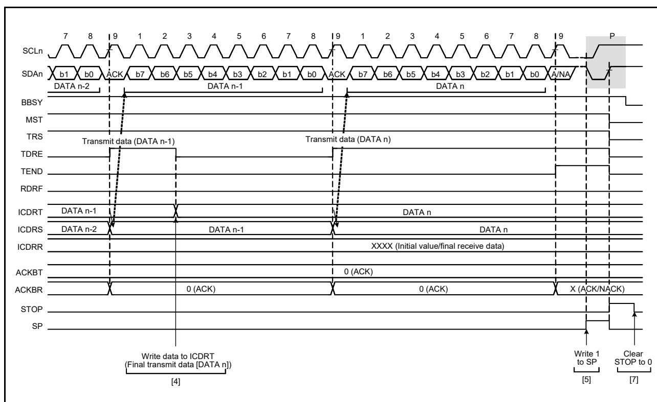
Figure 34.9 Master Transmit Operation Timing (3)
