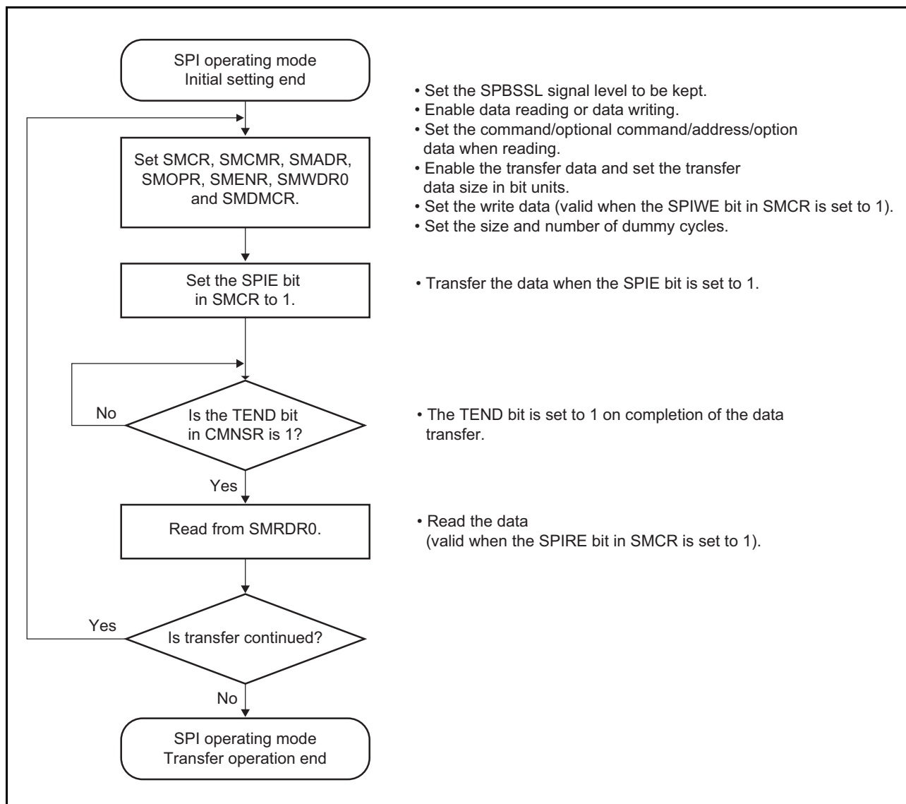
Figure 37.16 Example of a Data Transfer Setting Flow in SPI Operating Mode
