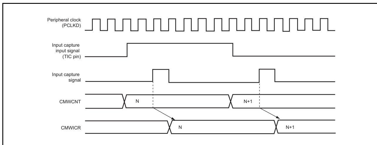
Figure 25.11 Input Capture Input Signal Timing
