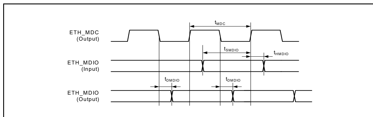
Figure 47.78 Serial Management Access Timing
