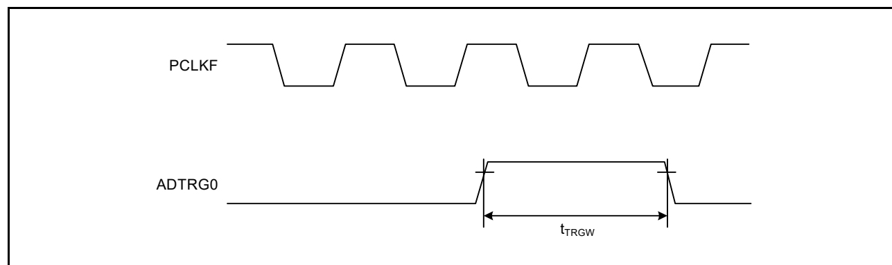
Figure 47.48 A/D Converter Trigger Input Timing (ADTRG0)
