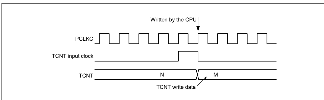
Figure 19.132 Contention between TCNT Write and Clear Operations
