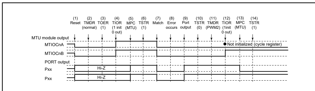
Figure 19.151 Error Occurrence in Normal Mode, Recovery in PWM Mode 2
