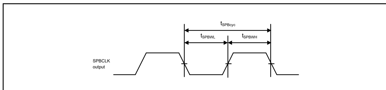
Figure 47.57 SPIBSC Clock Timing
