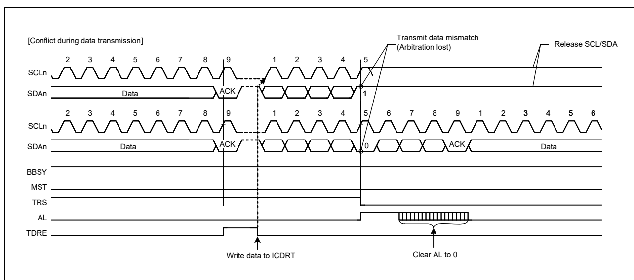
Figure 34.35 Example of Slave Arbitration-Lost Detection (SALE = 1)
