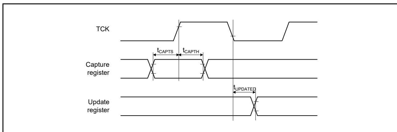
Figure 47.89 Boundary Scan Input/Output Timing
