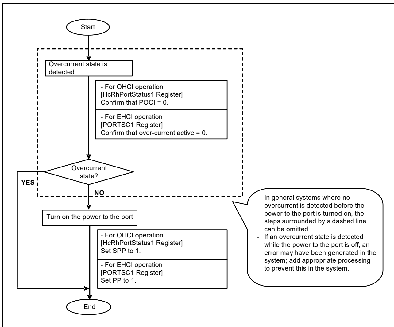
Figure 31.11 Flow for USB_VBUSEN Control Regarding Overcurrent Detection
