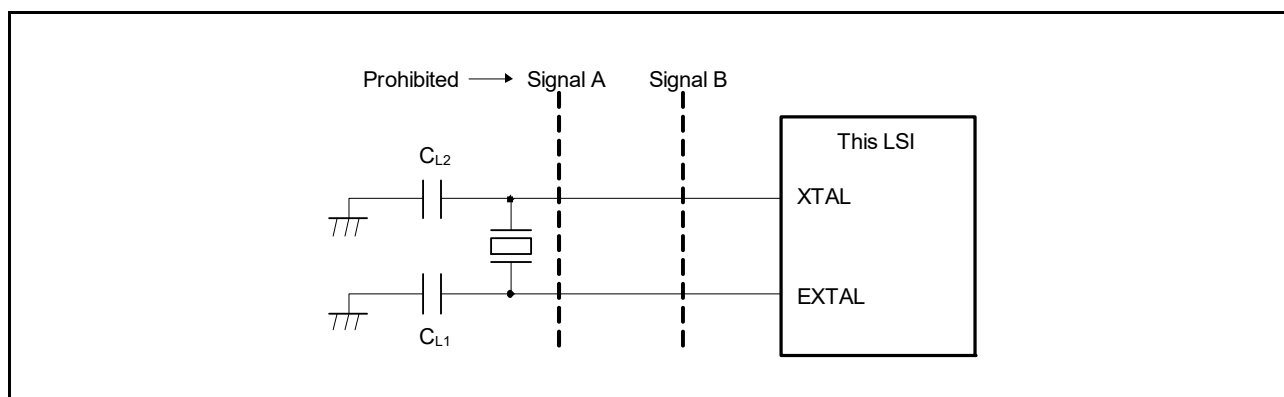
Figure 7.7 Notes on Board Design for Oscillation Circuit
