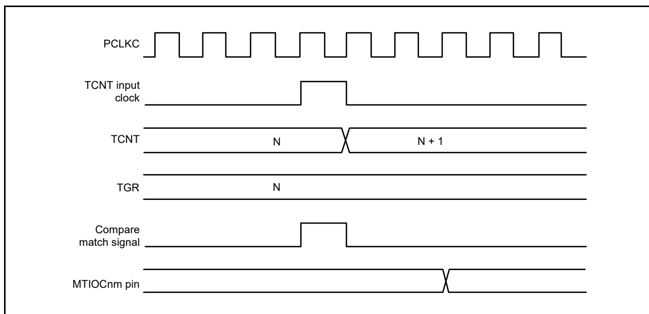
Figure 19.113 Output Compare Output Timing (Complementary PWM Mode or Reset-Synchronized PWM Mode) ( n = 0 to 4, 6, 7, or 8, m = A to D)
