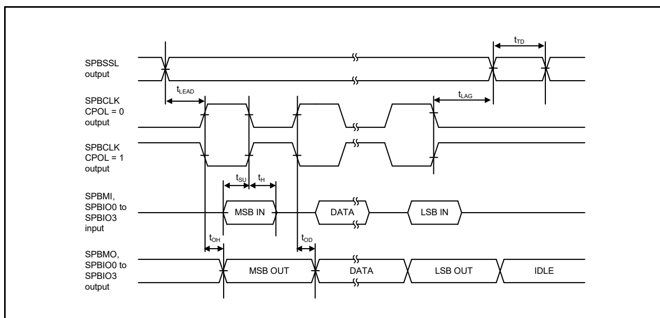
Figure 47.59 SPIBSC Transmit/Receive Timing (CPHAT = 1, CPHAR = 1)
