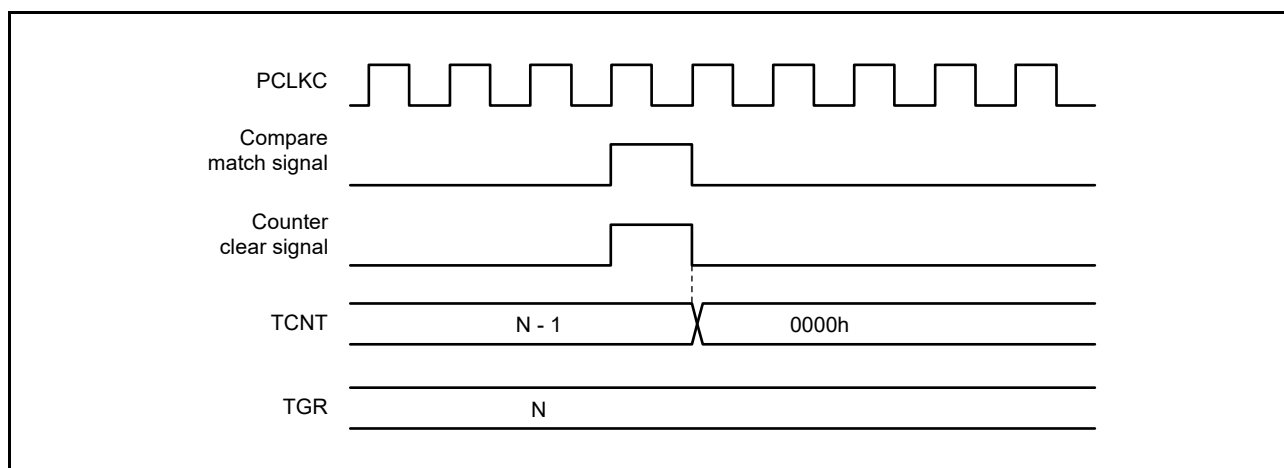
Figure 19.116 Counter Clear Timing (Compare Match) (MTU5)
