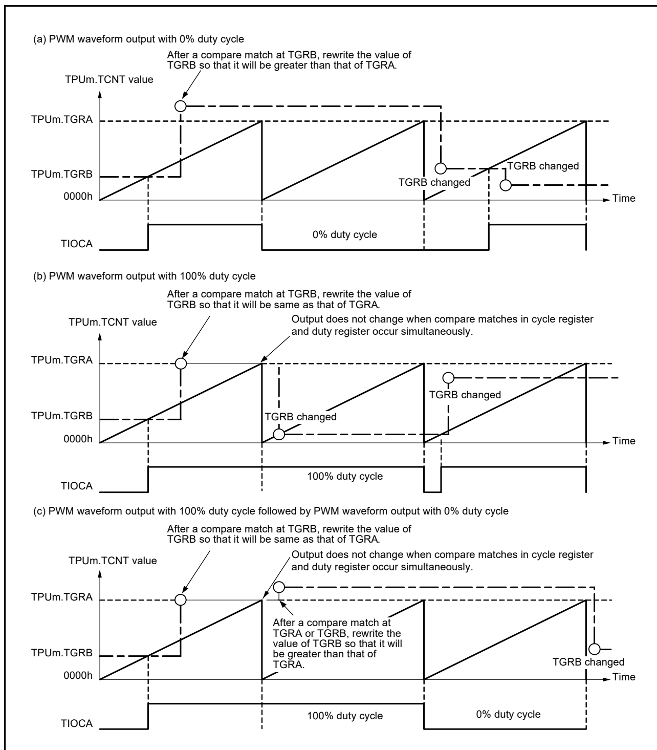
Figure 22.25 Example of PWM Mode Operation (3)
