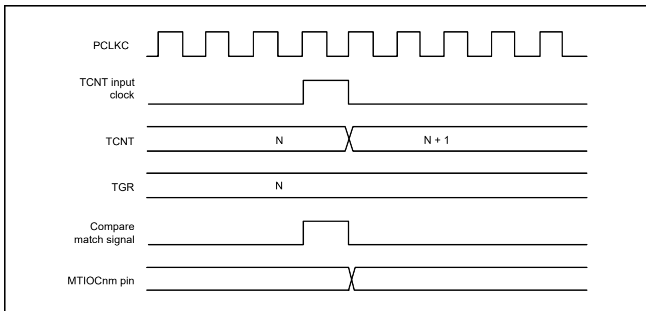
Figure 19.112 Output Compare Output Timing (Normal Mode or PWM Mode) ( n = 0 to 4, 6, 7, or 8, m = A to D)
