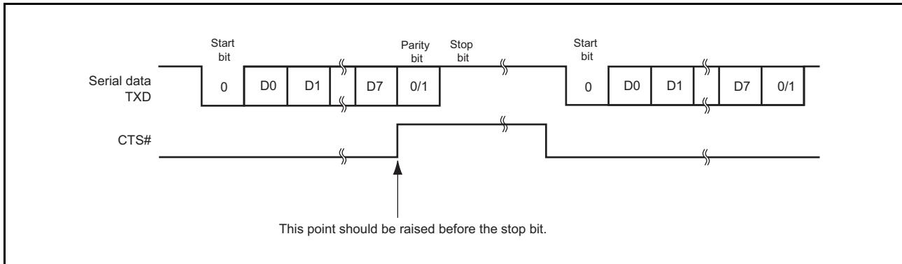
Figure 33.6 Example of Transmit Operation in Asynchronous Mode Using Modem Control Function (CTS#)
