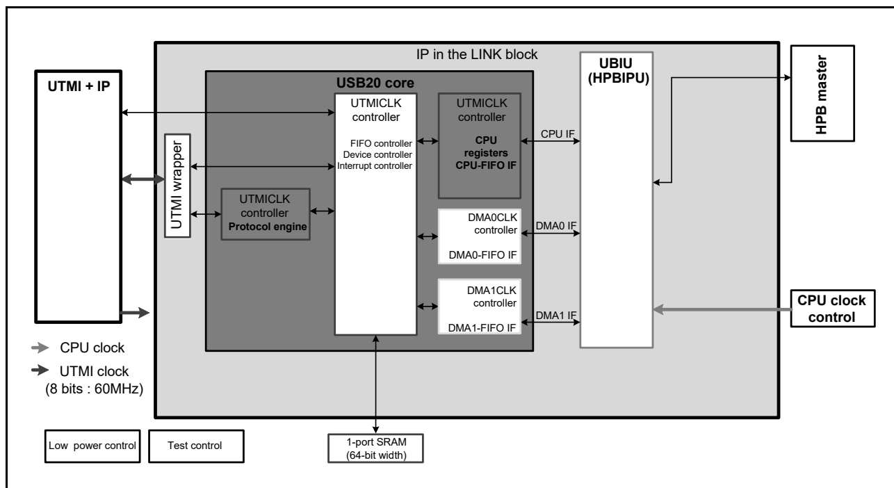
Figure 32.1 Block Diagram of the USB Module
