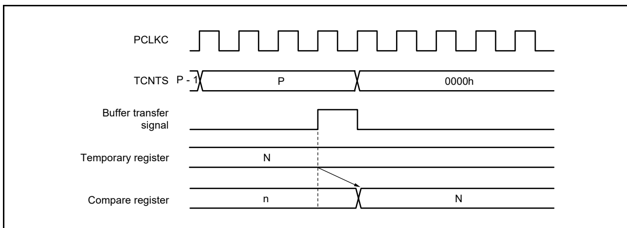
Figure 19.123 Transfer Timing from Temporary Register to Compare Register
