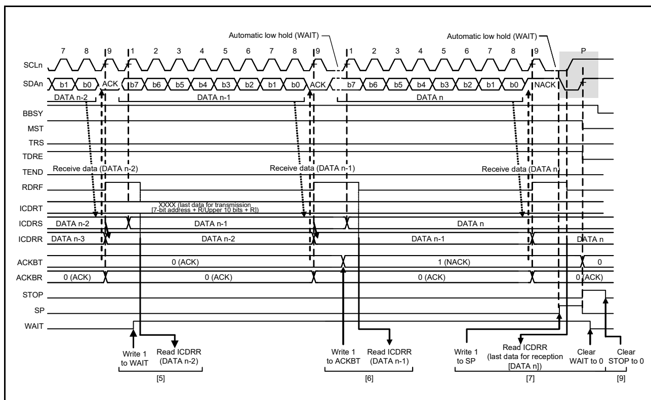
Figure 34.14 Master Receive Operation Timing (3) (when RDRFS = 0)
