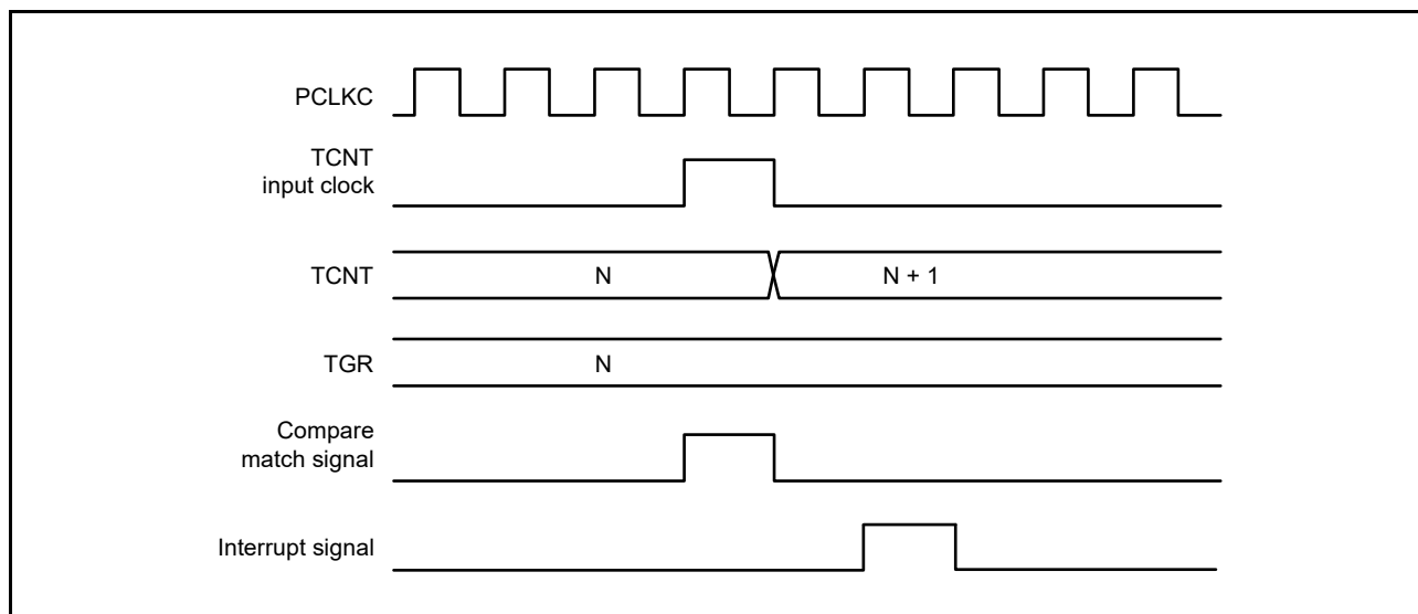
Figure 19.124 TGI Interrupt Timing (Compare Match) (MTU0 to MTU4 and MTU6 to MTU8)
