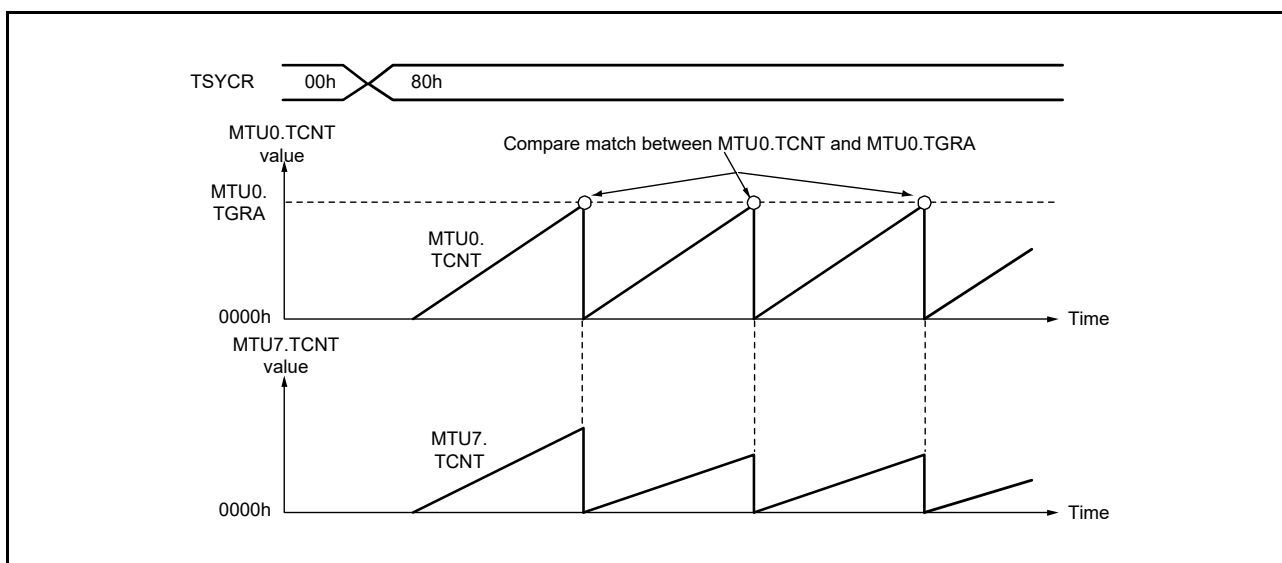
Figure 19.102 Example of Synchronous Counter Clearing for MTU6 and MTU7 (1)
