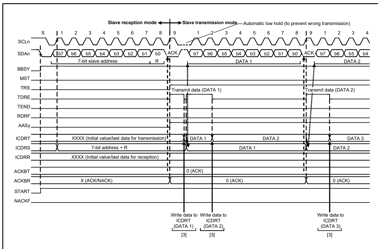
Figure 34.16 Slave Transmit Operation Timing (1) (7-Bit Address Format)
