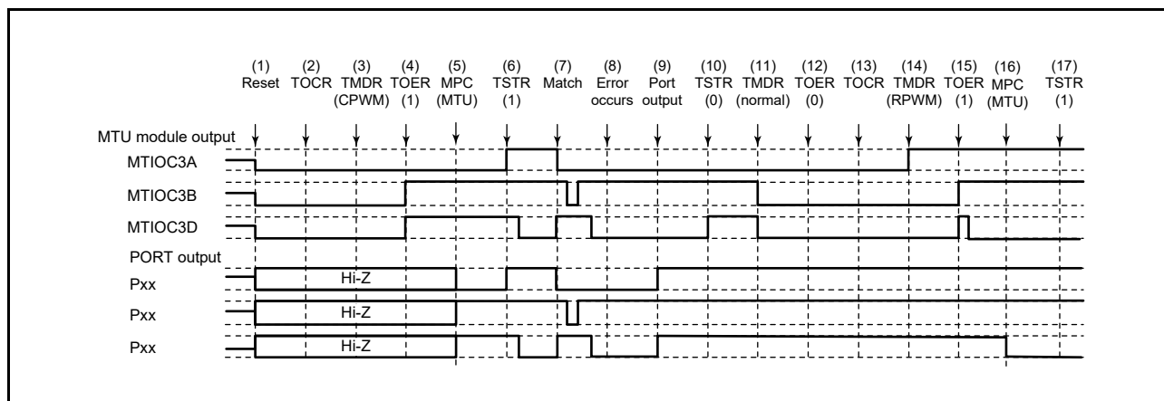
Figure 19.173 Error Occurrence in Complementary PWM Mode, Recovery in Reset-Synchronized PWM Mode
