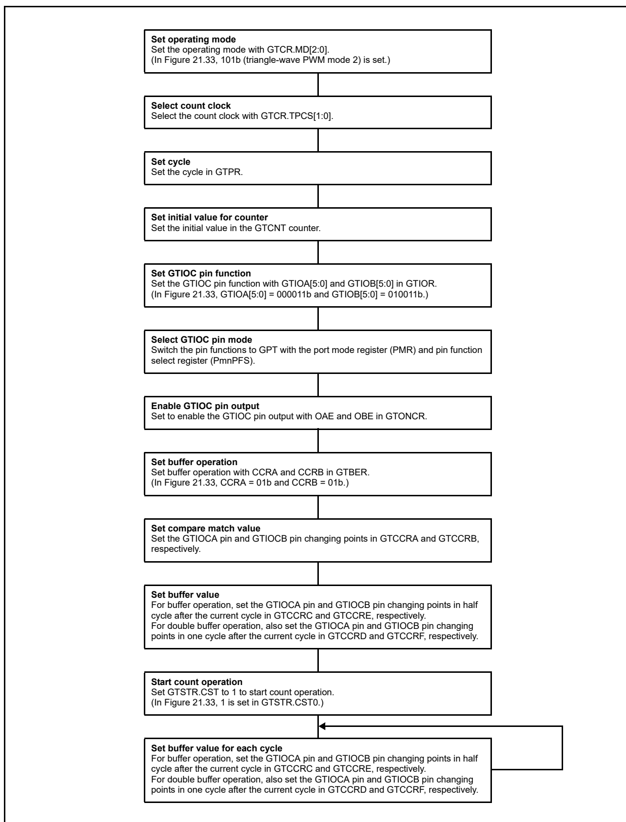
Figure 21.34 Example for Setting Triangle-Wave PWM Mode 2
