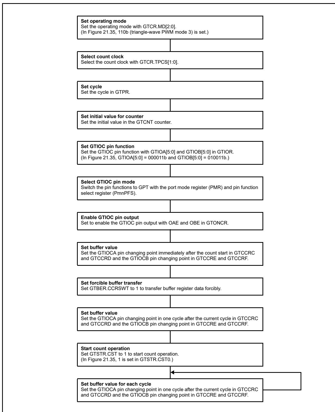
Figure 21.36 Example for Setting Triangle-Wave PWM Mode 3
