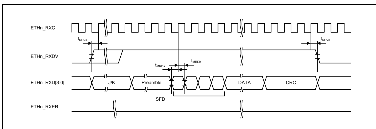
Figure 47.76 MII Reception Timing (Normal Operation)
