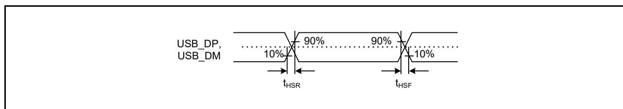
Figure 47.84 USB_DP, USB_DM Output Timing (High Speed)
