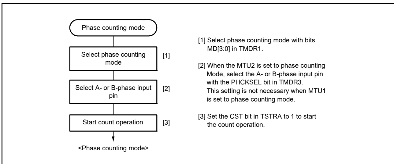
Figure 19.30 Example of Phase Counting Mode Setting Procedure
