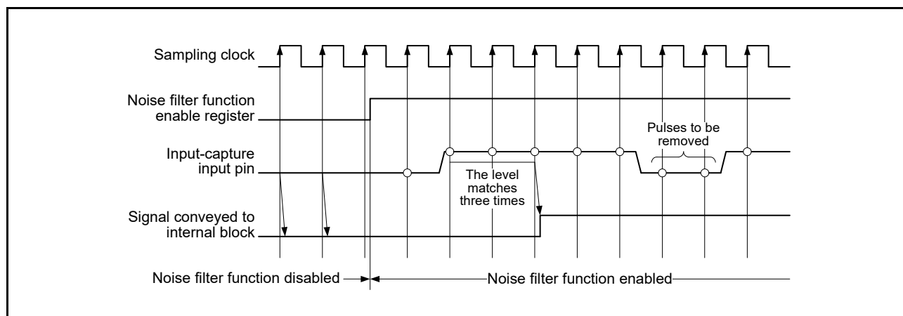
Figure 22.32 Timing Chart for the Noise Filter
