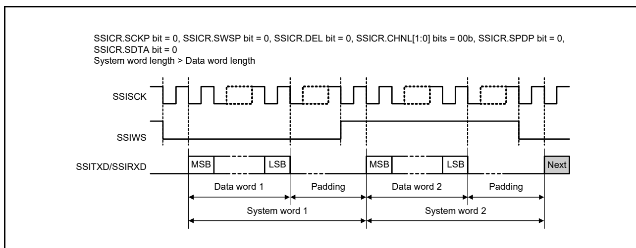
Figure 39.3 I 2 S Compatible Format (with Padding)
