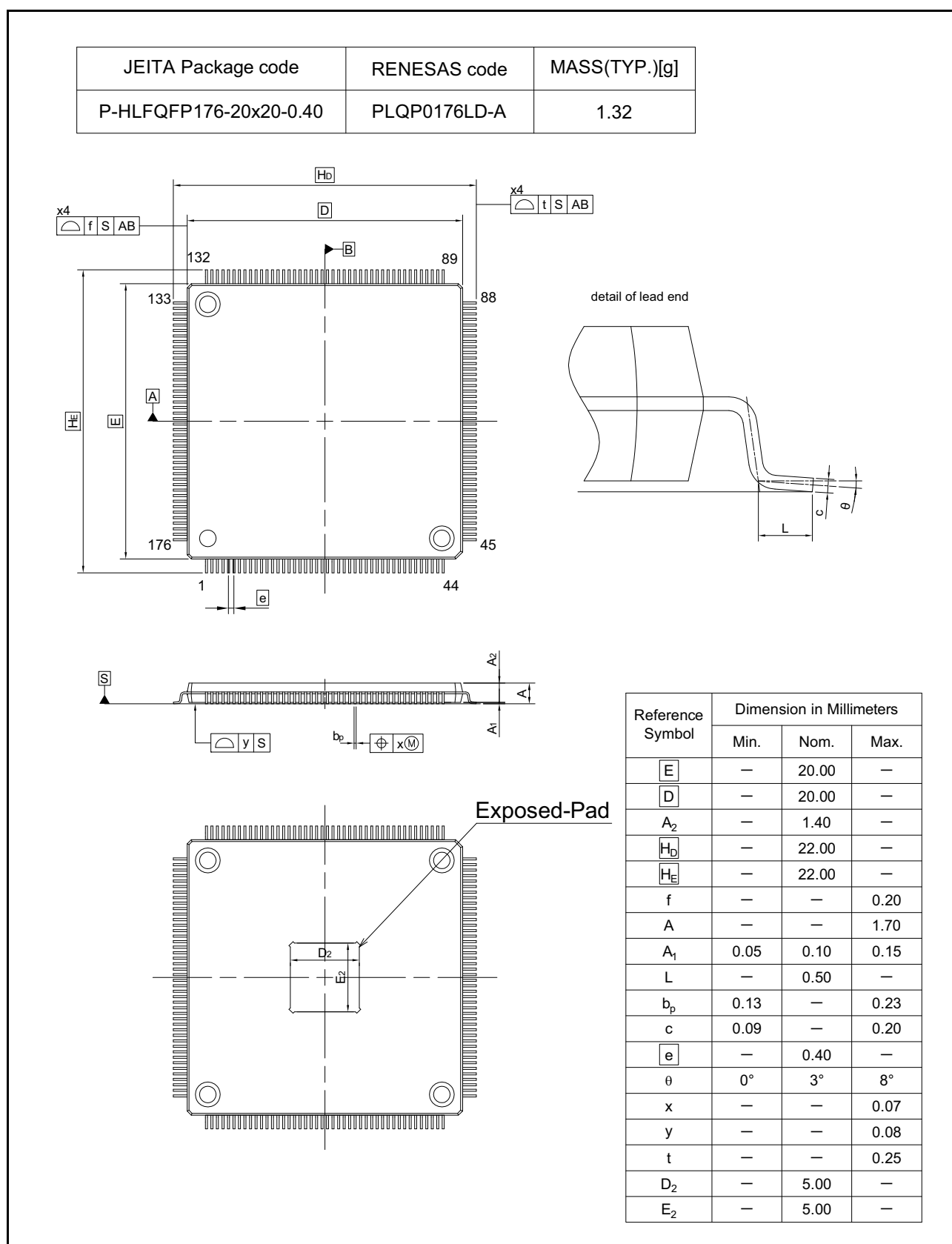
Figure D 176-Pin HLFQFP (PLQP0176LD-A)
