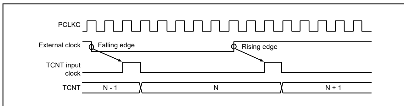
Figure 19.110 Count Timing in External Clock Operation (MTU0 to MTU4 and MTU8)
