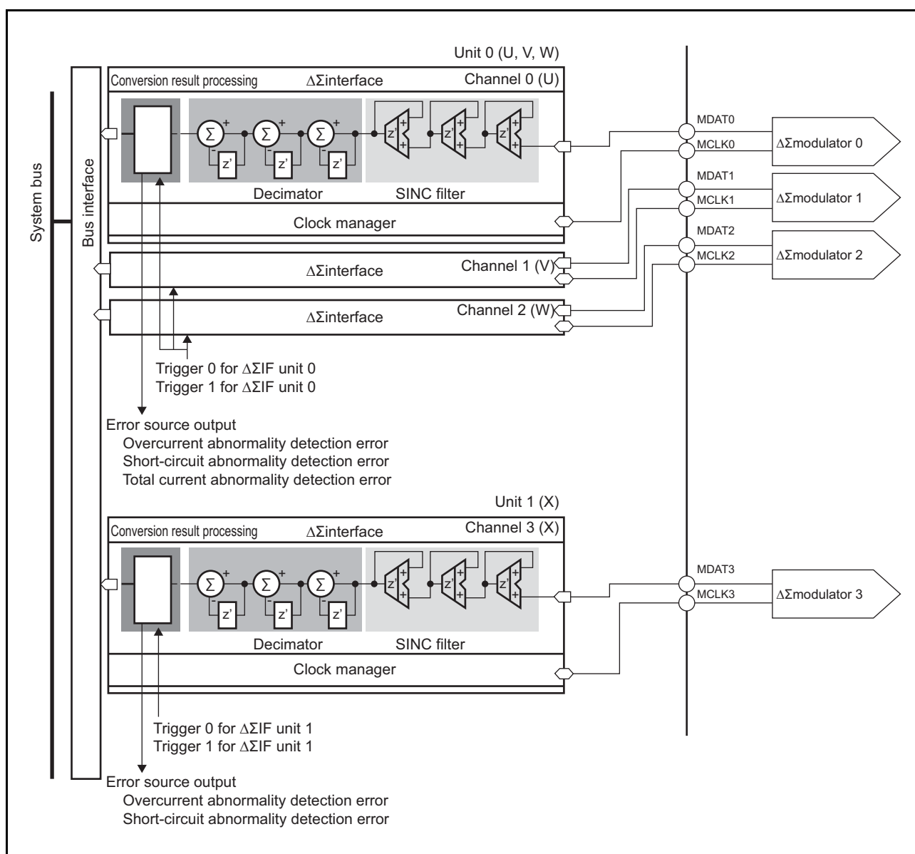
Figure 41.1 DSMIF Block Diagram
