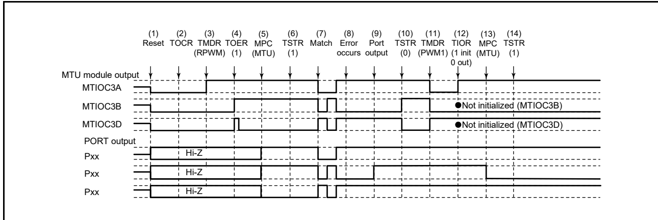
Figure 19.175 Error Occurrence in Reset-Synchronized PWM Mode, Recovery in PWM Mode 1
