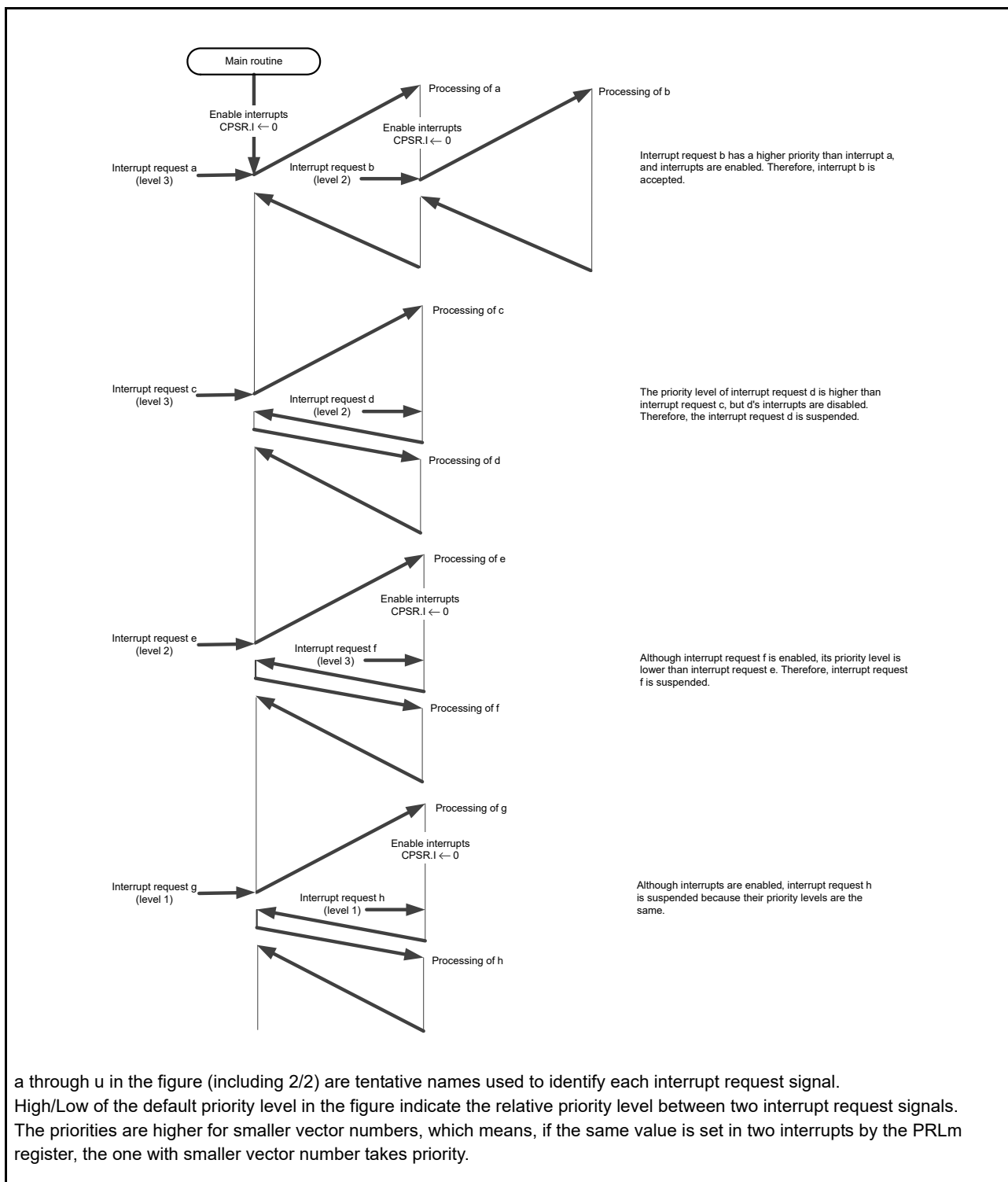
Figure 12.11 Concept of Multiple Interrupts (1 / 2)
