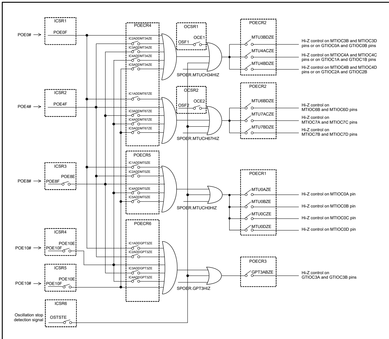
Figure 20.2 Target Pins and Conditions for High-Impedance Control
