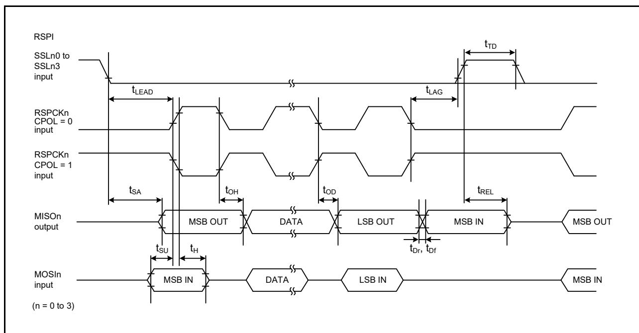
Figure 47.55 RSPI Timing (Slave, CPHA = 0)
