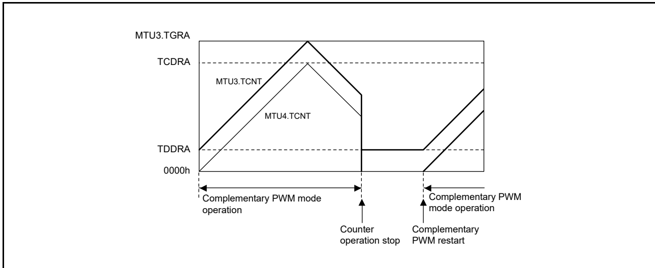
Figure 19.141 Counter Value when Stopped in Complementary PWM Mode
