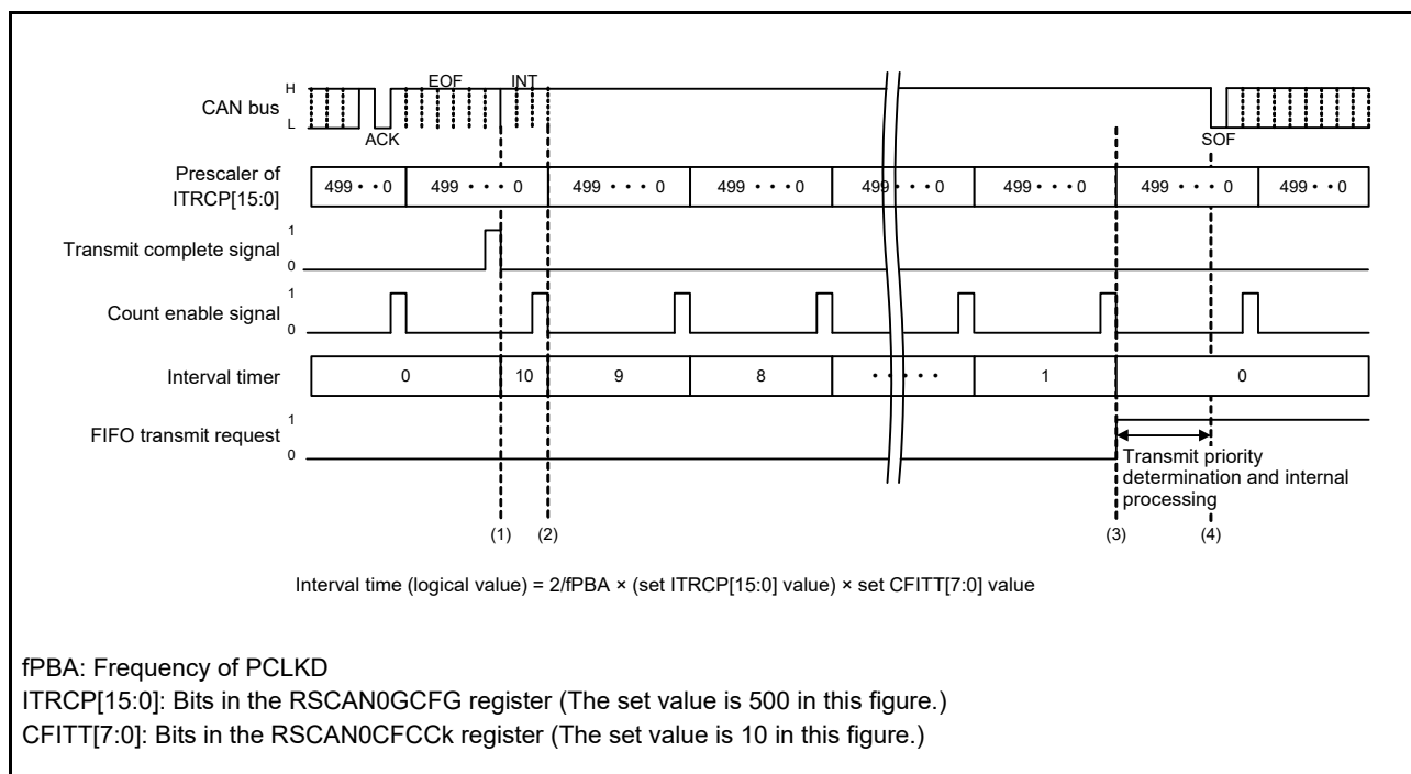
Figure 35.11 Interval Timer Timing Chart
