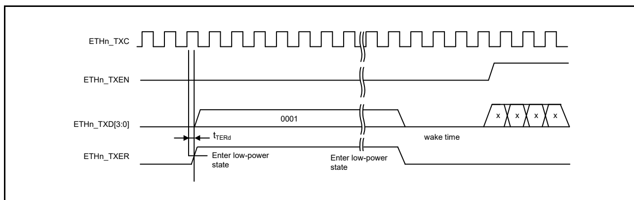
Figure 47.75 MII Transmission Timing
