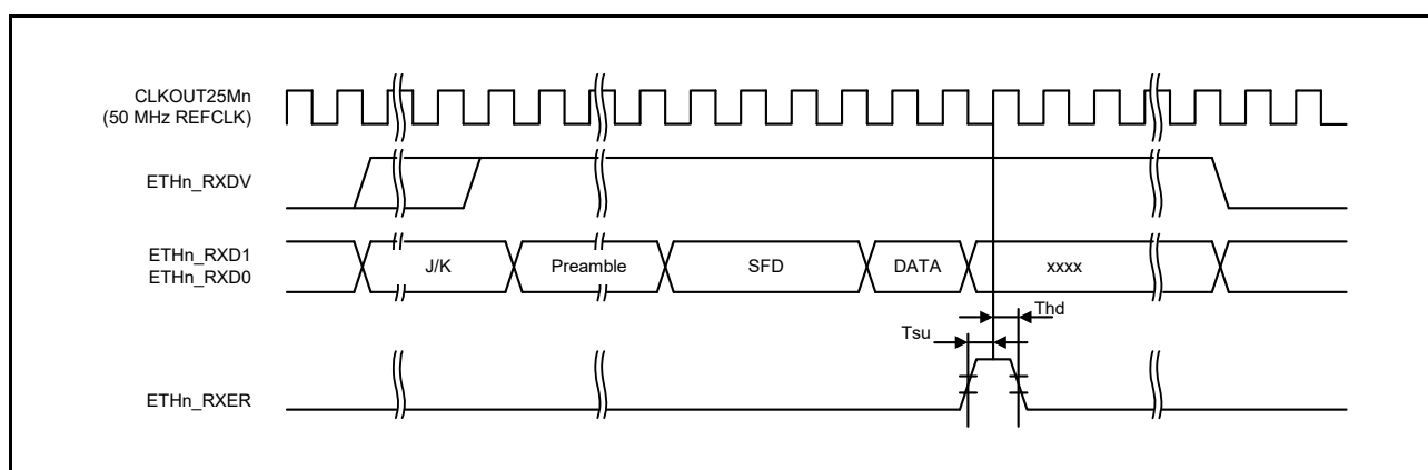
Figure 47.73 RMII Reception Timing (Error Occurrence)
