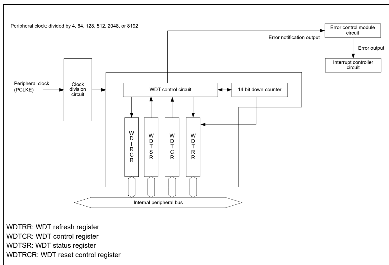
Figure 26.1 WDT Block Diagram
