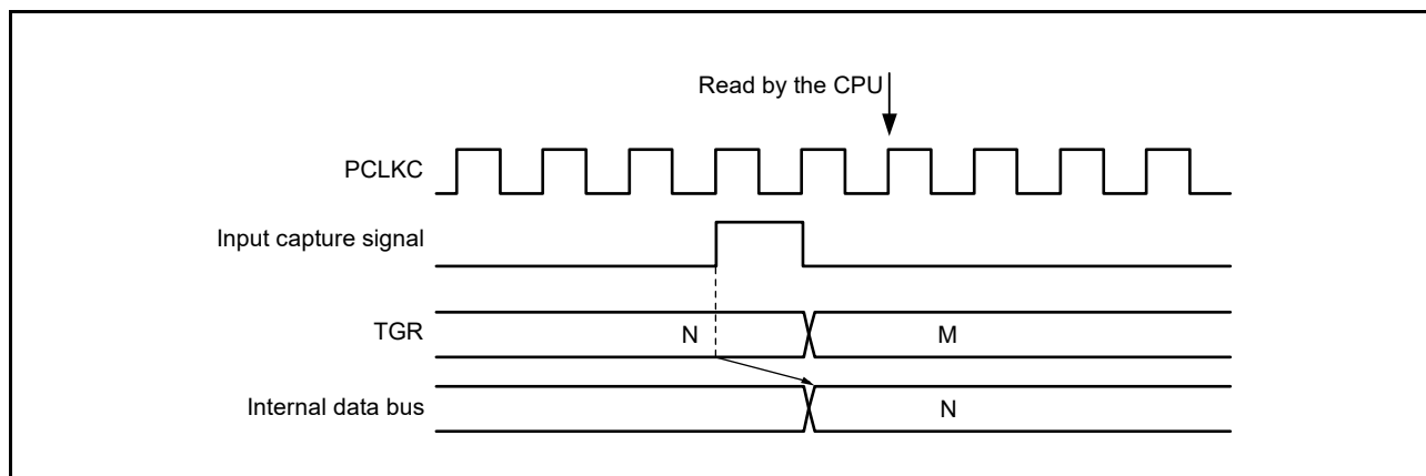
Figure 19.136 Contention between TGR Read Operation and Input Capture (MTU0 to MTU8)
