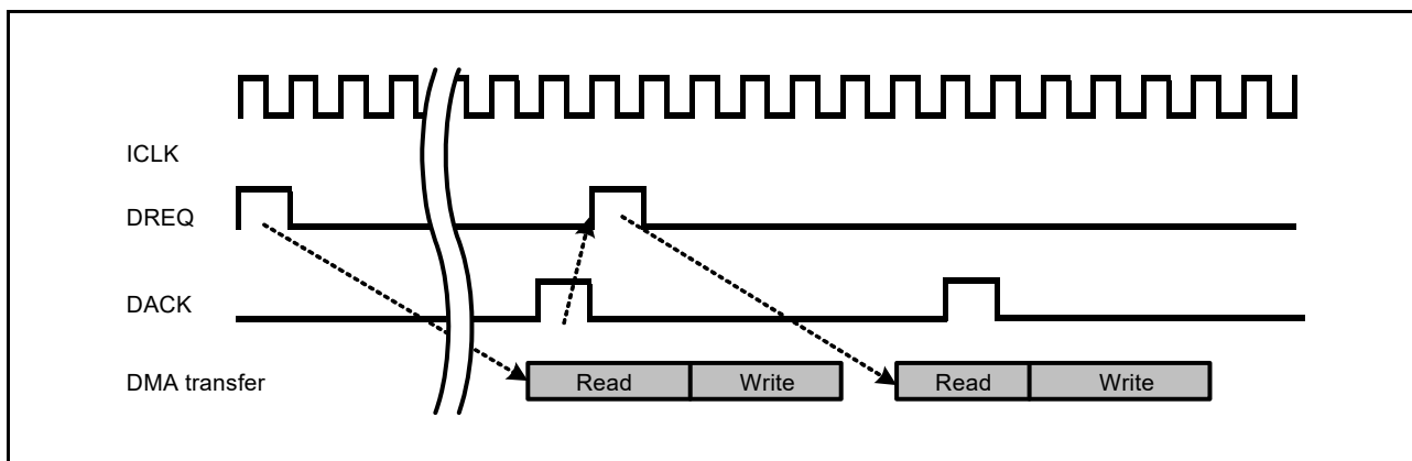
Figure 15.18 Edge Detection Timing (Rising Edge (HIEN = 1), DACK Output is Active during Reading (REQD = 0))
