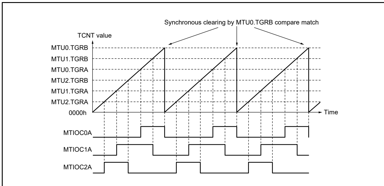
Figure 19.14 Example of Synchronous Operation
