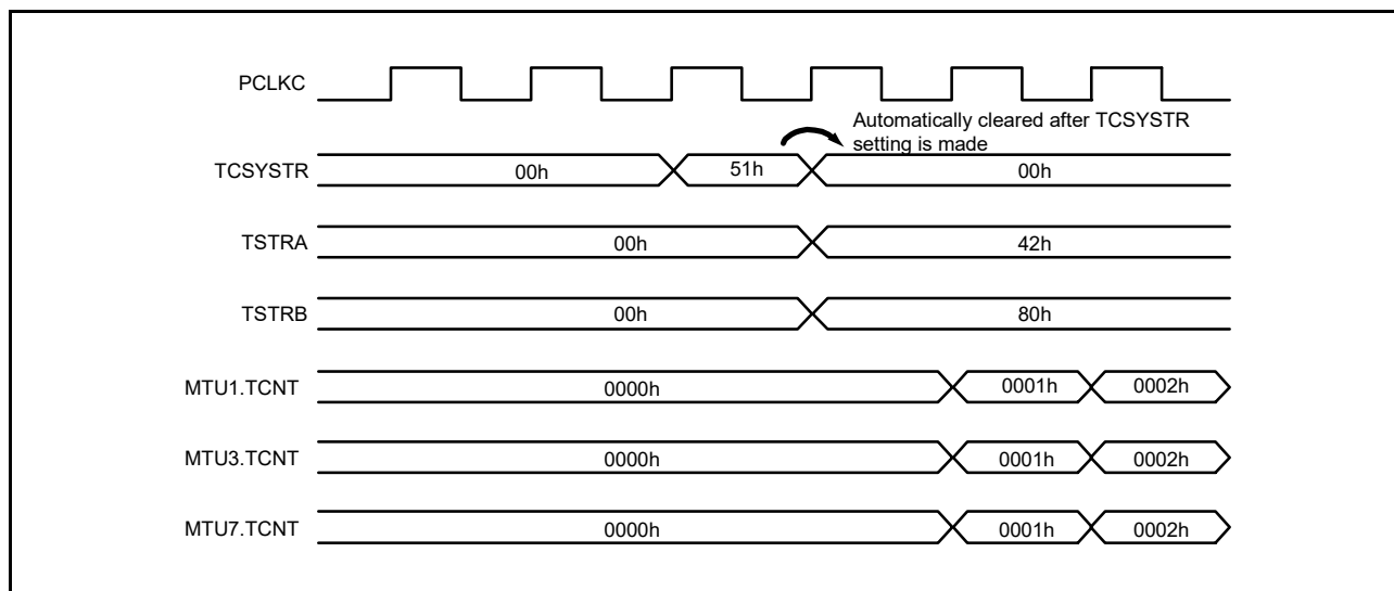
Figure 19.100 Example of Synchronous Counter Start Operation
