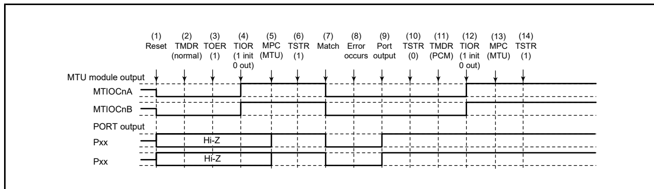
Figure 19.152 Error Occurrence in Normal Mode, Recovery in Phase Counting Mode
