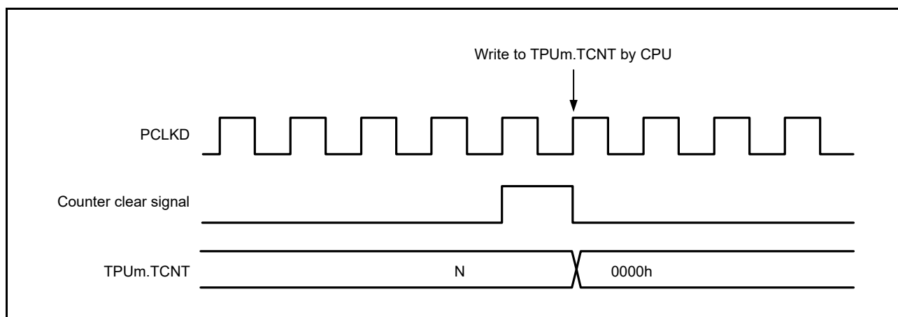
Figure 22.50 Conflict between TPUm.TCNT Write and Clear Operations
