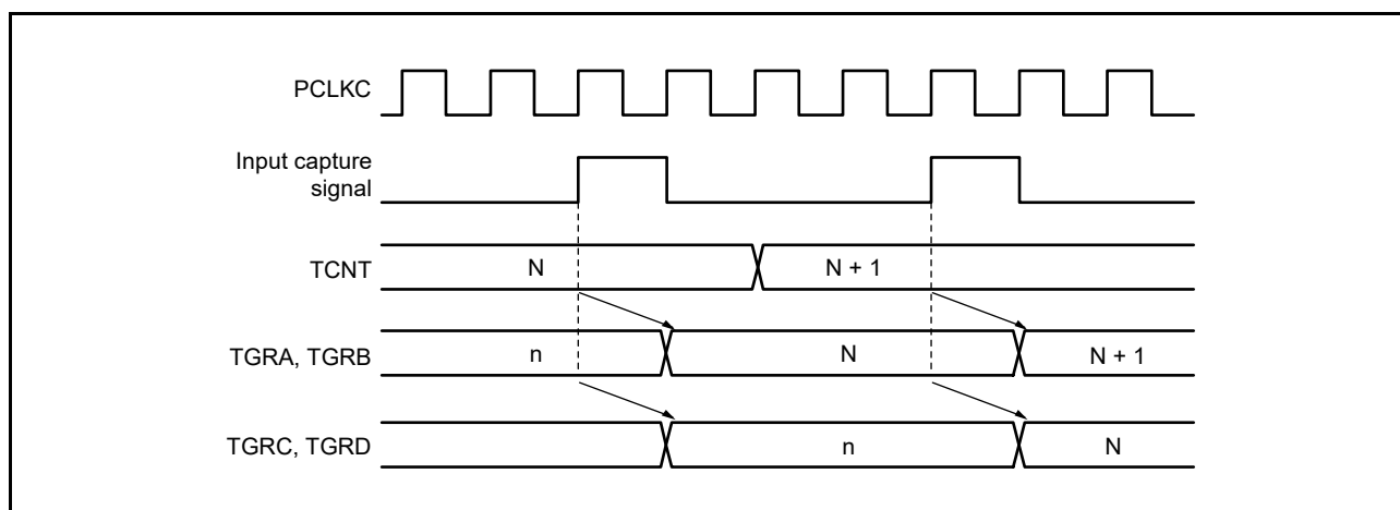
Figure 19.119 Buffer Operation Timing (Input Capture)
