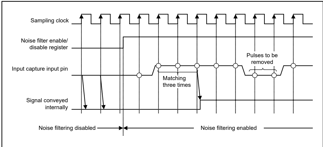
Figure 25.12 Timing of Digital Noise Filtering
