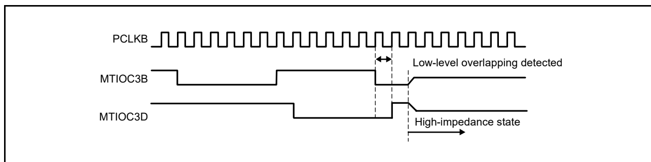
Figure 20.5 Output Level Compare Operation
