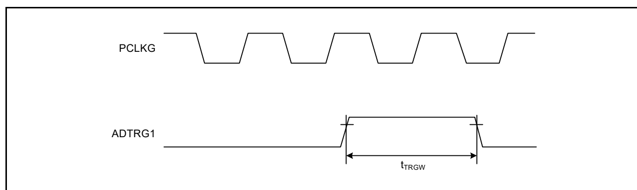
Figure 47.49 A/D Converter Trigger Input Timing (ADTRG1)
