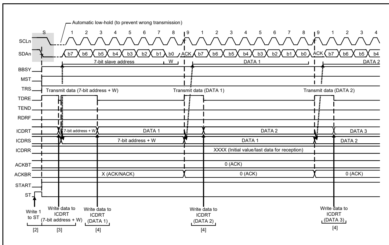
Figure 34.7 Master Transmit Operation Timing (1) (7-Bit Address Format)
