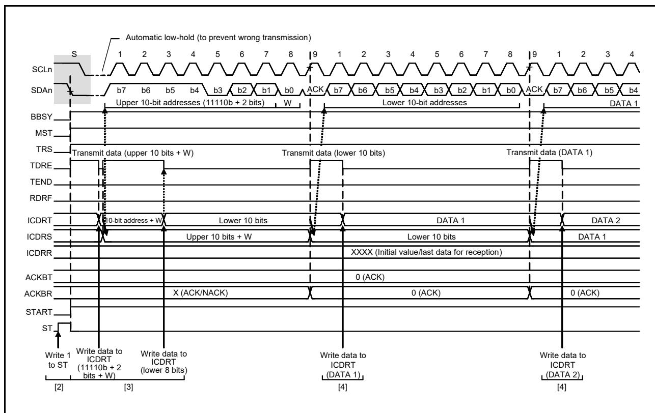
Figure 34.8 Master Transmit Operation Timing (2) (10-Bit Address Format)
