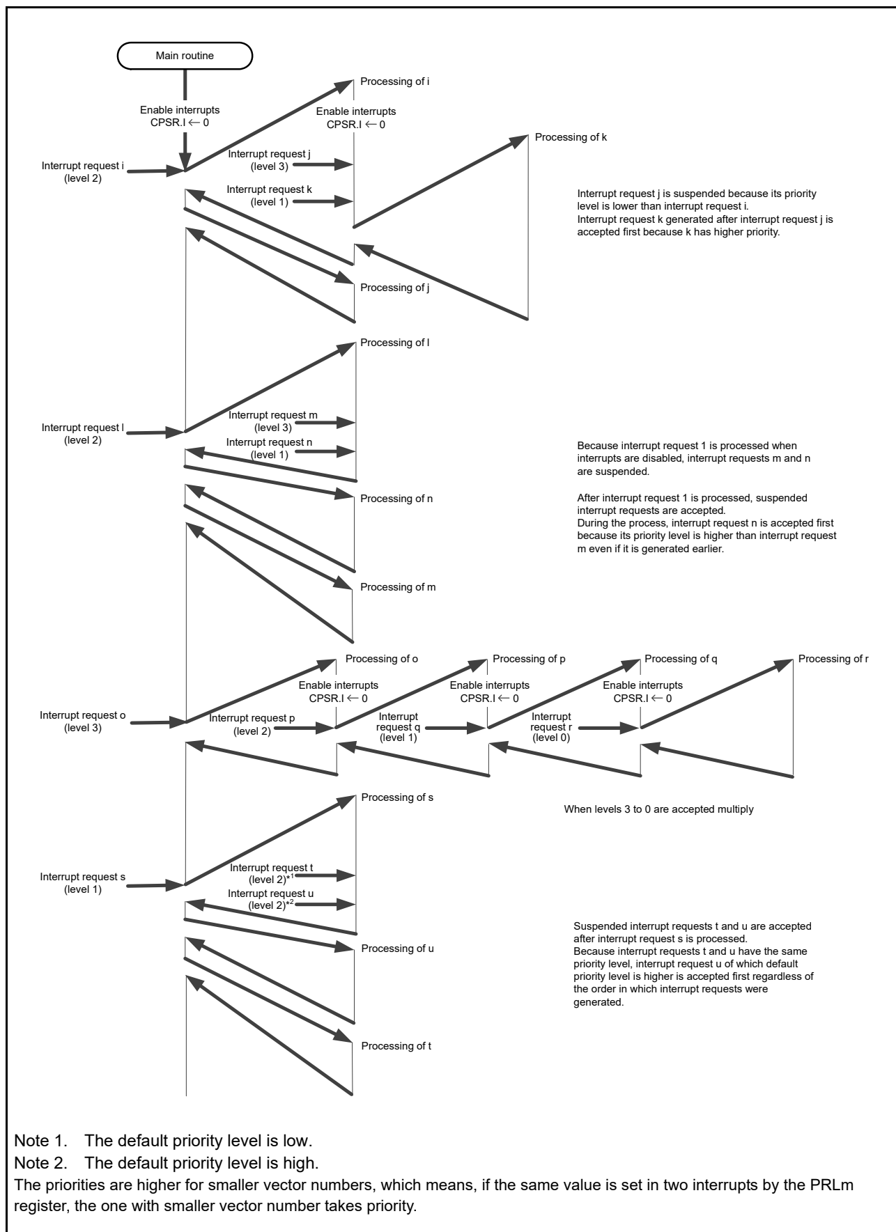
Figure 12.11 Concept of Multiple Interrupts (2 / 2)
