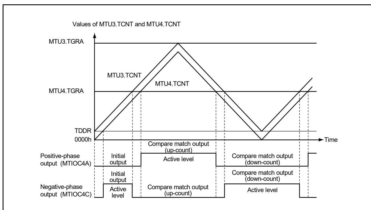
Figure 19.3 Example of Output in Complementary PWM Mode
