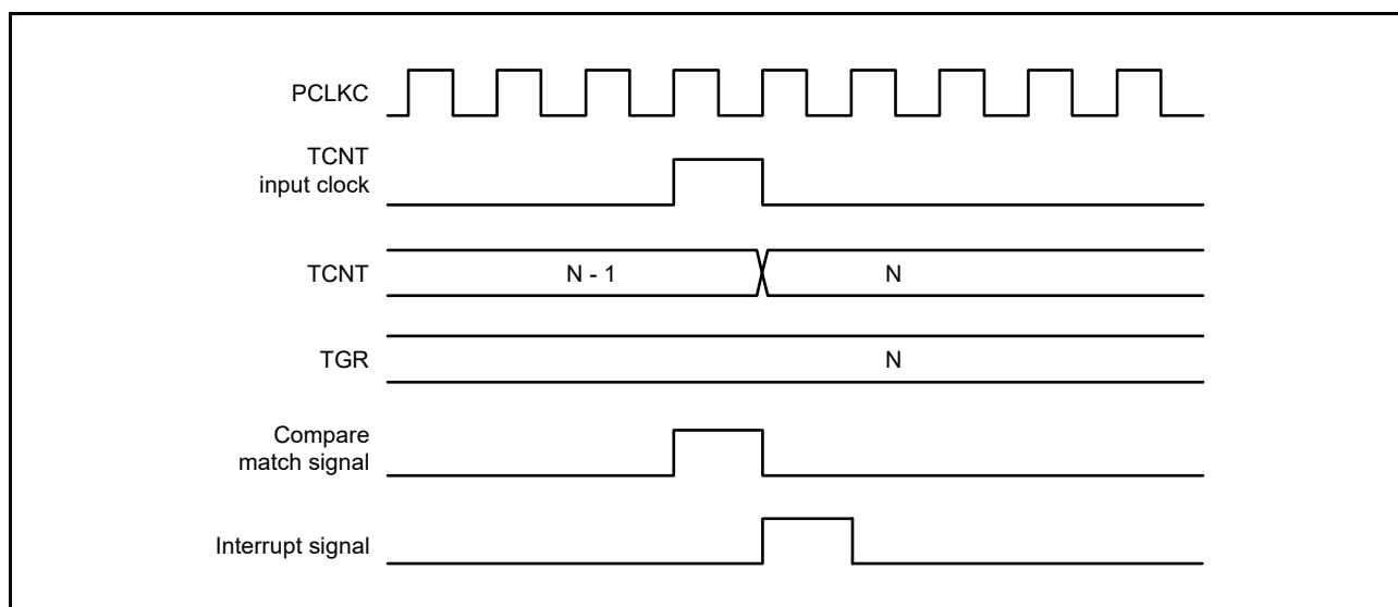
Figure 19.125 TGI Interrupt Timing (Compare Match) (MTU5)
