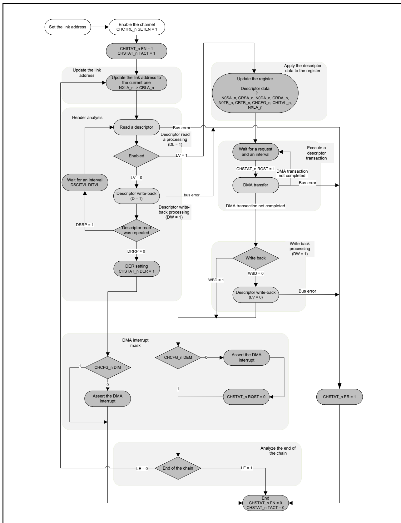
Figure 15.8 Link Mode Operation Flow
