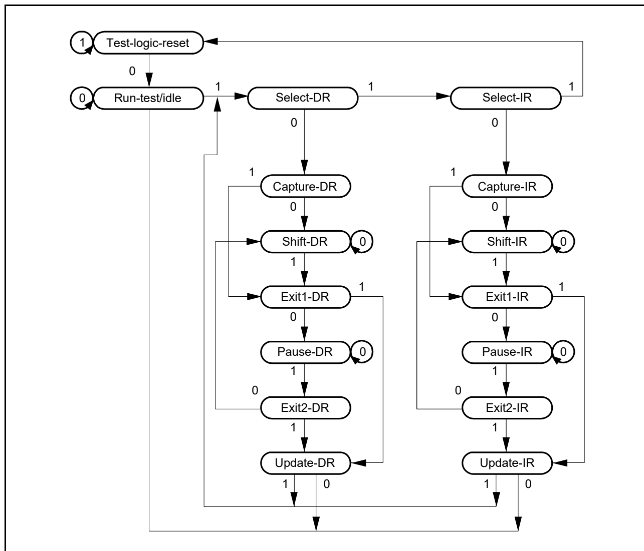
Figure 40.2 State Transition Diagram of TAP Controller
