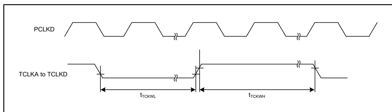
Figure 47.41 TPUa Clock Input Timing
