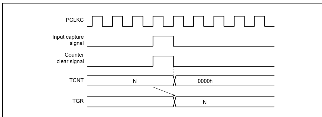
Figure 19.117 Counter Clear Timing (Input Capture) (MTU0 to MTU8)
