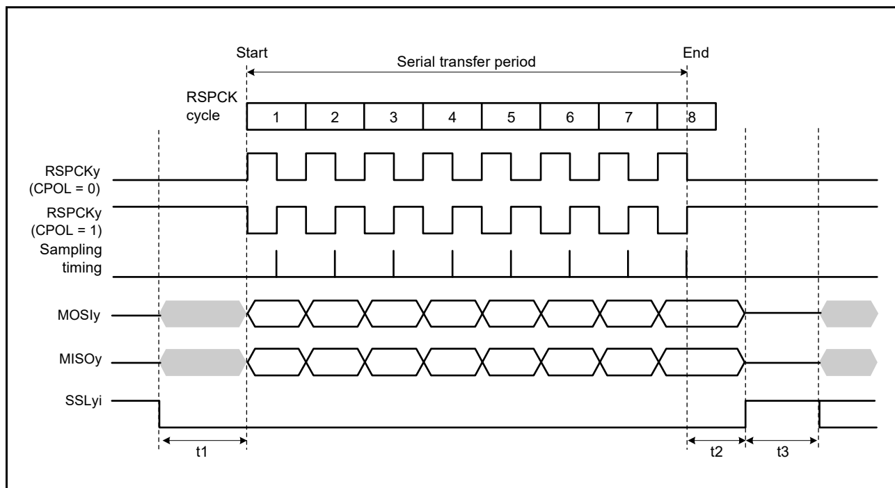
Figure 36.23 RSPI Transfer Format (CPHA = 1)
