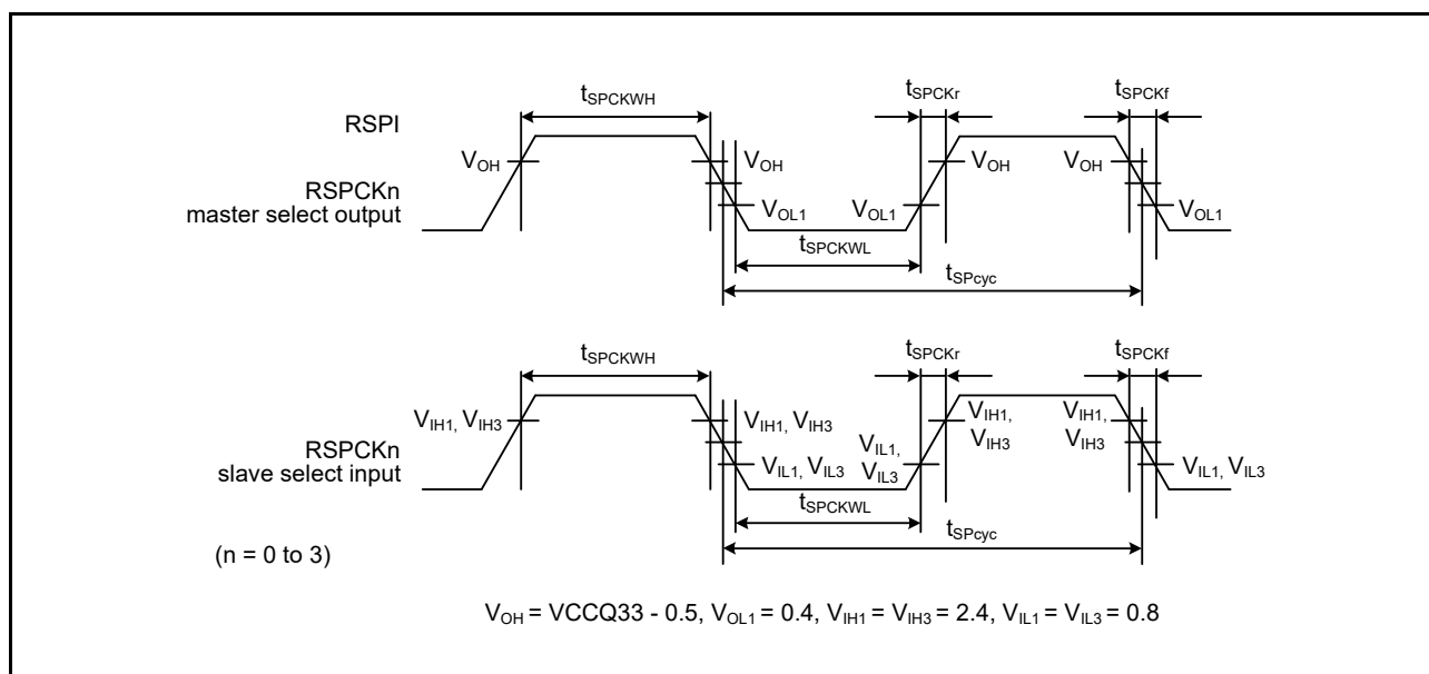
Figure 47.52 RSPIa Clock Timing
