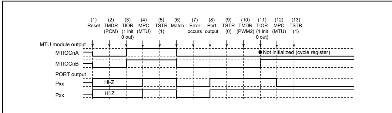
Figure 19.167 Error Occurrence in Phase Counting Mode, Recovery in PWM Mode 2
