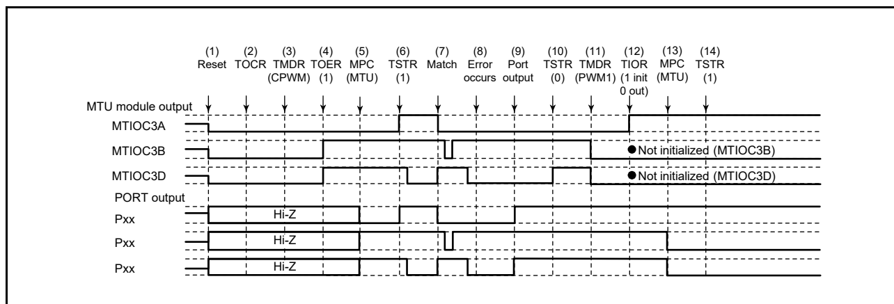
Figure 19.170 Error Occurrence in Complementary PWM Mode, Recovery in PWM Mode 1
