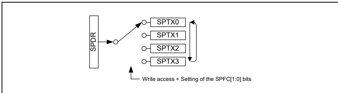
Figure 36.3 Configuration of SPDR (Writing)
