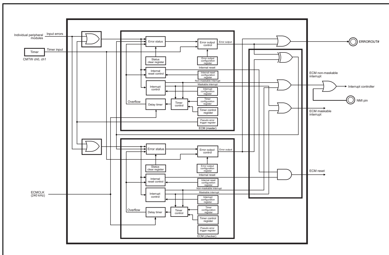
Figure 42.1 Block Diagram of ECM
