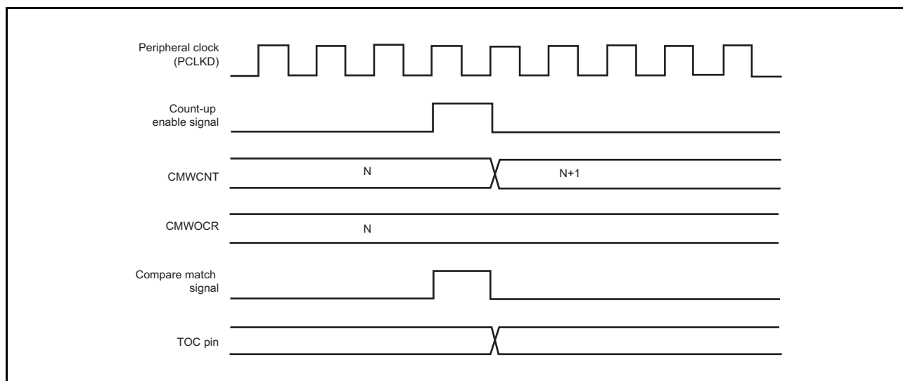
Figure 25.10 Output Compare Output Timing
