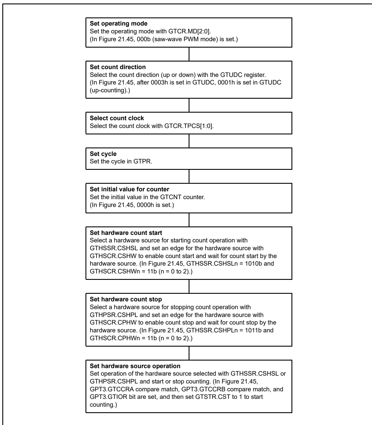
Figure 21.46 Example for Setting Count Stop Operation by Hardware Source
