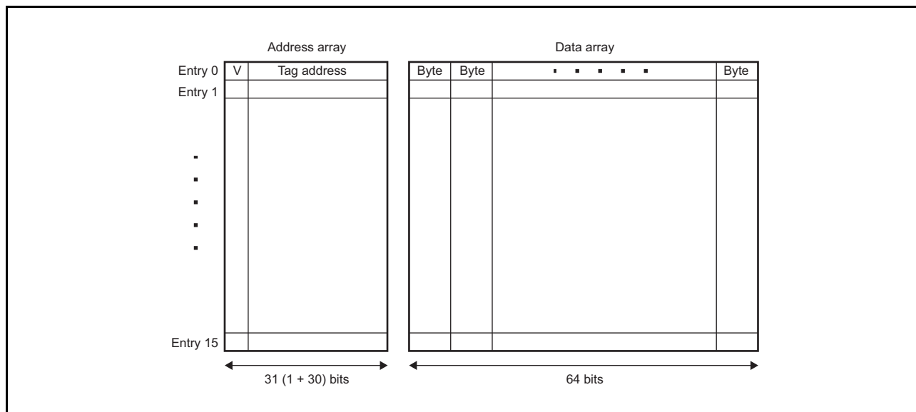
Figure 37.12 Read Cache Configuration
