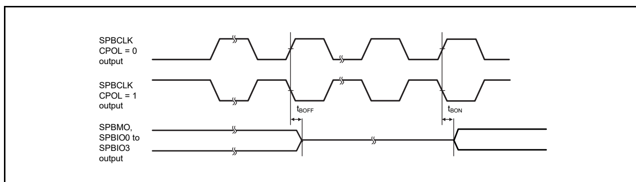
Figure 47.62 SPIBSC Buffer On/Off Timing (CPHAT = 1, CPHAR = 1)
