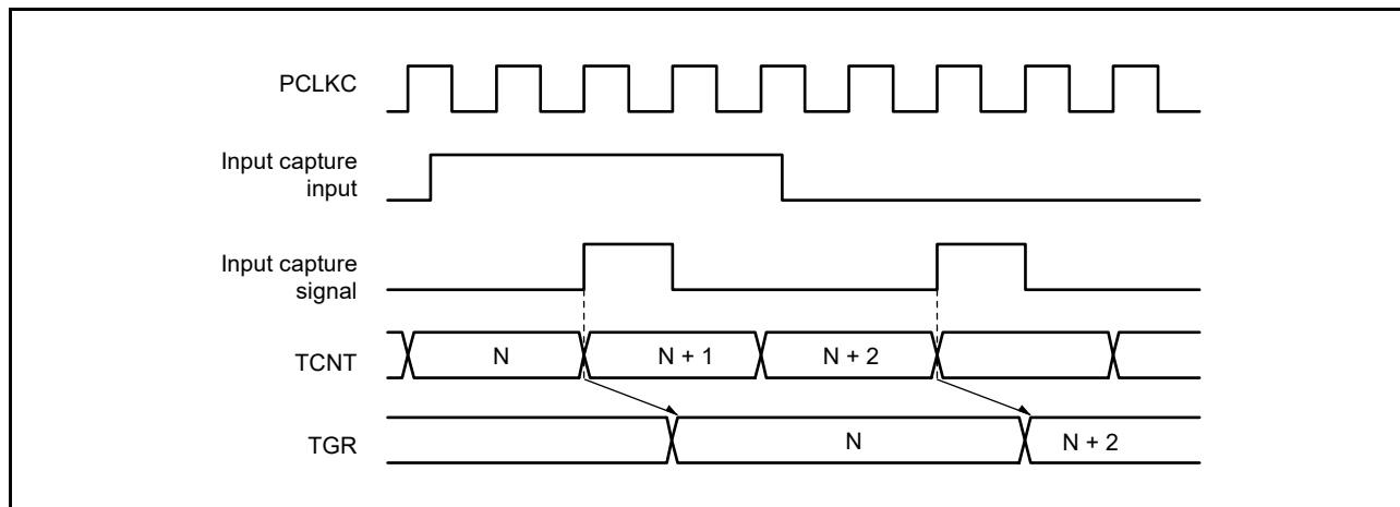
Figure 19.114 Input Capture Input Signal Timing
