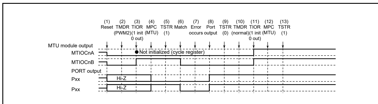
Figure 19.161 Error Occurrence in PWM Mode 2, Recovery in Normal Mode
