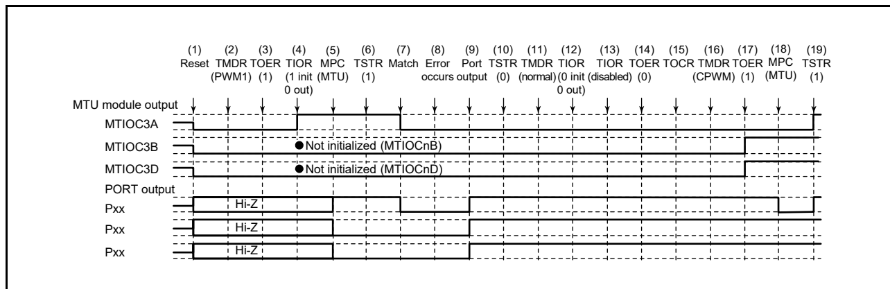
Figure 19.159 Error Occurrence in PWM Mode 1, Recovery in Complementary PWM Mode
