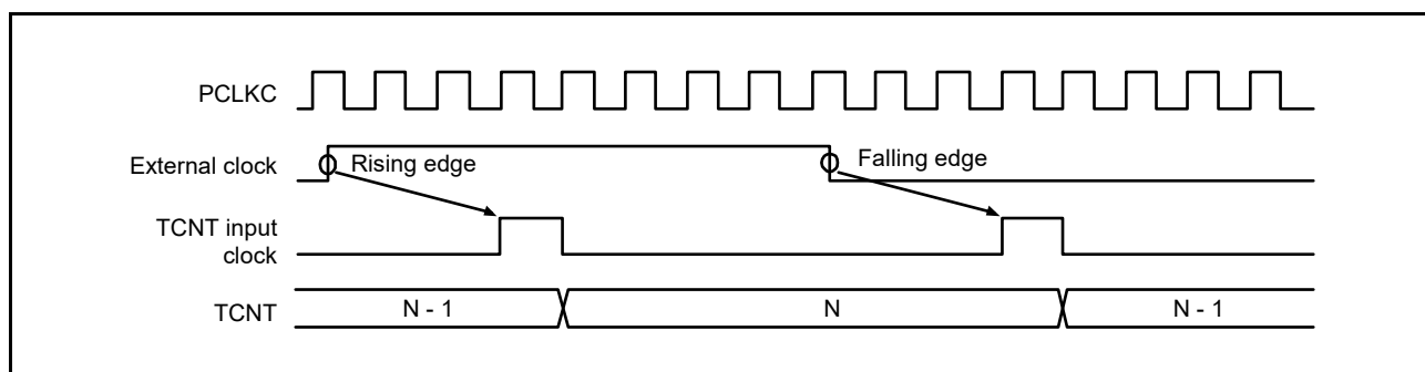
Figure 19.111 Count Timing in External Clock Operation (Phase Counting Mode)
