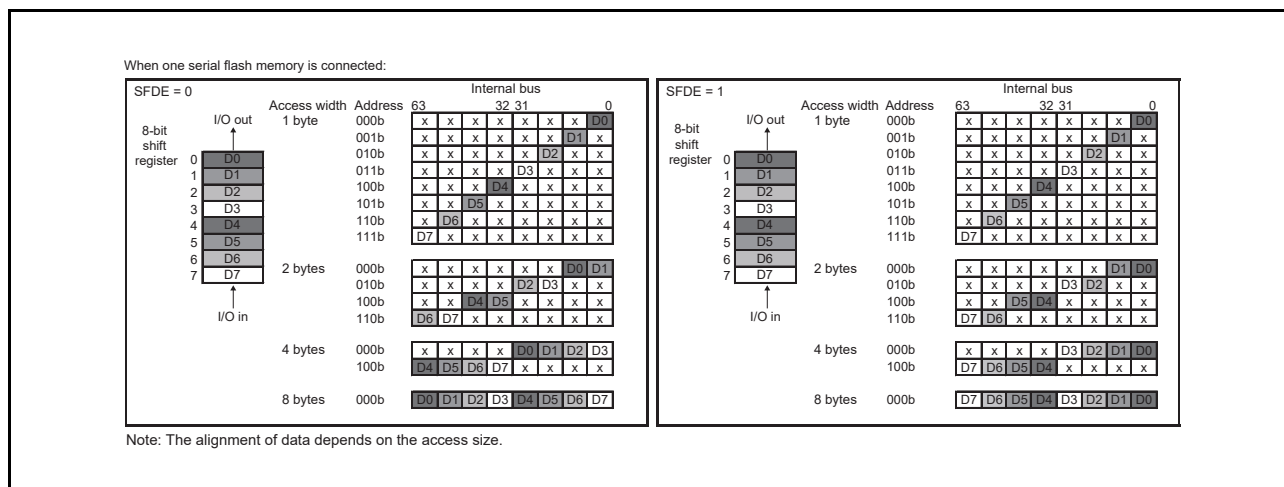
Figure 37.4 Data Alignment in External Address Space Read Mode
