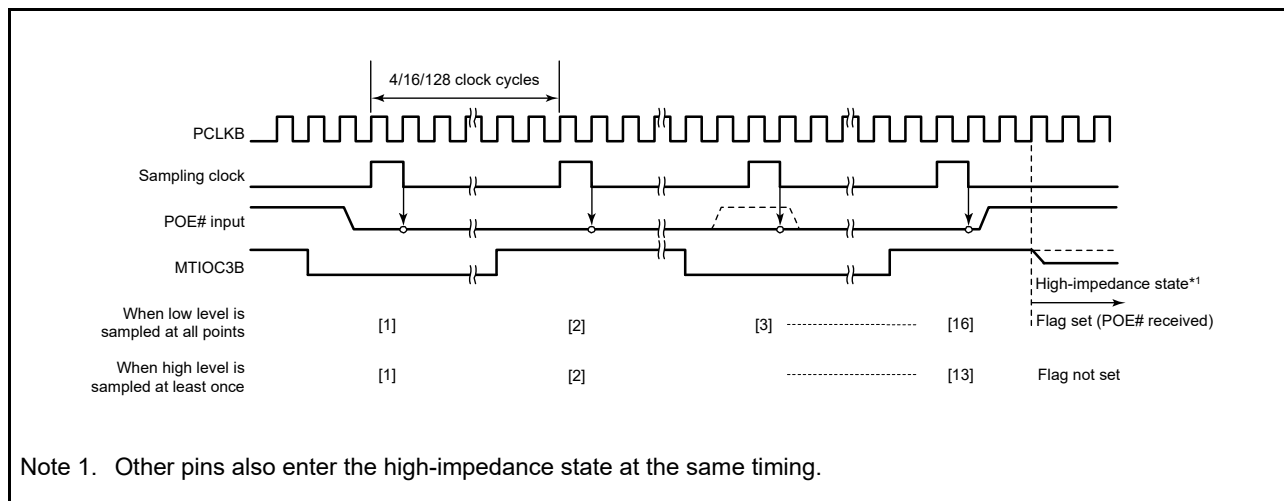
Figure 20.4 Low-Level Detection Operation
