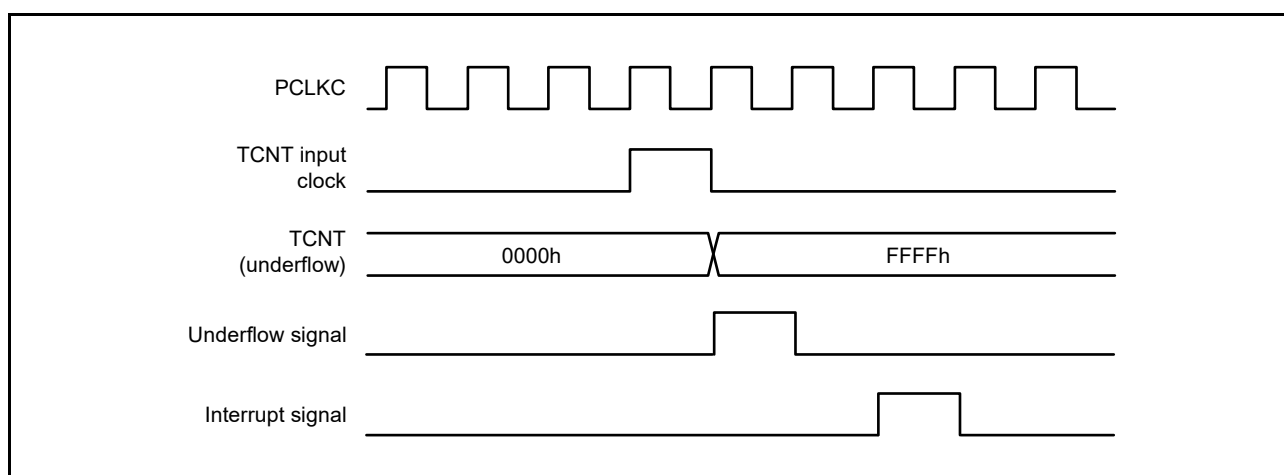
Figure 19.129 TCIU Interrupt Timing
