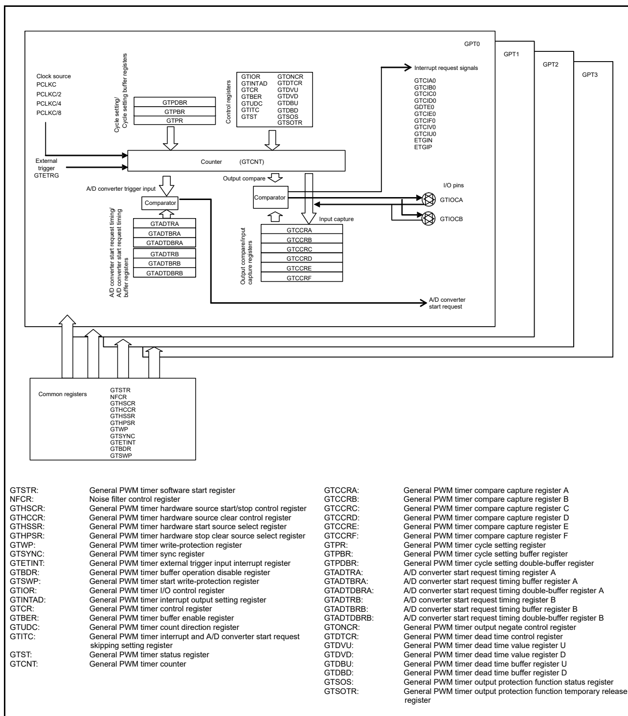
Figure 21.1 Block Diagram of GPT
