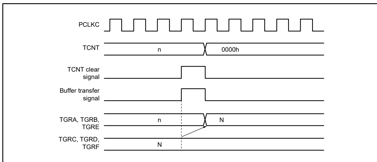
Figure 19.120 Buffer Operation Timing (when TCNT Cleared)
