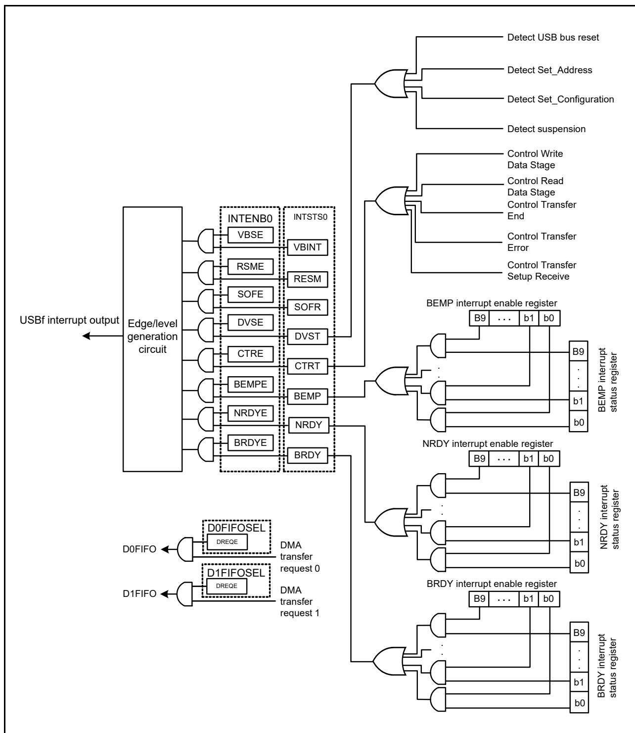
Figure 32.6 Interrupt Configuration Diagram
