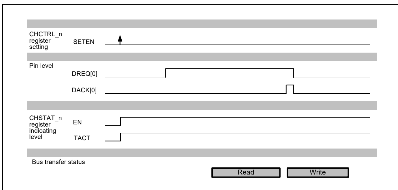
Figure 15.32 DMAC Status Example 1 (Hardware Request)
