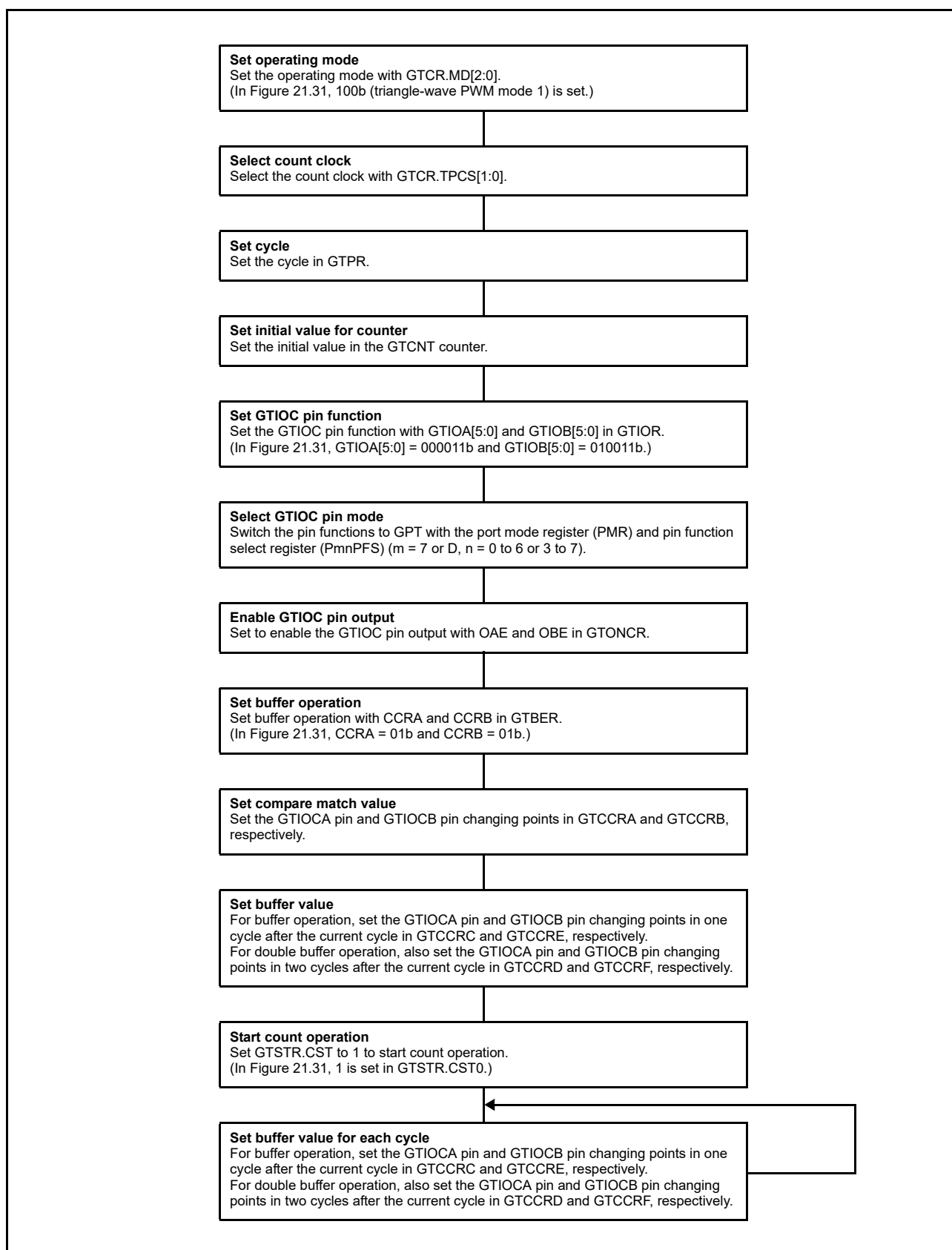
Figure 21.32 Example for Setting Triangle-Wave PWM Mode 1
