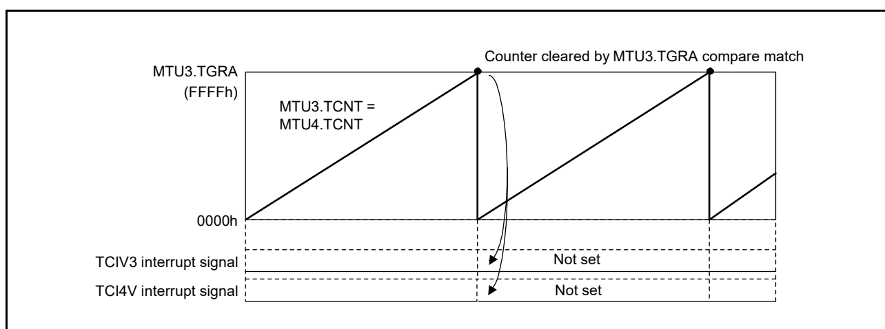
Figure 19.143 Overflow in Reset-Synchronized PWM Mode
