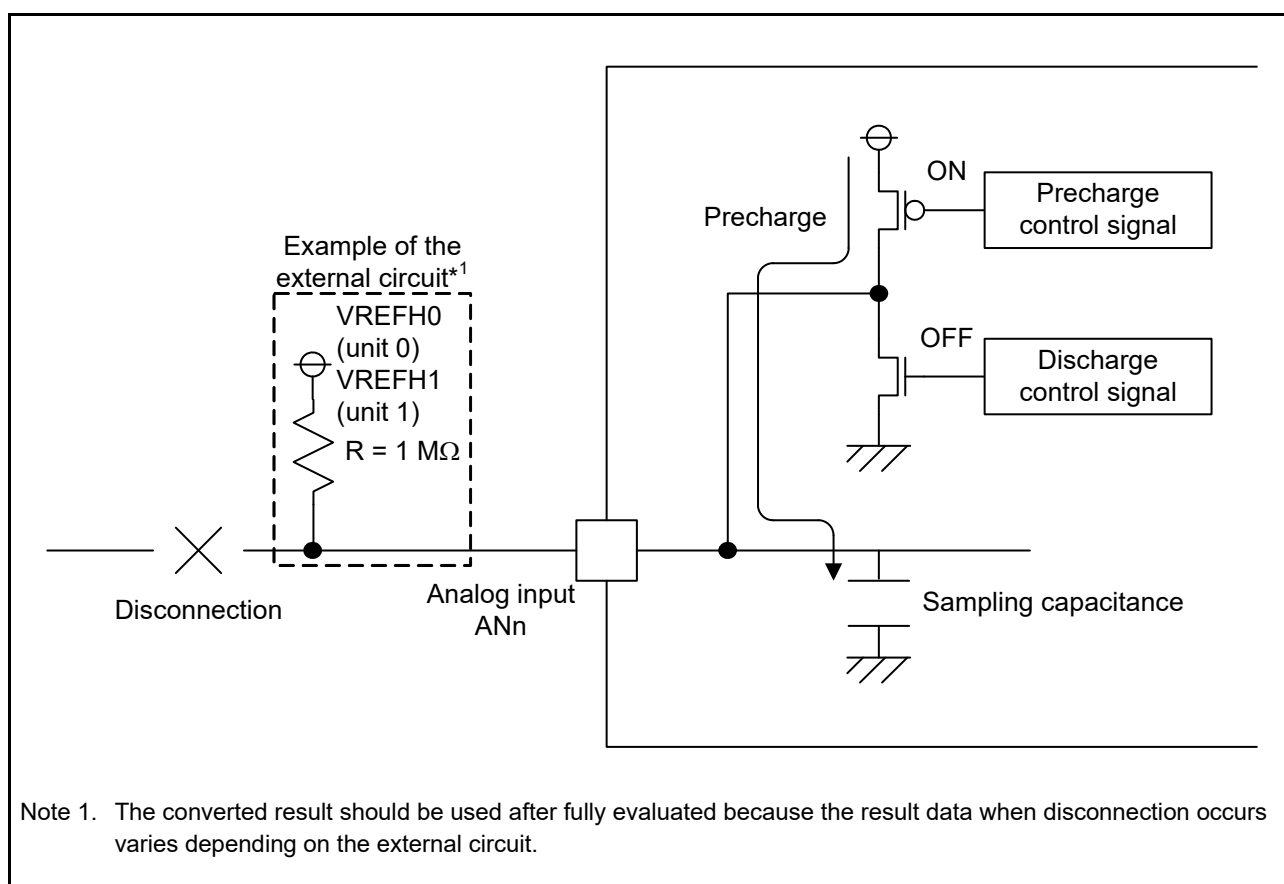
Figure 43.34 Example of Disconnection Detection when Precharge is Selected
