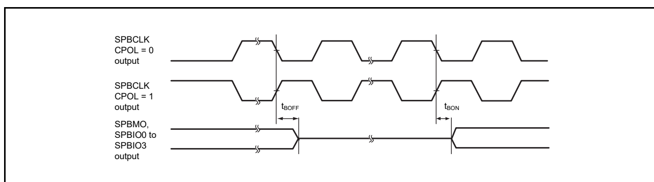
Figure 47.61 SPIBSC Buffer On/Off Timing (CPHAT = 0, CPHAR = 0)
