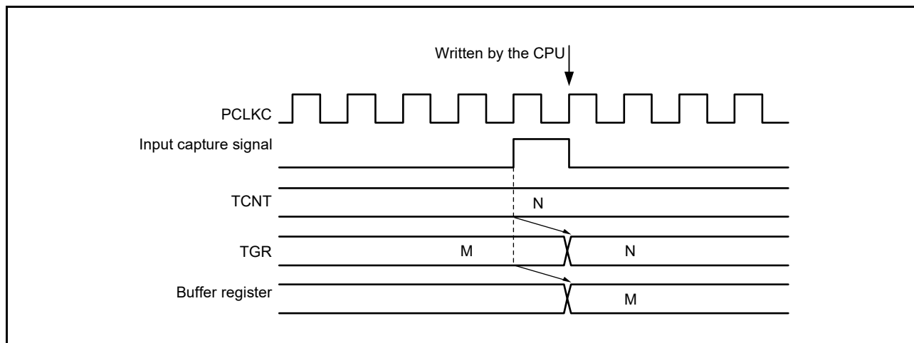
Figure 19.139 Contention between Buffer Register Write Operation and Input Capture
