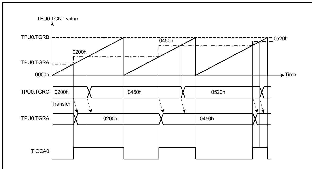
Figure 22.17 Example of Buffer Operation (1)
