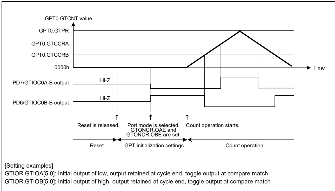
Figure 21.90 Example of Pin Settings after Reset
