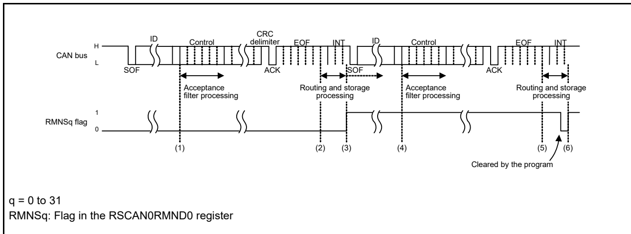
Figure 35.23 Reception Buffer Reception Timing Chart
