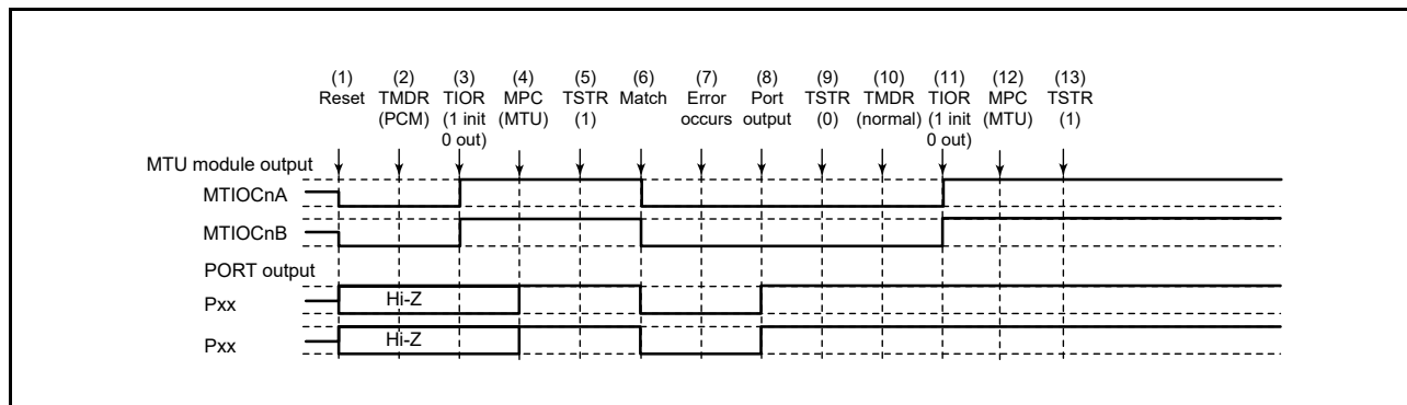
Figure 19.165 Error Occurrence in Phase Counting Mode, Recovery in Normal Mode
