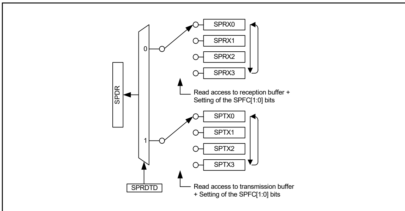
Figure 36.4 Configuration of SPDR (Reading)
