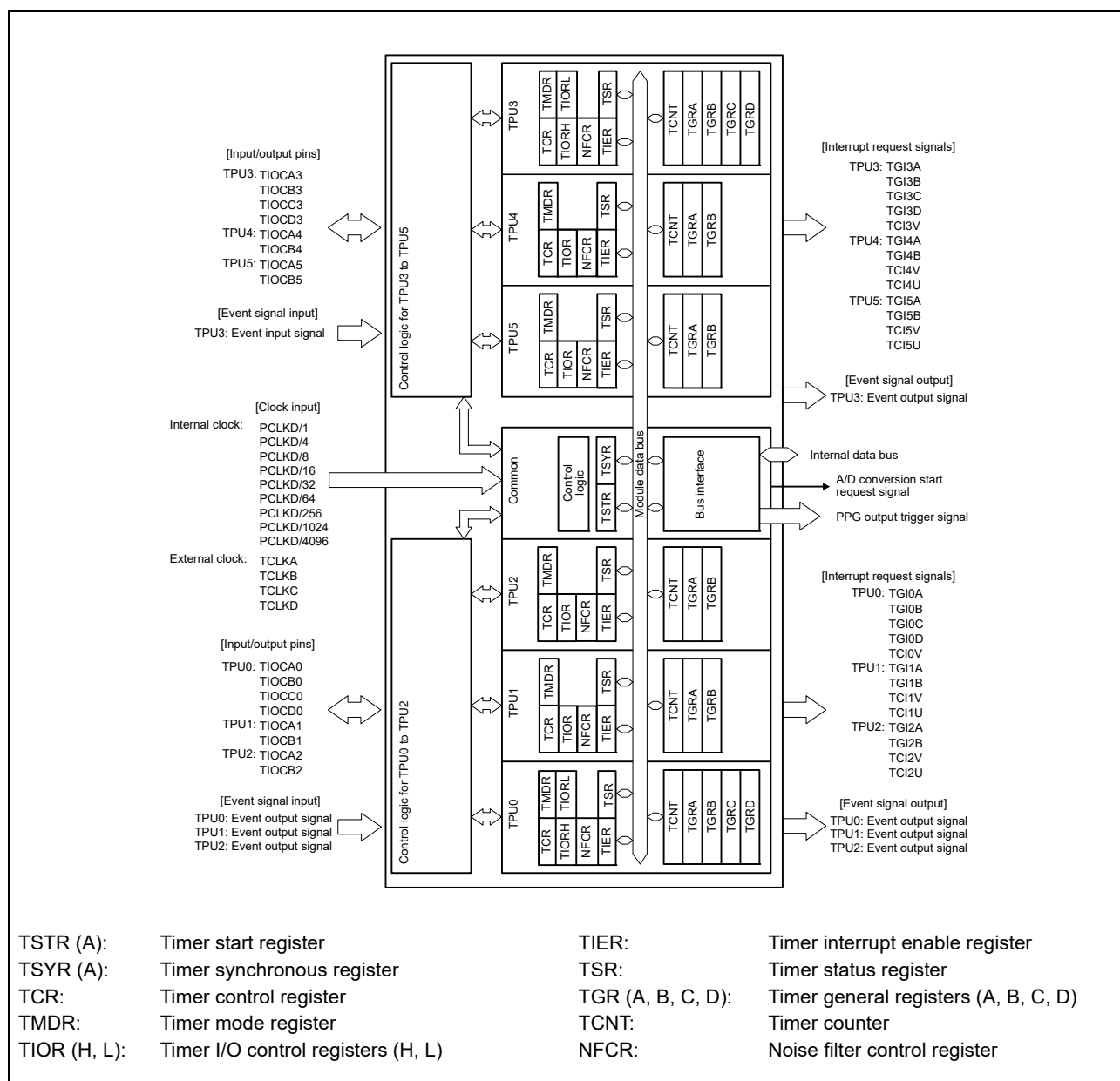
Figure 22.1 Block Diagram of TPU (Unit 0)
