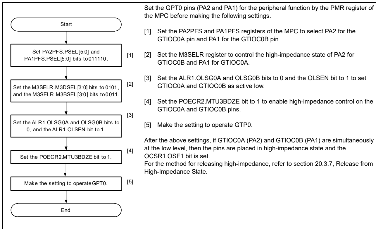
Figure 20.6 Procedure for Setting POE3
