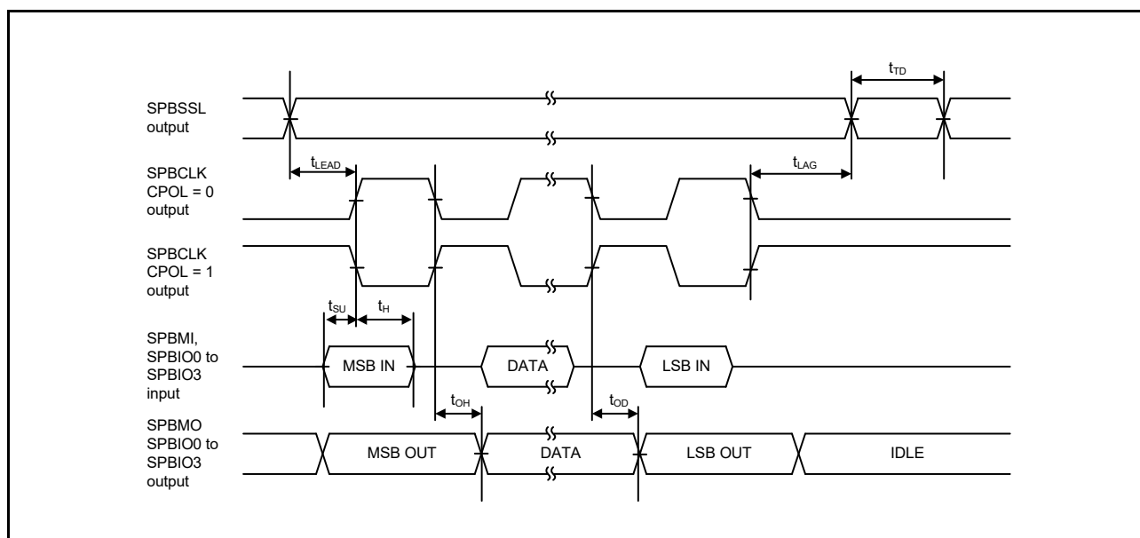
Figure 47.58 SPIBSC Transmit/Receive Timing (CPHAT = 0, CPHAR = 0)
