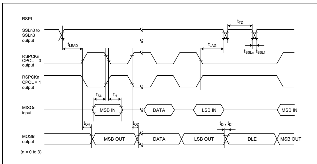
Figure 47.54 RSPIa Timing (Master, CPHA = 1)
