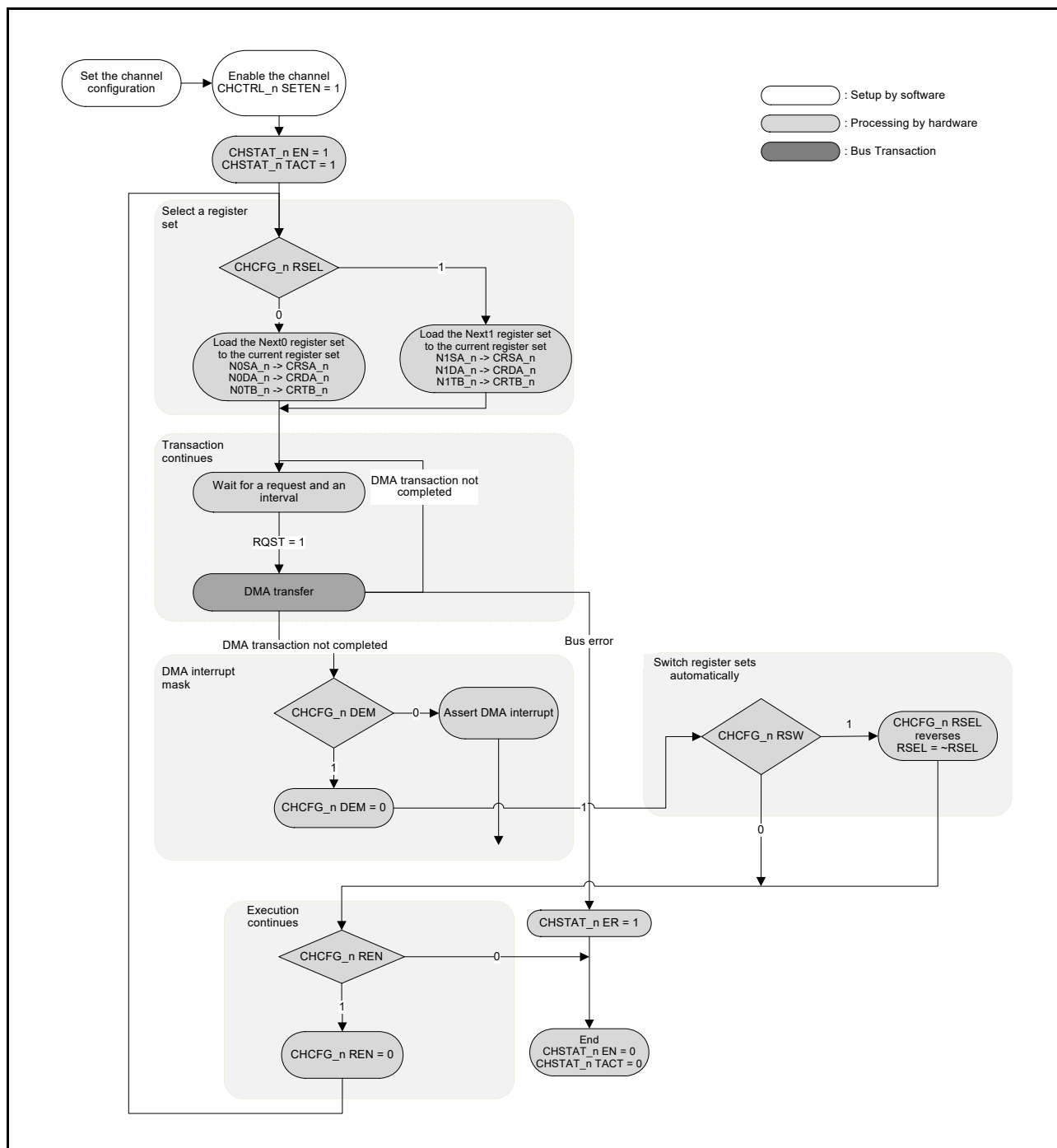
Figure 15.4 Register Mode Flow
