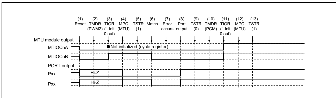
Figure 19.164 Error Occurrence in PWM Mode 2, Recovery in Phase Counting Mode
