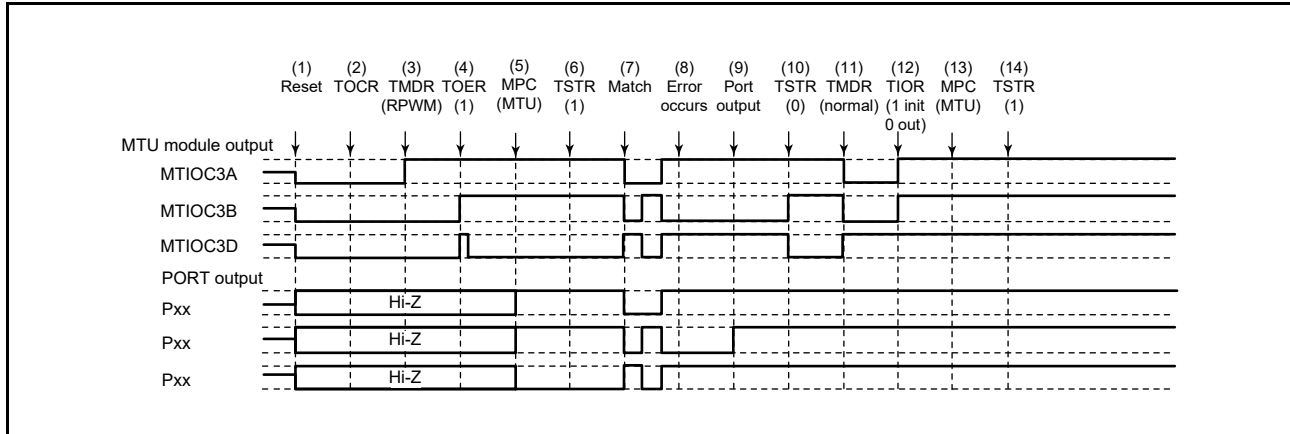
Figure 19.174 Error Occurrence in Reset-Synchronized PWM Mode, Recovery in Normal Mode
