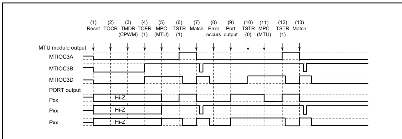
Figure 19.171 Error Occurrence in Complementary PWM Mode, Recovery in Complementary PWM Mode (1)
