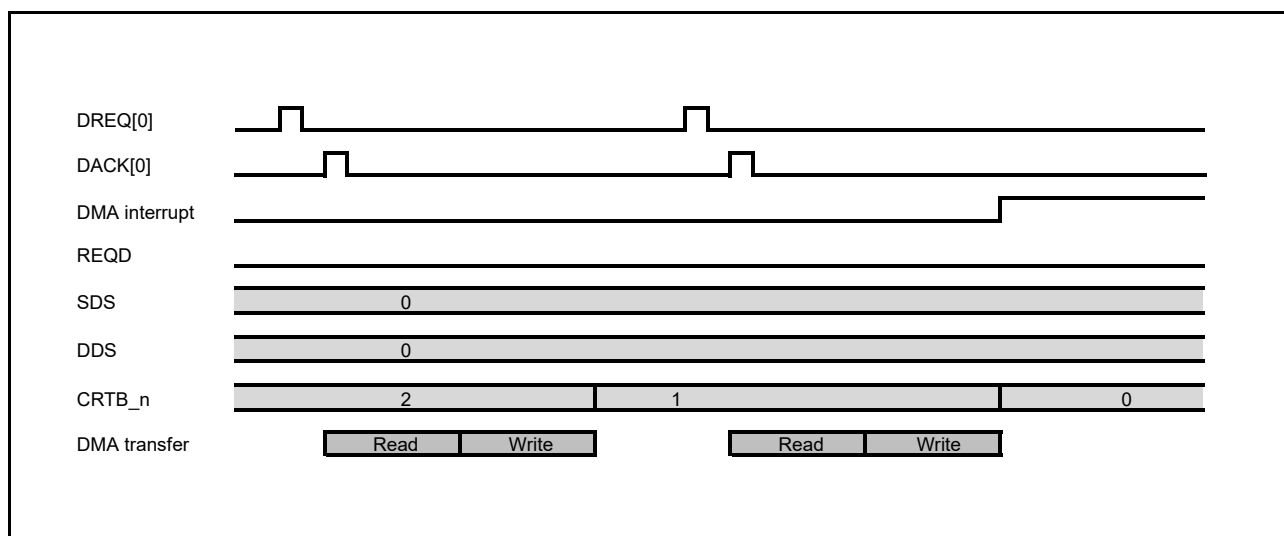
Figure 15.31 When the Sizes of Data on the Transfer Source and the Transfer Destination are the Same (LVL = 0, HIEN = 1, REQD = 0, and SDS = DDS in CHCFG_n)
