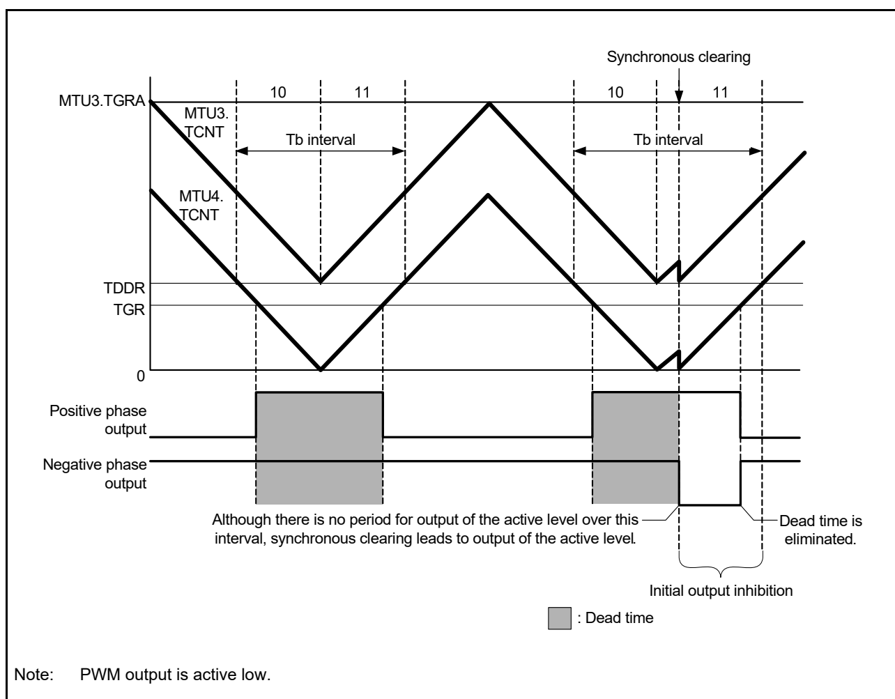
Figure 19.147 Example of Synchronous Clearing (when Condition 2 Applies)
