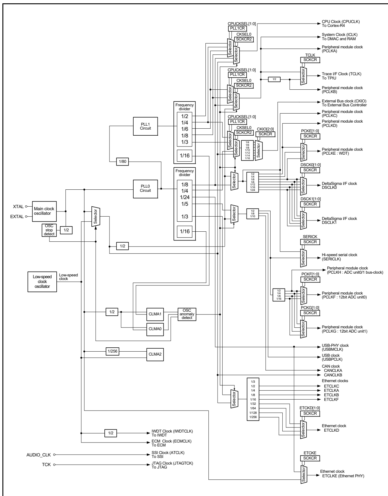
Figure 7.1 Block Diagram of Clock Generation Circuit
