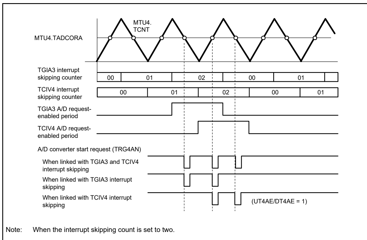
Figure 19.95 Example of A/D Converter Start Request Signal (TRG4AN) Operation Linked with Interrupt Skipping Function 1 (UT4AE and DT4AE = 1)
