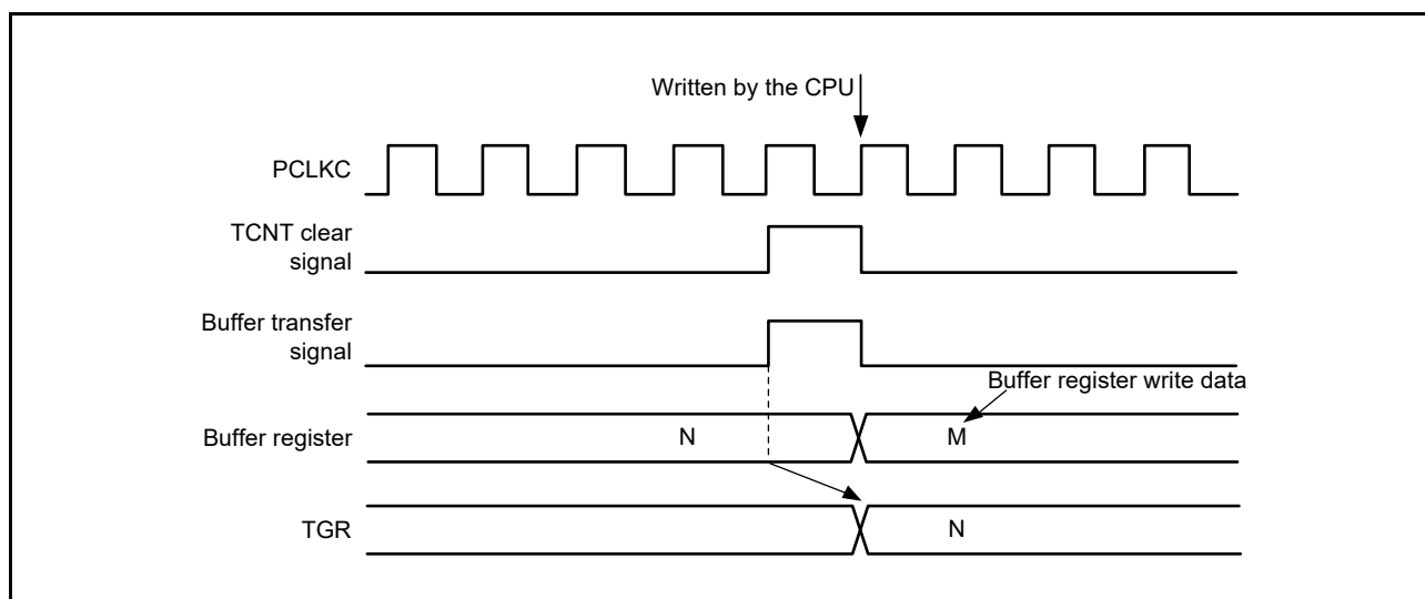
Figure 19.135 Contention between Buffer Register Write and TCNT Clear Operations
