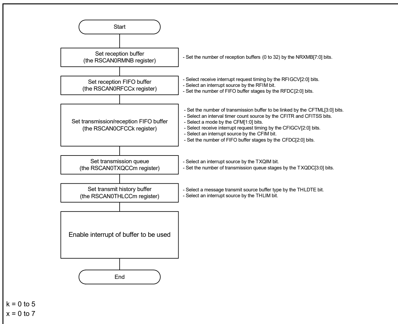
Figure 35.21 Buffer Setting Procedure
