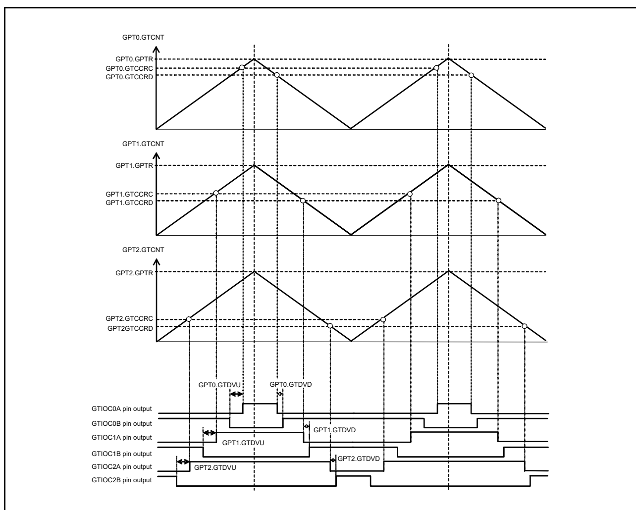
Figure 21.67 Example of Three-Phase Asymmetric Triangle-Wave Complementary PWM Output with Automatic Dead Time Setting
