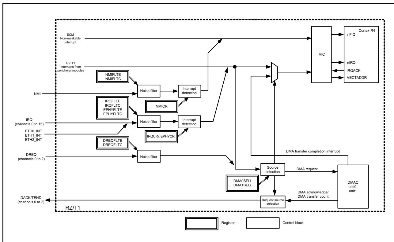
Figure 12.1 Block Diagram of Interrupt Controller
