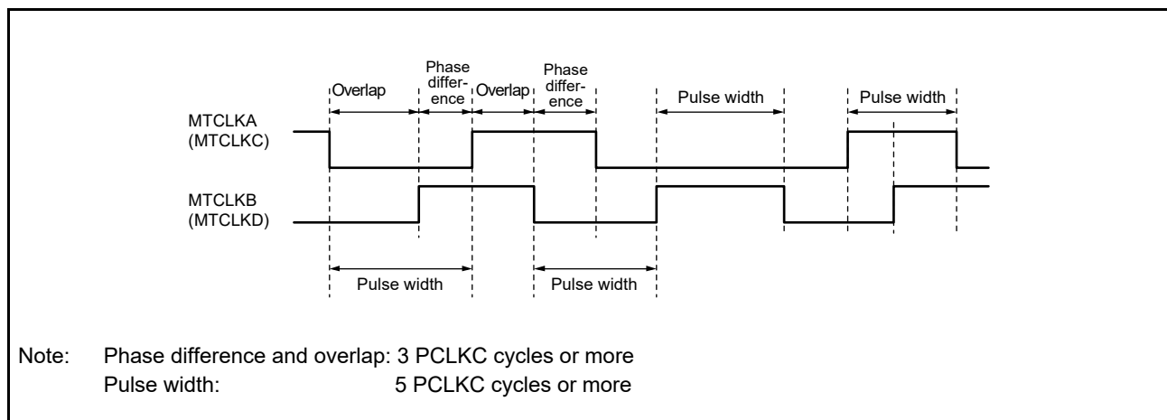
Figure 19.130 Phase Difference, Overlap, and Pulse Width in Phase Counting Mode
