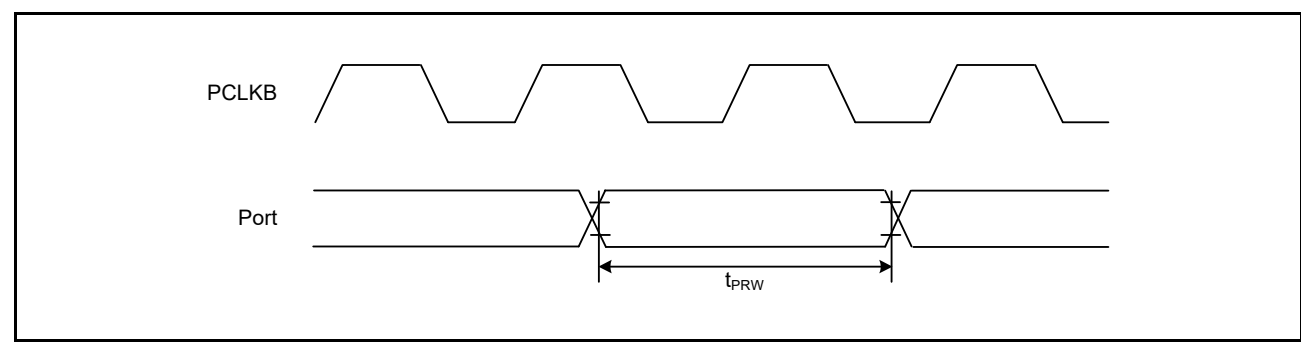
Figure 47.39 I/O Port Input Timing
