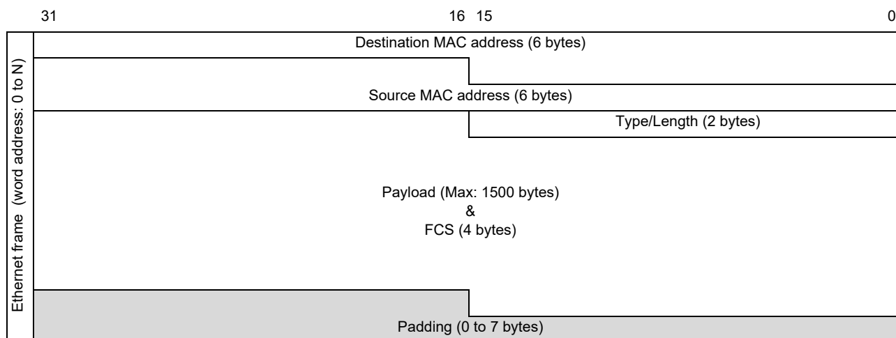
Figure 28.26 Received Ethernet Frame (TCPIPACC Disabled, VLAN Tag not Included)
