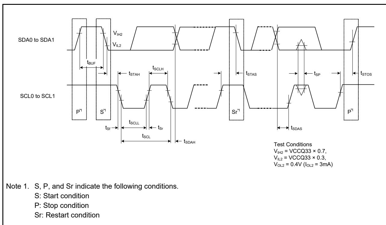
Figure 47.64 IICa Bus Interface Input/Output Timing
