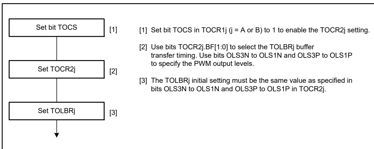
Figure 19.4 Example of PWM Output Level Setting Procedure in Buffer Operation
