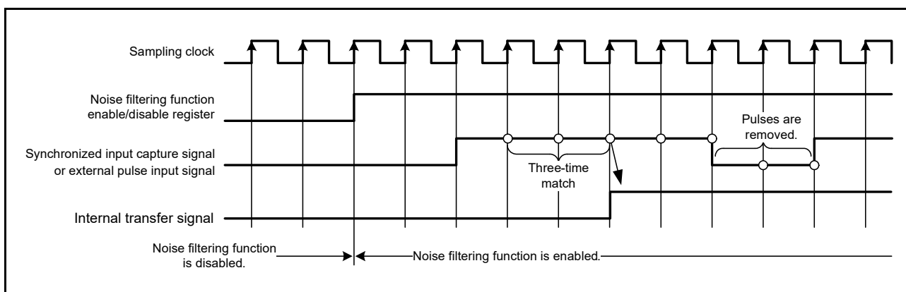
Figure 19.107 Timing of Noise Filtering
