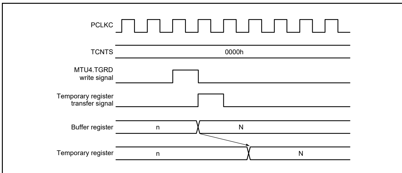
Figure 19.121 Transfer Timing from Buffer Register to Temporary Register (TCNTSA Stopped)
