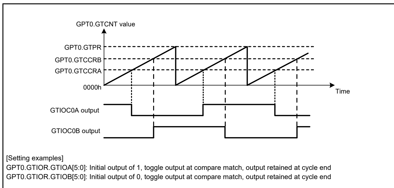
Figure 21.8 Example of Toggled Output Operation (1)
