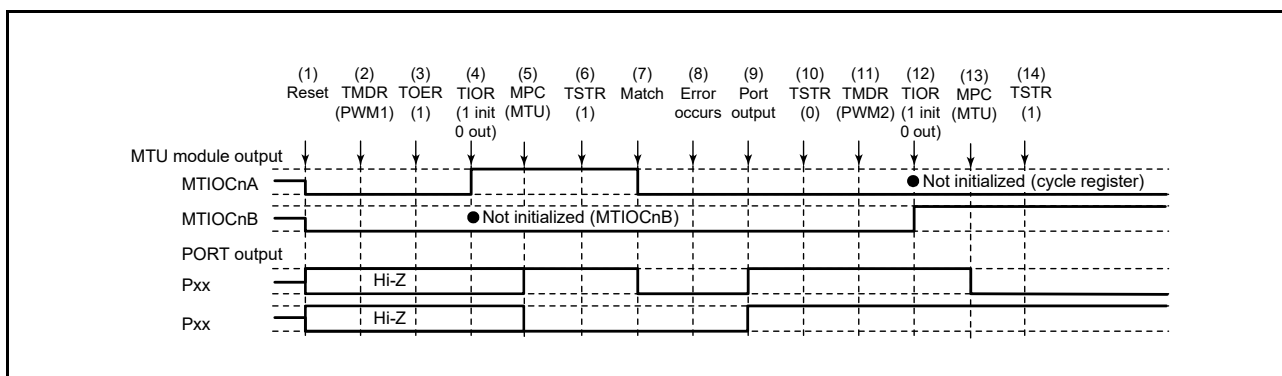
Figure 19.157 Error Occurrence in PWM Mode 1, Recovery in PWM Mode 2
