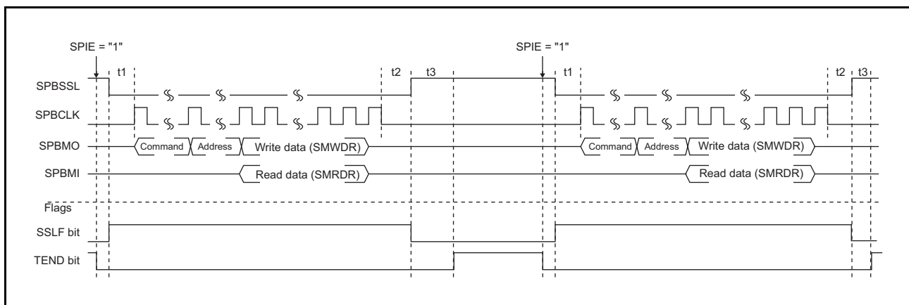
Figure 37.13 SPI Operation Timing
