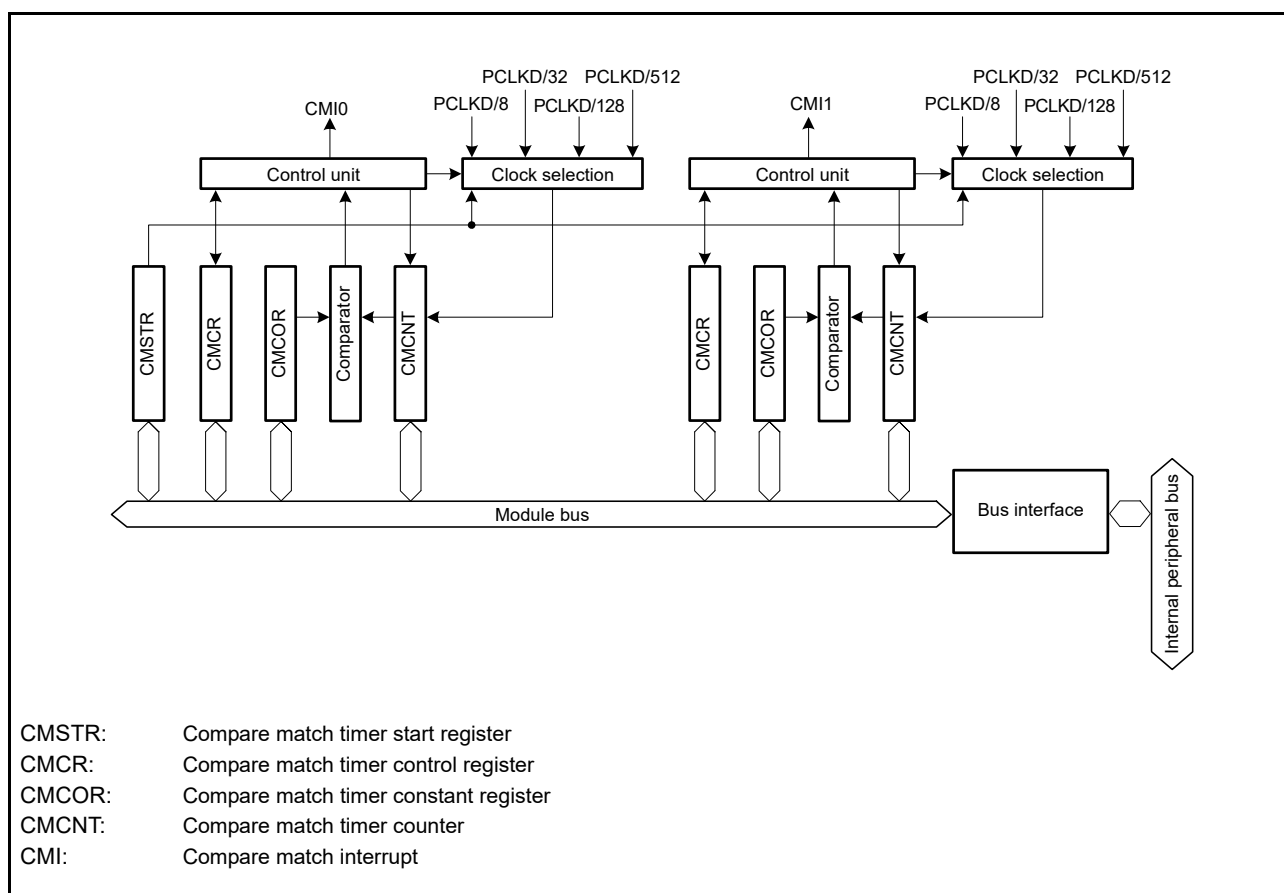
Figure 24.1 Block Diagram of CMT (Units 0 to 2)
