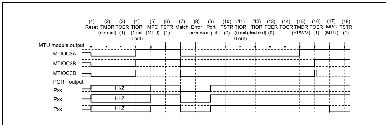
Figure 19.154 Error Occurrence in Normal Mode, Recovery in Reset-Synchronized PWM Mode
