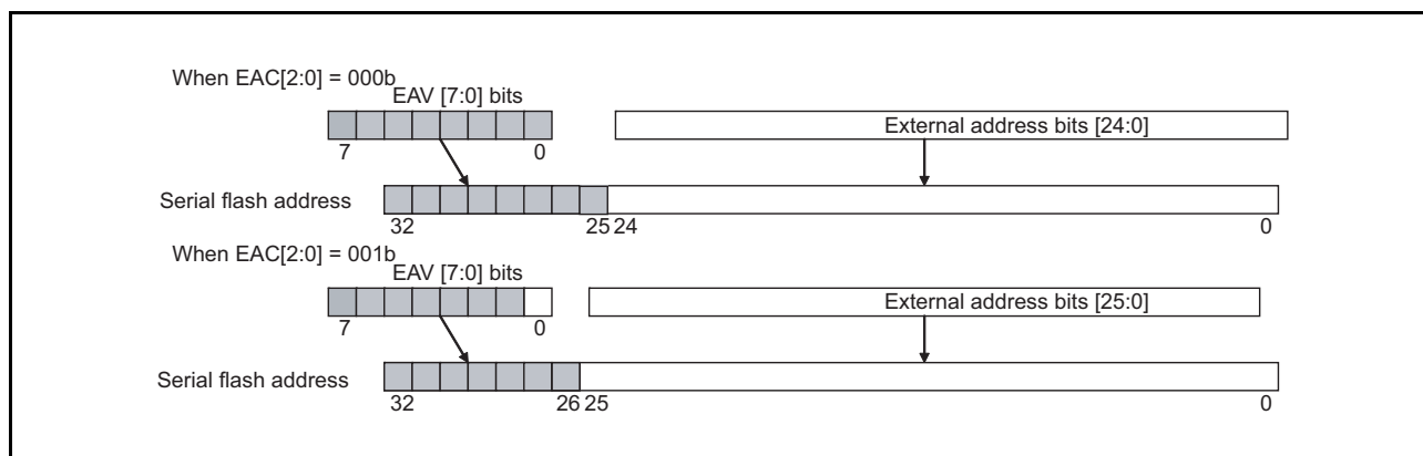
Figure 37.3 32-Bit Address Setting
