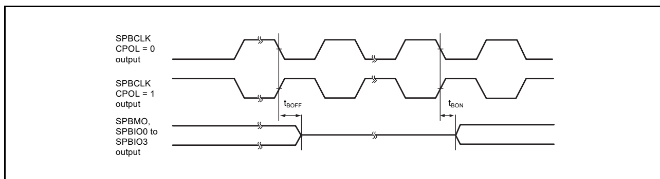
Figure 47.63 SPIBSC Buffer On/Off Timing (CPHAT = 0, CPHAR = 1)
