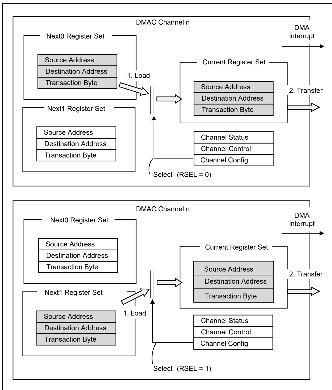
Figure 15.3 Overview of Register Normal Mode
