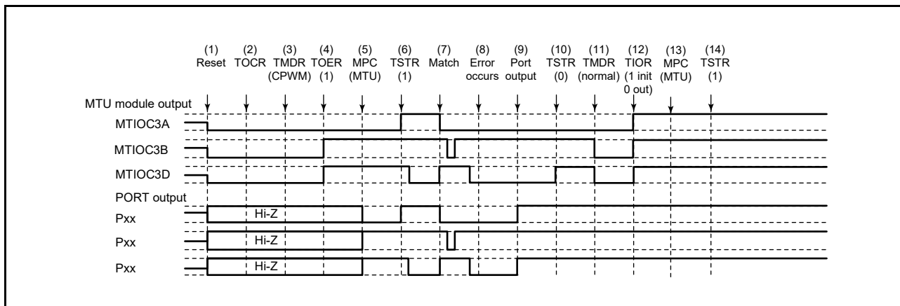
Figure 19.169 Error Occurrence in Complementary PWM Mode, Recovery in Normal Mode
