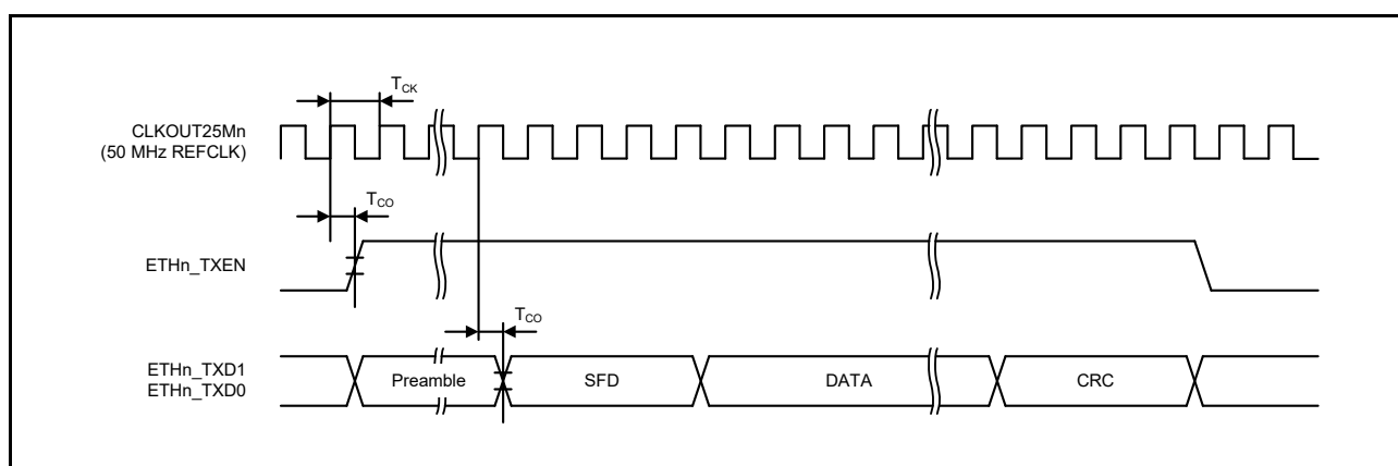
Figure 47.71 RMII Transmission Timing
