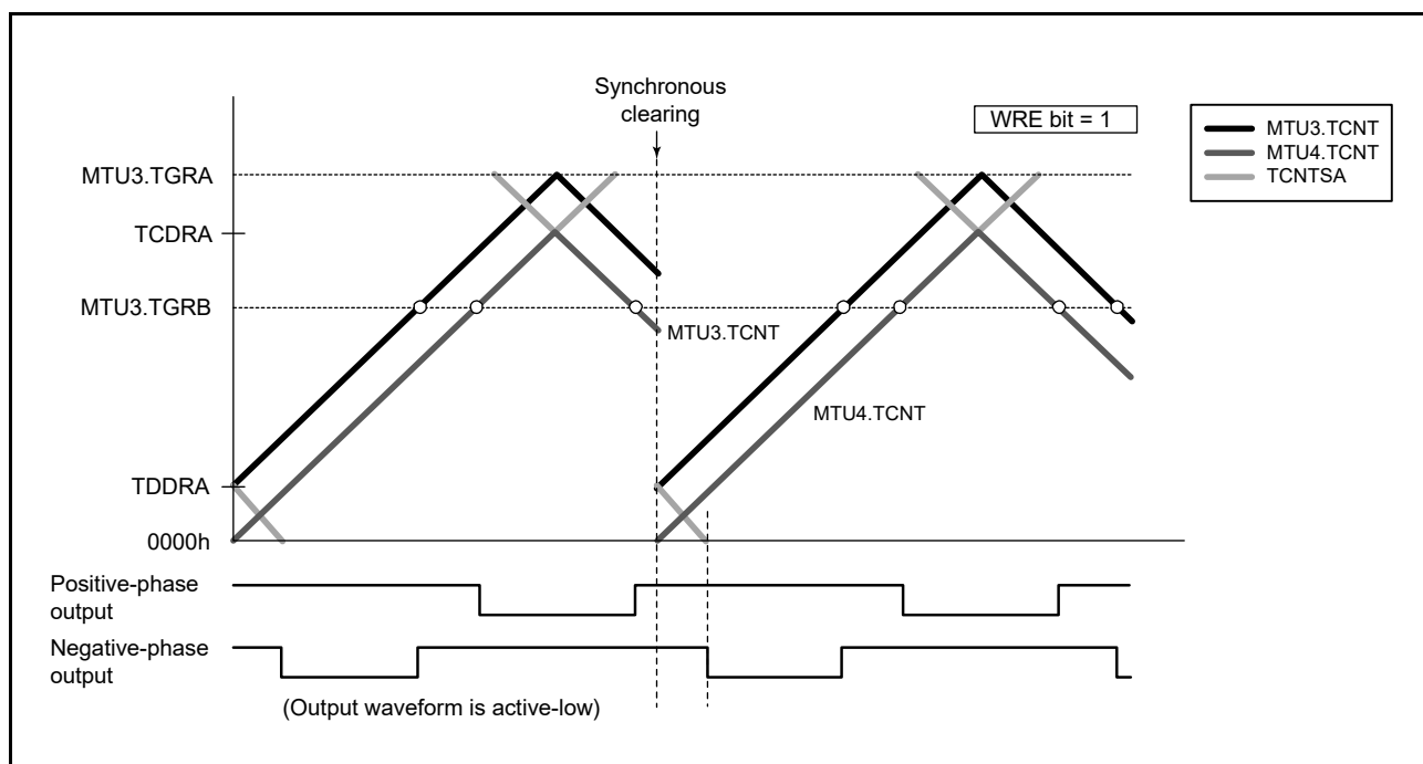
Figure 19.70 Example of Synchronous Clearing in Dead Time during Down-Counting (Timing (8) in Figure 19.66; Bit WRE of TWCRA is 1)
