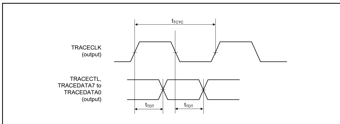
Figure 47.90 Trace Interface Timing
