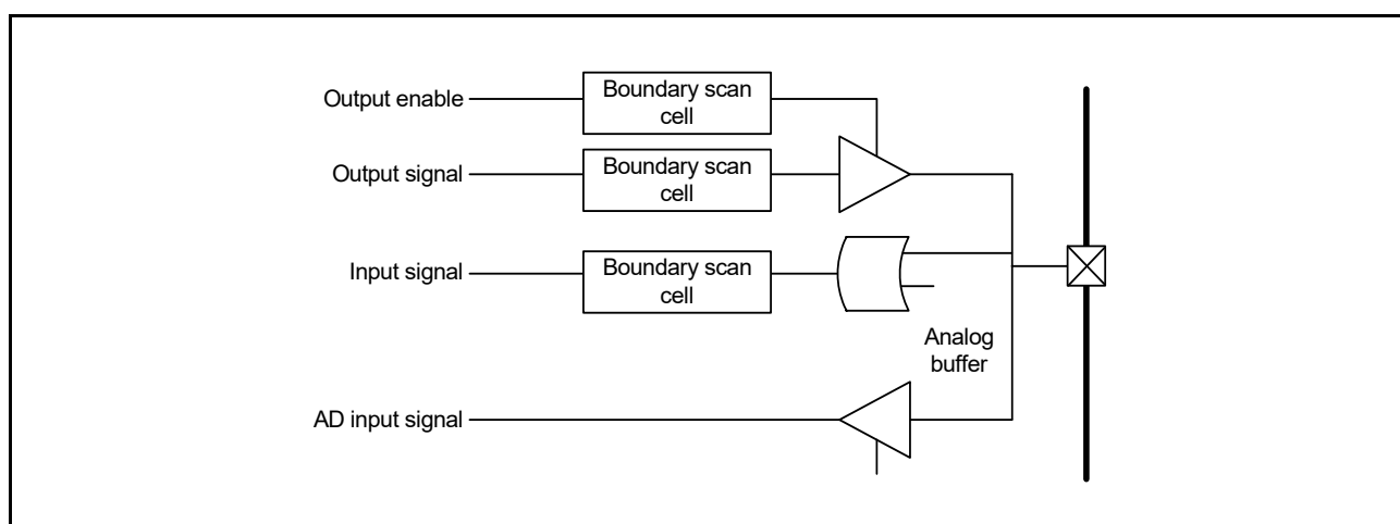
Figure 40.4 AD Pin Configuration
