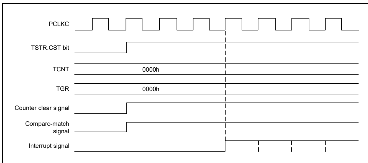
Figure 19.148 Continuous Output of Interrupt Signal in Response to a Compare Match
