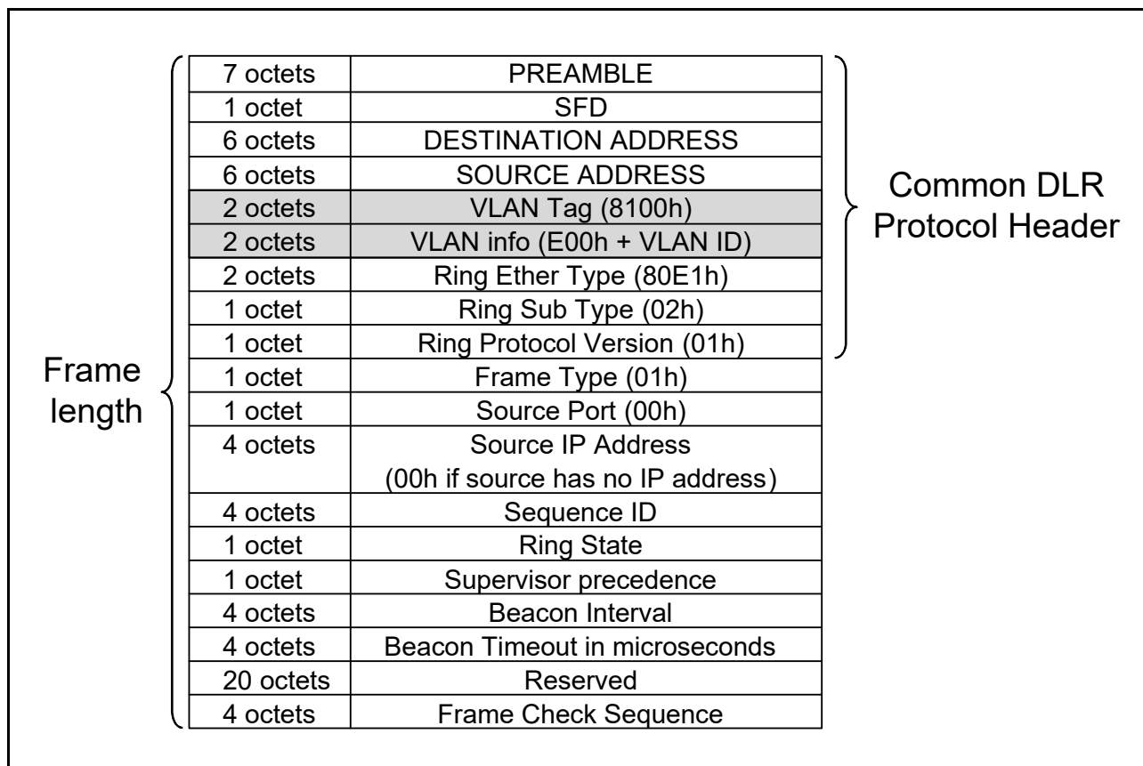
Figure 29.16 Beacon Frame Format
