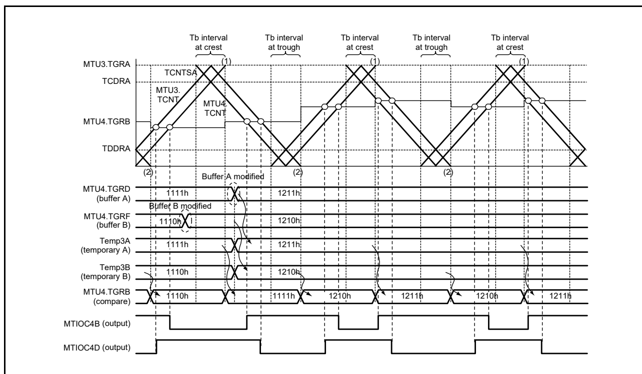
Figure 19.83 Example of Double Buffer Operation
