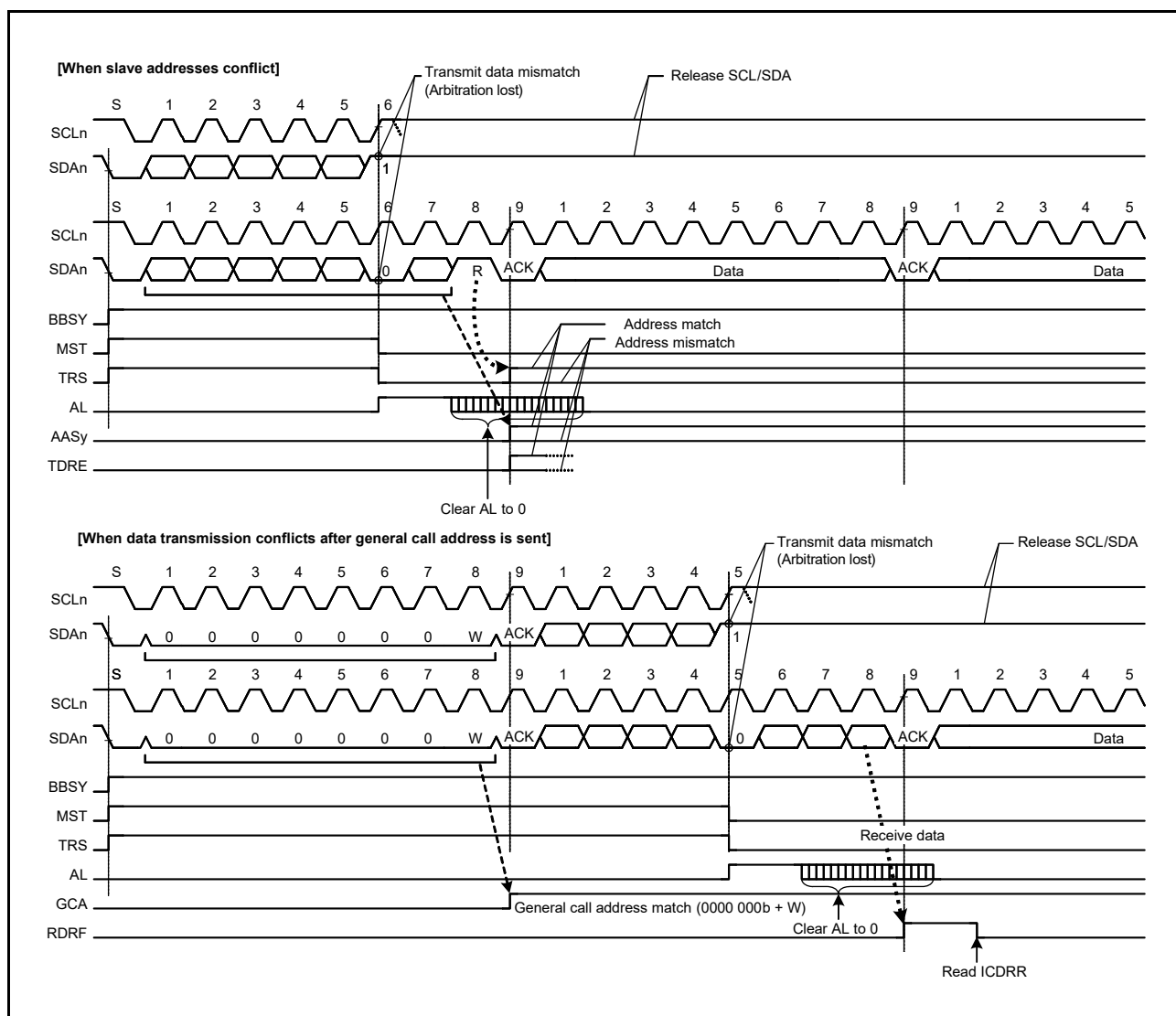
Figure 34.32 Examples of Master Arbitration-Lost Detection (MALE = 1)
