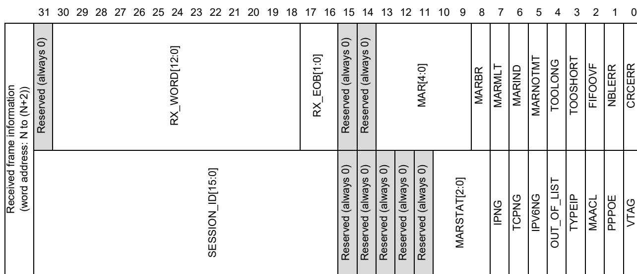
Figure 28.20 Received Frame Information
