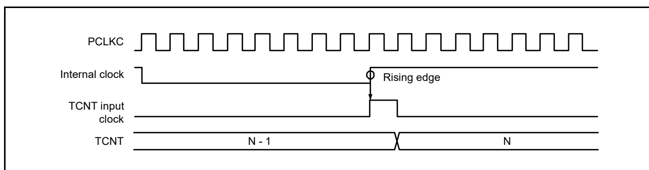
Figure 19.109 Count Timing in Internal Clock Operation (MTU5)
