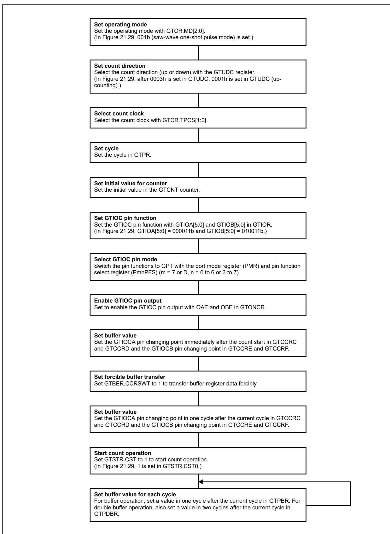
Figure 21.30 Example for Setting Saw-Wave One-Shot Pulse Mode
