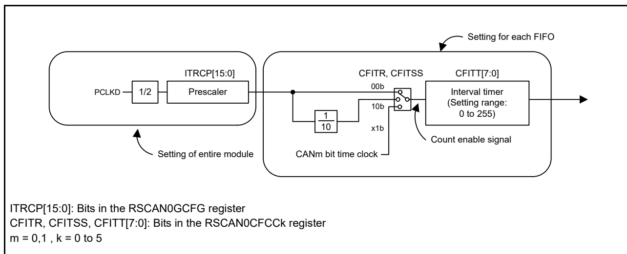
Figure 35.10 Interval Timer Block Diagram
