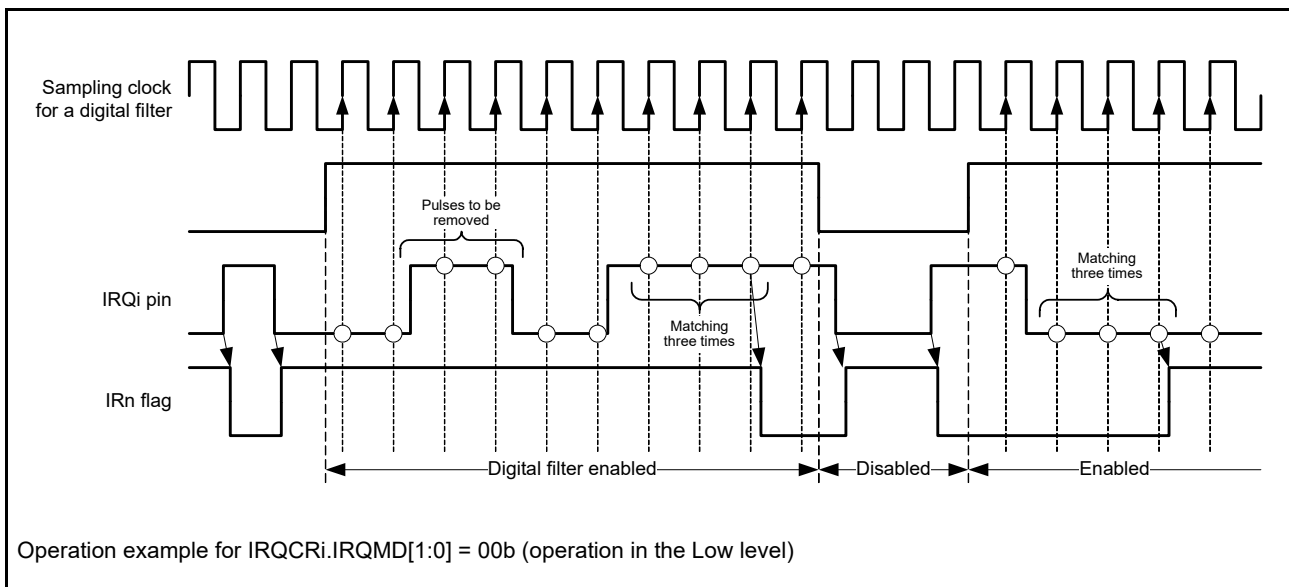
Figure 12.5 Digital Noise Filter Operation Example
