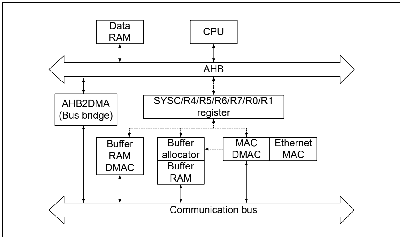
Figure 28.3 Schematic Block Diagram of the Hardware Functions
