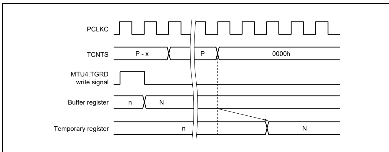
Figure 19.122 Transfer Timing from Buffer Register to Temporary Register (TCNTSA Operating)
