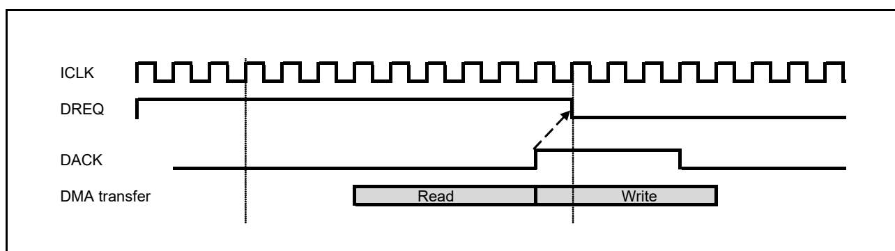
Figure 15.21 Level Detection Timing (High-Level Detection (HIEN = 1), DACK Output is Active during Writing (REQD = 1))
