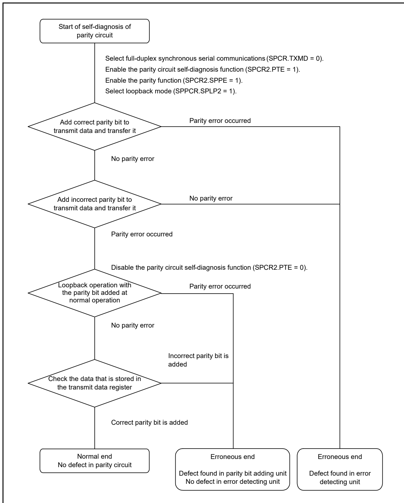
Figure 36.49 Flowchart for Self-Diagnosis of Parity Circuit
