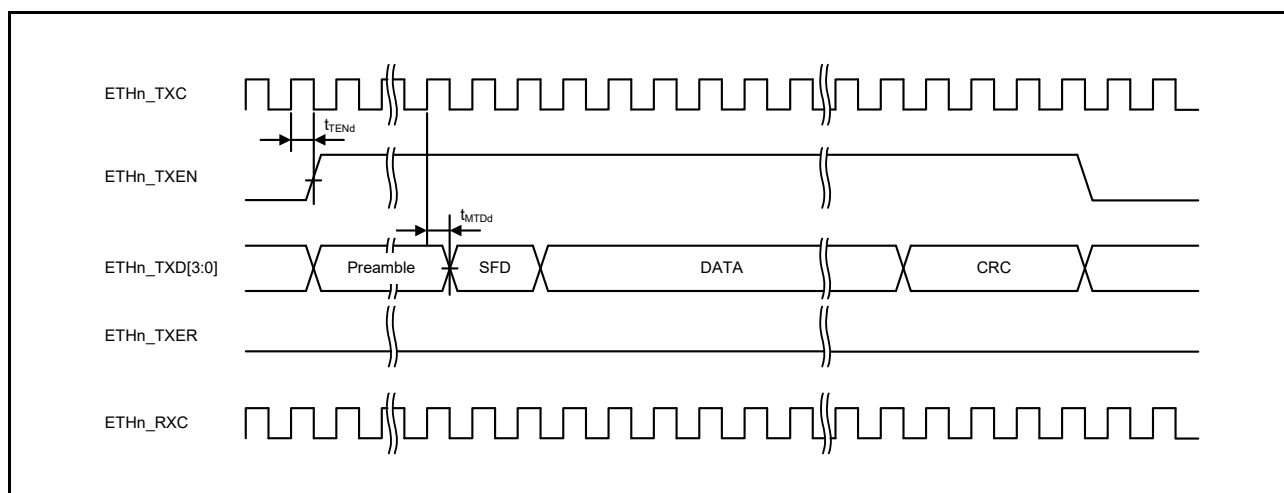
Figure 47.74 MII Transmission Timing
