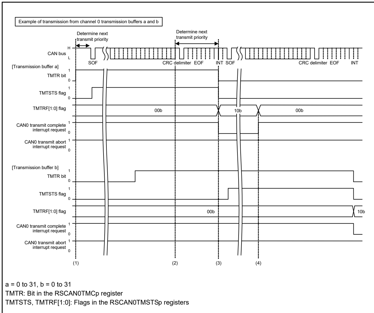
Figure 35.27 Transmission Buffer Transmission Timing Chart (Transmission Completed Successfully)
