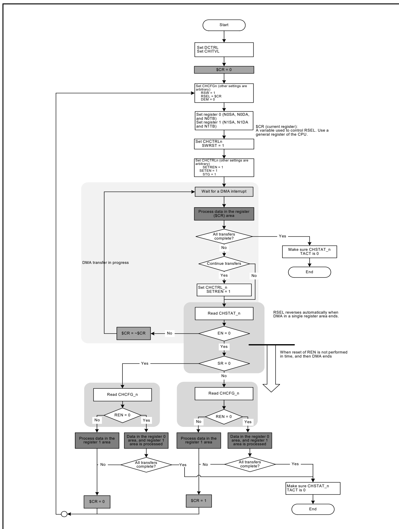
Figure 15.44 Setting Example of Next Register Continuous Execution
