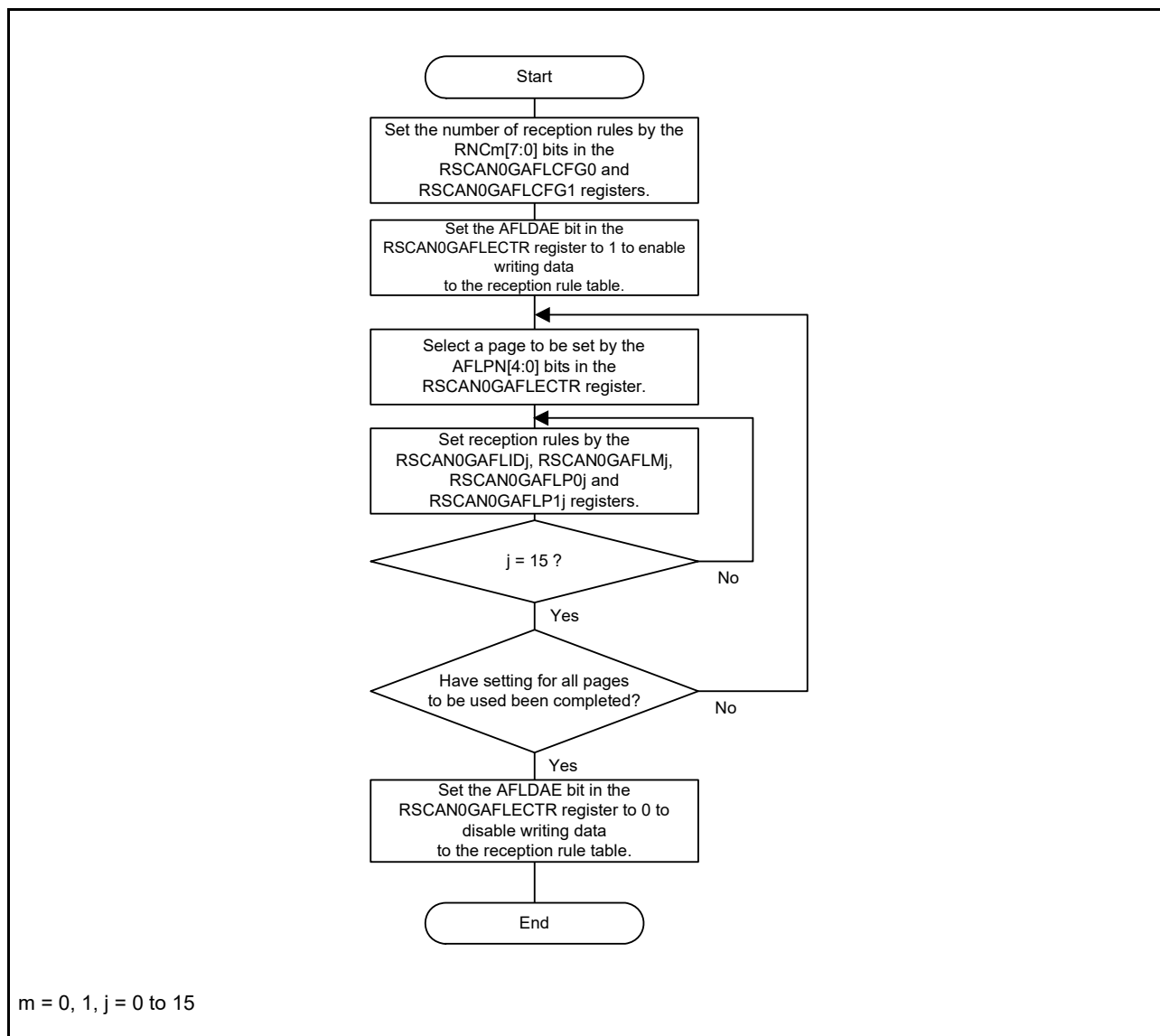
Figure 35.19 Reception Rule Setting Procedure
