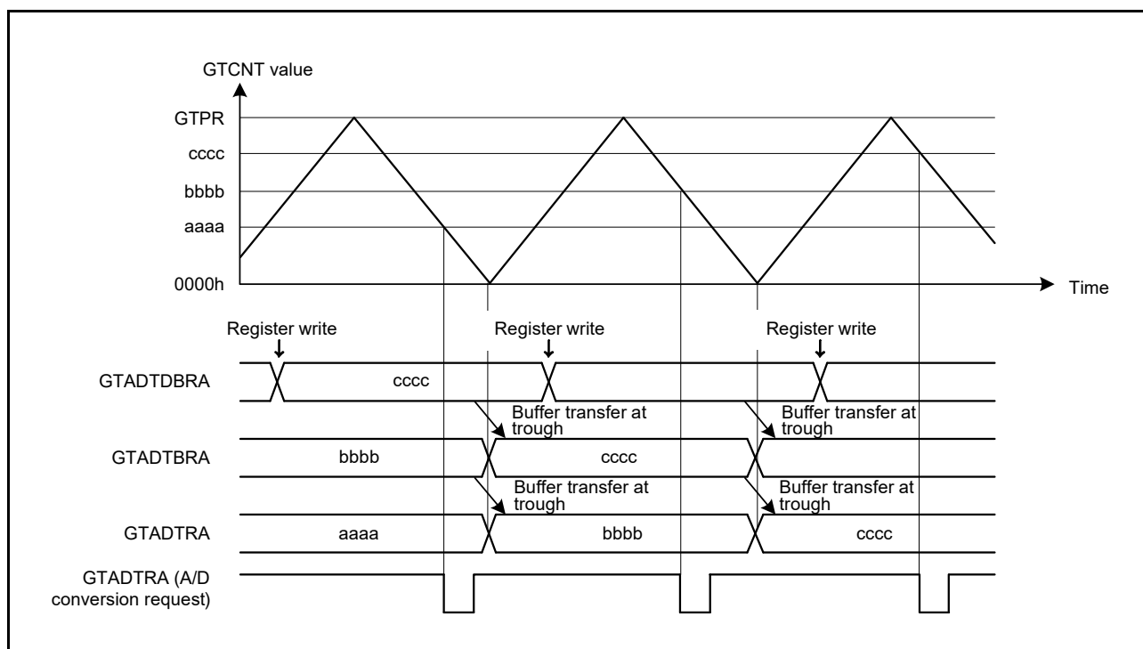
Figure 21.24 Example of GTADTRA and GTADTBRA Double Buffer Operation (Triangle Waves, Buffer Transfer at Troughs, A/D Converter Start Request Generated by Down-Counting)
