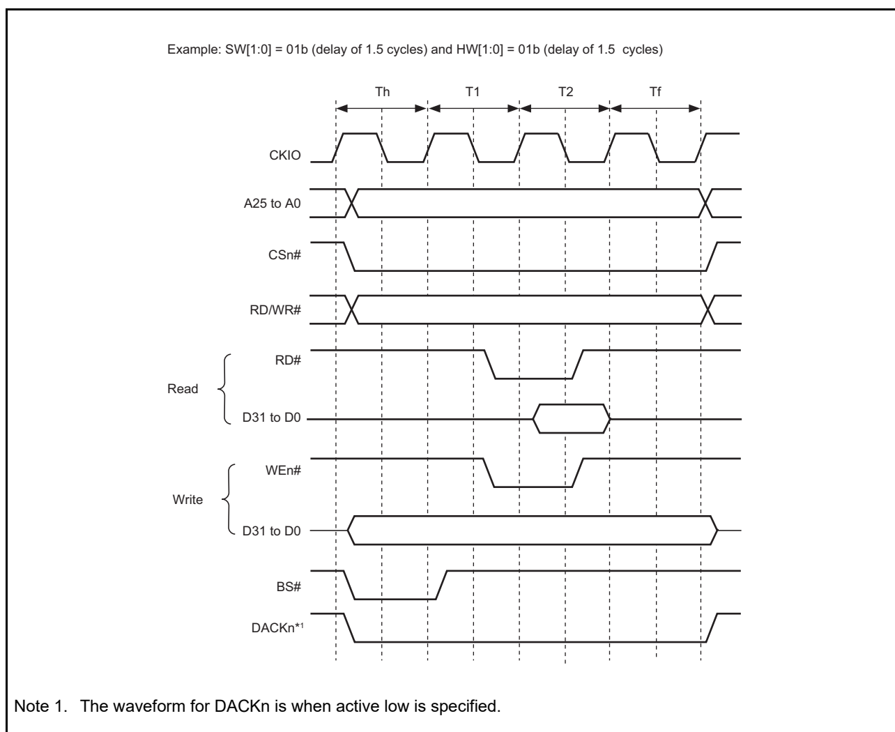
Figure 14.10 Active Period Expansion for the CSn Signal
