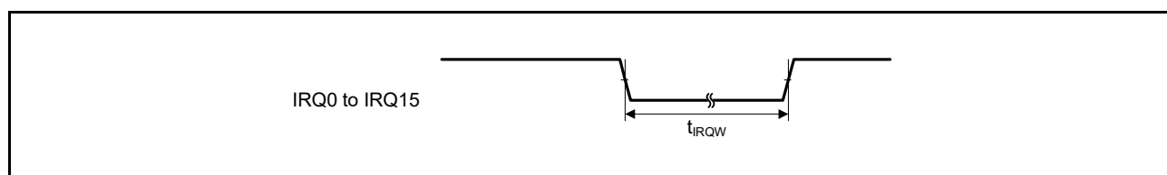
Figure 47.10 IRQ Interrupt Input Timing
