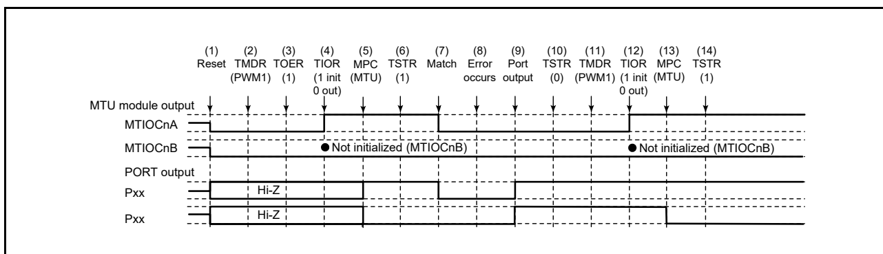
Figure 19.156 Error Occurrence in PWM Mode 1, Recovery in PWM Mode 1
