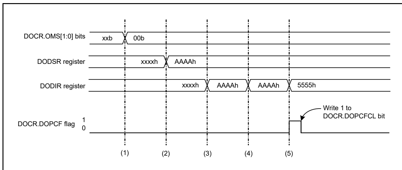
Figure 45.2 Example of Operation in Data Comparison Mode
