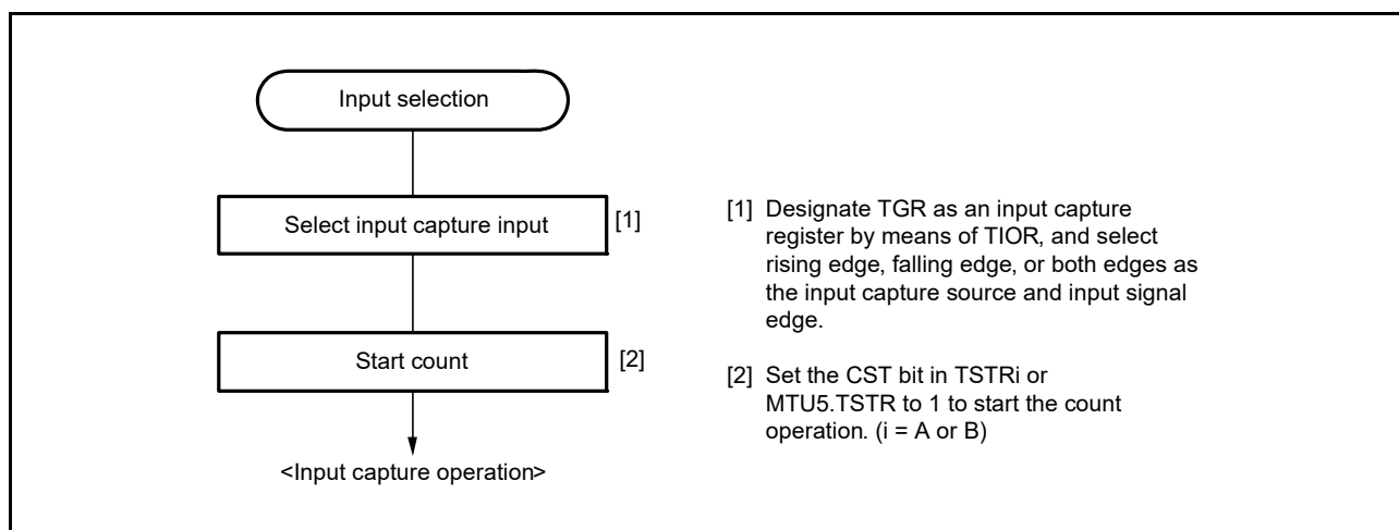
Figure 19.11 Example of Input Capture Operation Setting Procedure
