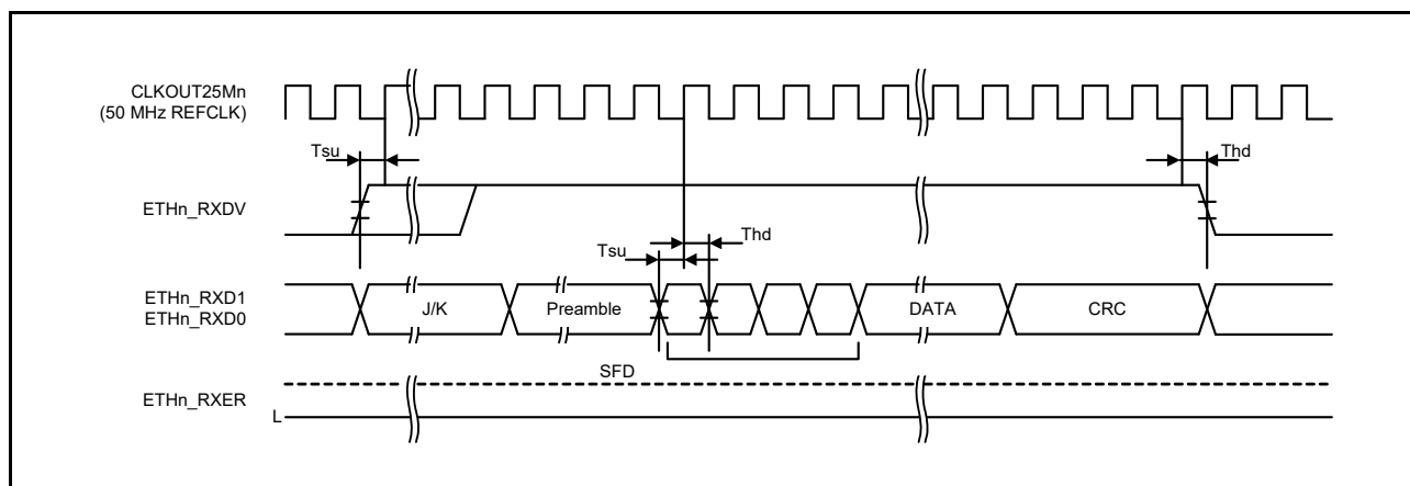
Figure 47.72 RMII Reception Timing (Normal Operation)
