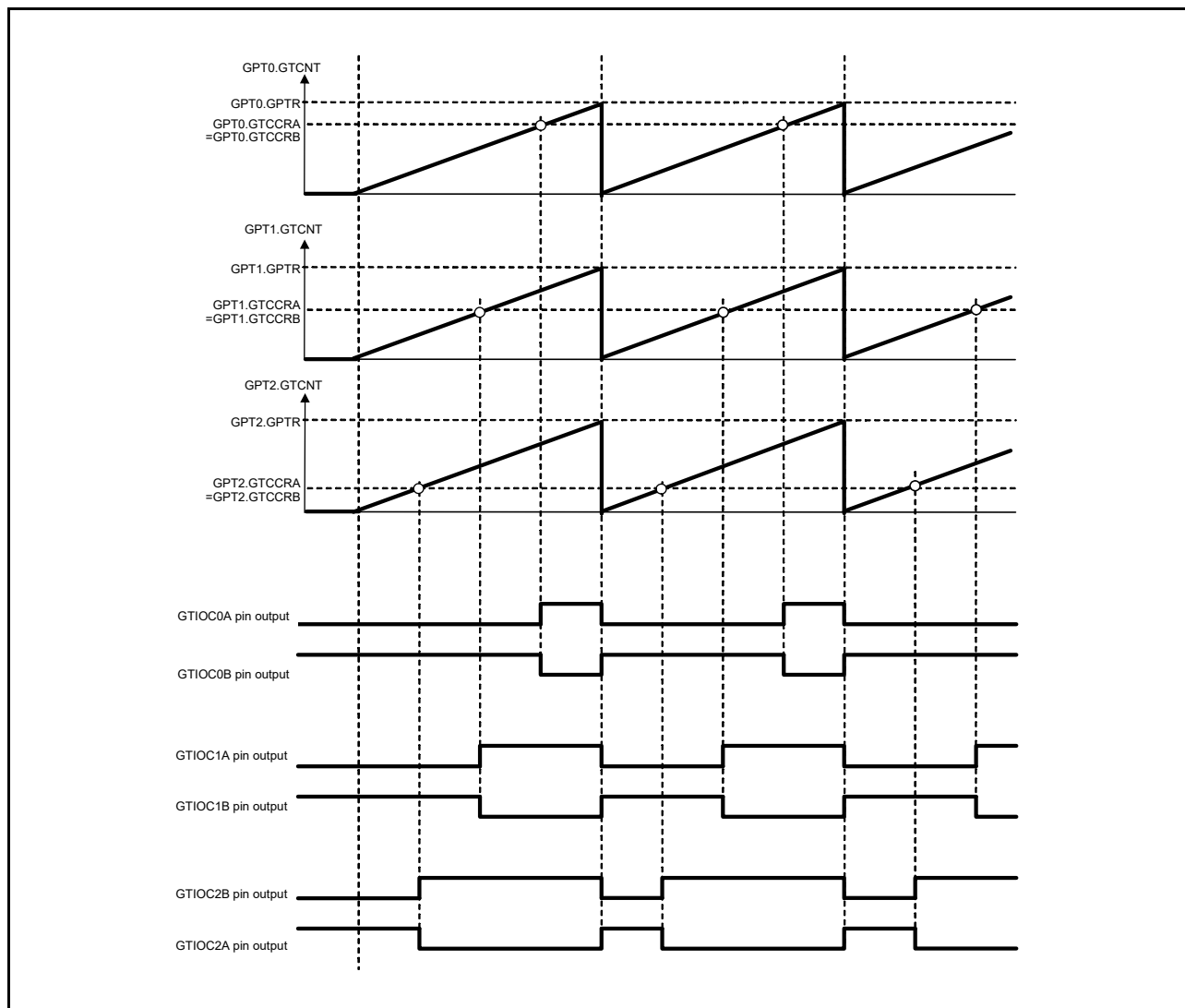
Figure 21.63 Example of Three-Phase Saw-Wave Complementary PWM Output
