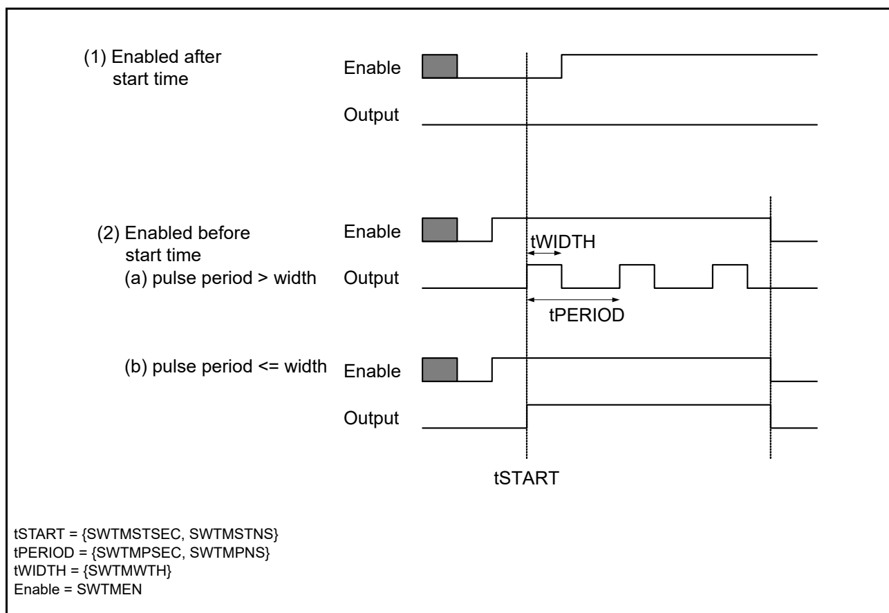
Figure 29.20 Timing Chart of Pulse Signal Generation Function
