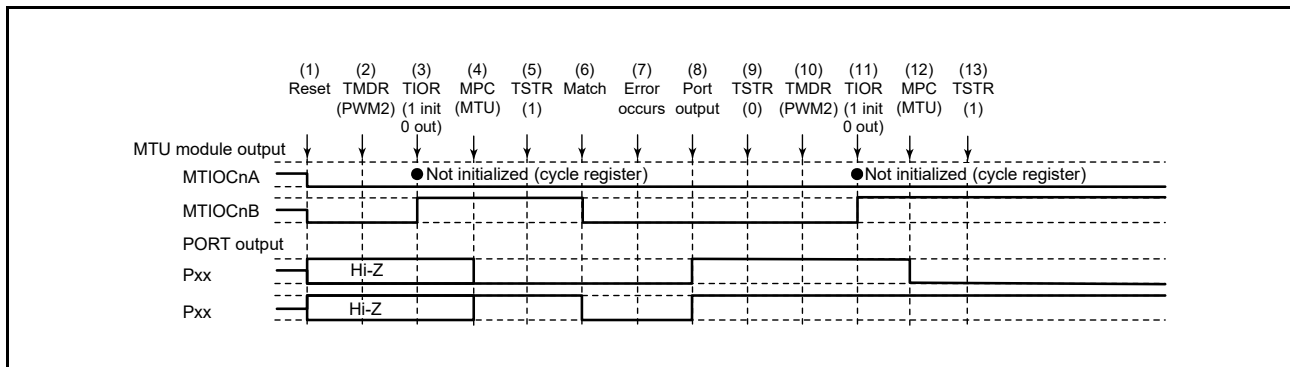
Figure 19.163 Error Occurrence in PWM Mode 2, Recovery in PWM Mode 2
