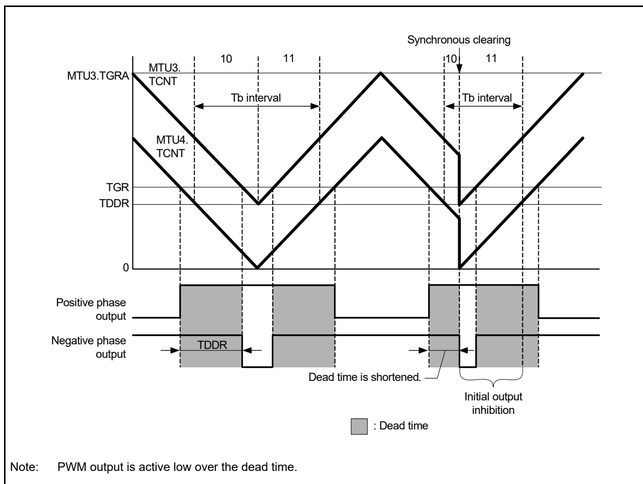
Figure 19.146 Example of Synchronous Clearing (when Condition 1 Applies)
