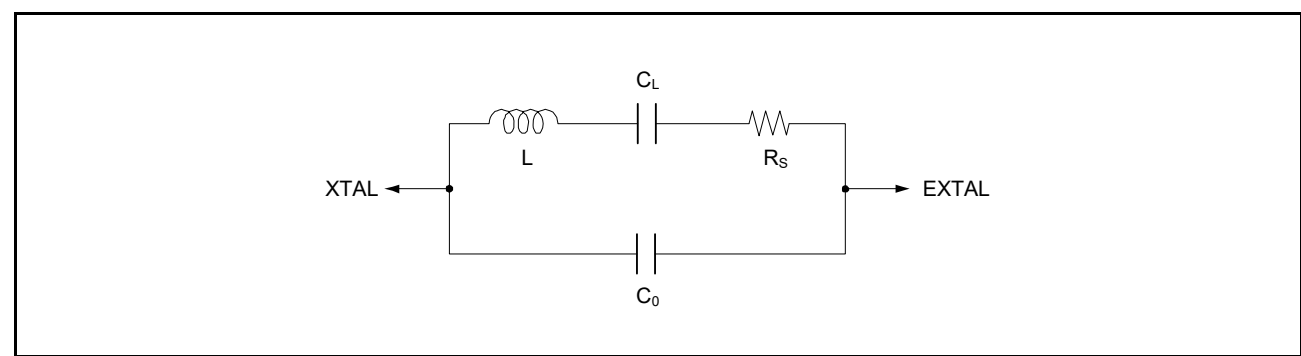
Figure 7.5 Equivalent Circuit of Crystal Resonator
