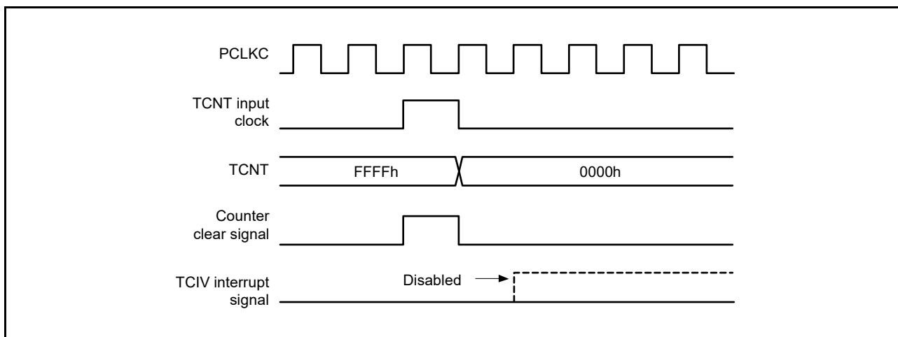
Figure 19.144 Contention between Overflow and Counter Clearing
