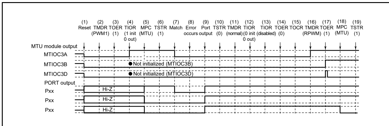
Figure 19.160 Error Occurrence in PWM Mode 1, Recovery in Reset-Synchronized PWM Mode
