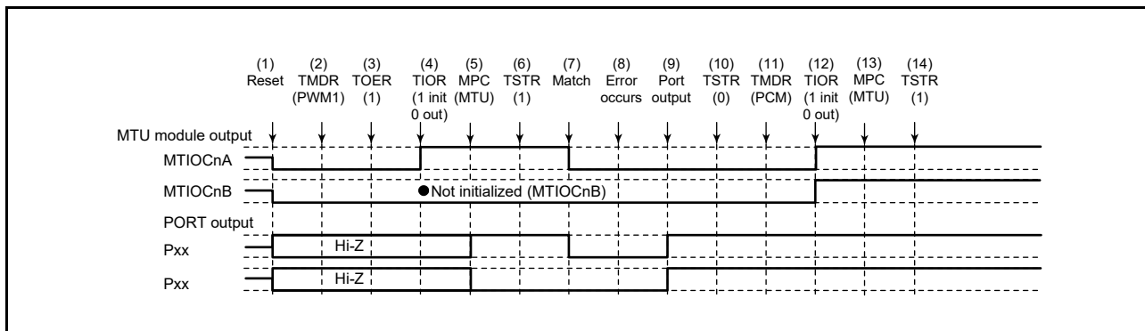
Figure 19.158 Error Occurrence in PWM Mode 1, Recovery in Phase Counting Mode
