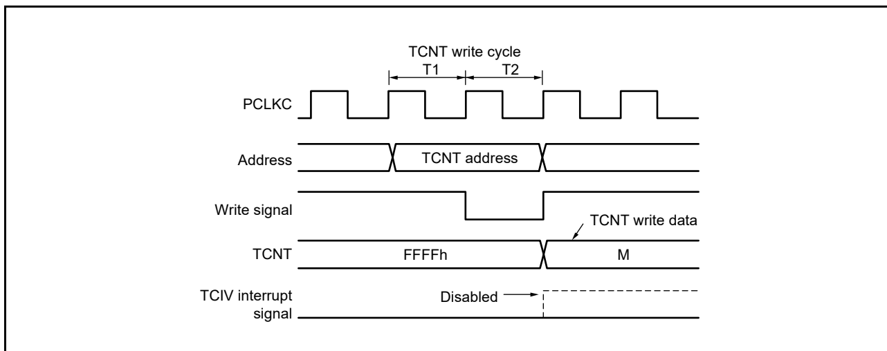
Figure 19.145 Contention between TCNT Write Operation and Overflow
