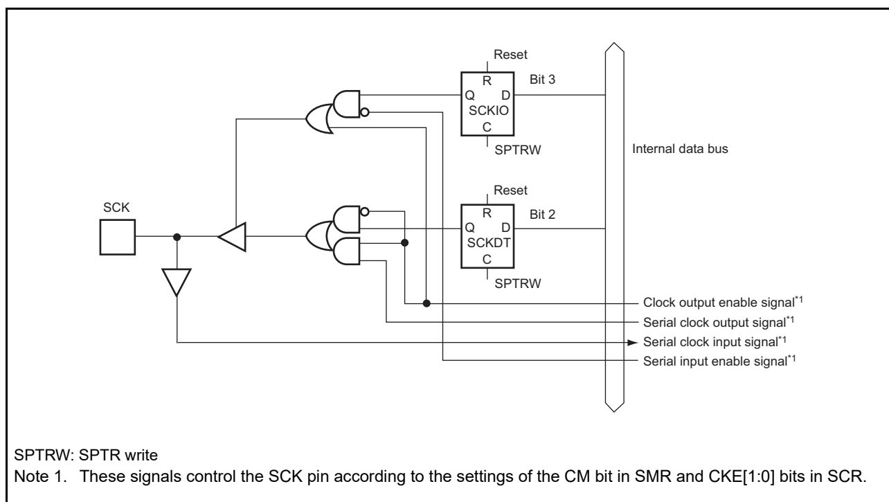
Figure 33.21 SCKIO Bit and SCKDT Bit in the SPTR Register, and SCK Pin
