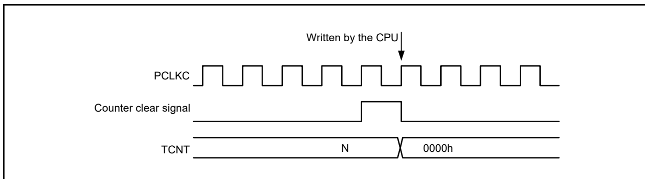
Figure 19.131 Contention between TCNT Write and Clear Operations
