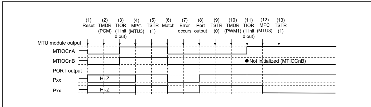
Figure 19.166 Error Occurrence in Phase Counting Mode, Recovery in PWM Mode 1
