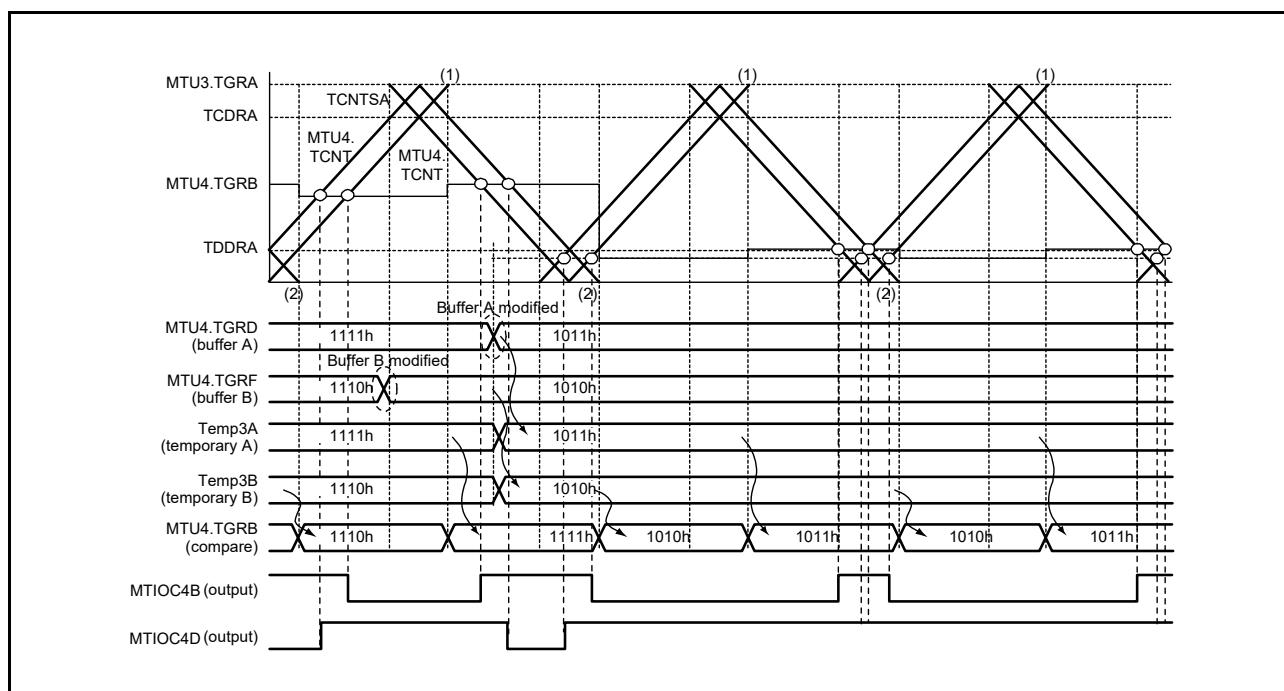
Figure 19.84 Example of Double Buffer Operation (Buffer Write Value is Smaller than TDDRA)
