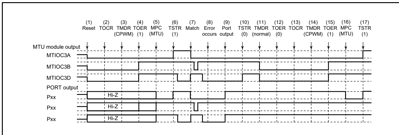
Figure 19.172 Error Occurrence in Complementary PWM Mode, Recovery in Complementary PWM Mode (2)
