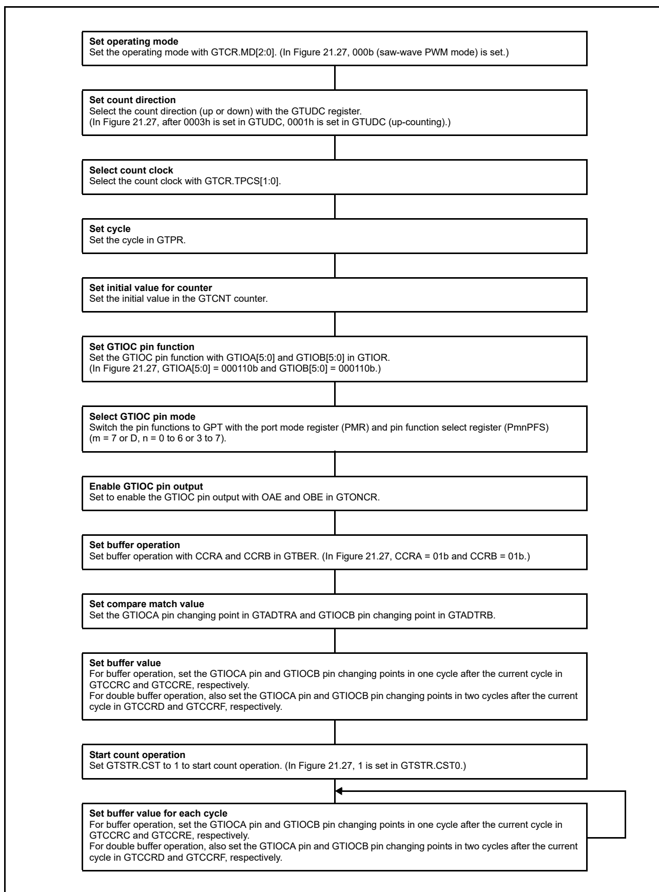
Figure 21.28 Example for Setting Saw-Wave PWM Mode
