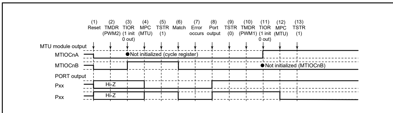
Figure 19.162 Error Occurrence in PWM Mode 2, Recovery in PWM Mode 1
