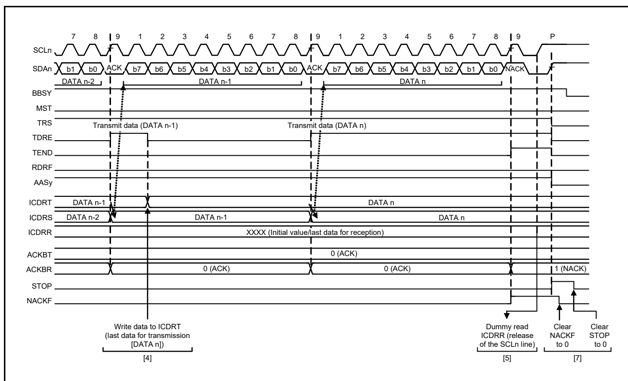
Figure 34.17 Slave Transmit Operation Timing (2)
