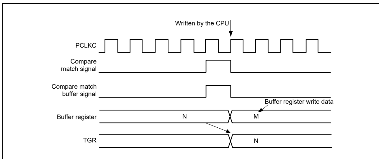
Figure 19.134 Contention between Buffer Register Write Operation and Compare Match
