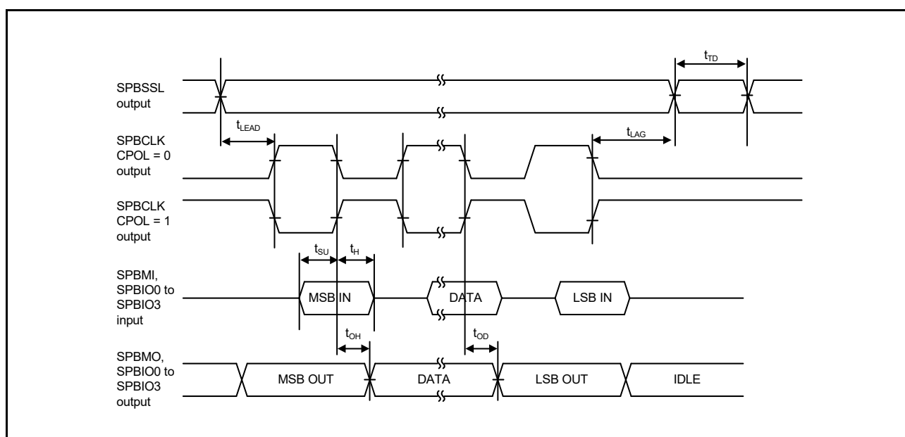
Figure 47.60 SPIBSC Transmit/Receive Timing (CPHAT = 0, CPHAR = 1)
