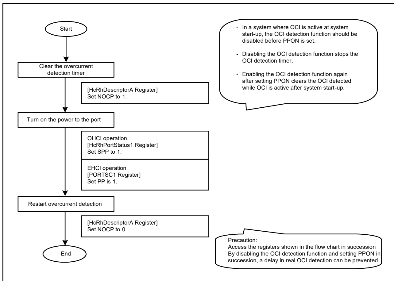
Figure 31.12 Flow for USB_VBUSEN Setting
