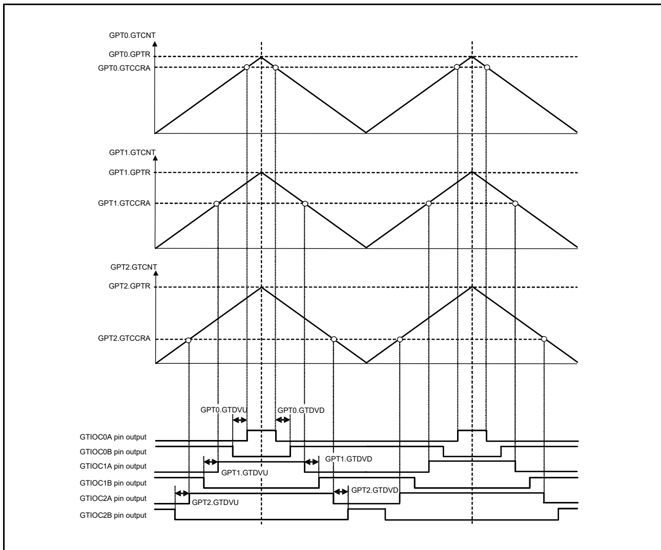
Figure 21.66 Example of Three-Phase Triangle-Wave Complementary PWM Output with Automatic Dead Time Setting
