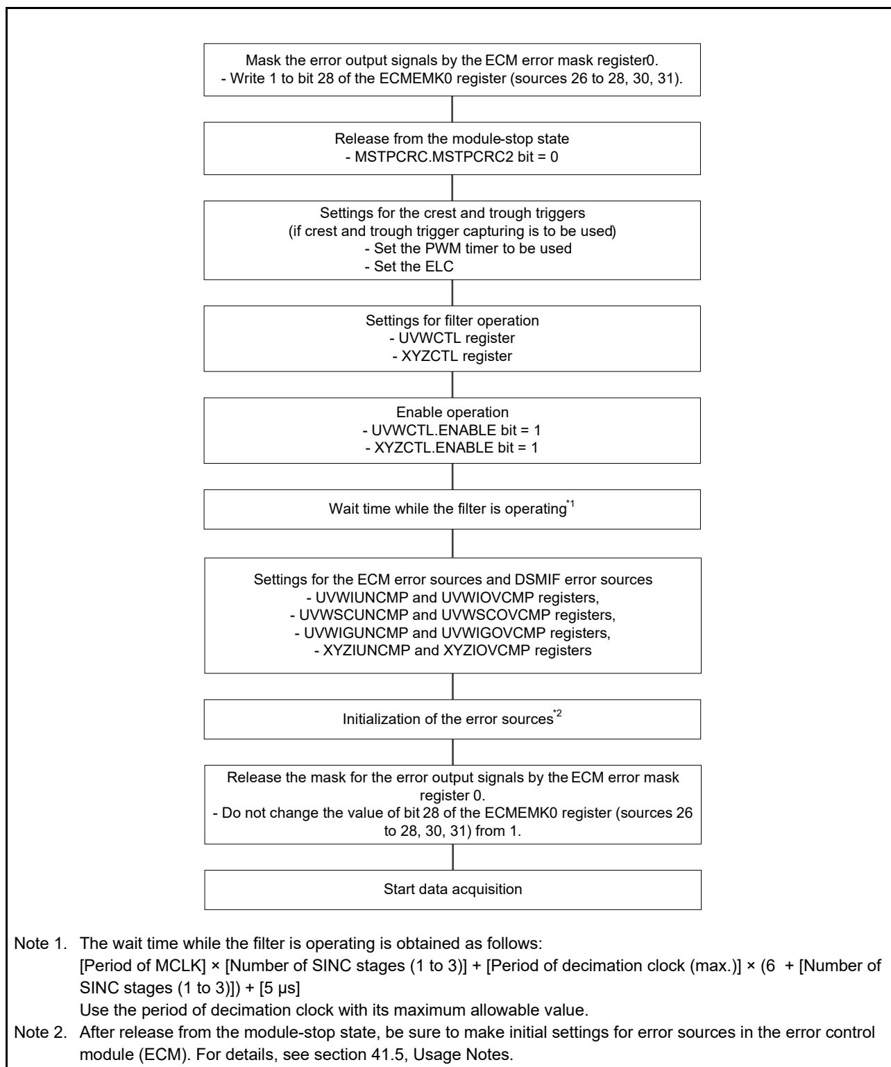
Figure 41.9 Setting Example of the Error Control Module
