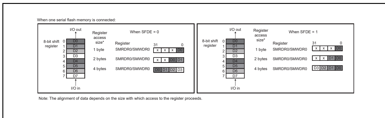
Figure 37.5 Data Alignment in SPI Operating Mode
