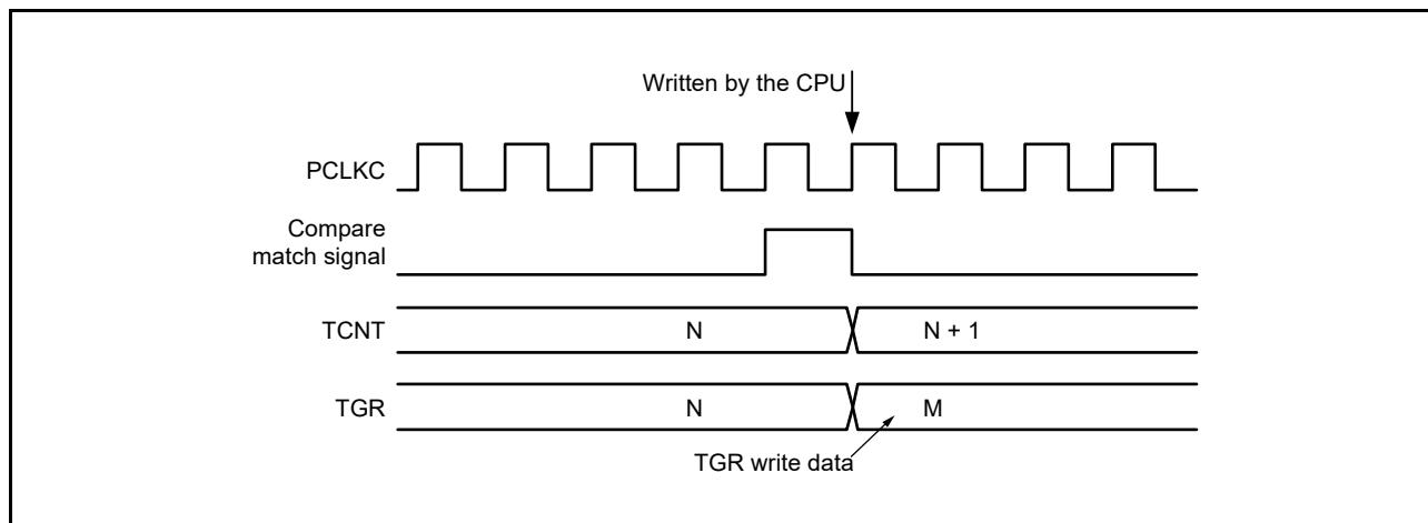
Figure 19.133 Contention between TGR Write Operation and Compare Match
