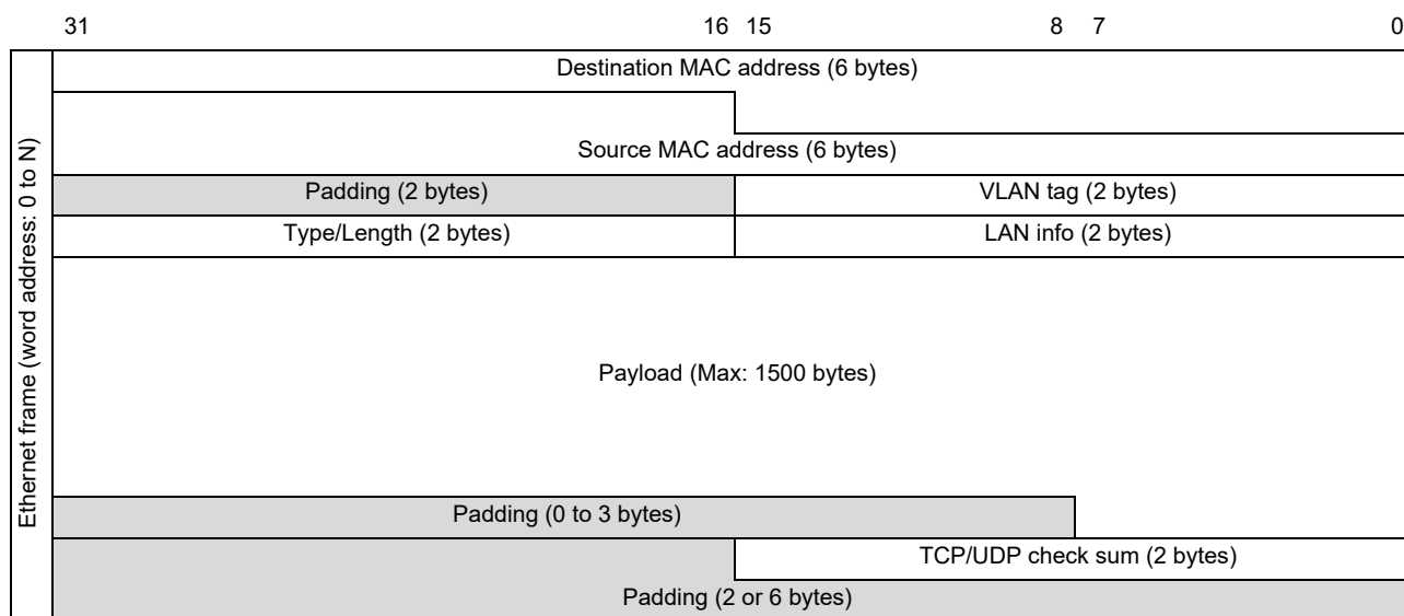
Figure 28.25 Received Ethernet Frame (TCPIPACC Enabled, VLAN Tag Included, TCP/UDP Included)
