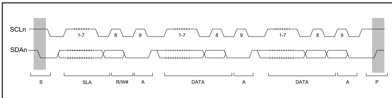
Figure 34.4 I 2 C Bus Timing (SLA = 7 Bits)
