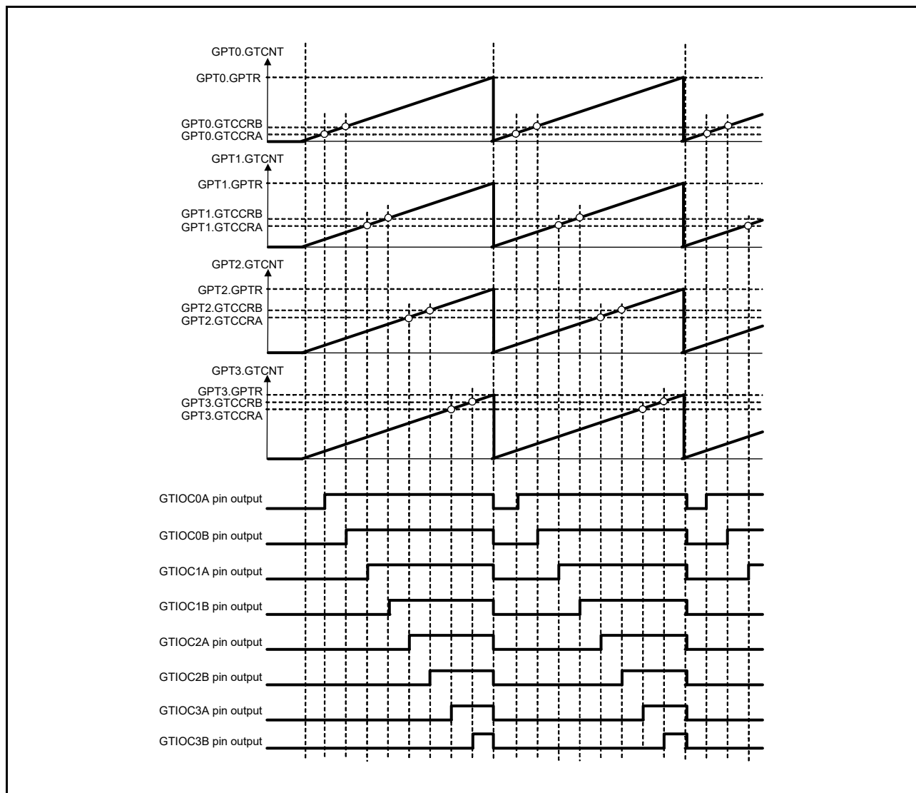
Figure 21.62 Example of Synchronized PWM Output
