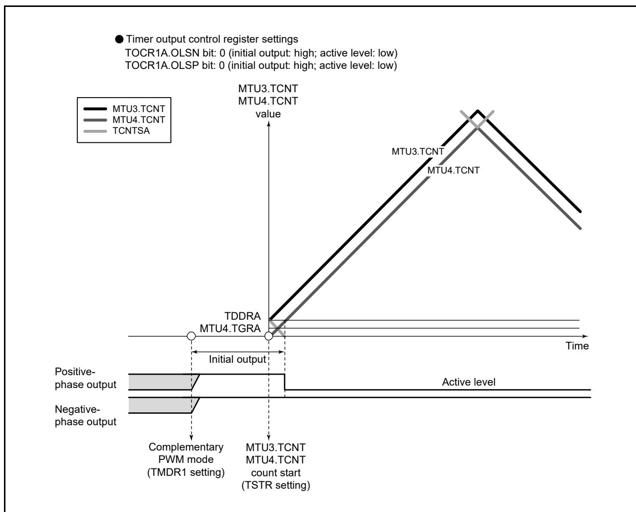
Figure 19.55 Example of Initial Output in Complementary PWM Mode (MTU3 and MTU4) (2)
