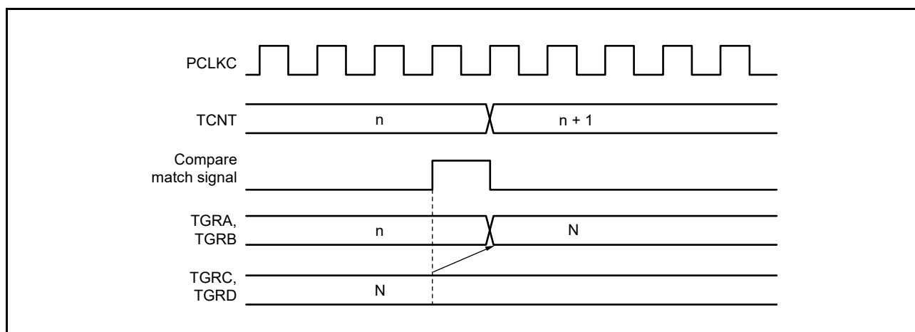
Figure 19.118 Buffer Operation Timing (Compare Match)
