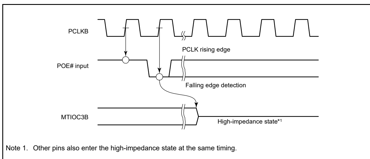
Figure 20.3 Falling Edge Detection
