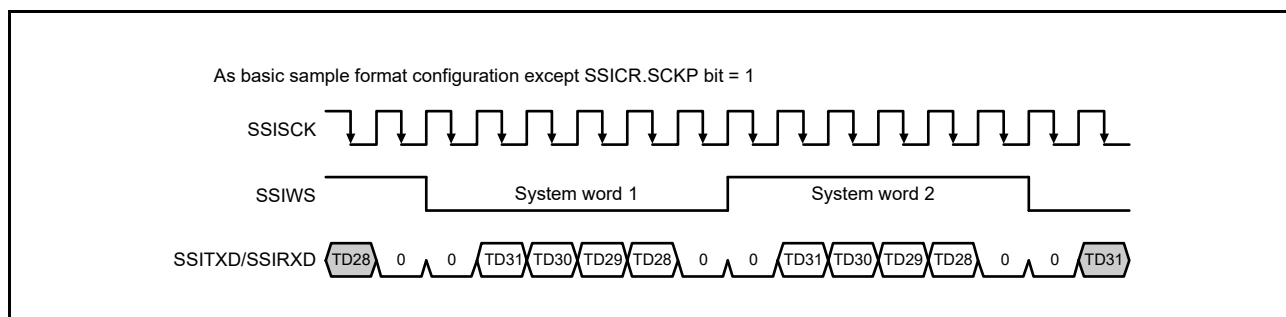
Figure 39.7 Inverted Clock
