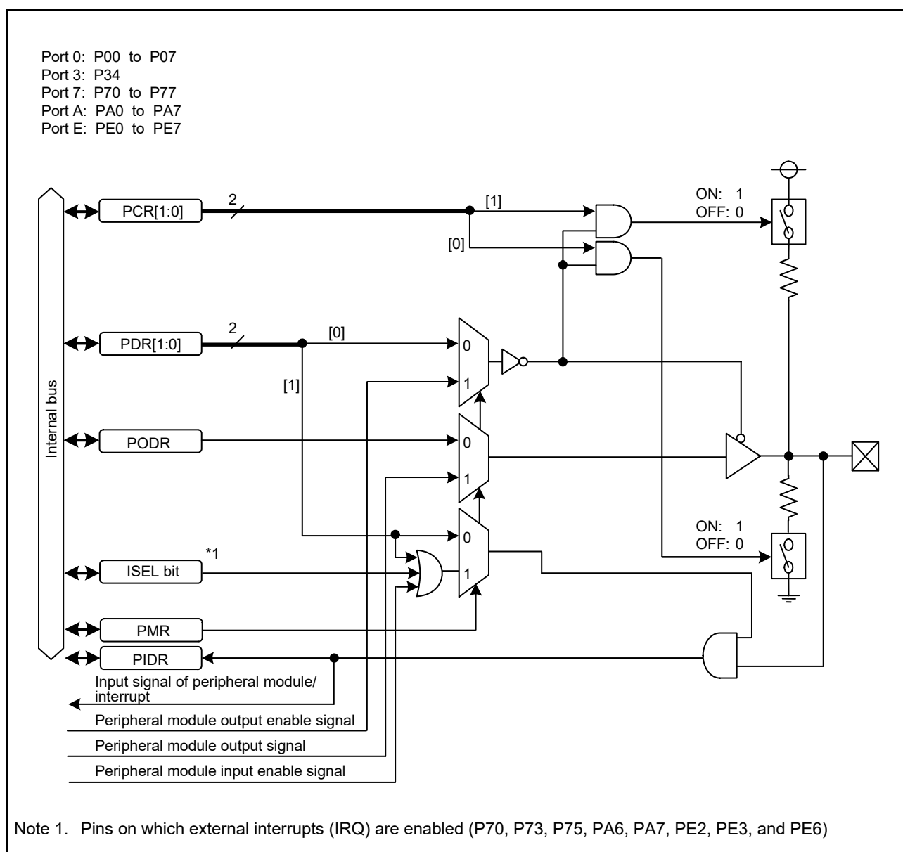
Figure 17.2 I/O Port Configuration (2)
