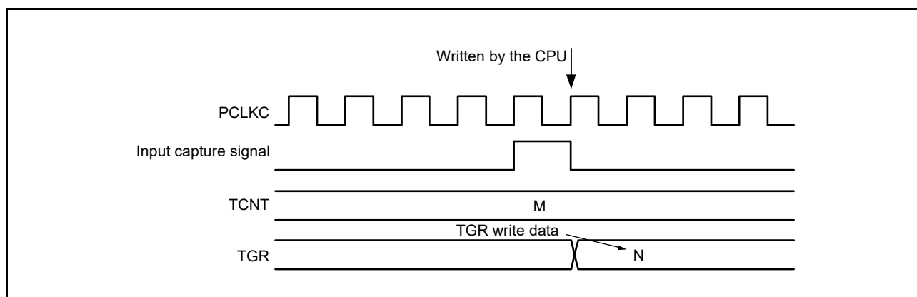
Figure 19.138 Contention between TGR Write Operation and Input Capture (MTU5)
