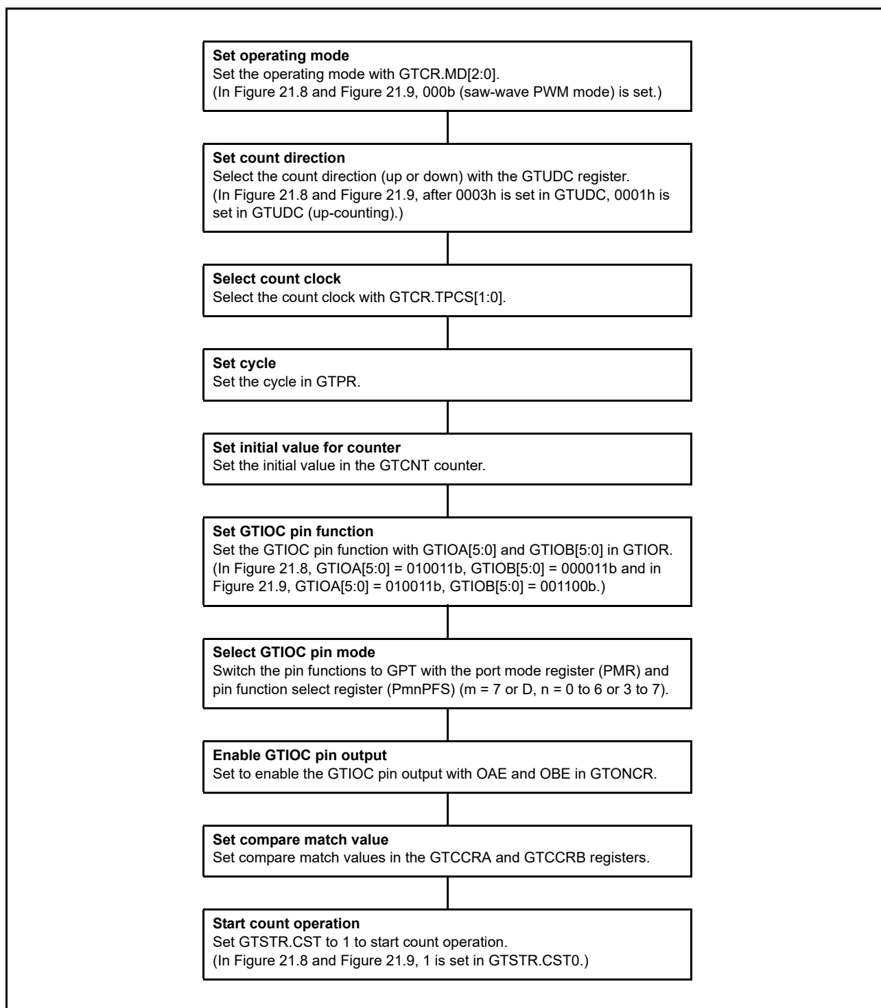
Figure 21.10 Example for Setting Toggled Output Operation
