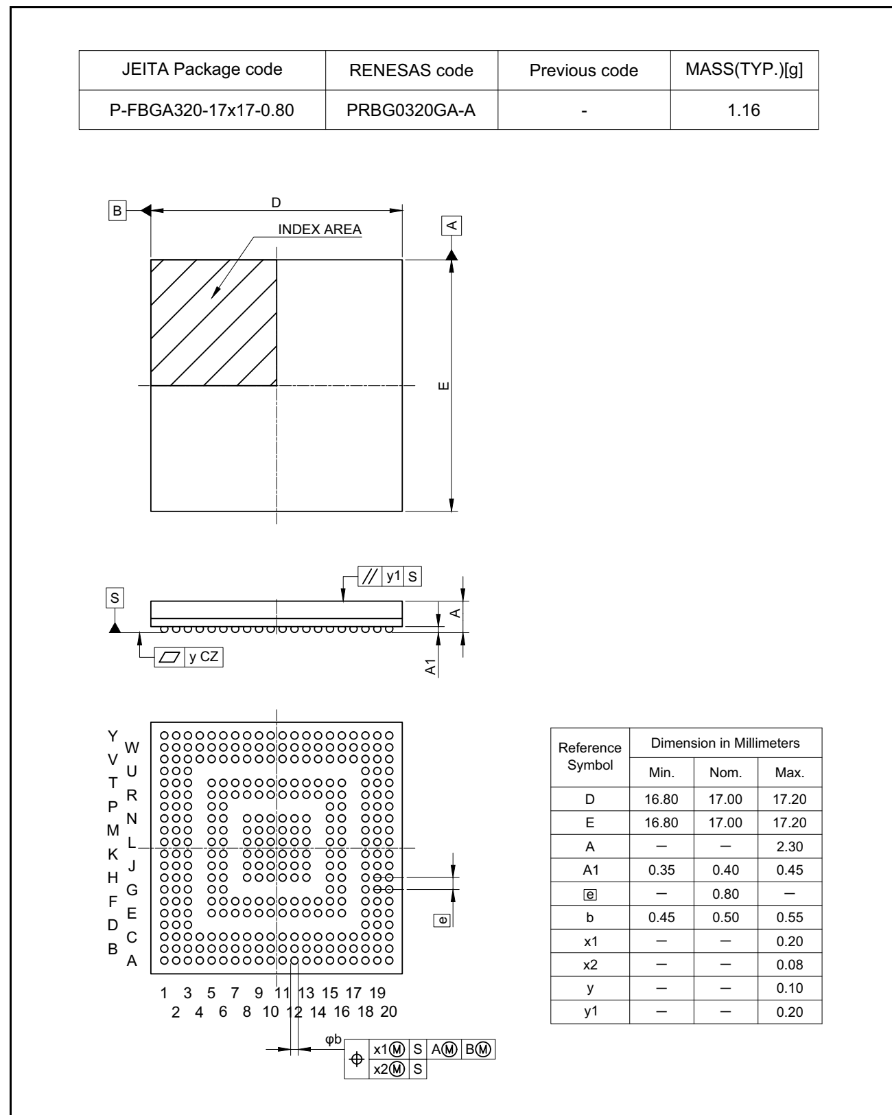
Figure A 320-Pin FBGA (PRBG0320GA-A)
