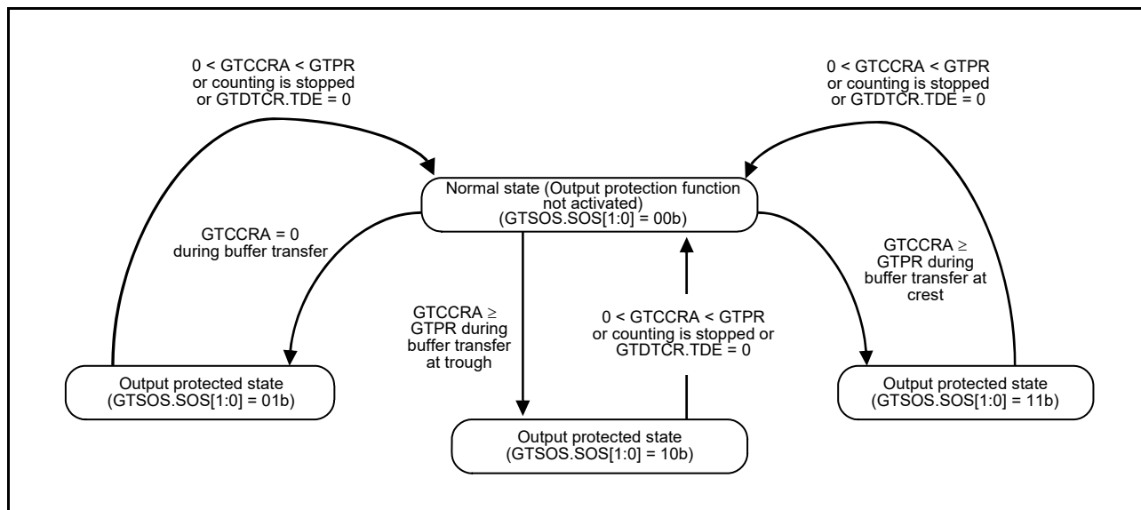
Figure 21.81 Output Protection Function
