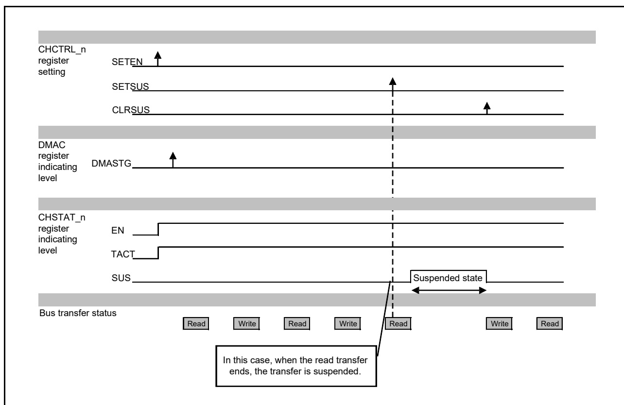
Figure 15.34 DMAC Suspended State (Software Request Block Transfer)
