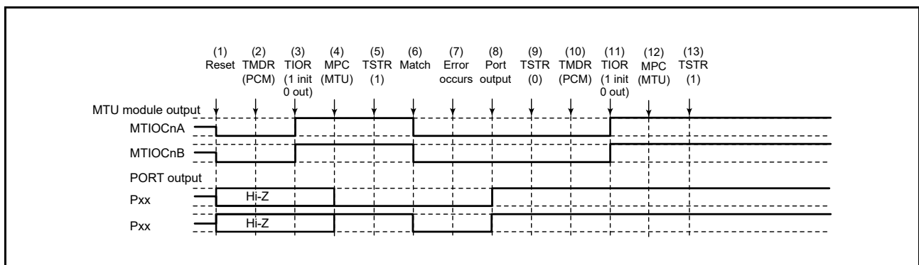
Figure 19.168 Error Occurrence in Phase Counting Mode, Recovery in Phase Counting Mode
