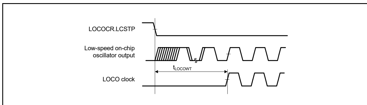
Figure 47.7 LOCO Clock Oscillation Start Timing
