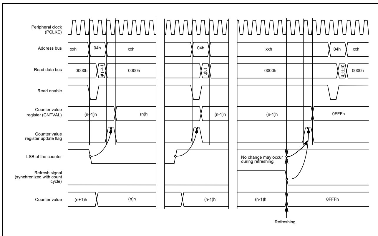
Figure 26.6 Processing for Reading WDT Down-Counter Value (WDTCR.CKS[3:0] = 0100b, WDTCR.TOPS[1:0] = 01b)
