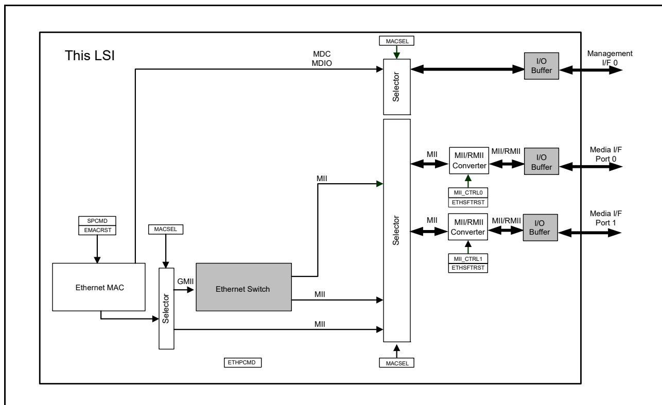
Figure 28.1 Block Diagram of the ETHERC
