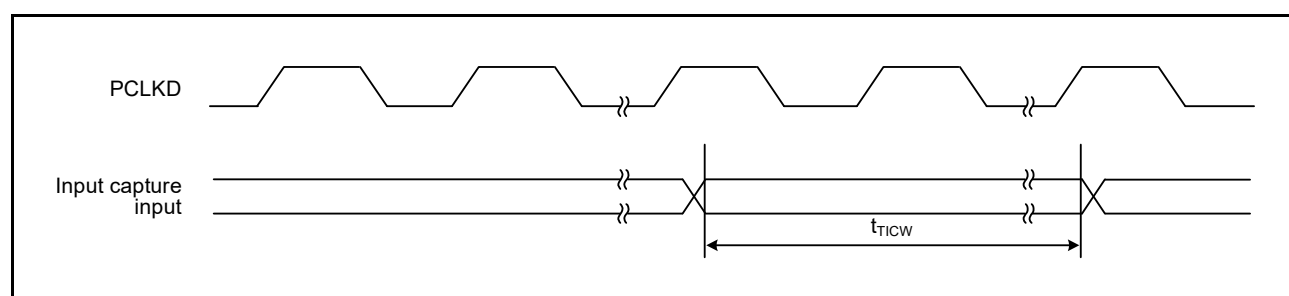
Figure 47.40 TPUa Input Capture Input Timing
