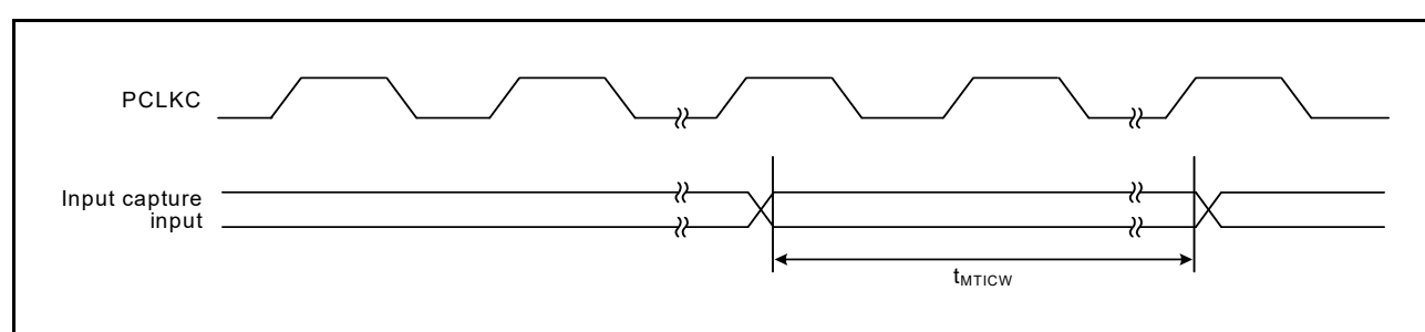
Figure 47.43 MTU3a Input Capture Input Timing
