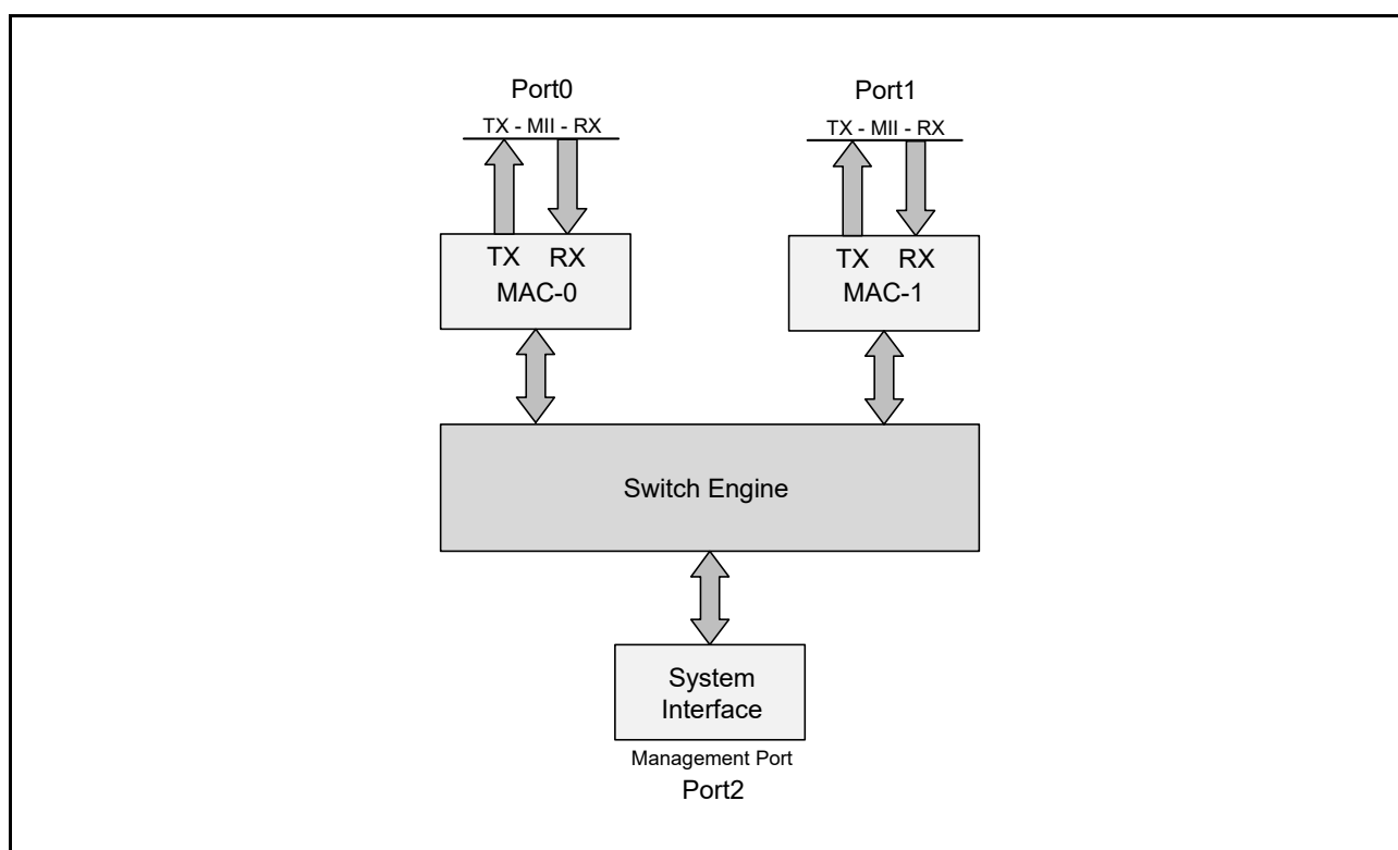
Figure 29.13 Normal Operation of Switch Mode
