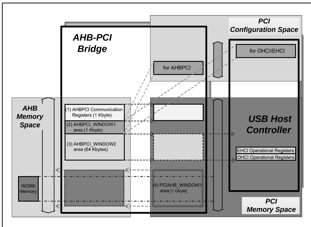
Figure 31.3 Image of AHB and PCI Space Mapping
