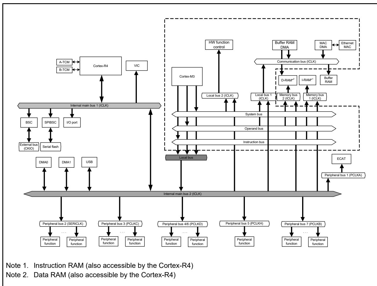
Figure 13.2 Internal Bus Configuration (for products incorporating an R-IN engine)
