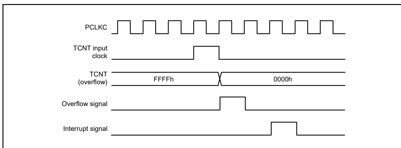
Figure 19.128 TCIV Interrupt Timing
