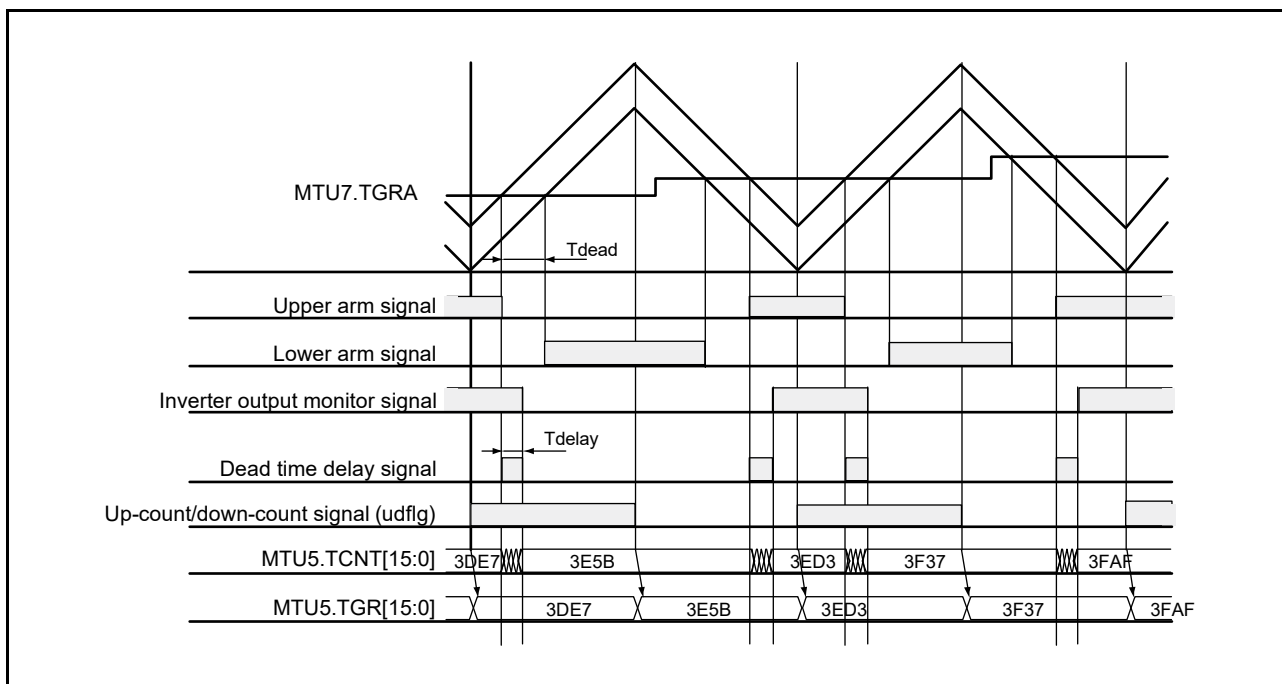
Figure 19.106 TCNT Capture at Crest and/or Trough in Complementary PWM Operation
