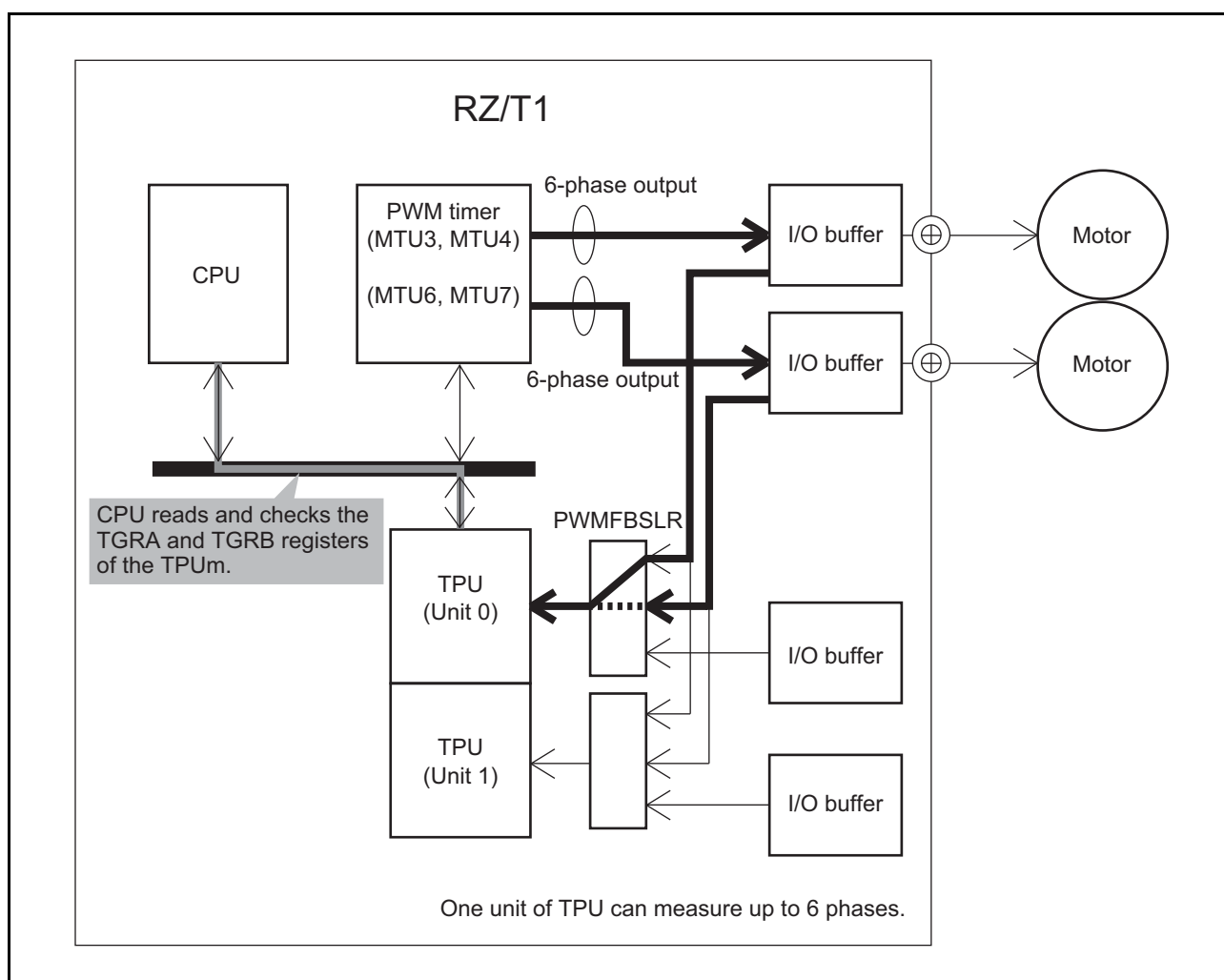
Figure 22.34 Connection Diagram of Example Setting for PWM 2-Axes Measurement
