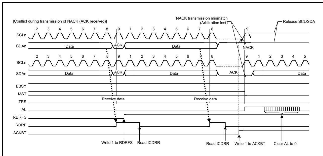
Figure 34.34 Example of Arbitration-Lost Detection during Transmission of NACK (NALE = 1)
