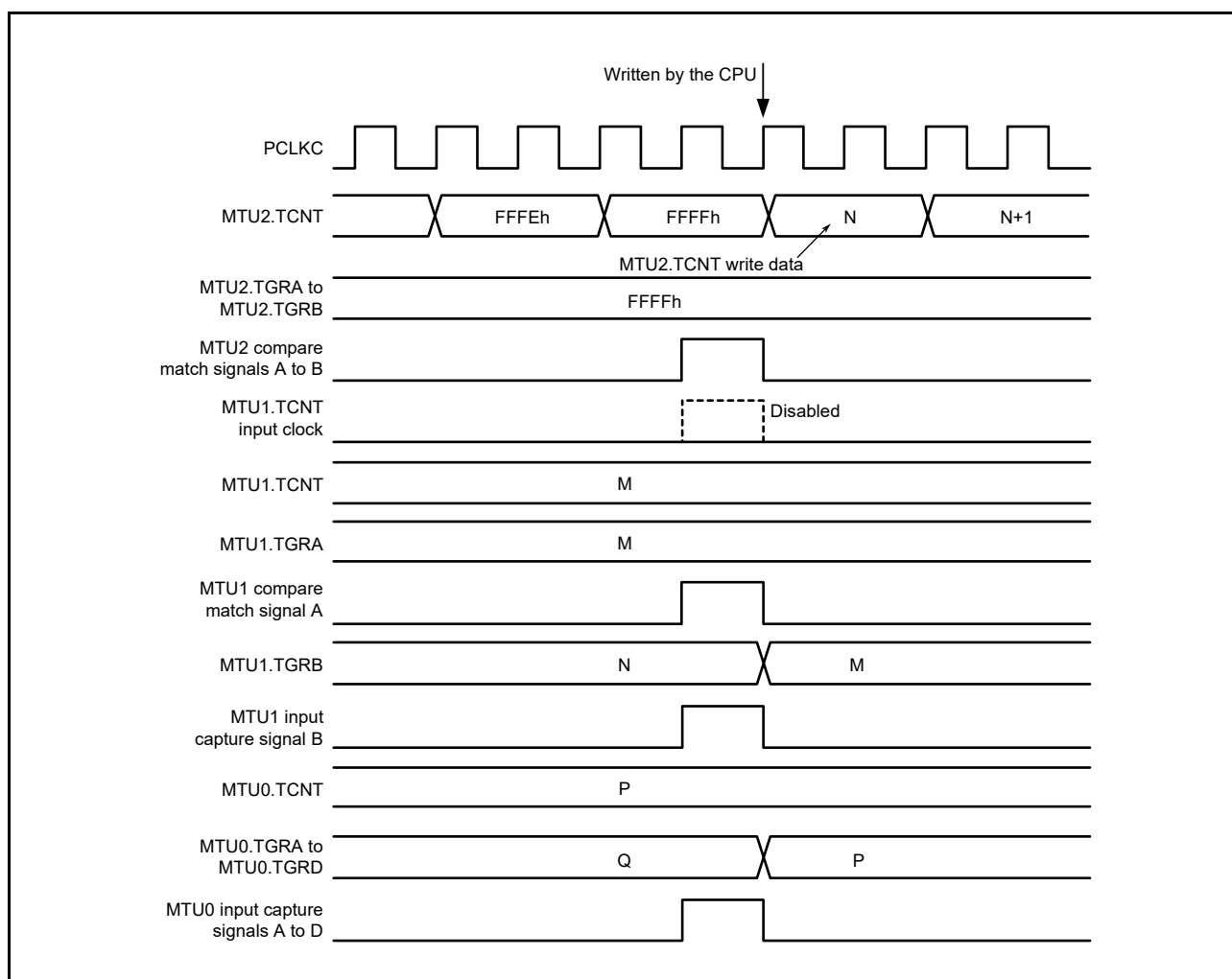
Figure 19.140 Contention between MTU2.TCNT Write Operation and Overflow/Underflow in Cascaded Operation
