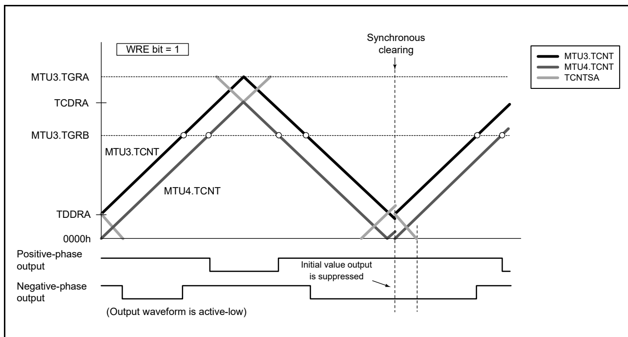
Figure 19.71 Example of Synchronous Clearing in Interval Tb at Trough (Timing (11) in Figure 19.66; Bit WRE of TWCRA is 1)
