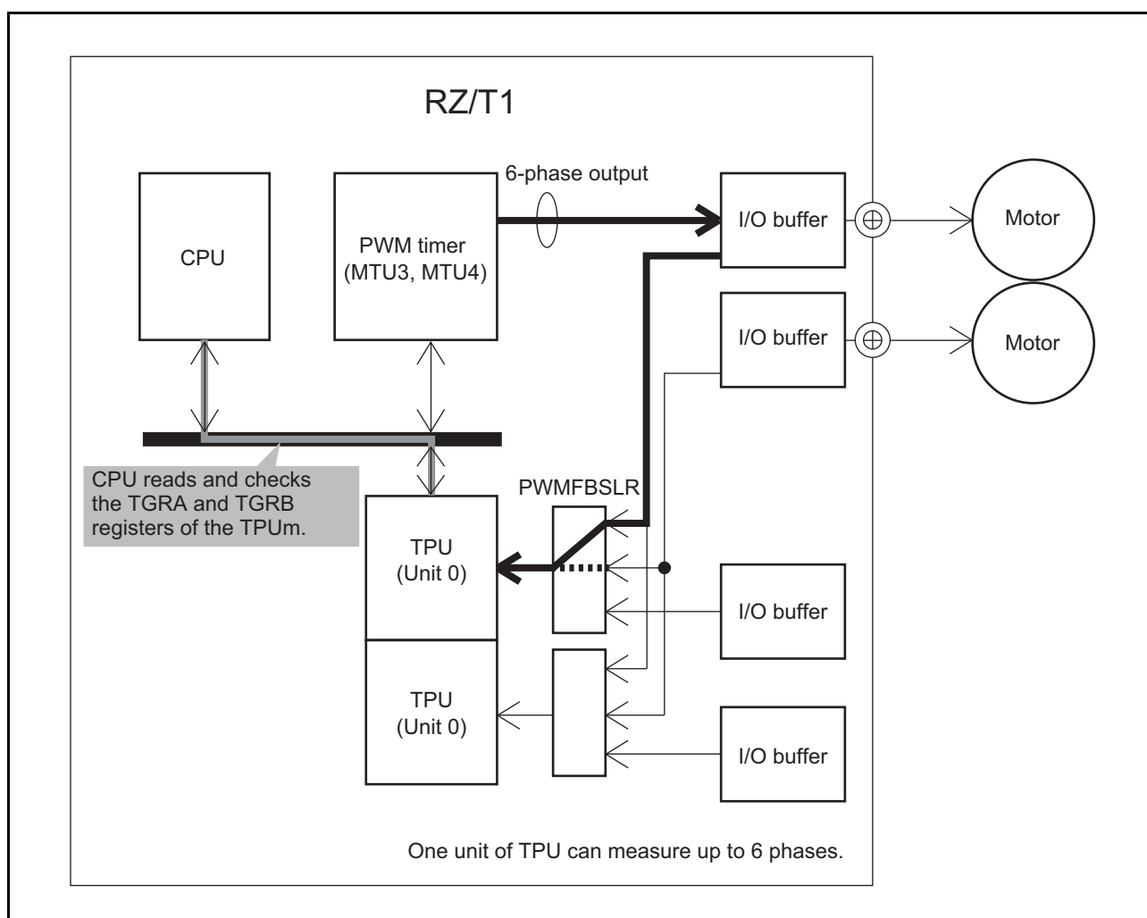
Figure 22.33 Connection Diagram of Example Setting for PWM 1-Axis Measurement
