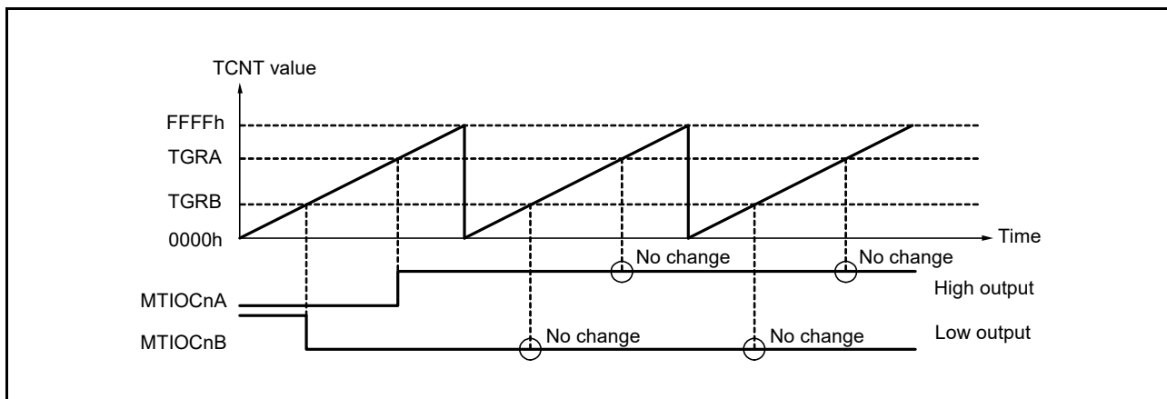
Figure 19.9 Example of low output and high output Operation
