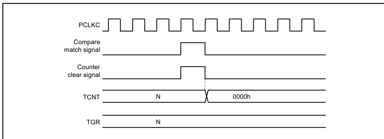
Figure 19.115 Counter Clear Timing (Compare Match) (MTU0 to MTU4 and MTU6 to MTU8)
