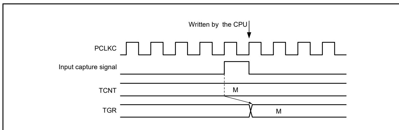
Figure 19.137 Contention between TGR Write Operation and Input Capture (MTU0 to MTU4 and MTU6 to MTU8)
