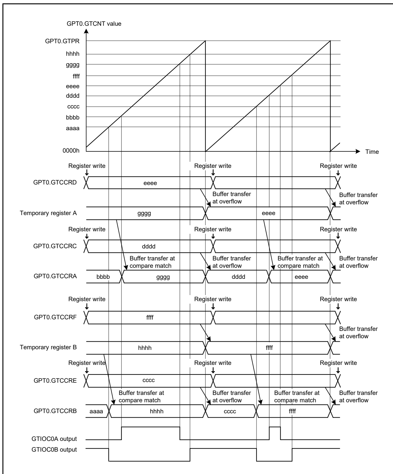
Figure 21.29 Example of Saw-Wave One-Shot Pulse Mode Operation (Up-Count Operation, Low Output from GTIOC0A and High Output from GTIOC0B at Count Start, Toggle Output at GTCCRA/GTCCRB Compare Match, Output Retained at Cycle End)
