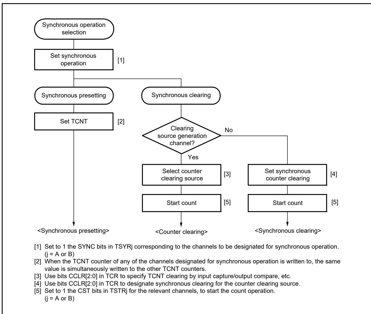
Figure 19.13 Example of Synchronous Operation Setting Procedure
