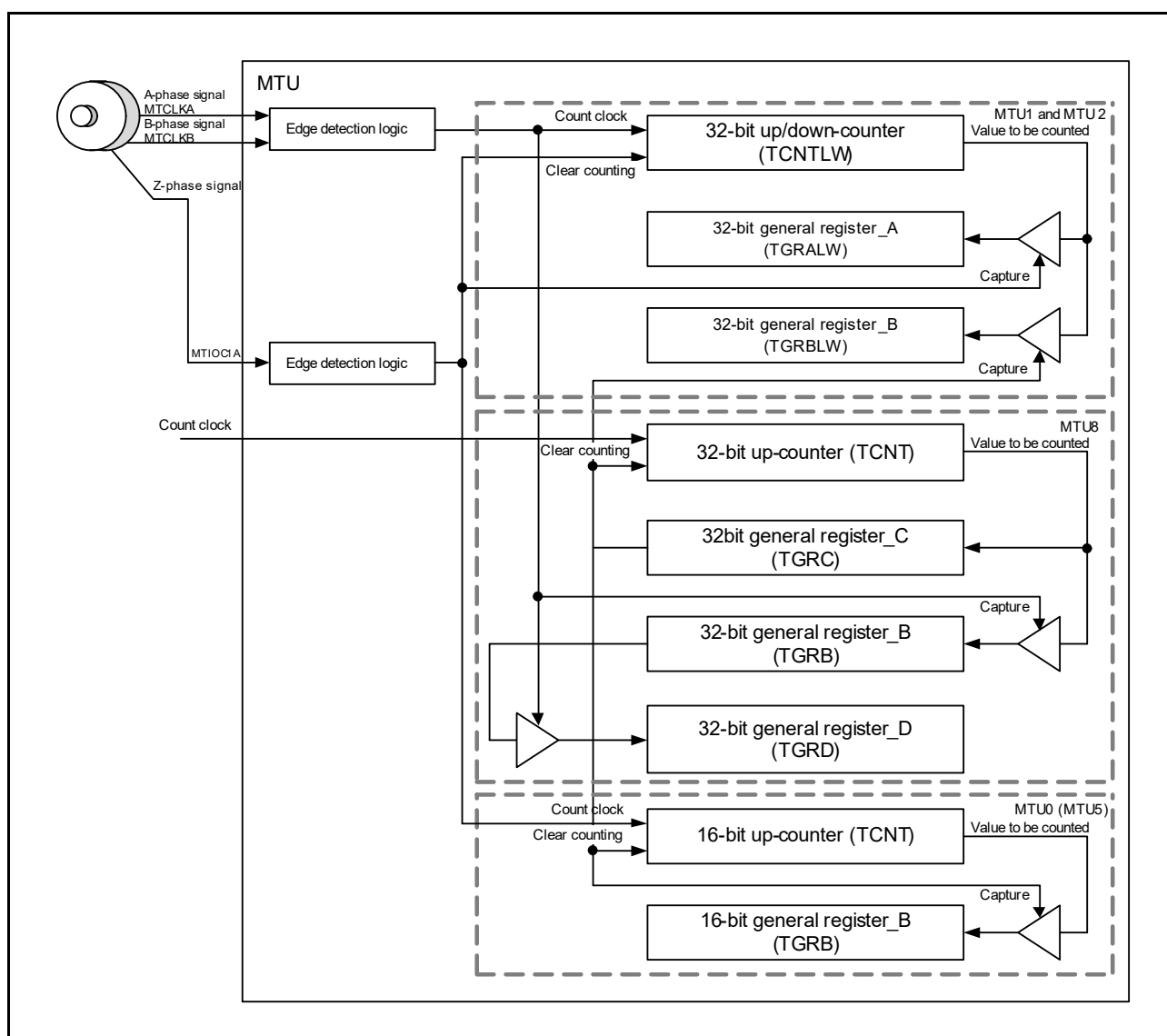
Figure 19.42 32-bit Phase Counting Mode Application Example
