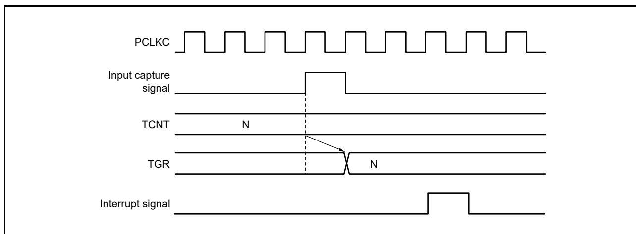
Figure 19.126 TGI Interrupt Timing (Input Capture) (MTU0 to MTU4 and MTU6 to MTU8)
