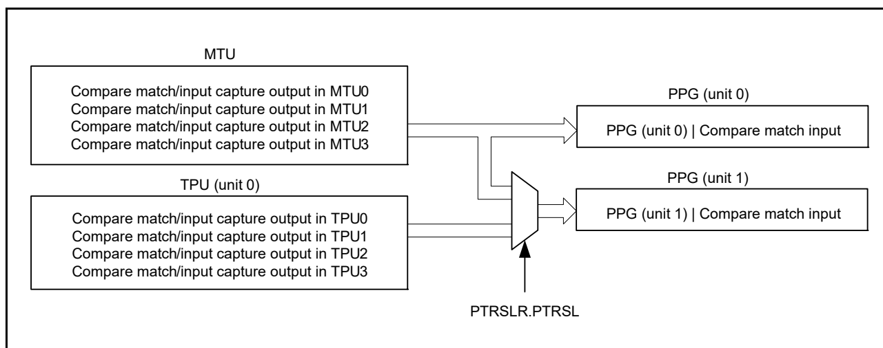
Figure 23.2 Block Diagram of PPG Trigger Selection
