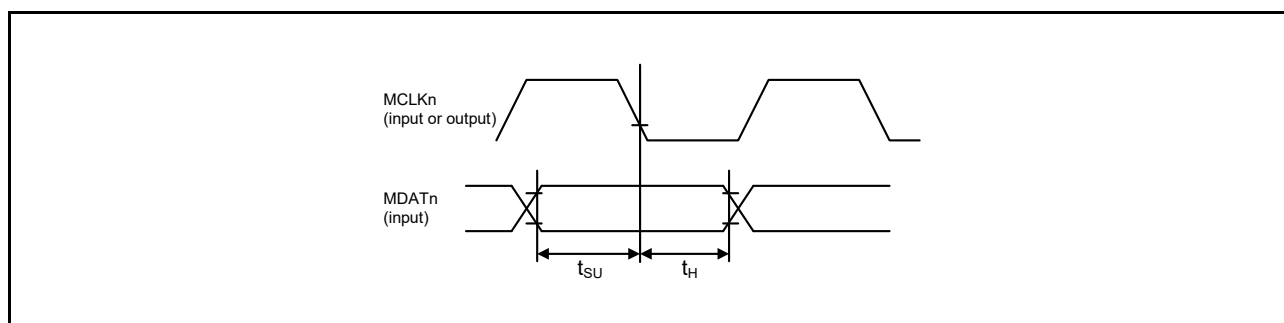
Figure 47.81 Reception Timing (MCLKn Falling Synchronous)
