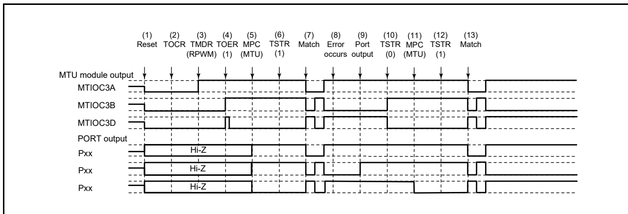
Figure 19.177 Error Occurrence in Reset-Synchronized PWM Mode, Recovery in Reset-Synchronized PWM Mode
