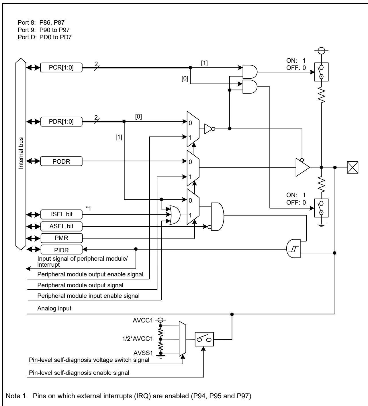
Figure 17.3 I/O Port Configuration (3)
