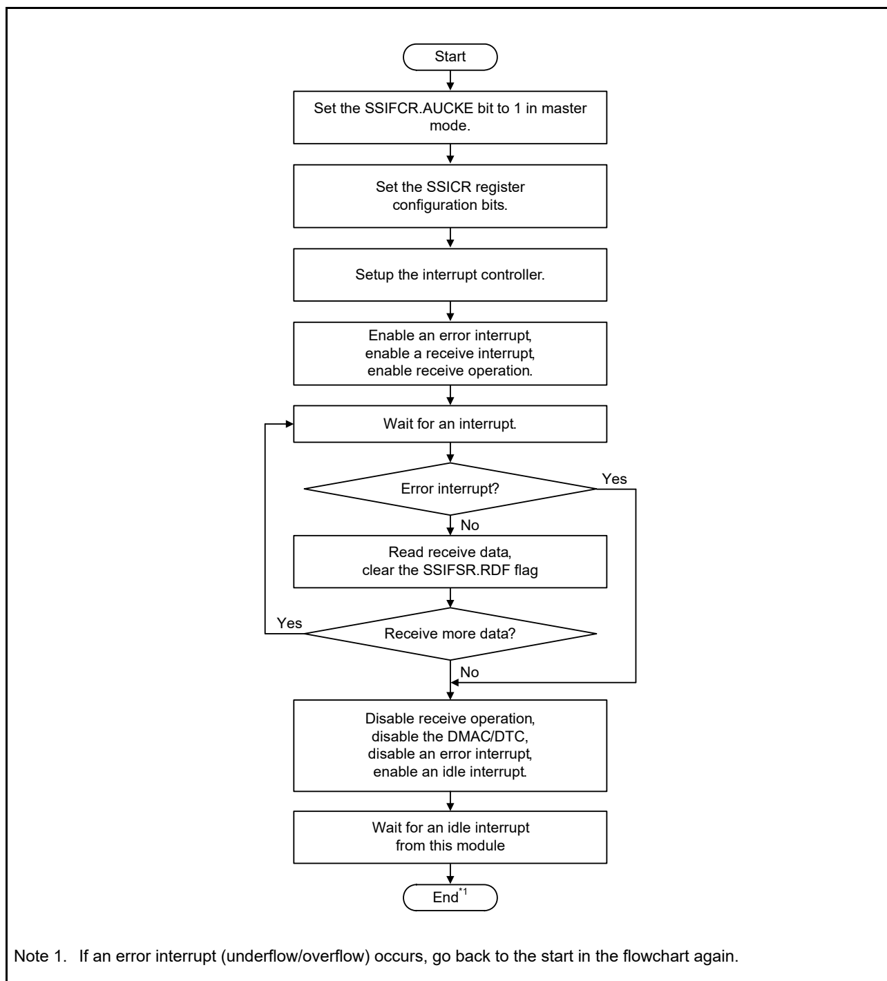
Figure 39.19 Reception Using Interrupts
