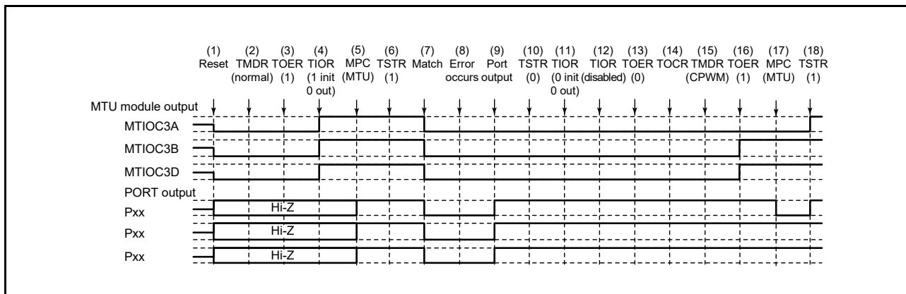
Figure 19.153 Error Occurrence in Normal Mode, Recovery in Complementary PWM Mode
