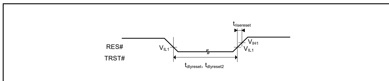
Figure 47.8 Reset Input Timing
