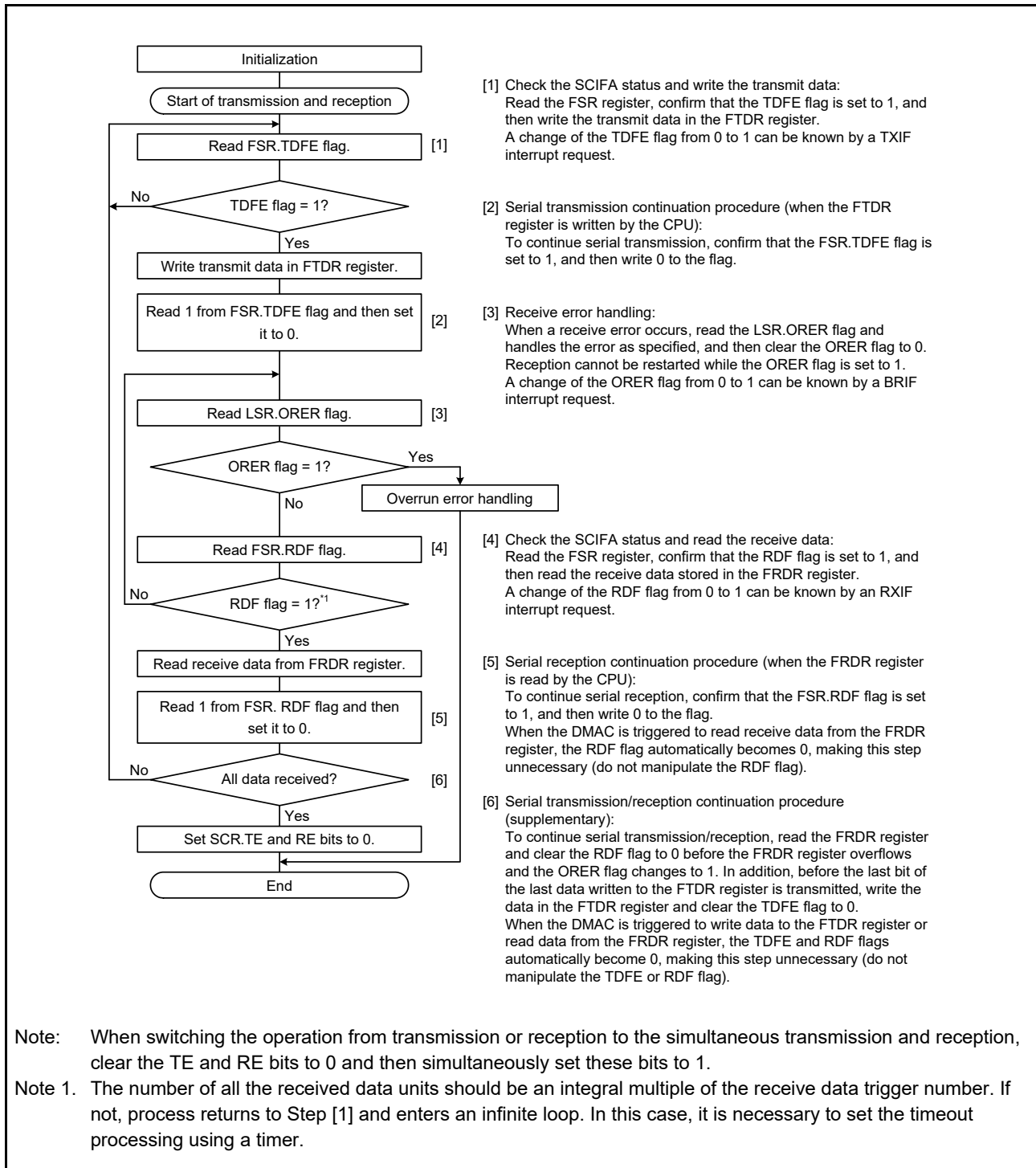
Figure 33.17 Sample Flowchart for Simultaneous Transmitting/Receiving Serial Data in Clock Synchronous Mode
