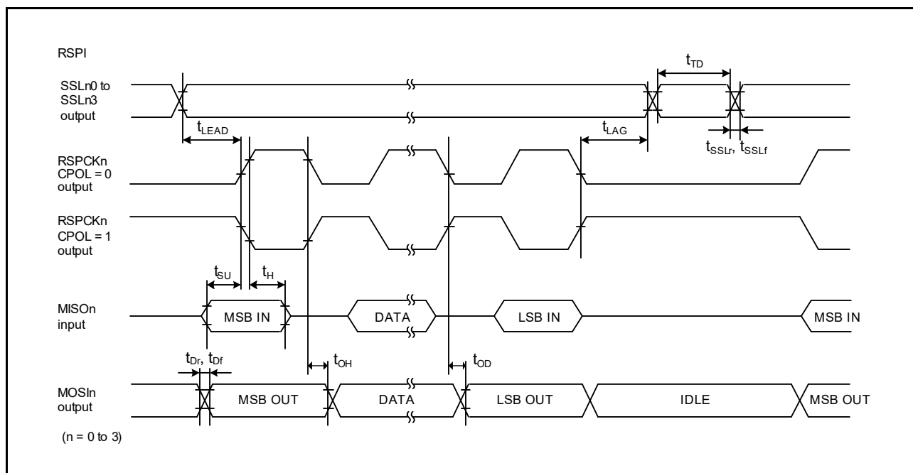
Figure 47.53 RSPIa Timing (Master, CPHA = 0)
