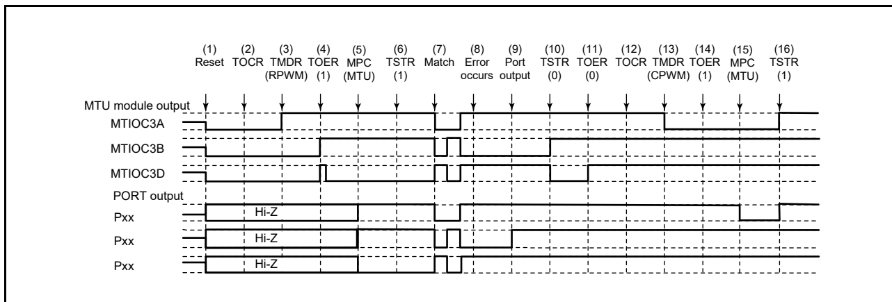
Figure 19.176 Error Occurrence in Reset-Synchronized PWM Mode, Recovery in Complementary PWM Mode
