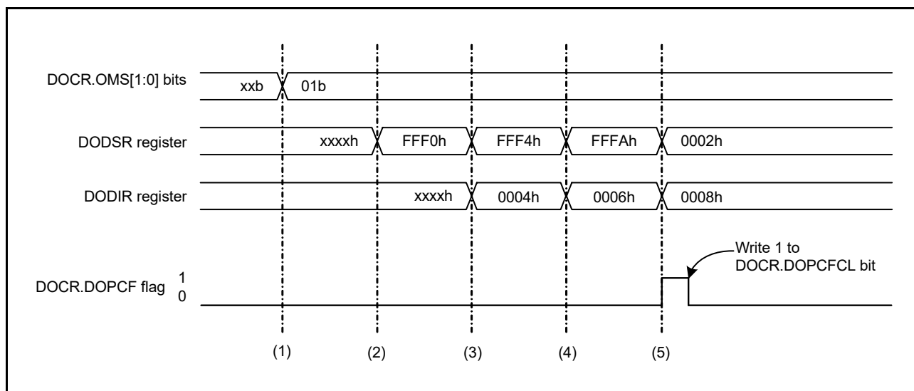
Figure 45.3 Example of Operation in Data Addition Mode
