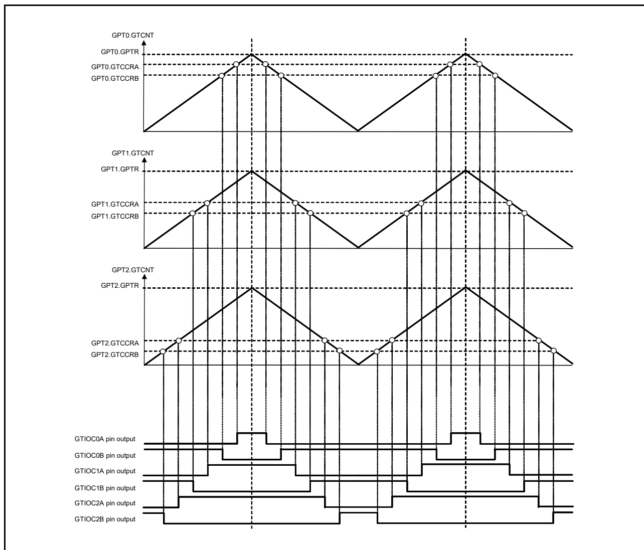
Figure 21.65 Example of Three-Phase Triangle-Wave Complementary PWM Output
