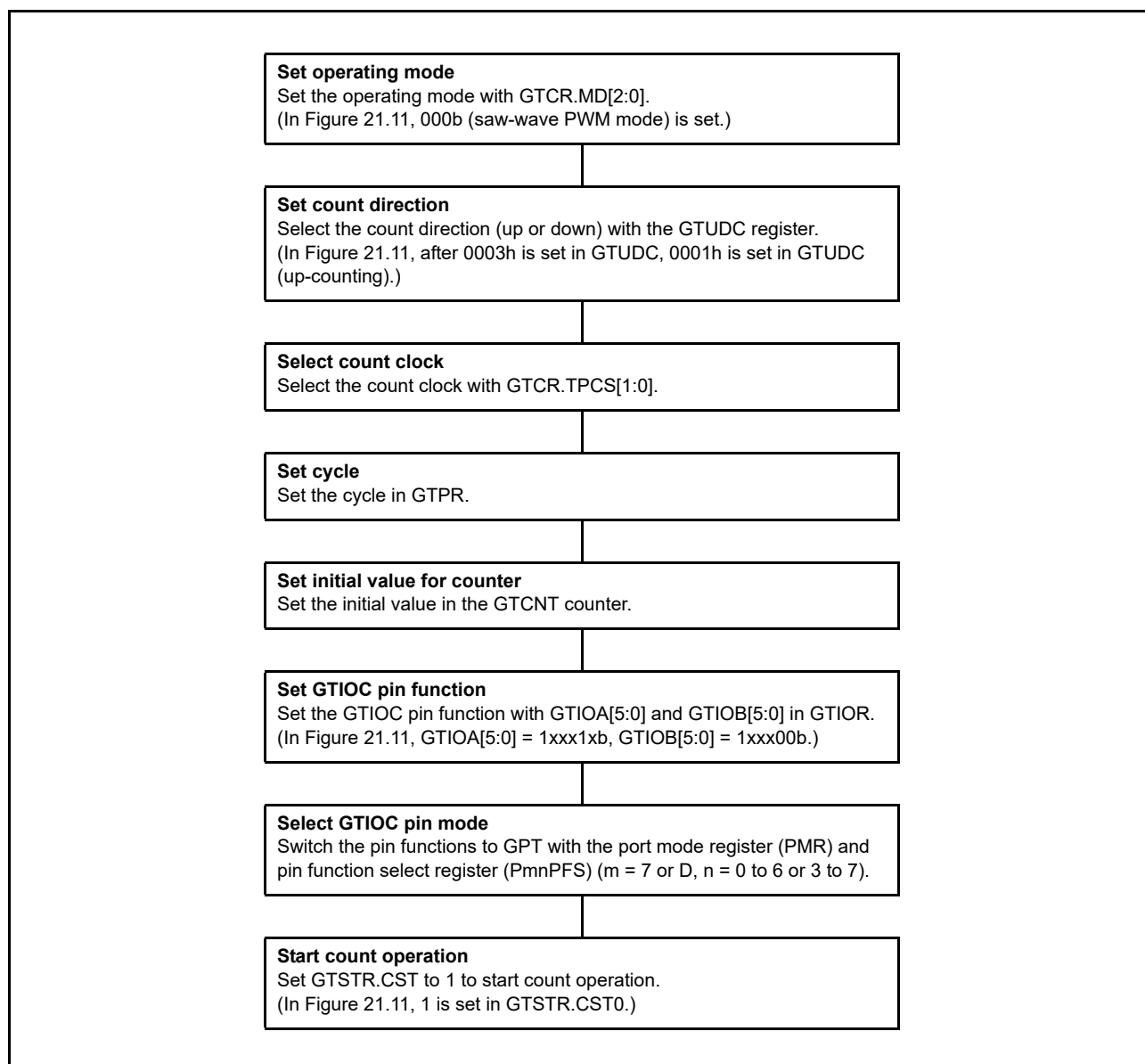
Figure 21.12 Example for Setting Input Capture Operation
