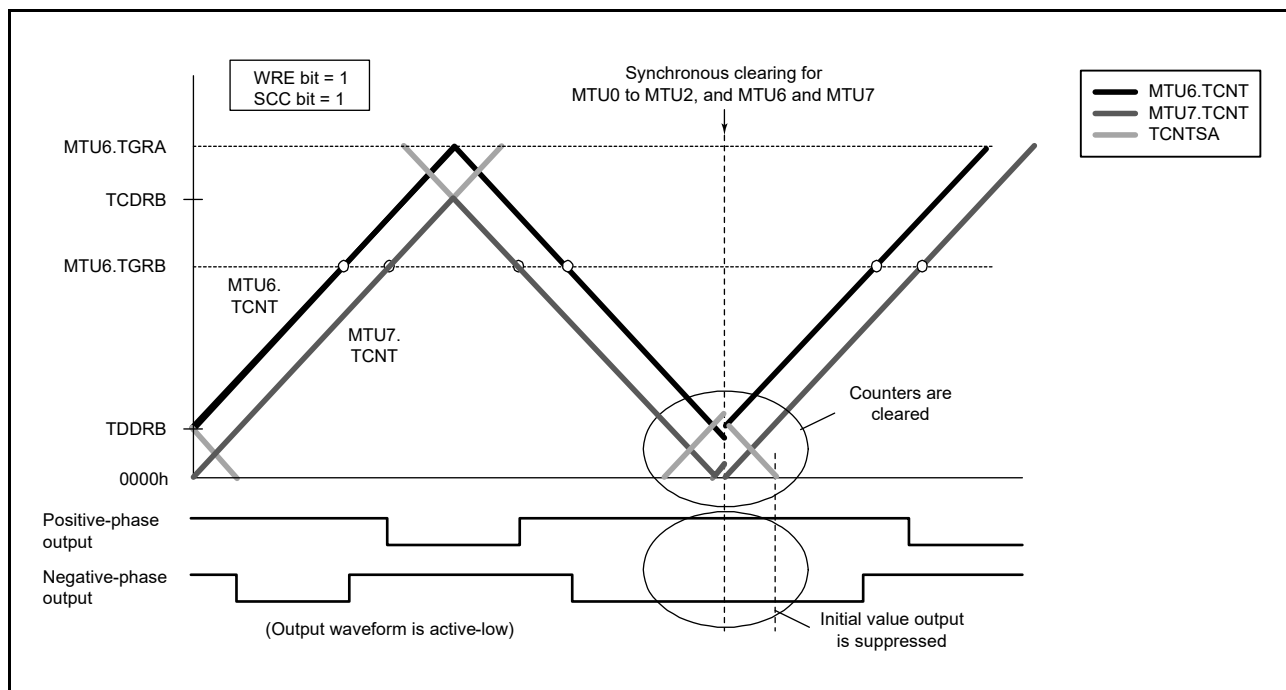
Figure 19.77 Example of Synchronous Clearing in Interval Tb at Trough (Timing (11) in Figure 19.66; Bit WRE is 1 and Bit SCC is 1 in TWCRB in MTU6 and MTU7)
