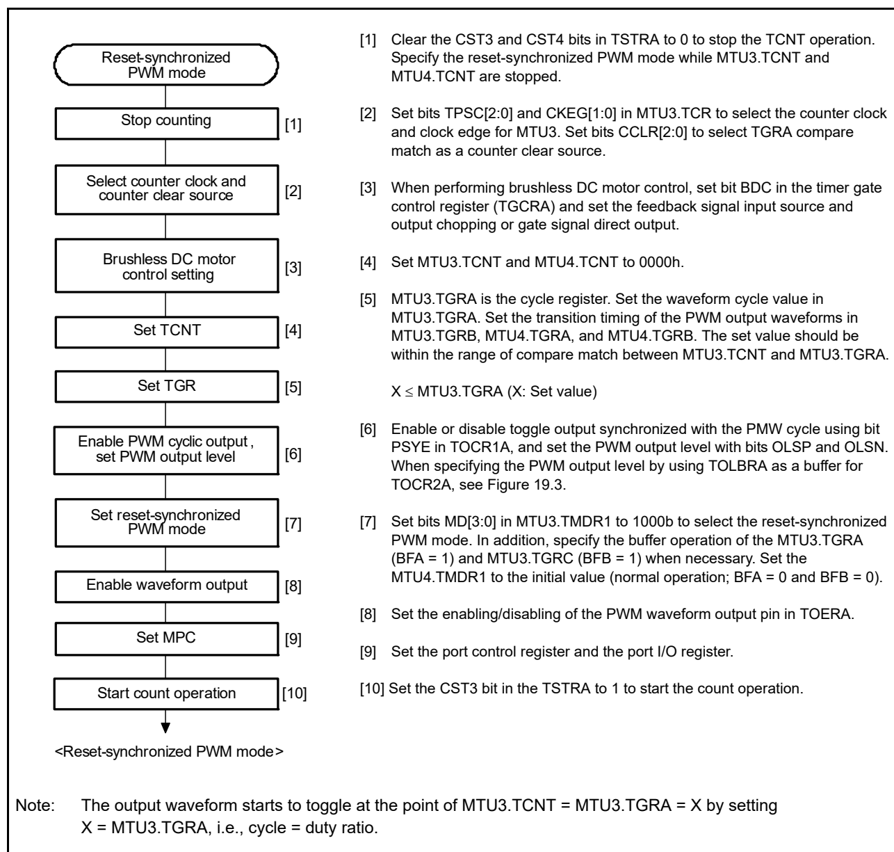
Figure 19.44 Procedure for Selecting Reset-Synchronized PWM Mode
