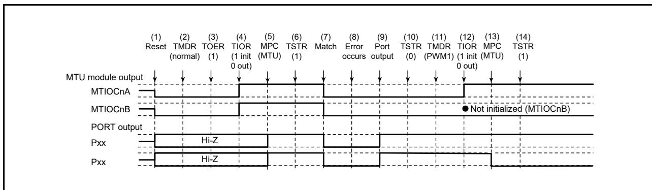
Figure 19.150 Error Occurrence in Normal Mode, Recovery in PWM Mode 1
