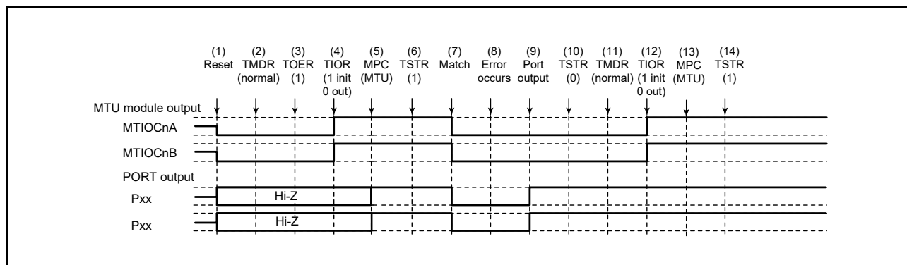
Figure 19.149 Error Occurrence in Normal Mode, Recovery in Normal Mode
