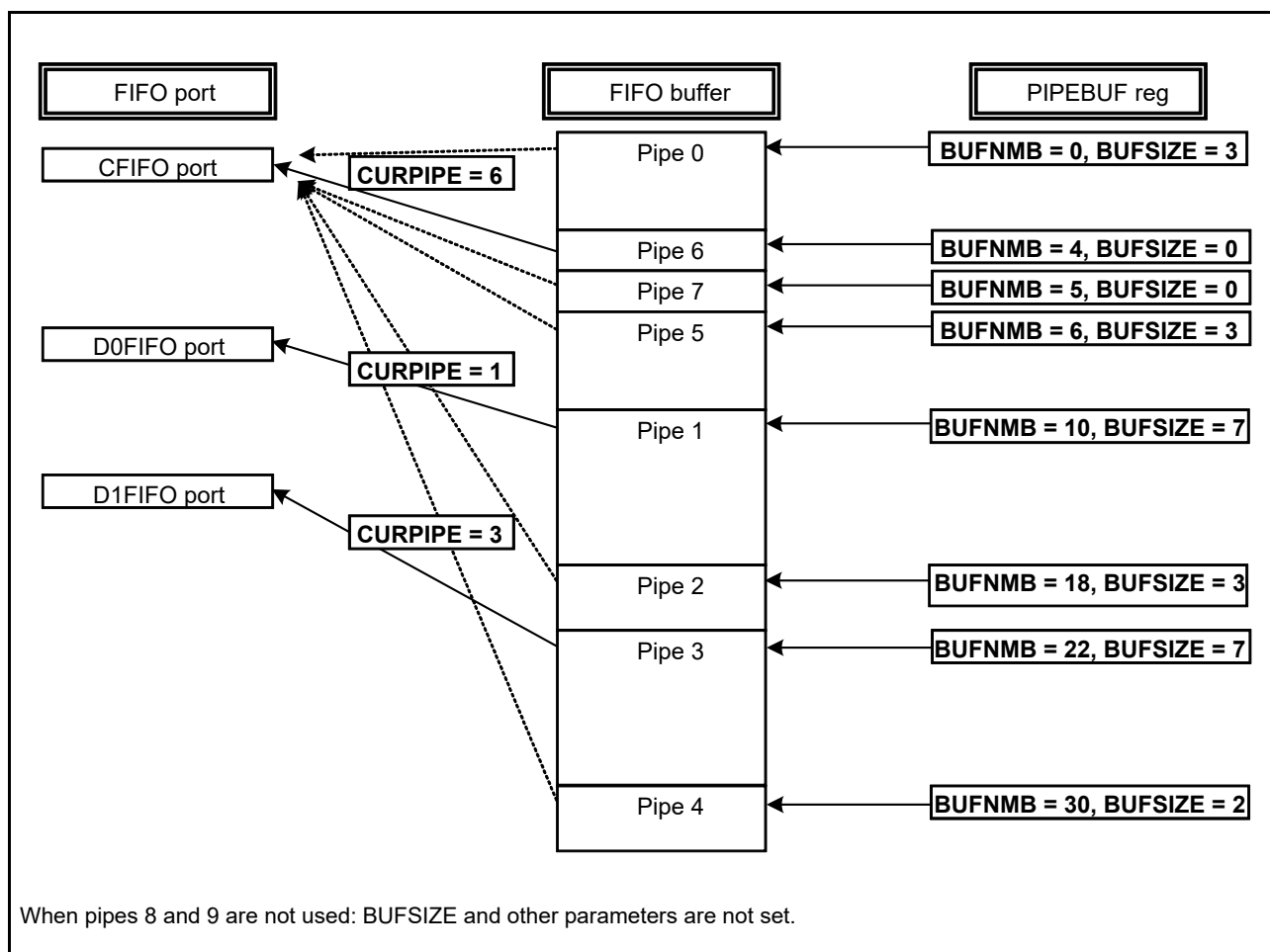
Figure 32.10 Example of FIFO Buffer Memory Map
