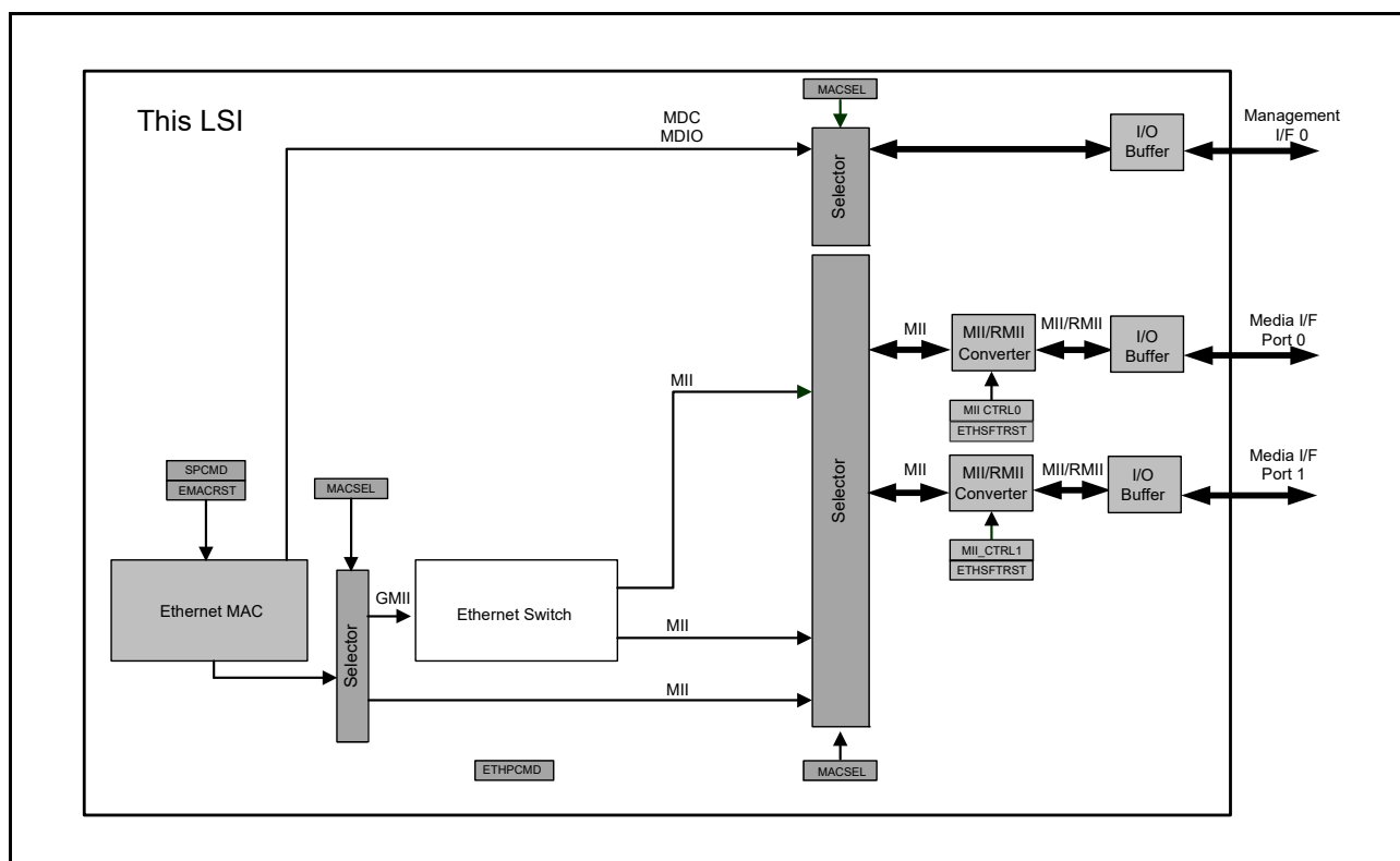
Figure 29.1 Block Diagram of the Ethernet Interface
