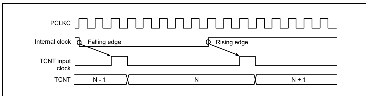
Figure 19.108 Count Timing in Internal Clock Operation (MTU0 to MTU4 and MTU6 to MTU8)
