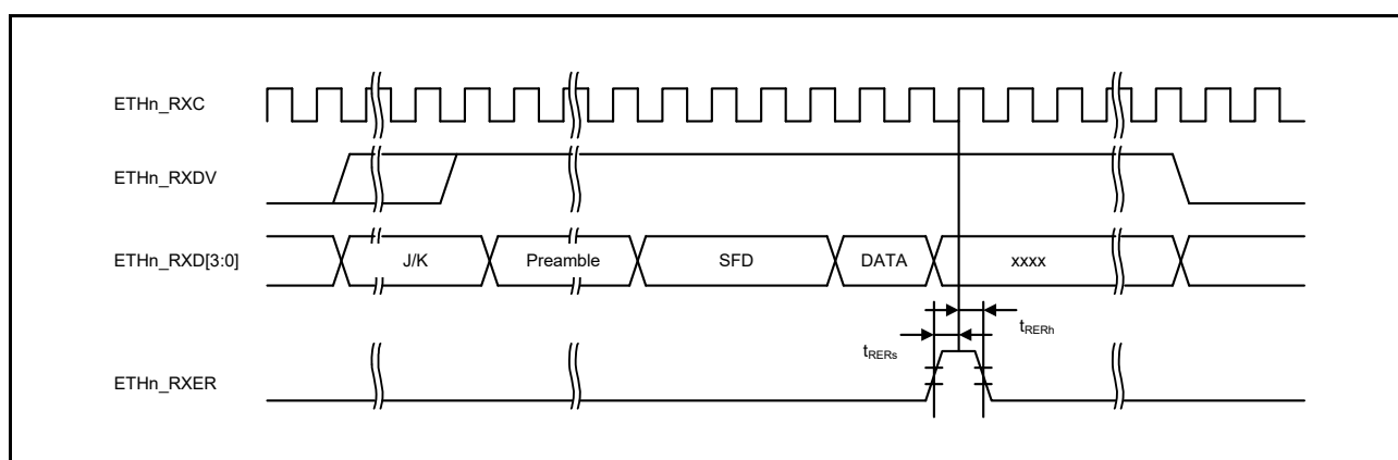
Figure 47.77 MII Reception Timing (Error Occurrence)
