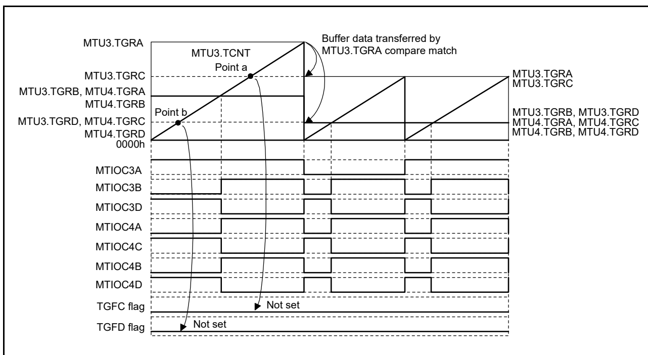
Figure 19.142 Buffer Operation and Compare Match in Reset-Synchronized PWM Mode
