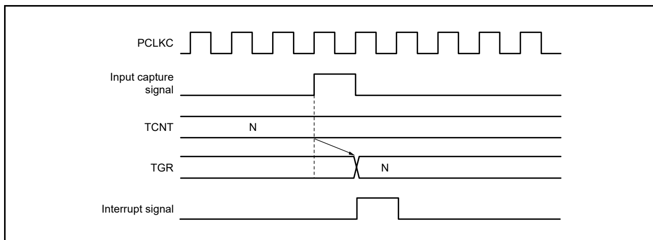
Figure 19.127 TGI Interrupt Timing (Input Capture) (MTU5)
