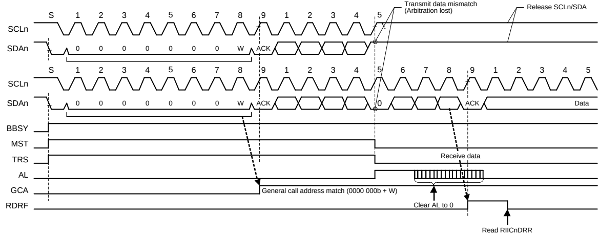
Figure 26.33 Examples of Master Arbitration-Lost Detection (MALE = 1)
