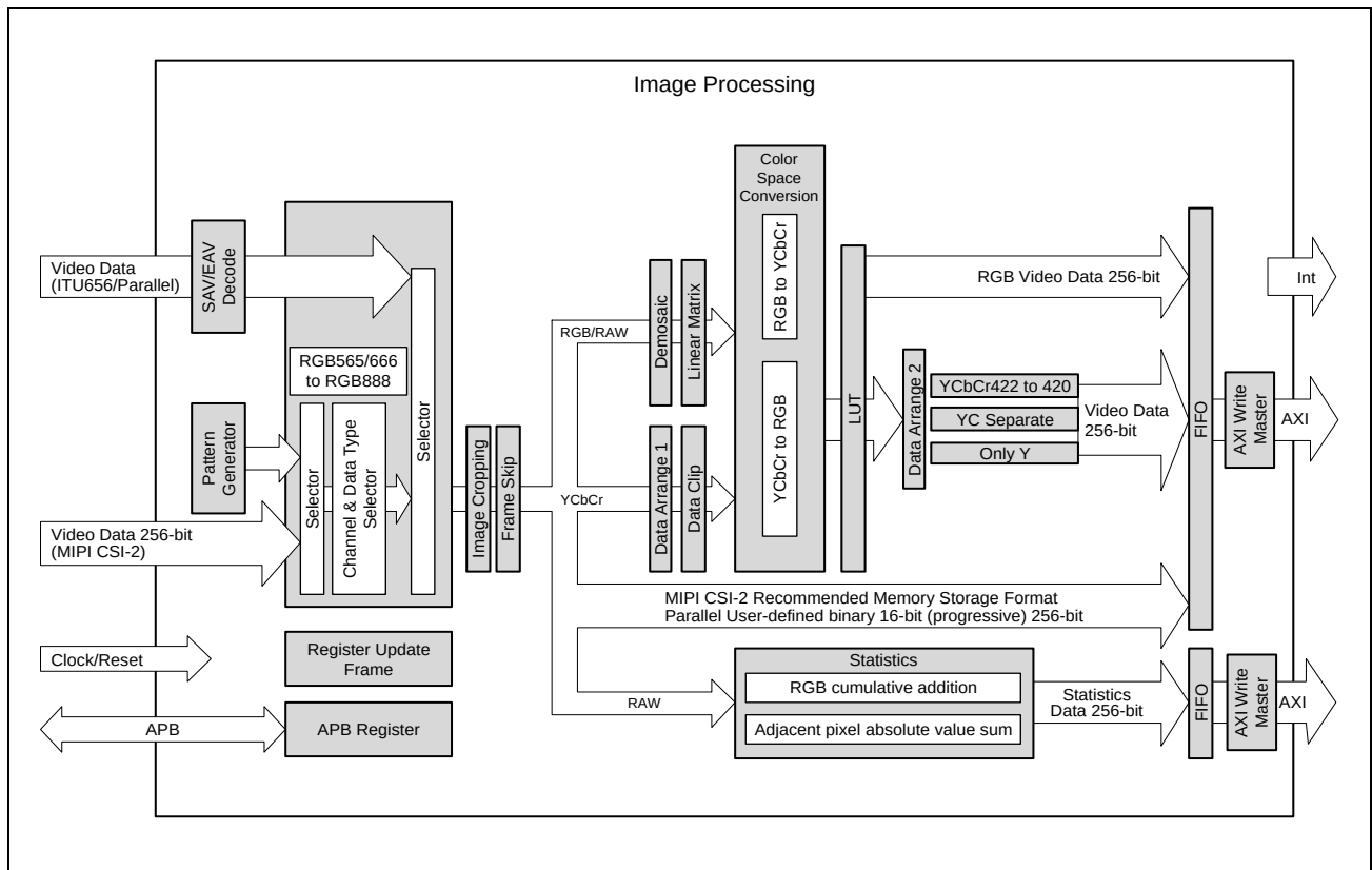
Figure 35.8 Block Diagram of the Image Processing Module
