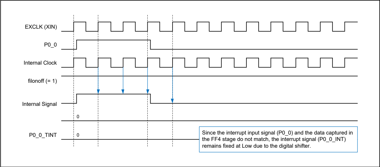
Figure 41.15 Digital noise filter (FILONOFF = 1) Timing chart (1)
