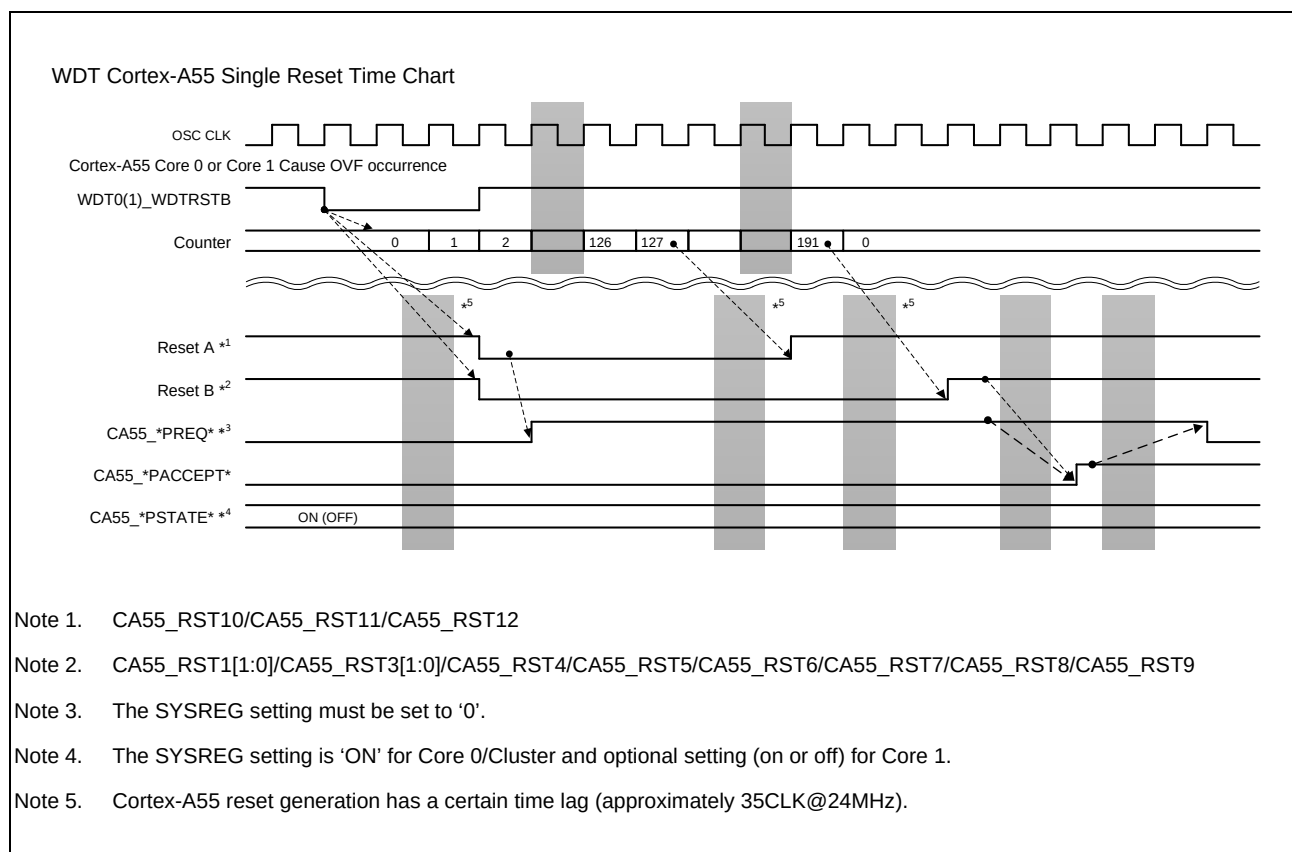
Figure 7.5 Timing of Cold Reset for the Cortex-A55 Alone due to the WDT Source
