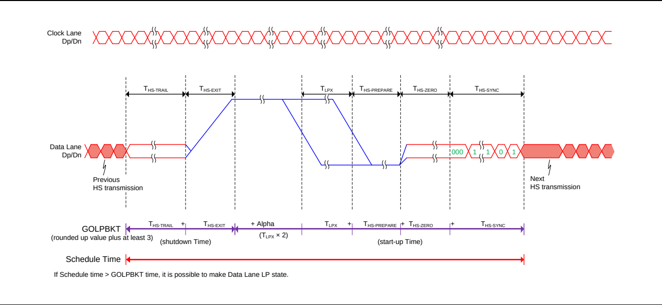
Figure 34.3 Switching the Data Lane between High-Speed Mode and Low-Power Mode
