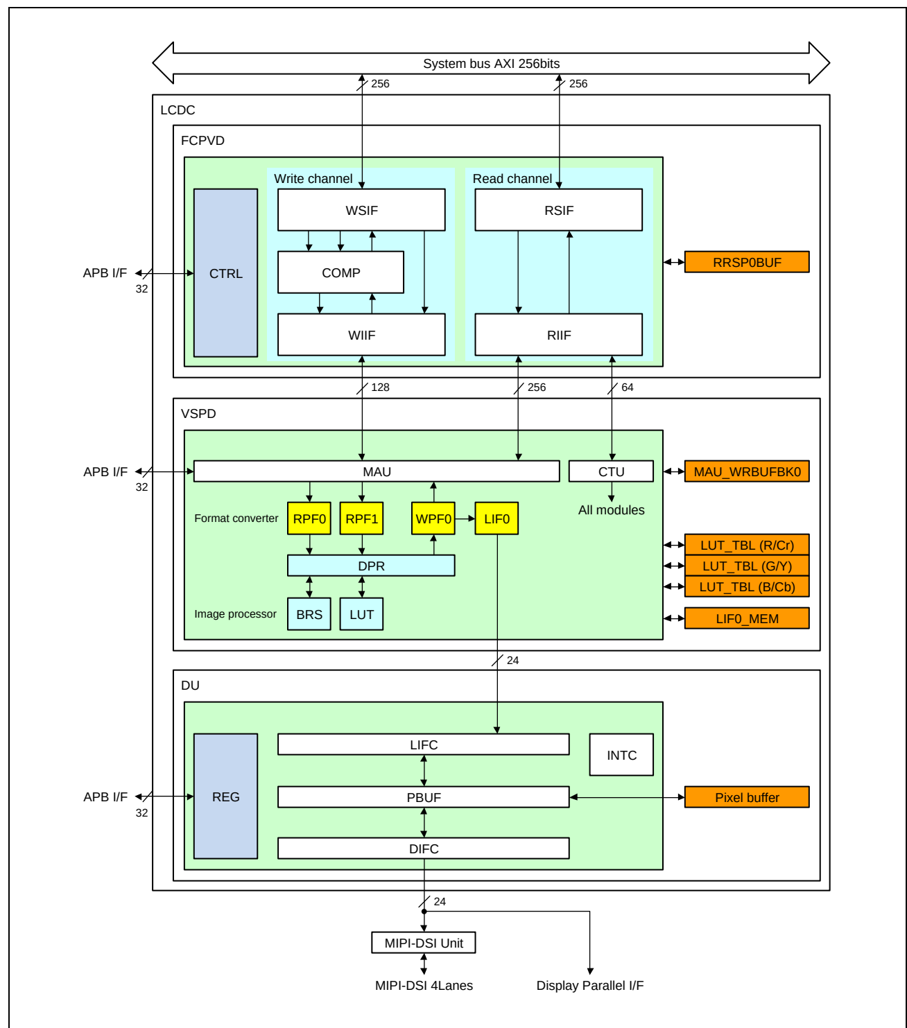
Figure 33.1 Block Diagram
