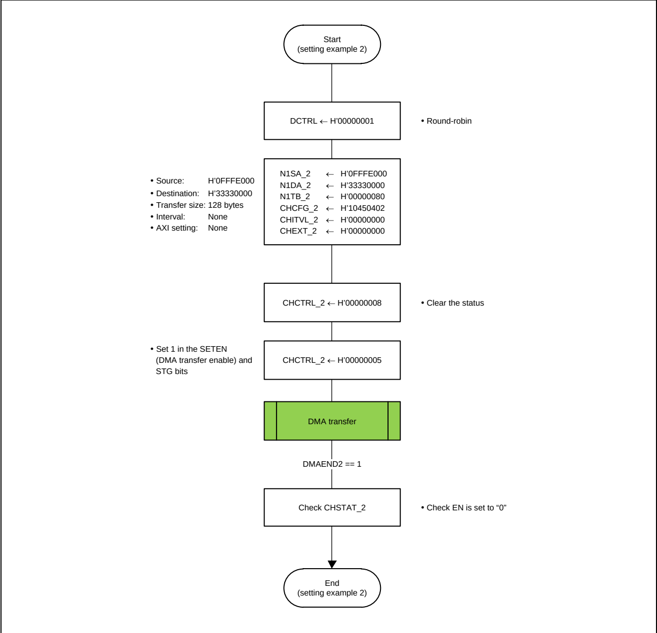
Figure 14.24 Setting Example 2
