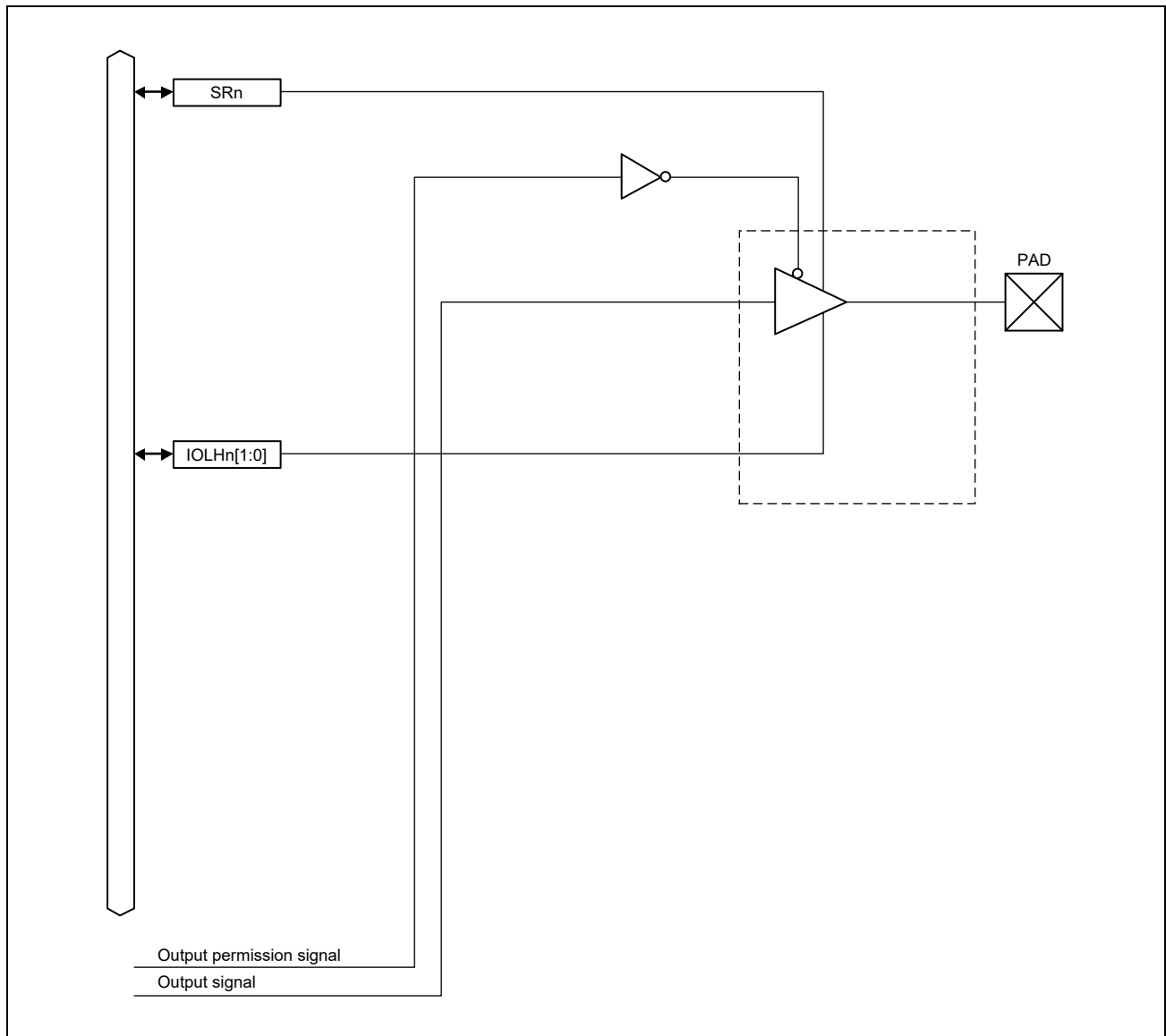
Figure 41.12 TDO, WDTOVF_PERROUT#
