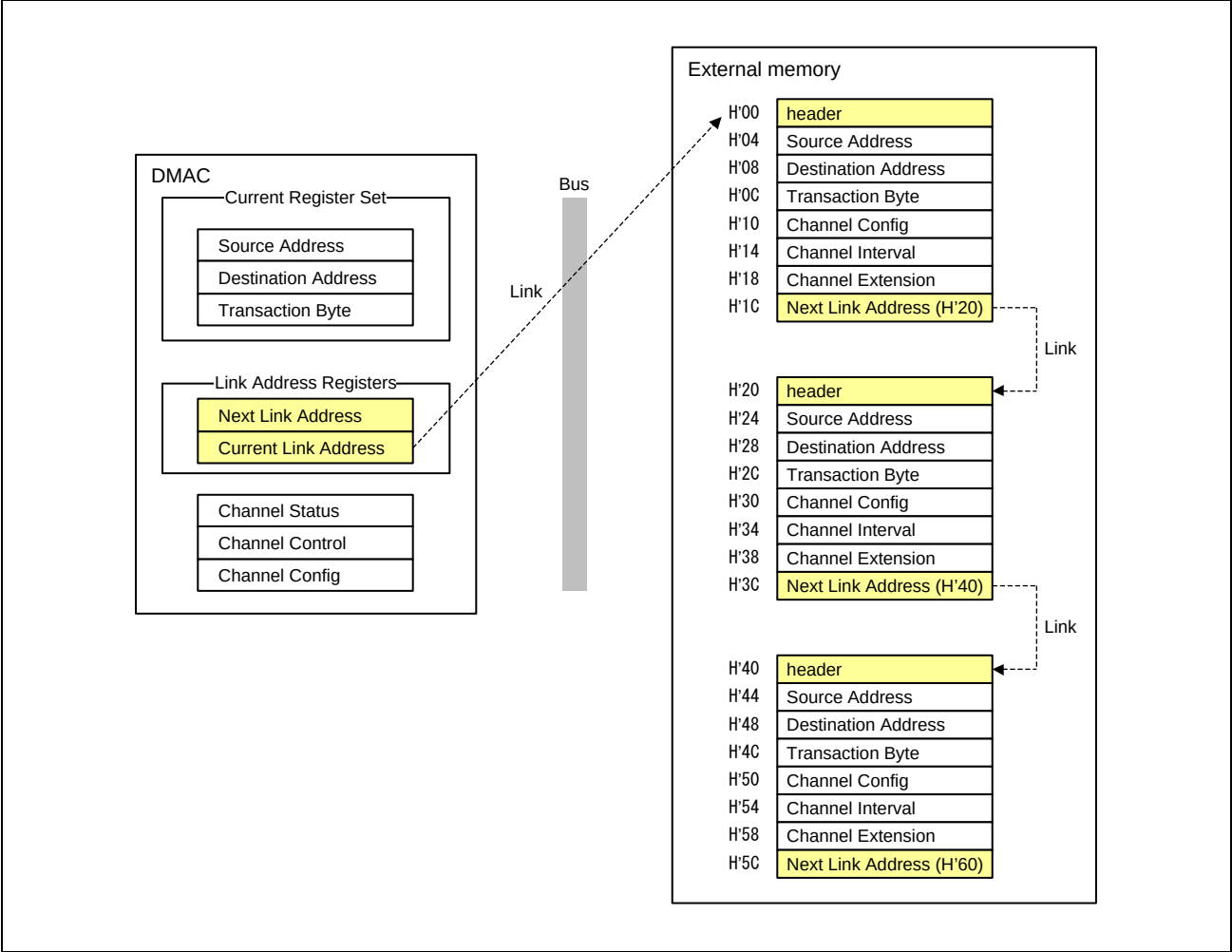
Figure 32B.18 Overview of Link Mode
