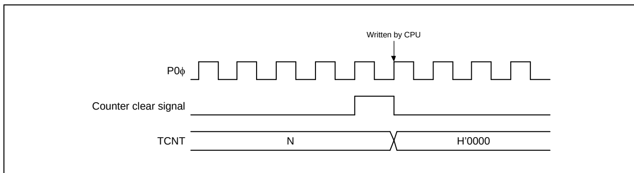
Figure 16.134 Contention between TCNT Write and Clear Operations
