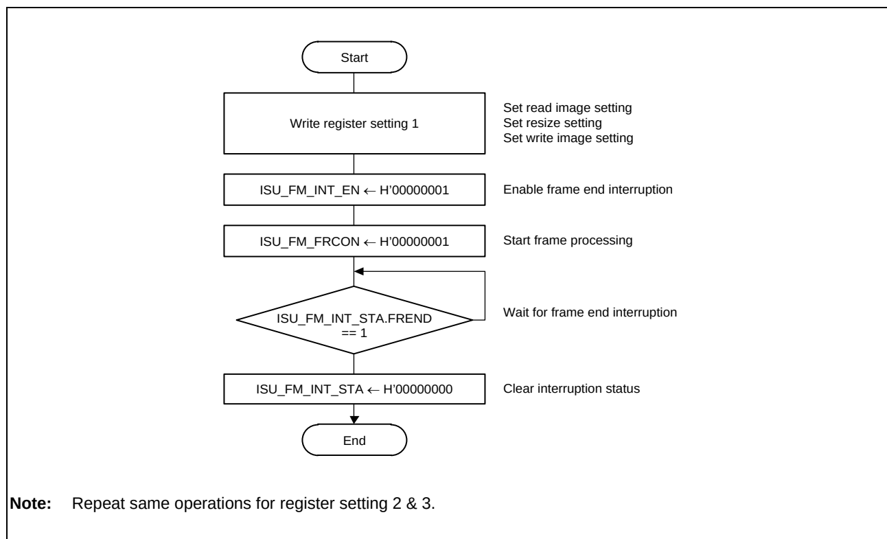
Figure 36.48 Flowchart of Image Size Conversion Example 3
