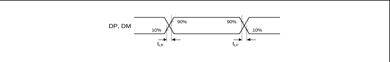
Figure 48.13 USB0_DP, USB1_DP, USB0_DM, and USB1_DM Output Timing (Low-Speed)
