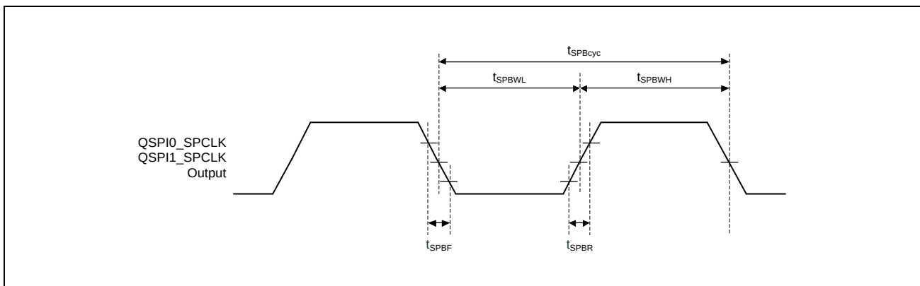
Figure 48.26 Clock Timing
