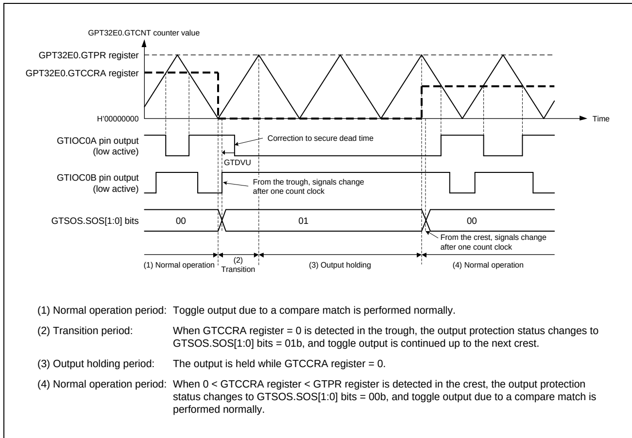
Figure 18.93 Example of output protection operation when GTCCRA is set to 0 during buffer transfer at troughs, with 0 < GTCCRA < GTPR restored during buffer transfer at crests, and active-low
