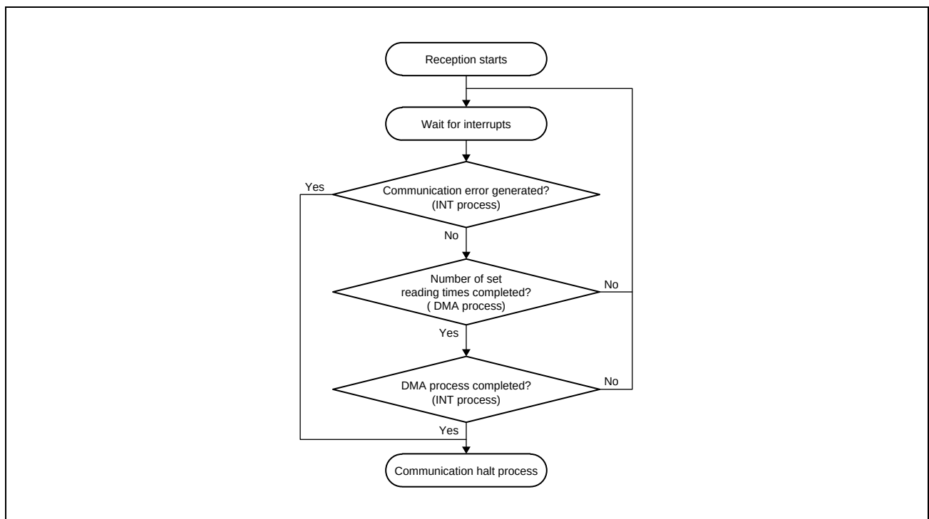
Figure 27.54 Reception Procedure
