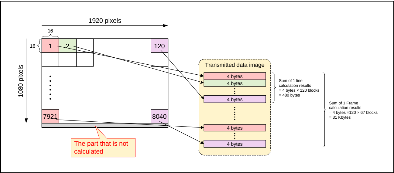
Figure 35.37 Illustration Diagram of the Amounts of Data in the Operations when a 1920×1080 Pixel Area is Set as 16×16 Blocks
