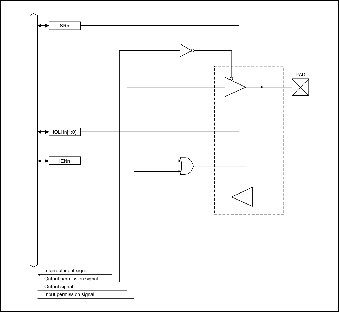
Figure 41.11 TMS/SWDIO
