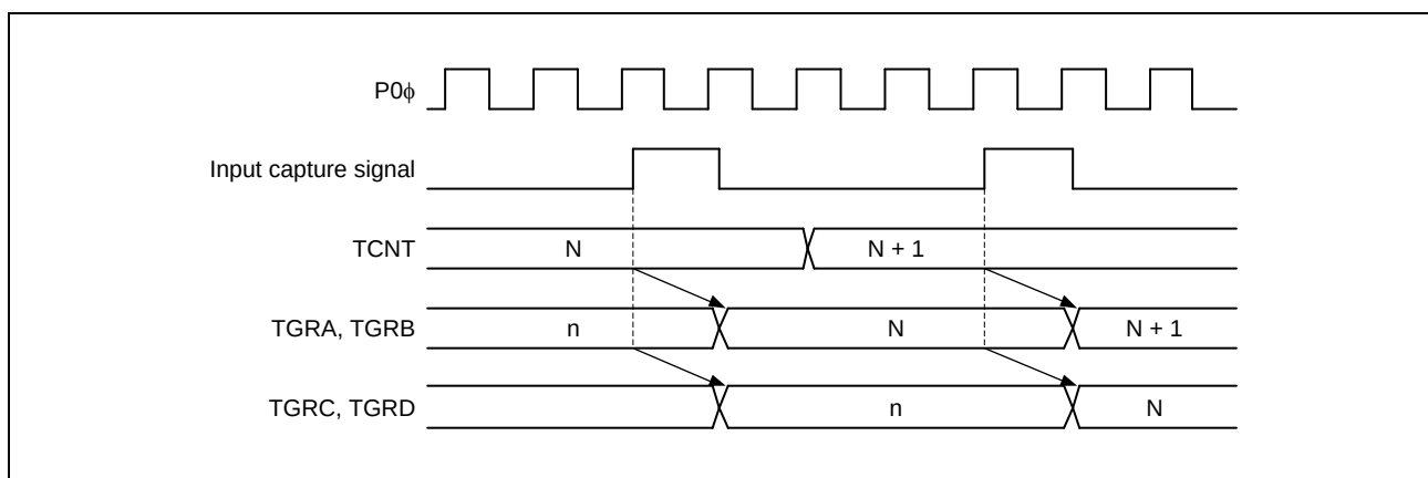
Figure 16.122 Buffer Operation Timing (Input Capture)
