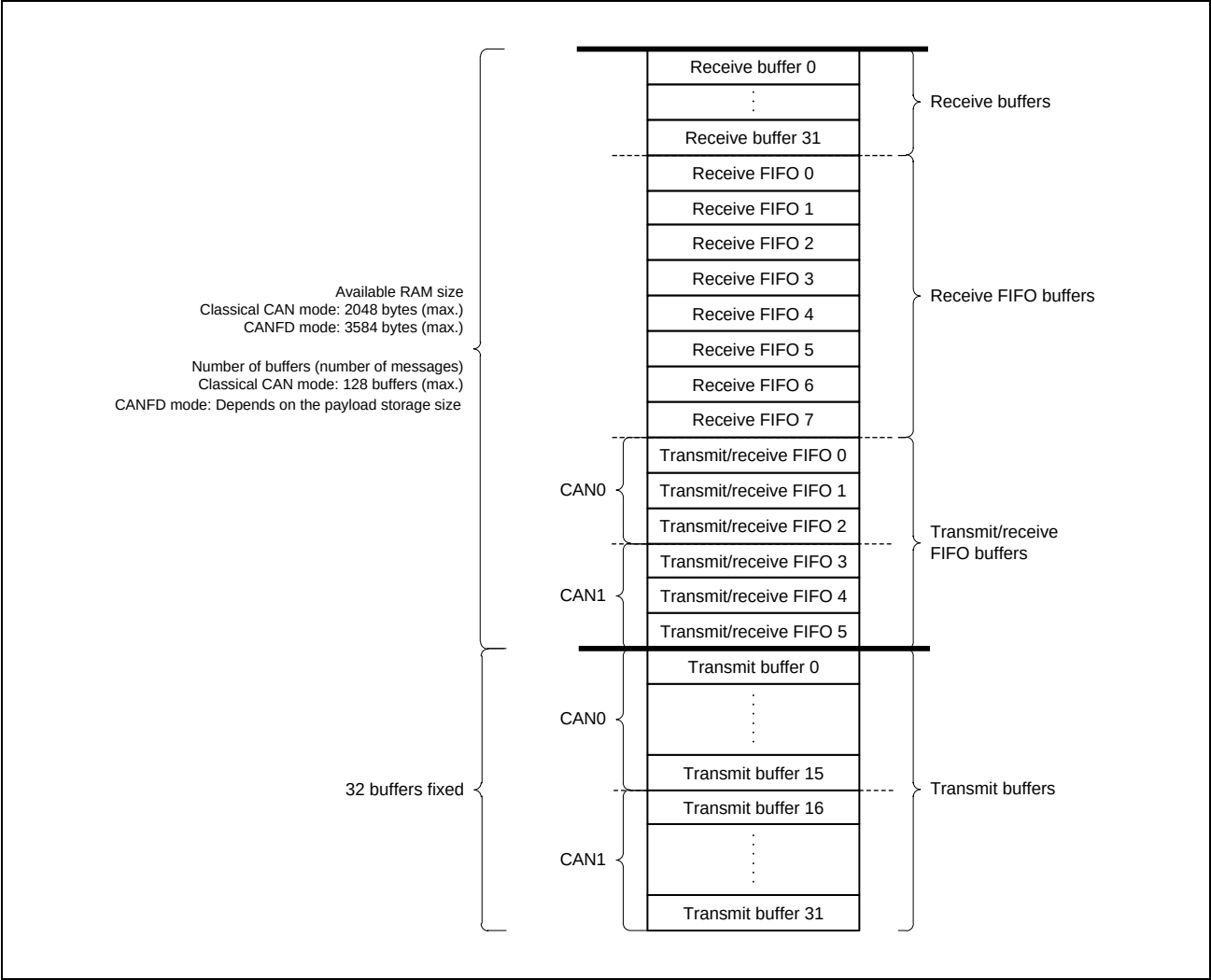
Figure 28.20 Buffer Configuration
