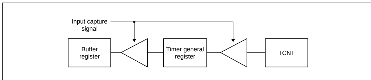
Figure 16.16 Input Capture Buffer Operation
