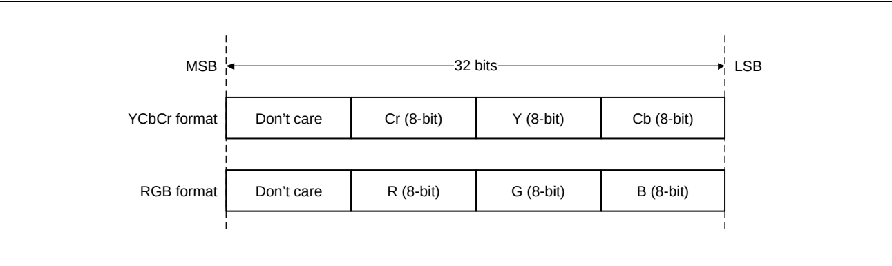
Figure 33.37 VI6_LUT_TBL Formats
