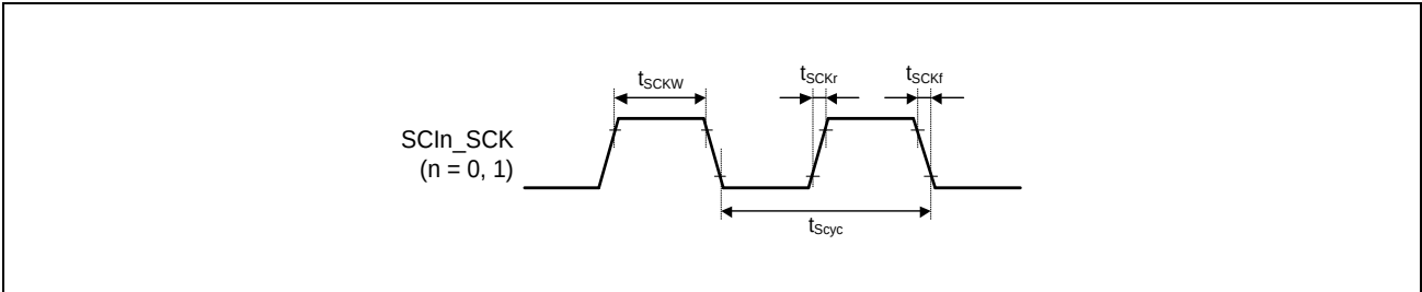
Figure 48.48 SCK Input Clock Timing
