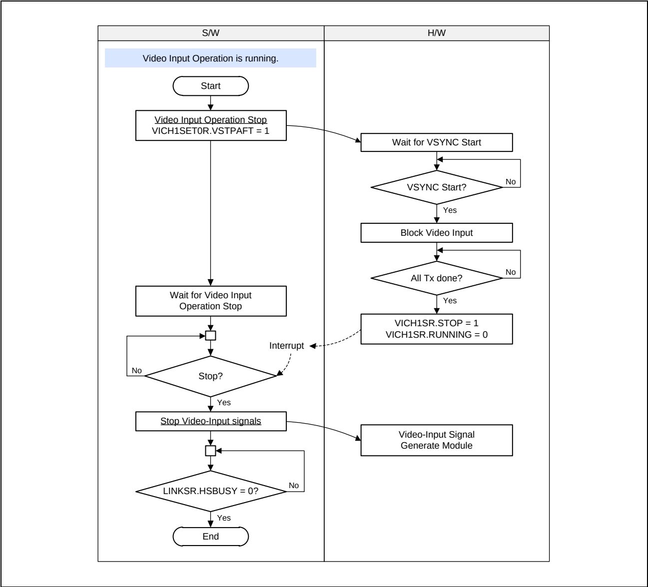
Figure 34.13 End of Video-Input Operation (VICH1SET0R.VSTPAFT)
