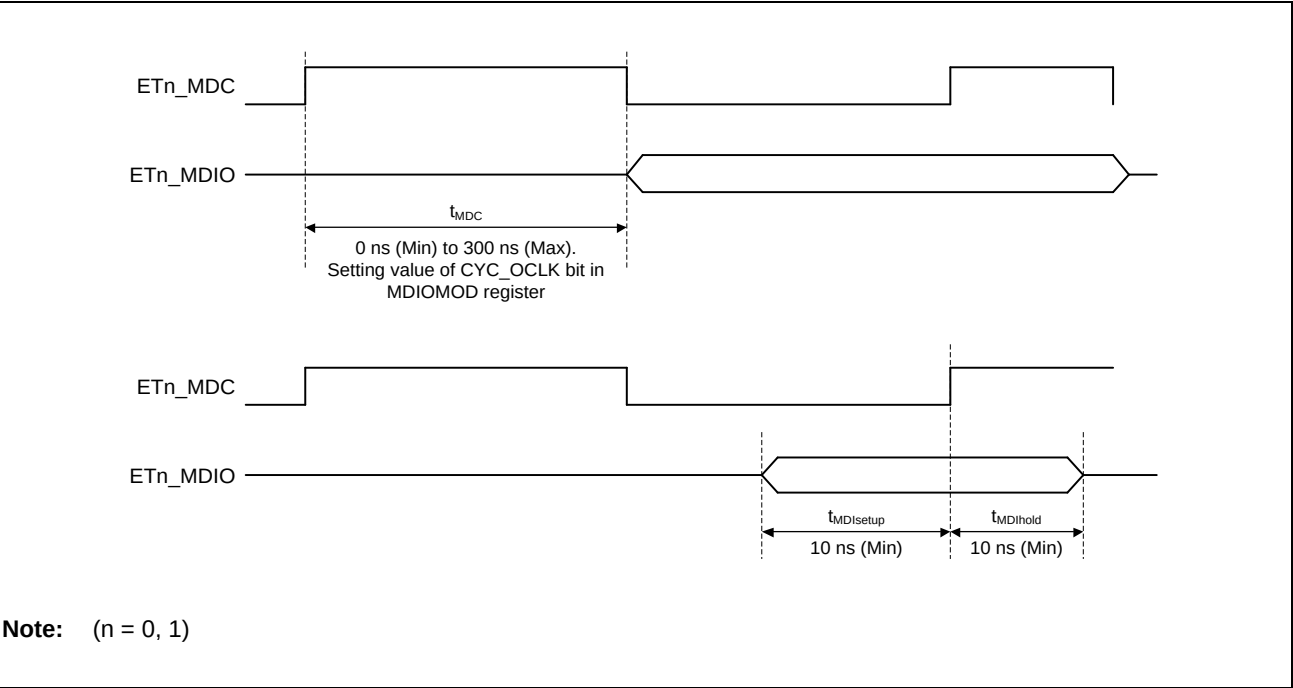
Figure 48.19 Management Interface
