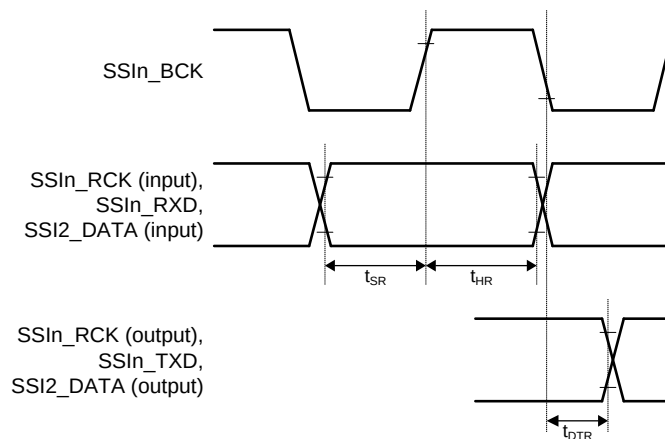
Figure 48.36 Transmission and Reception Timing (SSIBCK Falling Output)
