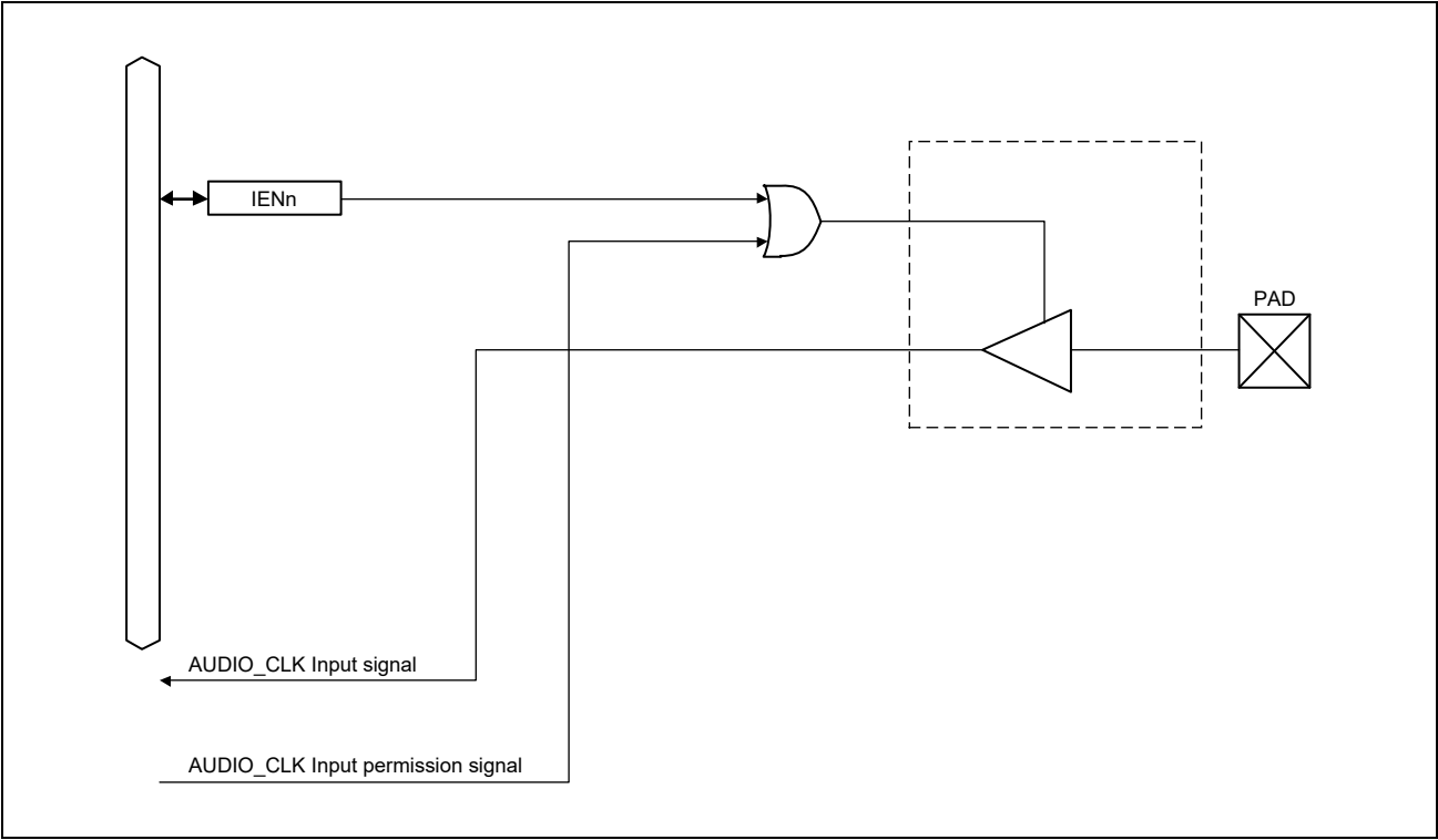
Figure 41.13 AUDIO_CLK1, AUDIO_CLK2
