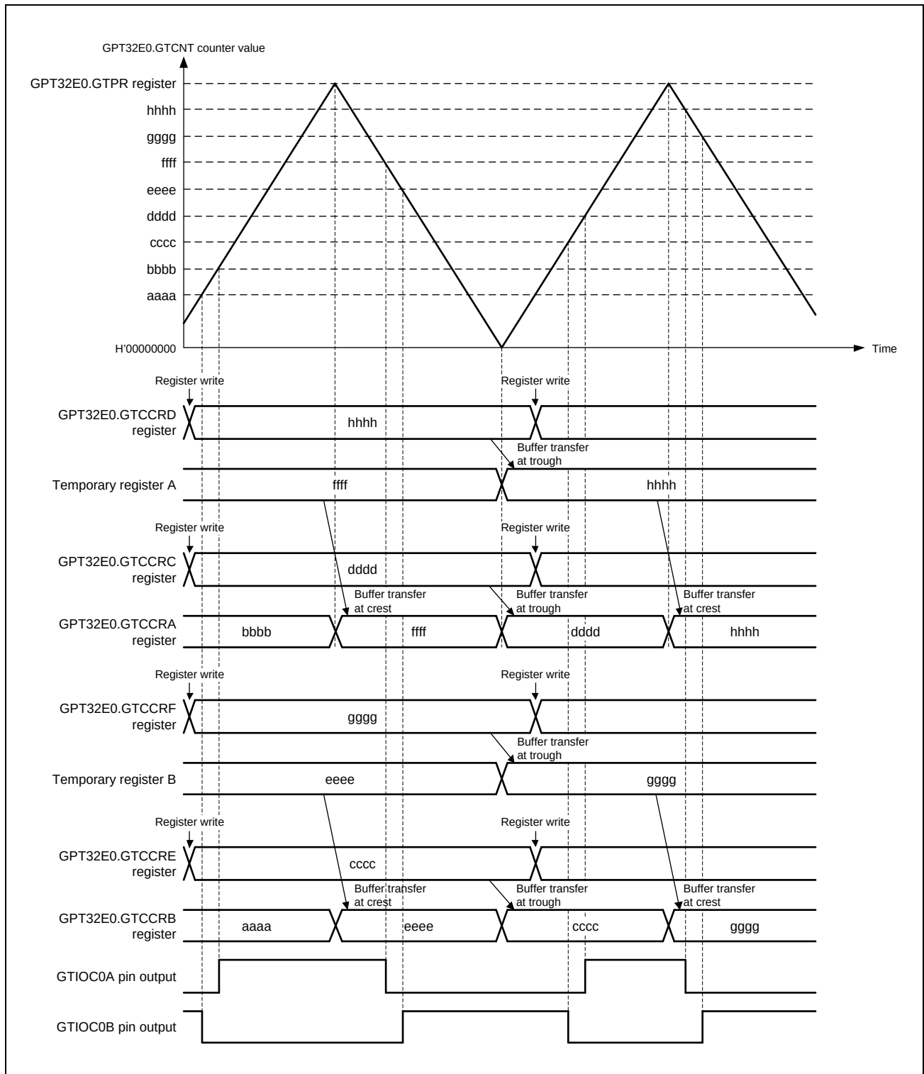
Figure 18.40 Example of triangle-wave PWM mode 3 operation with low output from the GTIOC0A pin and high output from the GTIOC0B pin at count start, output toggled at GTCCRc/GTCCRr compare match, and output retained at cycle end
