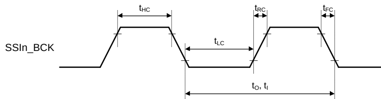
Figure 48.35 Bit Clock Input/Output Timing
