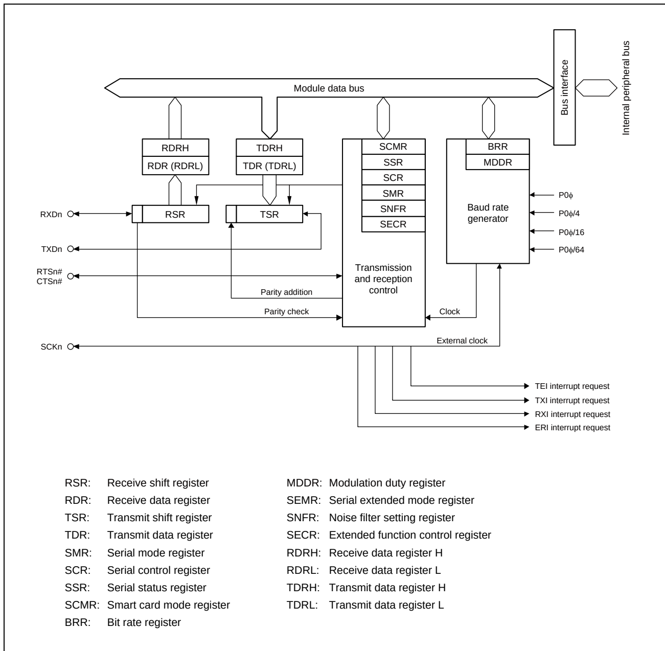
Figure 23.1 Block Diagram of SC1g (SCI0 and SCI1)
