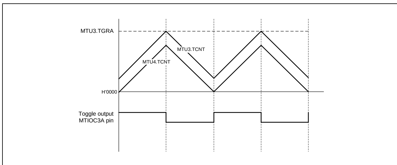
Figure 16.64 Example of Toggle Output Waveform Synchronized with PWM Output (MTU3 and MTU4)
