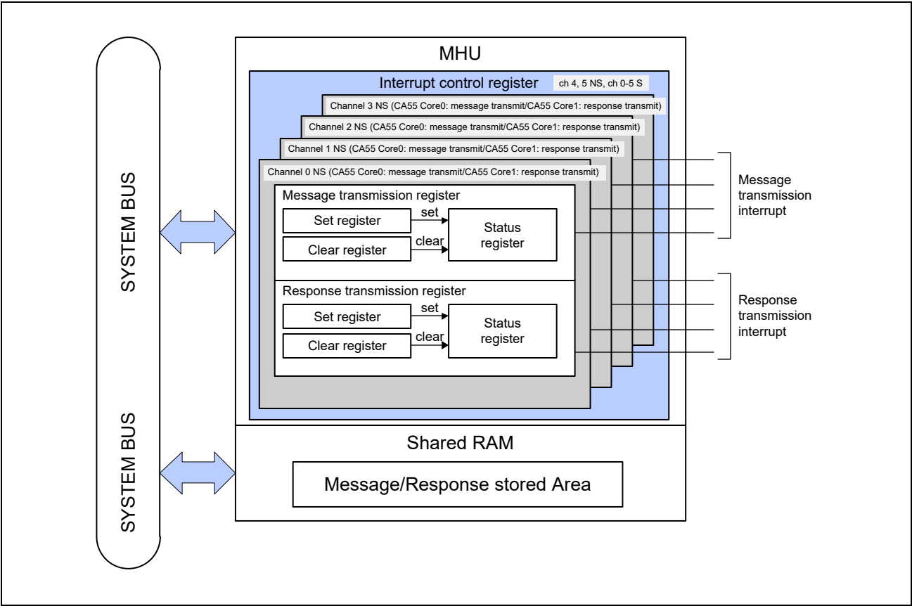
Figure 12.2 Hardware configuration
