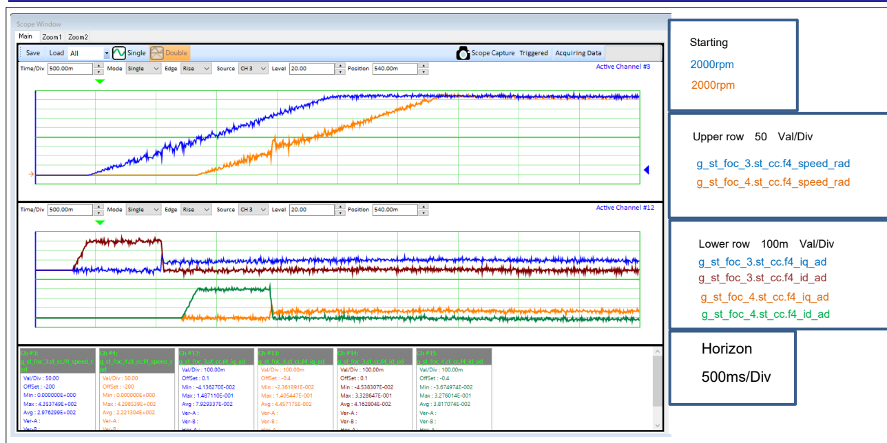
Figure 5-3 Driving Waveforms When Motors 3 and 4 are Starting up (3/3)
