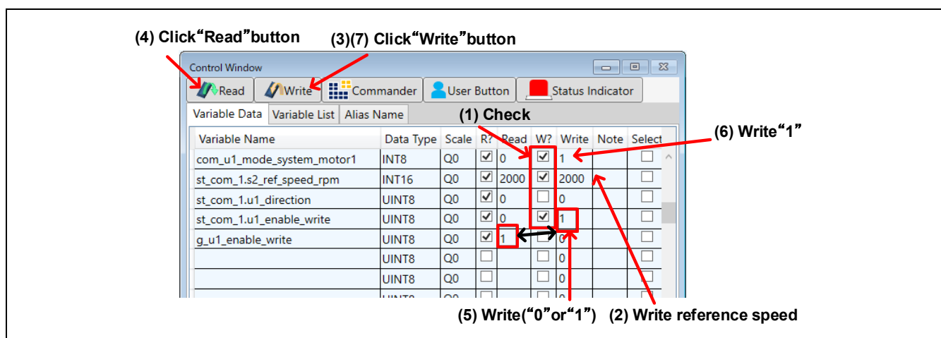
Figure 4-2 Procedure – Driving the Motor
