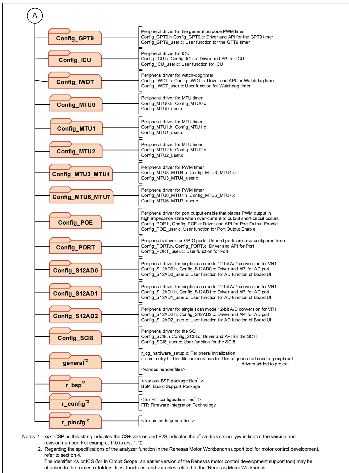
Figure 2-8 Smart Configurator Folder and File Configurations (2)
