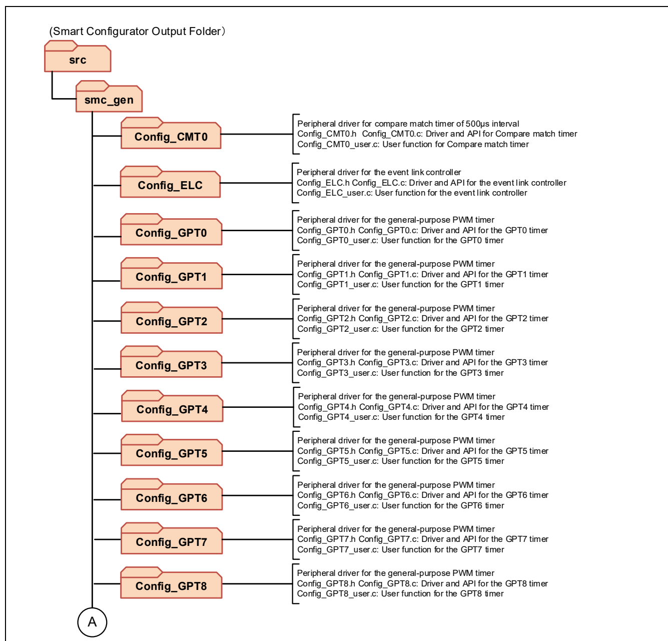
Figure 2-8 Smart Configurator Folder and File Configurations (1)
