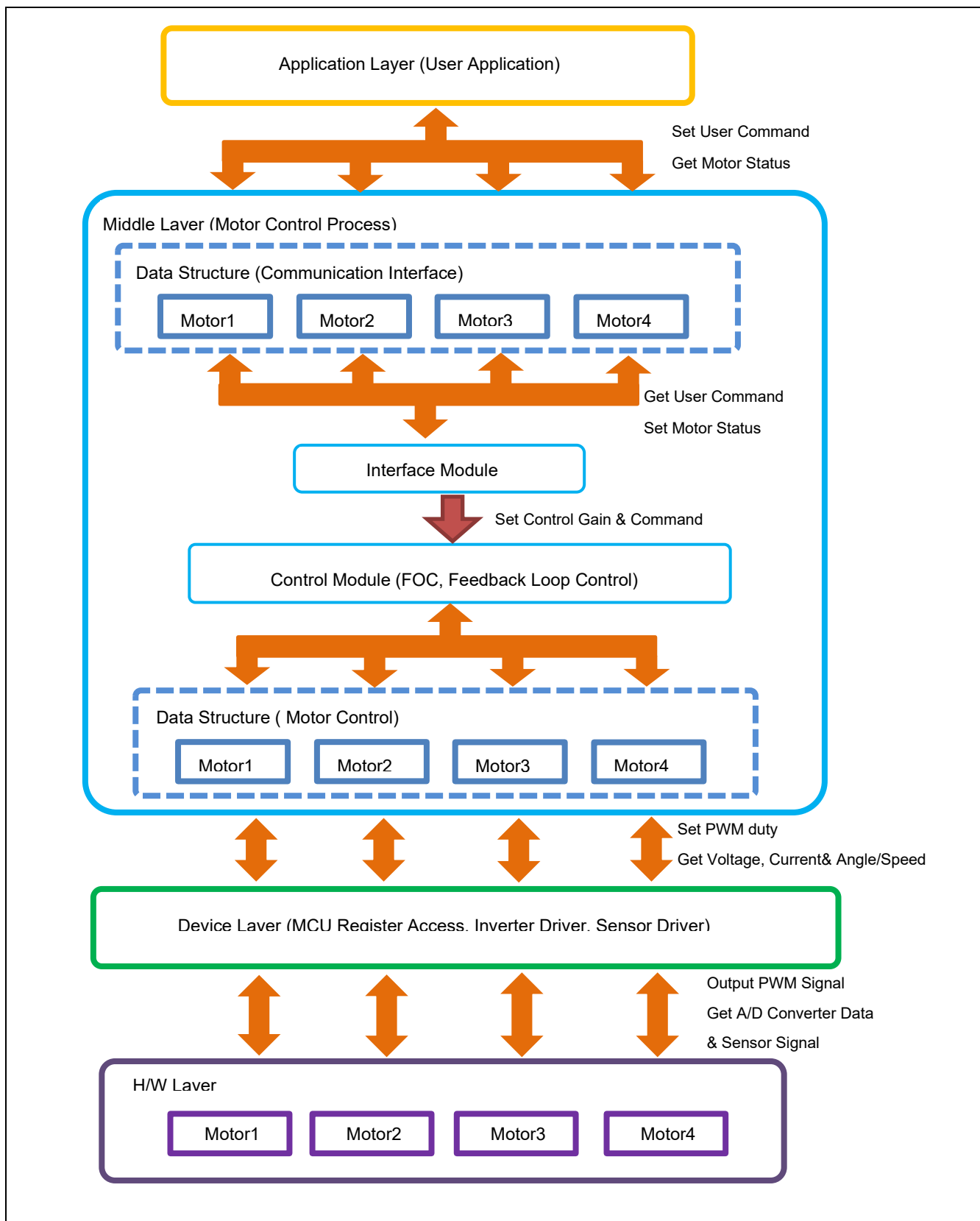
Figure 2-9 Module Configuration
