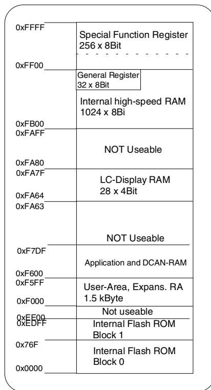
Figure 1-4: Normal-mode memory-layout
