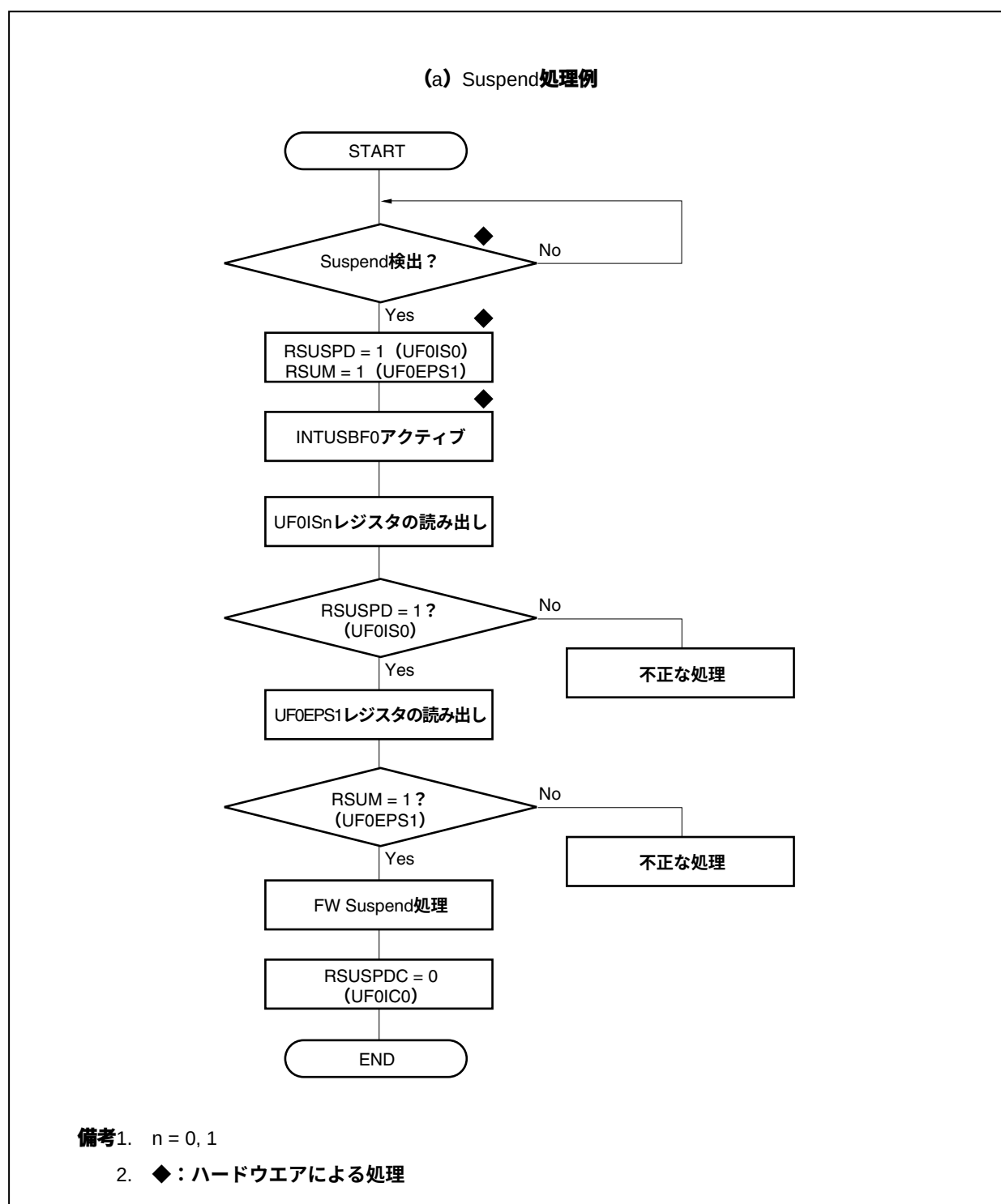
図20-30 Suspend/Resume処理例 (1/3)
