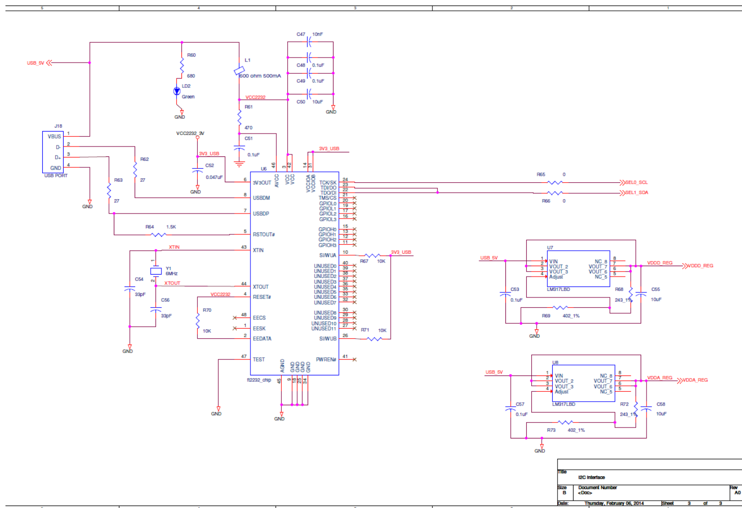
Figure 7. Evaluation Board Schematics – Page 3
