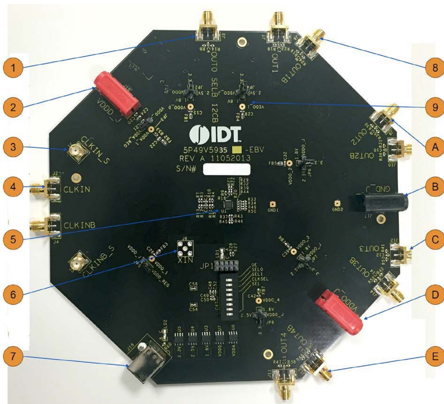
Figure 1. Board Overview
