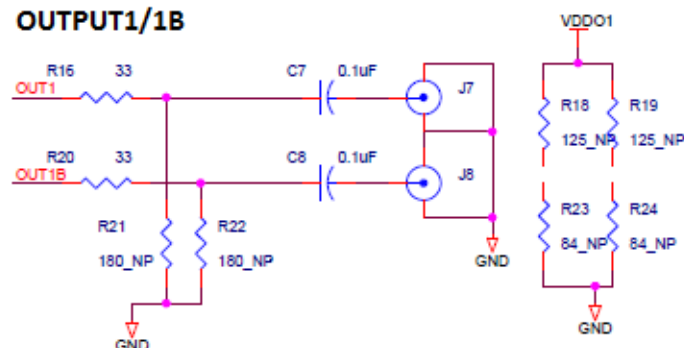
Figure 8. Output Termination Options
