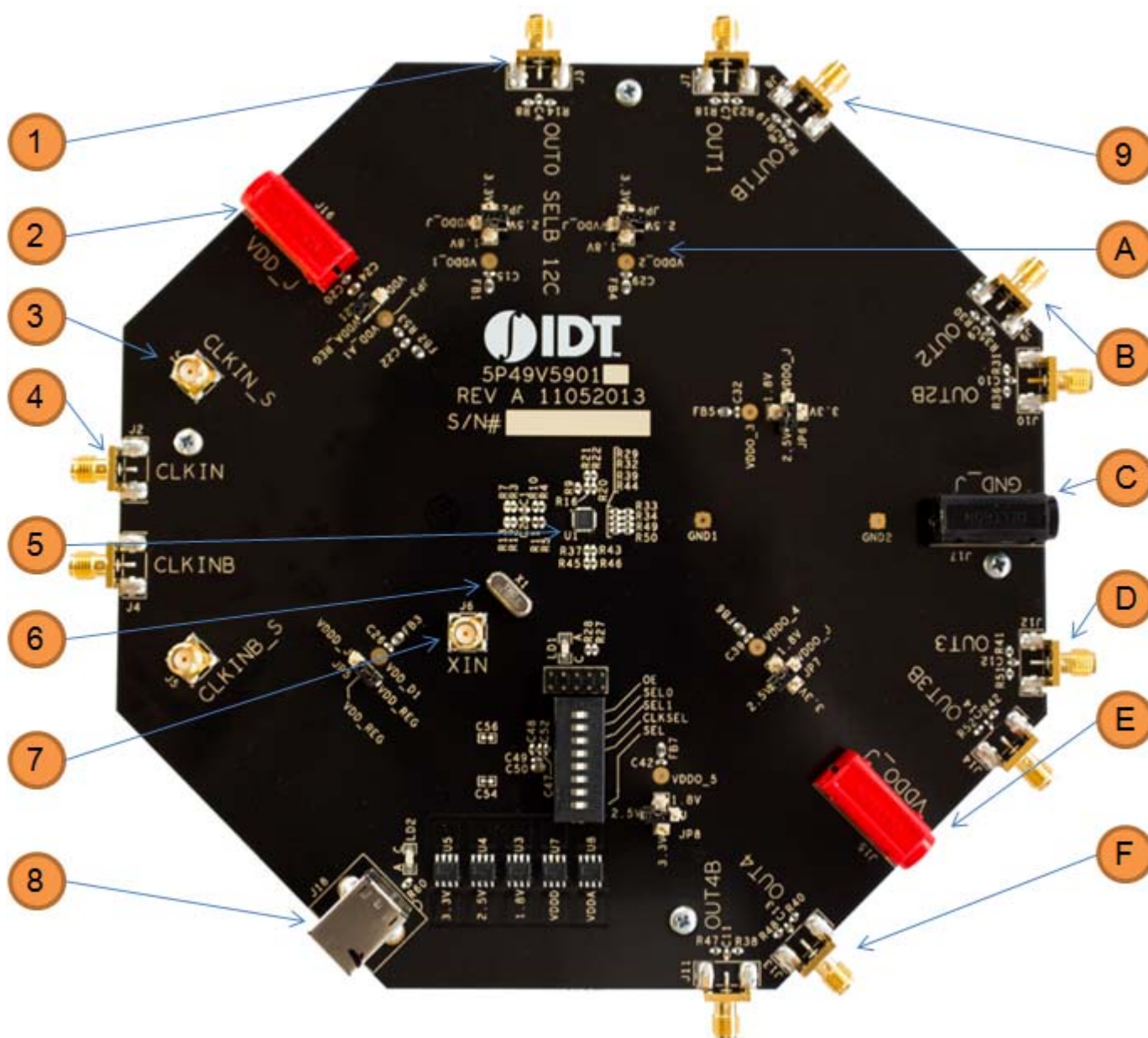
Figure 1. Board Overview
