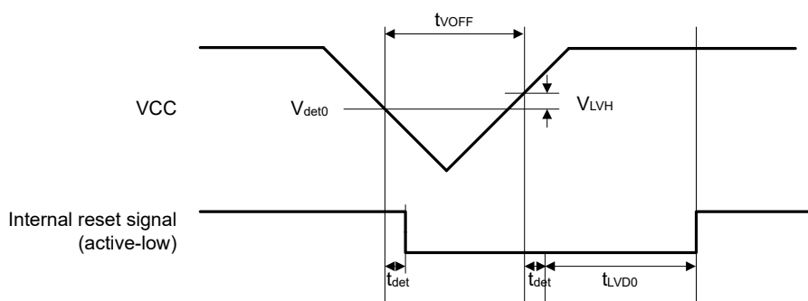
Figure 39.43 Voltage detection circuit timing ( V_{det0} )
