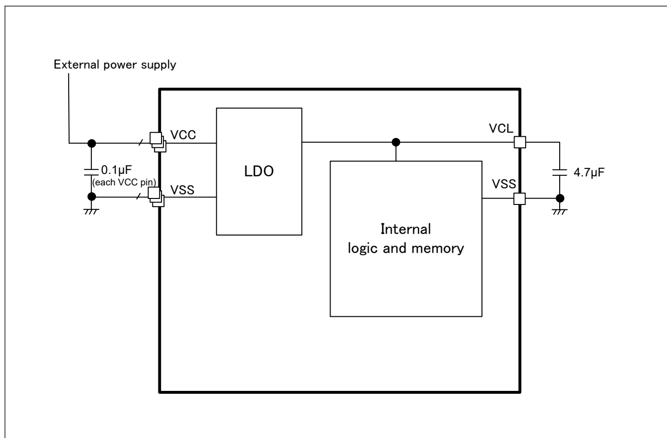
Figure 38.1 LDO settings
