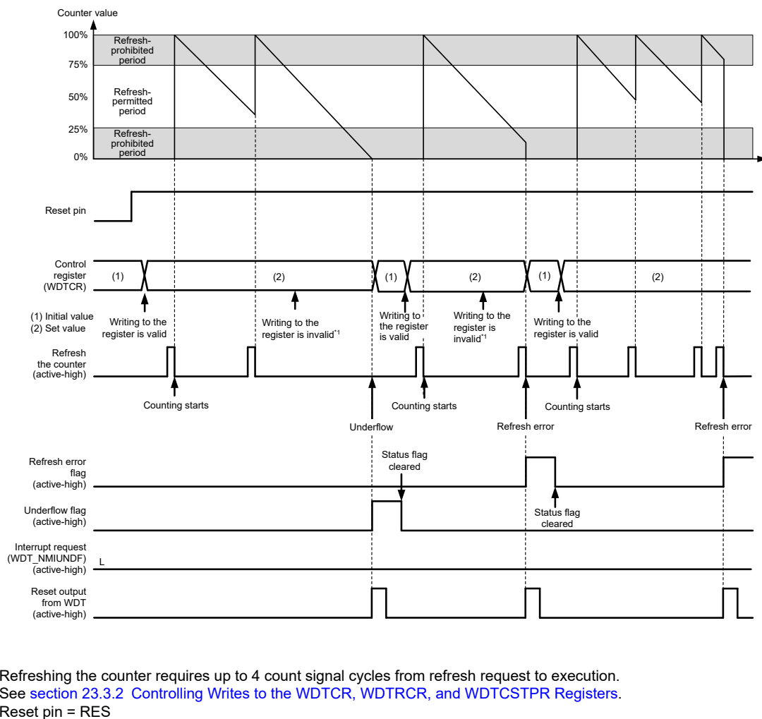
Figure 23.3 Operation example in register start mode
