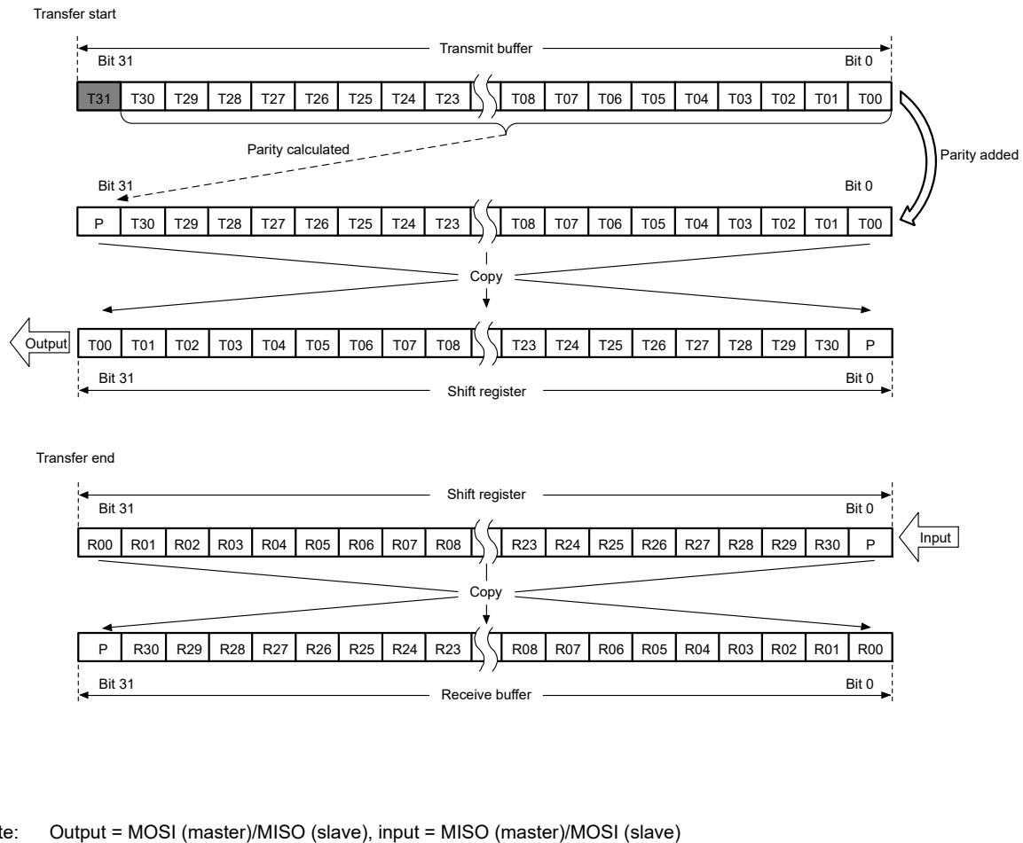
Figure 27.20 LSB-first transfer with 32-bit data and parity enabled
