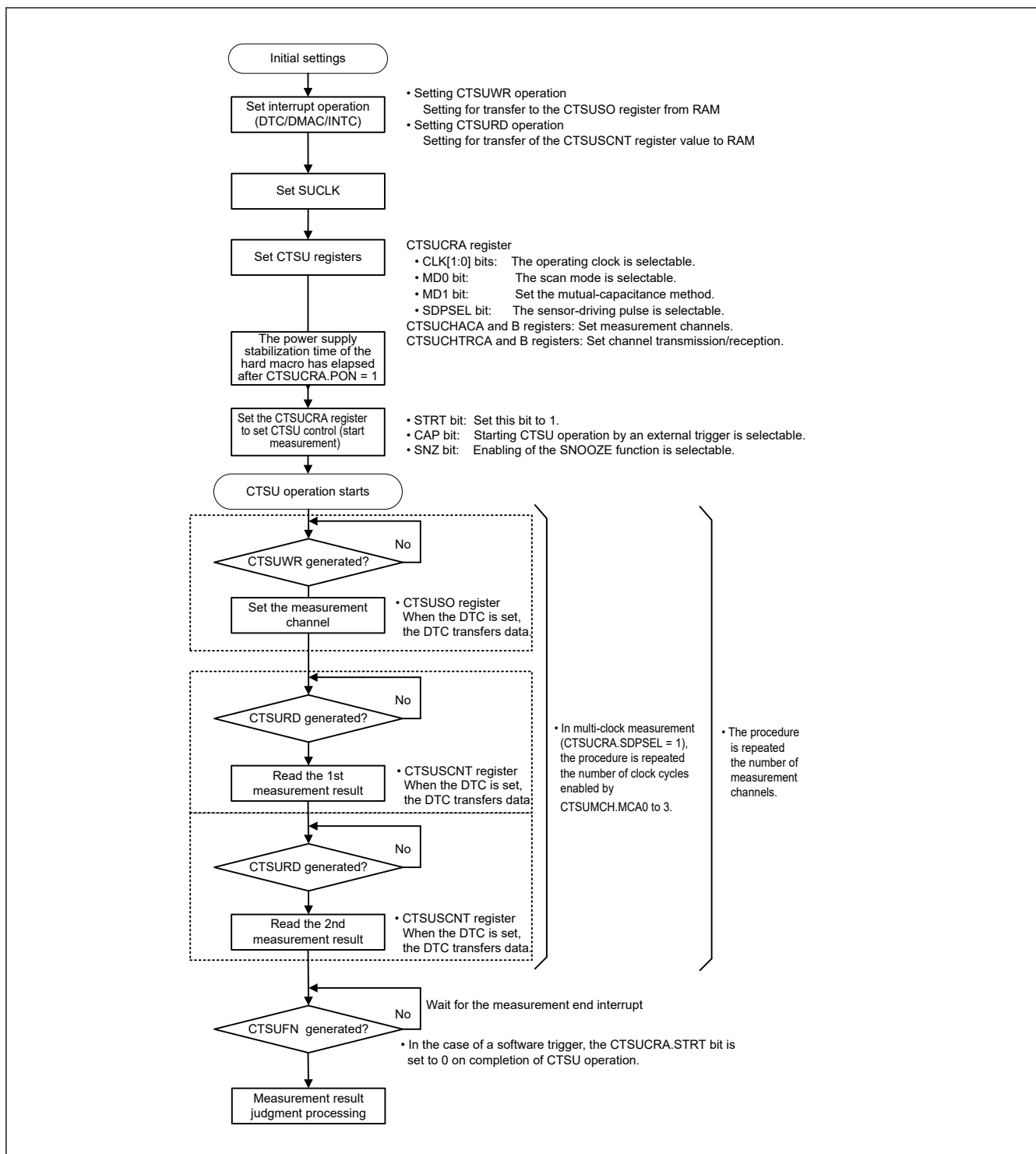
Figure 32.13 Software flow and operation example of mutual capacitance method
