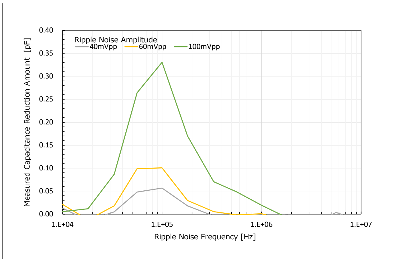
Figure 39.46 Measured capacitance reduction amount
