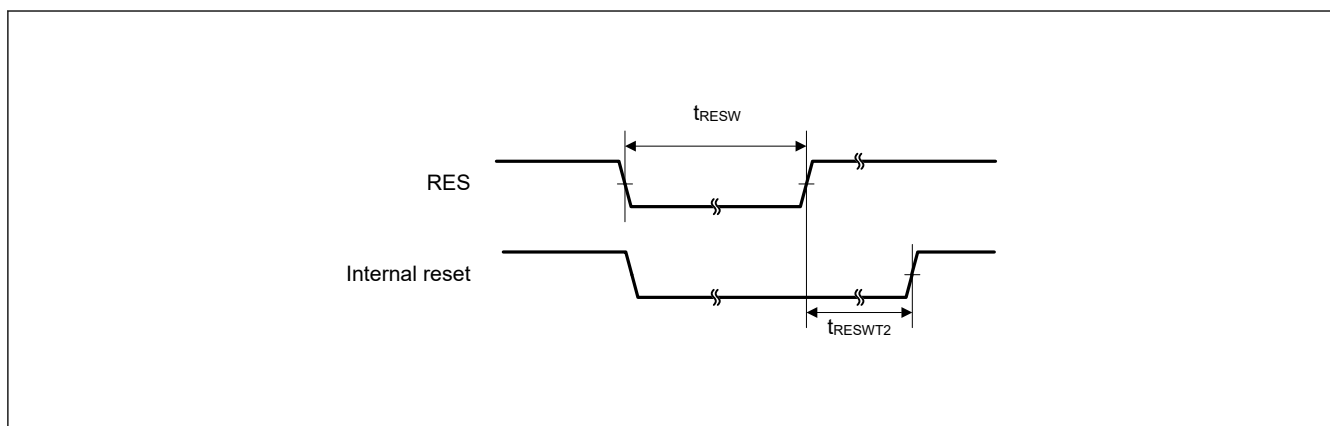
Figure 39.8 Reset input timing (1)
