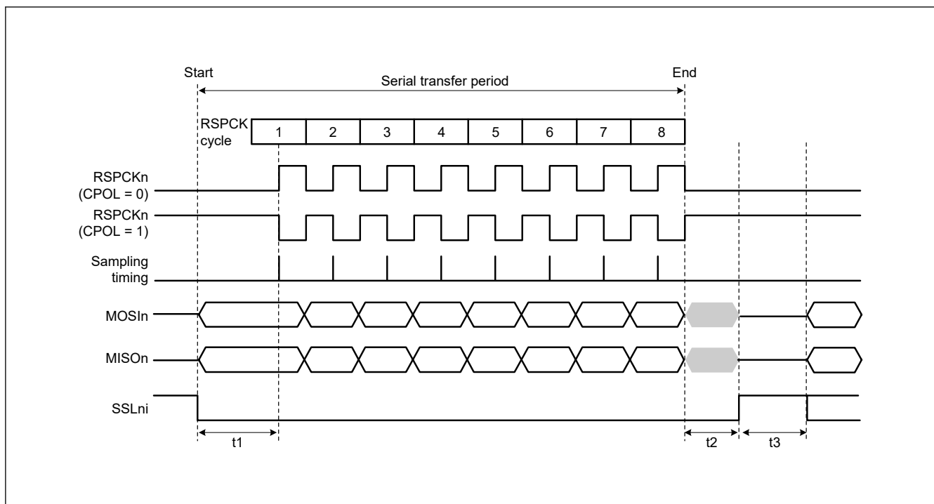
Figure 27.22 SPI transfer format when CPHA = 0
