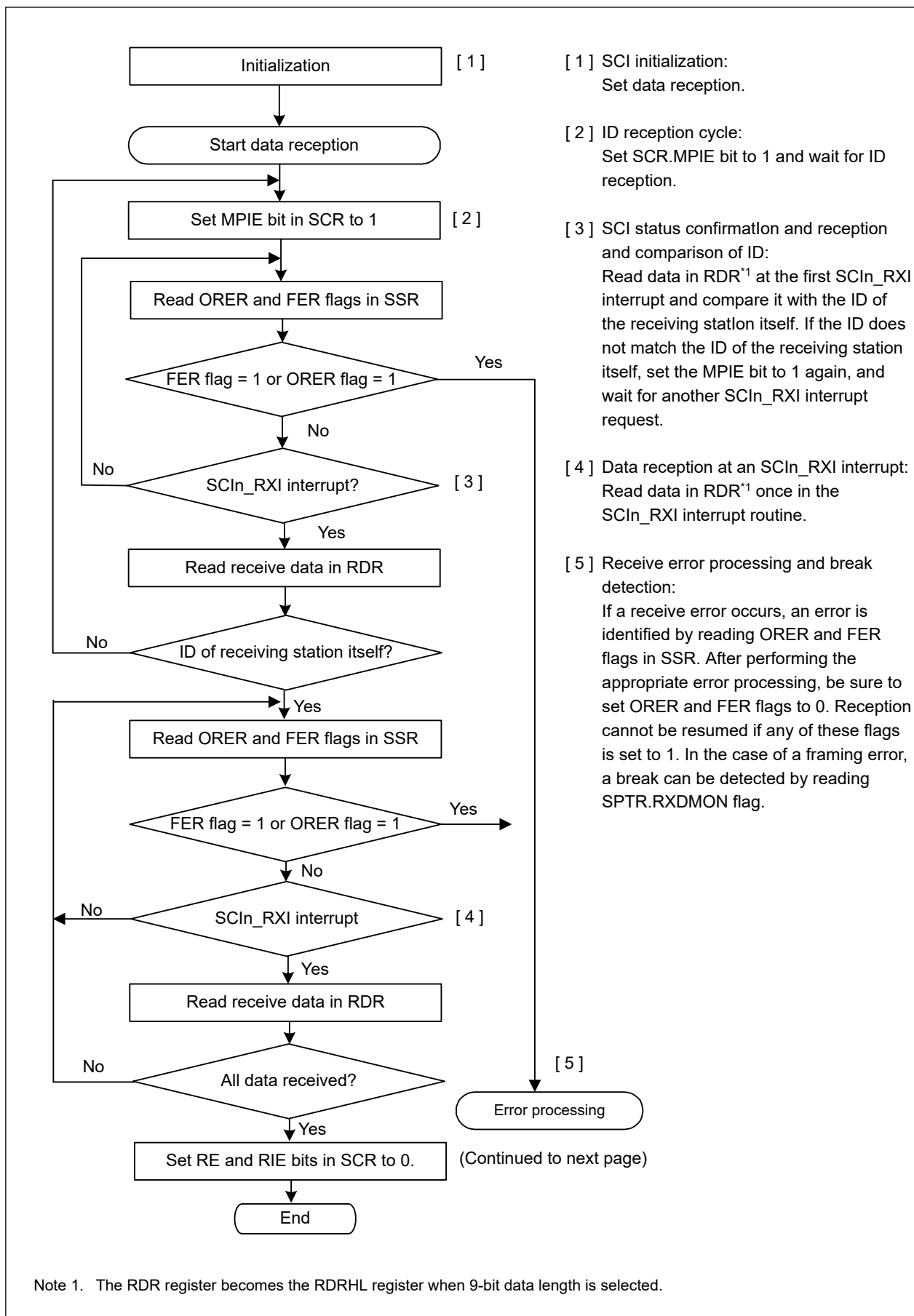
Figure 25.31 Example flow of multi-processor serial reception with non-FIFO selected (1)
