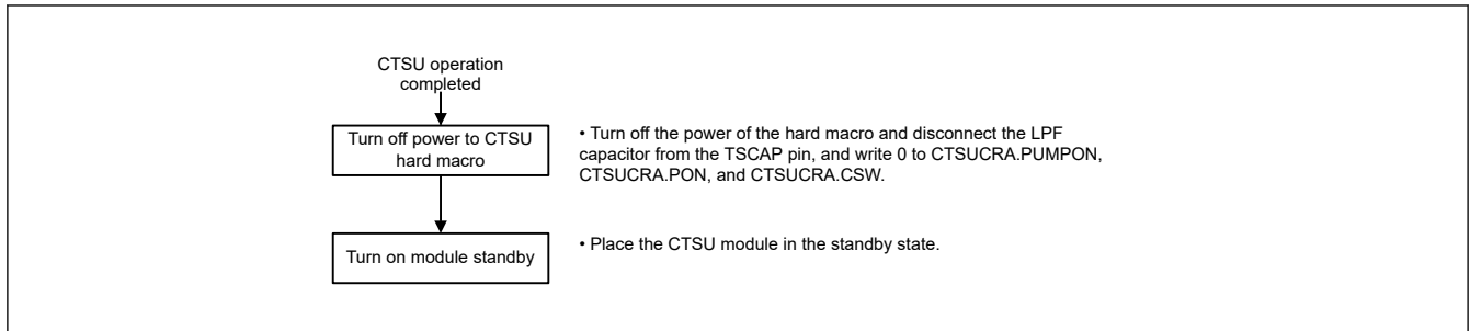
Figure 32.9 Flow of stopping CTSU
