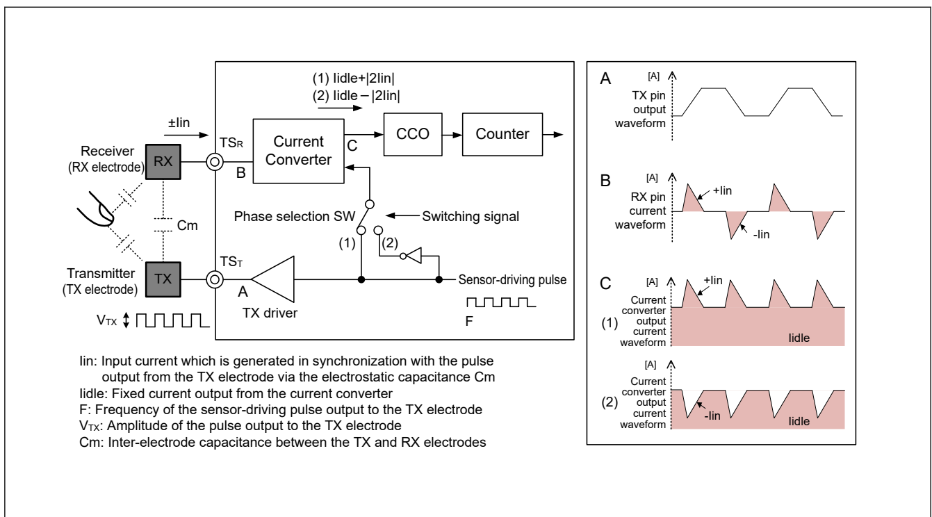
Figure 32.14 Measurement block circuit for high-speed measurement
