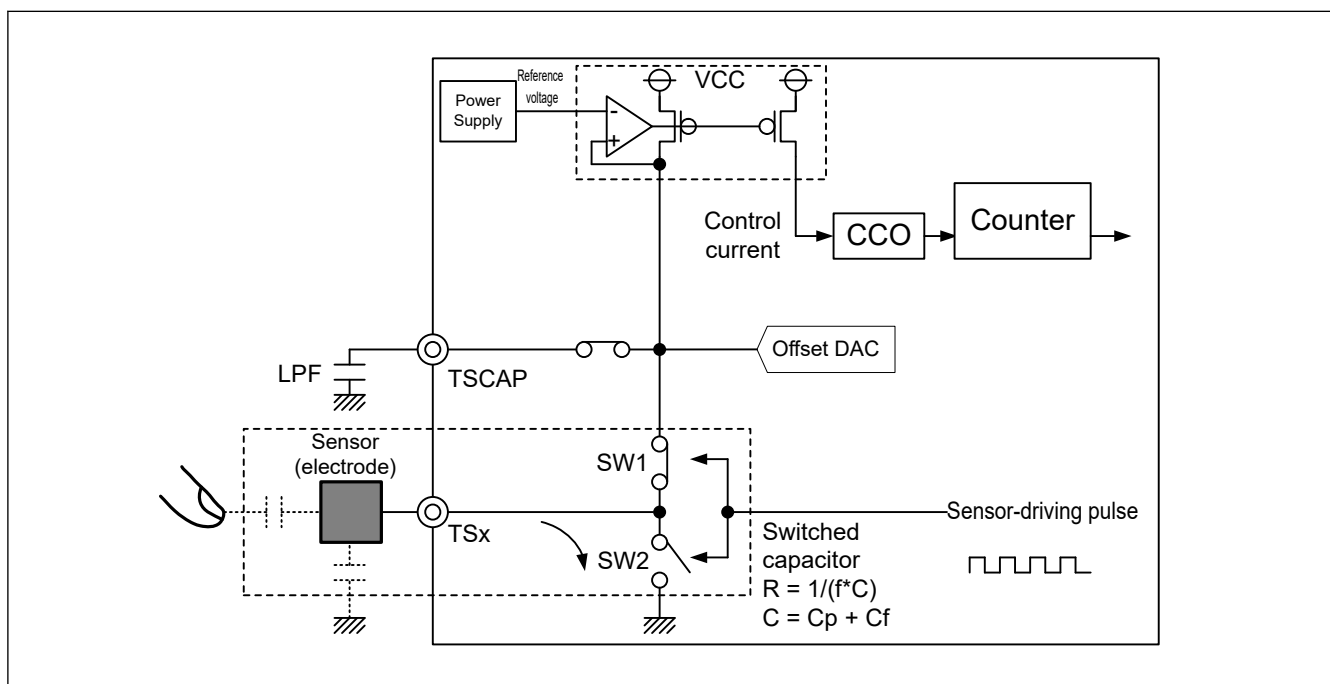
Figure 32.6 Self-capacitance discharging operation
