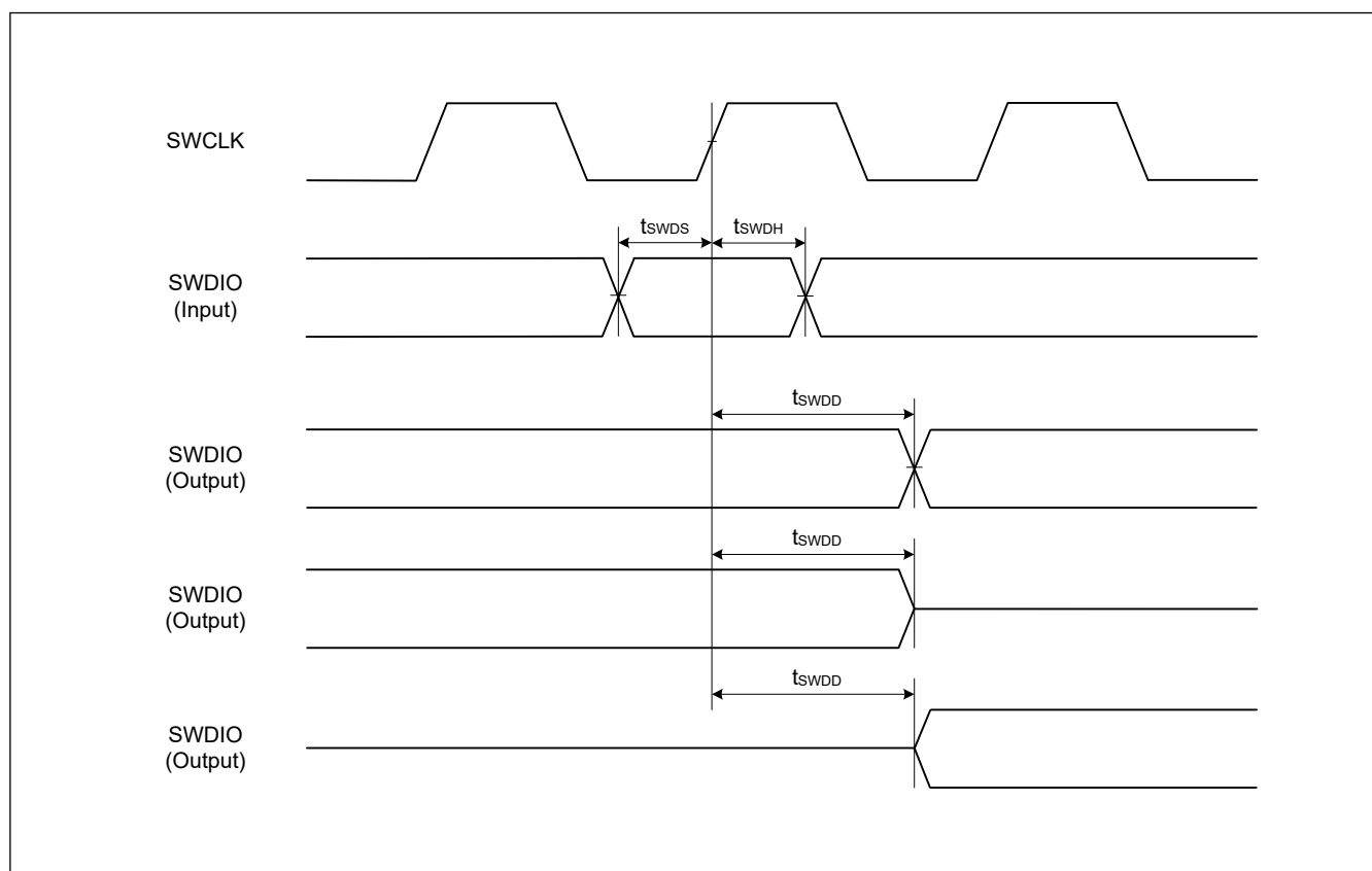
Figure 39.49 SWD input/output timing
