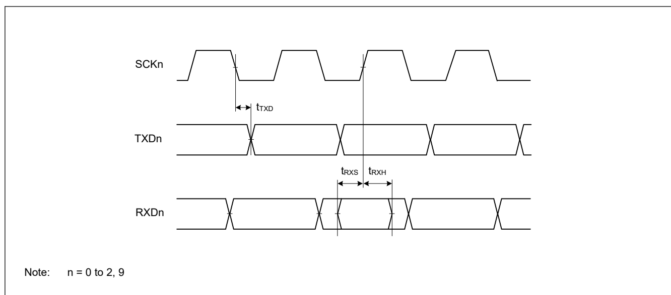
Figure 39.21 SCI input/output timing in clock synchronous mode
