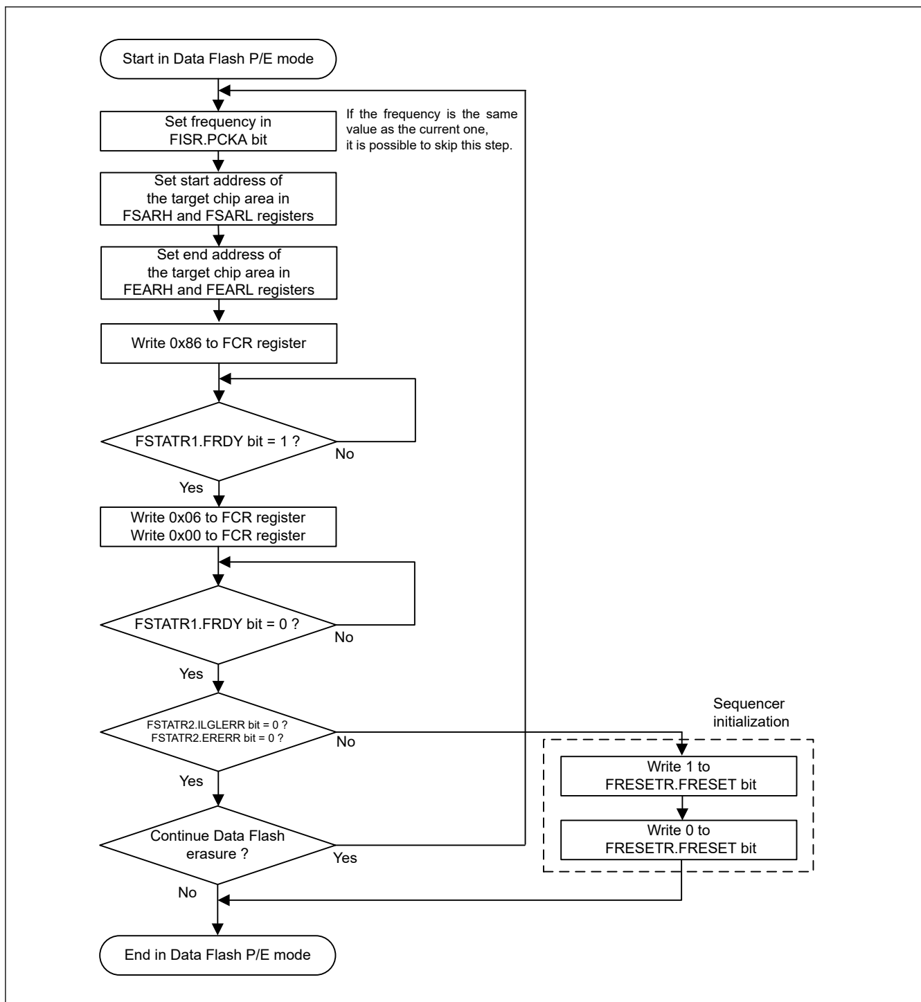
Figure 35.26 Flowchart for the data flash chip erase procedure
