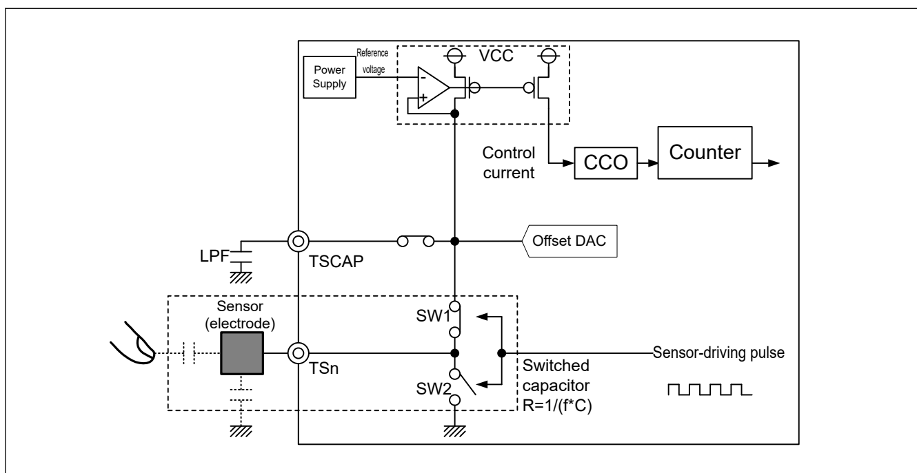
Figure 32.4 Self-capacitance measurement block circuit
