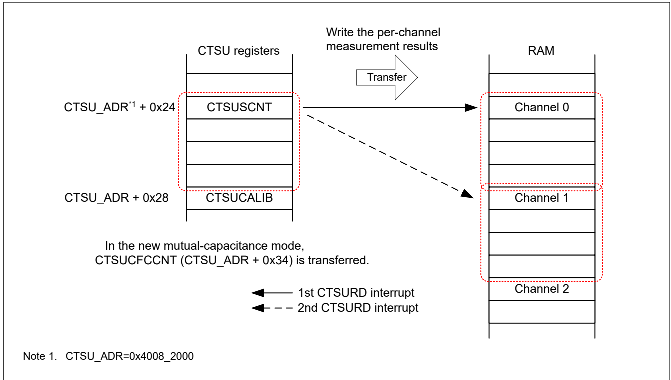
Figure 32.17 Example of DTC transfer operation using CTSURD interrupt
