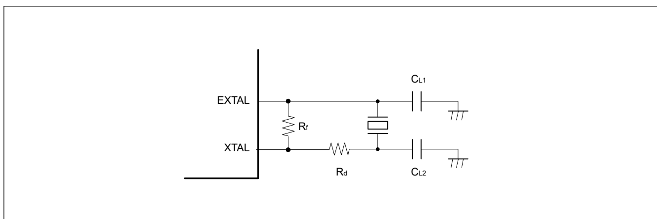
Figure 8.5 Example of crystal resonator connection
