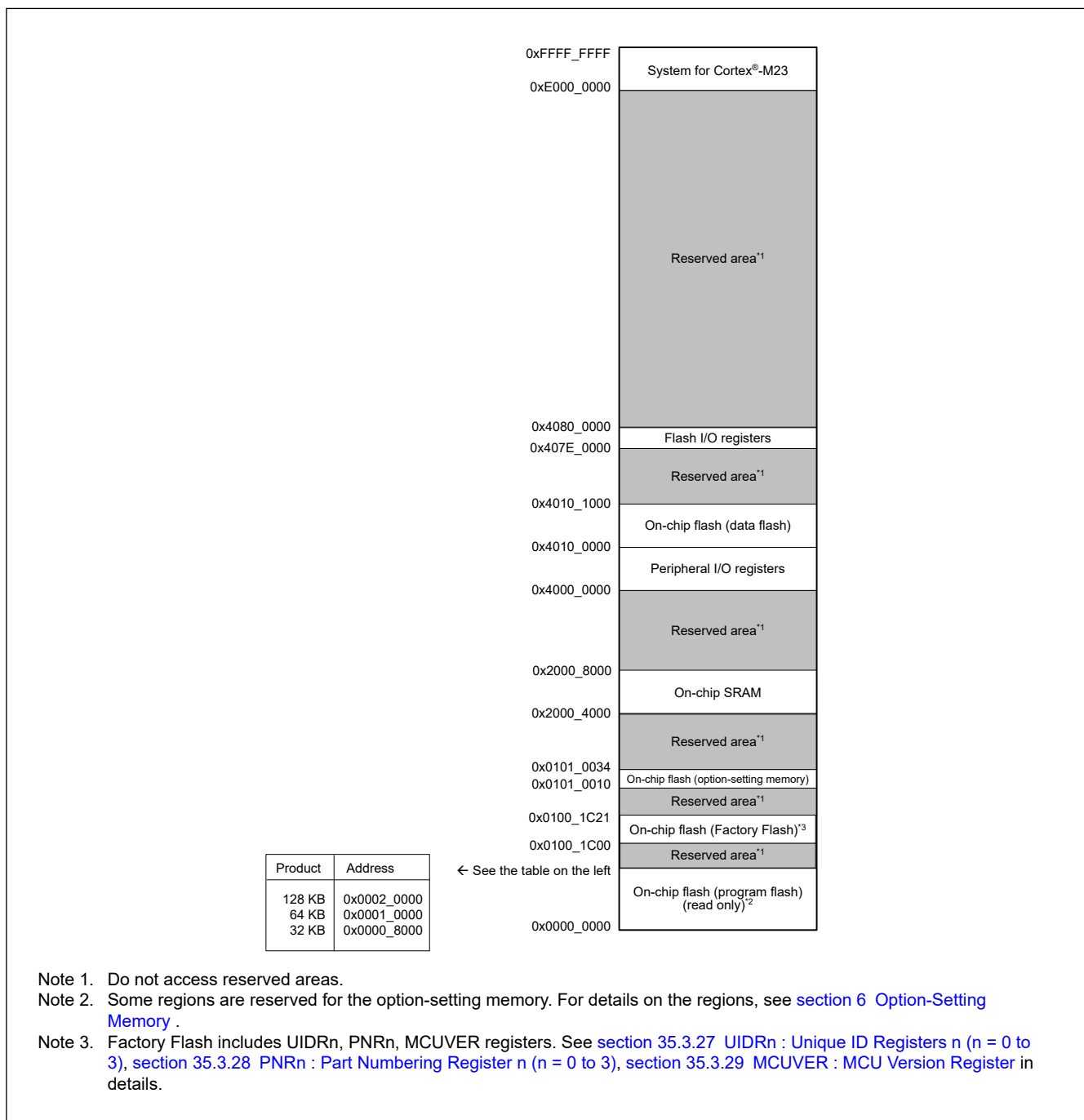
Figure 4.1 Memory map
