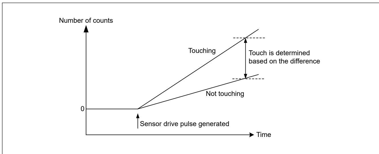
Figure 32.7 Change in measured value when finger is touching and not touching
