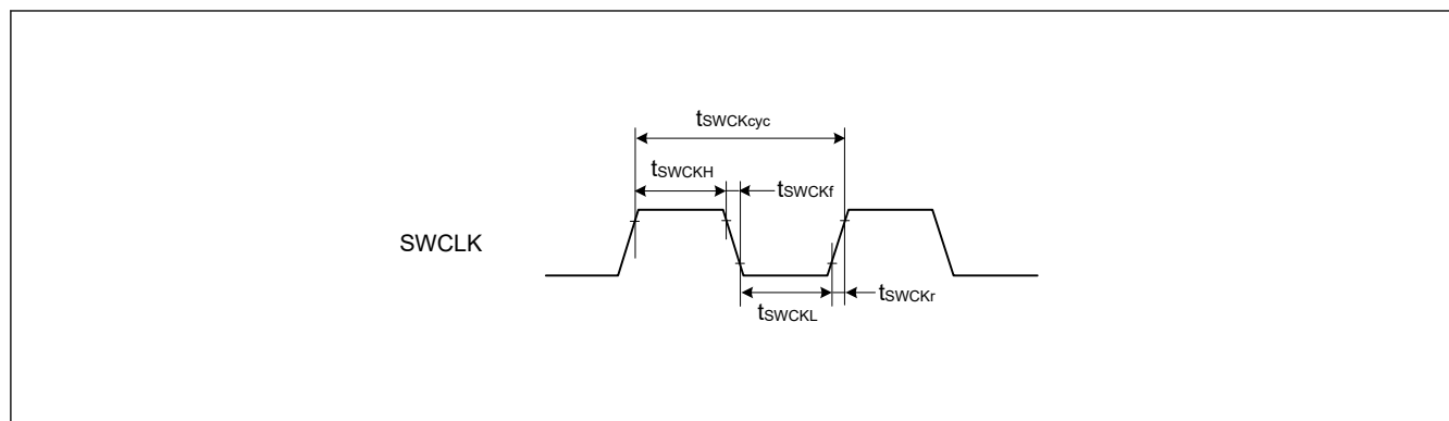
Figure 39.48 SWD SWCLK timing
