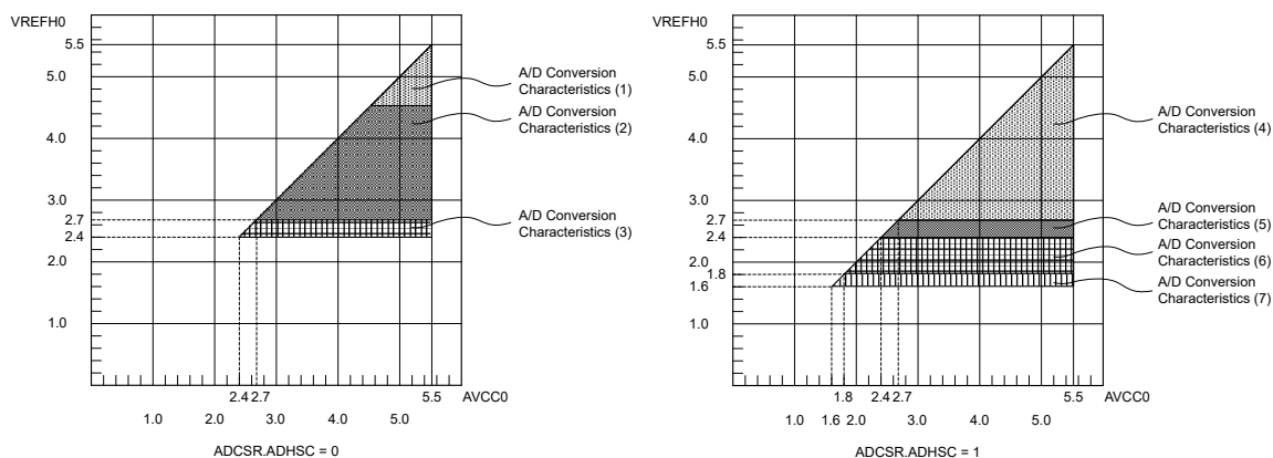
Figure 39.37 AVCC0 to VREFH0 voltage range
