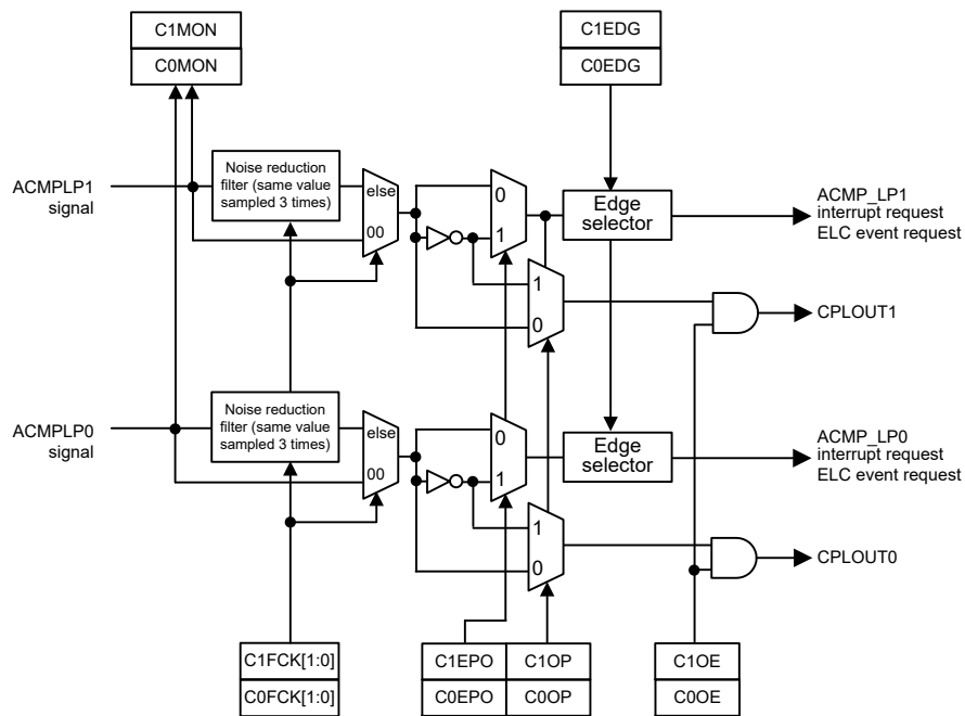
Figure 31.5 Noise filter and edge detection configuration
