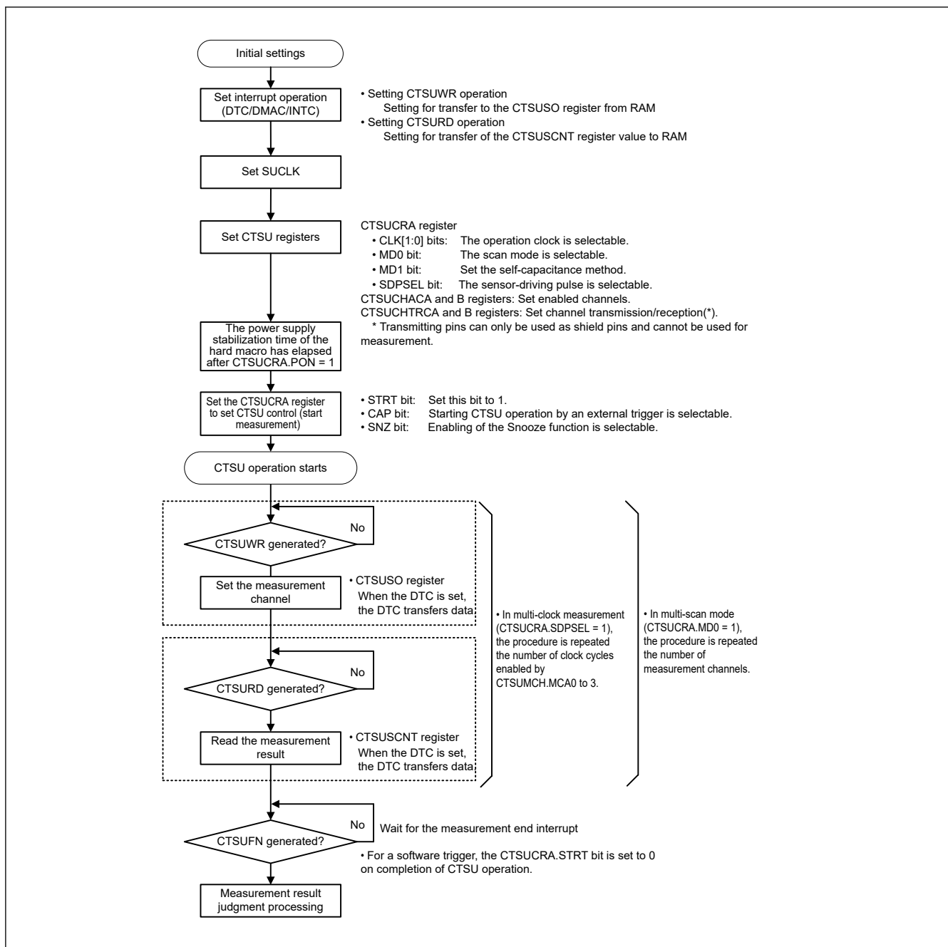
Figure 32.12 Software flow and operation example of self-capacitance method
