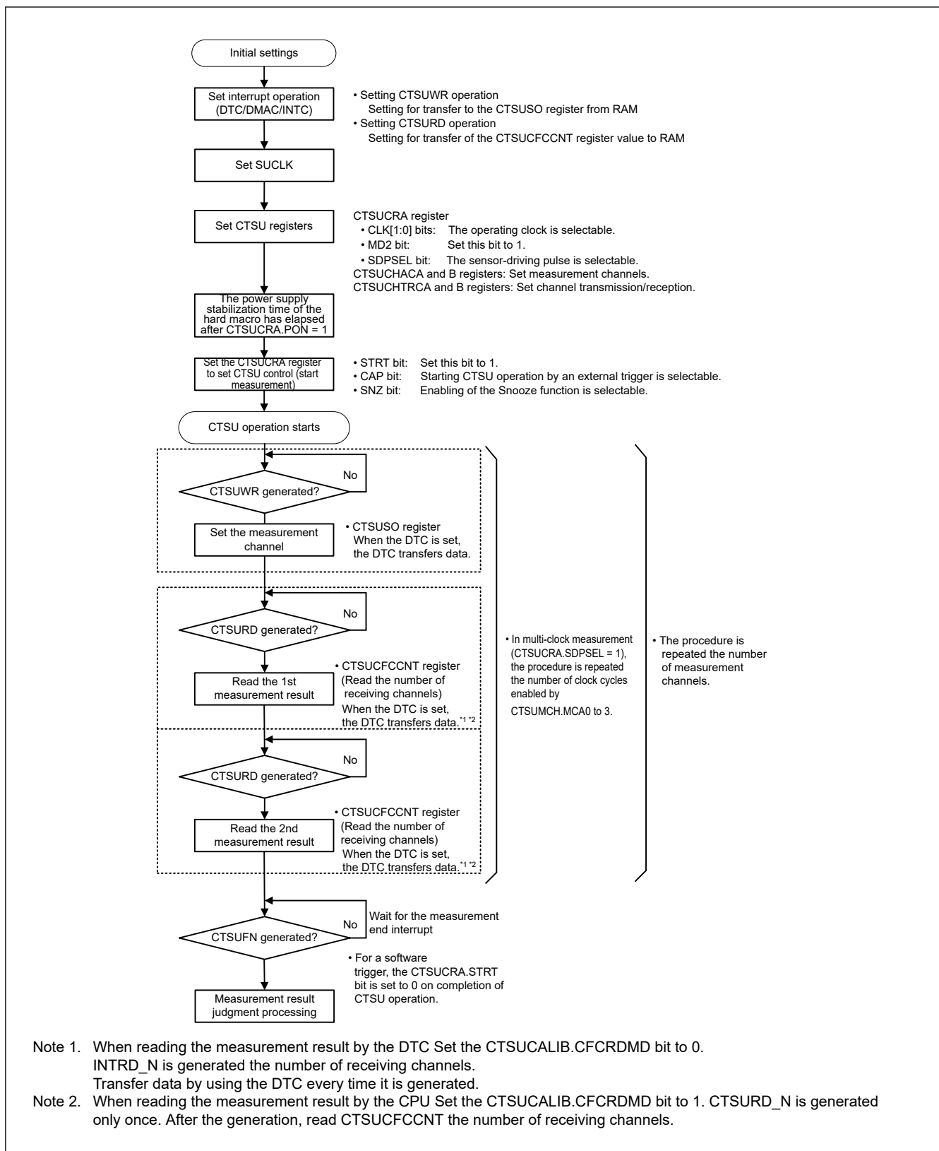
Figure 32.15 Software flow and operation example of high-speed measurement method
