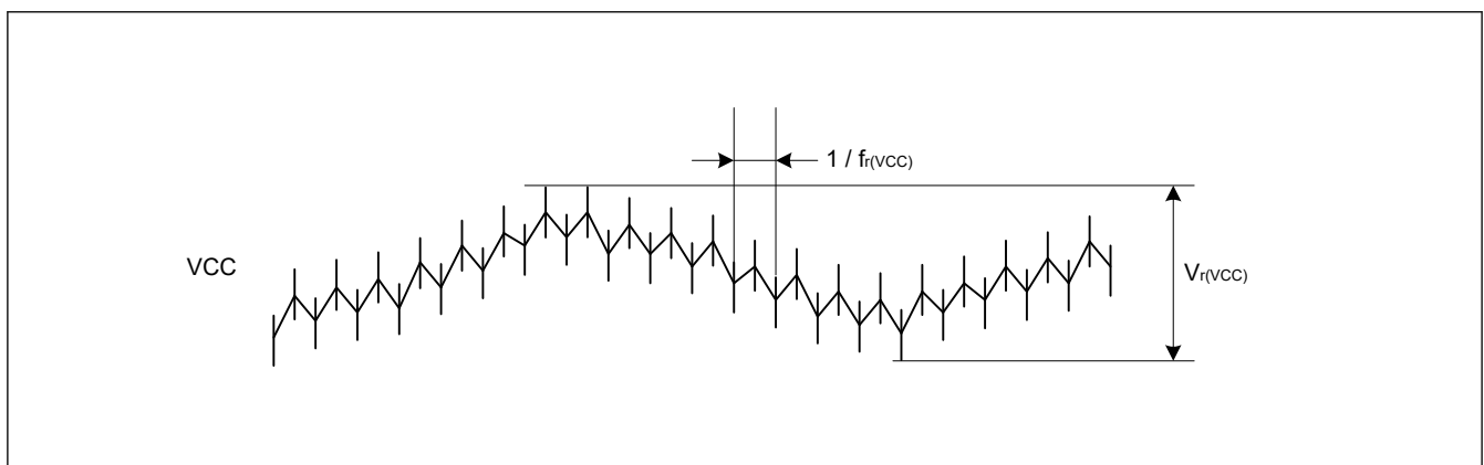
Figure 39.2 Ripple waveform
