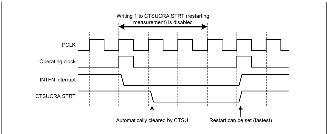
Figure 32.18 Notes on restarting measurement
