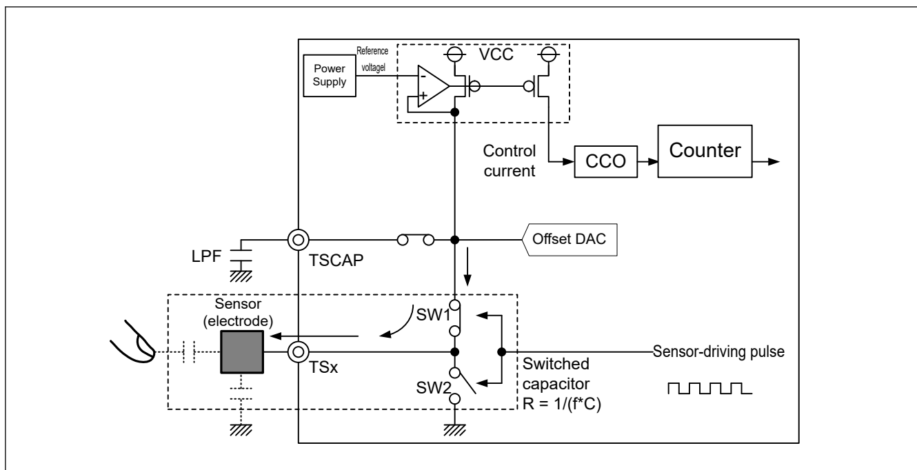
Figure 32.5 Self-capacitance charging operation
