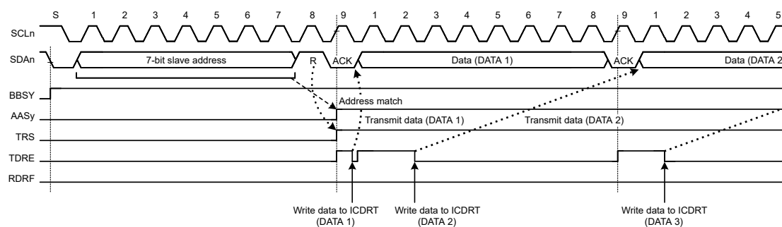
Figure 26.24 AASy flag set timing with 7-bit address format
