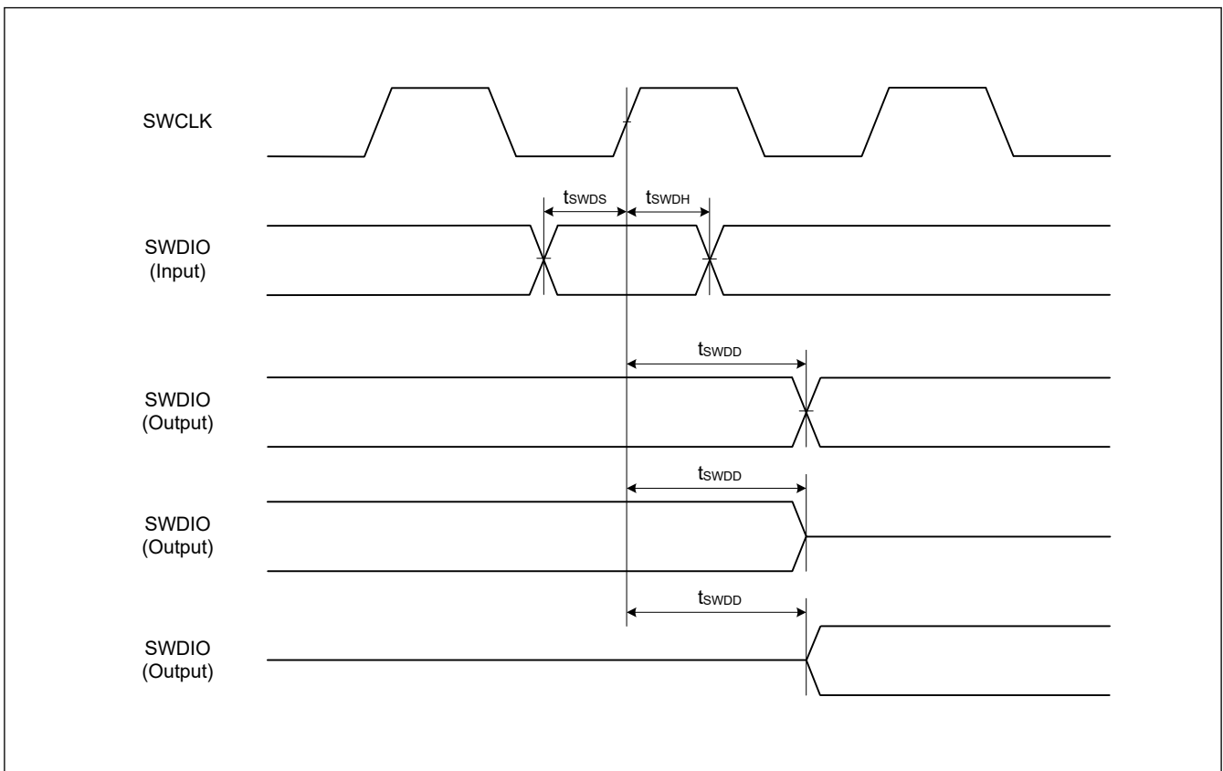
Figure 39.49 SWD input/output timing
