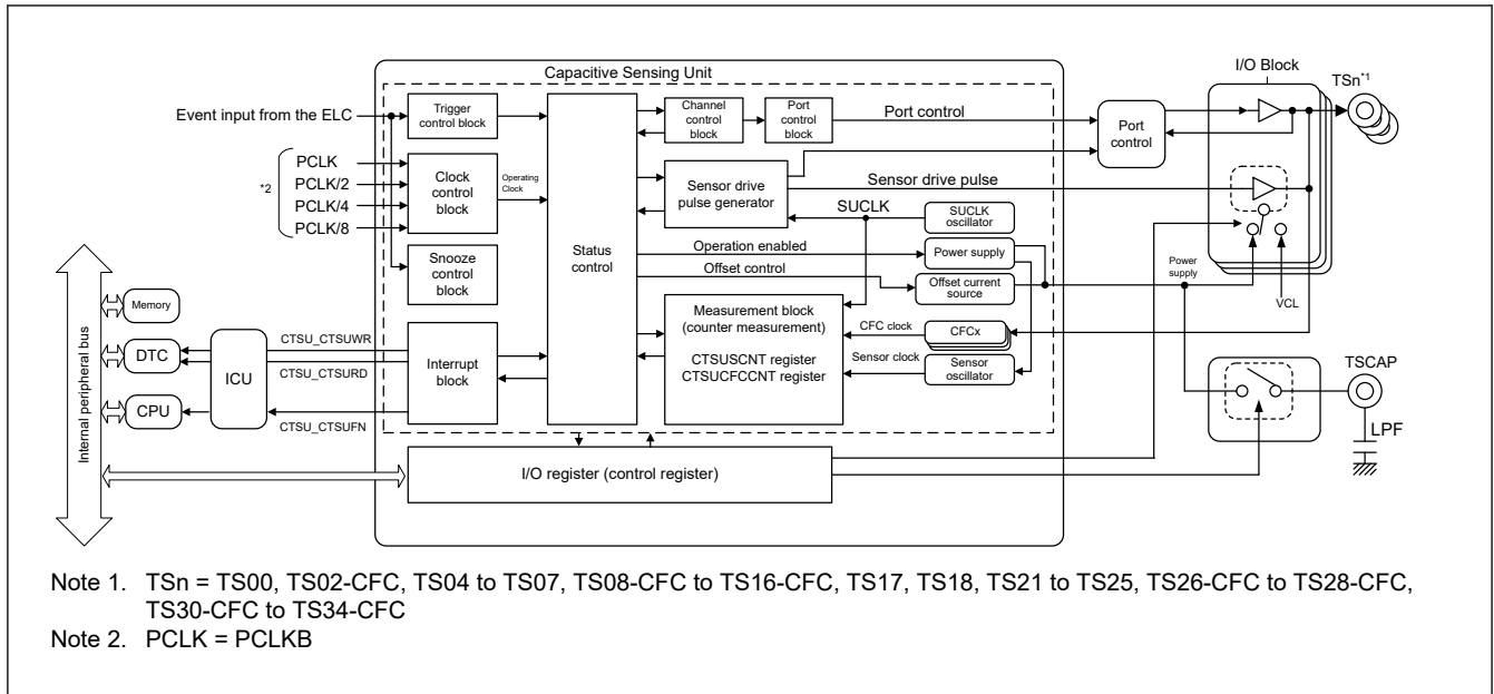
Figure 32.3 CTS2U block diagram
