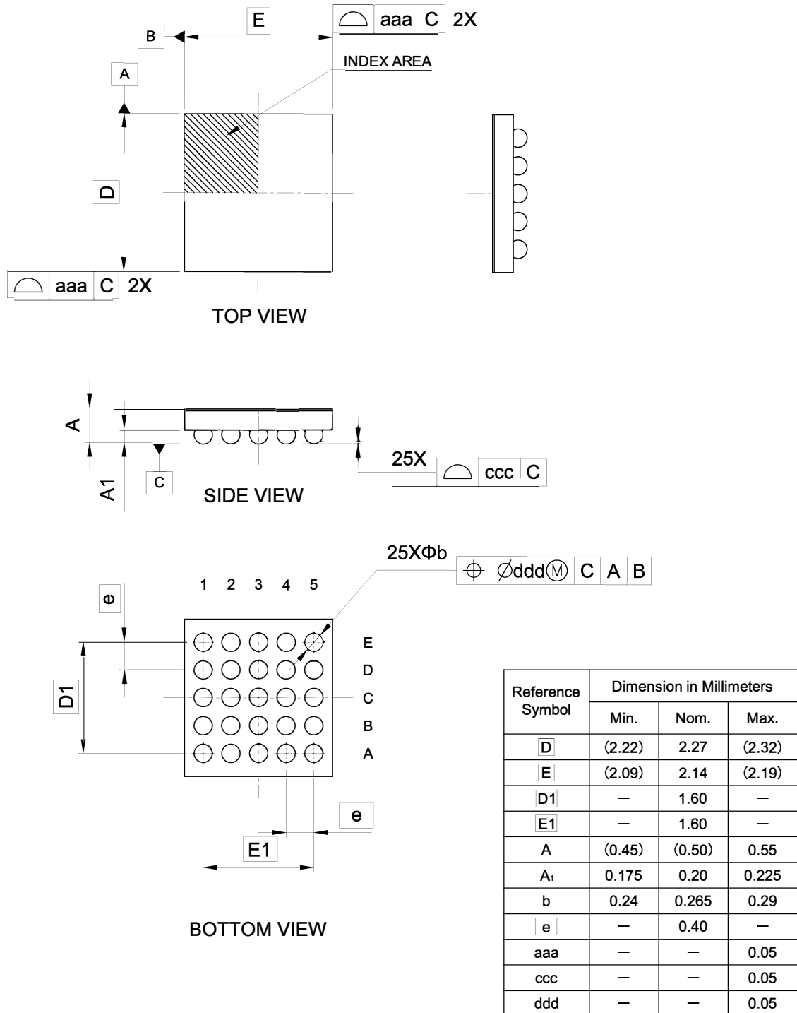
Figure A2.12 WLCSP 25-pin
