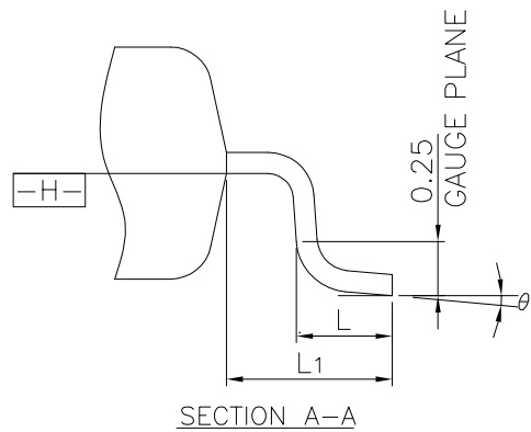
Figure A2.8 LQFP 32-pin (2)
