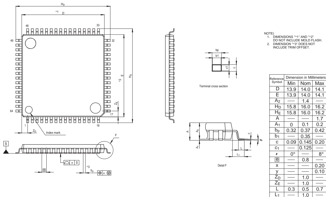
Figure A2.3 LQFP 64-pin 0.8mm pitch
